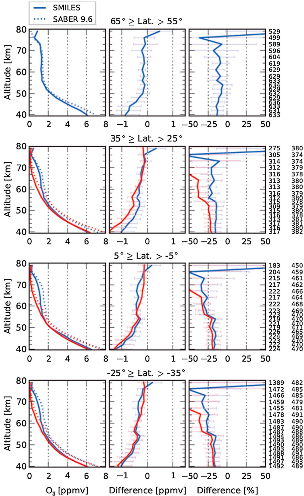
Figure 11. Same as for Figure 10 except for comparisons between SMILES and SABER 9.6.
