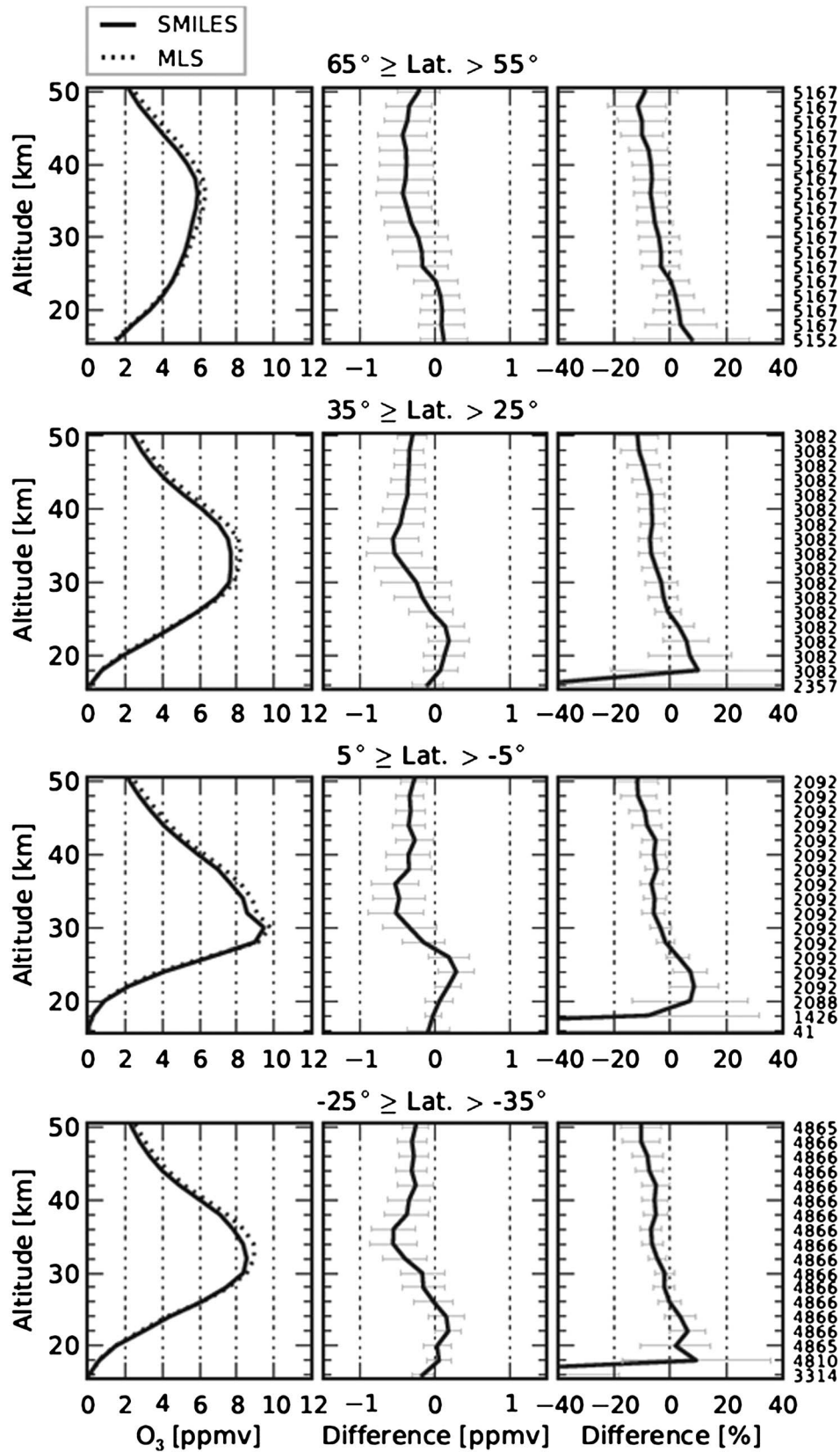
Figure 3. SMILES-MLS coincidences in the stratosphere at four representative latitudes: (from top to bottom) 55°N–65°N, 25°N–35°N, 5°S–5°N, and 35°S–25°S, (left) average ozone values, (middle) average differences ( D ), and (right) average relative differences ( RD ). The solid and dashed lines represent SMILES and MLS profiles, respectively. The error bars represent \pm 1 standard deviations. The numbers shown on each SMILES altitude level on the right axes are the profile numbers for the statistics.
