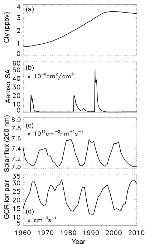
Figure 10. Forcing used in the GSFC 2-D model over the 1960–2010 time period. These include: (a) background total chlorine ( \text{Cl}_y , in ppbv); (b) aerosol surface area (SA) at 50 hPa and the Equator in 10^{-8} \text{ cm}^2 \text{ cm}^{-3} ; (c) solar flux at 200 nm in 10^{11} \text{ cm}^{-2} \text{ nm}^{-1} \text{ s}^{-1} ; and (d) GCR ion pair production at 200 hPa and 90^\circ \text{ S} in \text{cm}^{-3} \text{ s}^{-1} .
