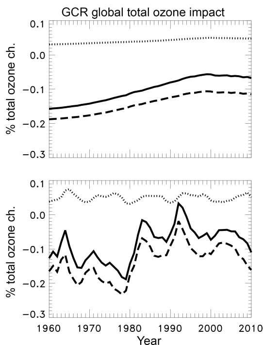
Figure 8. GSFC 2-D model GCR-computed impacts of AAGTO between 1000 and 100 hPa (dotted black), between 100 and 1 hPa (dashed black), and for the entire troposphere and stratosphere, 1000 to 1 hPa, (solid black) over the 1960–2010 time period. The top plot shows the comparison of simulation AI_GCR_GSFC to A_Base_GSFC . The bottom plot shows the comparison of simulation E_GCR_GSFC to E_Base_GSFC .
