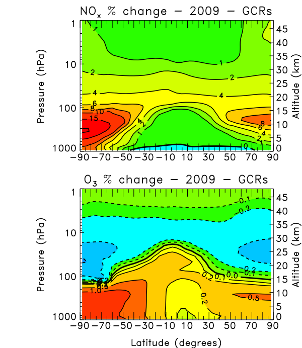
Figure 5. Annual average percentage change for year 2009 in zonal mean \text{NO}_x (top) and ozone (bottom) due to GCRs in the GSFC 2-D model (simulation B2_GCR_GSFC compared to B_Base_GSFC ). The contour intervals for the \text{NO}_x changes are 0, 1, 2, 4, 6, 8, 10, 15, and 20%. The contour intervals for the ozone changes are -1 , -0.5 , -0.2 , -0.1 , 0, 0.1, 0.2, 0.5, and 1%.
