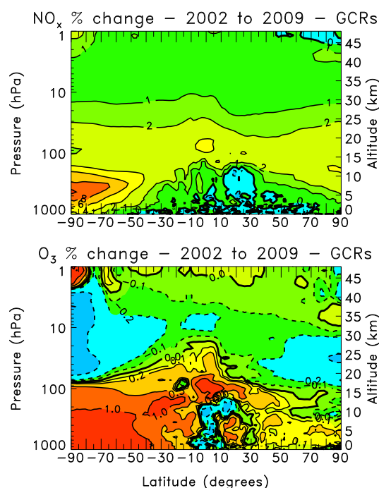
Figure 7. Annual average percentage change from year 2002 (solar maximum) to 2009 (solar minimum) in zonal mean \text{NO}_x (top) and ozone (bottom) in the SD-WACCM. Simulations GCR_SD-W and Base_SD-W were used for this comparison. The annual average percentage change from GCRs was computed for years 2002 and 2009 separately and then differenced from each other. The contour intervals for the \text{NO}_x changes are 0 , 1 , 2 , 4 , 6 , 8 , and 10 %. The contour intervals for the ozone changes are -1 , -0.5 , -0.2 , -0.1 , 0 , 0.1 , 0.2 , 0.5 , and 1 %.
