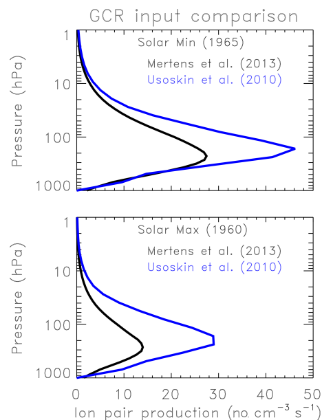
Figure 3. NAIAS model computed galactic cosmic ray annual average ionization rates (Mertens et al., 2013) compared to those given in Usoskin et al. (2010) for solar minimum (1965, top plot) and solar maximum (1960, bottom plot).
