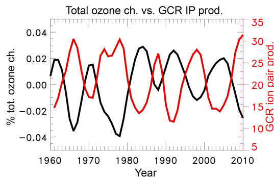
Figure 13. GSFC 2-D model GCR-computed AAGTO change (black line) over the 1960–2010 time period caused by the interannual GCR variation. The global total ozone change shown in Fig. 11c is differenced from that shown in Fig. 11a. A 2-year boxcar (running) average of the GCR ion pair production (in \text{cm}^{-3} \text{s}^{-1} ) at 200 hPa and 90^\circ \text{S} with a 1-year lag is also shown (red line).
