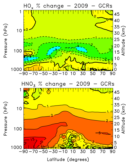
Figure 6. Annual average percentage change for year 2009 in zonal mean \text{HO}_x (top) and \text{HNO}_3 (bottom) due to GCRs in the SD-WACCM (simulation Base_SD_W compared to GCR_SD_W ). The contour intervals for the \text{HO}_x changes are -6 , -4 , -2 , -1 , 0 , and 1 %. The contour intervals for the \text{HNO}_3 are -1 , 0 , 1 , 2 , 5 , 10 , 15 , and 20 %.
