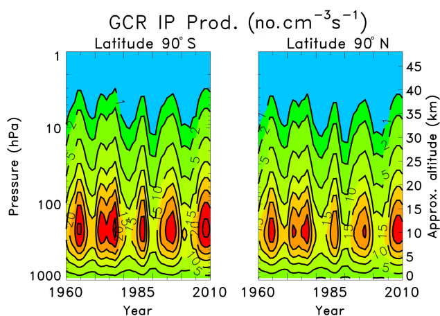
Figure 2. NAIAS model computed galactic cosmic ray annual average ionization rates at 90^\circ \text{S} (left) and 90^\circ \text{N} (right) over the time period 1960–2010. Contour intervals are 1, 2, 5, 10, 15, 20, 25, and 30 ( \text{#cm}^{-3} \text{s}^{-1} ).
