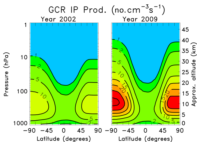
Figure 1. NAIAS model computed GCR annual average ionization rates for years 2002 (left) and 2009 (right). Contour intervals are 1, 2, 5, 10, 15, 20, 25, and 30 ( \text{#cm}^{-3} \text{s}^{-1} ).
