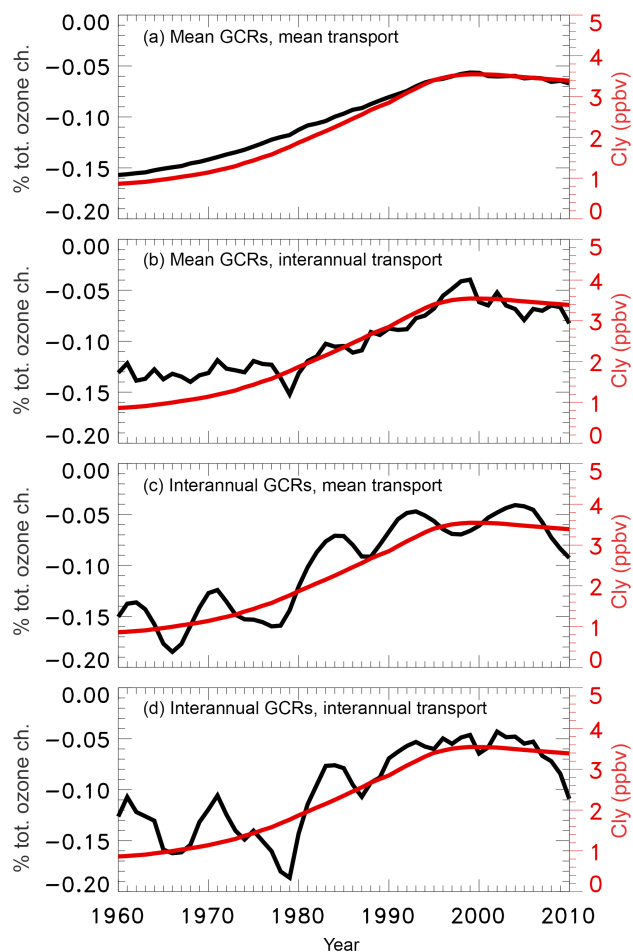
Figure 11. GSFC 2-D model GCR-computed AAGTO impacts (black lines) over the 1960–2010 time period. The \text{Cl}_y levels are also shown (red lines). The GSFC 2-D model comparisons include (a) mean GCRs, mean transport (simulation A1\_GCR\_GSFC compared to A\_Base\_GSFC ); (b) mean GCRs, interannual transport (simulation B1\_GCR\_GSFC compared to B\_Base\_GSFC ); (c) interannual GCRs, mean transport (simulation A2\_GCR\_GSFC compared to A\_Base\_GSFC ); and (d) interannual GCRs, interannual transport (simulation B2\_GCR\_GSFC compared to B\_Base\_GSFC ).
