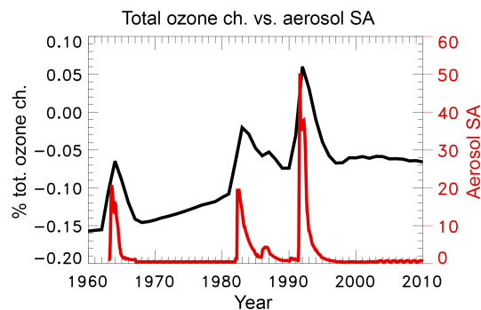
Figure 12. GSFC 2-D model GCR-computed AAGTO impacts (black line) over the 1960–2010 time period (simulation C\_GCR\_GSFC compared to C\_Base\_GSFC ). The aerosol surface area (SA) at 50 hPa and the Equator is also shown (red lines), given in 10^{-8} \text{ cm}^2 \text{ cm}^{-3} .
