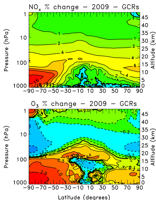
Figure 4. Annual average percentage change for year 2009 in zonal mean \text{NO}_x (top) and ozone (bottom) due to GCRs in the SD-WACCM (simulation Base_SD_W compared to GCR_SD_W ). The contour intervals for the \text{NO}_x changes are 0, 1, 2, 4, 6, 8, 10, and 15%. The contour intervals for the ozone changes are -1 , -0.5 , -0.2 , -0.1 , 0, 0.1, 0.2, 0.5, 1, and 2%.
