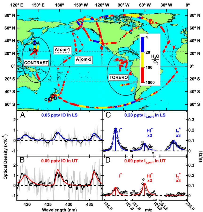
Fig. 1. Overview of iodine measurements in the UTLS. ( Top ) The CU AMAX-DOAS aboard the NSF/NCAR GV measured IO during TORERO (January to February 2012) and CONTRAST (January to February 2014); the CU HR-AMS measured I_{y,part} during ATom-1 (July to August 2016) and ATom-2 (January to February 2017). Lower values of the H_2O/O_3 ratio indicate stratospheric air (blue), while higher values (red) are tropospheric; (yellow) intermediate air. A–D refer to locations of measurements on the map. (A and B) Spectral proof of IO absorption, showing the scaled IO reference spectrum (red, blue), overlaying the residual noise (gray, unsmoothed; black, single-pass triangular smoothing to help guide the eye; fit results are indistinguishable for the gray and black lines). (C and D) Mass spectral proof of iodine measurements (black) and fitted ion signals (red, blue) in particles; the vertical bars show the ion exact mass. Increasing HI^+ relative to I^+ is indicative of iodide, and I_2^+ is indicative of iodate, and I^+ is the dominant HR-AMS ion signal for both oxidation states.
