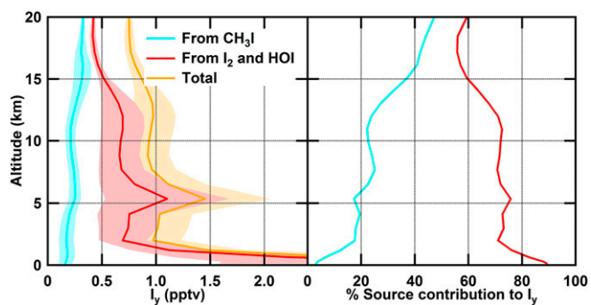
Fig. 4. Contribution of organic ( \text{CH}_3\text{I} ) and inorganic iodine ( \text{I}_2 + \text{HOI} ) emissions to the I_y burden of the CAM-Chem model within the Tropics ( 20^\circ\text{N} to 20^\circ\text{S} ). (Left) I_y from a simulation including both organic and inorganic emissions of iodine (orange), a simulation including only emissions of \text{CH}_3\text{I} (blue), and a simulation including only inorganic iodine emissions (red). (Right) Percentage contribution of \text{CH}_3\text{I} (blue) and inorganic emissions (red) to the total iodine burden.
