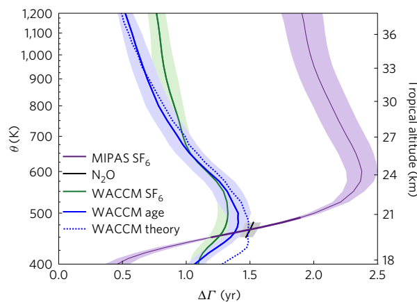
Figure 2 | The average age difference between downwelling and upwelling age of air on each isentrope between 2007–2011. \Delta\Gamma is plotted in solid lines: MIPAS SF 6 -age in purple, GOZCARDS N 2 O-age in black, WACCM SF 6 -age in green, and WACCM ideal age of air in the blue. The blue dotted line shows the ratio of the total mass above each isentrope to the mass flux through the isentrope ( M/\mathcal{M} ) from WACCM. The shading shows one standard deviation of the five annual averages that are averaged to get the mean. The mean height of each isentrope in the tropics (calculated from MIPAS pressure and temperature) is on the right y-axis. Where the line for the MIPAS SF 6 -age difference is thinner, we believe there is a bias in either the data or the SF 6 to age conversion (see discussion in Supplementary Information).
