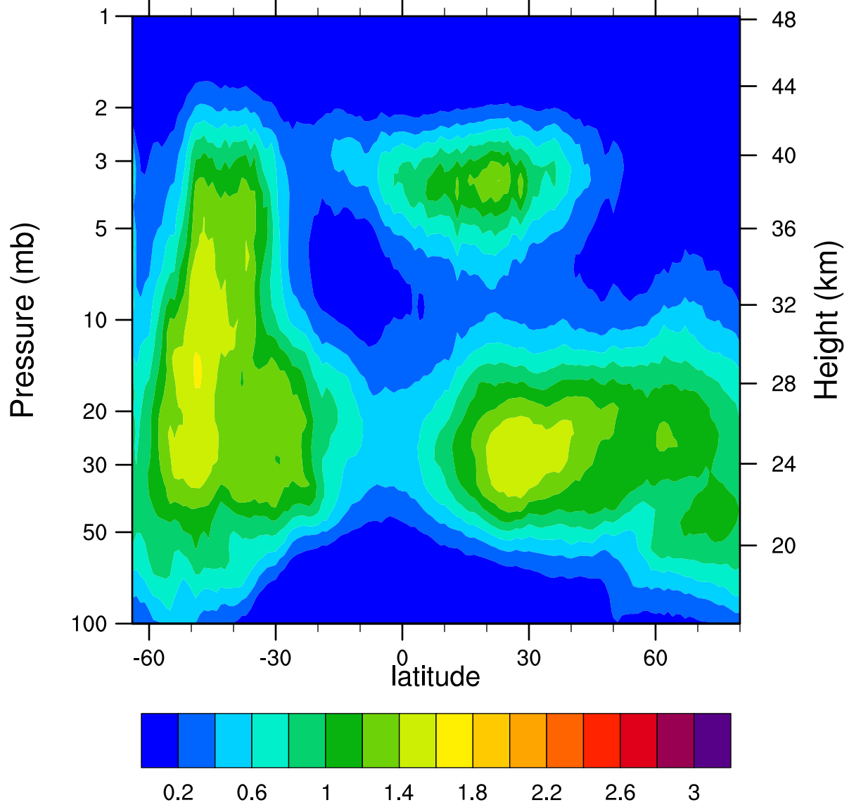
HIRDLSv6 2007d146 ClONO2_Ascending (ppbv)
