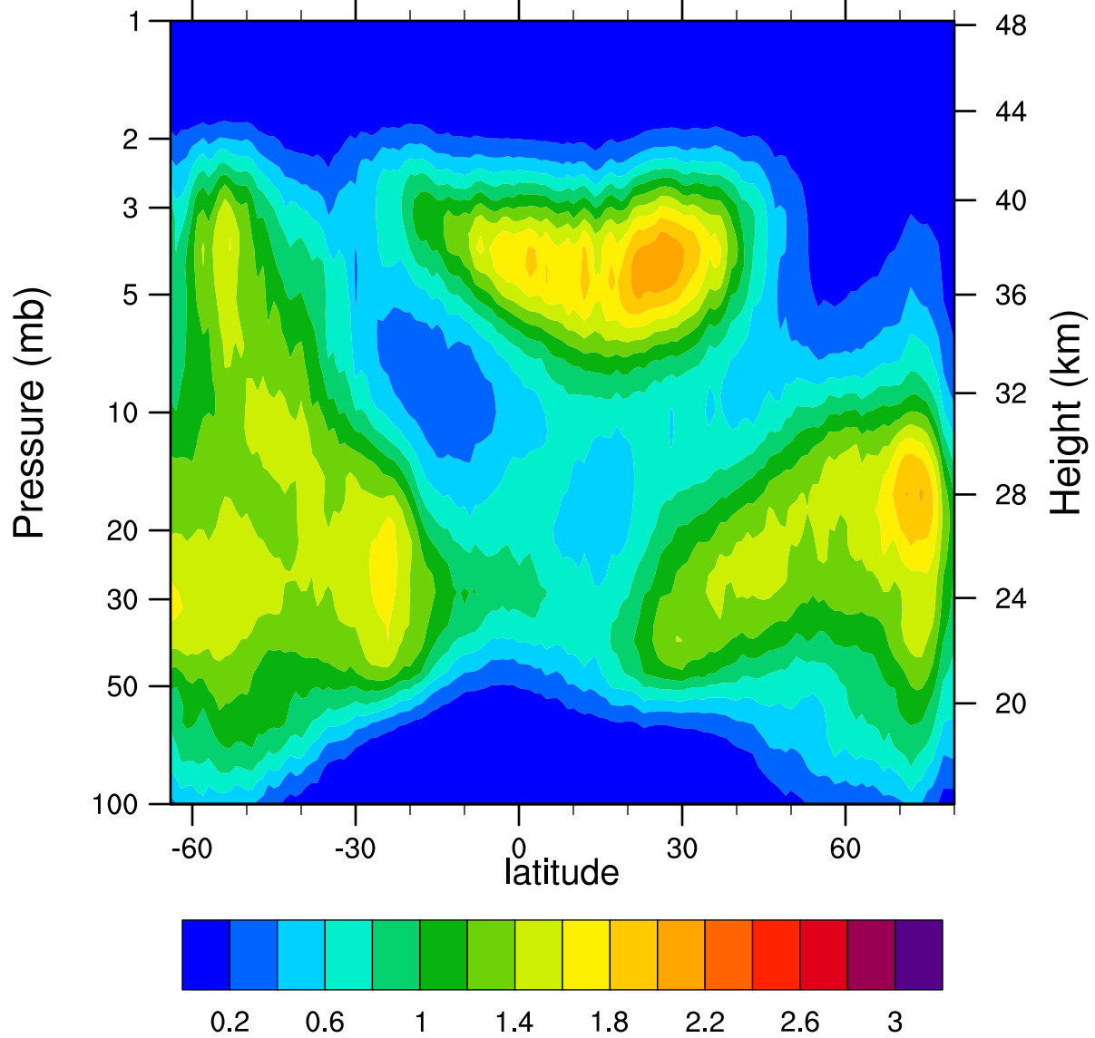
HIRDLSv6 2007d303 ClONO2_Ascending (ppbv)
