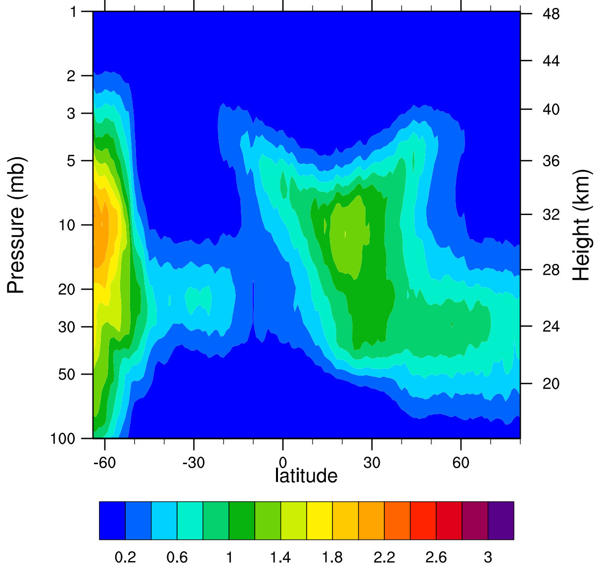
HIRDLSv6 2005d118 ClONO2_Ascending (ppbv)
