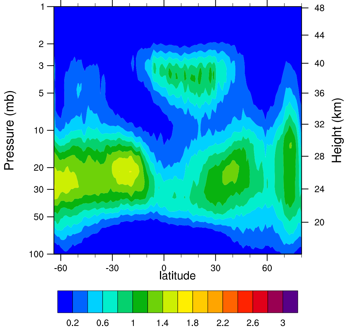
HIRDLSv6 2006d310 ClONO2_Ascending (ppbv)
