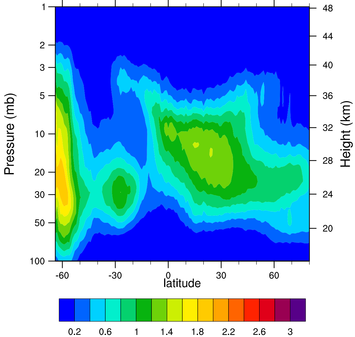
HIRDLSv6 2005d210 ClONO2_Ascending (ppbv)
