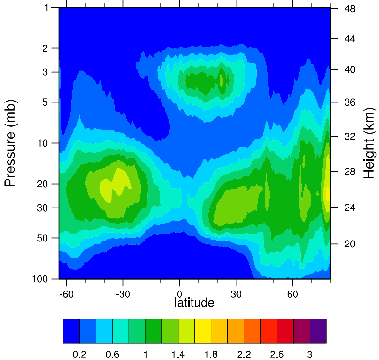
HIRDLSv6 2007d029 ClONO2_Ascending (ppbv)
