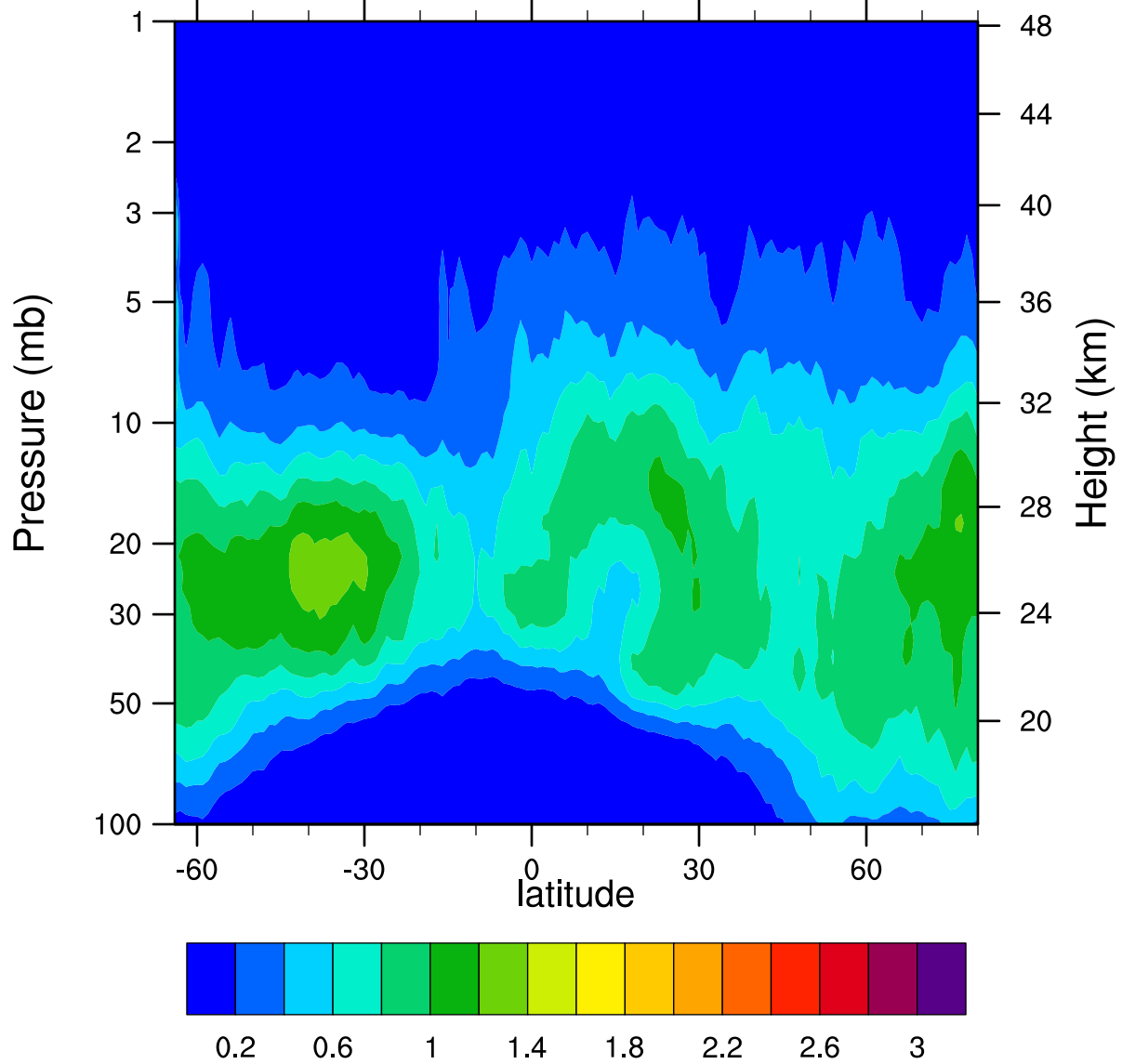
HIRDLSv6 2006d020 ClONO2_Ascending (ppbv)
