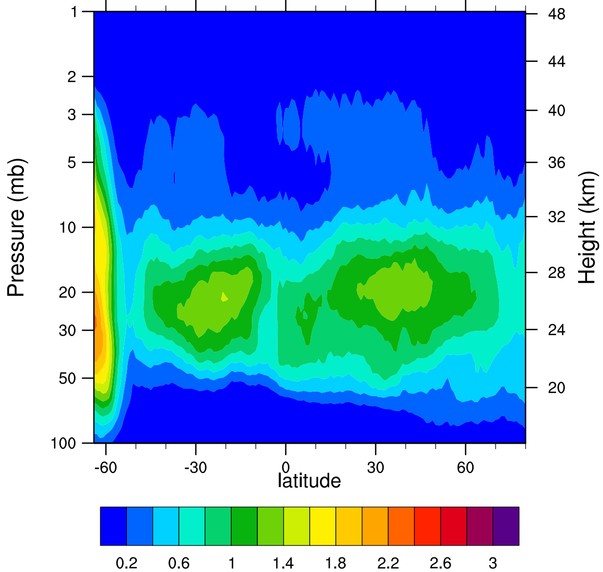
HIRDLSv6 2006d257 ClONO2_Ascending (ppbv)
