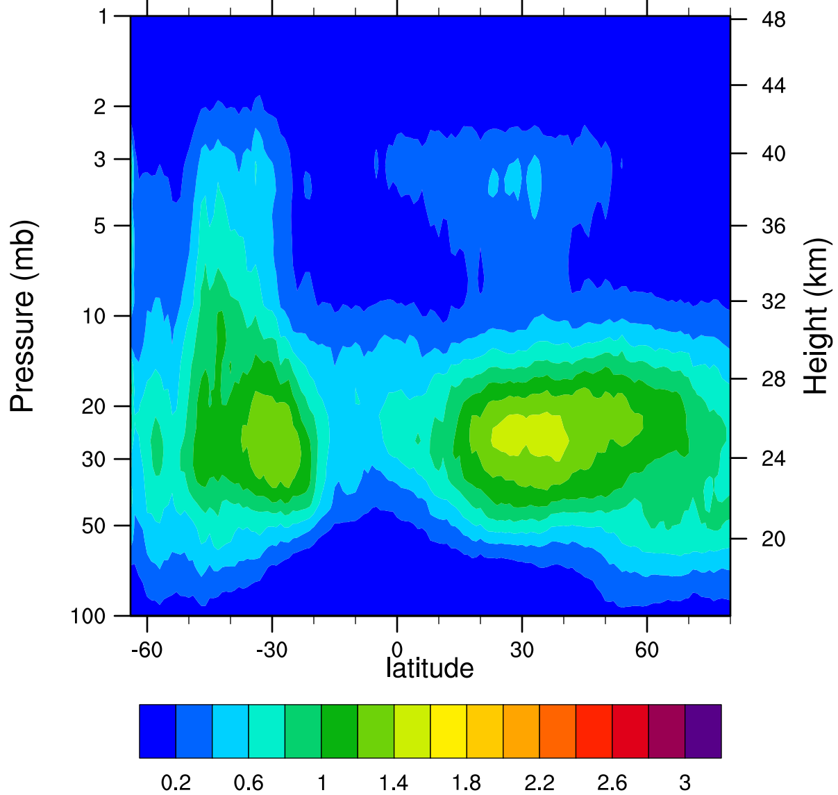
HIRDLSv6 2007d176 ClONO2_Ascending (ppbv)
