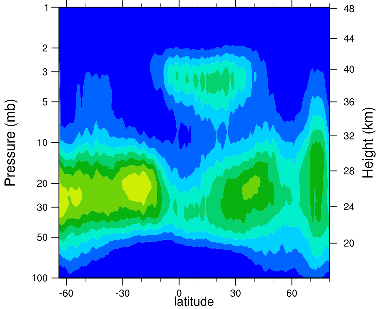
HIRDLSv6 2006d308 ClONO2_Ascending (ppbv)
