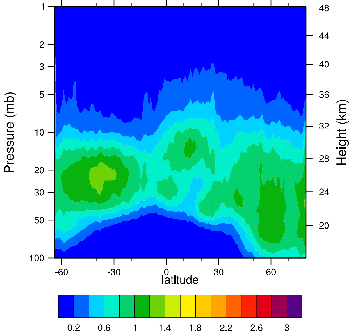
HIRDLSv6 2006d039 ClONO2_Ascending (ppbv)
