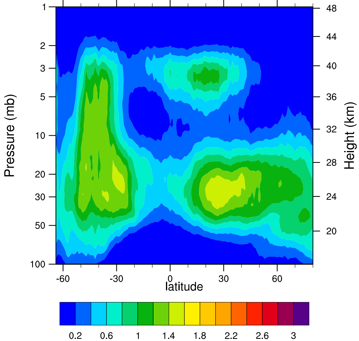
HIRDLSv6 2007d153 ClONO2_Ascending (ppbv)
