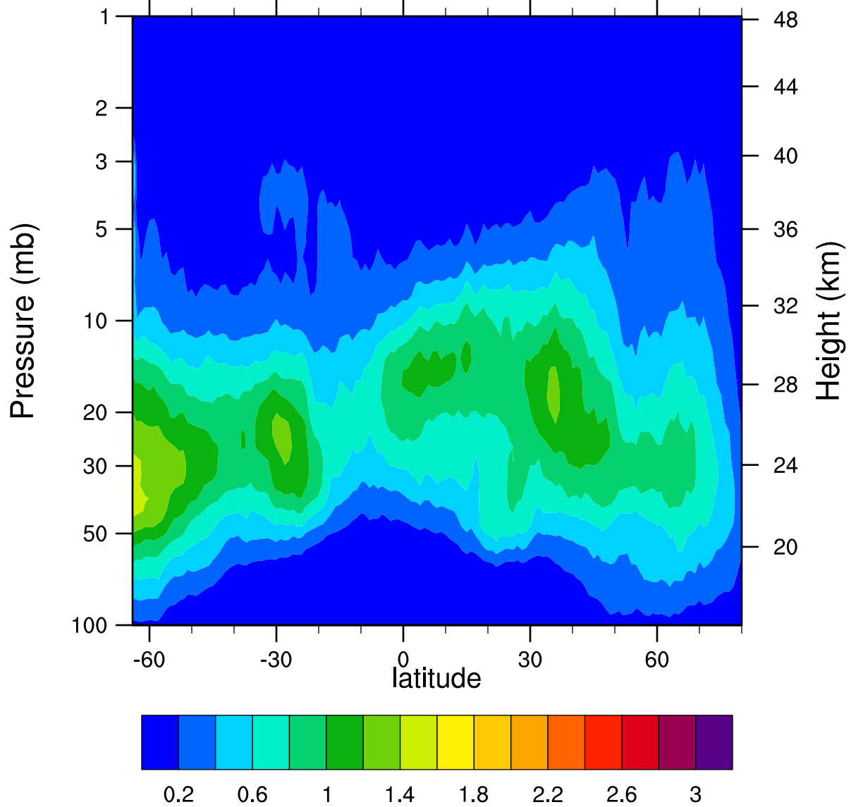
HIRDLSv6 2005d323 ClONO2_Ascending (ppbv)
