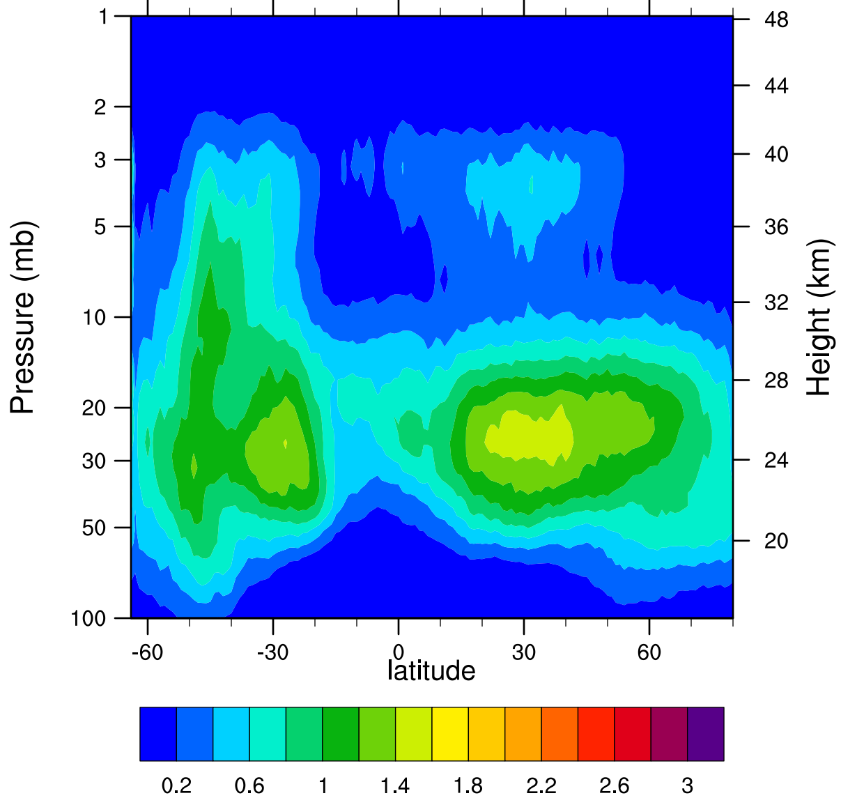
HIRDLSv6 2007d184 ClONO2_Ascending (ppbv)
