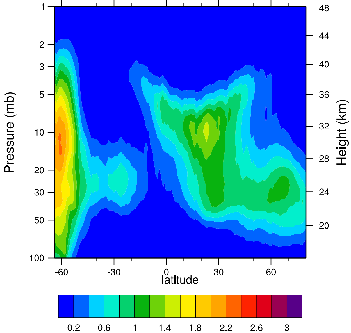
HIRDLSv6 2005d127 ClONO2_Ascending (ppbv)
