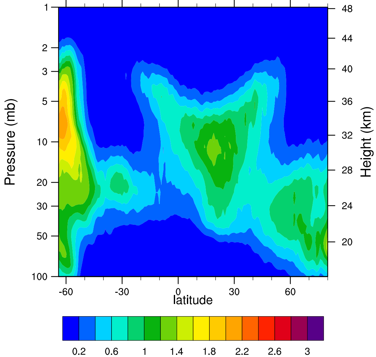
HIRDLSv6 2005d080 ClONO2_Ascending (ppbv)
