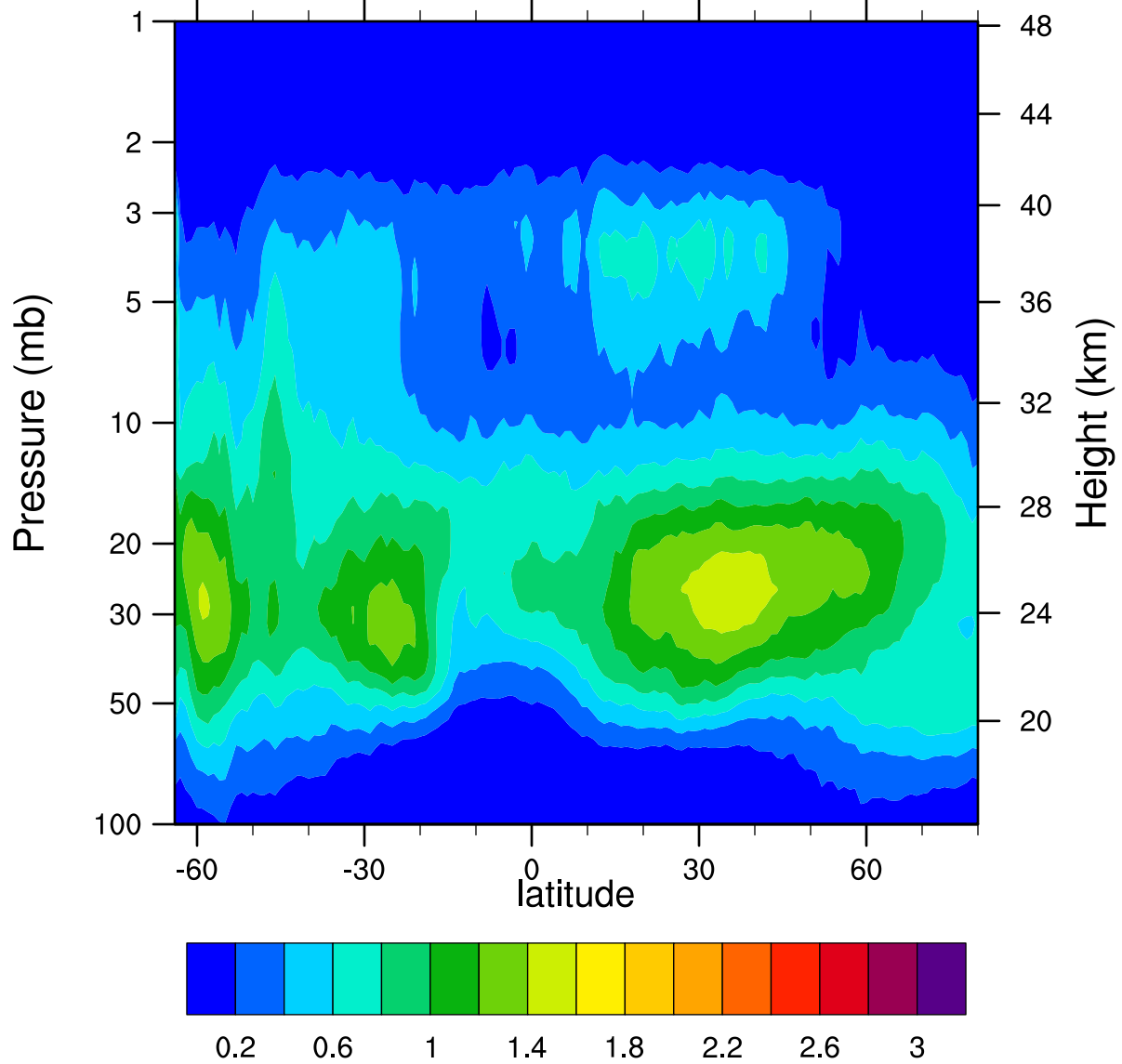
HIRDLSv6 2007d205 ClONO2_Ascending (ppbv)
