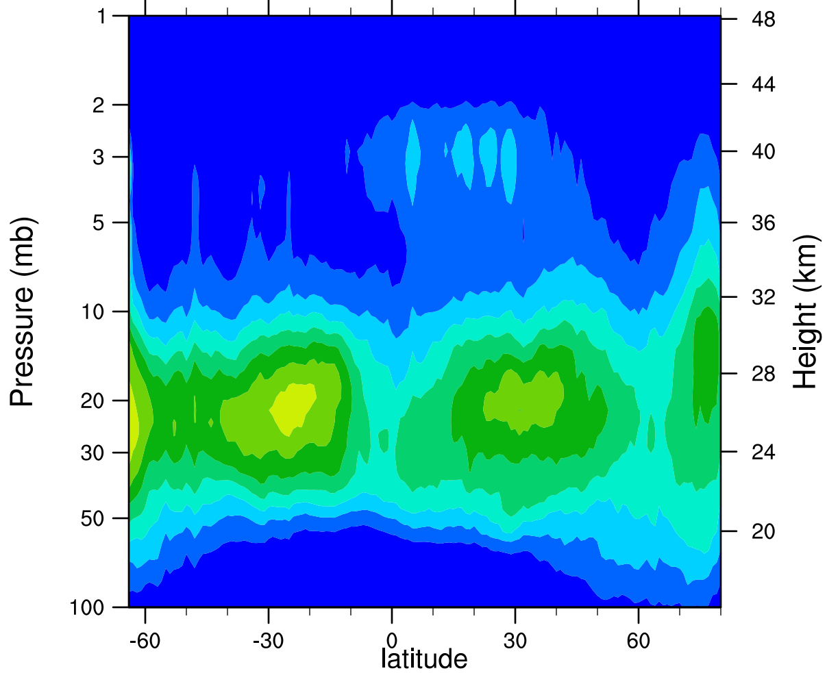
HIRDLSv6 2006d296 ClONO2_Ascending (ppbv)
