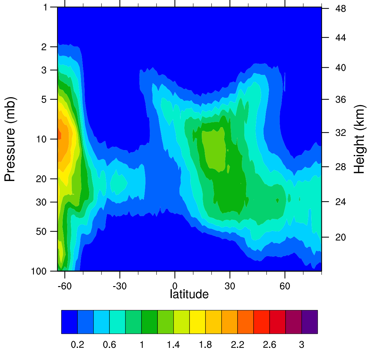
HIRDLSv6 2005d1115 ClONO2_Ascending (ppbv)
