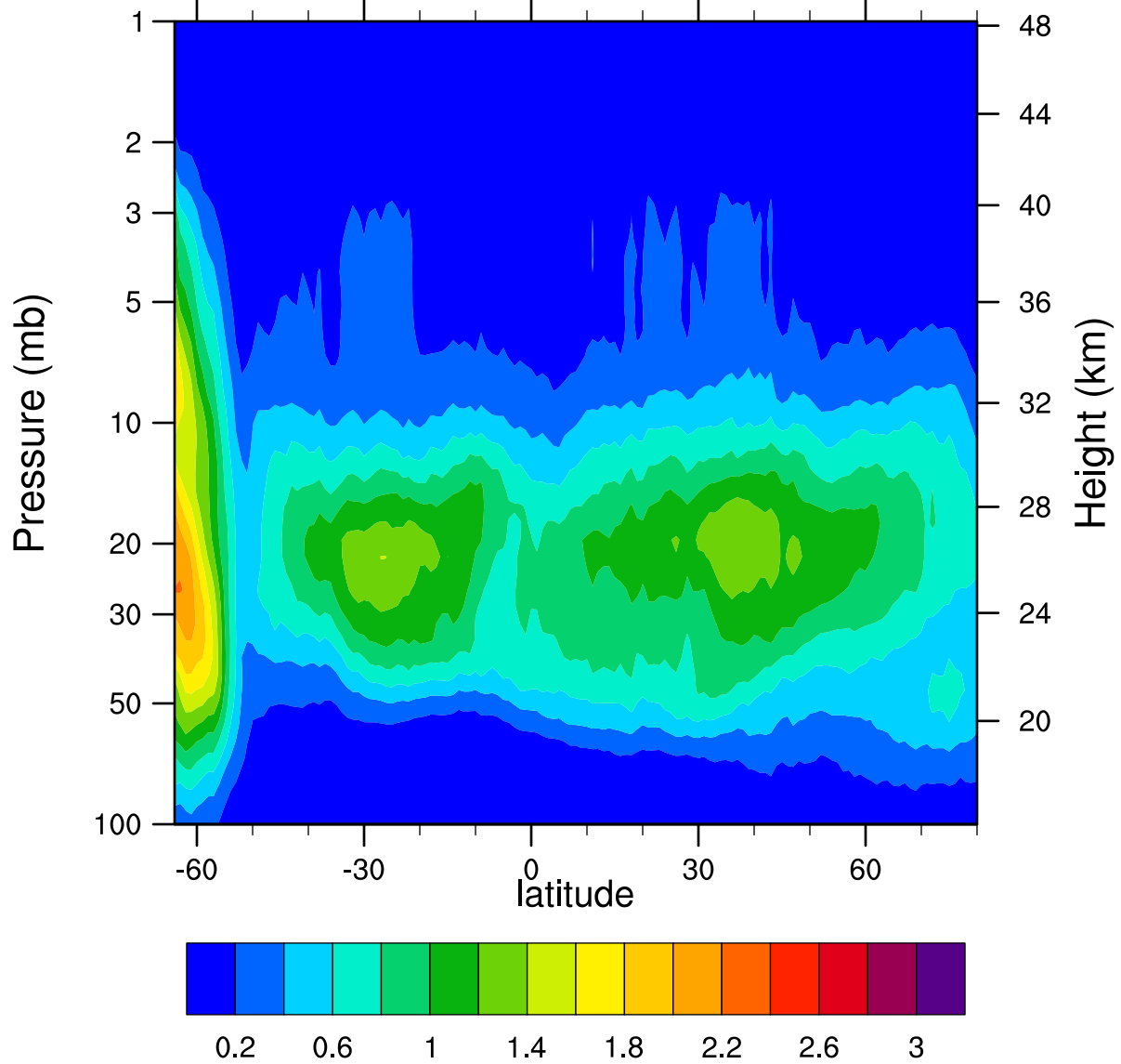
HIRDLSv6 2006d237 ClONO2_Ascending (ppbv)
