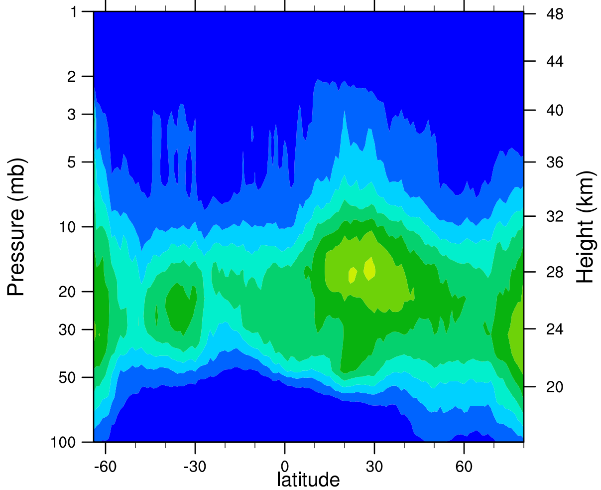
HIRDLSv6 2006d112 ClONO2_Ascending (ppbv)
