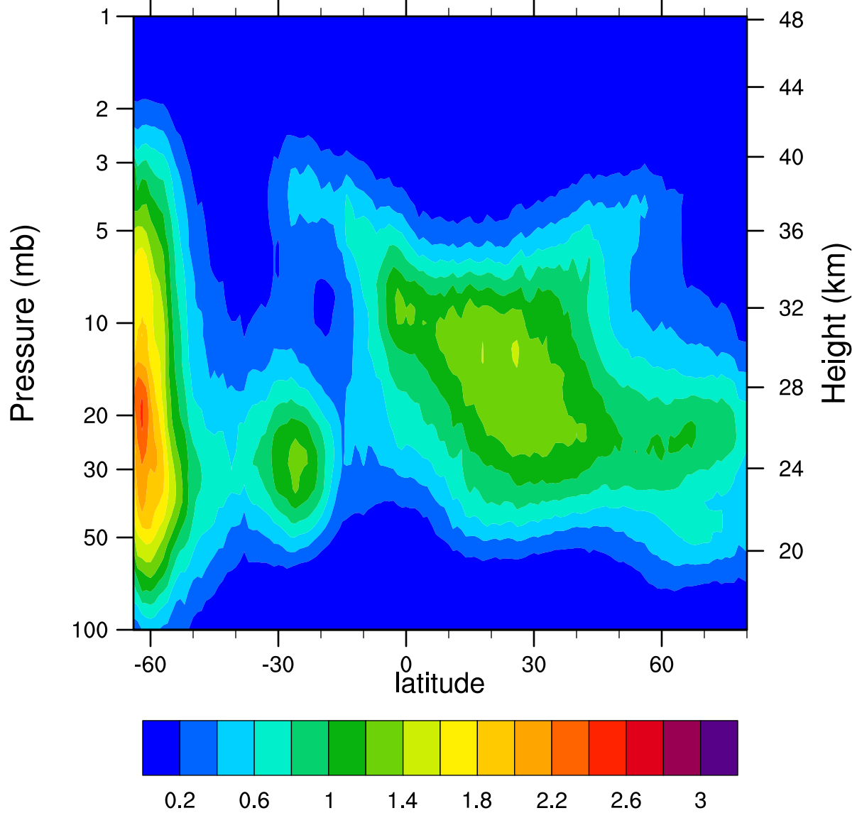
HIRDLSv6 2005d204 ClONO2_Ascending (ppbv)
