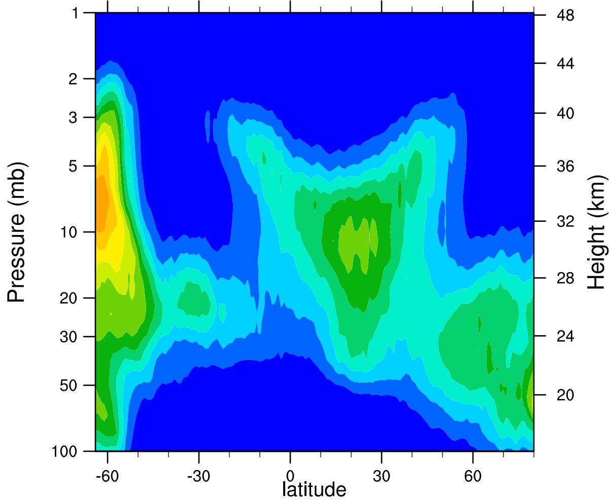
HIRDLSv6 2005d081 ClONO2_Ascending (ppbv)
