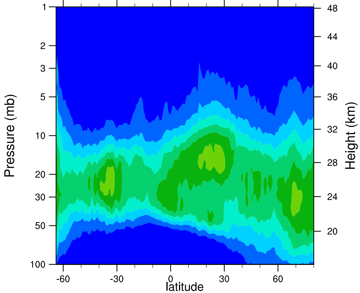
HIRDLSv6 2006d084 ClONO2_Ascending (ppbv)
