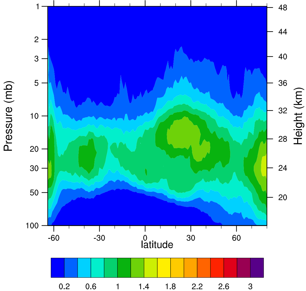
HIRDLSv6 2006d099 ClONO2_Ascending (ppbv)
