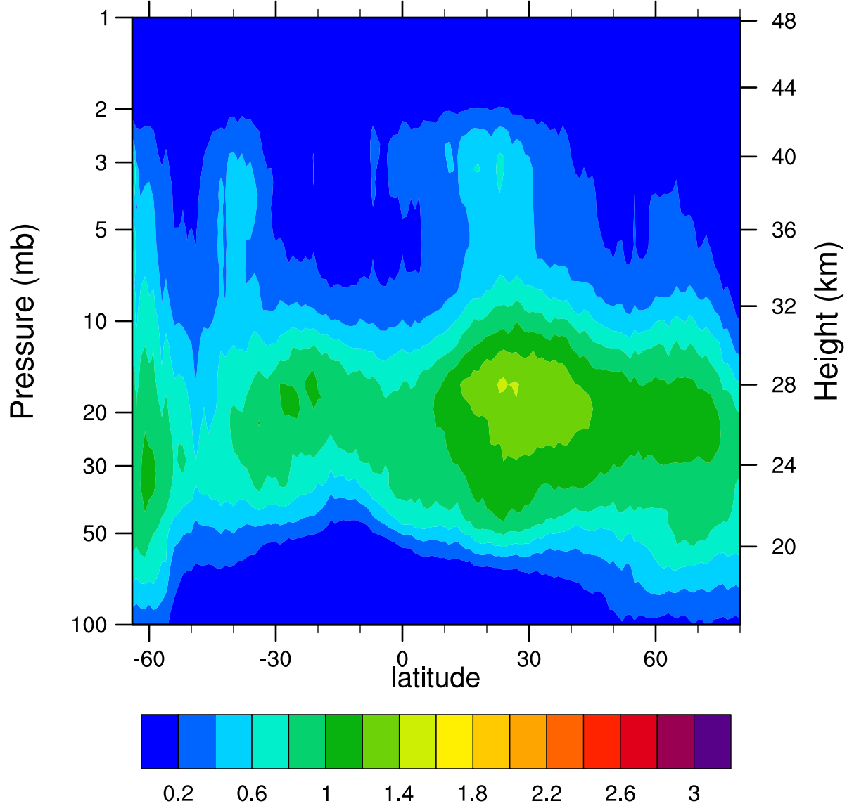
HIRDLSv6 2006d140 ClONO2_Ascending (ppbv)
