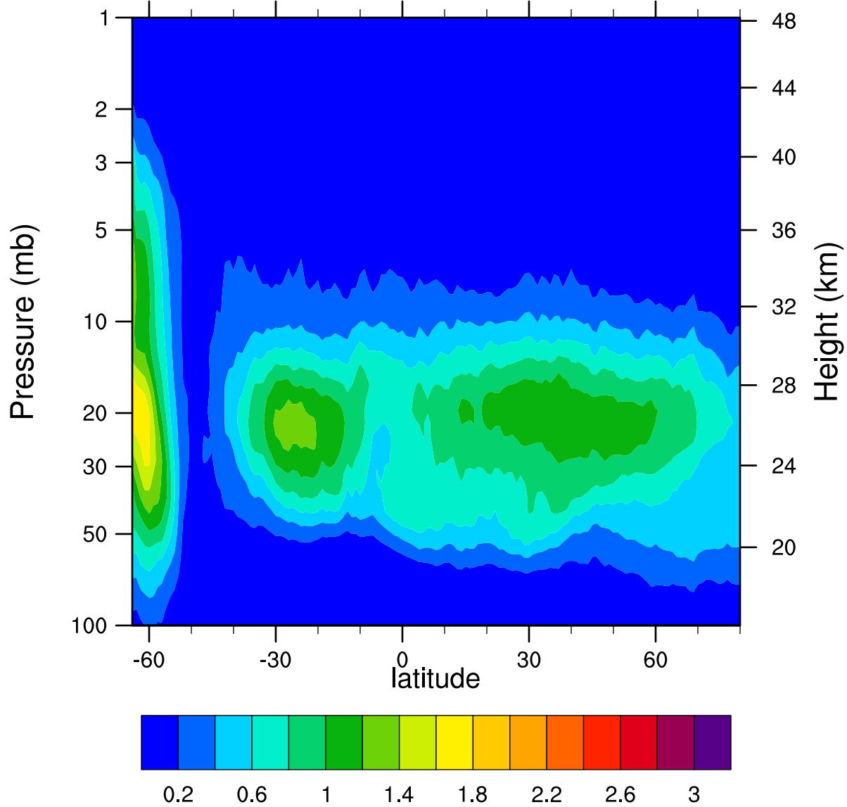
HIRDLSv6 2006d211 ClONO2_Ascending (ppbv)
