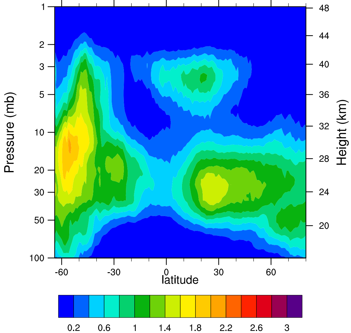
HIRDLSv6 2007d132 ClONO2_Ascending (ppbv)
