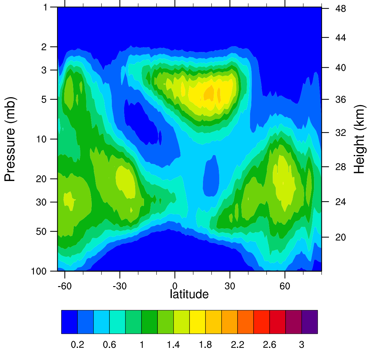
HIRDLSv6 2007d348 ClONO2_Ascending (ppbv)
