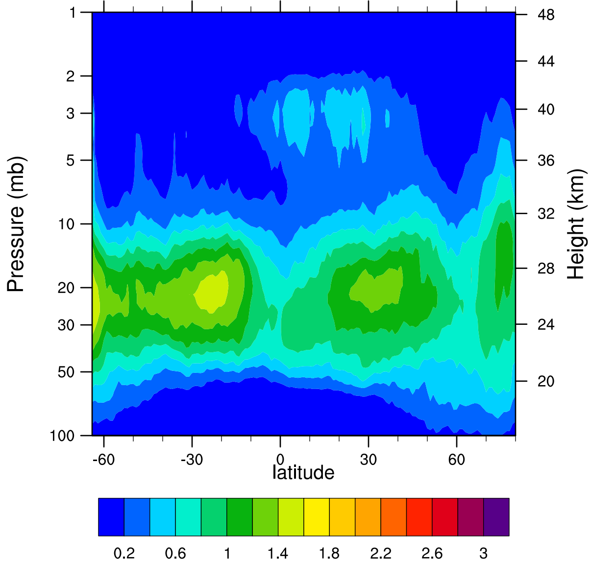
HIRDLSv6 2006d298 ClONO2_Ascending (ppbv)
