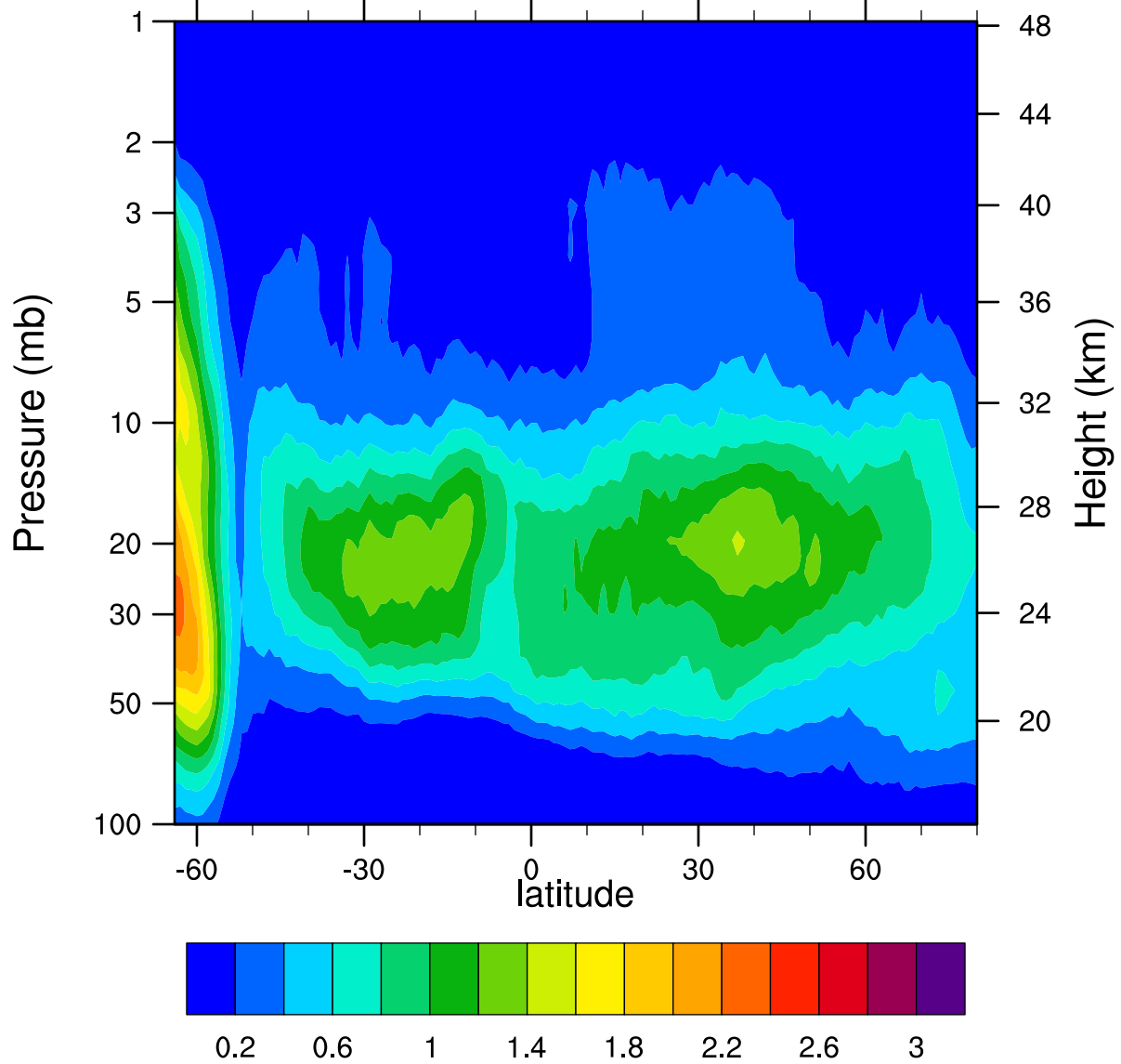
HIRDLSv6 2006d246 ClONO2_Ascending (ppbv)
