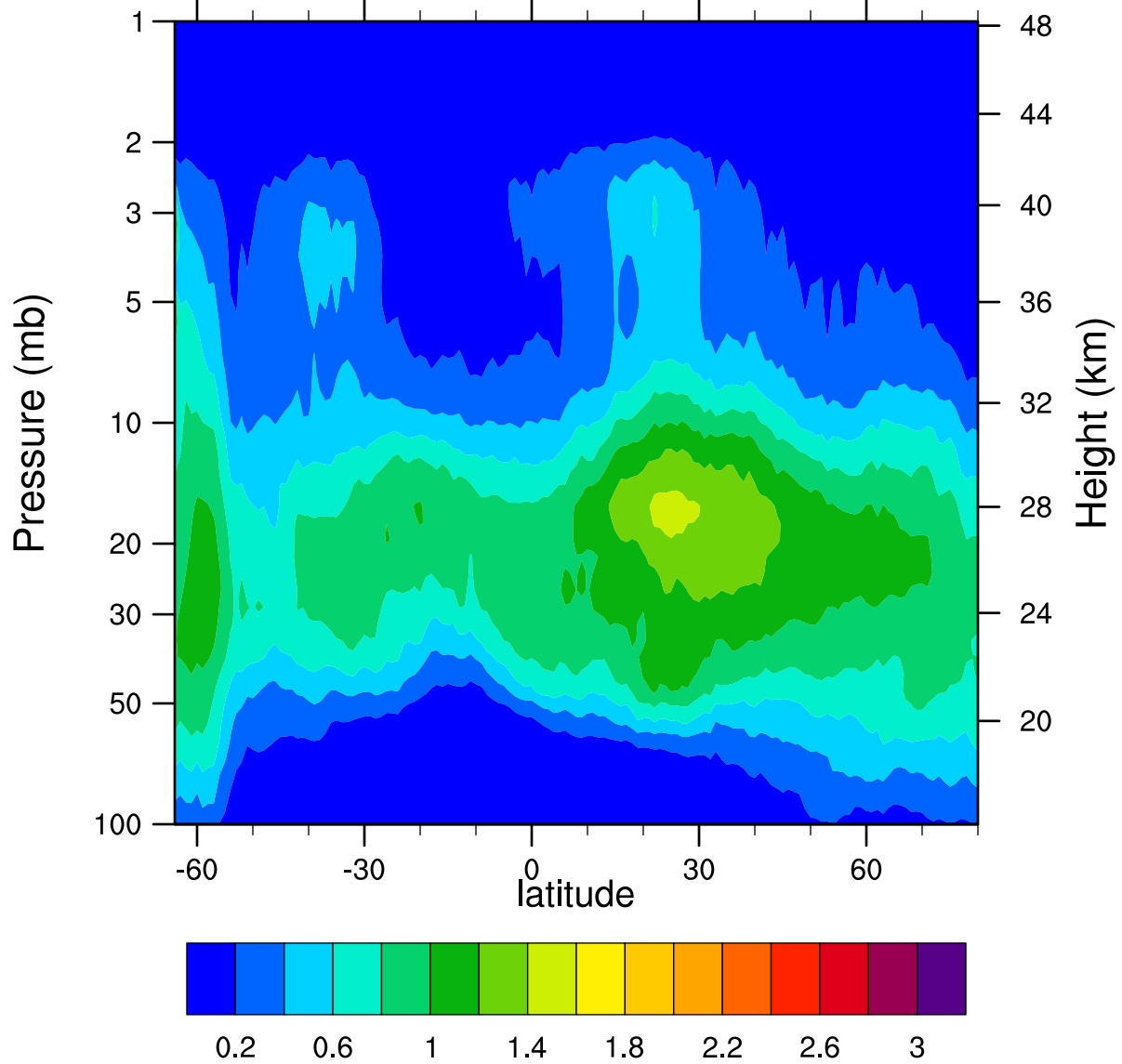
HIRDLSv6 2006d134 ClONO2_Ascending (ppbv)
