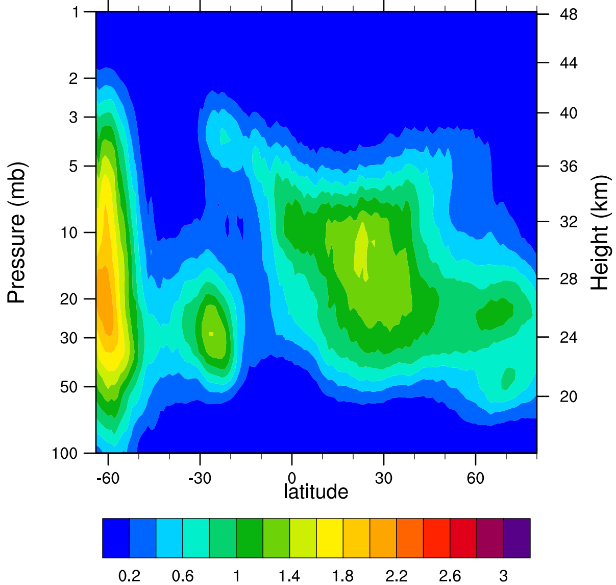
HIRDLSv6 2005d190 ClONO2_Ascending (ppbv)
