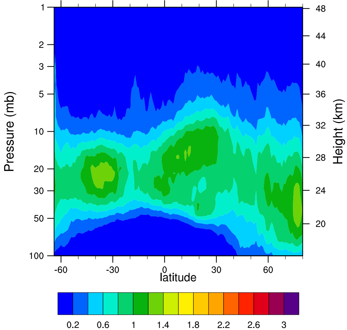
HIRDLSv6 2006d063 ClONO2_Ascending (ppbv)
