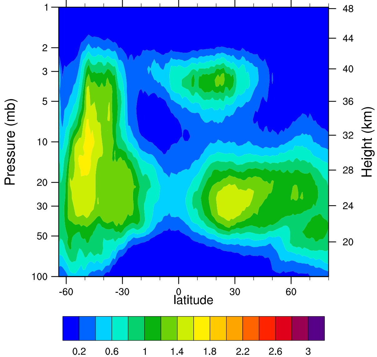
HIRDLSv6 2007d144 ClONO2_Ascending (ppbv)
