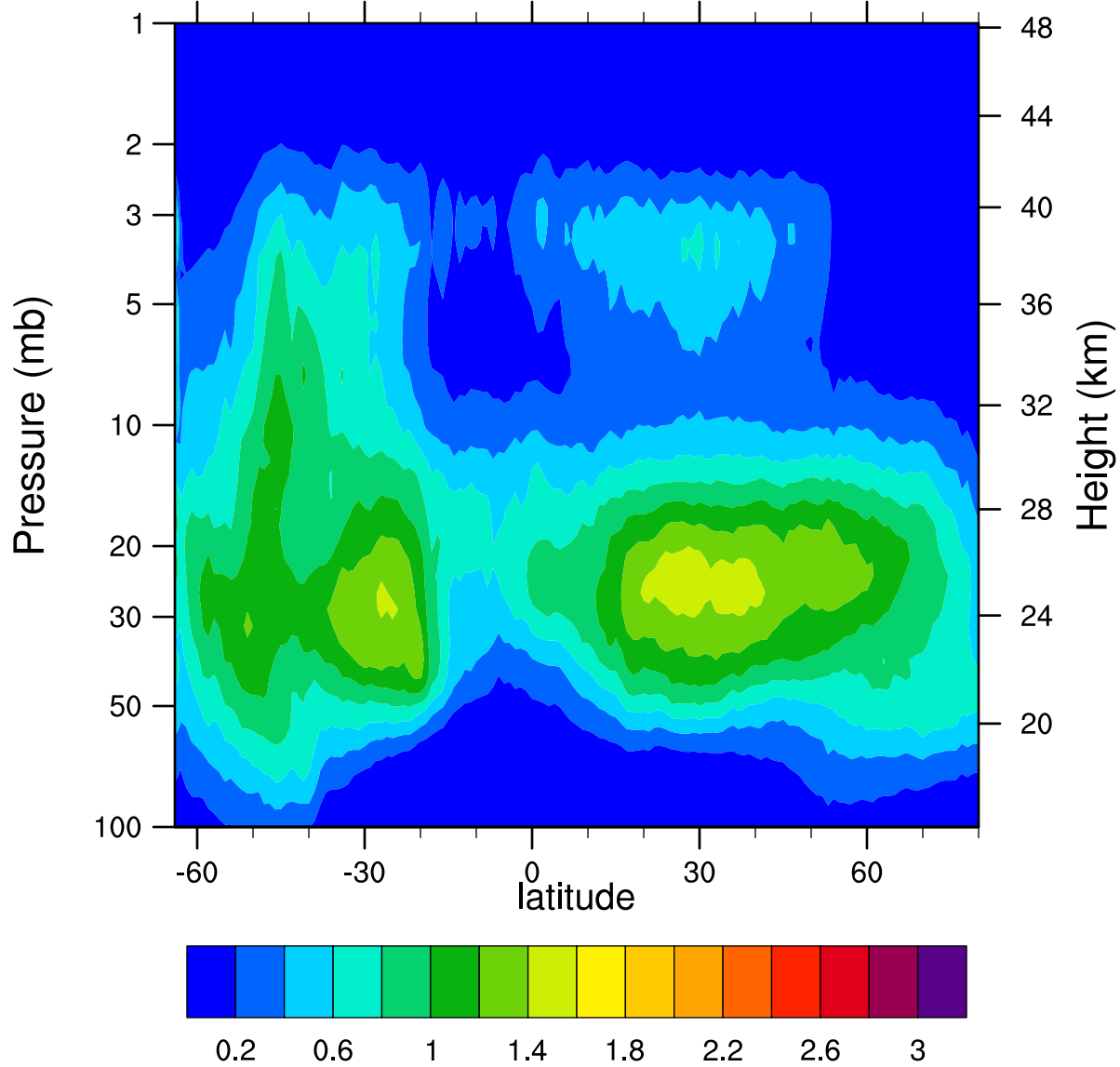
HIRDLSv6 2007d187 ClONO2_Ascending (ppbv)
