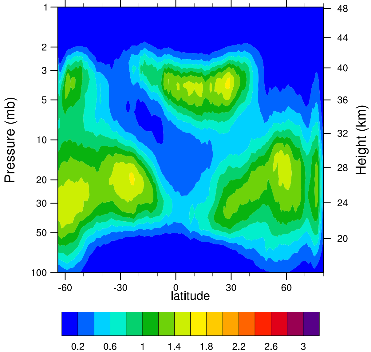
HIRDLSv6 2006d343 ClONO2_Ascending (ppbv)
