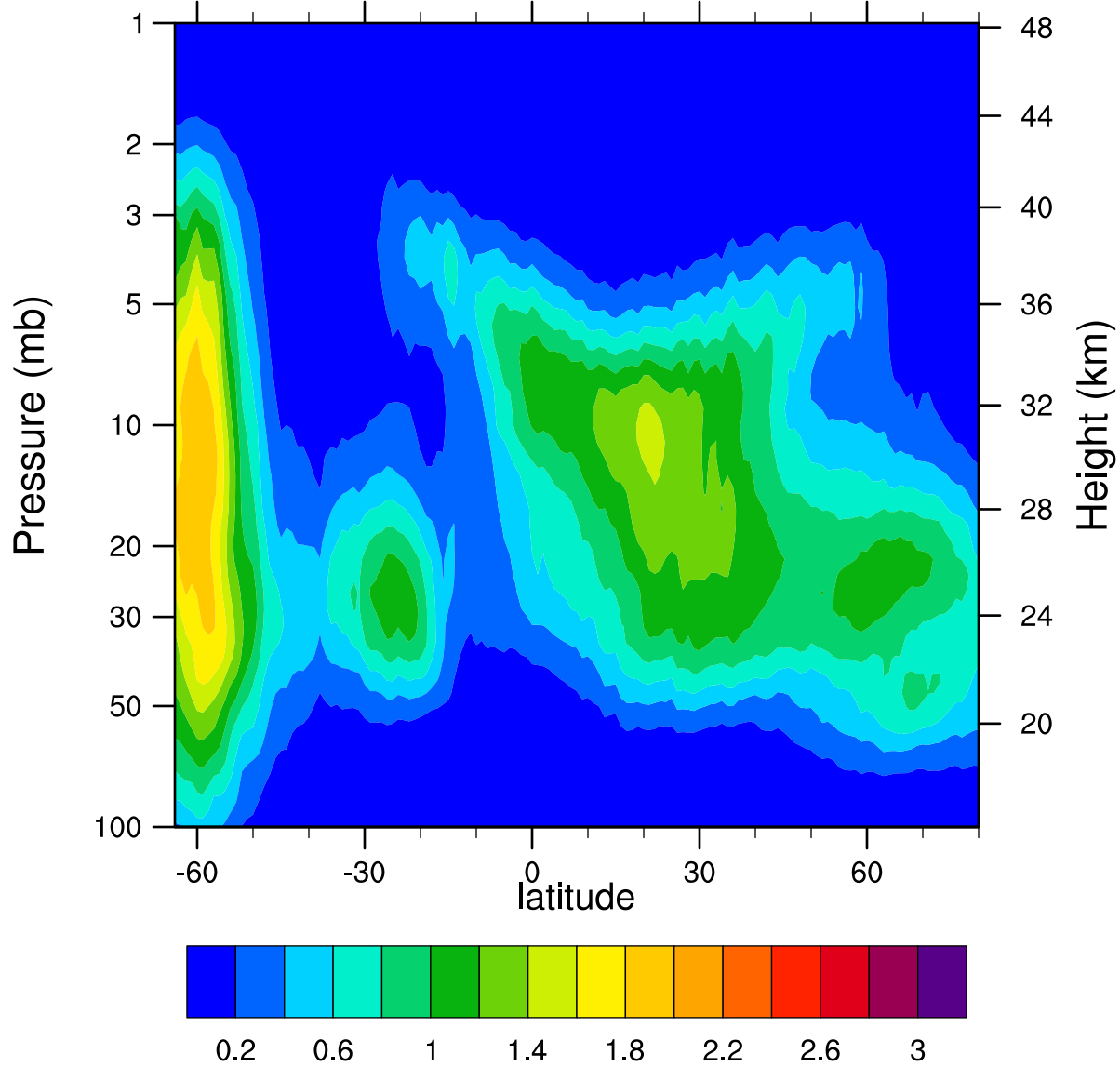
HIRDLSv6 2005d177 ClONO2_Ascending (ppbv)
