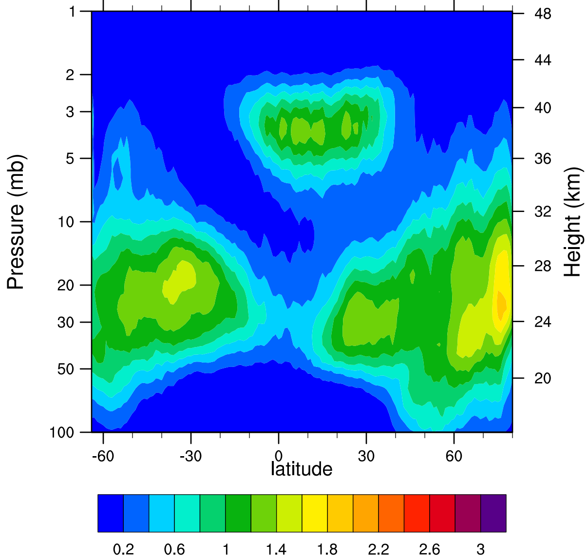
HIRDLSv6 2007d015 ClONO2_Ascending (ppbv)
