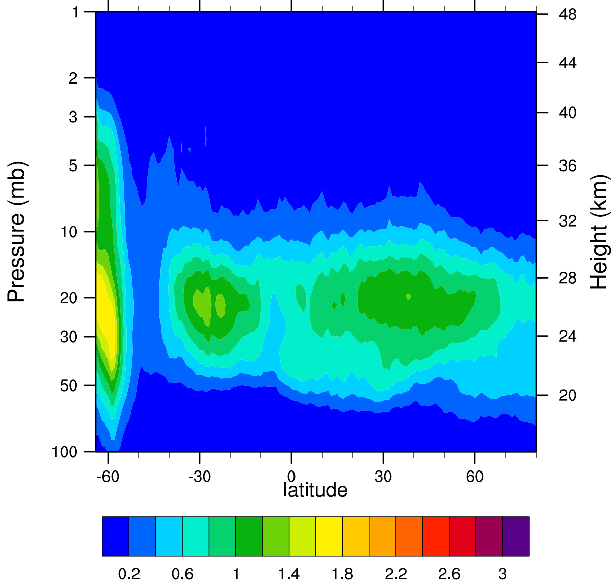
HIRDLSv6 2006d198 ClONO2_Ascending (ppbv)
