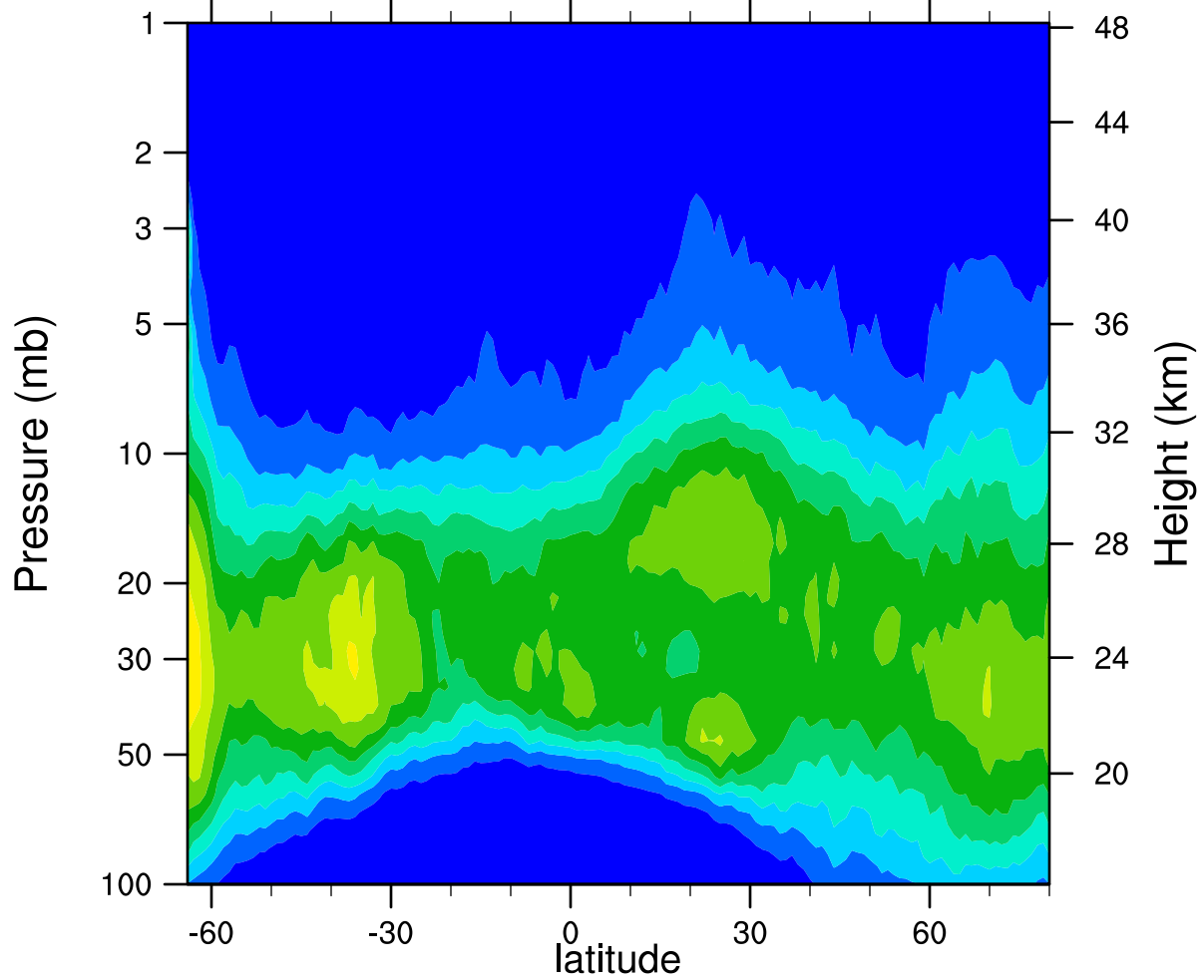
HIRDLSv6 2006d090 ClONO2_Ascending (ppbv)
