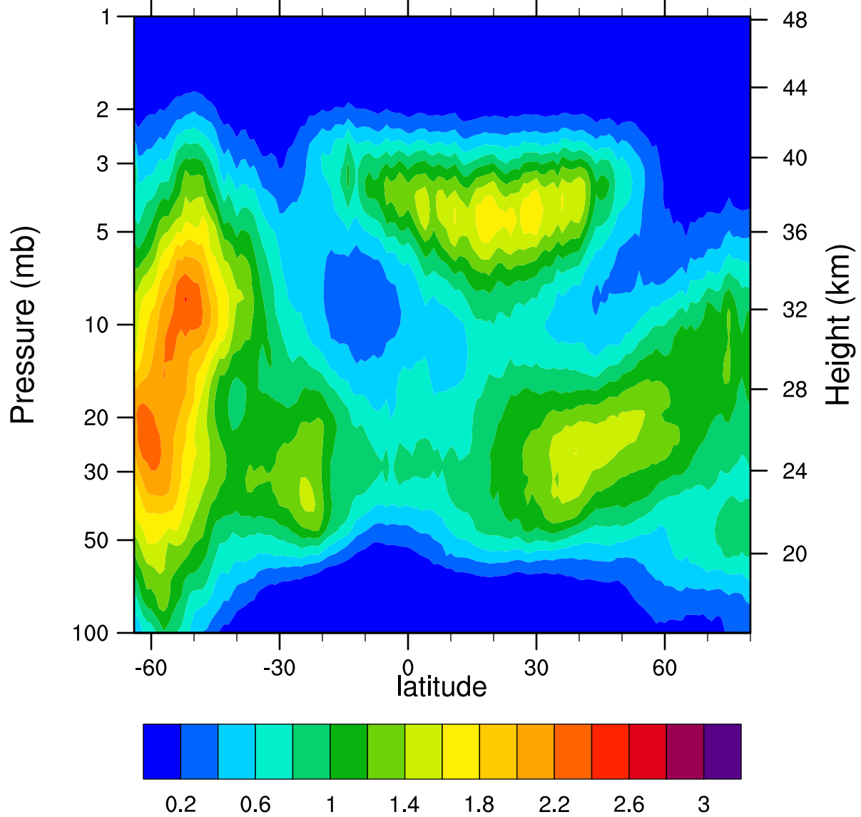
HIRDLSv6 2007d237 ClONO2_Ascending (ppbv)
