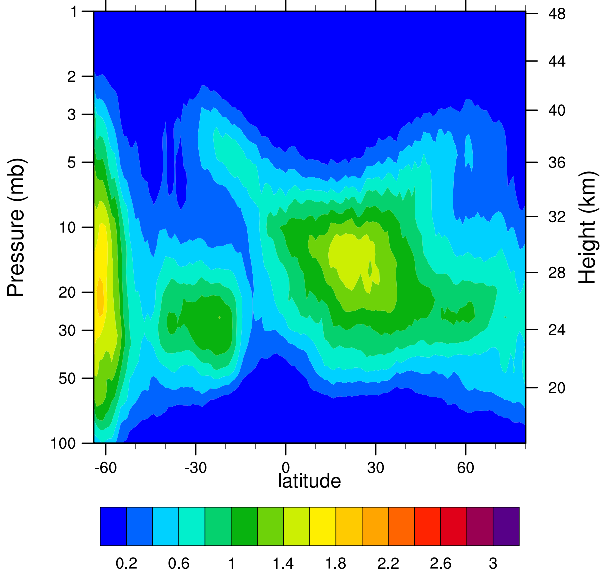
HIRDLSv6 2005d245 ClONO2_Ascending (ppbv)
