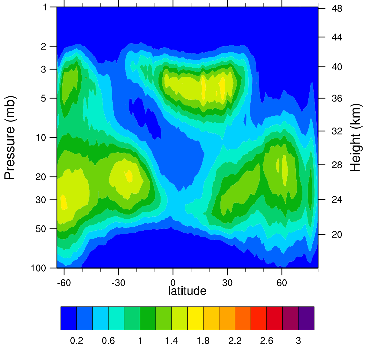
HIRDLSv6 2006d339 ClONO2_Ascending (ppbv)
