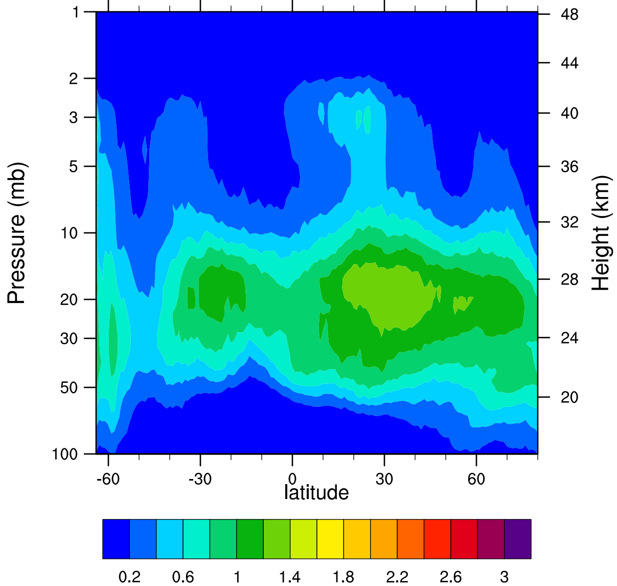
HIRDLSv6 2006d151 ClONO2_Ascending (ppbv)
