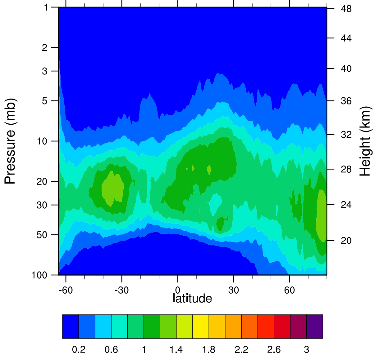
HIRDLSv6 2006d068 ClONO2_Ascending (ppbv)
