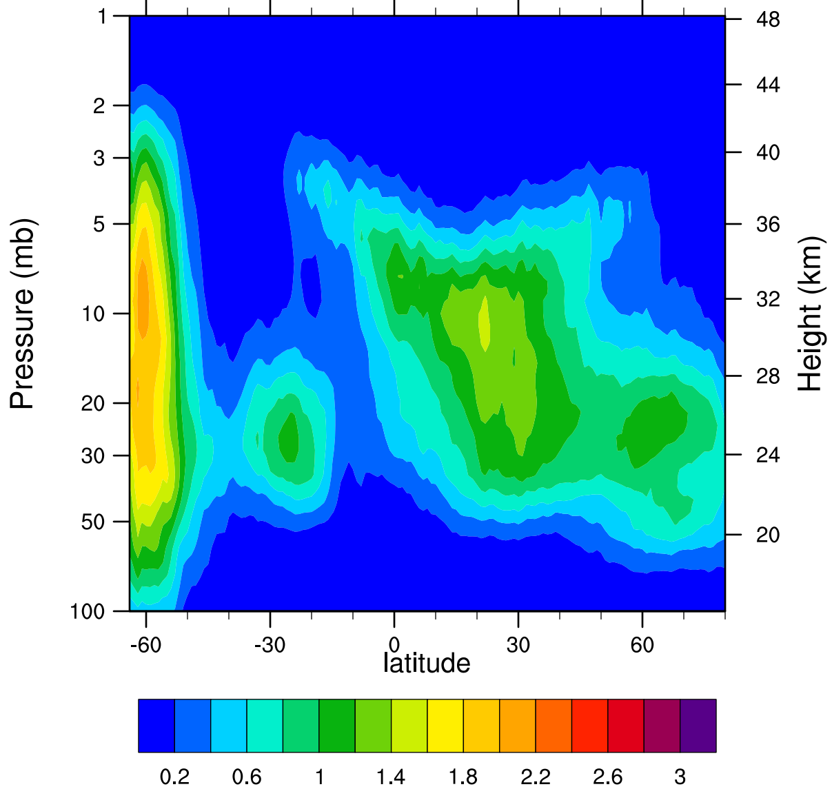
HIRDLSv6 2005d173 ClONO2_Ascending (ppbv)
