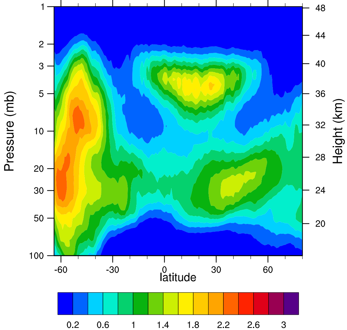
HIRDLSv6 2007d223 ClONO2_Ascending (ppbv)
