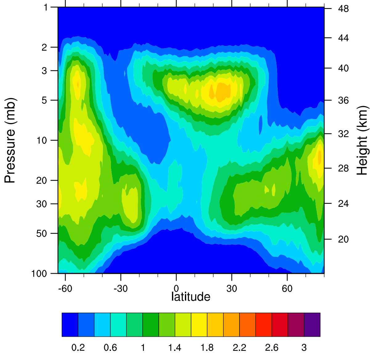
HIRDLSv6 2007d283 ClONO2_Ascending (ppbv)
