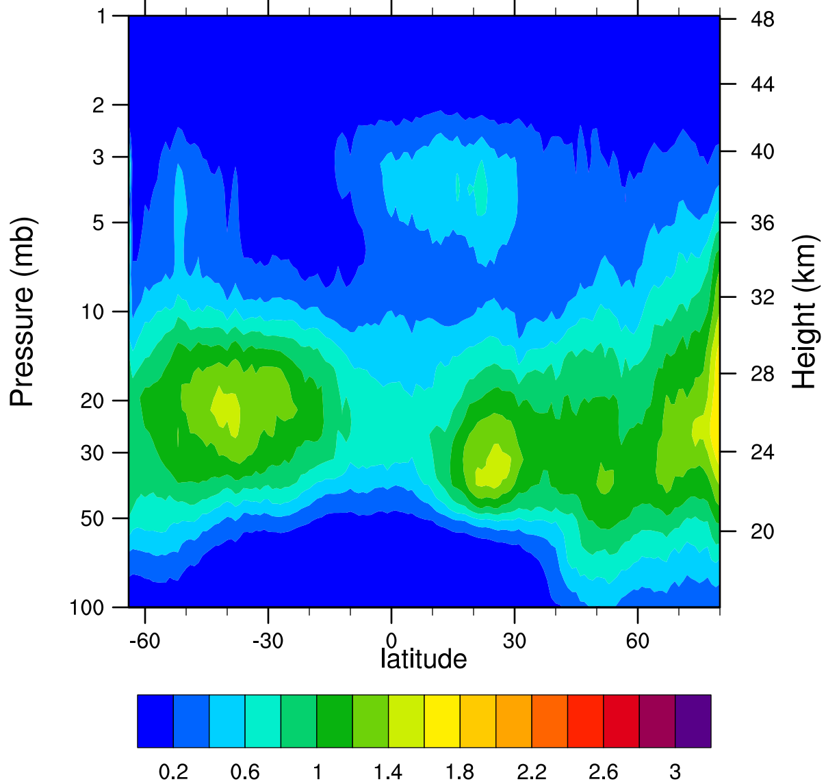
HIRDLSv6 2007d040 ClONO2_Ascending (ppbv)
