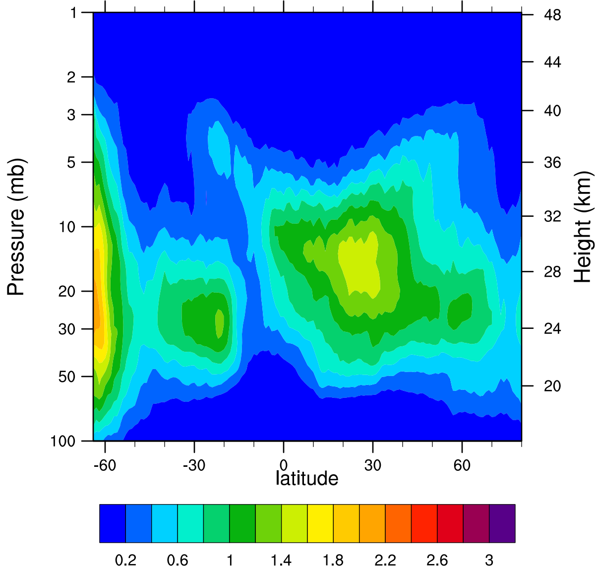
HIRDLSv6 2005d259 ClONO2_Ascending (ppbv)
