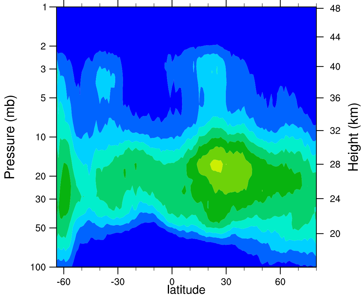
HIRDLSv6 2006d135 ClONO2_Ascending (ppbv)
