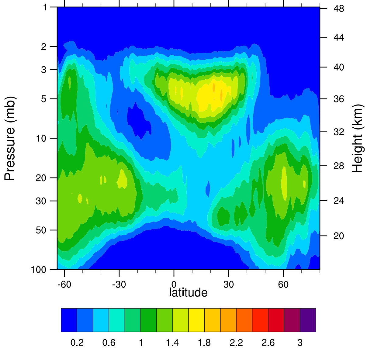
HIRDLSv6 2007d361 ClONO2_Ascending (ppbv)
