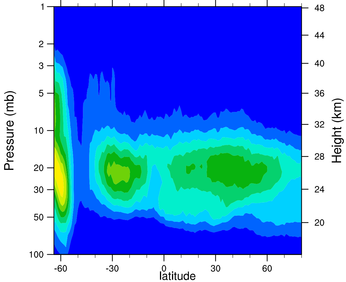
HIRDLSv6 2006d202 ClONO2_Ascending (ppbv)
