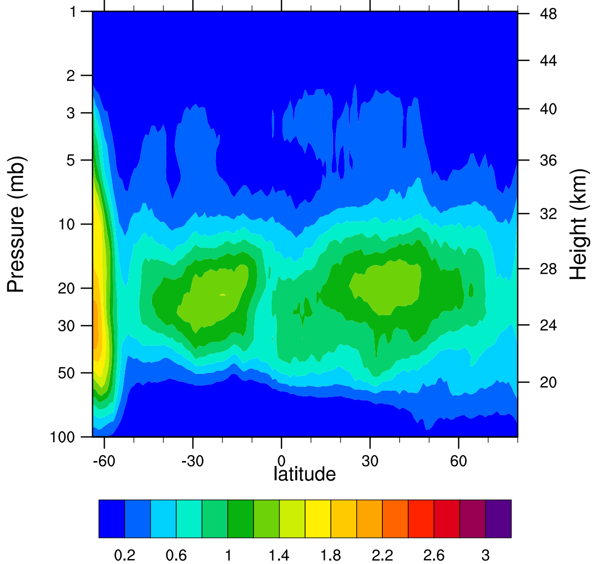
HIRDLSv6 2006d260 ClONO2_Ascending (ppbv)
