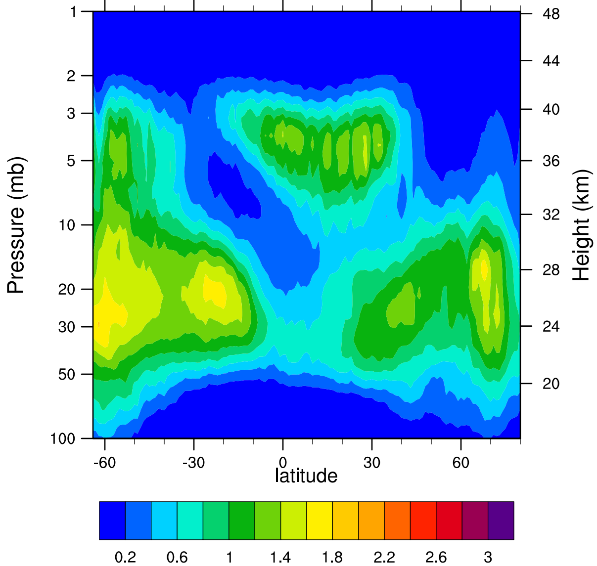
HIRDLSv6 2006d316 ClONO2_Ascending (ppbv)
