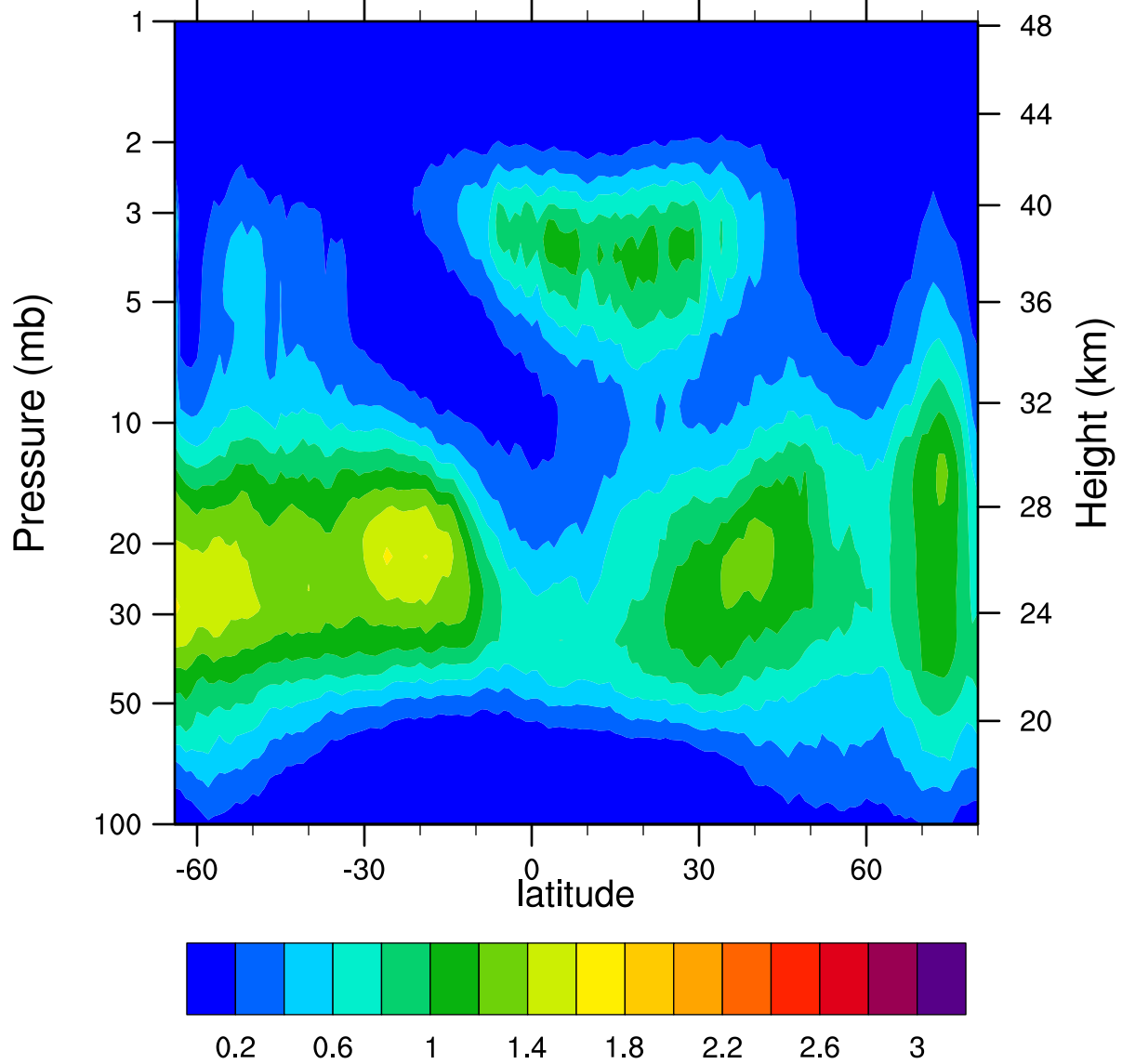
HIRDLSv6 2006d311 ClONO2_Ascending (ppbv)
