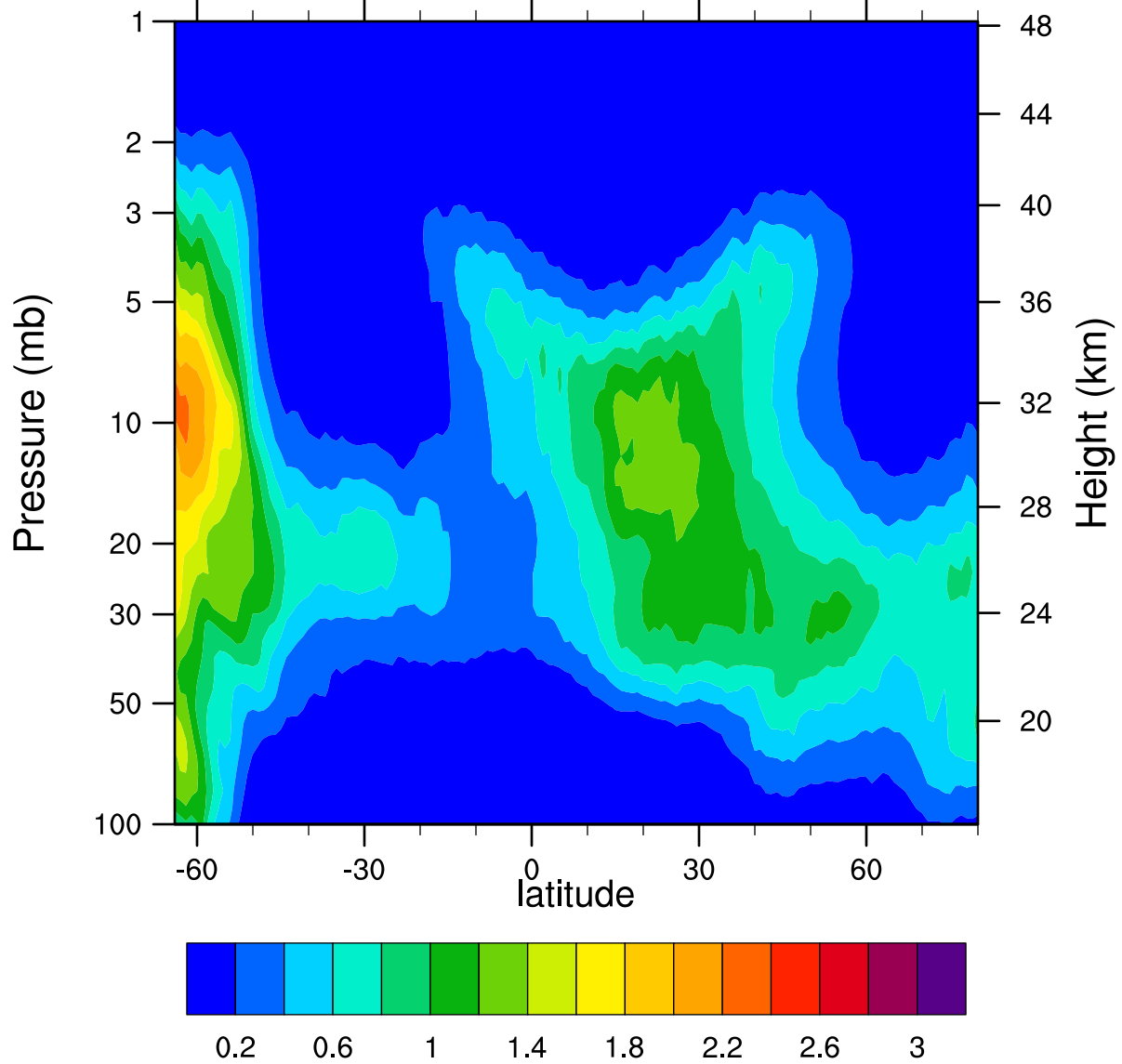
HIRDLSv6 2005d110 ClONO2_Ascending (ppbv)
