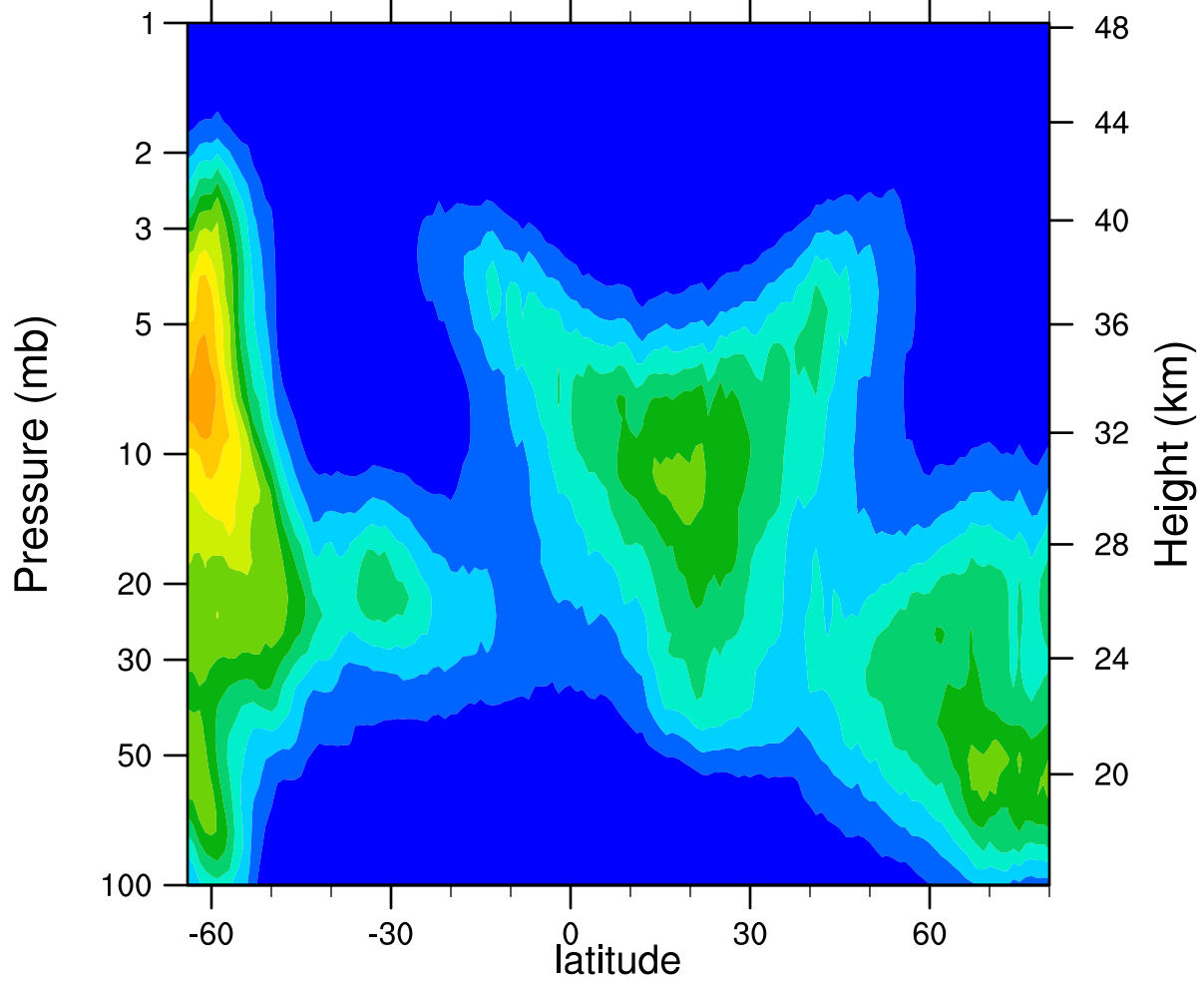
HIRDLSv6 2005d078 ClONO2_Ascending (ppbv)
