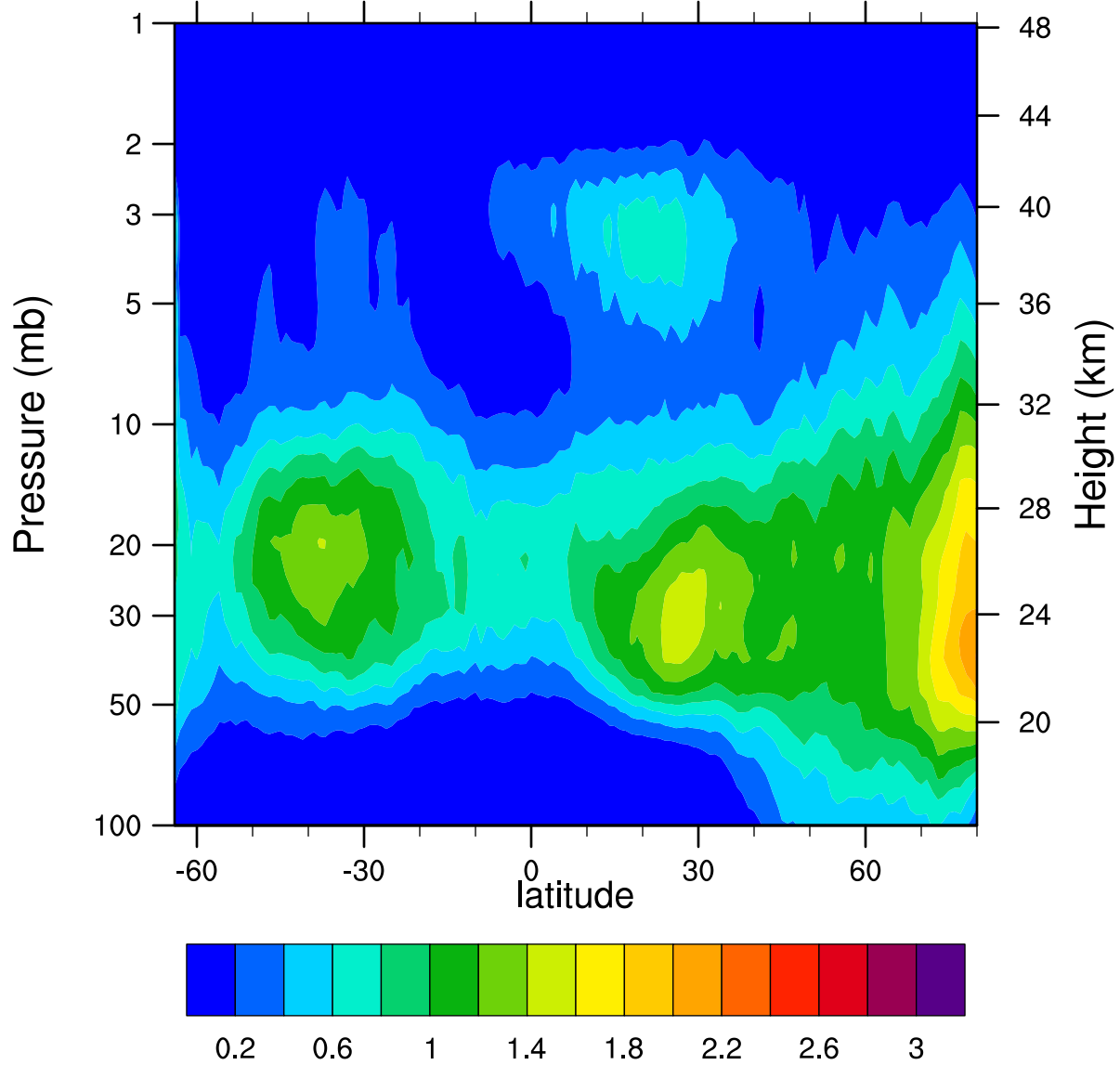
HIRDLSv6 2007d070 ClONO2_Ascending (ppbv)
