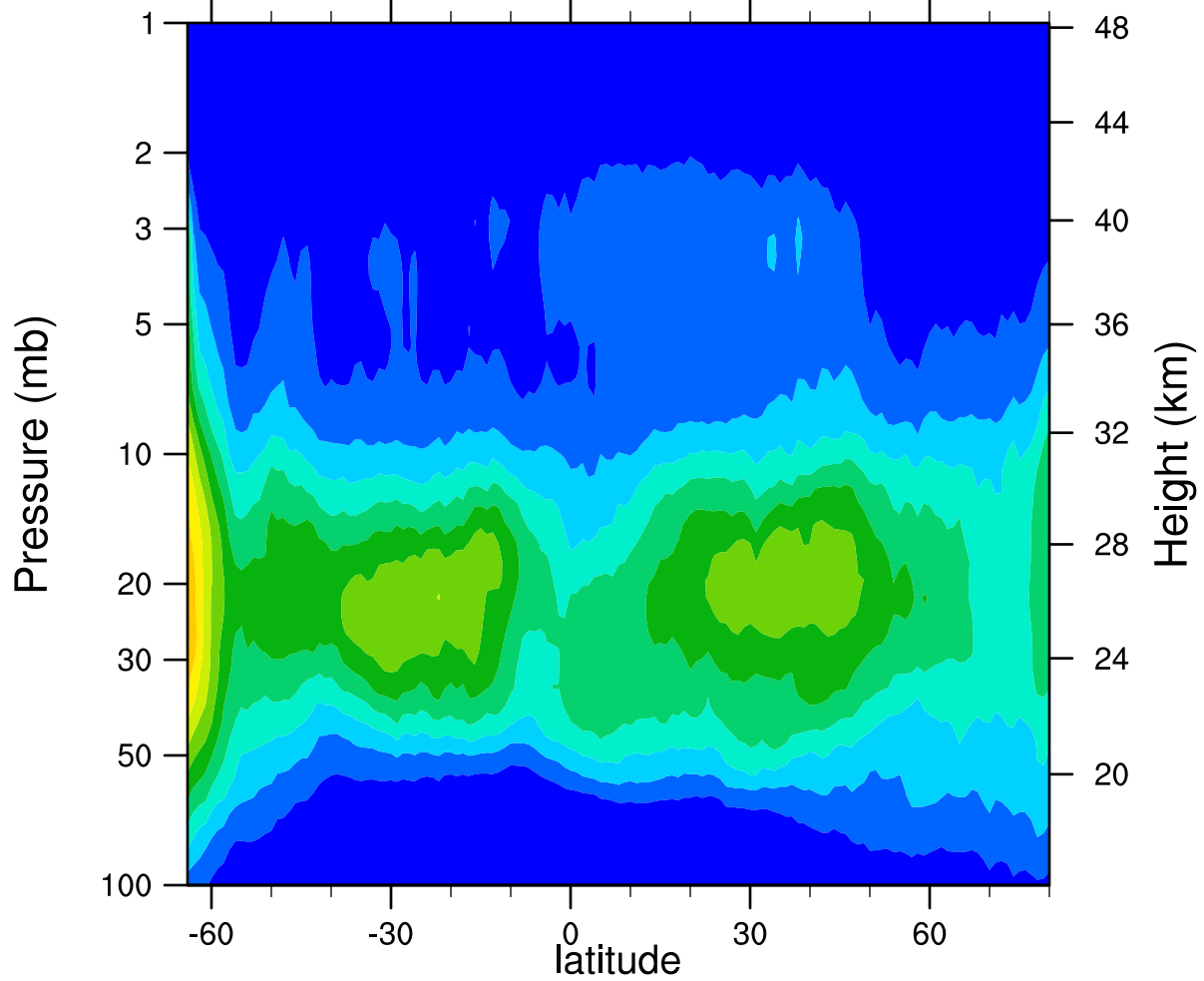
HIRDLSv6 2006d273 ClONO2_Ascending (ppbv)
