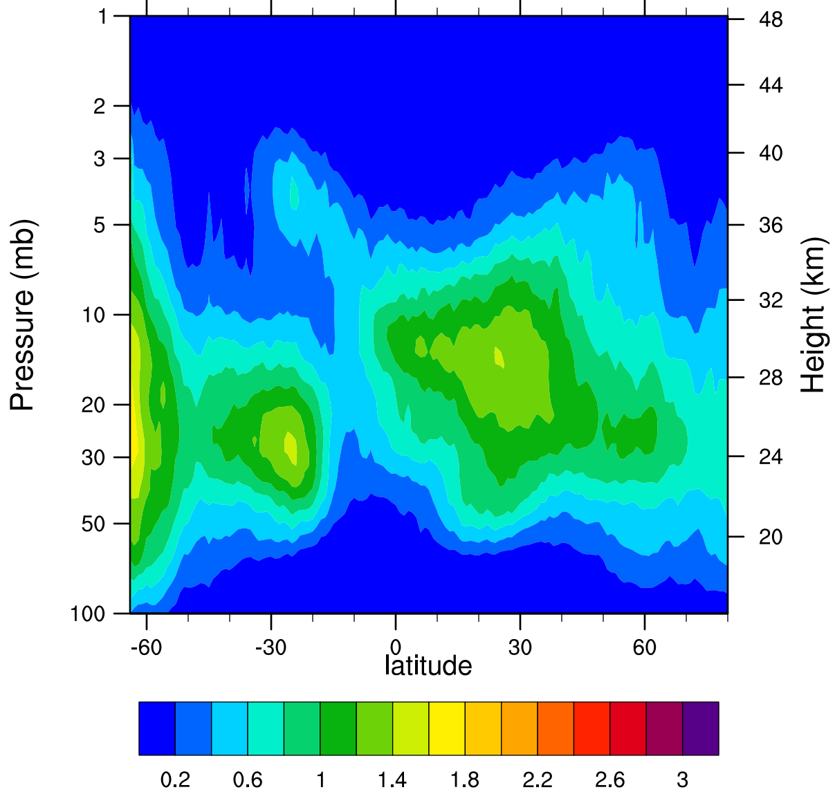
HIRDLSv6 2005d276 ClONO2_Ascending (ppbv)
