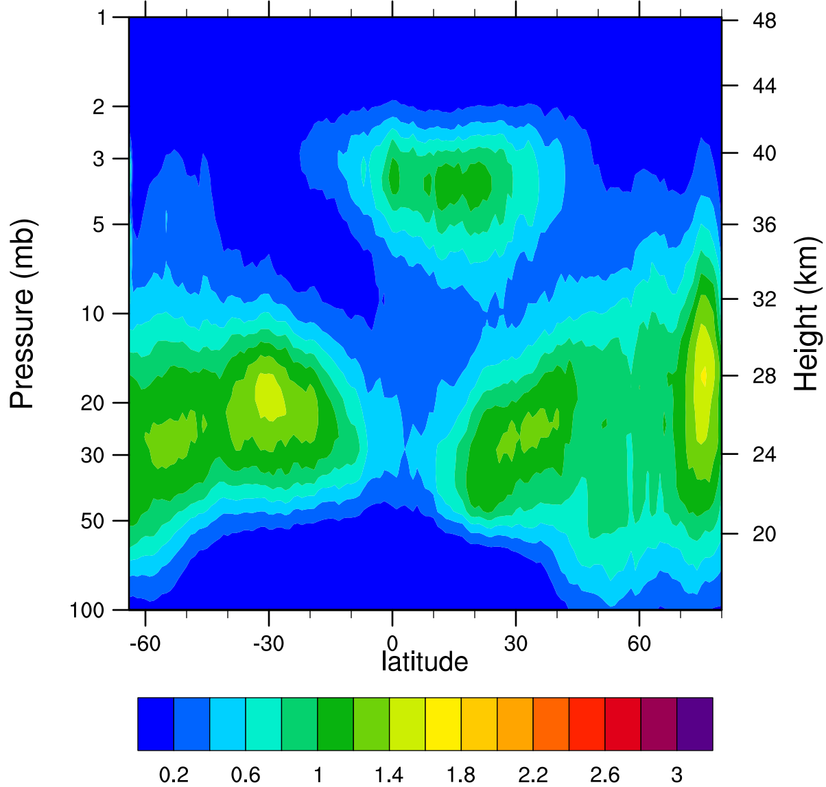
HIRDLSv6 2006d362 ClONO2_Ascending (ppbv)
