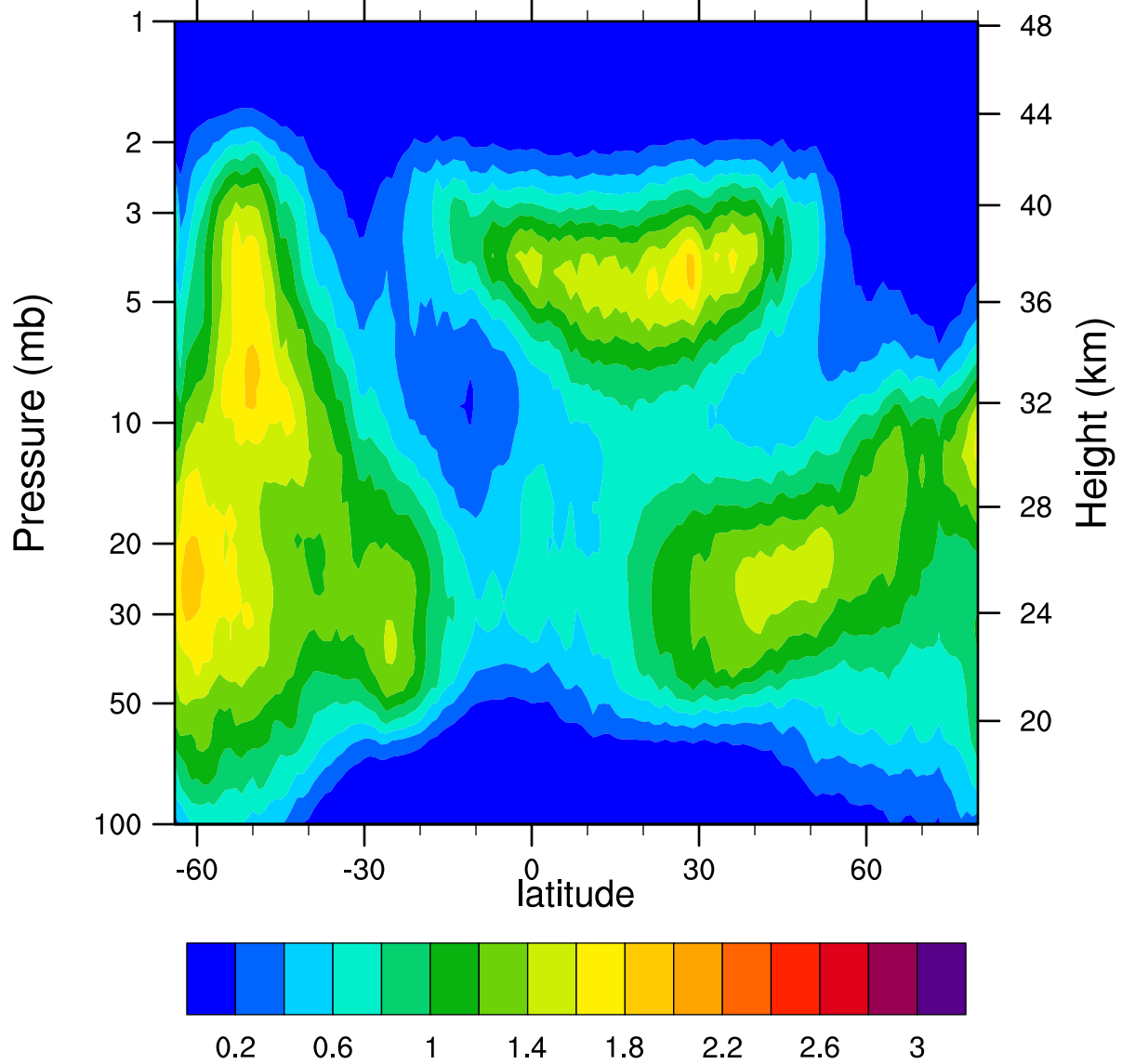
HIRDLSv6 2007d260 ClONO2_Ascending (ppbv)
