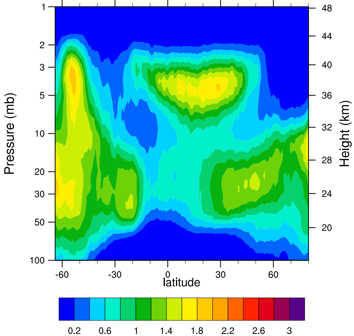
HIRDLSv6 2007d272 ClONO2_Ascending (ppbv)
