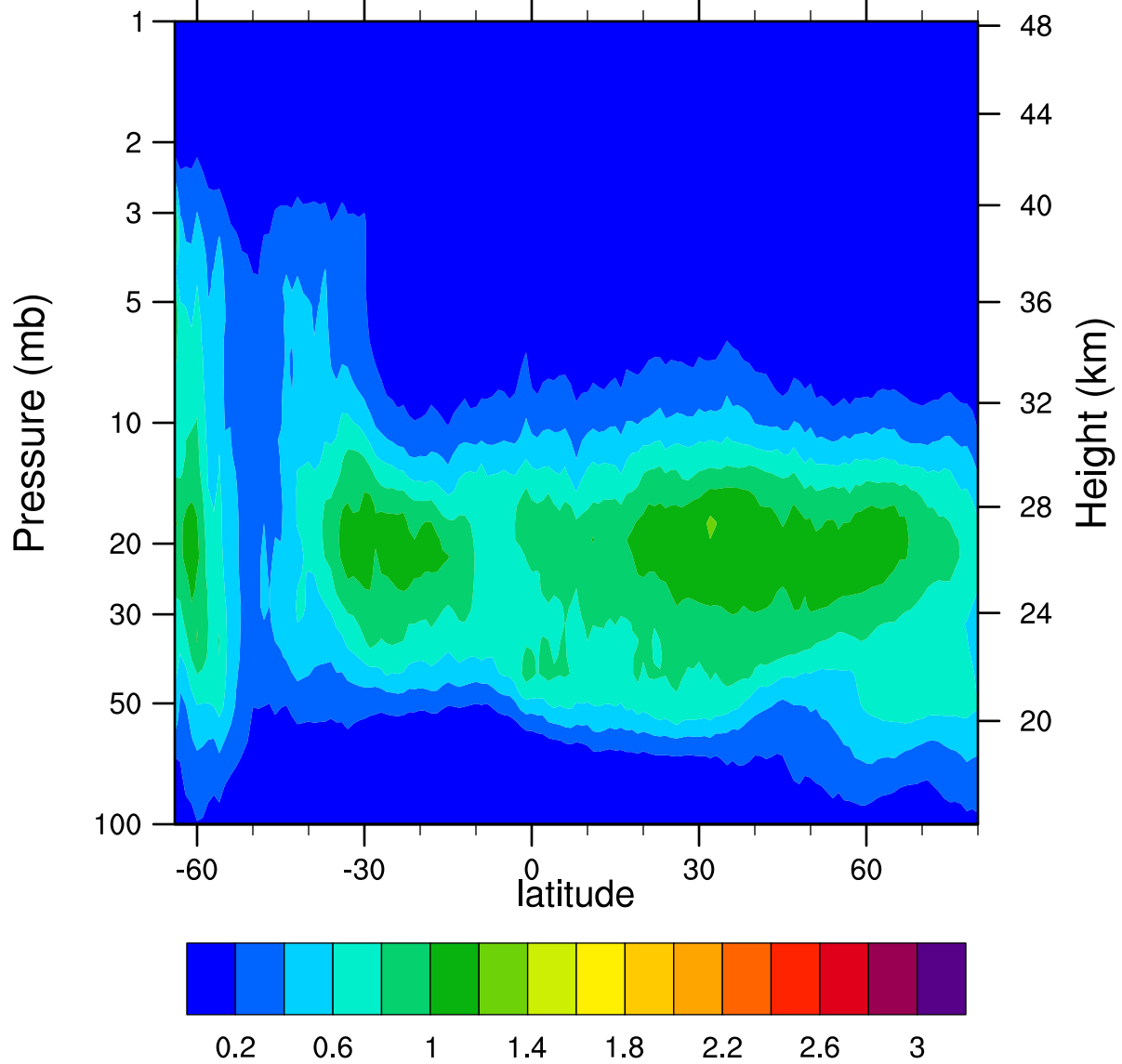
HIRDLSv6 2006d181 ClONO2_Ascending (ppbv)
