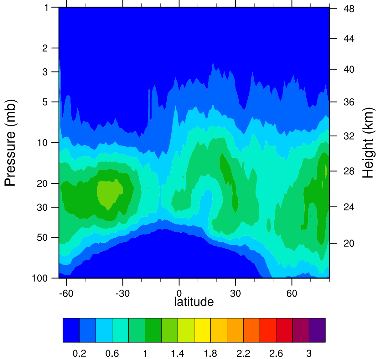
HIRDLSv6 2006d021 ClONO2_Ascending (ppbv)
