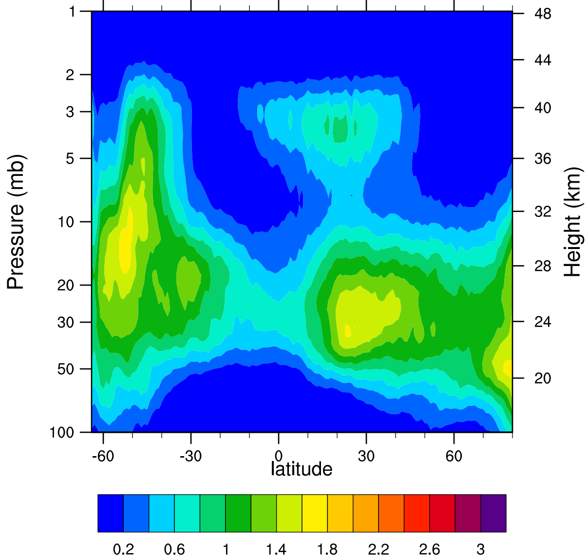
HIRDLSv6 2007d112 ClONO2_Ascending (ppbv)
