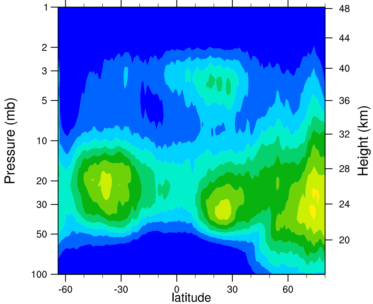
HIRDLSv6 2007d054 ClONO2_Ascending (ppbv)
