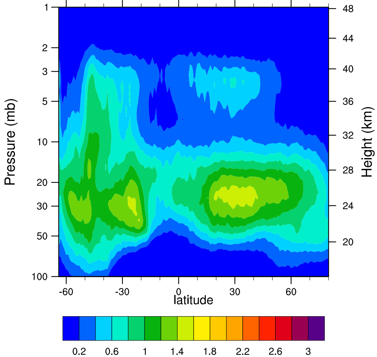
HIRDLSv6 2007d192 ClONO2_Ascending (ppbv)
