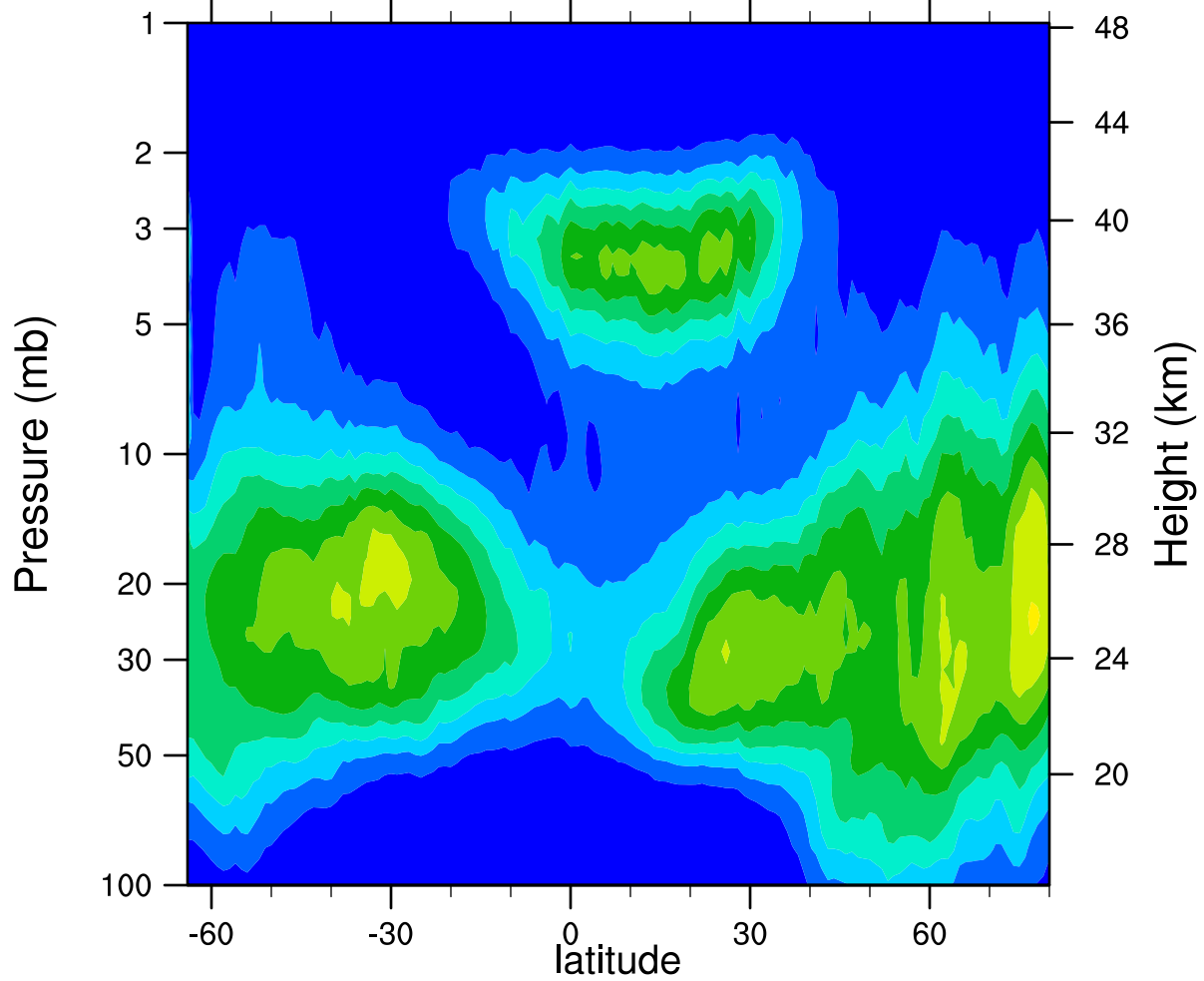
HIRDLSv6 2007d022 ClONO2_Ascending (ppbv)
