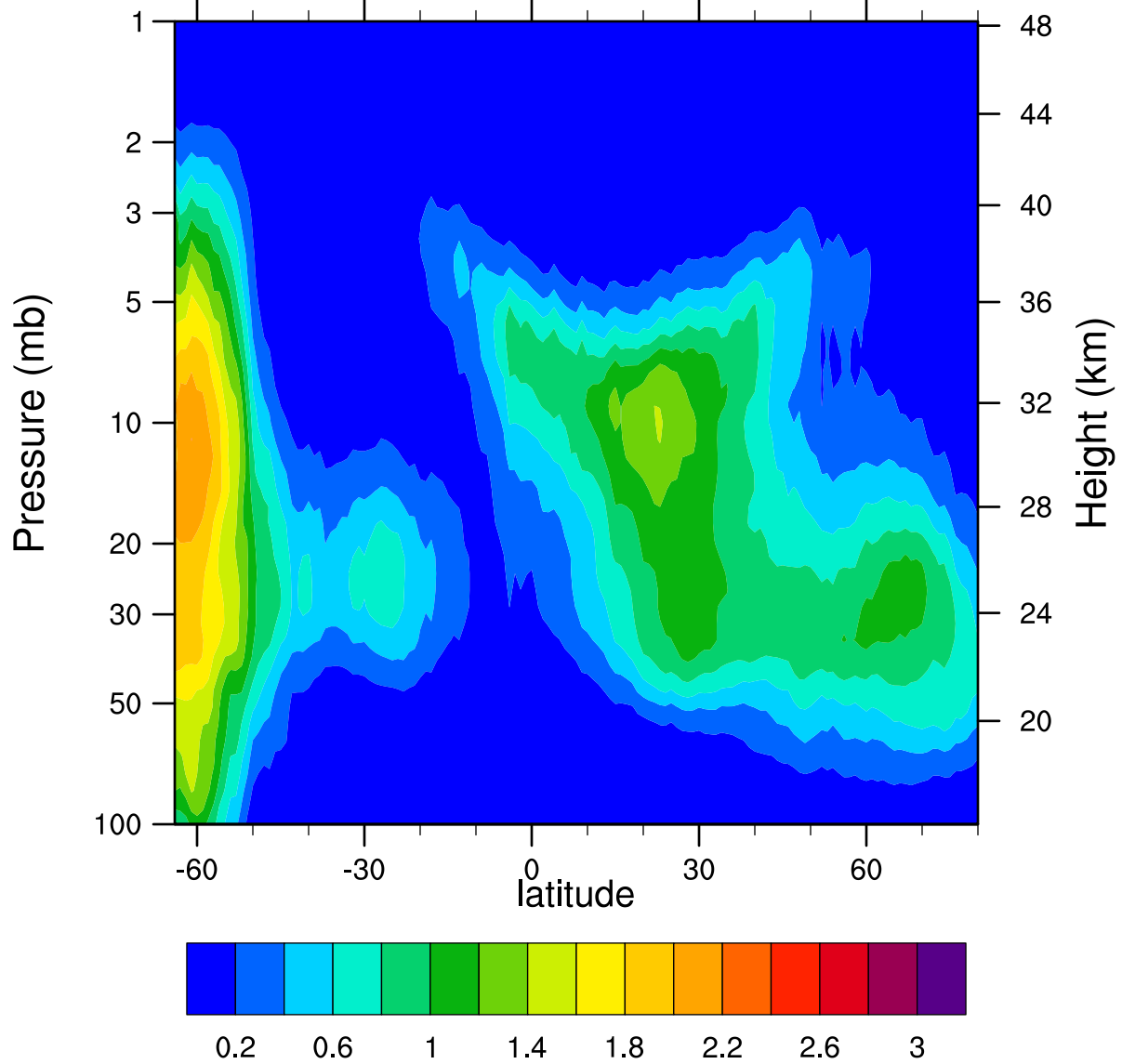
HIRDLSv6 2005d130 ClONO2_Ascending (ppbv)
