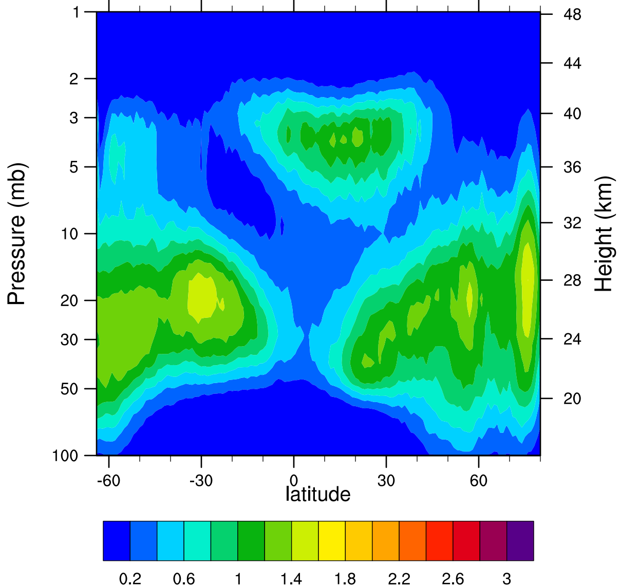
HIRDLSv6 2006d356 ClONO2_Ascending (ppbv)
