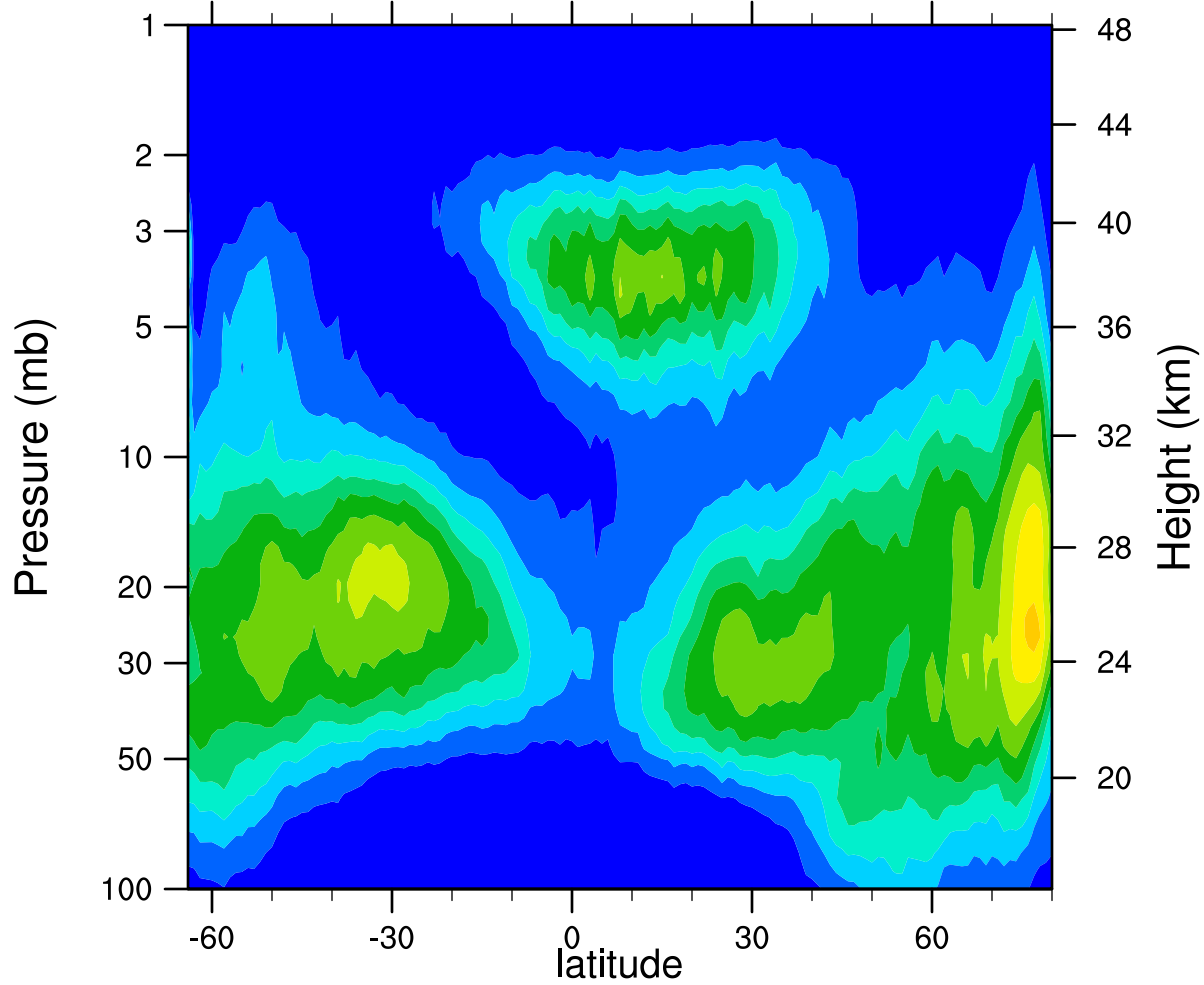
HIRDLSv6 2007d010 ClONO2_Ascending (ppbv)
