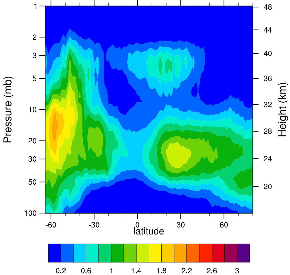
HIRDLSv6 2007d135 ClONO2_Ascending (ppbv)
