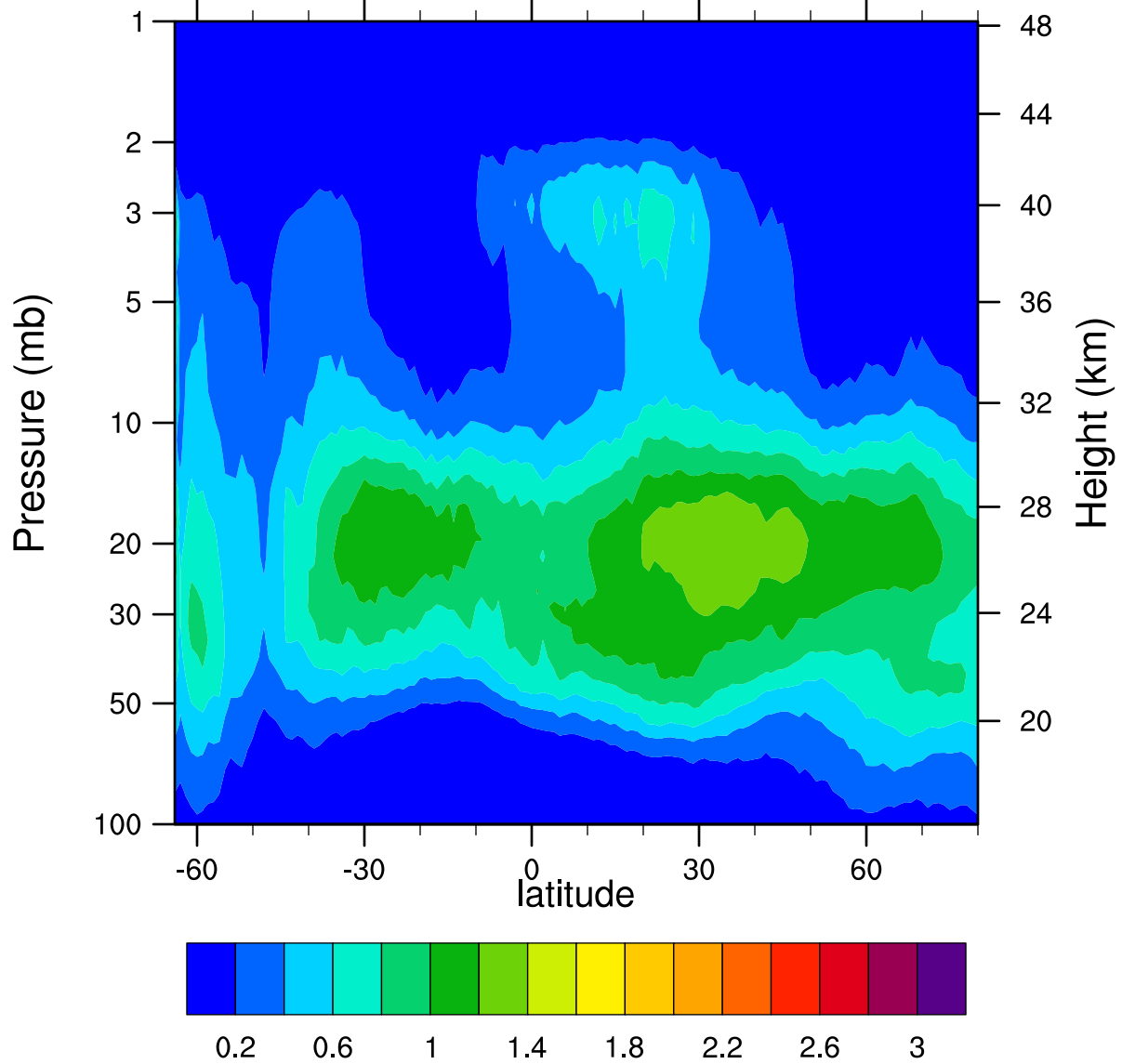
HIRDLSv6 2006d169 ClONO2_Ascending (ppbv)
