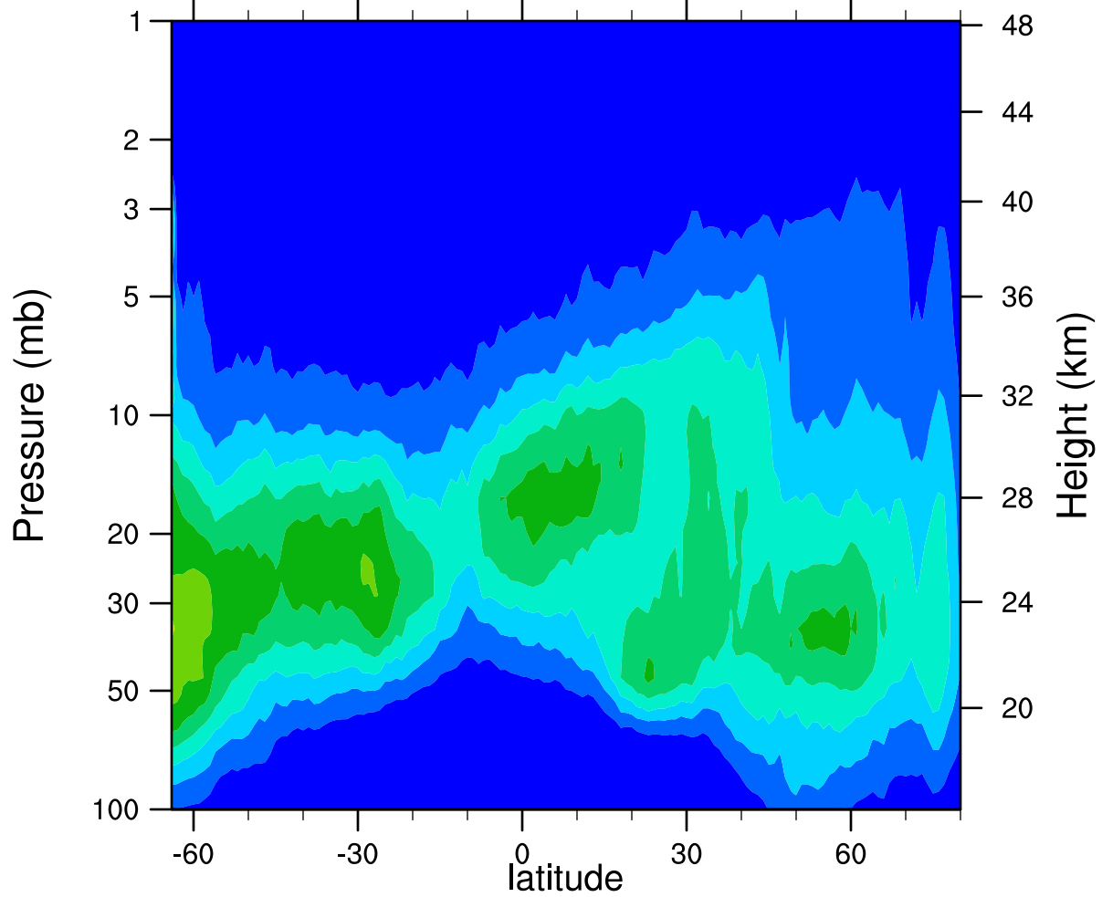
HIRDLSv6 2005d342 ClONO2_Ascending (ppbv)
