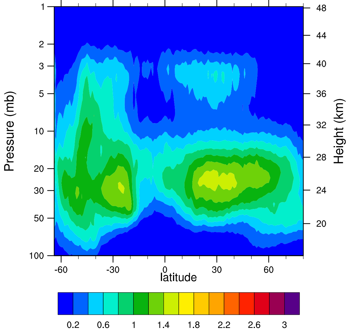
HIRDLSv6 2007d188 ClONO2_Ascending (ppbv)
