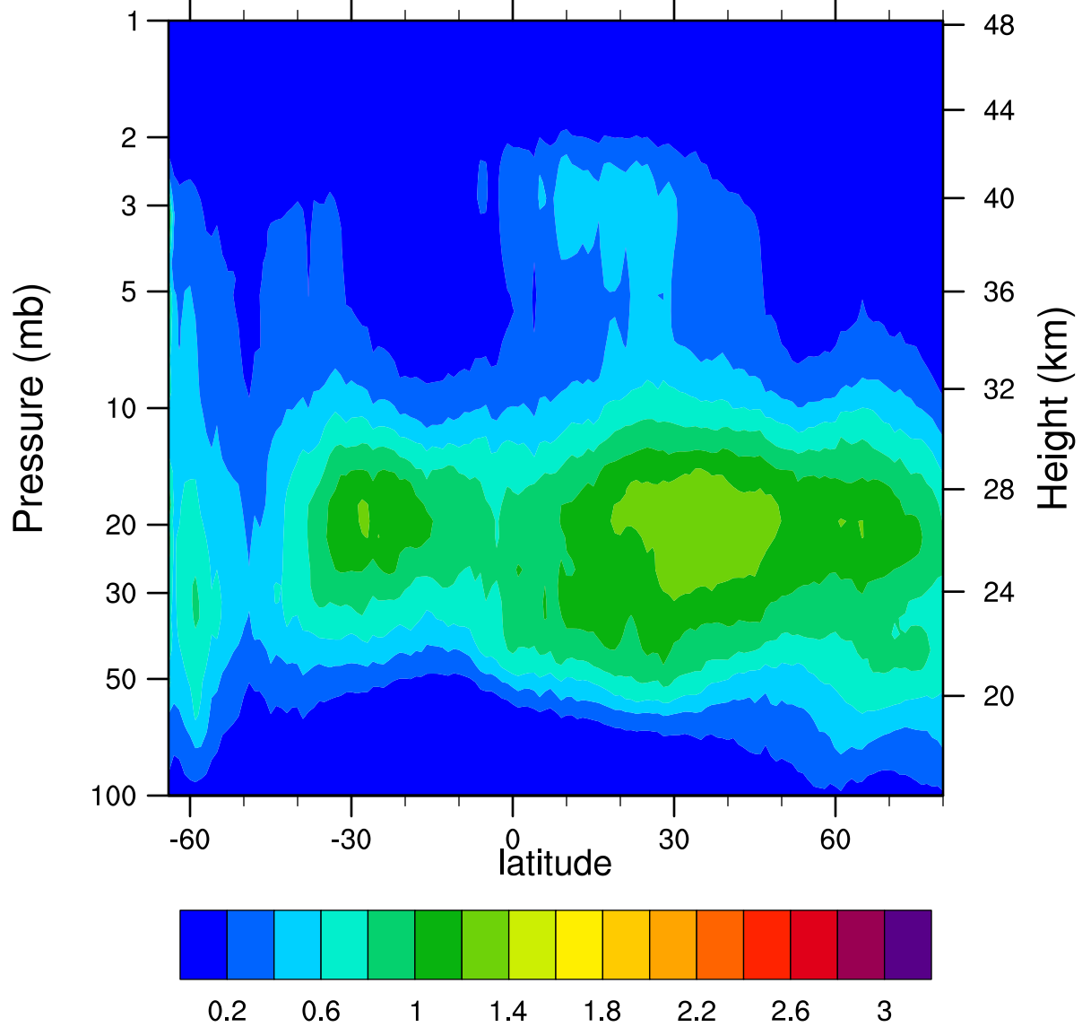
HIRDLSv6 2006d164 ClONO2_Ascending (ppbv)
