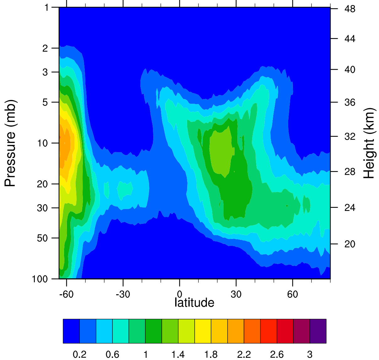
HIRDLSv6 2005d117 ClONO2_Ascending (ppbv)
