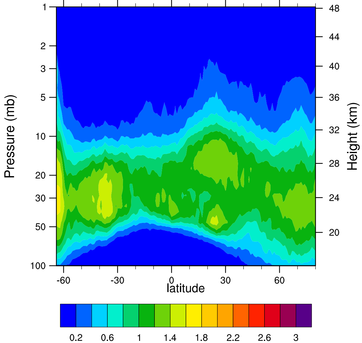
HIRDLSv6 2006d092 ClONO2_Ascending (ppbv)
