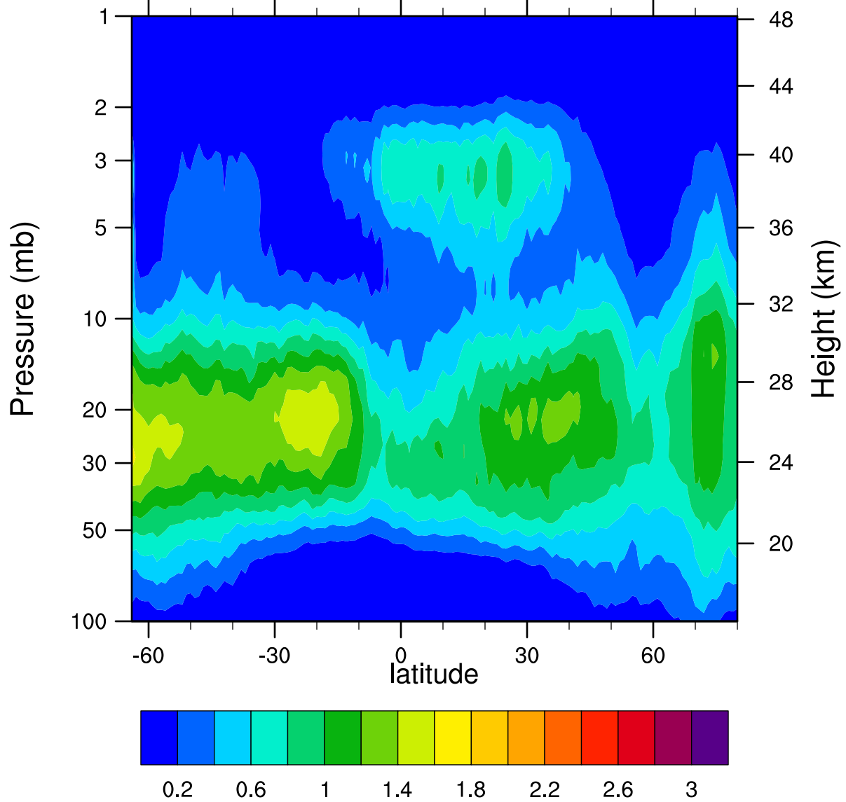
HIRDLSv6 2006d306 ClONO2_Ascending (ppbv)
