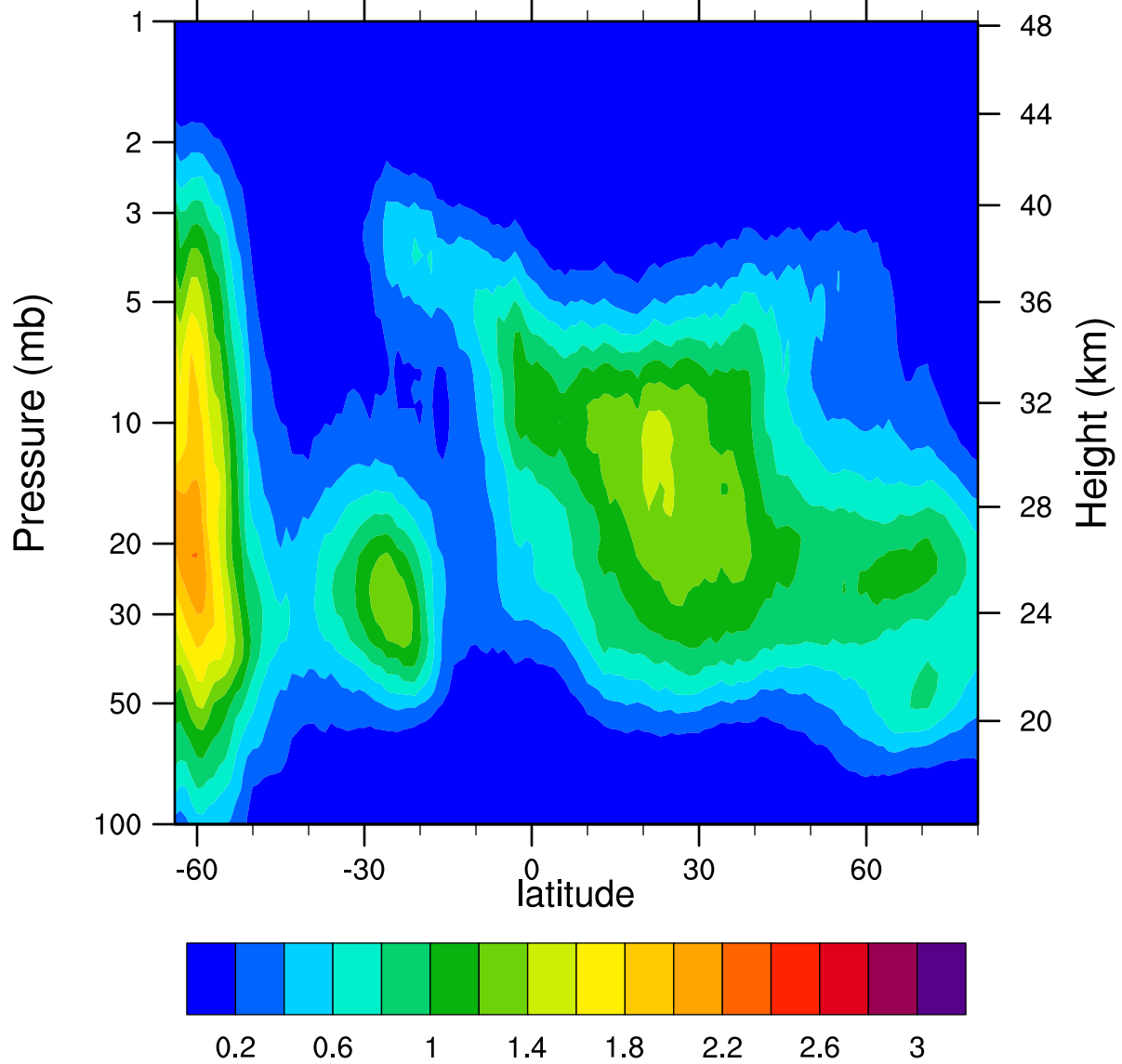
HIRDLSv6 2005d187 ClONO2_Ascending (ppbv)
