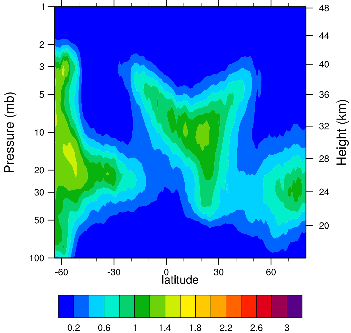
HIRDLSv6 2005d047 ClONO2_Ascending (ppbv)
