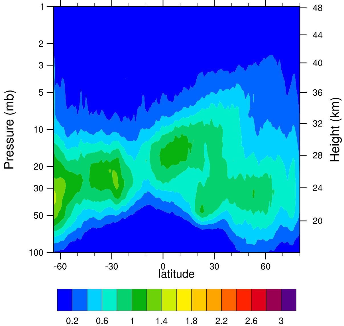
HIRDLSv6 2005d339 ClONO2_Ascending (ppbv)
