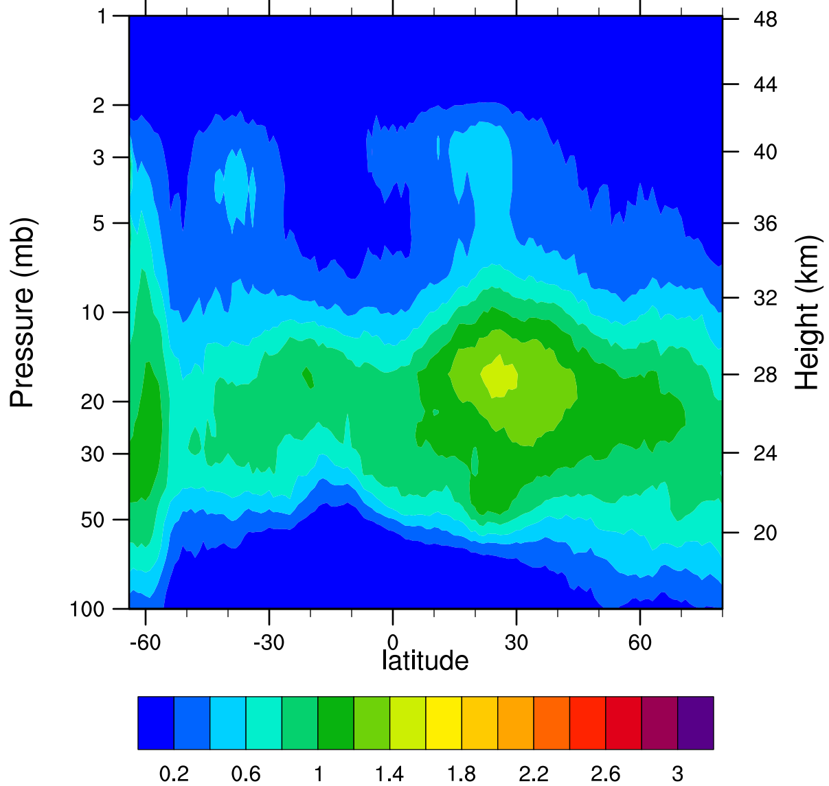
HIRDLSv6 2006d132 ClONO2_Ascending (ppbv)
