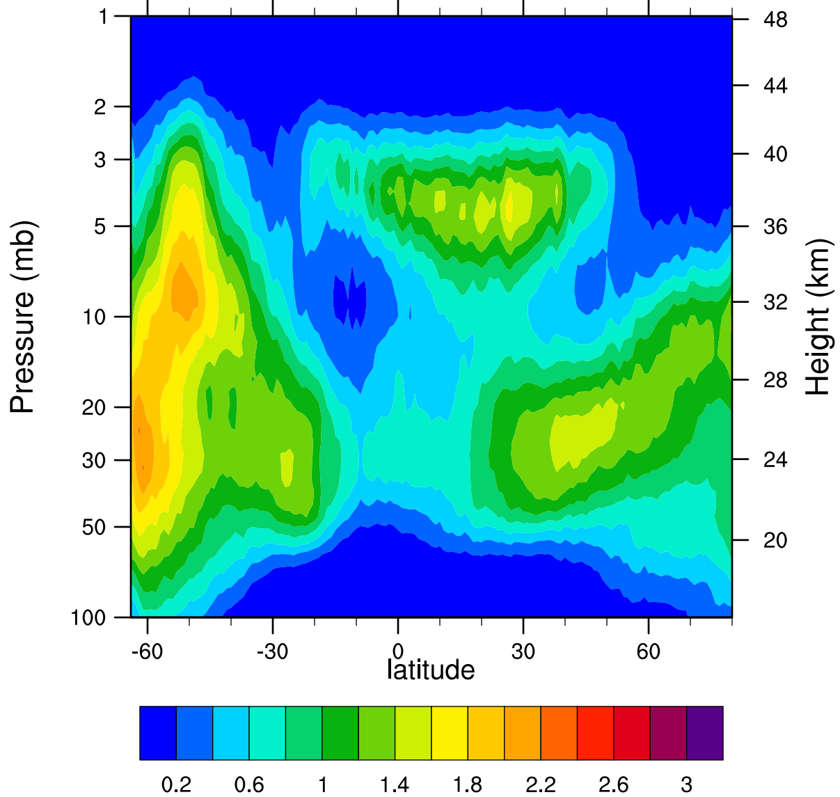
HIRDLSv6 2007d253 ClONO2_Ascending (ppbv)
