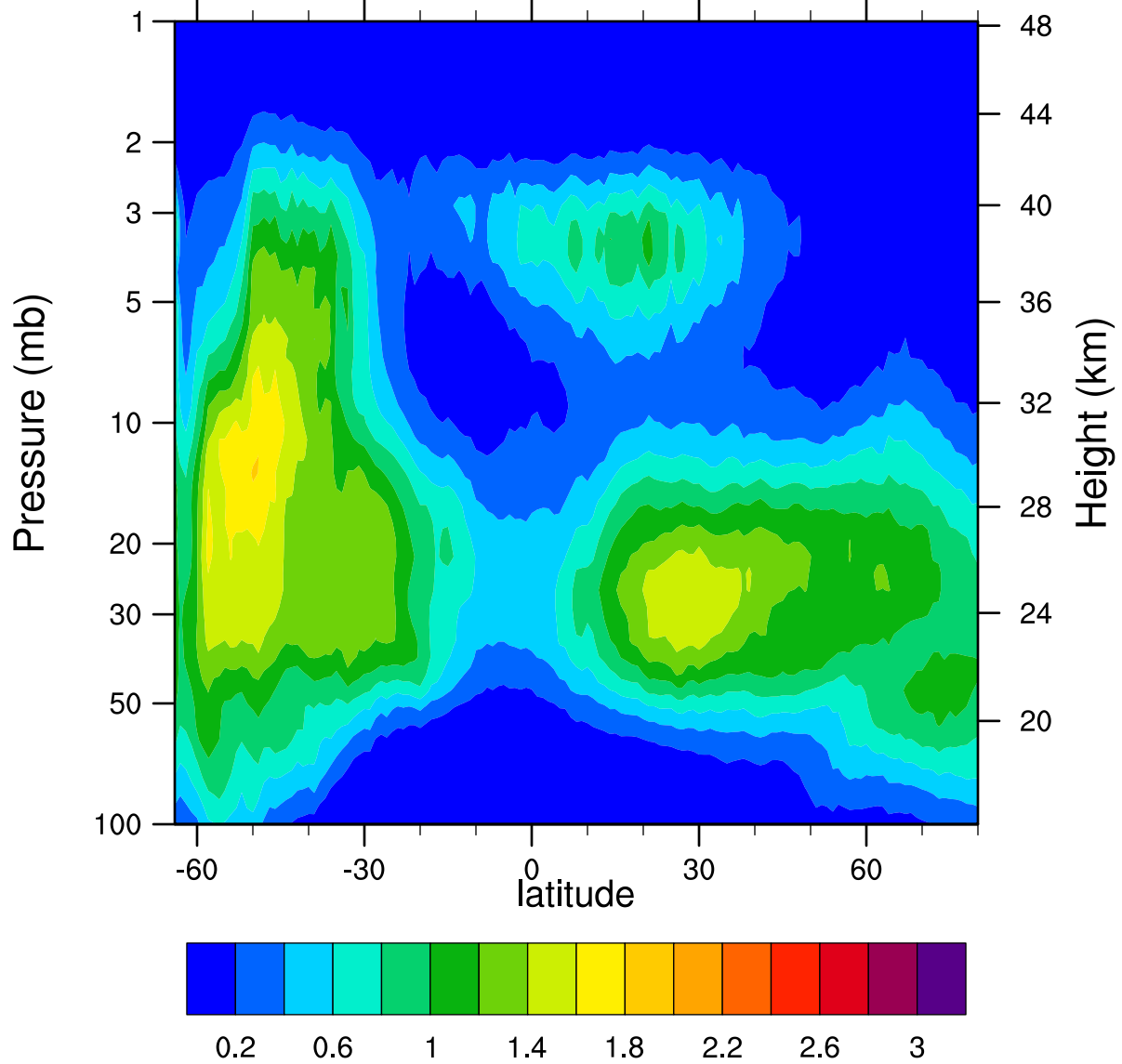
HIRDLSv6 2007d142 ClONO2_Ascending (ppbv)
