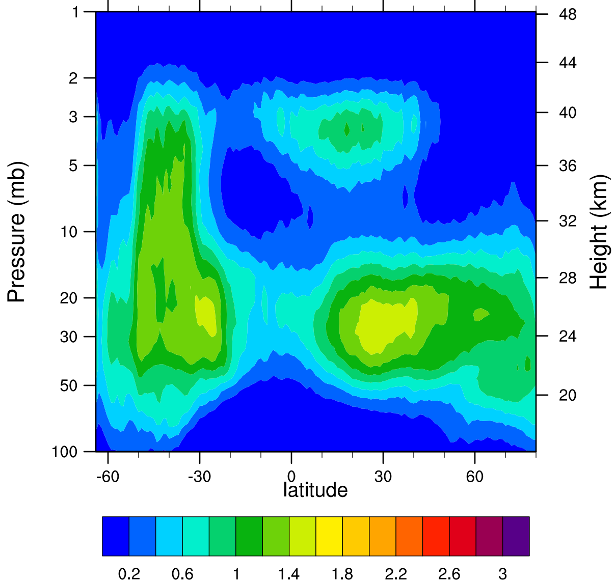
HIRDLSv6 2007d158 ClONO2_Ascending (ppbv)
