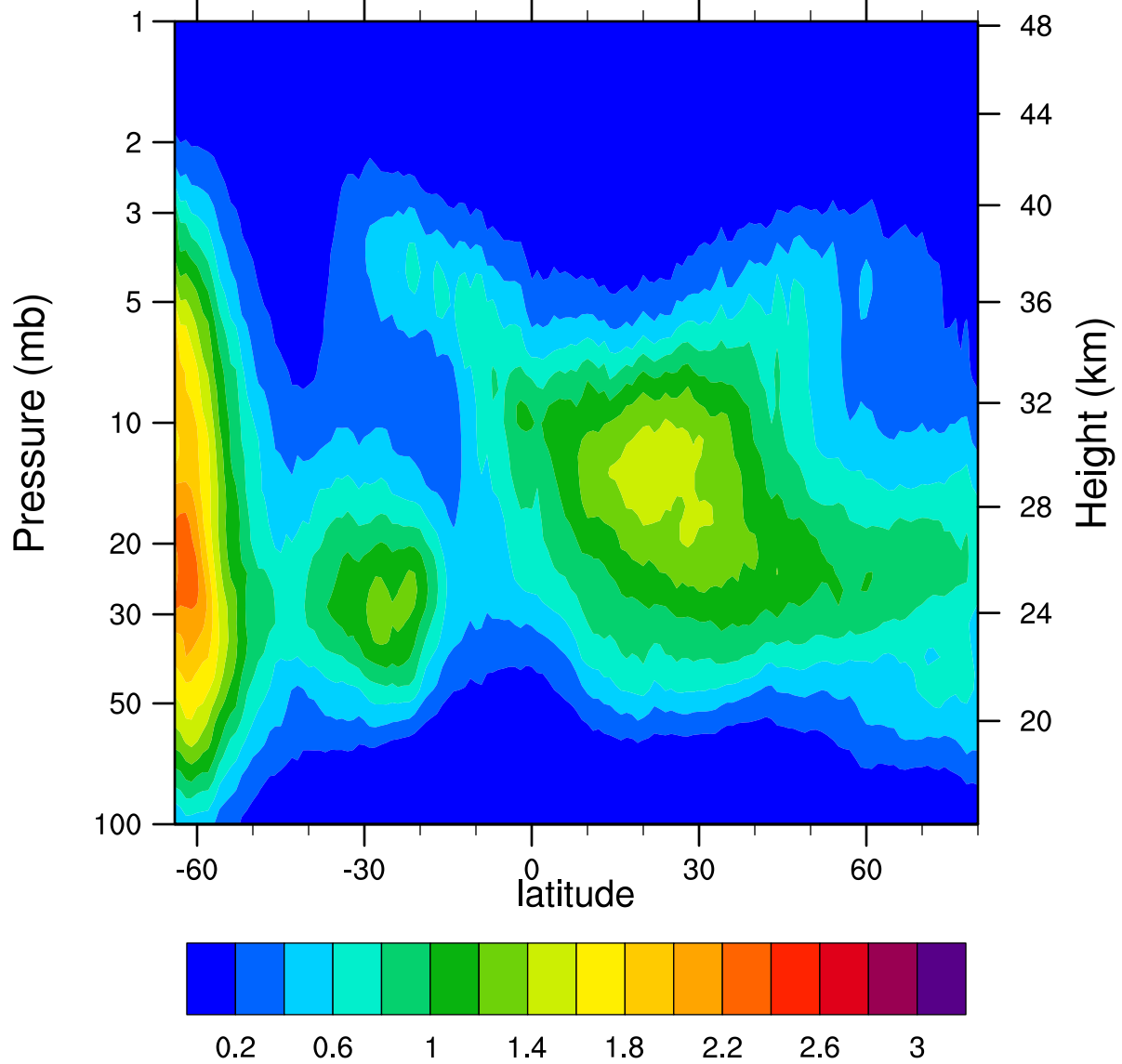
HIRDLSv6 2005d228 ClONO2_Ascending (ppbv)
