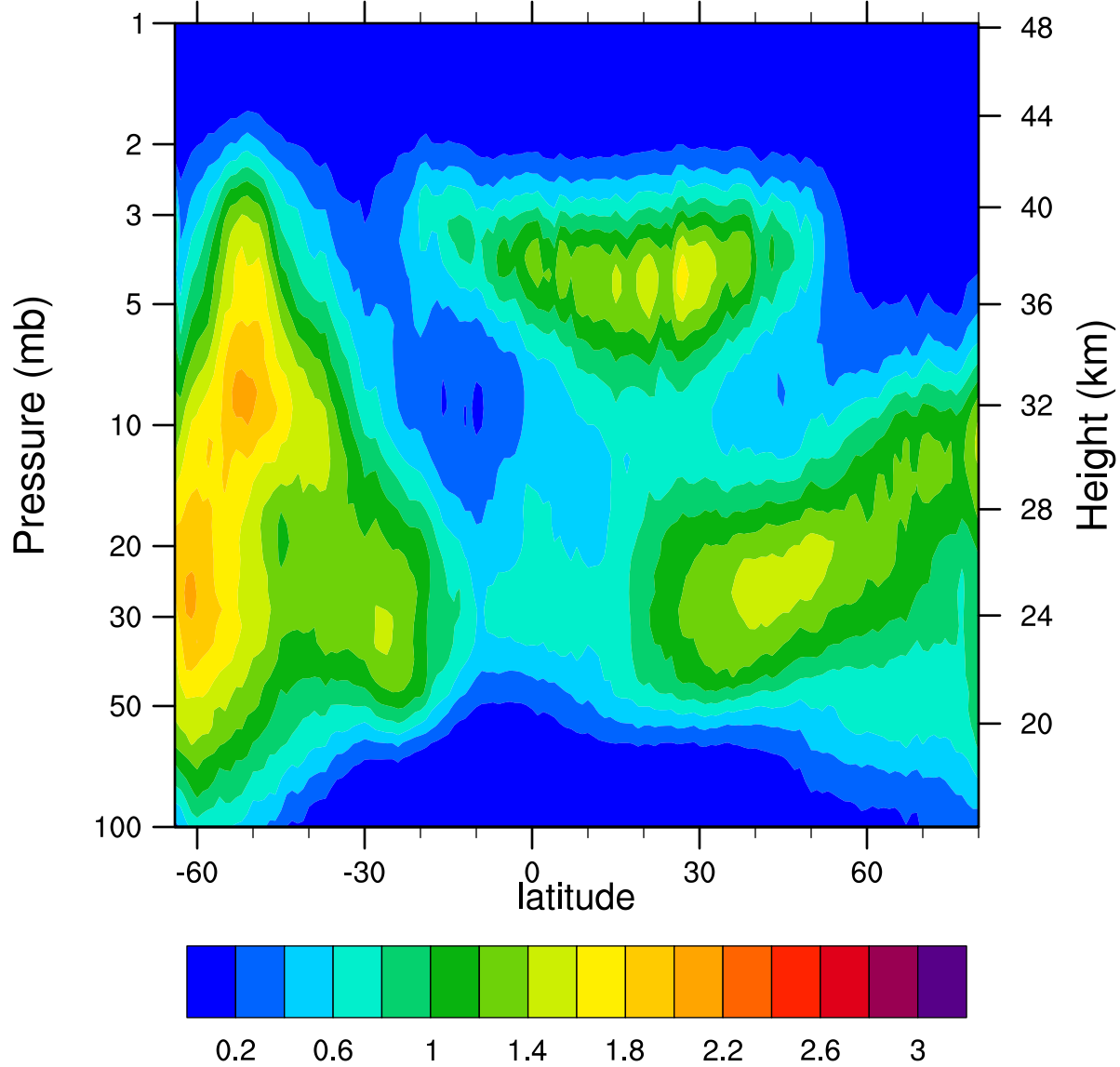
HIRDLSv6 2007d255 ClONO2_Ascending (ppbv)
