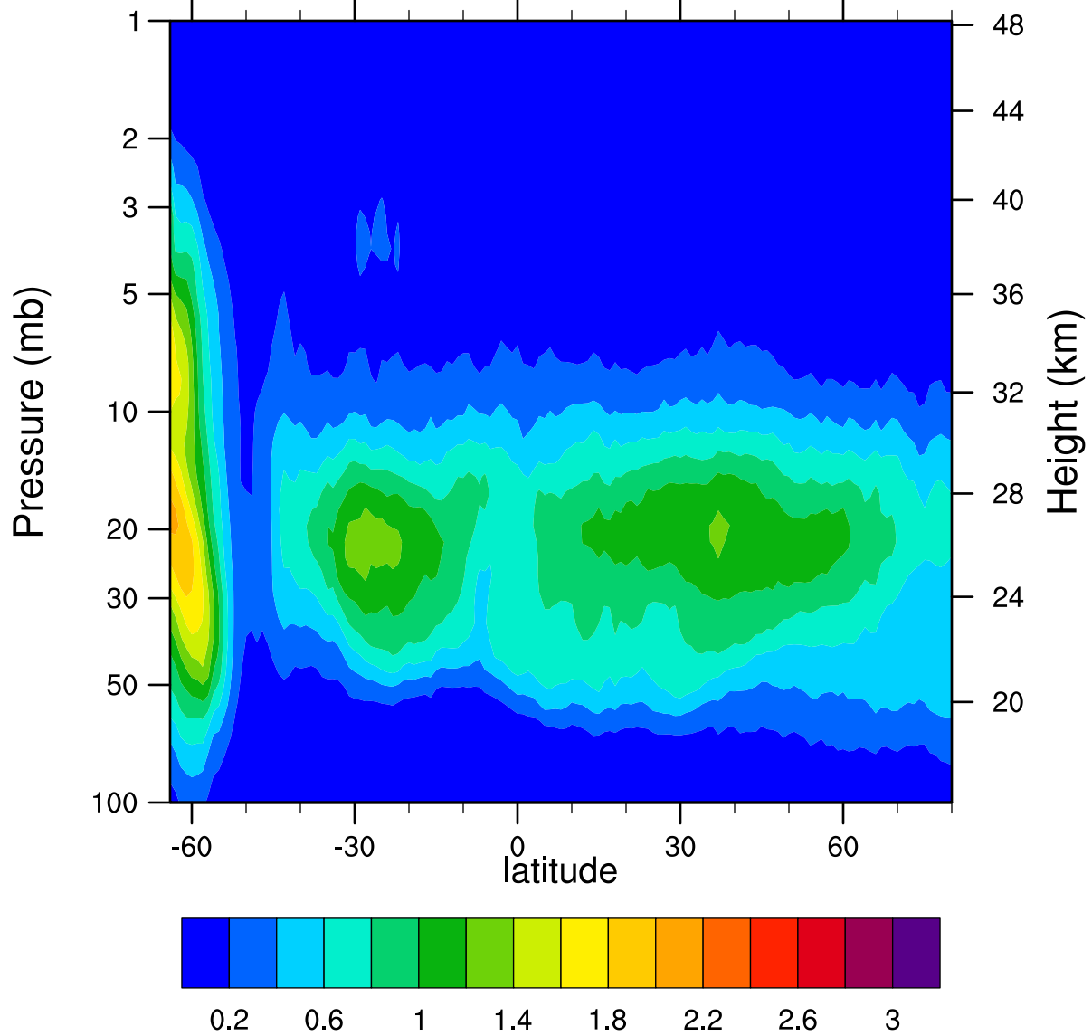
HIRDLSv6 2006d220 ClONO2_Ascending (ppbv)
