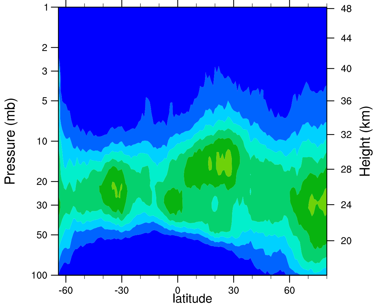
HIRDLSv6 2006d080 ClONO2_Ascending (ppbv)
