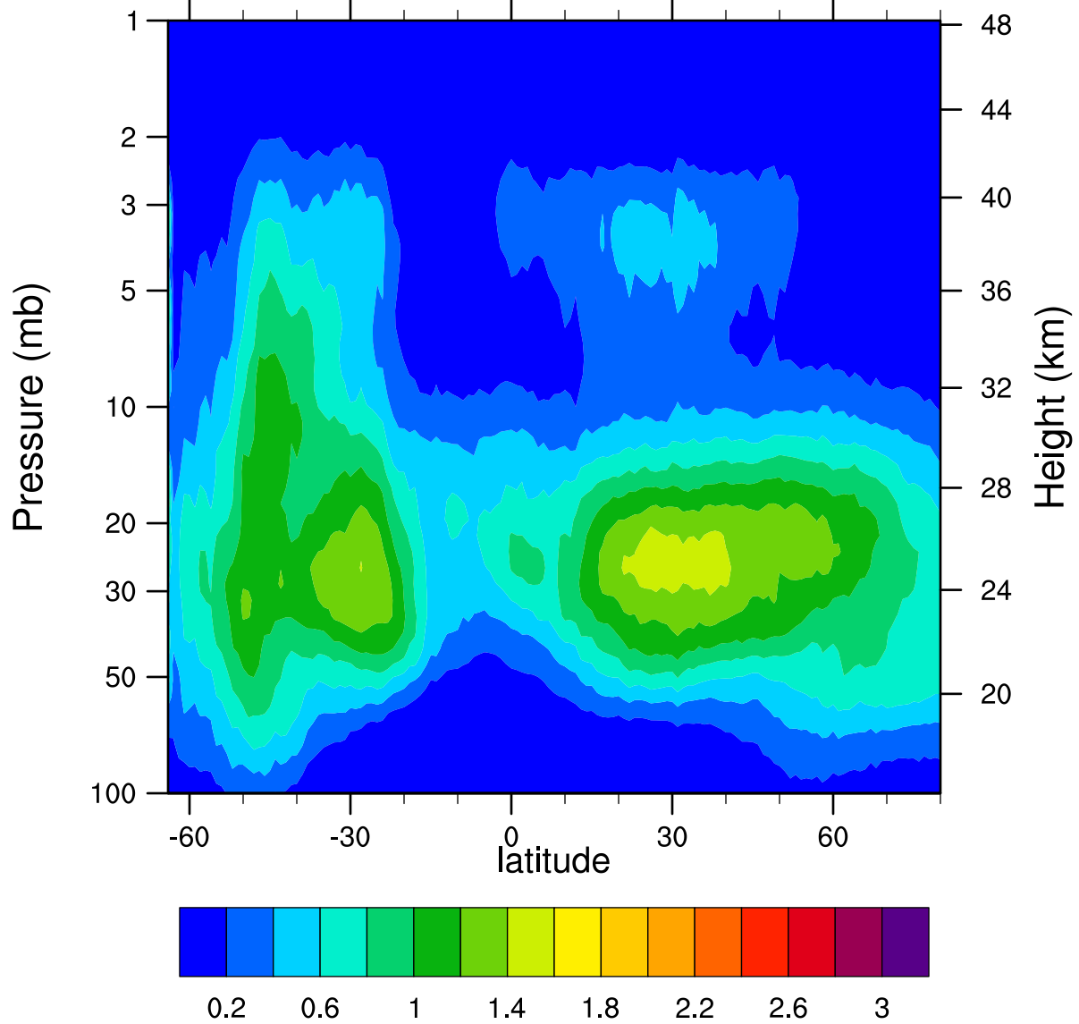
HIRDLSv6 2007d182 ClONO2_Ascending (ppbv)
