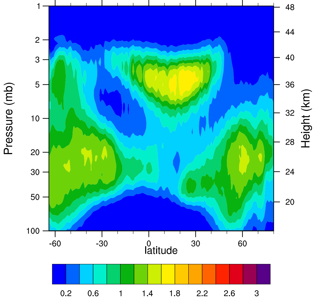
HIRDLSv6 2007d363 ClONO2_Ascending (ppbv)
