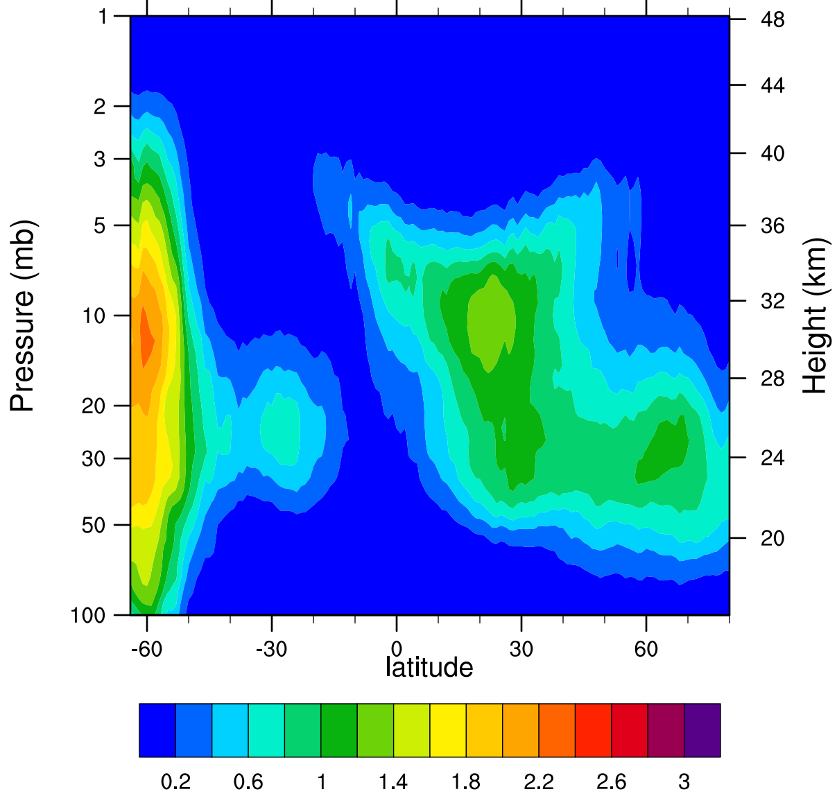
HIRDLSv6 2005d133 ClONO2_Ascending (ppbv)
