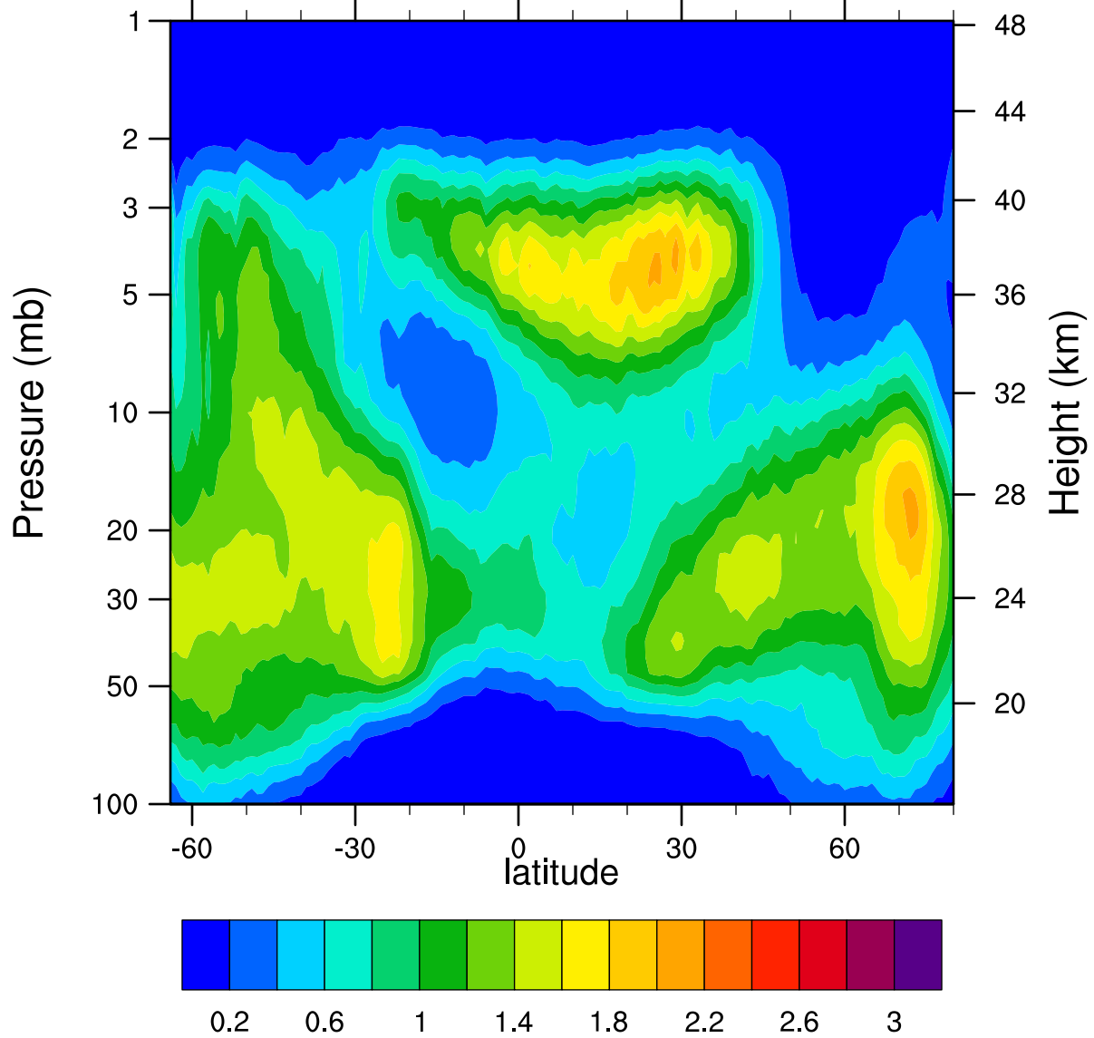
HIRDLSv6 2007d311 ClONO2_Ascending (ppbv)
