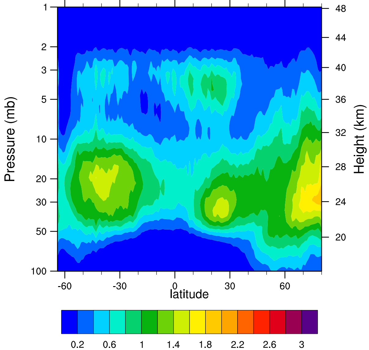
HIRDLSv6 2007d048 ClONO2_Ascending (ppbv)
