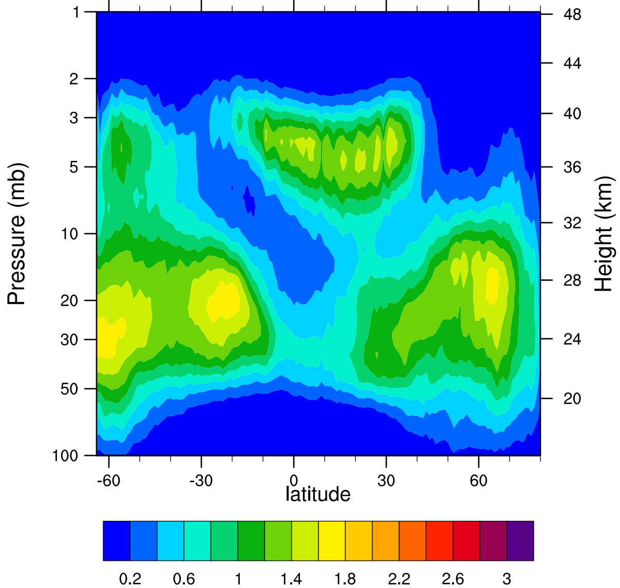
HIRDLSv6 2006d326 ClONO2_Ascending (ppbv)
