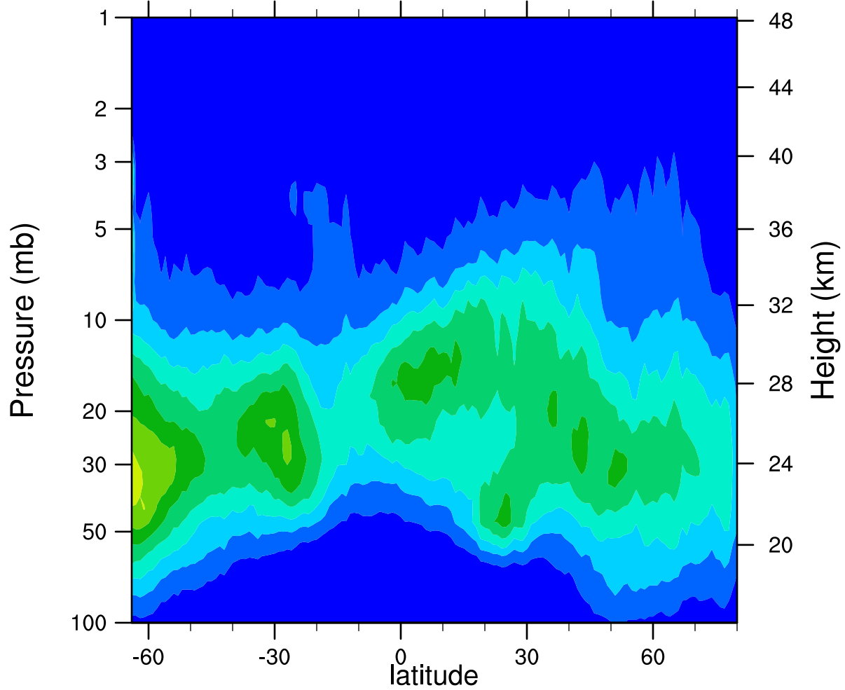
HIRDLSv6 2005d330 ClONO2_Ascending (ppbv)
