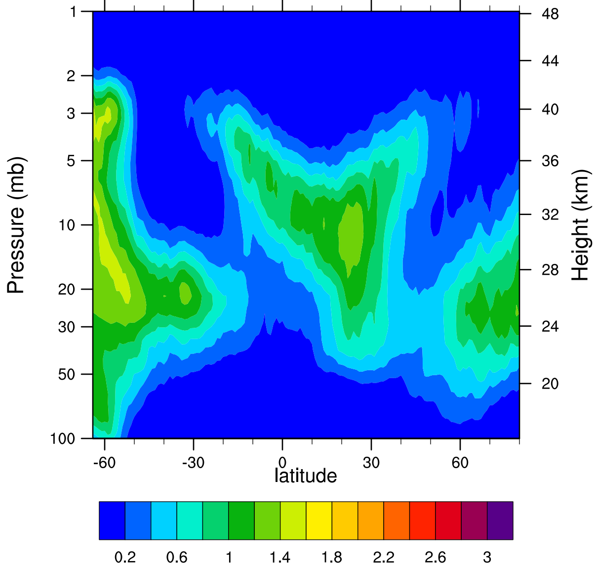
HIRDLSv6 2005d037 ClONO2_Ascending (ppbv)
