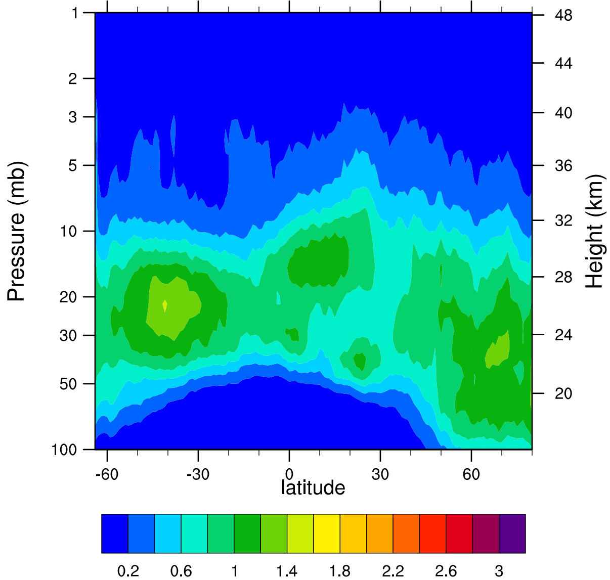
HIRDLSv6 2006d048 ClONO2_Ascending (ppbv)
