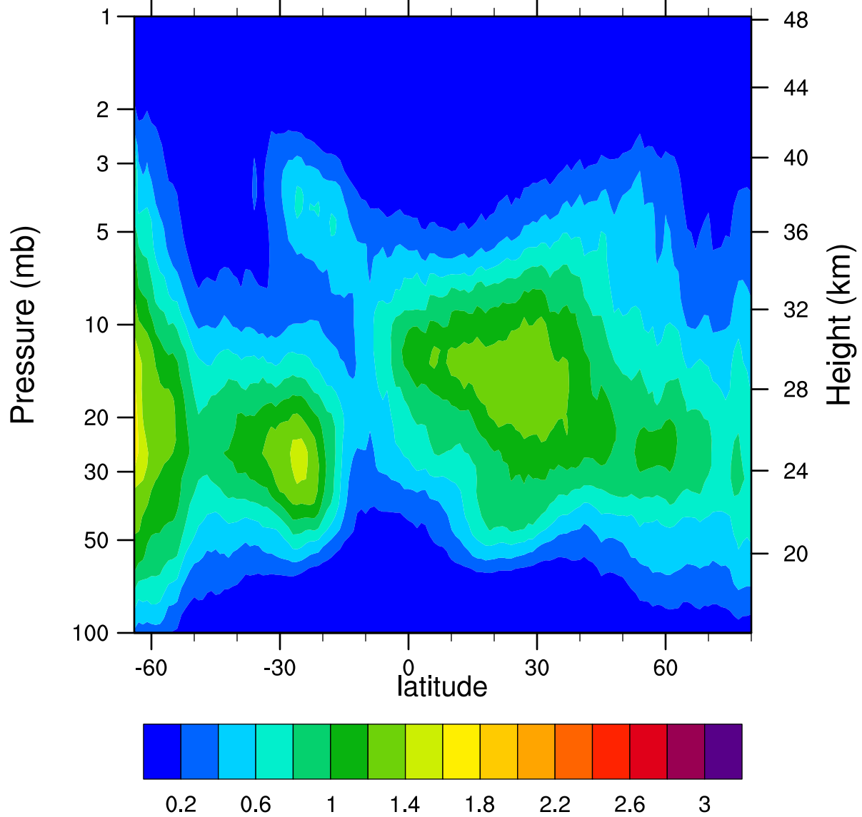
HIRDLSv6 2005d279 ClONO2_Ascending (ppbv)
