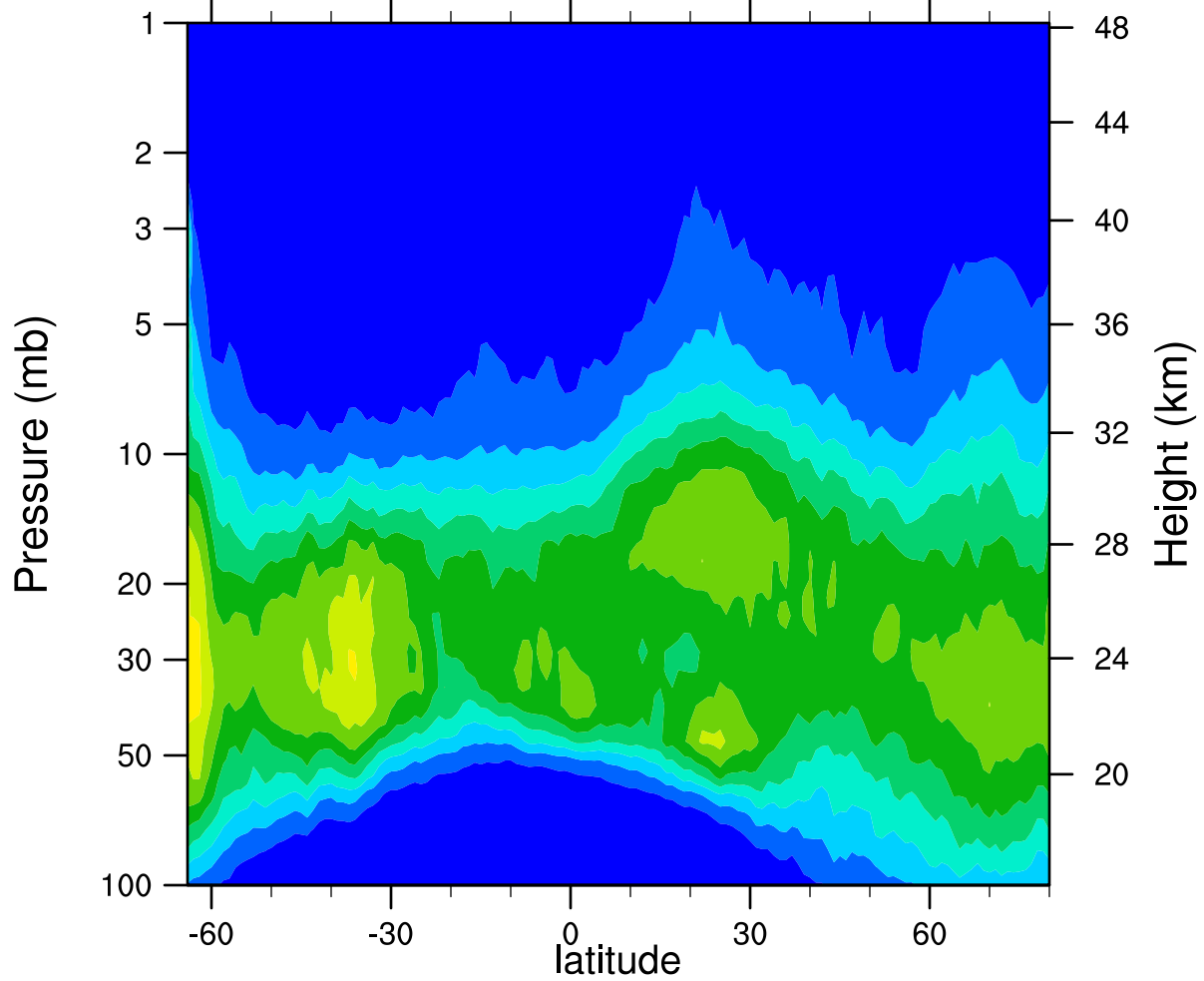
HIRDLSv6 2006d091 ClONO2_Ascending (ppbv)
