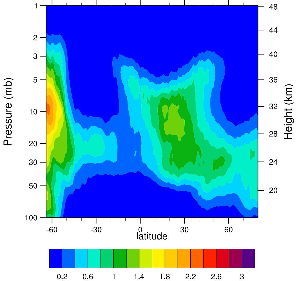
HIRDLSv6 2005d109 ClONO2_Ascending (ppbv)
