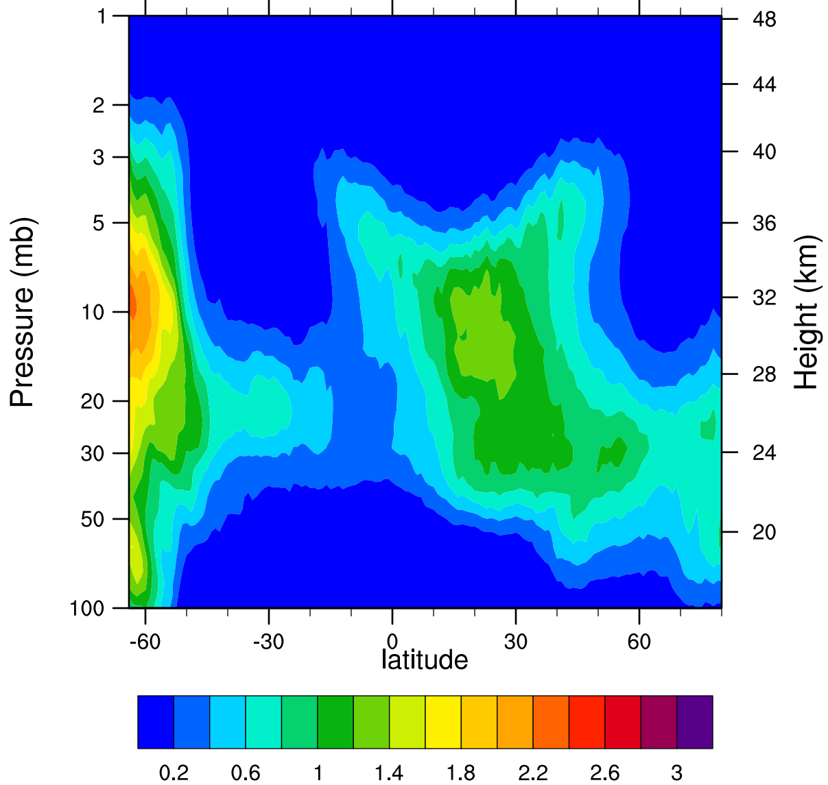
HIRDLSv6 2005d111 ClONO2_Ascending (ppbv)
