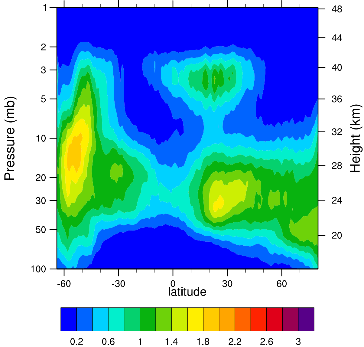
HIRDLSv6 2007d119 ClONO2_Ascending (ppbv)
