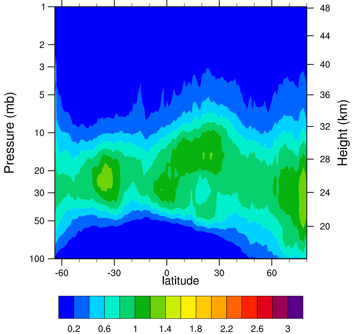
HIRDLSv6 2006d075 ClONO2_Ascending (ppbv)
