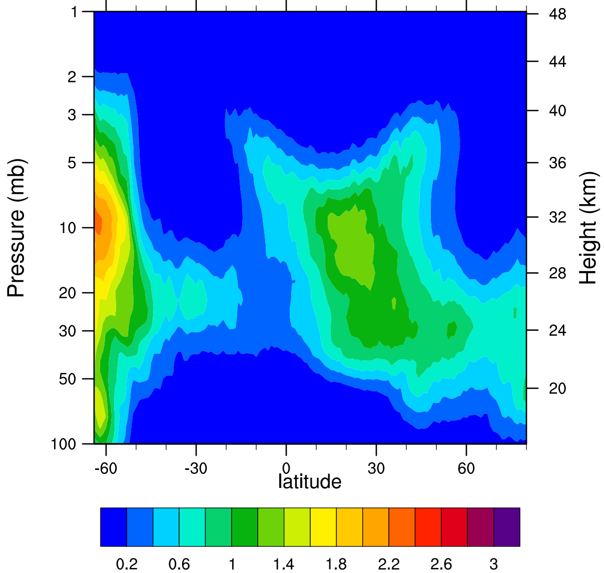
HIRDLSv6 2005d1113 ClONO2_Ascending (ppbv)
