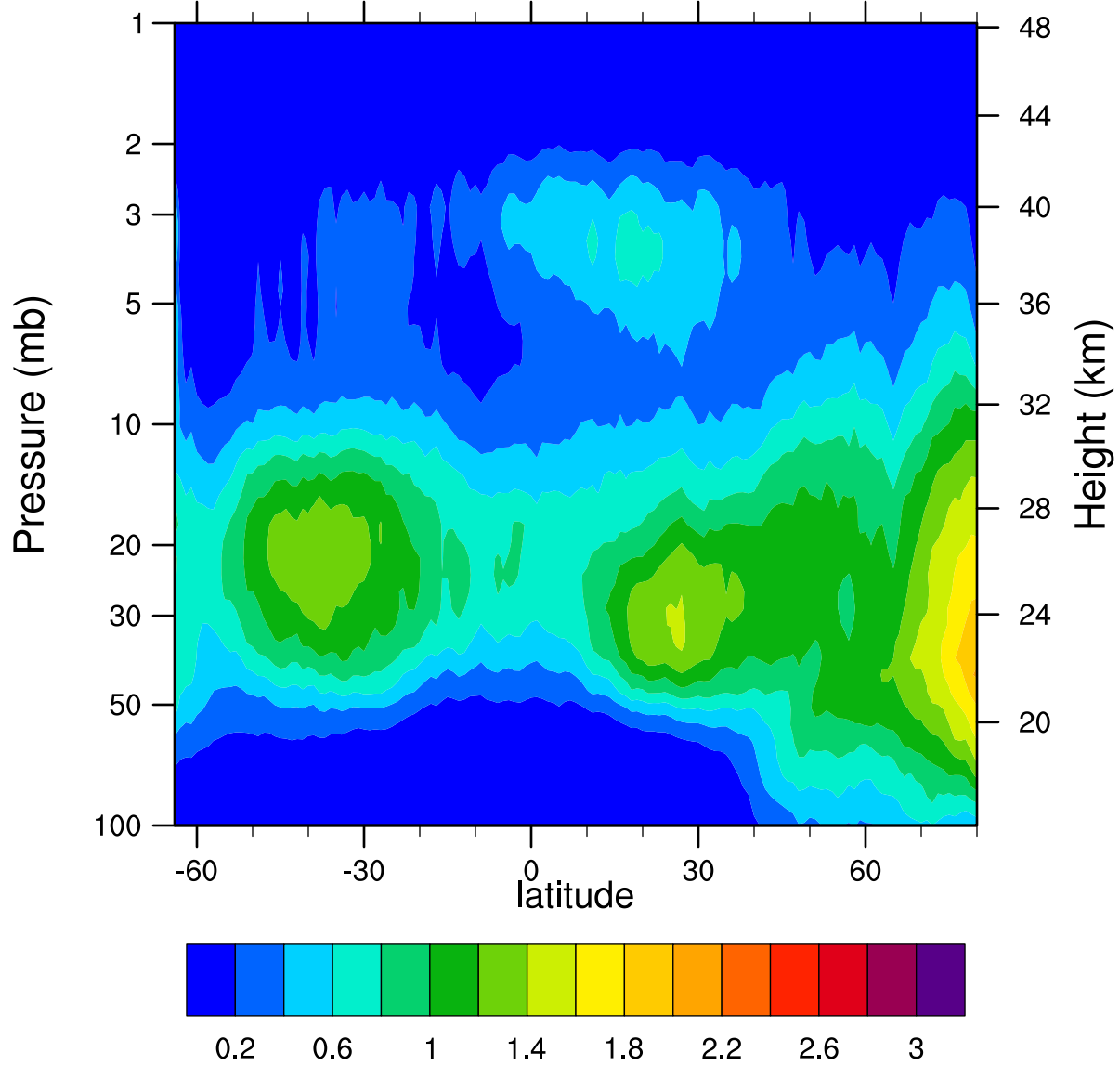
HIRDLSv6 2007d061 ClONO2_Ascending (ppbv)
