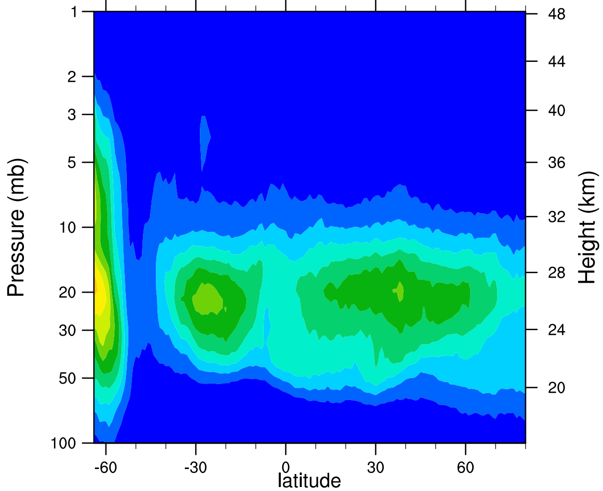
HIRDLSv6 2006d214 ClONO2_Ascending (ppbv)
