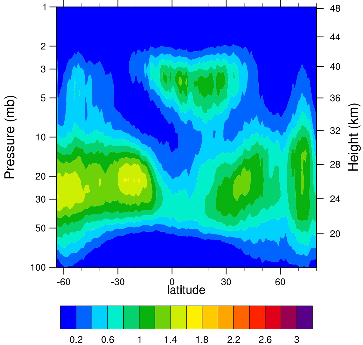
HIRDLSv6 2006d312 ClONO2_Ascending (ppbv)
