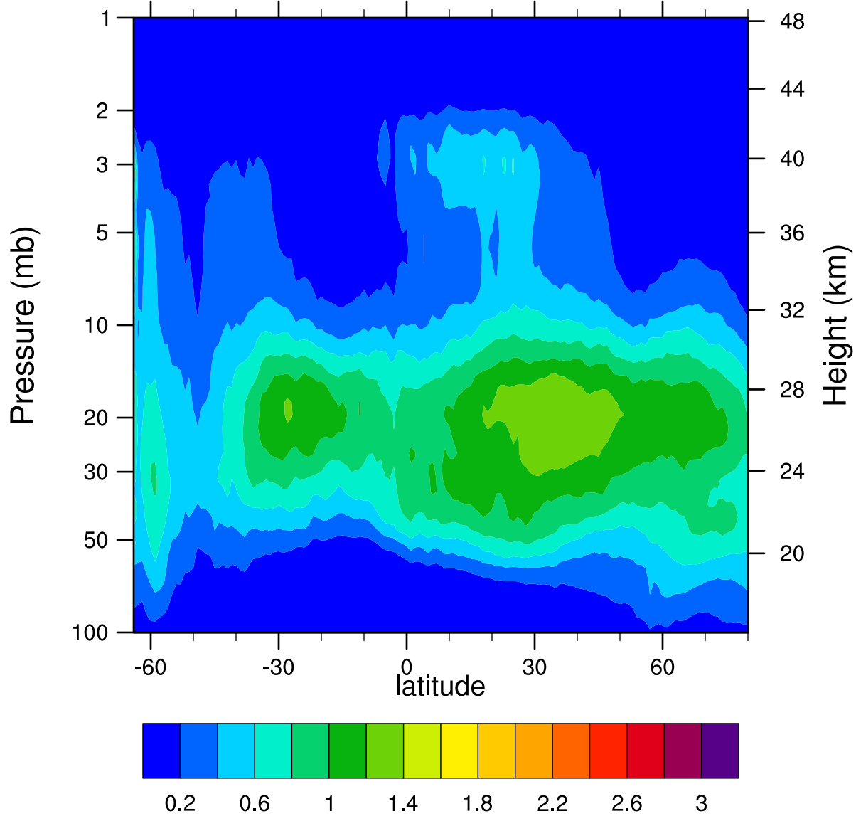
HIRDLSv6 2006d165 ClONO2_Ascending (ppbv)
