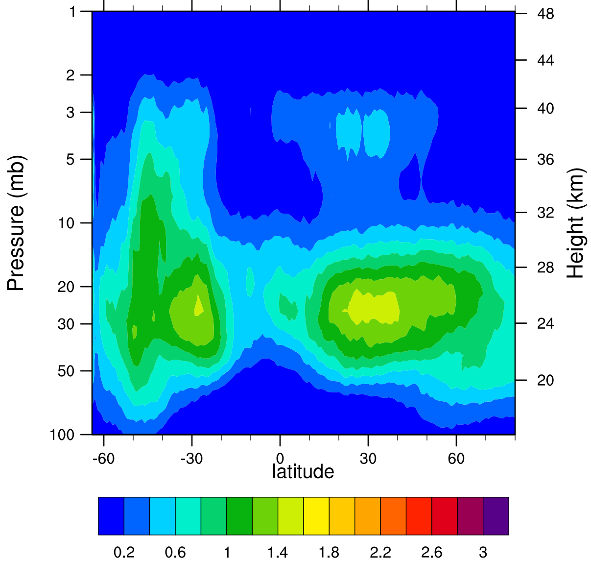
HIRDLSv6 2007d181 ClONO2_Ascending (ppbv)
