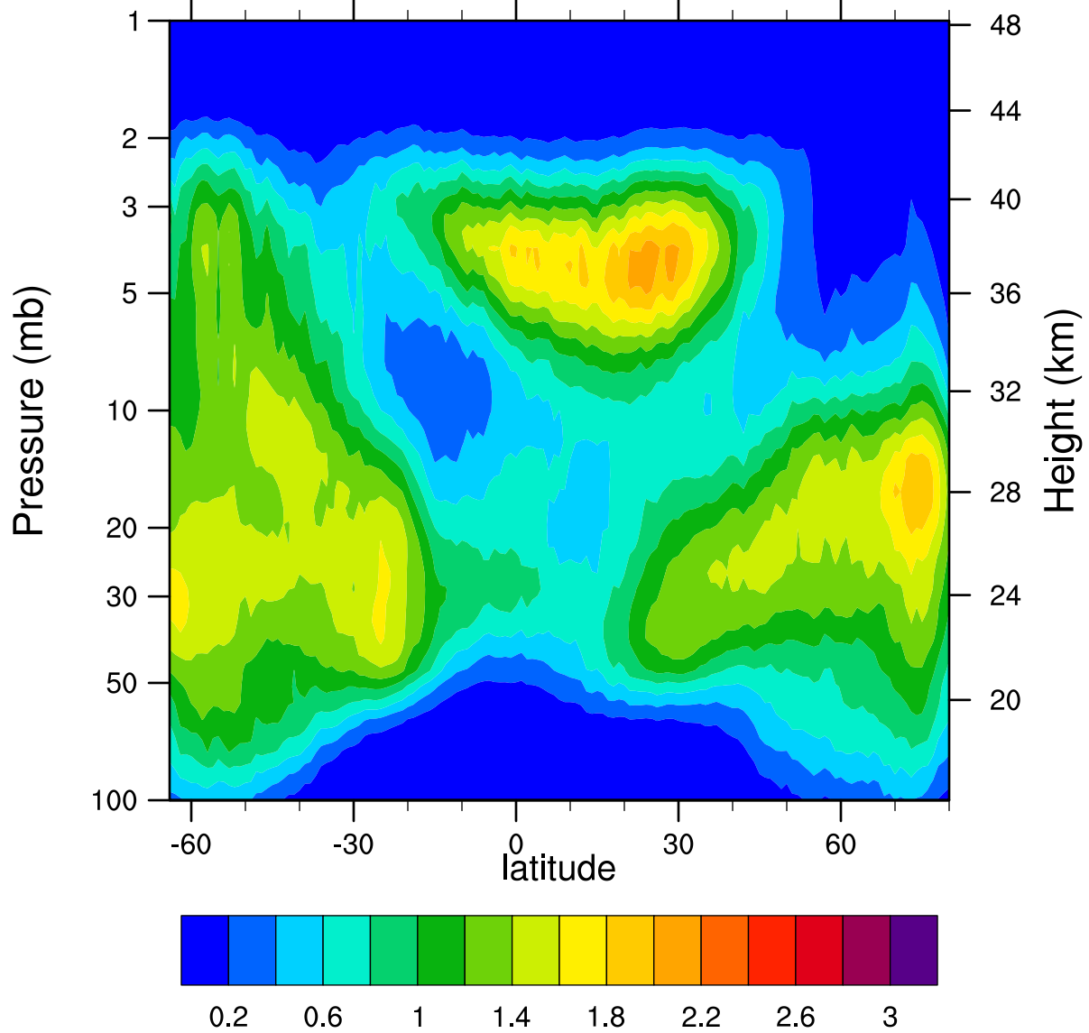
HIRDLSv6 2007d297 ClONO2_Ascending (ppbv)
