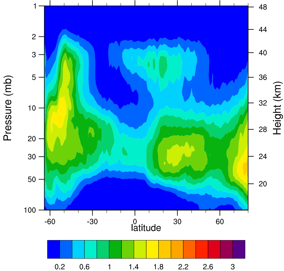
HIRDLSv6 2007d101 ClONO2_Ascending (ppbv)
