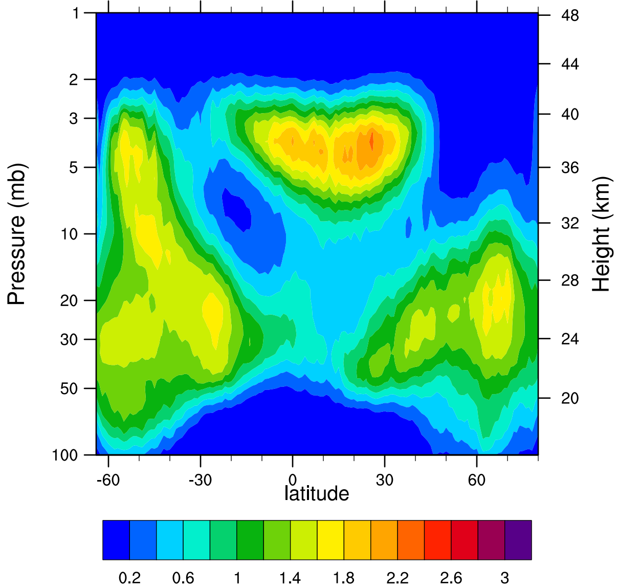
HIRDLSv6 2007d320 ClONO2_Ascending (ppbv)
