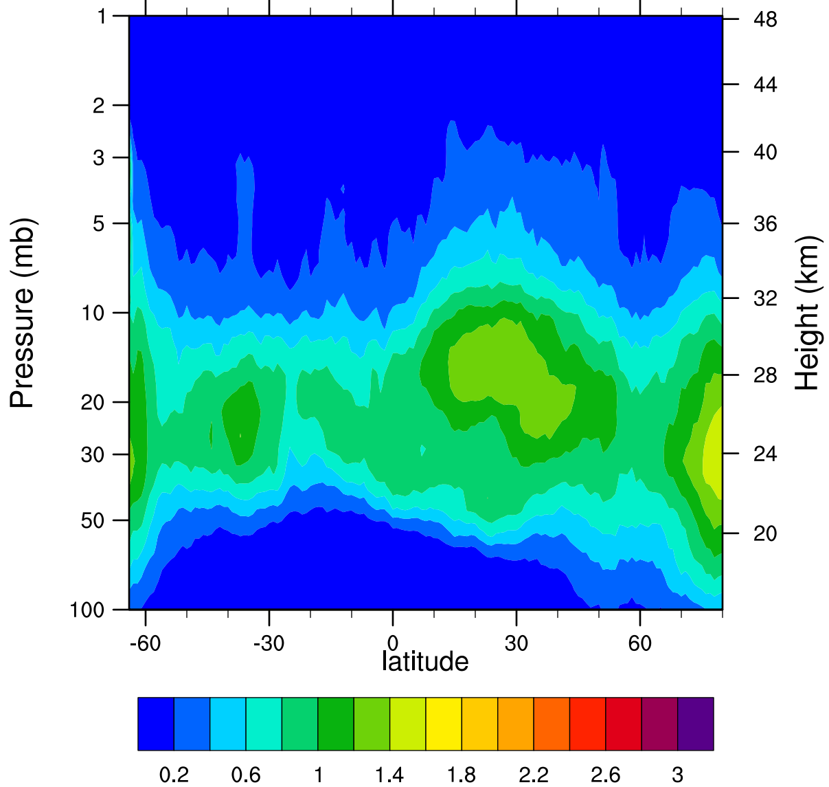
HIRDLSv6 2006d104 ClONO2_Ascending (ppbv)
