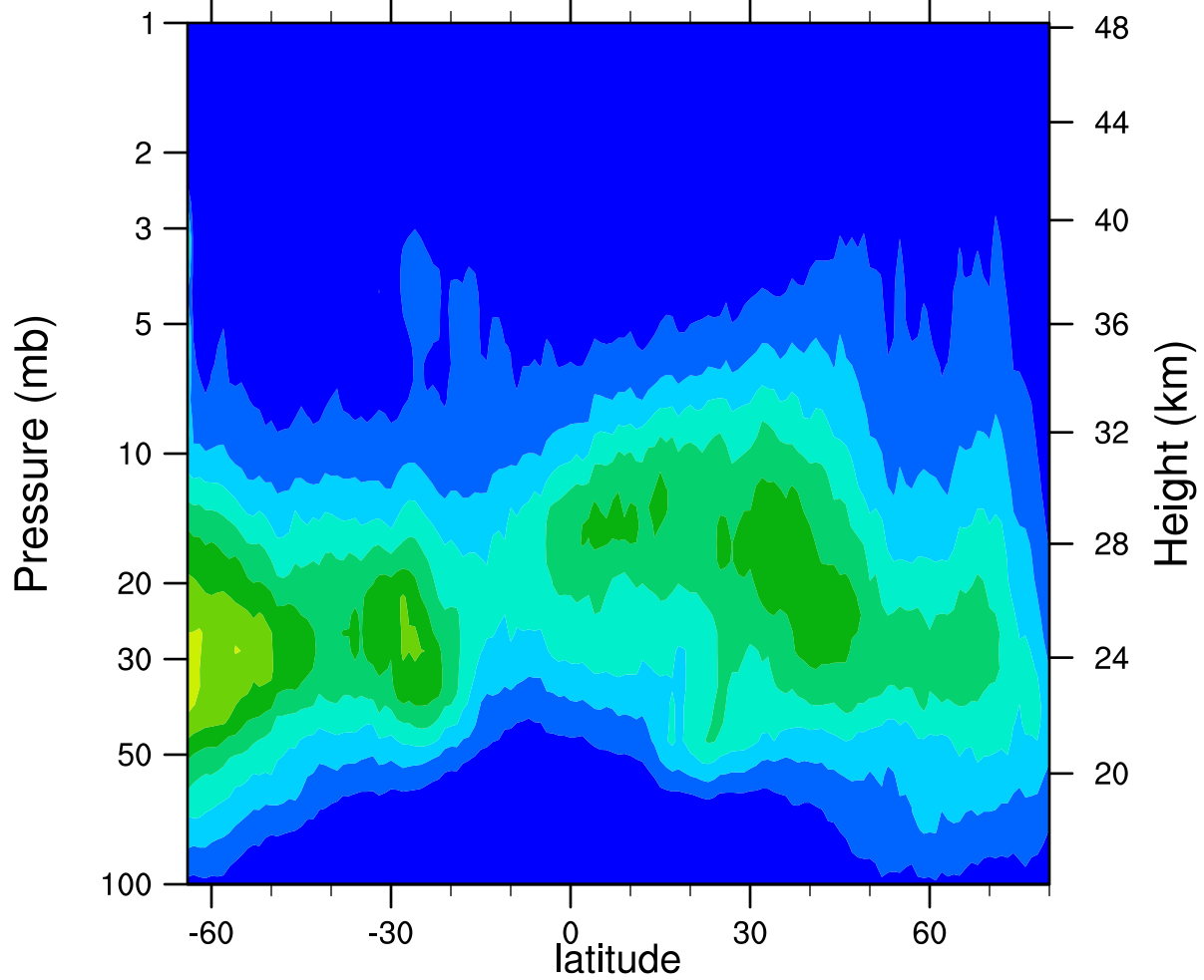
HIRDLSv6 2005d318 ClONO2_Ascending (ppbv)
