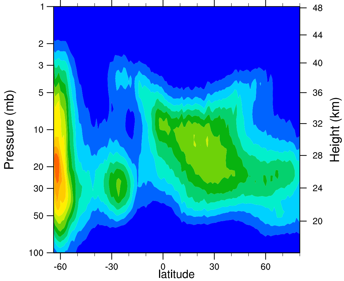
HIRDLSv6 2005d205 ClONO2_Ascending (ppbv)
