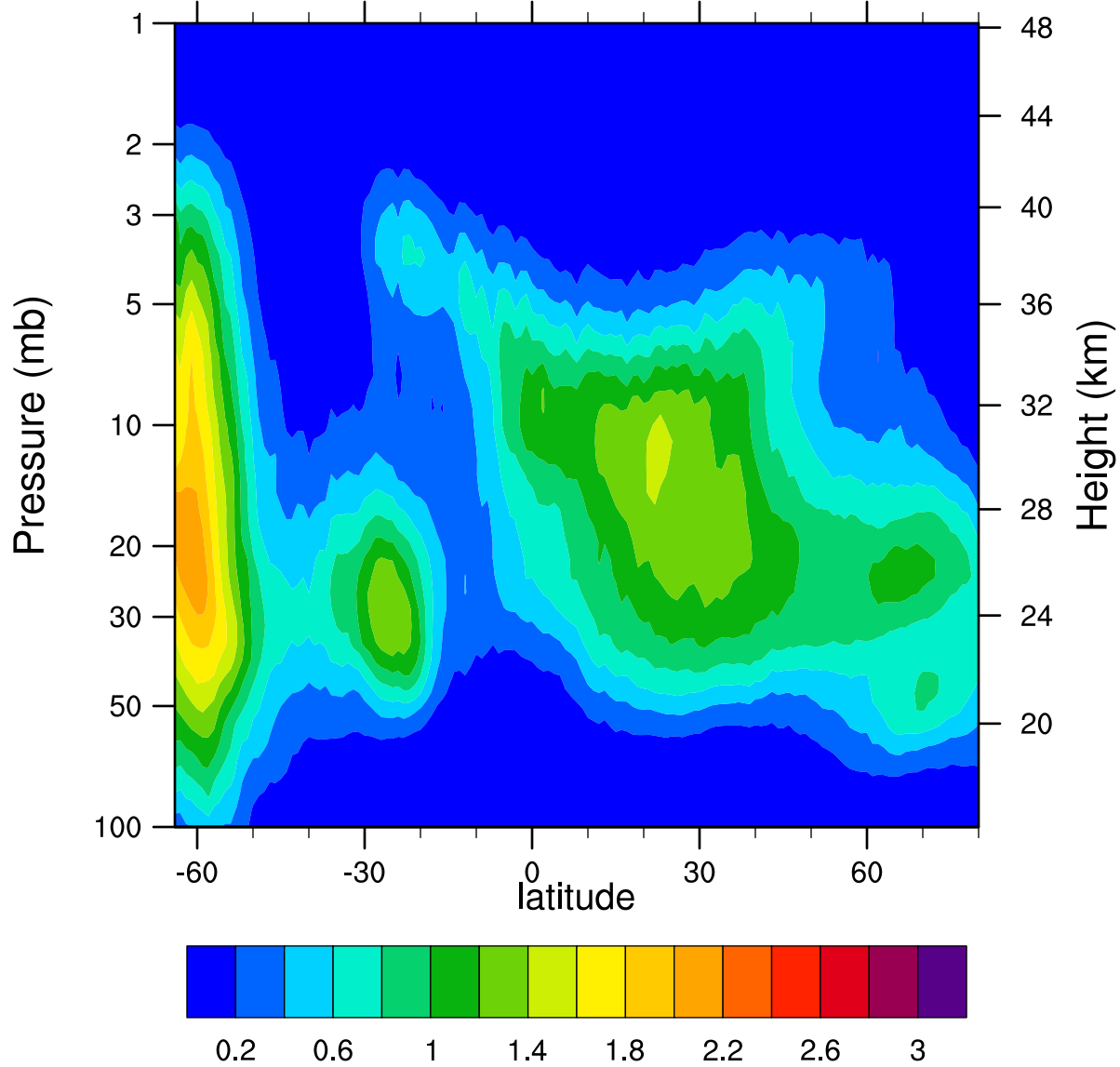
HIRDLSv6 2005d191 ClONO2_Ascending (ppbv)
