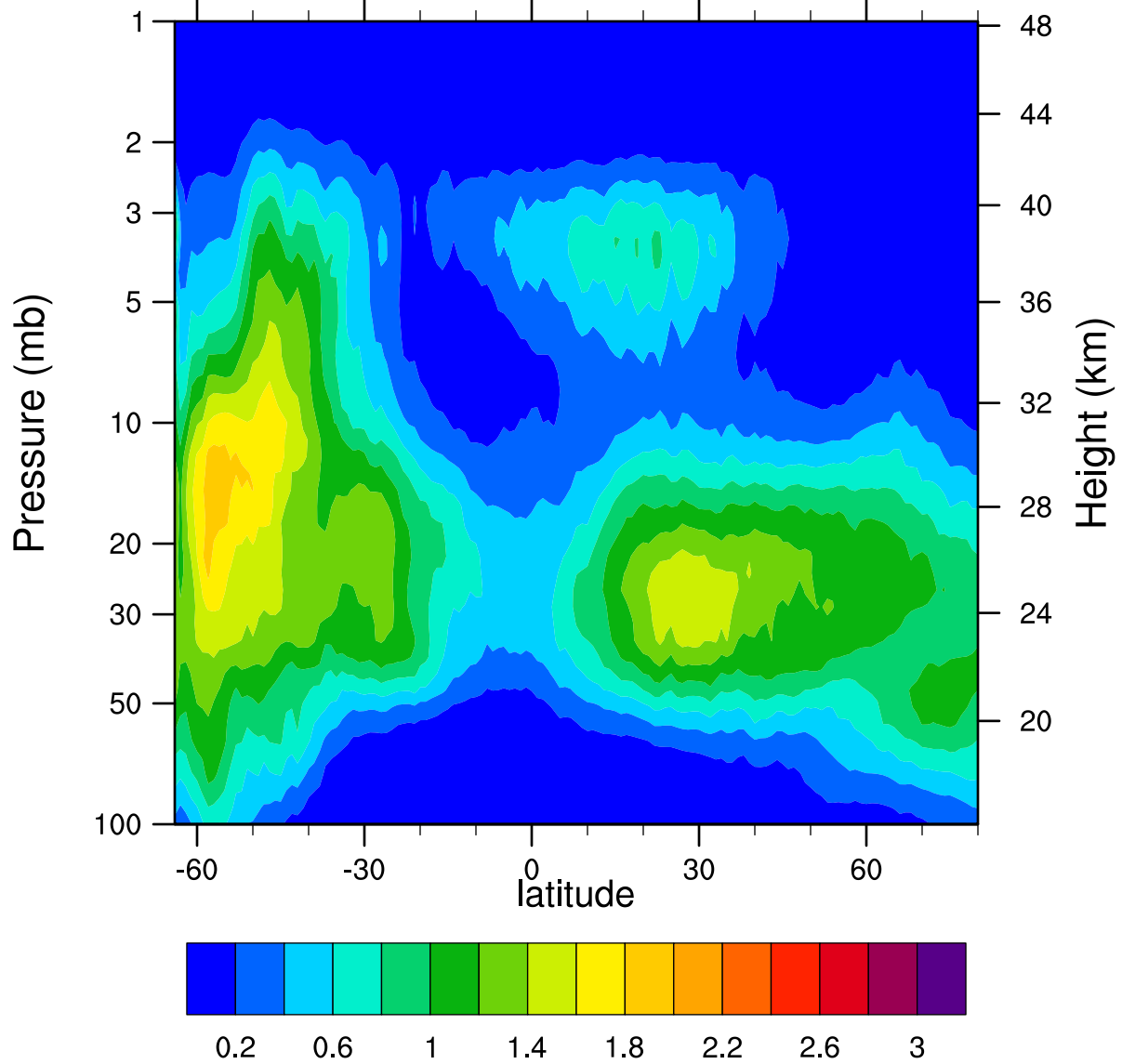
HIRDLSv6 2007d139 ClONO2_Ascending (ppbv)
