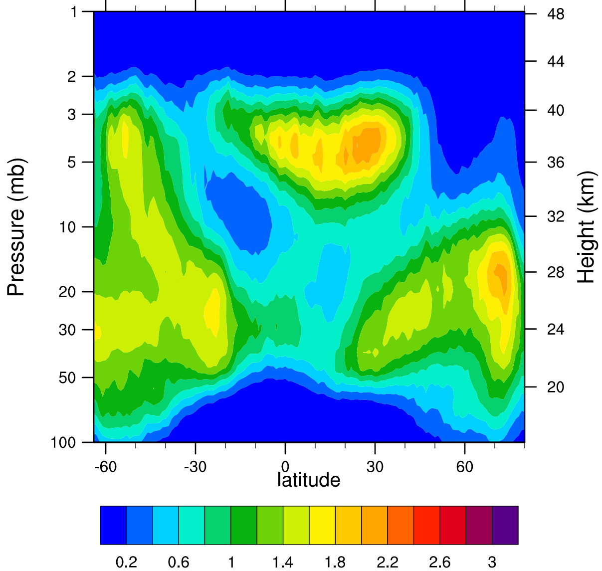
HIRDLSv6 2007d307 ClONO2_Ascending (ppbv)
