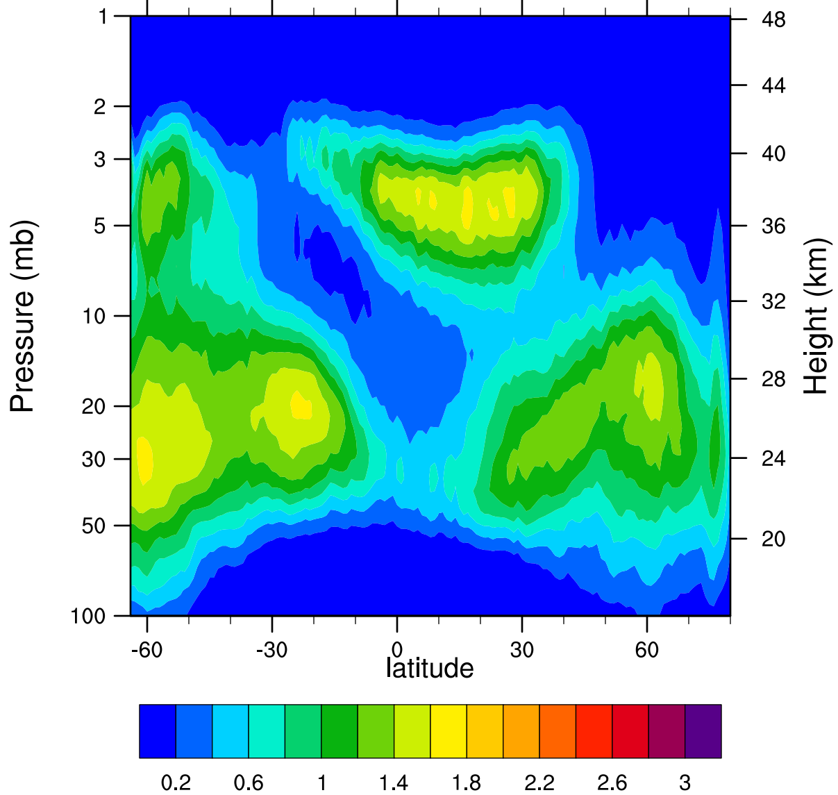
HIRDLSv6 2006d337 ClONO2_Ascending (ppbv)
