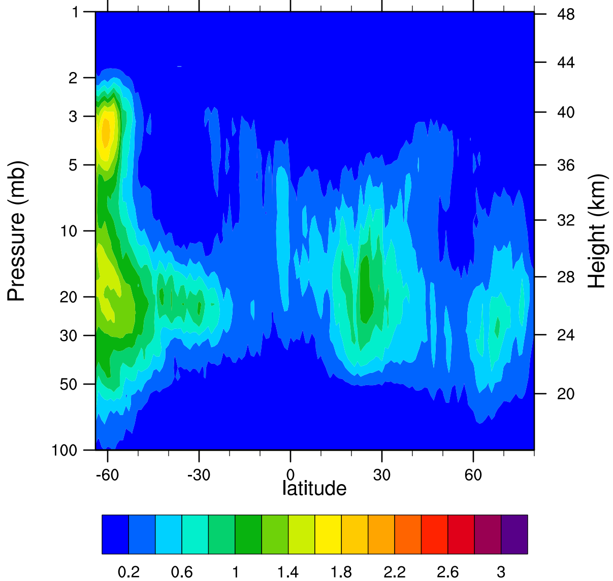
HIRDLSv6 2005d027 ClONO2_Ascending (ppbv)
