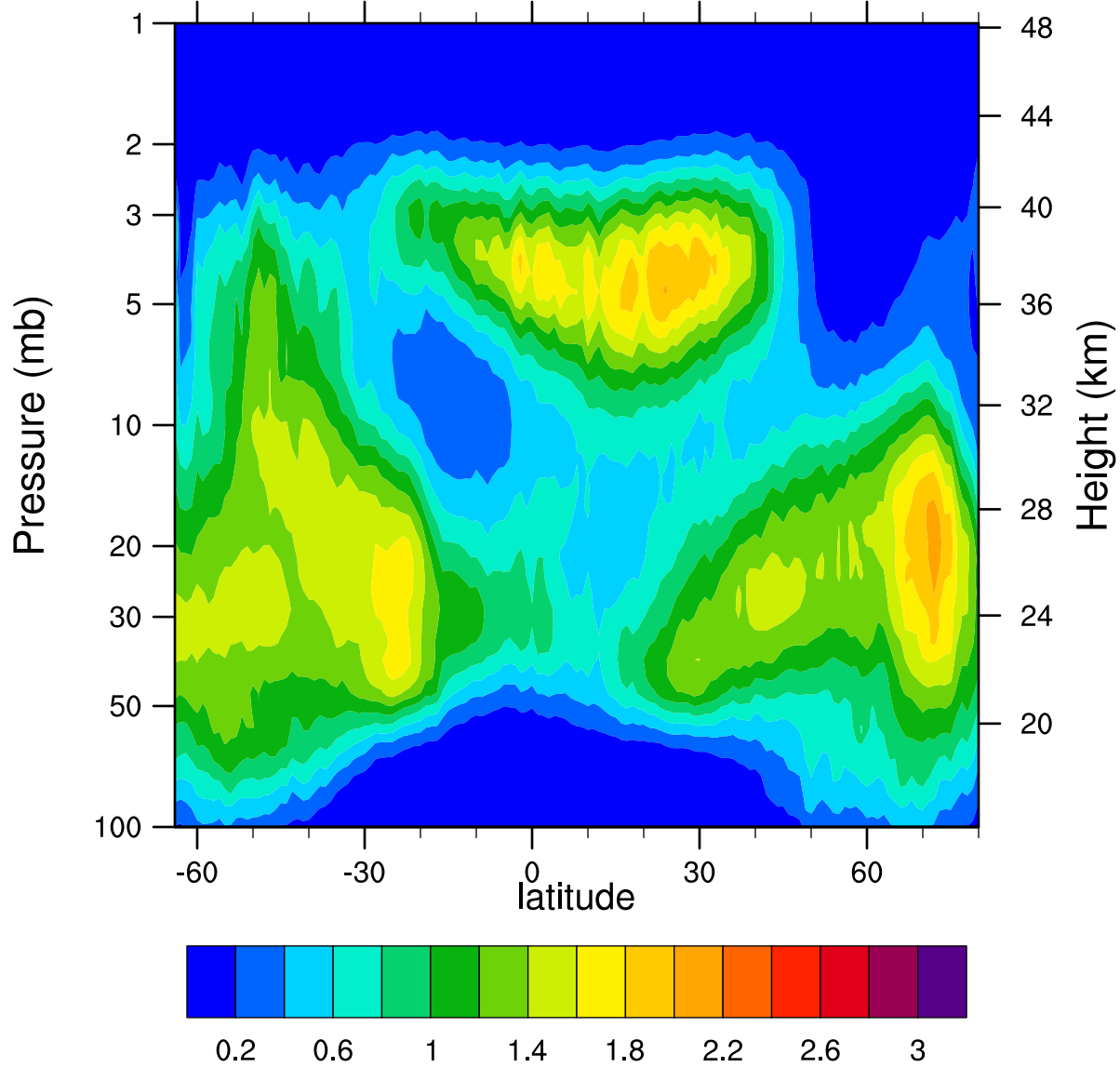
HIRDLSv6 2007d313 ClONO2_Ascending (ppbv)
