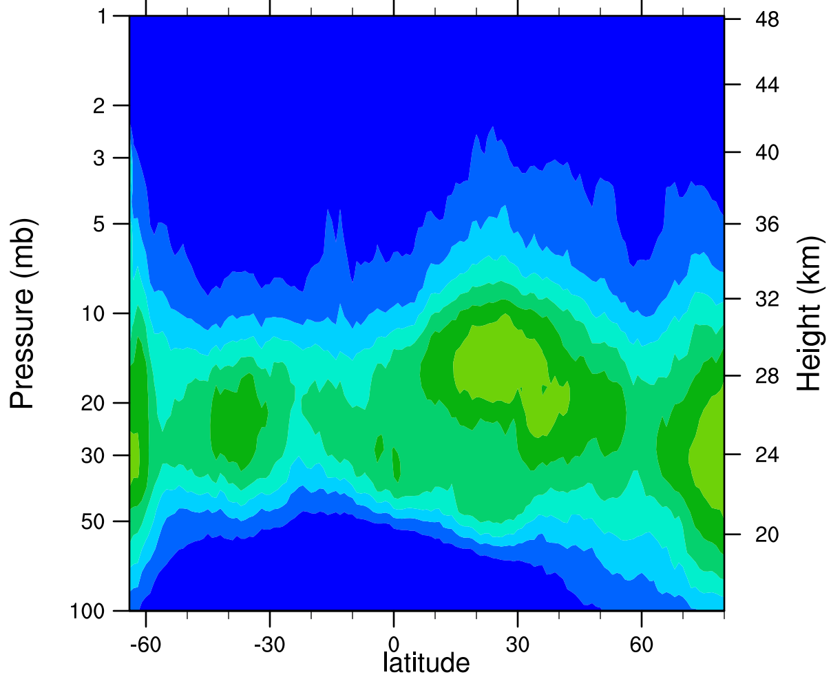
HIRDLSv6 2006d098 ClONO2_Ascending (ppbv)
