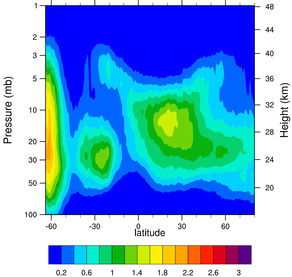
HIRDLSv6 2005d233 ClONO2_Ascending (ppbv)
