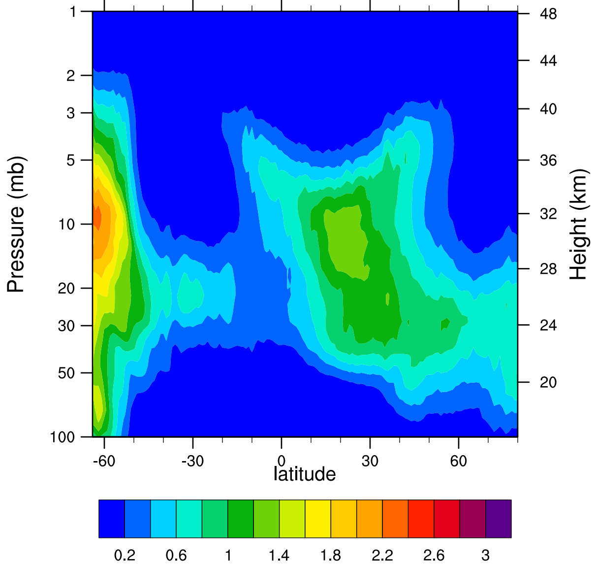
HIRDLSv6 2005d114 ClONO2_Ascending (ppbv)
