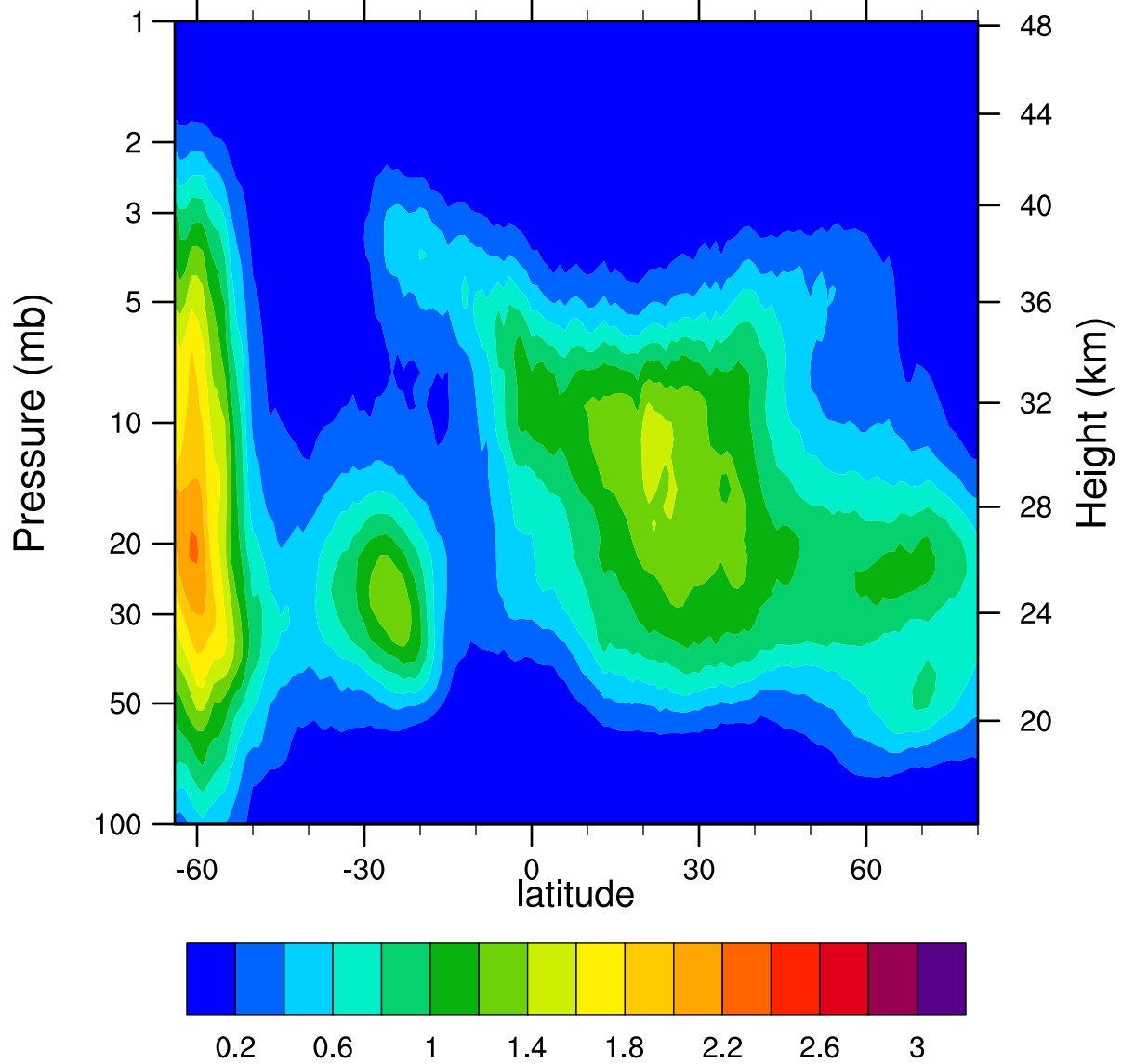
HIRDLSv6 2005d186 ClONO2_Ascending (ppbv)
