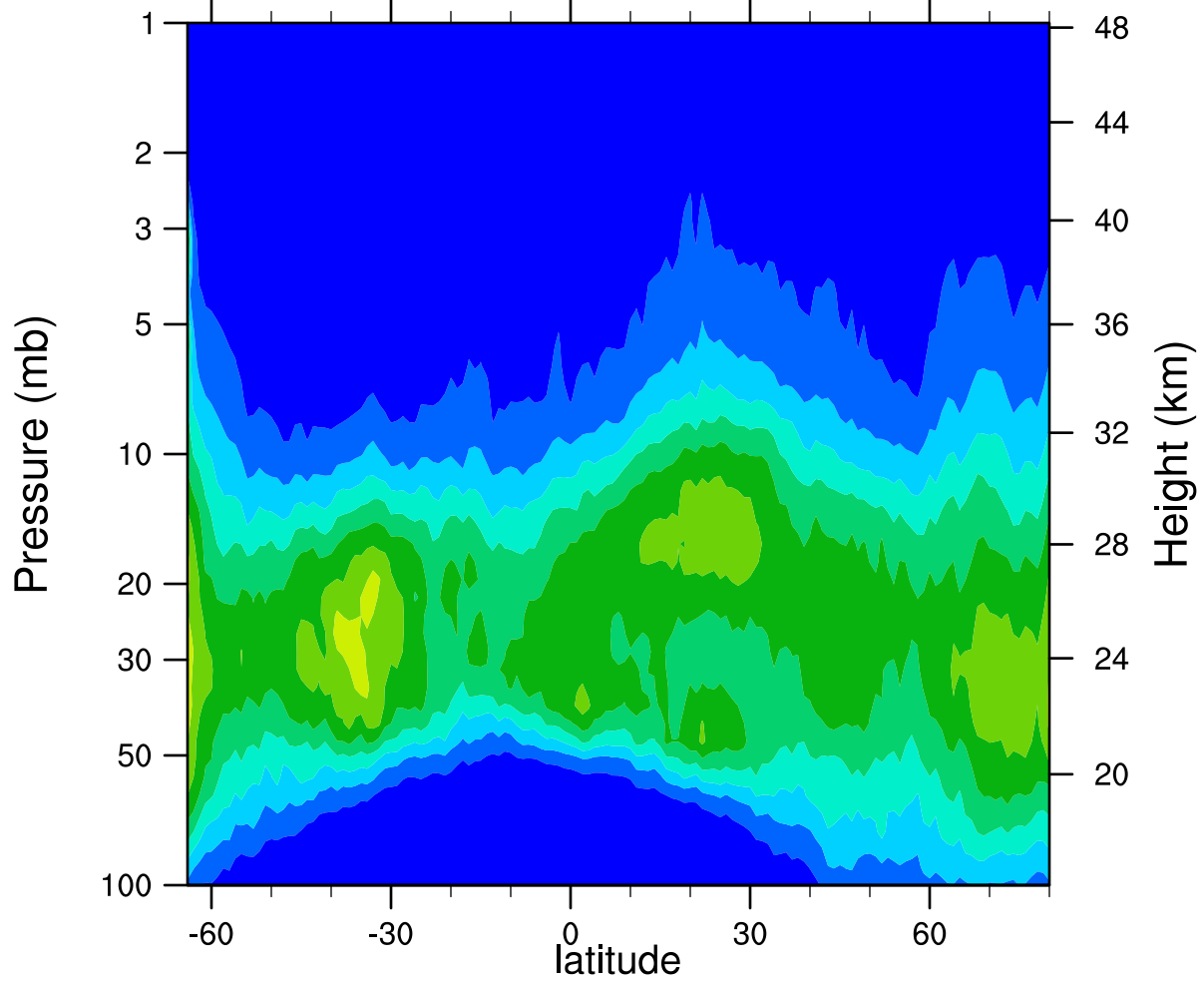
HIRDLSv6 2006d086 ClONO2_Ascending (ppbv)
