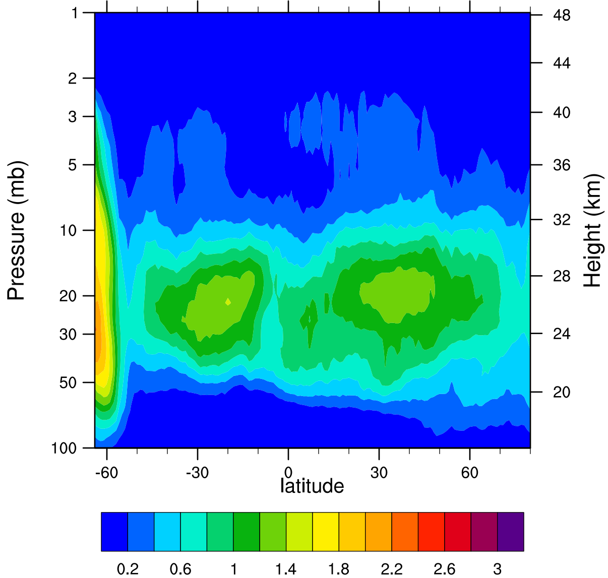
HIRDLSv6 2006d259 ClONO2_Ascending (ppbv)
