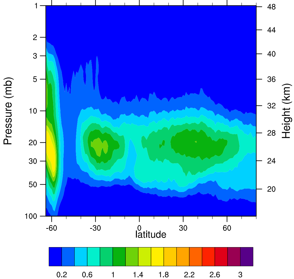
HIRDLSv6 2006d199 ClONO2_Ascending (ppbv)
