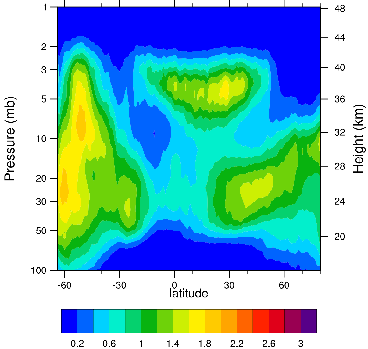
HIRDLSv6 2007d258 ClONO2_Ascending (ppbv)
