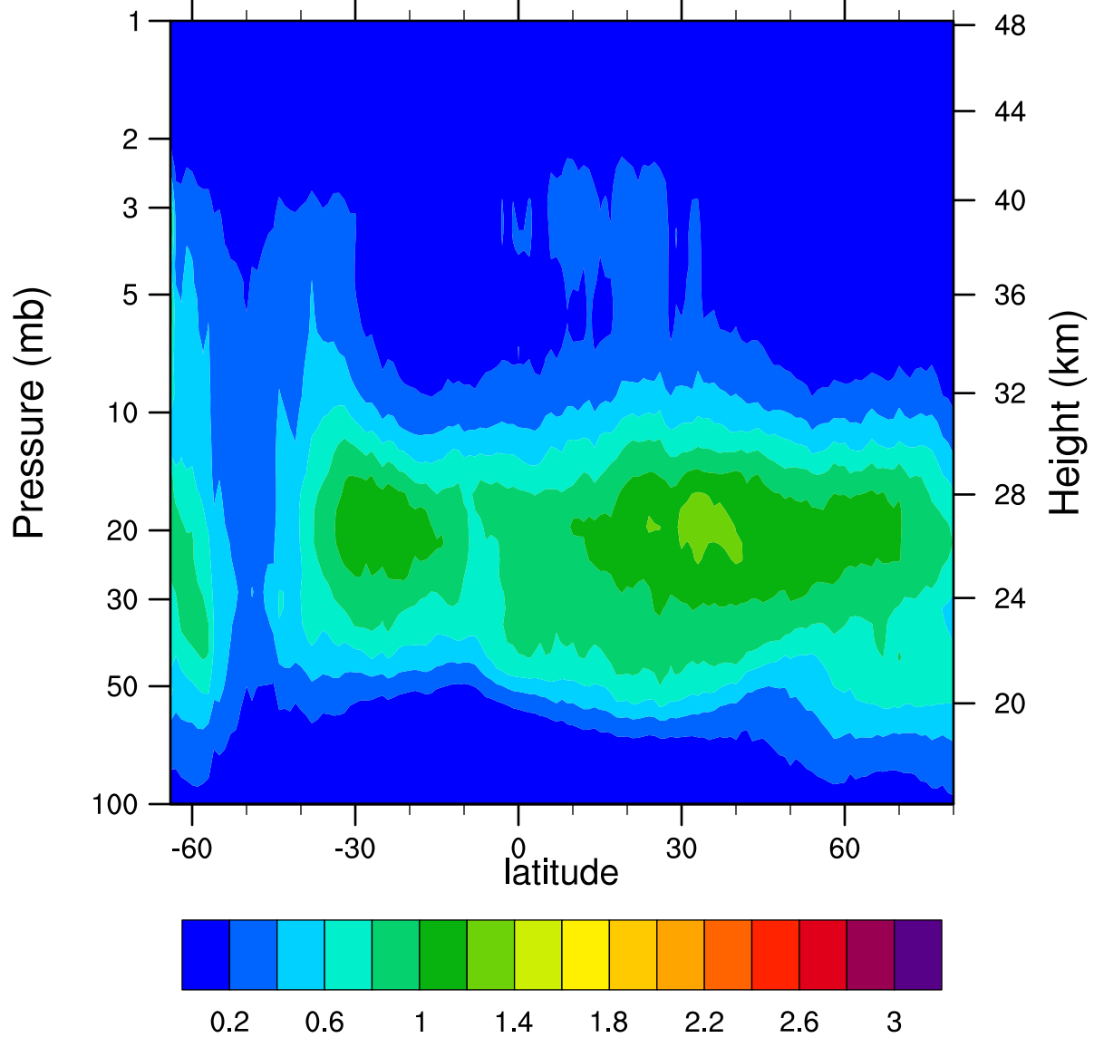
HIRDLSv6 2006d176 ClONO2_Ascending (ppbv)
