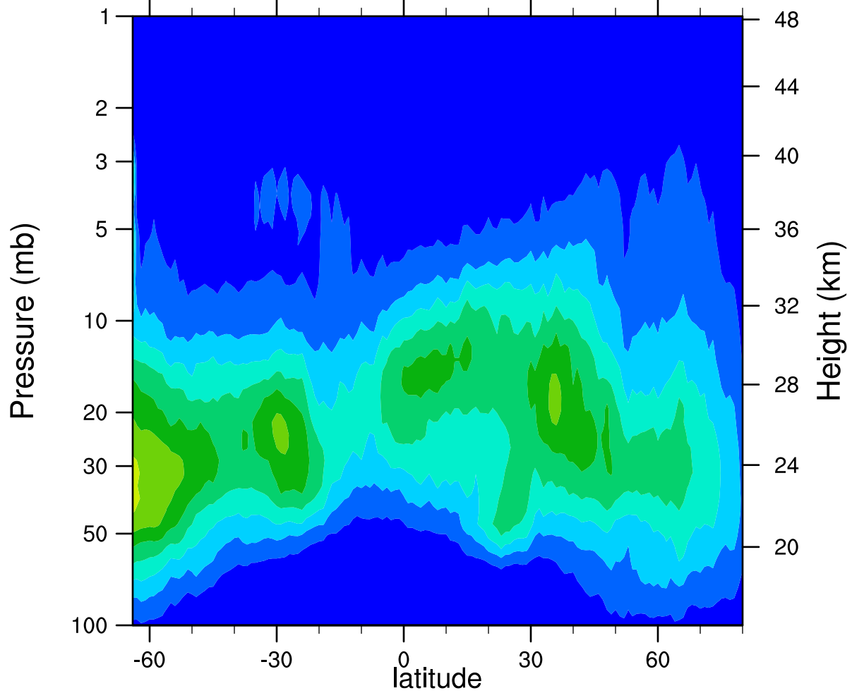
HIRDLSv6 2005d325 ClONO2_Ascending (ppbv)
