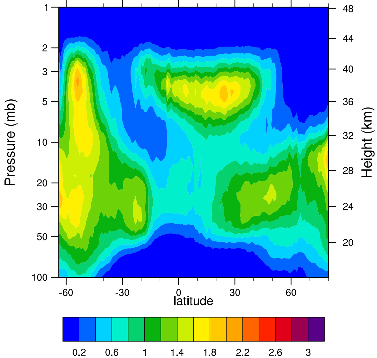
HIRDLSv6 2007d277 ClONO2_Ascending (ppbv)
