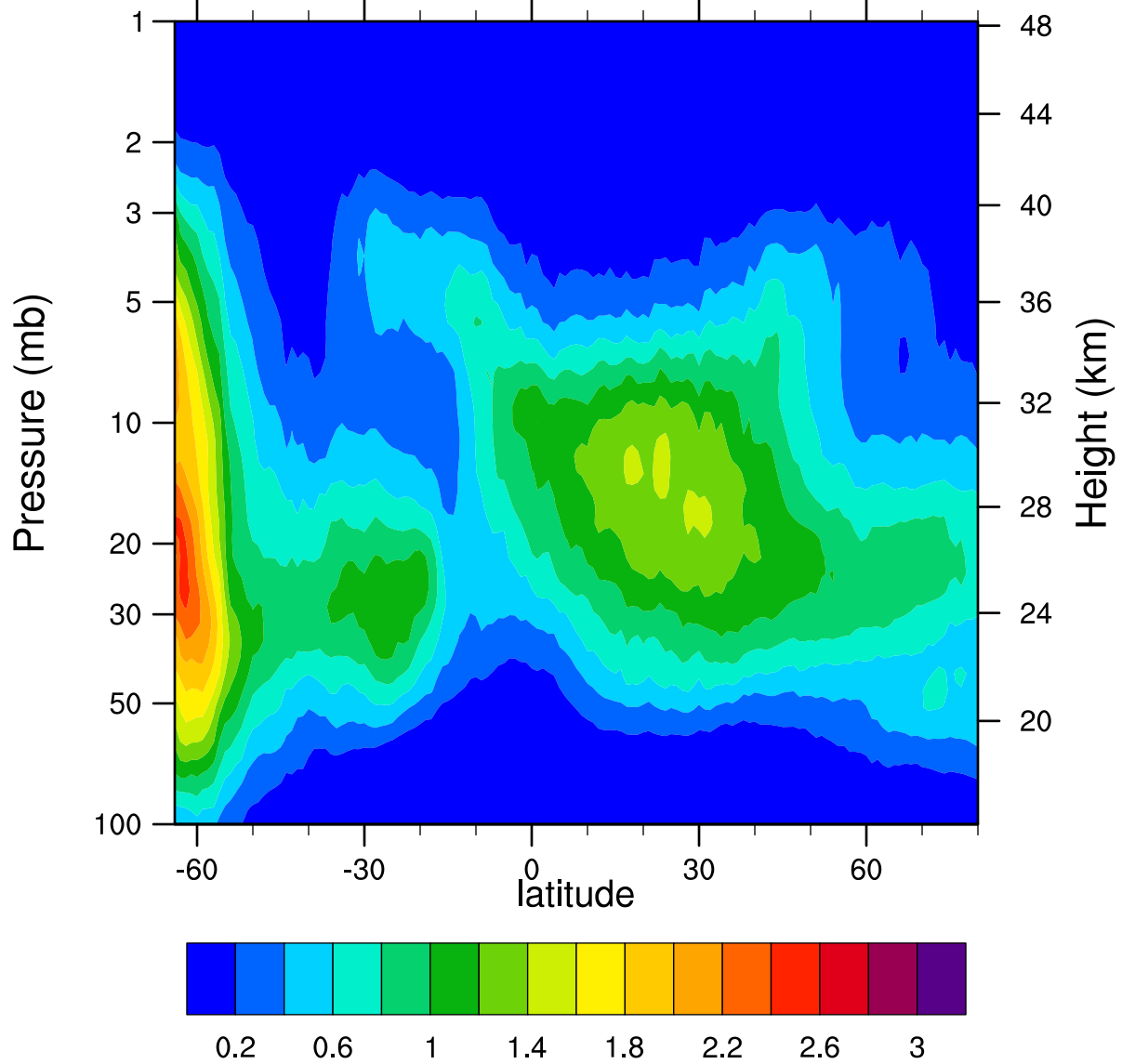
HIRDLSv6 2005d221 ClONO2_Ascending (ppbv)
