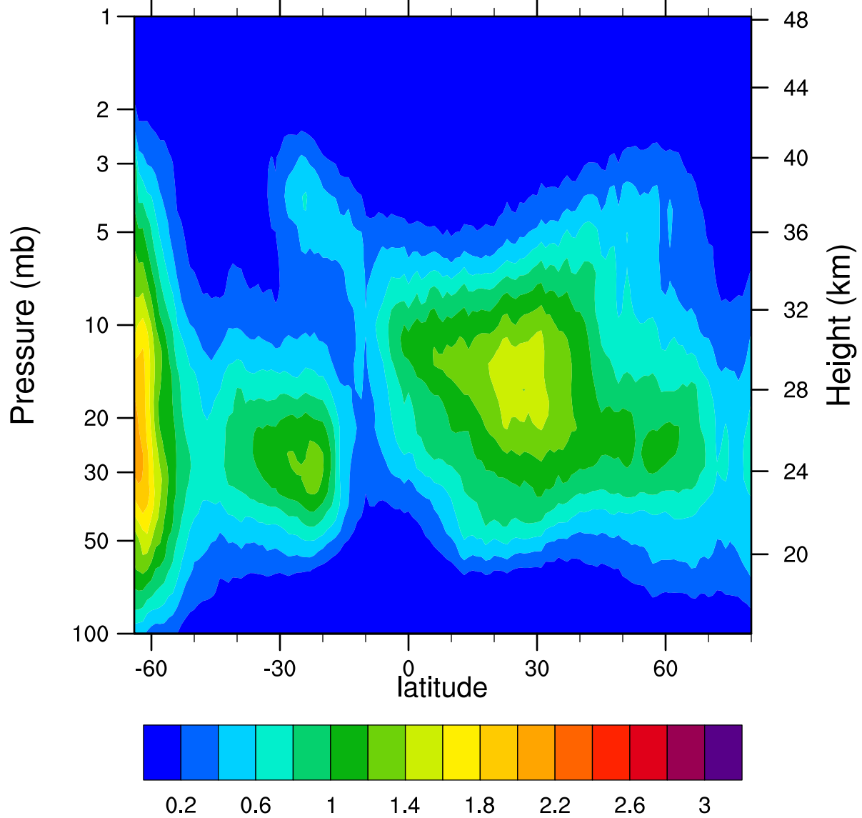
HIRDLSv6 2005d261 ClONO2_Ascending (ppbv)
