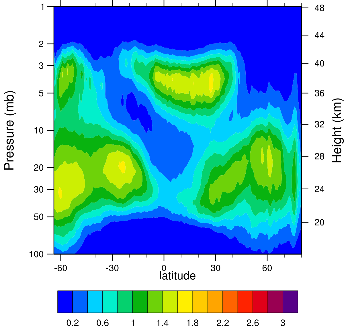
HIRDLSv6 2006d340 ClONO2_Ascending (ppbv)
