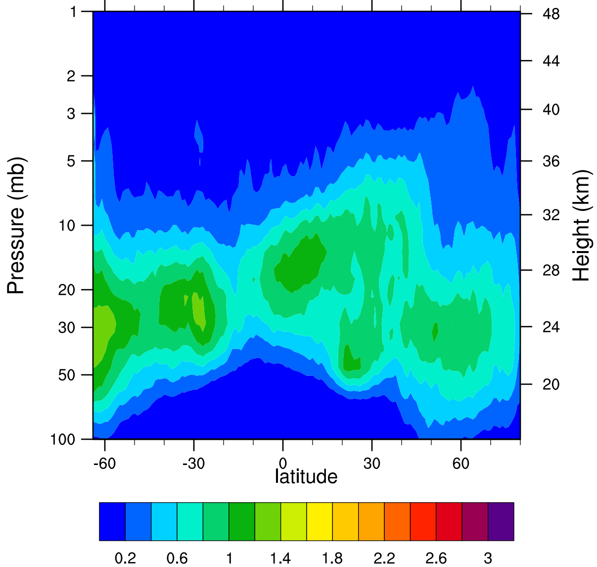
HIRDLSv6 2005d336 ClONO2_Ascending (ppbv)
