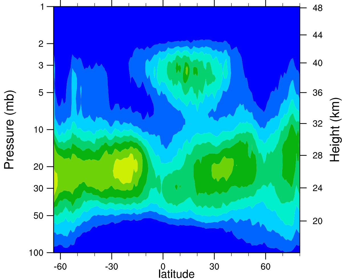
HIRDLSv6 2006d301 ClONO2_Ascending (ppbv)
