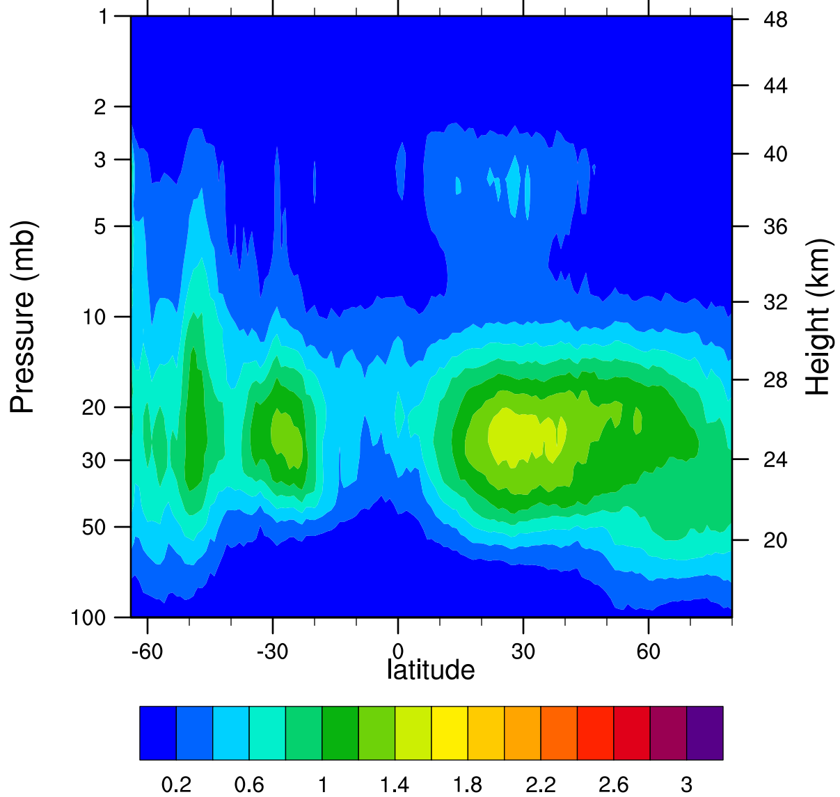
HIRDLSv6 2007d166 ClONO2_Ascending (ppbv)
