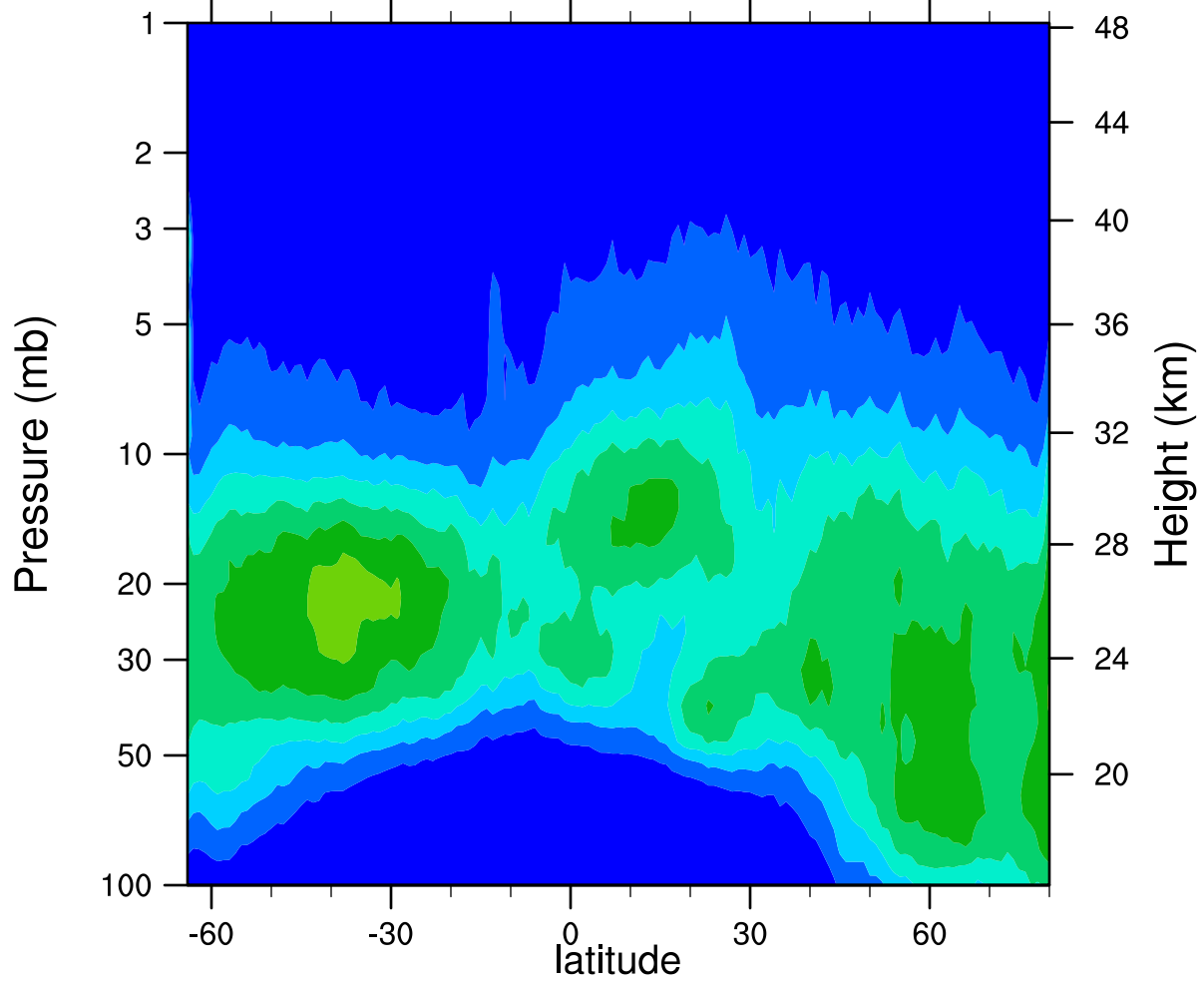
HIRDLSv6 2006d041 ClONO2_Ascending (ppbv)
