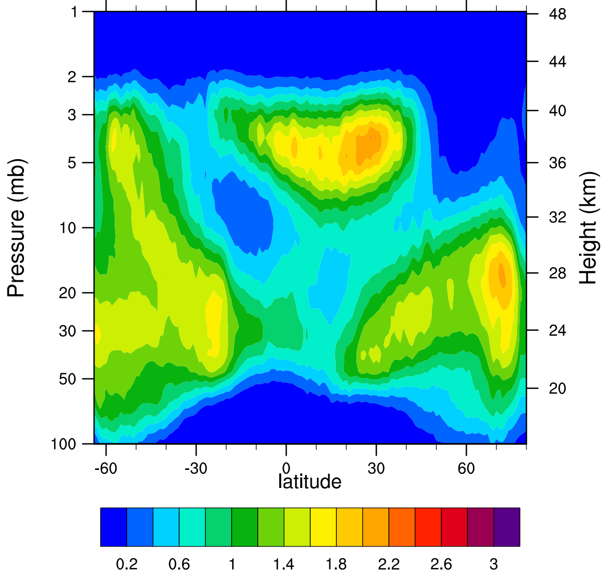
HIRDLSv6 2007d309 ClONO2_Ascending (ppbv)
