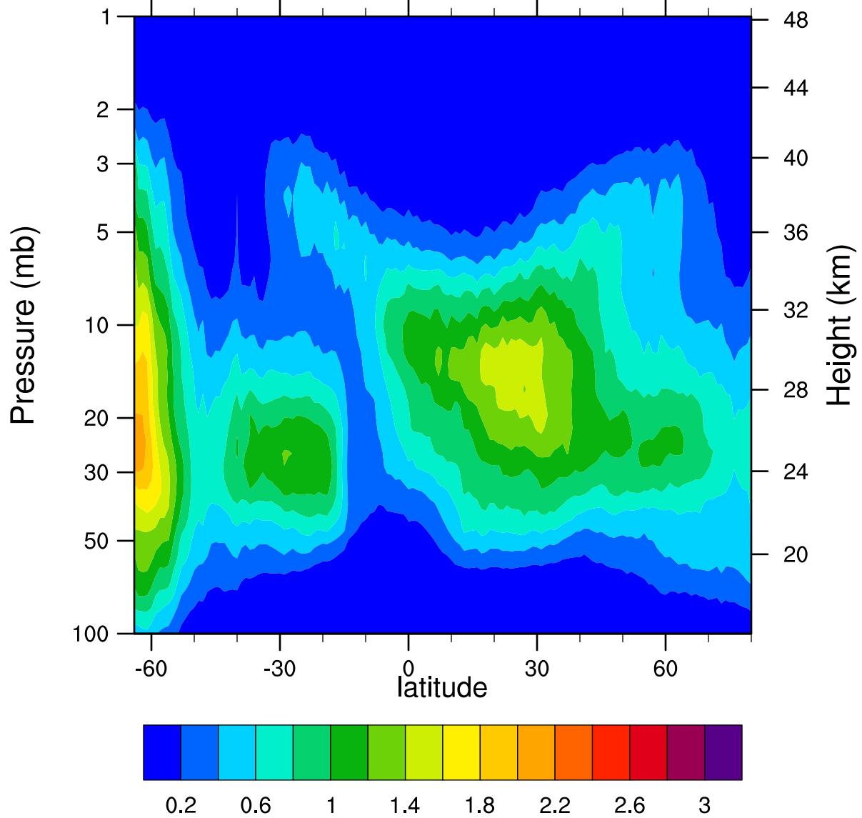
HIRDLSv6 2005d253 ClONO2_Ascending (ppbv)
