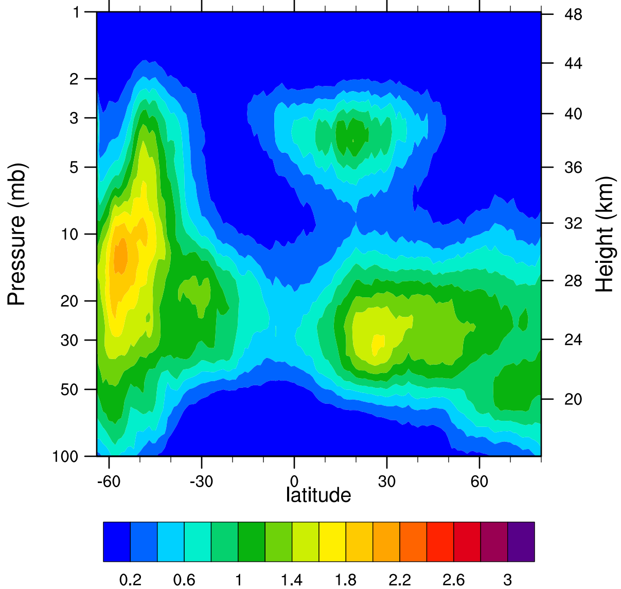
HIRDLSv6 2007d127 ClONO2_Ascending (ppbv)
