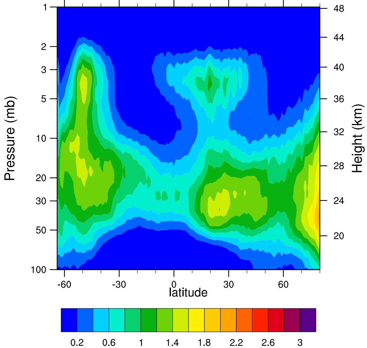
HIRDLSv6 2007d090 ClONO2_Ascending (ppbv)
