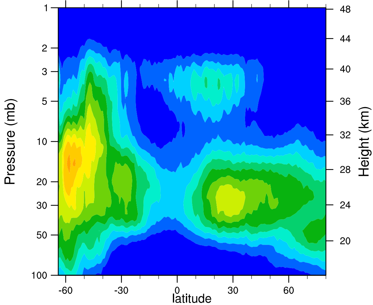
HIRDLSv6 2007d137 ClONO2_Ascending (ppbv)
