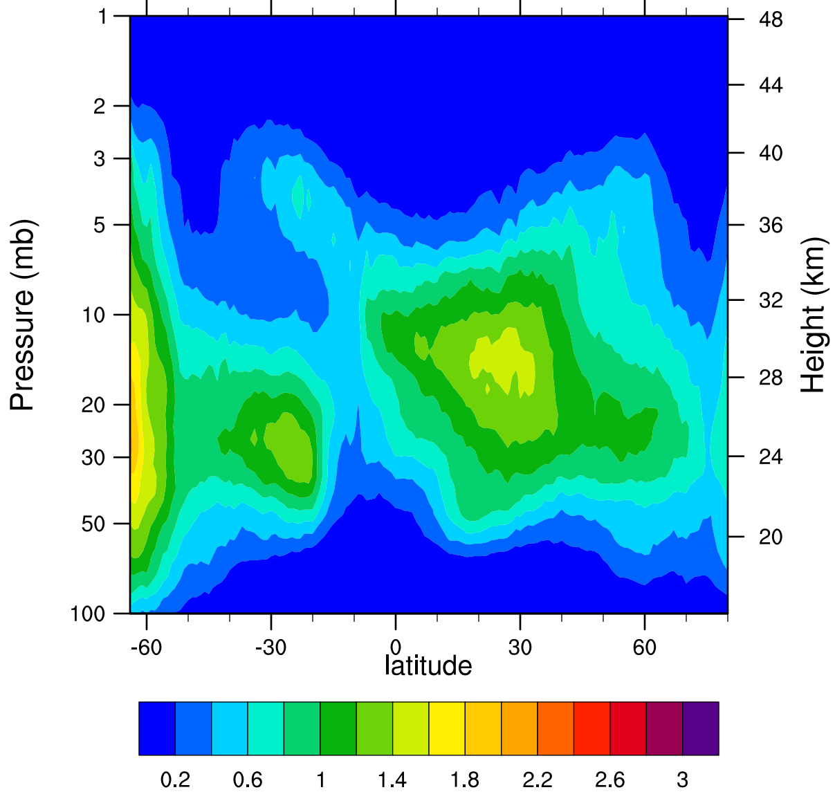
HIRDLSv6 2005d269 ClONO2_Ascending (ppbv)
