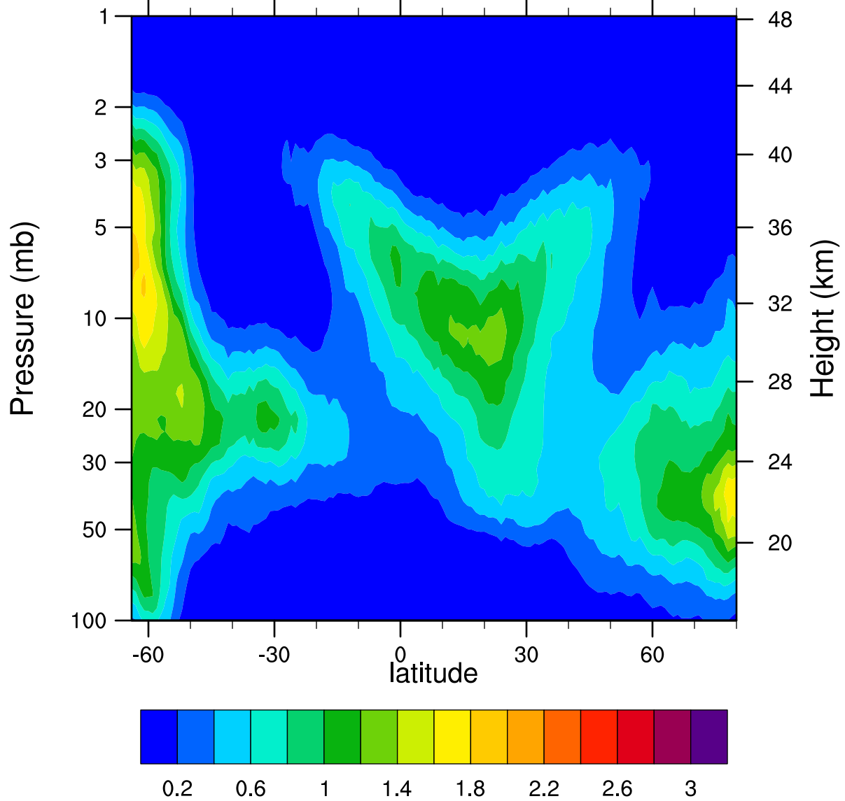
HIRDLSv6 2005d064 ClONO2_Ascending (ppbv)
