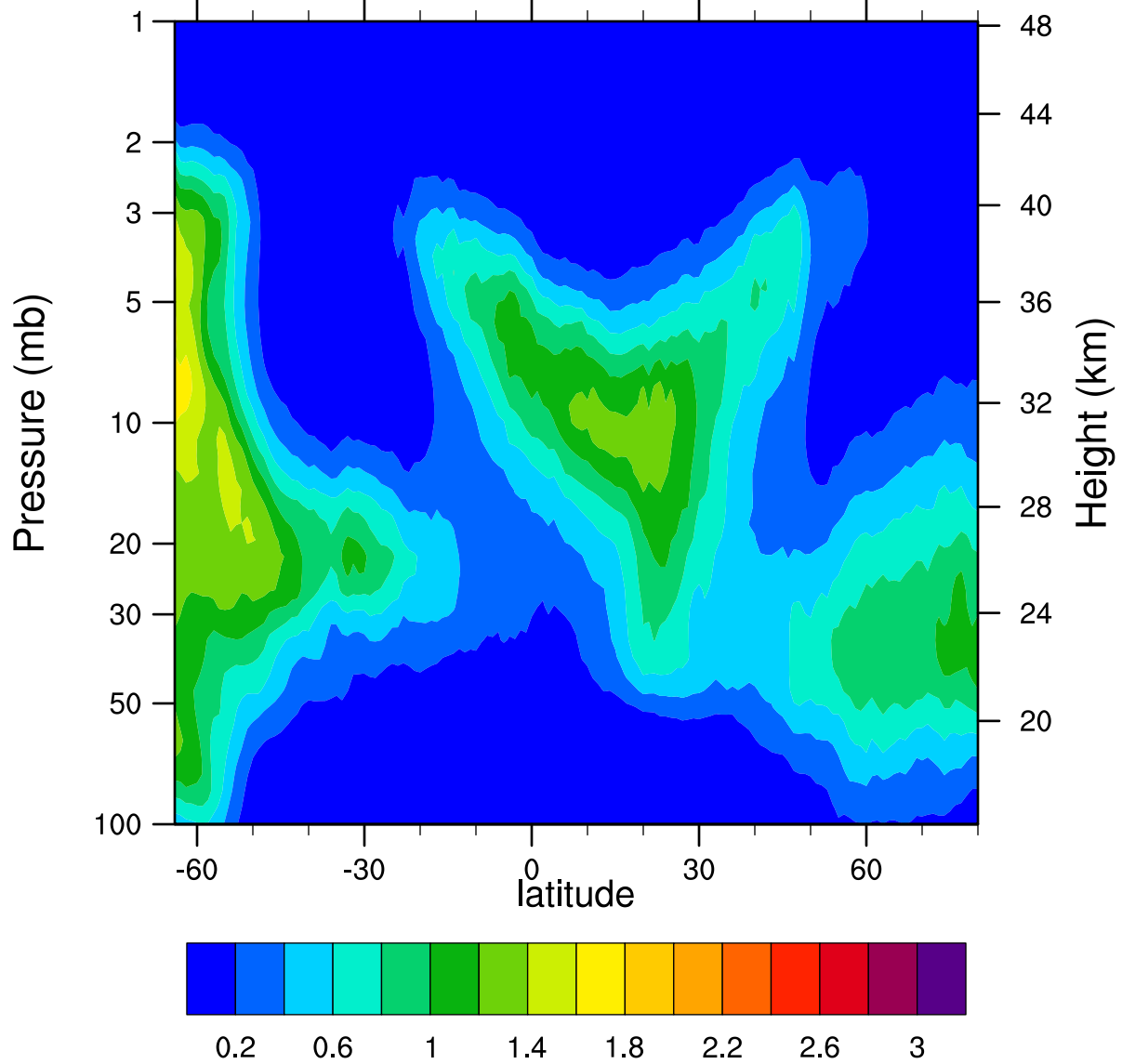
HIRDLSv6 2005d054 ClONO2_Ascending (ppbv)
