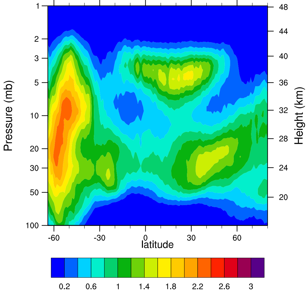
HIRDLSv6 2007d230 ClONO2_Ascending (ppbv)
