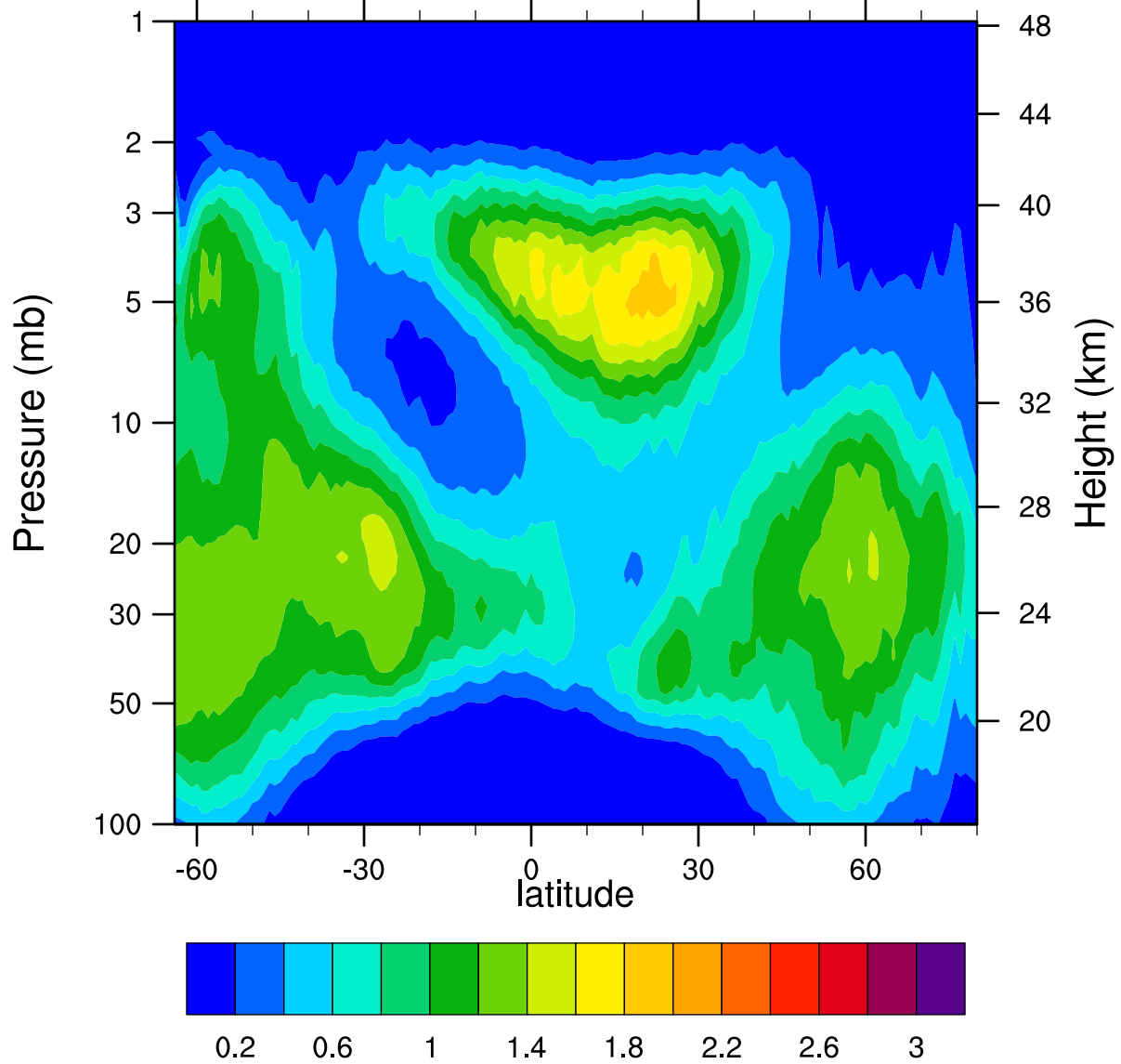
HIRDLSv6 2007d356 ClONO2_Ascending (ppbv)
