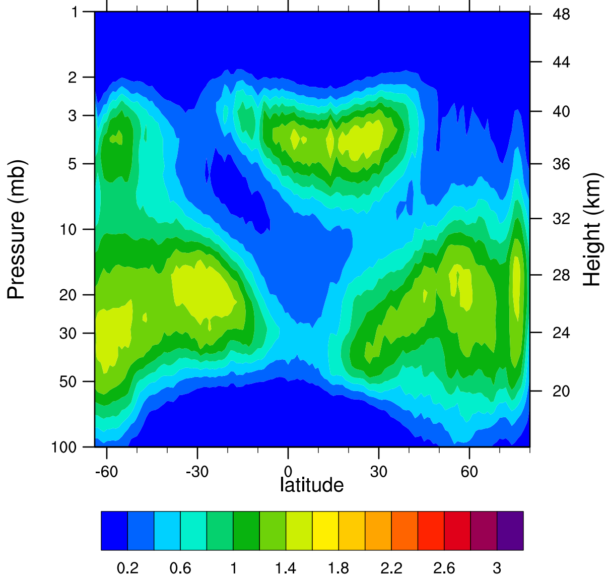
HIRDLSv6 2006d348 ClONO2_Ascending (ppbv)
