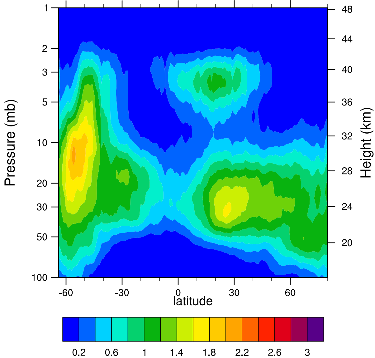
HIRDLSv6 2007d123 ClONO2_Ascending (ppbv)
