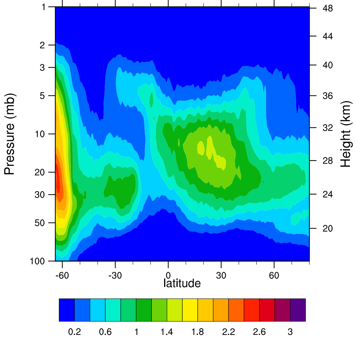
HIRDLSv6 2005d222 ClONO2_Ascending (ppbv)
