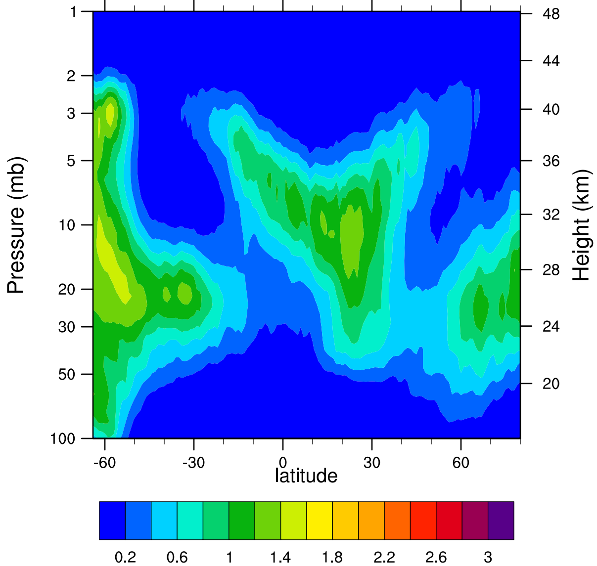
HIRDLSv6 2005d034 ClONO2_Ascending (ppbv)
