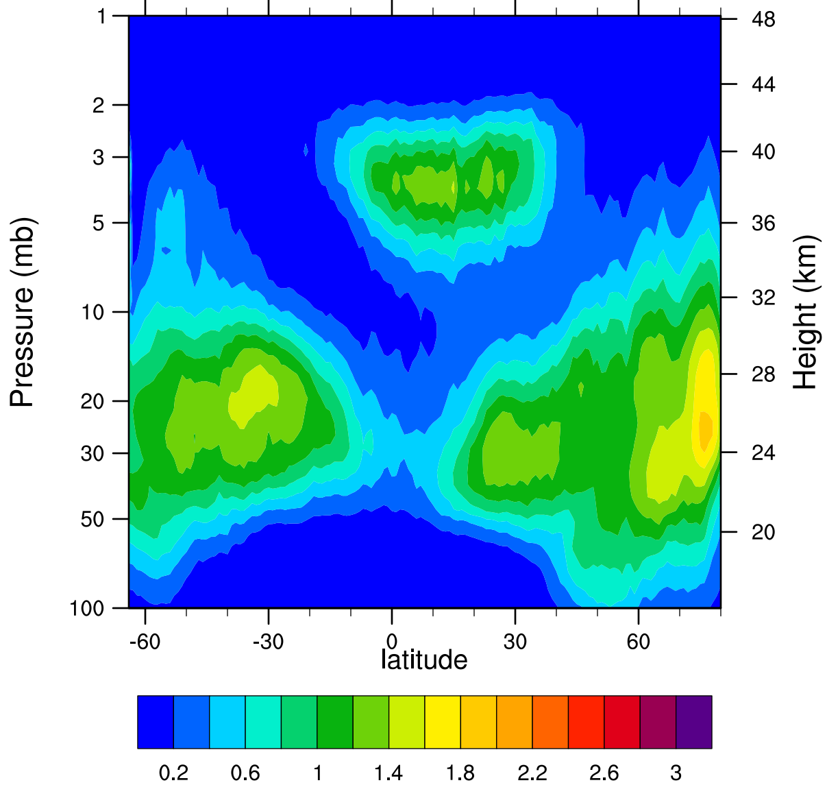
HIRDLSv6 2007d014 ClONO2_Ascending (ppbv)
