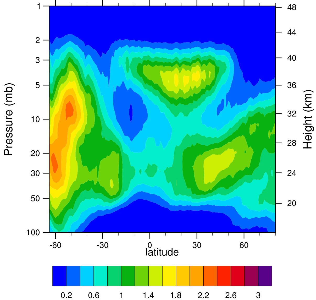
HIRDLSv6 2007d243 ClONO2_Ascending (ppbv)
