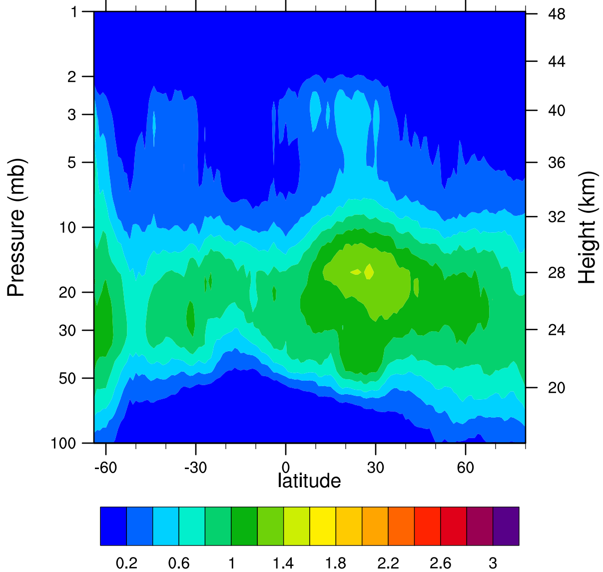
HIRDLSv6 2006d124 ClONO2_Ascending (ppbv)
