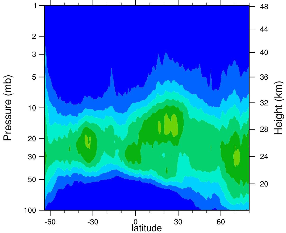
HIRDLSv6 2006d082 ClONO2_Ascending (ppbv)
