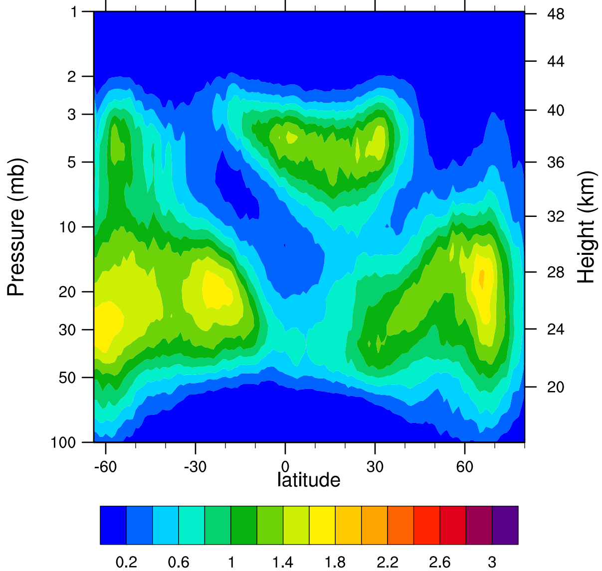
HIRDLSv6 2006d320 ClONO2_Ascending (ppbv)
