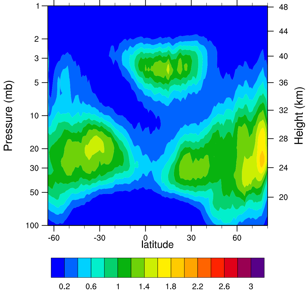
HIRDLSv6 2007d013 ClONO2_Ascending (ppbv)
