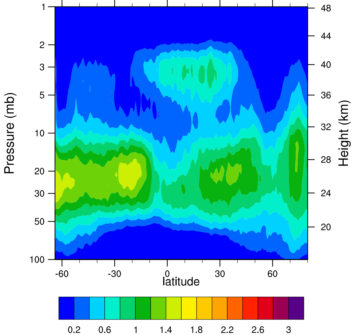
HIRDLSv6 2006d305 ClONO2_Ascending (ppbv)
