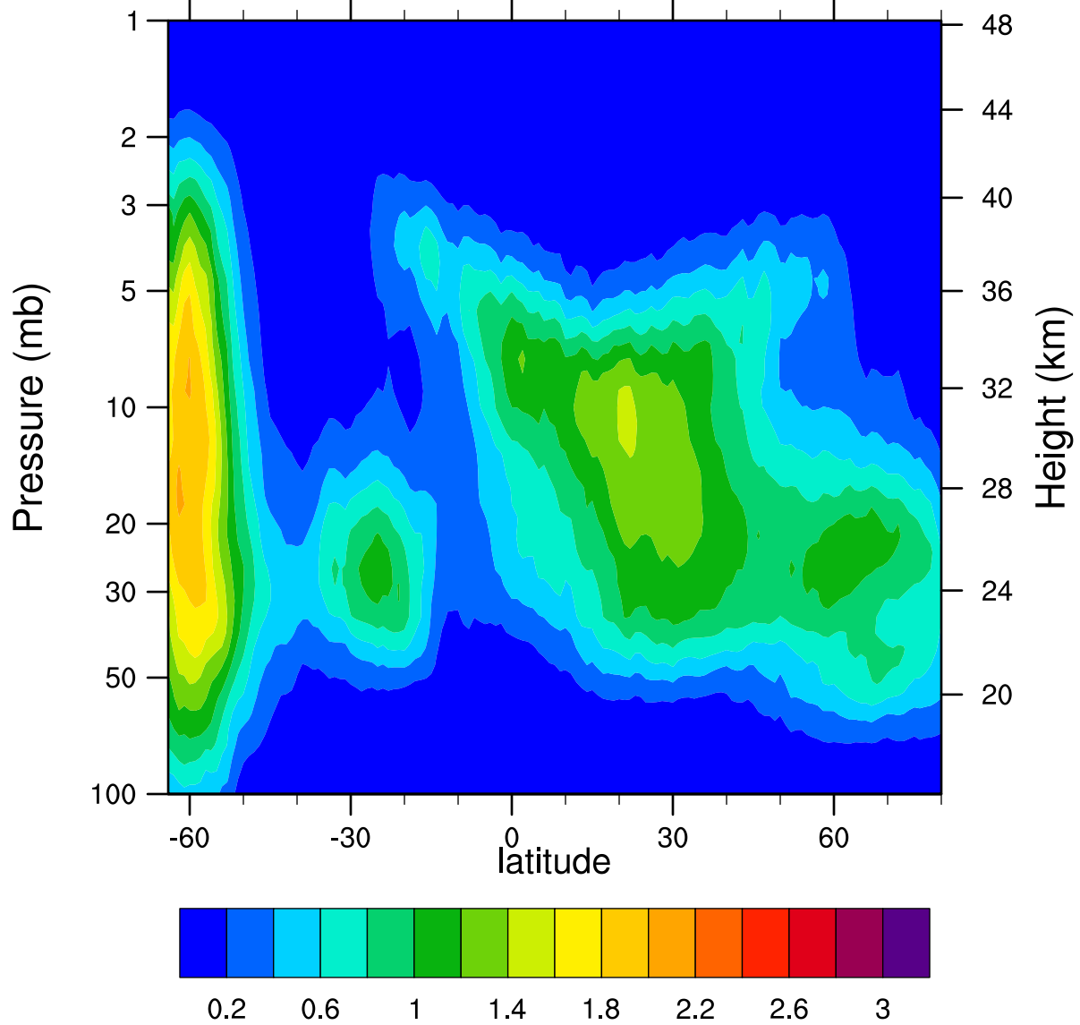
HIRDLSv6 2005d175 ClONO2_Ascending (ppbv)
