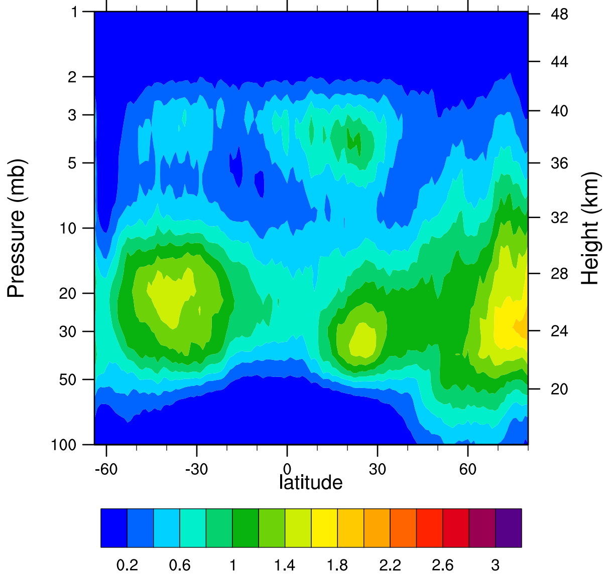
HIRDLSv6 2007d049 ClONO2_Ascending (ppbv)
