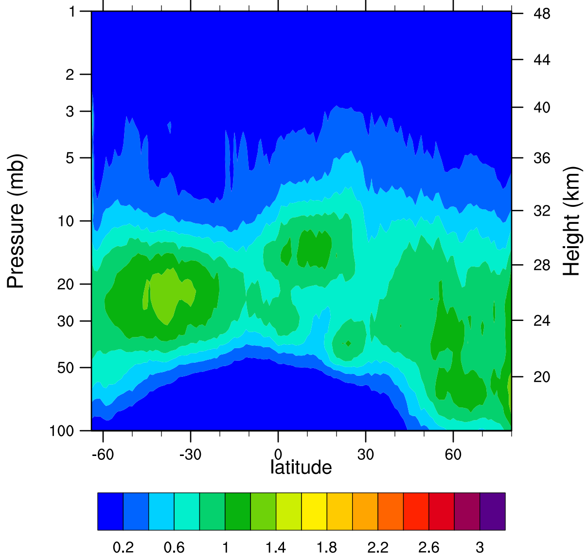
HIRDLSv6 2006d043 ClONO2_Ascending (ppbv)
