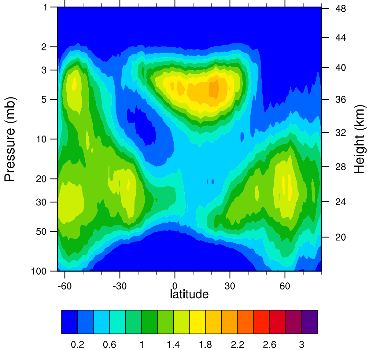
HIRDLSv6 2007d334 ClONO2_Ascending (ppbv)
