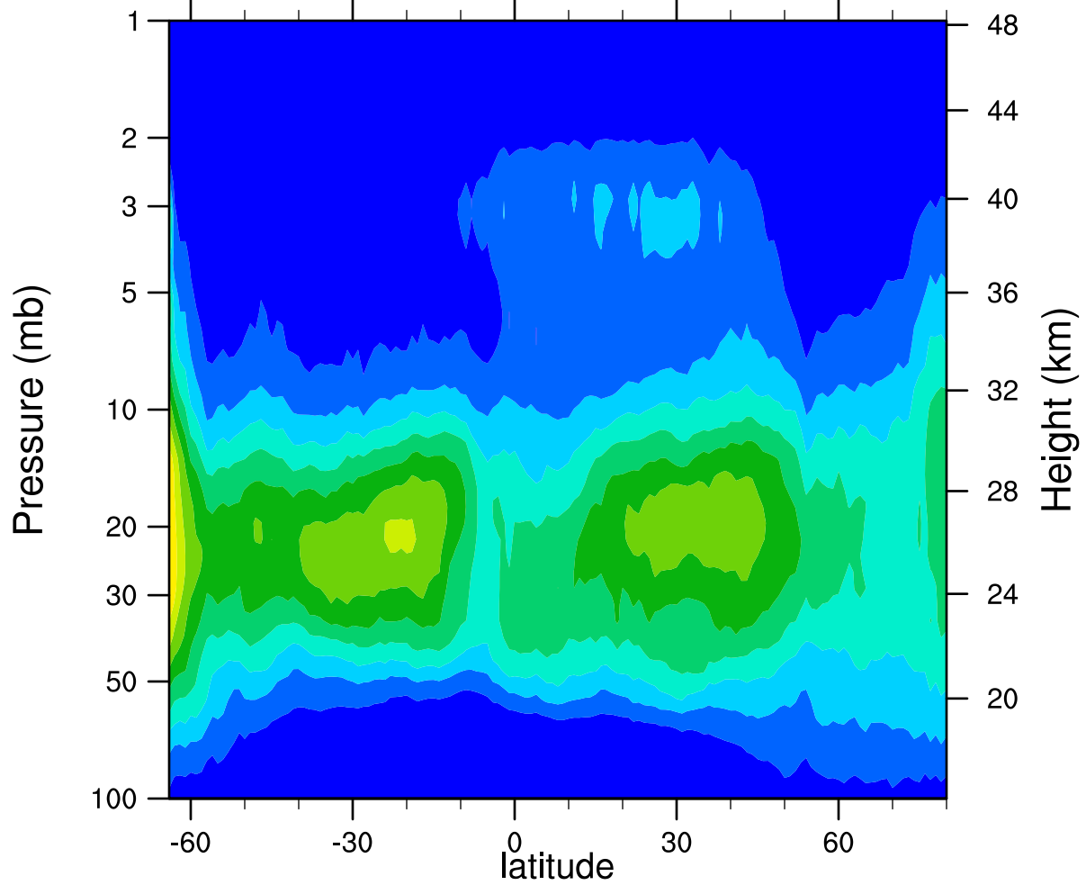
HIRDLSv6 2006d284 ClONO2_Ascending (ppbv)
