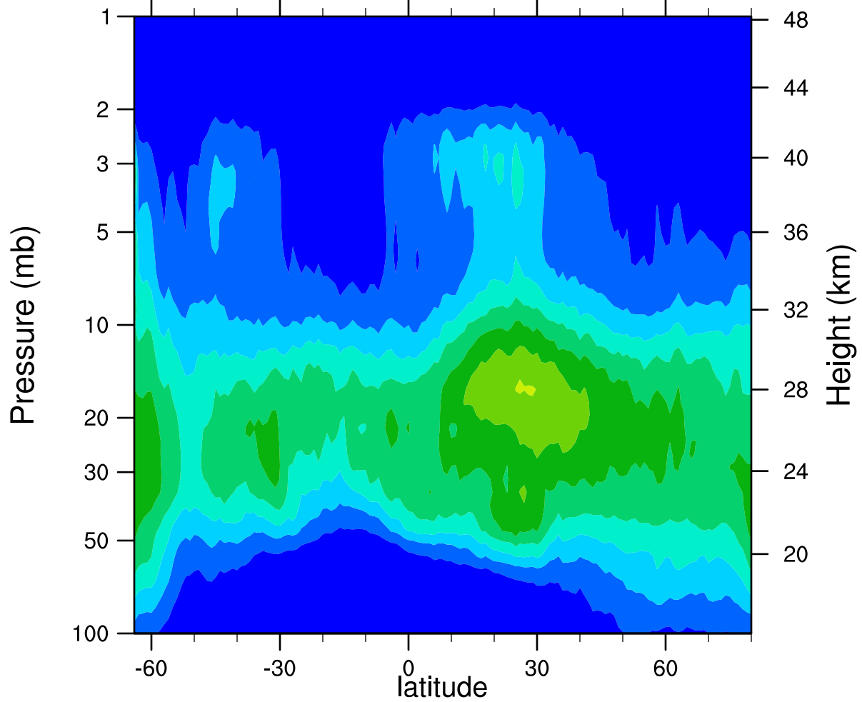
HIRDLSv6 2006d120 ClONO2_Ascending (ppbv)
