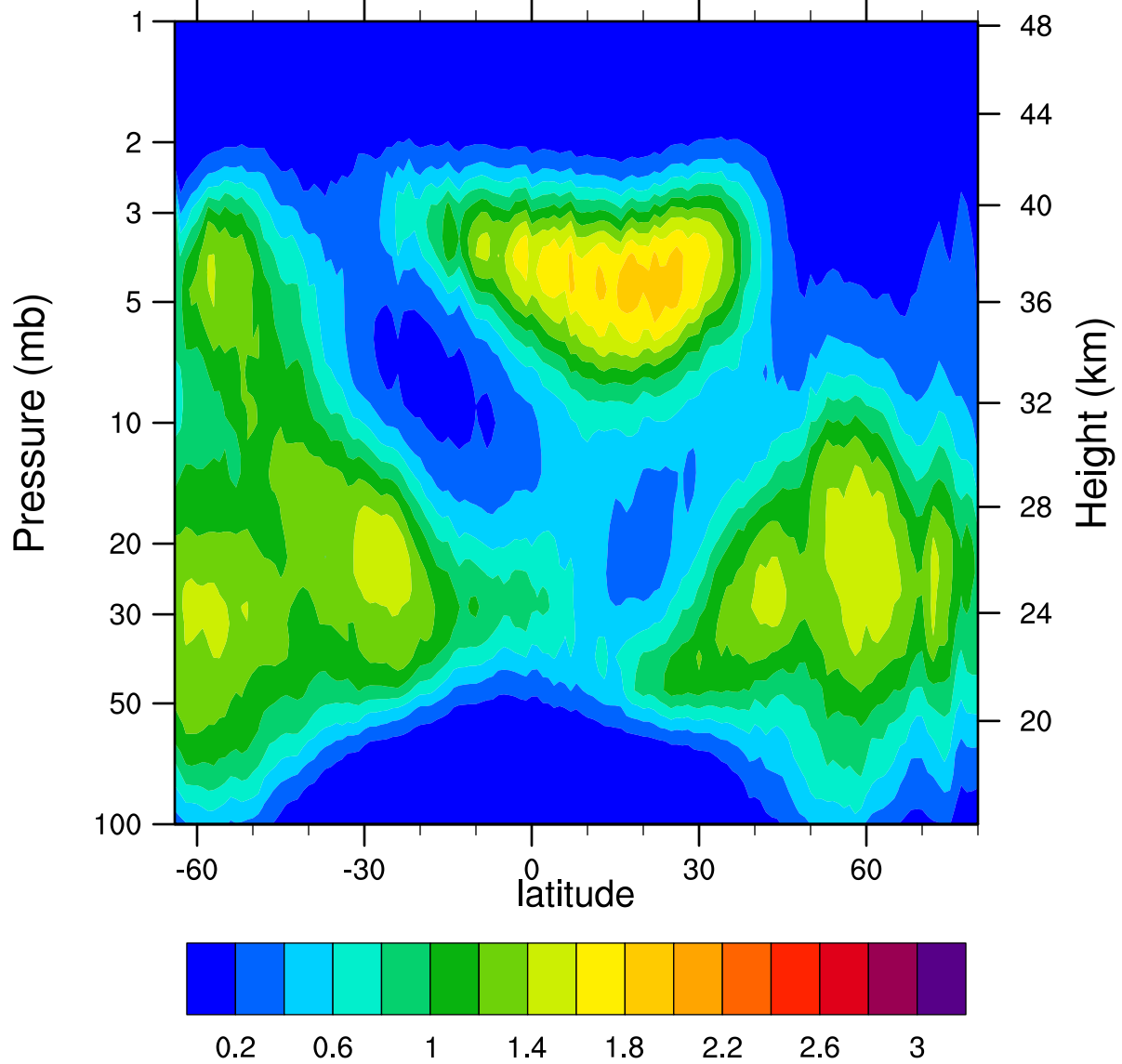
HIRDLSv6 2007d343 ClONO2_Ascending (ppbv)
