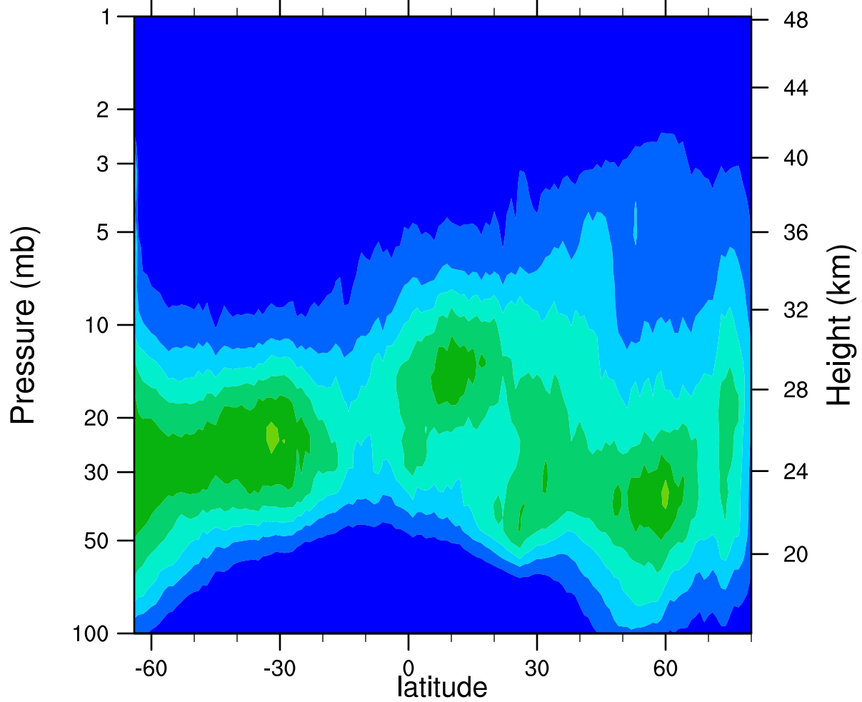
HIRDLSv6 2005d355 ClONO2_Ascending (ppbv)
