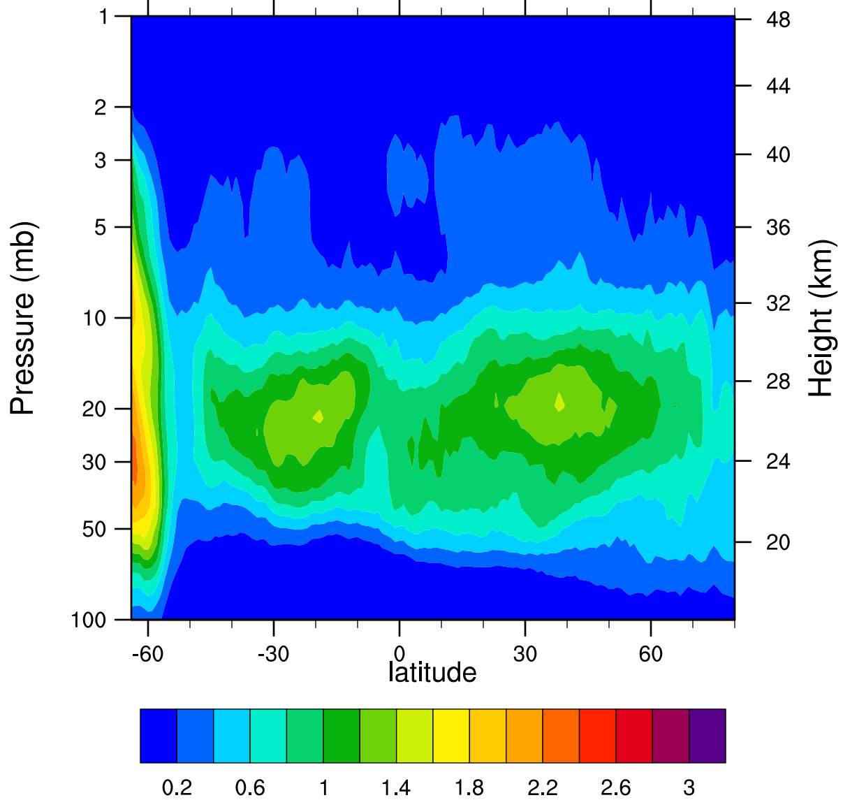
HIRDLSv6 2006d251 ClONO2_Ascending (ppbv)
