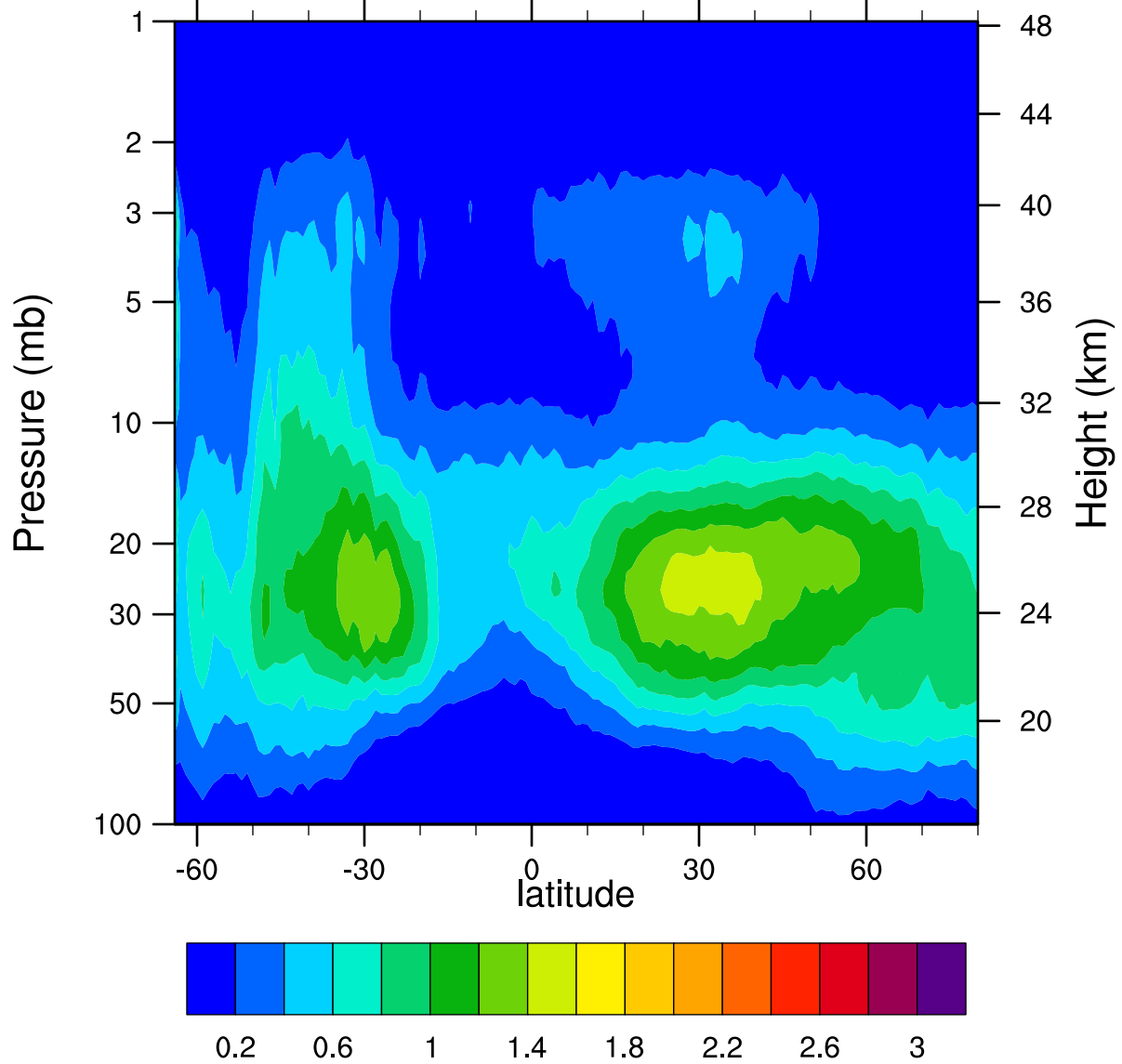
HIRDLSv6 2007d173 ClONO2_Ascending (ppbv)
