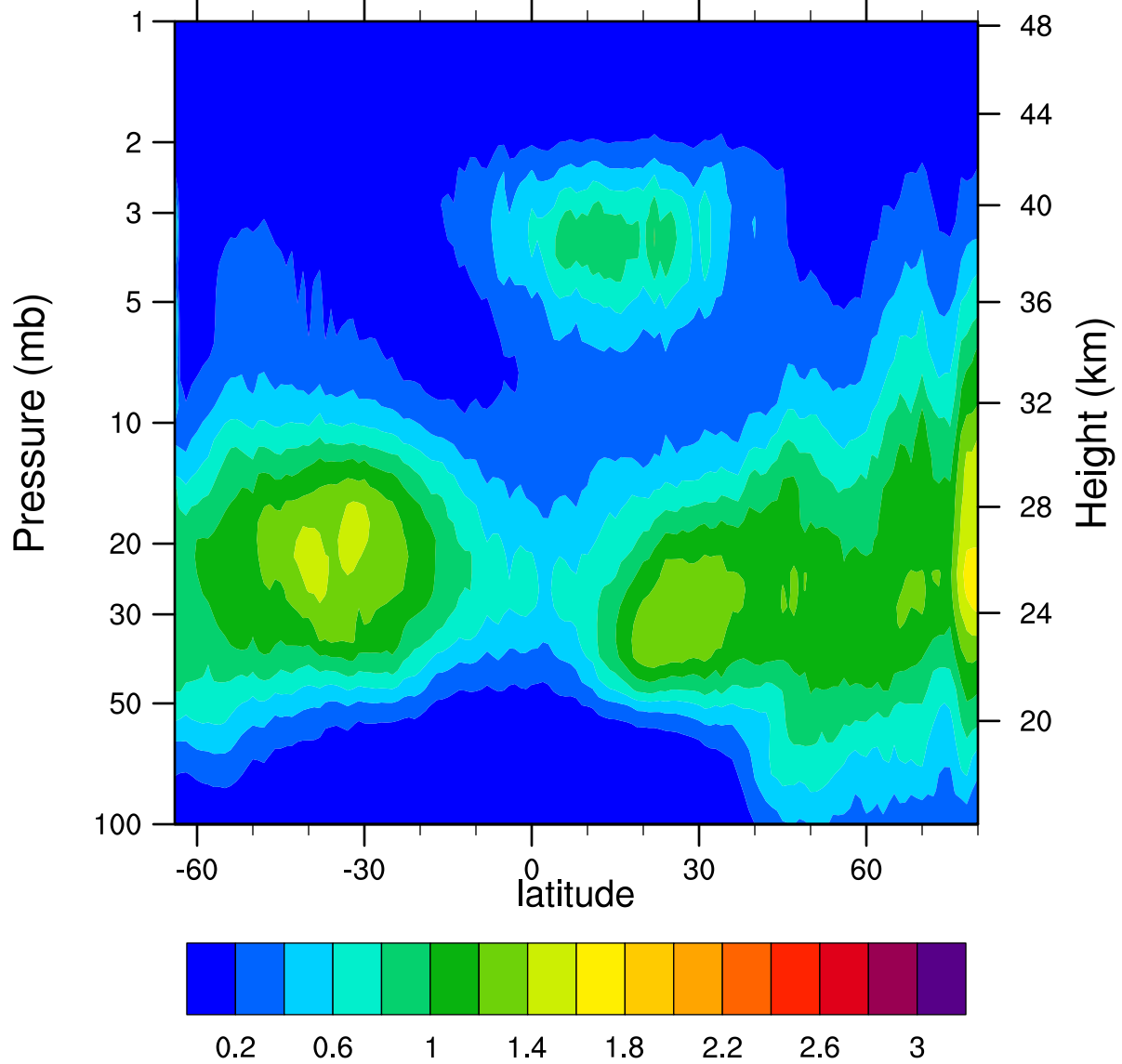
HIRDLSv6 2007d031 ClONO2_Ascending (ppbv)
