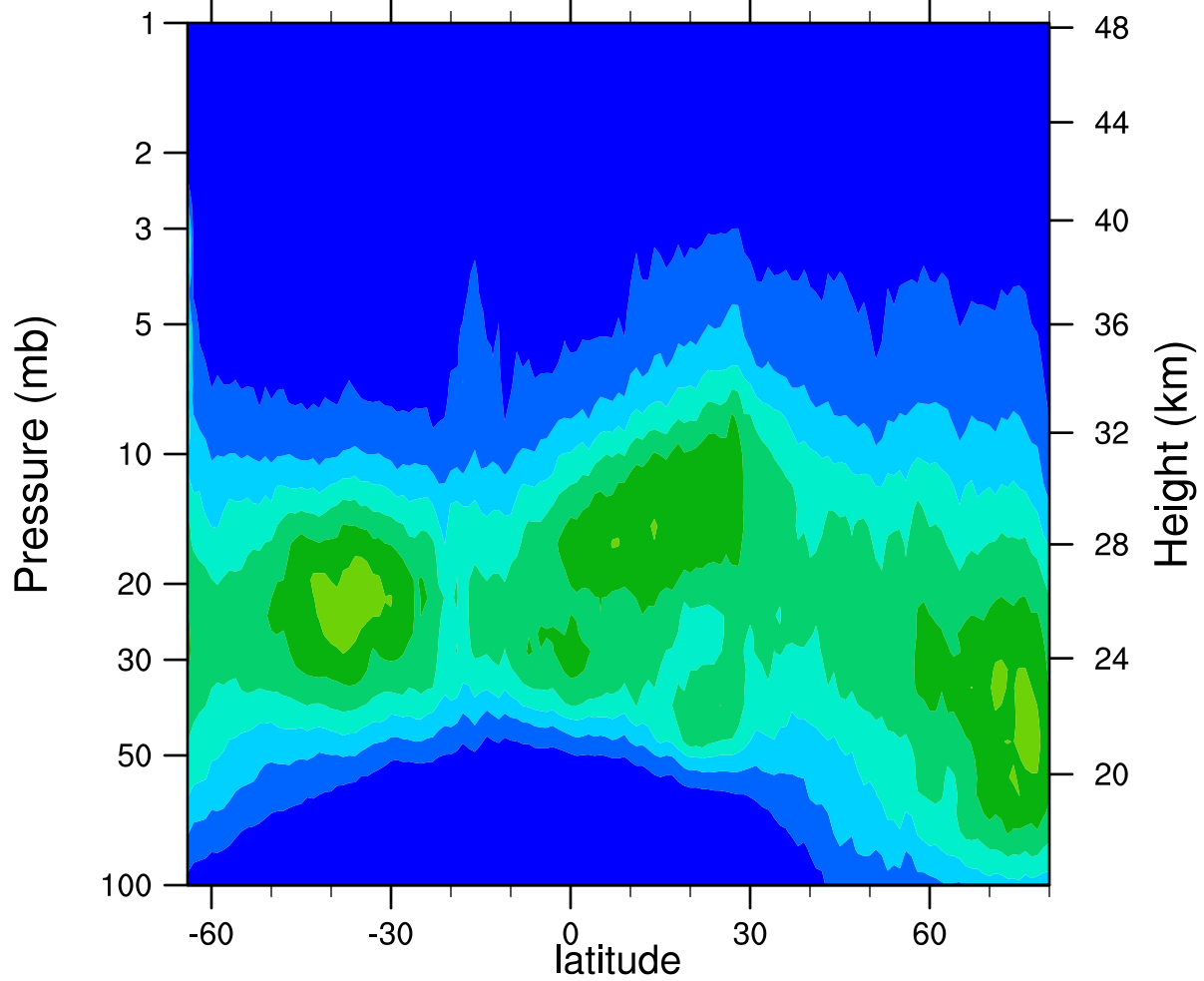
HIRDLSv6 2006d060 ClONO2_Ascending (ppbv)
