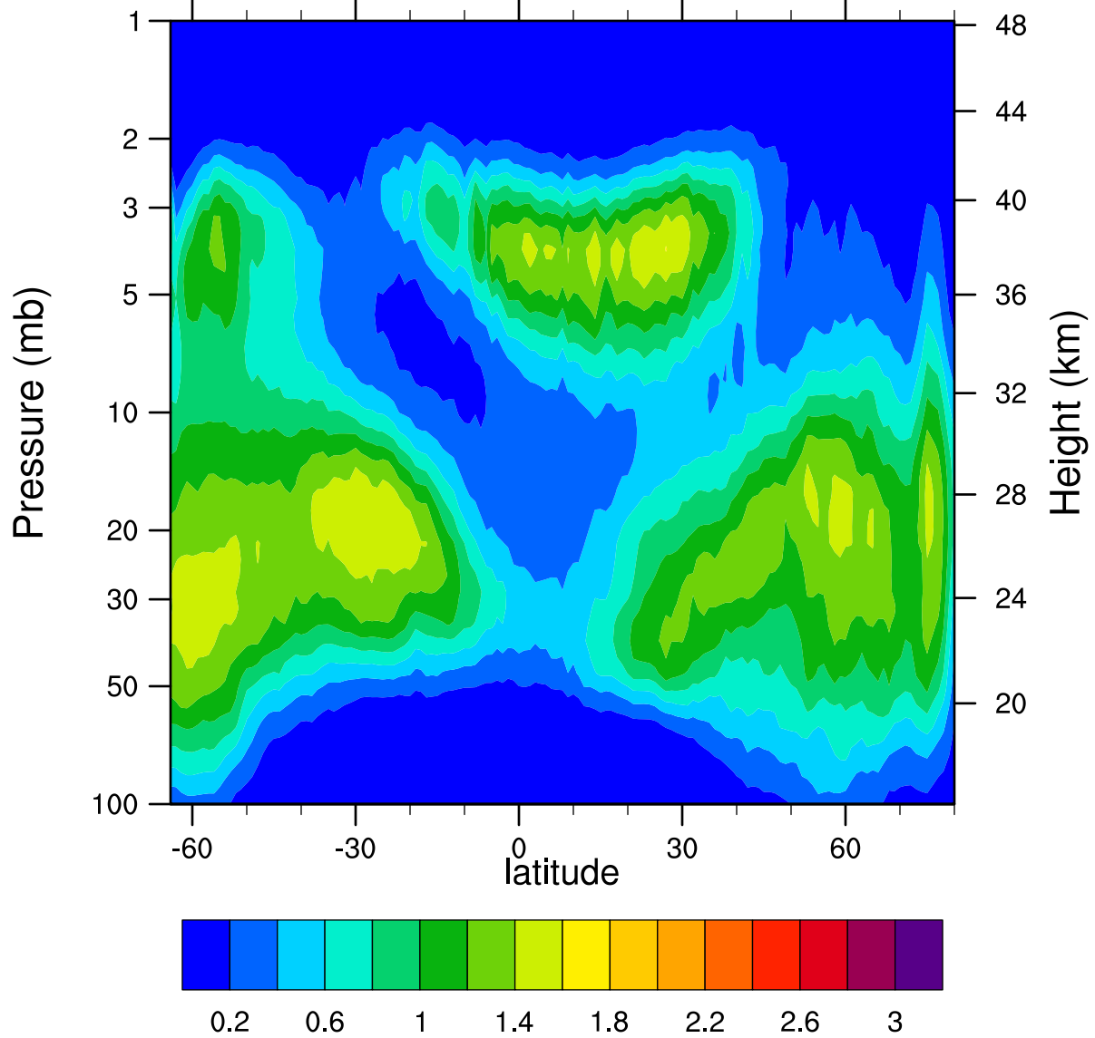
HIRDLSv6 2006d347 ClONO2_Ascending (ppbv)
