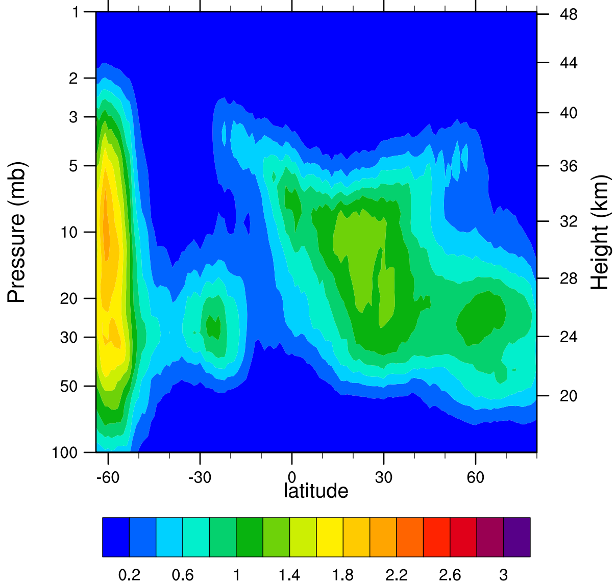
HIRDLSv6 2005d170 ClONO2_Ascending (ppbv)
