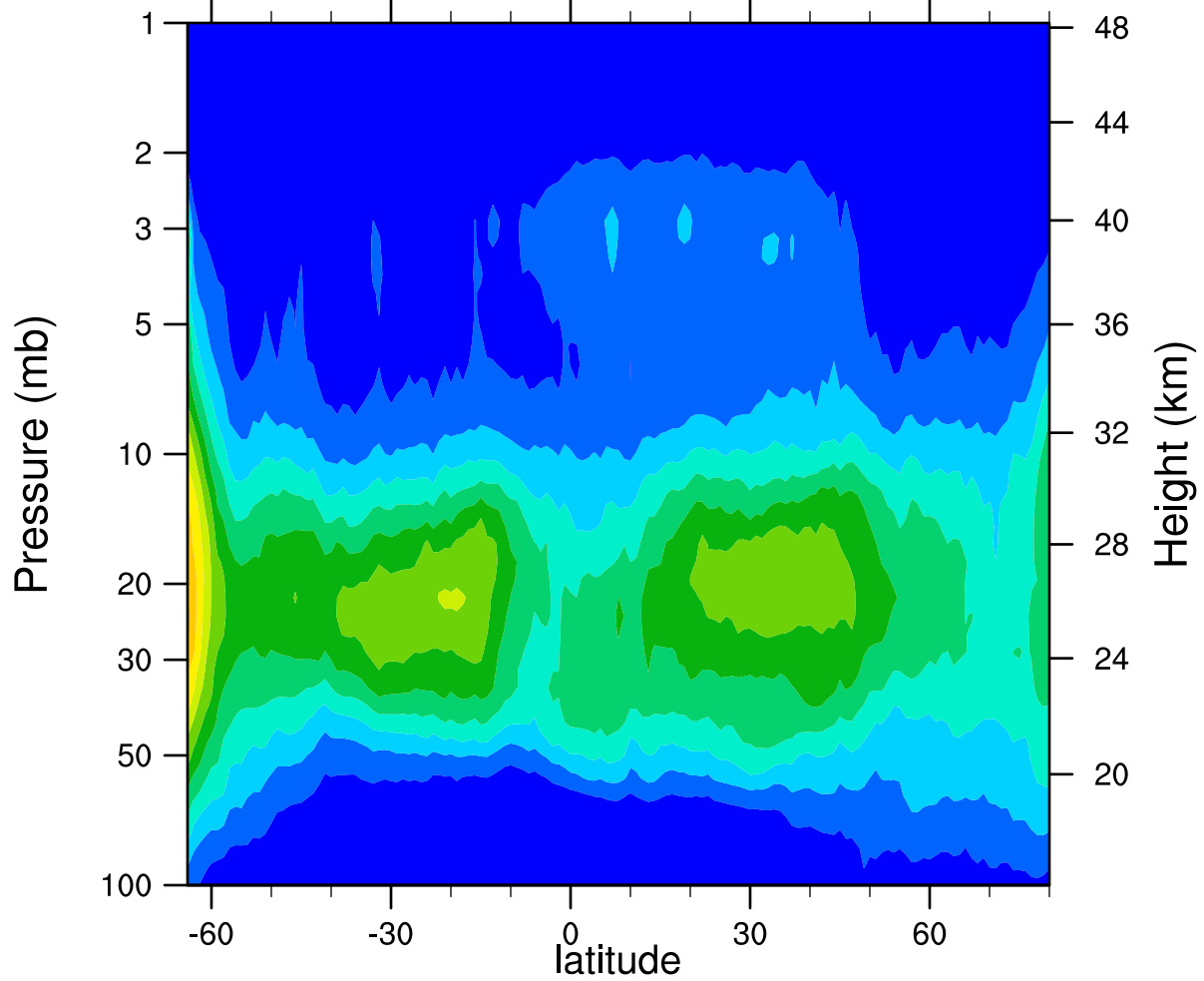
HIRDLSv6 2006d277 ClONO2_Ascending (ppbv)
