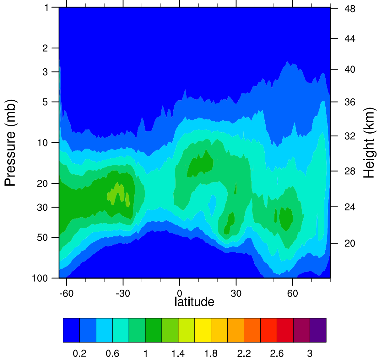
HIRDLSv6 2005d361 ClONO2_Ascending (ppbv)
