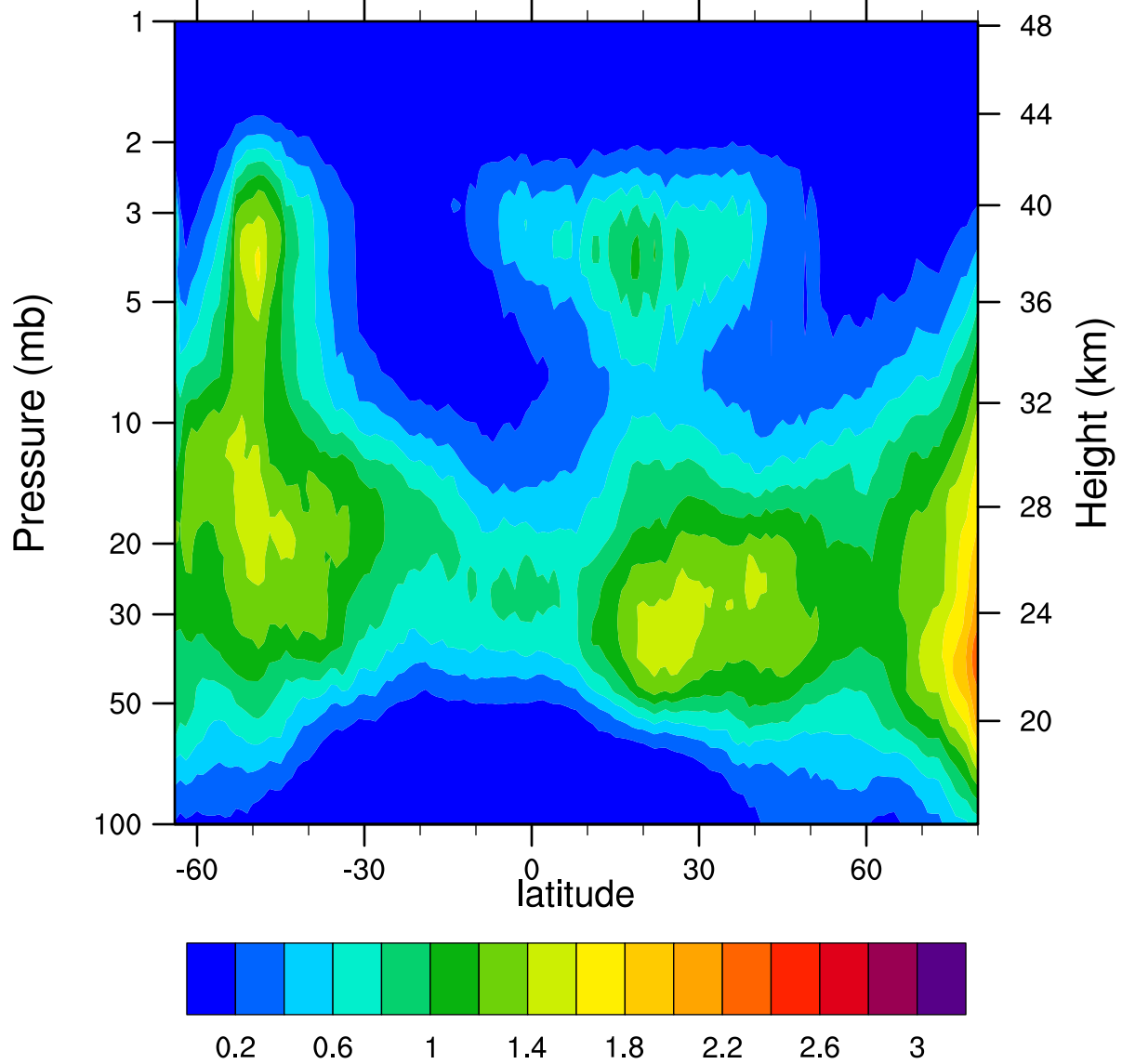
HIRDLSv6 2007d087 ClONO2_Ascending (ppbv)
