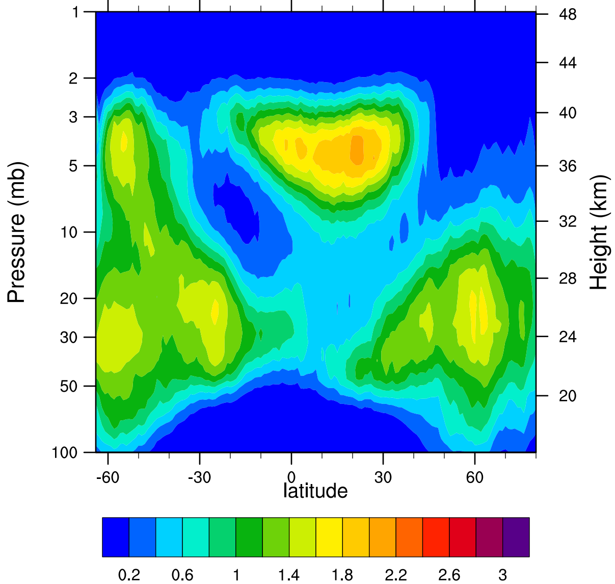
HIRDLSv6 2007d333 ClONO2_Ascending (ppbv)
