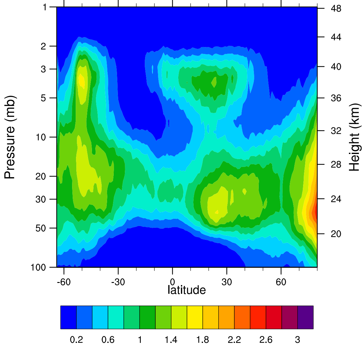
HIRDLSv6 2007d085 ClONO2_Ascending (ppbv)
