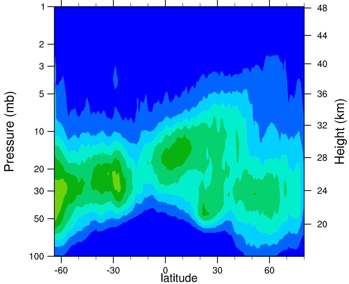
HIRDLSv6 2005d337 ClONO2_Ascending (ppbv)
