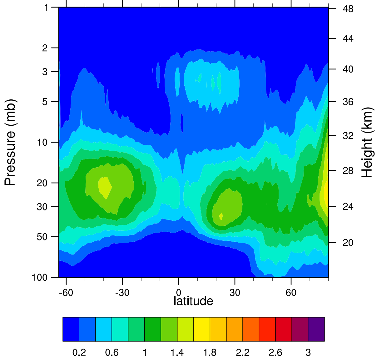
HIRDLSv6 2007d035 ClONO2_Ascending (ppbv)
