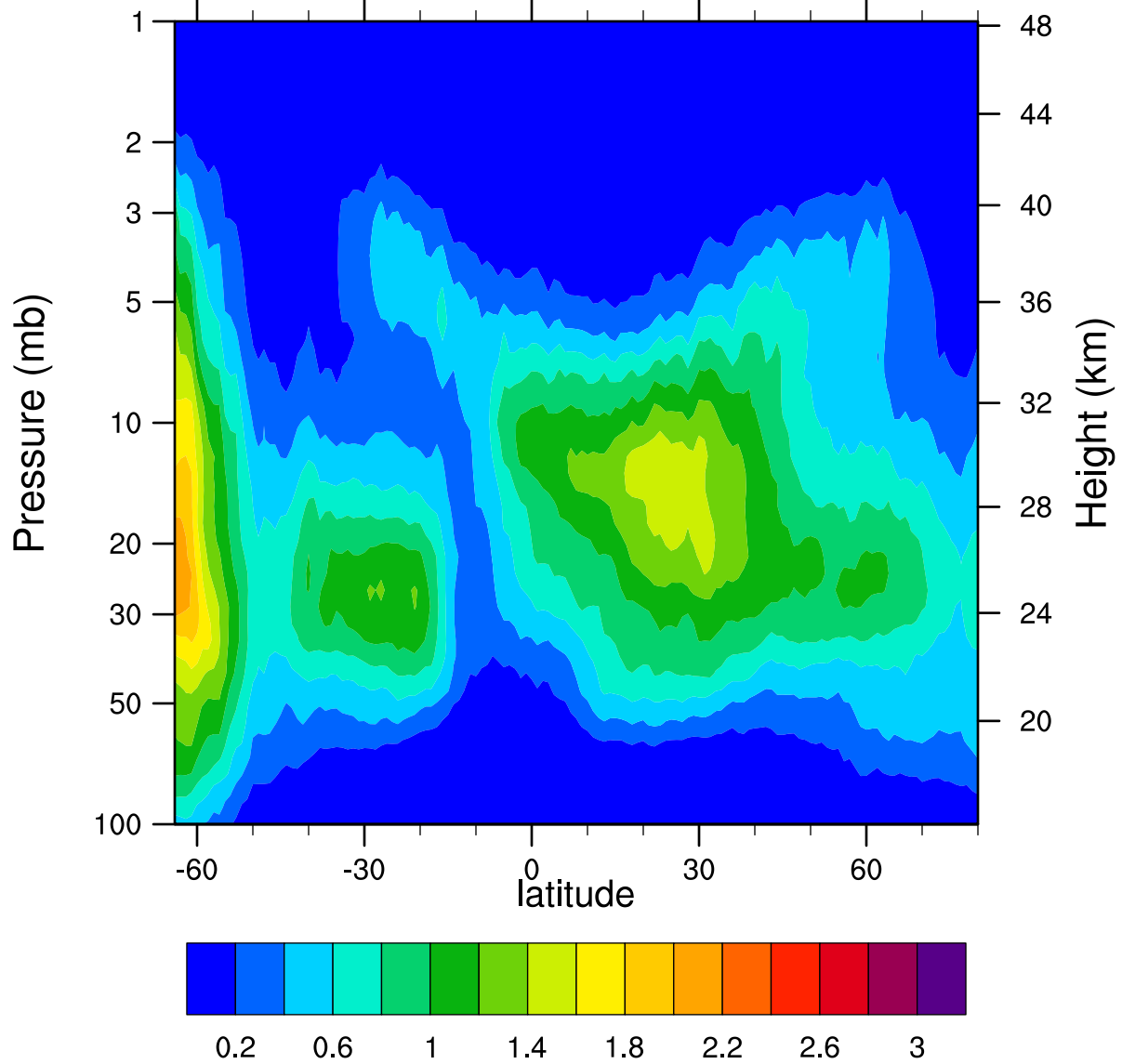
HIRDLSv6 2005d255 ClONO2_Ascending (ppbv)
