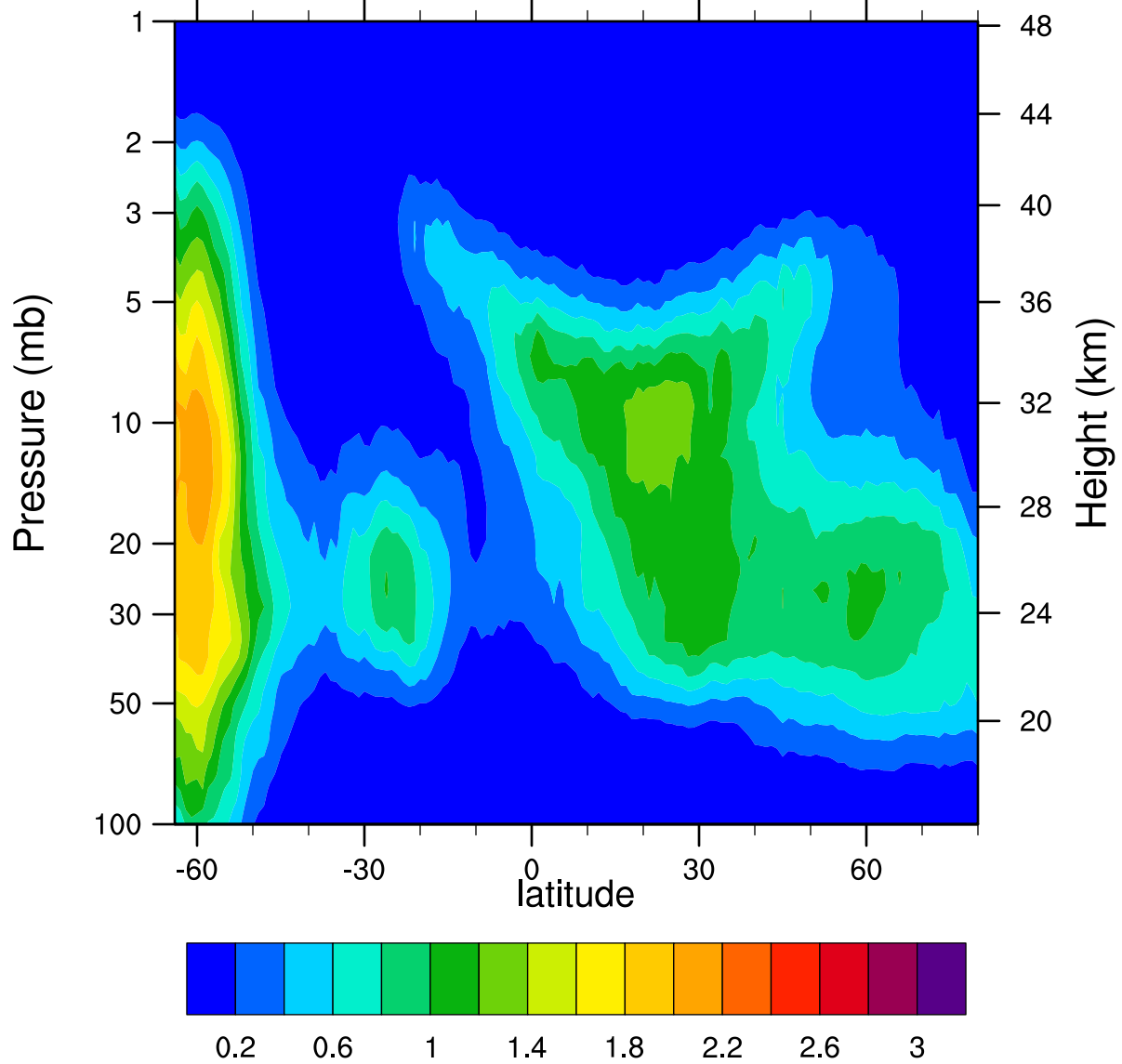
HIRDLSv6 2005d153 ClONO2_Ascending (ppbv)
