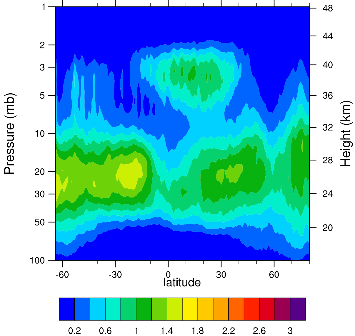
HIRDLSv6 2006d303 ClONO2_Ascending (ppbv)
