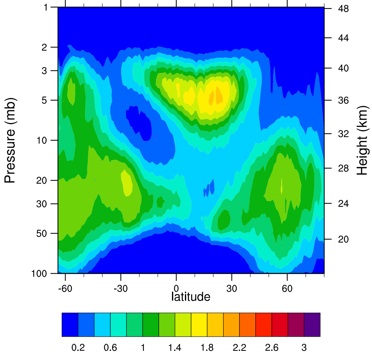
HIRDLSv6 2007d355 ClONO2_Ascending (ppbv)
