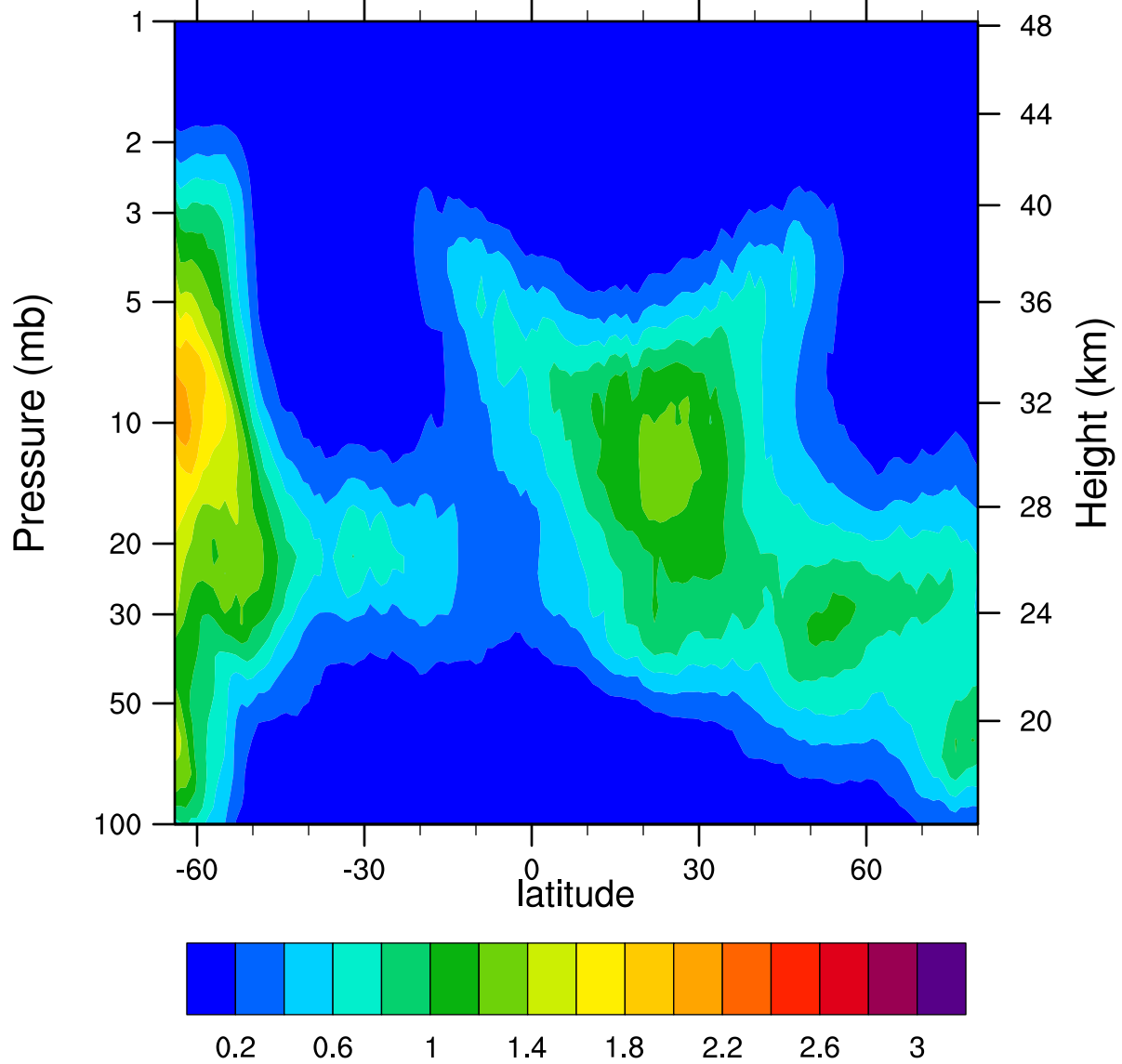
HIRDLSv6 2005d100 ClONO2_Ascending (ppbv)
