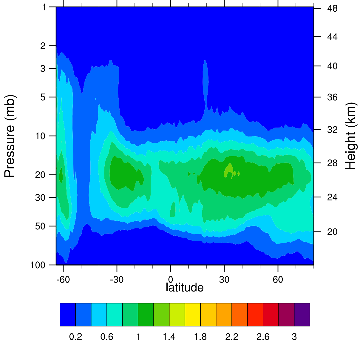
HIRDLSv6 2006d178 ClONO2_Ascending (ppbv)
