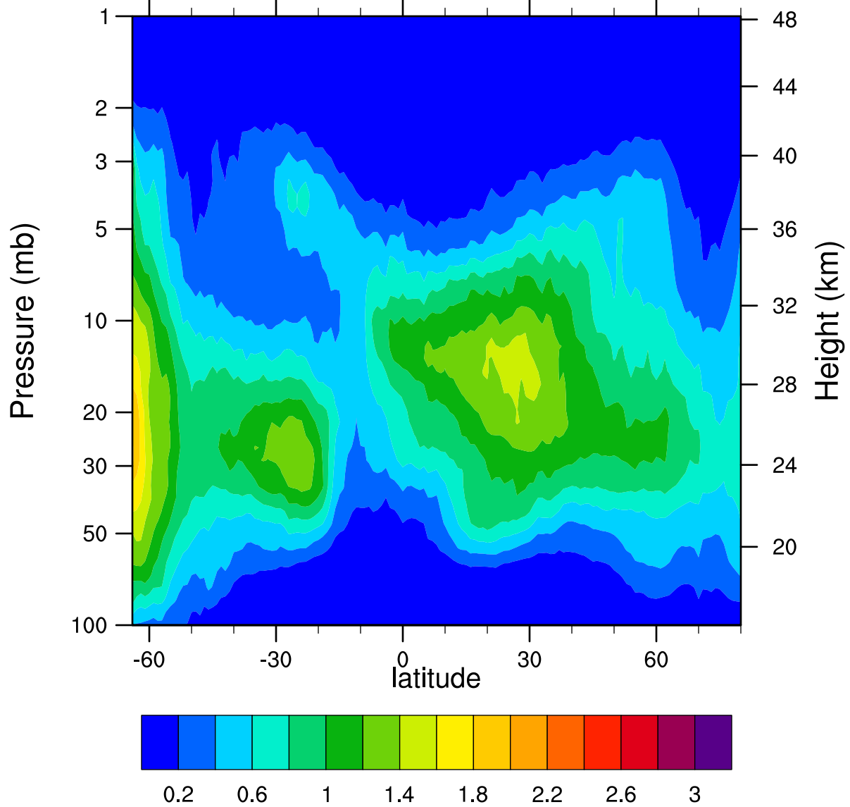
HIRDLSv6 2005d271 ClONO2_Ascending (ppbv)
