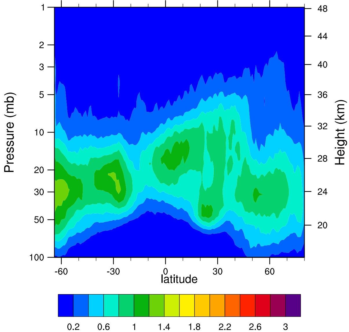
HIRDLSv6 2005d334 ClONO2_Ascending (ppbv)
