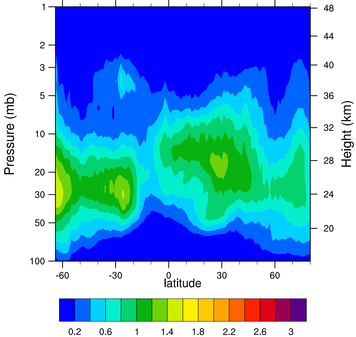
HIRDLSv6 2005d300 ClONO2_Ascending (ppbv)
