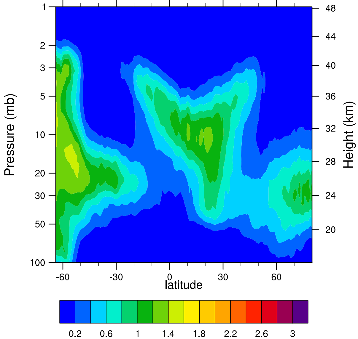
HIRDLSv6 2005d048 ClONO2_Ascending (ppbv)
