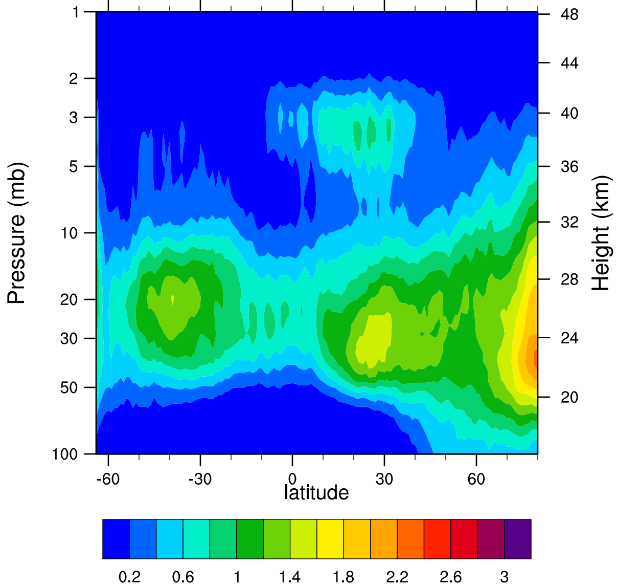
HIRDLSv6 2007d073 ClONO2_Ascending (ppbv)
