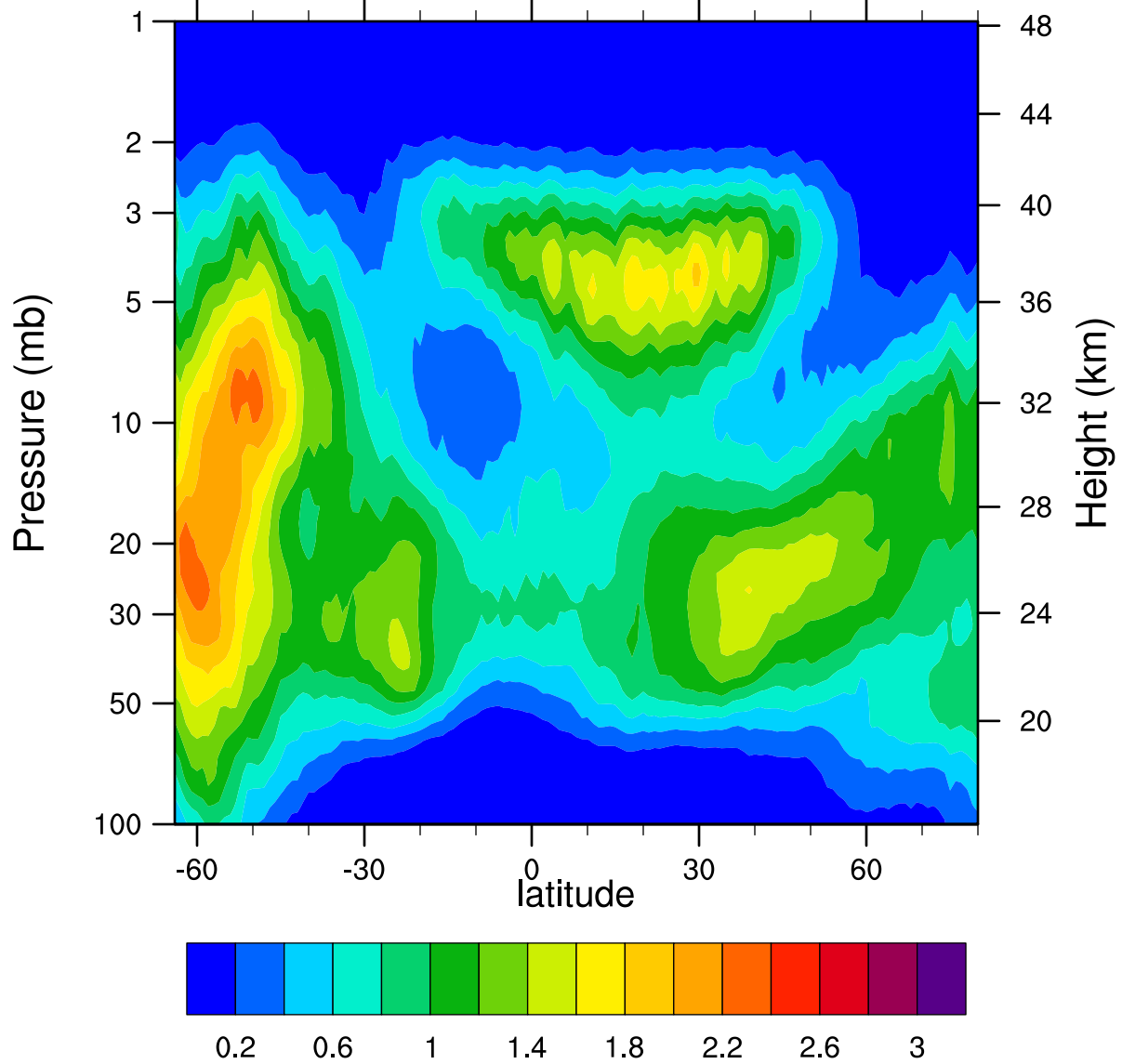
HIRDLSv6 2007d239 ClONO2_Ascending (ppbv)
