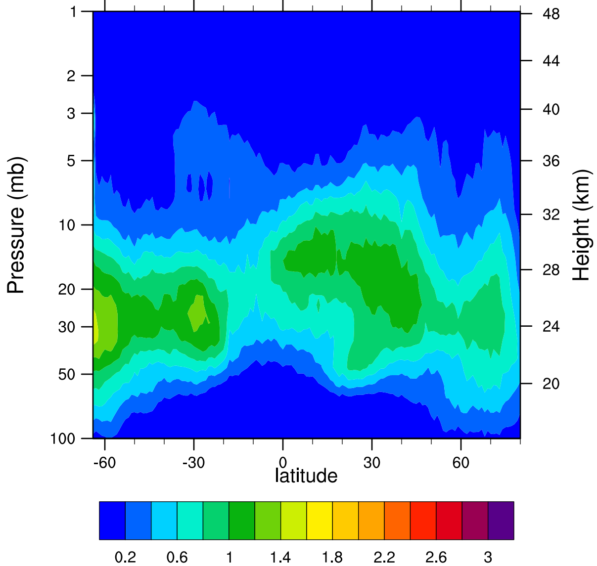
HIRDLSv6 2005d313 ClONO2_Ascending (ppbv)
