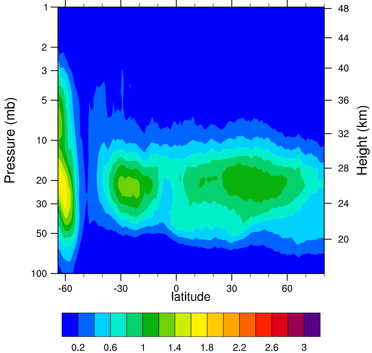
HIRDLSv6 2006d204 ClONO2_Ascending (ppbv)
