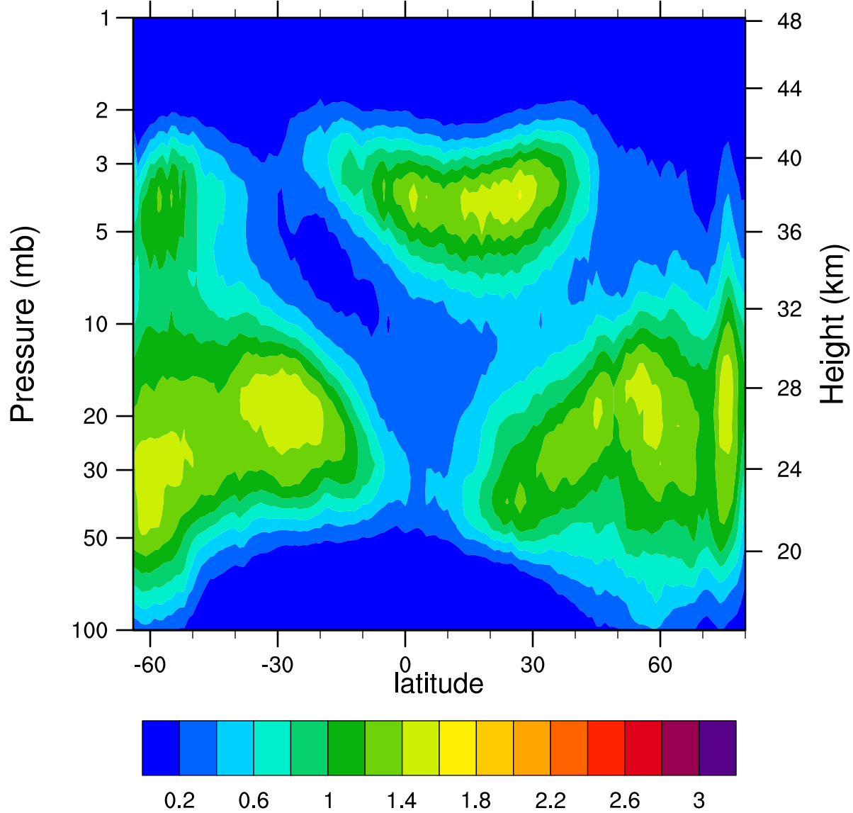
HIRDLSv6 2006d350 ClONO2_Ascending (ppbv)
