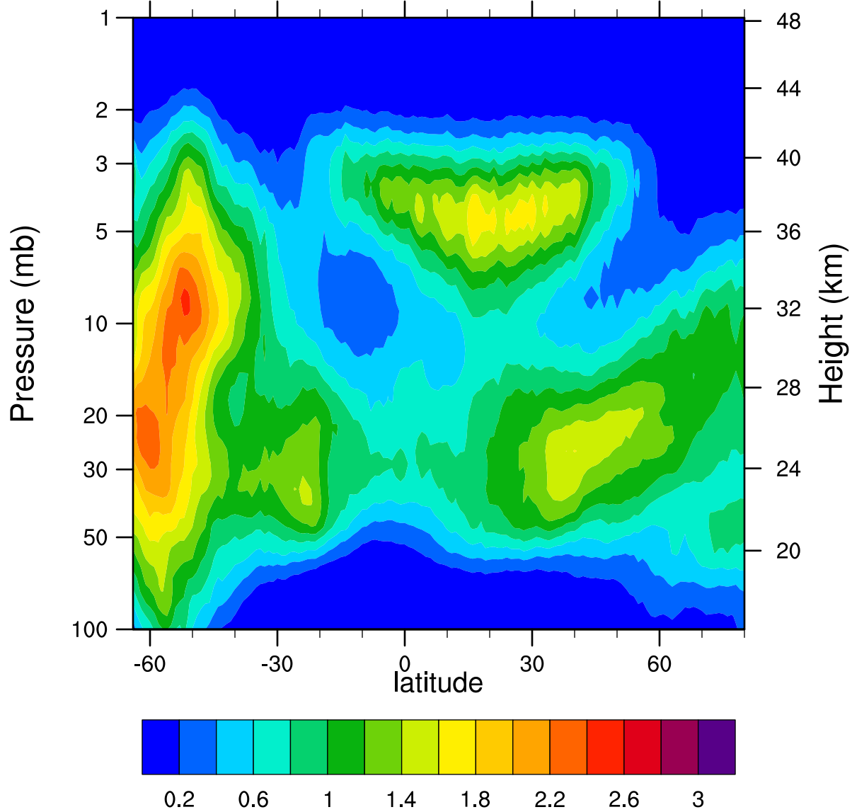
HIRDLSv6 2007d235 ClONO2_Ascending (ppbv)
