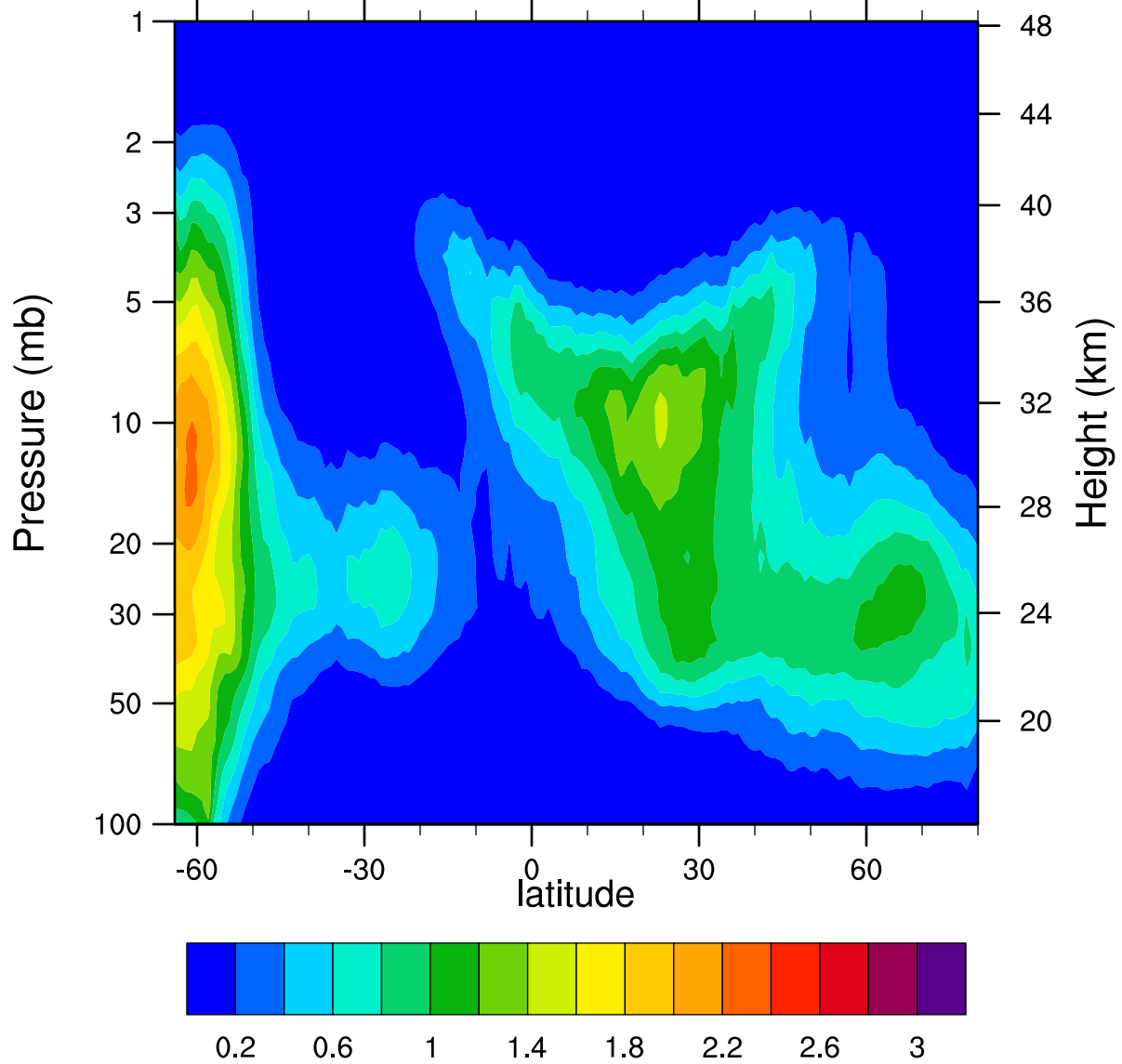
HIRDLSv6 2005d126 ClONO2_Ascending (ppbv)
