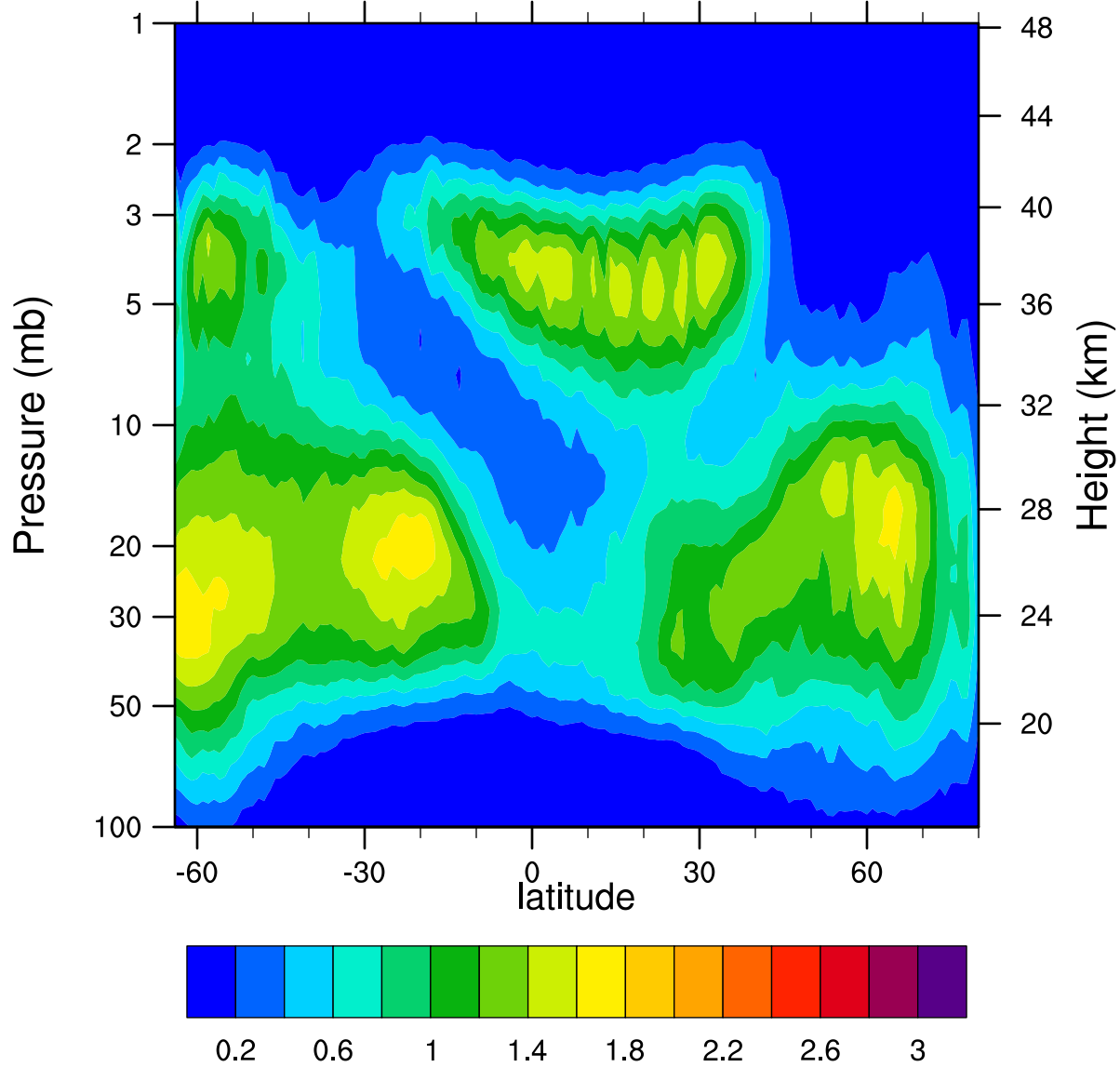
HIRDLSv6 2006d327 ClONO2_Ascending (ppbv)
