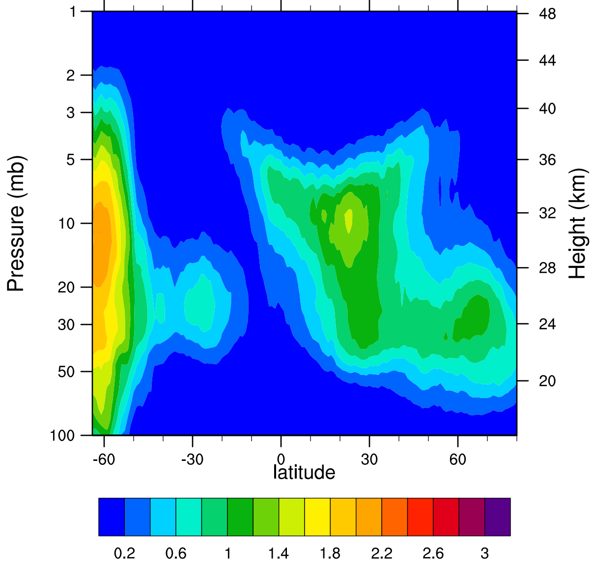
HIRDLSv6 2005d129 ClONO2_Ascending (ppbv)
