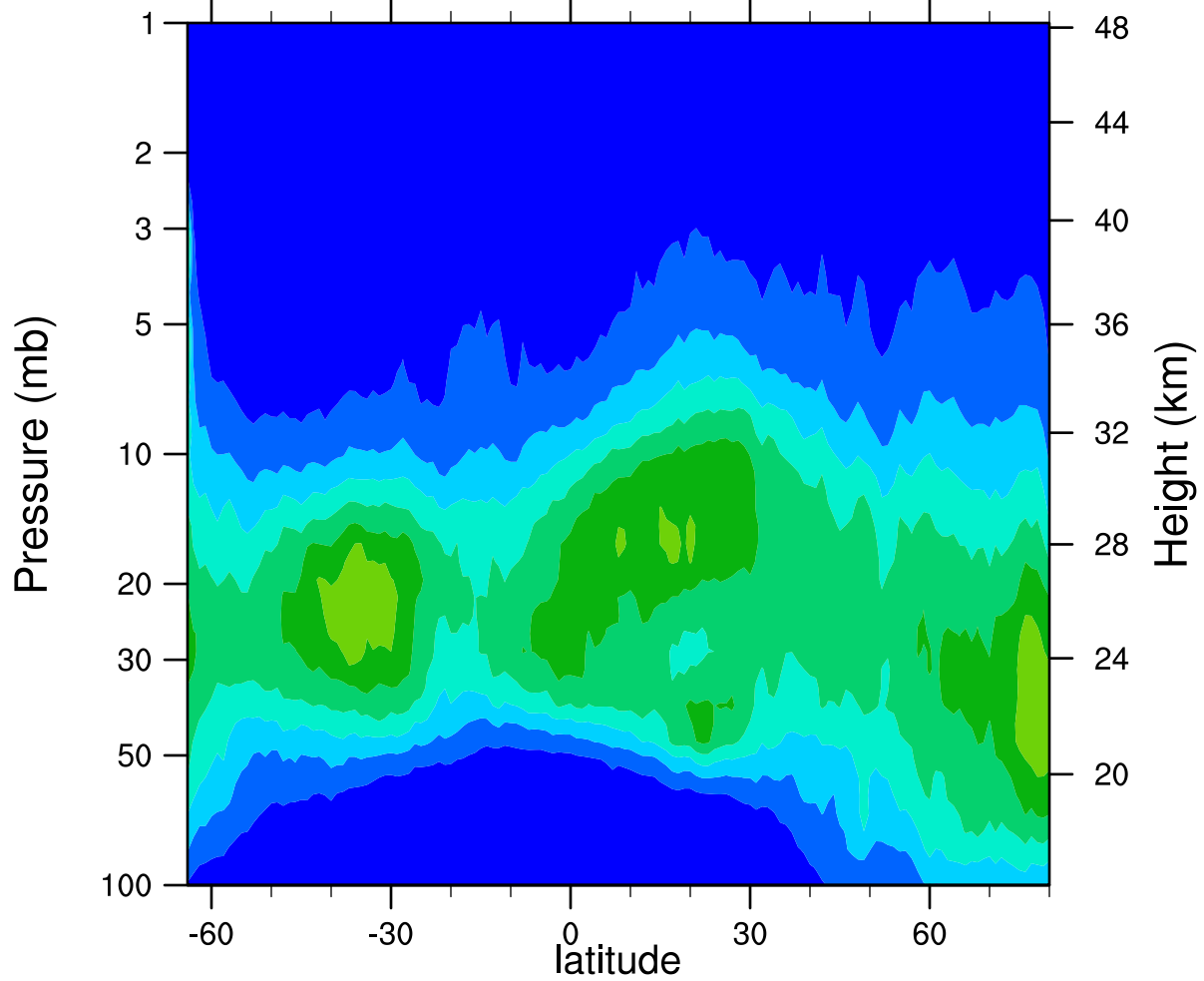
HIRDLSv6 2006d066 ClONO2_Ascending (ppbv)
