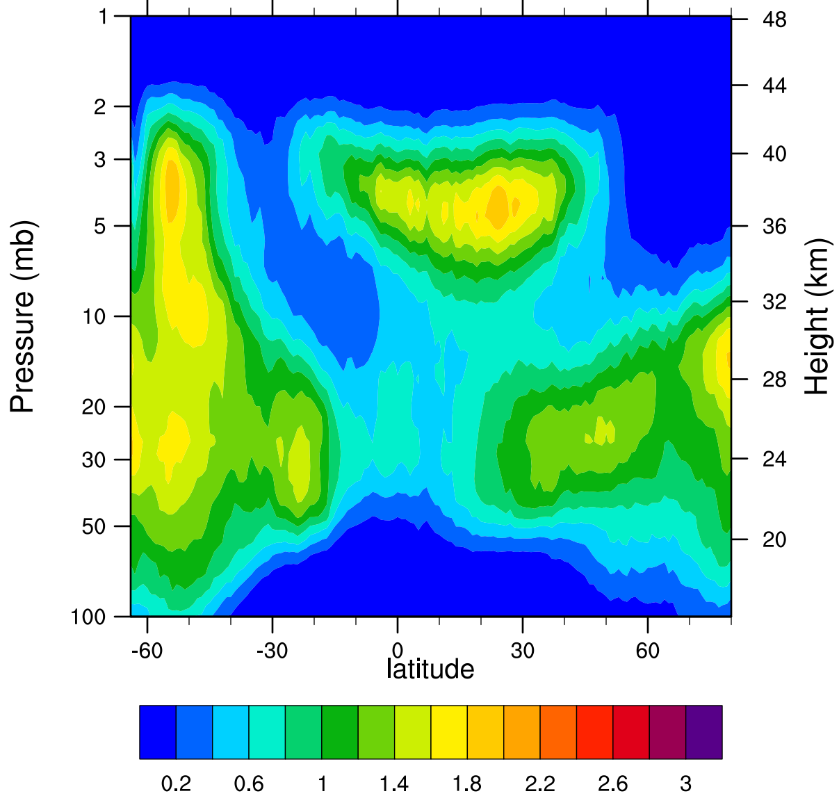
HIRDLSv6 2007d280 ClONO2_Ascending (ppbv)
