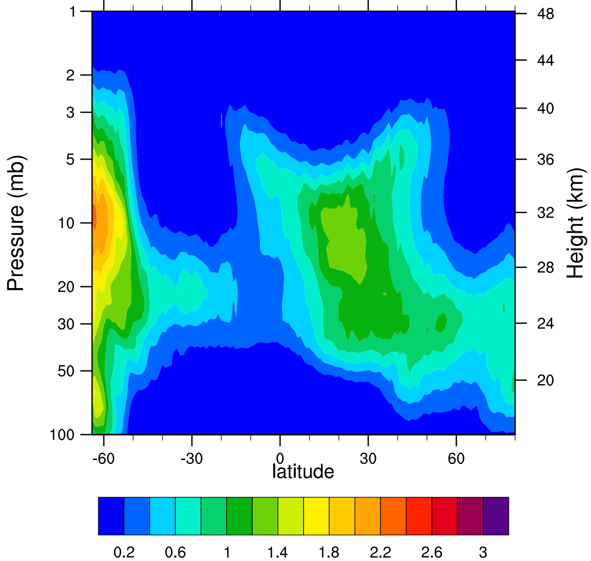
HIRDLSv6 2005d112 ClONO2_Ascending (ppbv)
