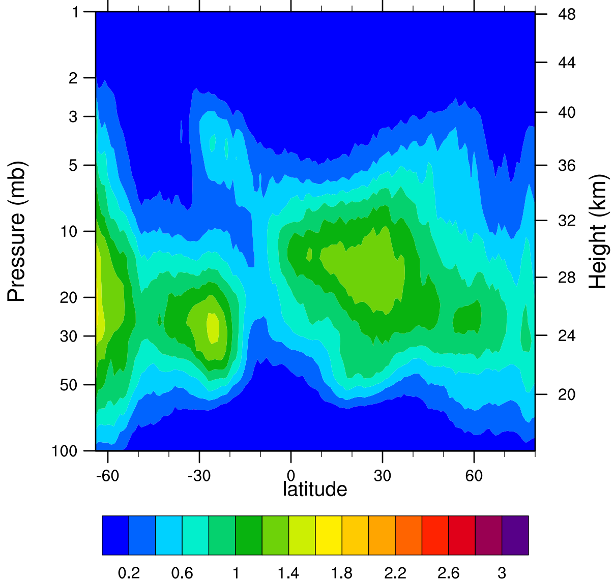
HIRDLSv6 2005d280 ClONO2_Ascending (ppbv)
