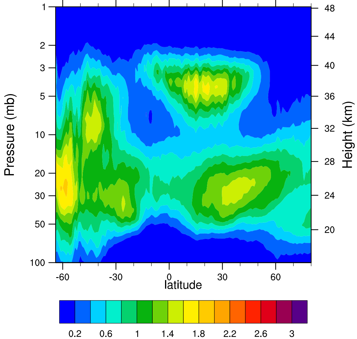
HIRDLSv6 2007d213 ClONO2_Ascending (ppbv)
