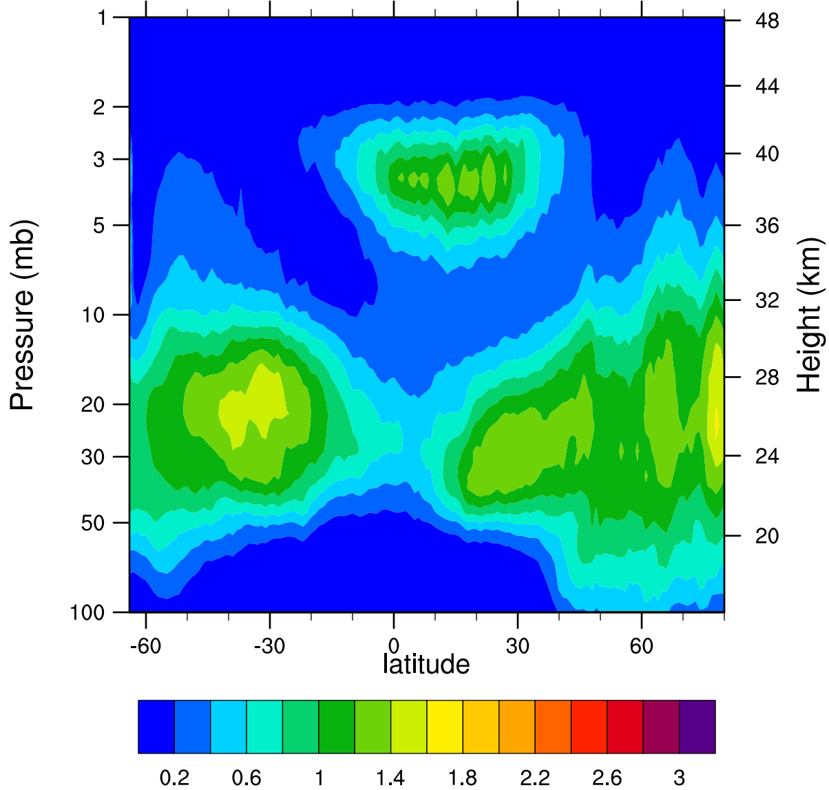
HIRDLSv6 2007d027 ClONO2_Ascending (ppbv)
