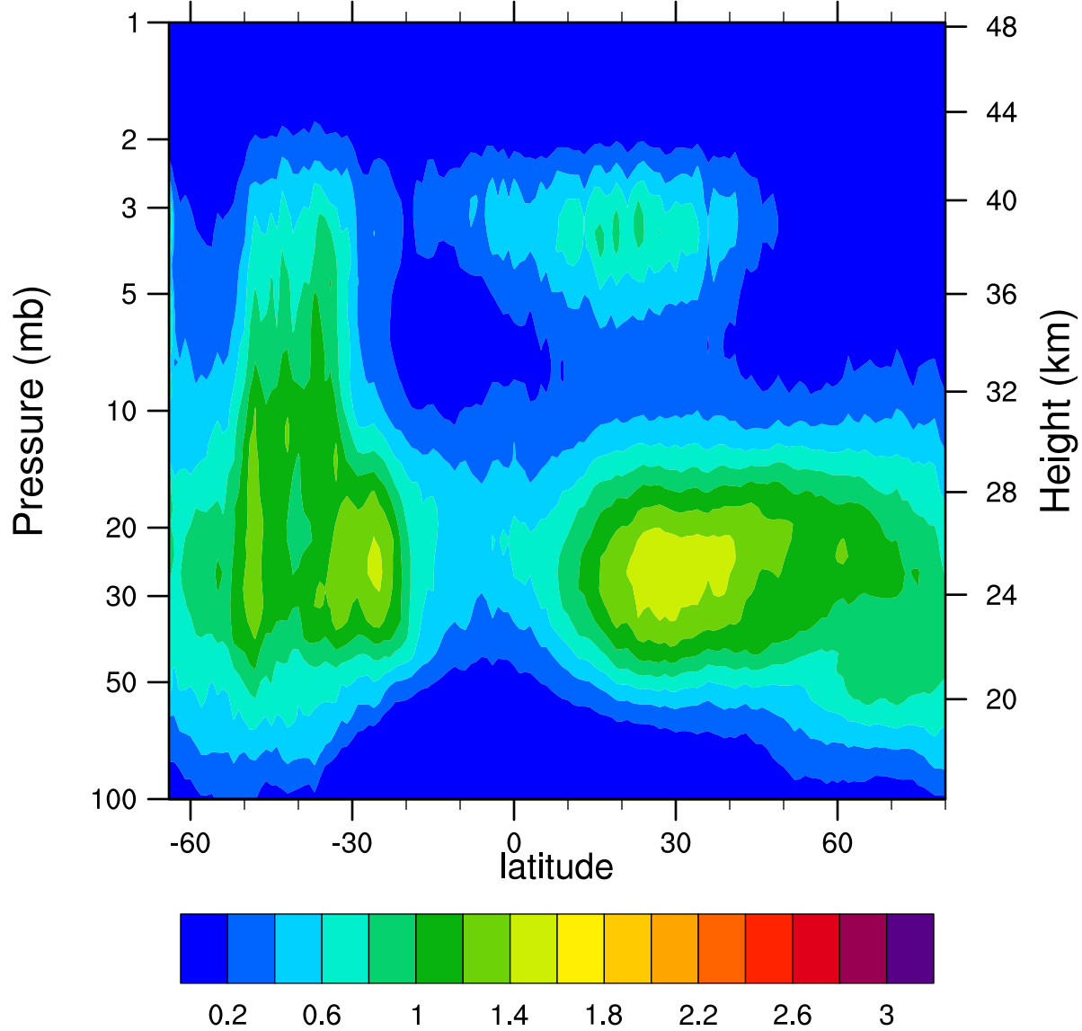
HIRDLSv6 2007d162 ClONO2_Ascending (ppbv)
