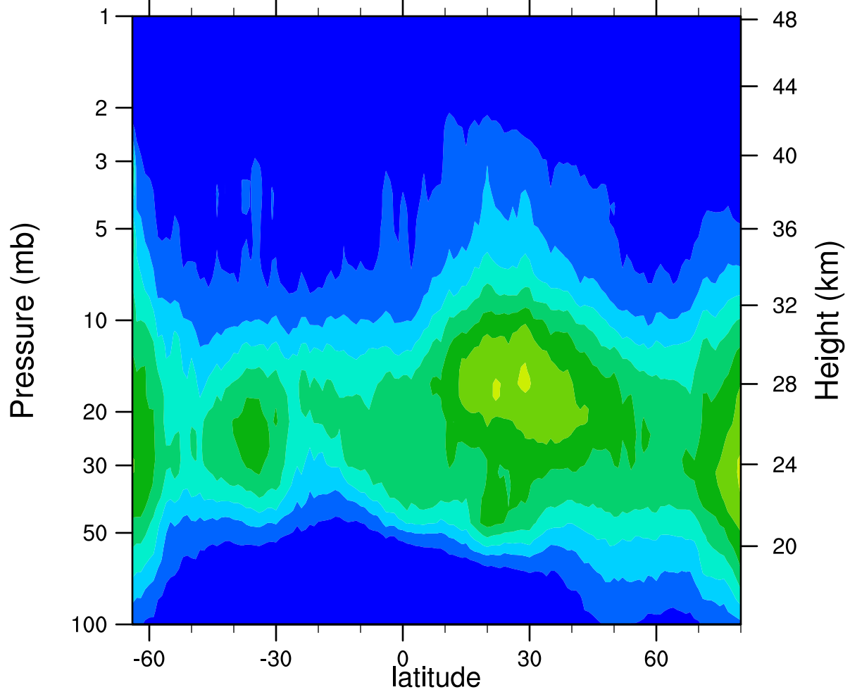
HIRDLSv6 2006d111 ClONO2_Ascending (ppbv)
