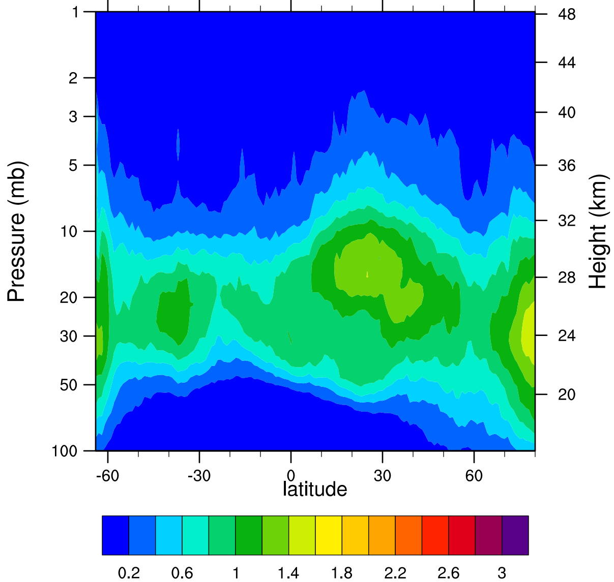
HIRDLSv6 2006d100 ClONO2_Ascending (ppbv)
