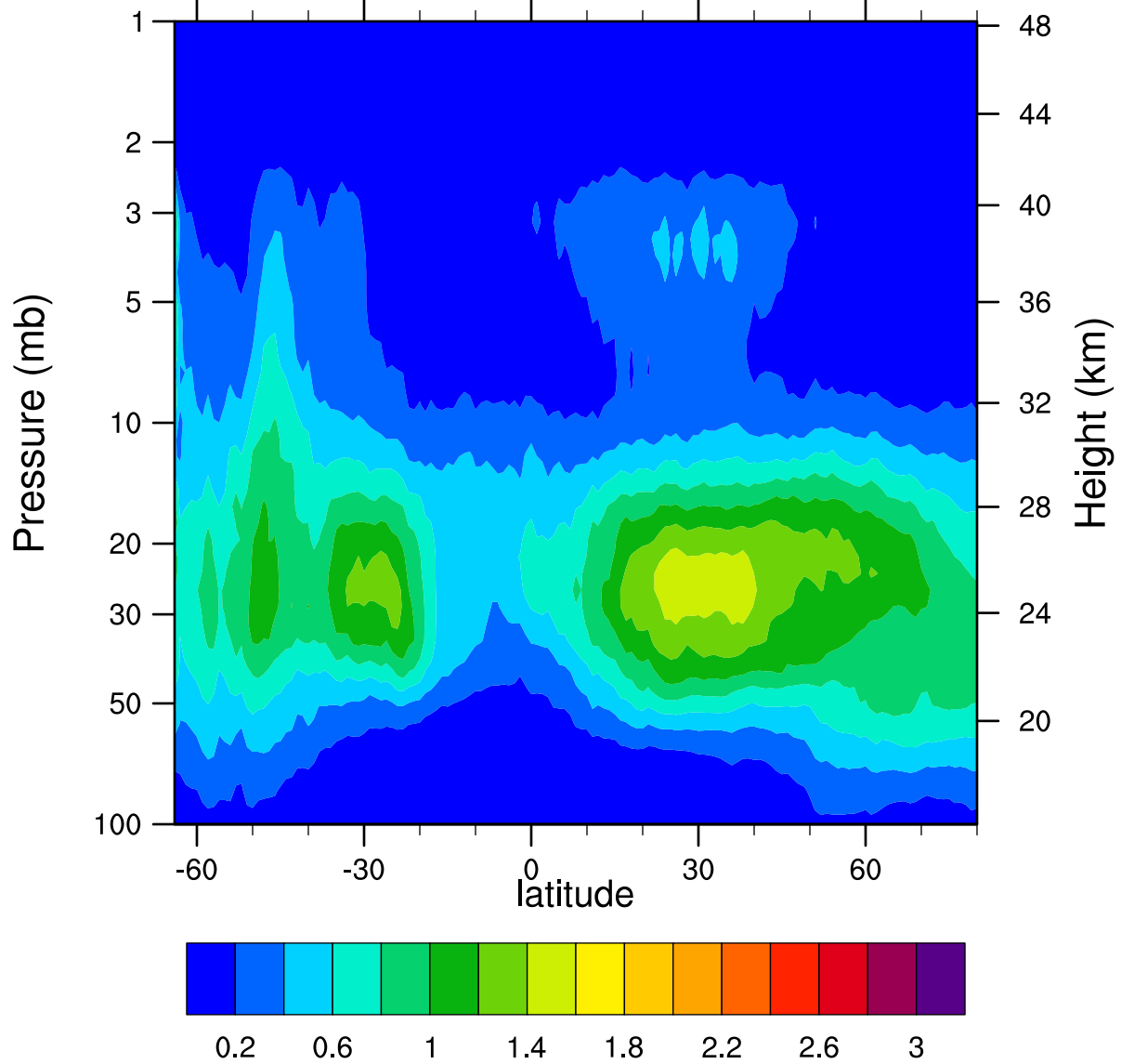
HIRDLSv6 2007d170 ClONO2_Ascending (ppbv)
