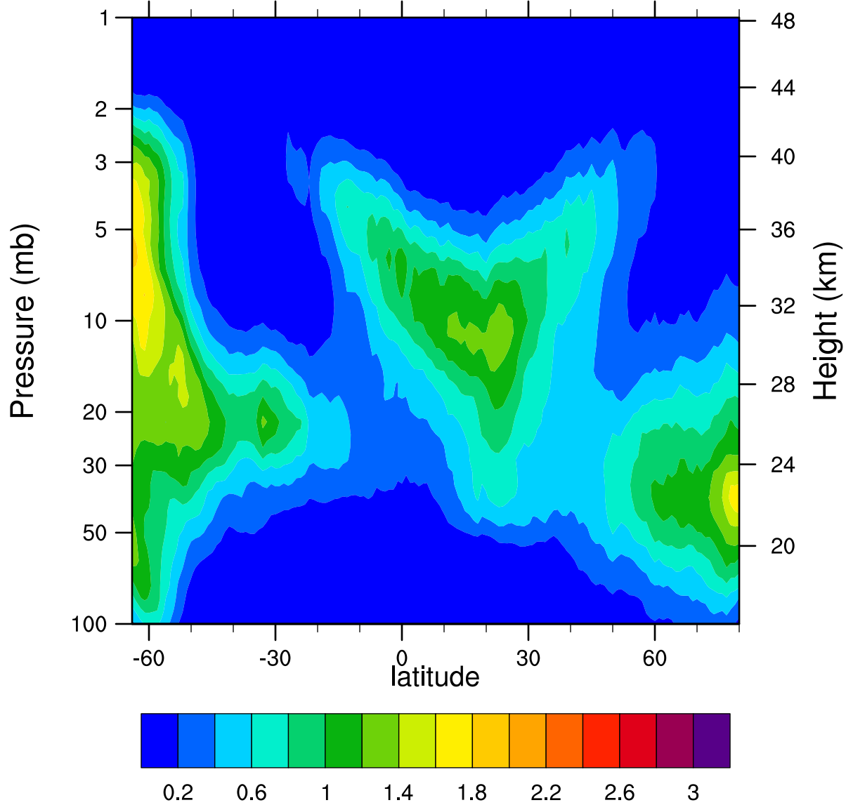
HIRDLSv6 2005d061 ClONO2_Ascending (ppbv)
