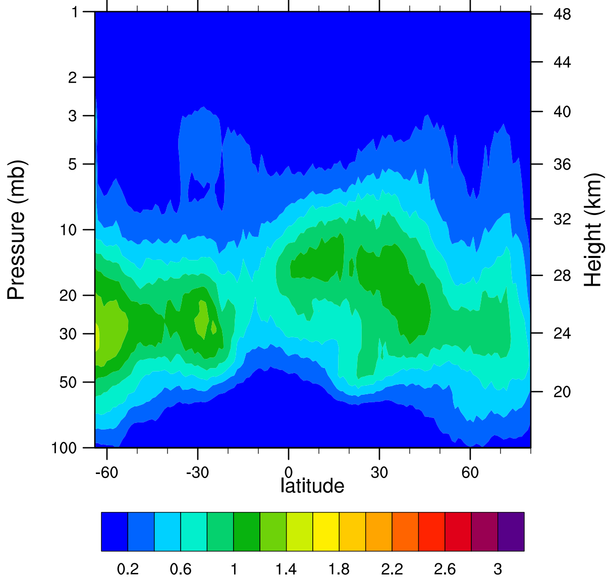
HIRDLSv6 2005d315 ClONO2_Ascending (ppbv)
