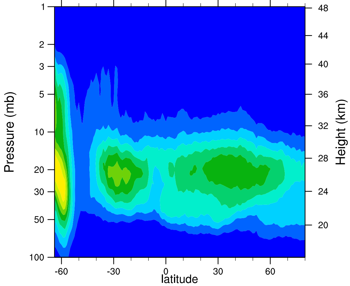
HIRDLSv6 2006d200 ClONO2_Ascending (ppbv)
