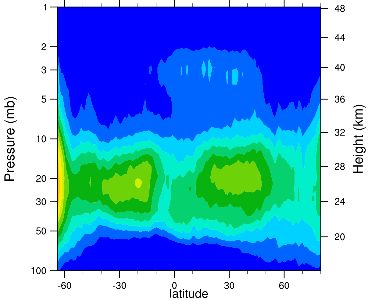
HIRDLSv6 2006d278 ClONO2_Ascending (ppbv)
