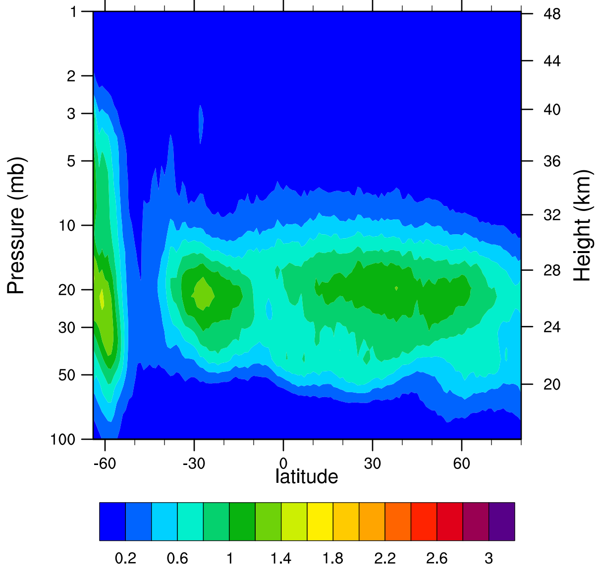
HIRDLSv6 2006d190 ClONO2_Ascending (ppbv)
