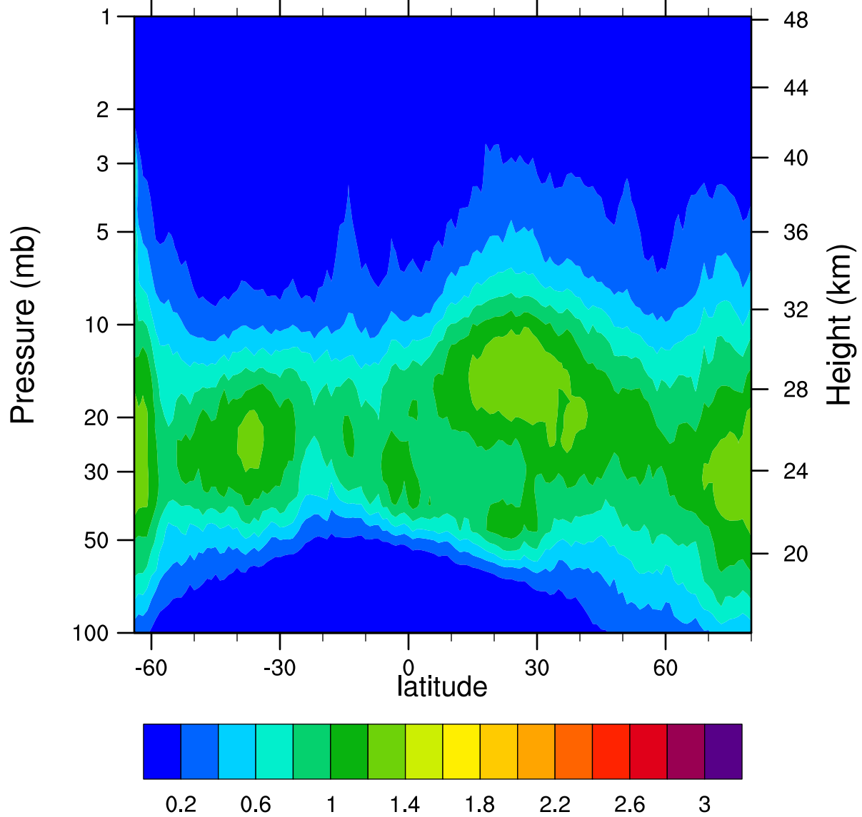
HIRDLSv6 2006d096 ClONO2_Ascending (ppbv)
