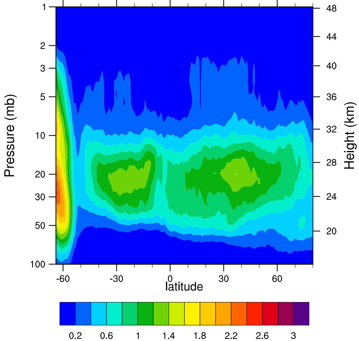
HIRDLSv6 2006d243 ClONO2_Ascending (ppbv)
