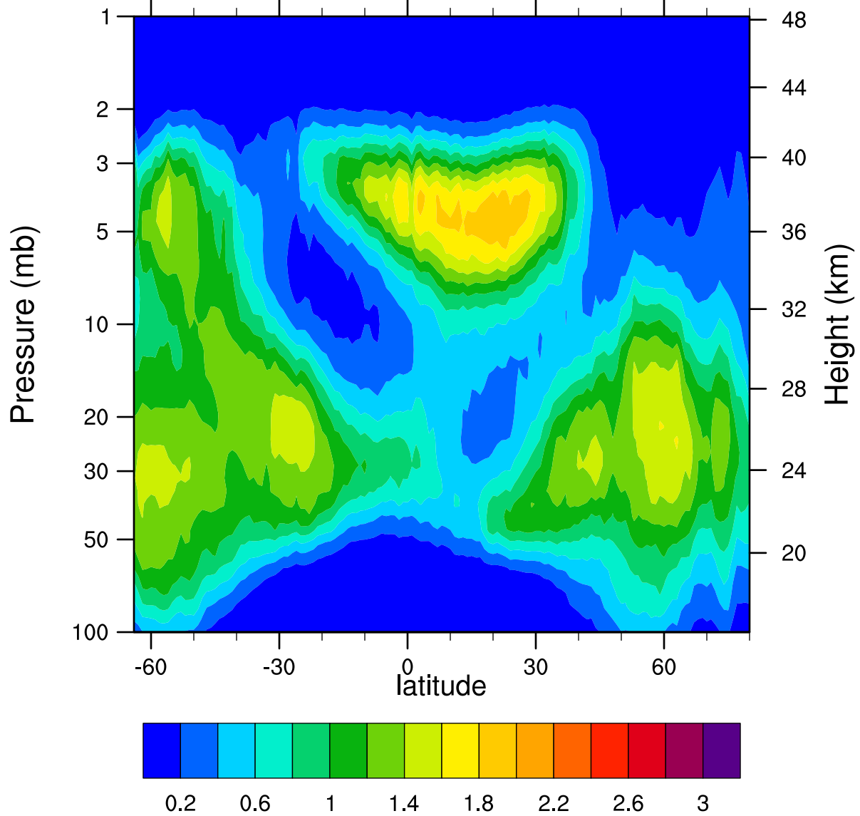
HIRDLSv6 2007d341 ClONO2_Ascending (ppbv)
