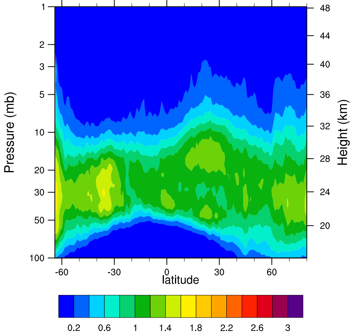
HIRDLSv6 2006d088 ClONO2_Ascending (ppbv)
