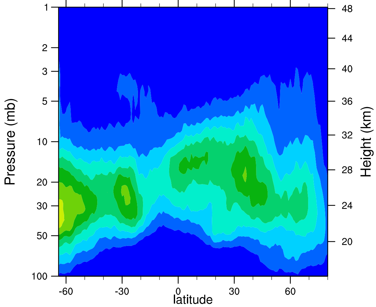
HIRDLSv6 2005d321 ClONO2_Ascending (ppbv)
