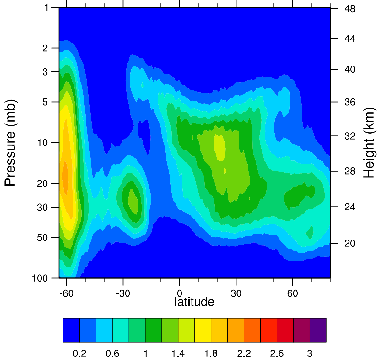
HIRDLSv6 2005d181 ClONO2_Ascending (ppbv)
