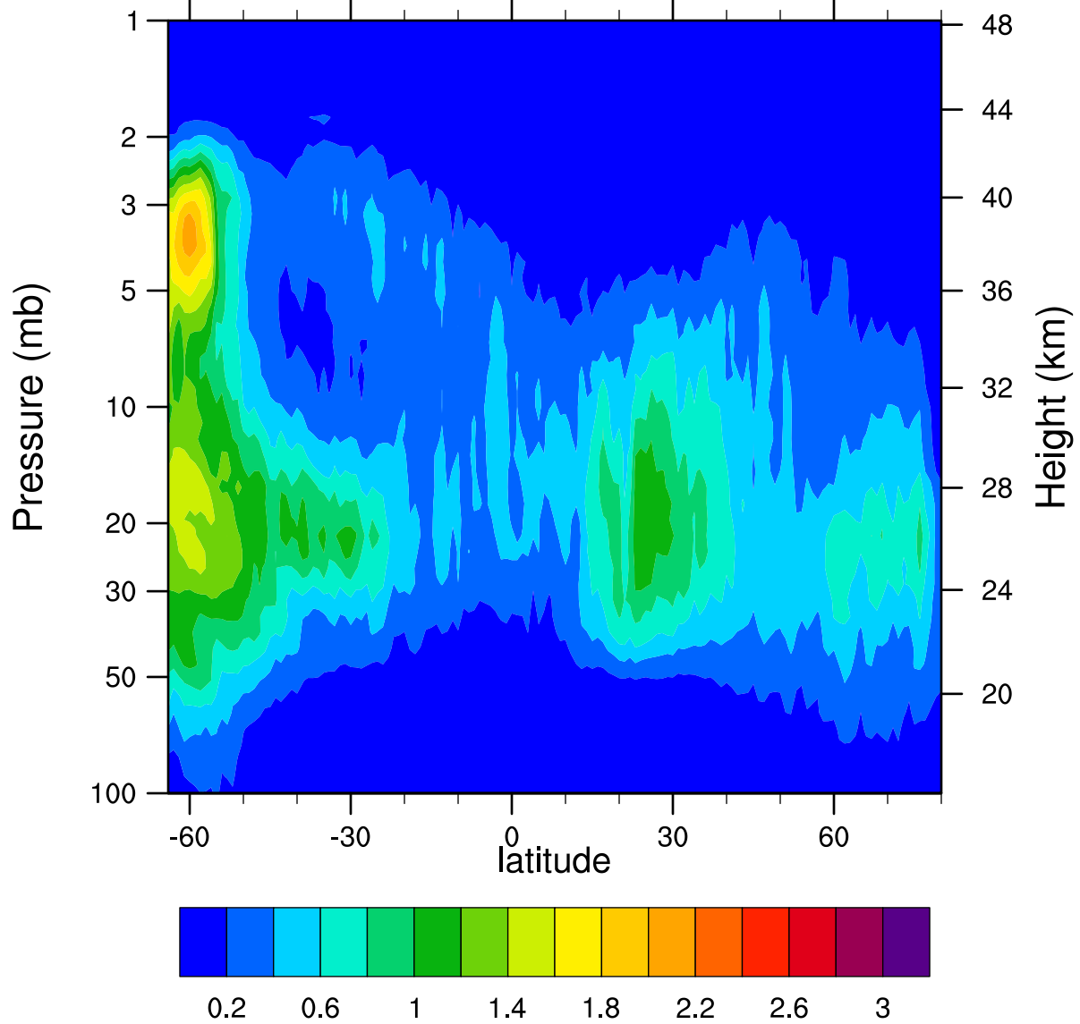
HIRDLSv6 2005d026 ClONO2_Ascending (ppbv)
