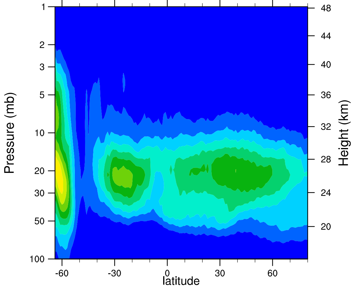
HIRDLSv6 2006d205 ClONO2_Ascending (ppbv)
