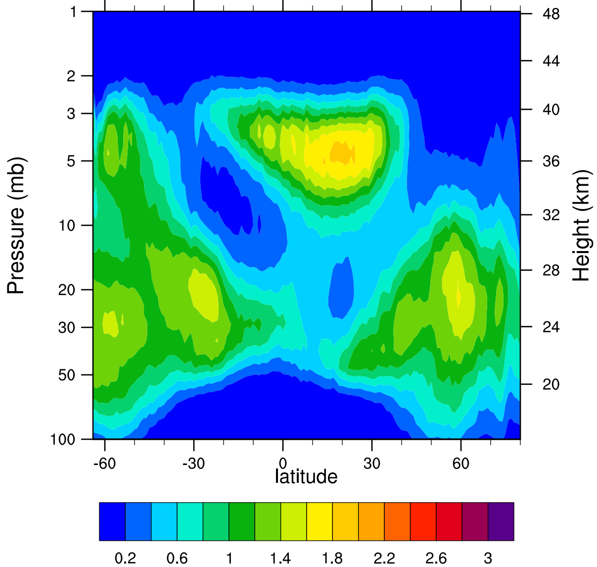
HIRDLSv6 2007d349 ClONO2_Ascending (ppbv)
