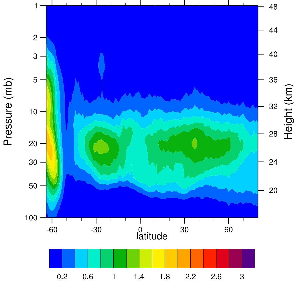
HIRDLSv6 2006d218 ClONO2_Ascending (ppbv)
