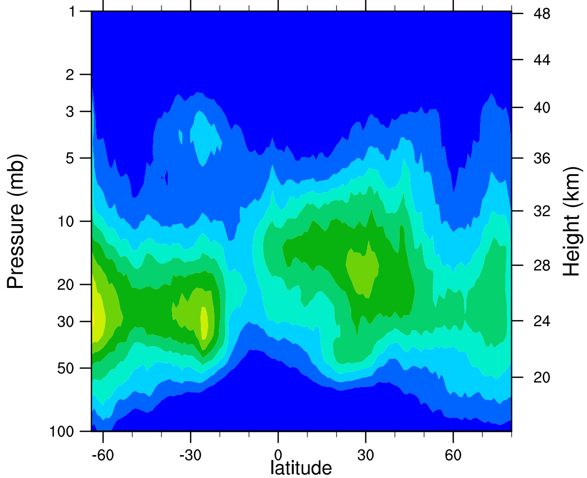
HIRDLSv6 2005d299 ClONO2_Ascending (ppbv)
