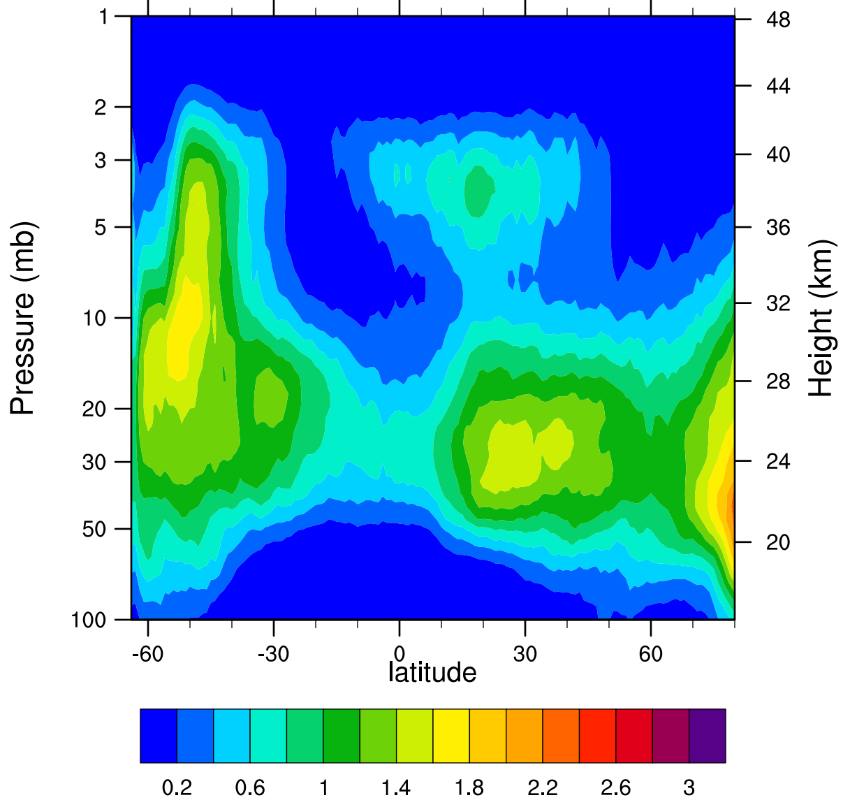
HIRDLSv6 2007d105 ClONO2_Ascending (ppbv)
