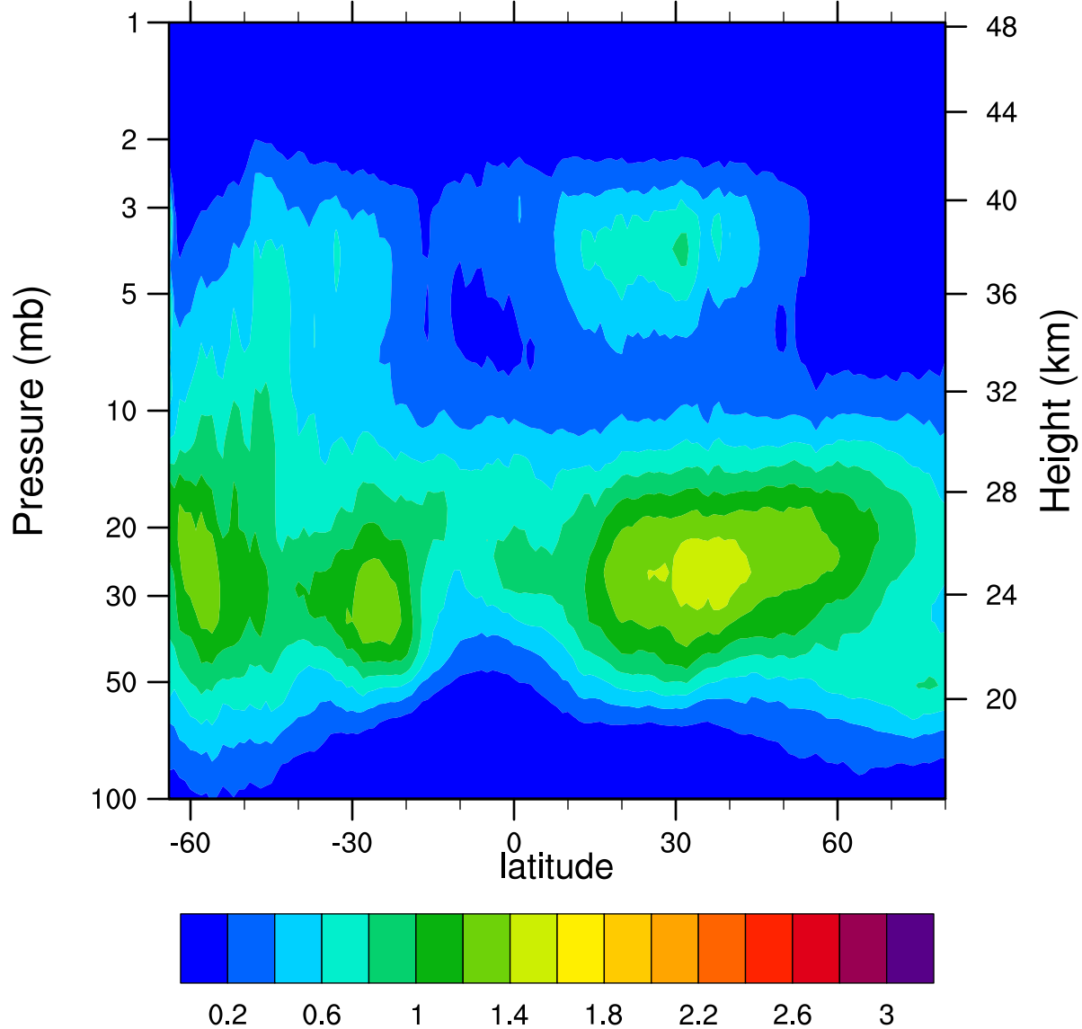
HIRDLSv6 2007d200 ClONO2_Ascending (ppbv)
