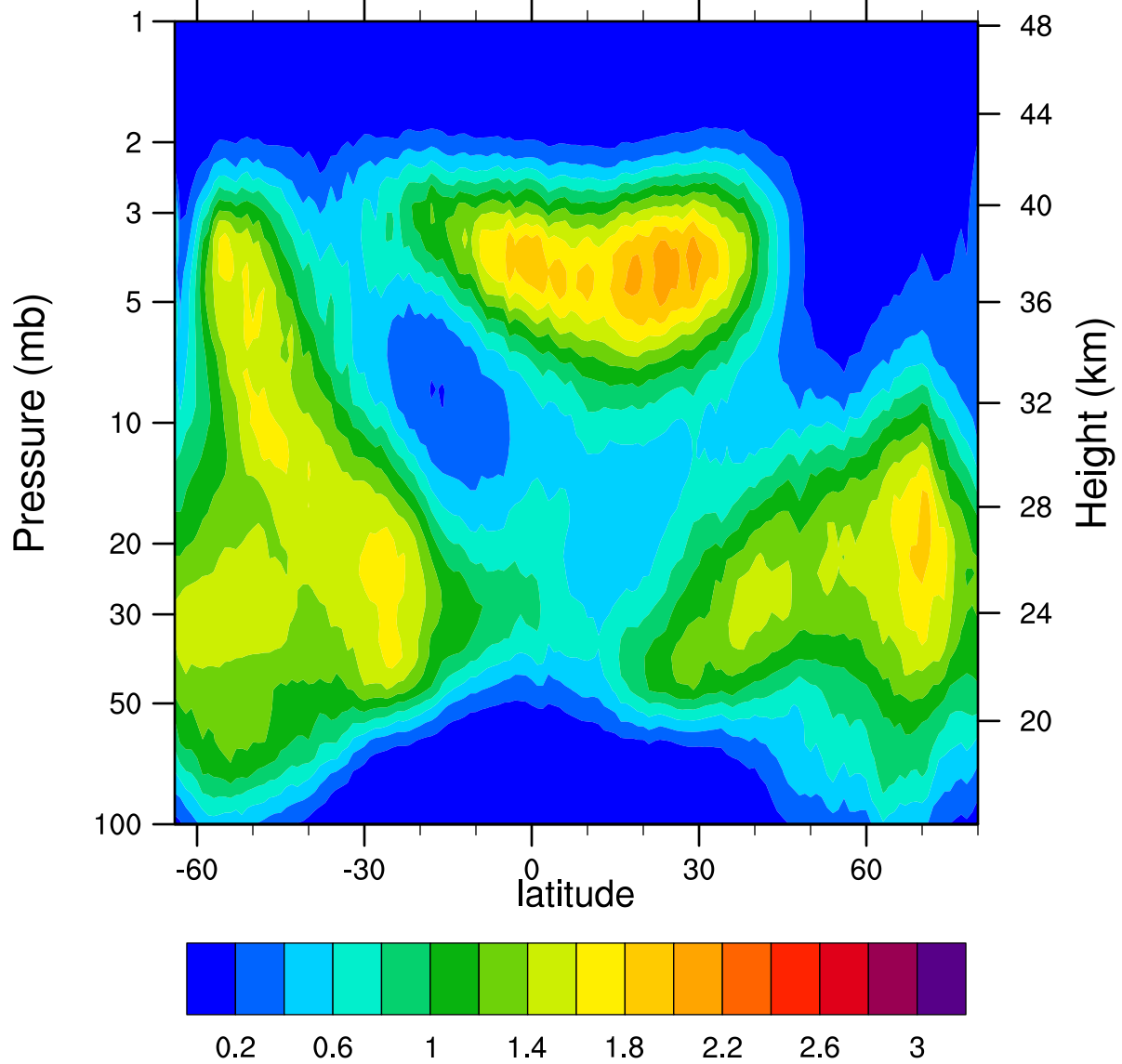
HIRDLSv6 2007d317 ClONO2_Ascending (ppbv)
