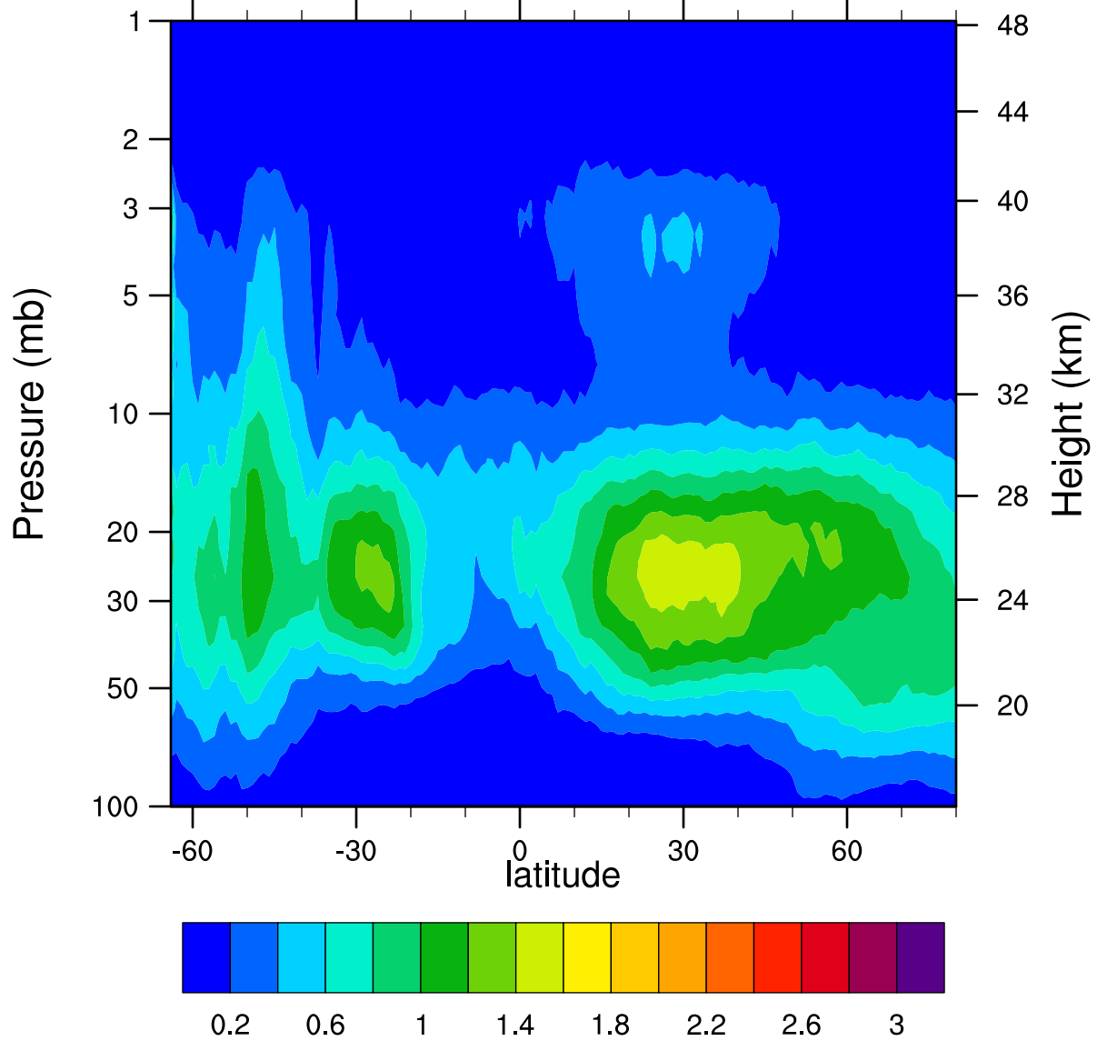
HIRDLSv6 2007d168 ClONO2_Ascending (ppbv)
