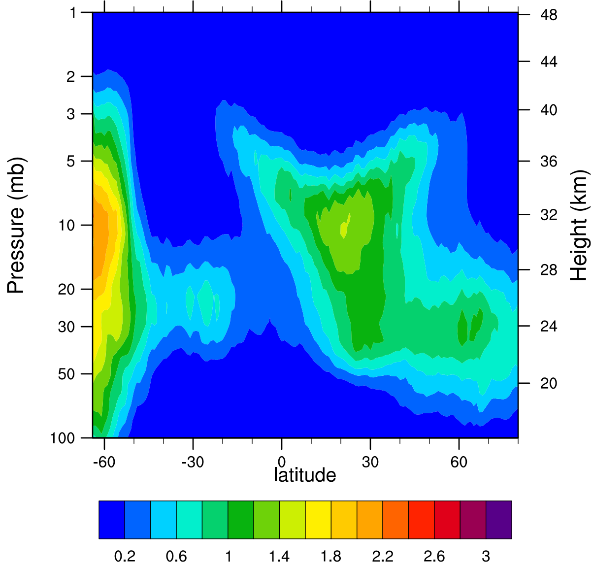
HIRDLSv6 2005d120 ClONO2_Ascending (ppbv)
