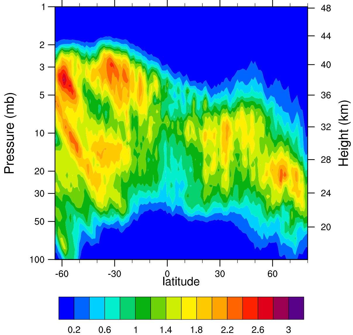
HIRDLSv6 2005d023 ClONO2_Ascending (ppbv)
