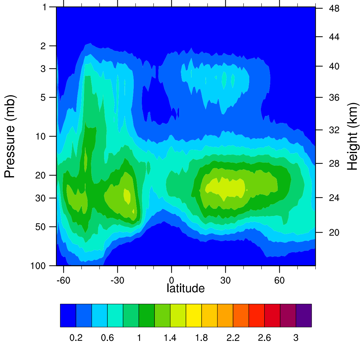
HIRDLSv6 2007d191 ClONO2_Ascending (ppbv)
