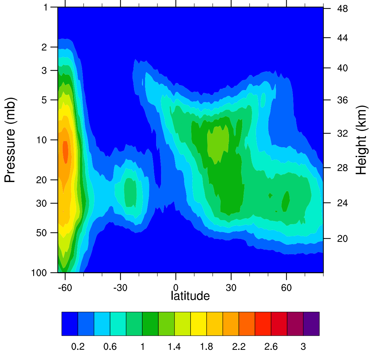
HIRDLSv6 2005d151 ClONO2_Ascending (ppbv)
