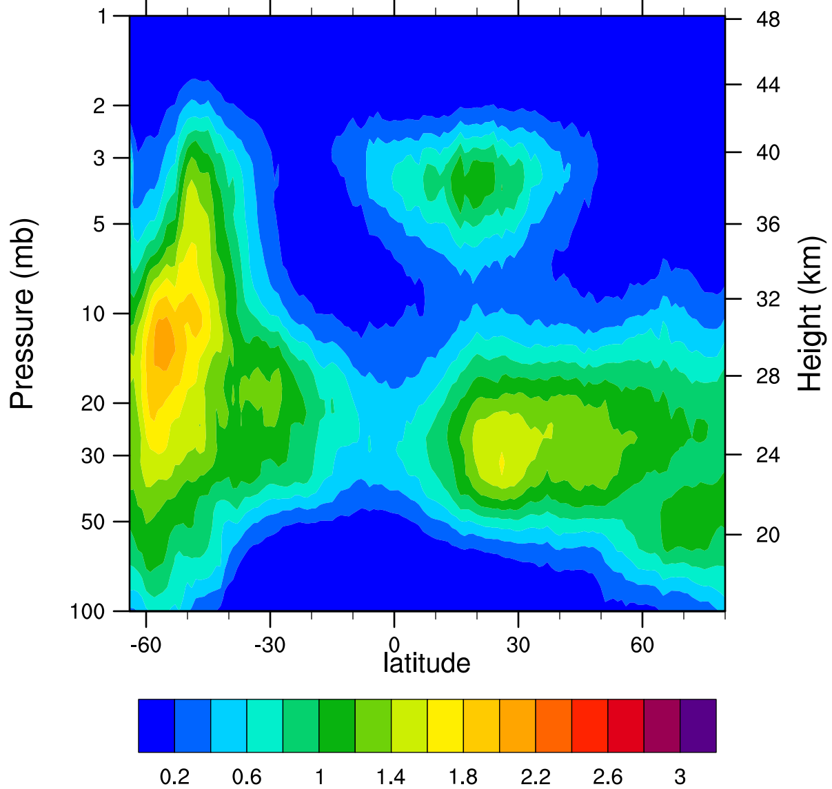
HIRDLSv6 2007d128 ClONO2_Ascending (ppbv)
