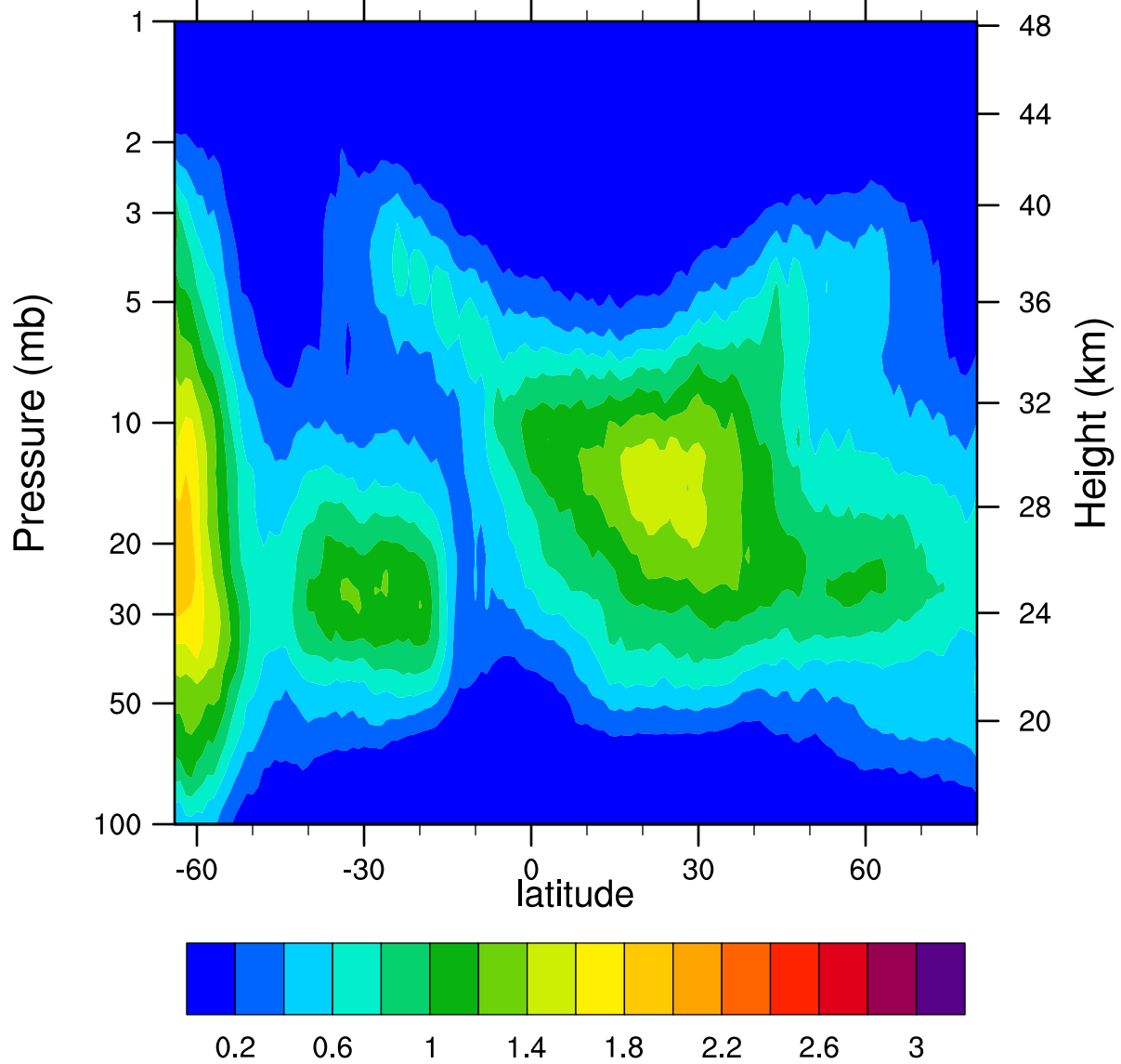
HIRDLSv6 2005d250 ClONO2_Ascending (ppbv)
