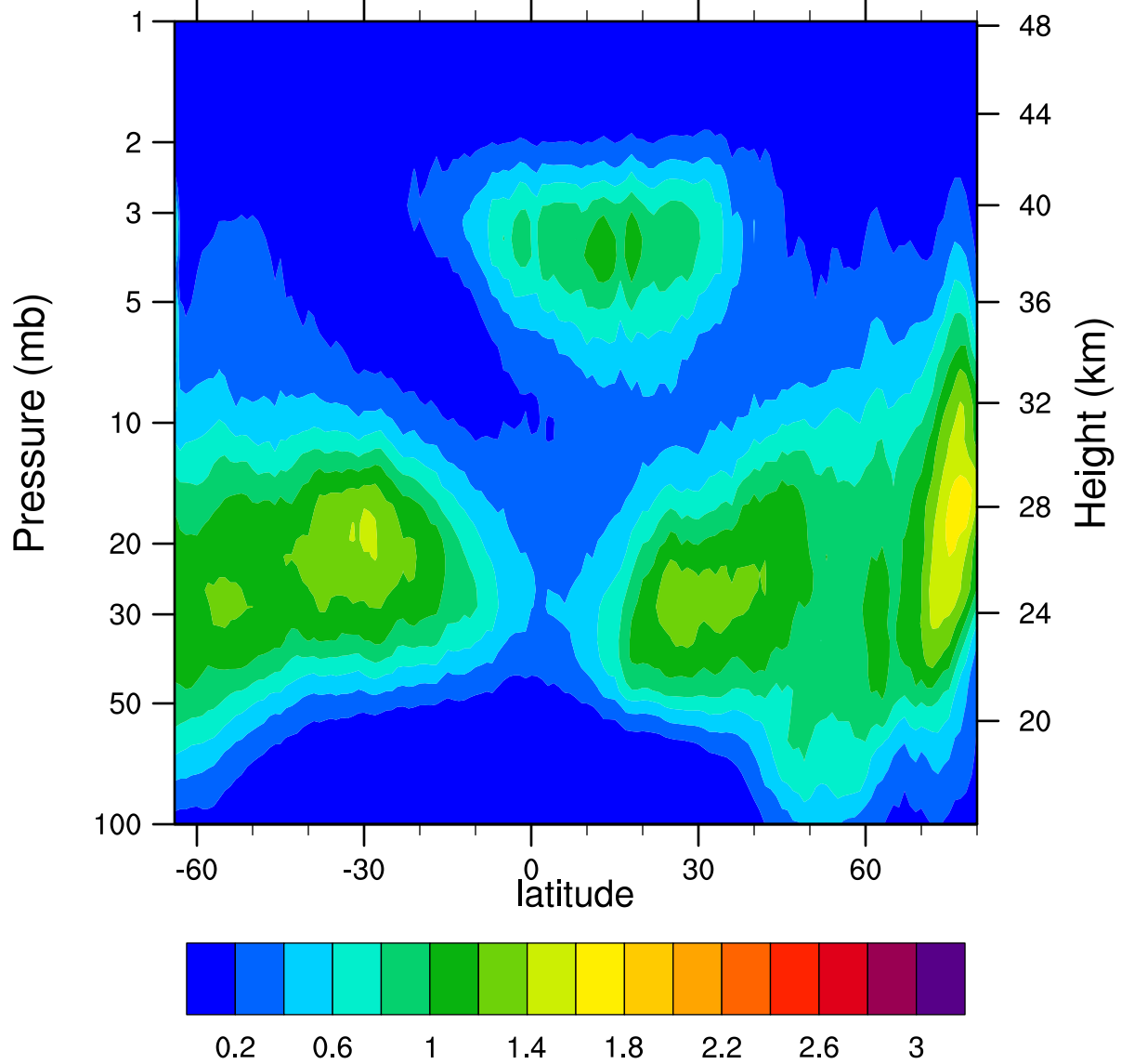
HIRDLSv6 2007d003 ClONO2_Ascending (ppbv)
