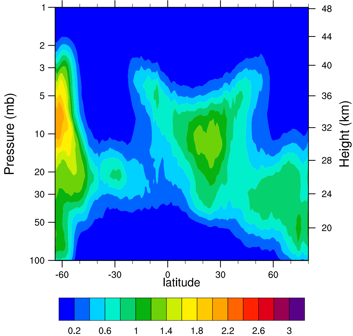
HIRDLSv6 2005d085 ClONO2_Ascending (ppbv)
