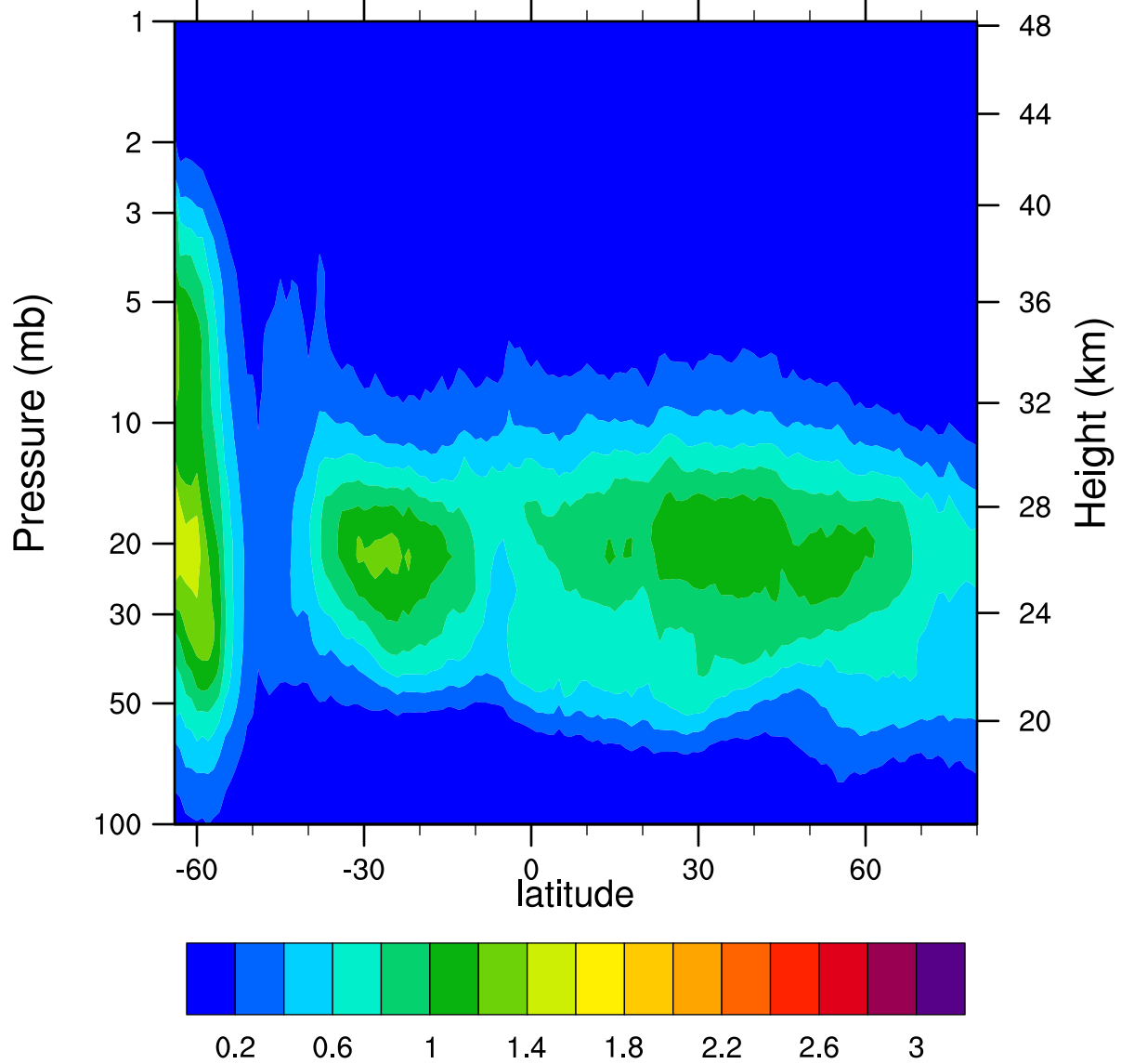
HIRDLSv6 2006d194 ClONO2_Ascending (ppbv)
