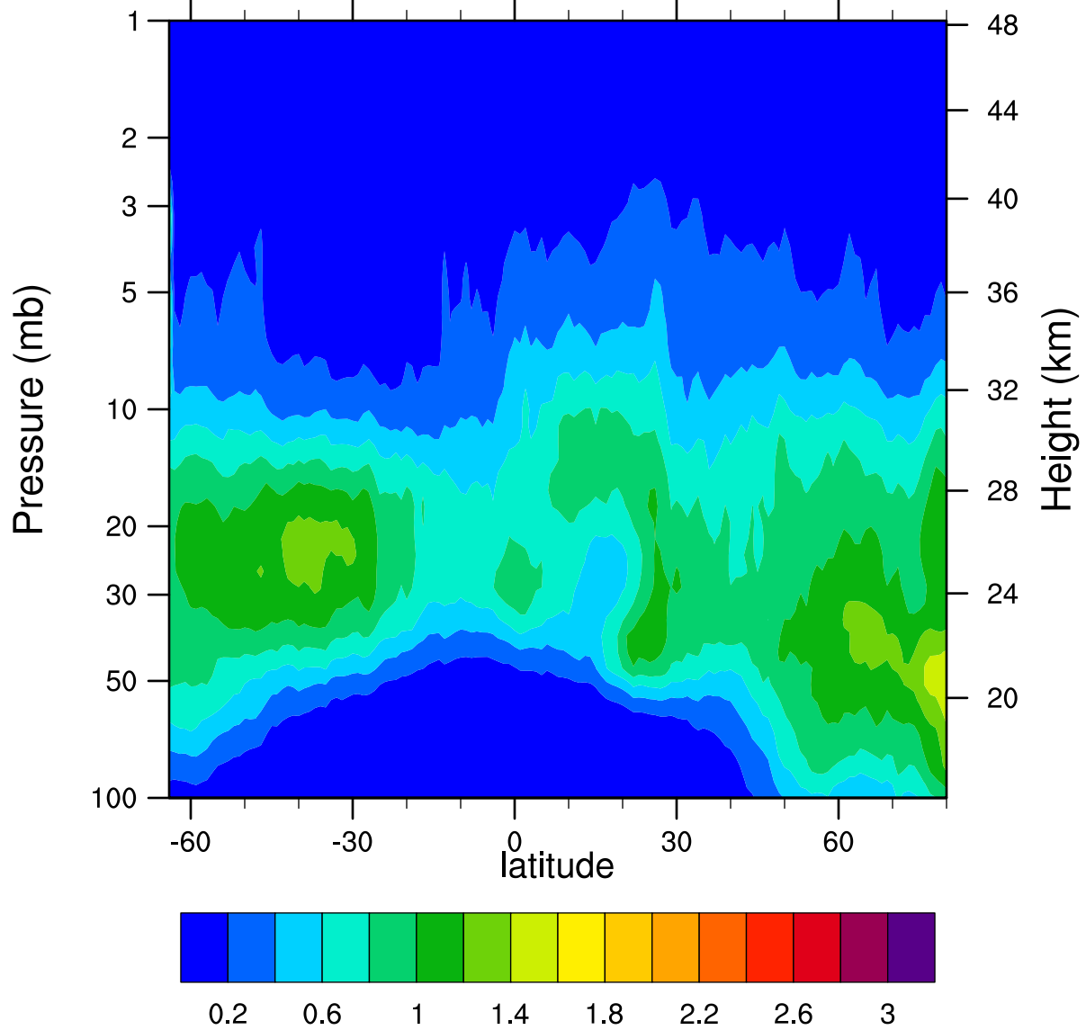
HIRDLSv6 2006d029 ClONO2_Ascending (ppbv)
