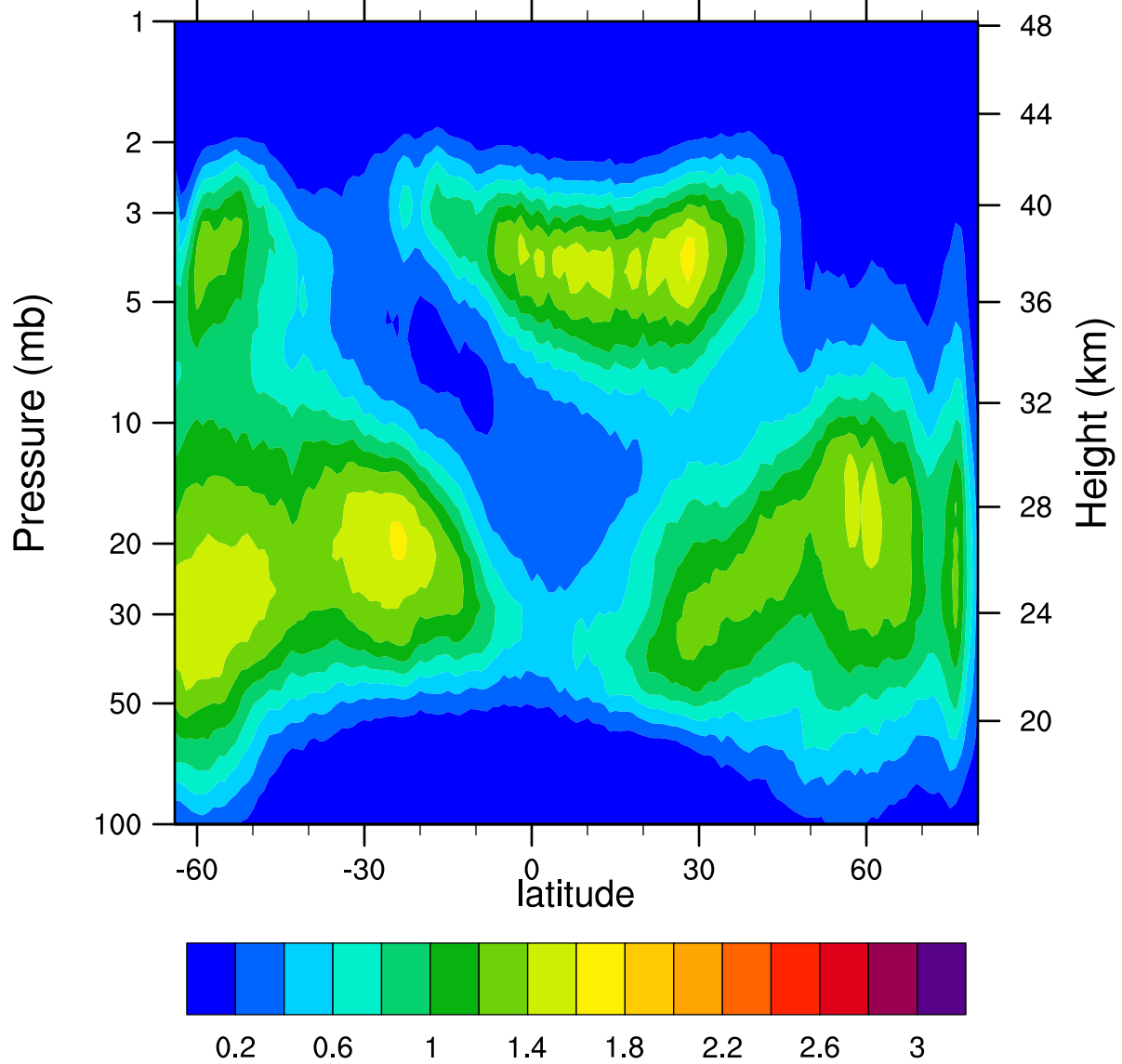
HIRDLSv6 2006d342 ClONO2_Ascending (ppbv)
