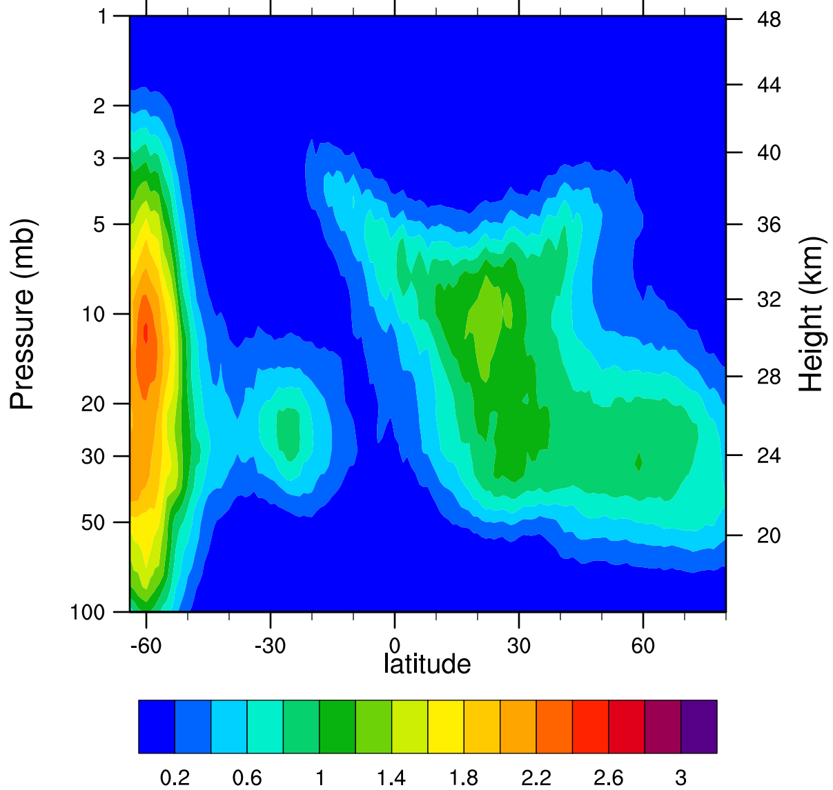
HIRDLSv6 2005d146 ClONO2_Ascending (ppbv)
