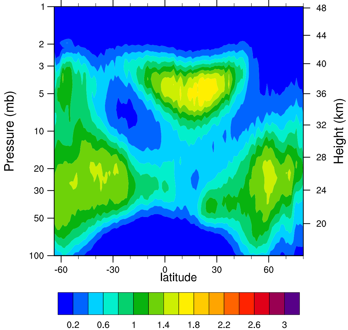
HIRDLSv6 2007d364 ClONO2_Ascending (ppbv)
