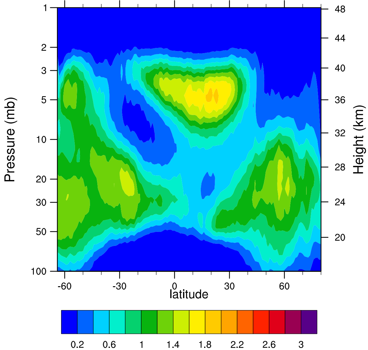
HIRDLSv6 2007d352 ClONO2_Ascending (ppbv)
