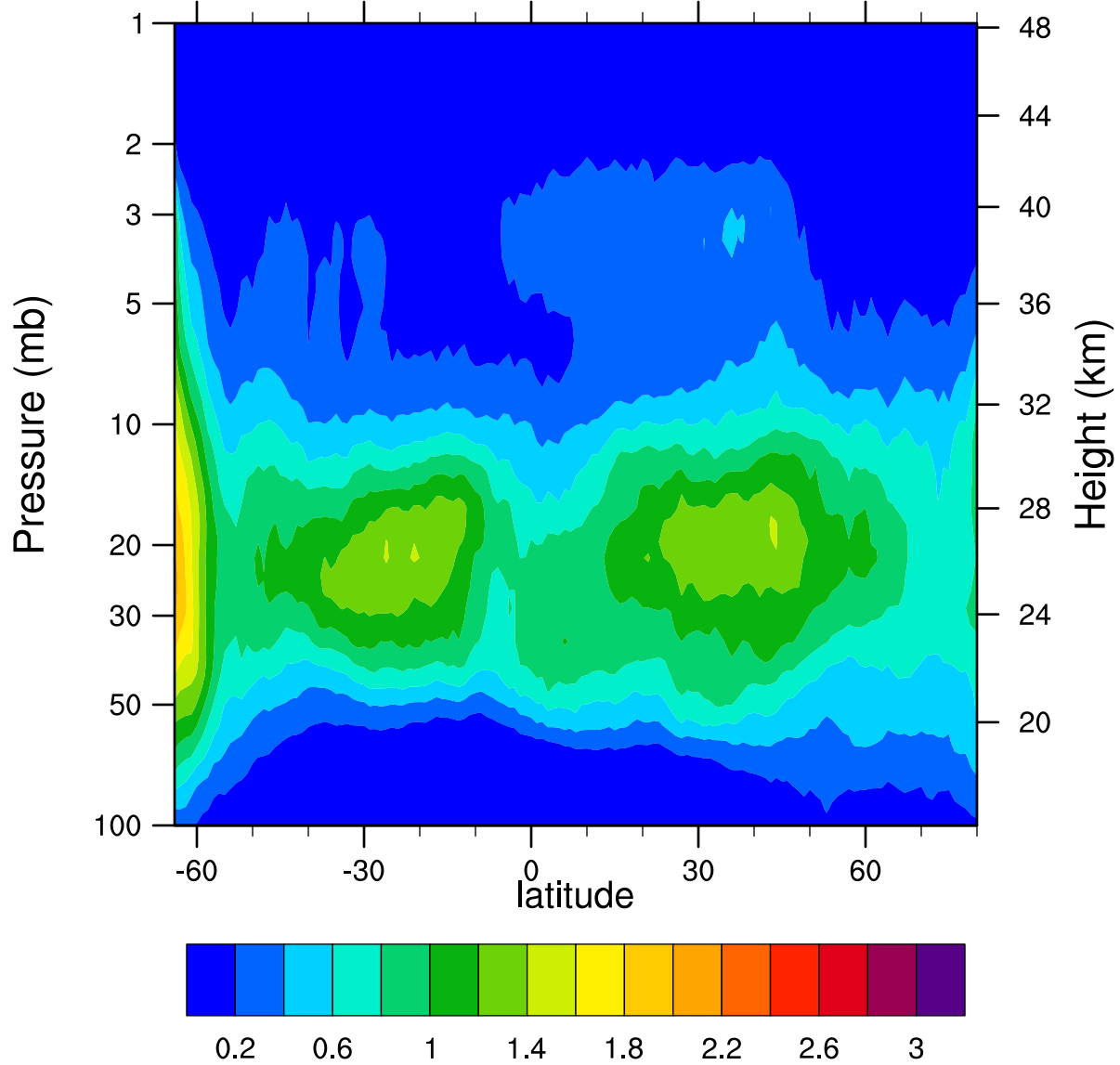
HIRDLSv6 2006d268 ClONO2_Ascending (ppbv)
