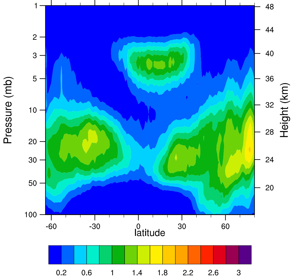
HIRDLSv6 2007d018 ClONO2_Ascending (ppbv)
