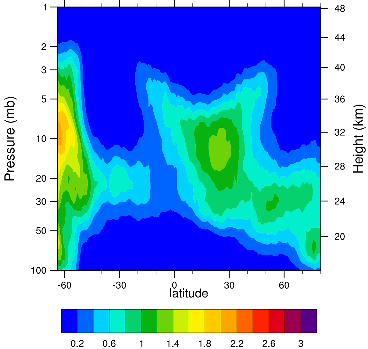
HIRDLSv6 2005d098 ClONO2_Ascending (ppbv)
