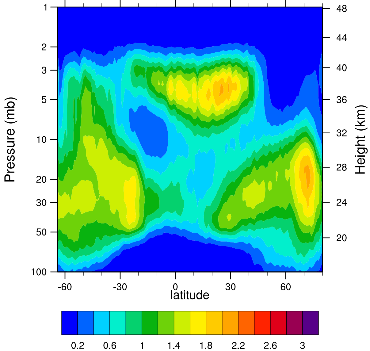
HIRDLSv6 2007d312 ClONO2_Ascending (ppbv)
