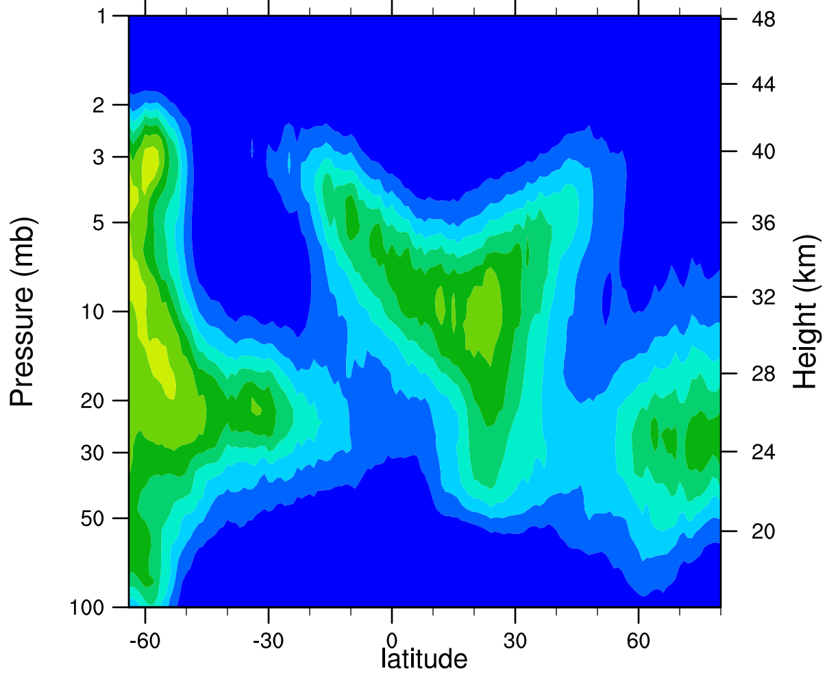
HIRDLSv6 2005d043 ClONO2_Ascending (ppbv)
