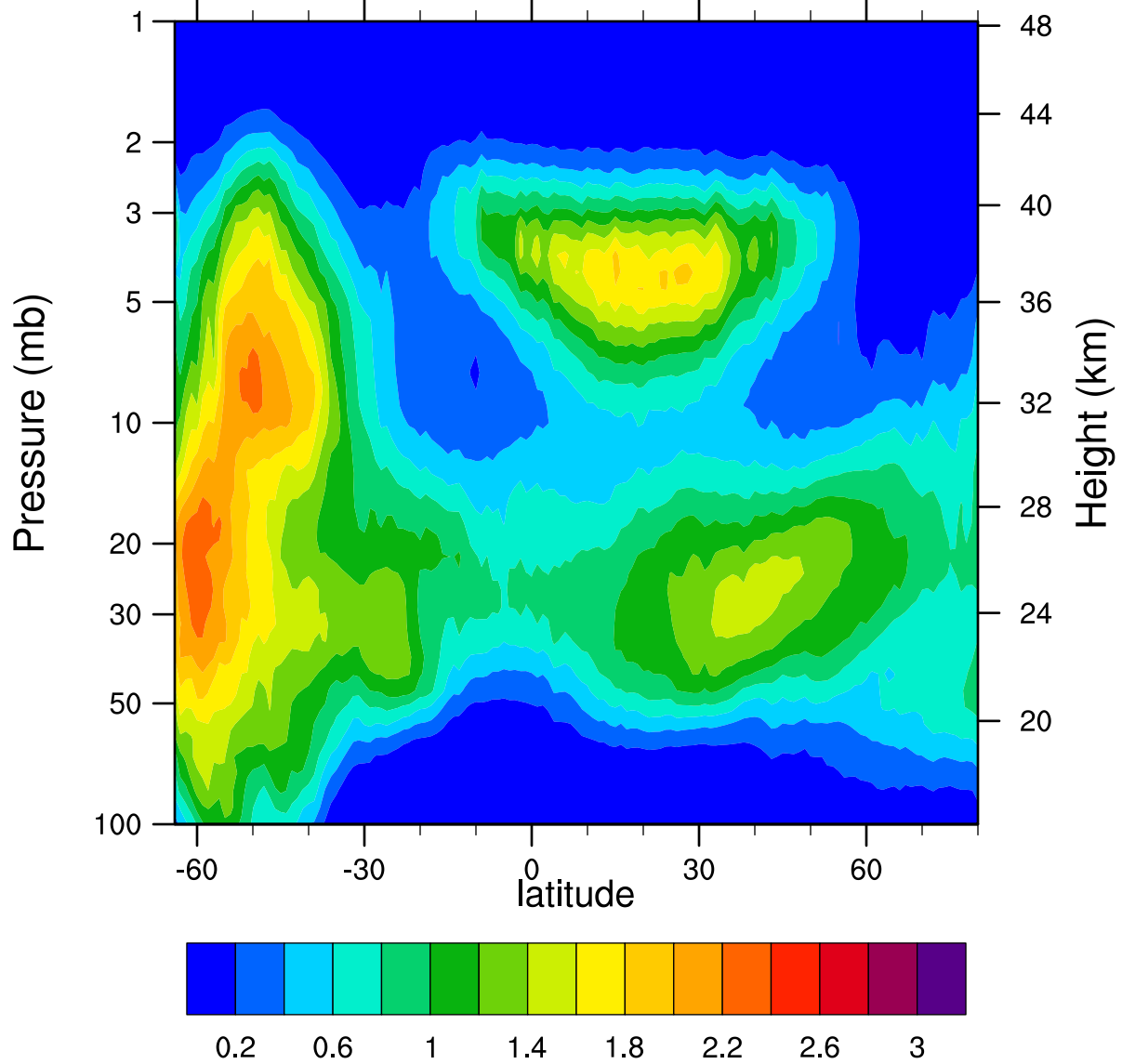
HIRDLSv6 2007d218 ClONO2_Ascending (ppbv)
