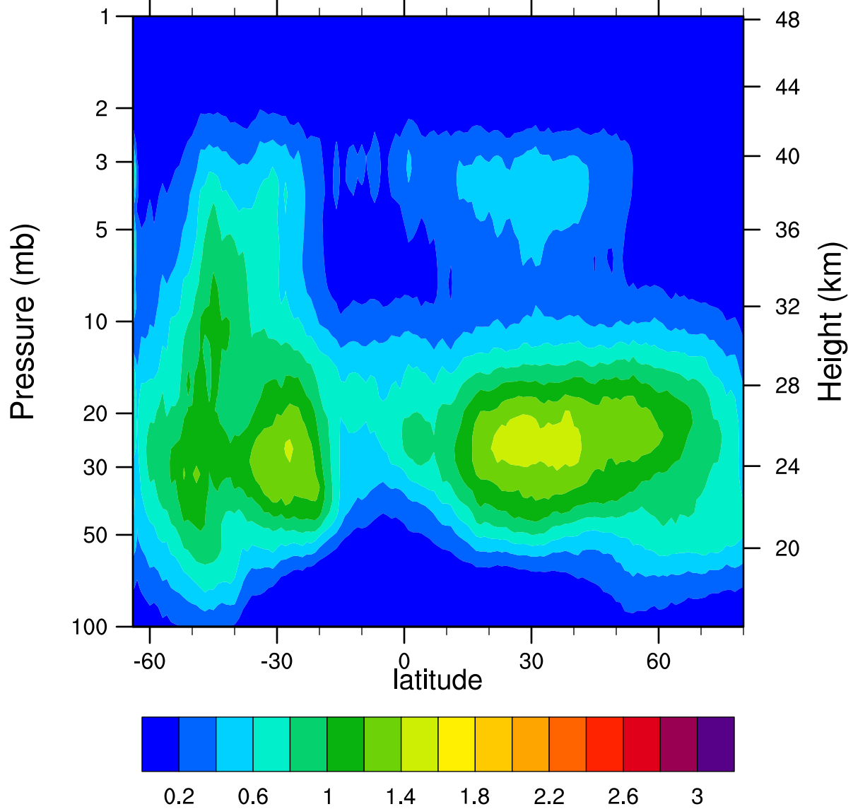
HIRDLSv6 2007d185 ClONO2_Ascending (ppbv)
