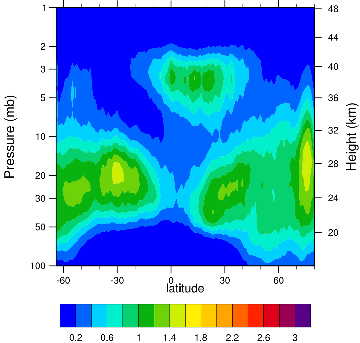
HIRDLSv6 2006d361 ClONO2_Ascending (ppbv)
