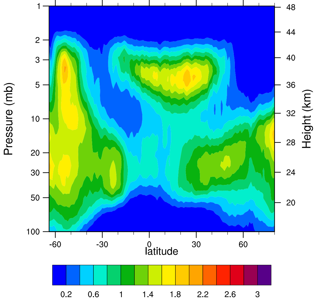
HIRDLSv6 2007d279 ClONO2_Ascending (ppbv)
