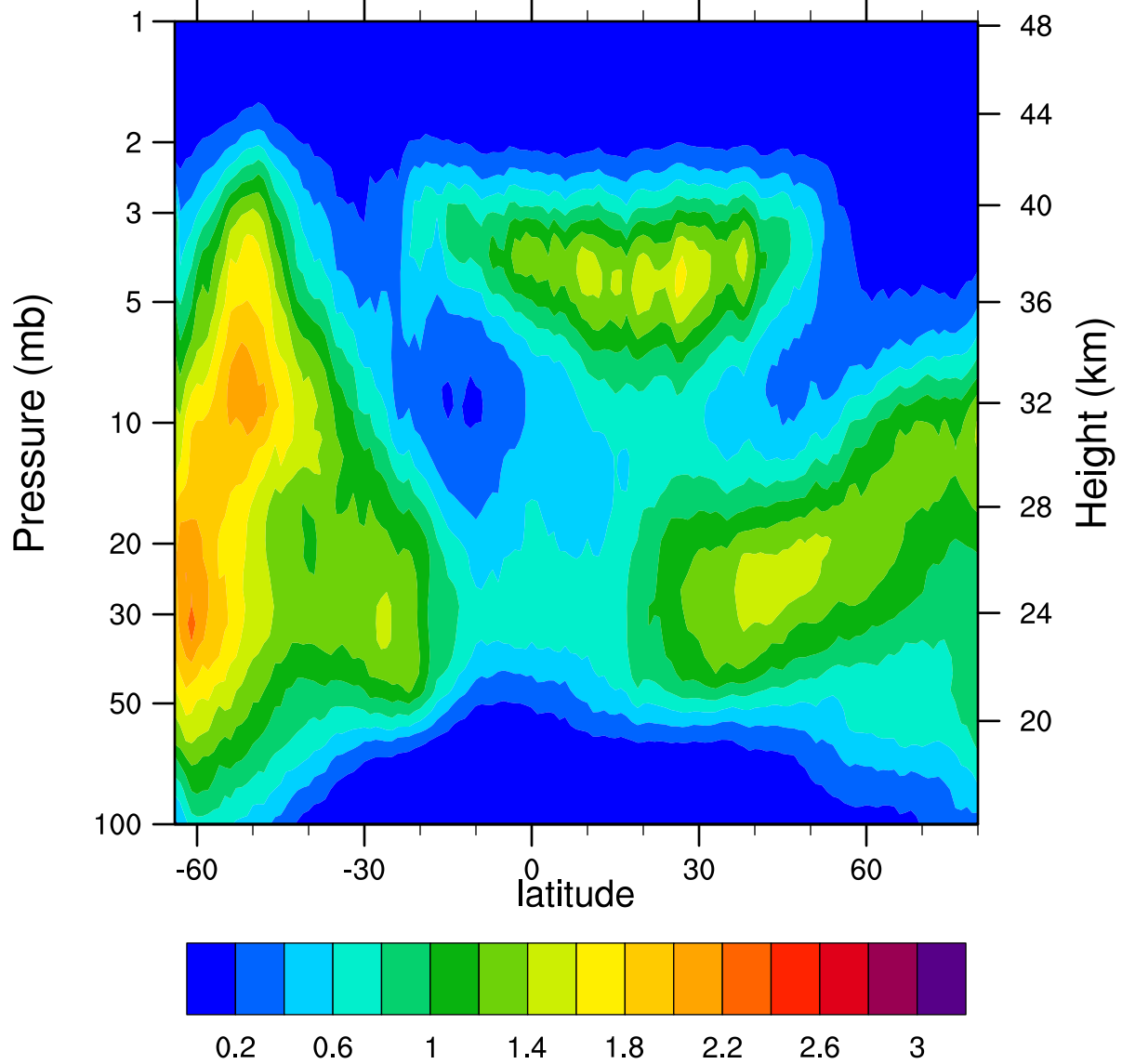
HIRDLSv6 2007d252 ClONO2_Ascending (ppbv)
