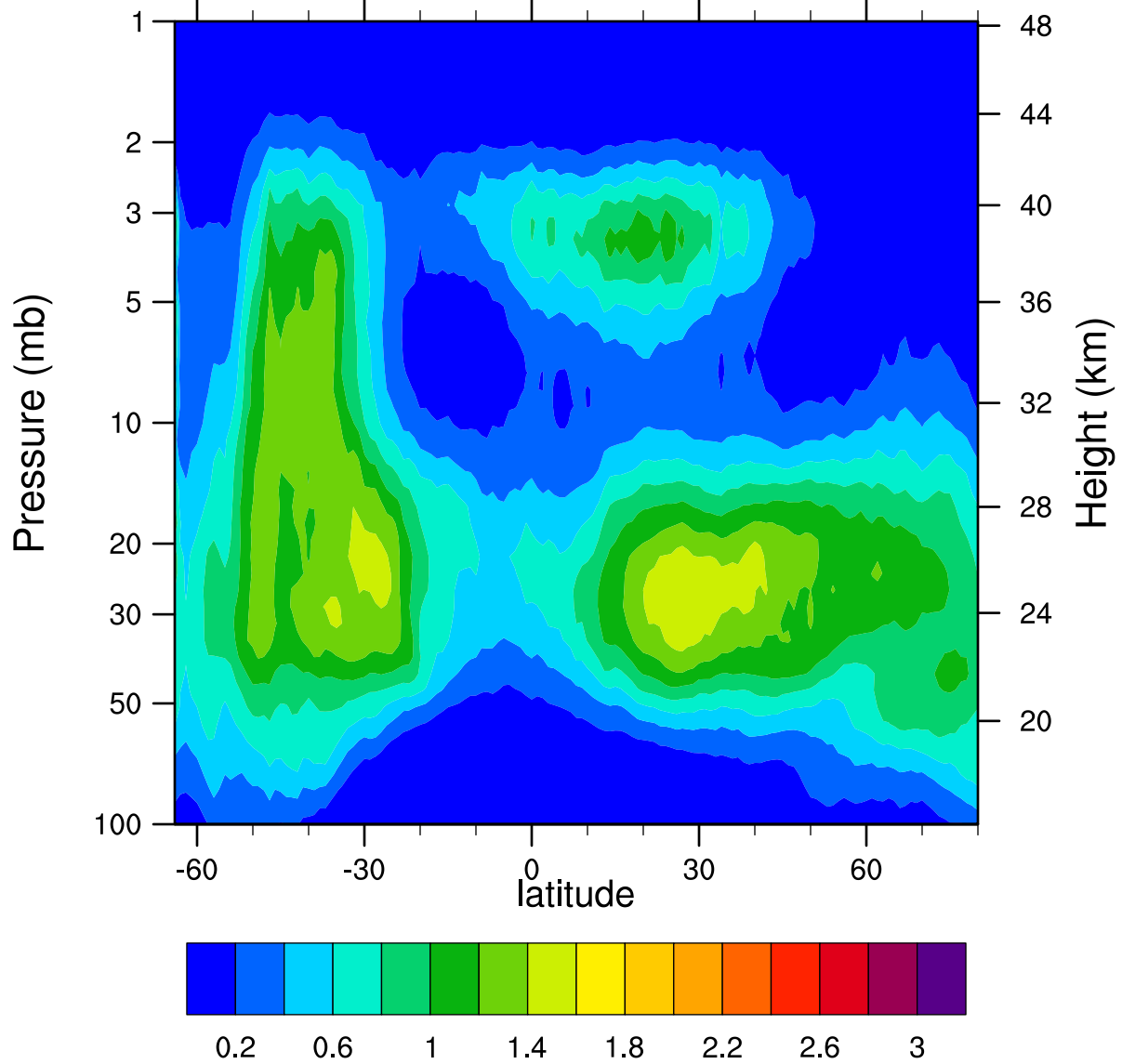
HIRDLSv6 2007d154 ClONO2_Ascending (ppbv)
