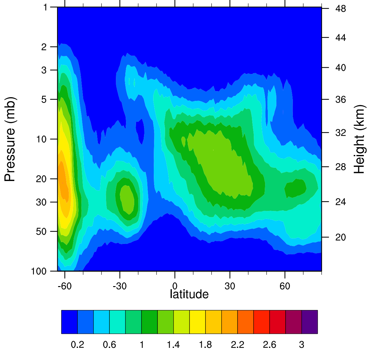
HIRDLSv6 2005d197 ClONO2_Ascending (ppbv)
