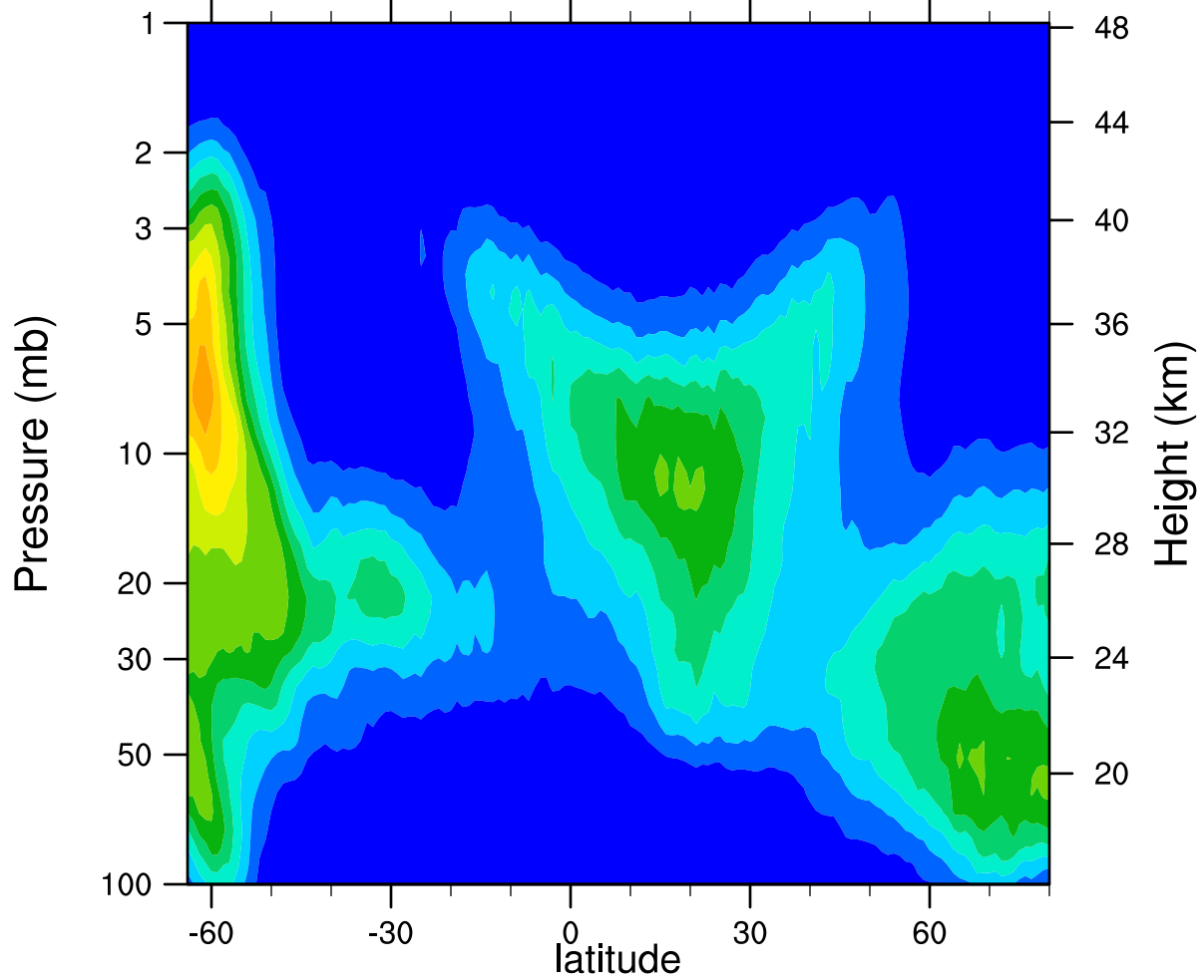
HIRDLSv6 2005d075 ClONO2_Ascending (ppbv)
