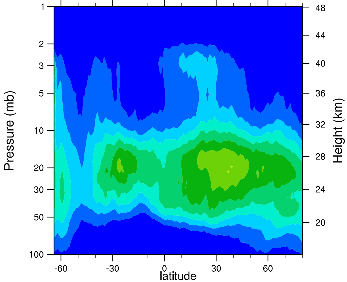
HIRDLSv6 2006d158 ClONO2_Ascending (ppbv)
