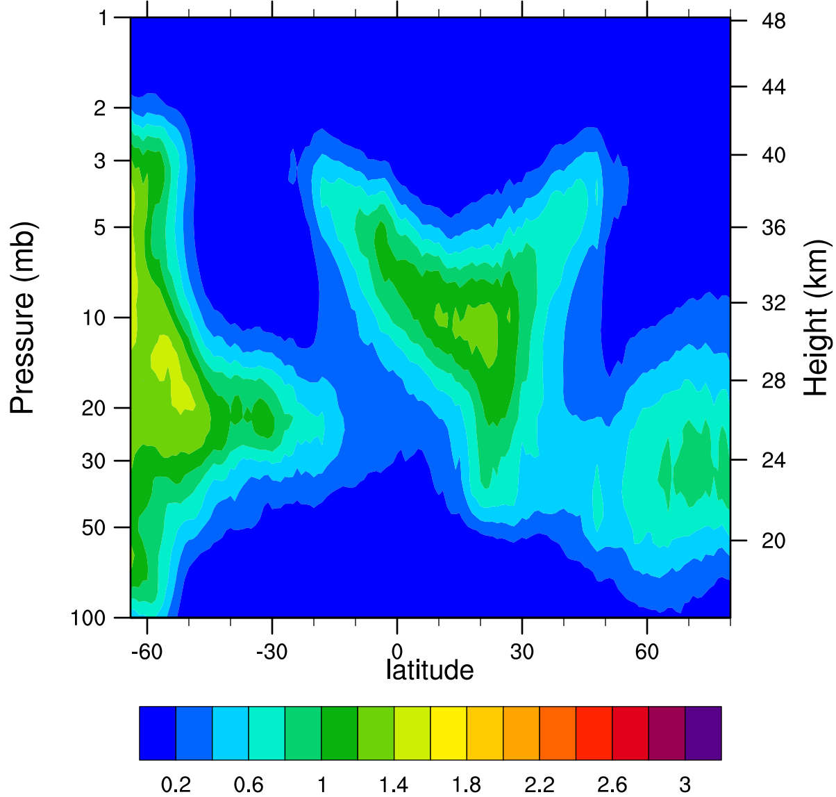
HIRDLSv6 2005d051 ClONO2_Ascending (ppbv)
