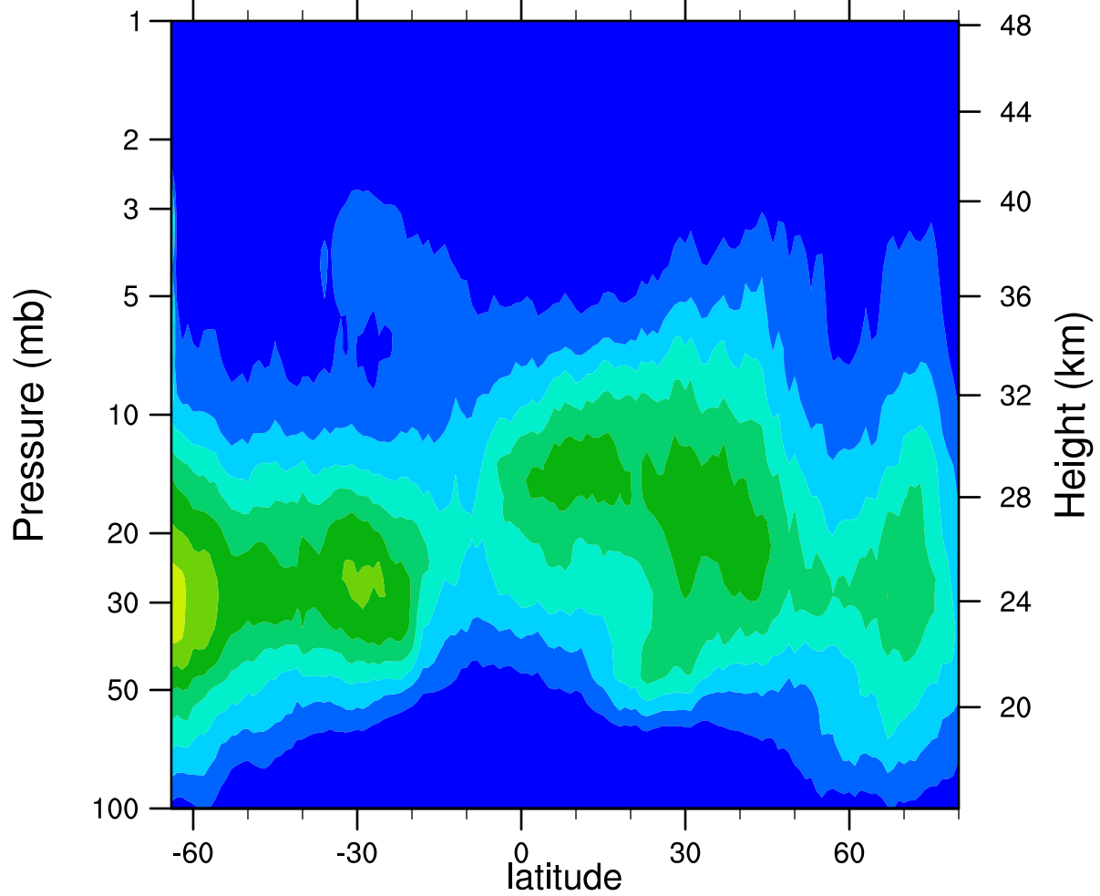
HIRDLSv6 2005d311 ClONO2_Ascending (ppbv)
