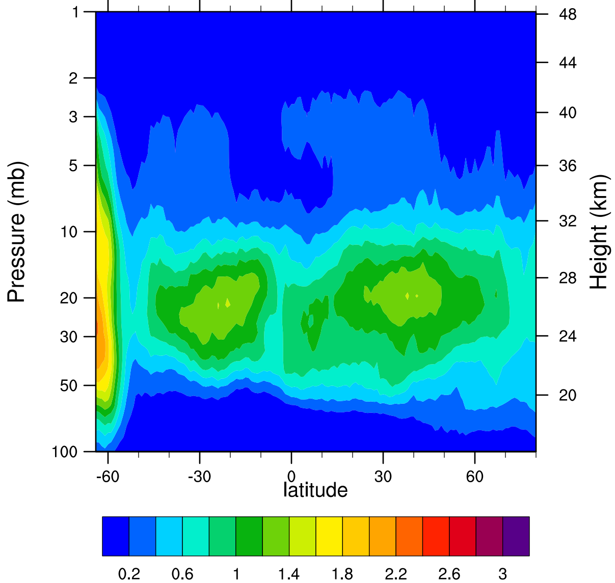
HIRDLSv6 2006d256 ClONO2_Ascending (ppbv)
