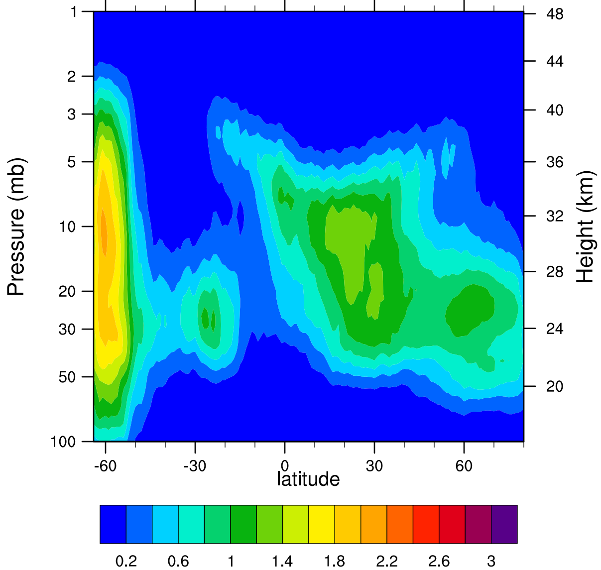
HIRDLSv6 2005d169 ClONO2_Ascending (ppbv)
