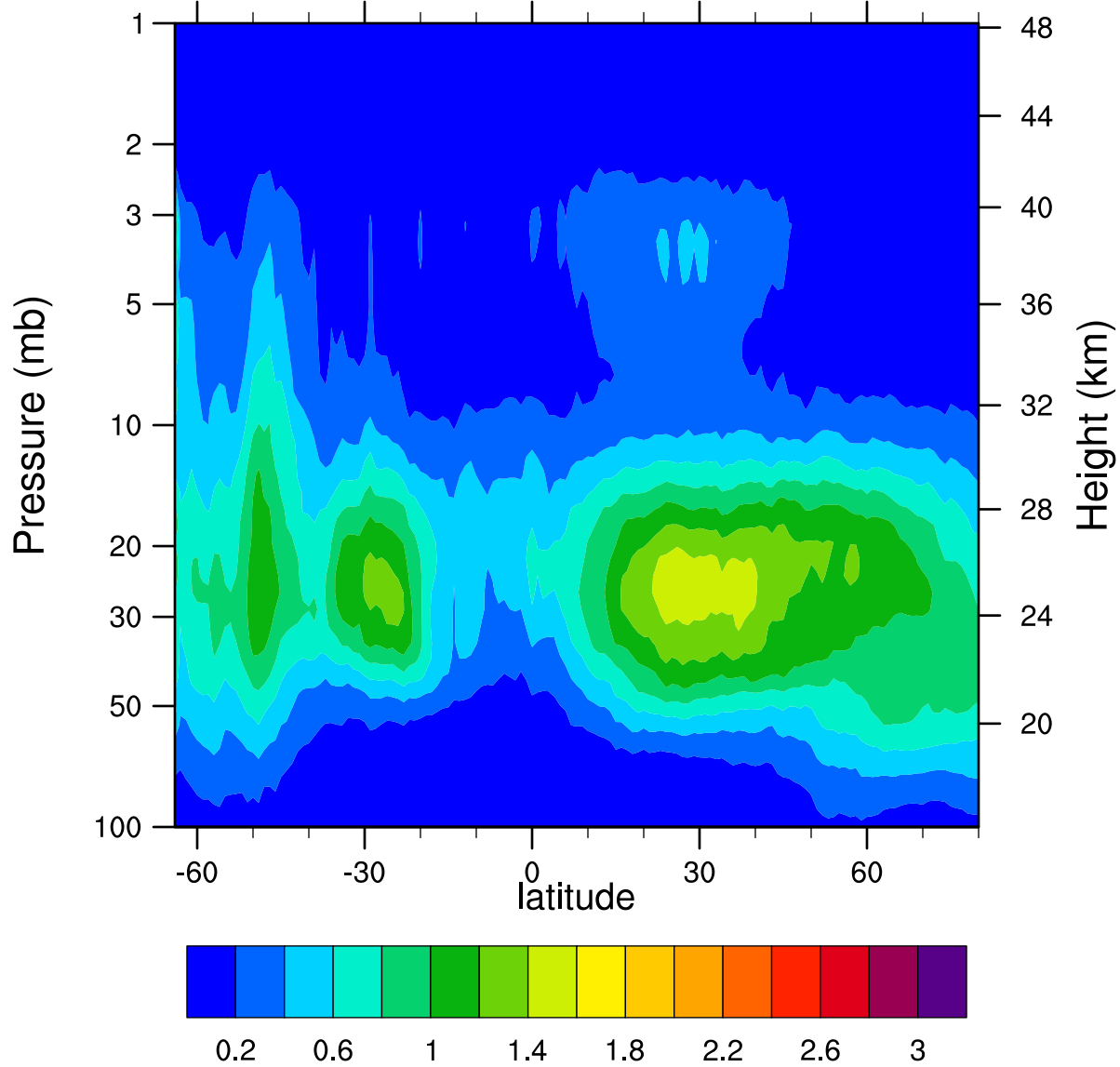
HIRDLSv6 2007d167 ClONO2_Ascending (ppbv)
