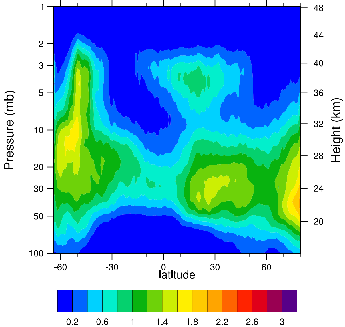
HIRDLSv6 2007d097 ClONO2_Ascending (ppbv)
