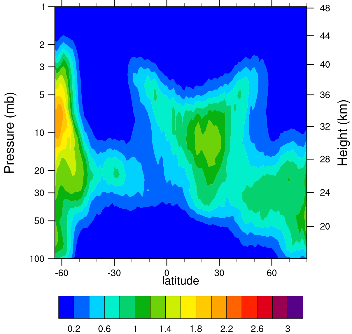
HIRDLSv6 2005d087 ClONO2_Ascending (ppbv)
