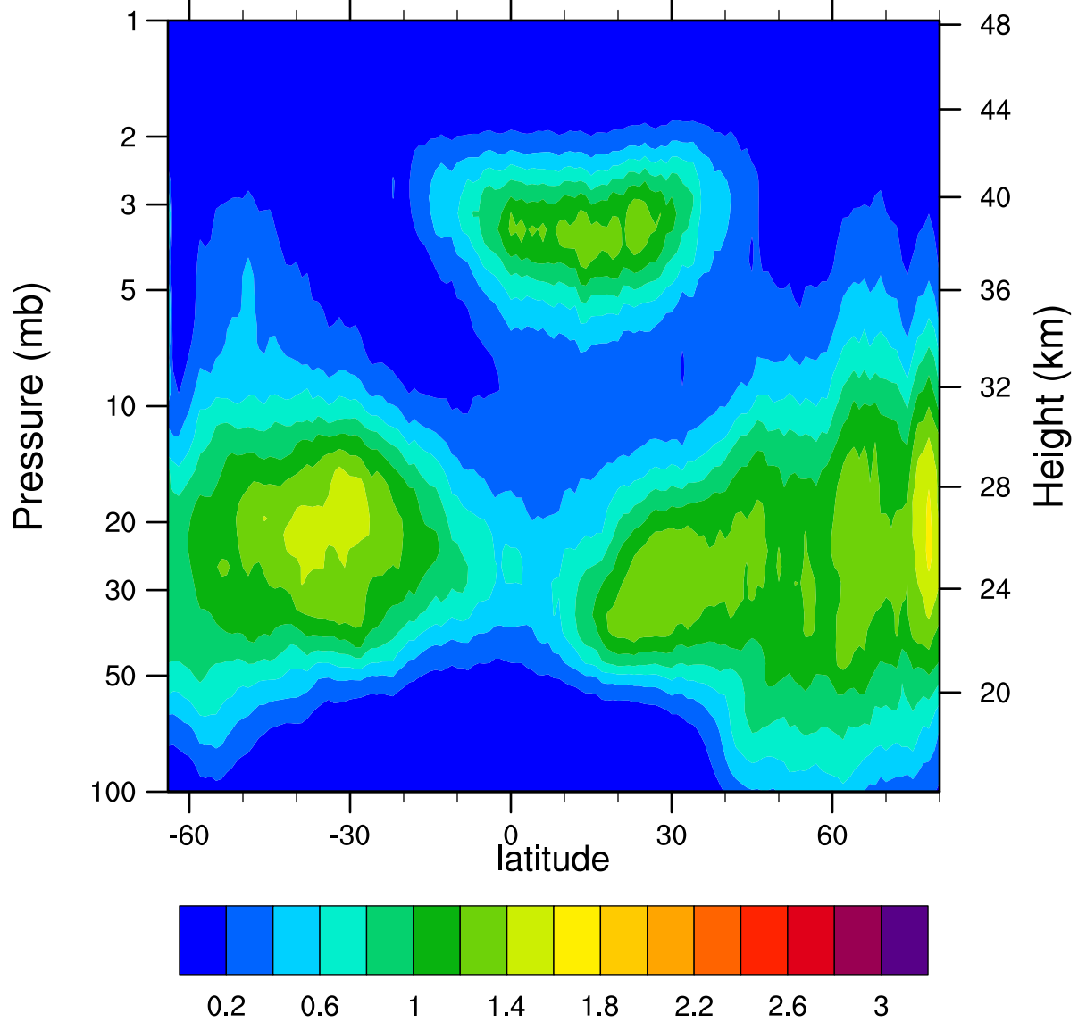
HIRDLSv6 2007d025 ClONO2_Ascending (ppbv)
