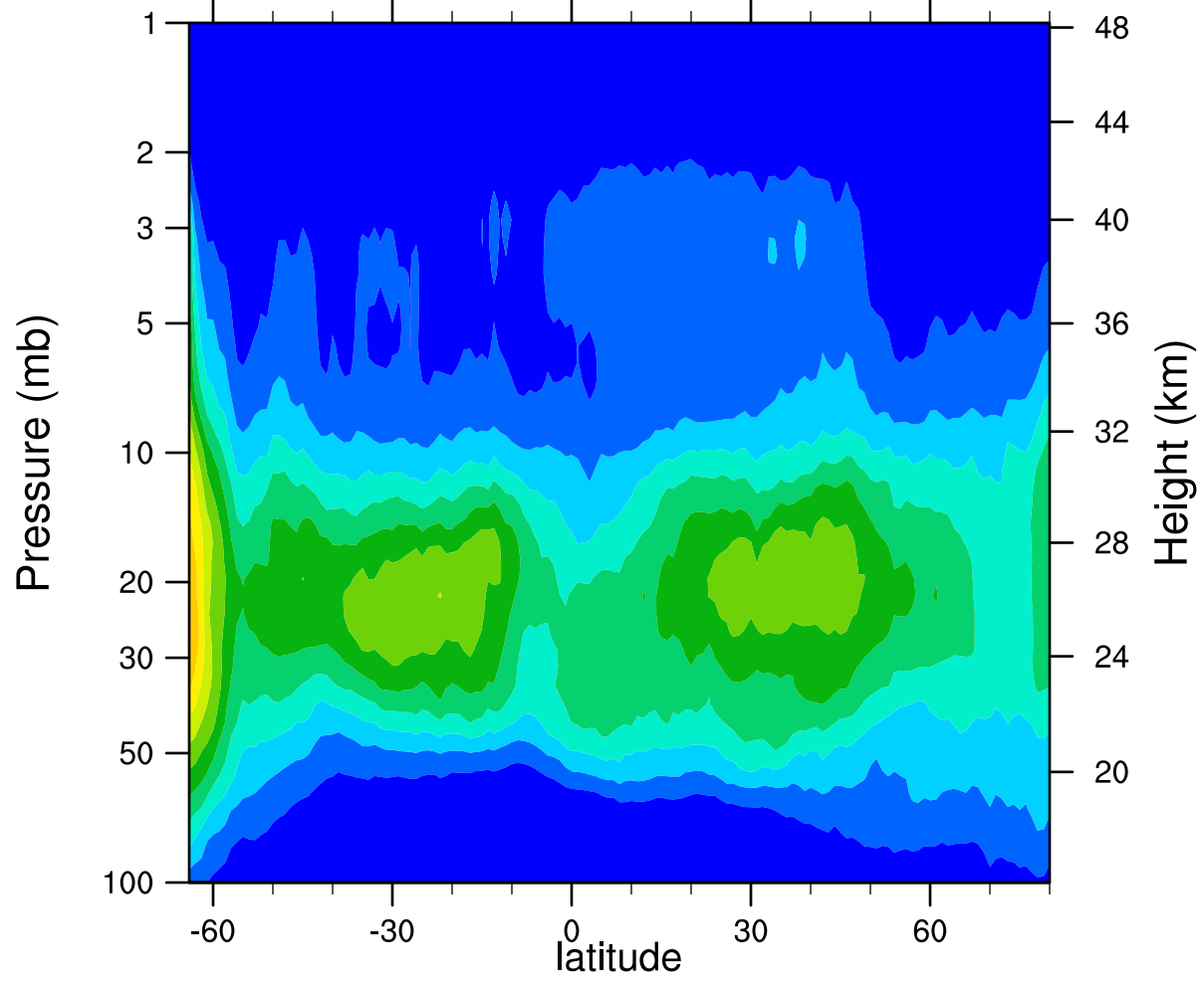
HIRDLSv6 2006d272 ClONO2_Ascending (ppbv)
