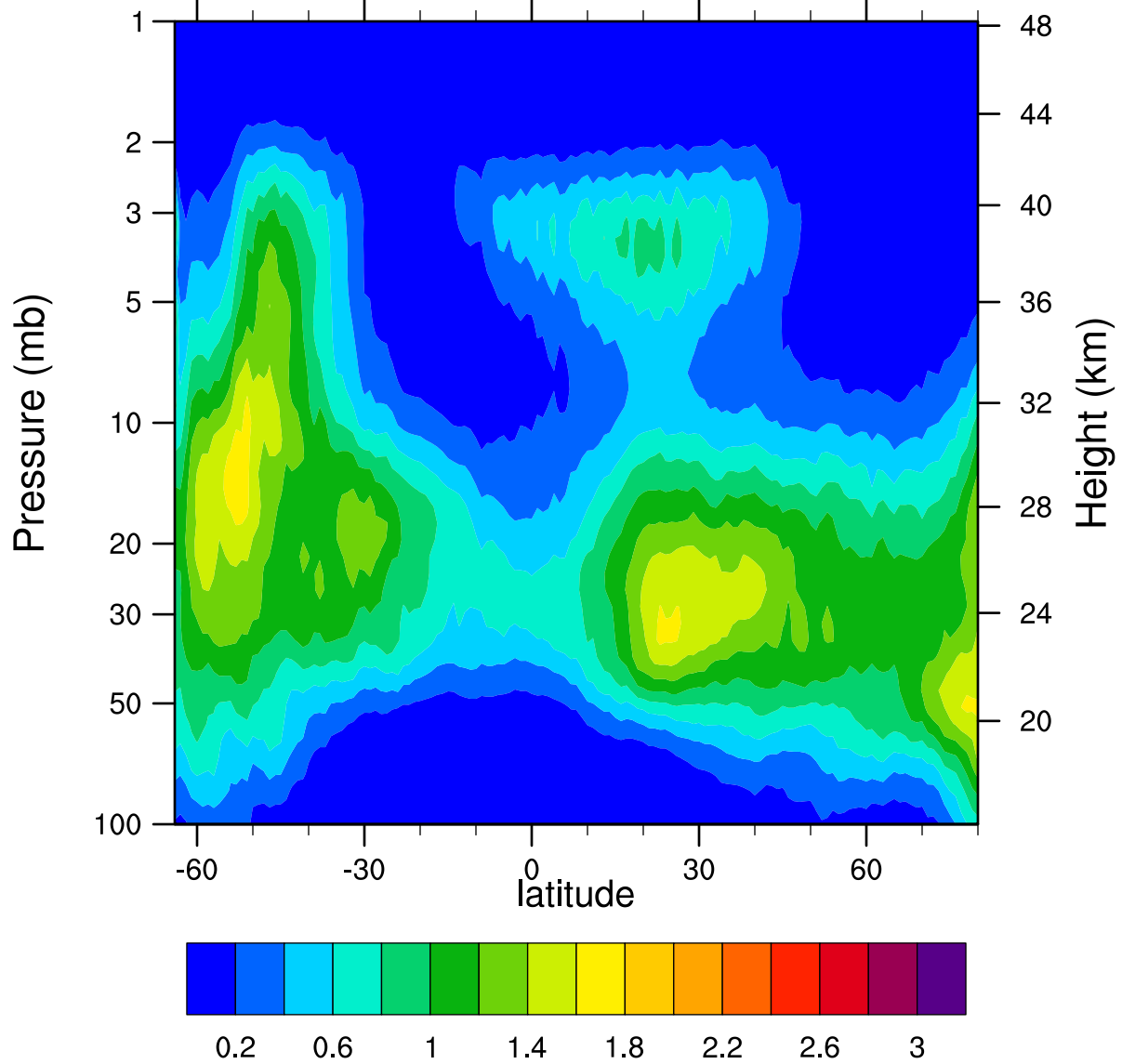
HIRDLSv6 2007d1113 ClONO2_Ascending (ppbv)
