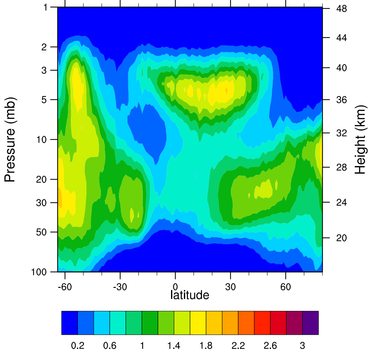
HIRDLSv6 2007d270 ClONO2_Ascending (ppbv)
