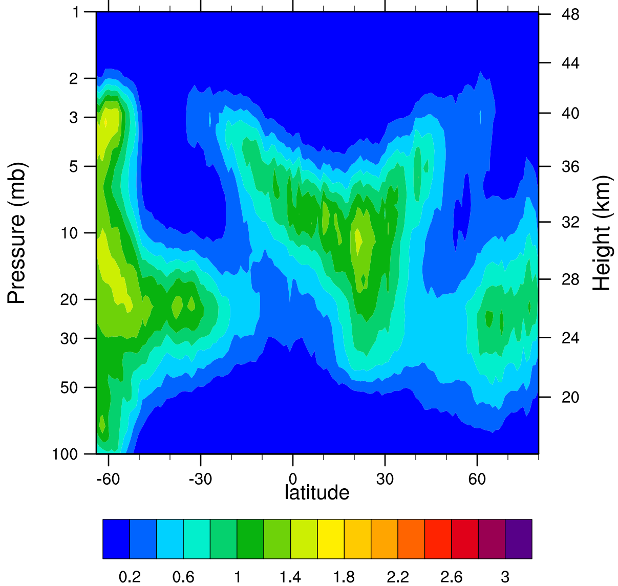
HIRDLSv6 2005d030 ClONO2_Ascending (ppbv)
