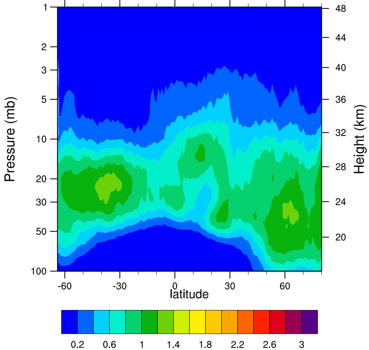
HIRDLSv6 2006d035 ClONO2_Ascending (ppbv)
