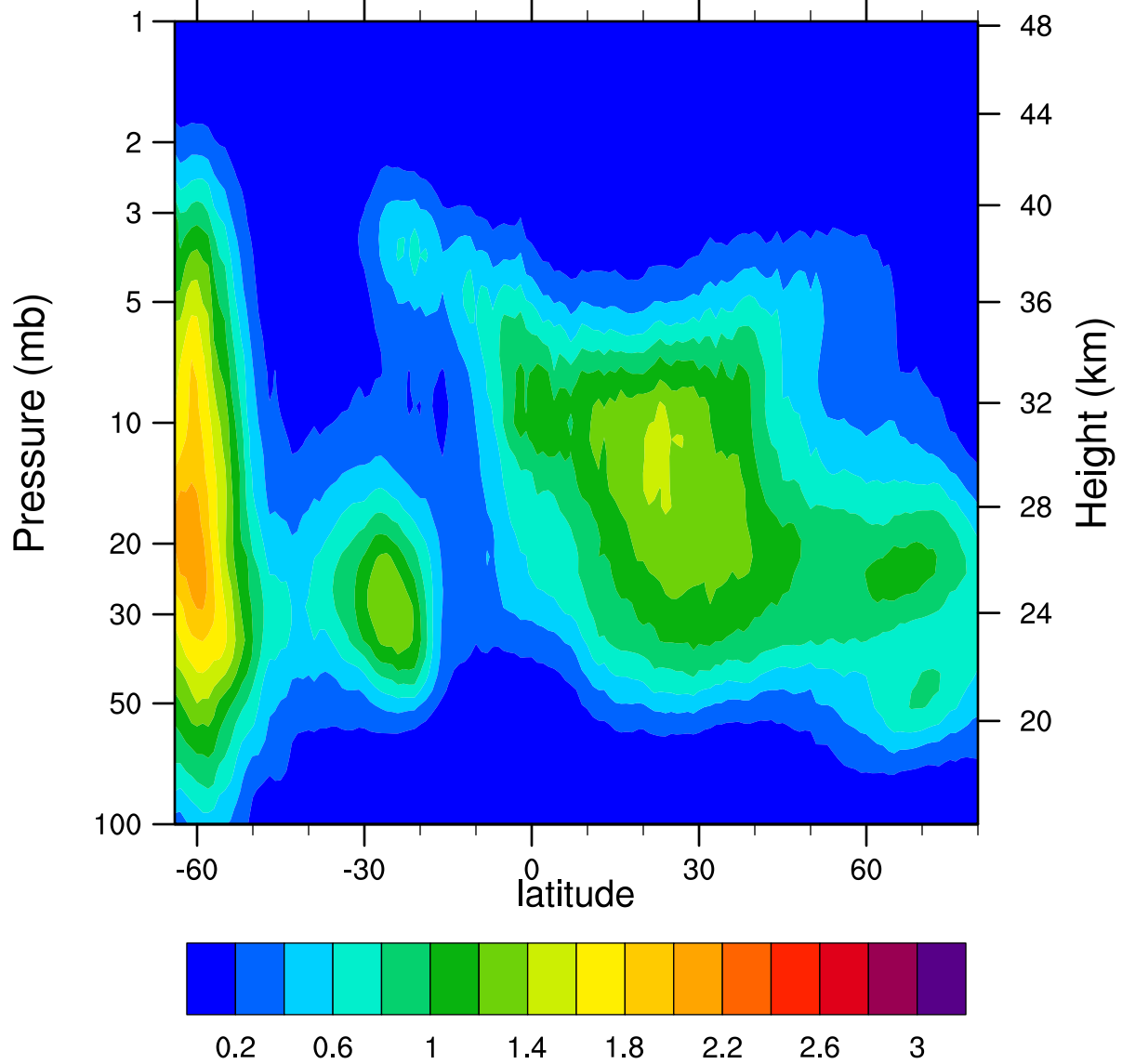
HIRDLSv6 2005d189 ClONO2_Ascending (ppbv)
