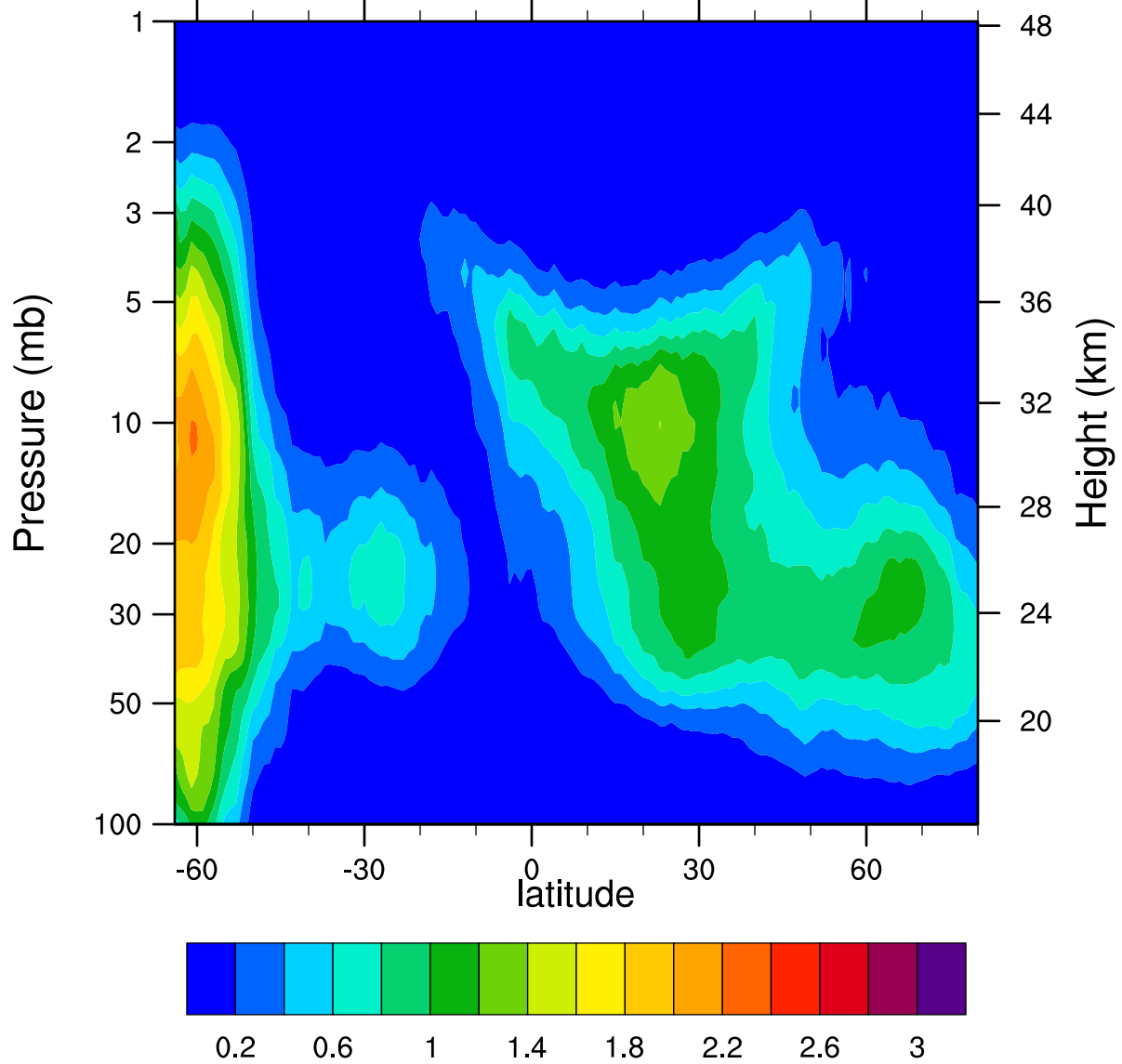
HIRDLSv6 2005d131 ClONO2_Ascending (ppbv)
