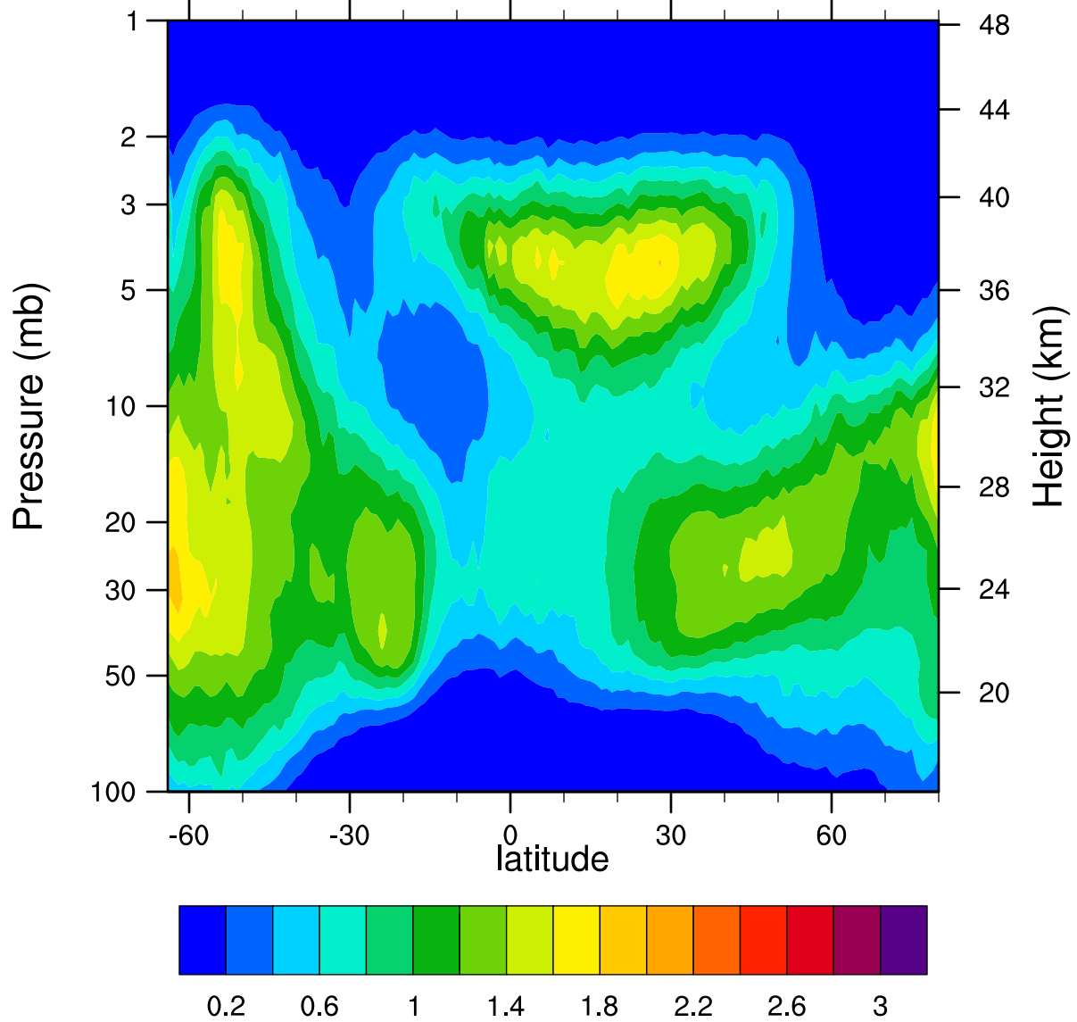
HIRDLSv6 2007d269 ClONO2_Ascending (ppbv)
