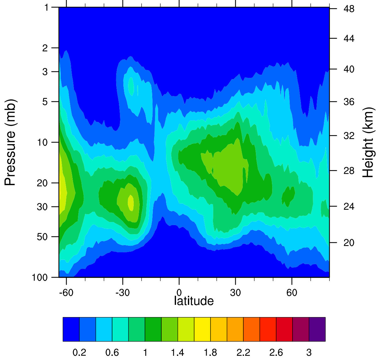
HIRDLSv6 2005d283 ClONO2_Ascending (ppbv)
