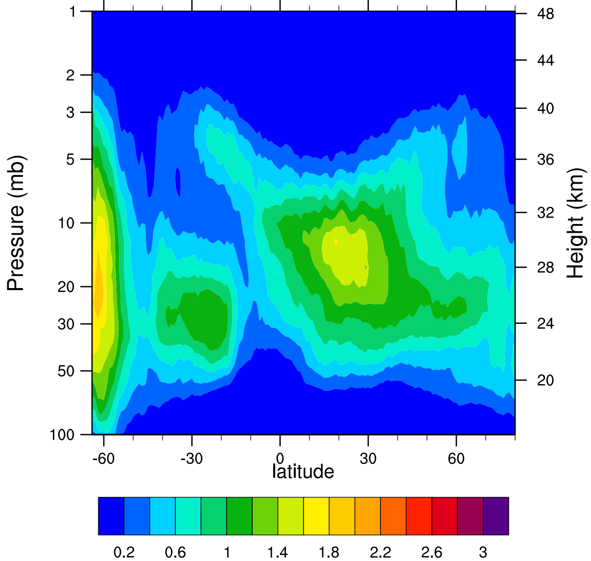
HIRDLSv6 2005d243 ClONO2_Ascending (ppbv)
