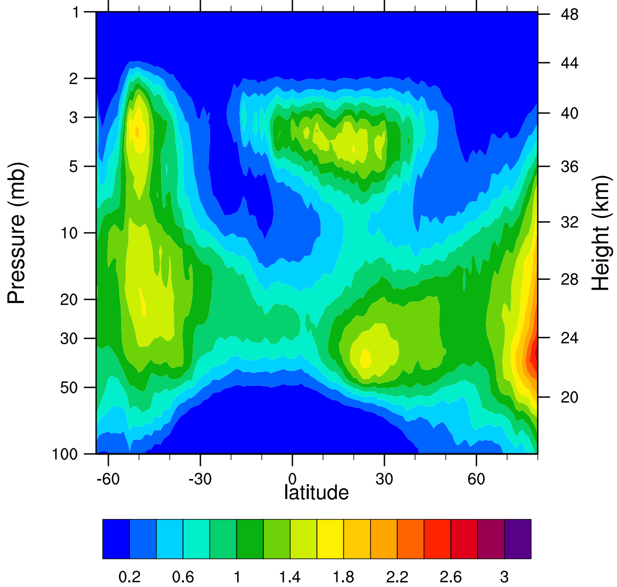
HIRDLSv6 2007d082 ClONO2_Ascending (ppbv)
