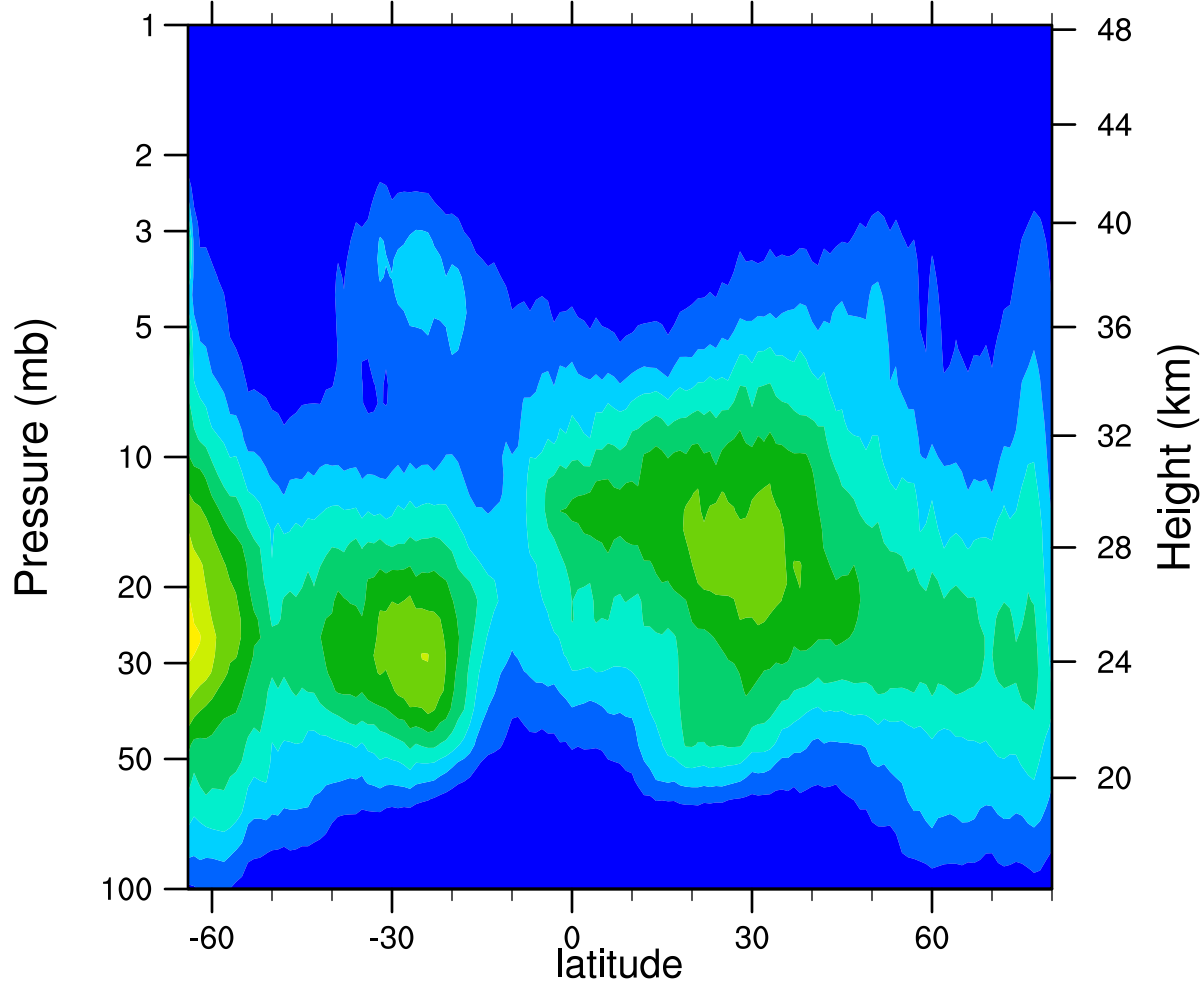
HIRDLSv6 2005d291 ClONO2_Ascending (ppbv)
