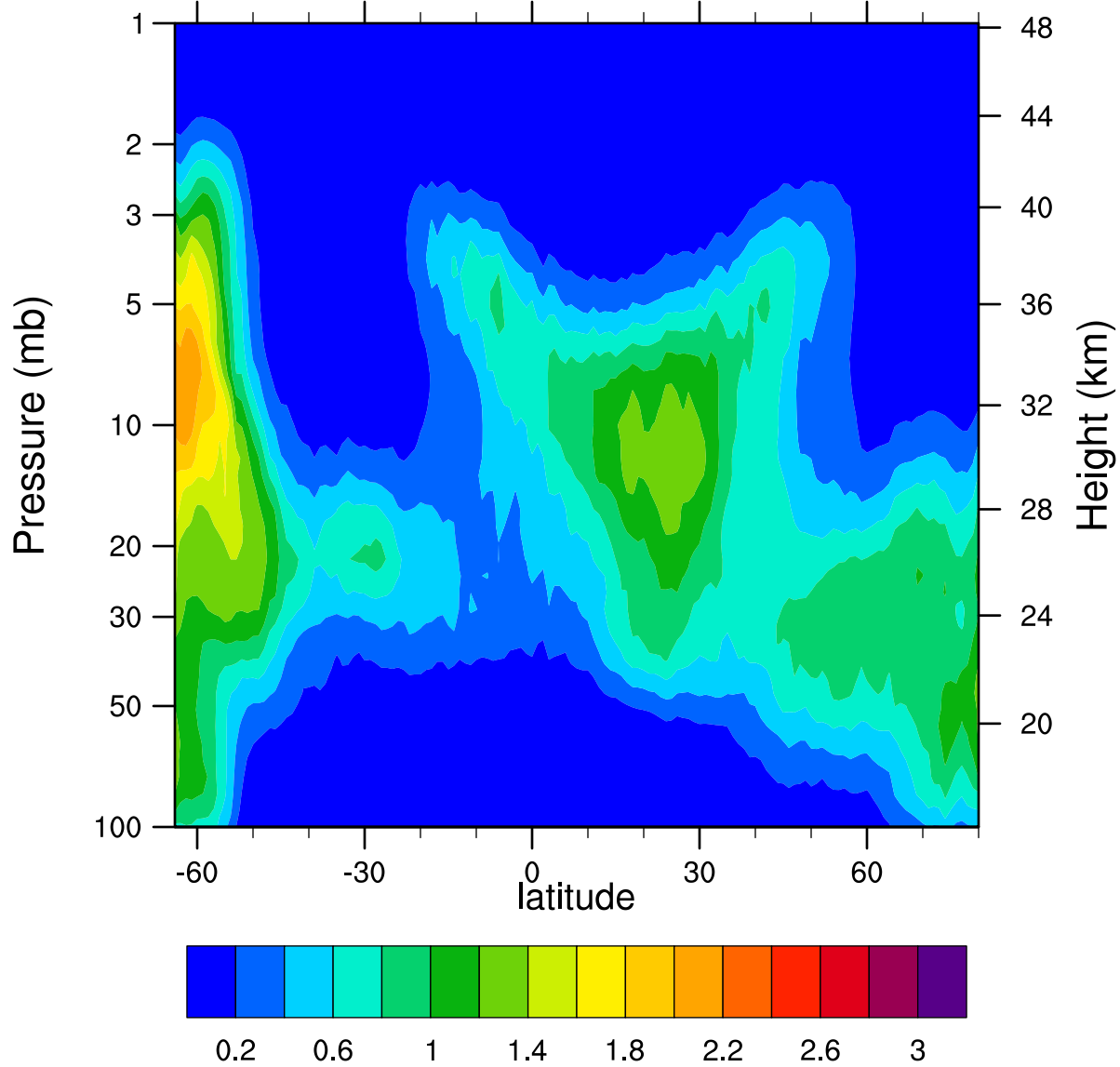
HIRDLSv6 2005d086 ClONO2_Ascending (ppbv)
