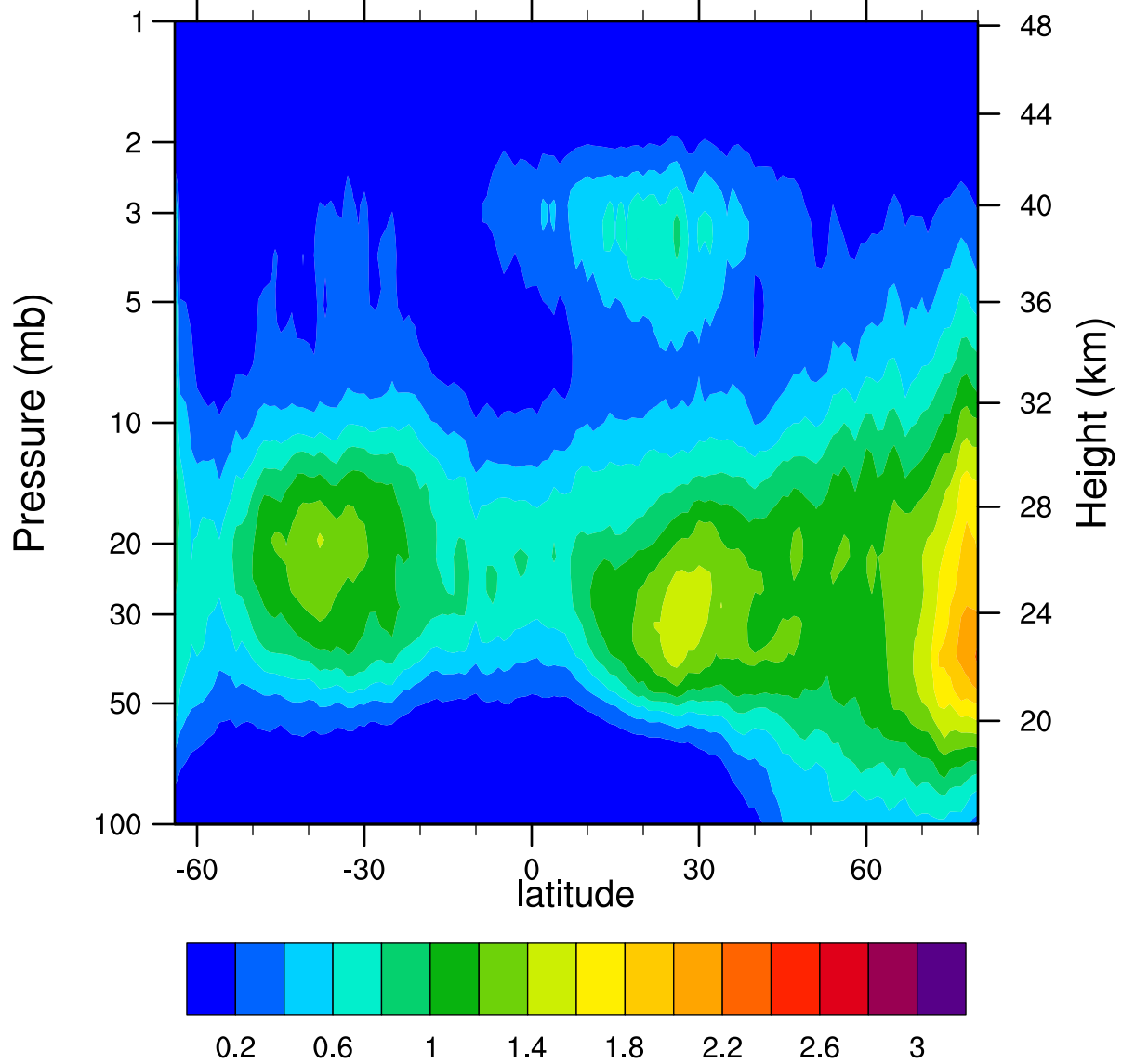
HIRDLSv6 2007d071 ClONO2_Ascending (ppbv)
