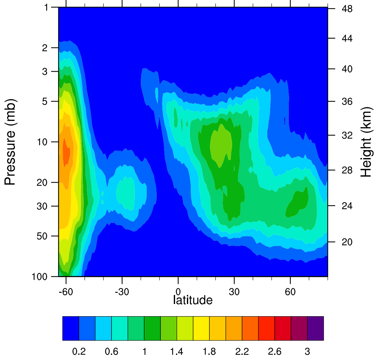
HIRDLSv6 2005d134 ClONO2_Ascending (ppbv)
