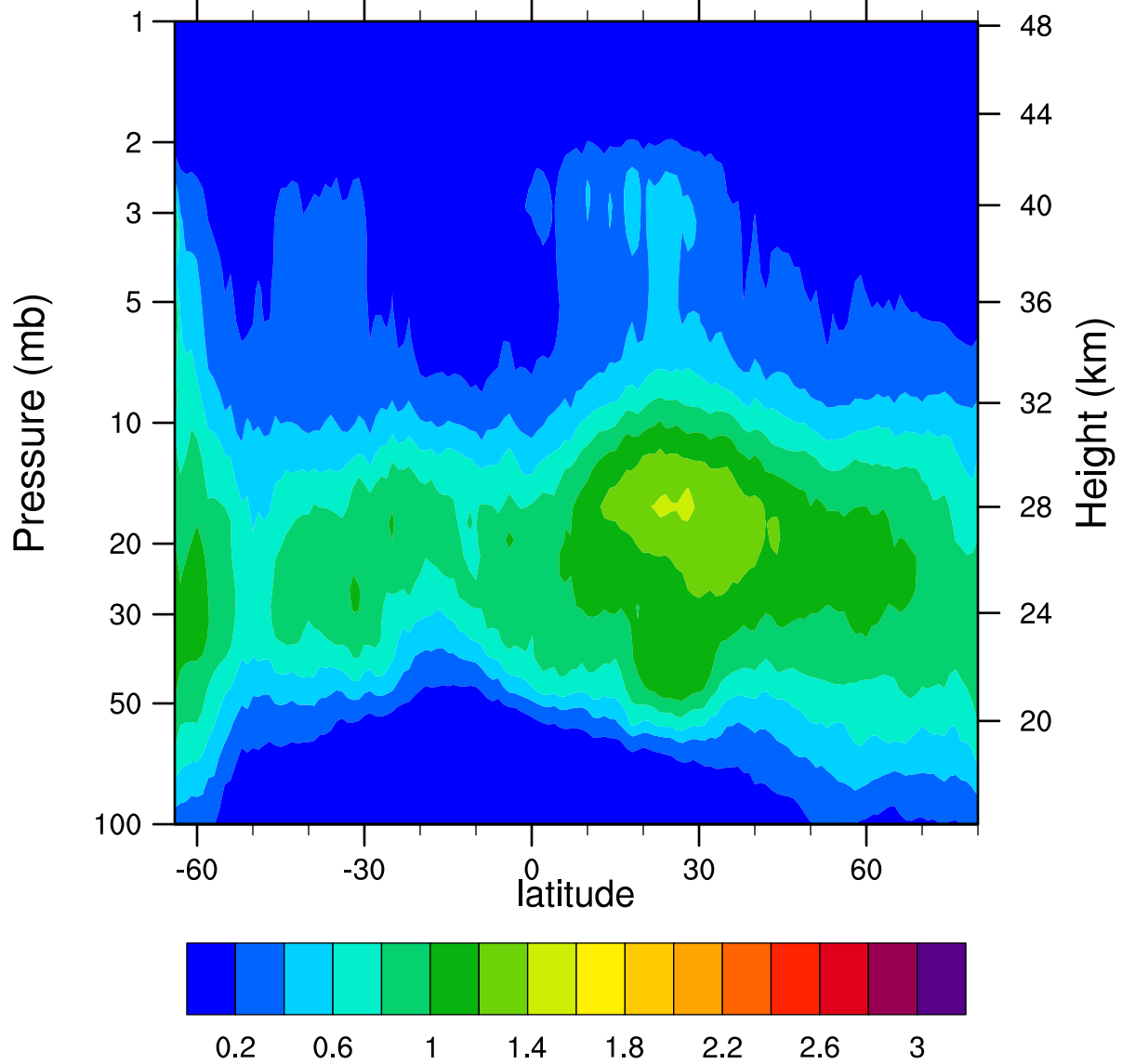
HIRDLSv6 2006d125 ClONO2_Ascending (ppbv)
