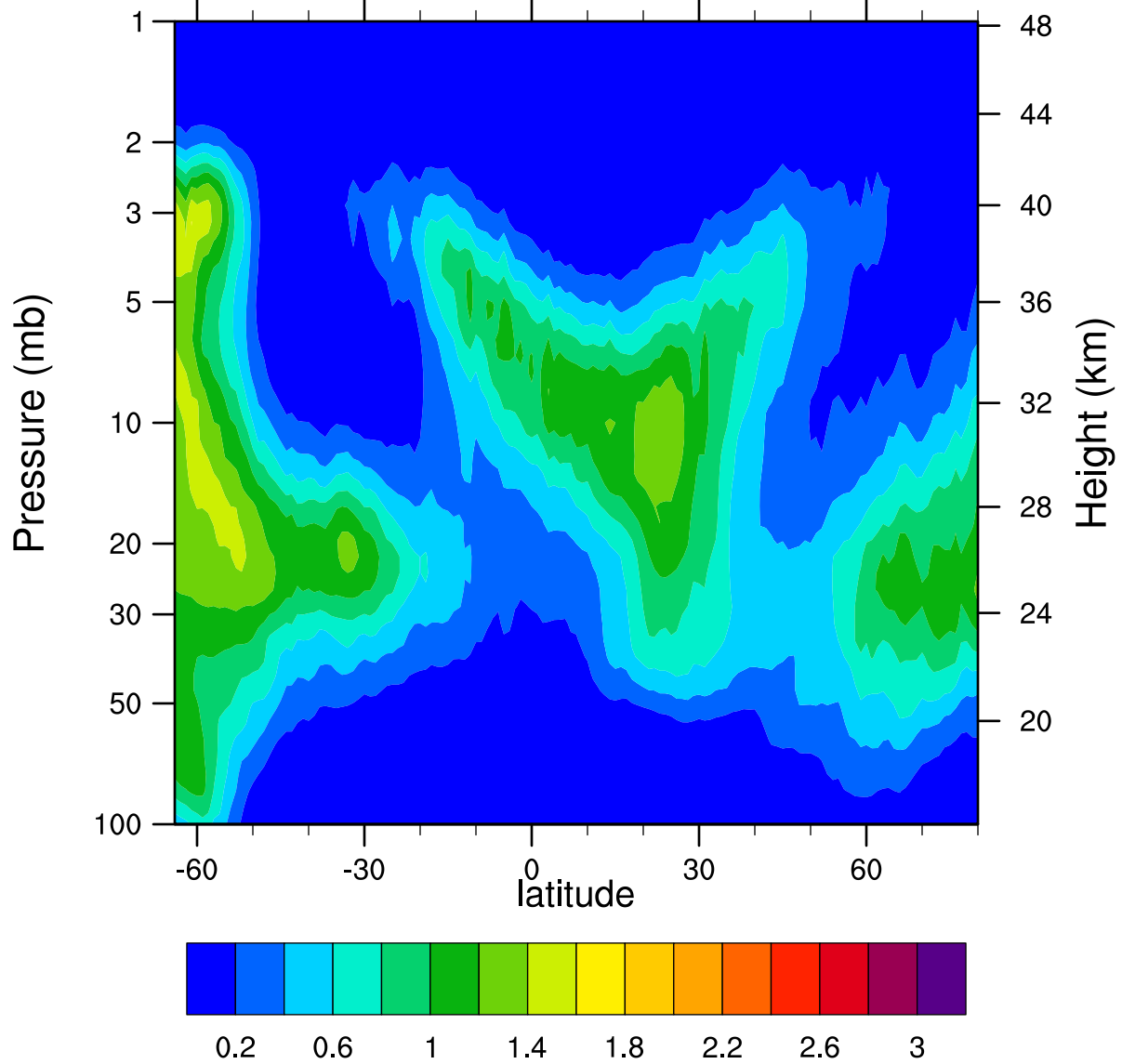
HIRDLSv6 2005d038 ClONO2_Ascending (ppbv)
