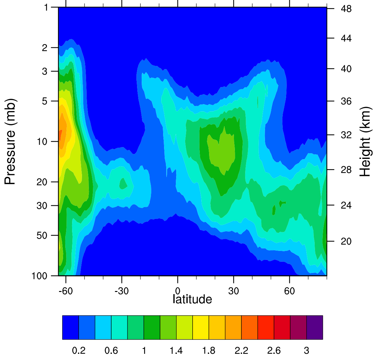
HIRDLSv6 2005d091 ClONO2_Ascending (ppbv)
