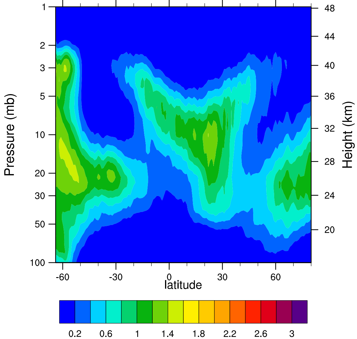
HIRDLSv6 2005d036 ClONO2_Ascending (ppbv)
