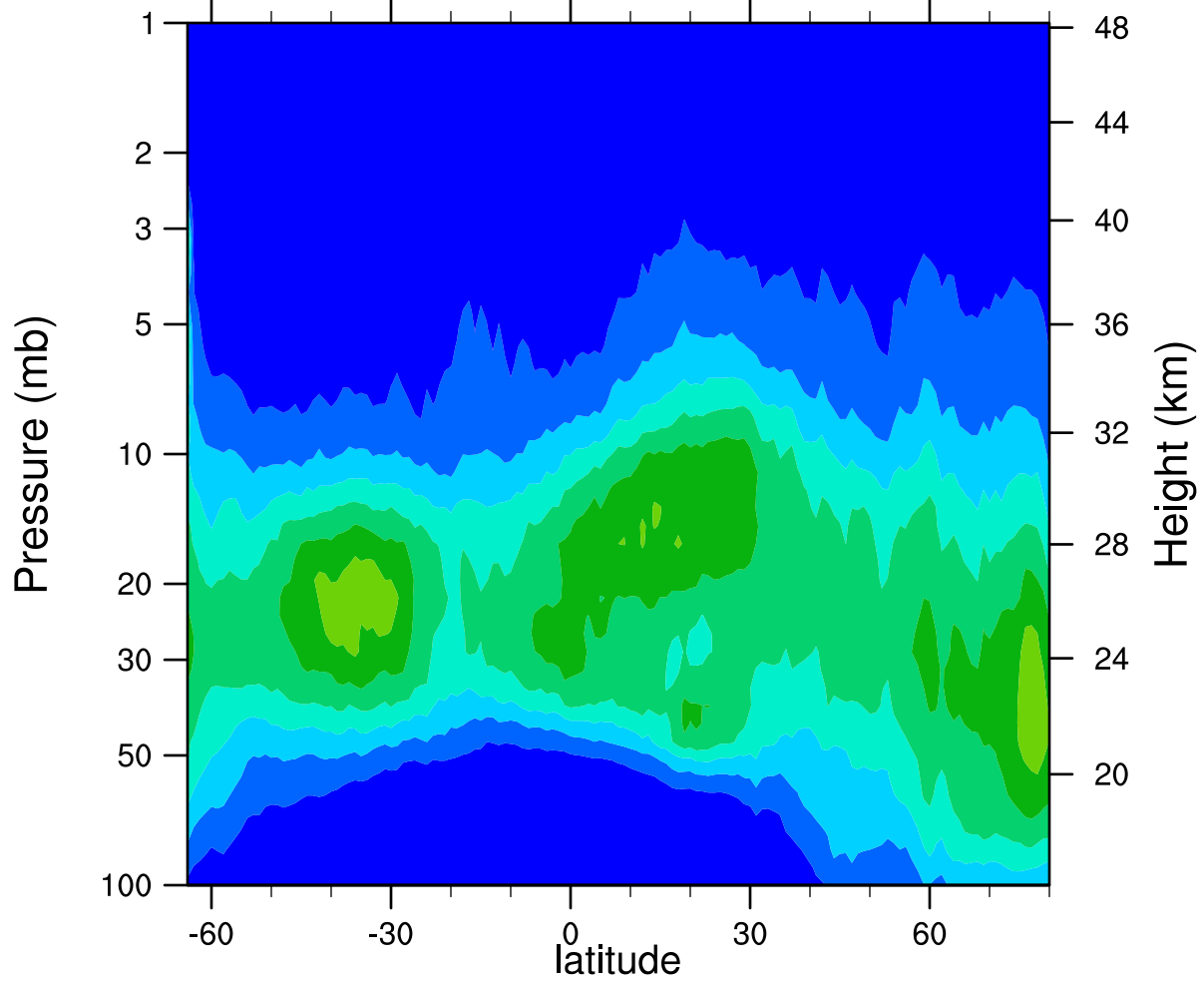
HIRDLSv6 2006d064 ClONO2_Ascending (ppbv)
