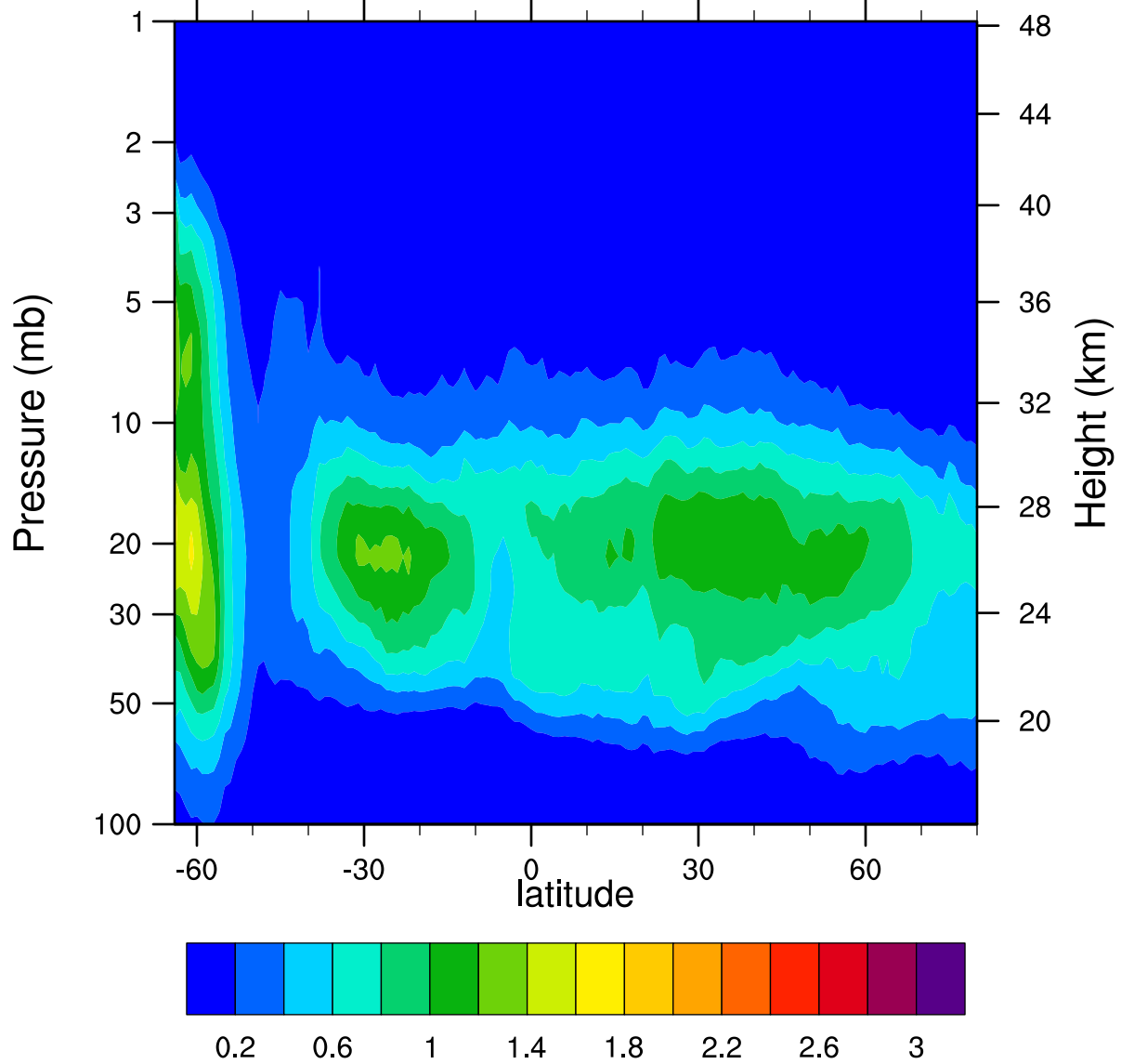
HIRDLSv6 2006d195 ClONO2_Ascending (ppbv)
