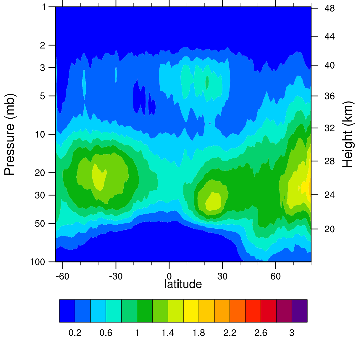
HIRDLSv6 2007d045 ClONO2_Ascending (ppbv)
