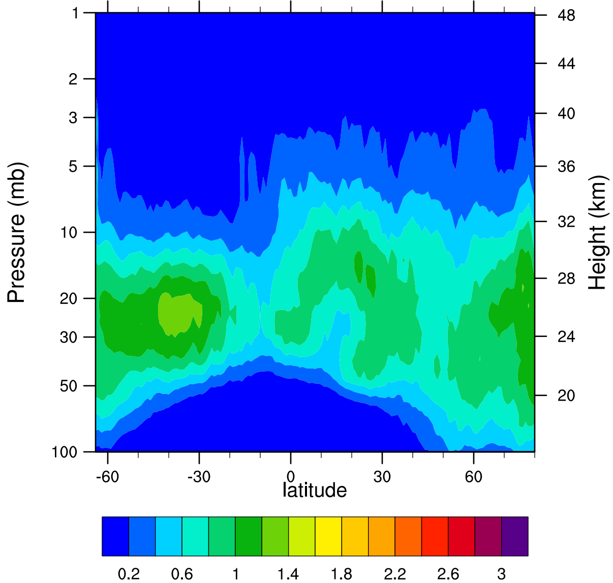
HIRDLSv6 2006d019 ClONO2_Ascending (ppbv)
