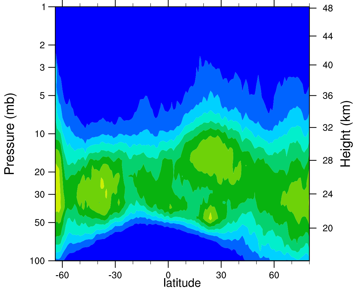
HIRDLSv6 2006d094 ClONO2_Ascending (ppbv)
