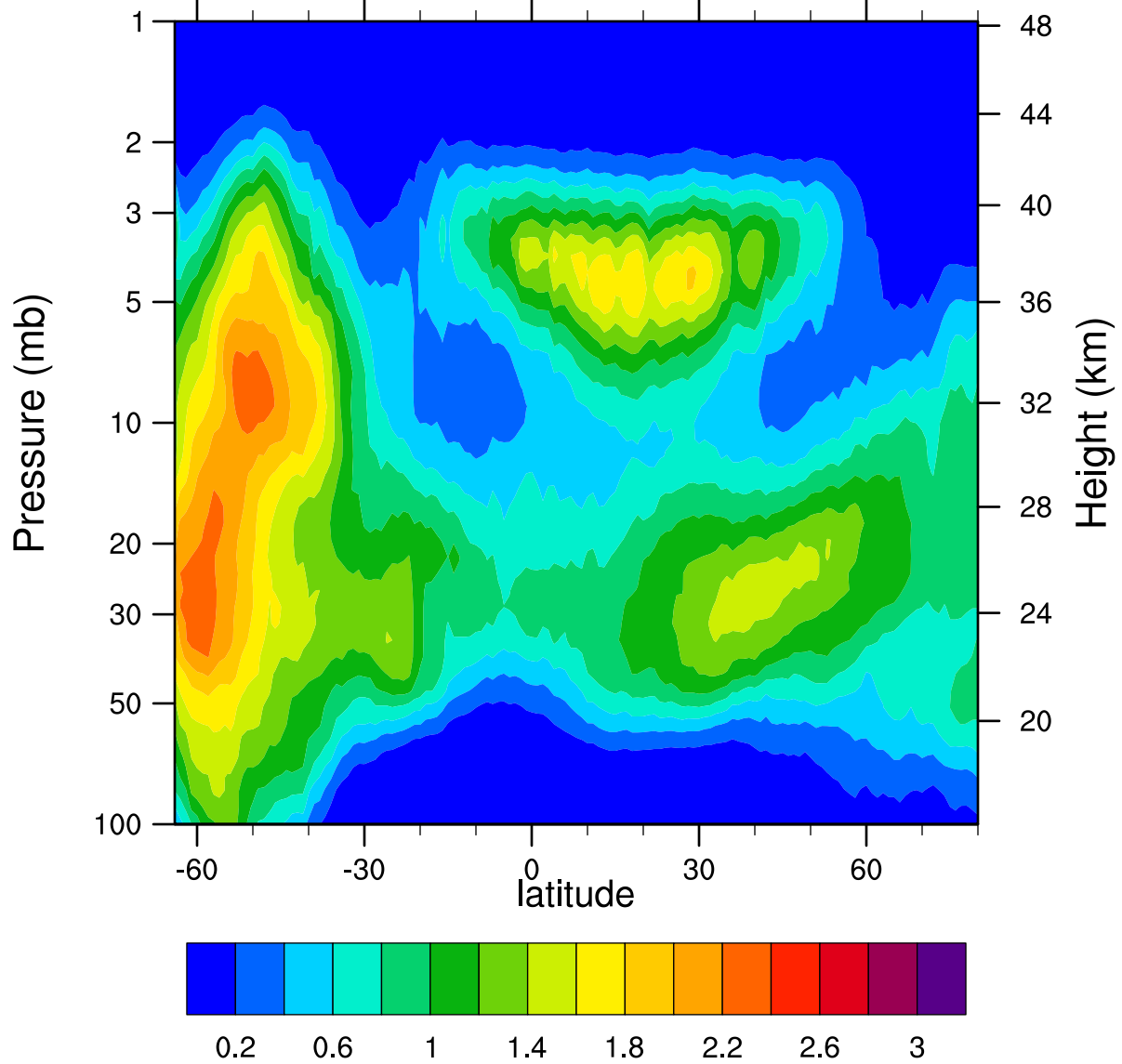
HIRDLSv6 2007d225 ClONO2_Ascending (ppbv)
