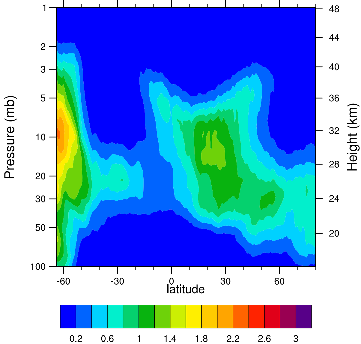
HIRDLSv6 2005d108 ClONO2_Ascending (ppbv)
