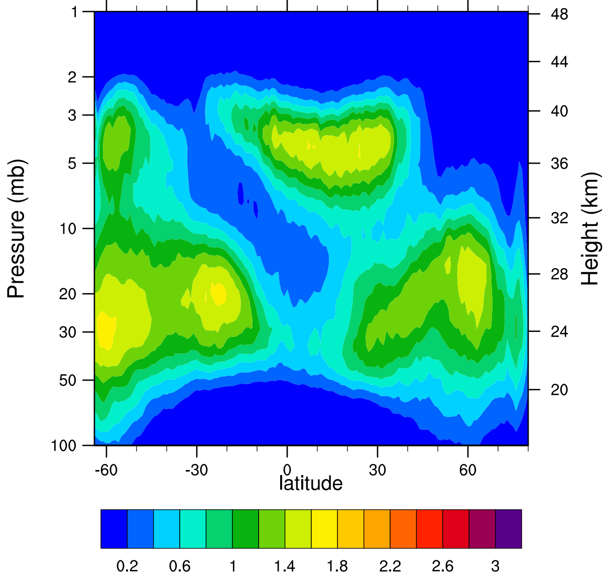
HIRDLSv6 2006d335 ClONO2_Ascending (ppbv)
