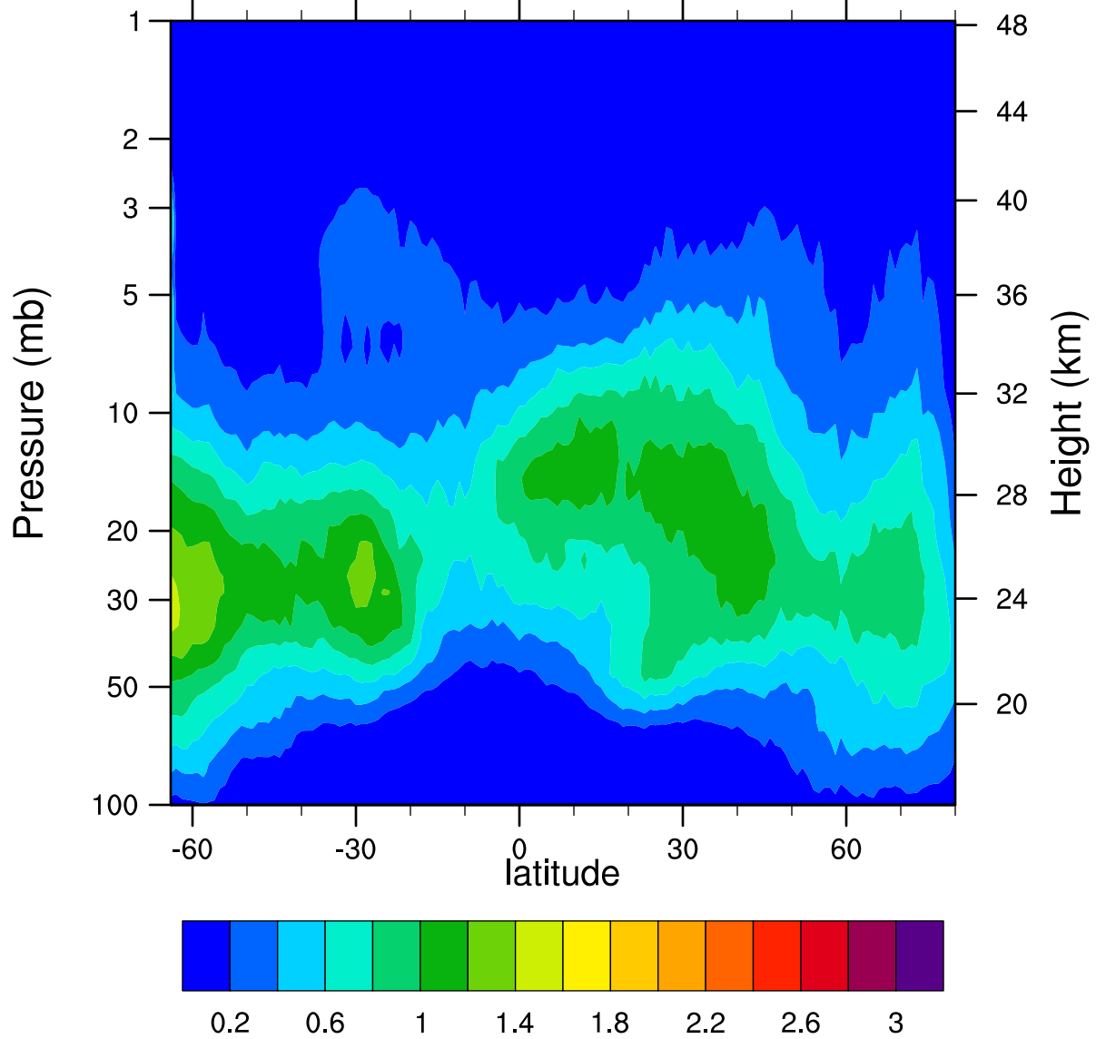
HIRDLSv6 2005d314 ClONO2_Ascending (ppbv)
