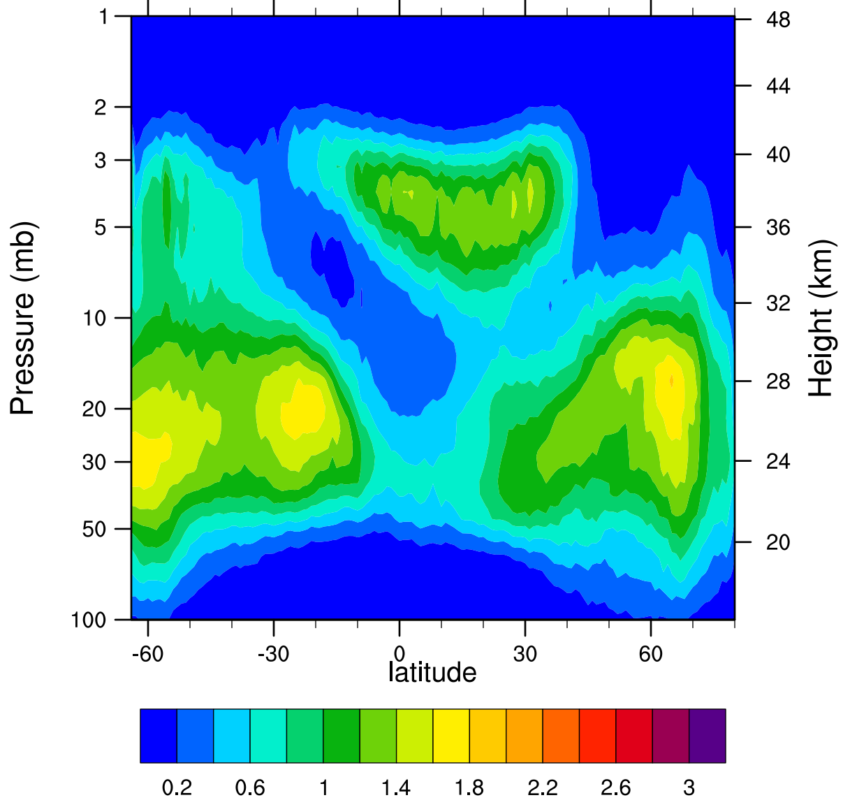
HIRDLSv6 2006d324 ClONO2_Ascending (ppbv)
