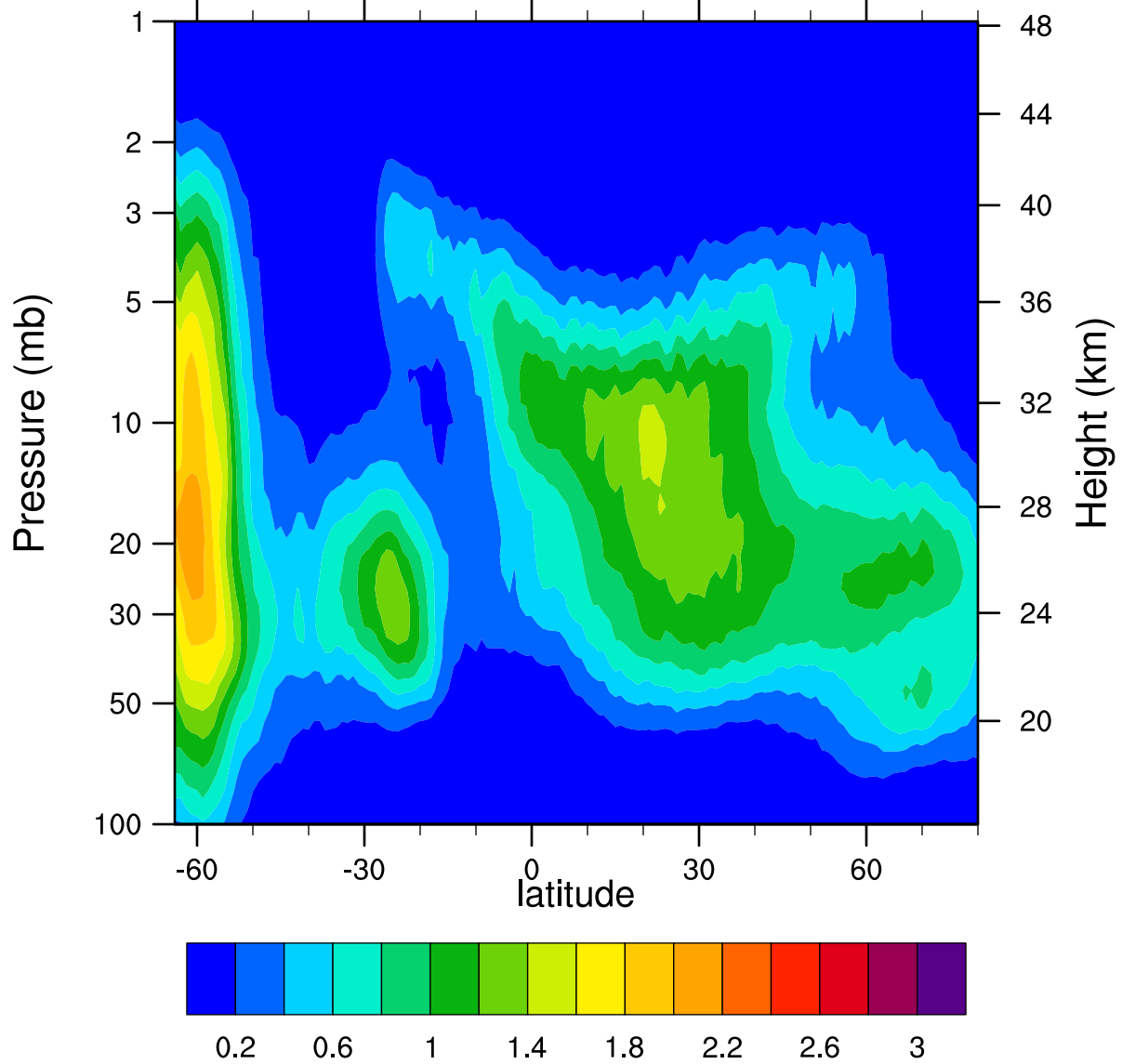
HIRDLSv6 2005d183 ClONO2_Ascending (ppbv)
