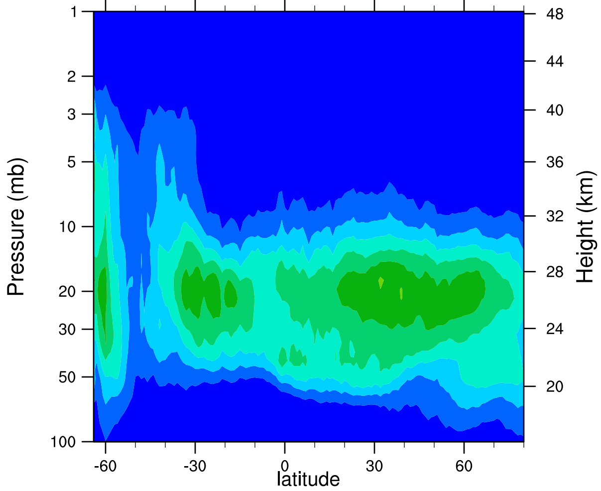
HIRDLSv6 2006d182 ClONO2_Ascending (ppbv)
