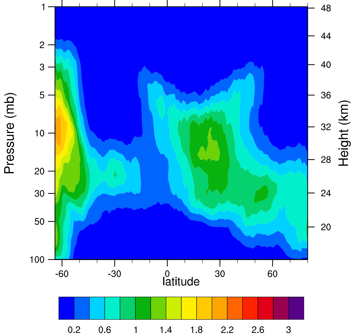
HIRDLSv6 2005d106 ClONO2_Ascending (ppbv)
