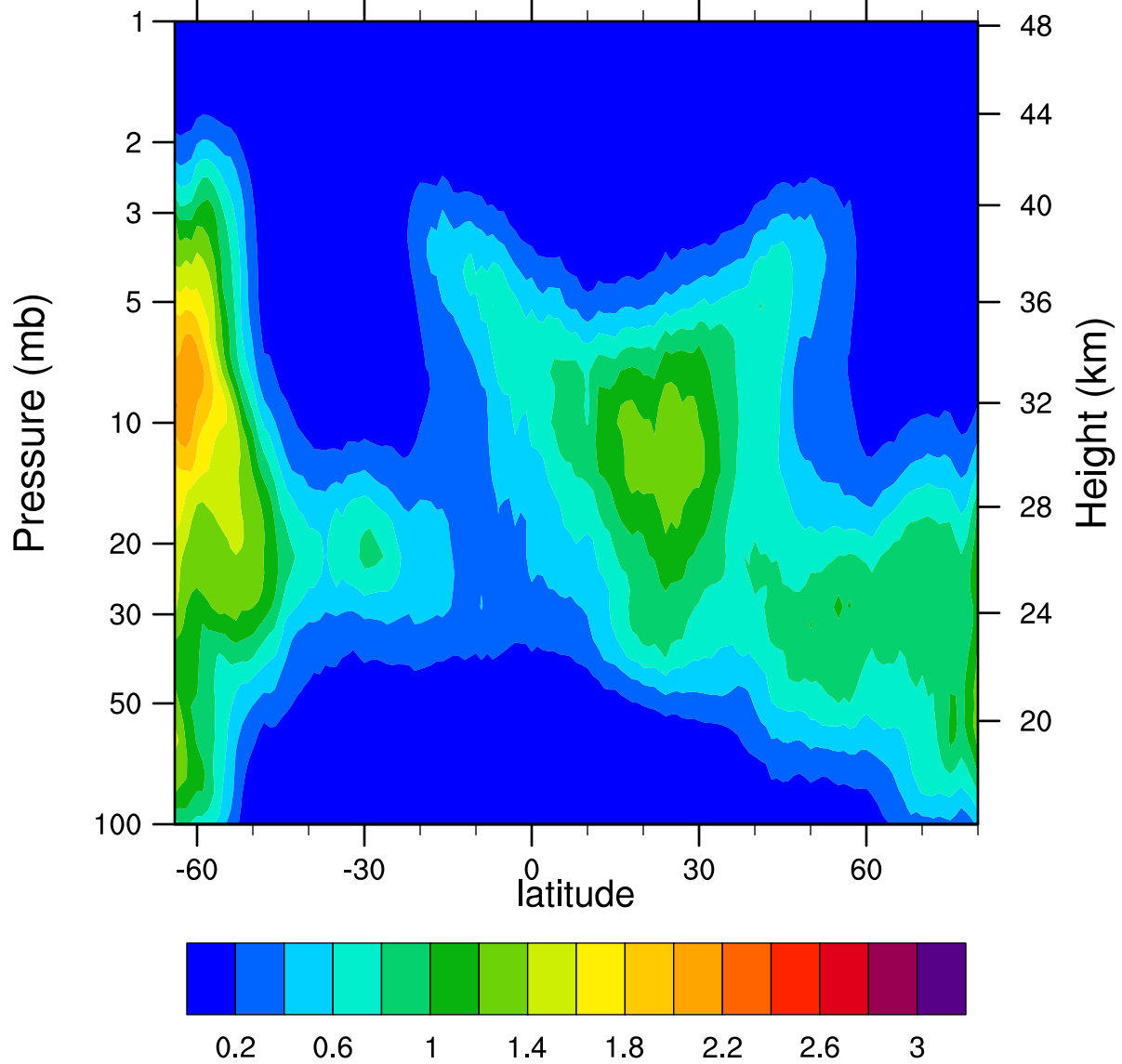
HIRDLSv6 2005d089 ClONO2_Ascending (ppbv)
