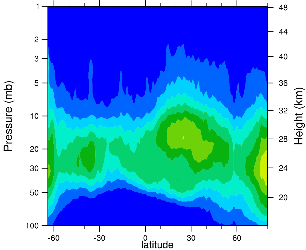
HIRDLSv6 2006d102 ClONO2_Ascending (ppbv)
