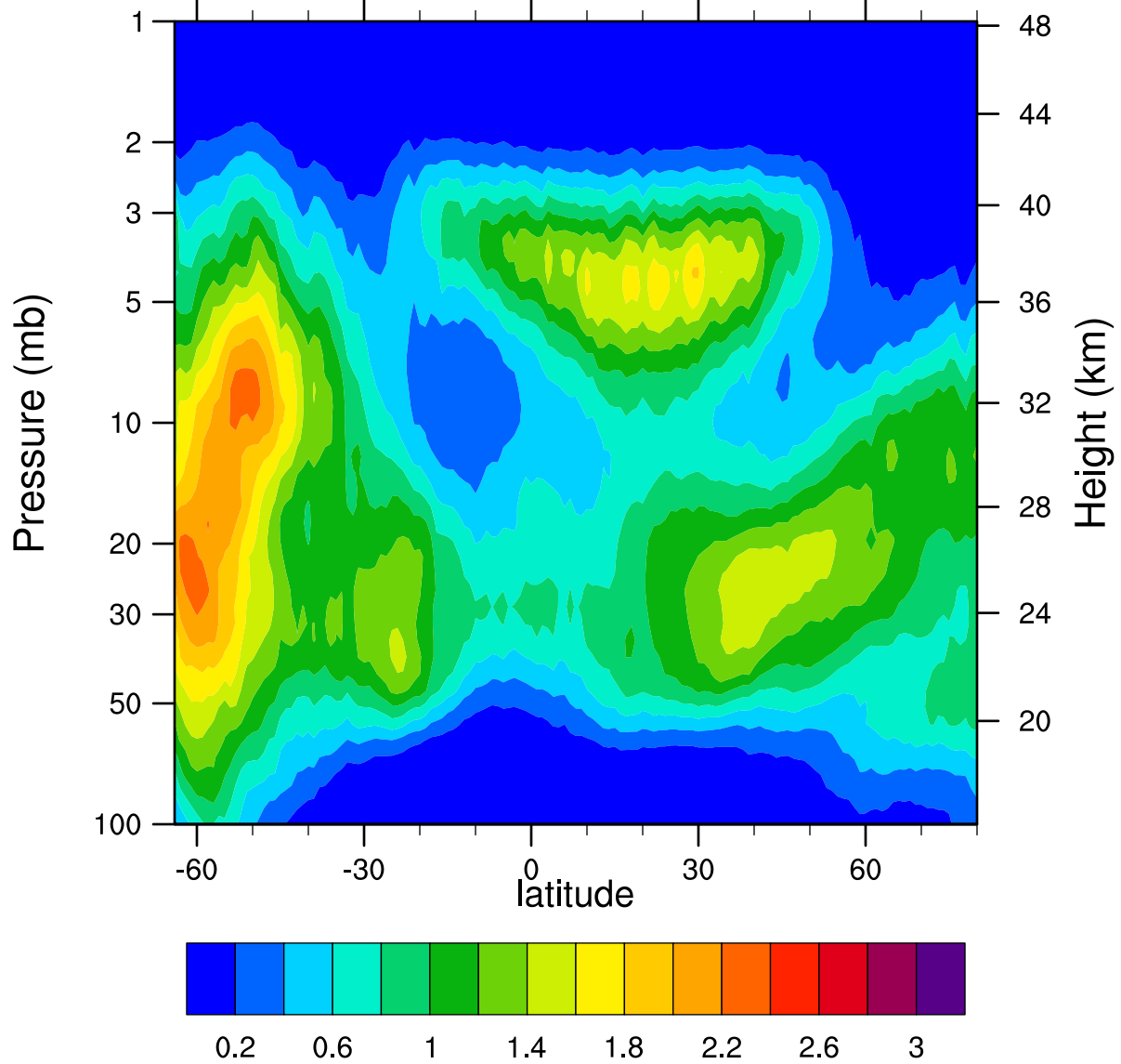
HIRDLSv6 2007d241 ClONO2_Ascending (ppbv)
