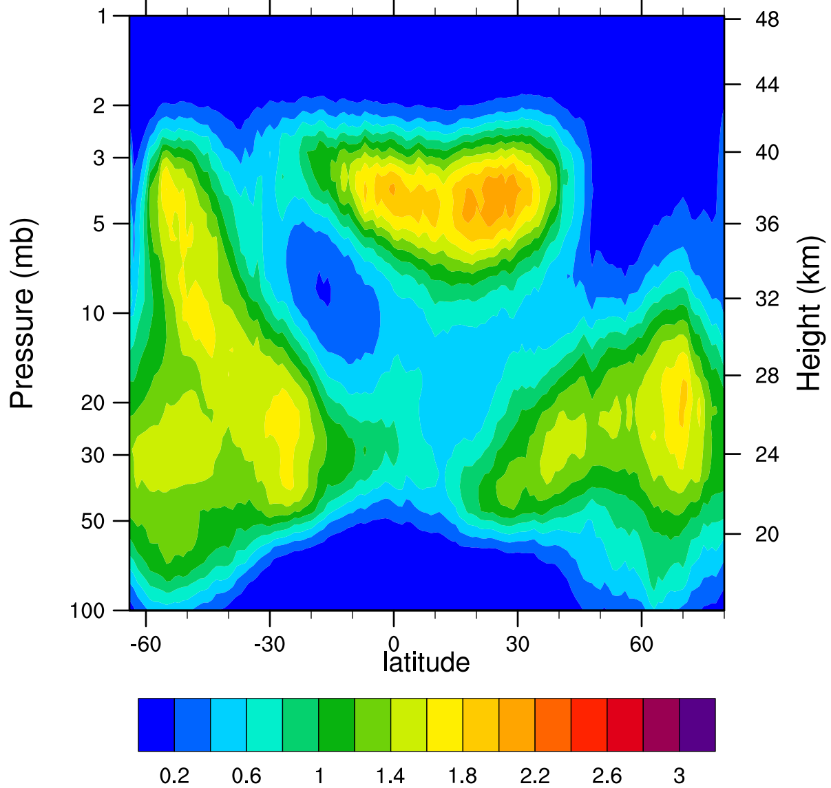
HIRDLSv6 2007d318 ClONO2_Ascending (ppbv)
