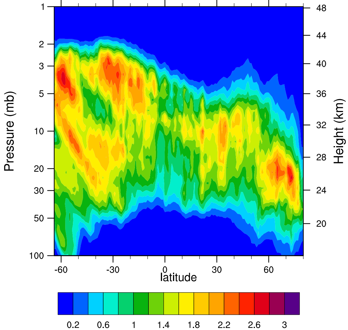
HIRDLSv6 2005d022 ClONO2_Ascending (ppbv)
