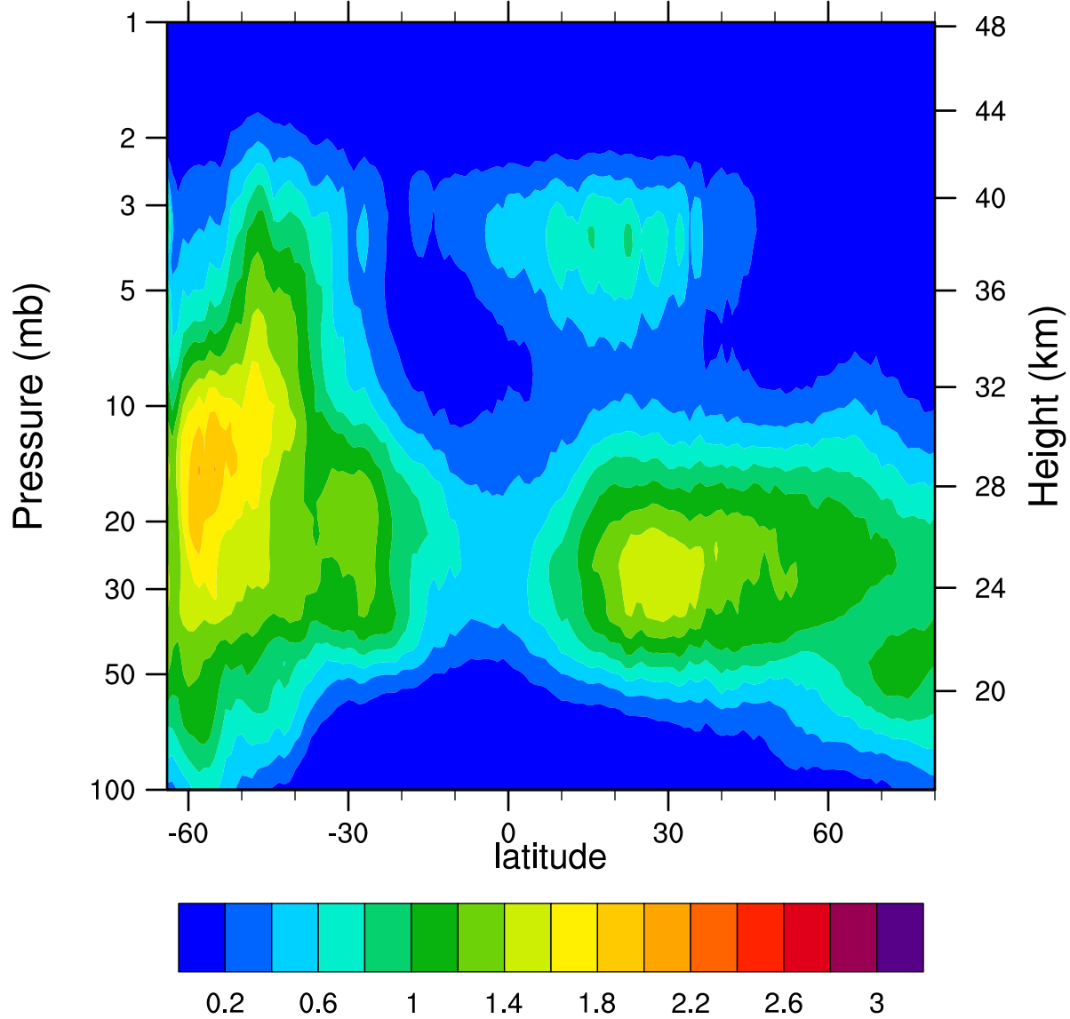
HIRDLSv6 2007d138 ClONO2_Ascending (ppbv)
