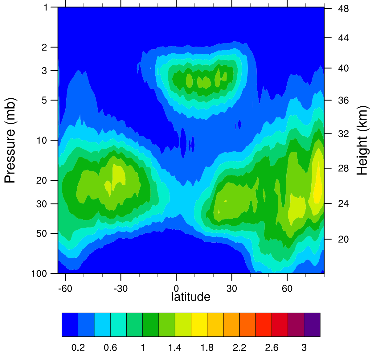
HIRDLSv6 2007d020 ClONO2_Ascending (ppbv)
