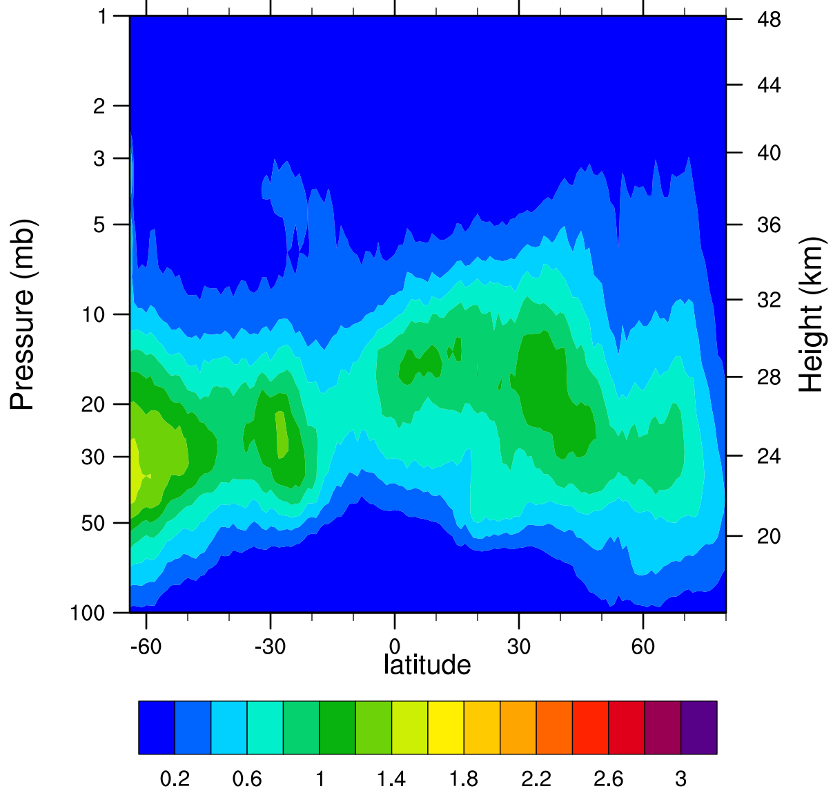
HIRDLSv6 2005d320 ClONO2_Ascending (ppbv)
