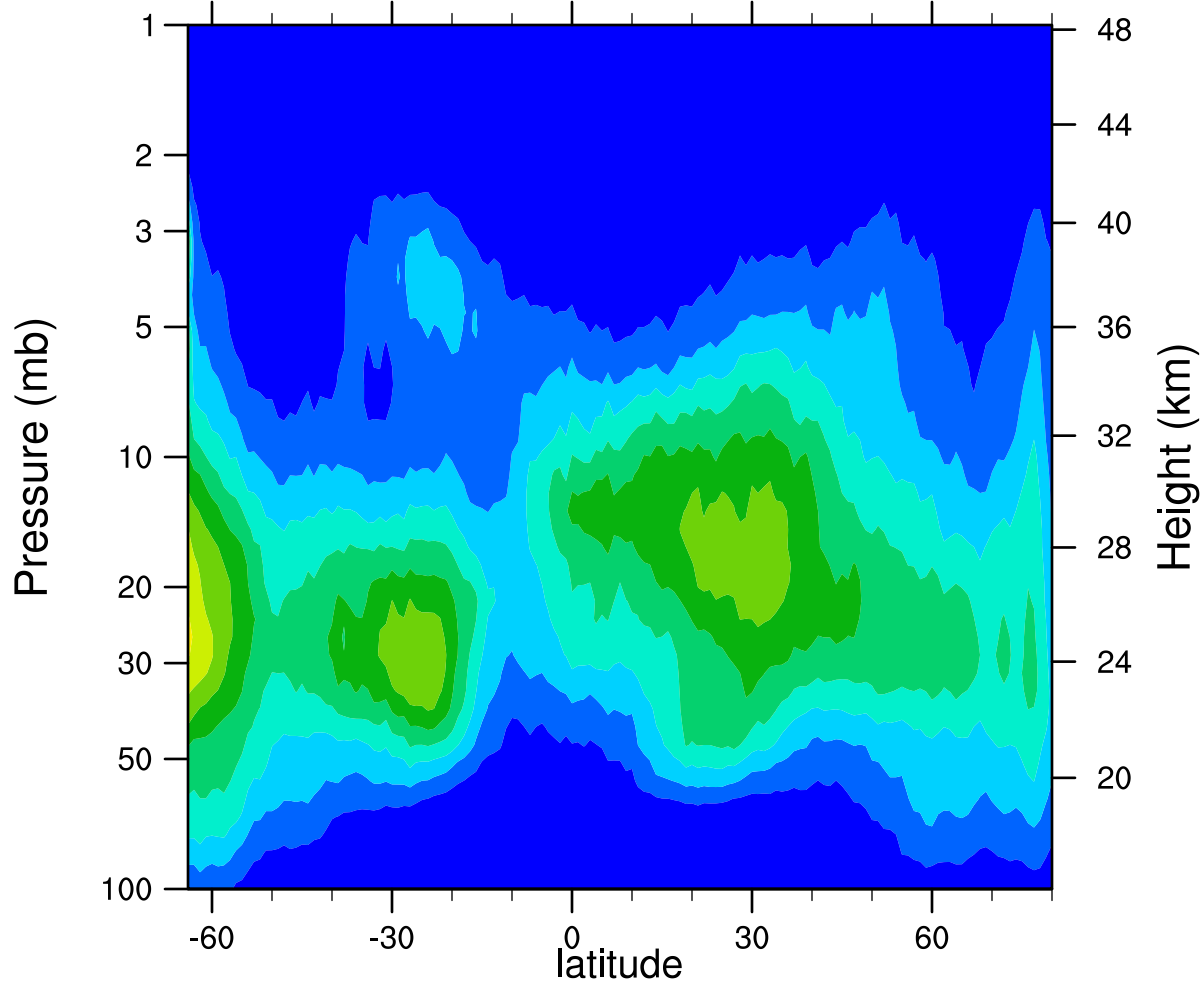
HIRDLSv6 2005d290 ClONO2_Ascending (ppbv)
