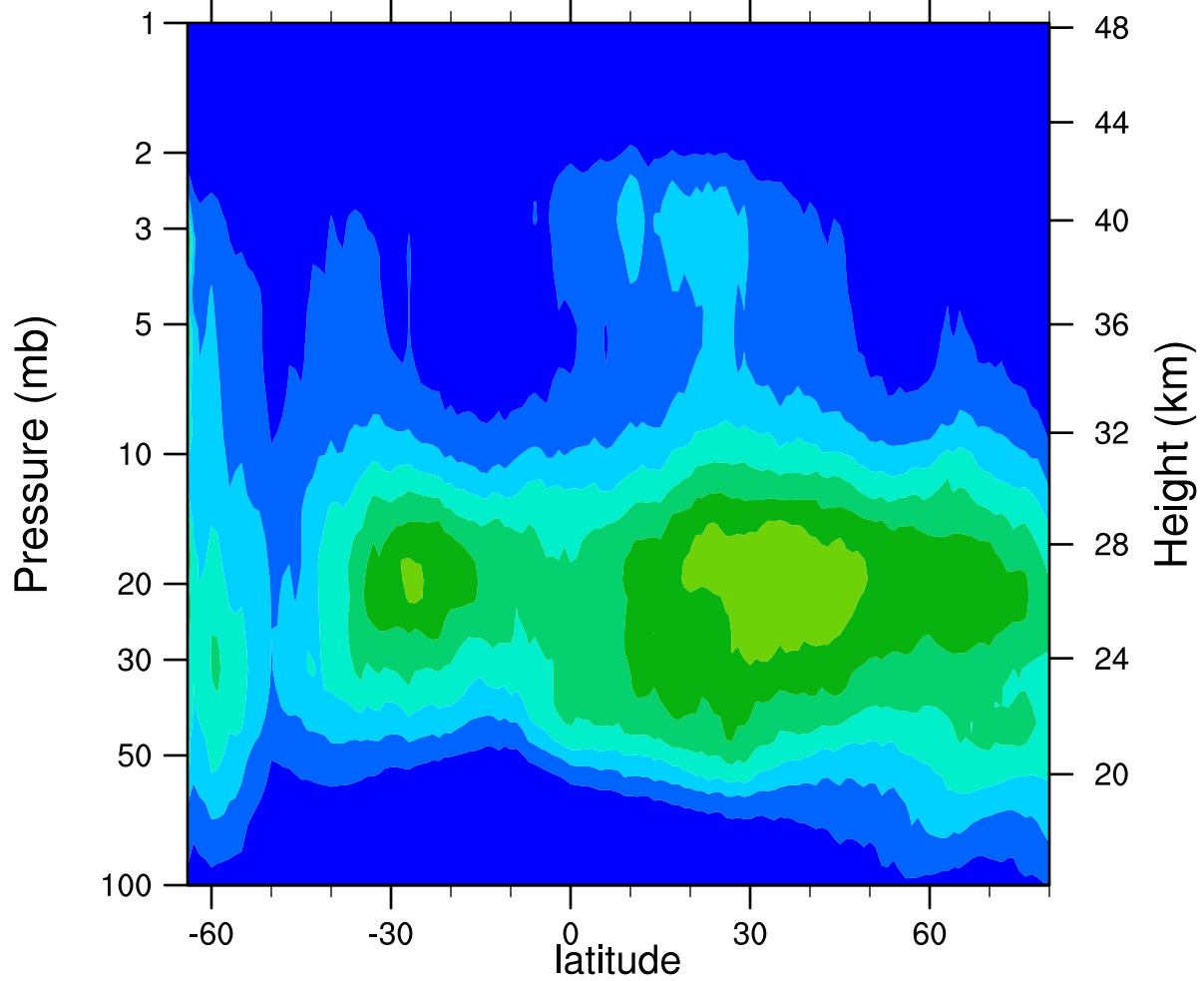
HIRDLSv6 2006d162 ClONO2_Ascending (ppbv)
