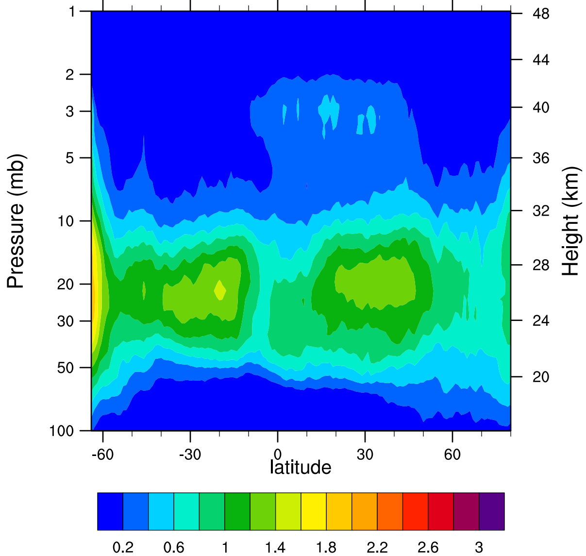
HIRDLSv6 2006d279 ClONO2_Ascending (ppbv)
