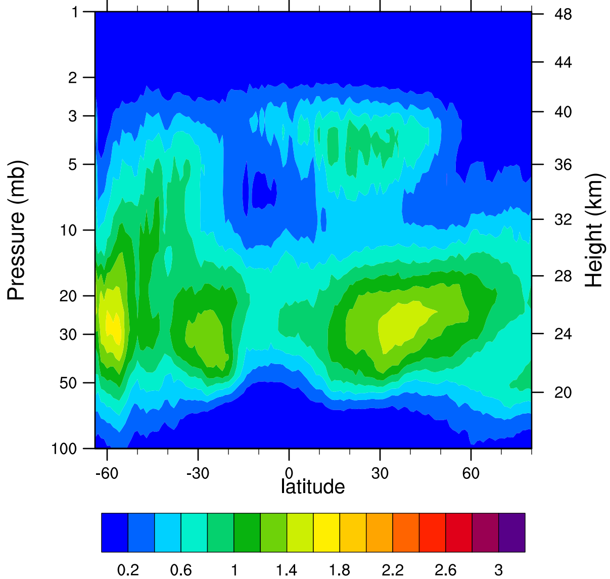
HIRDLSv6 2007d210 ClONO2_Ascending (ppbv)
