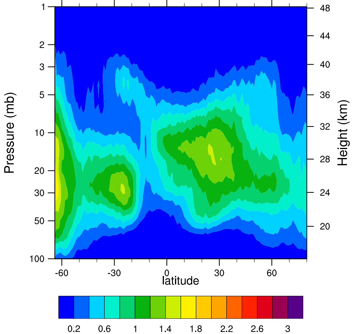
HIRDLSv6 2005d275 ClONO2_Ascending (ppbv)
