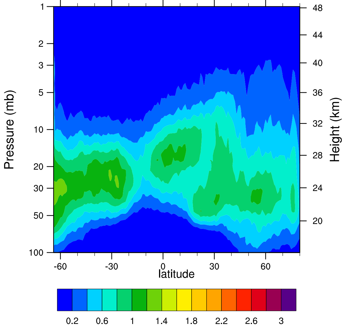
HIRDLSv6 2005d345 ClONO2_Ascending (ppbv)
