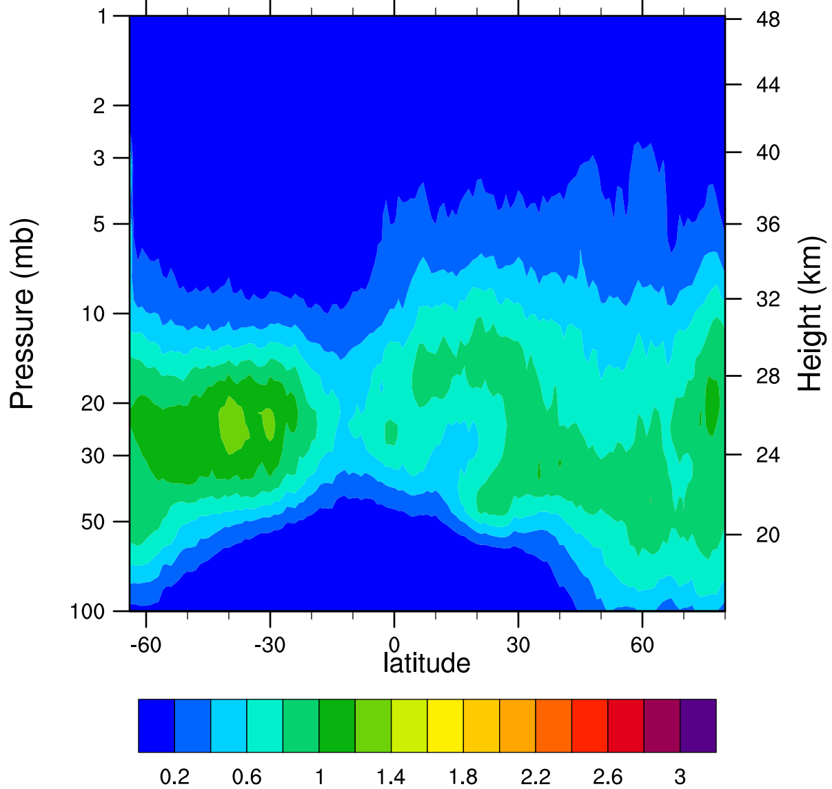
HIRDLSv6 2006d012 ClONO2_Ascending (ppbv)
