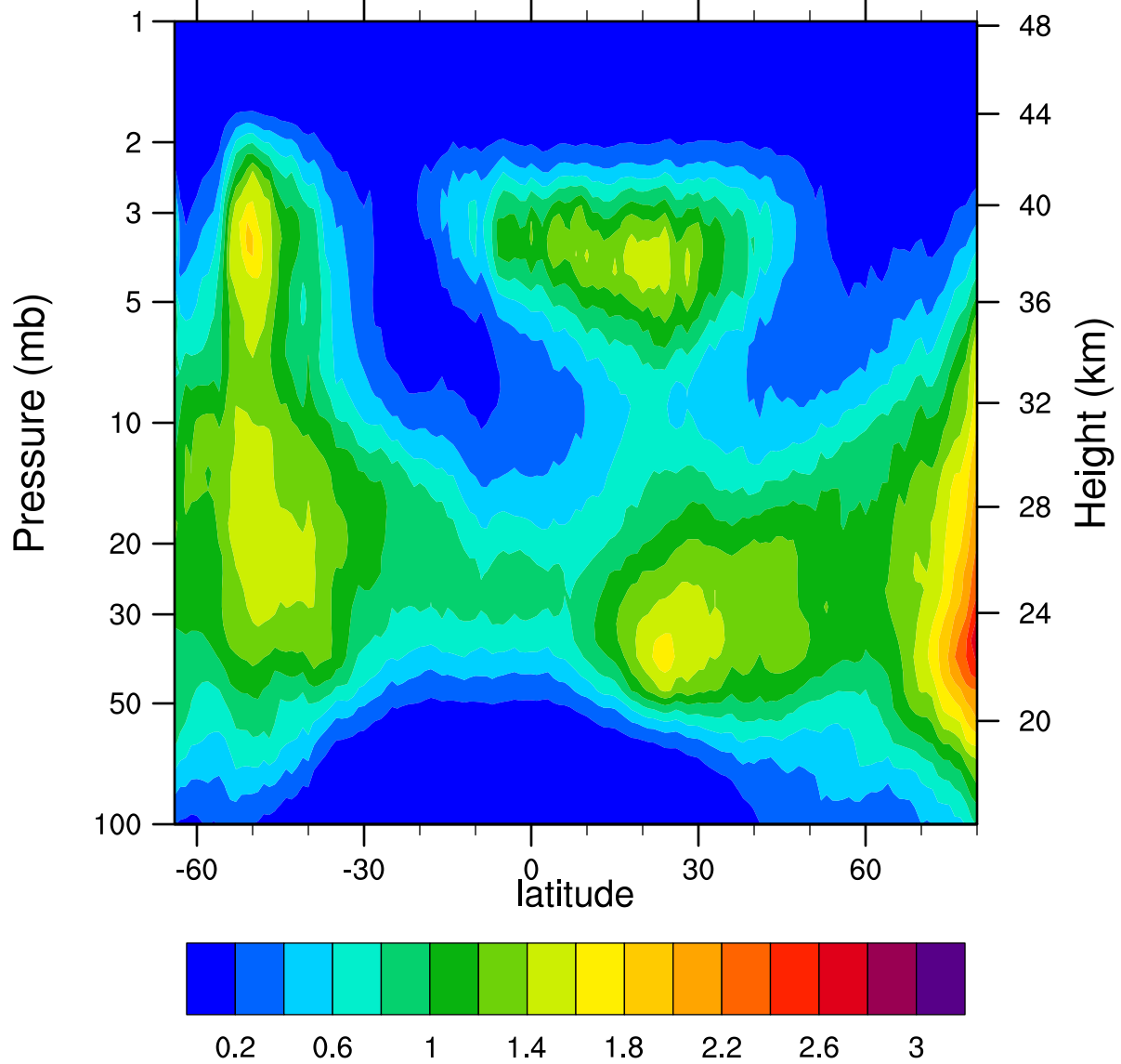
HIRDLSv6 2007d083 ClONO2_Ascending (ppbv)
