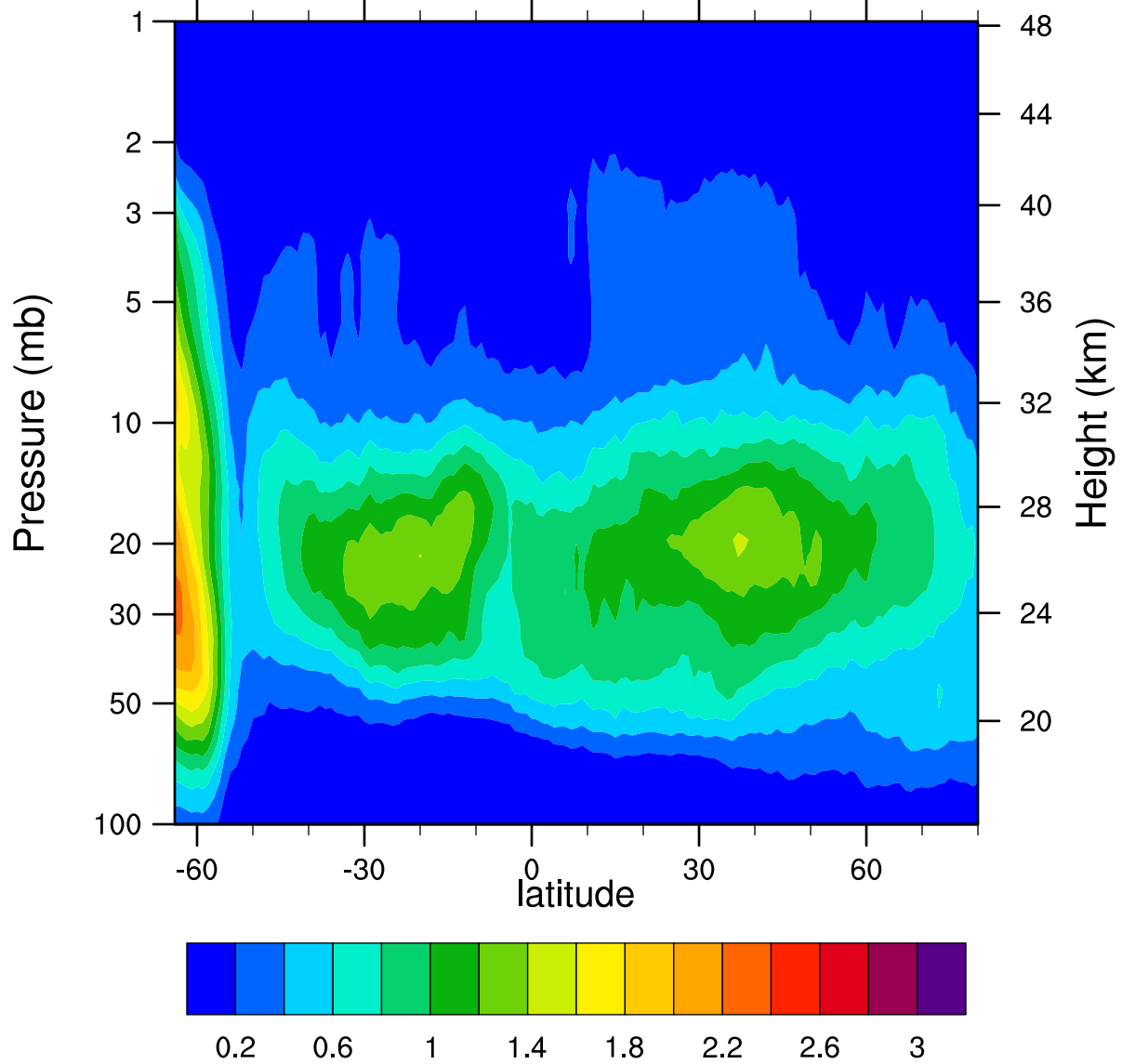
HIRDLSv6 2006d247 ClONO2_Ascending (ppbv)
