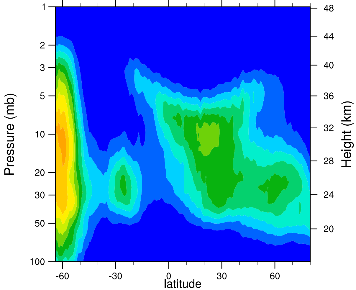
HIRDLSv6 2005d156 ClONO2_Ascending (ppbv)
