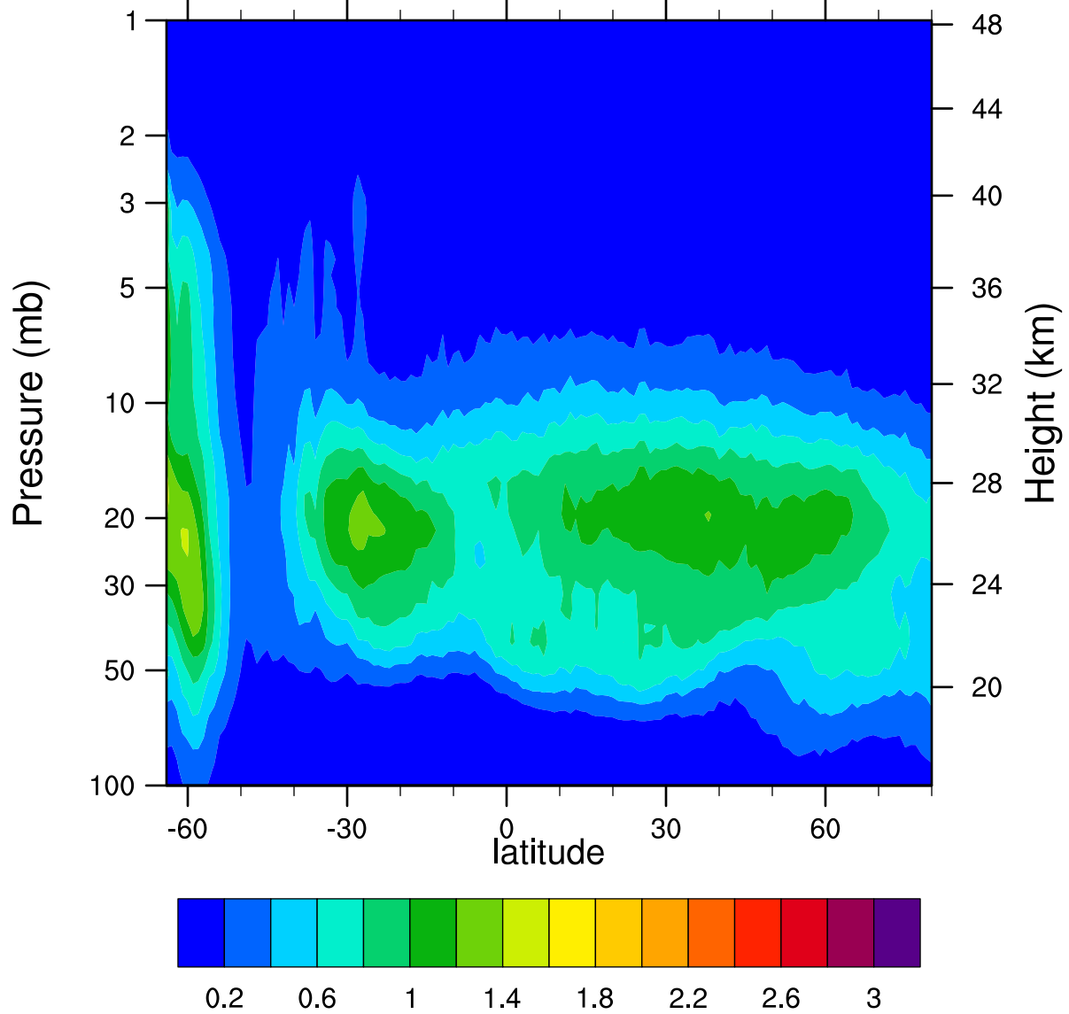
HIRDLSv6 2006d189 ClONO2_Ascending (ppbv)
