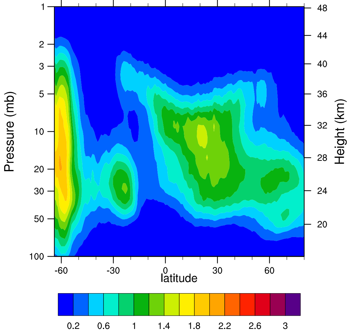
HIRDLSv6 2005d180 ClONO2_Ascending (ppbv)
