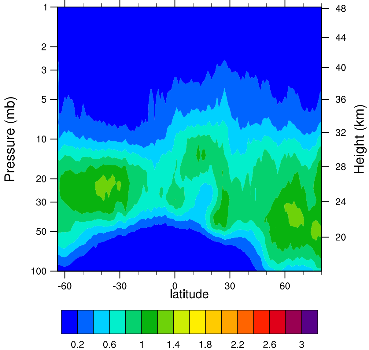
HIRDLSv6 2006d032 ClONO2_Ascending (ppbv)
