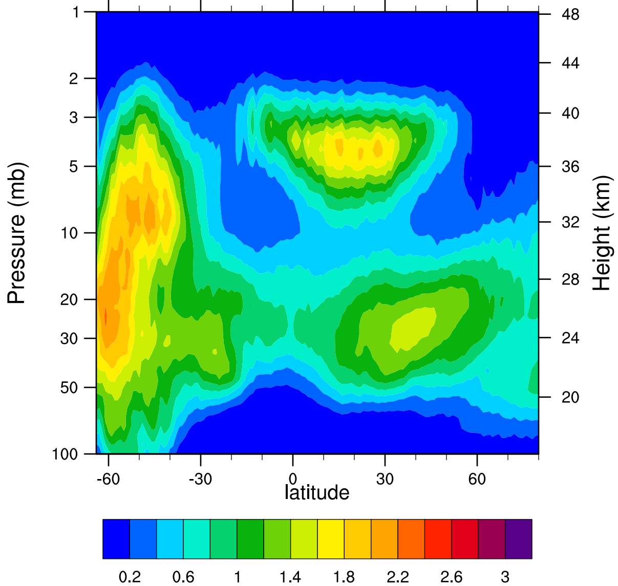
HIRDLSv6 2007d215 ClONO2_Ascending (ppbv)
