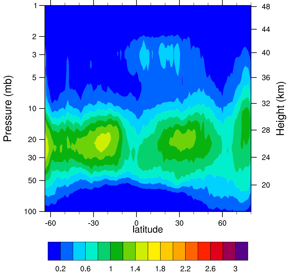
HIRDLSv6 2006d297 ClONO2_Ascending (ppbv)
