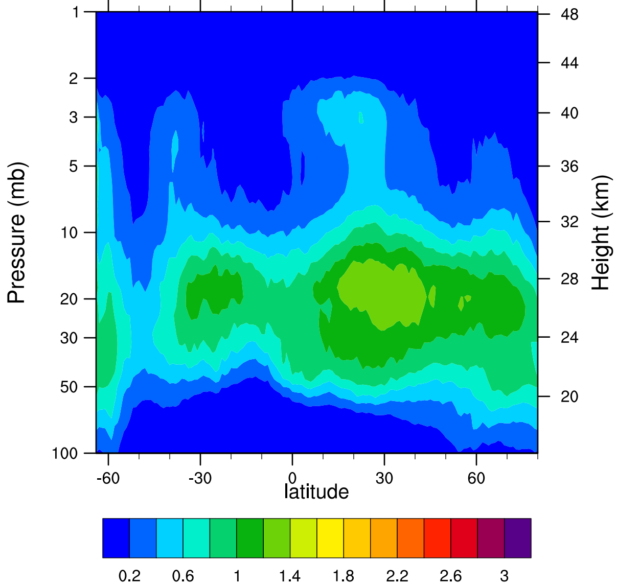
HIRDLSv6 2006d148 ClONO2_Ascending (ppbv)
