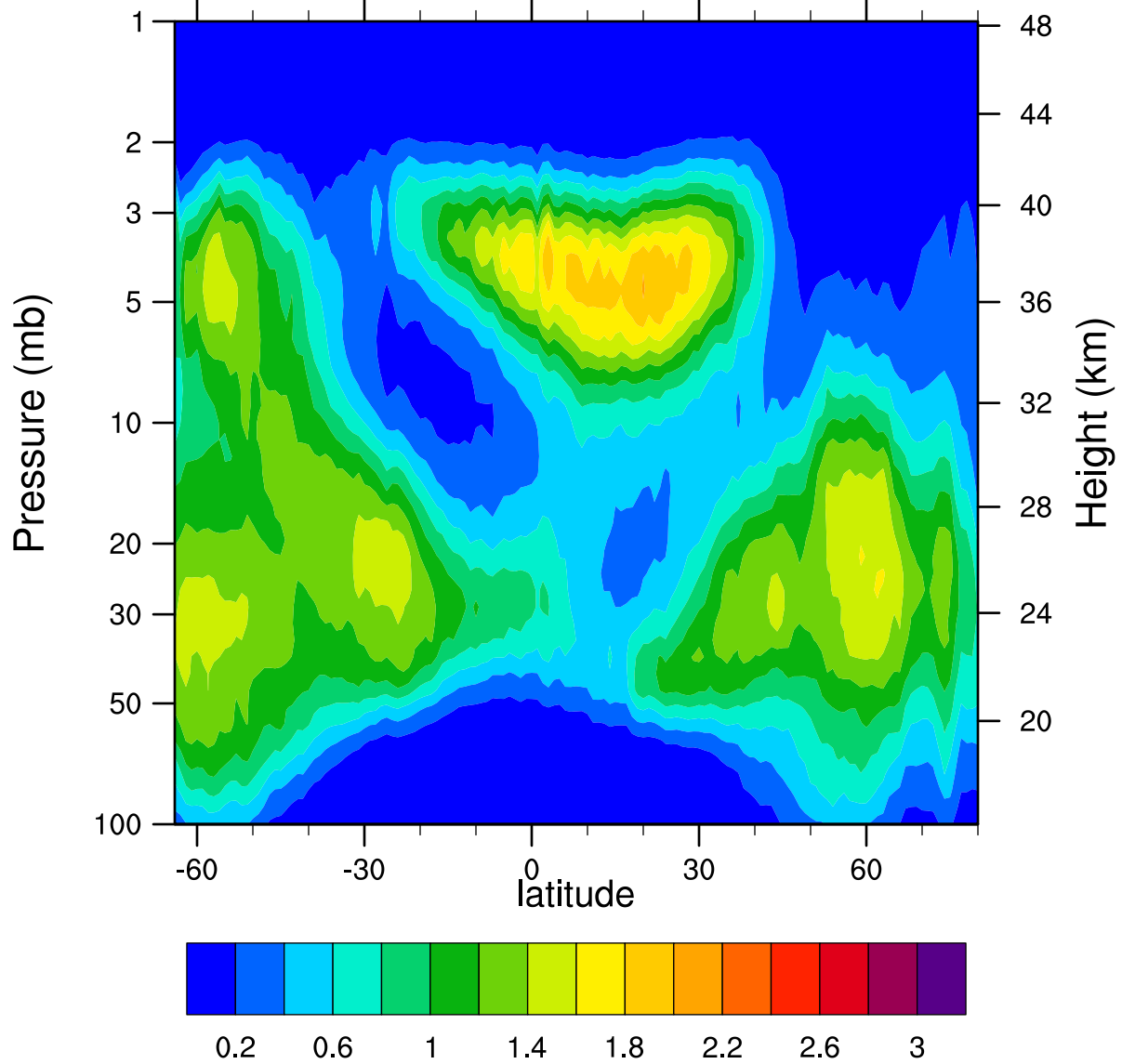
HIRDLSv6 2007d340 ClONO2_Ascending (ppbv)
