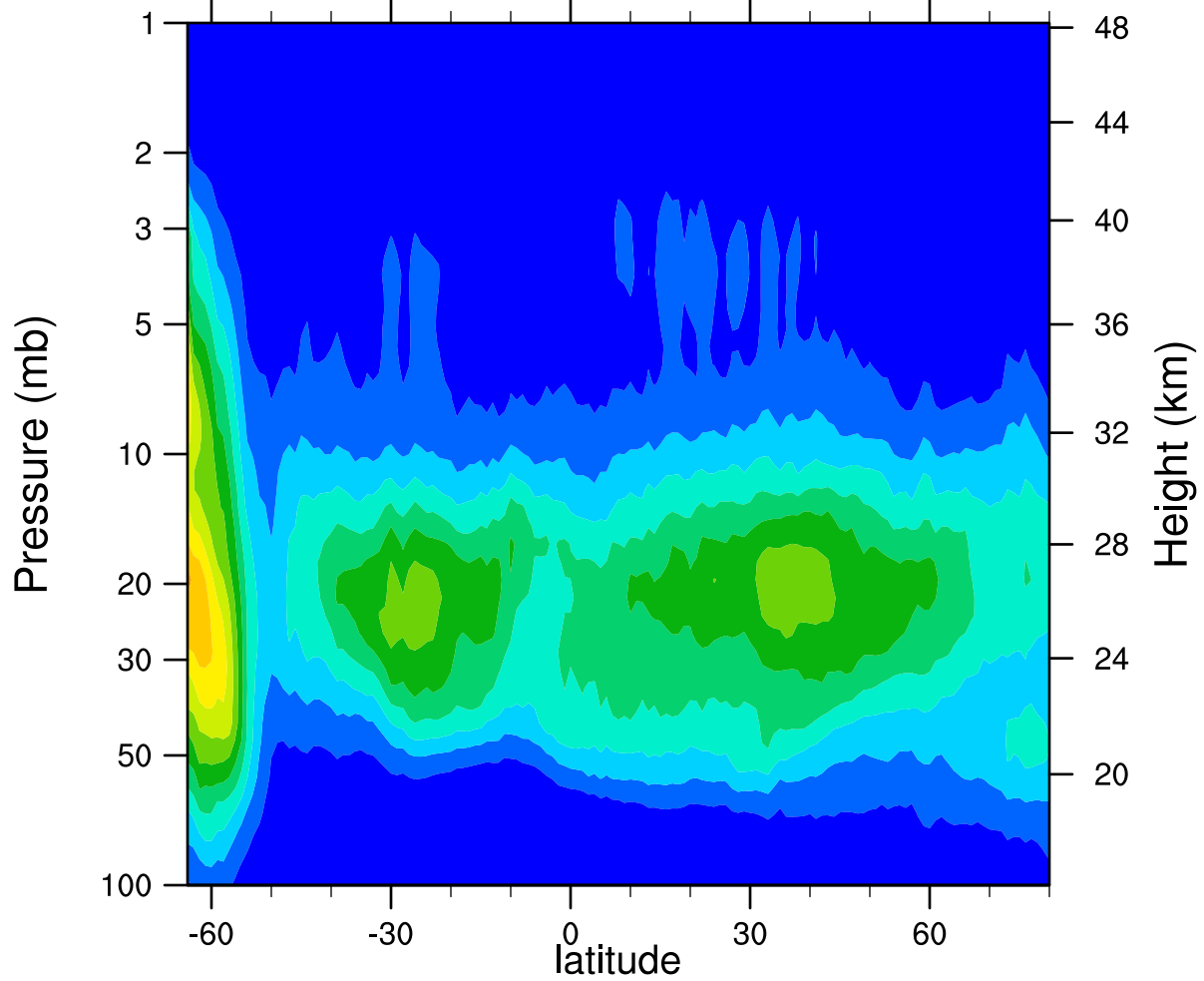
HIRDLSv6 2006d231 ClONO2_Ascending (ppbv)
