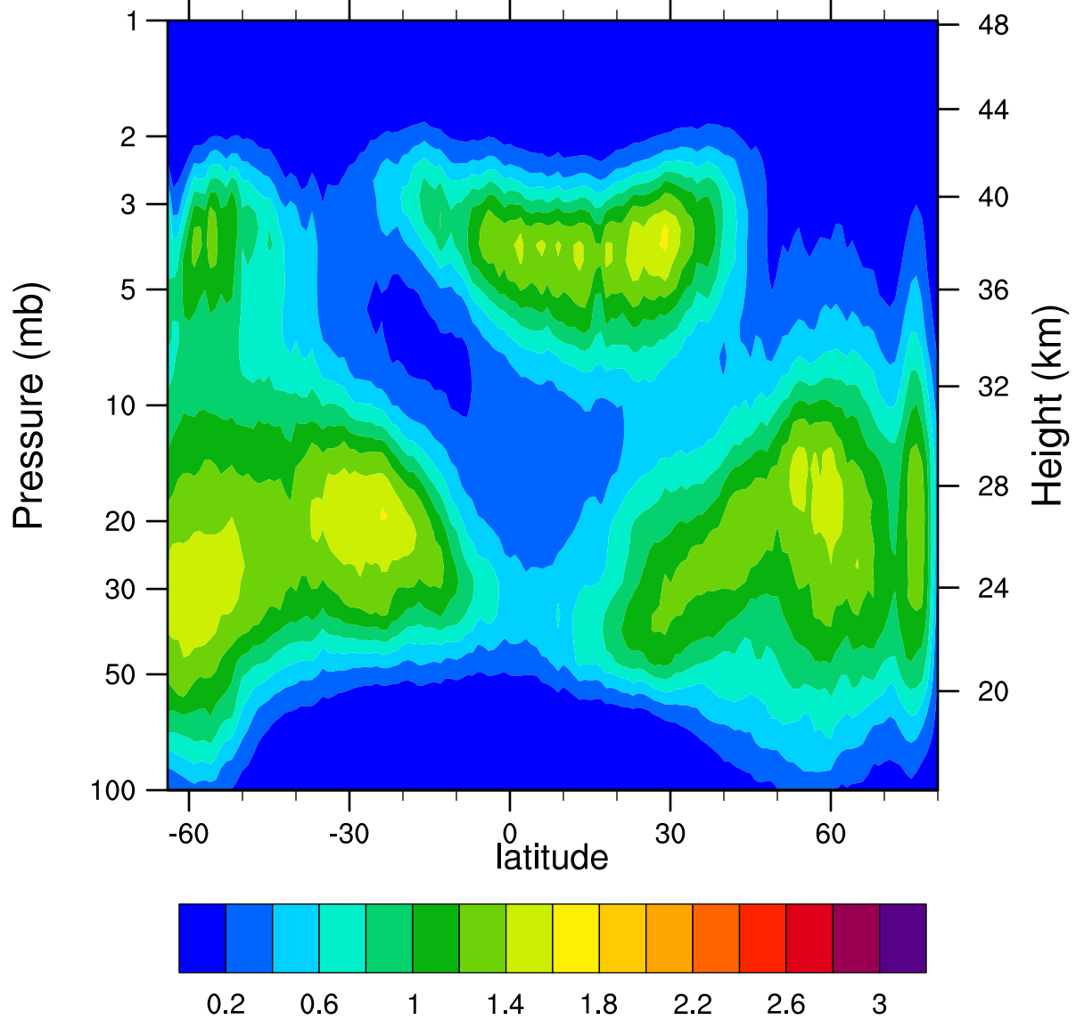
HIRDLSv6 2006d345 ClONO2_Ascending (ppbv)
