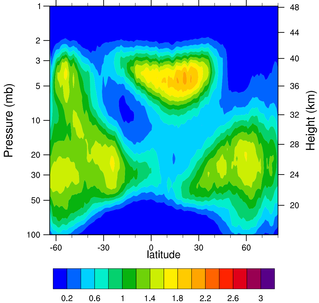
HIRDLSv6 2007d329 ClONO2_Ascending (ppbv)
