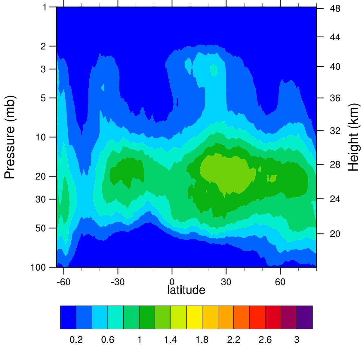
HIRDLSv6 2006d150 ClONO2_Ascending (ppbv)
