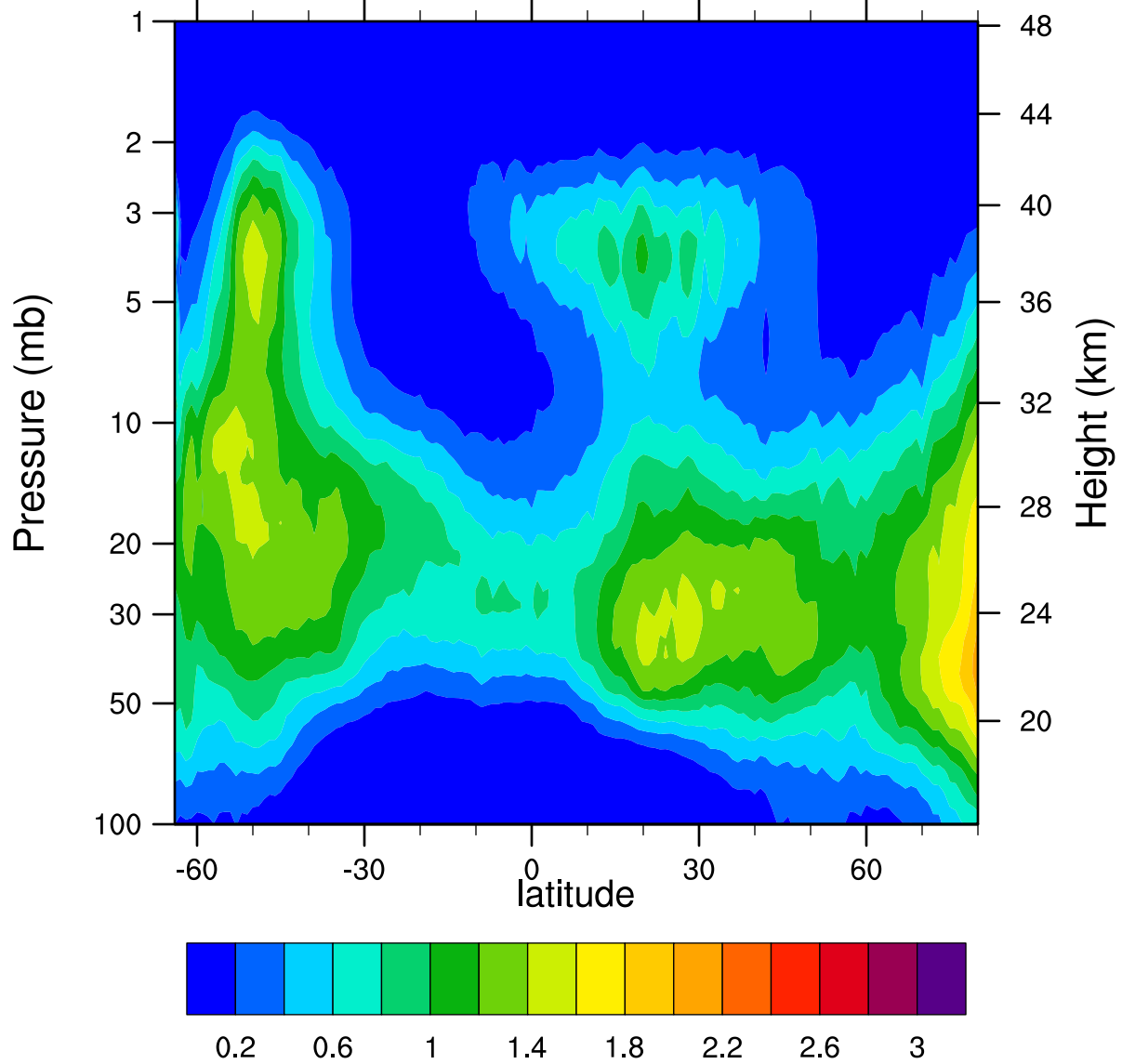
HIRDLSv6 2007d091 ClONO2_Ascending (ppbv)
