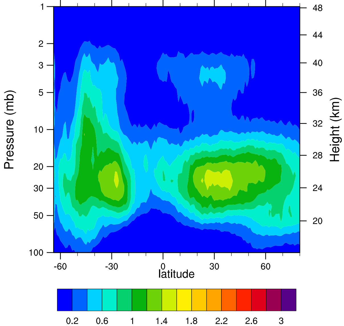
HIRDLSv6 2007d179 ClONO2_Ascending (ppbv)
