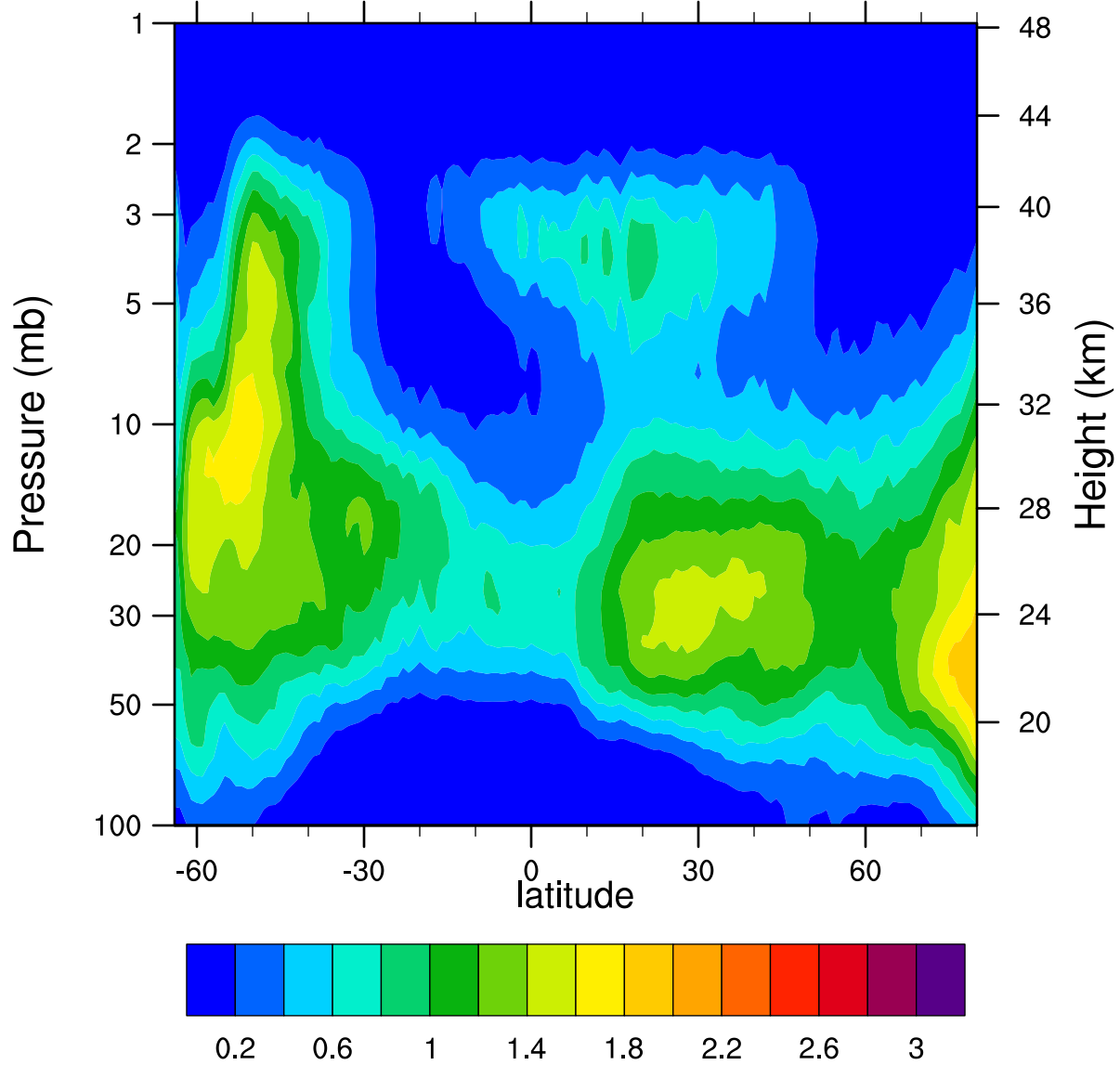
HIRDLSv6 2007d102 ClONO2_Ascending (ppbv)
