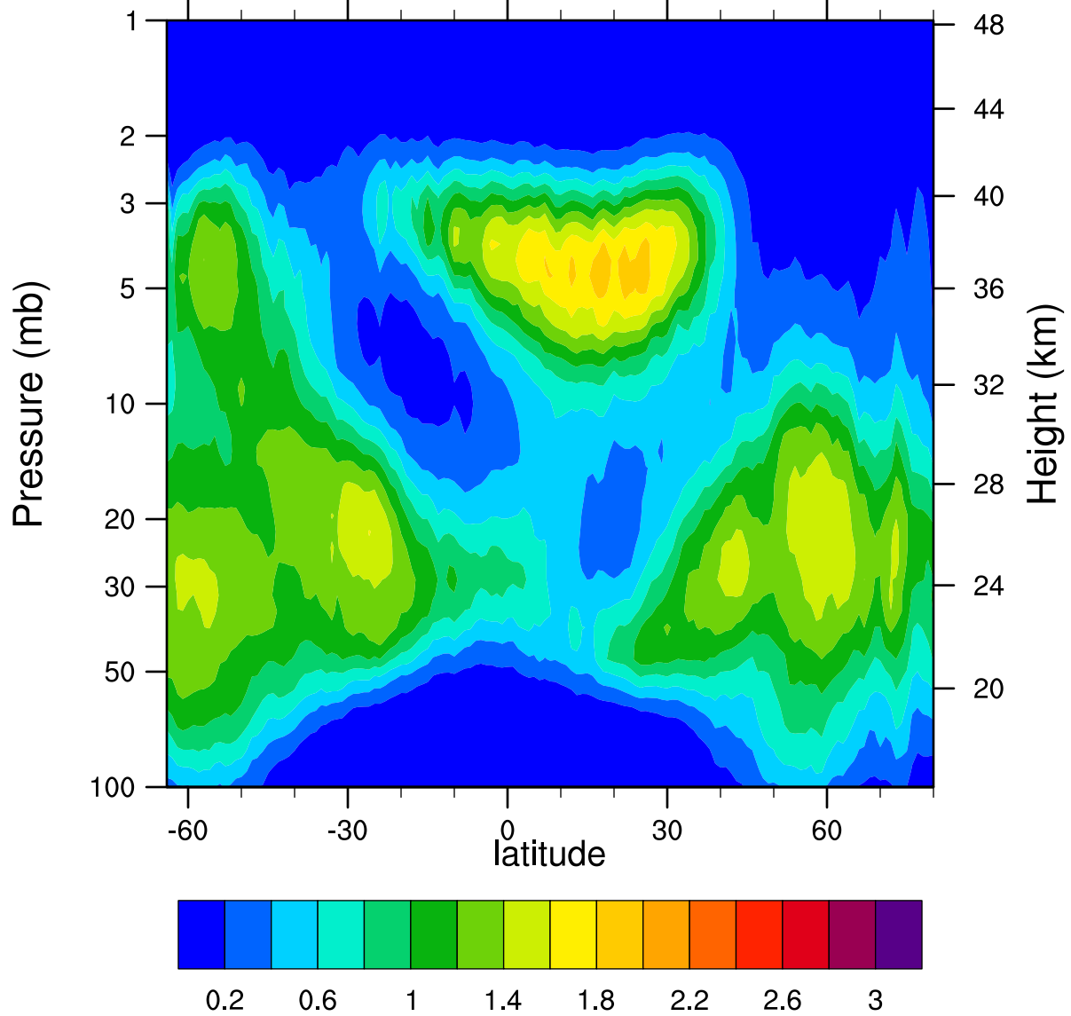
HIRDLSv6 2007d344 ClONO2_Ascending (ppbv)
