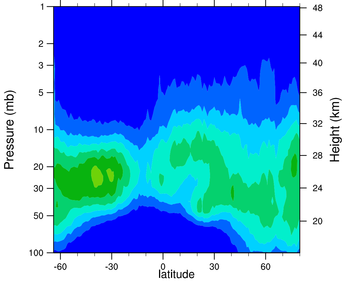
HIRDLSv6 2006d011 ClONO2_Ascending (ppbv)
