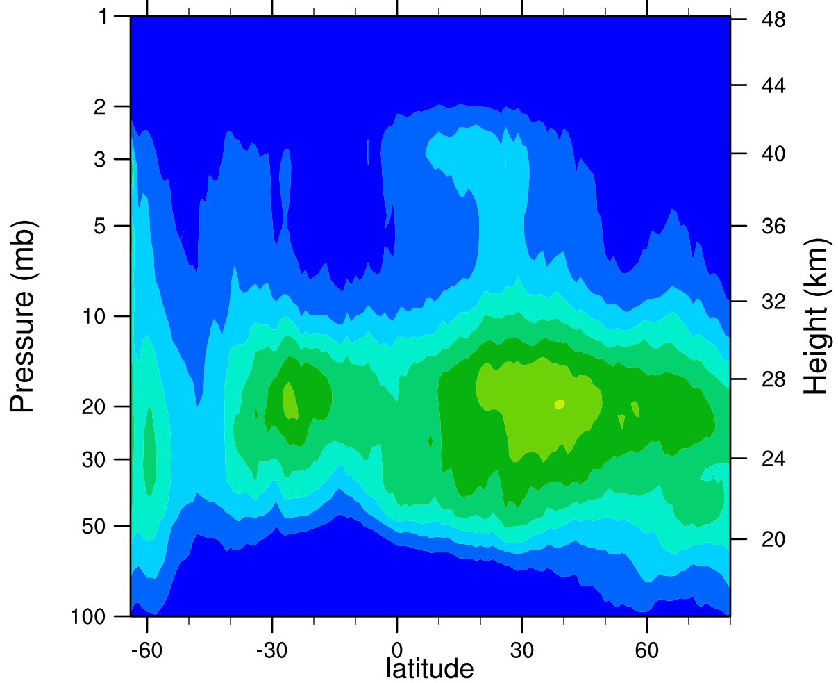
HIRDLSv6 2006d157 ClONO2_Ascending (ppbv)
