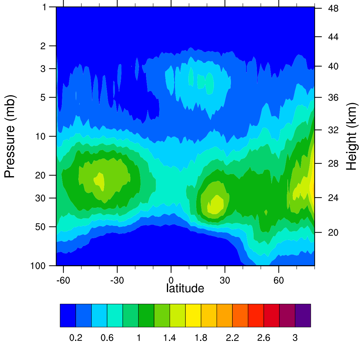
HIRDLSv6 2007d042 ClONO2_Ascending (ppbv)
