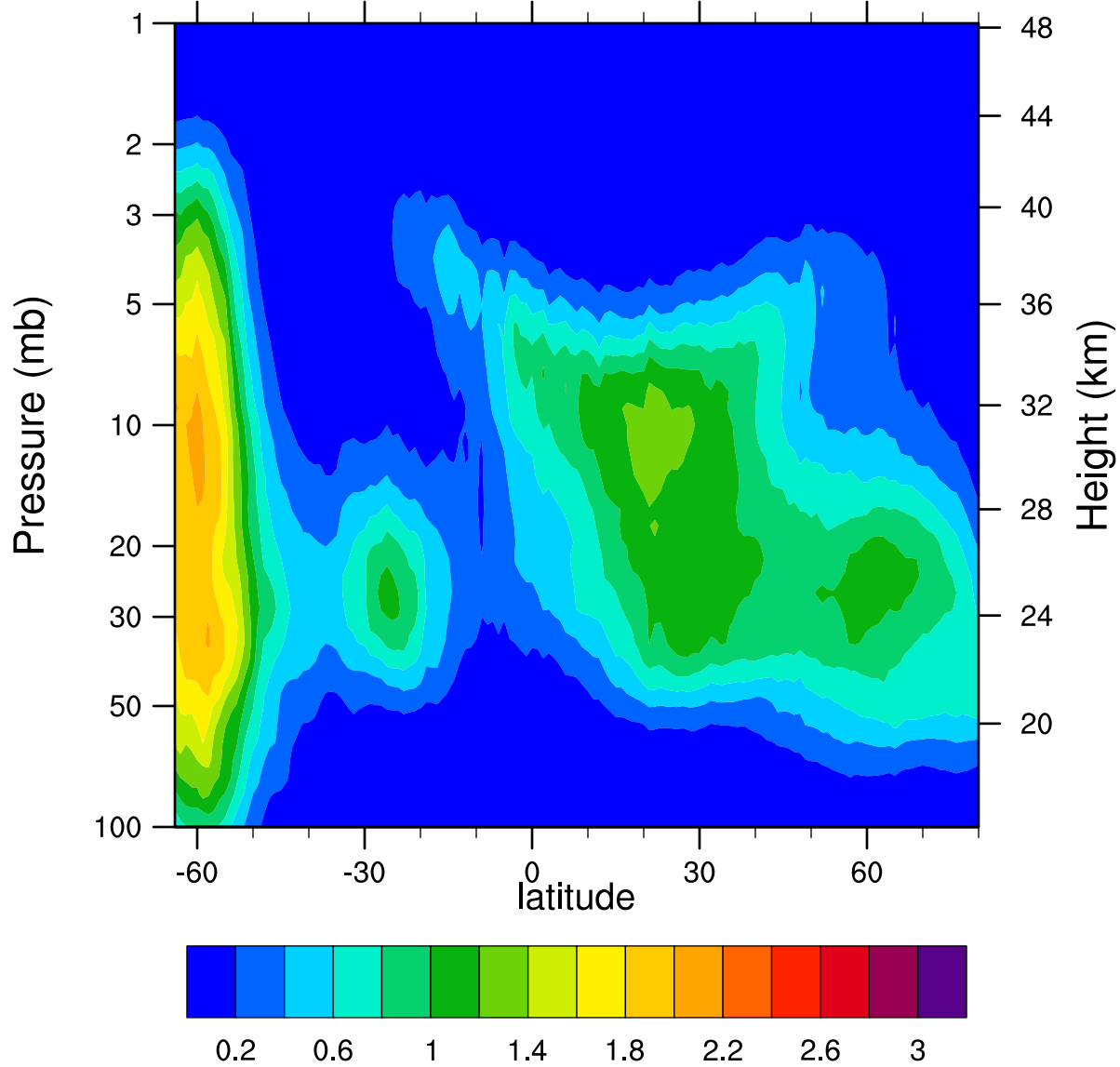
HIRDLSv6 2005d159 ClONO2_Ascending (ppbv)
