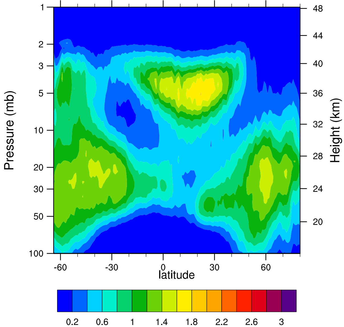
HIRDLSv6 2007d365 ClONO2_Ascending (ppbv)
