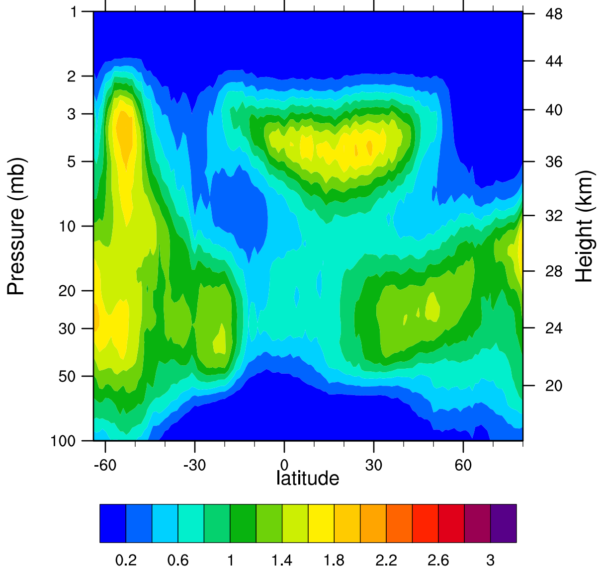
HIRDLSv6 2007d273 ClONO2_Ascending (ppbv)
