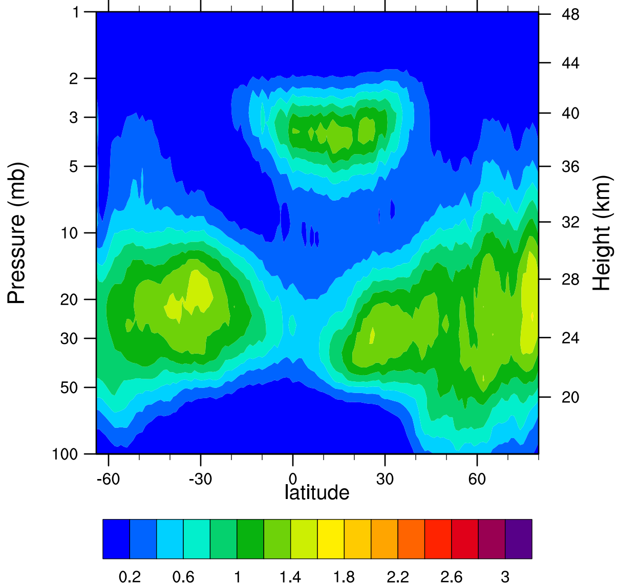
HIRDLSv6 2007d023 ClONO2_Ascending (ppbv)
