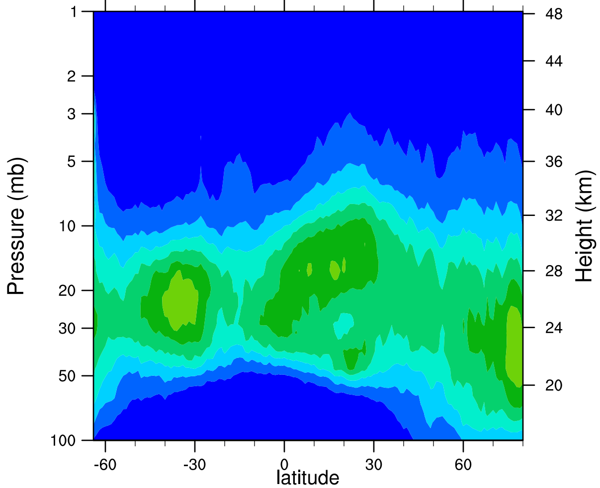
HIRDLSv6 2006d067 ClONO2_Ascending (ppbv)
