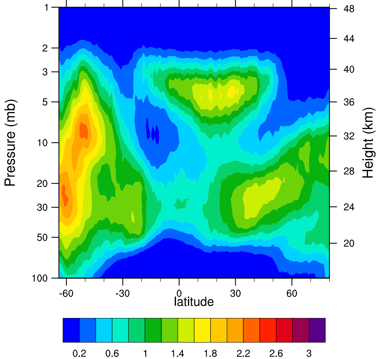
HIRDLSv6 2007d245 ClONO2_Ascending (ppbv)
