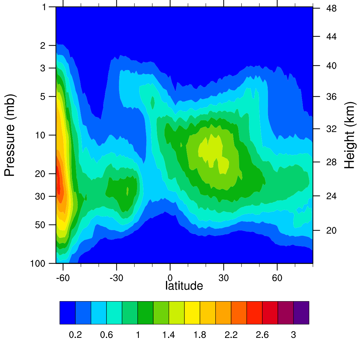
HIRDLSv6 2005d224 ClONO2_Ascending (ppbv)
