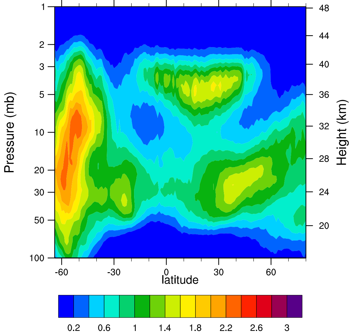
HIRDLSv6 2007d232 ClONO2_Ascending (ppbv)
