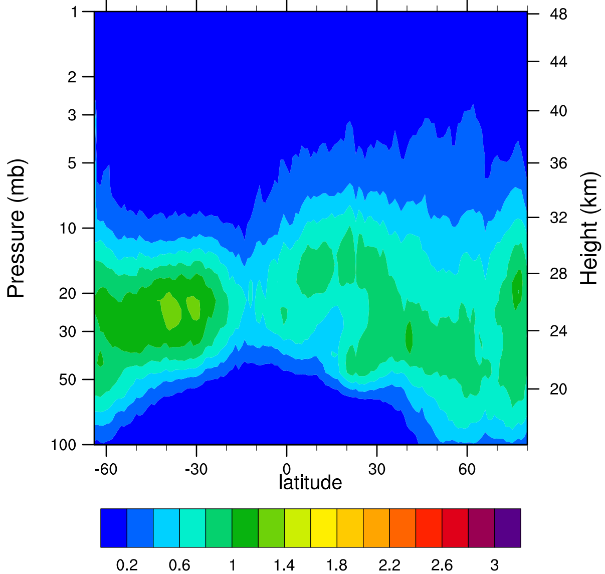
HIRDLSv6 2006d010 ClONO2_Ascending (ppbv)
