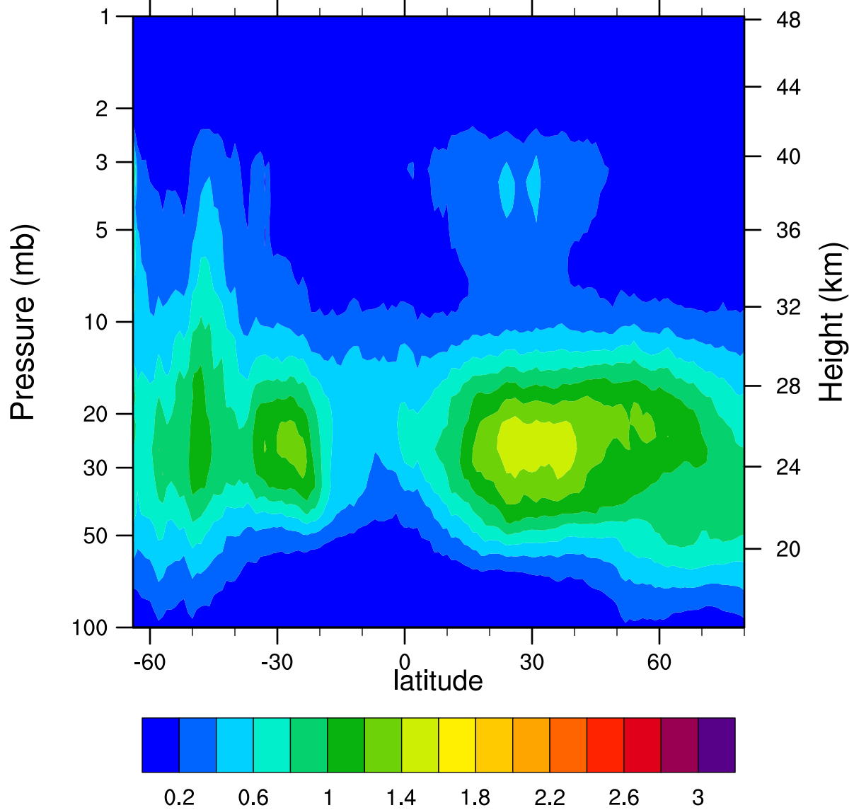
HIRDLSv6 2007d169 ClONO2_Ascending (ppbv)
