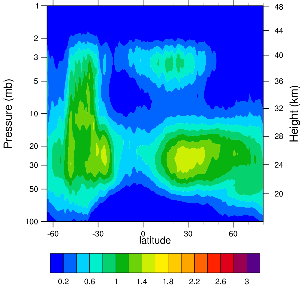
HIRDLSv6 2007d161 ClONO2_Ascending (ppbv)
