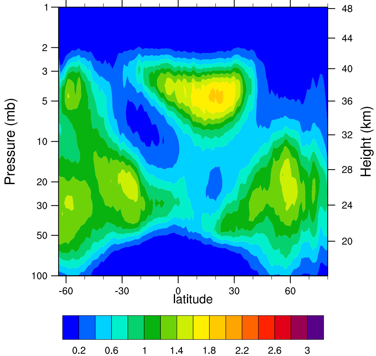
HIRDLSv6 2007d350 ClONO2_Ascending (ppbv)
