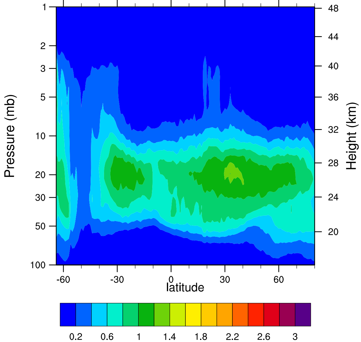
HIRDLSv6 2006d177 ClONO2_Ascending (ppbv)
