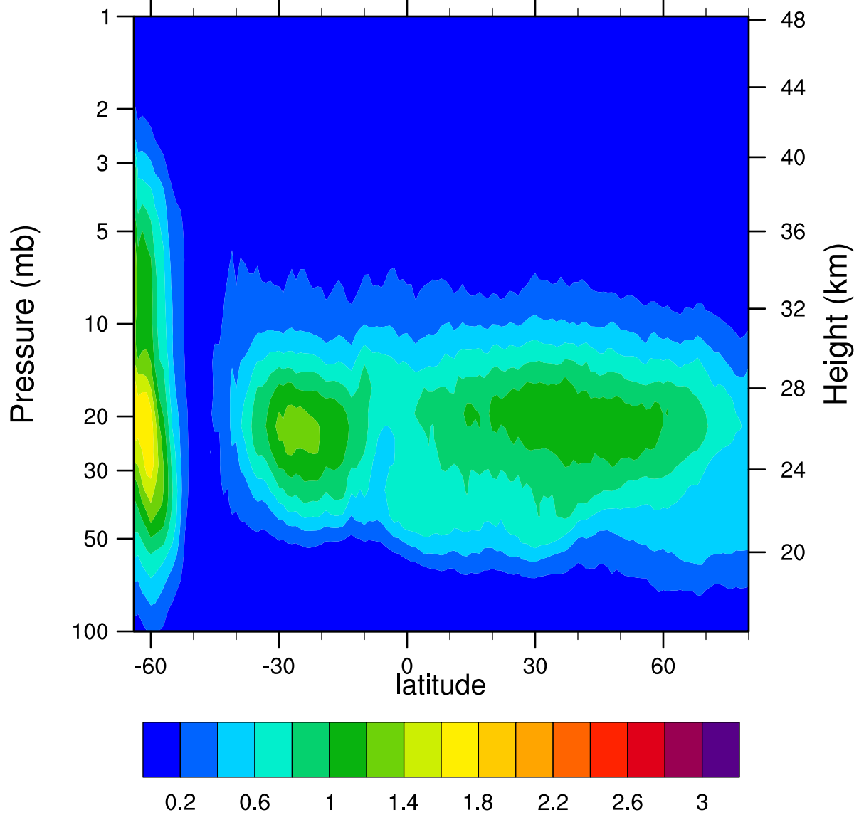
HIRDLSv6 2006d210 ClONO2_Ascending (ppbv)
