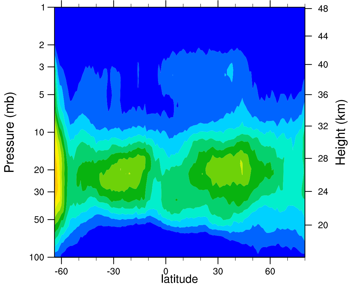
HIRDLSv6 2006d269 ClONO2_Ascending (ppbv)
