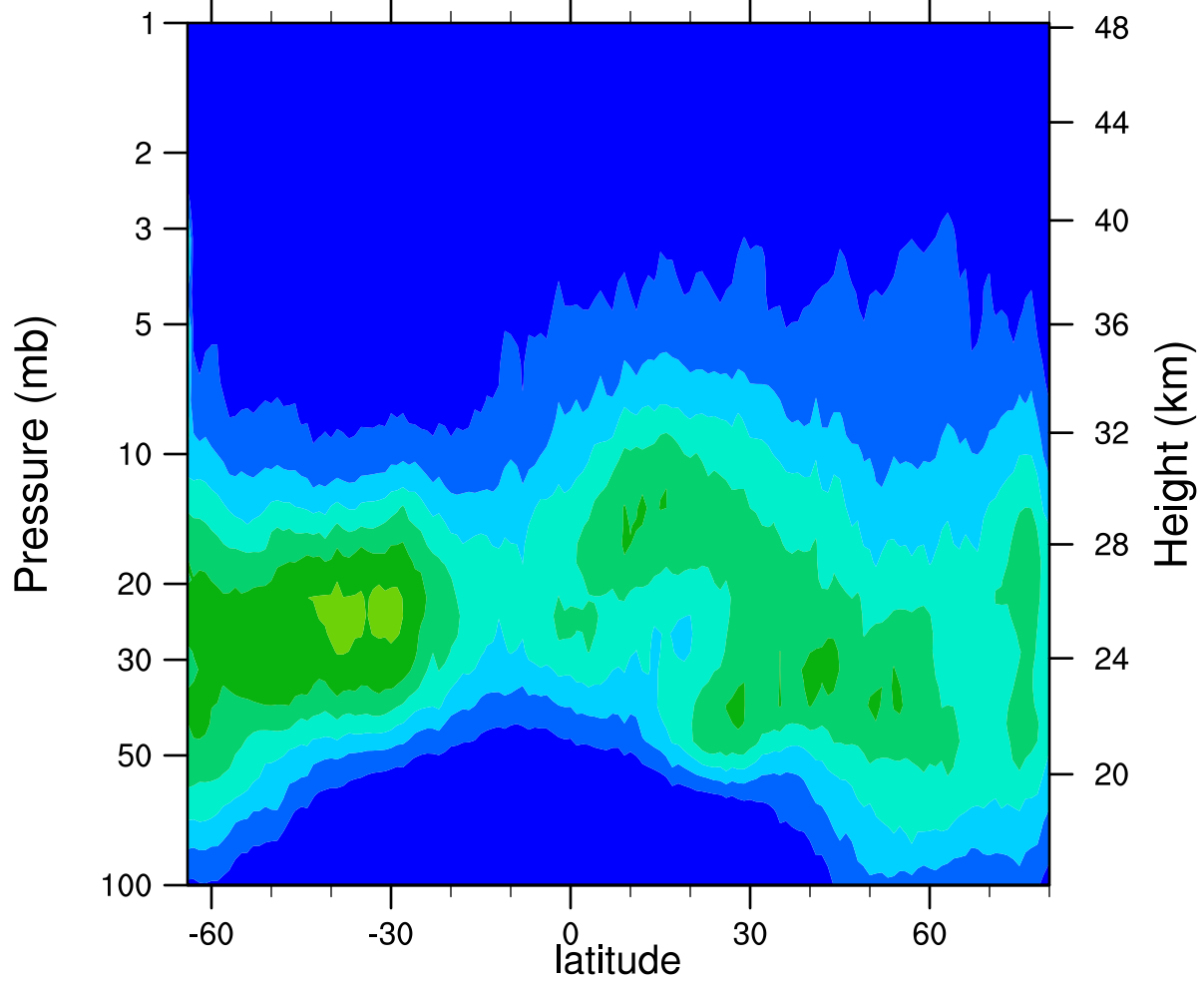
HIRDLSv6 2006d006 ClONO2_Ascending (ppbv)
