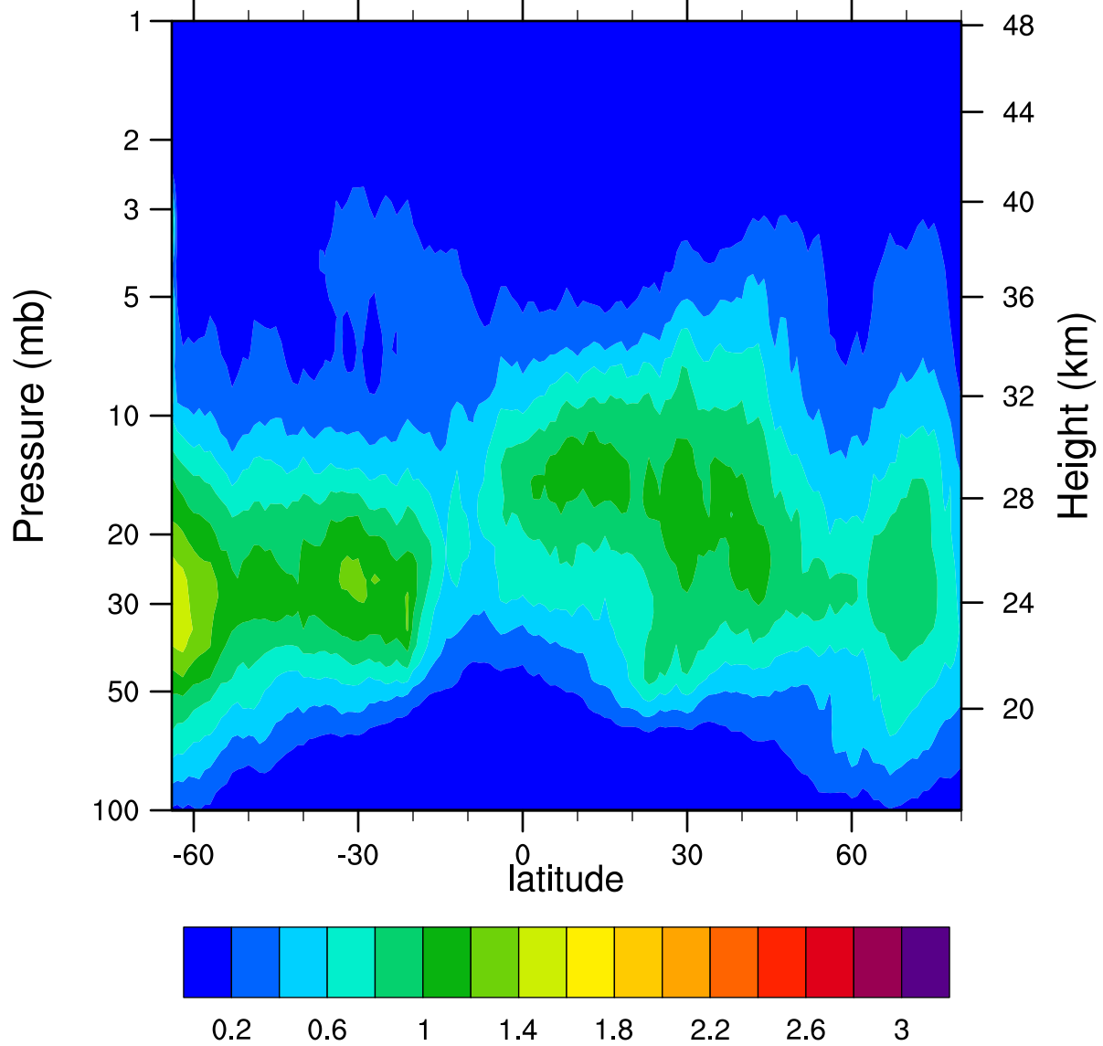
HIRDLSv6 2005d309 ClONO2_Ascending (ppbv)
