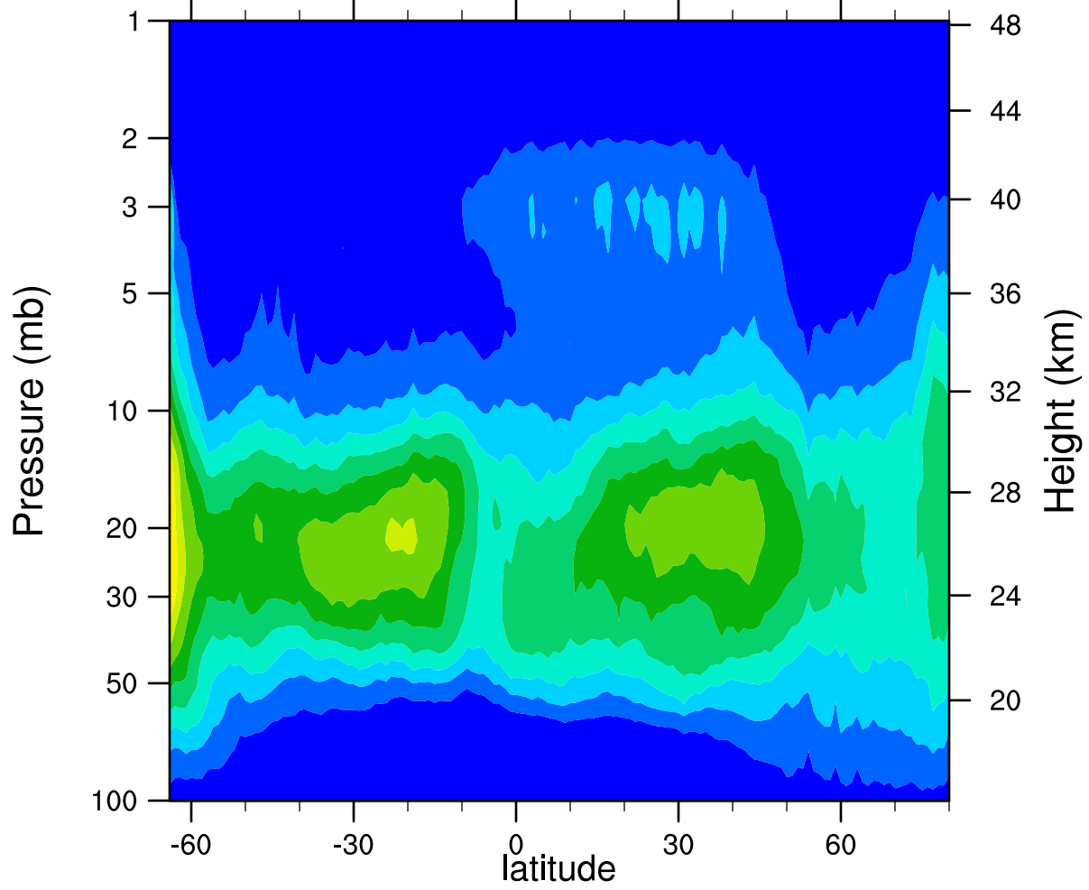
HIRDLSv6 2006d285 ClONO2_Ascending (ppbv)
