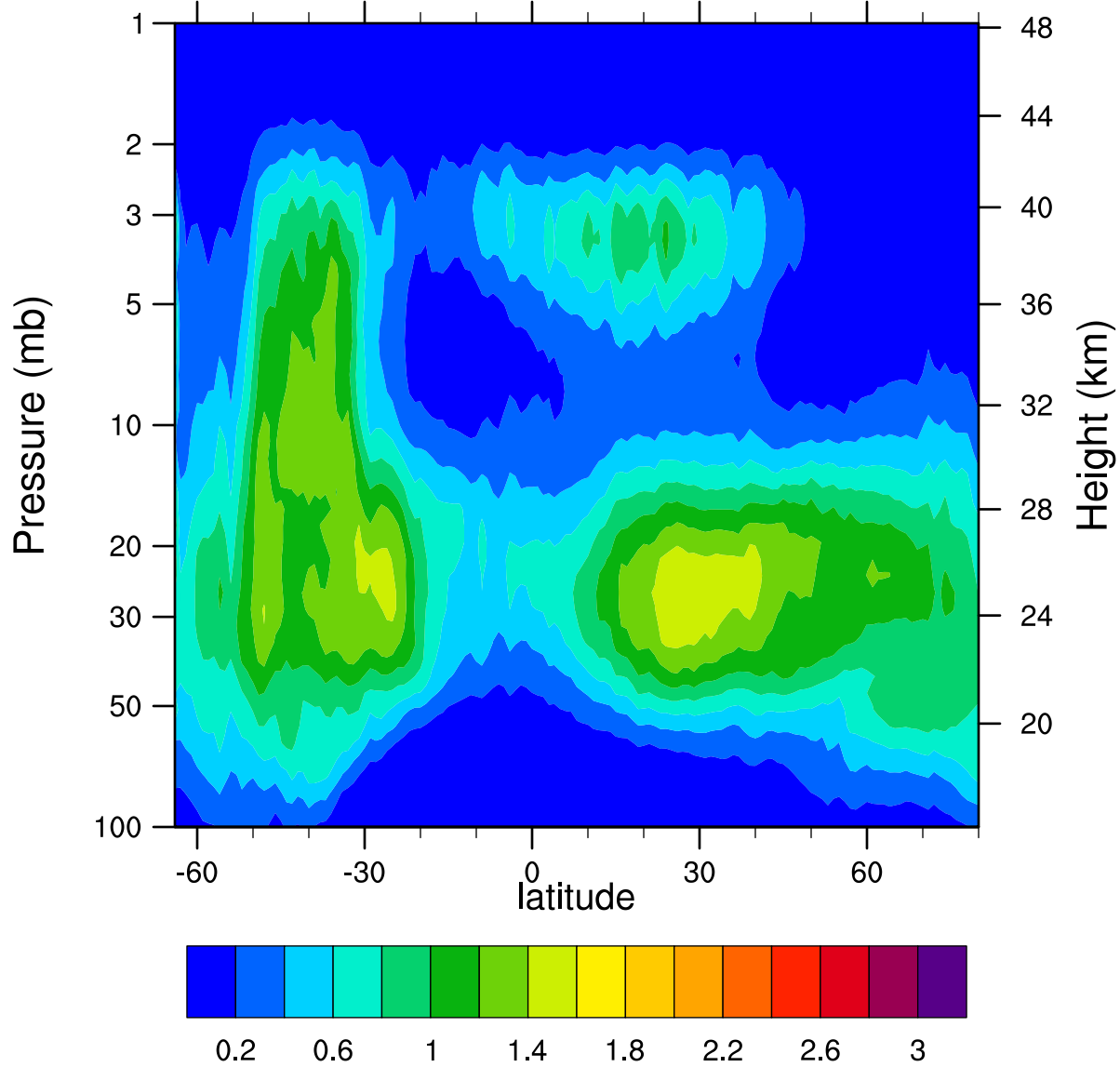
HIRDLSv6 2007d160 ClONO2_Ascending (ppbv)
