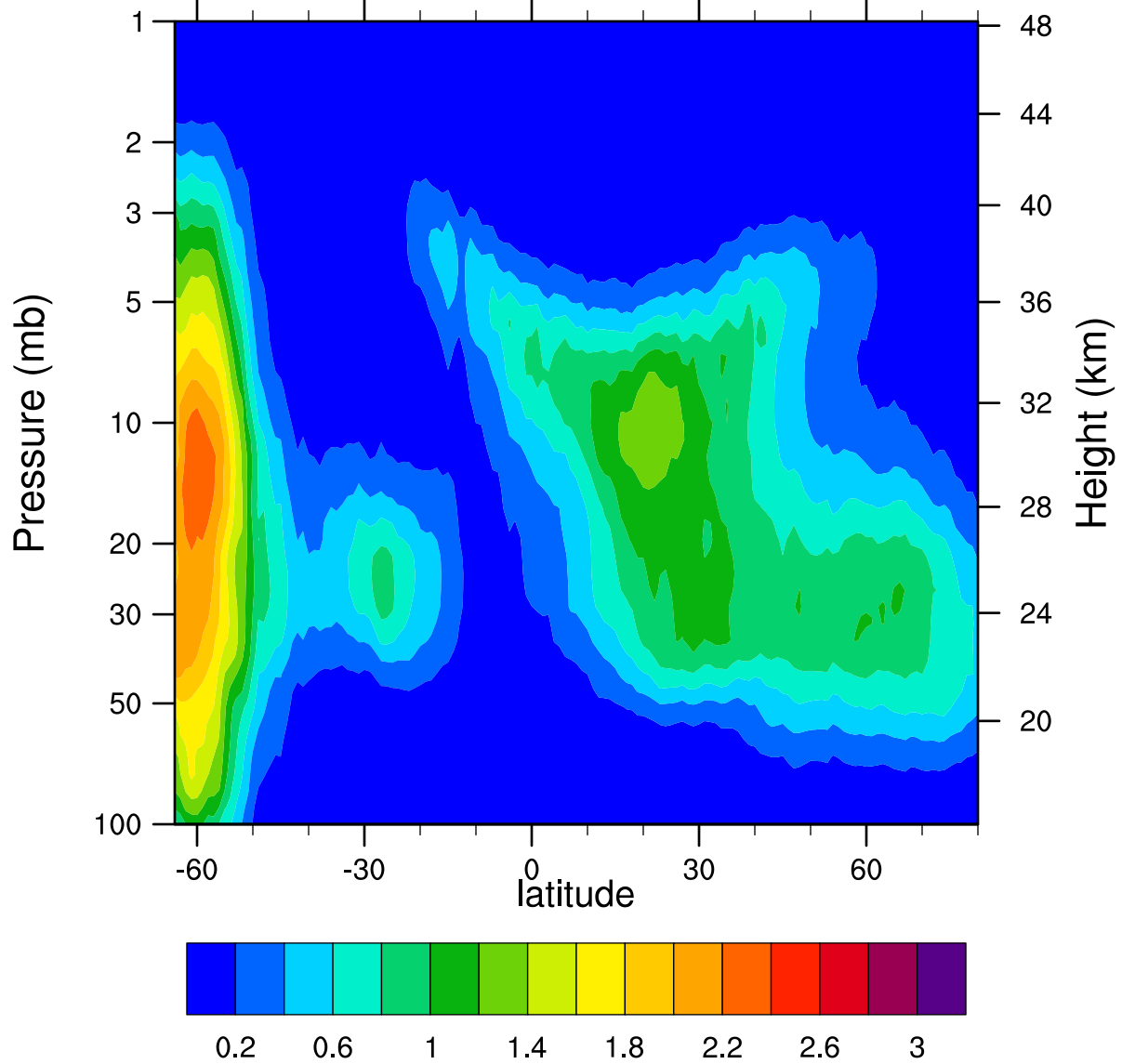
HIRDLSv6 2005d142 ClONO2_Ascending (ppbv)
