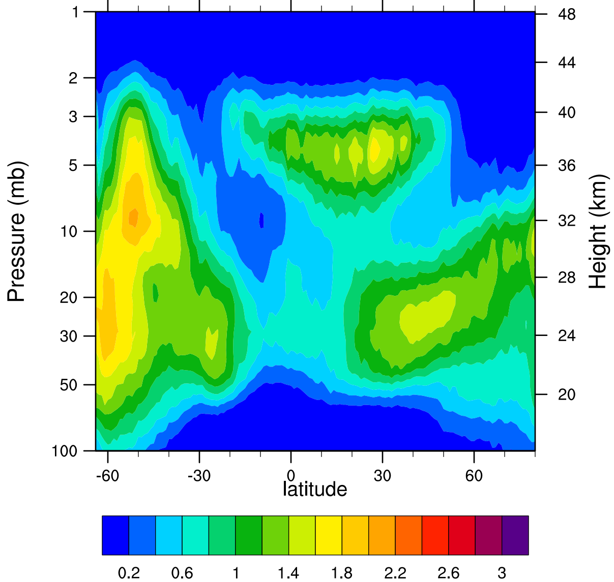
HIRDLSv6 2007d256 ClONO2_Ascending (ppbv)
