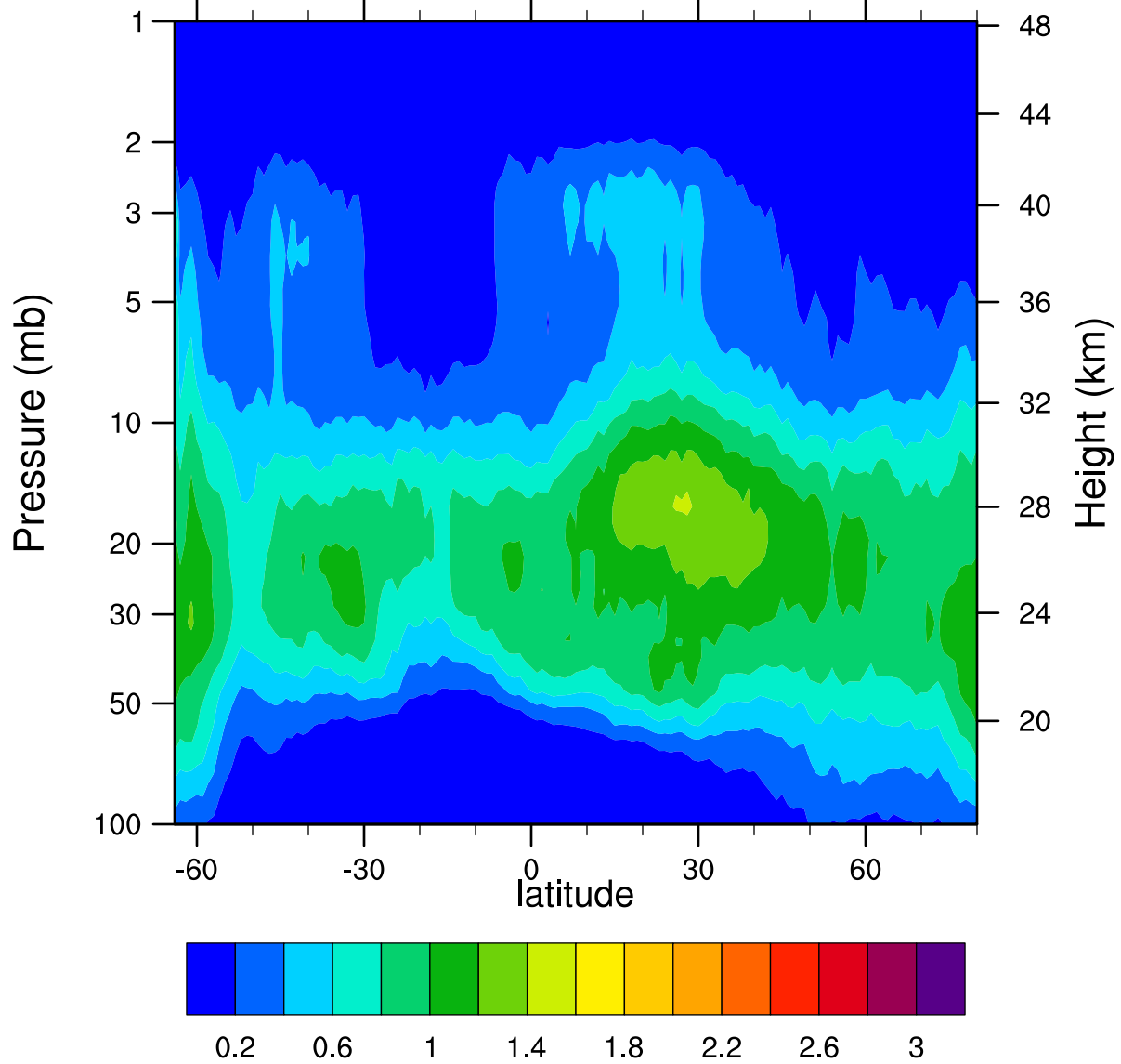
HIRDLSv6 2006d117 ClONO2_Ascending (ppbv)
