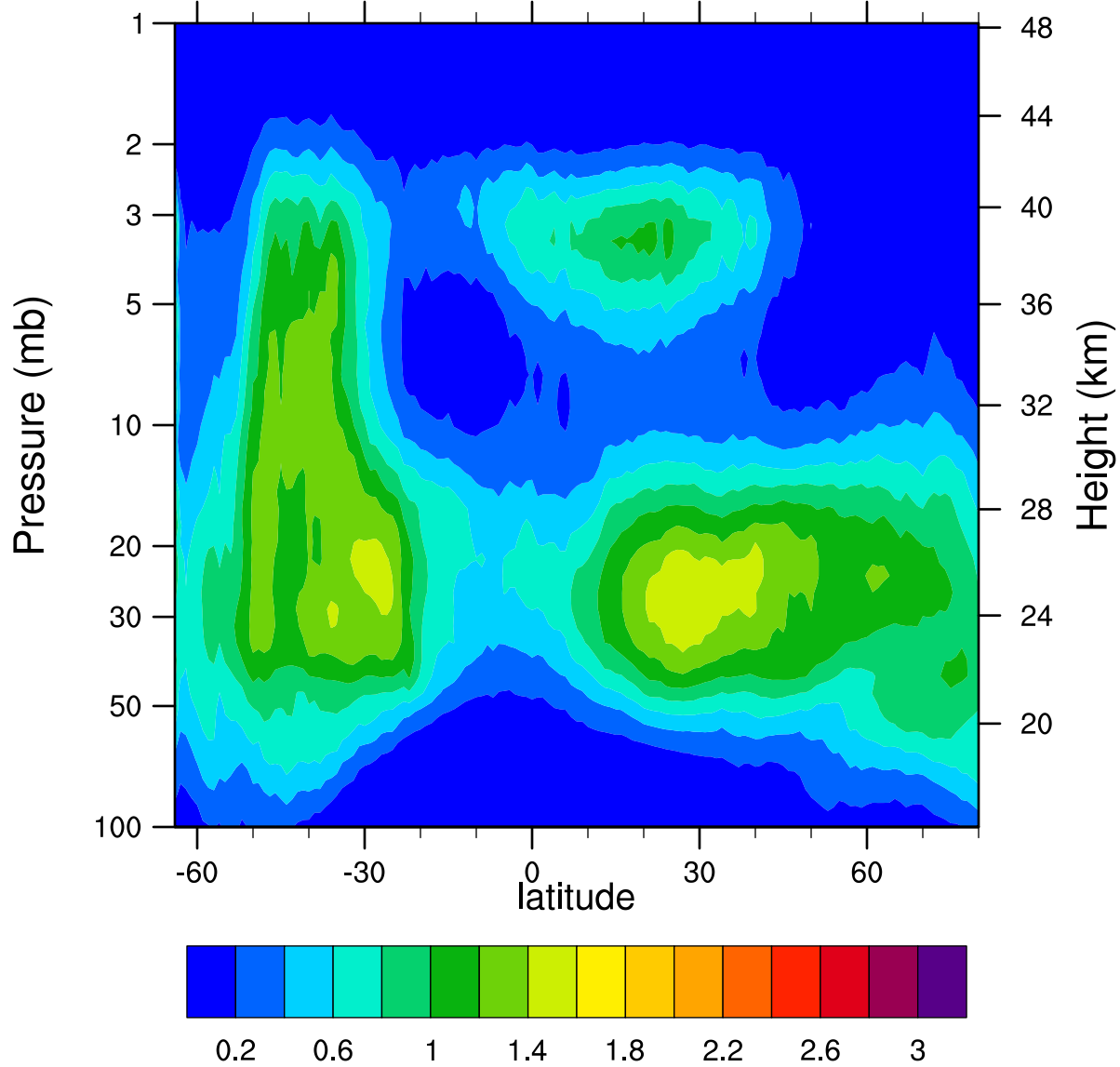
HIRDLSv6 2007d156 ClONO2_Ascending (ppbv)
