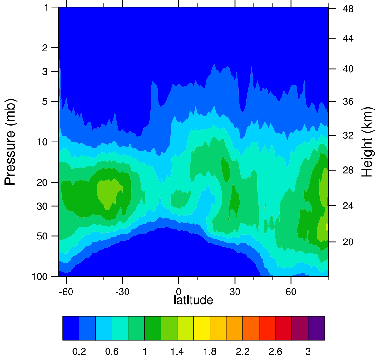
HIRDLSv6 2006d023 ClONO2_Ascending (ppbv)
