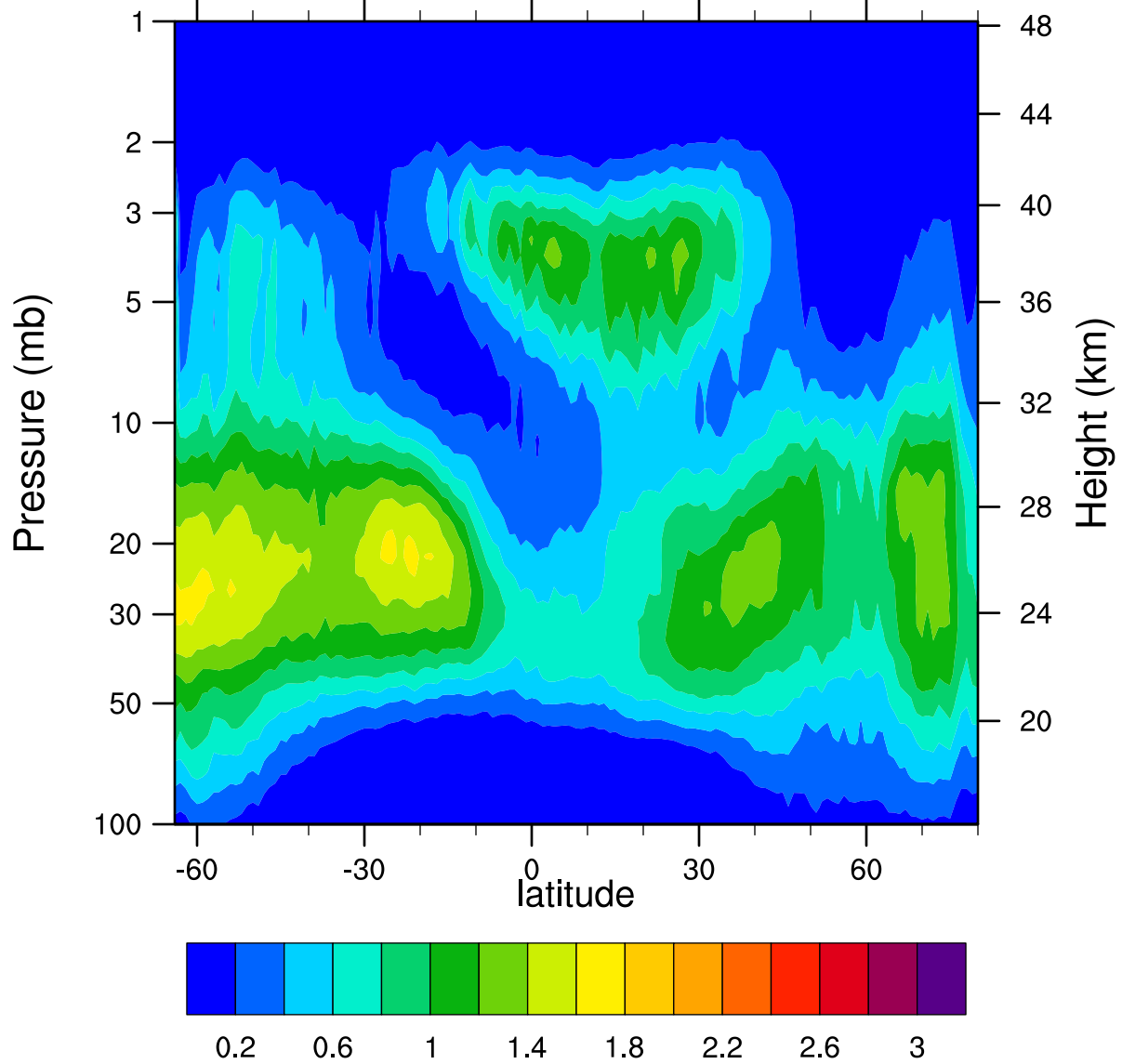
HIRDLSv6 2006d314 ClONO2_Ascending (ppbv)
