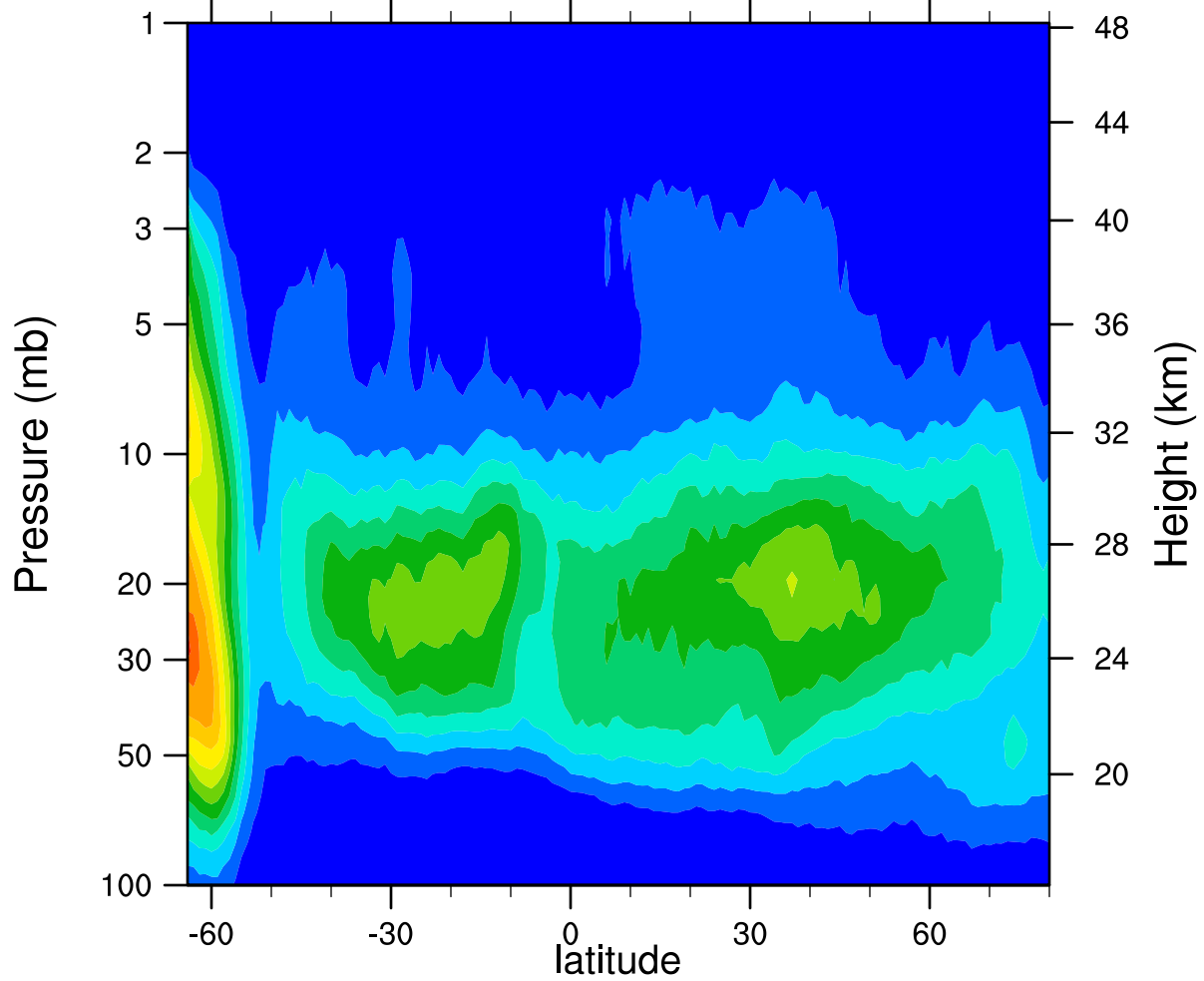
HIRDLSv6 2006d245 ClONO2_Ascending (ppbv)
