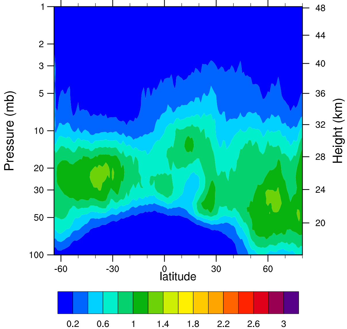
HIRDLSv6 2006d034 ClONO2_Ascending (ppbv)
