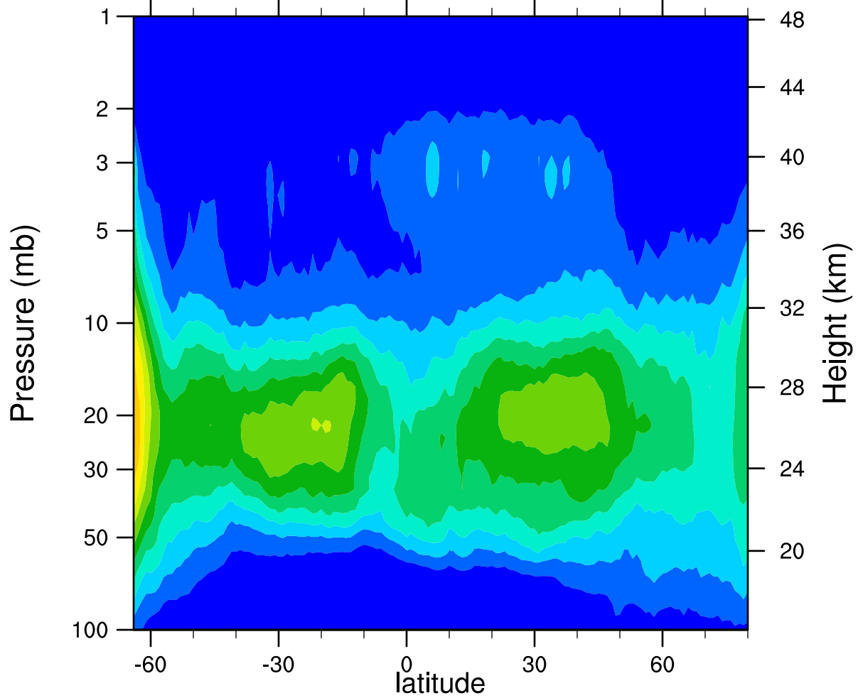
HIRDLSv6 2006d276 ClONO2_Ascending (ppbv)
