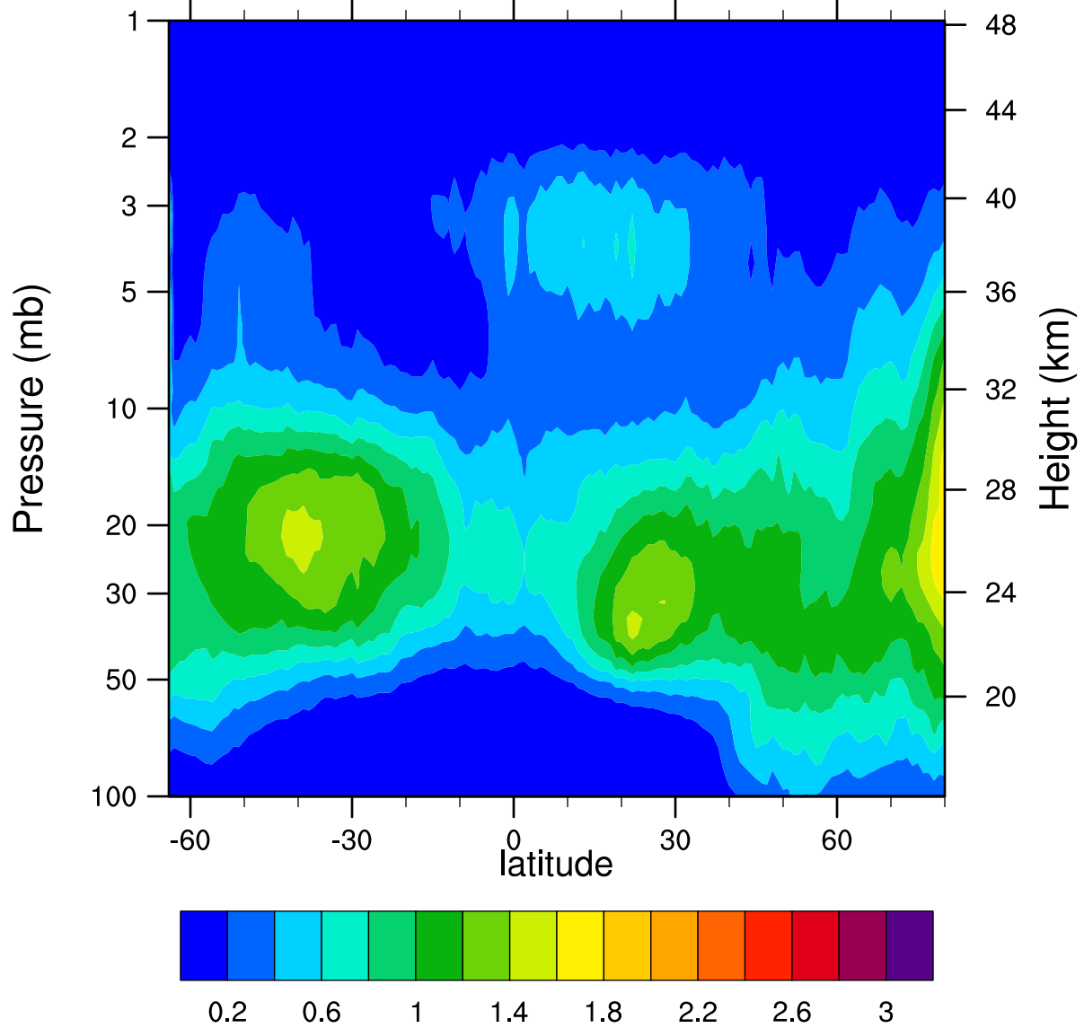
HIRDLSv6 2007d036 ClONO2_Ascending (ppbv)
