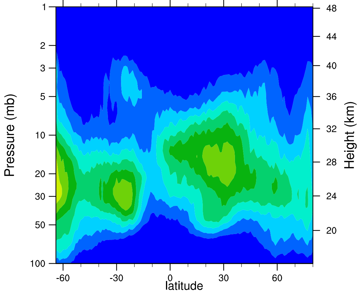
HIRDLSv6 2005d289 ClONO2_Ascending (ppbv)
