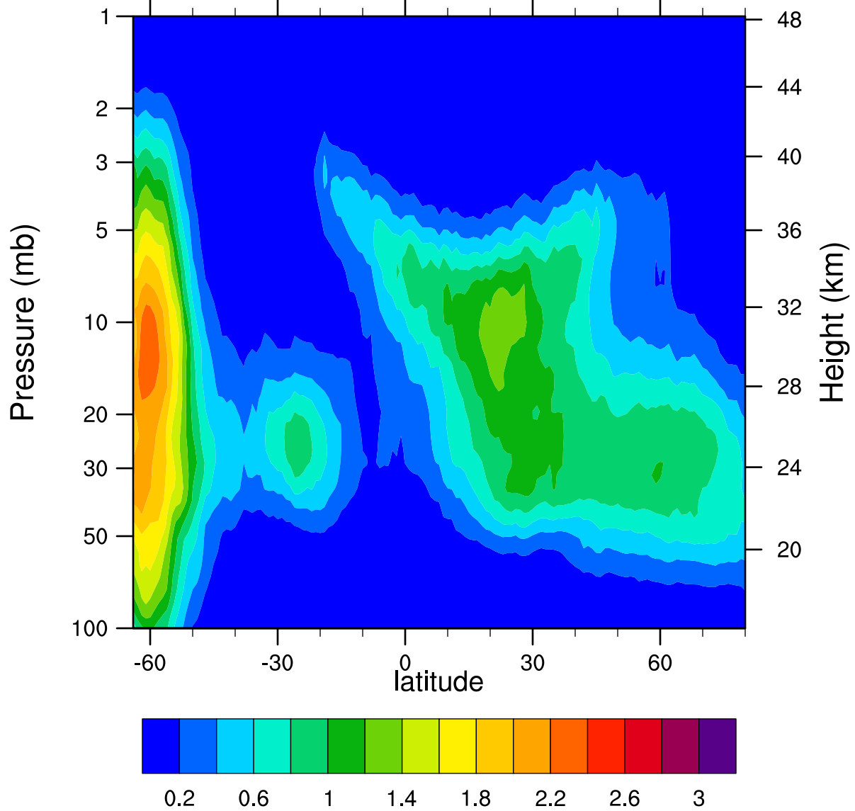
HIRDLSv6 2005d148 ClONO2_Ascending (ppbv)
