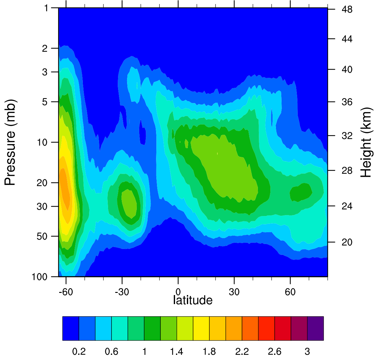
HIRDLSv6 2005d198 ClONO2_Ascending (ppbv)
