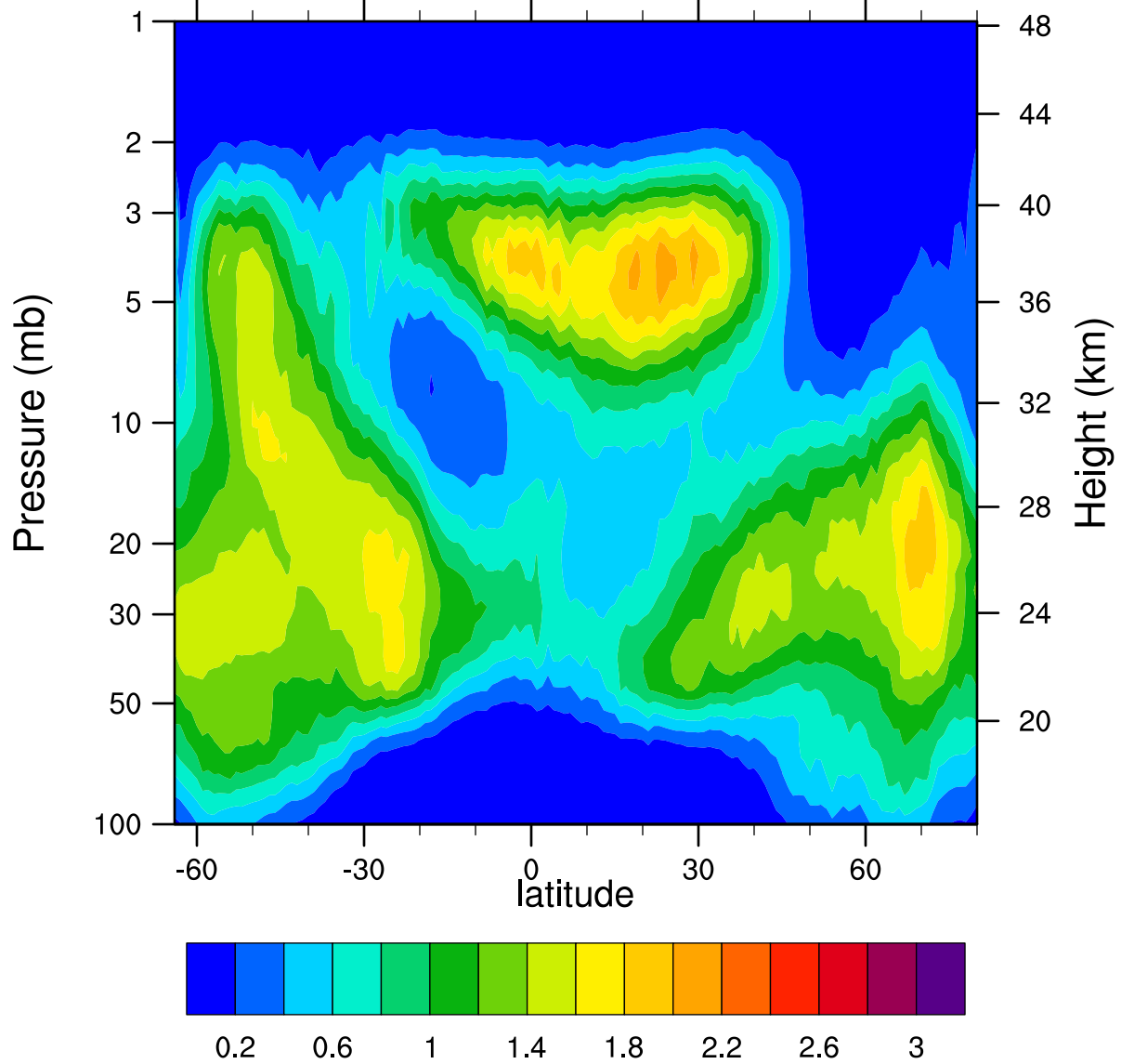
HIRDLSv6 2007d316 ClONO2_Ascending (ppbv)
