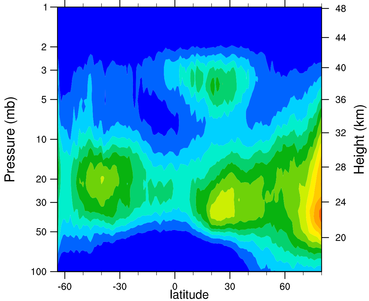
HIRDLSv6 2007d075 ClONO2_Ascending (ppbv)
