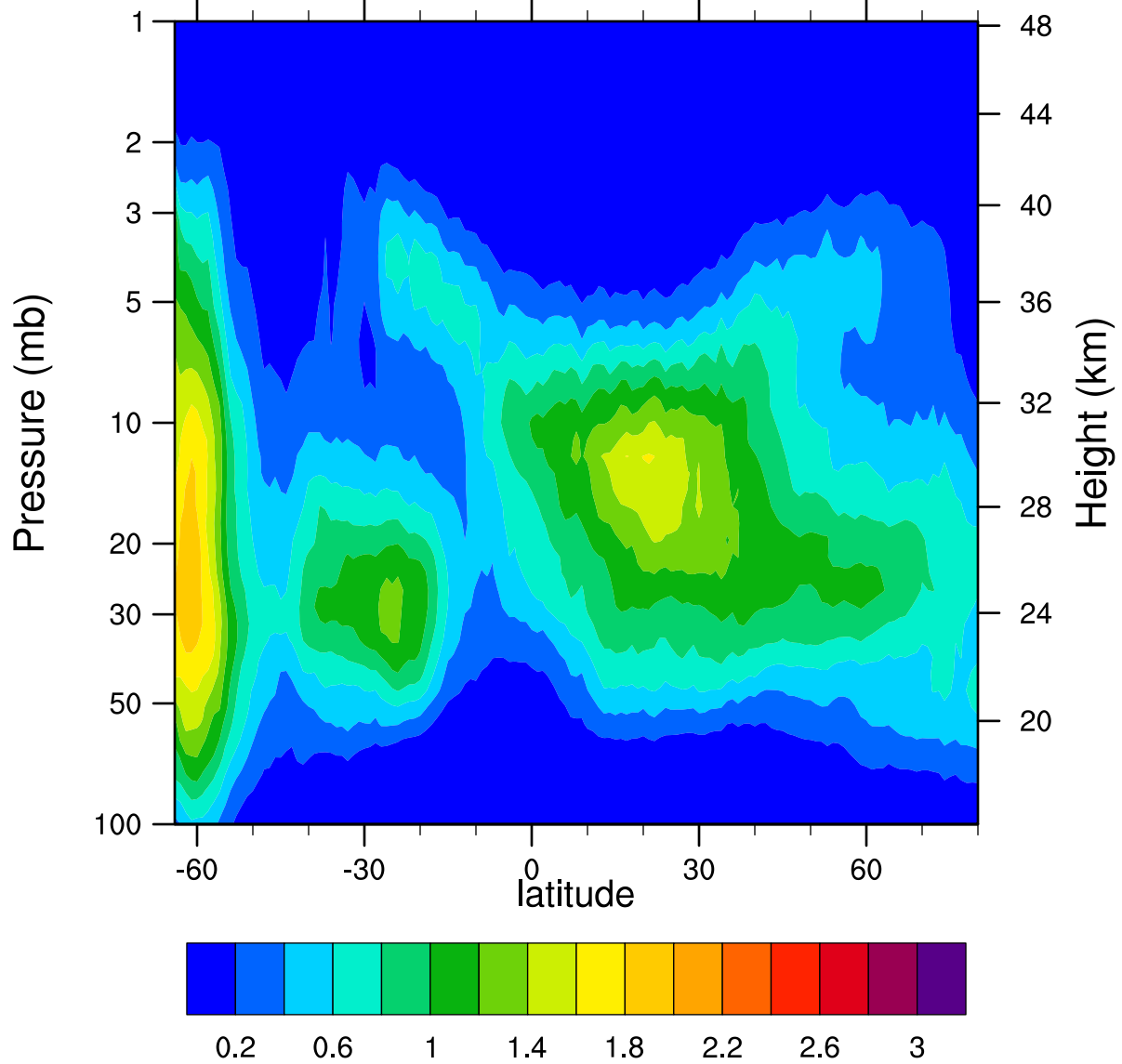
HIRDLSv6 2005d239 ClONO2_Ascending (ppbv)
