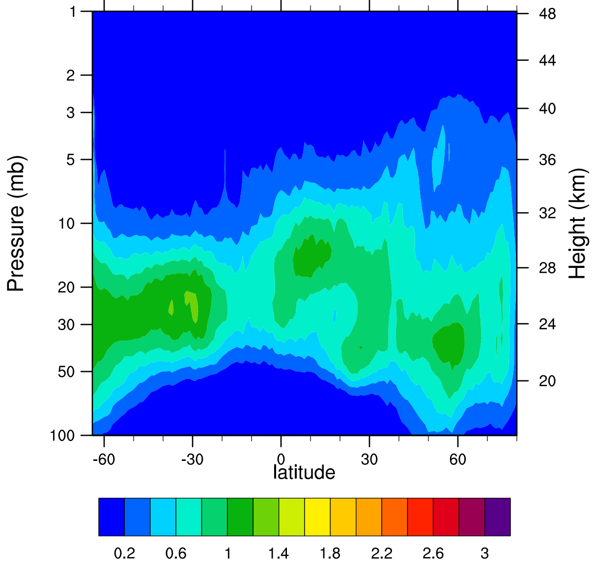
HIRDLSv6 2005d358 ClONO2_Ascending (ppbv)
