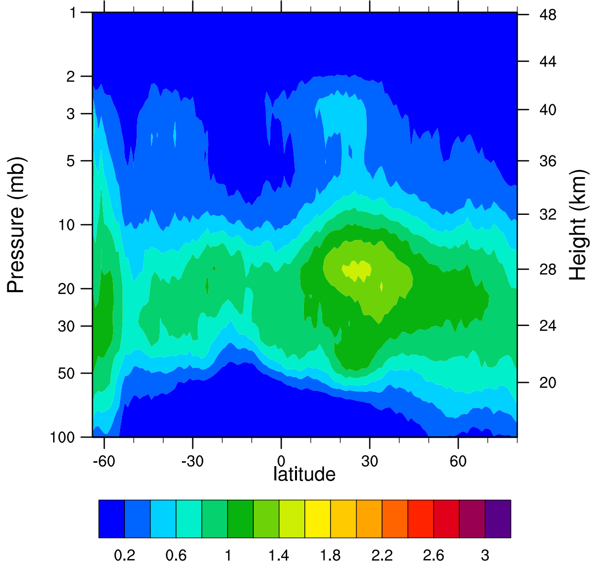
HIRDLSv6 2006d129 ClONO2_Ascending (ppbv)
