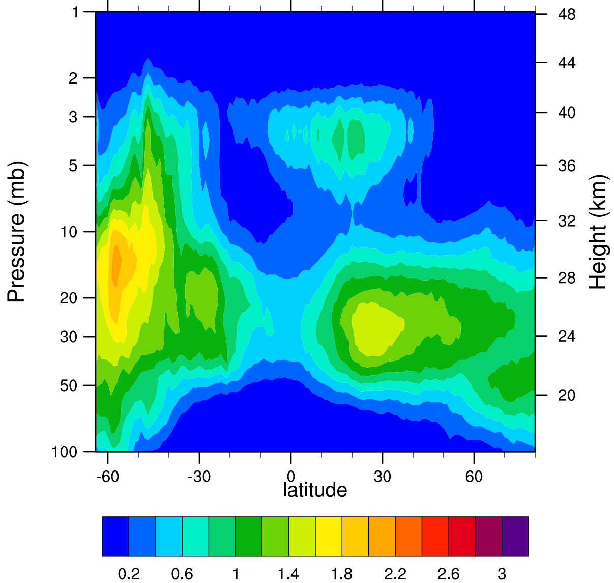
HIRDLSv6 2007d134 ClONO2_Ascending (ppbv)
