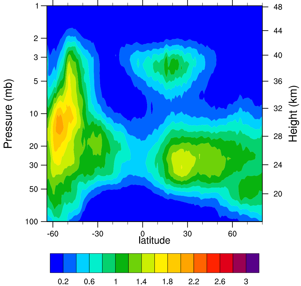
HIRDLSv6 2007d129 ClONO2_Ascending (ppbv)
