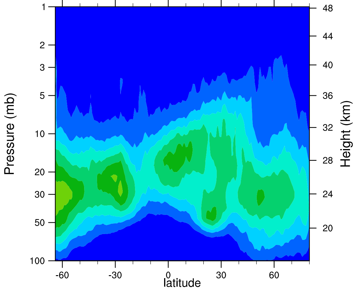
HIRDLSv6 2005d333 ClONO2_Ascending (ppbv)
