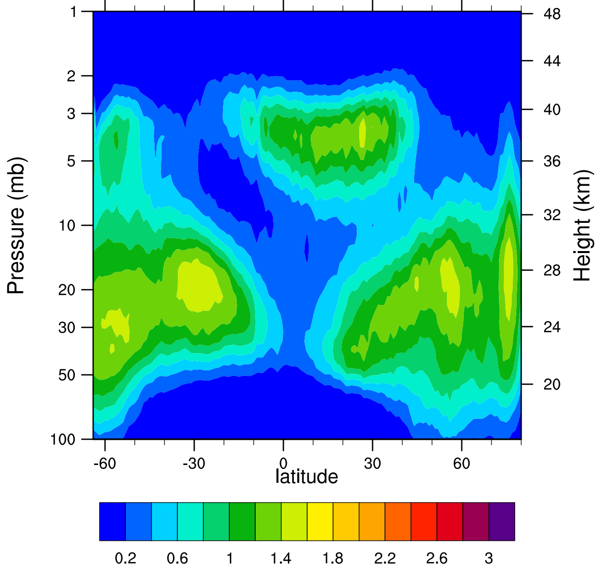
HIRDLSv6 2006d353 ClONO2_Ascending (ppbv)
