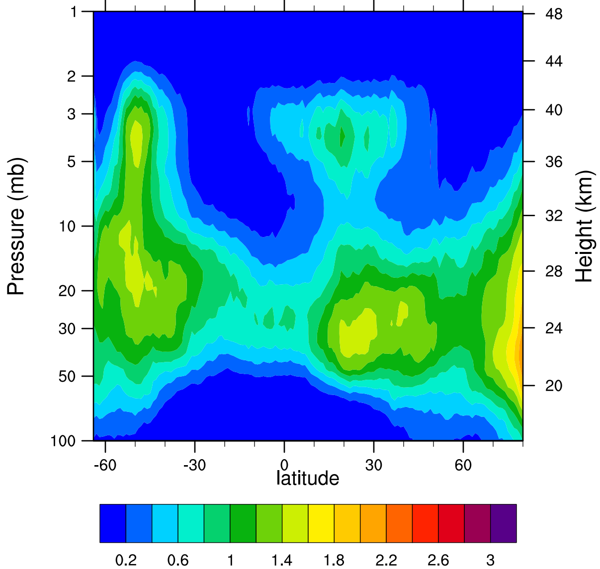
HIRDLSv6 2007d089 ClONO2_Ascending (ppbv)
