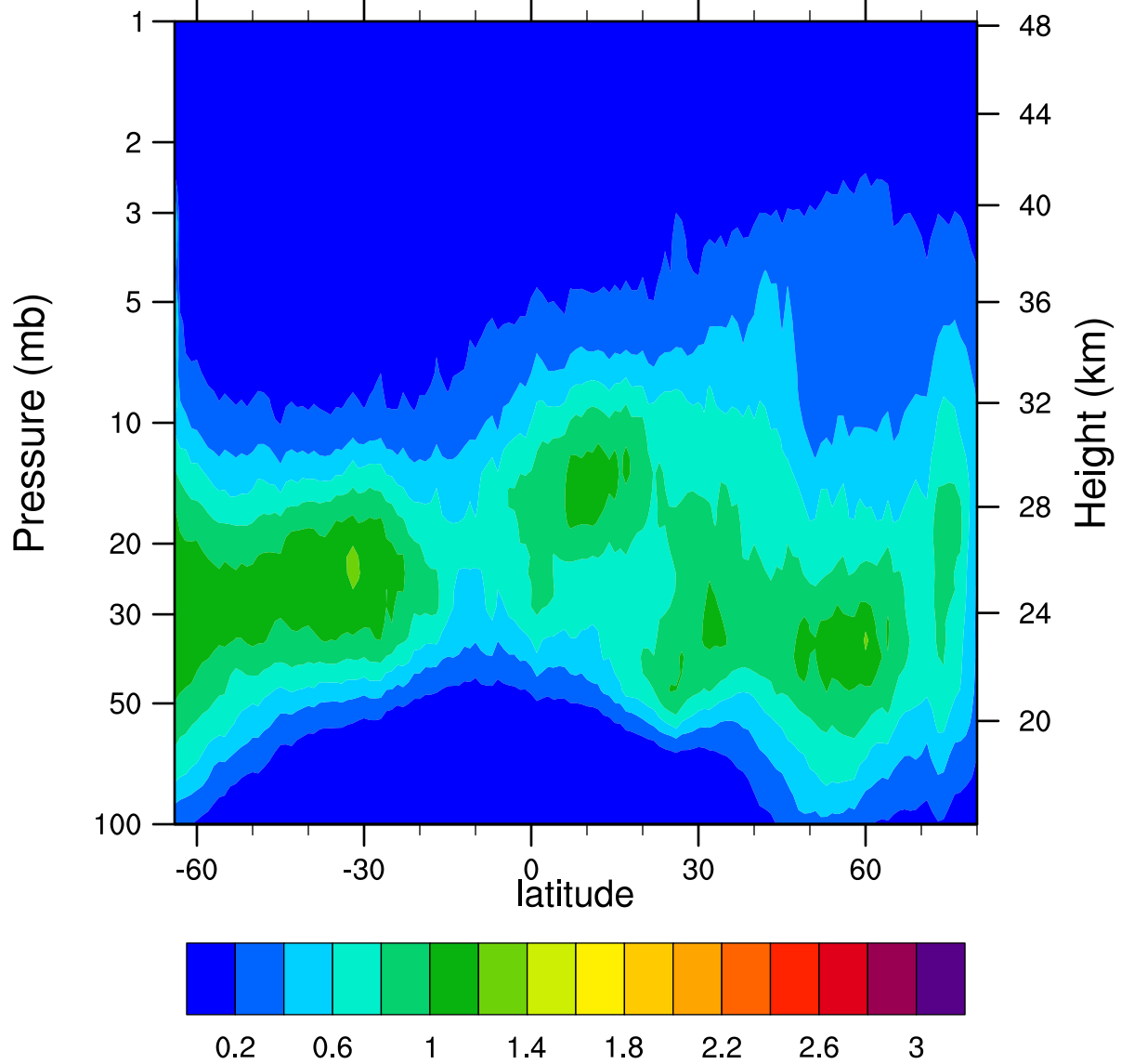
HIRDLSv6 2005d354 ClONO2_Ascending (ppbv)
