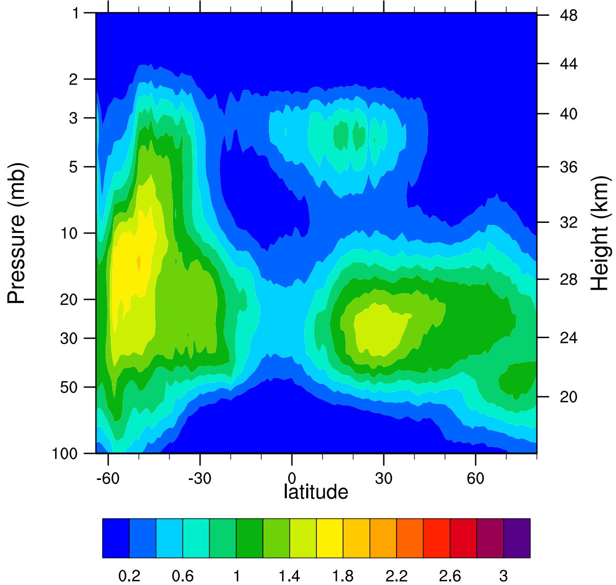
HIRDLSv6 2007d141 ClONO2_Ascending (ppbv)
