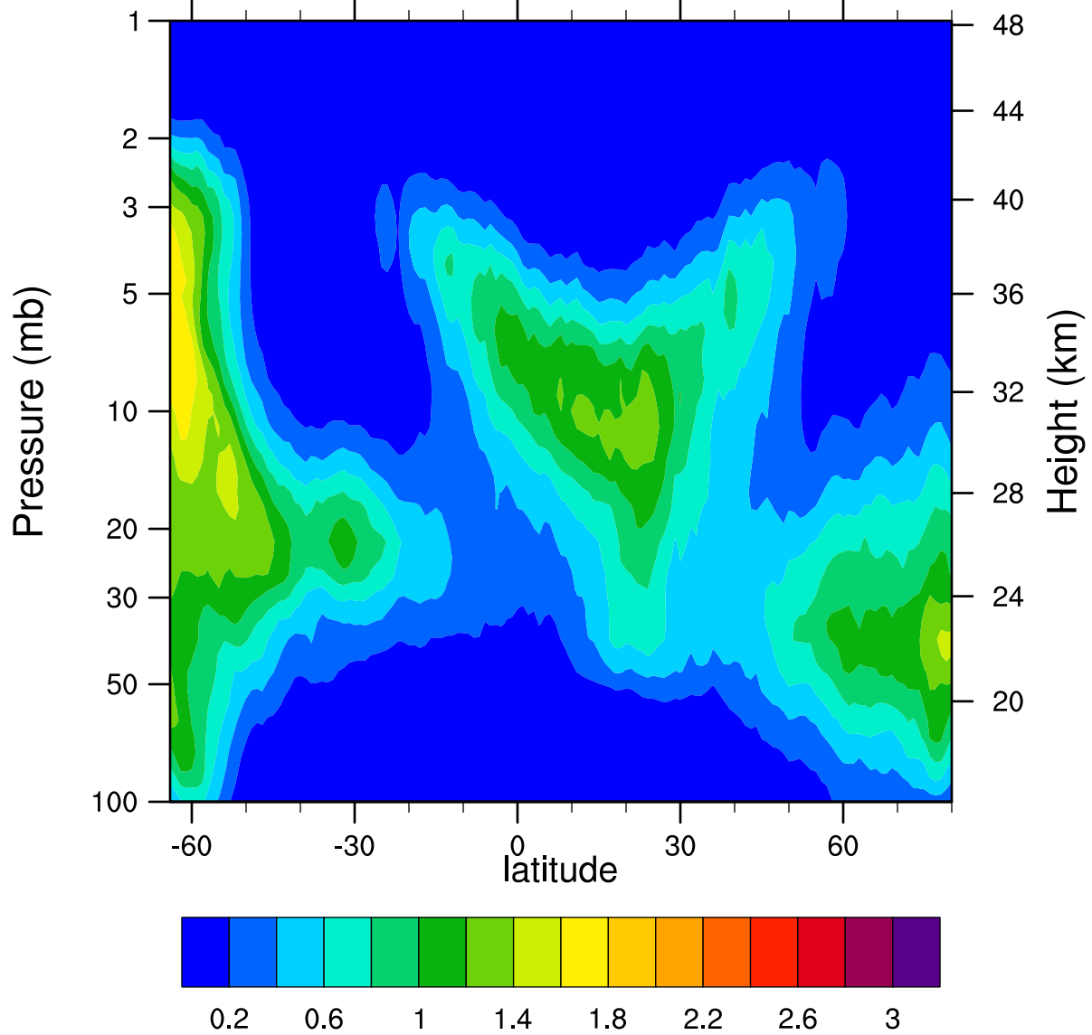
HIRDLSv6 2005d059 ClONO2_Ascending (ppbv)
