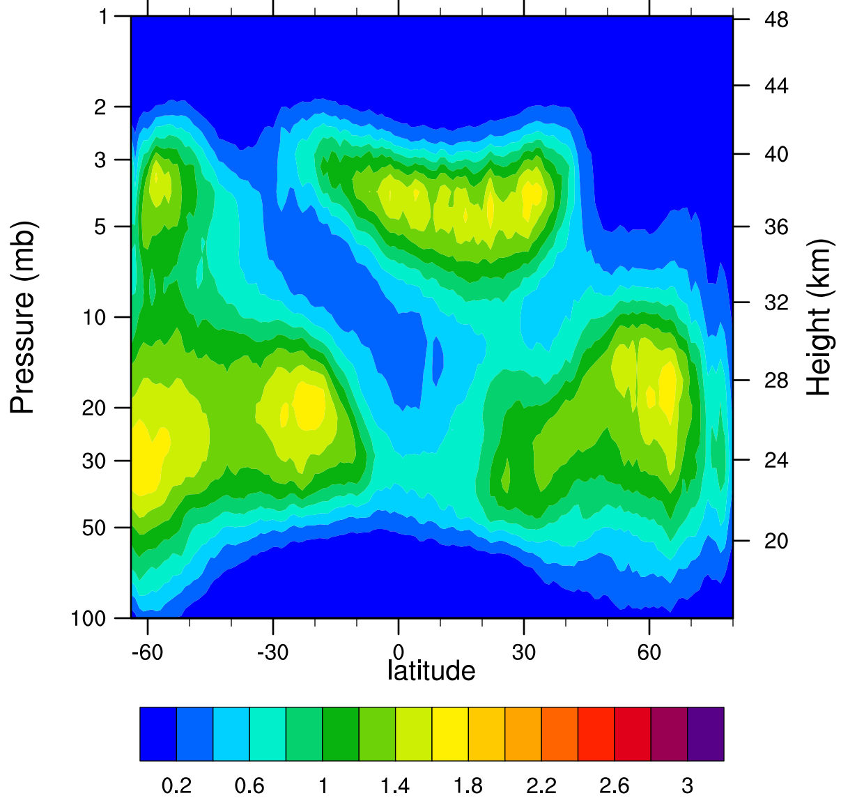
HIRDLSv6 2006d329 ClONO2_Ascending (ppbv)
