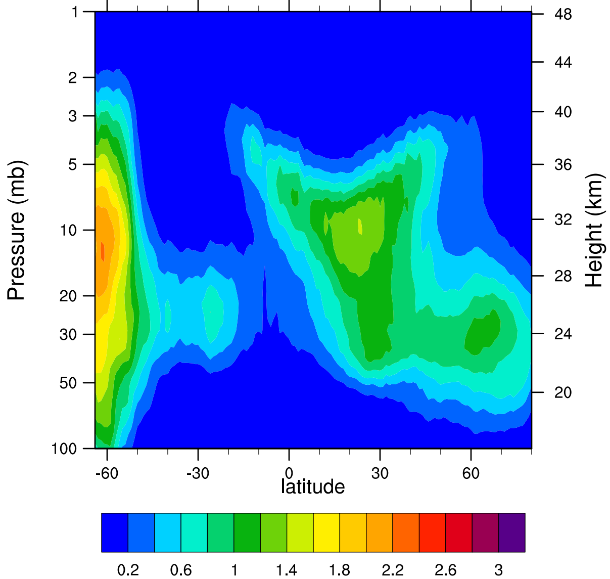
HIRDLSv6 2005d123 ClONO2_Ascending (ppbv)
