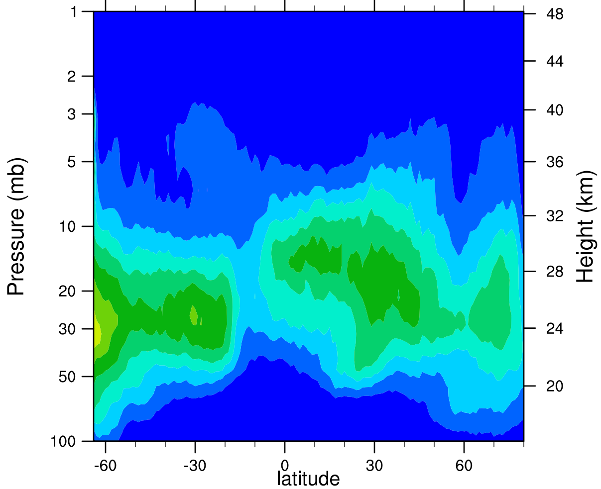
HIRDLSv6 2005d305 ClONO2_Ascending (ppbv)
