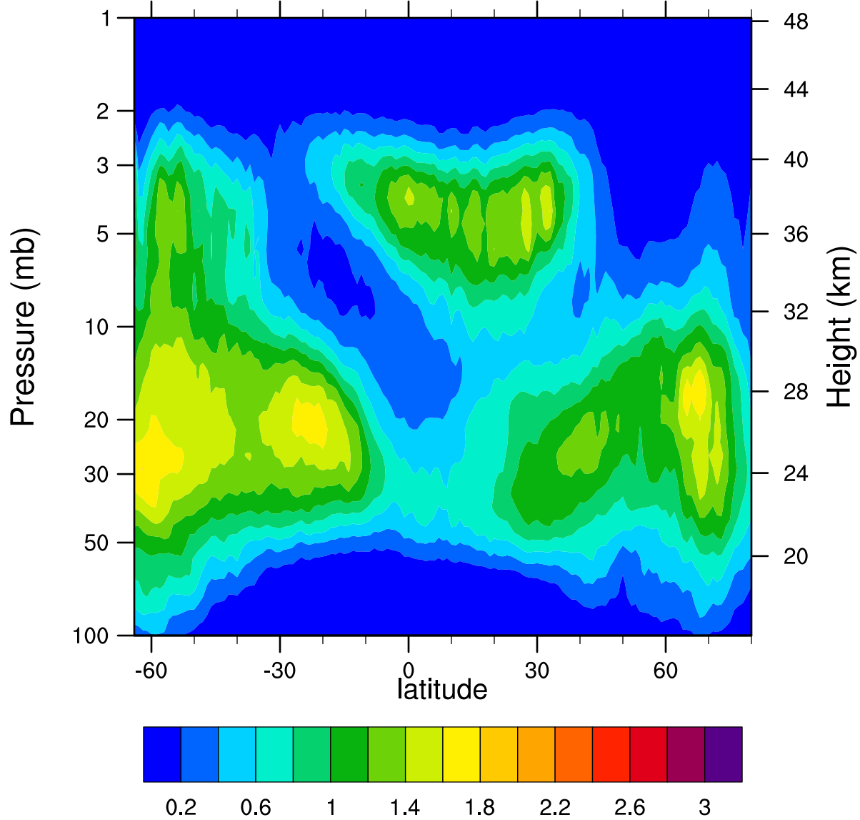
HIRDLSv6 2006d317 ClONO2_Ascending (ppbv)
