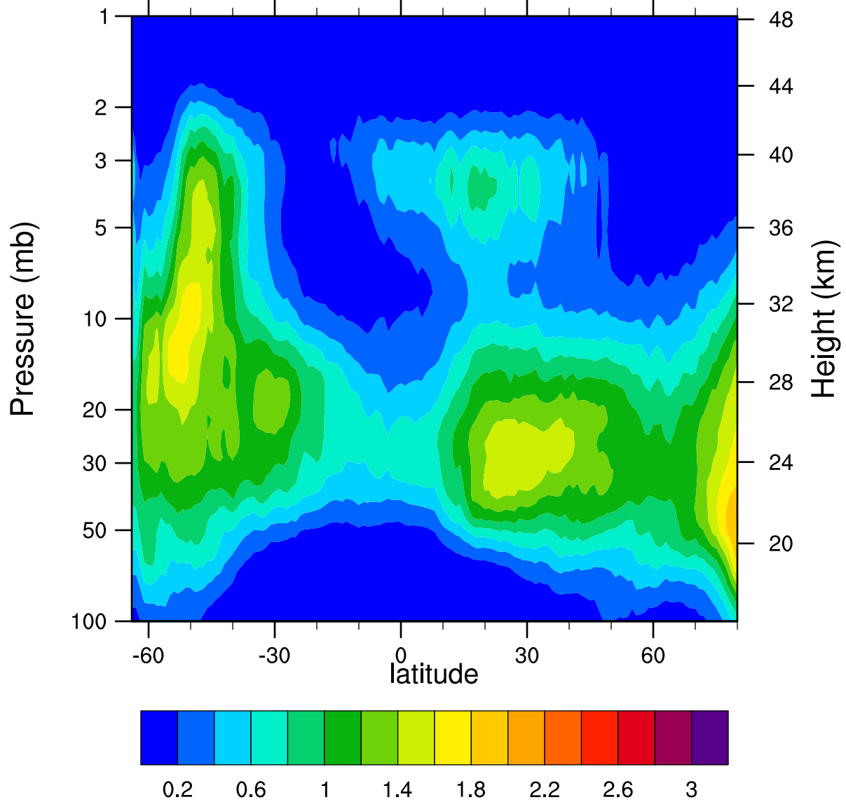
HIRDLSv6 2007d107 ClONO2_Ascending (ppbv)
