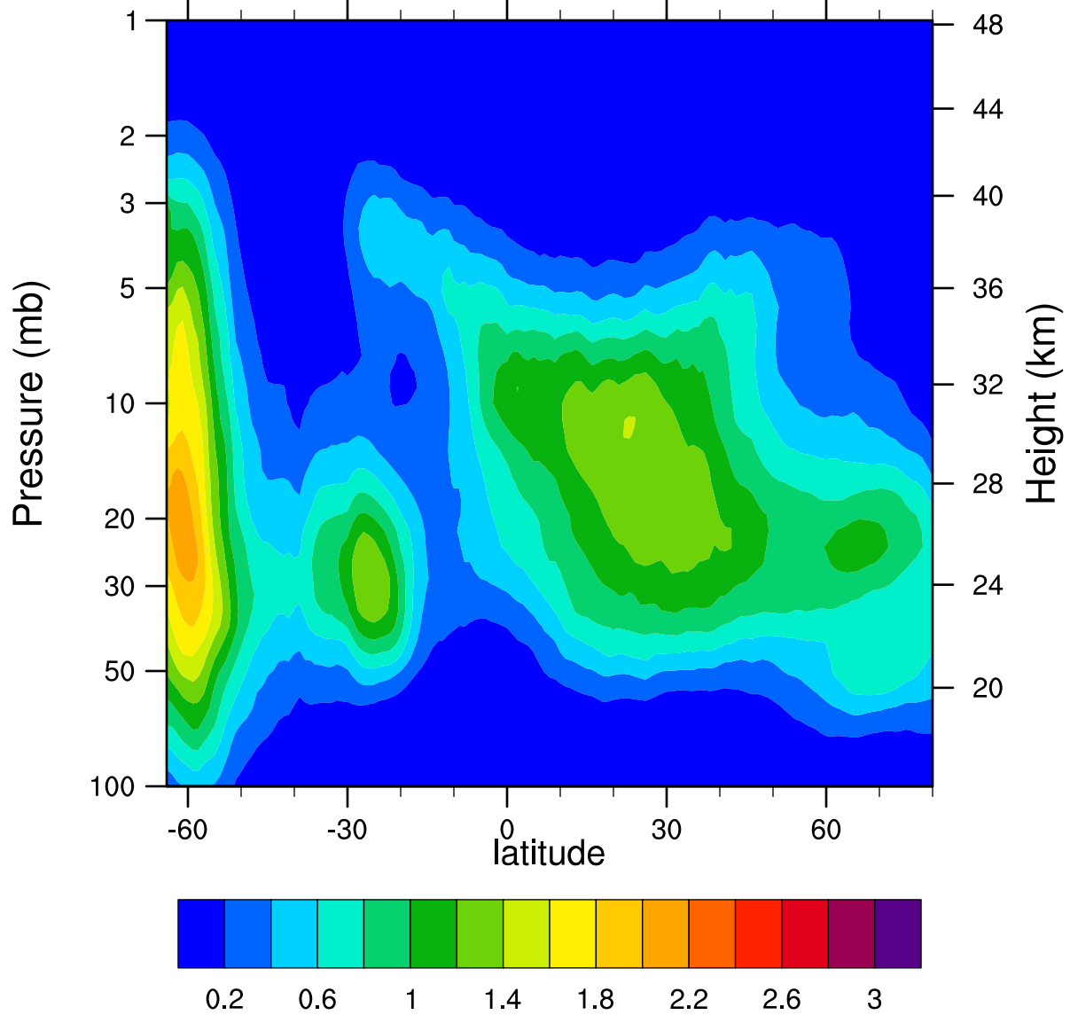
HIRDLSv6 2005d194 ClONO2_Ascending (ppbv)
