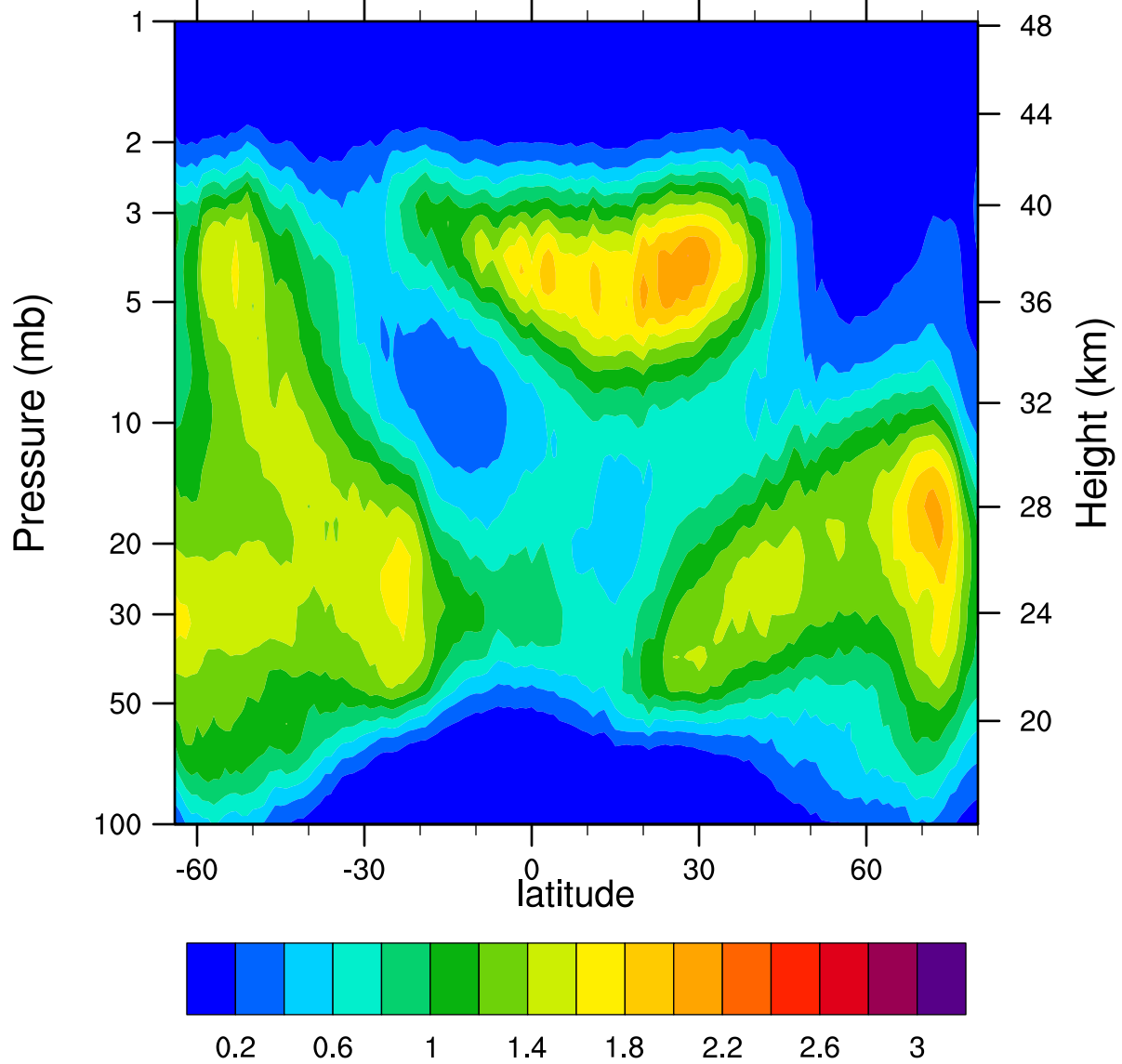
HIRDLSv6 2007d308 ClONO2_Ascending (ppbv)
