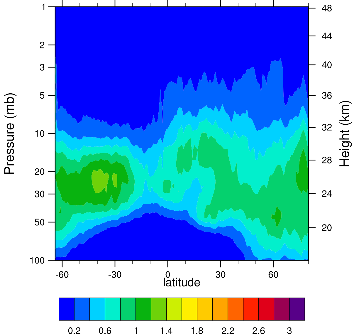
HIRDLSv6 2006d014 ClONO2_Ascending (ppbv)
