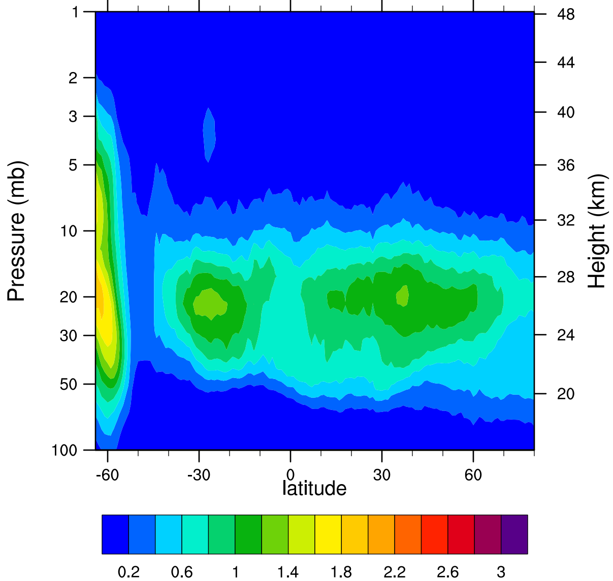
HIRDLSv6 2006d217 ClONO2_Ascending (ppbv)
