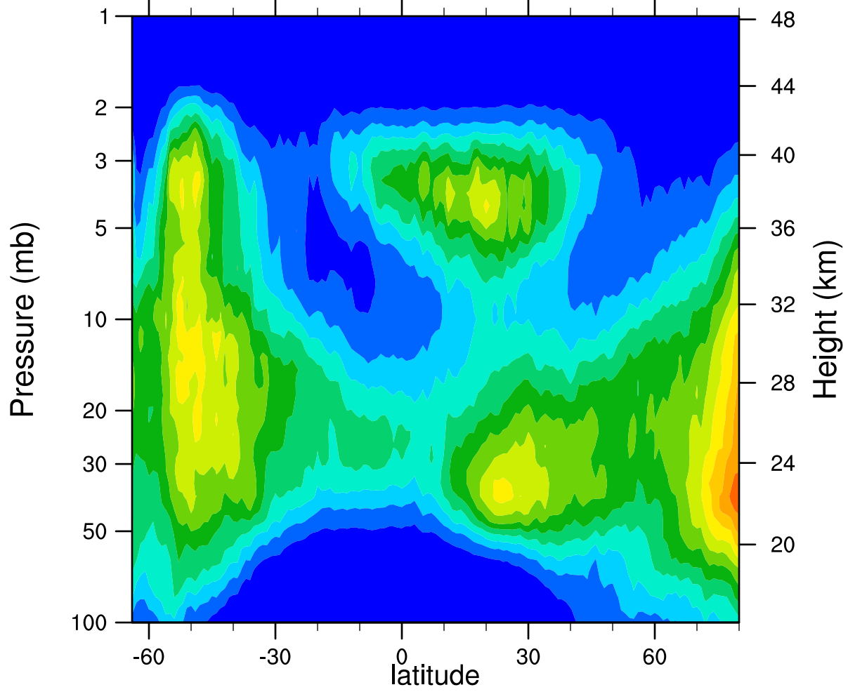
HIRDLSv6 2007d079 ClONO2_Ascending (ppbv)
