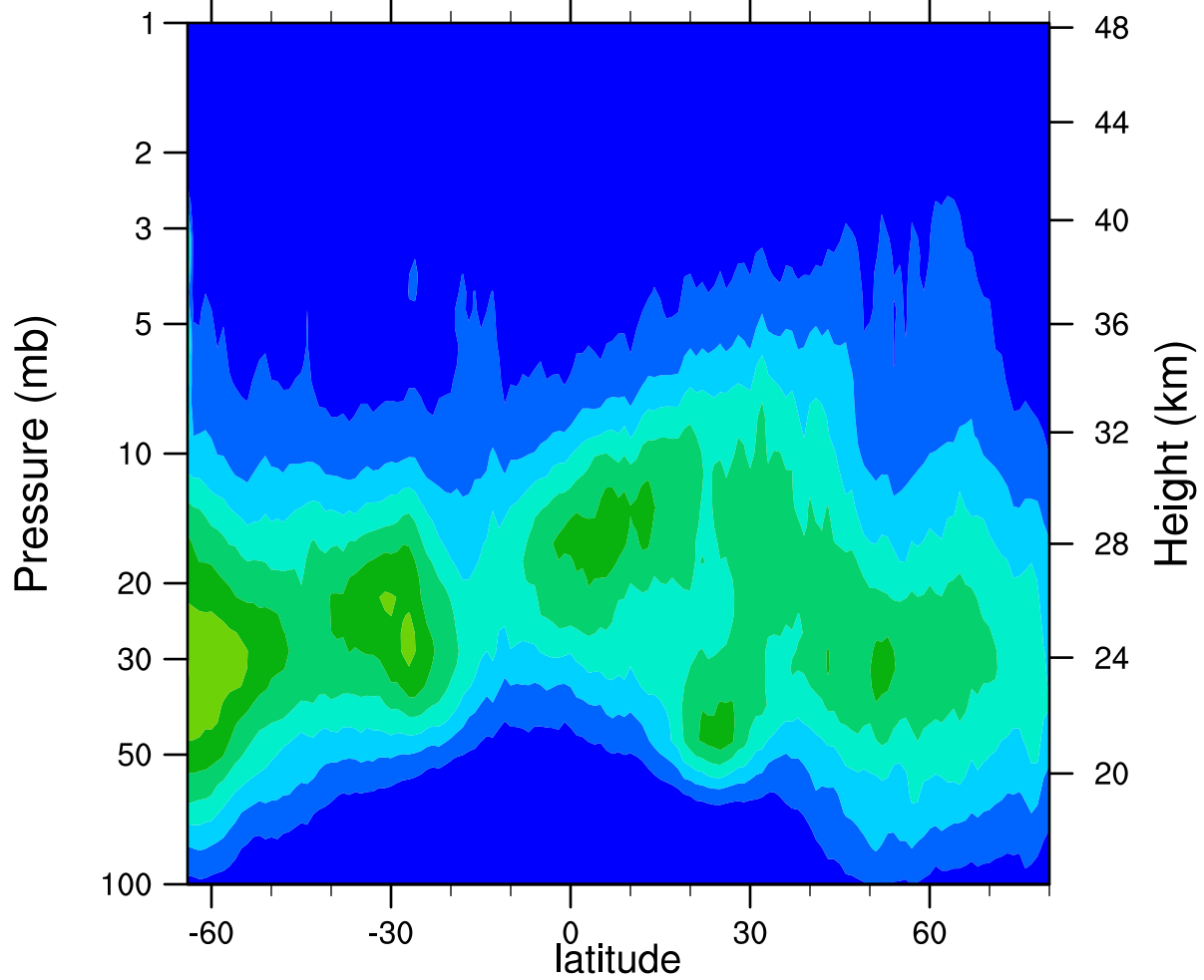
HIRDLSv6 2005d332 ClONO2_Ascending (ppbv)
