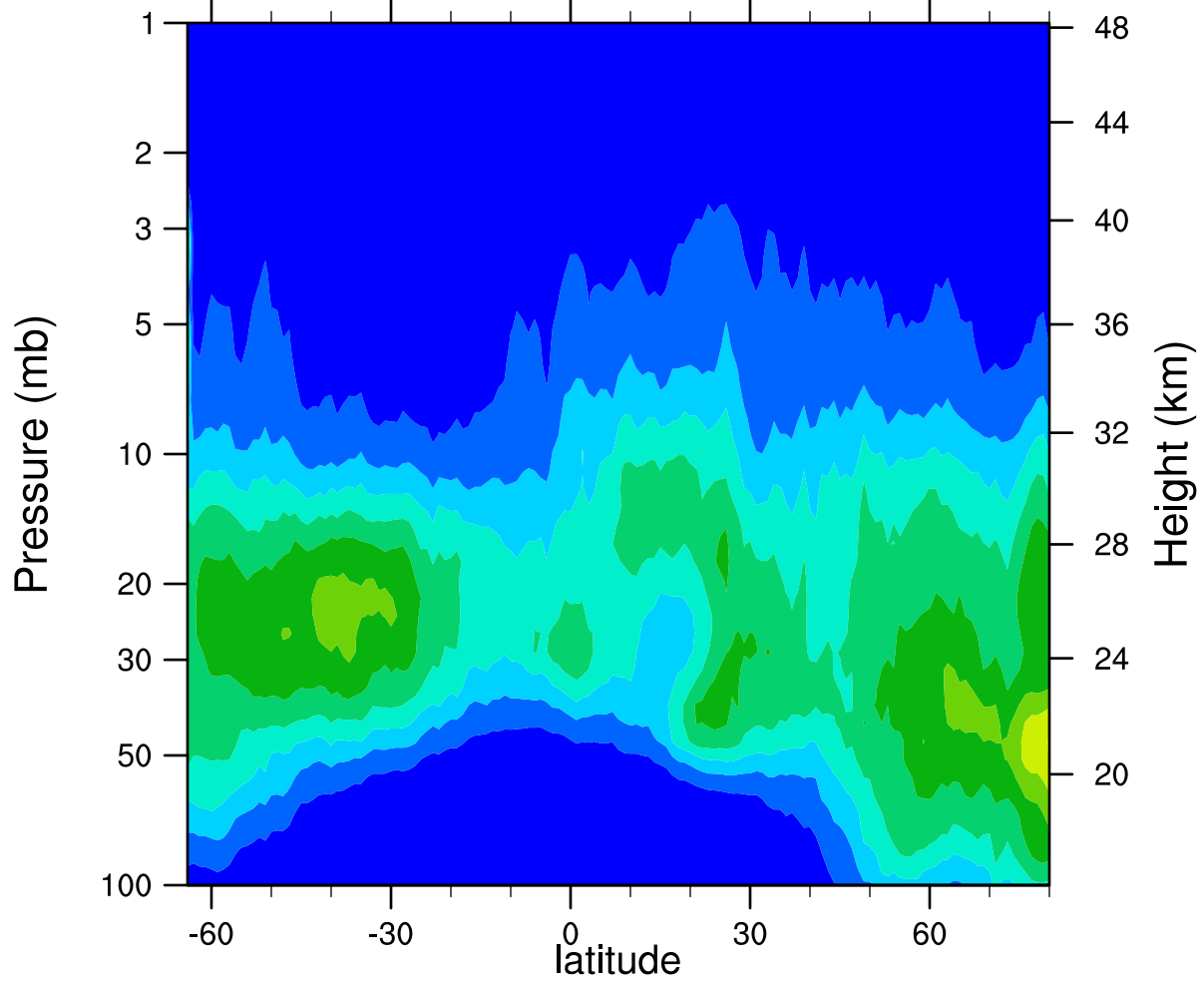
HIRDLSv6 2006d028 ClONO2_Ascending (ppbv)
