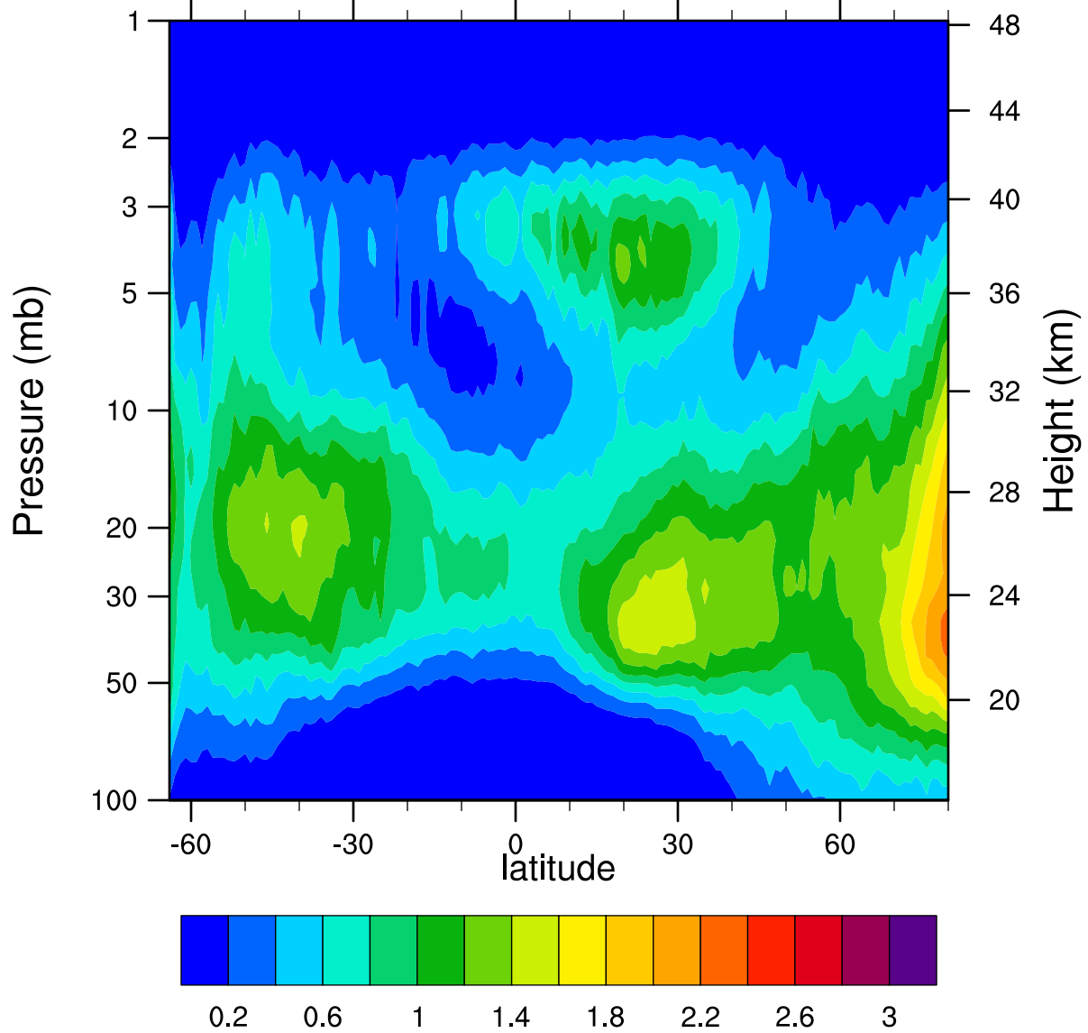
HIRDLSv6 2007d076 ClONO2_Ascending (ppbv)
