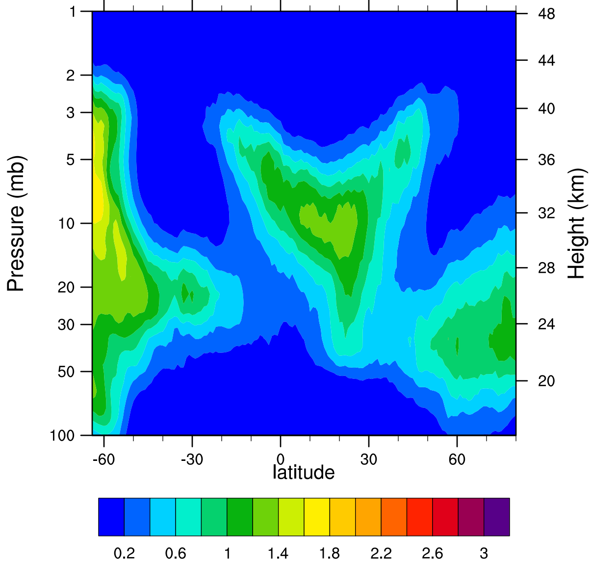
HIRDLSv6 2005d055 ClONO2_Ascending (ppbv)
