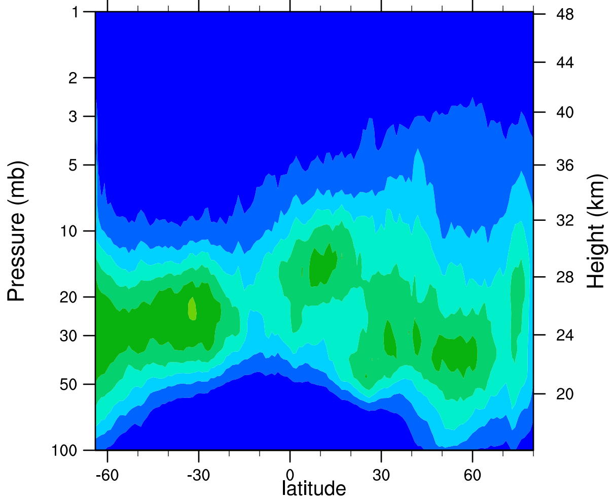
HIRDLSv6 2005d353 ClONO2_Ascending (ppbv)
