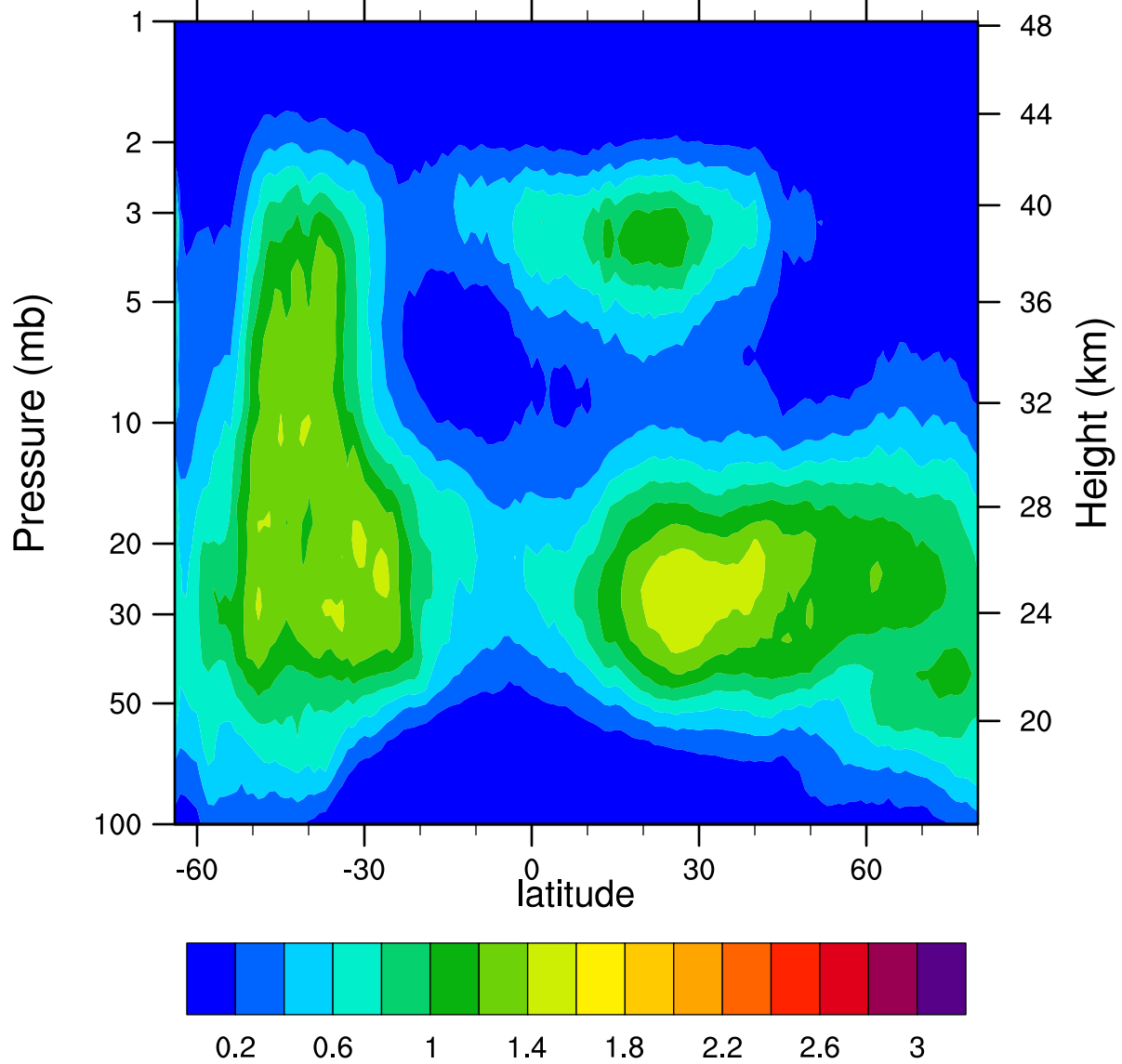
HIRDLSv6 2007d152 ClONO2_Ascending (ppbv)
