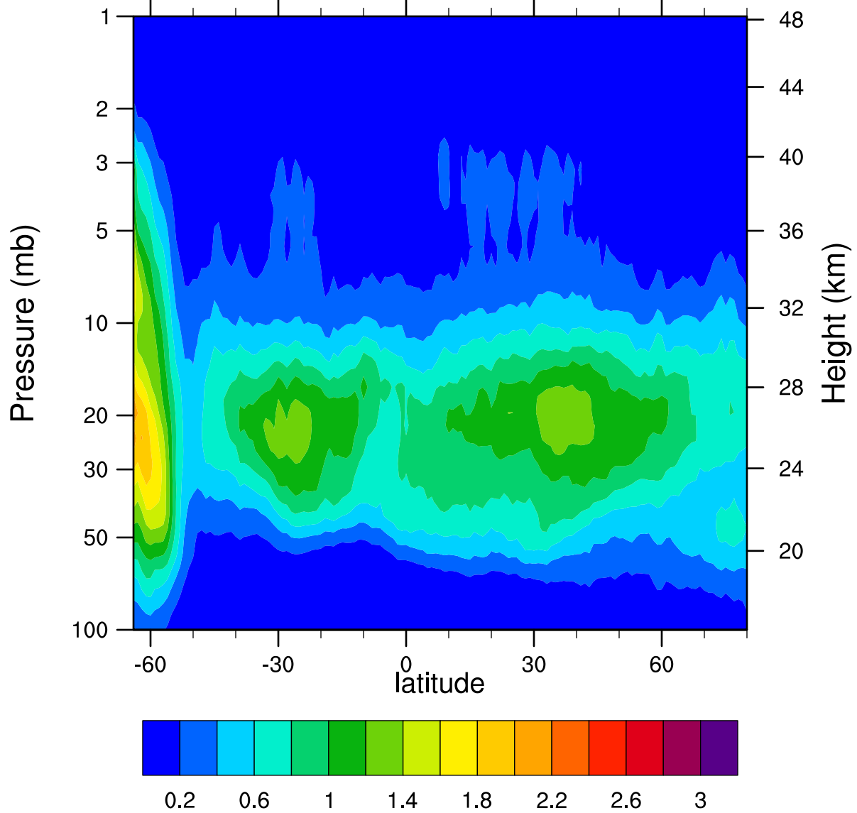
HIRDLSv6 2006d232 ClONO2_Ascending (ppbv)
