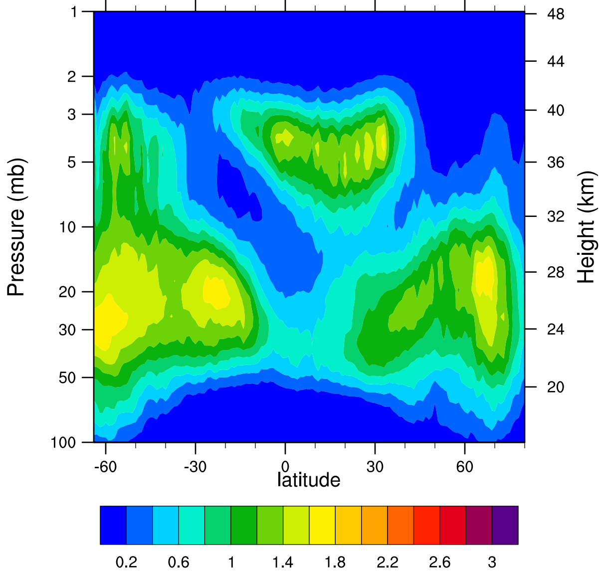
HIRDLSv6 2006d318 ClONO2_Ascending (ppbv)
