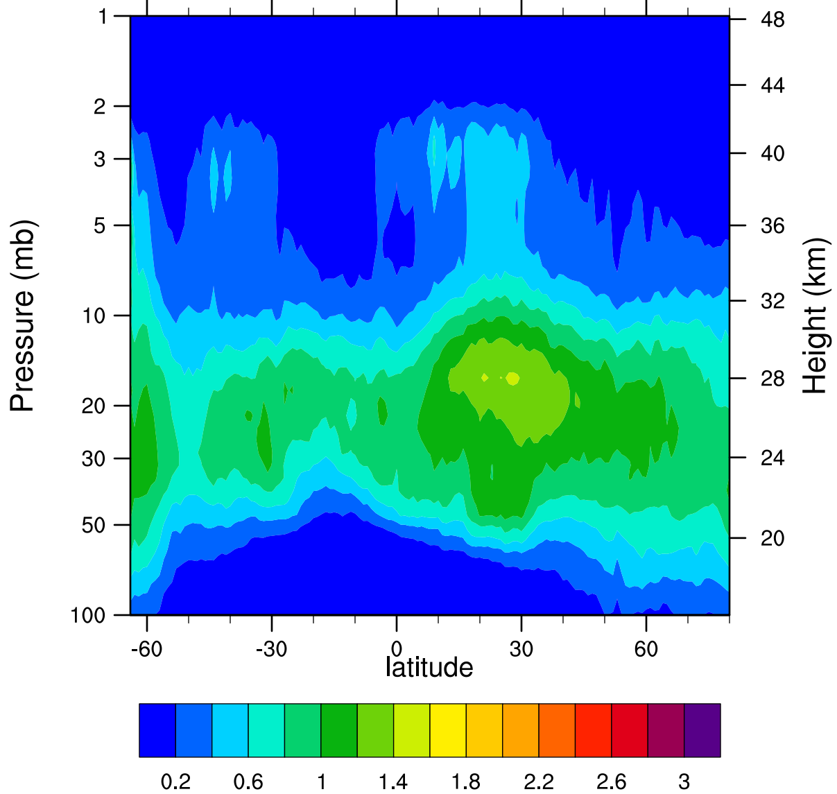
HIRDLSv6 2006d123 ClONO2_Ascending (ppbv)
