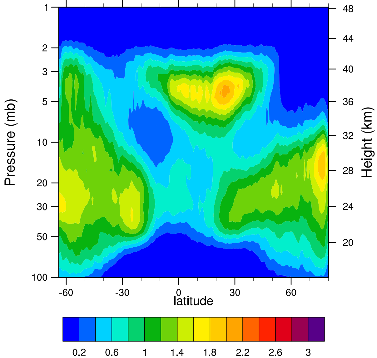
HIRDLSv6 2007d290 ClONO2_Ascending (ppbv)
