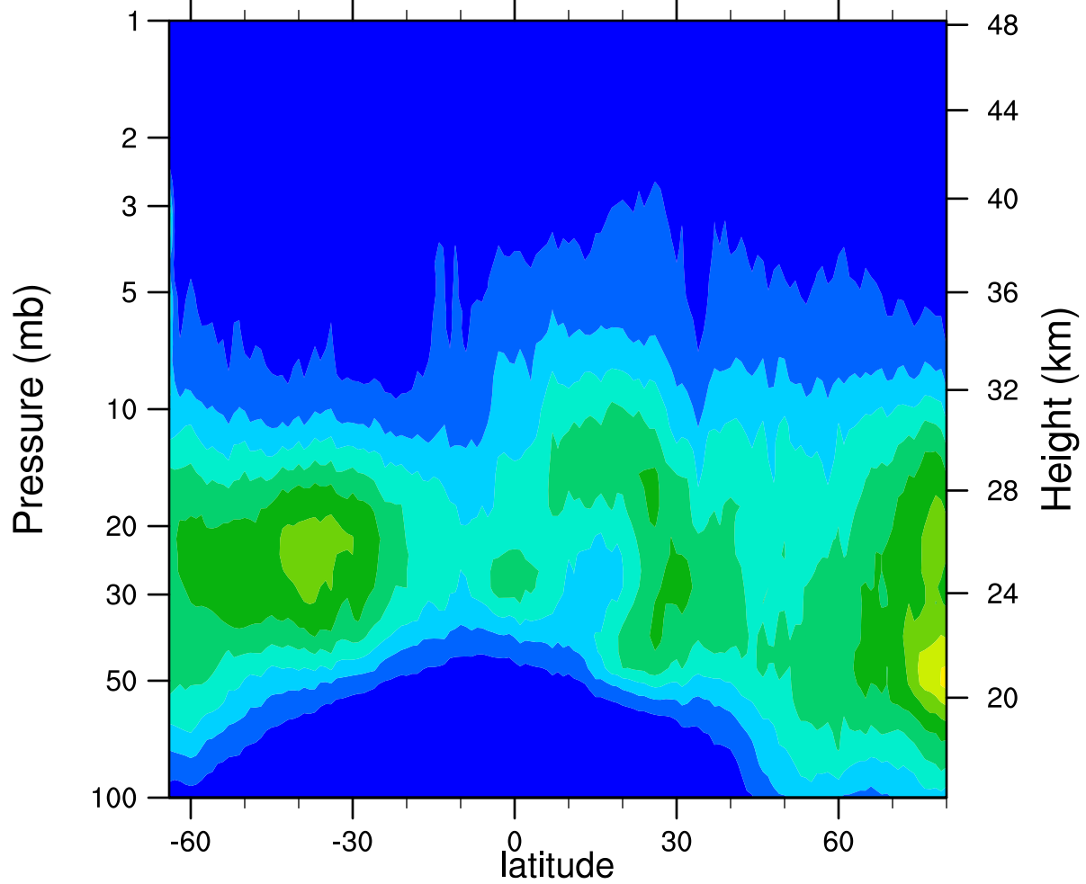
HIRDLSv6 2006d024 ClONO2_Ascending (ppbv)
