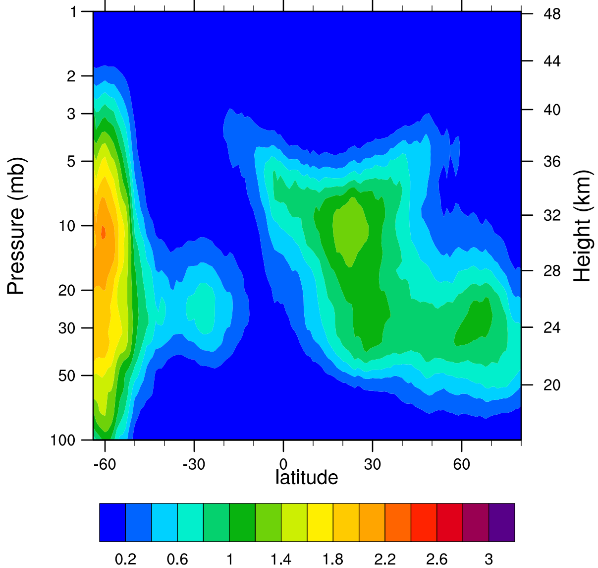
HIRDLSv6 2005d132 ClONO2_Ascending (ppbv)
