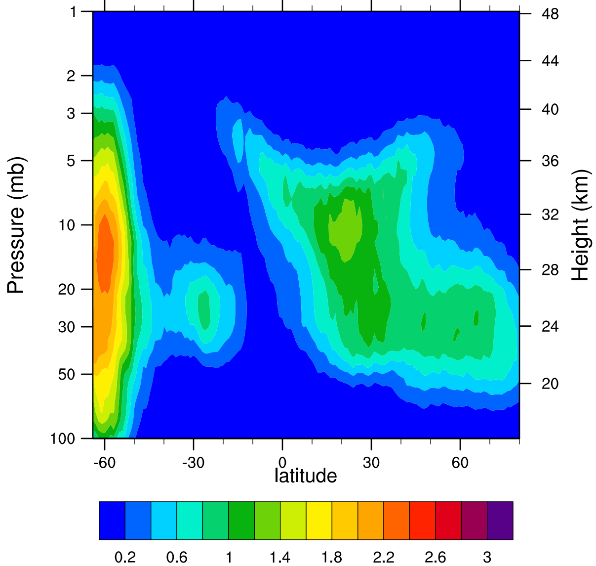
HIRDLSv6 2005d143 ClONO2_Ascending (ppbv)
