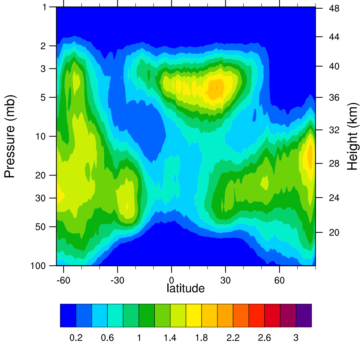
HIRDLSv6 2007d287 ClONO2_Ascending (ppbv)
