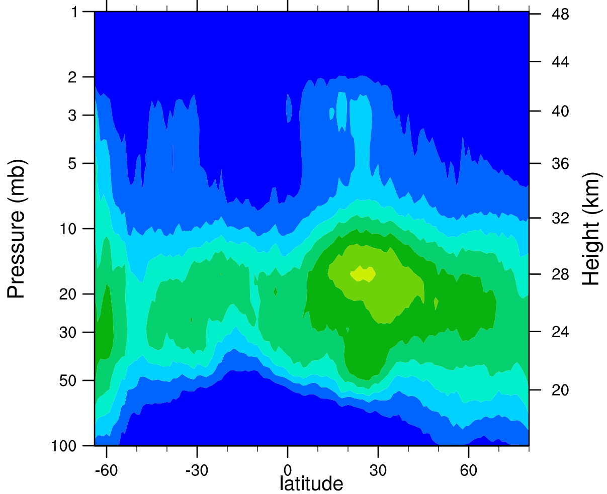
HIRDLSv6 2006d126 ClONO2_Ascending (ppbv)
