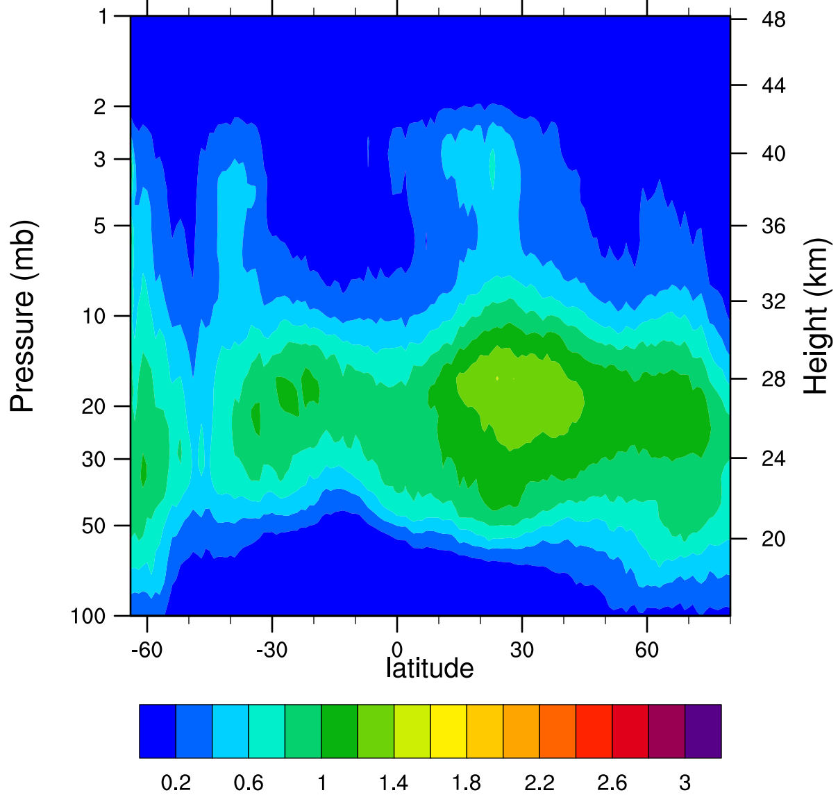
HIRDLSv6 2006d142 ClONO2_Ascending (ppbv)
