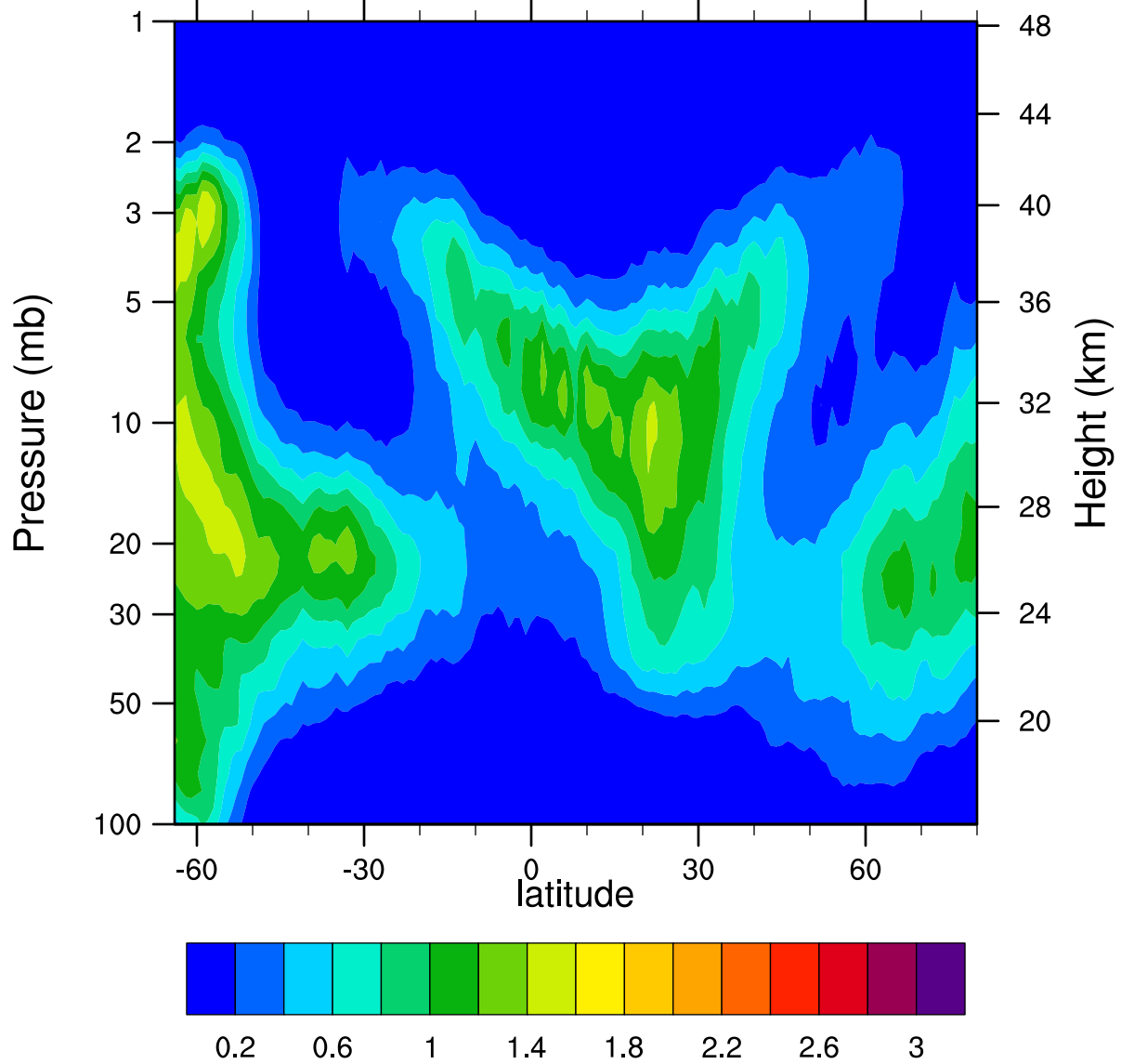
HIRDLSv6 2005d032 ClONO2_Ascending (ppbv)
