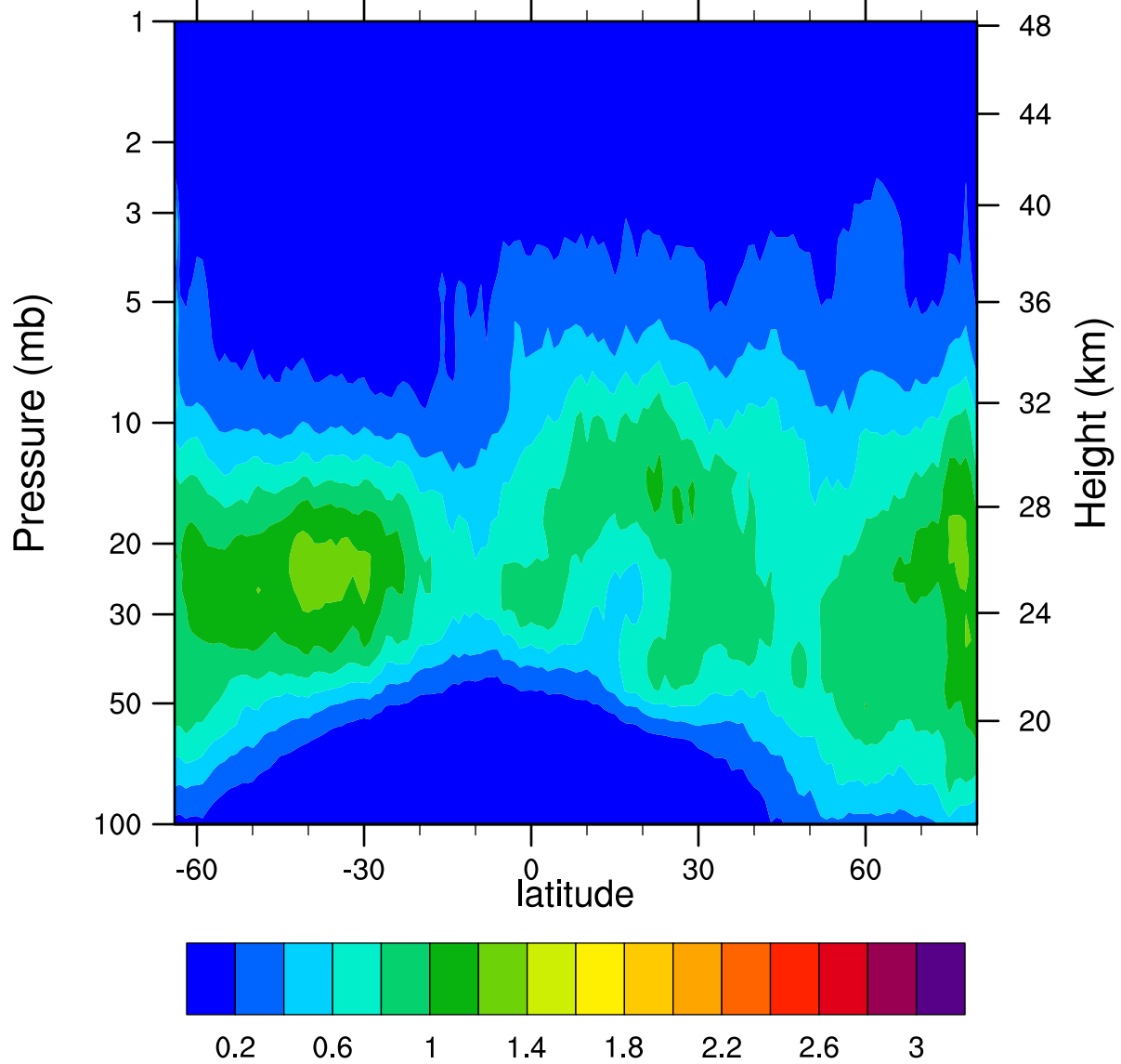
HIRDLSv6 2006d018 ClONO2_Ascending (ppbv)
