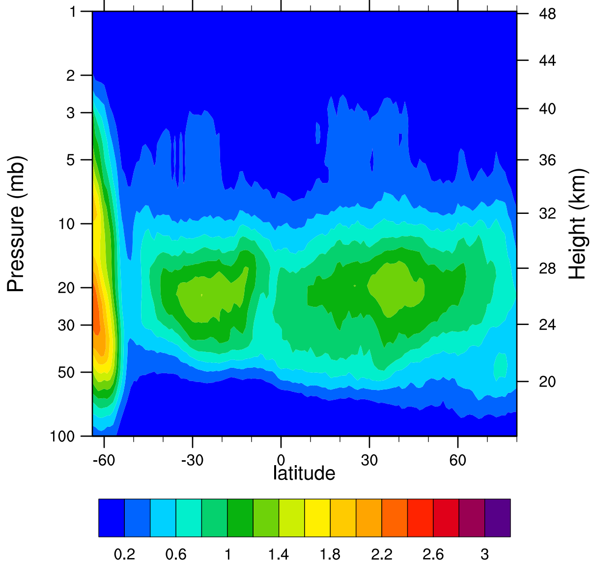
HIRDLSv6 2006d241 ClONO2_Ascending (ppbv)
