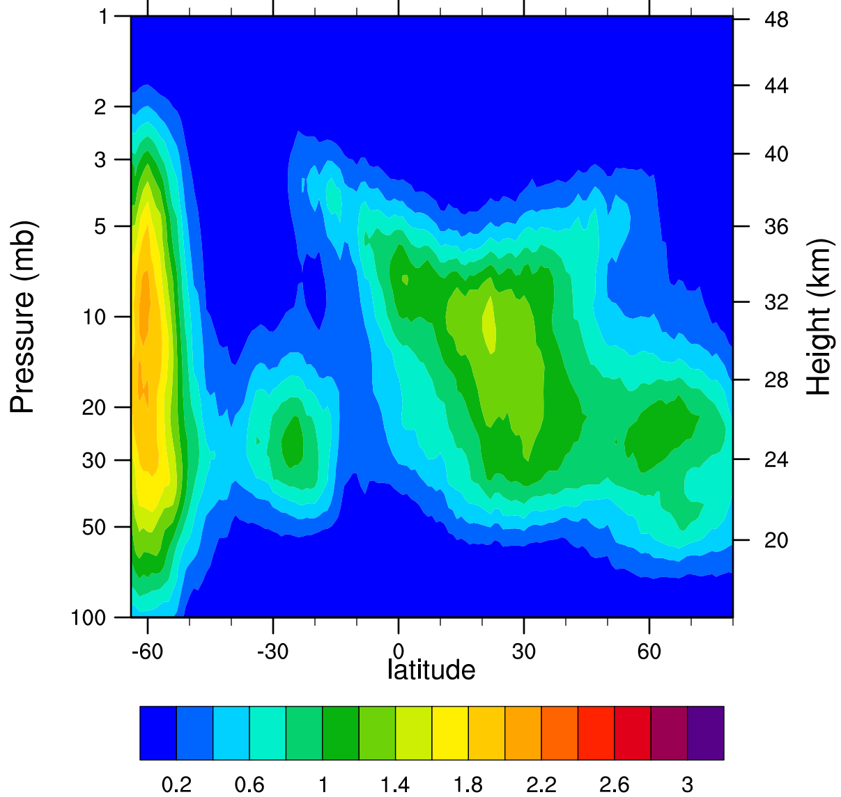
HIRDLSv6 2005d174 ClONO2_Ascending (ppbv)
