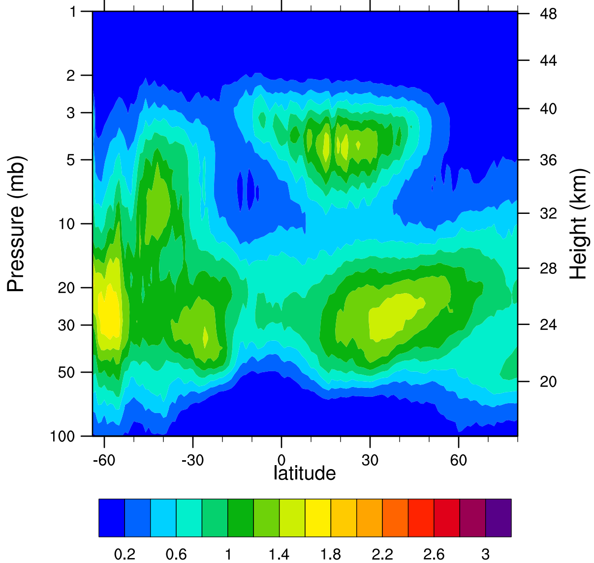
HIRDLSv6 2007d212 ClONO2_Ascending (ppbv)
