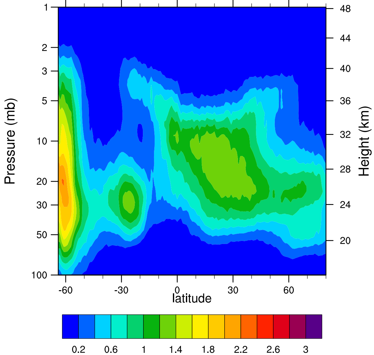
HIRDLSv6 2005d202 ClONO2_Ascending (ppbv)
