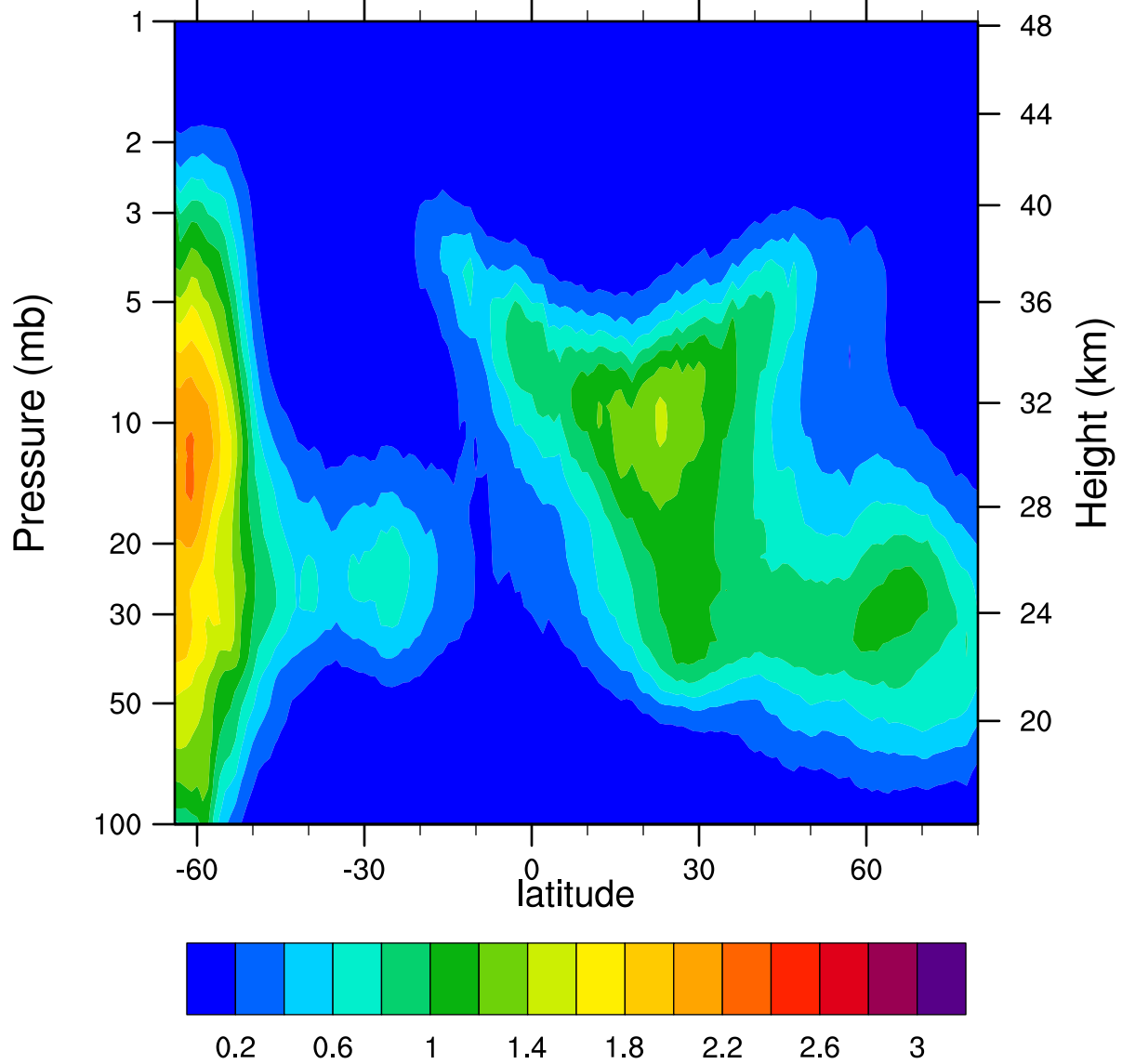
HIRDLSv6 2005d125 ClONO2_Ascending (ppbv)
