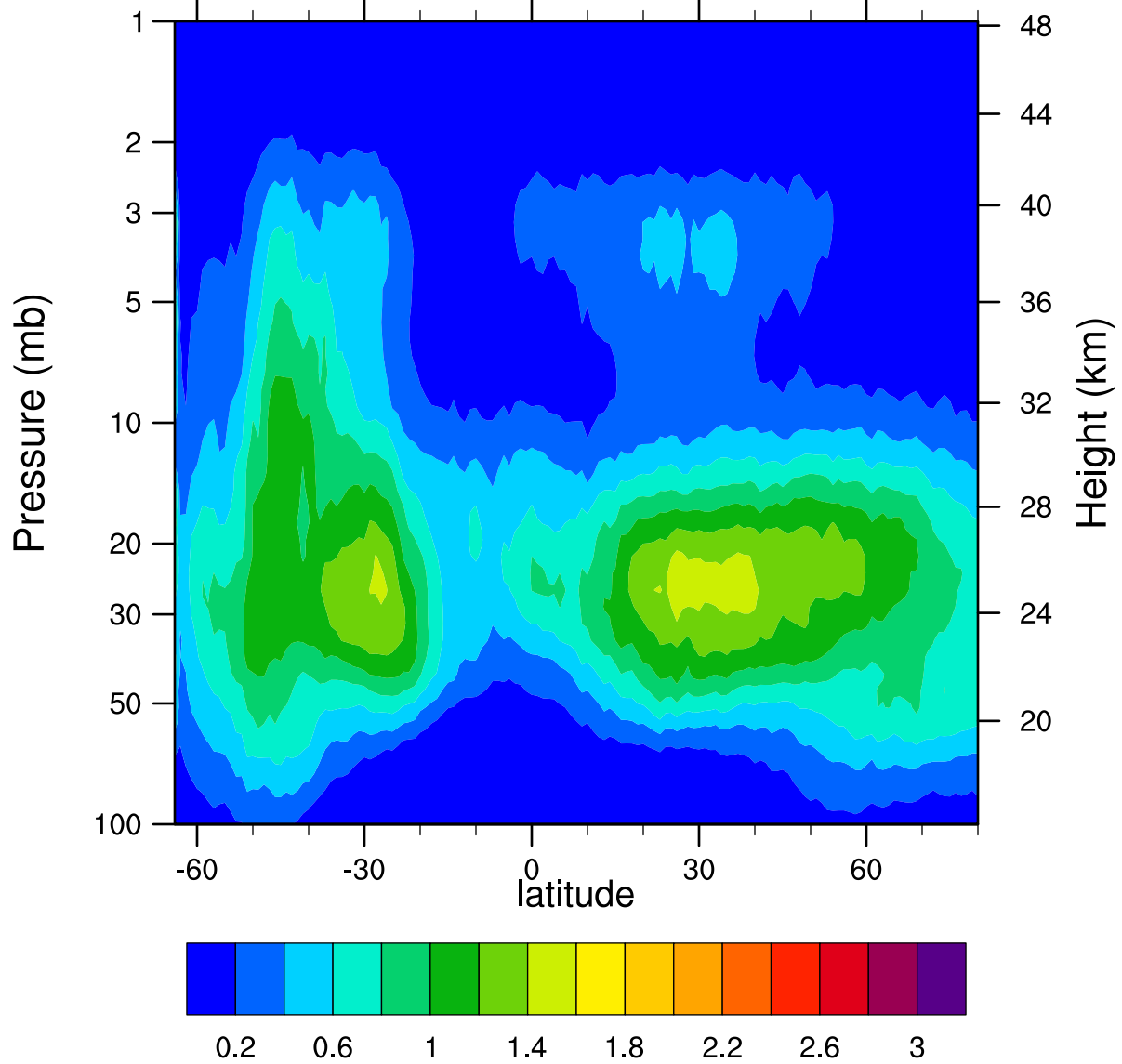
HIRDLSv6 2007d180 ClONO2_Ascending (ppbv)
