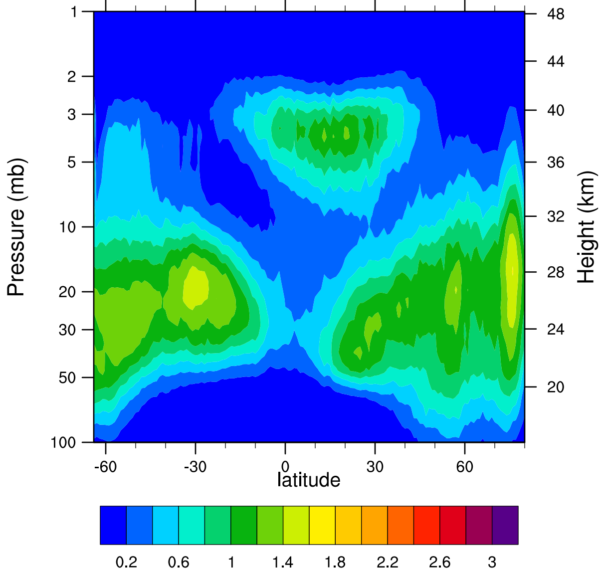
HIRDLSv6 2006d357 ClONO2_Ascending (ppbv)
