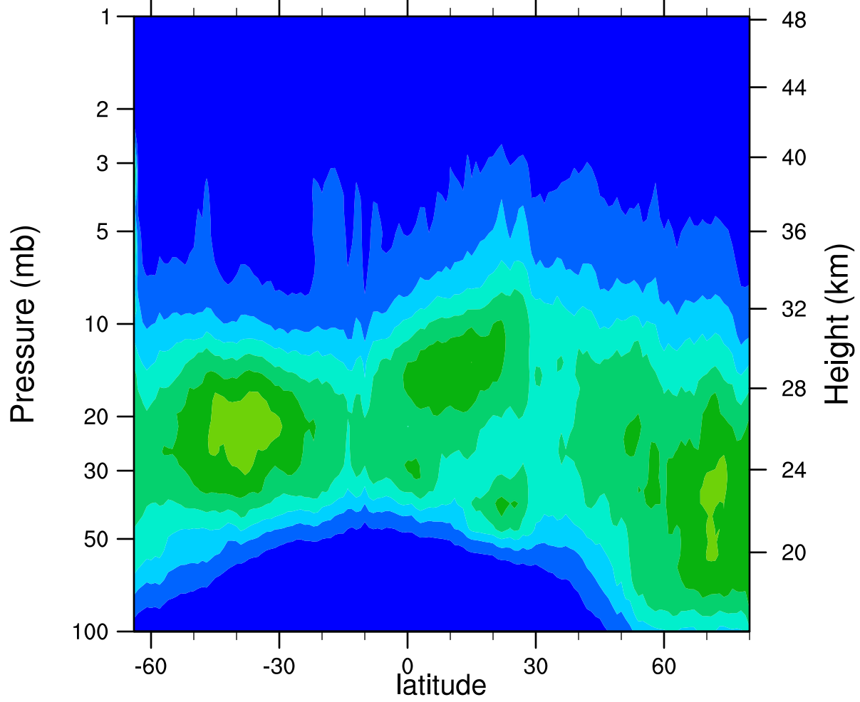
HIRDLSv6 2006d052 ClONO2_Ascending (ppbv)
