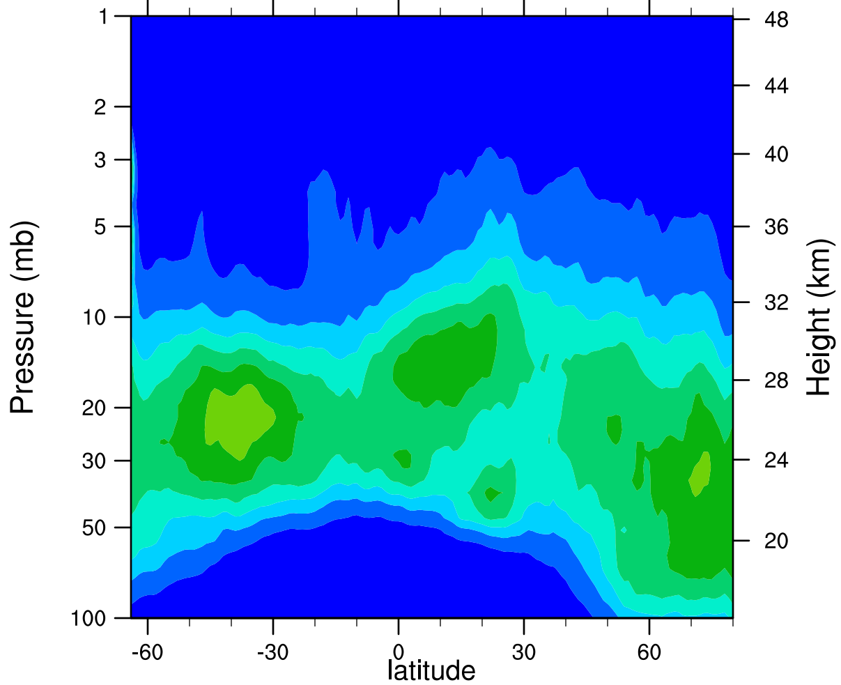
HIRDLSv6 2006d053 ClONO2_Ascending (ppbv)
