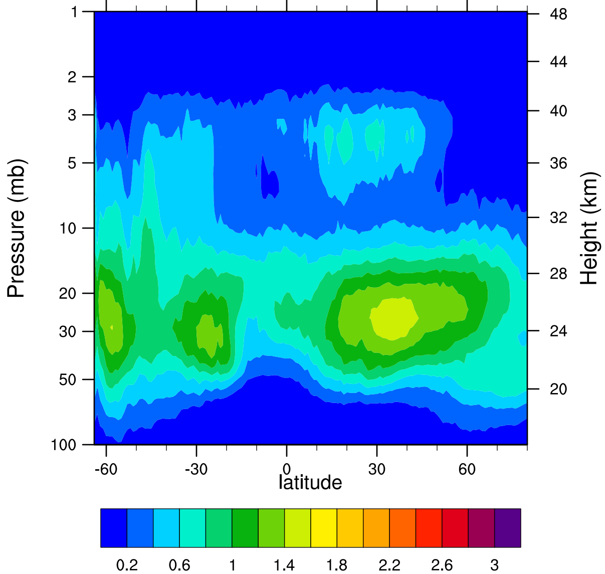
HIRDLSv6 2007d204 ClONO2_Ascending (ppbv)
