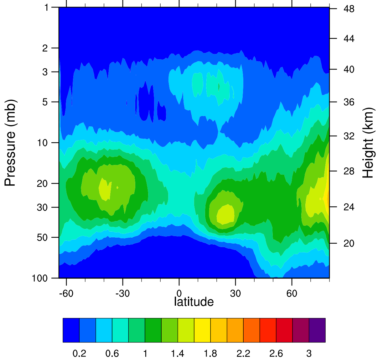
HIRDLSv6 2007d044 ClONO2_Ascending (ppbv)
