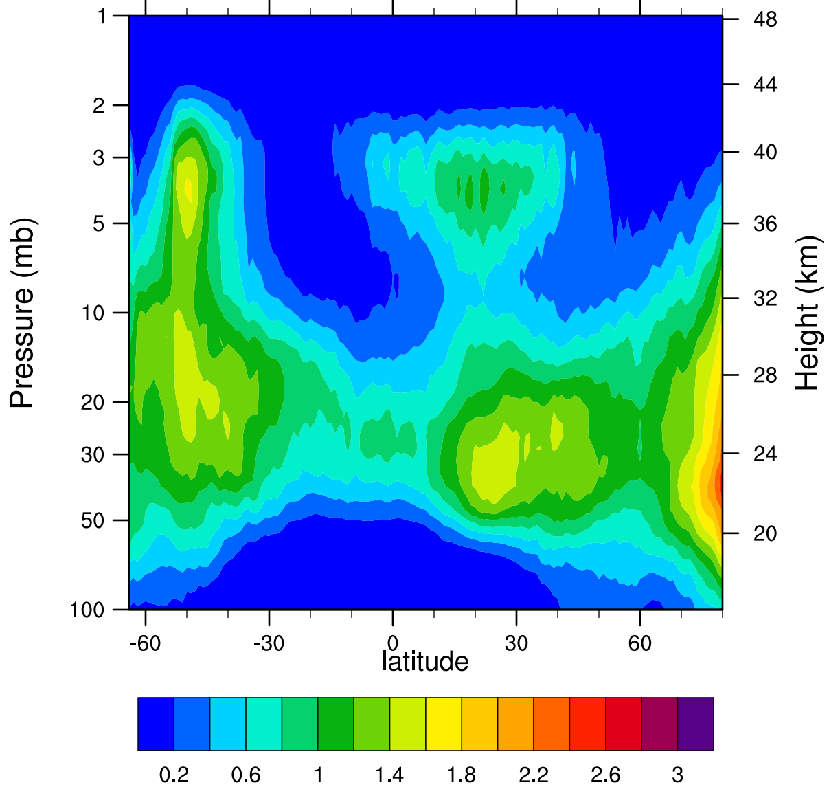
HIRDLSv6 2007d086 ClONO2_Ascending (ppbv)
