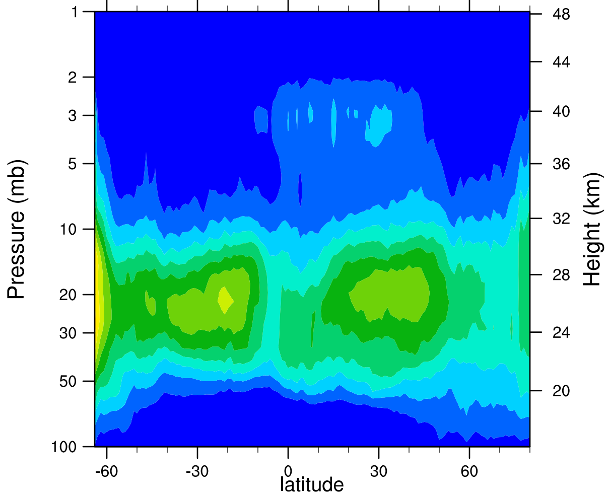
HIRDLSv6 2006d282 ClONO2_Ascending (ppbv)
