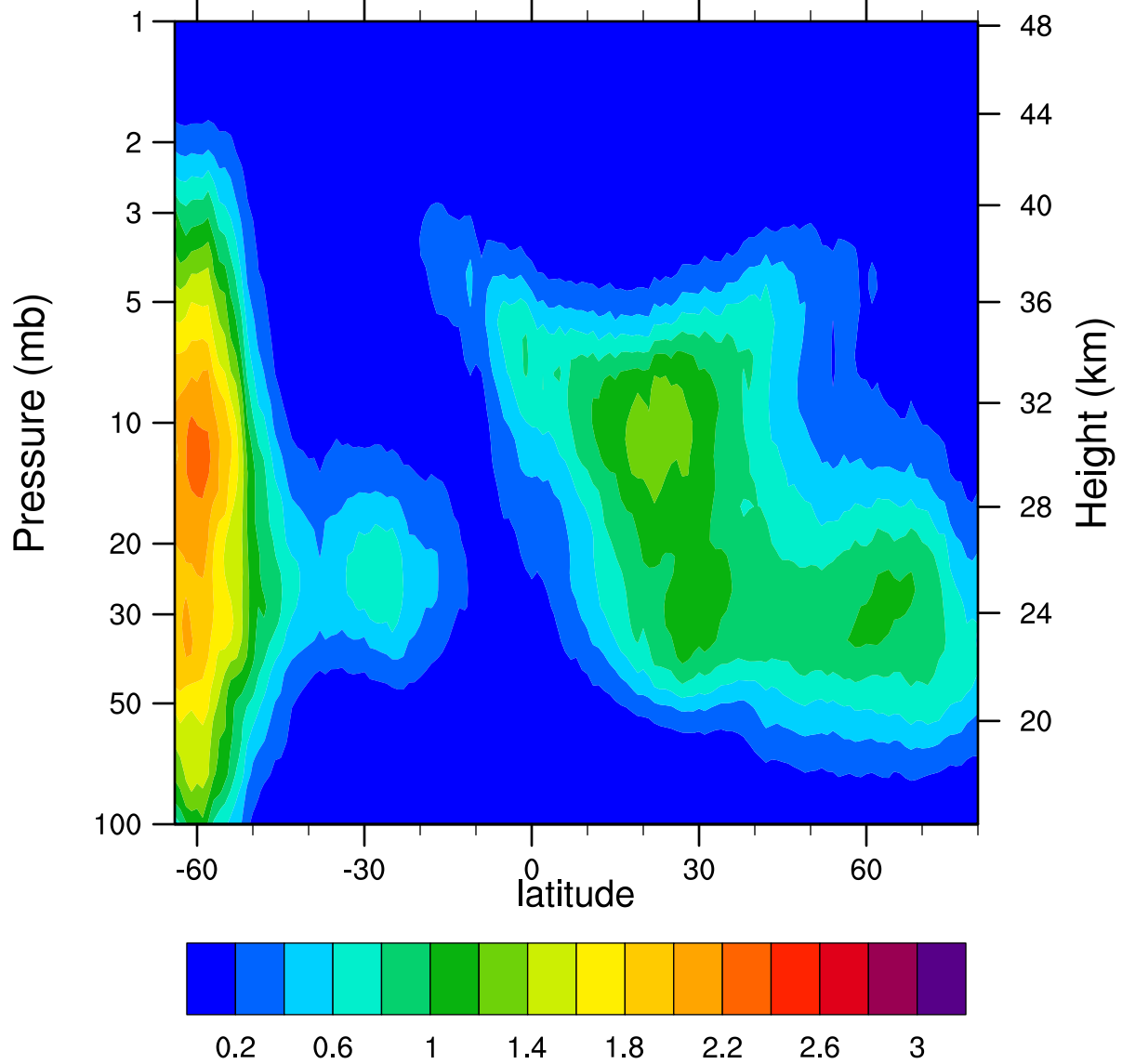
HIRDLSv6 2005d135 ClONO2_Ascending (ppbv)
