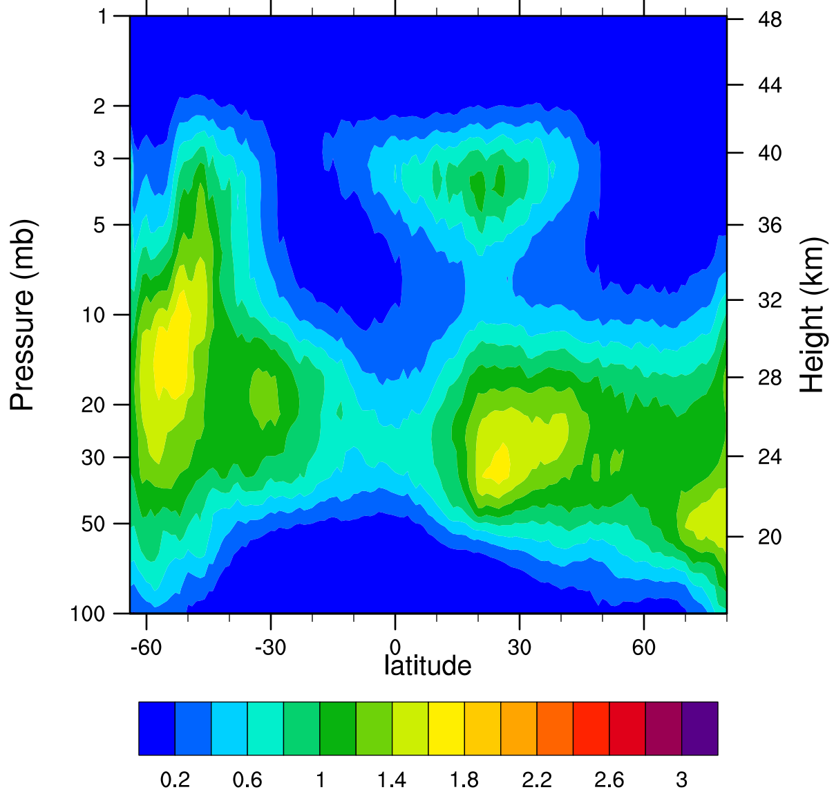
HIRDLSv6 2007d116 ClONO2_Ascending (ppbv)
