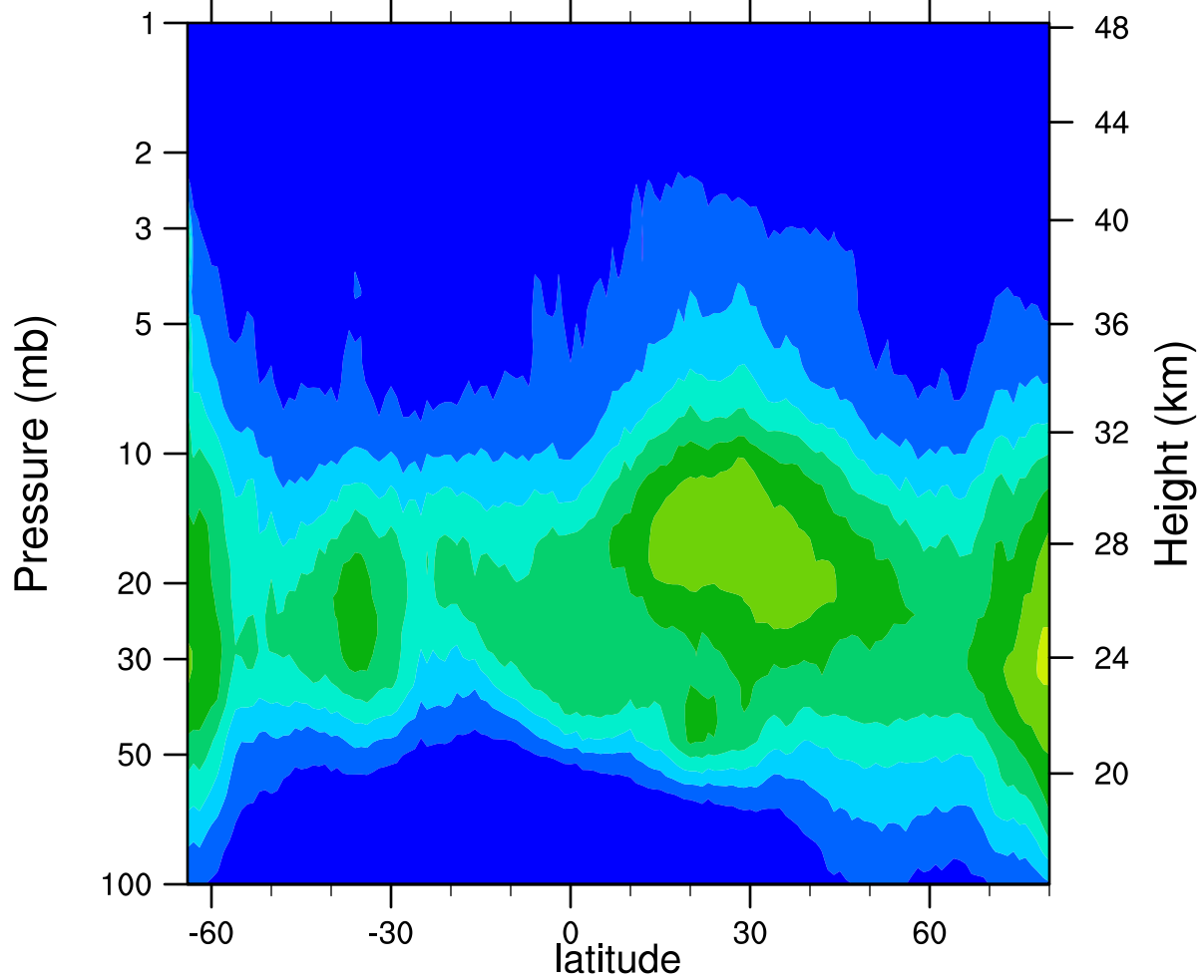
HIRDLSv6 2006d109 ClONO2_Ascending (ppbv)
