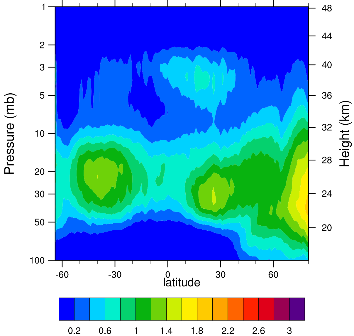
HIRDLSv6 2007d060 ClONO2_Ascending (ppbv)
