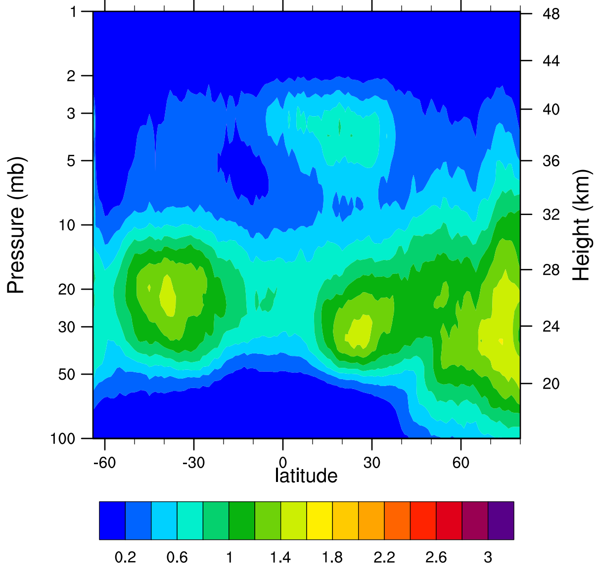
HIRDLSv6 2007d056 ClONO2_Ascending (ppbv)
