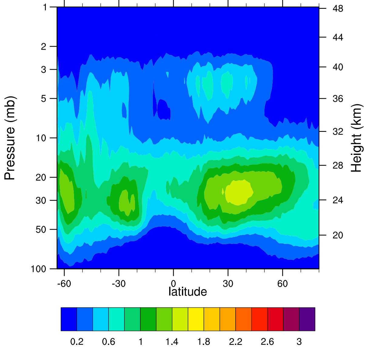
HIRDLSv6 2007d203 ClONO2_Ascending (ppbv)
