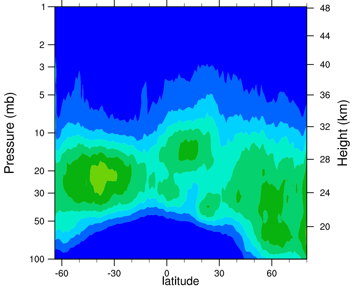
HIRDLSv6 2006d042 ClONO2_Ascending (ppbv)
