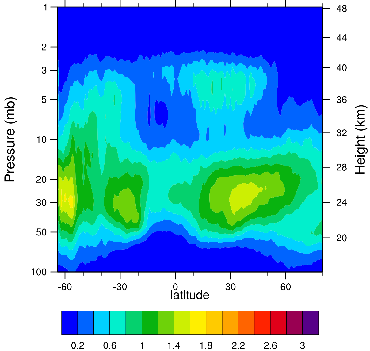
HIRDLSv6 2007d209 ClONO2_Ascending (ppbv)
