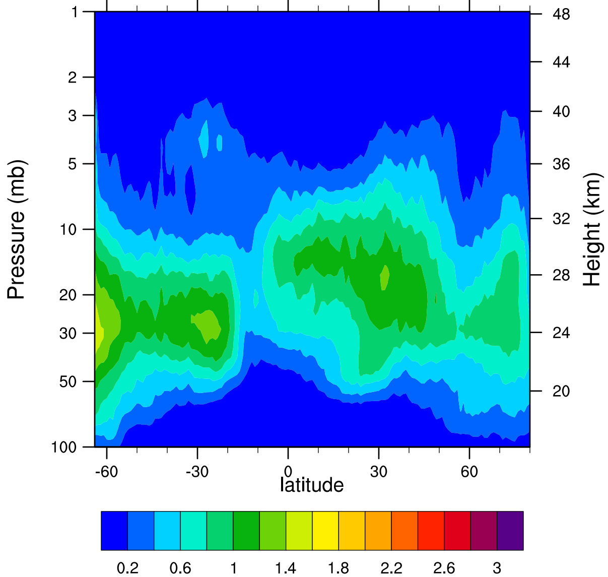
HIRDLSv6 2005d302 ClONO2_Ascending (ppbv)
