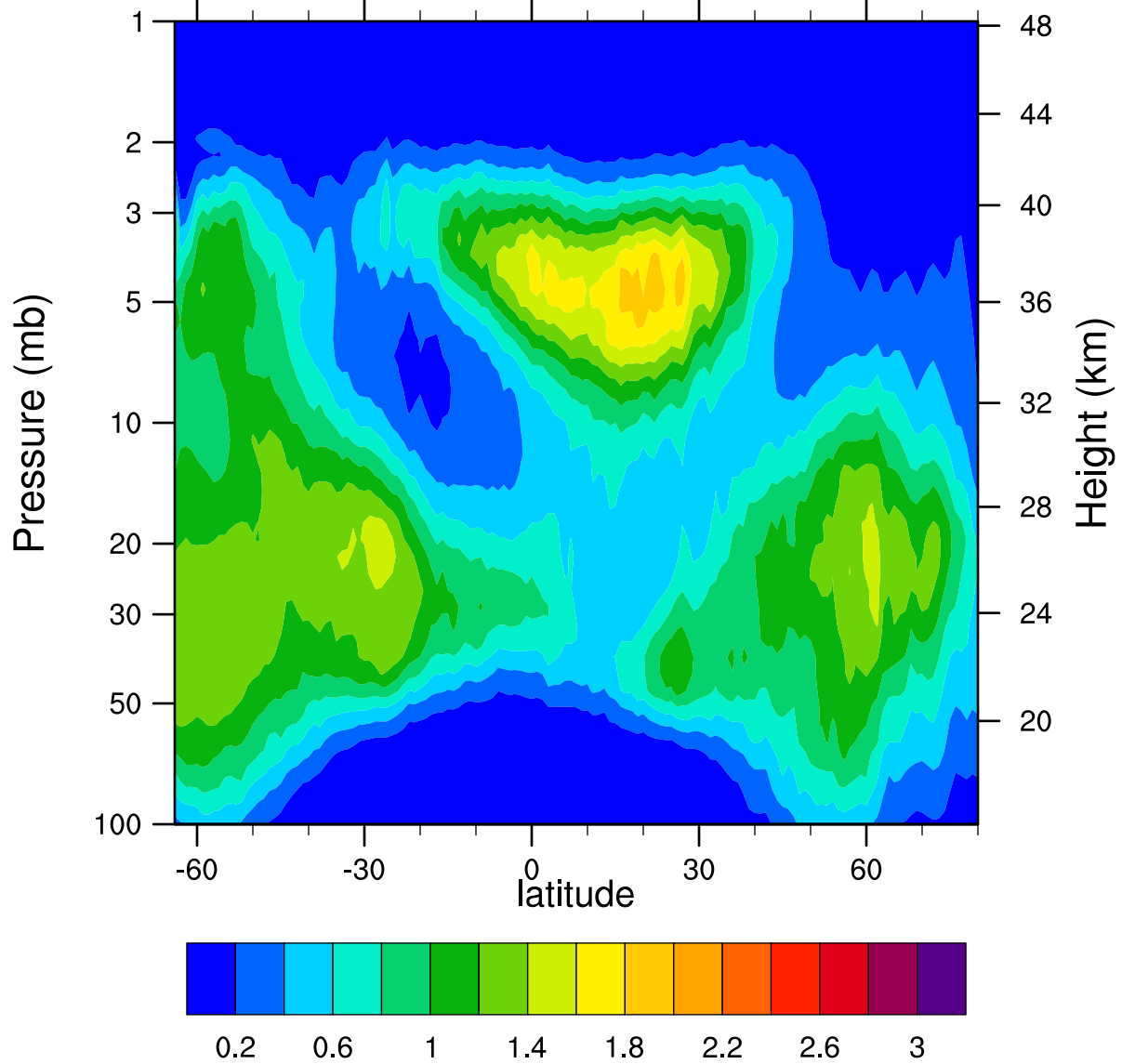
HIRDLSv6 2007d358 ClONO2_Ascending (ppbv)
