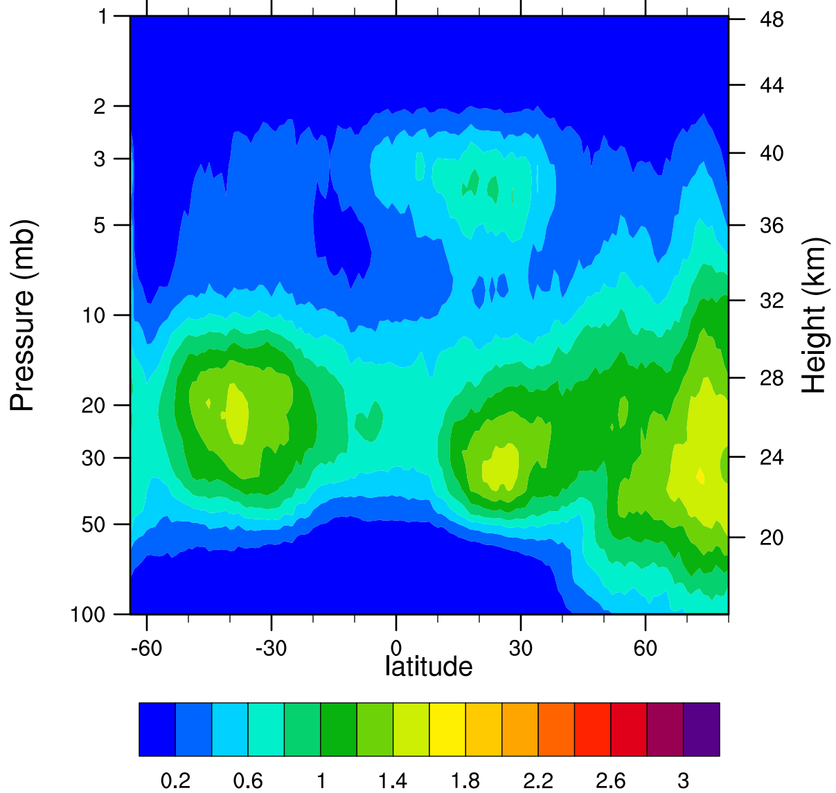
HIRDLSv6 2007d055 ClONO2_Ascending (ppbv)
