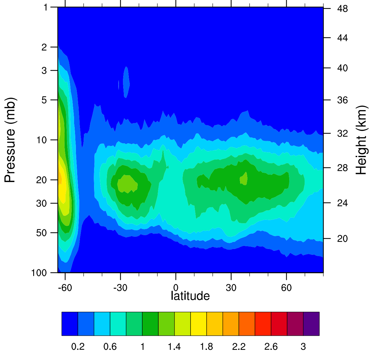
HIRDLSv6 2006d216 ClONO2_Ascending (ppbv)
