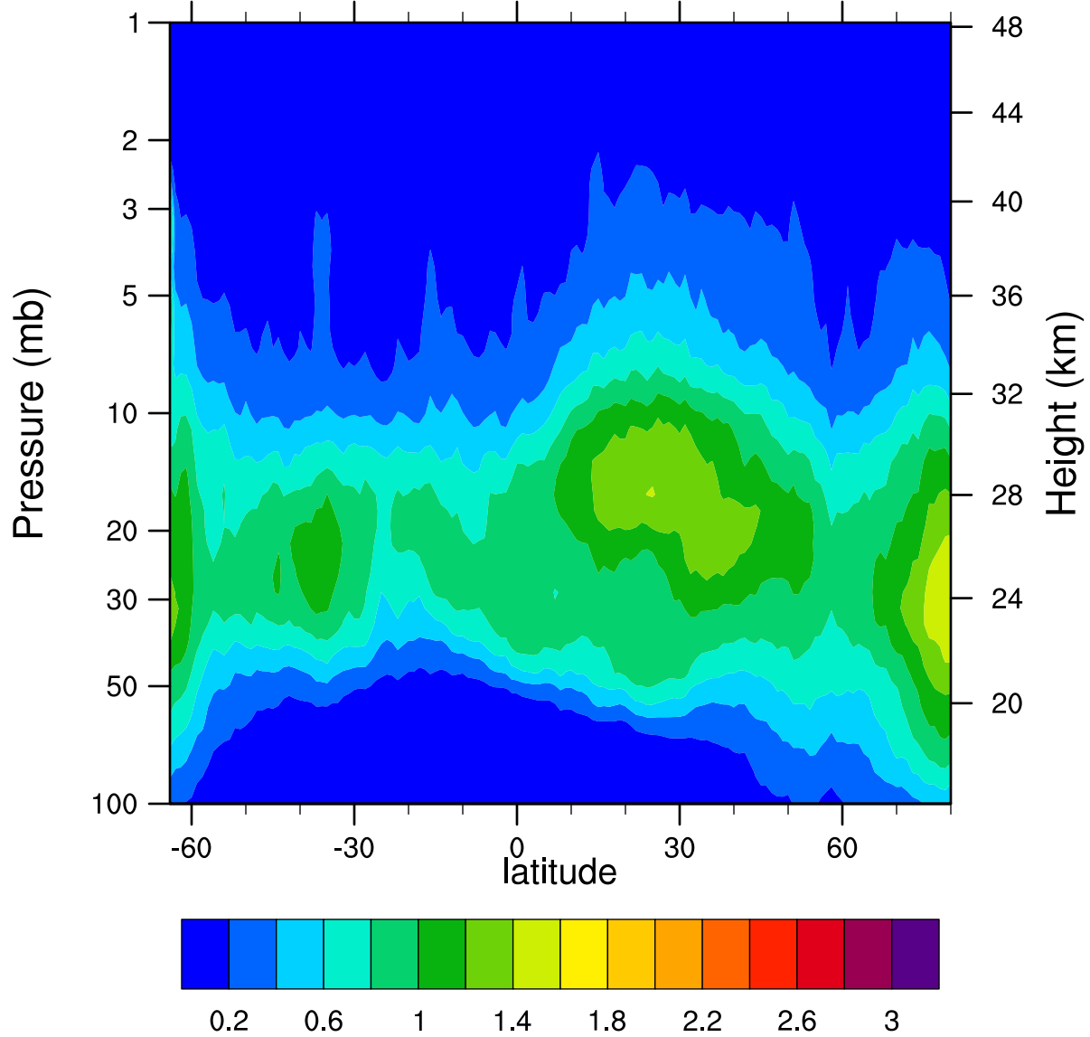
HIRDLSv6 2006d103 ClONO2_Ascending (ppbv)
