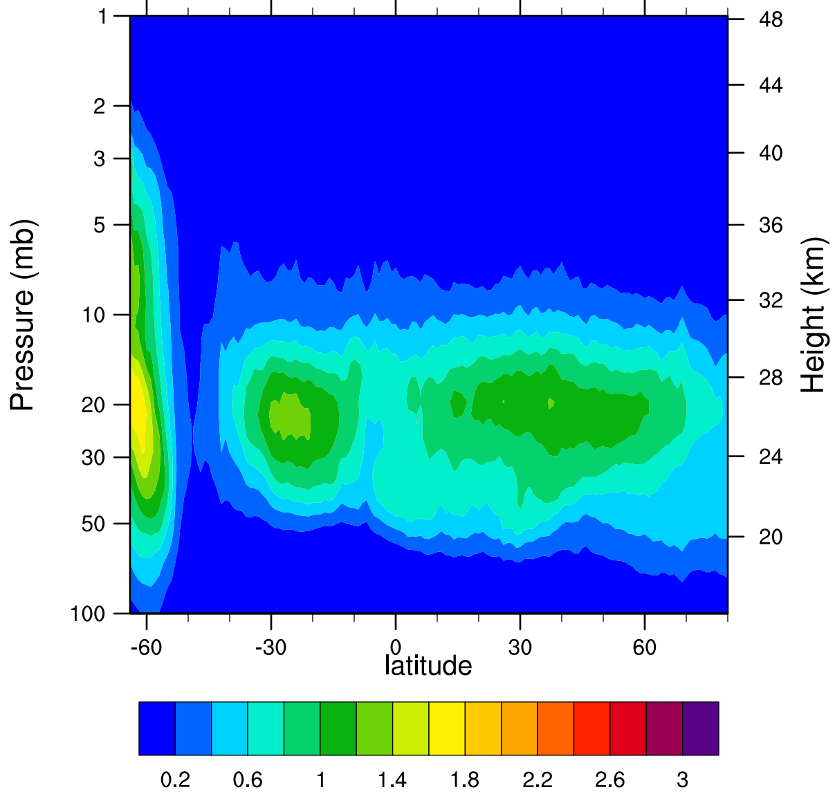
HIRDLSv6 2006d212 ClONO2_Ascending (ppbv)
