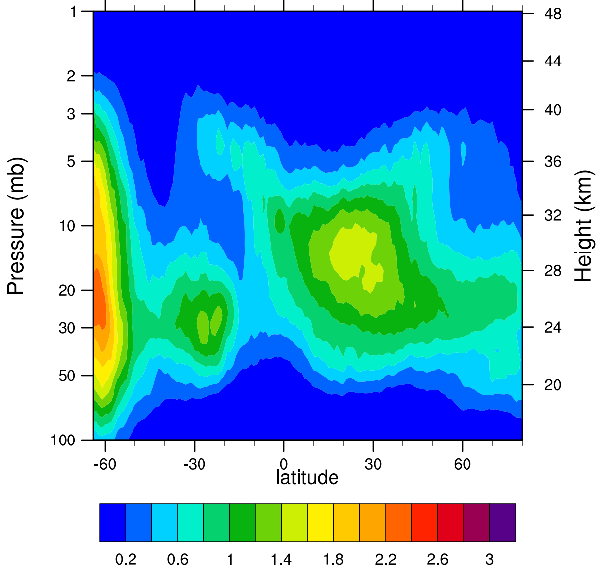
HIRDLSv6 2005d227 ClONO2_Ascending (ppbv)
