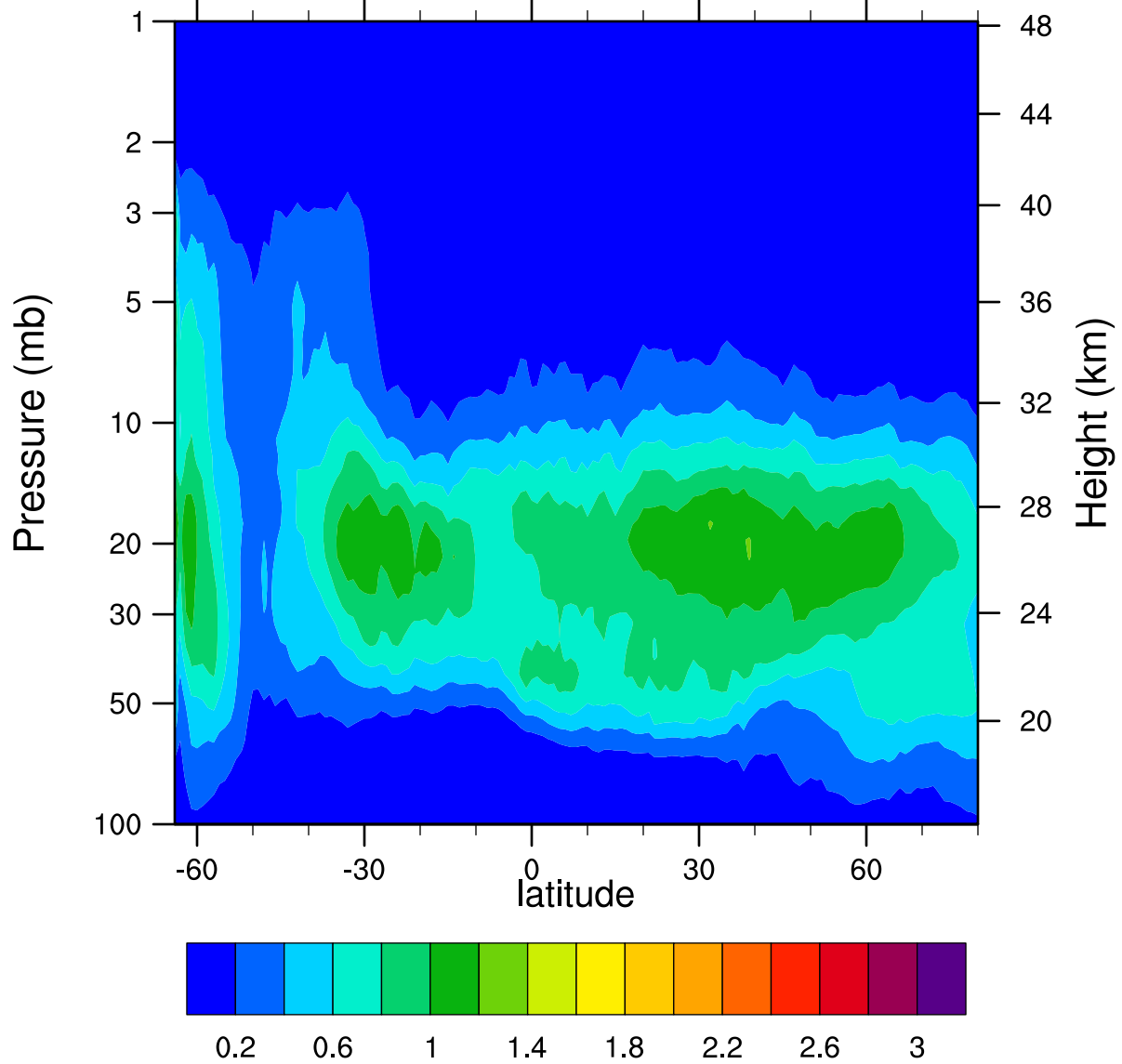
HIRDLSv6 2006d183 ClONO2_Ascending (ppbv)
