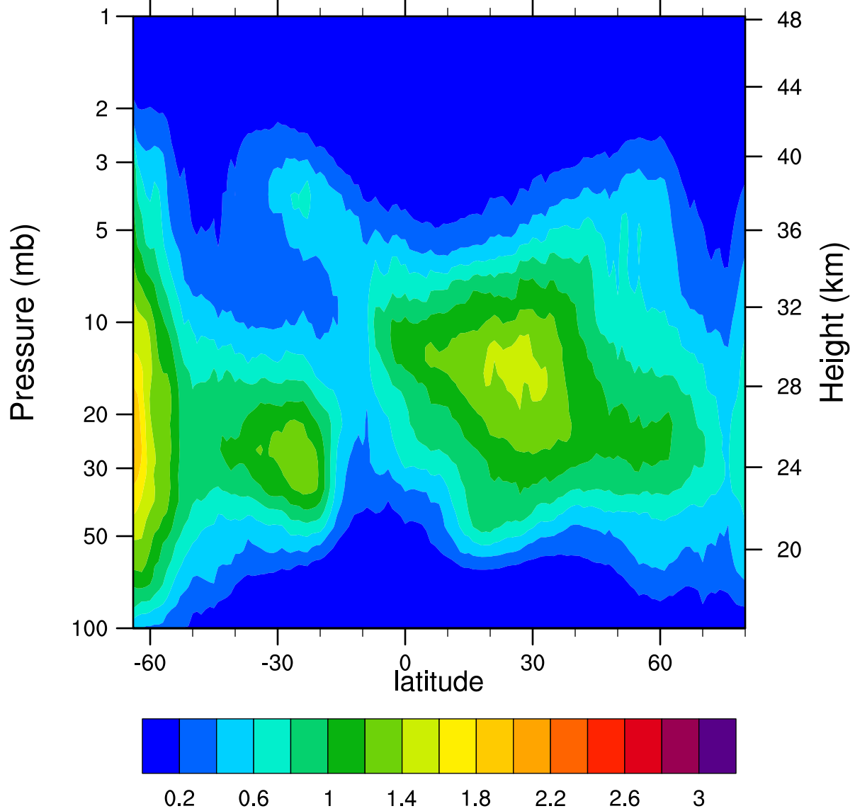
HIRDLSv6 2005d270 ClONO2_Ascending (ppbv)
