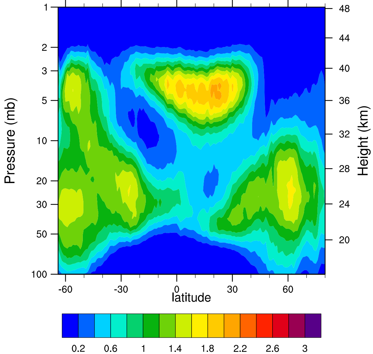
HIRDLSv6 2007d337 ClONO2_Ascending (ppbv)
