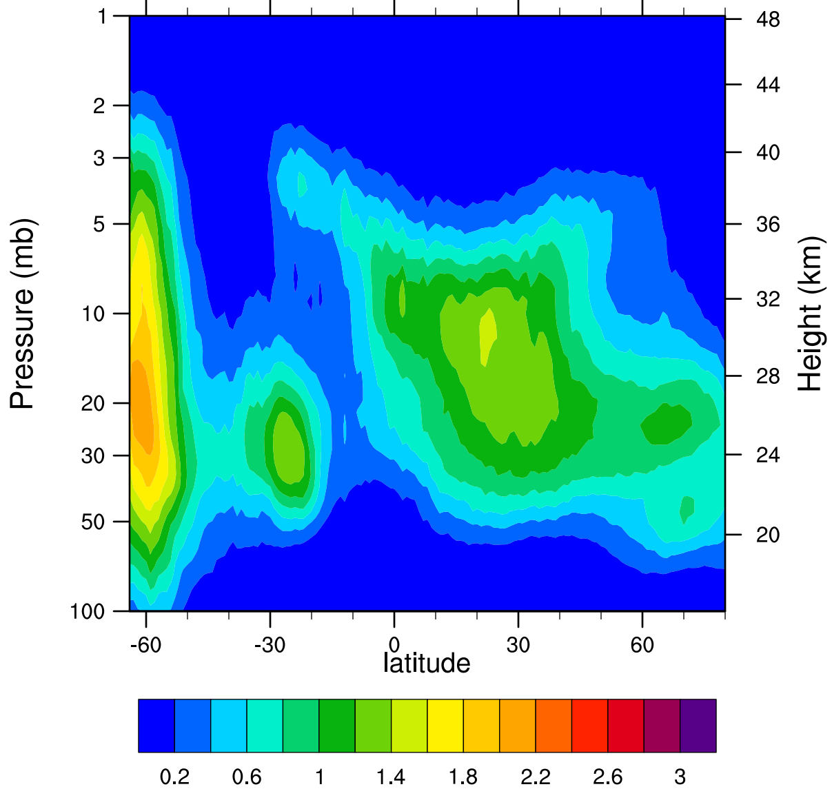
HIRDLSv6 2005d192 ClONO2_Ascending (ppbv)
