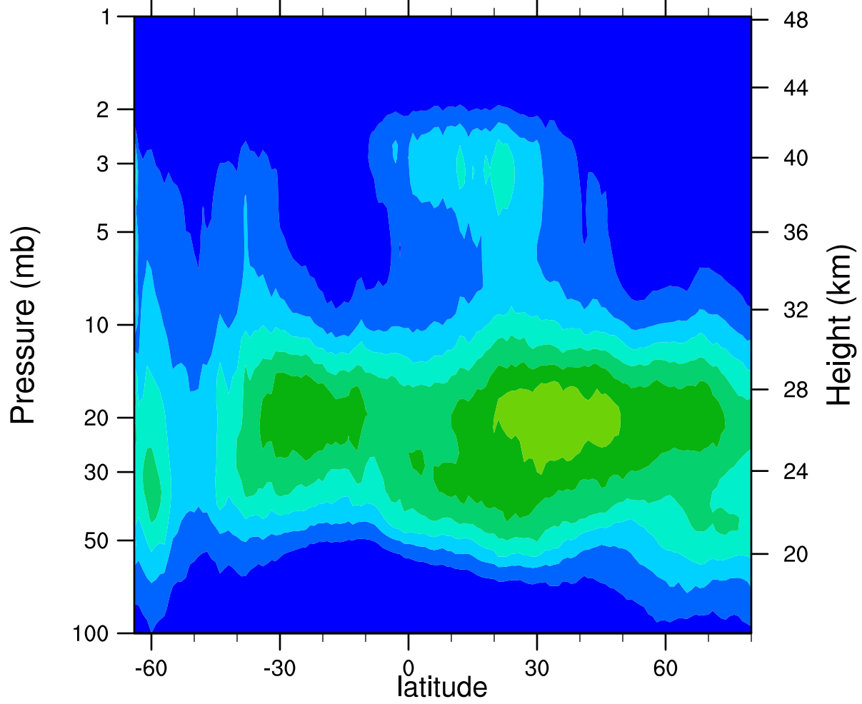
HIRDLSv6 2006d171 ClONO2_Ascending (ppbv)
