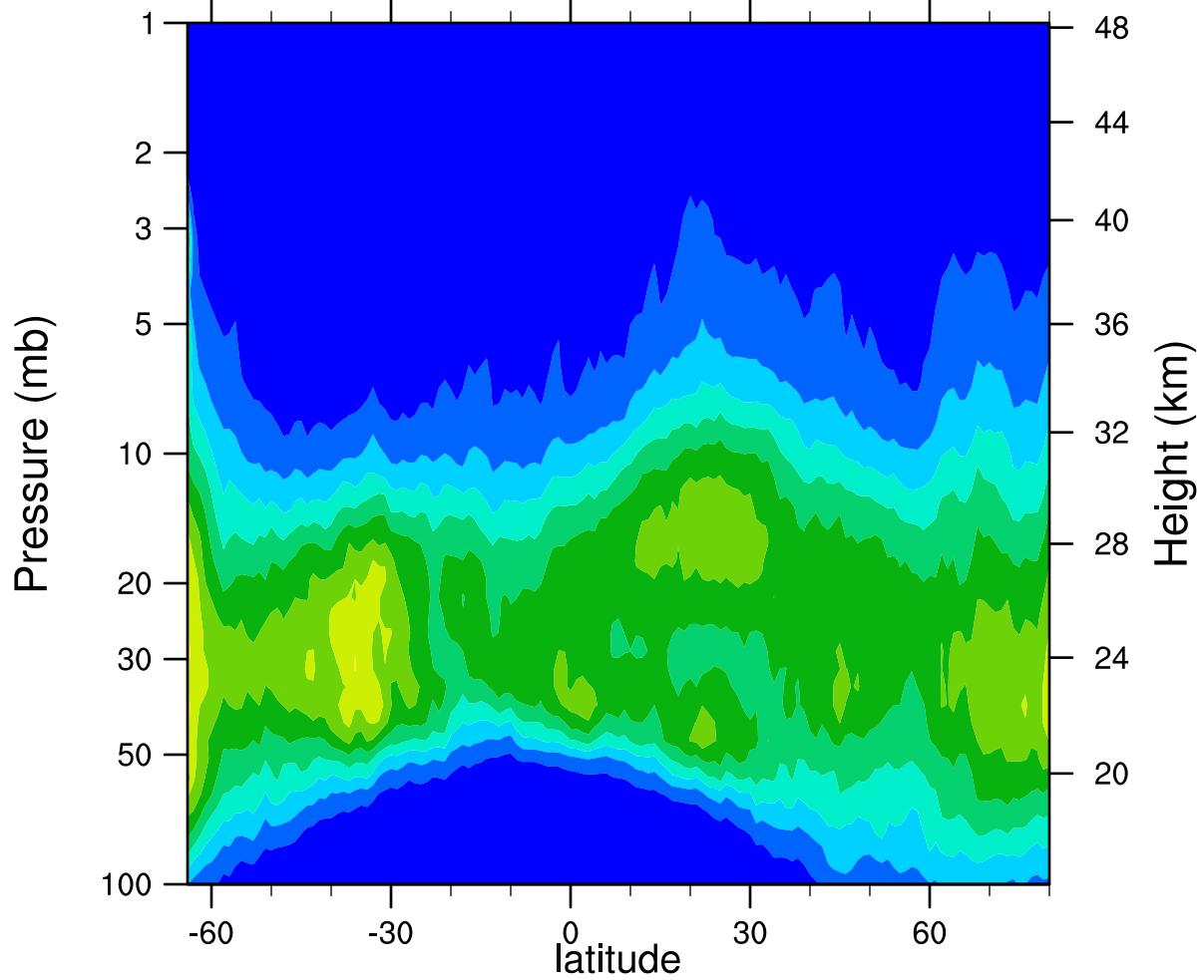
HIRDLSv6 2006d087 ClONO2_Ascending (ppbv)
