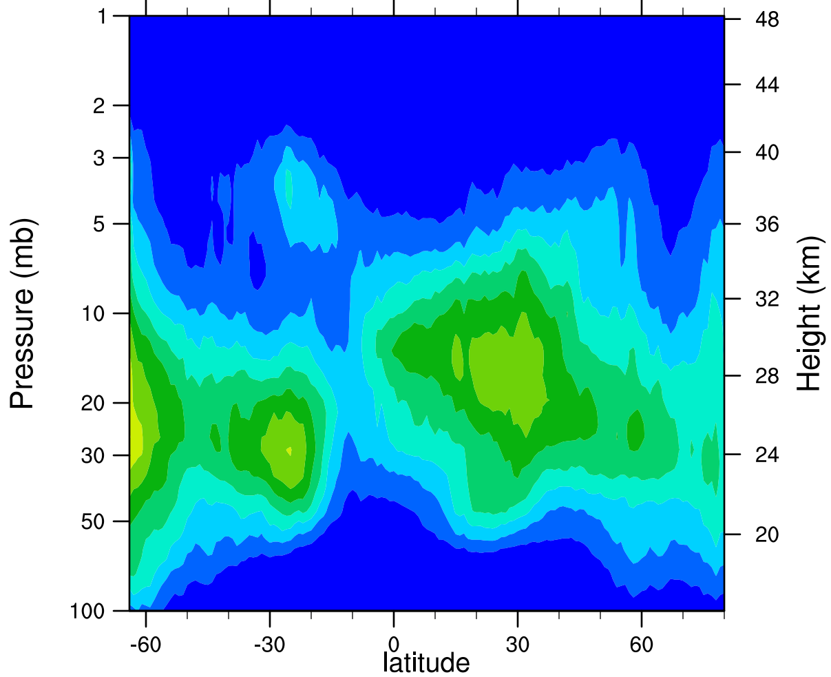
HIRDLSv6 2005d287 ClONO2_Ascending (ppbv)
