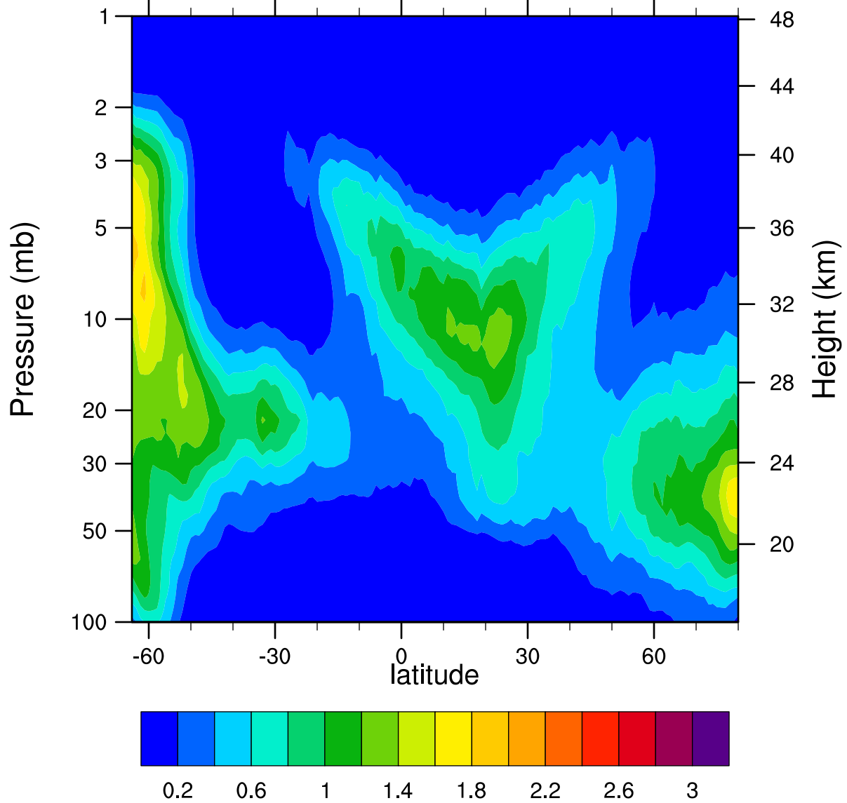
HIRDLSv6 2005d062 ClONO2_Ascending (ppbv)
