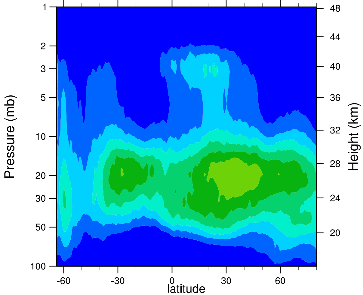
HIRDLSv6 2006d166 ClONO2_Ascending (ppbv)
