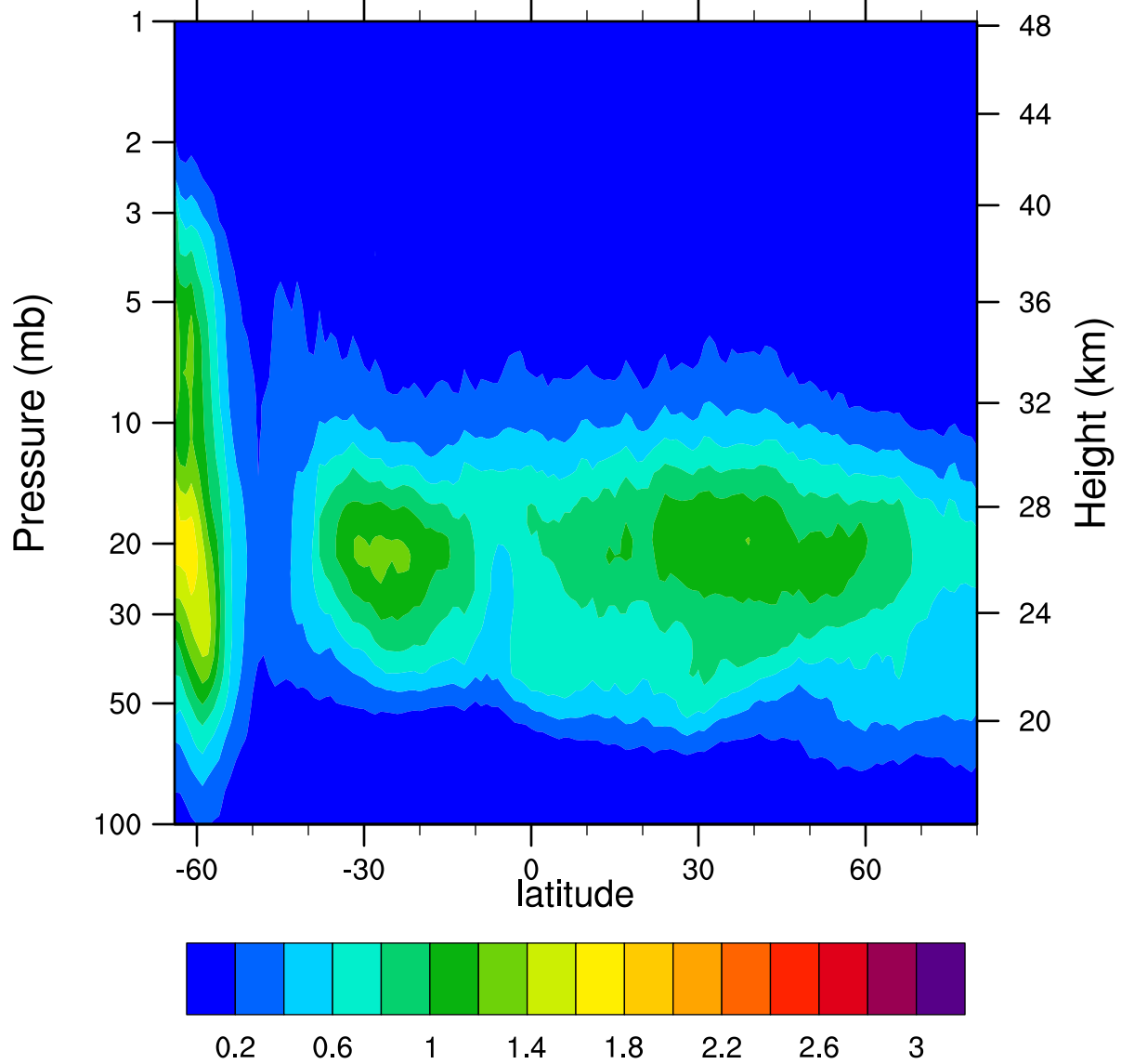
HIRDLSv6 2006d196 ClONO2_Ascending (ppbv)
