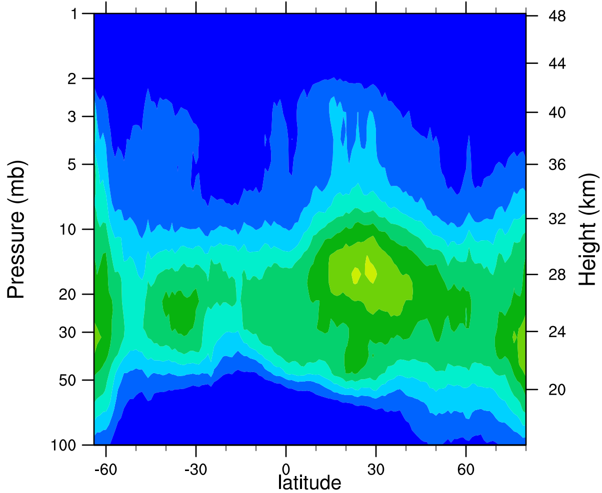
HIRDLSv6 2006d114 ClONO2_Ascending (ppbv)
