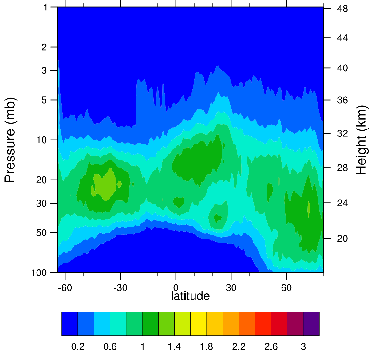
HIRDLSv6 2006d055 ClONO2_Ascending (ppbv)
