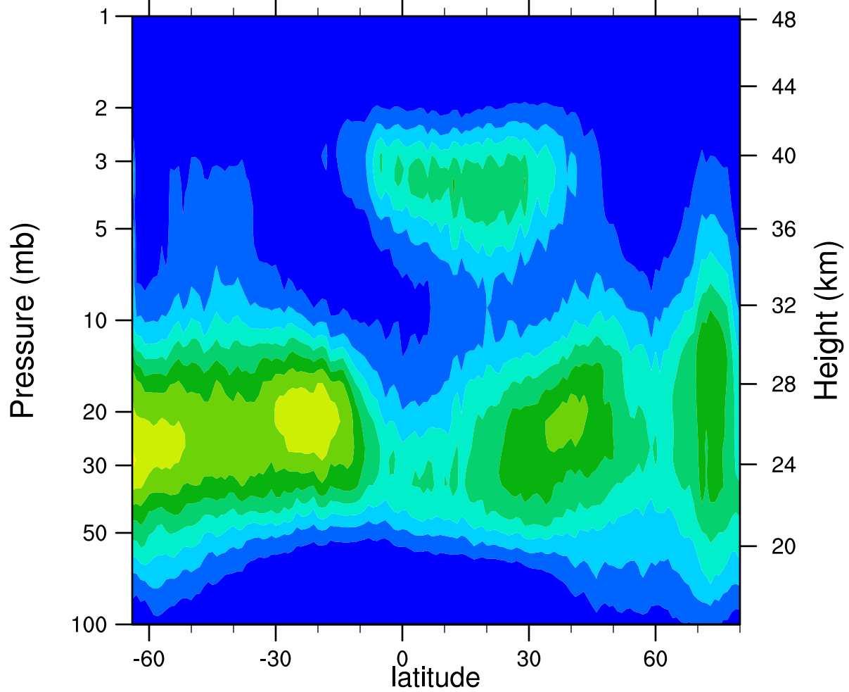
HIRDLSv6 2006d309 ClONO2_Ascending (ppbv)
