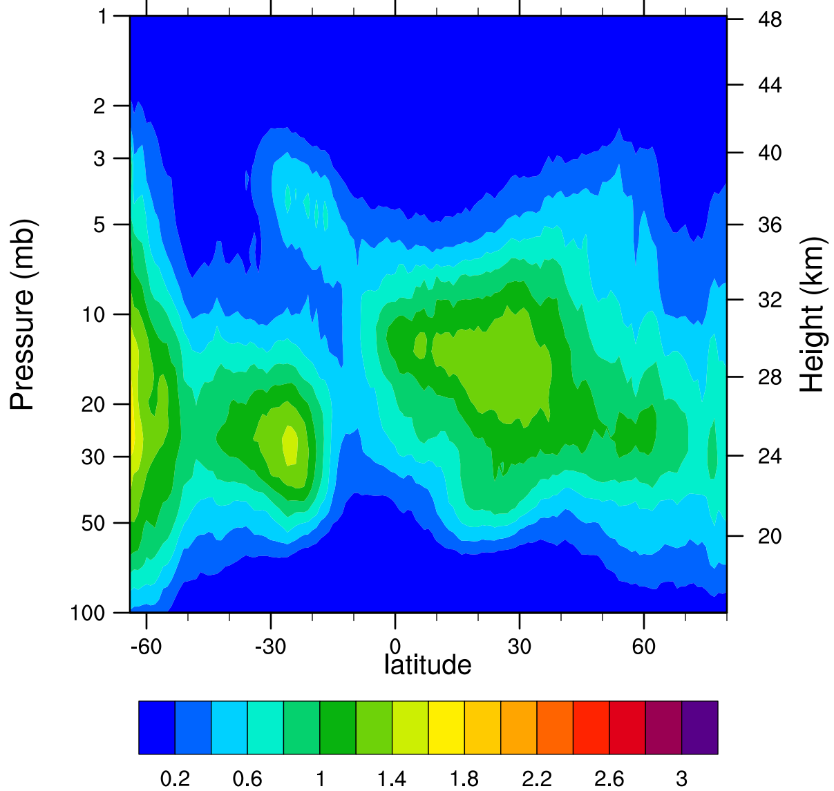
HIRDLSv6 2005d278 ClONO2_Ascending (ppbv)
