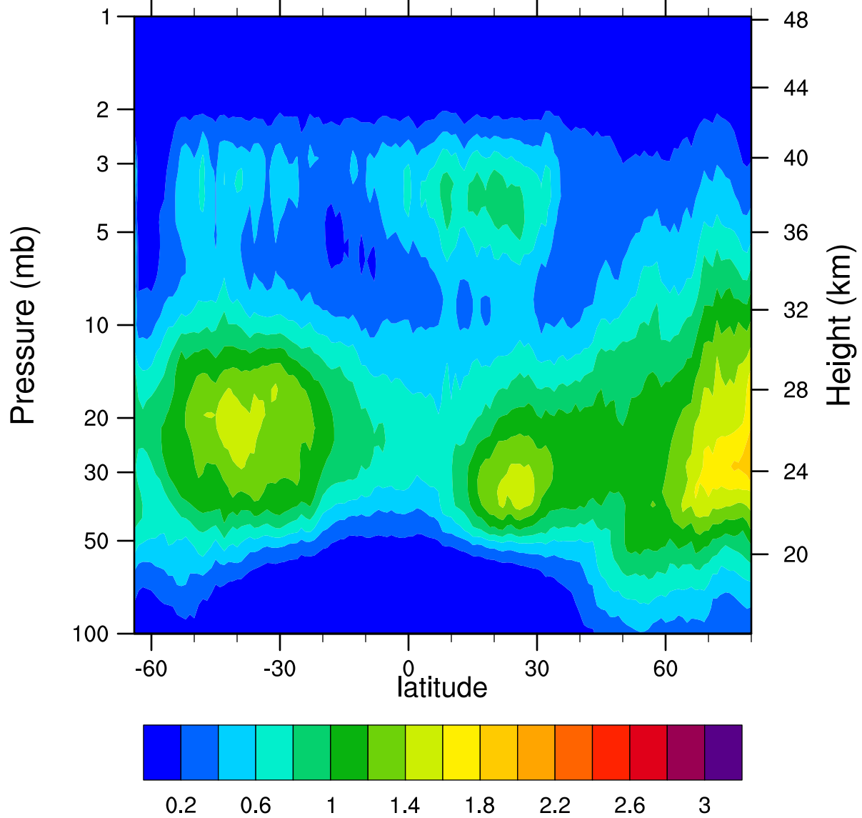
HIRDLSv6 2007d047 ClONO2_Ascending (ppbv)
