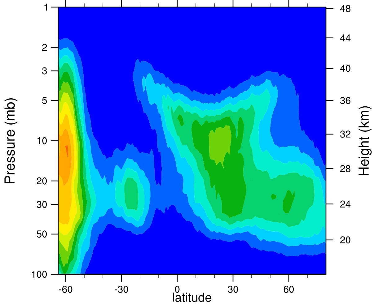
HIRDLSv6 2005d152 ClONO2_Ascending (ppbv)
