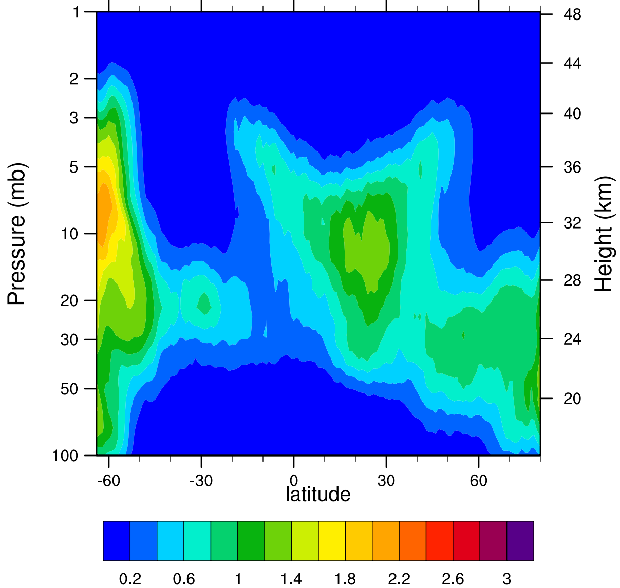
HIRDLSv6 2005d088 ClONO2_Ascending (ppbv)
