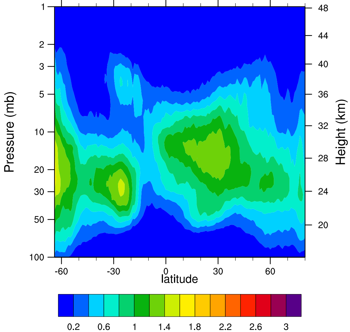
HIRDLSv6 2005d281 ClONO2_Ascending (ppbv)
