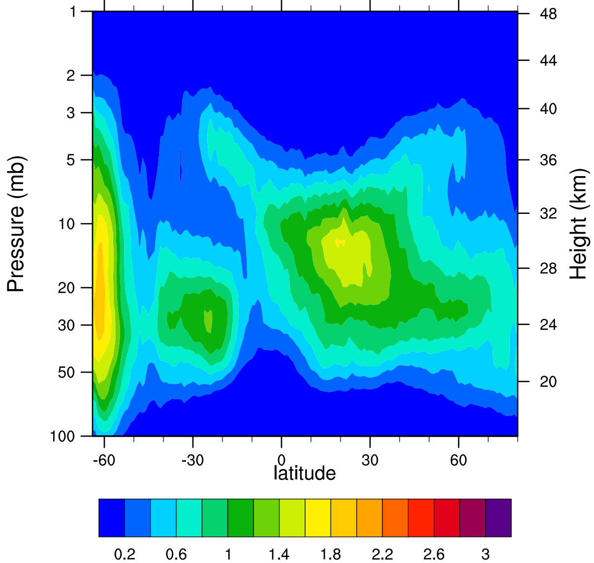
HIRDLSv6 2005d241 ClONO2_Ascending (ppbv)
