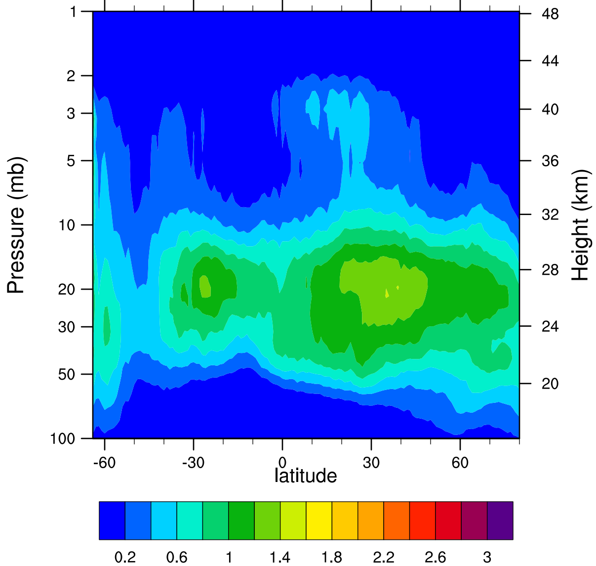
HIRDLSv6 2006d160 ClONO2_Ascending (ppbv)
