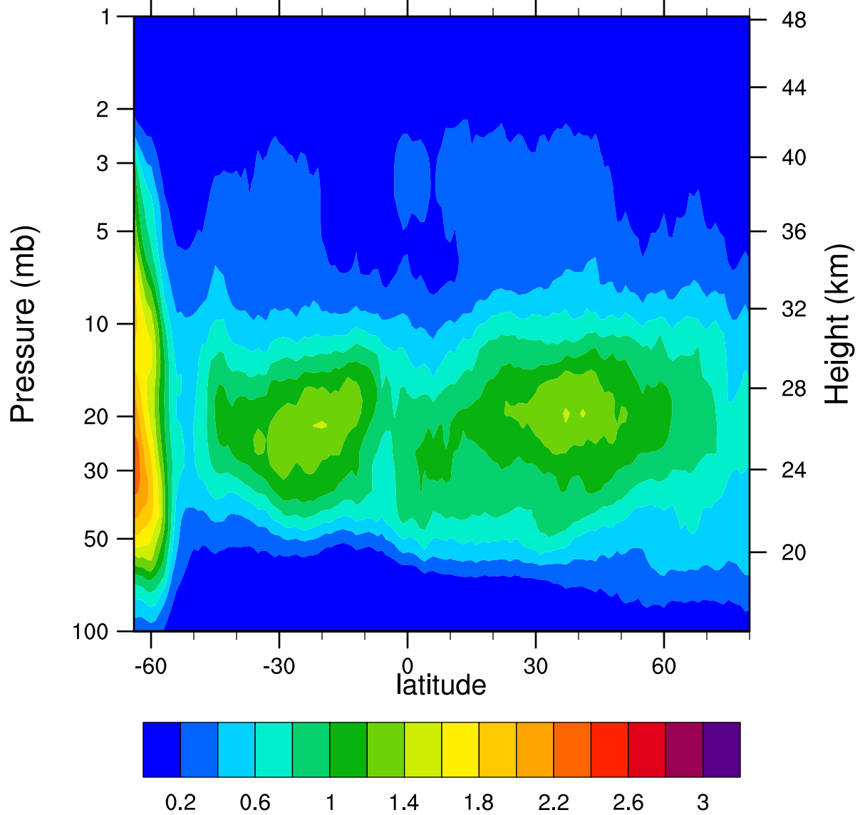
HIRDLSv6 2006d253 ClONO2_Ascending (ppbv)
