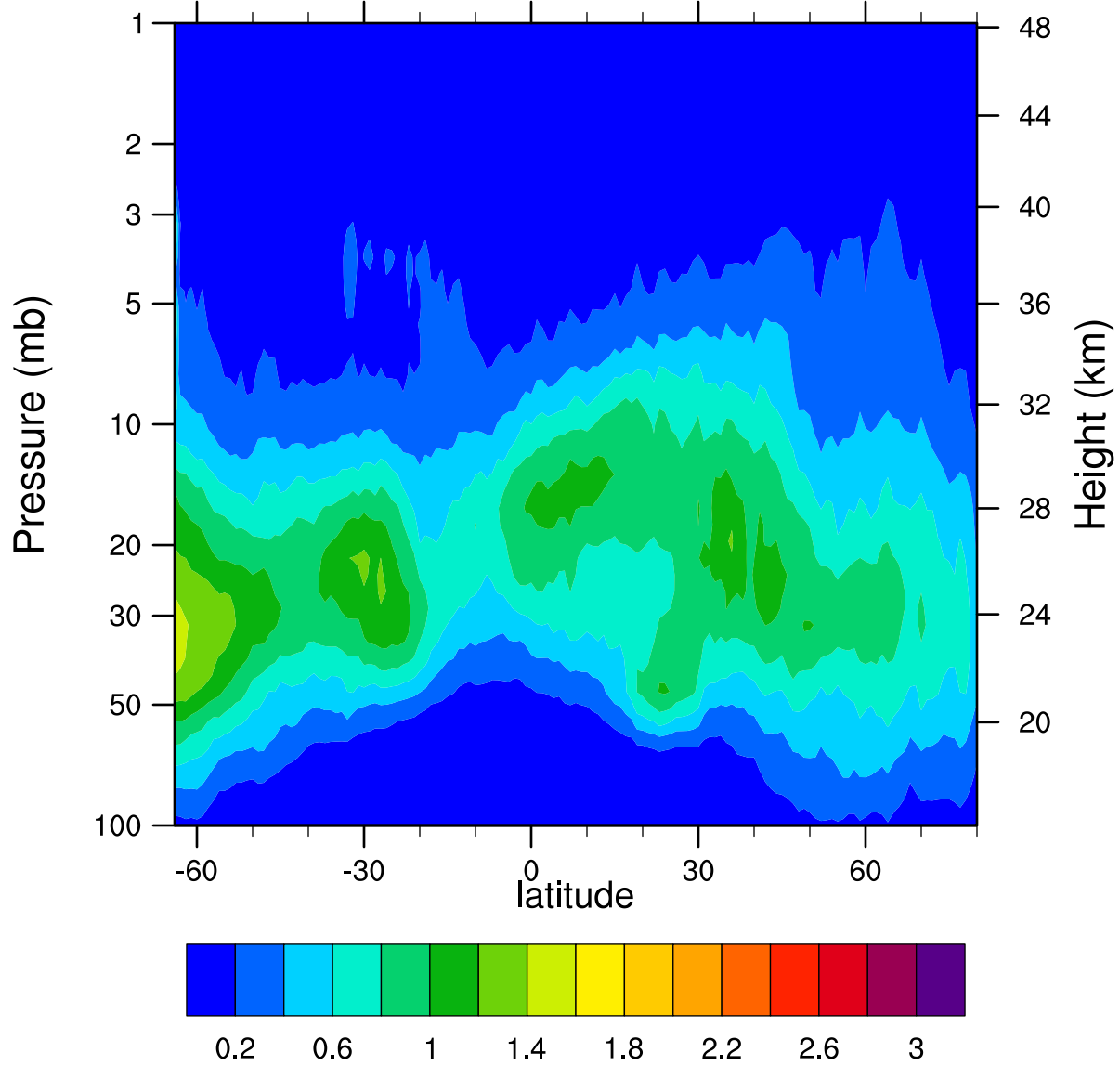
HIRDLSv6 2005d328 ClONO2_Ascending (ppbv)
