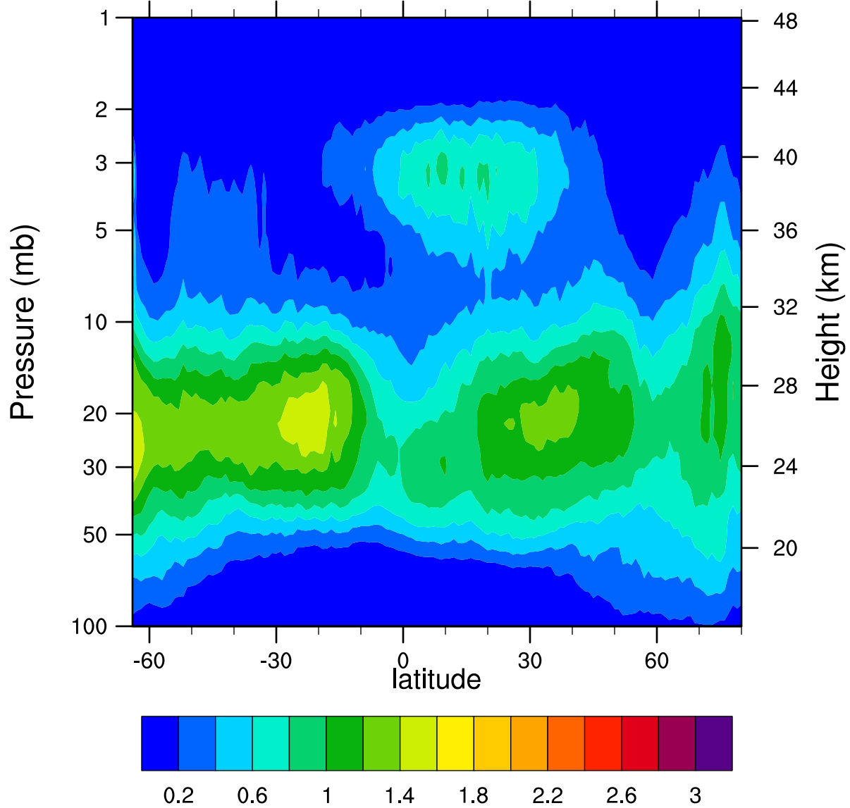
HIRDLSv6 2006d300 ClONO2_Ascending (ppbv)
