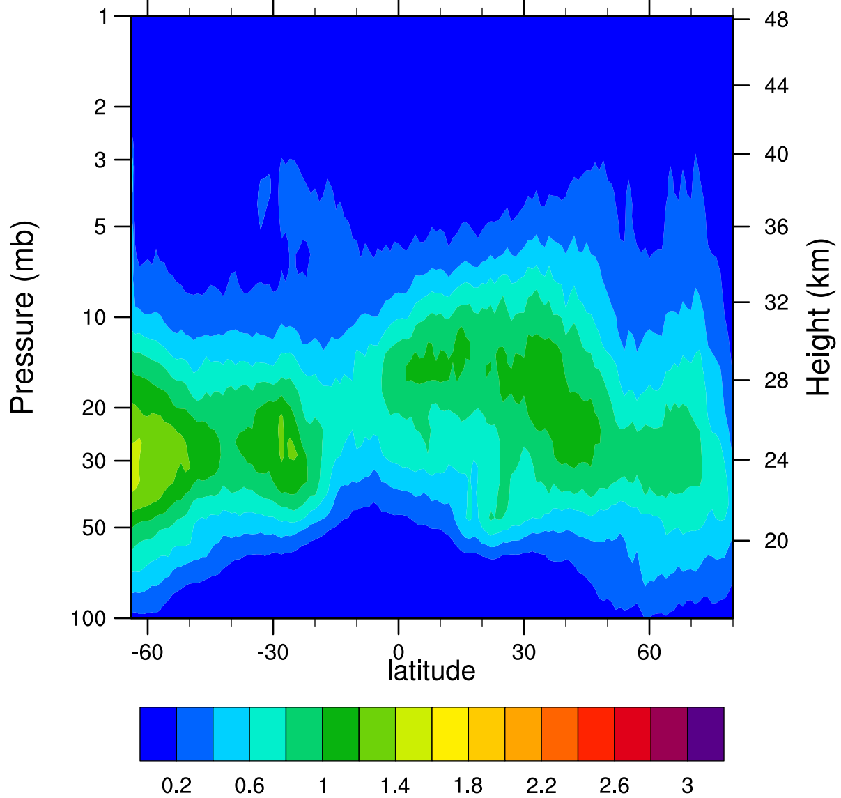
HIRDLSv6 2005d317 ClONO2_Ascending (ppbv)
