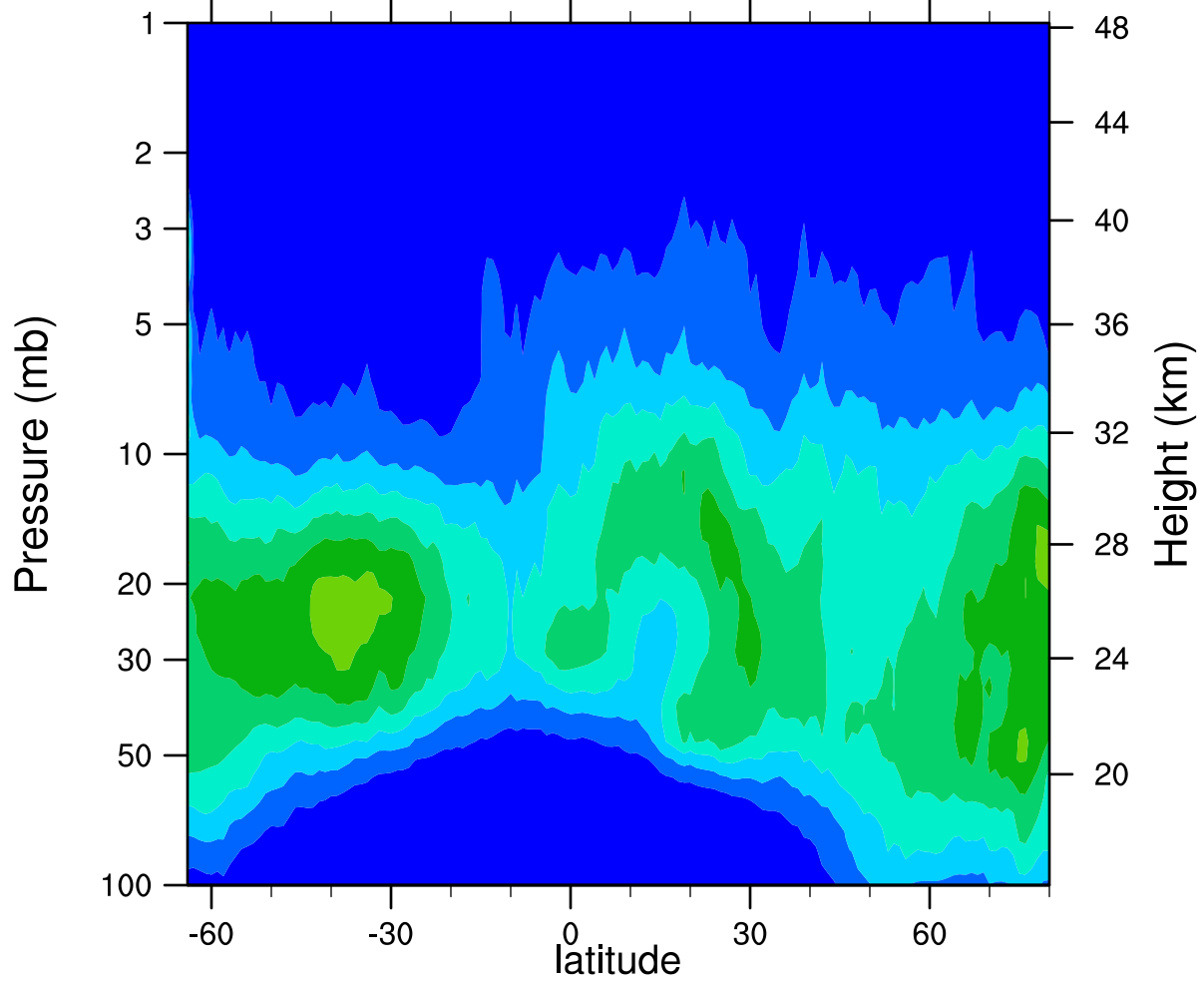
HIRDLSv6 2006d022 ClONO2_Ascending (ppbv)
