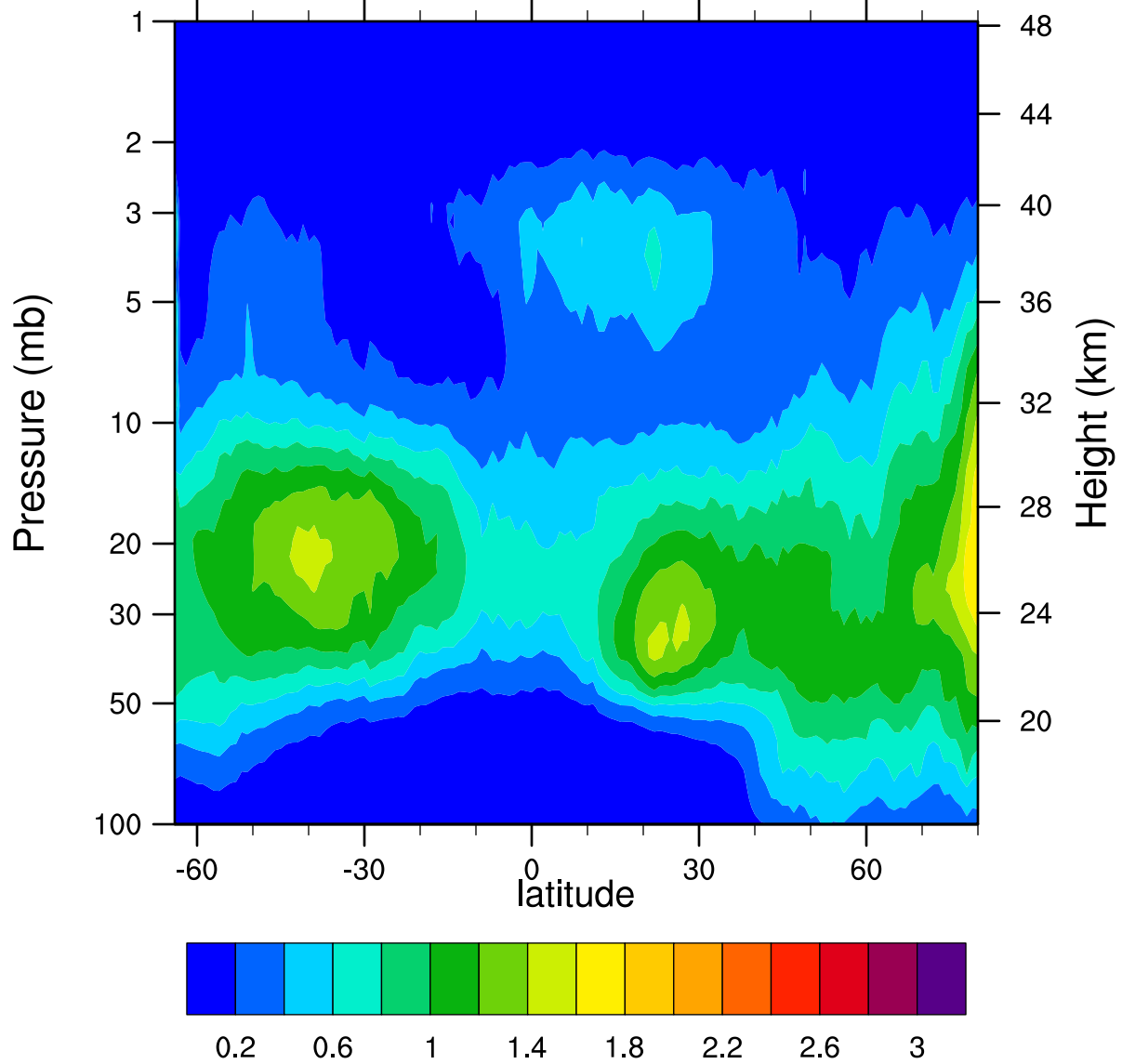
HIRDLSv6 2007d037 ClONO2_Ascending (ppbv)
