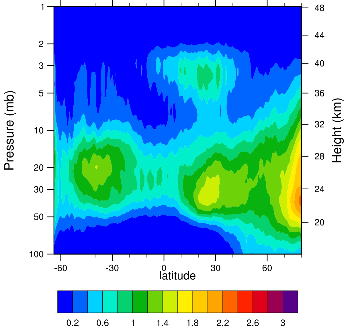
HIRDLSv6 2007d074 ClONO2_Ascending (ppbv)
