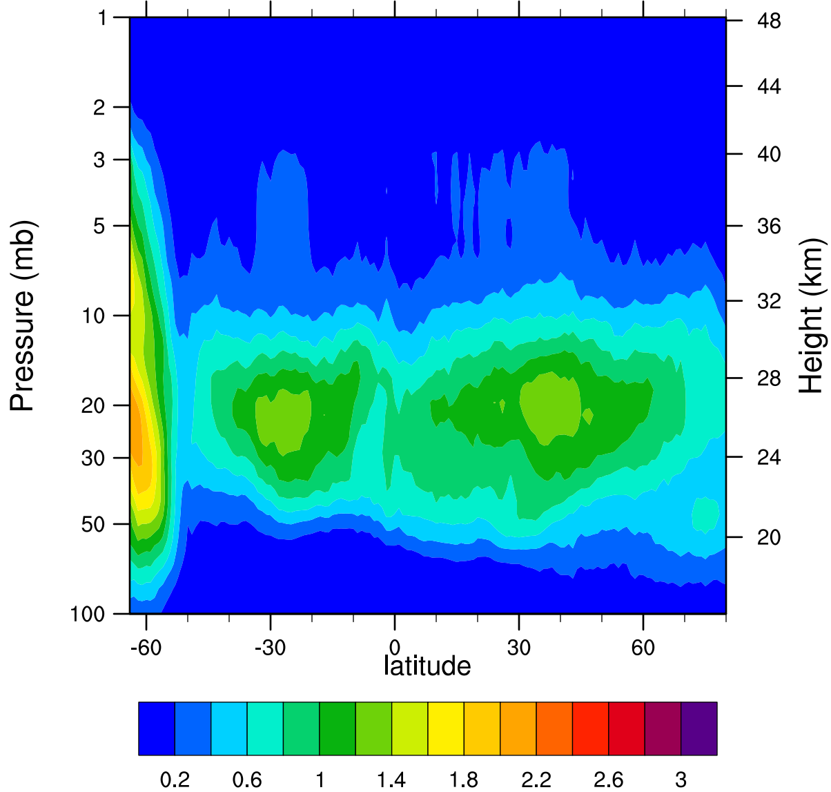
HIRDLSv6 2006d235 ClONO2_Ascending (ppbv)
