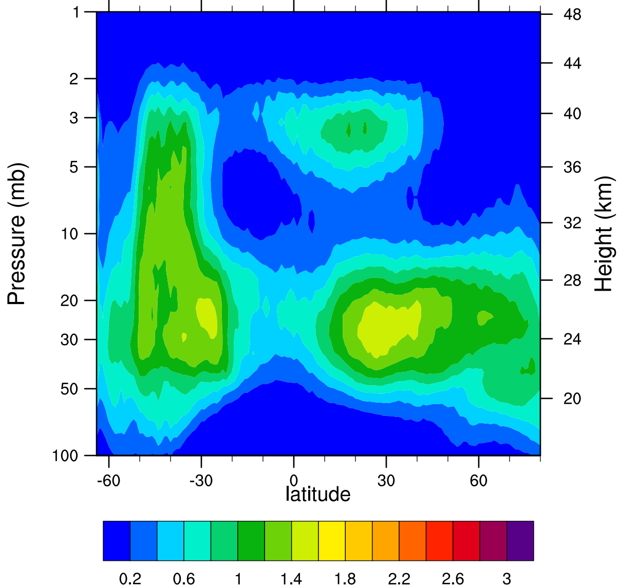
HIRDLSv6 2007d157 ClONO2_Ascending (ppbv)
