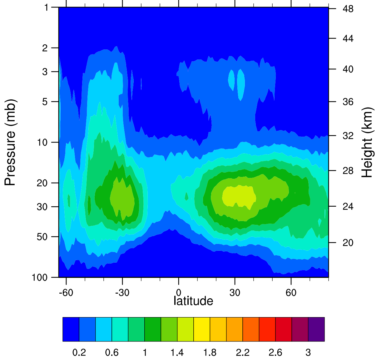
HIRDLSv6 2007d174 ClONO2_Ascending (ppbv)
