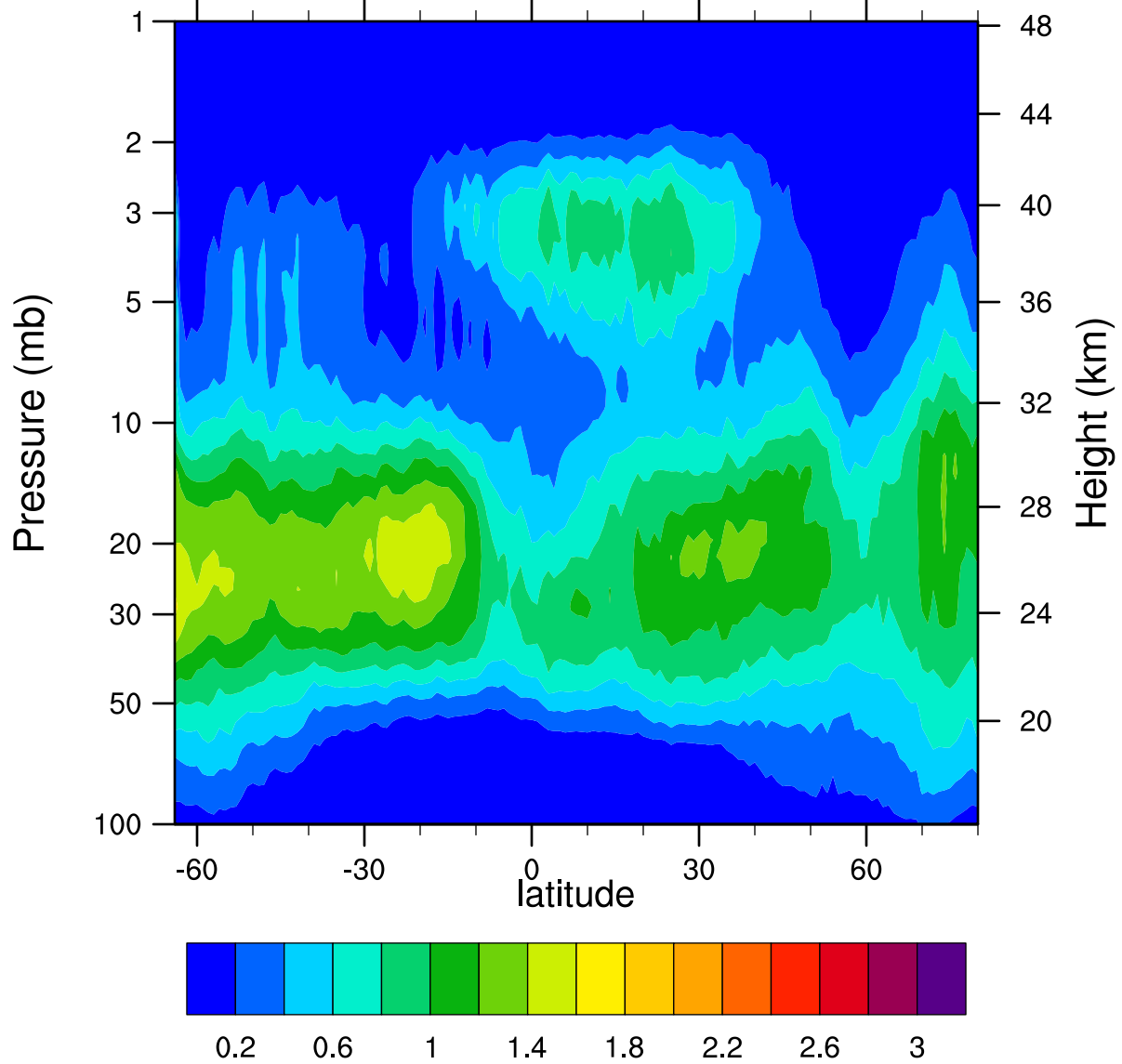
HIRDLSv6 2006d304 ClONO2_Ascending (ppbv)
