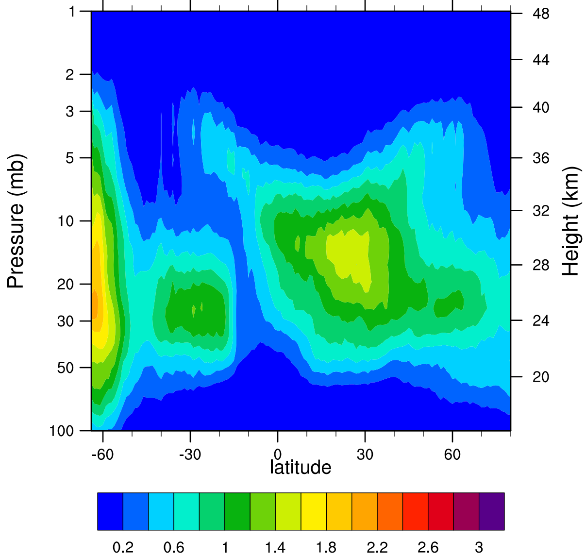
HIRDLSv6 2005d252 ClONO2_Ascending (ppbv)
