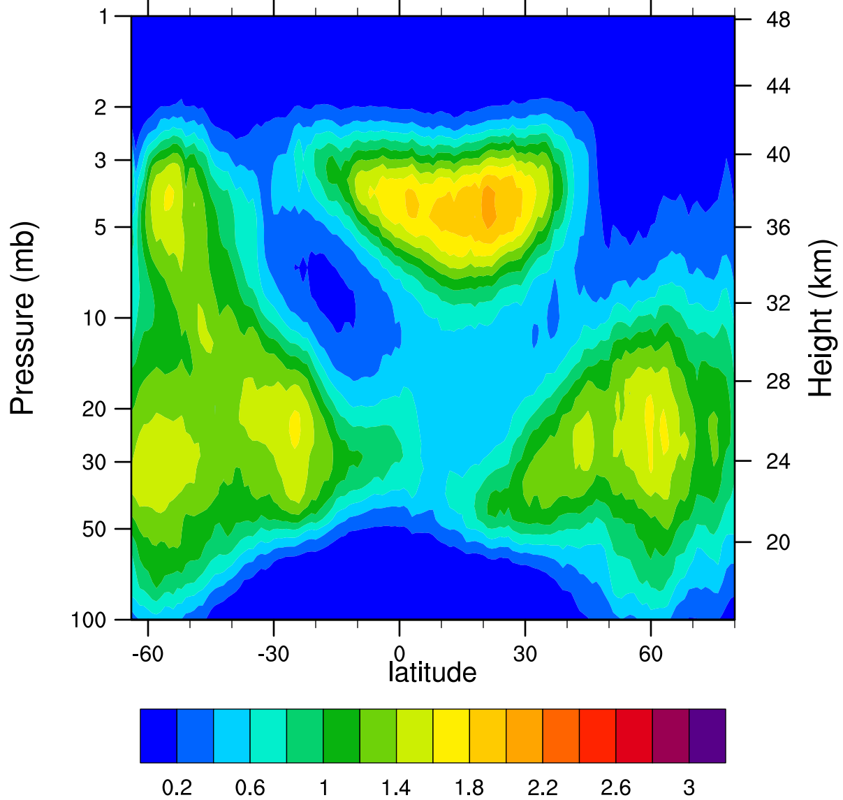
HIRDLSv6 2007d332 ClONO2_Ascending (ppbv)
