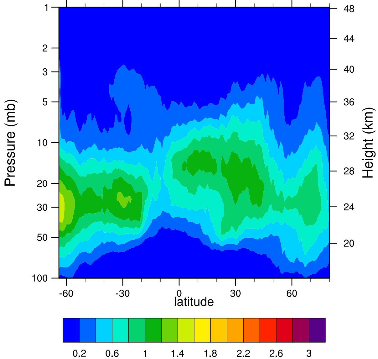
HIRDLSv6 2005d310 ClONO2_Ascending (ppbv)
