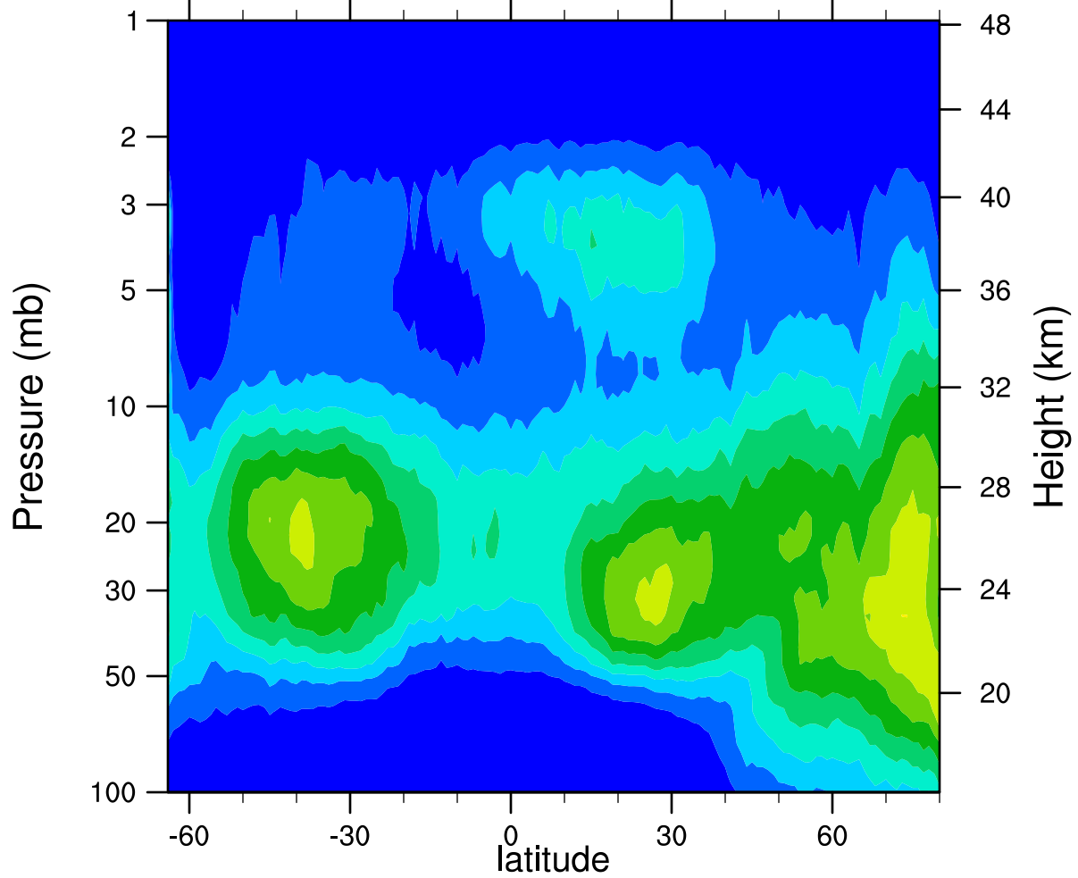
HIRDLSv6 2007d057 ClONO2_Ascending (ppbv)
