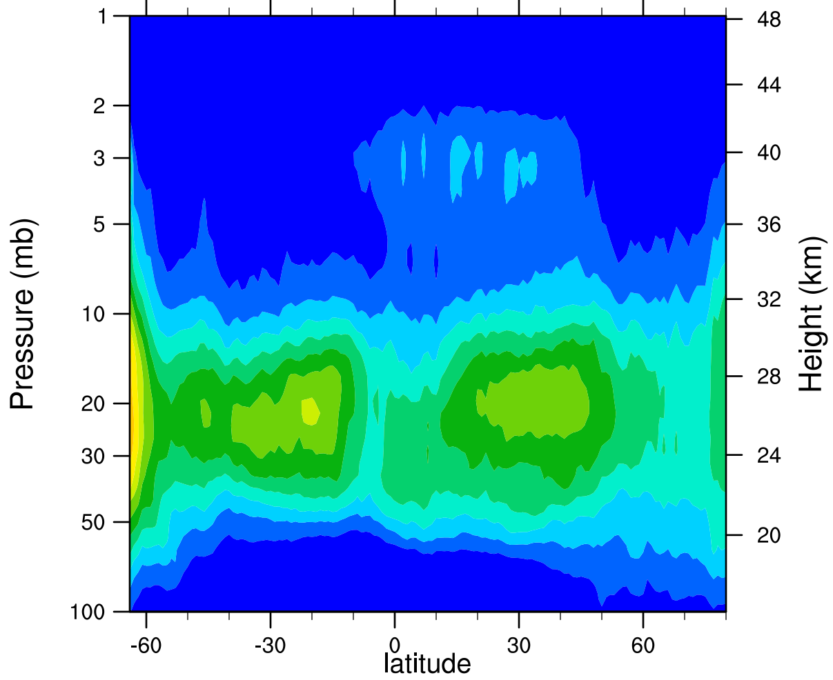
HIRDLSv6 2006d280 ClONO2_Ascending (ppbv)
