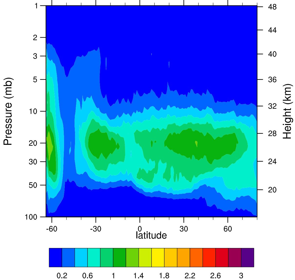
HIRDLSv6 2006d185 ClONO2_Ascending (ppbv)
