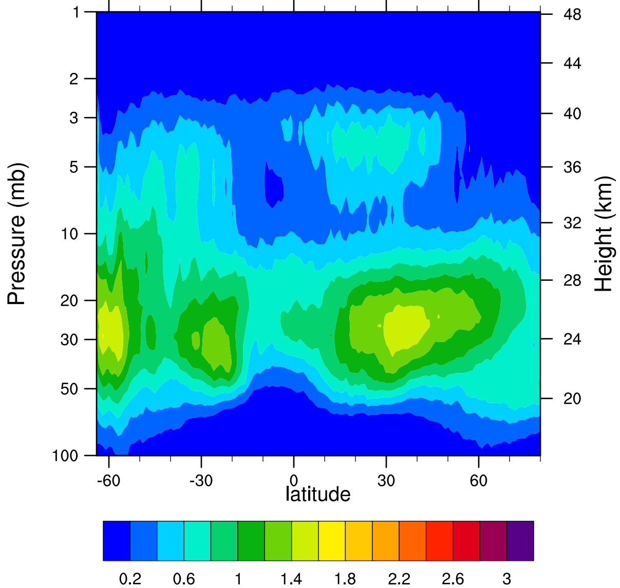
HIRDLSv6 2007d207 ClONO2_Ascending (ppbv)
