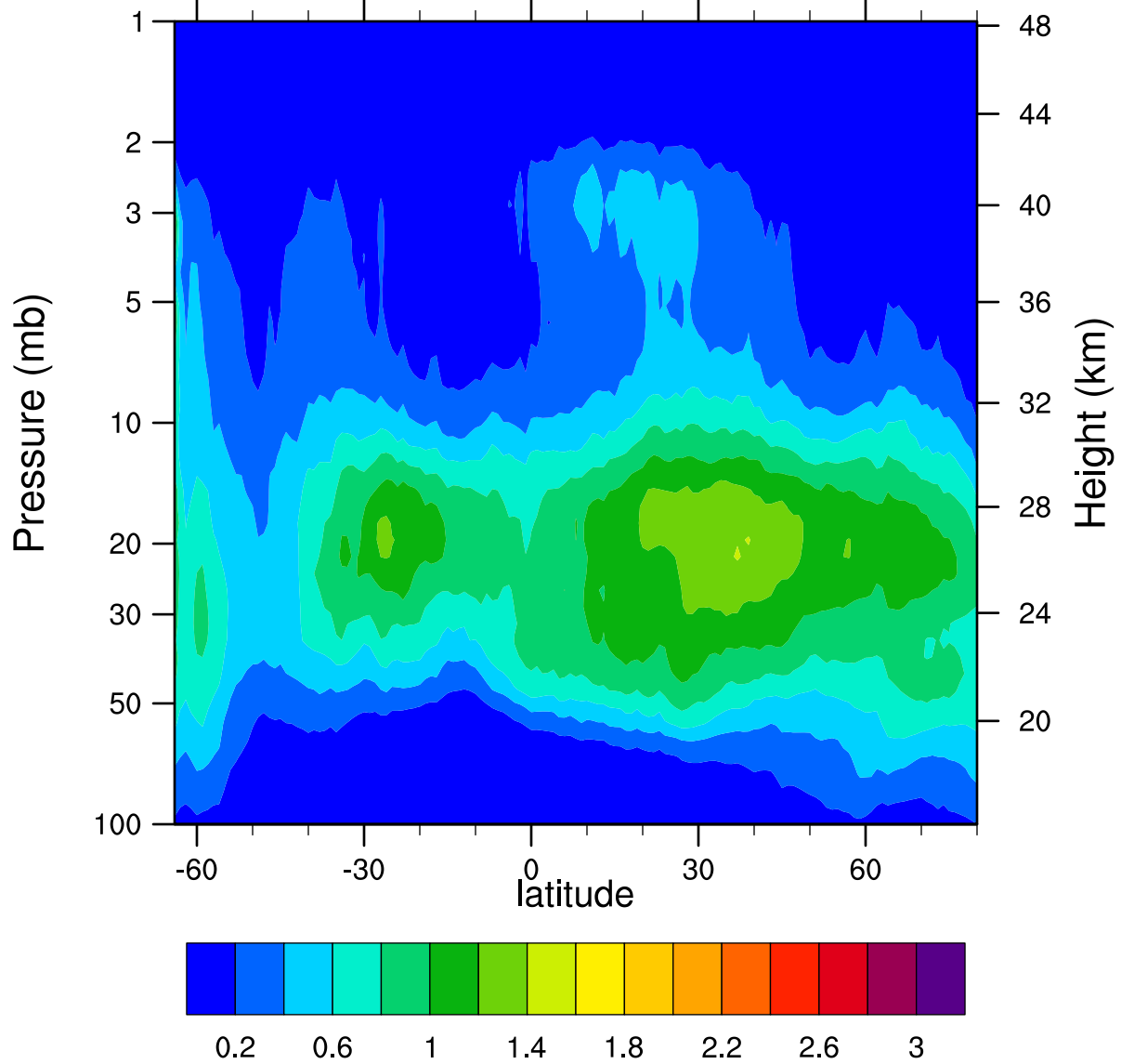
HIRDLSv6 2006d159 ClONO2_Ascending (ppbv)
