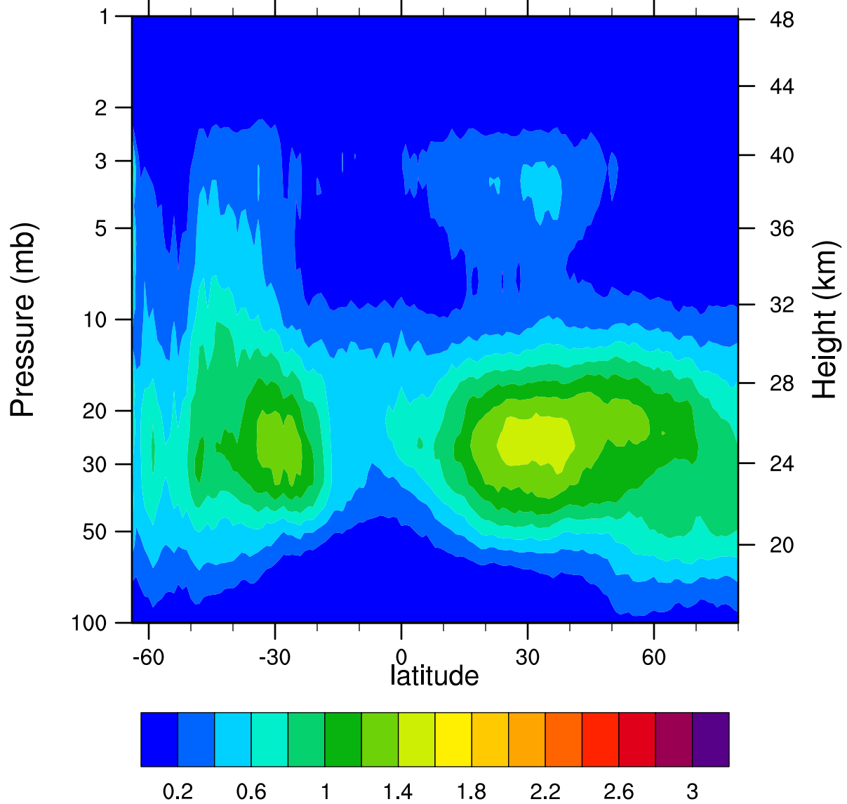
HIRDLSv6 2007d172 ClONO2_Ascending (ppbv)
