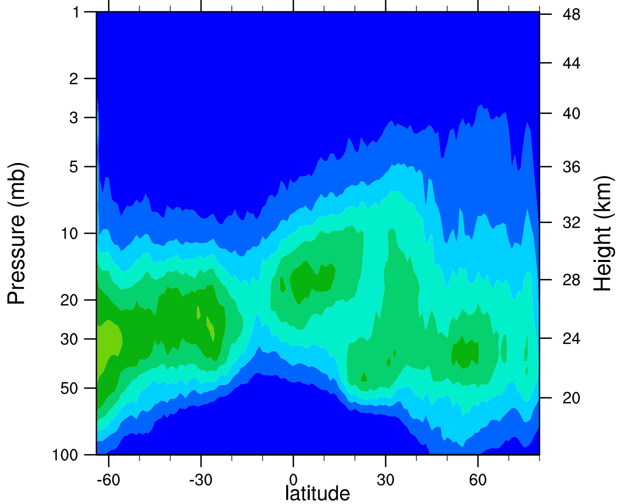
HIRDLSv6 2005d344 ClONO2_Ascending (ppbv)
