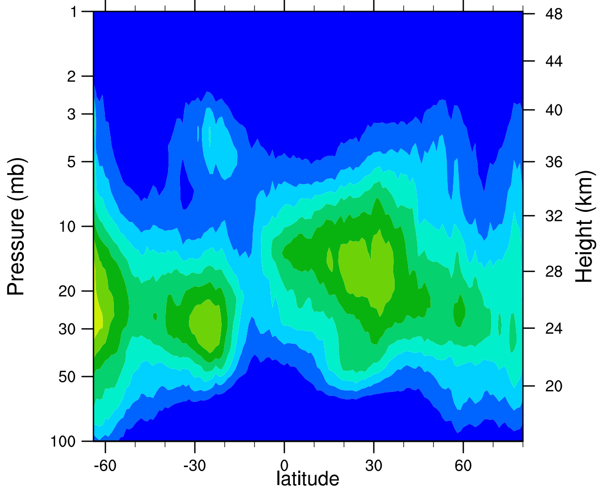
HIRDLSv6 2005d288 ClONO2_Ascending (ppbv)
