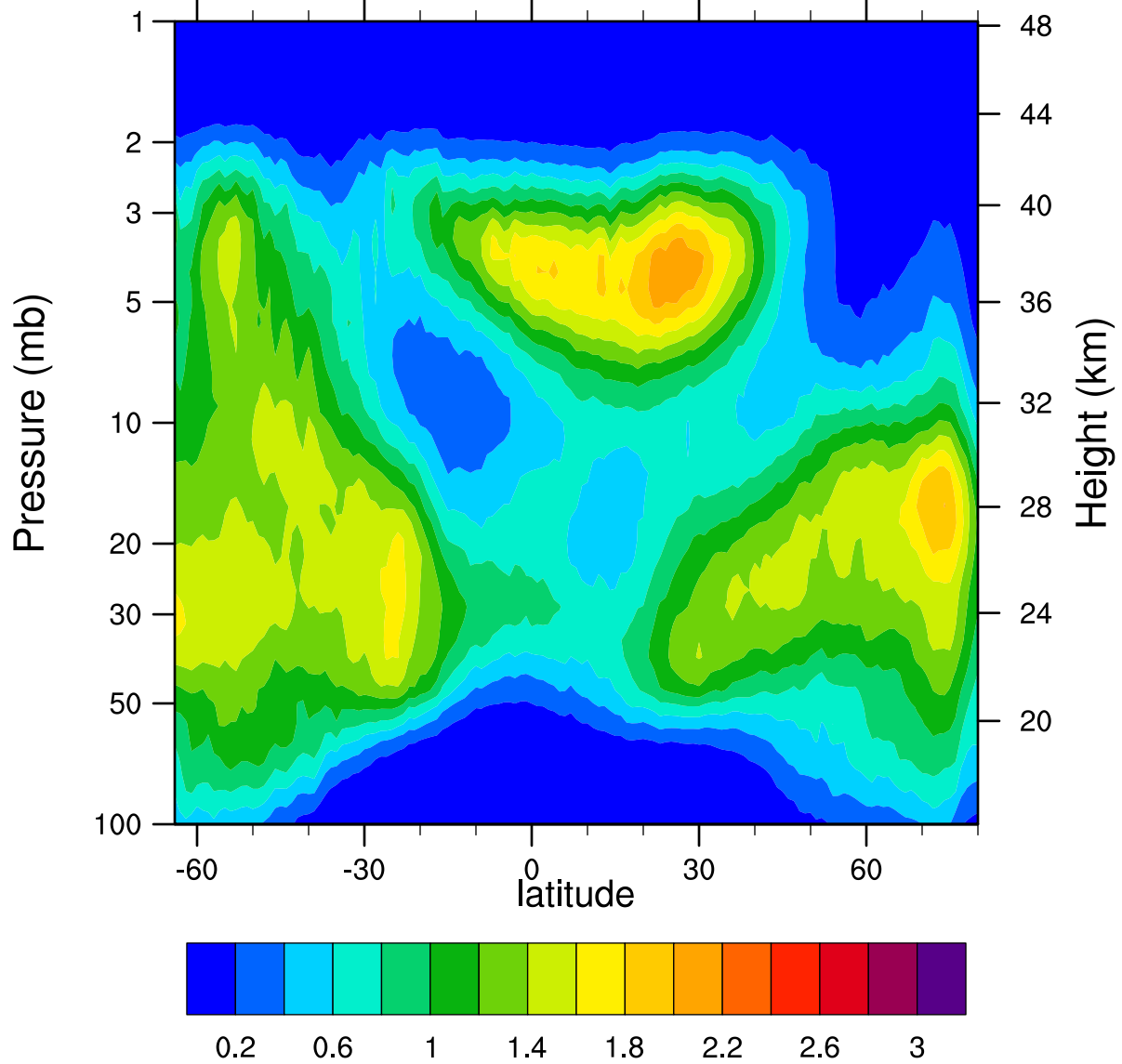
HIRDLSv6 2007d301 ClONO2_Ascending (ppbv)
