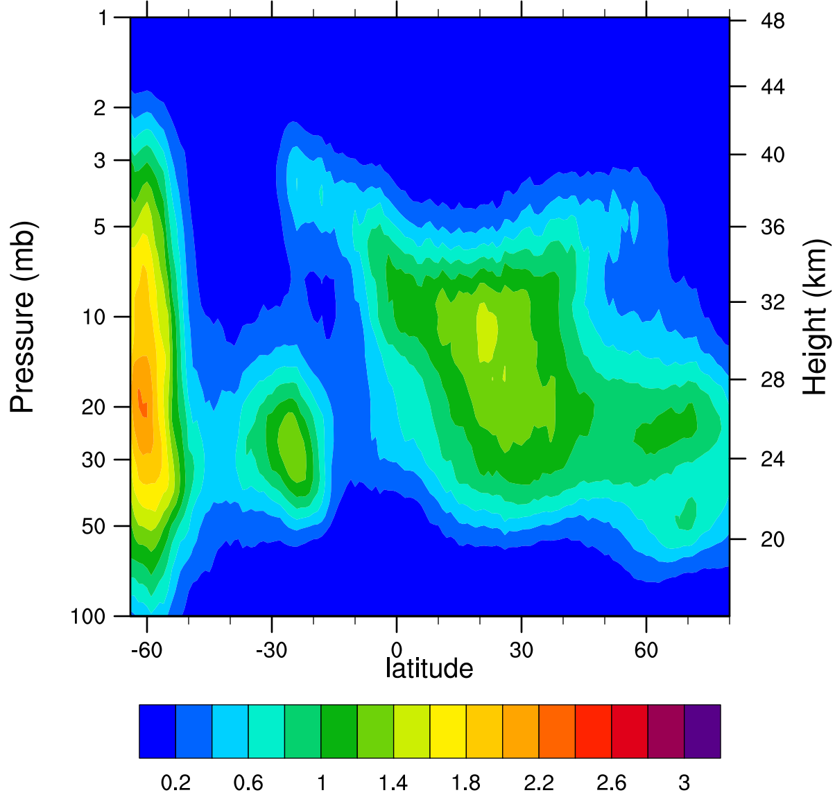
HIRDLSv6 2005d184 ClONO2_Ascending (ppbv)
