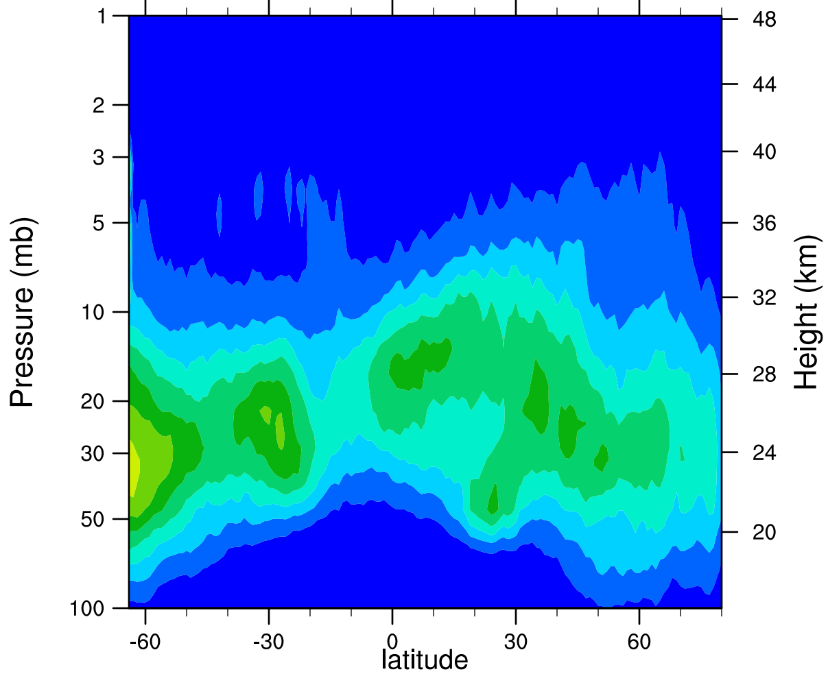
HIRDLSv6 2005d329 ClONO2_Ascending (ppbv)
