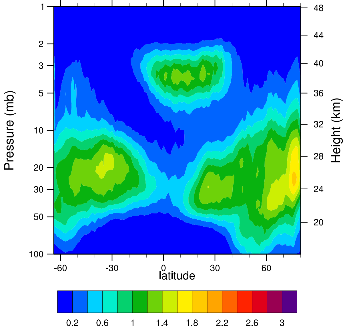
HIRDLSv6 2007d016 ClONO2_Ascending (ppbv)
