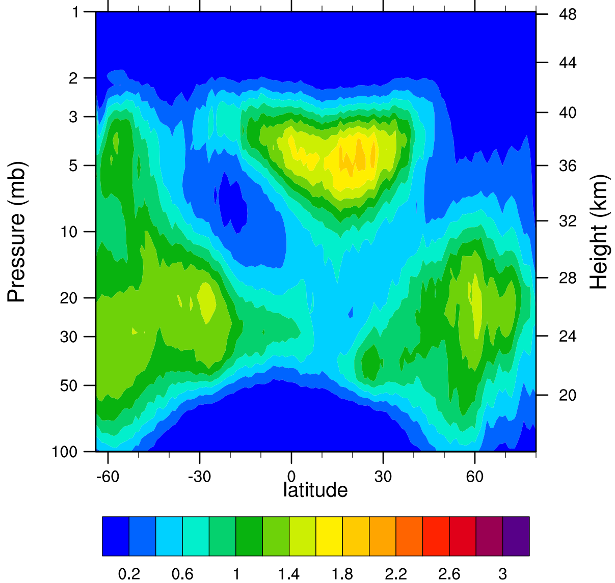
HIRDLSv6 2007d359 ClONO2_Ascending (ppbv)
