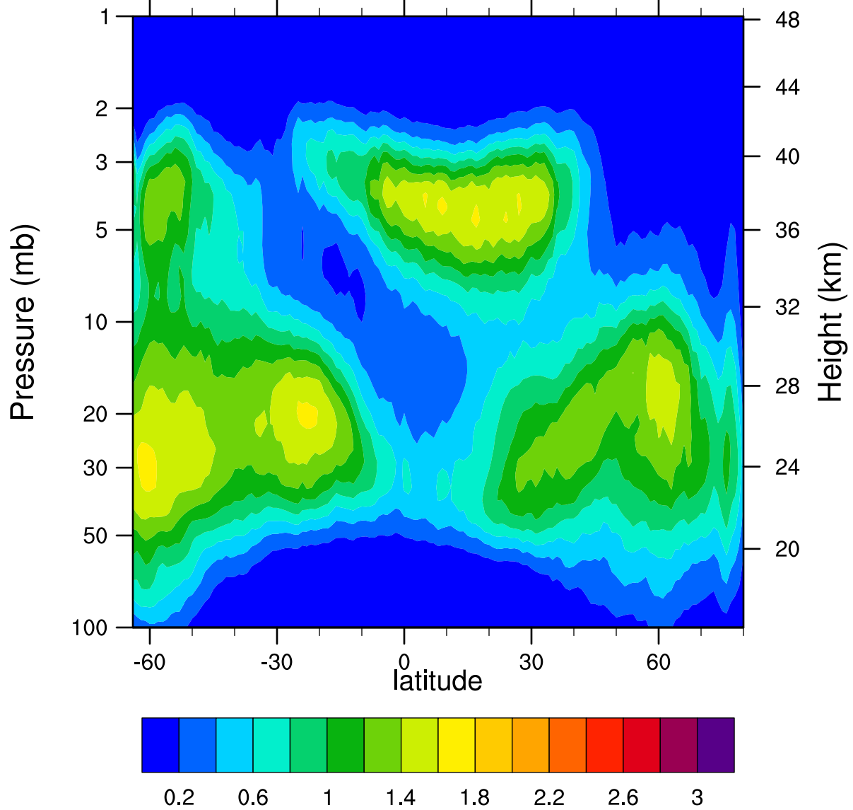
HIRDLSv6 2006d336 ClONO2_Ascending (ppbv)
