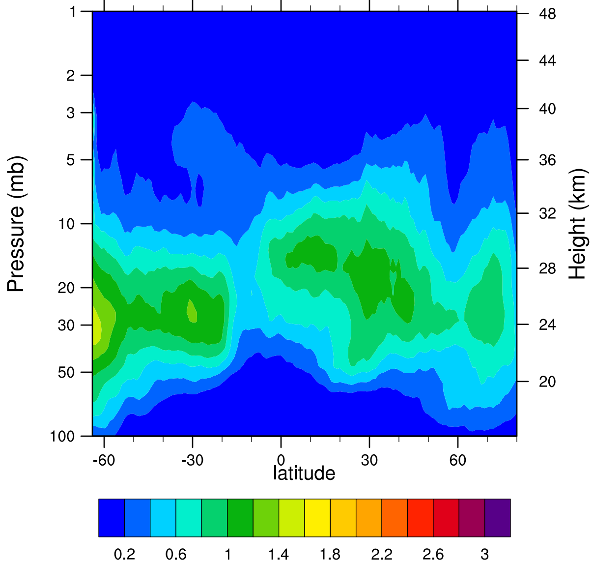
HIRDLSv6 2005d306 ClONO2_Ascending (ppbv)
