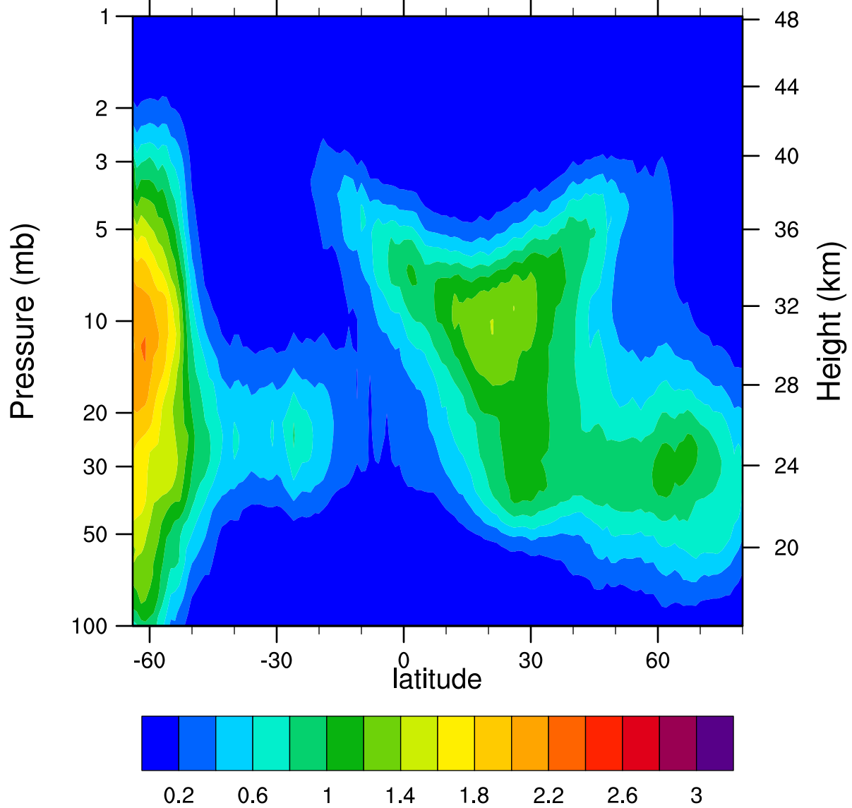
HIRDLSv6 2005d122 ClONO2_Ascending (ppbv)
