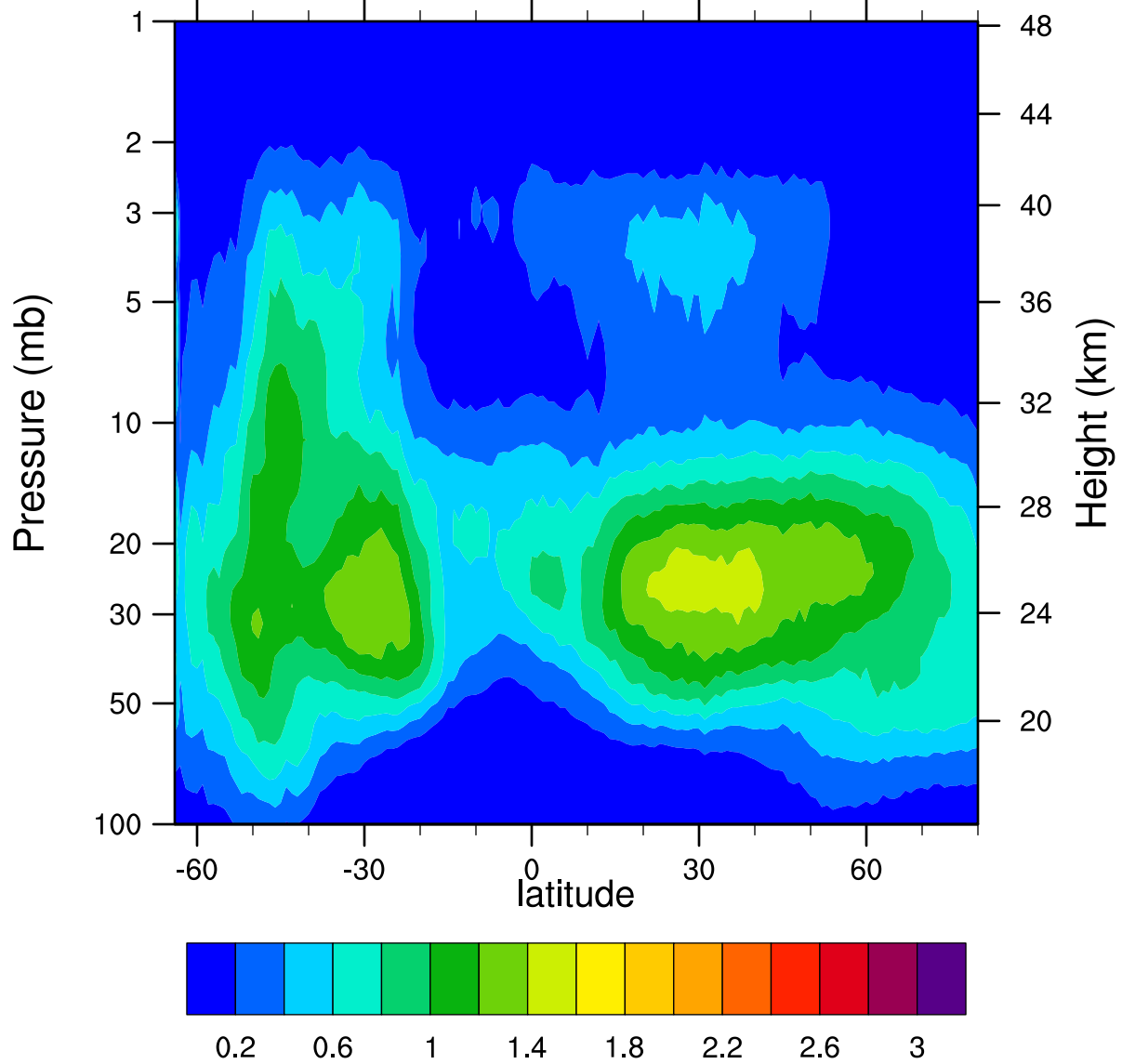
HIRDLSv6 2007d183 ClONO2_Ascending (ppbv)
