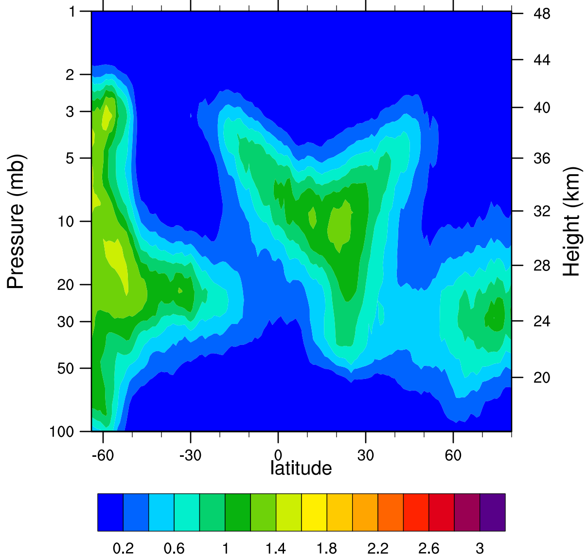
HIRDLSv6 2005d046 ClONO2_Ascending (ppbv)
