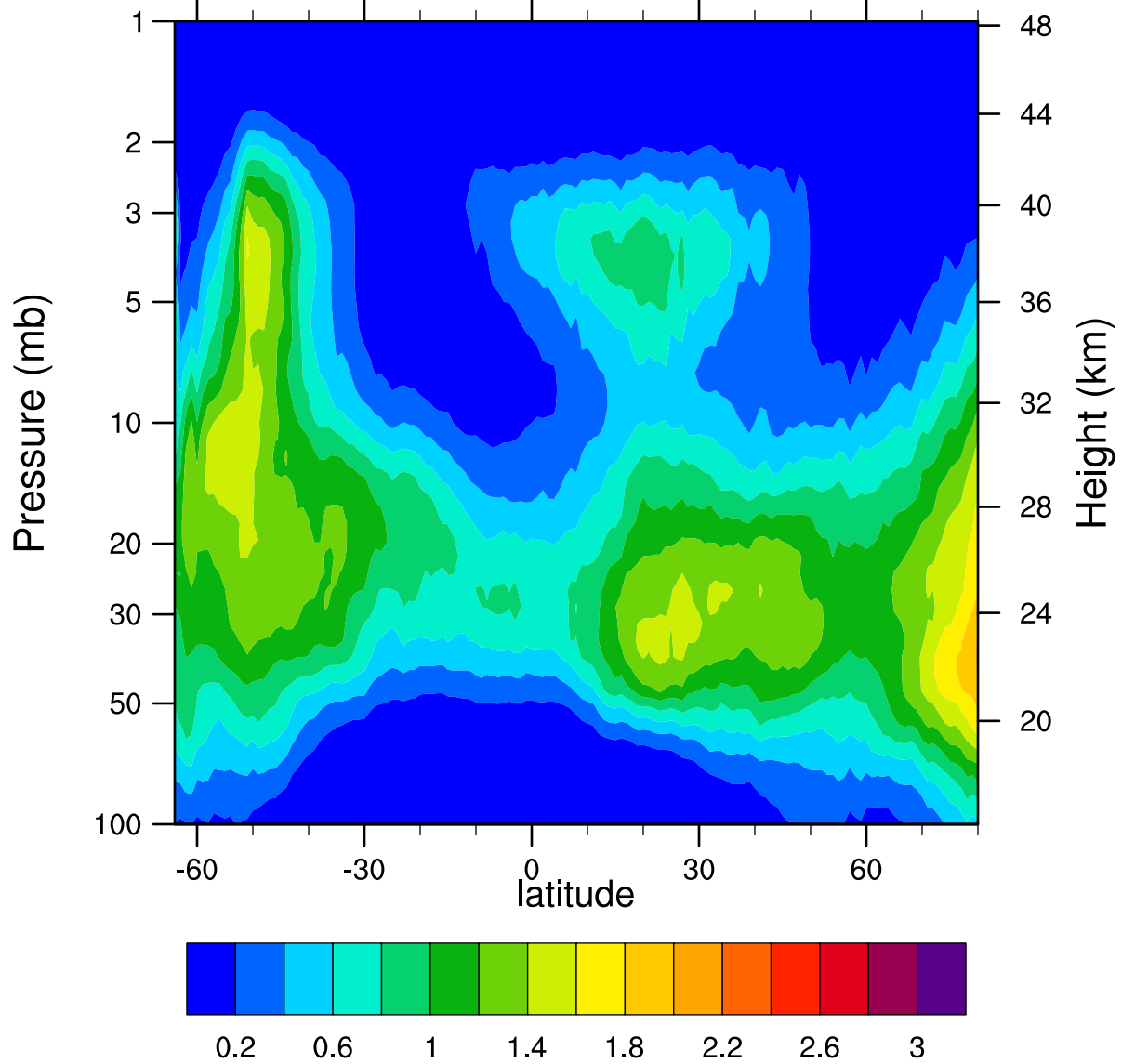
HIRDLSv6 2007d094 ClONO2_Ascending (ppbv)
