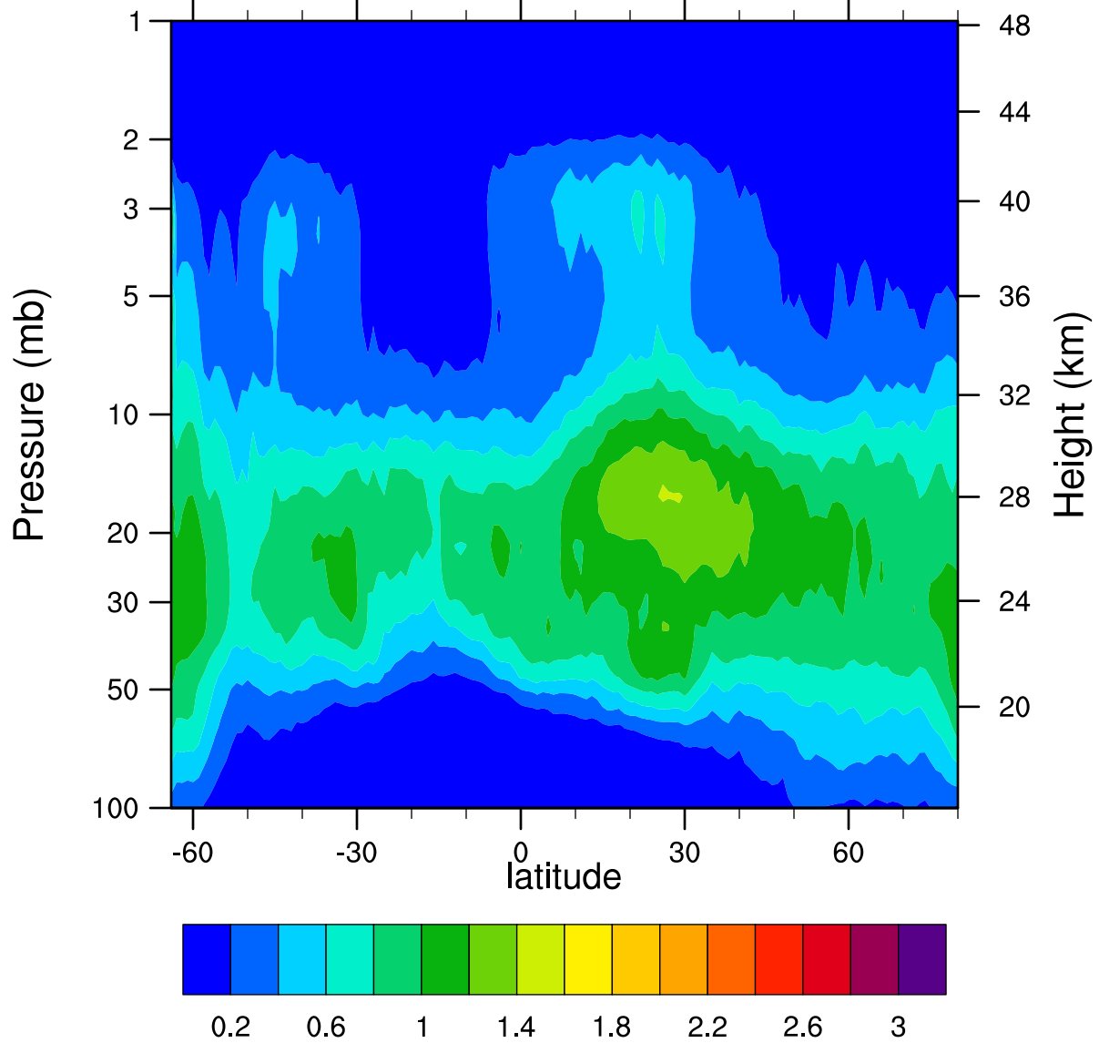
HIRDLSv6 2006d119 ClONO2_Ascending (ppbv)
