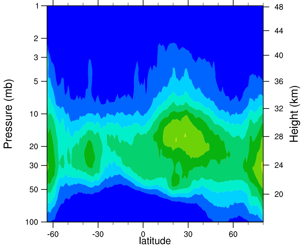
HIRDLSv6 2006d110 ClONO2_Ascending (ppbv)
