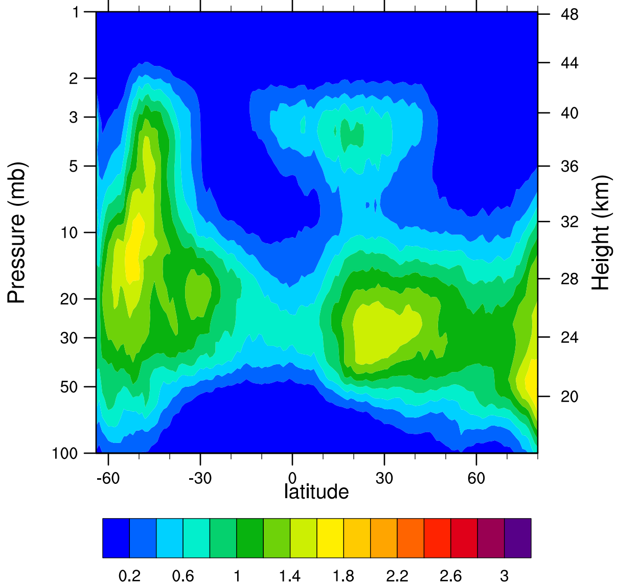
HIRDLSv6 2007d110 ClONO2_Ascending (ppbv)
