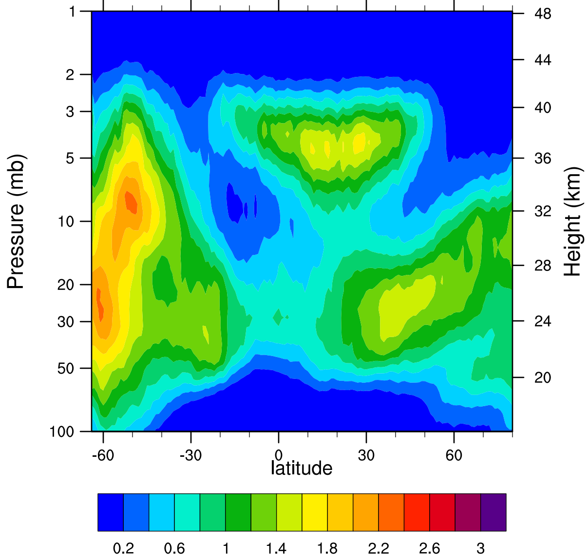
HIRDLSv6 2007d246 ClONO2_Ascending (ppbv)
