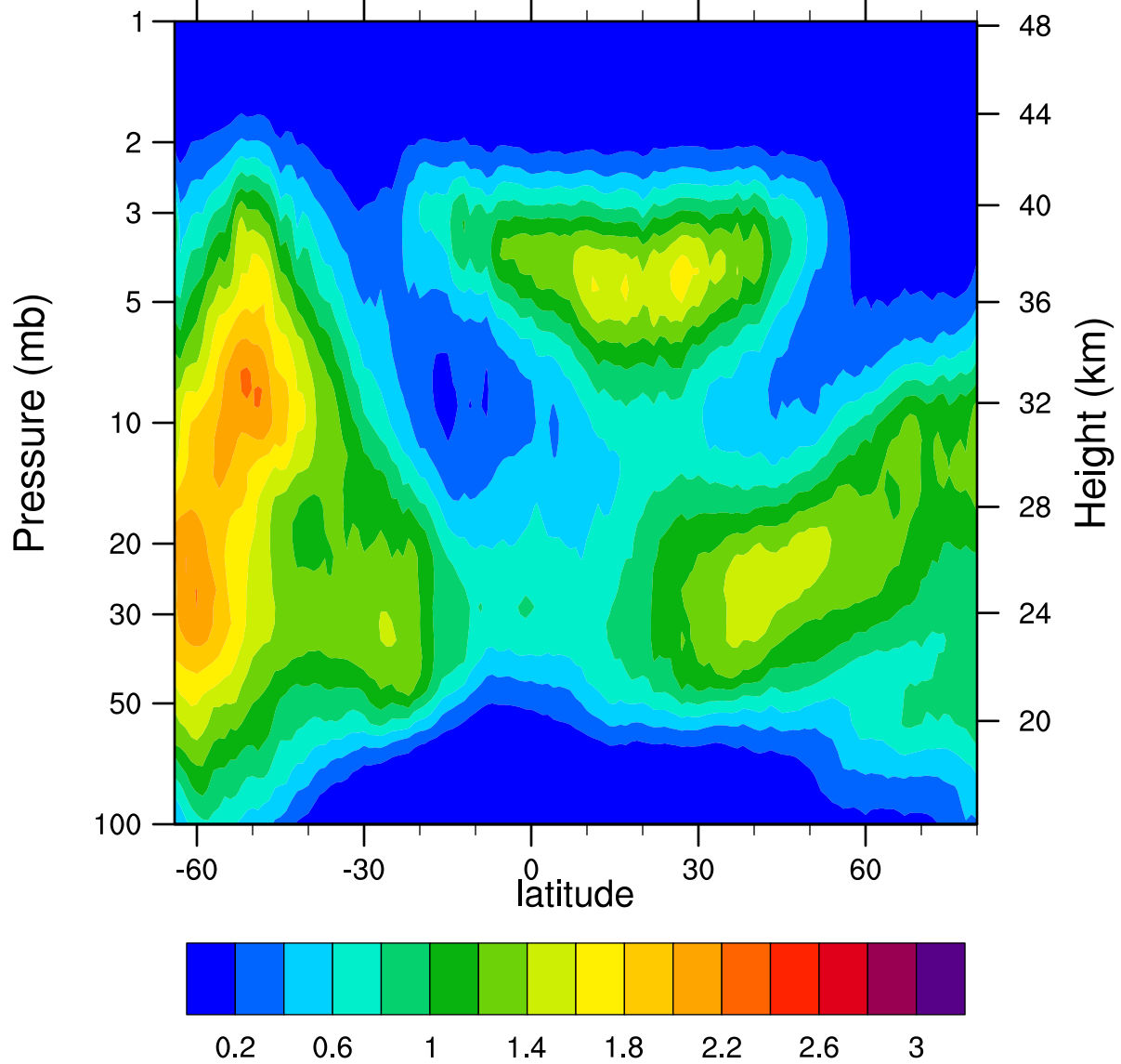
HIRDLSv6 2007d247 ClONO2_Ascending (ppbv)
