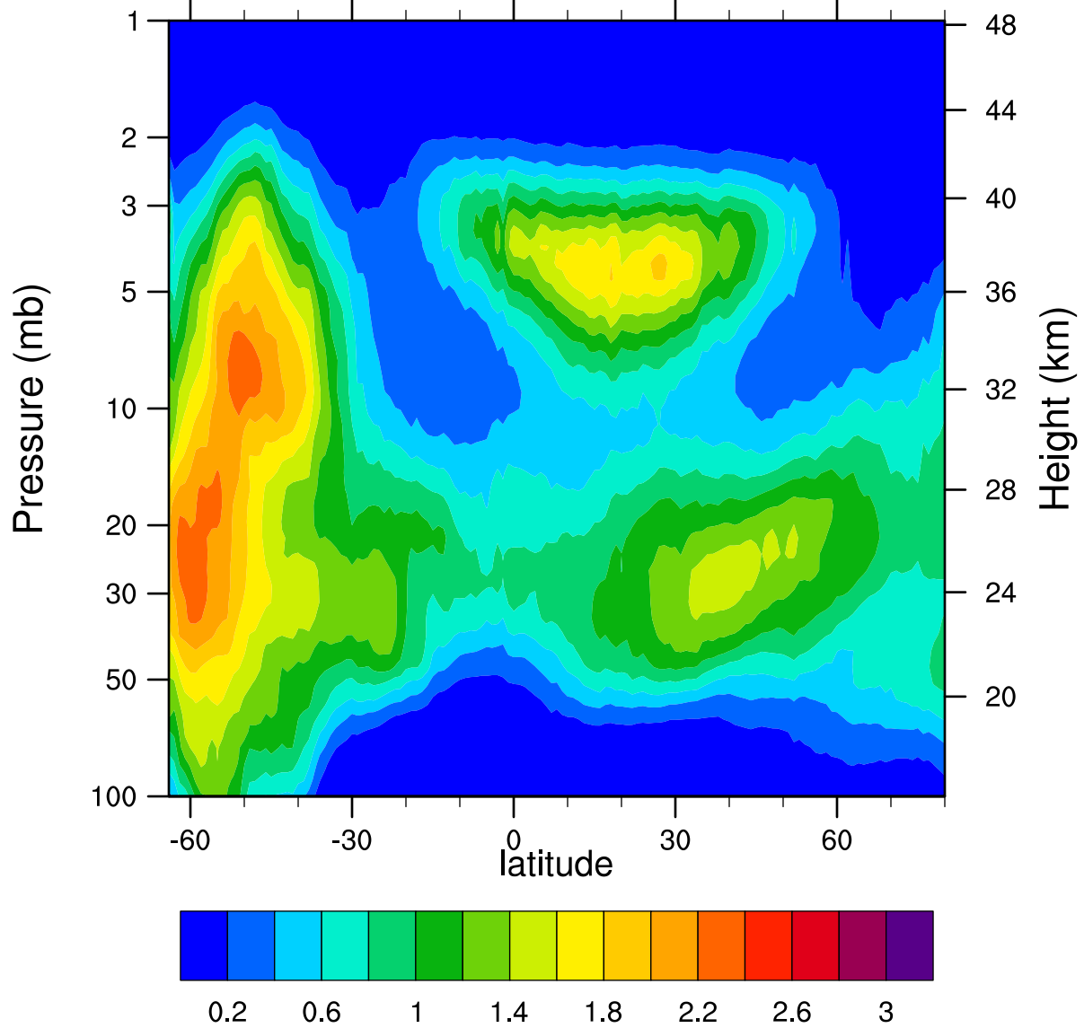
HIRDLSv6 2007d221 ClONO2_Ascending (ppbv)
