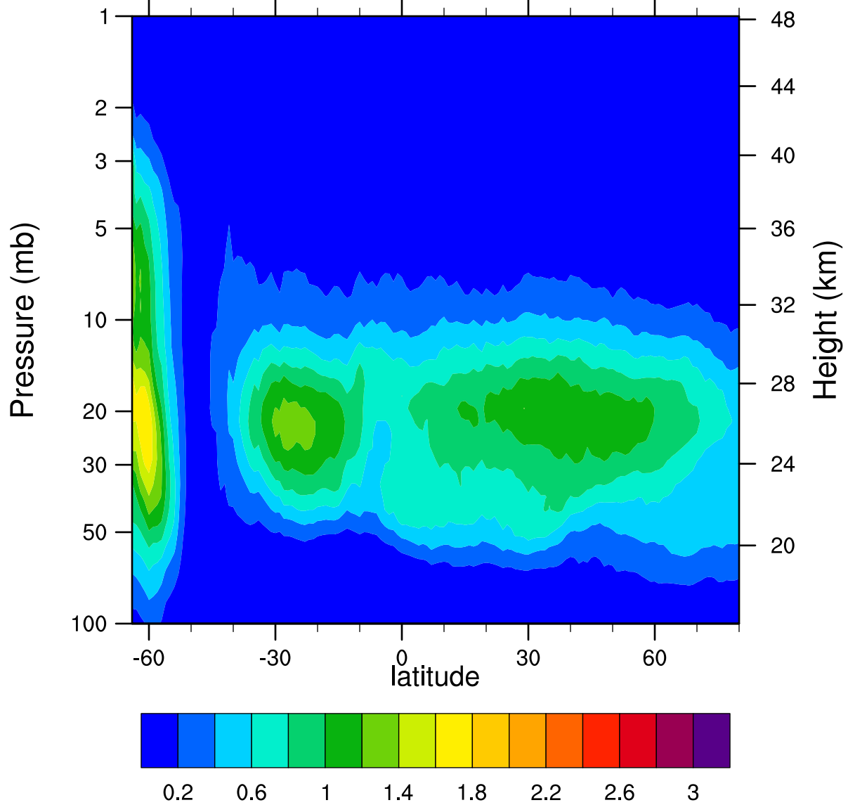
HIRDLSv6 2006d209 ClONO2_Ascending (ppbv)
