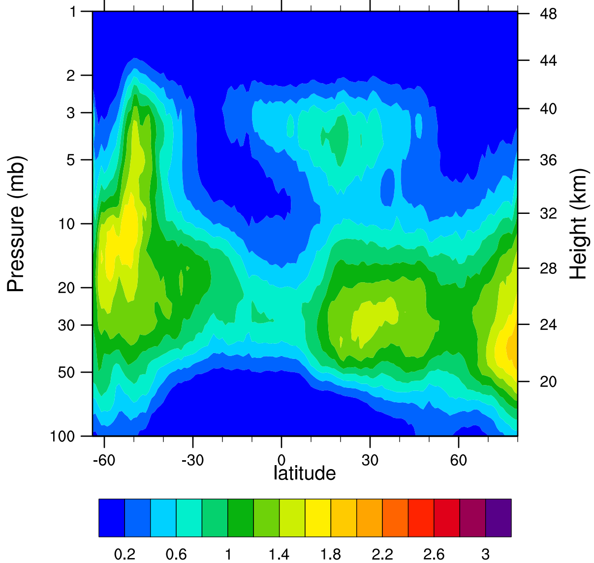
HIRDLSv6 2007d099 ClONO2_Ascending (ppbv)
