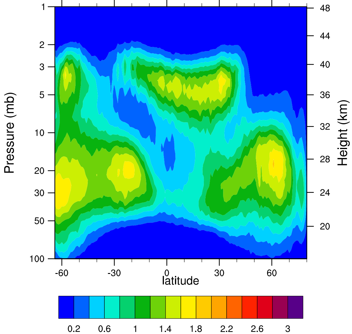
HIRDLSv6 2006d331 ClONO2_Ascending (ppbv)
