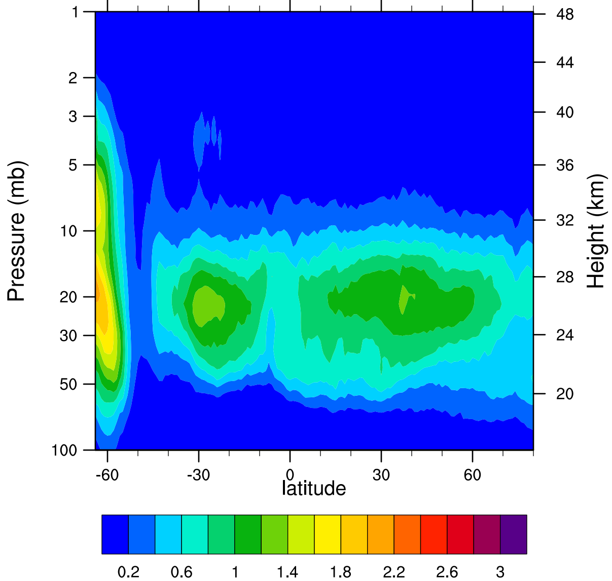
HIRDLSv6 2006d221 ClONO2_Ascending (ppbv)
