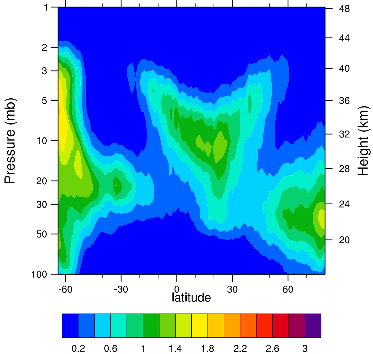
HIRDLSv6 2005d060 ClONO2_Ascending (ppbv)
