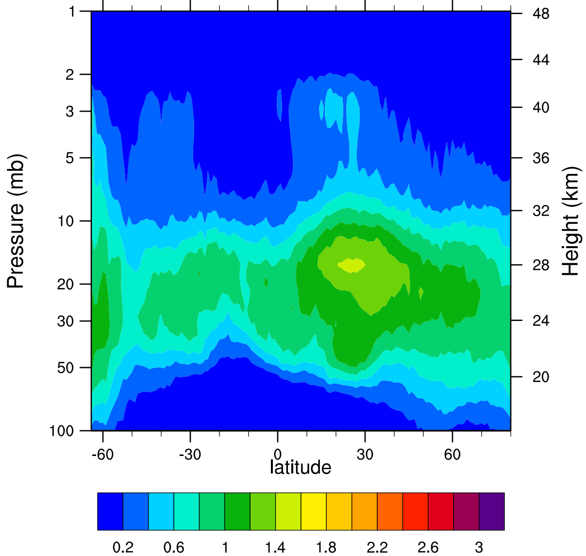
HIRDLSv6 2006d127 ClONO2_Ascending (ppbv)
