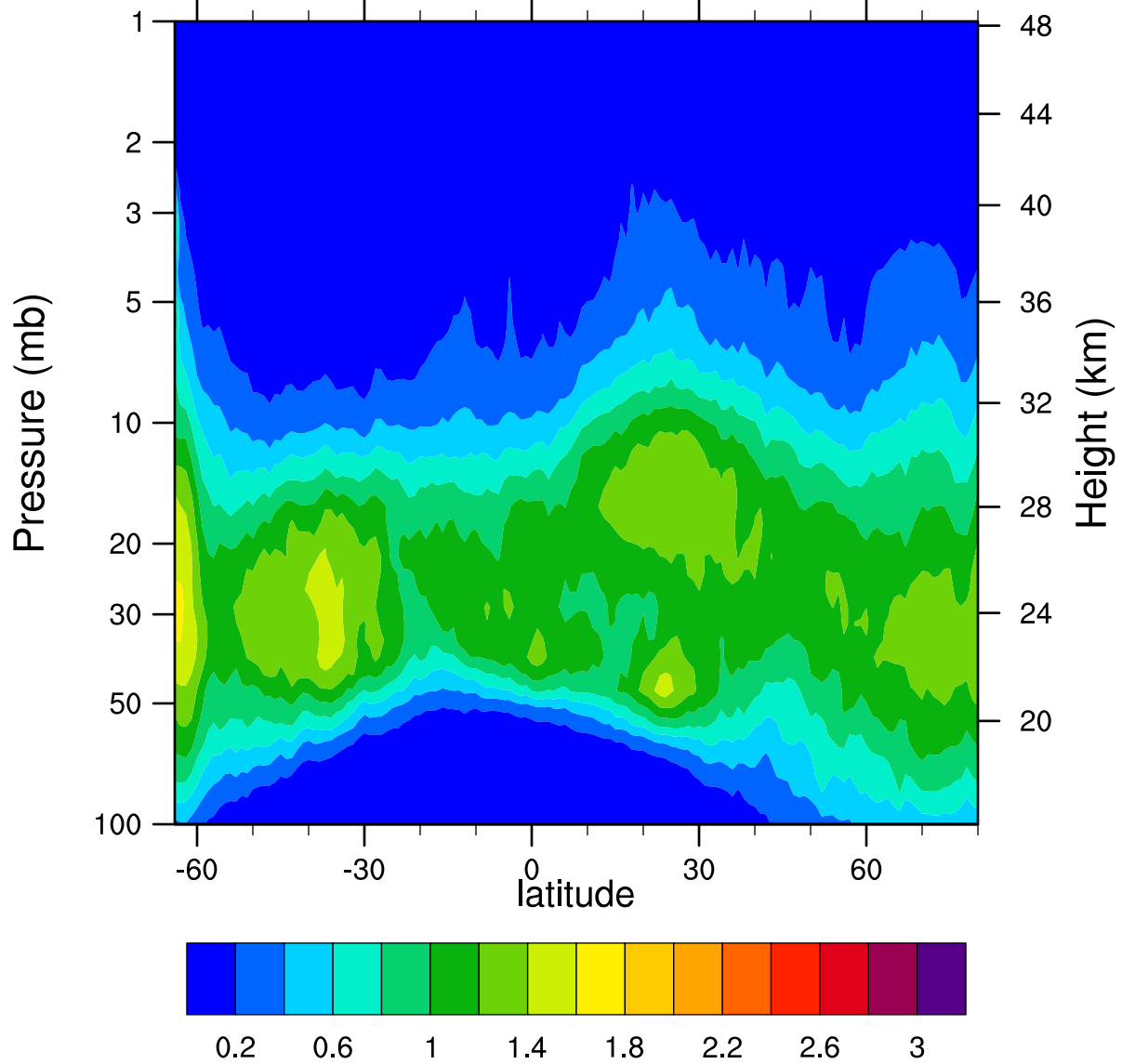
HIRDLSv6 2006d093 ClONO2_Ascending (ppbv)
