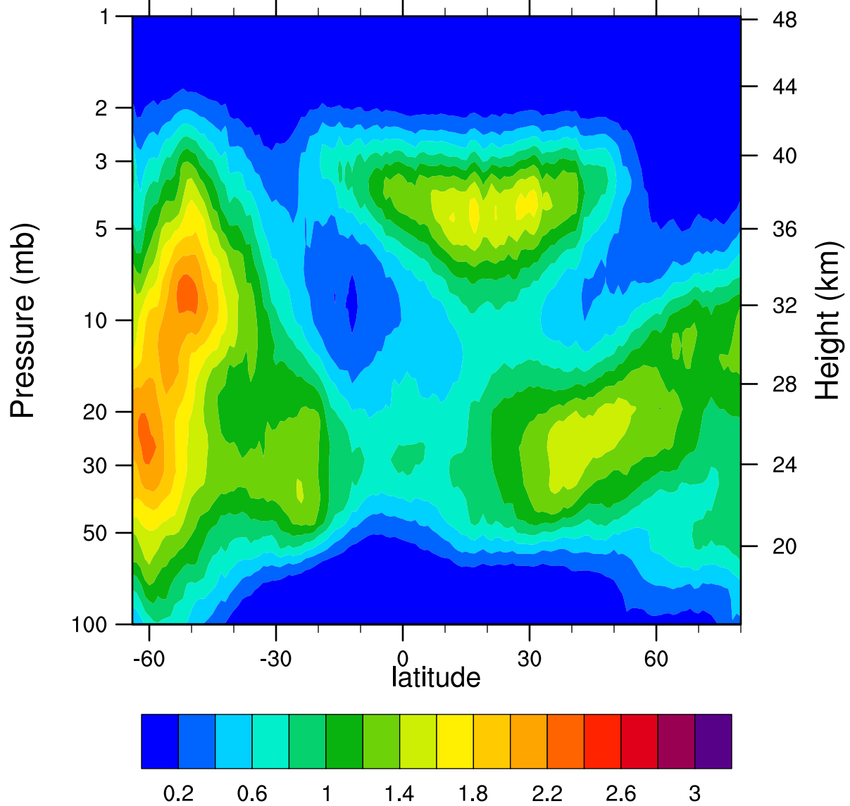
HIRDLSv6 2007d244 ClONO2_Ascending (ppbv)
