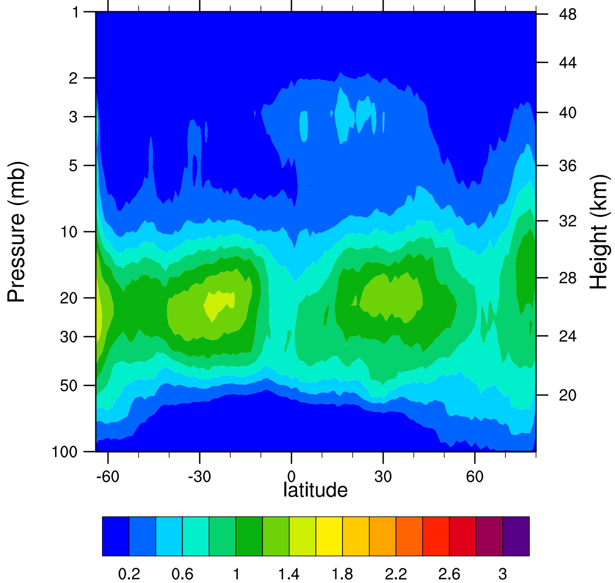
HIRDLSv6 2006d292 ClONO2_Ascending (ppbv)
