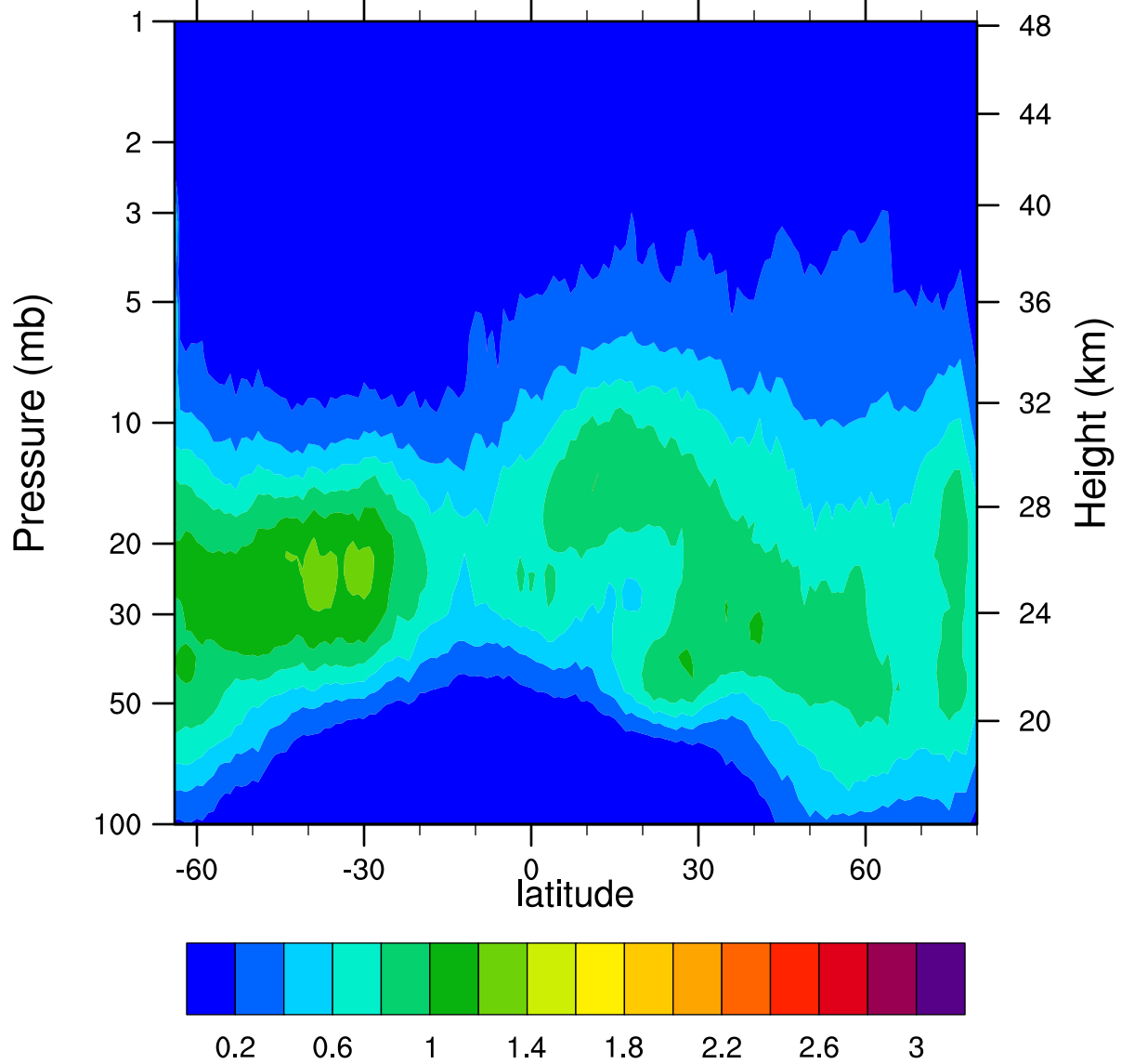
HIRDLSv6 2006d007 ClONO2_Ascending (ppbv)
