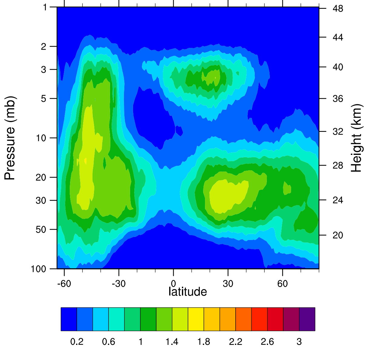
HIRDLSv6 2007d147 ClONO2_Ascending (ppbv)
