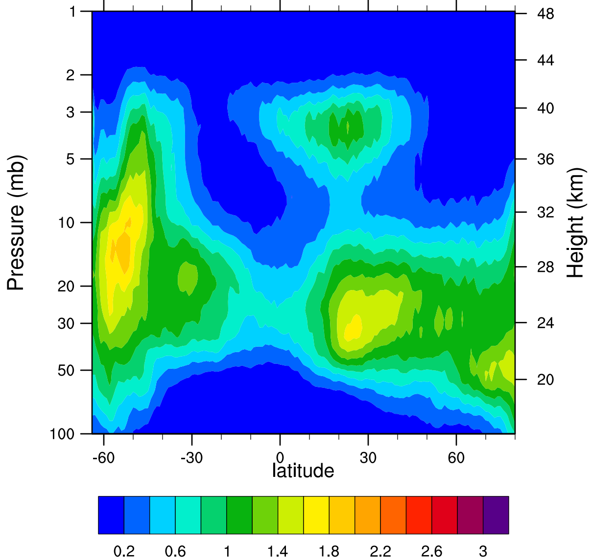
HIRDLSv6 2007d118 ClONO2_Ascending (ppbv)
