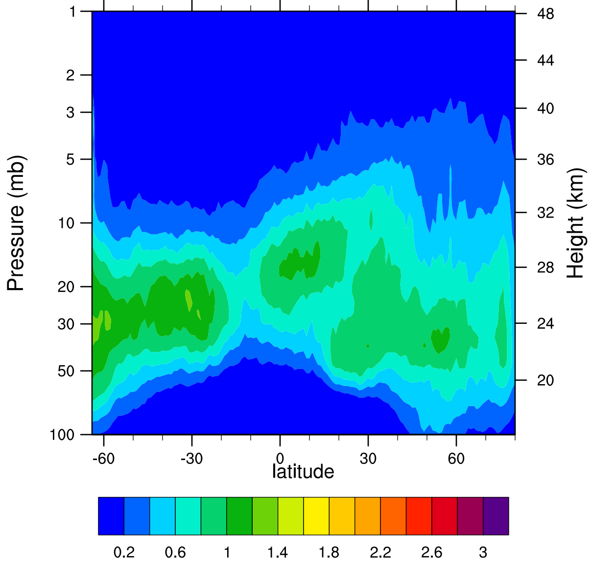
HIRDLSv6 2005d347 ClONO2_Ascending (ppbv)
