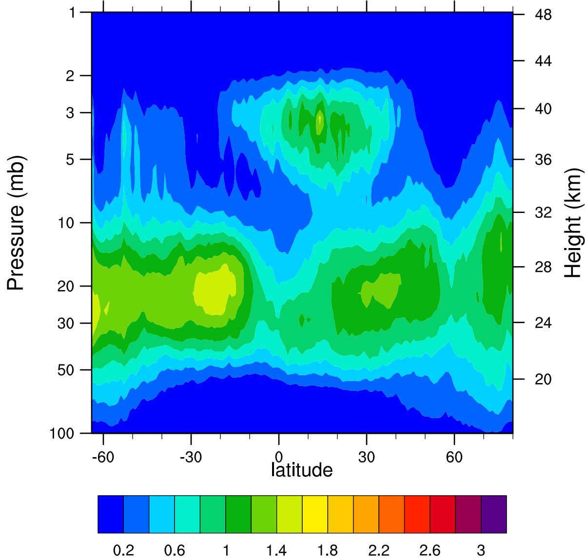
HIRDLSv6 2006d302 ClONO2_Ascending (ppbv)
