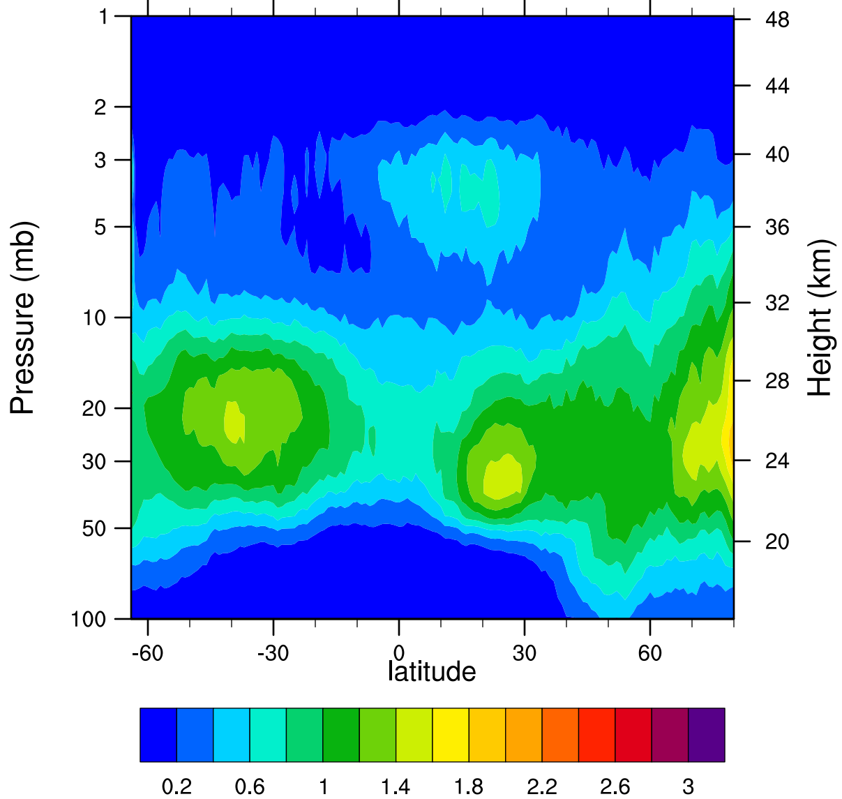
HIRDLSv6 2007d043 ClONO2_Ascending (ppbv)
