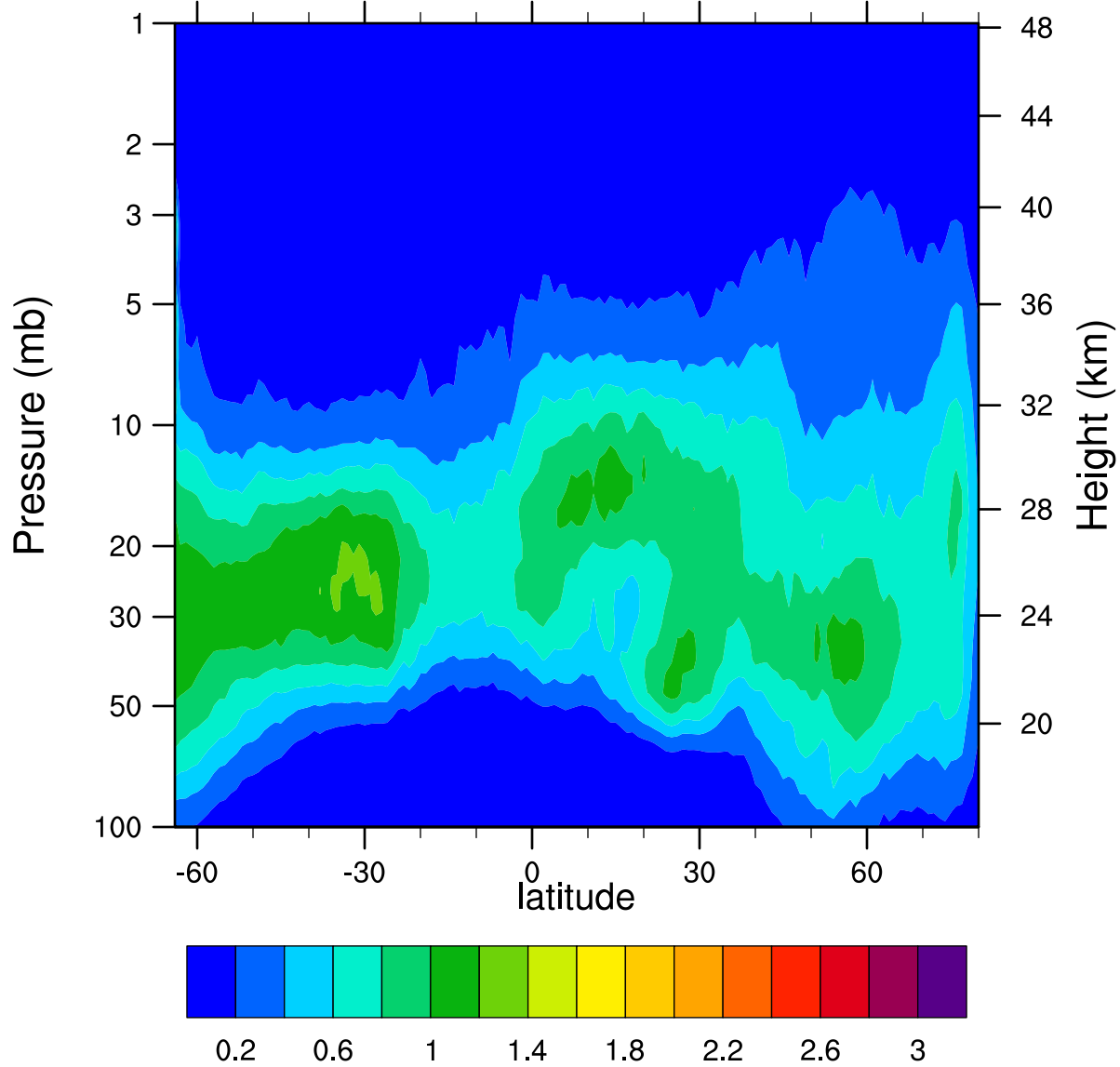
HIRDLSv6 2005d362 ClONO2_Ascending (ppbv)
