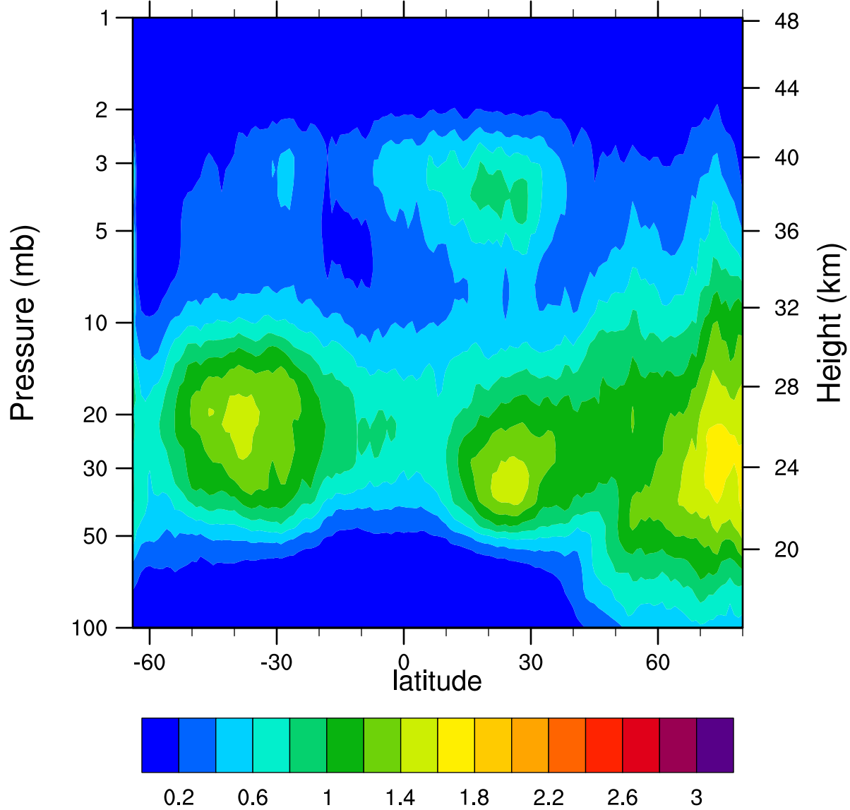
HIRDLSv6 2007d053 ClONO2_Ascending (ppbv)
