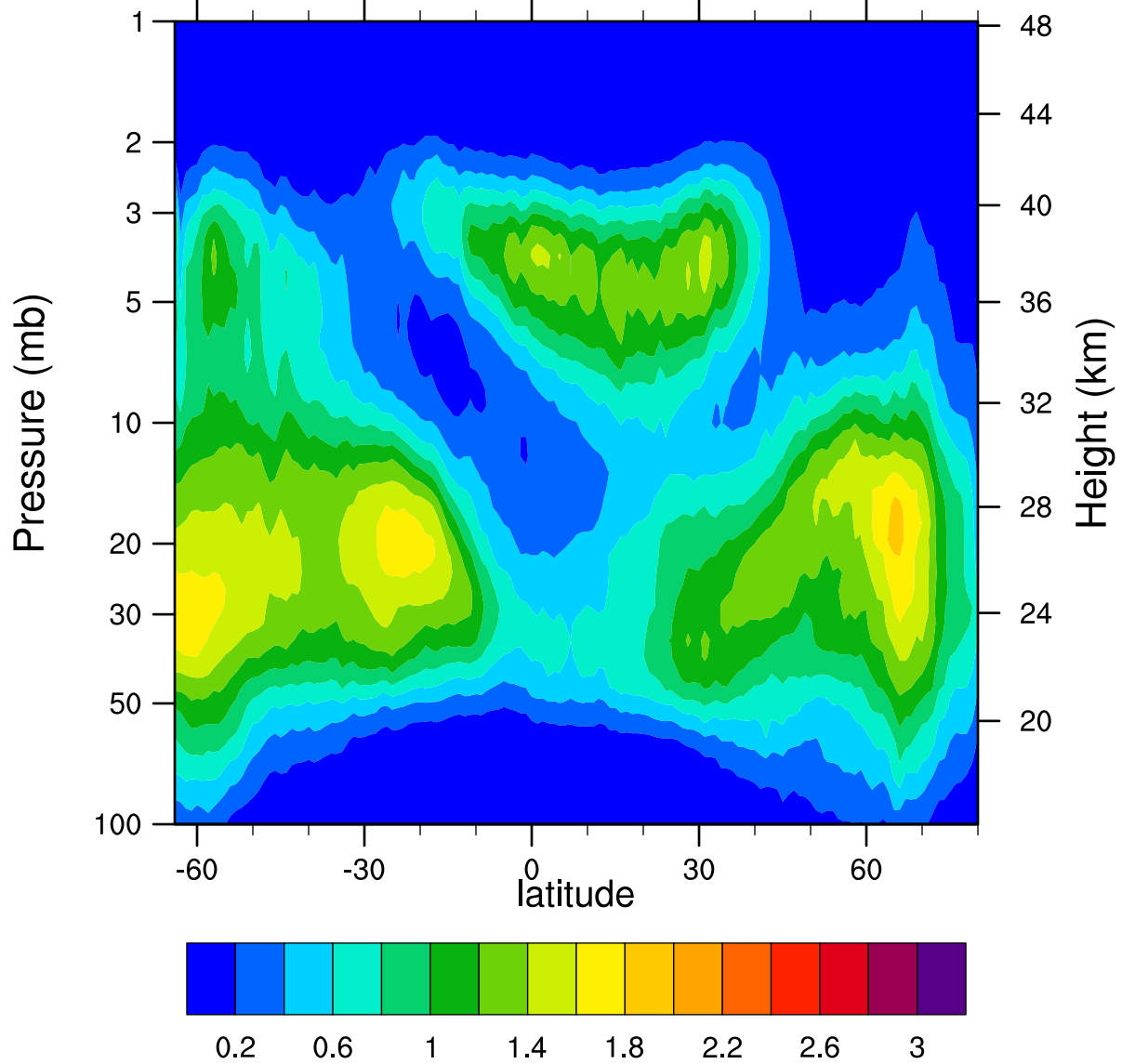
HIRDLSv6 2006d322 ClONO2_Ascending (ppbv)
