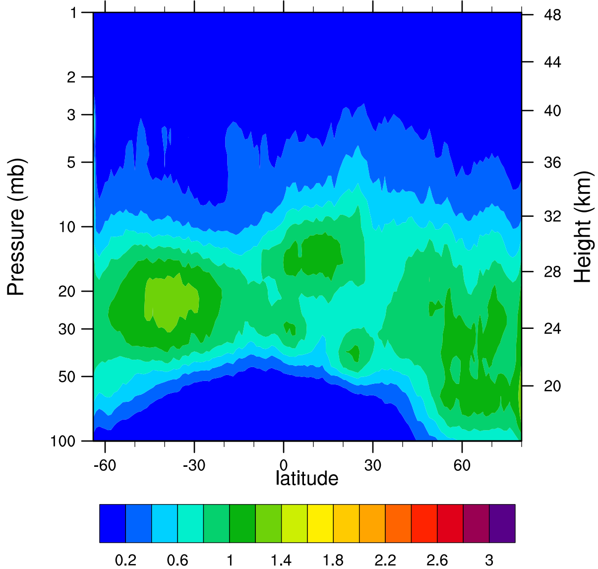
HIRDLSv6 2006d045 ClONO2_Ascending (ppbv)
