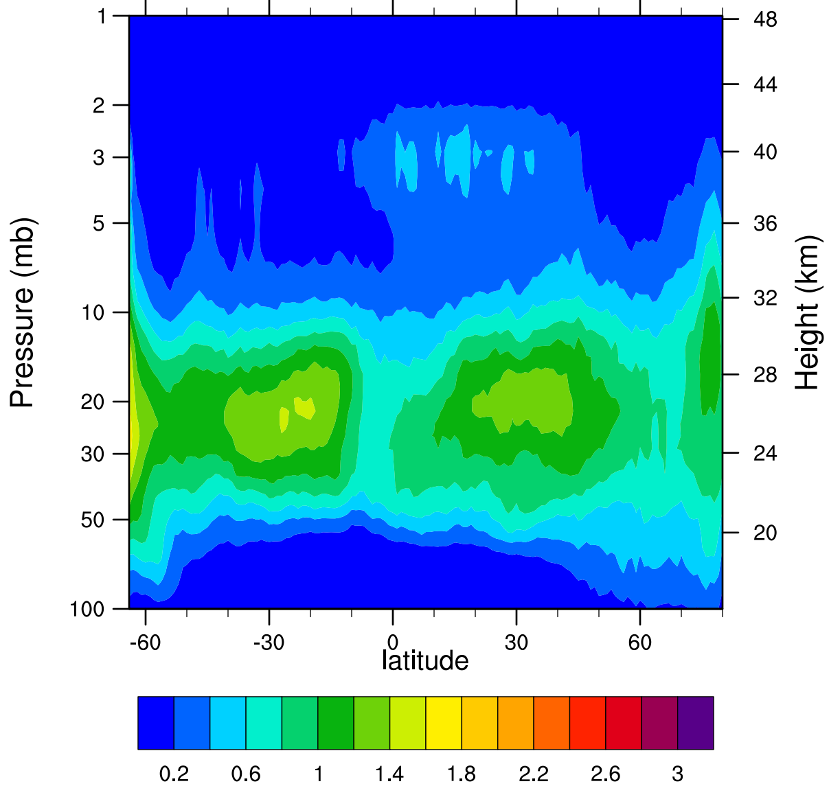
HIRDLSv6 2006d288 ClONO2_Ascending (ppbv)
