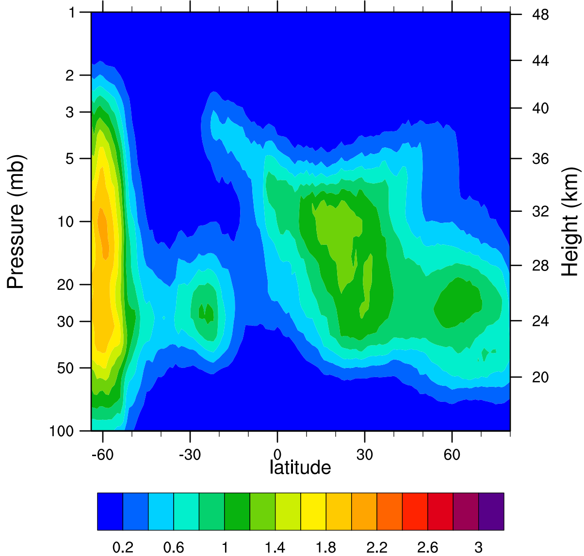
HIRDLSv6 2005d166 ClONO2_Ascending (ppbv)
