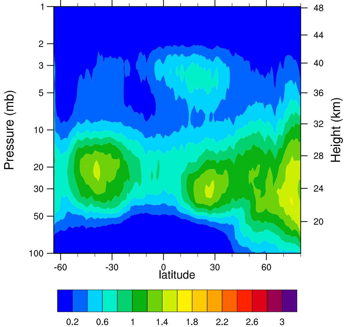
HIRDLSv6 2007d058 ClONO2_Ascending (ppbv)
