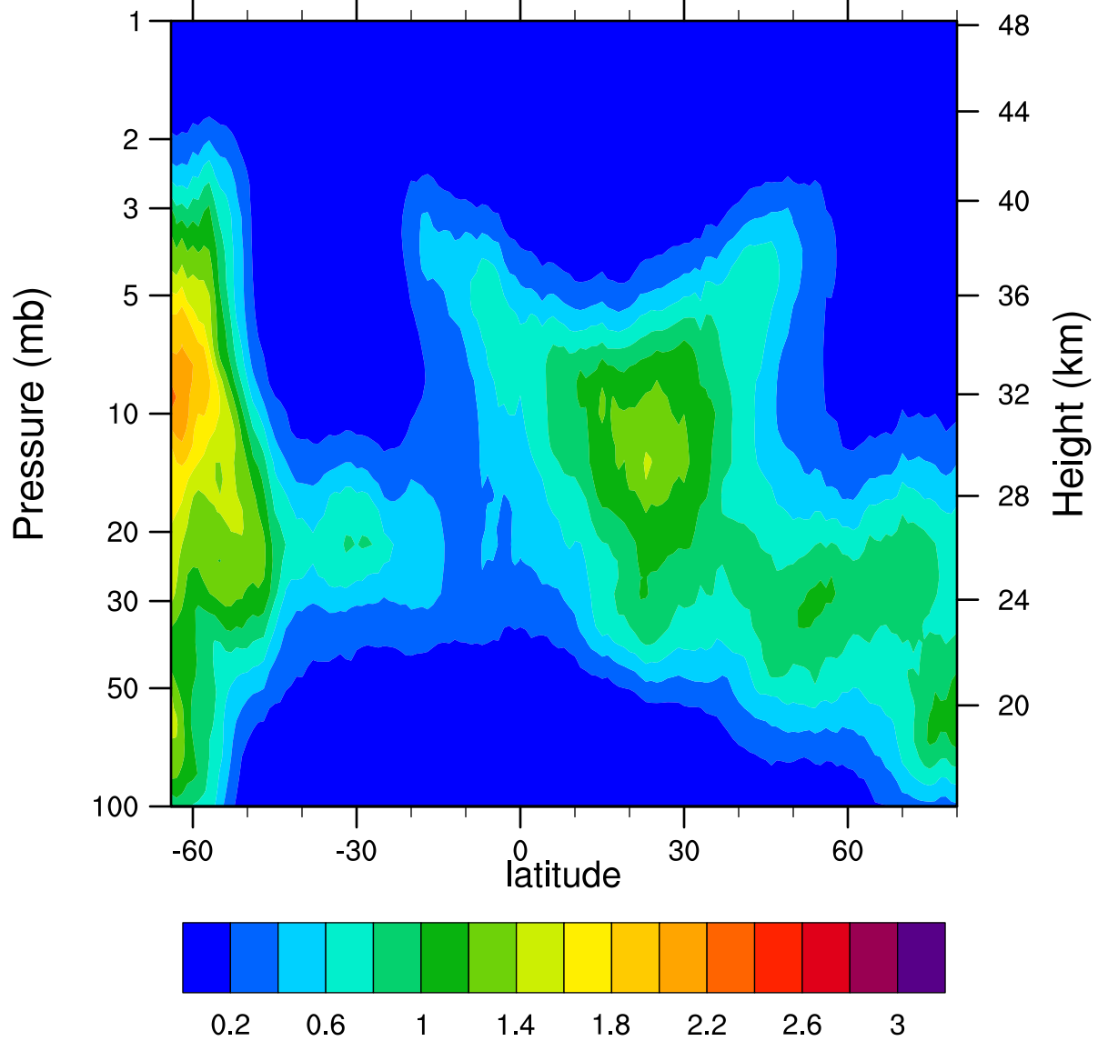
HIRDLSv6 2005d094 ClONO2_Ascending (ppbv)
