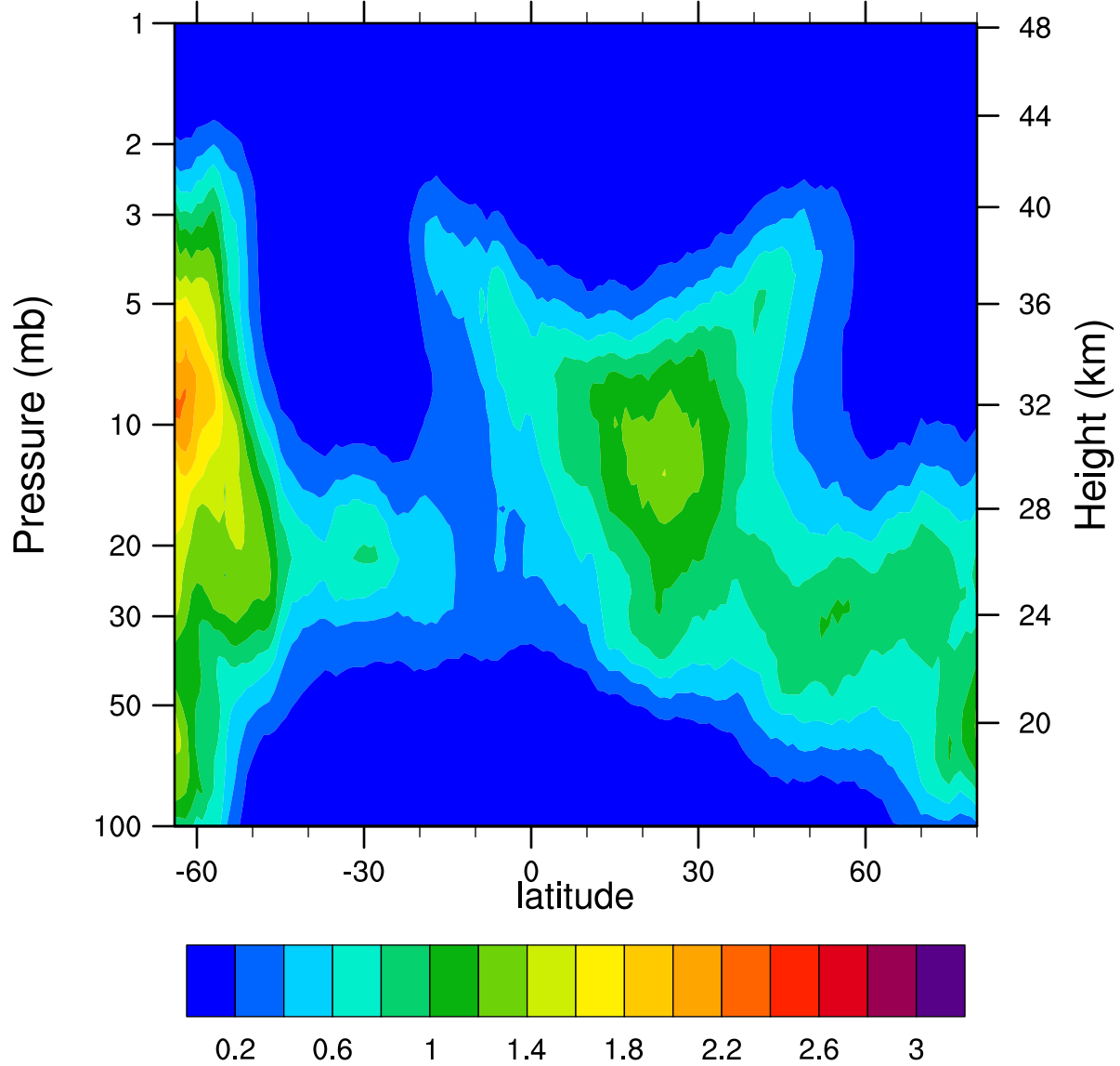
HIRDLSv6 2005d093 ClONO2_Ascending (ppbv)
