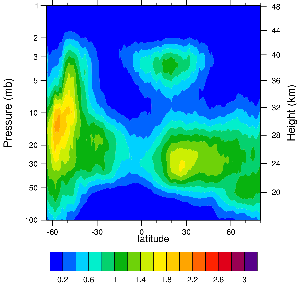
HIRDLSv6 2007d125 ClONO2_Ascending (ppbv)
