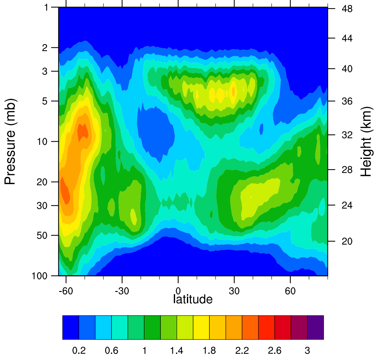
HIRDLSv6 2007d240 ClONO2_Ascending (ppbv)
