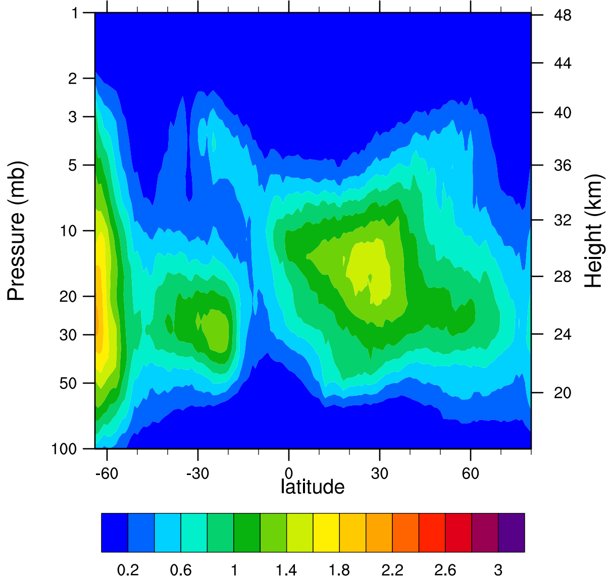
HIRDLSv6 2005d265 ClONO2_Ascending (ppbv)
