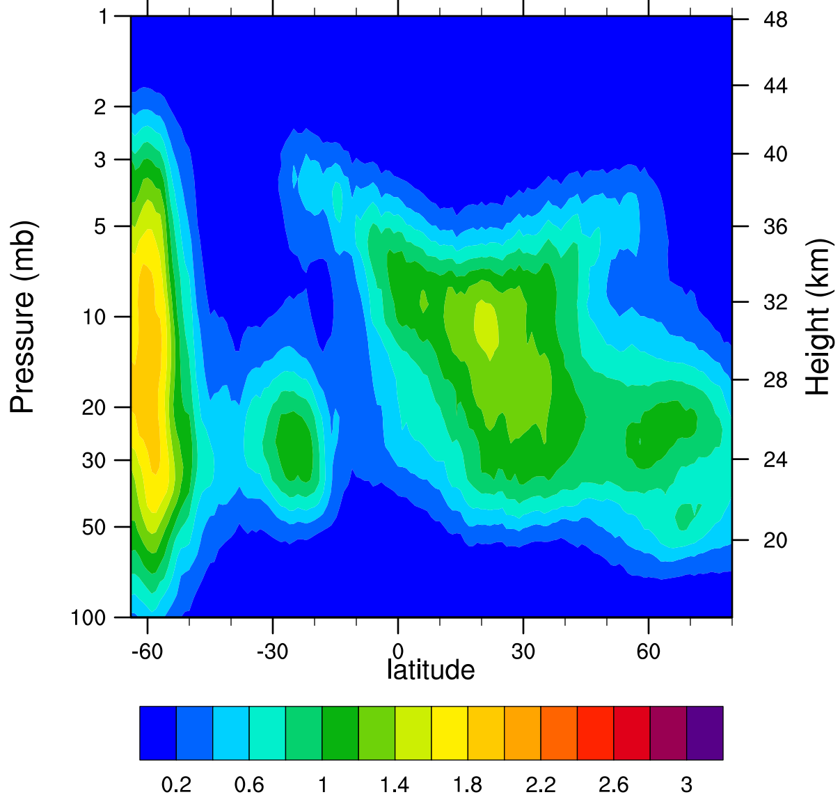
HIRDLSv6 2005d178 ClONO2_Ascending (ppbv)
