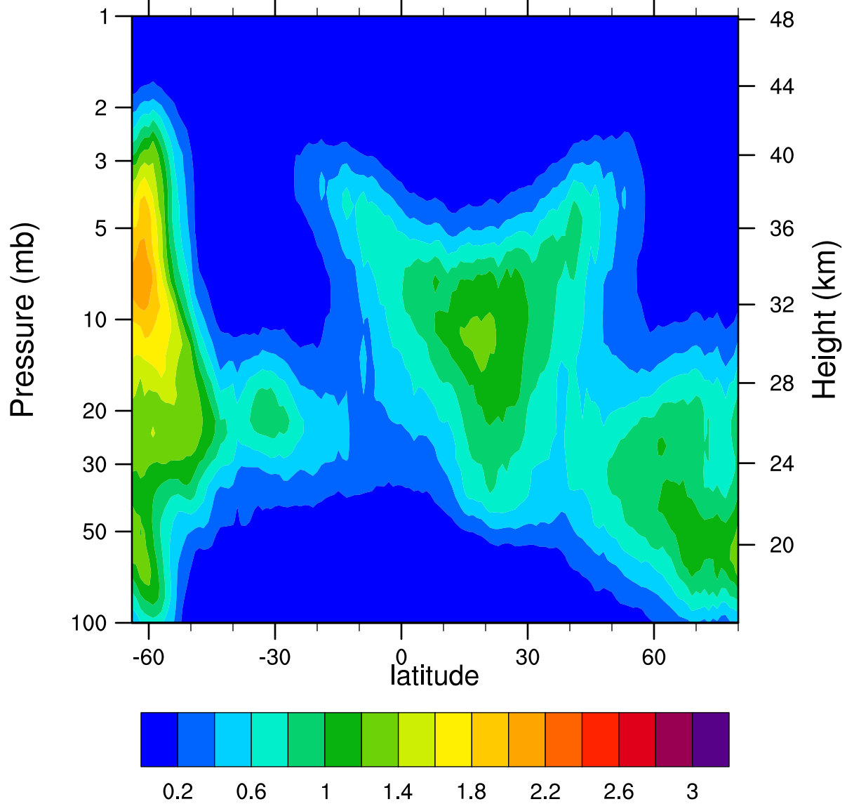
HIRDLSv6 2005d079 ClONO2_Ascending (ppbv)
