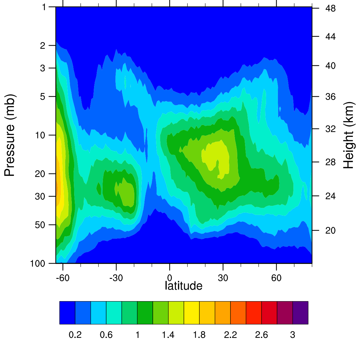
HIRDLSv6 2005d266 ClONO2_Ascending (ppbv)
