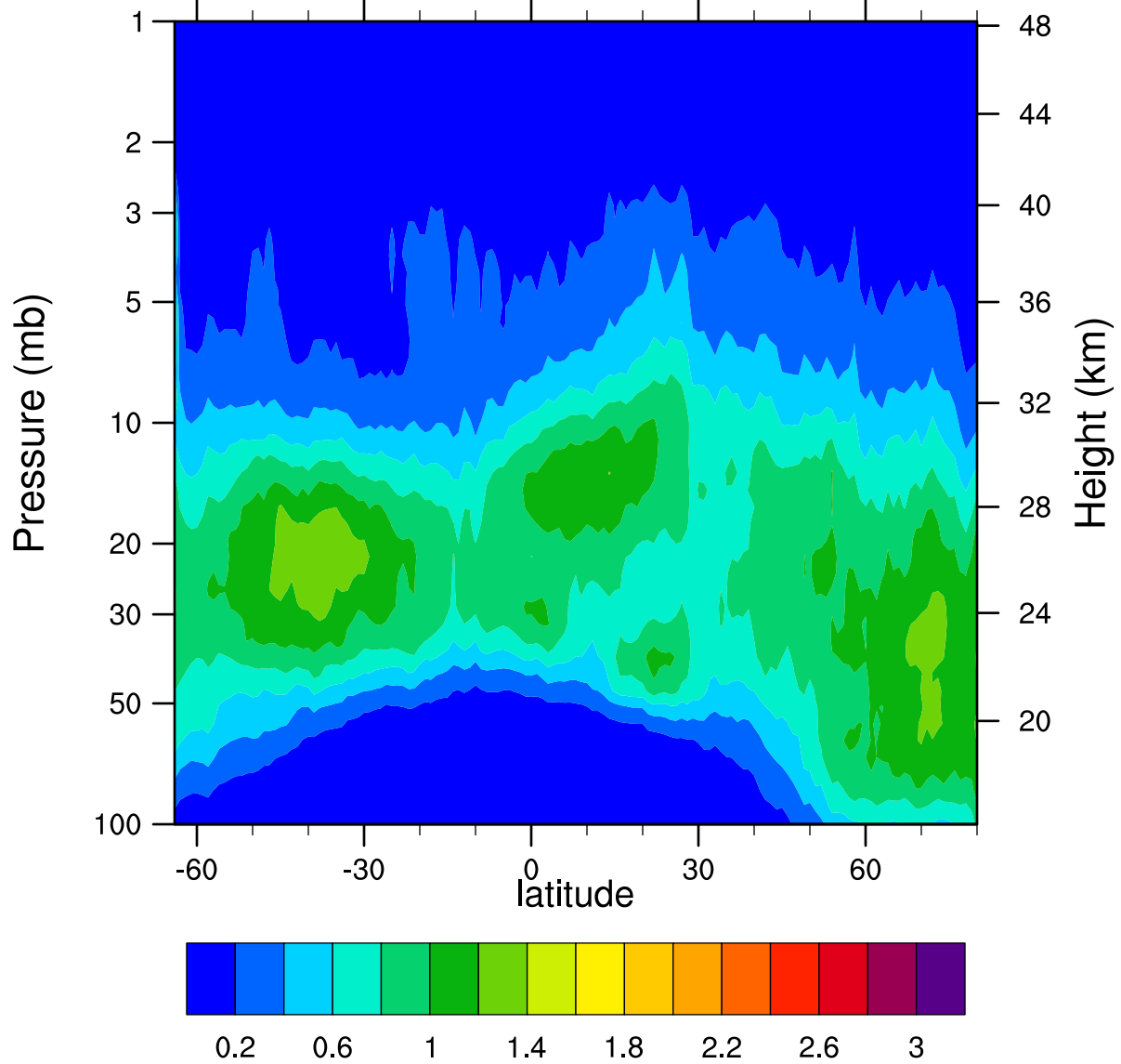
HIRDLSv6 2006d051 ClONO2_Ascending (ppbv)
