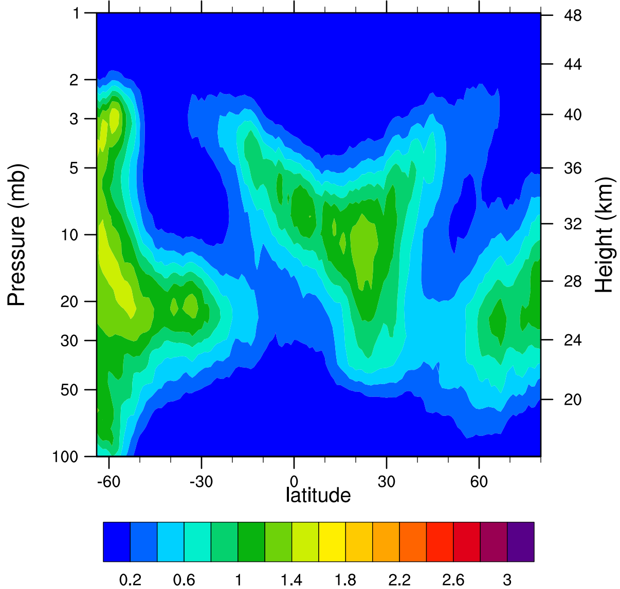
HIRDLSv6 2005d033 ClONO2_Ascending (ppbv)
