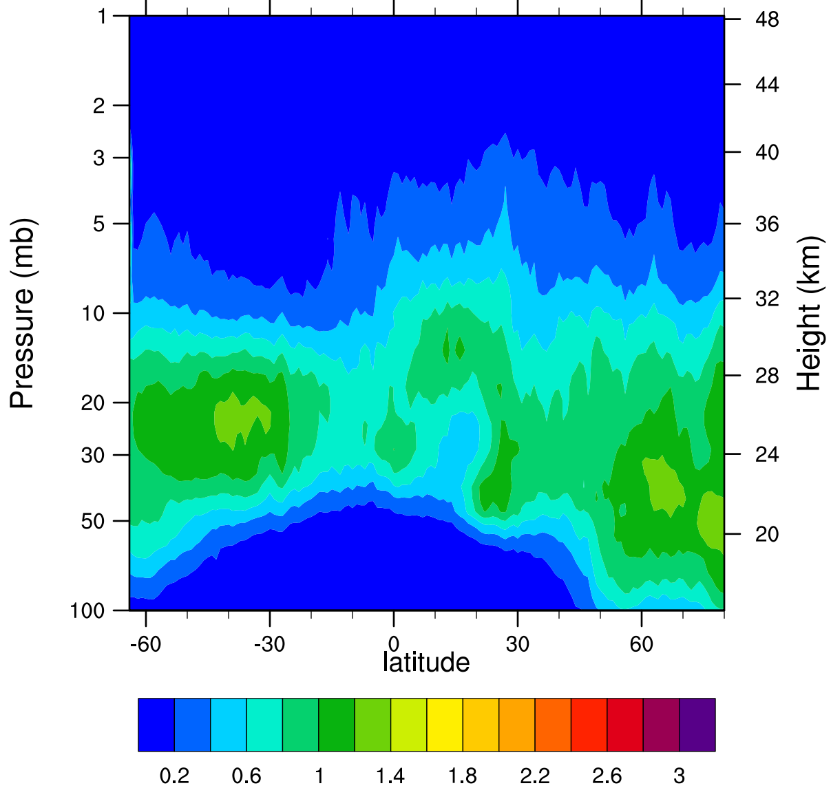
HIRDLSv6 2006d031 ClONO2_Ascending (ppbv)
