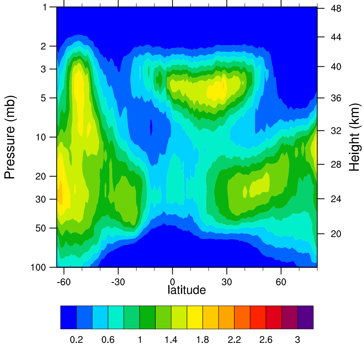
HIRDLSv6 2007d266 ClONO2_Ascending (ppbv)
