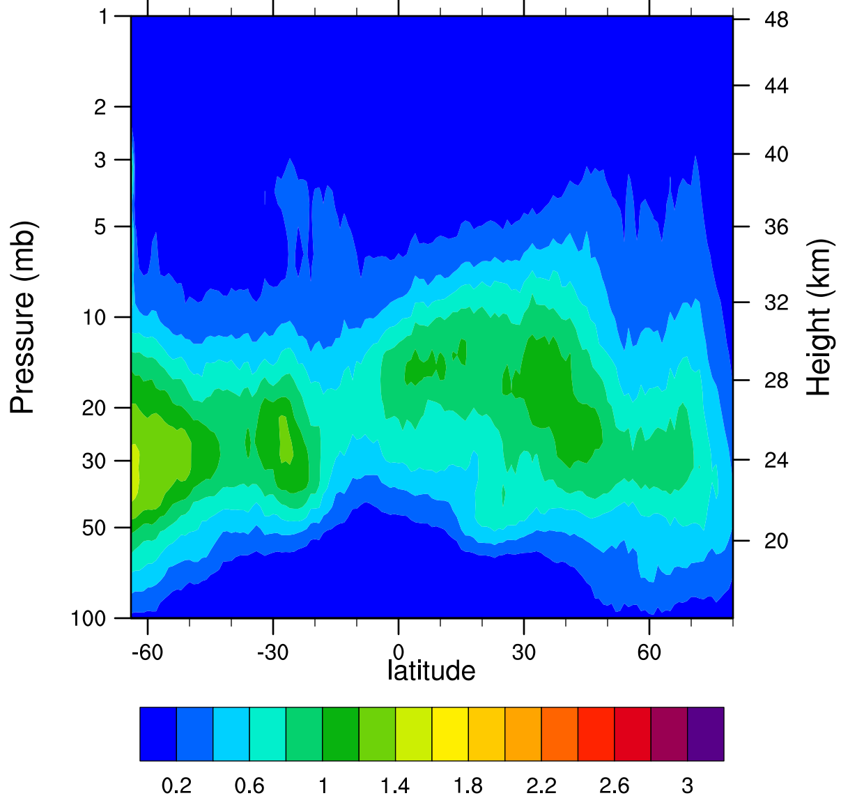
HIRDLSv6 2005d319 ClONO2_Ascending (ppbv)
