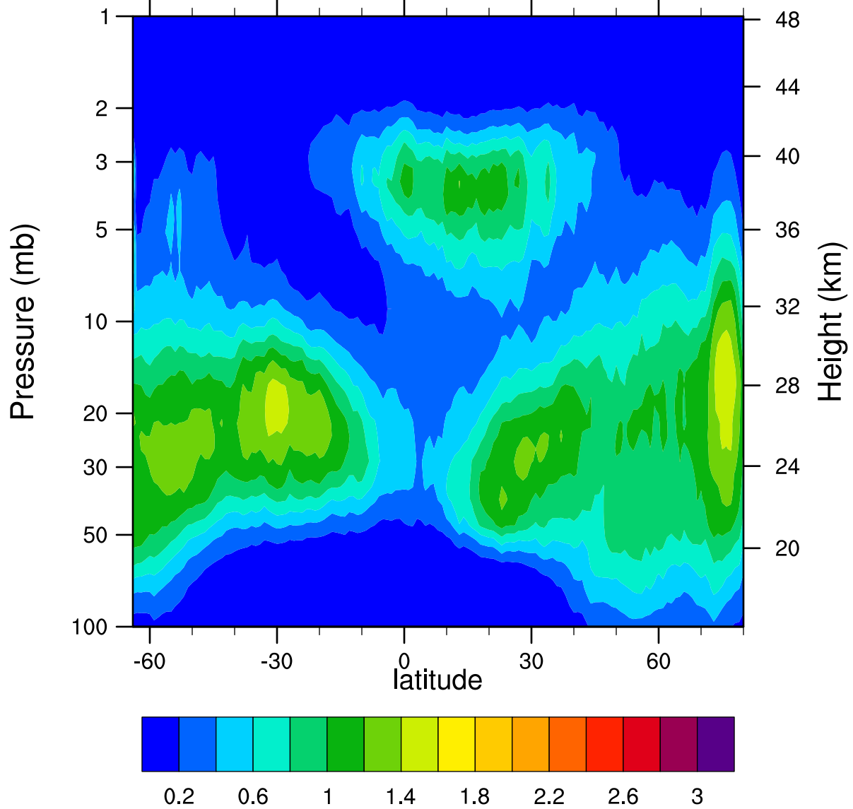
HIRDLSv6 2006d360 ClONO2_Ascending (ppbv)
