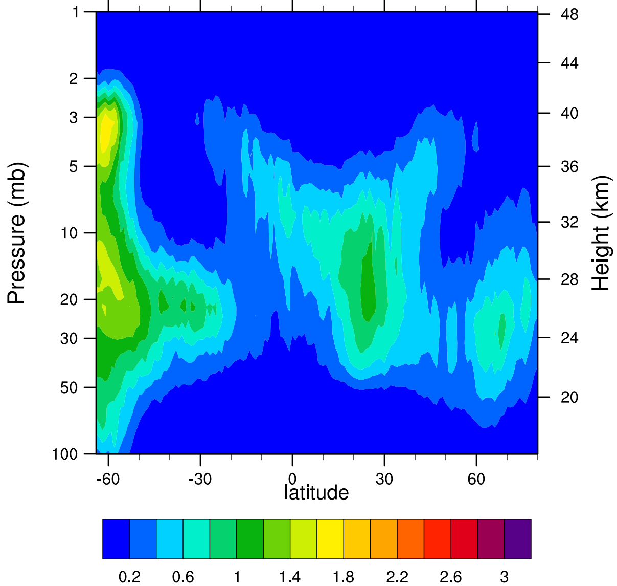
HIRDLSv6 2005d028 ClONO2_Ascending (ppbv)
