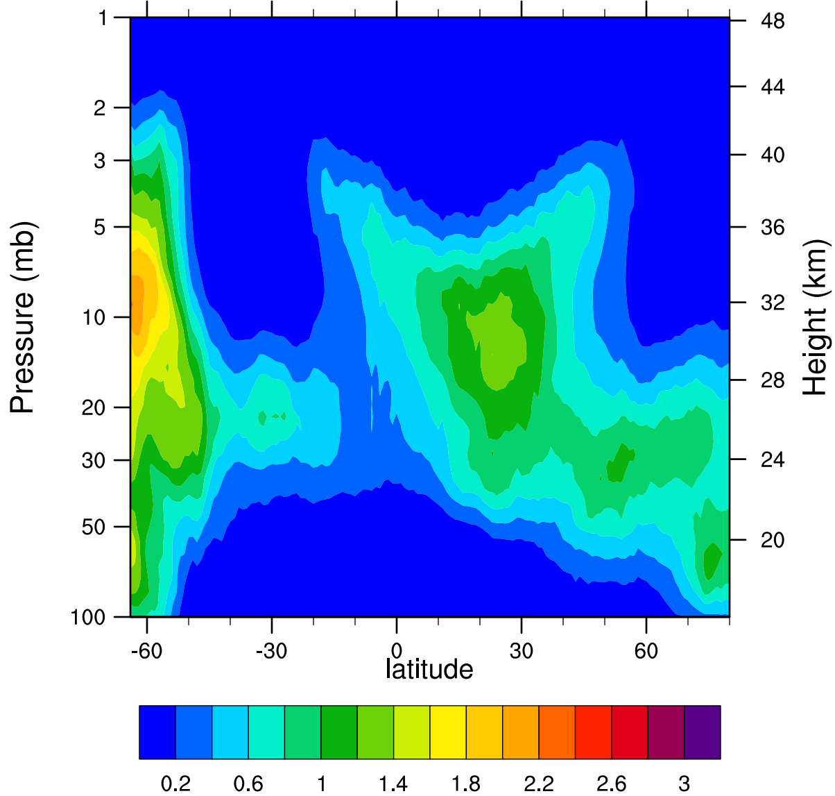
HIRDLSv6 2005d096 ClONO2_Ascending (ppbv)
