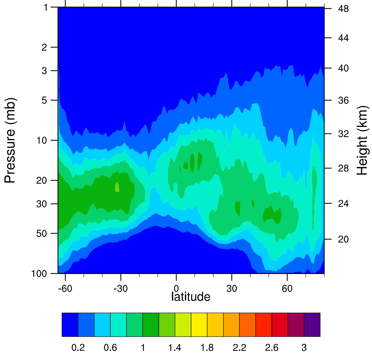
HIRDLSv6 2005d351 ClONO2_Ascending (ppbv)
