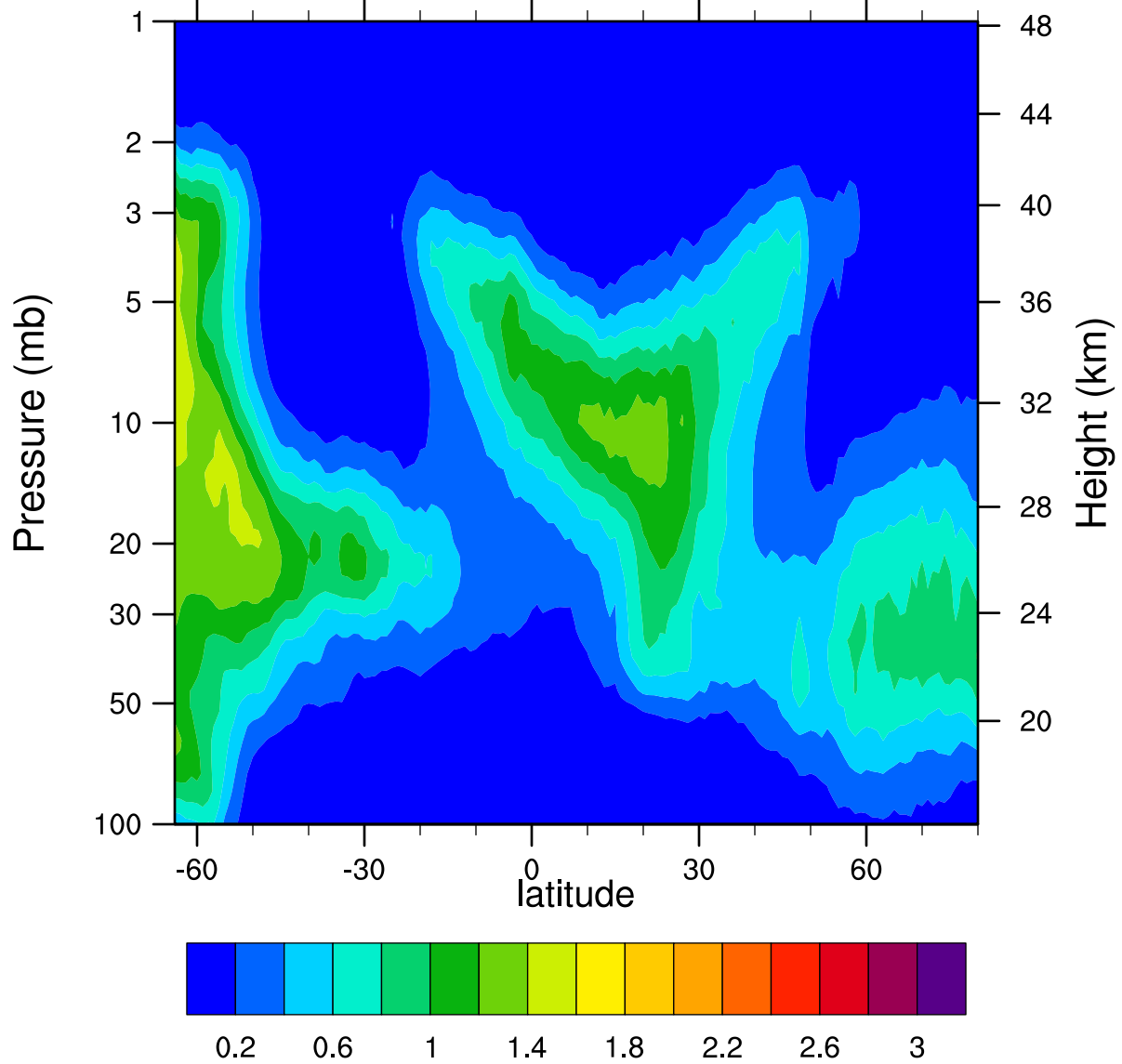
HIRDLSv6 2005d052 ClONO2_Ascending (ppbv)
