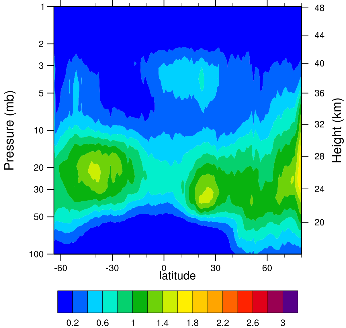
HIRDLSv6 2007d039 ClONO2_Ascending (ppbv)
