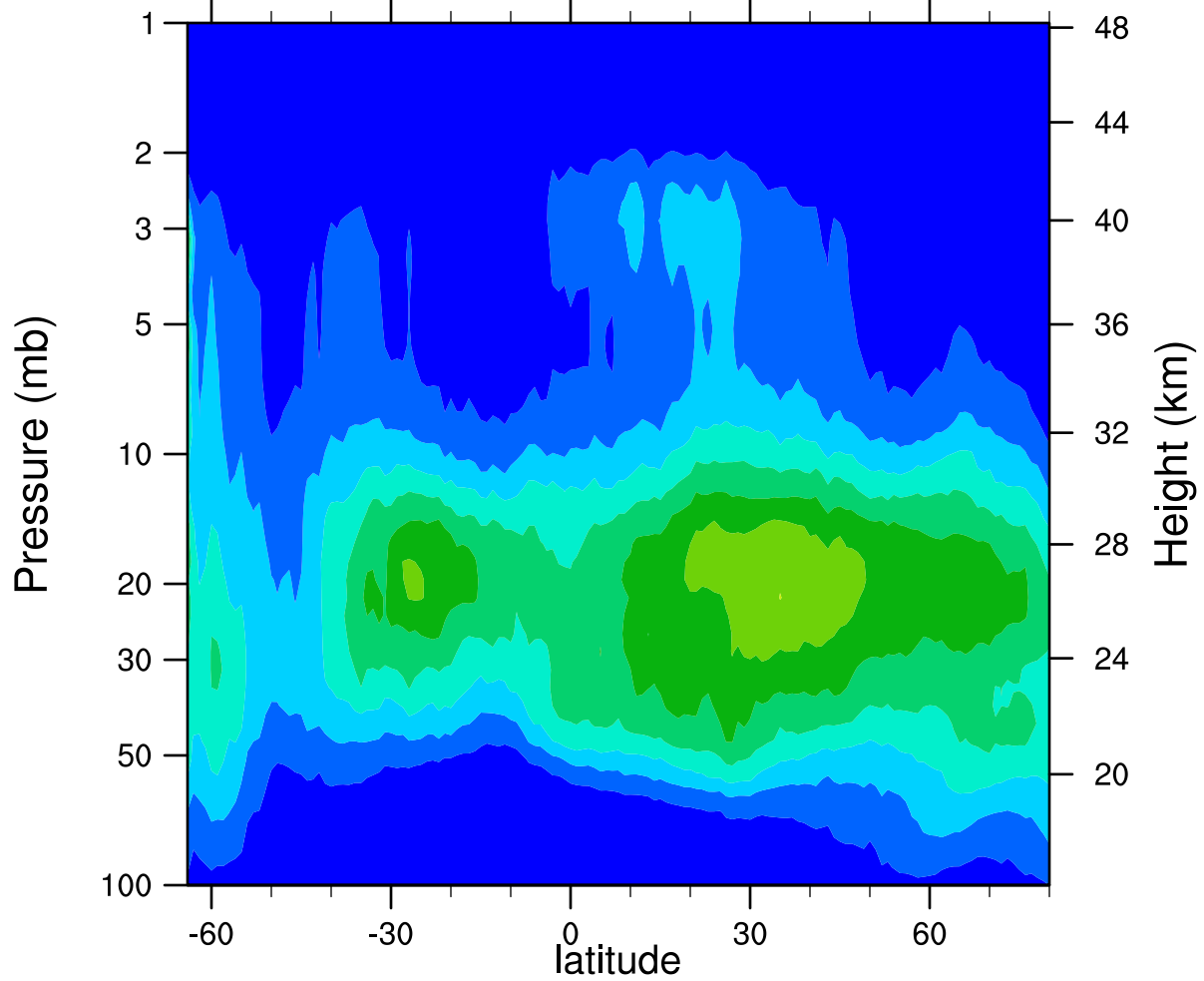
HIRDLSv6 2006d161 ClONO2_Ascending (ppbv)
