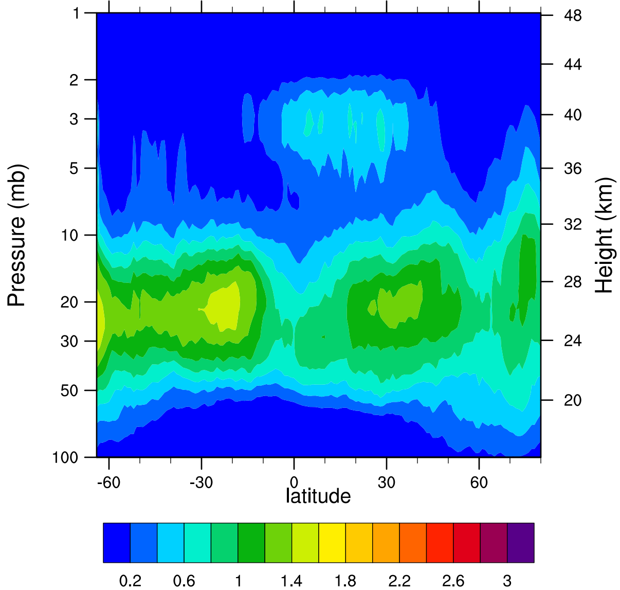
HIRDLSv6 2006d299 ClONO2_Ascending (ppbv)
