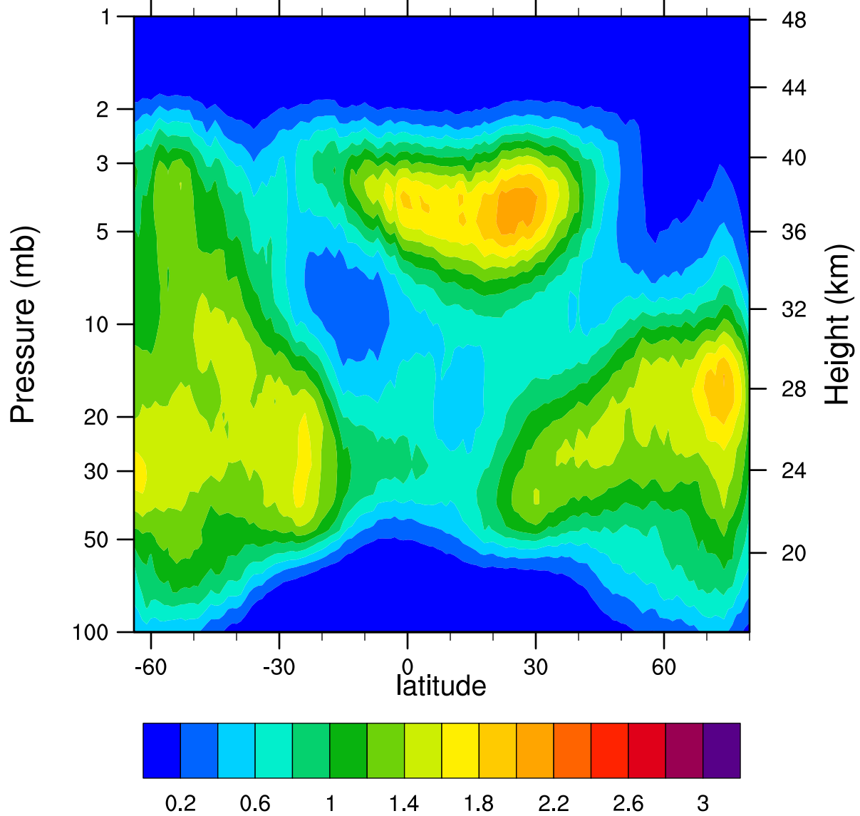
HIRDLSv6 2007d299 ClONO2_Ascending (ppbv)
