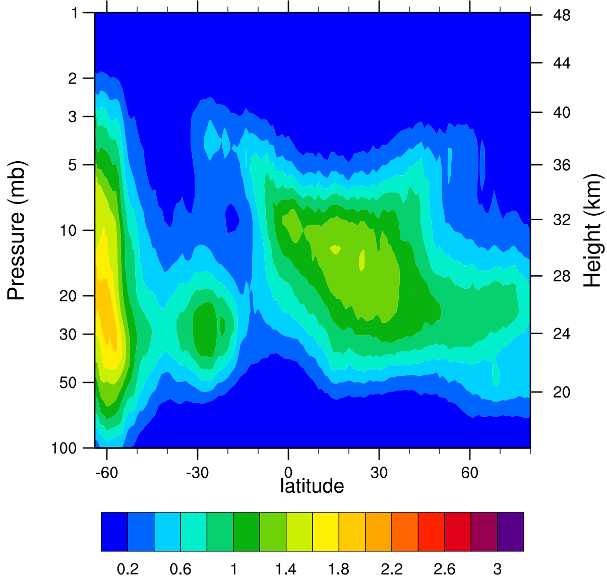
HIRDLSv6 2005d209 ClONO2_Ascending (ppbv)
