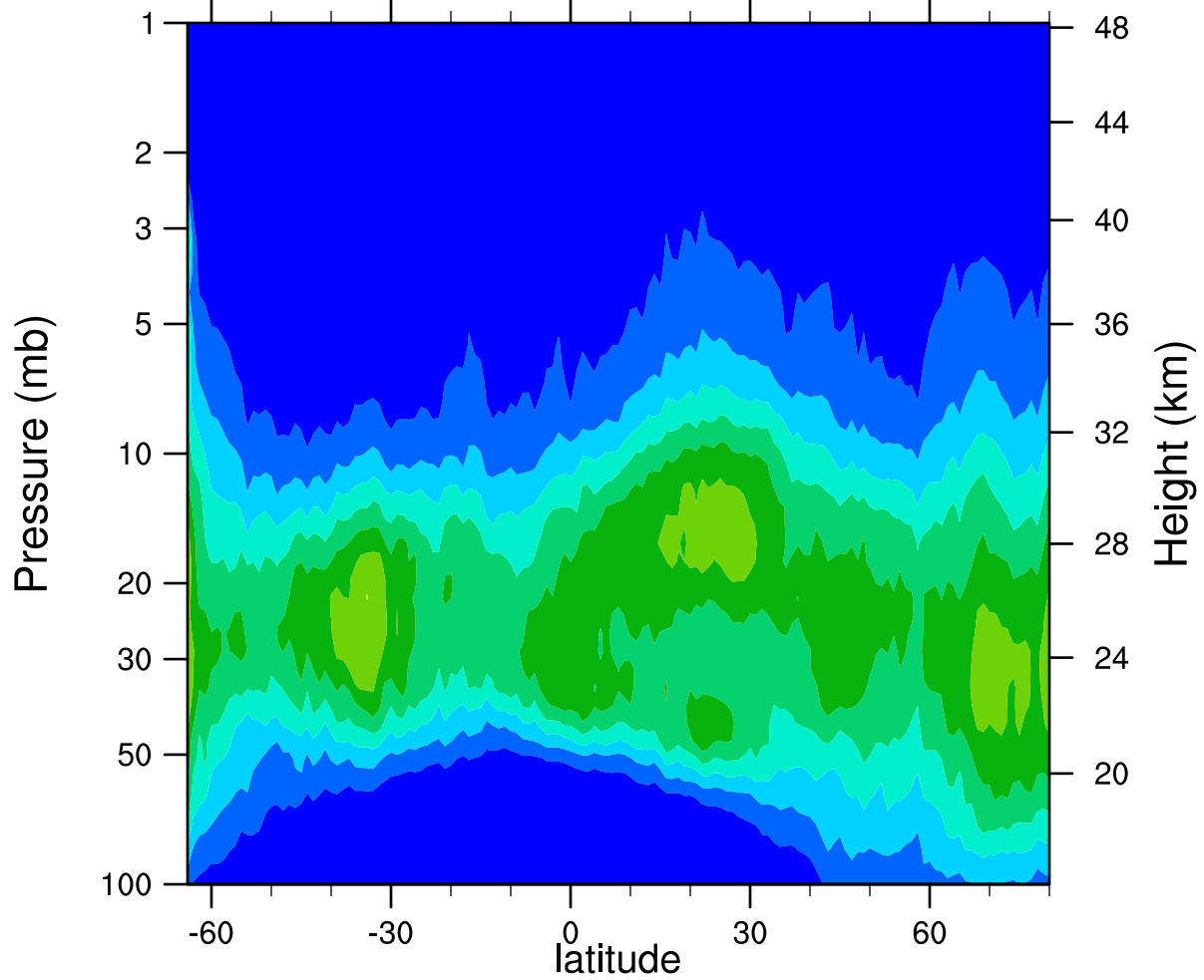
HIRDLSv6 2006d085 ClONO2_Ascending (ppbv)
