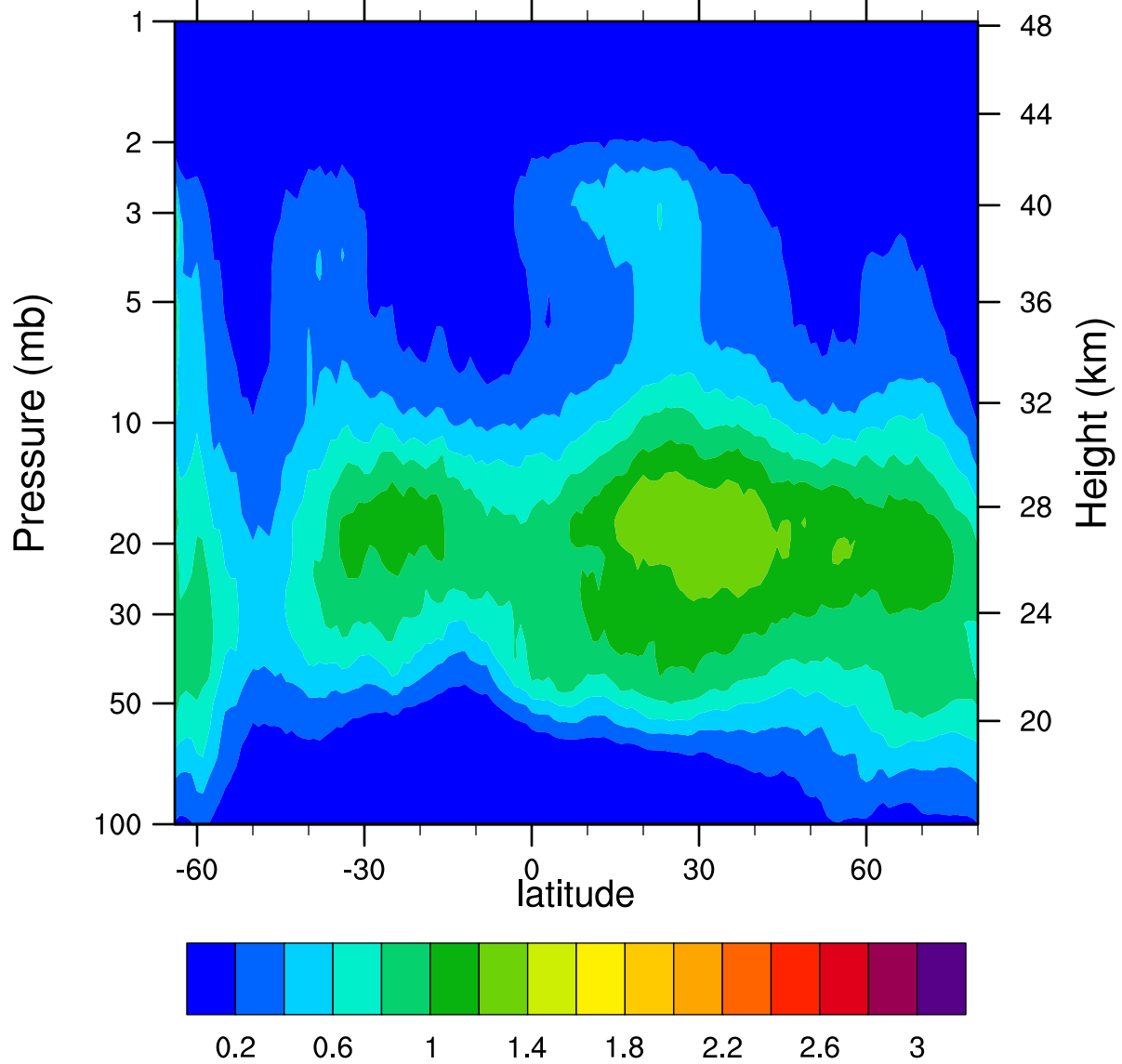
HIRDLSv6 2006d149 ClONO2_Ascending (ppbv)
