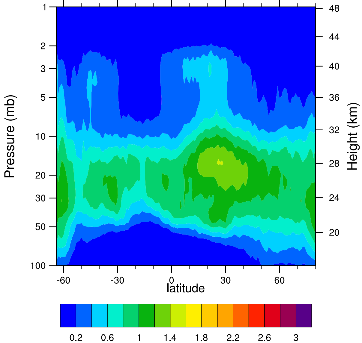
HIRDLSv6 2006d118 ClONO2_Ascending (ppbv)
