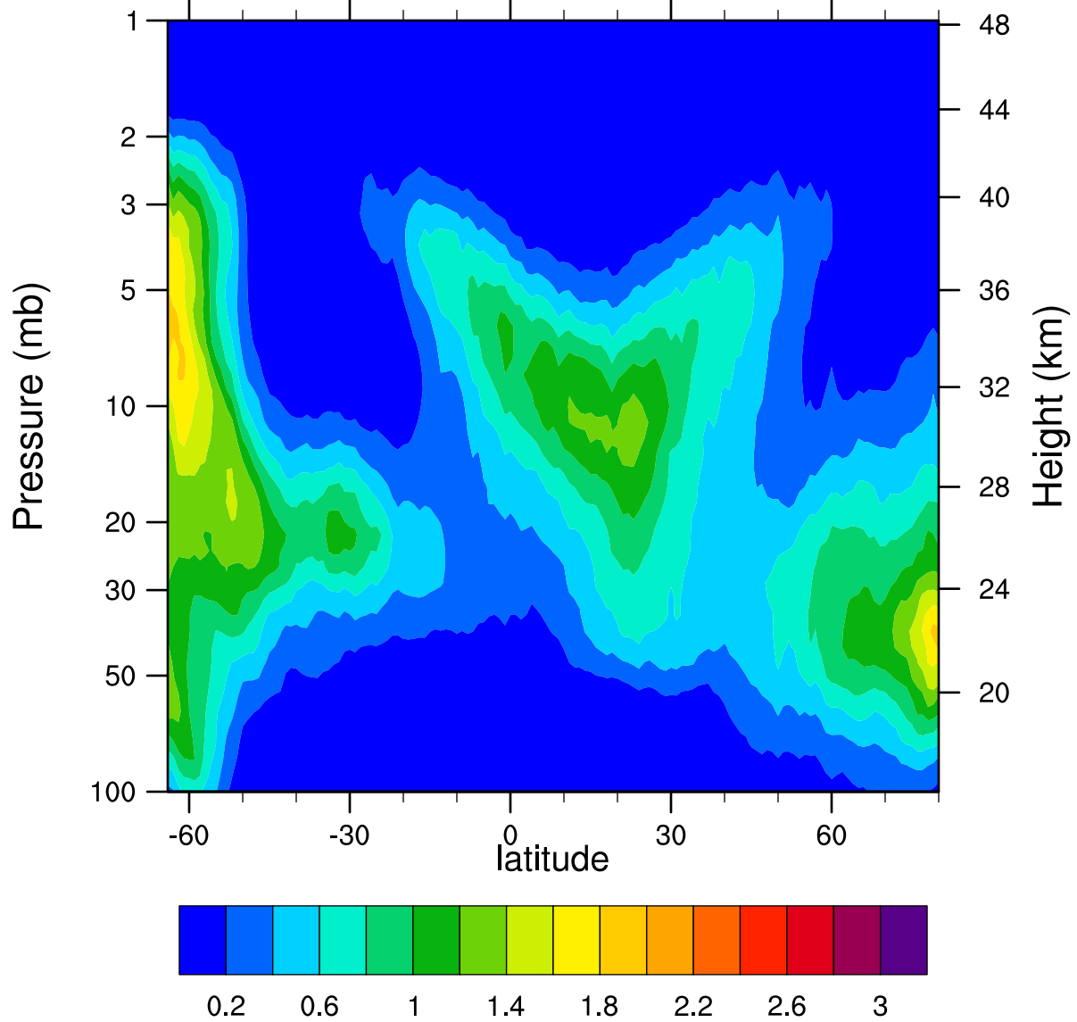
HIRDLSv6 2005d063 ClONO2_Ascending (ppbv)
