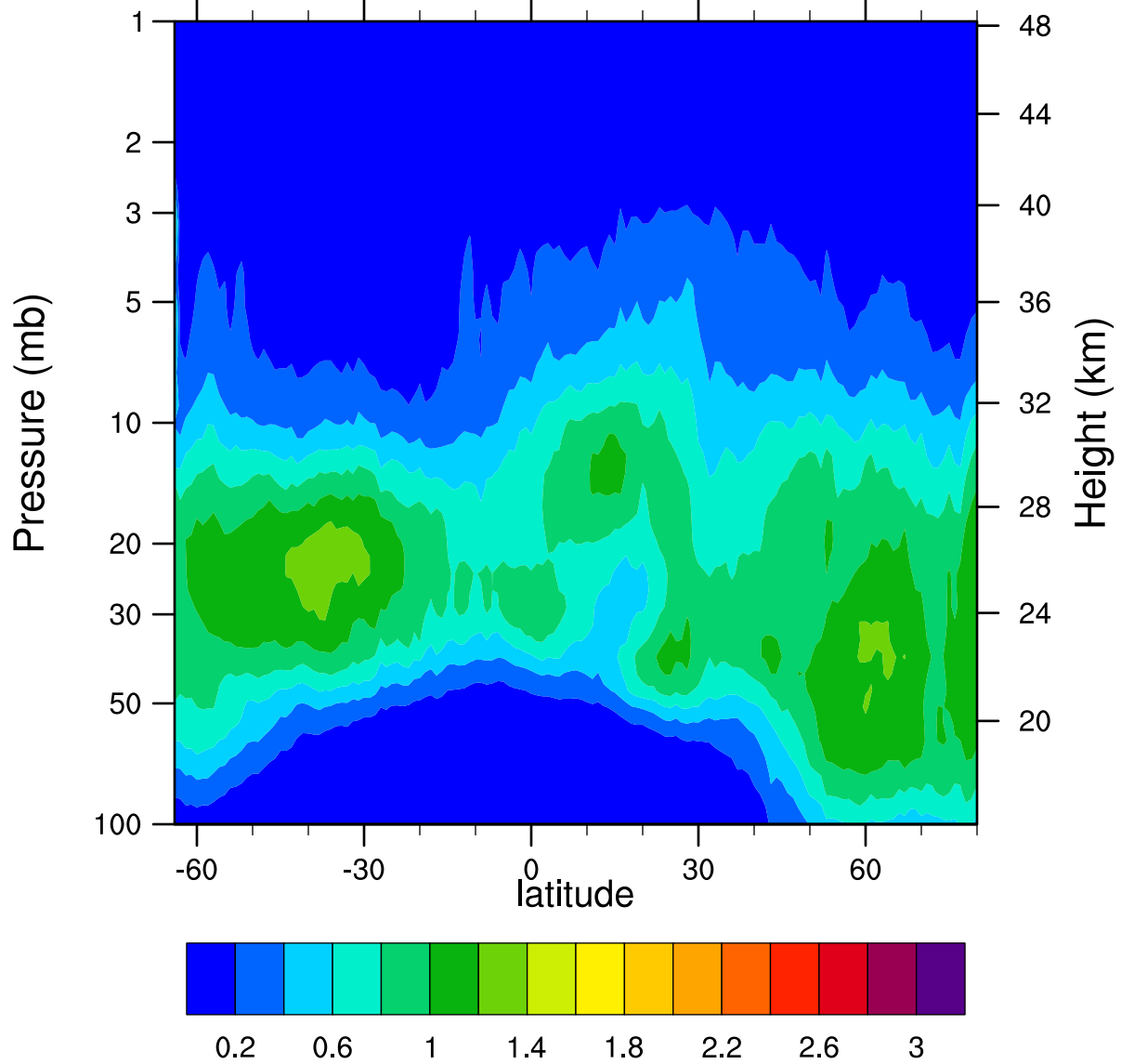
HIRDLSv6 2006d036 ClONO2_Ascending (ppbv)
