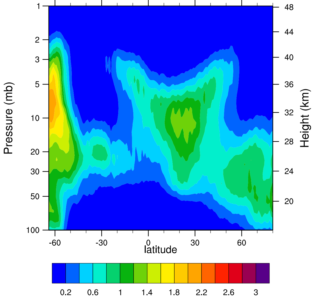
HIRDLSv6 2005d082 ClONO2_Ascending (ppbv)
