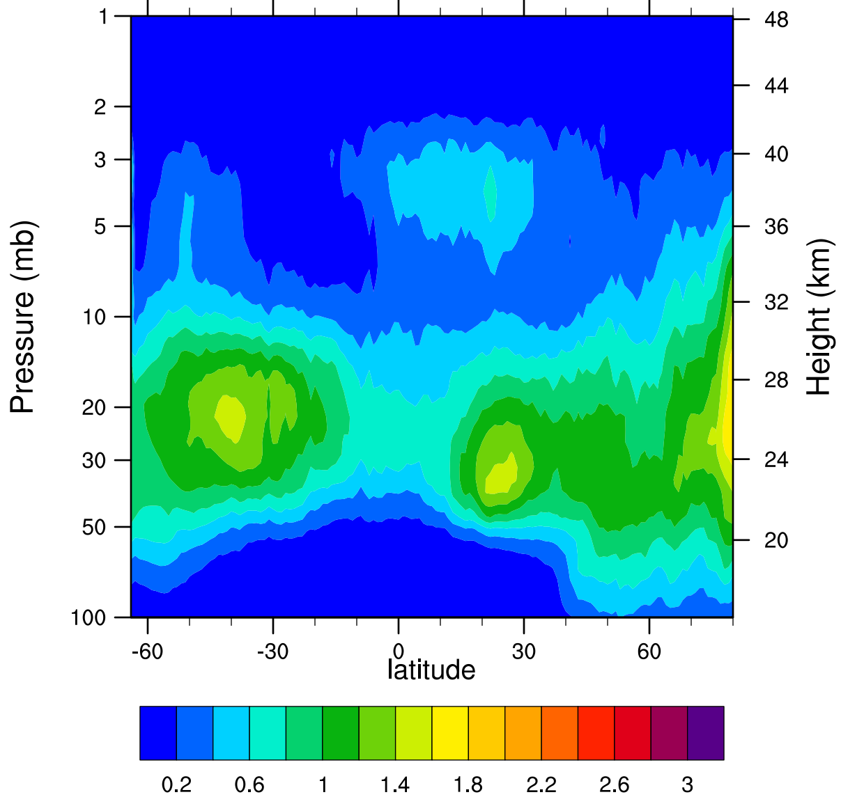
HIRDLSv6 2007d038 ClONO2_Ascending (ppbv)
