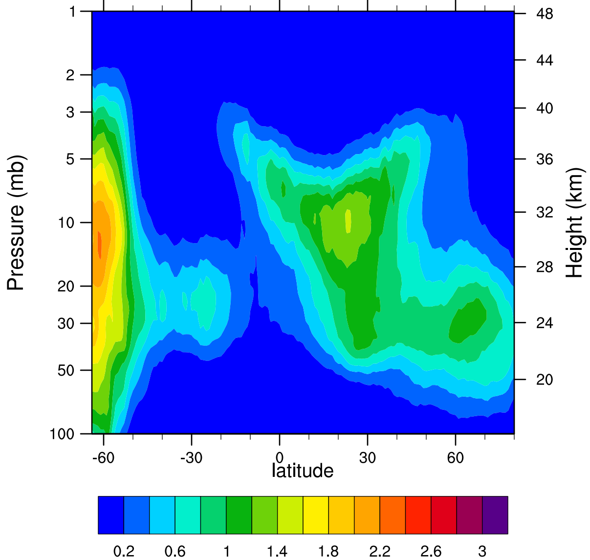
HIRDLSv6 2005d124 ClONO2_Ascending (ppbv)
