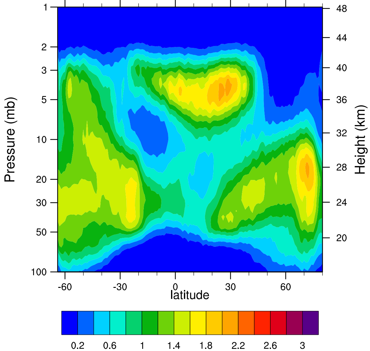
HIRDLSv6 2007d310 ClONO2_Ascending (ppbv)
