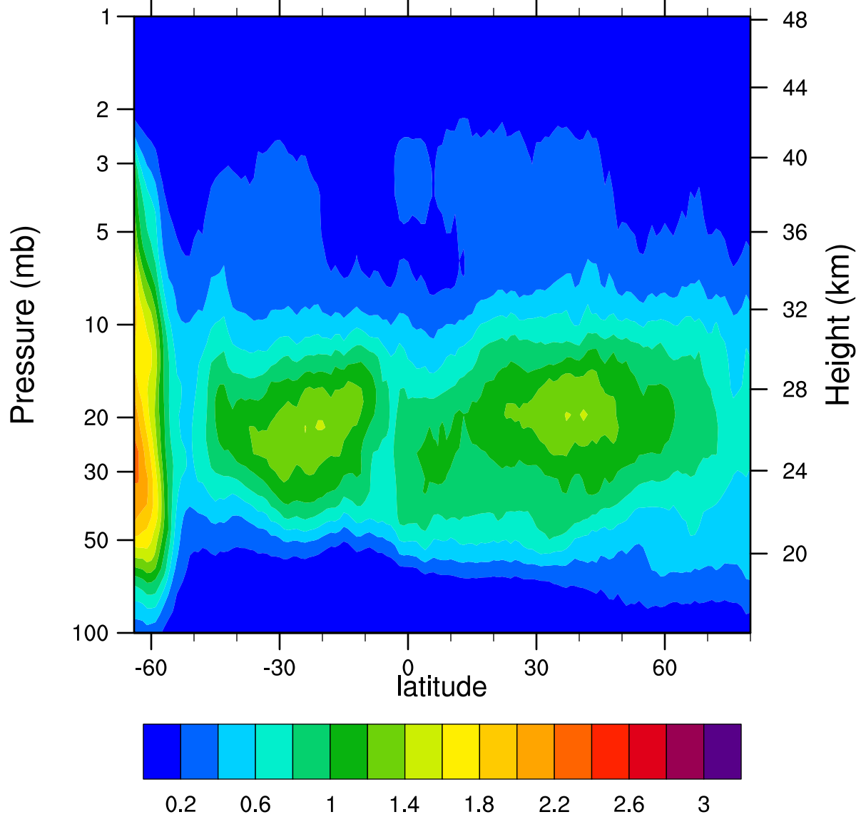
HIRDLSv6 2006d254 ClONO2_Ascending (ppbv)
