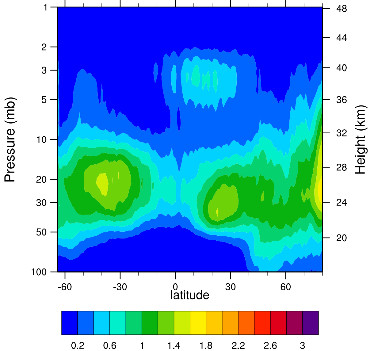
HIRDLSv6 2007d034 ClONO2_Ascending (ppbv)
