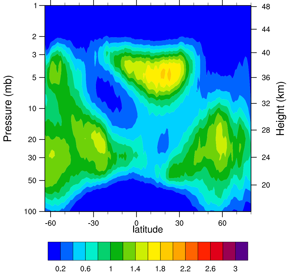
HIRDLSv6 2007d351 ClONO2_Ascending (ppbv)
