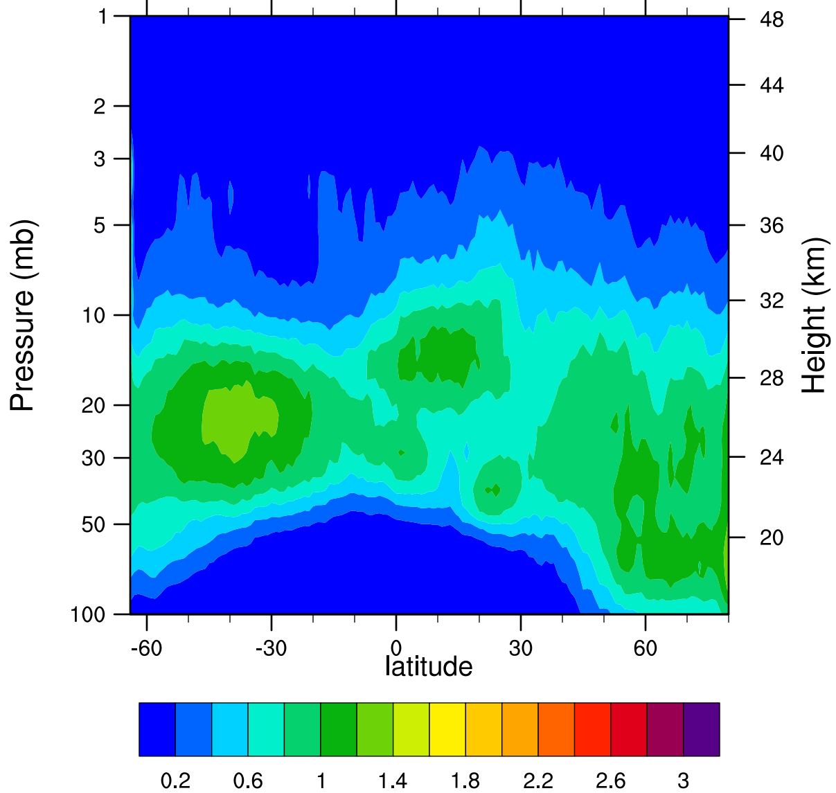
HIRDLSv6 2006d044 ClONO2_Ascending (ppbv)
