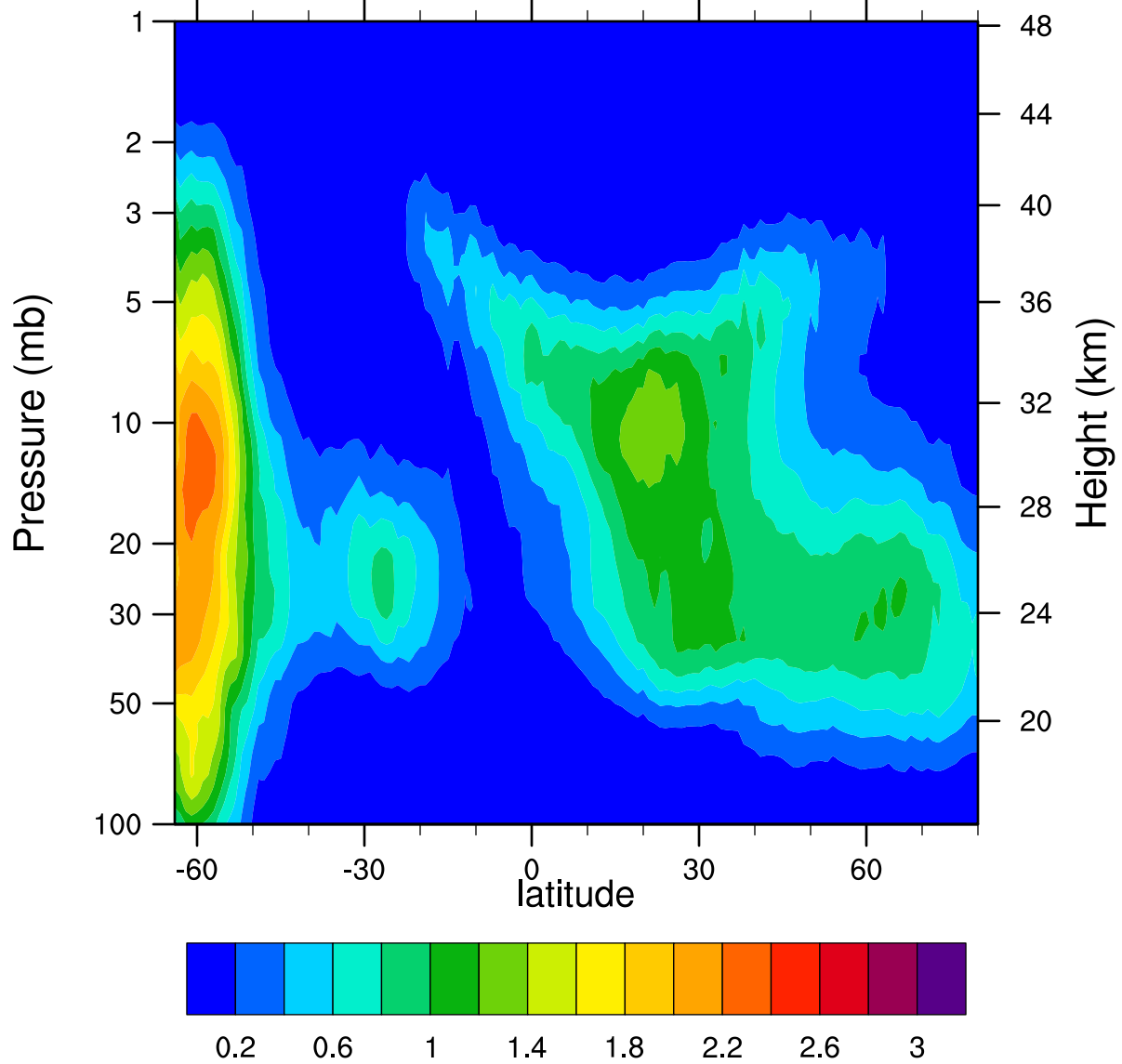
HIRDLSv6 2005d141 ClONO2_Ascending (ppbv)
