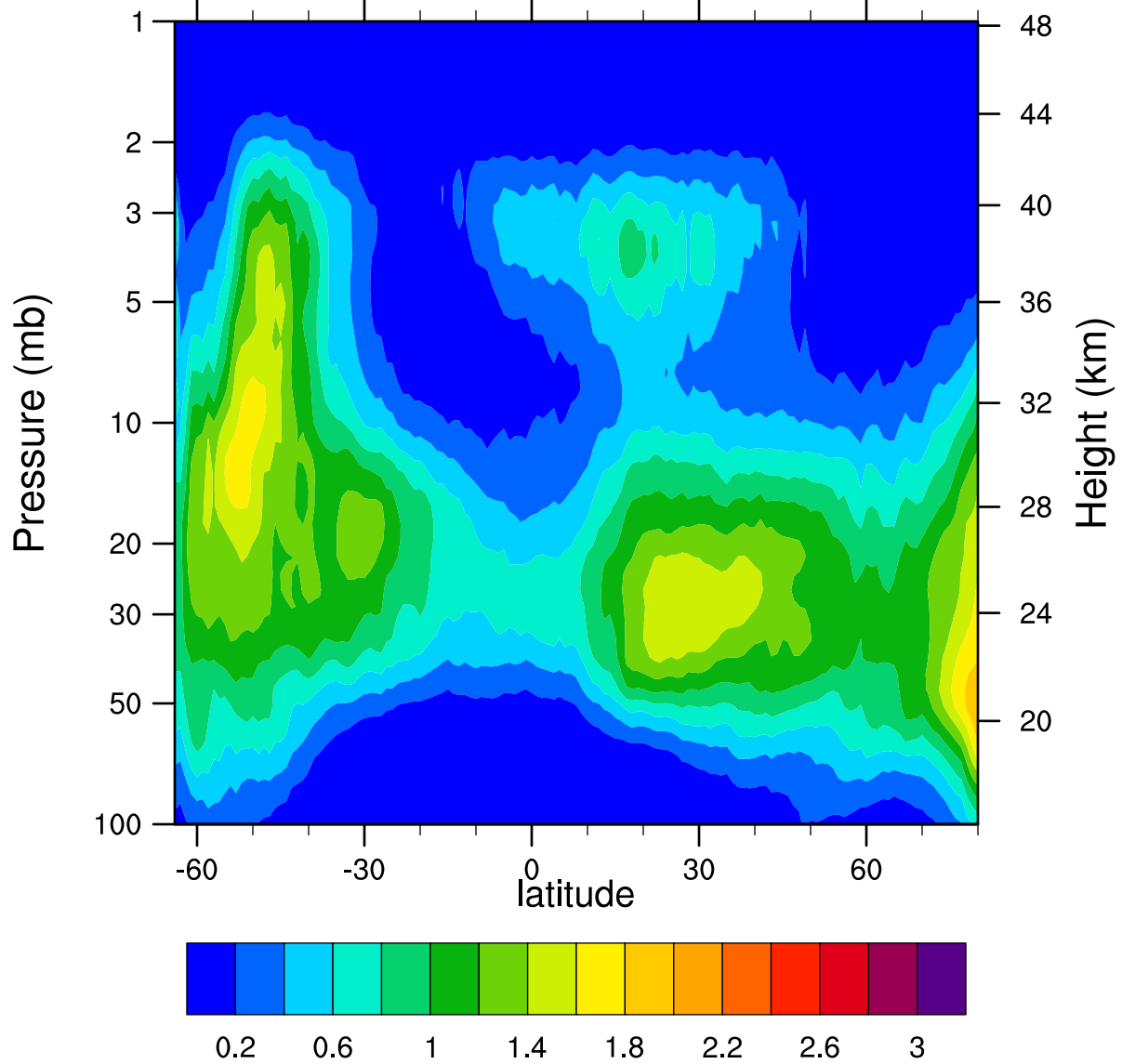
HIRDLSv6 2007d108 ClONO2_Ascending (ppbv)
