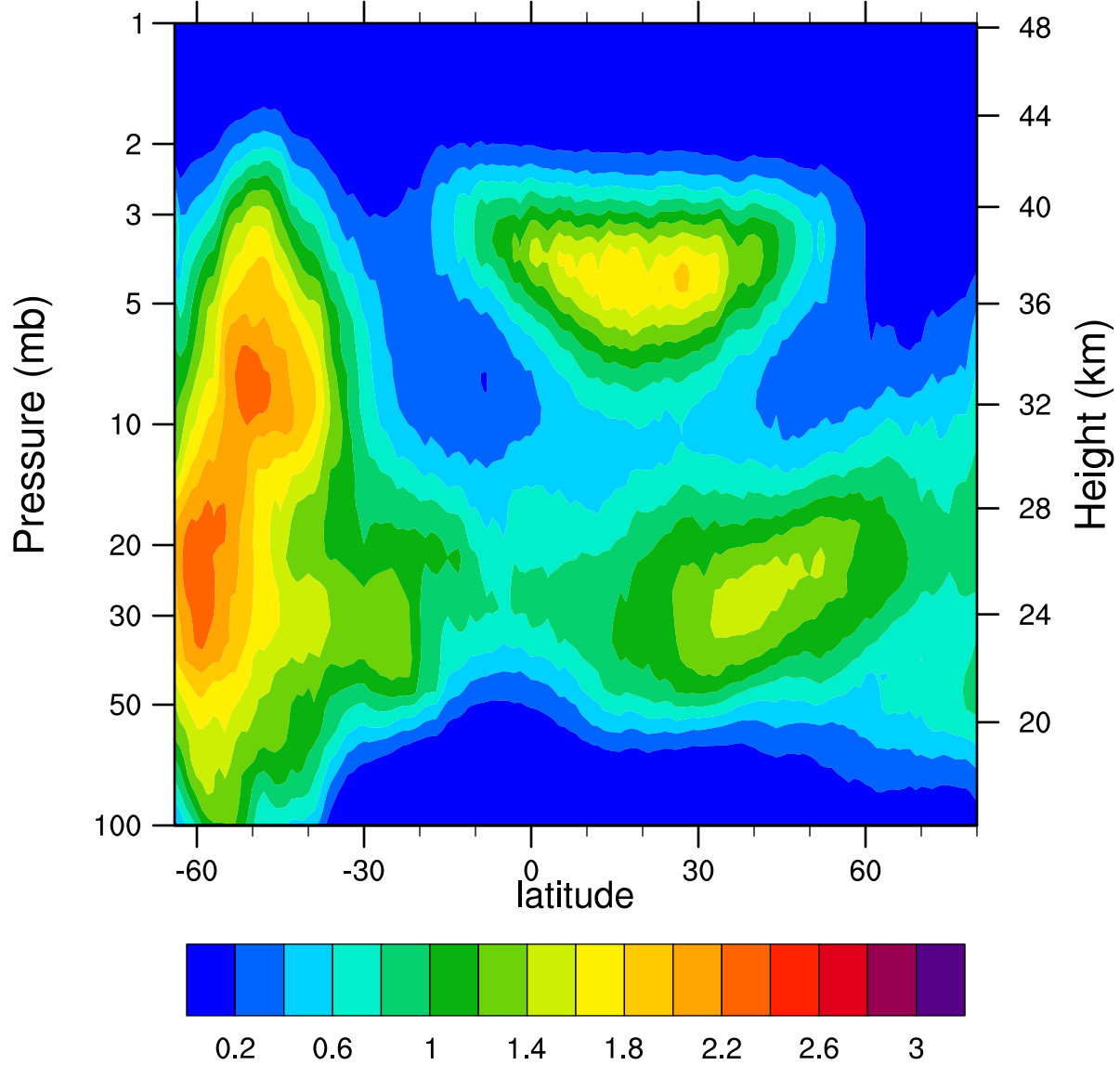
HIRDLSv6 2007d220 ClONO2_Ascending (ppbv)
