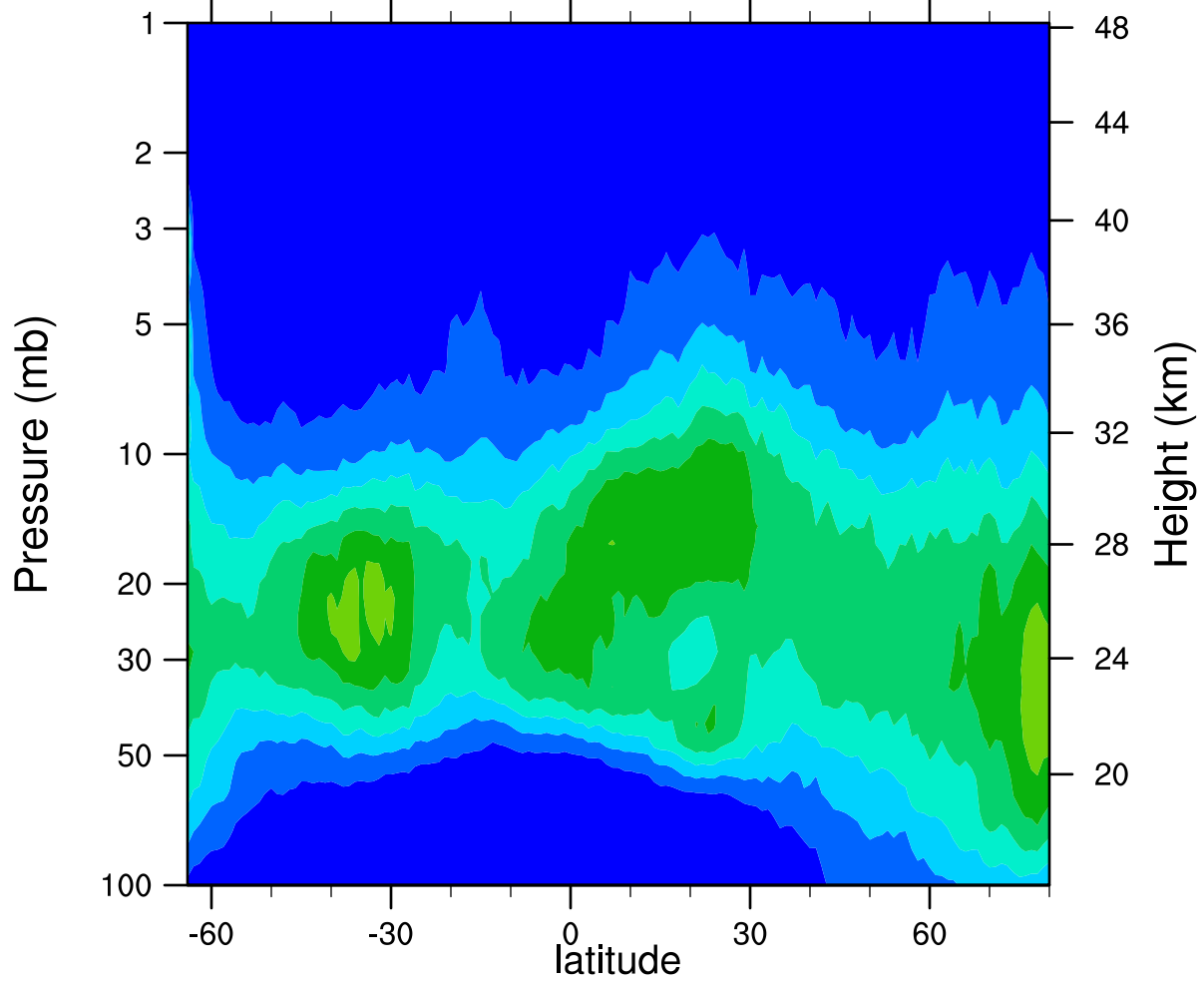
HIRDLSv6 2006d070 ClONO2_Ascending (ppbv)
