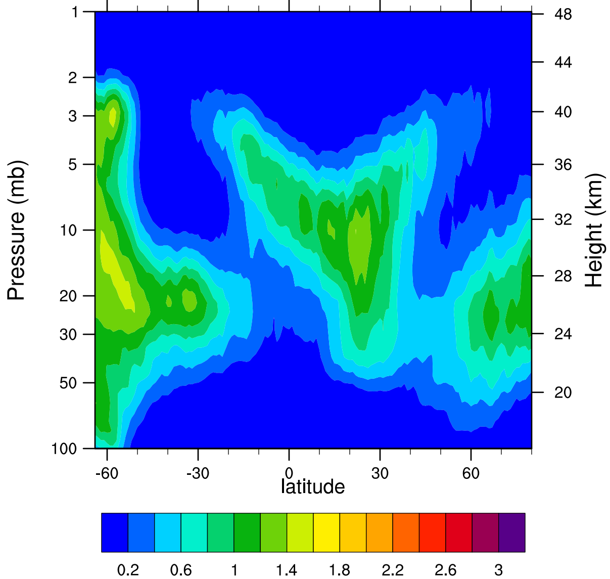
HIRDLSv6 2005d035 ClONO2_Ascending (ppbv)
