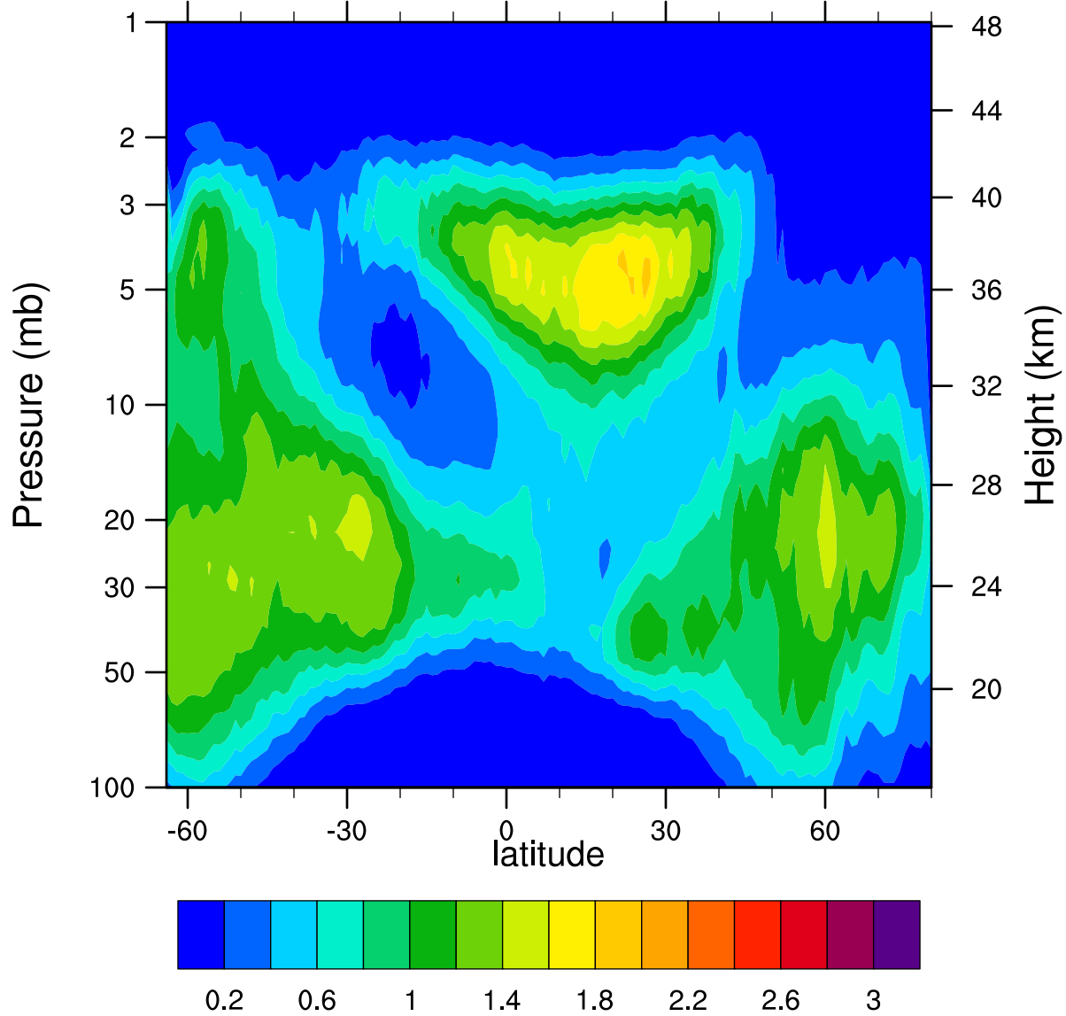
HIRDLSv6 2007d360 ClONO2_Ascending (ppbv)
