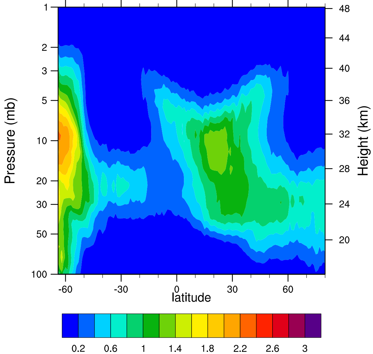
HIRDLSv6 2005d116 ClONO2_Ascending (ppbv)
