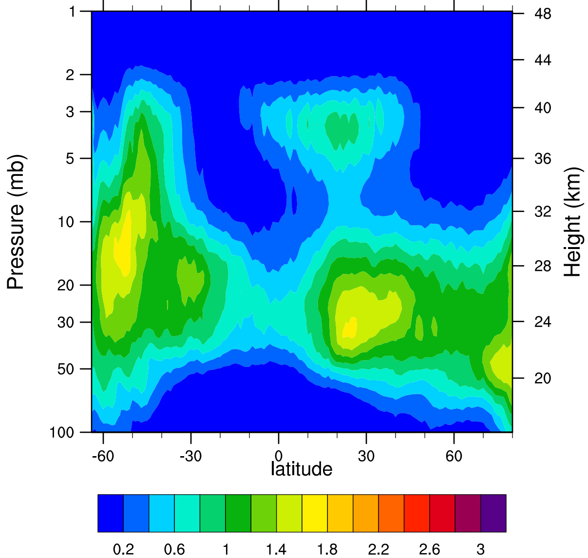
HIRDLSv6 2007d114 ClONO2_Ascending (ppbv)
