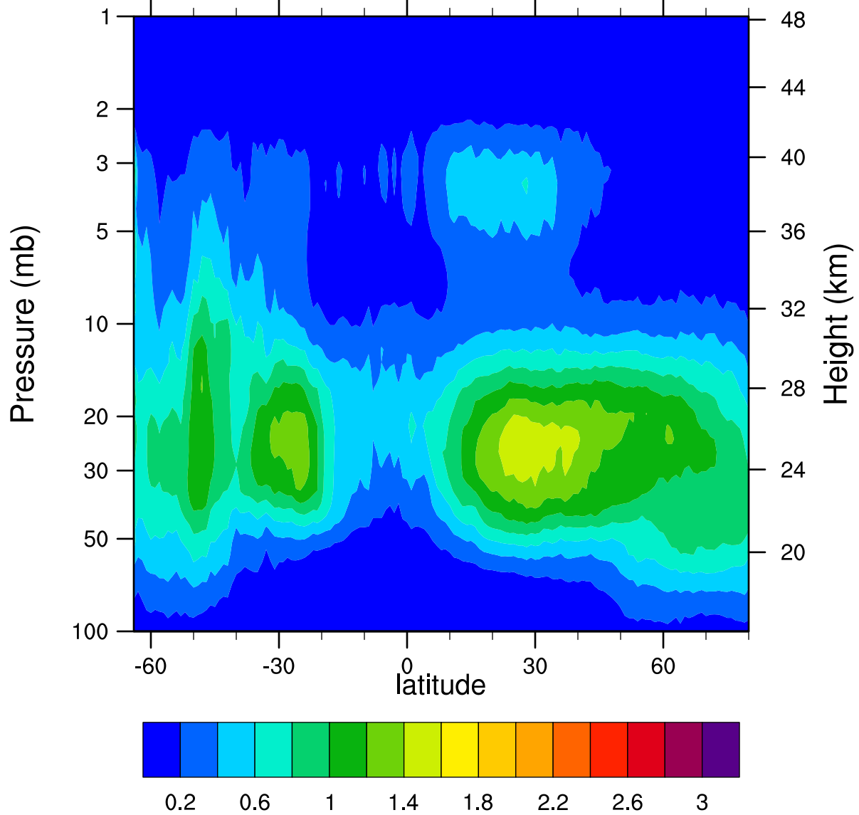
HIRDLSv6 2007d164 ClONO2_Ascending (ppbv)
