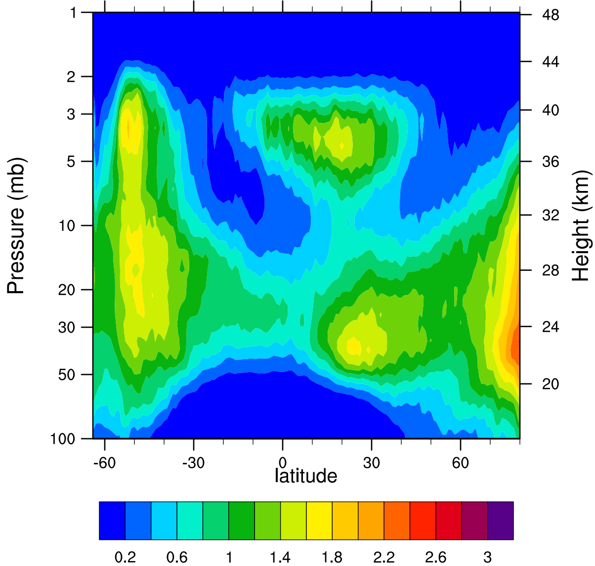
HIRDLSv6 2007d080 ClONO2_Ascending (ppbv)
