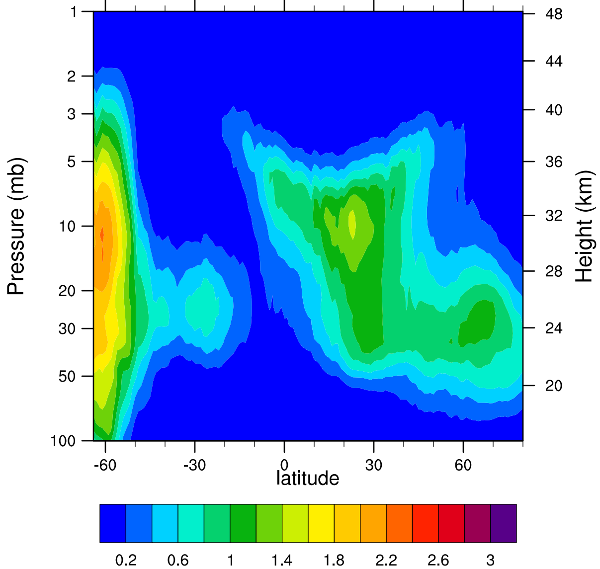
HIRDLSv6 2005d128 ClONO2_Ascending (ppbv)
