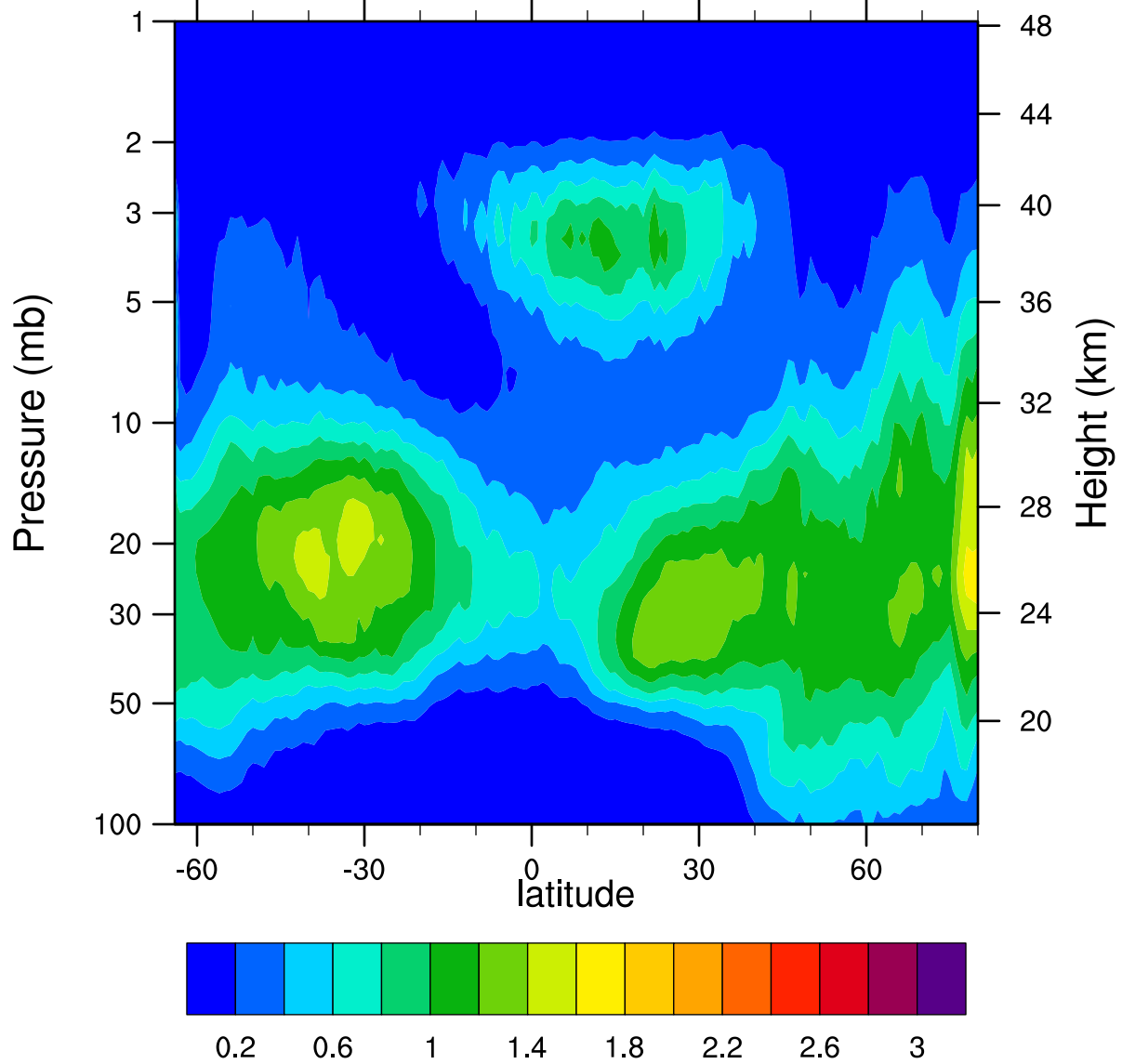
HIRDLSv6 2007d030 ClONO2_Ascending (ppbv)
