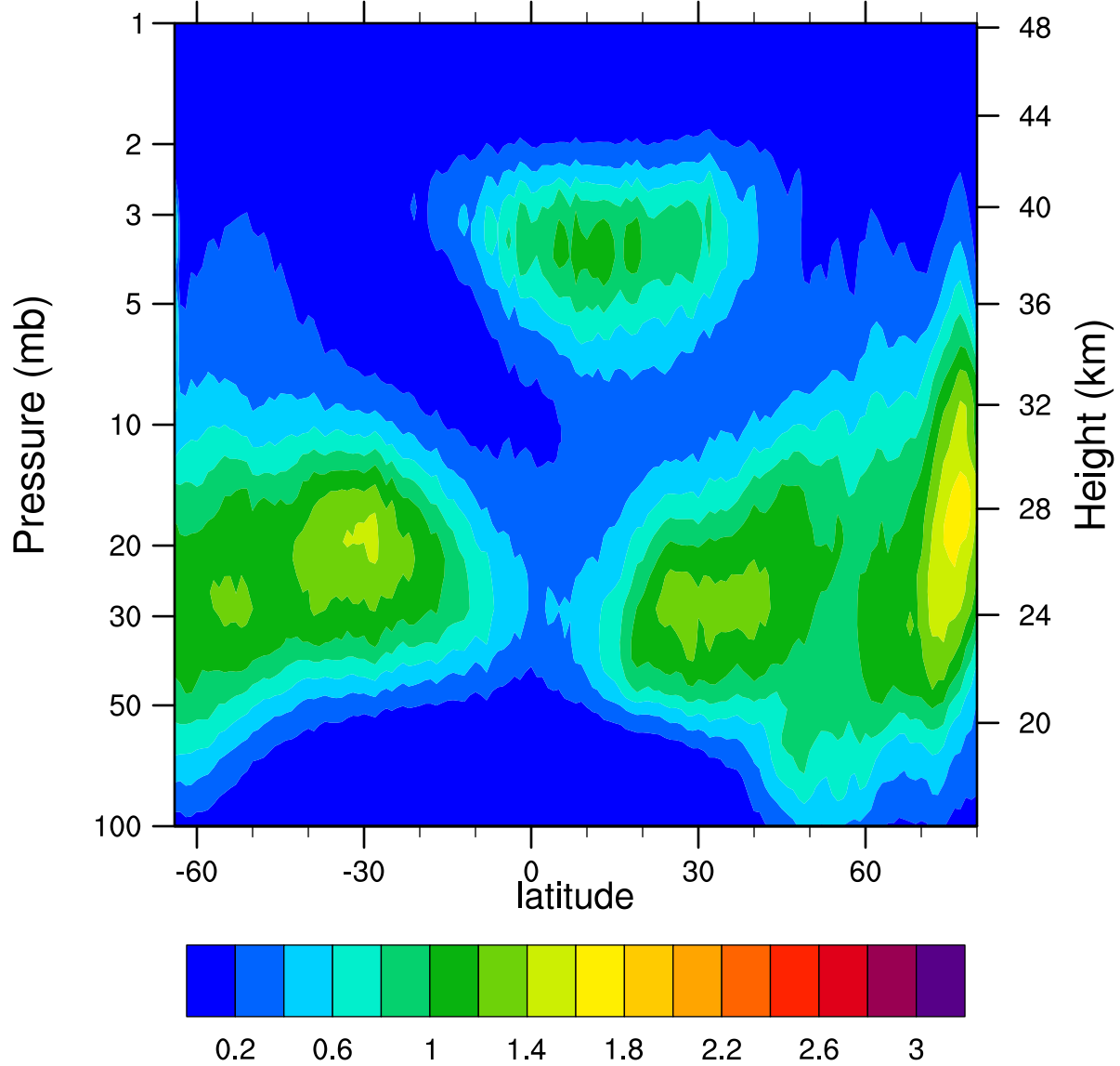
HIRDLSv6 2007d005 ClONO2_Ascending (ppbv)
