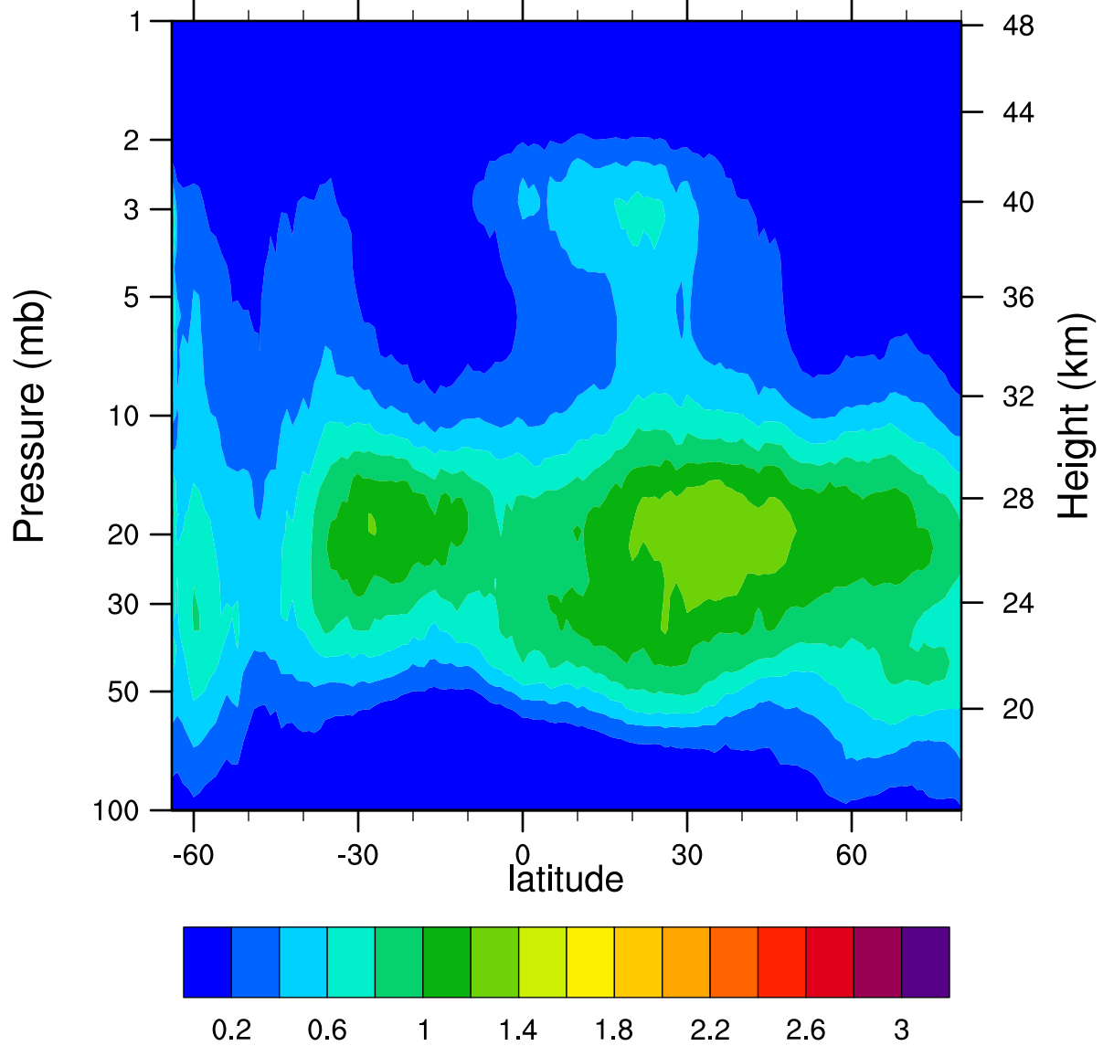
HIRDLSv6 2006d167 ClONO2_Ascending (ppbv)
