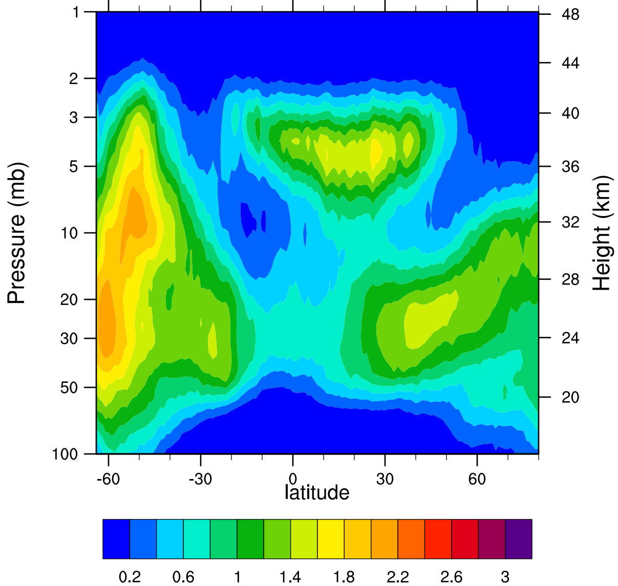
HIRDLSv6 2007d250 ClONO2_Ascending (ppbv)
