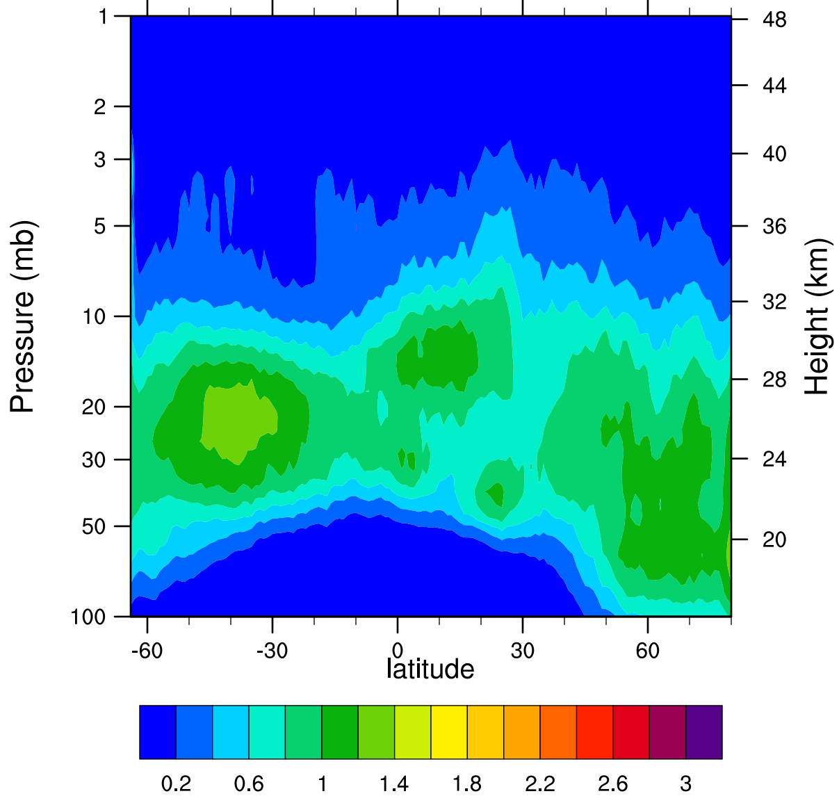
HIRDLSv6 2006d046 ClONO2_Ascending (ppbv)
