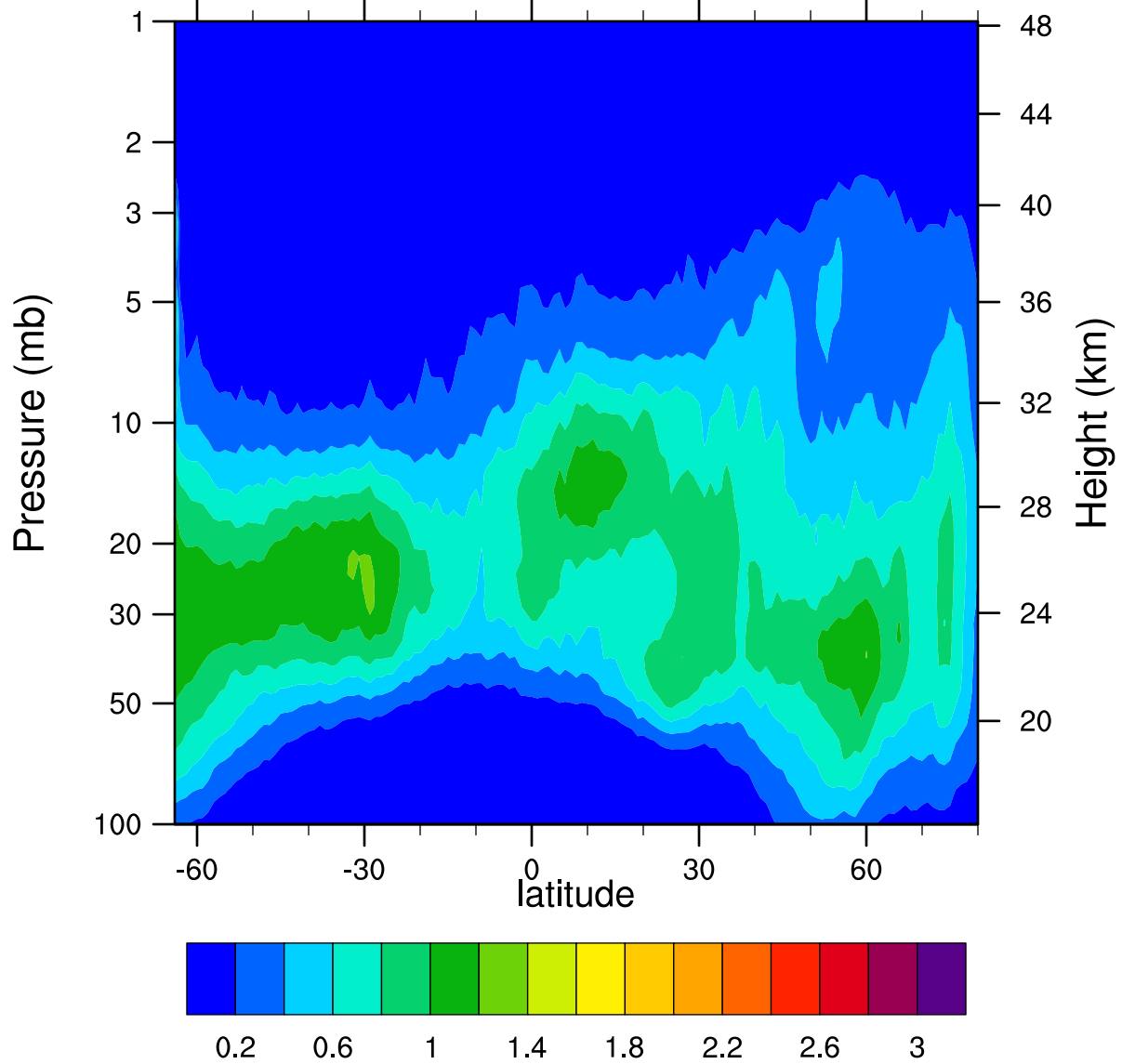
HIRDLSv6 2005d357 ClONO2_Ascending (ppbv)
