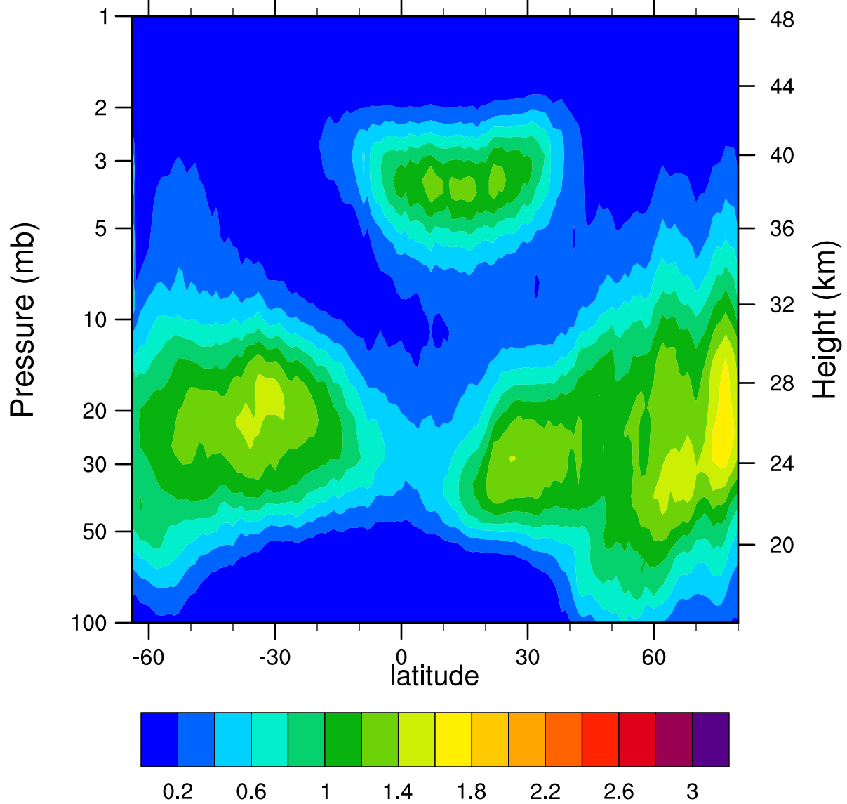
HIRDLSv6 2007d019 ClONO2_Ascending (ppbv)
