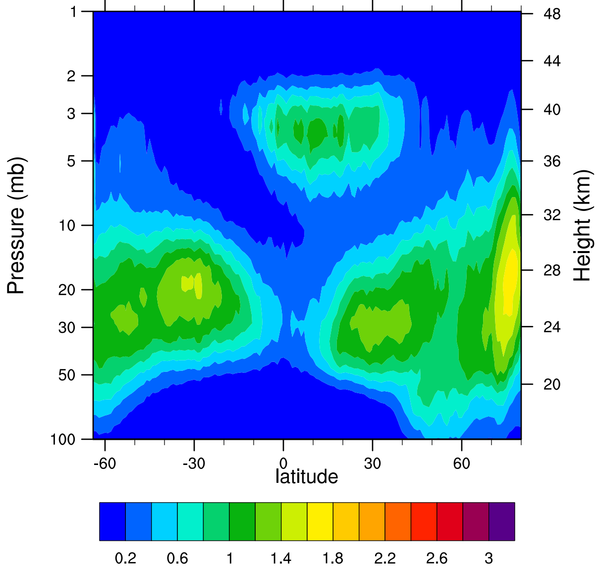
HIRDLSv6 2007d006 ClONO2_Ascending (ppbv)
