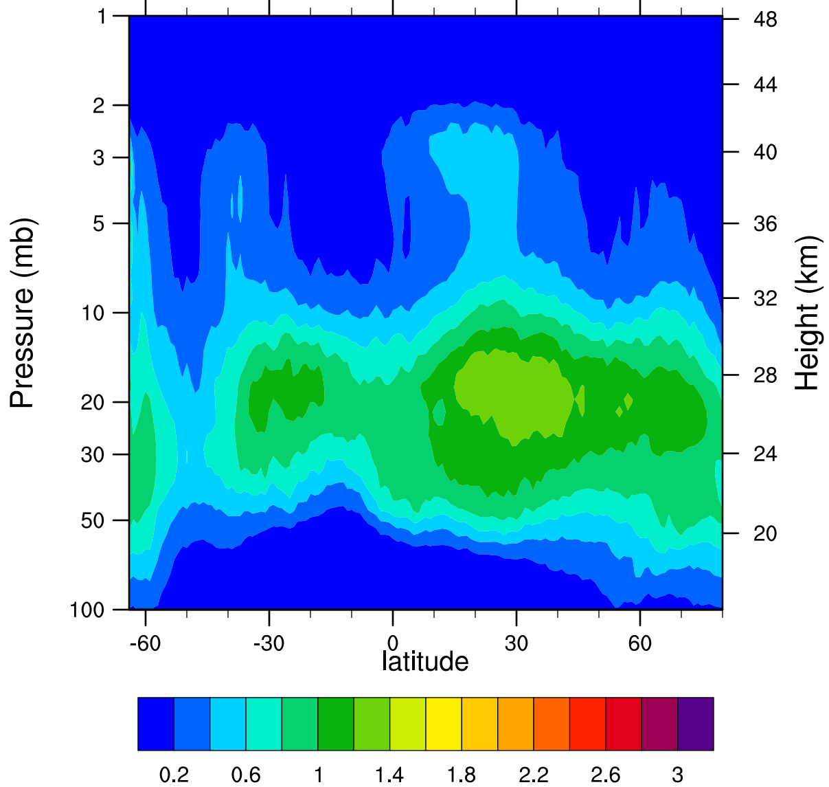
HIRDLSv6 2006d147 ClONO2_Ascending (ppbv)
