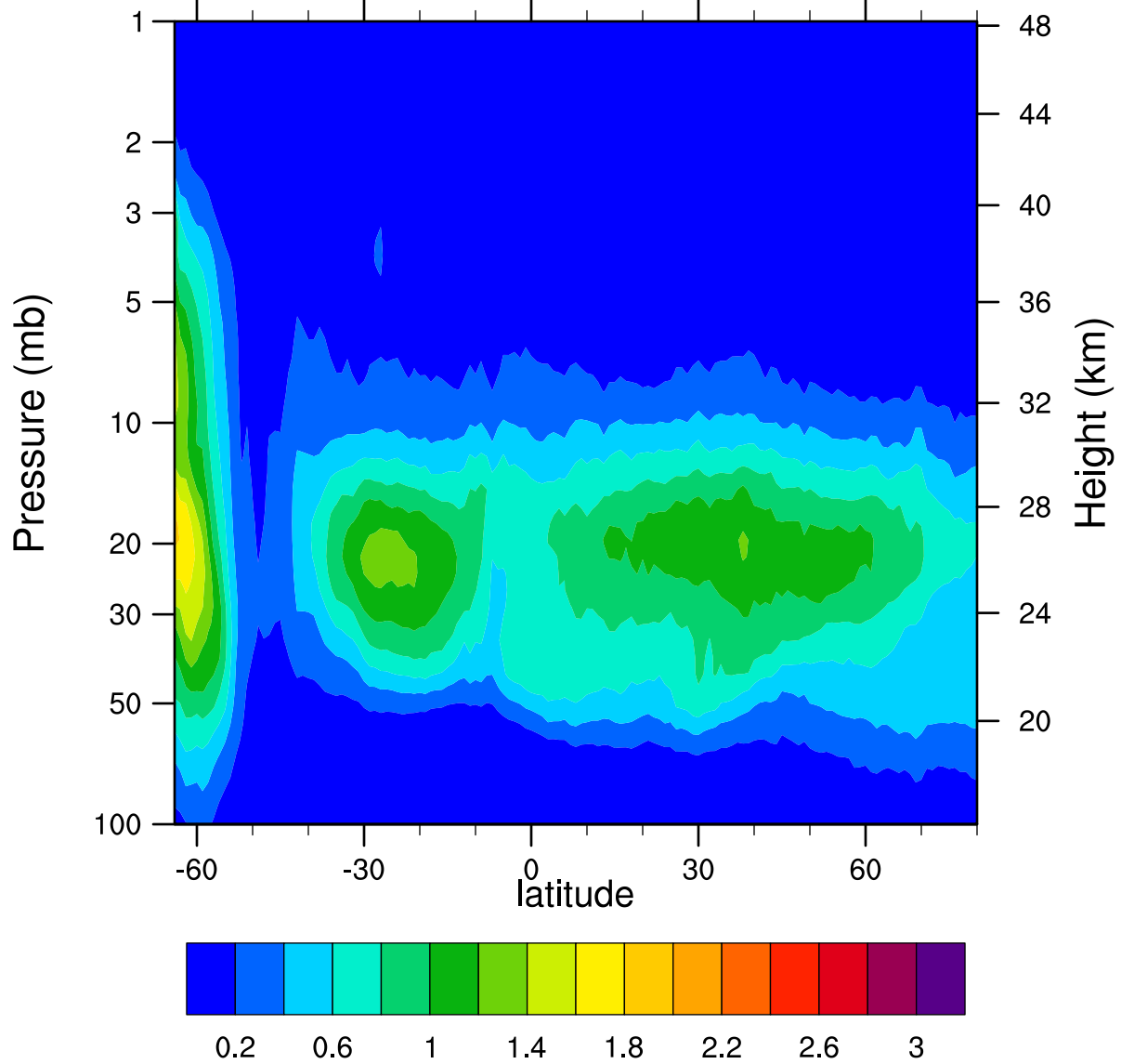
HIRDLSv6 2006d213 ClONO2_Ascending (ppbv)
