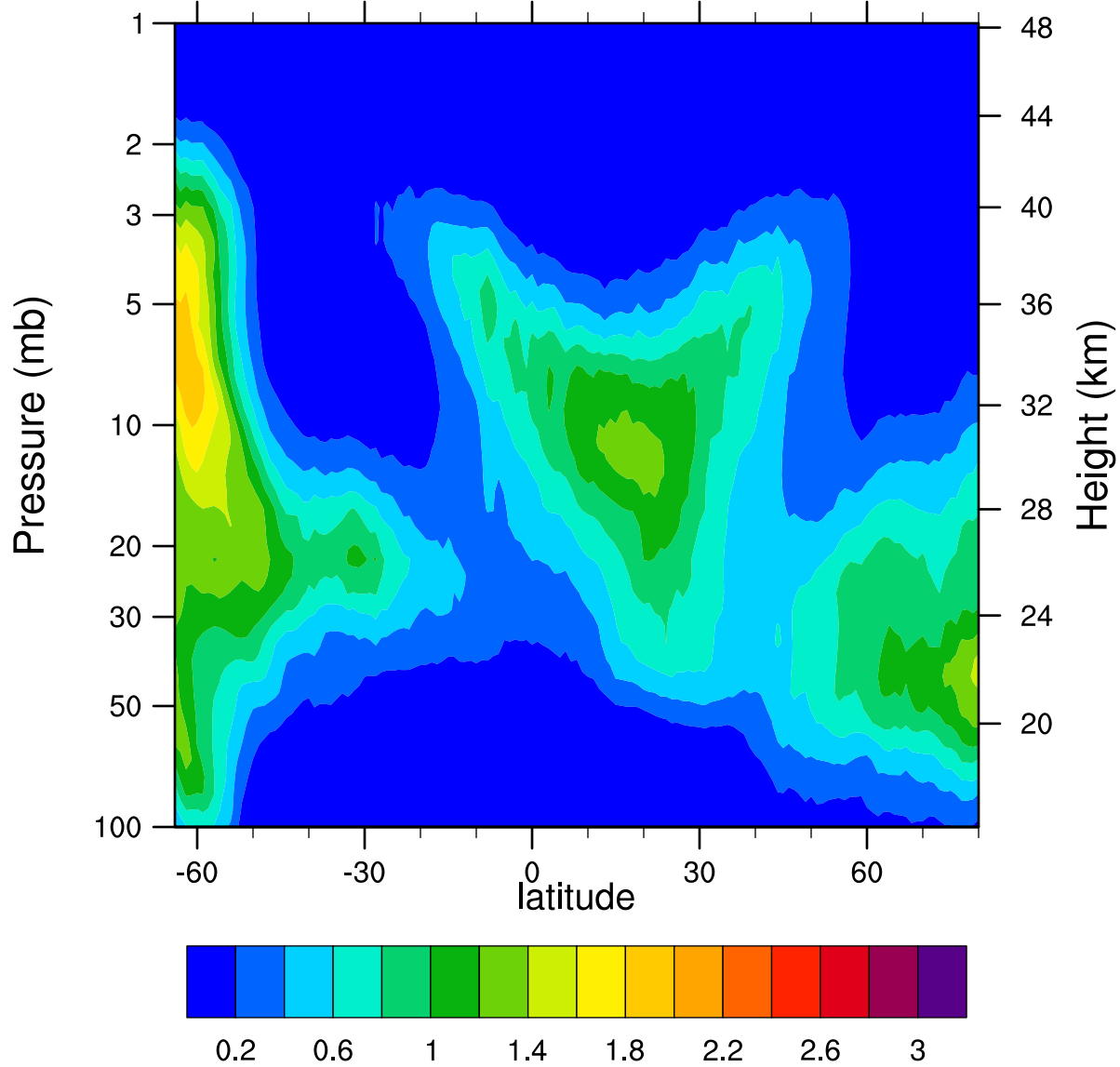
HIRDLSv6 2005d069 ClONO2_Ascending (ppbv)
