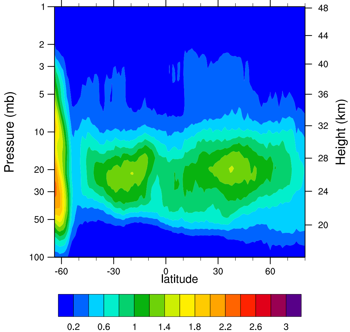
HIRDLSv6 2006d248 ClONO2_Ascending (ppbv)
