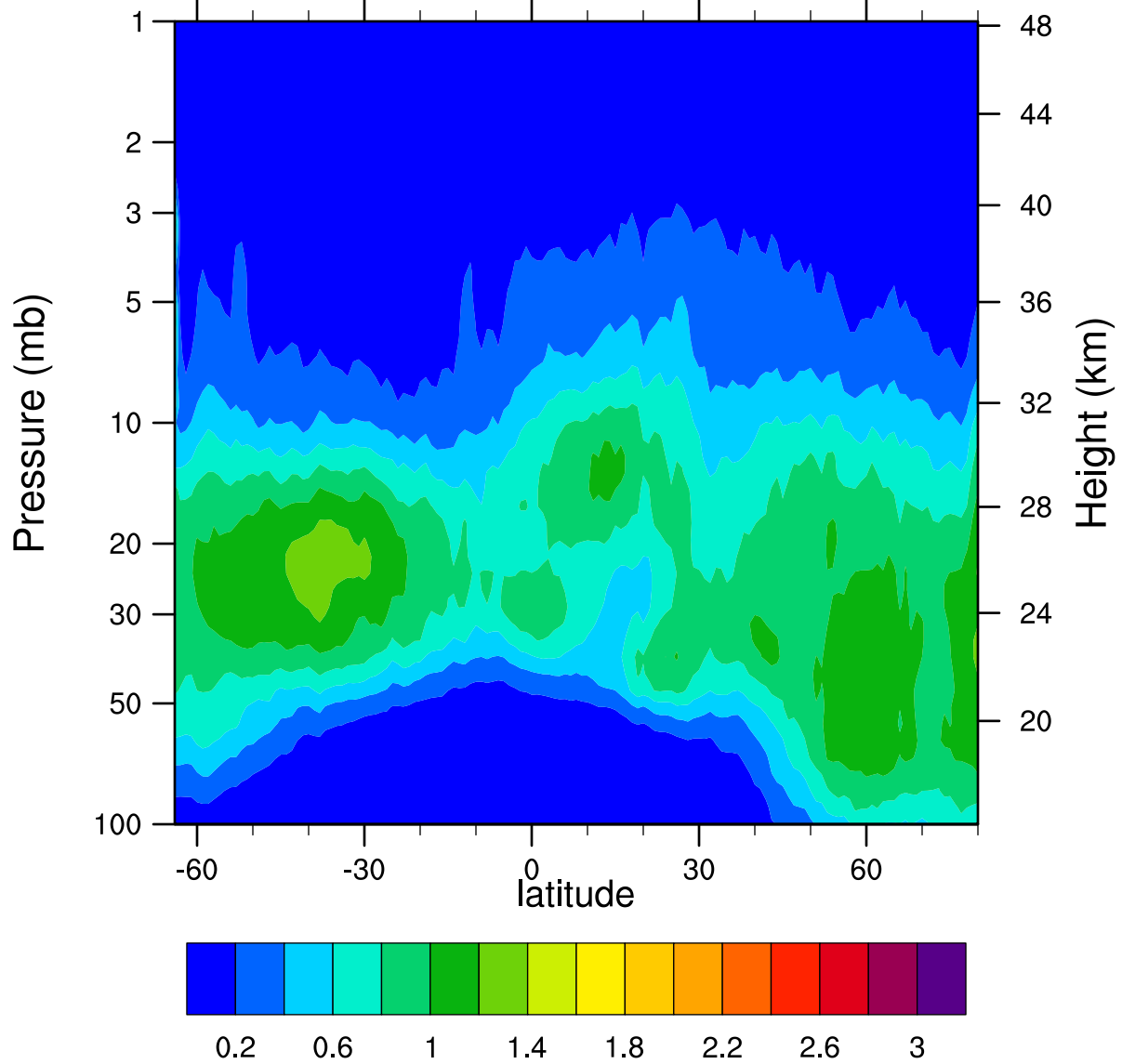
HIRDLSv6 2006d038 ClONO2_Ascending (ppbv)
