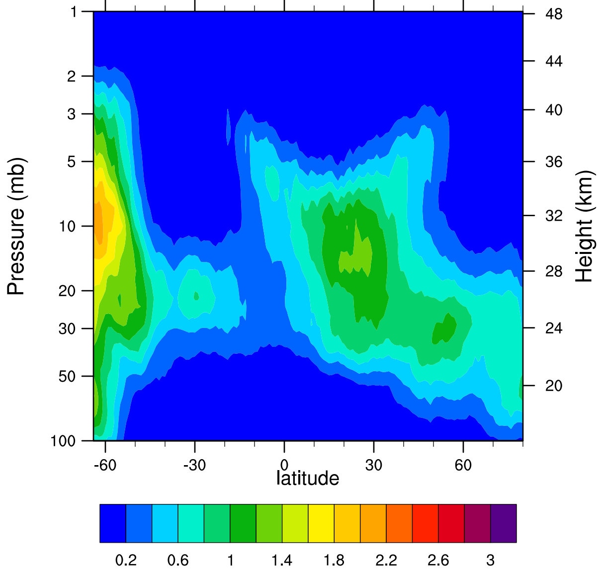
HIRDLSv6 2005d105 ClONO2_Ascending (ppbv)
