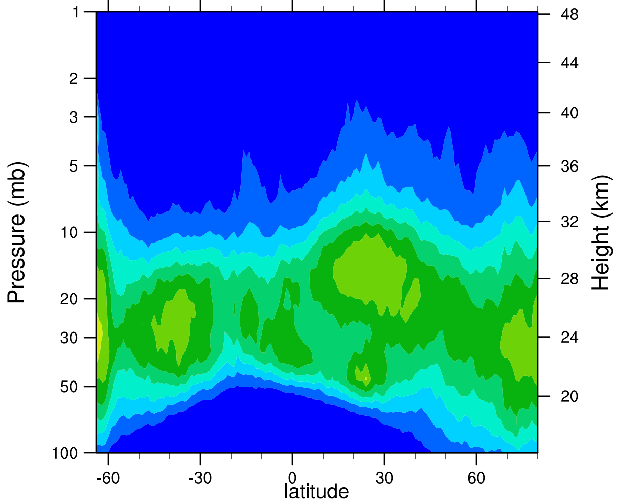
HIRDLSv6 2006d095 ClONO2_Ascending (ppbv)
