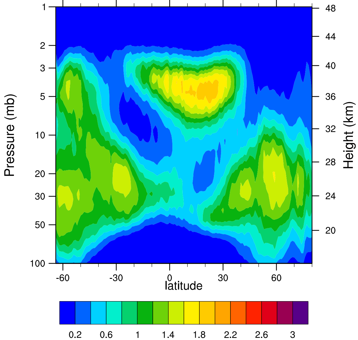
HIRDLSv6 2007d342 ClONO2_Ascending (ppbv)
