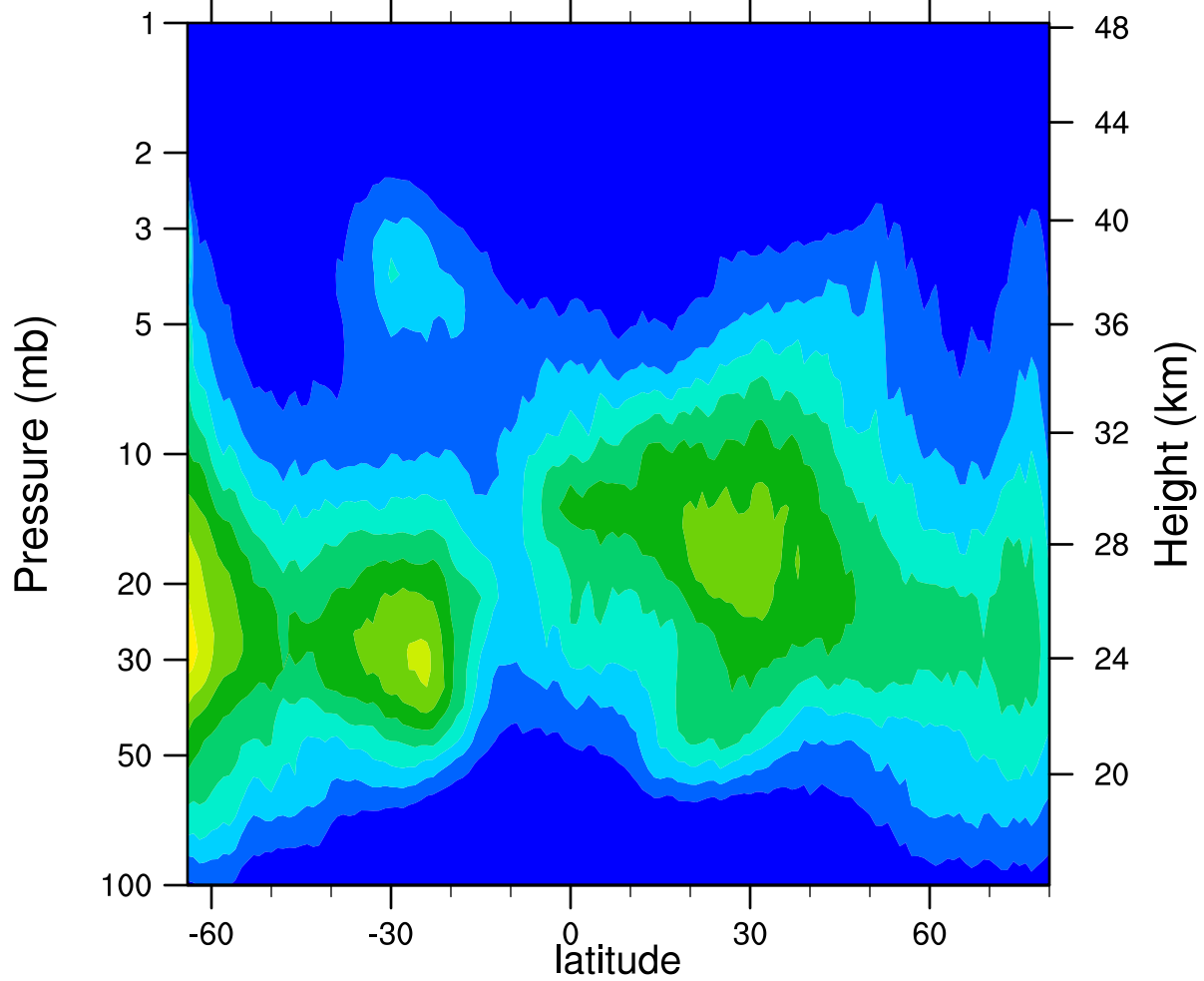
HIRDLSv6 2005d293 ClONO2_Ascending (ppbv)
