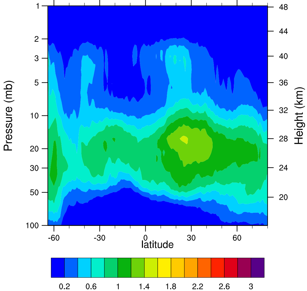
HIRDLSv6 2006d137 ClONO2_Ascending (ppbv)
