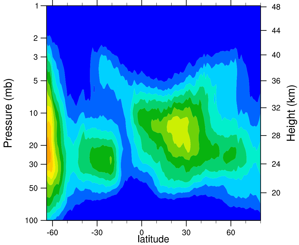
HIRDLSv6 2005d256 ClONO2_Ascending (ppbv)
