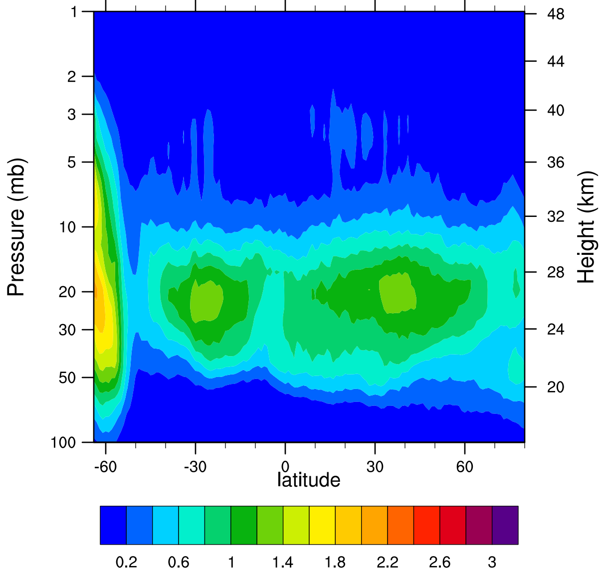
HIRDLSv6 2006d229 ClONO2_Ascending (ppbv)
