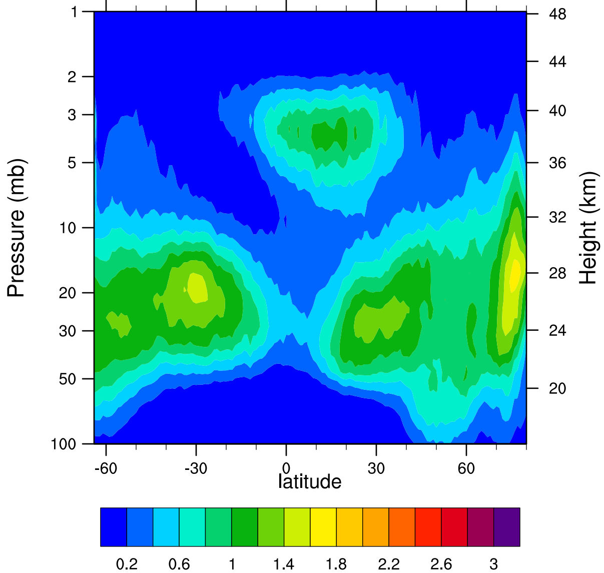
HIRDLSv6 2007d001 ClONO2_Ascending (ppbv)
