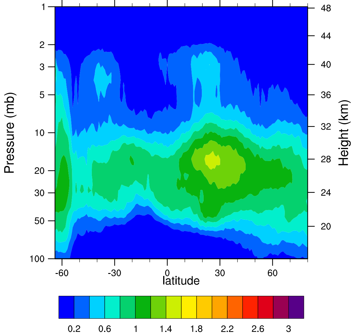
HIRDLSv6 2006d133 ClONO2_Ascending (ppbv)
