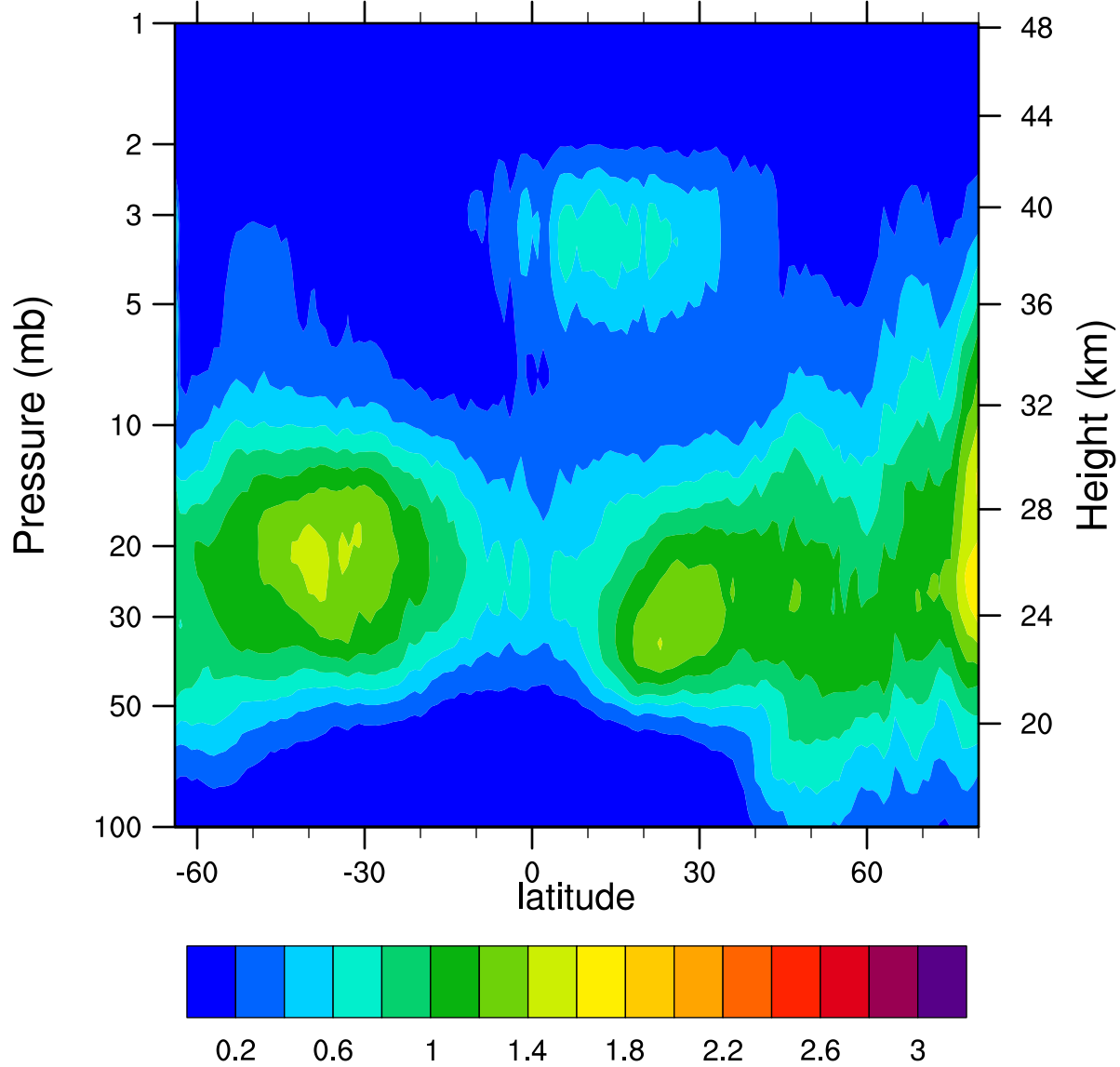
HIRDLSv6 2007d033 ClONO2_Ascending (ppbv)
