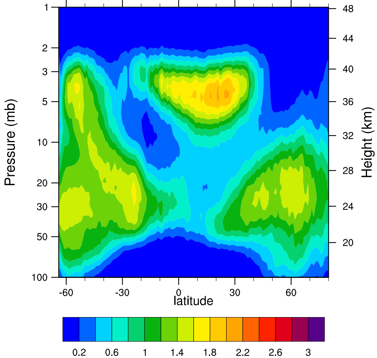
HIRDLSv6 2007d327 ClONO2_Ascending (ppbv)
