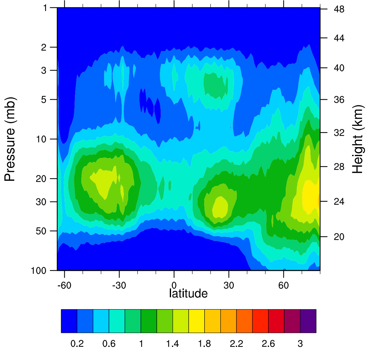
HIRDLSv6 2007d051 ClONO2_Ascending (ppbv)
