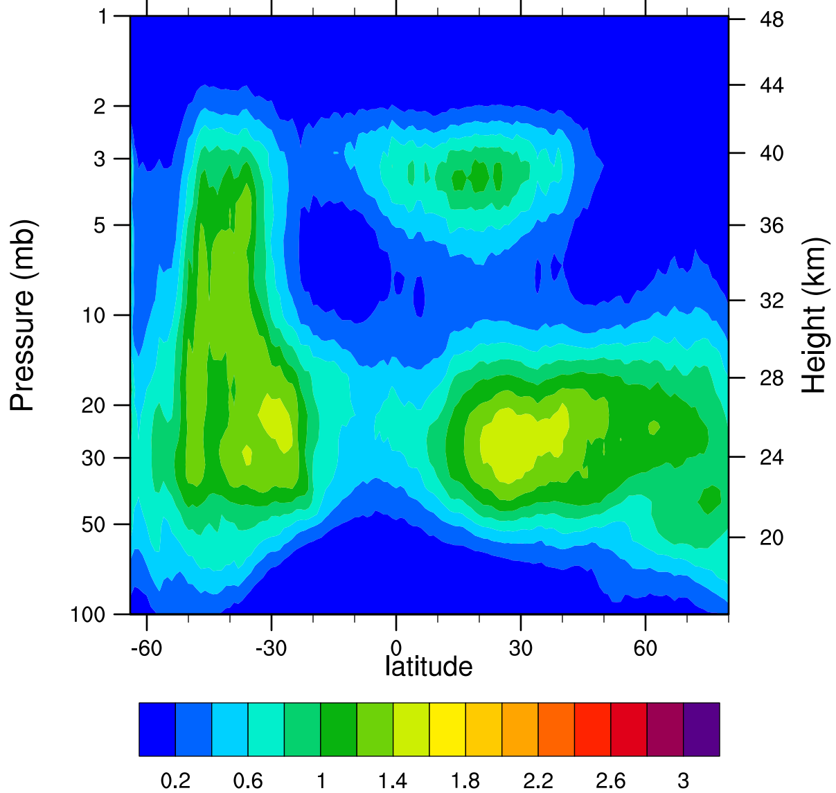
HIRDLSv6 2007d155 ClONO2_Ascending (ppbv)
