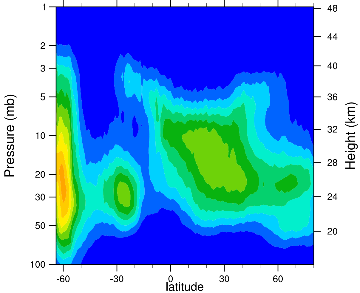
HIRDLSv6 2005d200 ClONO2_Ascending (ppbv)
