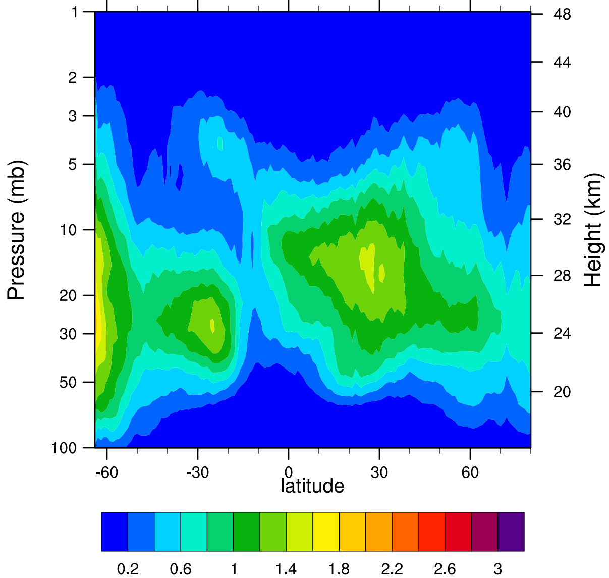
HIRDLSv6 2005d274 ClONO2_Ascending (ppbv)
