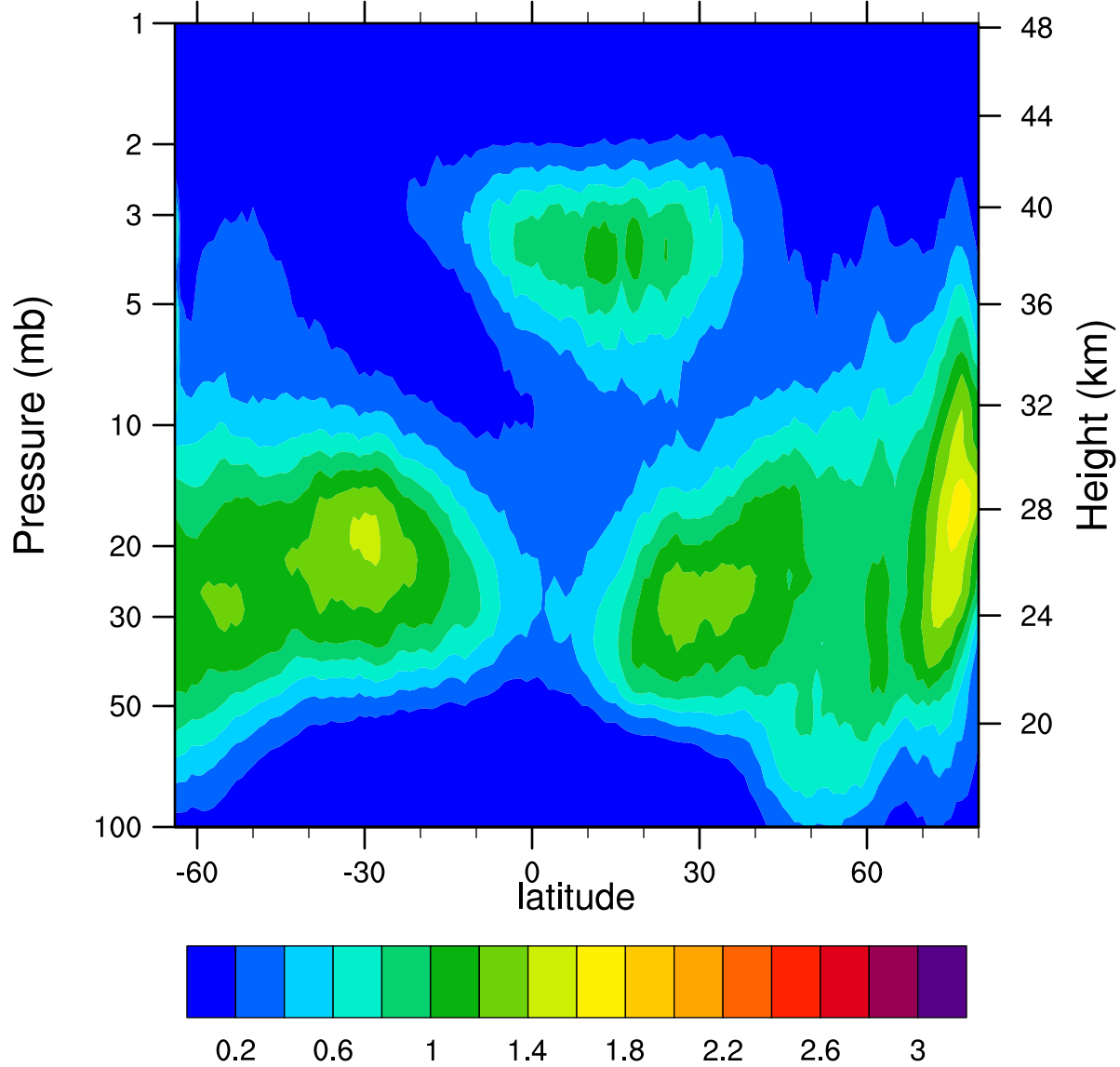
HIRDLSv6 2007d002 ClONO2_Ascending (ppbv)
