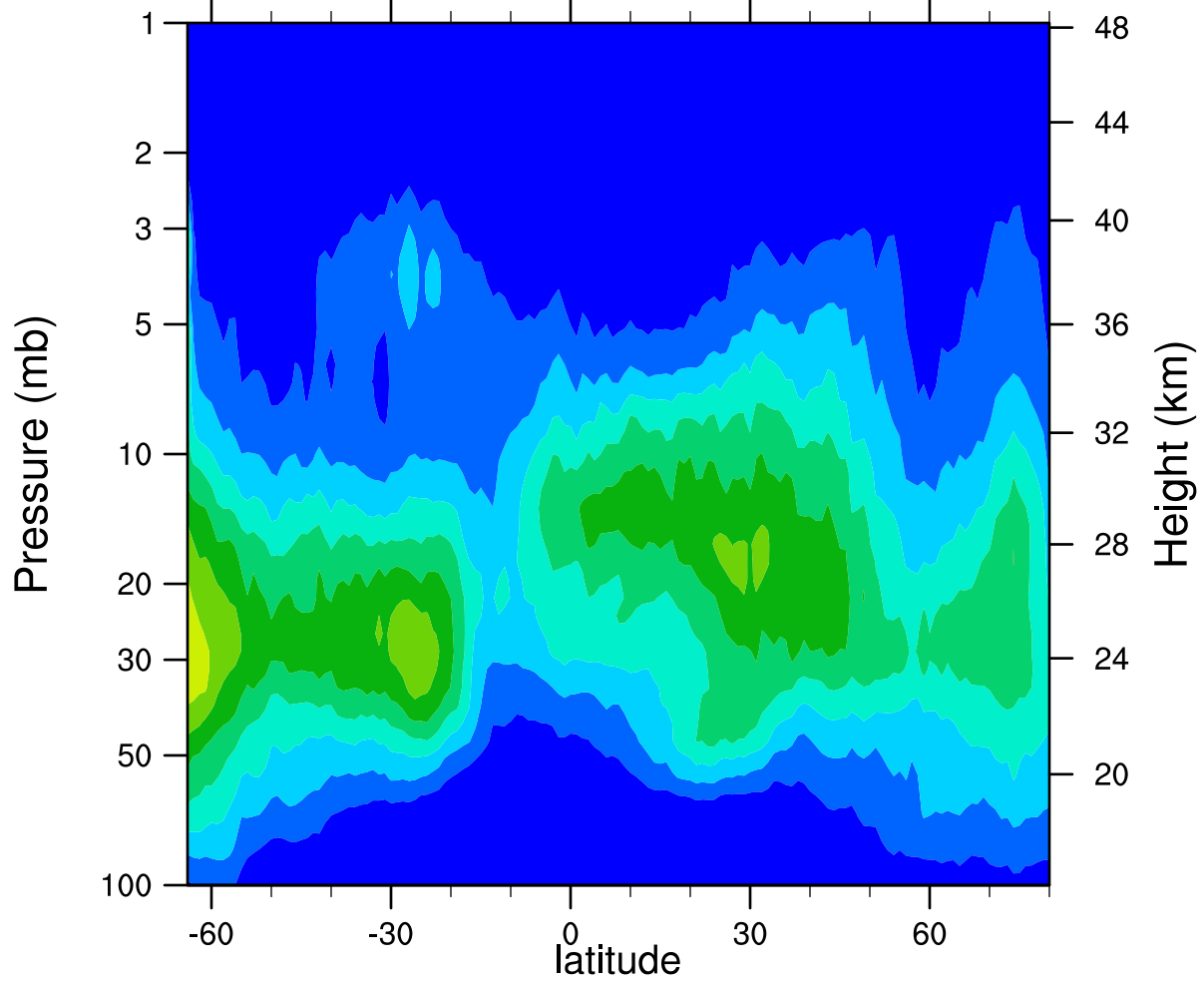
HIRDLSv6 2005d301 ClONO2_Ascending (ppbv)
