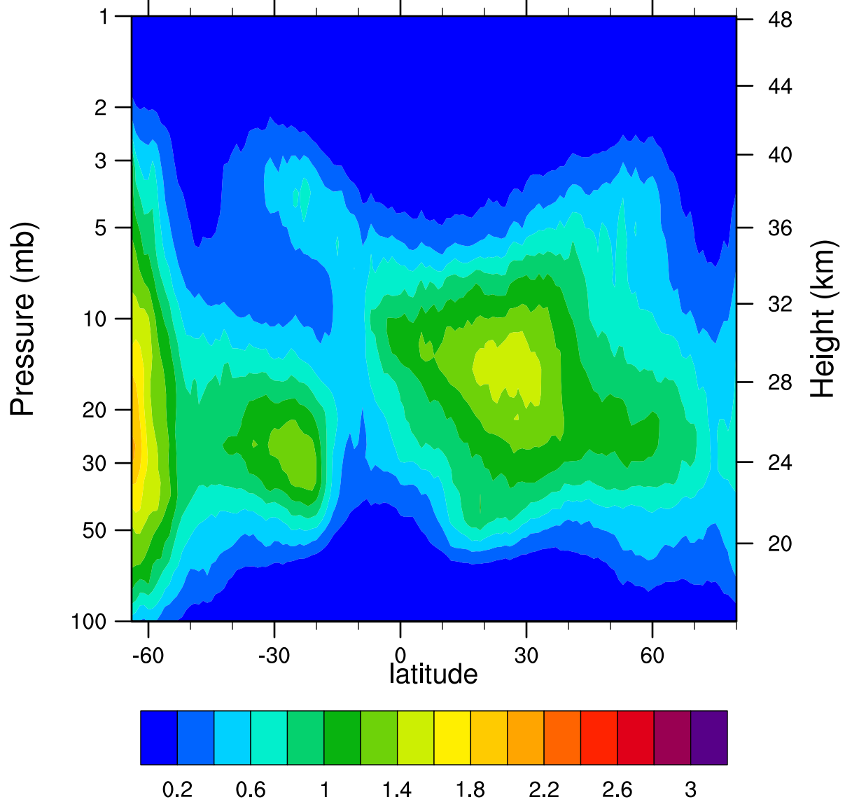
HIRDLSv6 2005d268 ClONO2_Ascending (ppbv)
