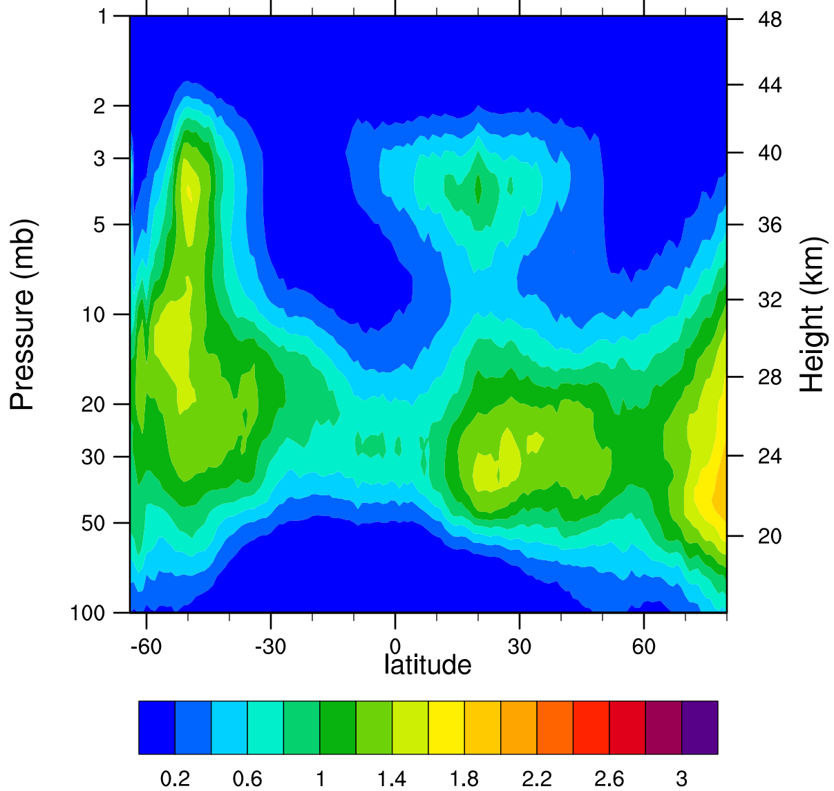
HIRDLSv6 2007d093 ClONO2_Ascending (ppbv)
