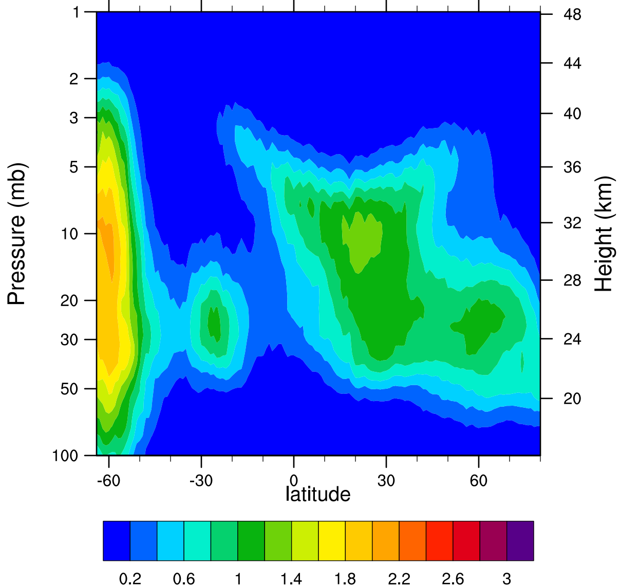
HIRDLSv6 2005d157 ClONO2_Ascending (ppbv)
