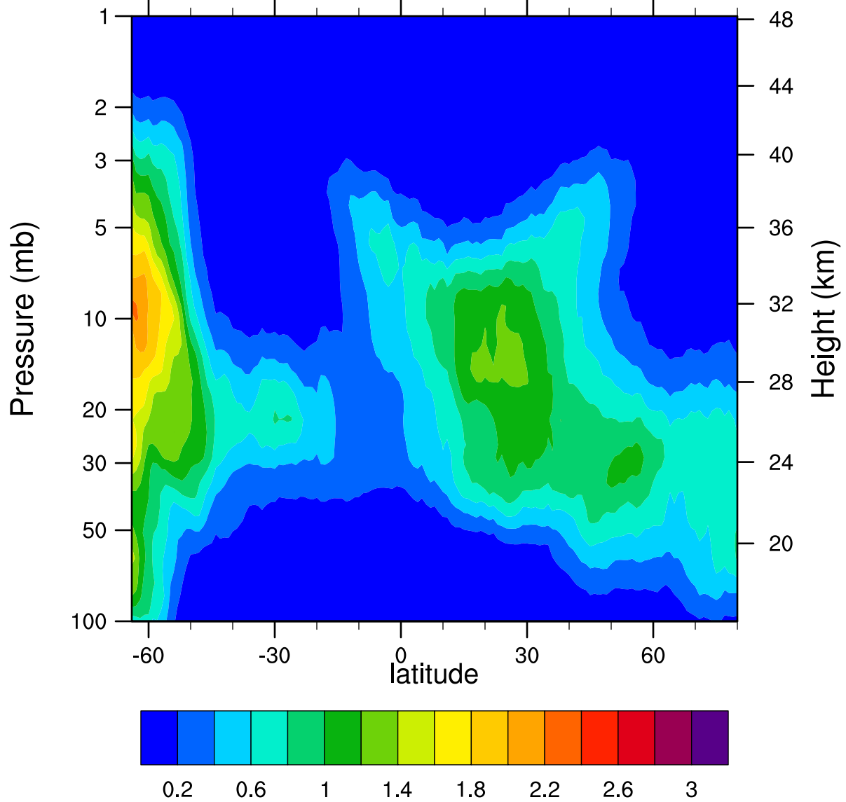
HIRDLSv6 2005d107 ClONO2_Ascending (ppbv)
