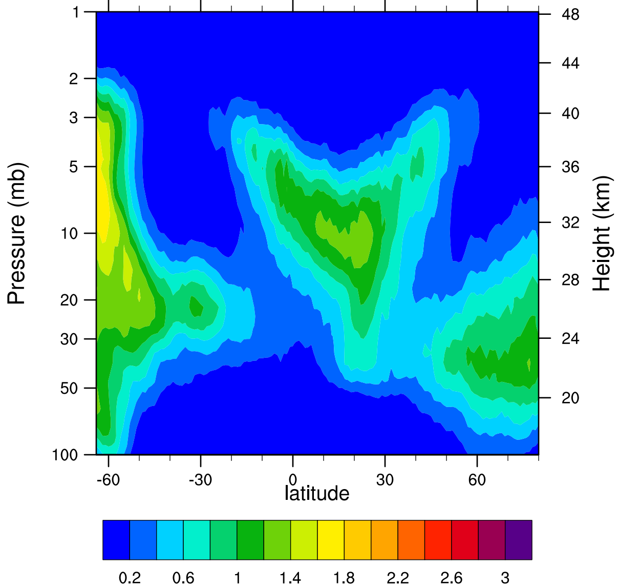
HIRDLSv6 2005d057 ClONO2_Ascending (ppbv)
