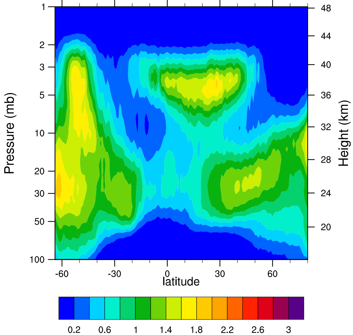
HIRDLSv6 2007d265 ClONO2_Ascending (ppbv)
