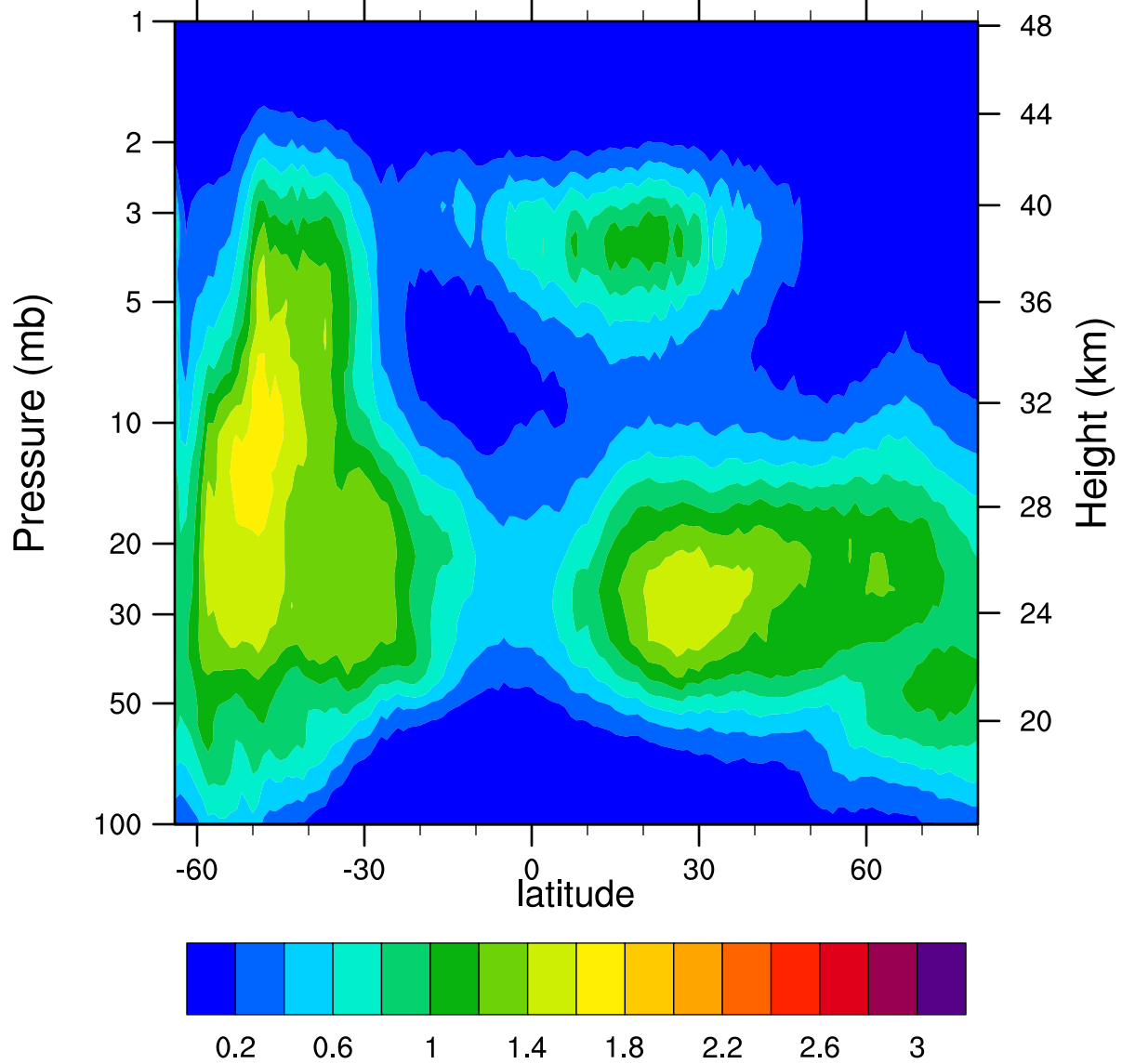
HIRDLSv6 2007d143 ClONO2_Ascending (ppbv)
