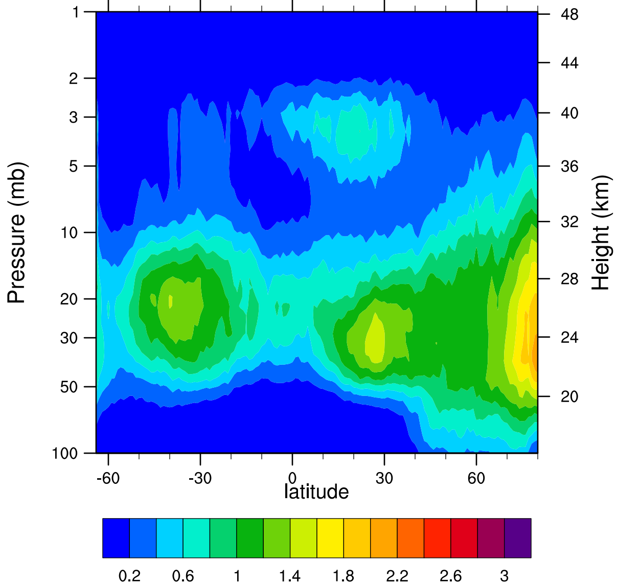
HIRDLSv6 2007d067 ClONO2_Ascending (ppbv)
