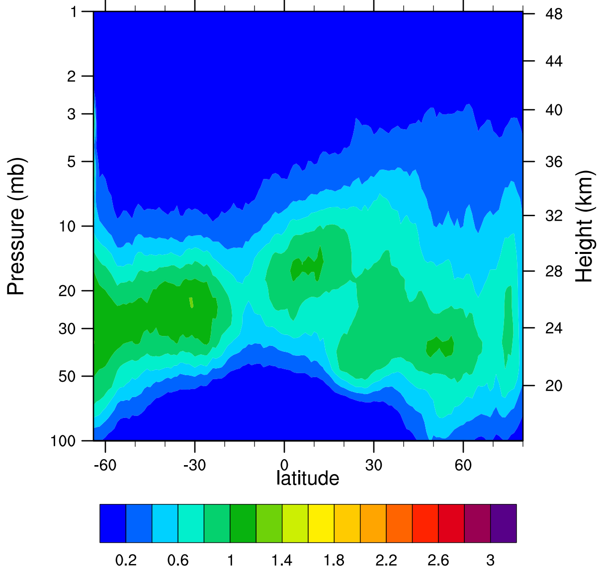
HIRDLSv6 2005d349 ClONO2_Ascending (ppbv)
