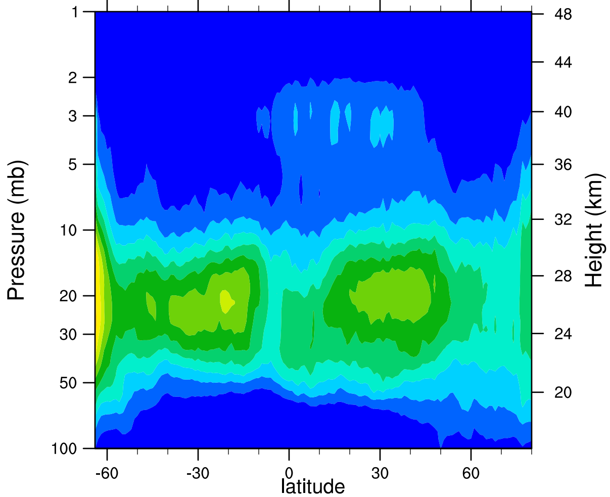
HIRDLSv6 2006d281 ClONO2_Ascending (ppbv)
