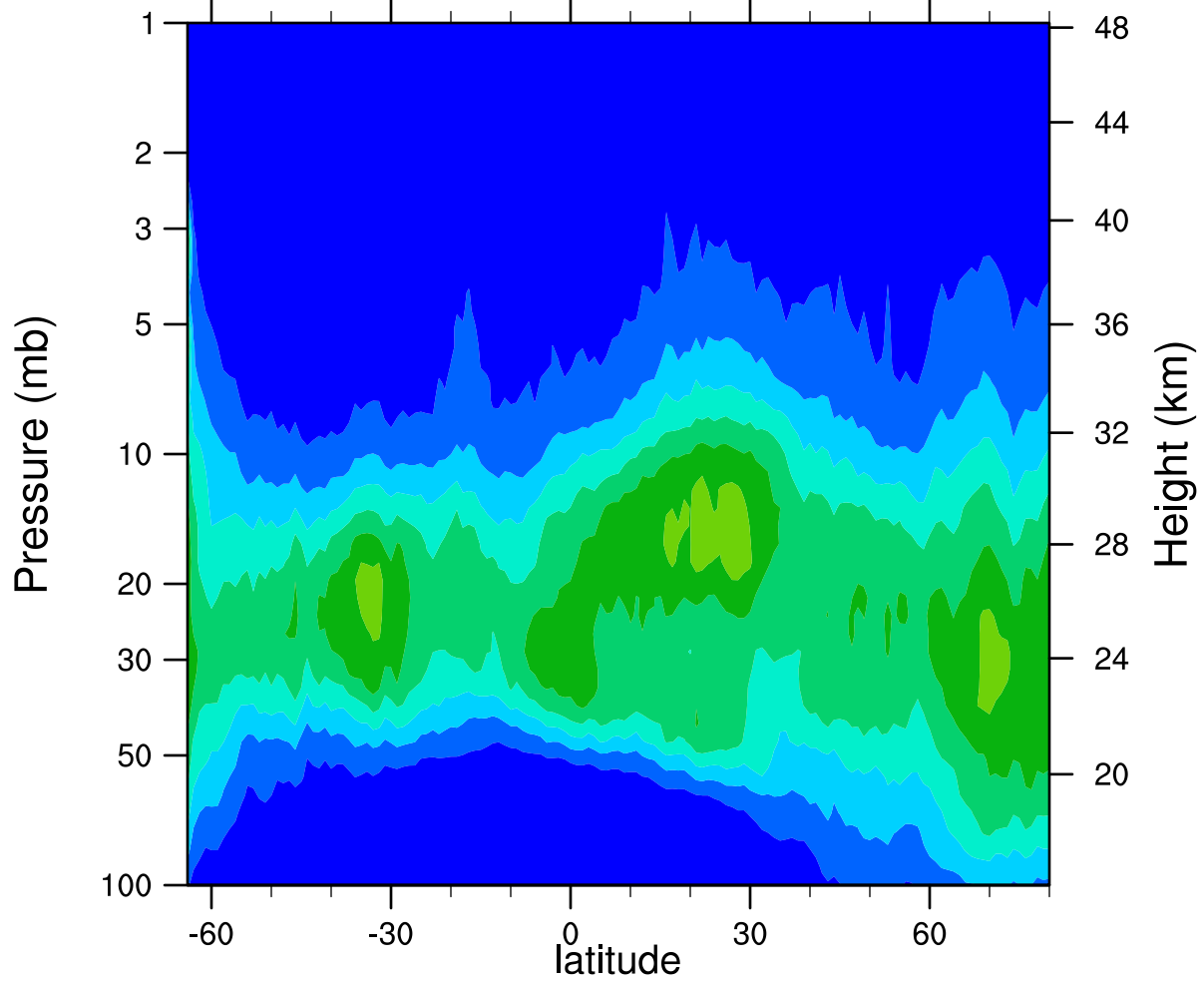
HIRDLSv6 2006d083 ClONO2_Ascending (ppbv)
