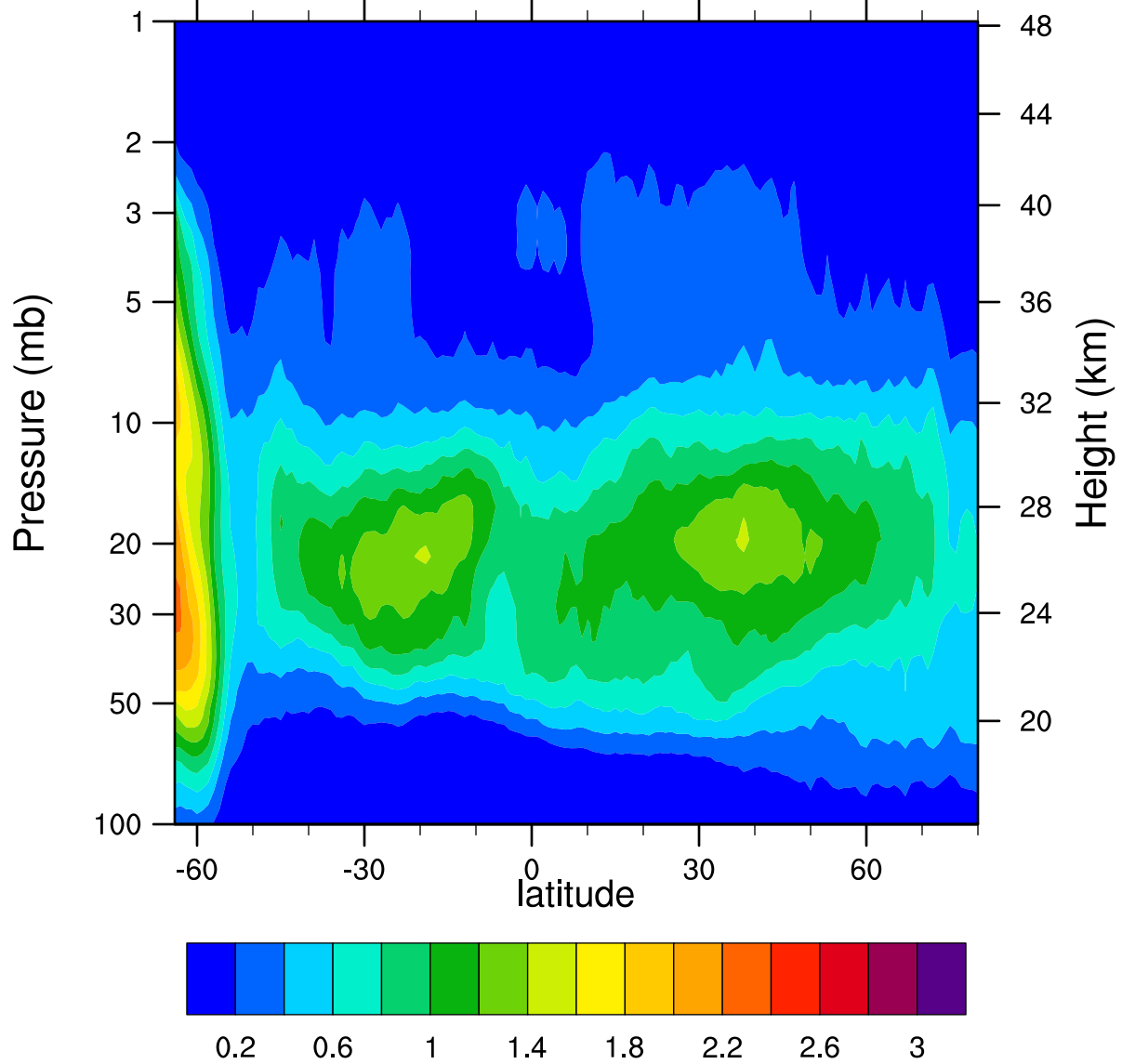
HIRDLSv6 2006d250 ClONO2_Ascending (ppbv)
