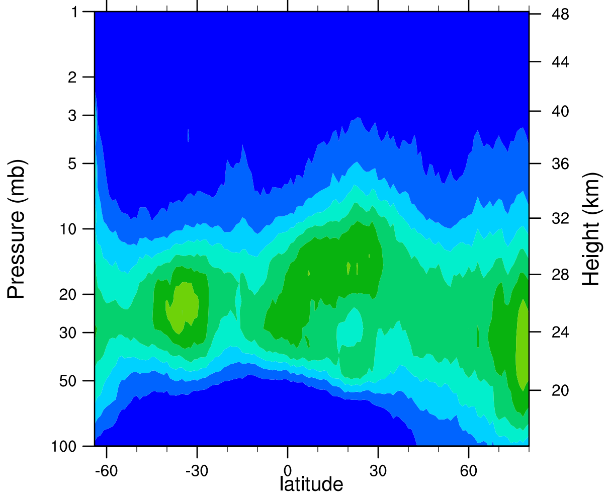
HIRDLSv6 2006d071 ClONO2_Ascending (ppbv)
