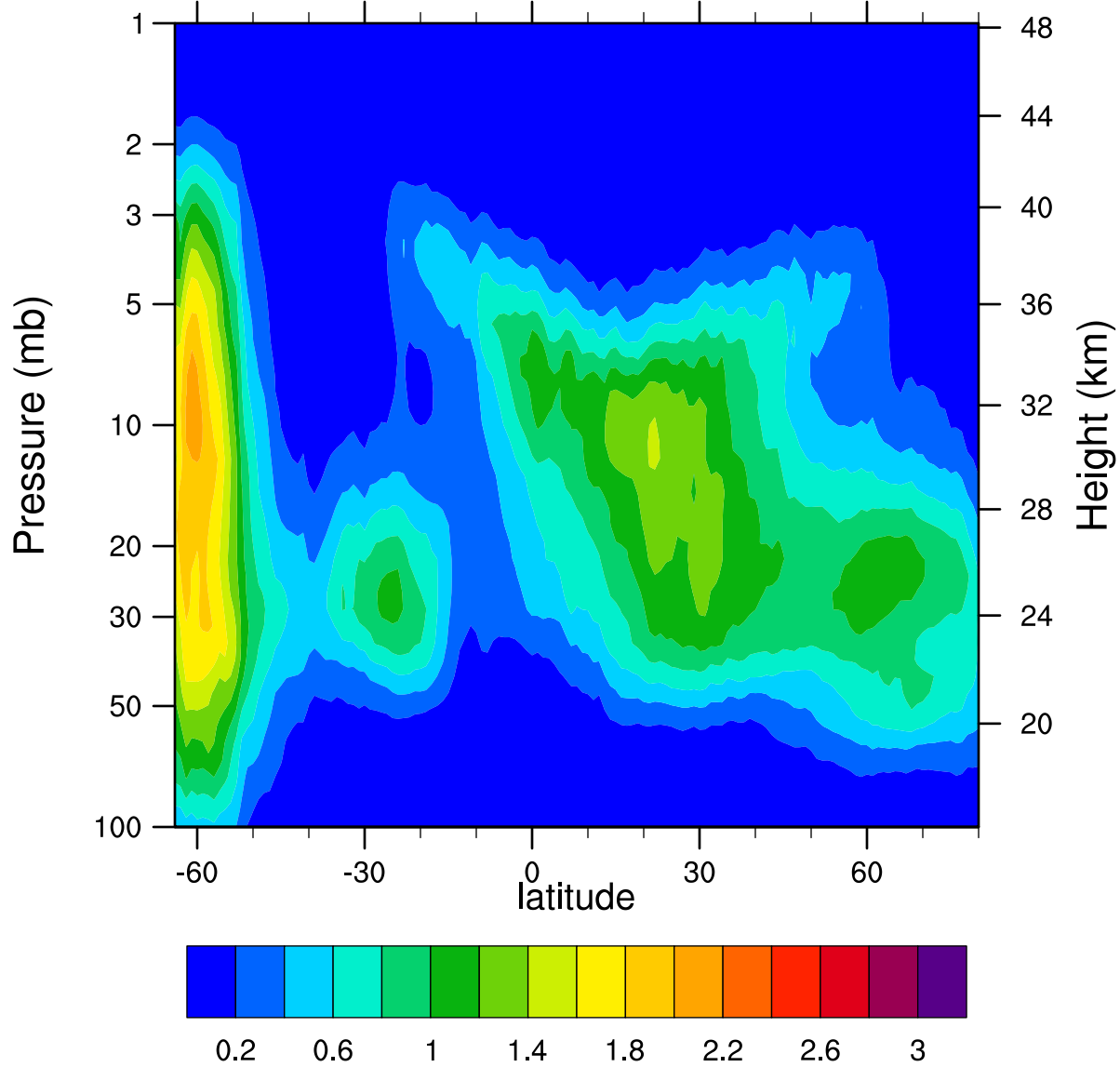
HIRDLSv6 2005d172 ClONO2_Ascending (ppbv)
