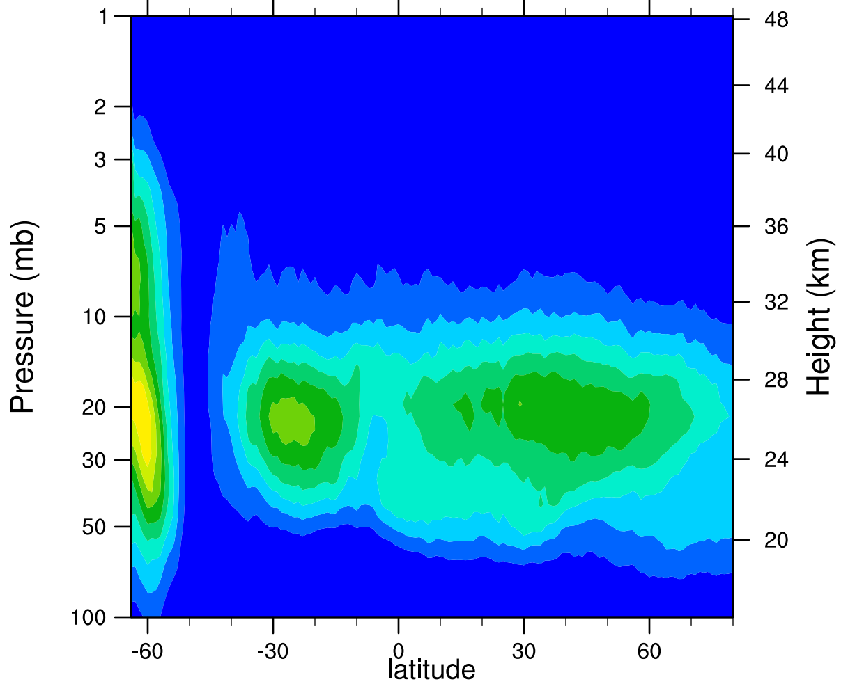
HIRDLSv6 2006d208 ClONO2_Ascending (ppbv)
