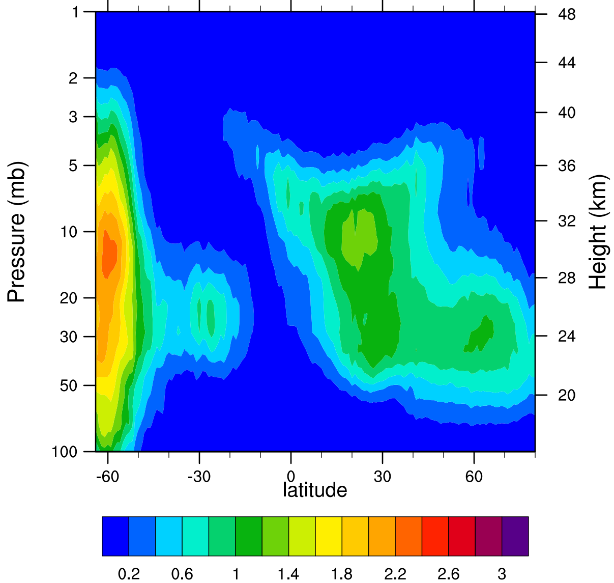
HIRDLSv6 2005d138 ClONO2_Ascending (ppbv)
