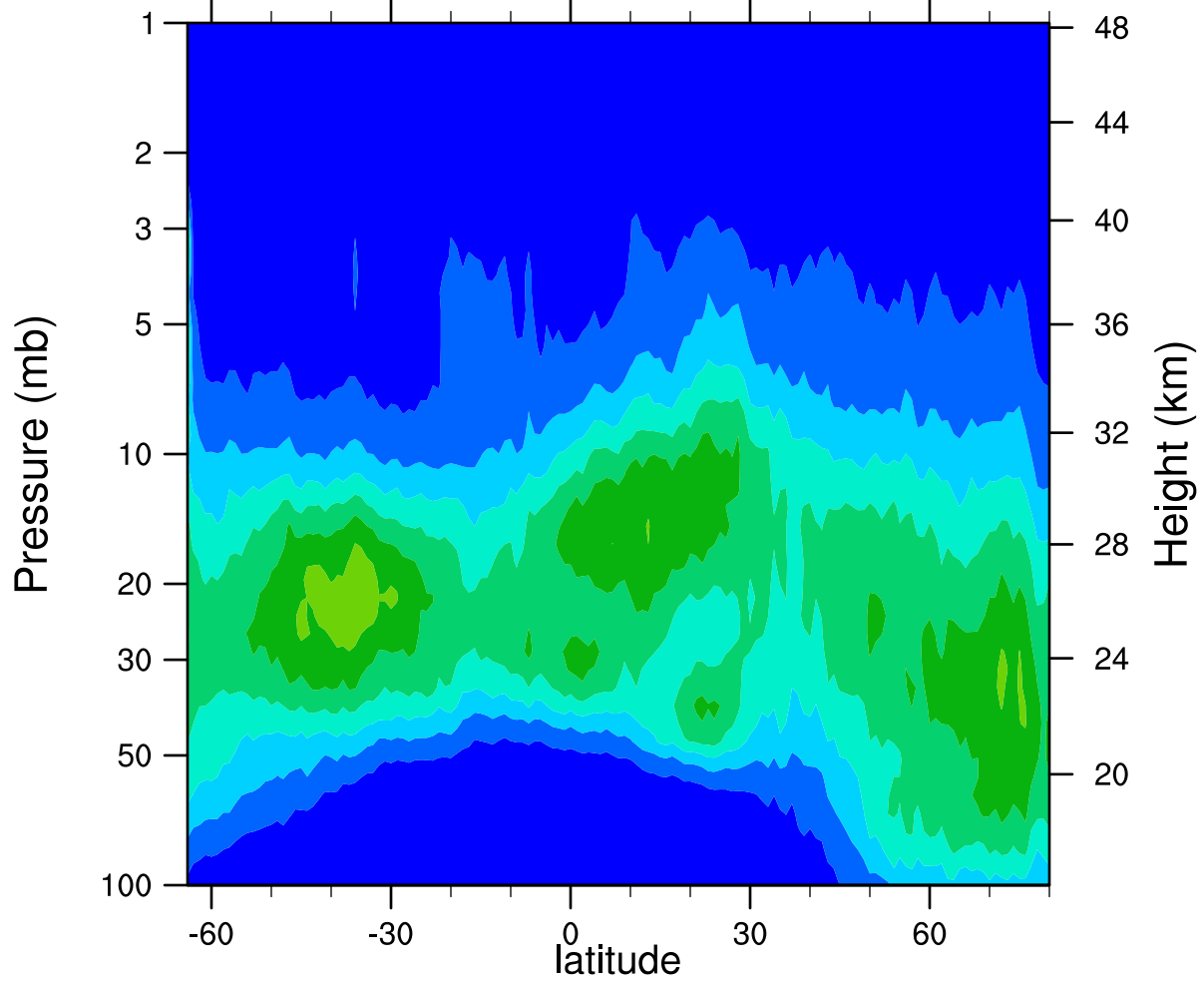
HIRDLSv6 2006d056 ClONO2_Ascending (ppbv)
