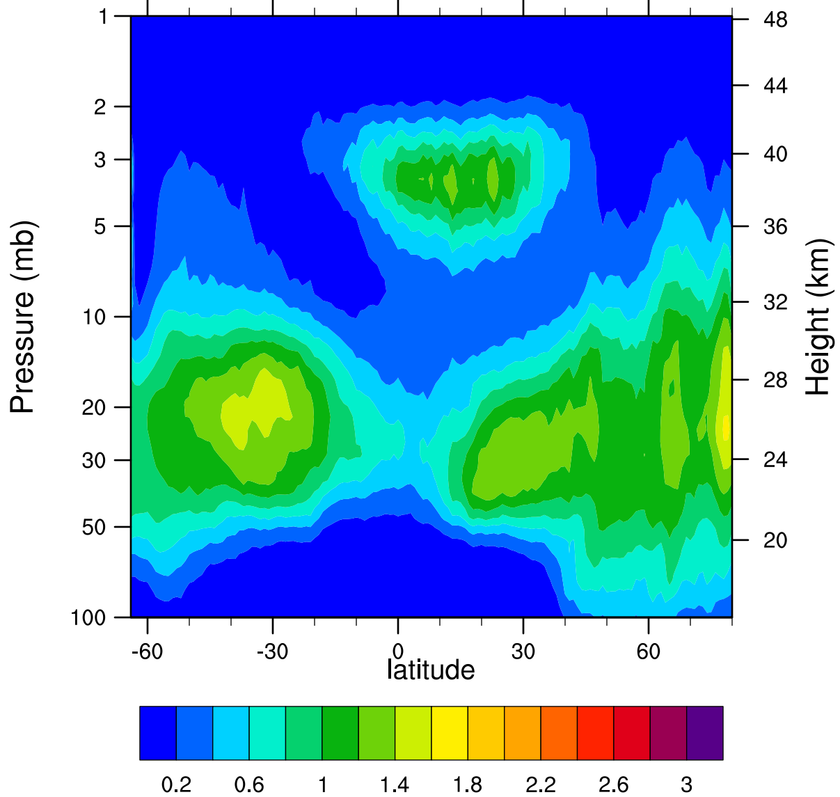
HIRDLSv6 2007d028 ClONO2_Ascending (ppbv)
