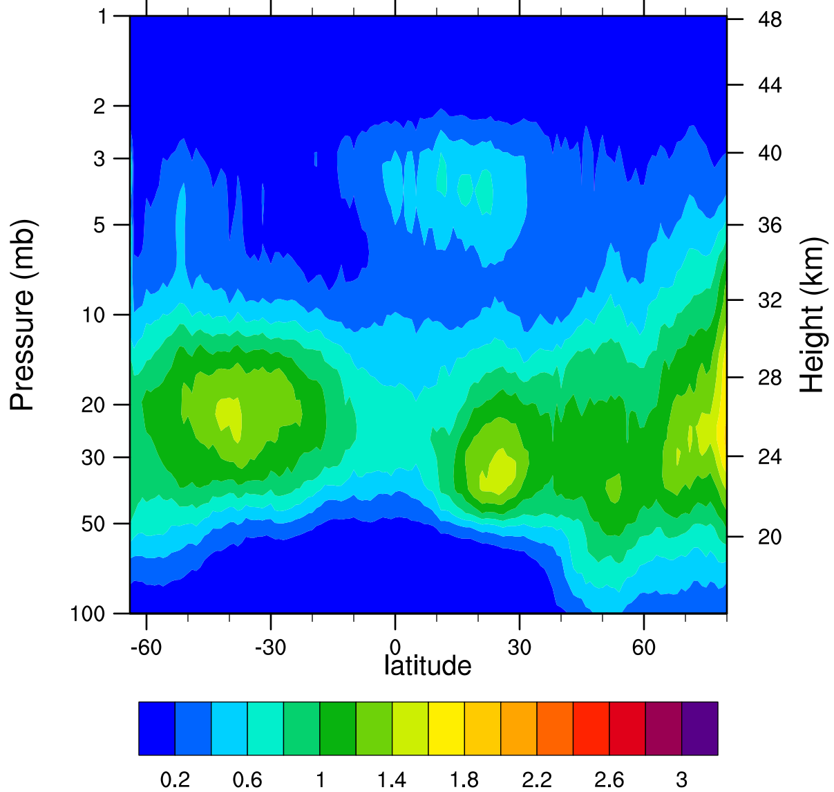
HIRDLSv6 2007d041 ClONO2_Ascending (ppbv)
