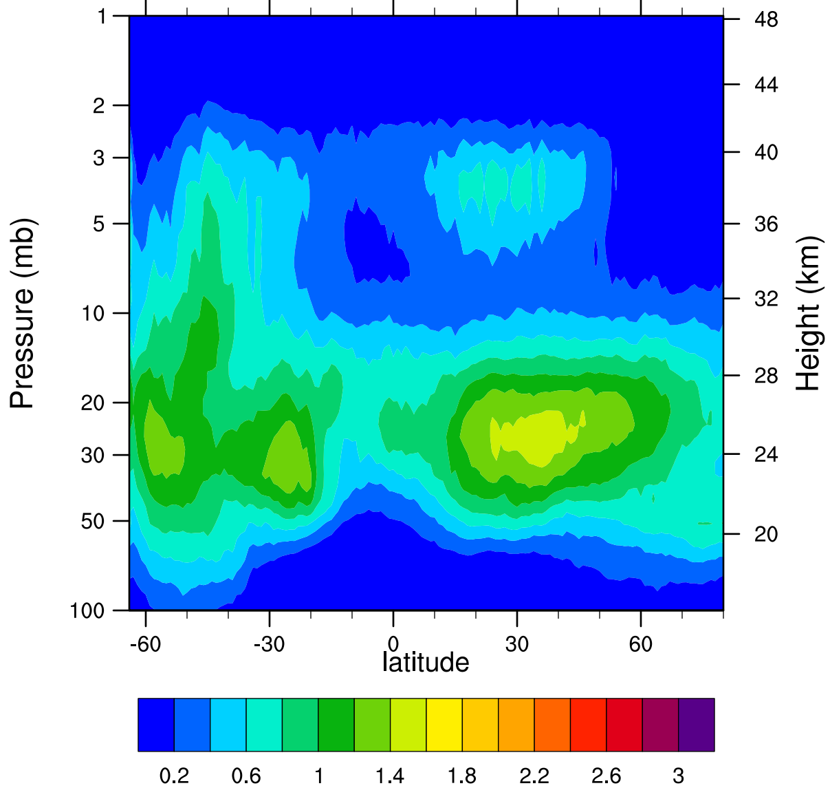
HIRDLSv6 2007d196 ClONO2_Ascending (ppbv)
