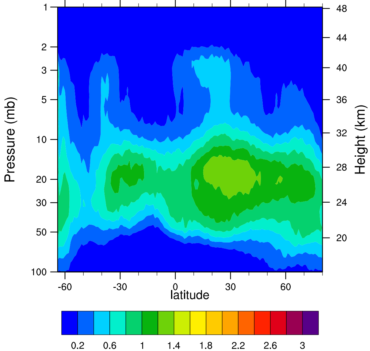
HIRDLSv6 2006d146 ClONO2_Ascending (ppbv)
