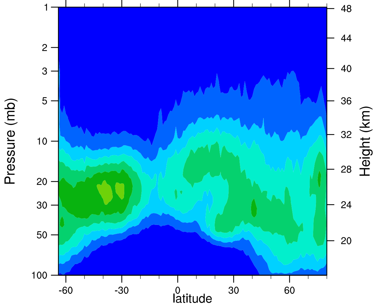
HIRDLSv6 2006d009 ClONO2_Ascending (ppbv)
