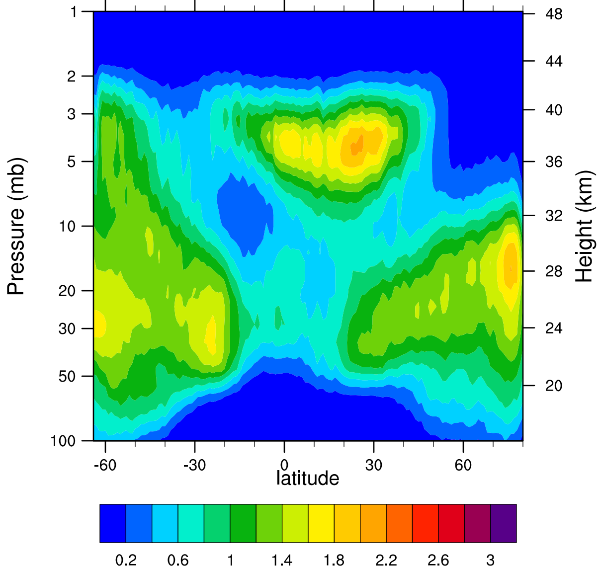
HIRDLSv6 2007d292 ClONO2_Ascending (ppbv)
