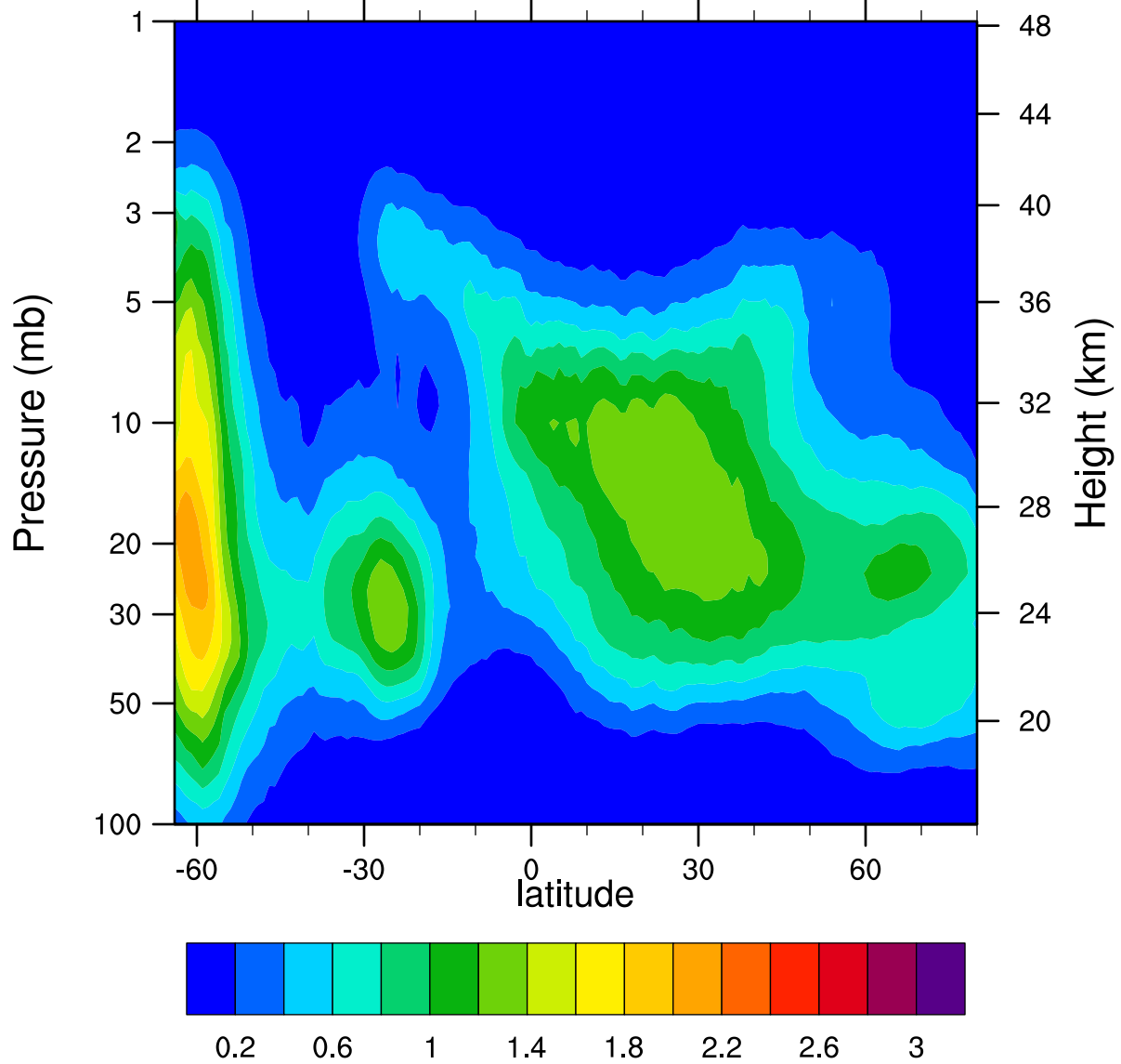
HIRDLSv6 2005d195 ClONO2_Ascending (ppbv)
