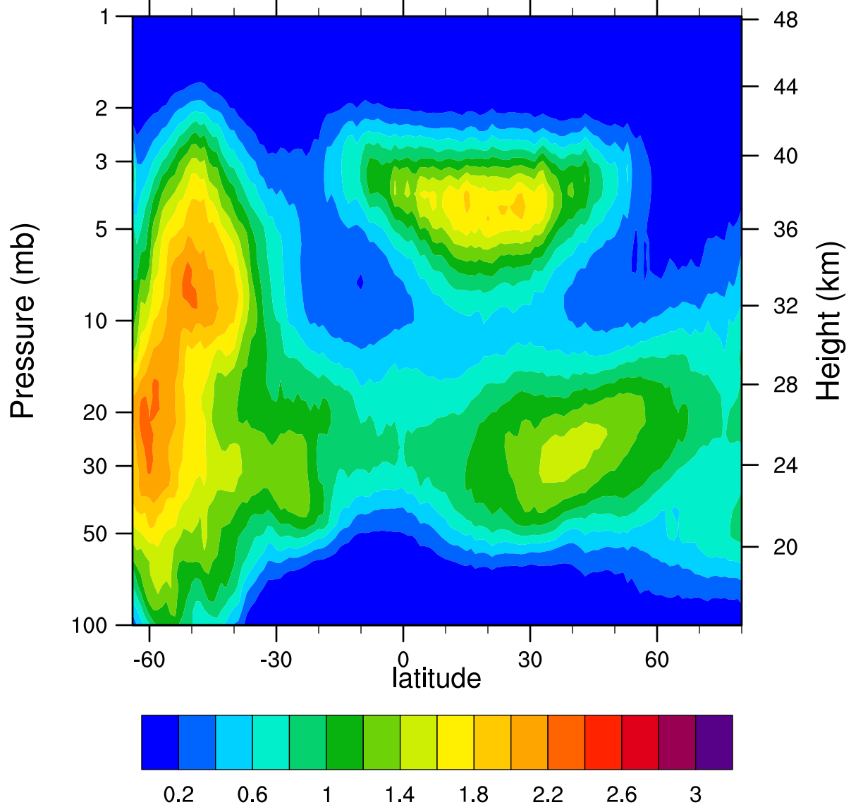
HIRDLSv6 2007d217 ClONO2_Ascending (ppbv)
