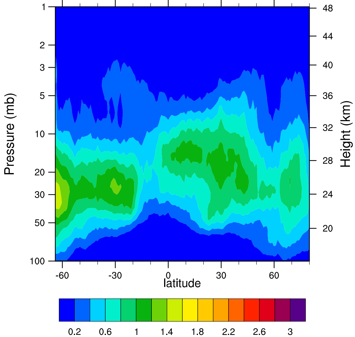
HIRDLSv6 2005d308 ClONO2_Ascending (ppbv)
