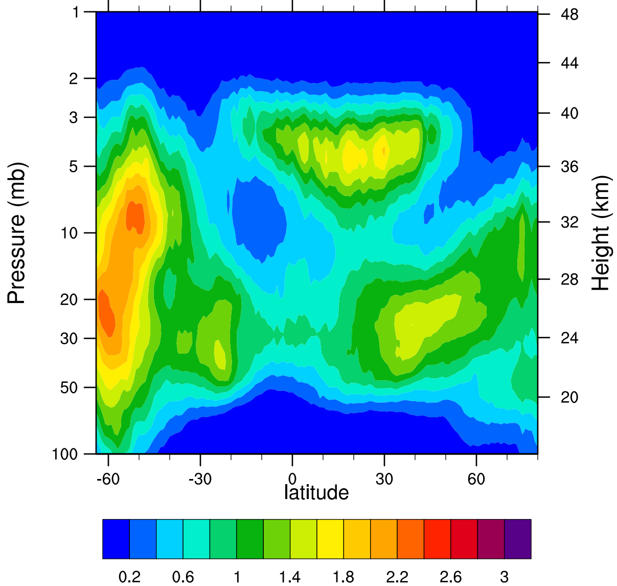
HIRDLSv6 2007d238 ClONO2_Ascending (ppbv)
