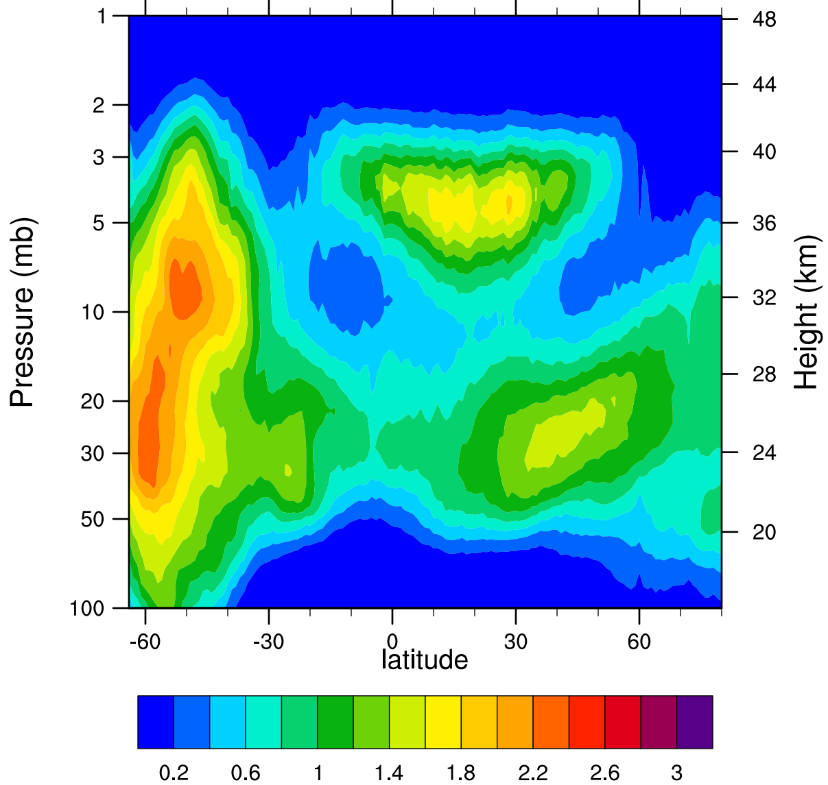
HIRDLSv6 2007d226 ClONO2_Ascending (ppbv)
