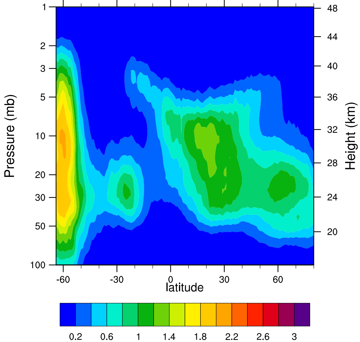
HIRDLSv6 2005d165 ClONO2_Ascending (ppbv)
