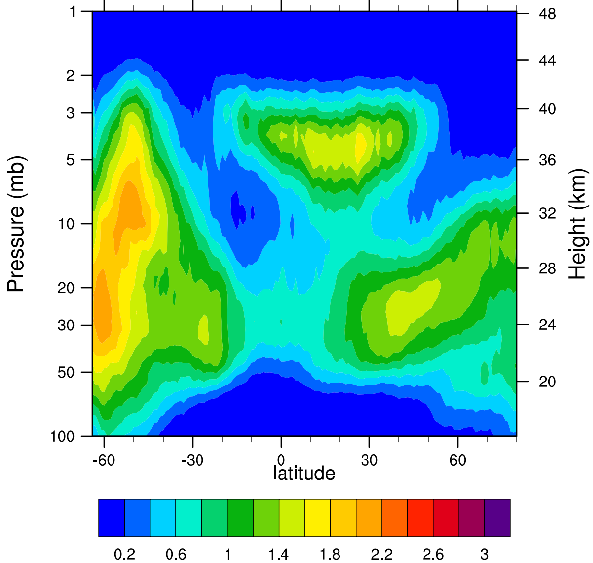
HIRDLSv6 2007d249 ClONO2_Ascending (ppbv)
