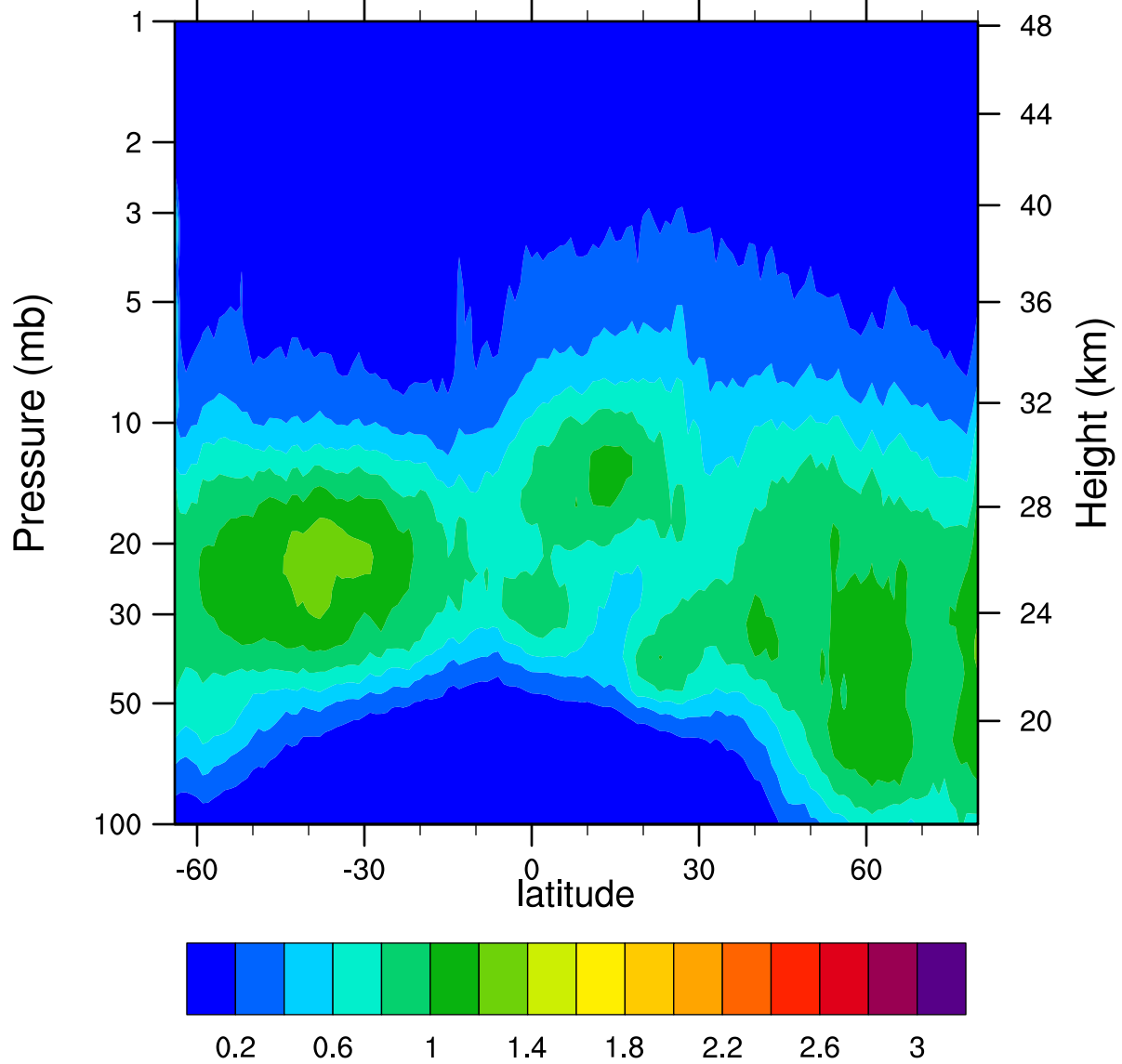
HIRDLSv6 2006d040 ClONO2_Ascending (ppbv)
