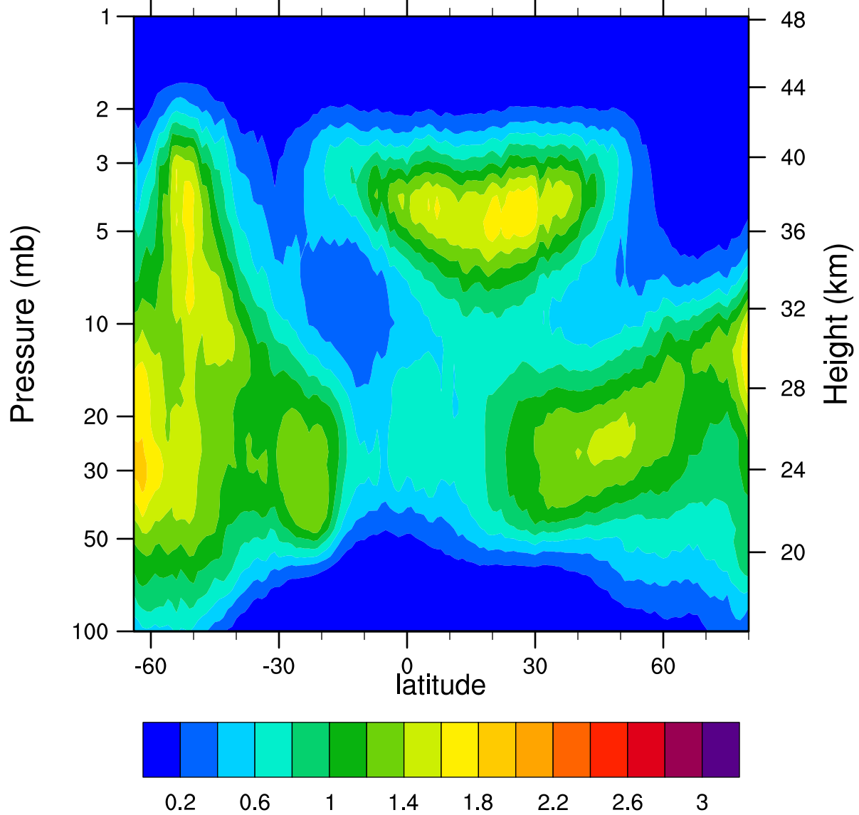
HIRDLSv6 2007d268 ClONO2_Ascending (ppbv)
