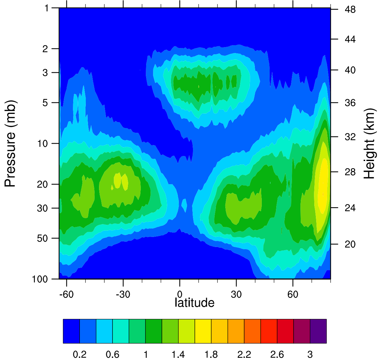
HIRDLSv6 2007d008 ClONO2_Ascending (ppbv)
