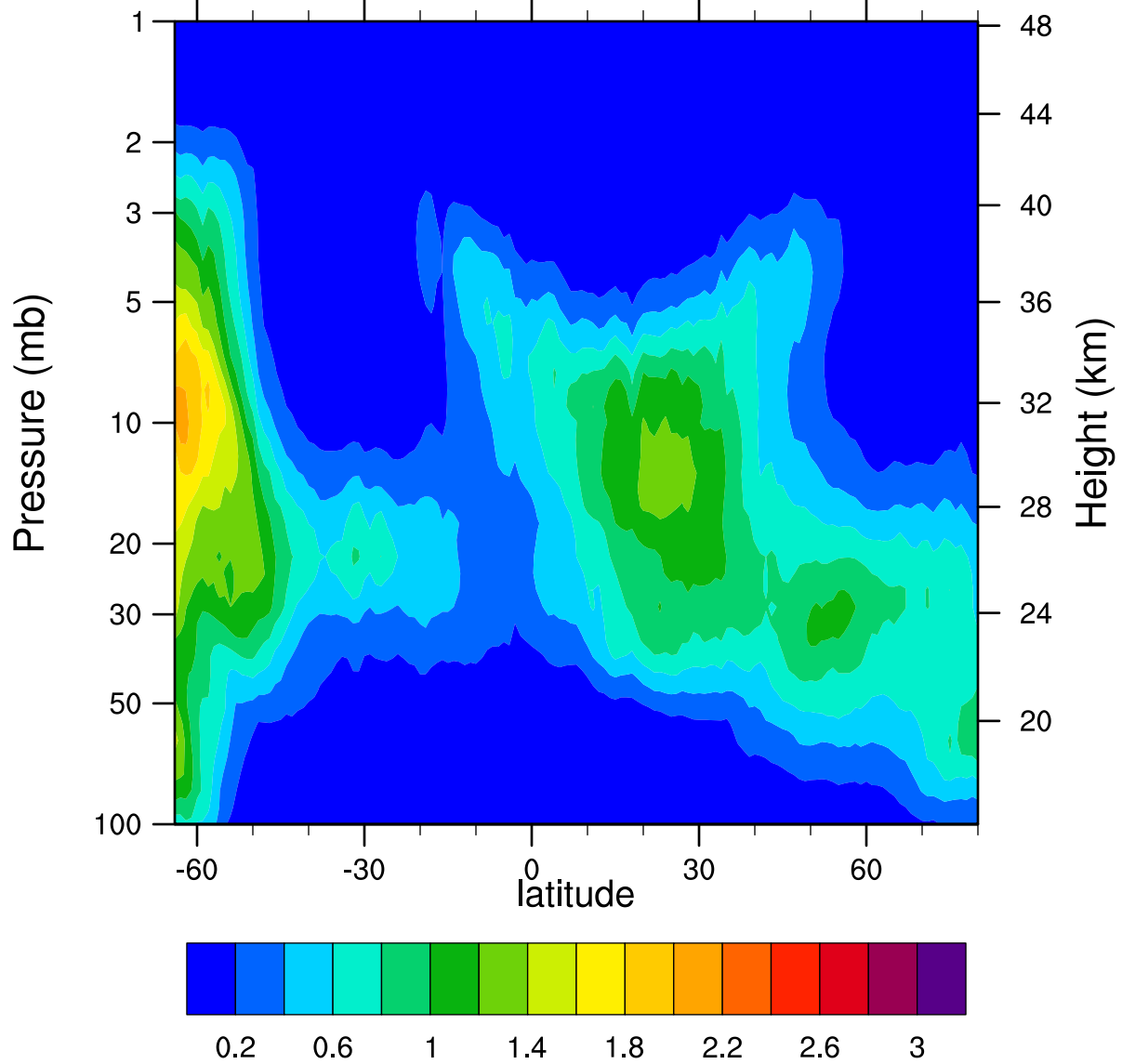
HIRDLSv6 2005d102 ClONO2_Ascending (ppbv)
