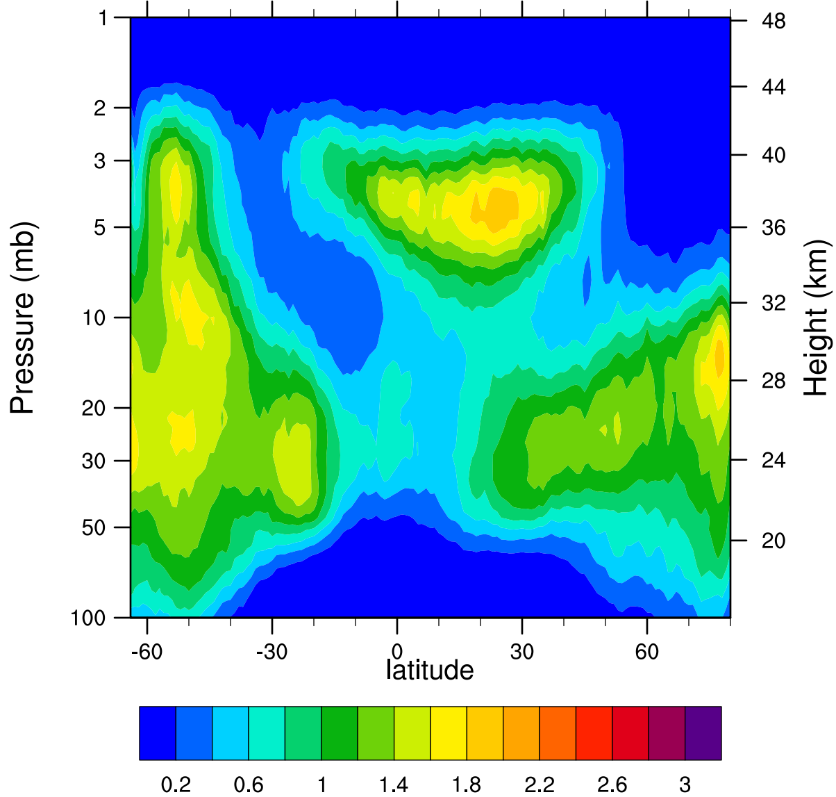
HIRDLSv6 2007d284 ClONO2_Ascending (ppbv)
