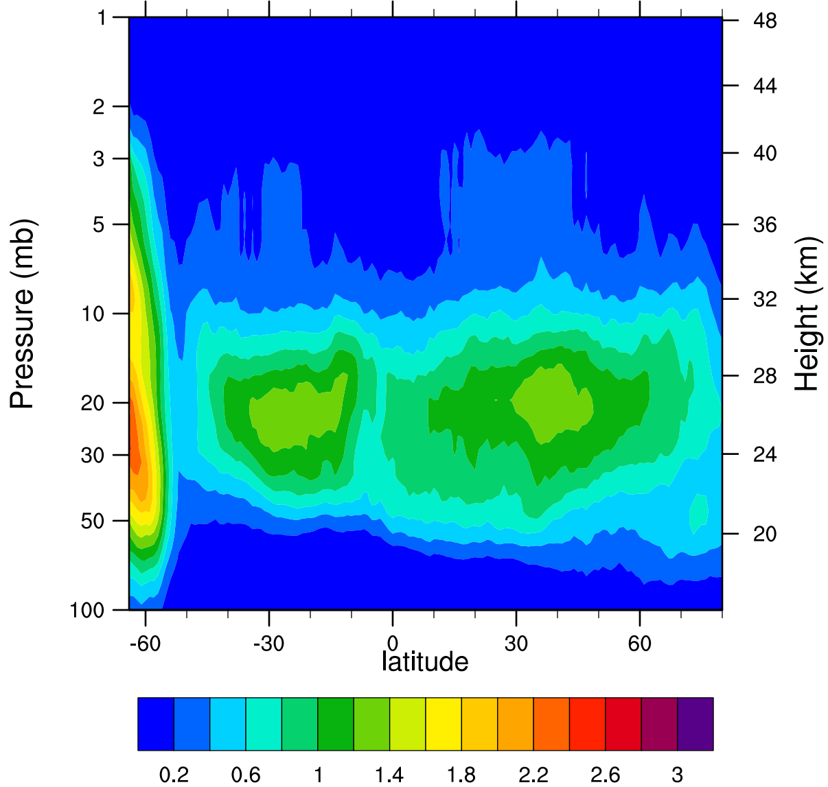
HIRDLSv6 2006d242 ClONO2_Ascending (ppbv)
