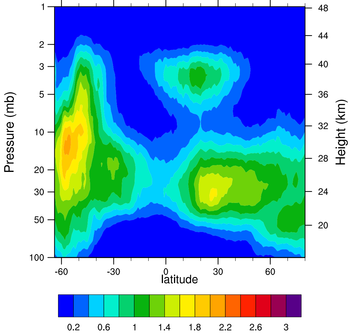
HIRDLSv6 2007d126 ClONO2_Ascending (ppbv)
