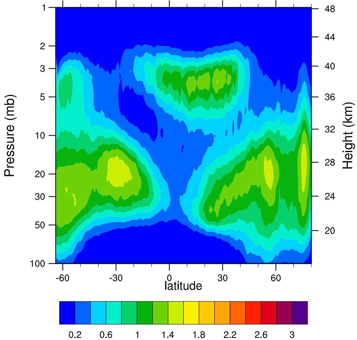
HIRDLSv6 2006d354 ClONO2_Ascending (ppbv)
