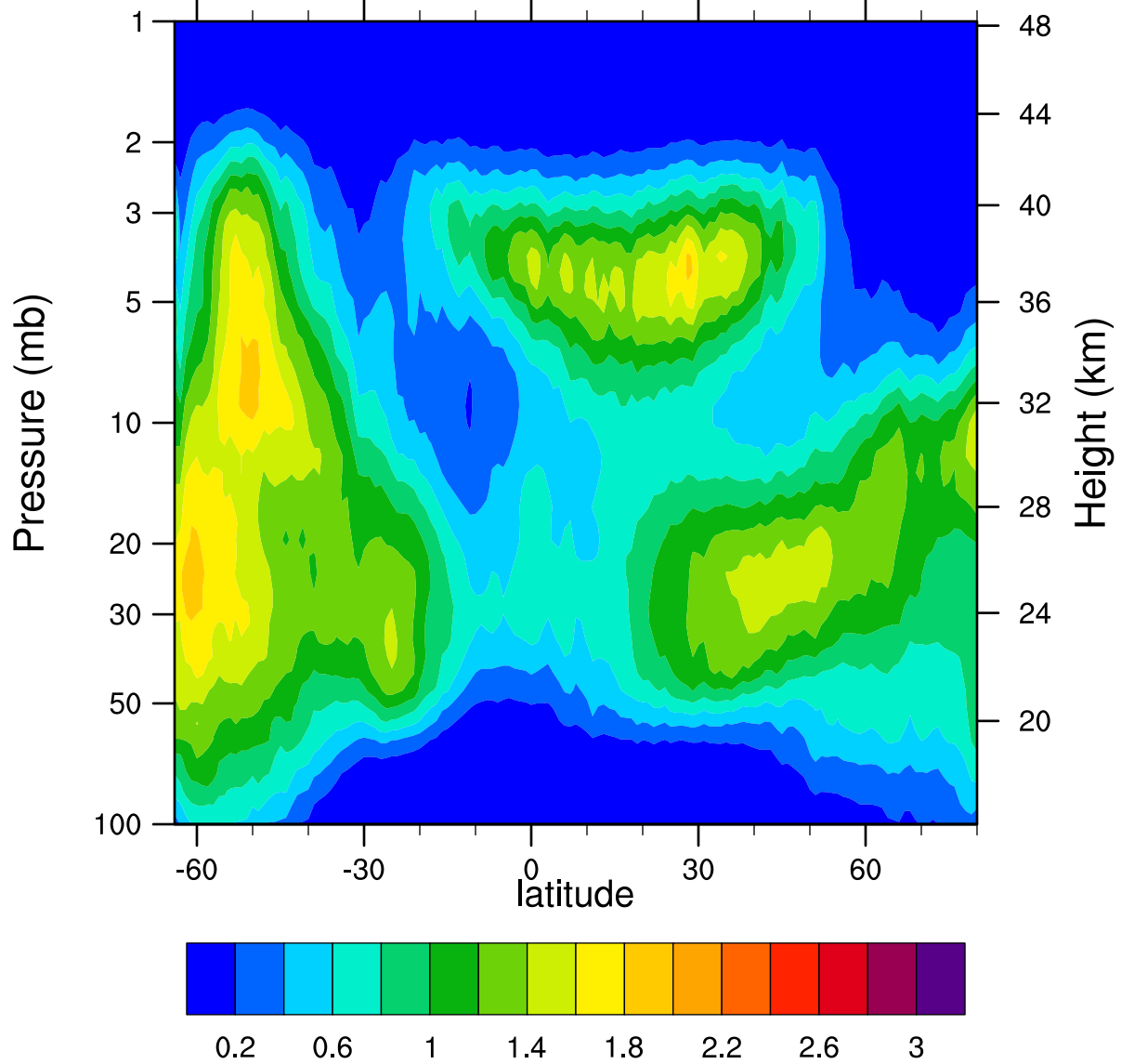
HIRDLSv6 2007d259 ClONO2_Ascending (ppbv)
