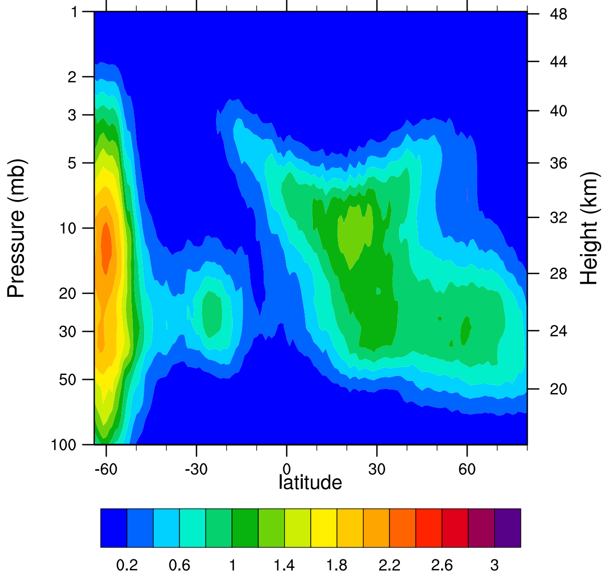
HIRDLSv6 2005d150 ClONO2_Ascending (ppbv)
