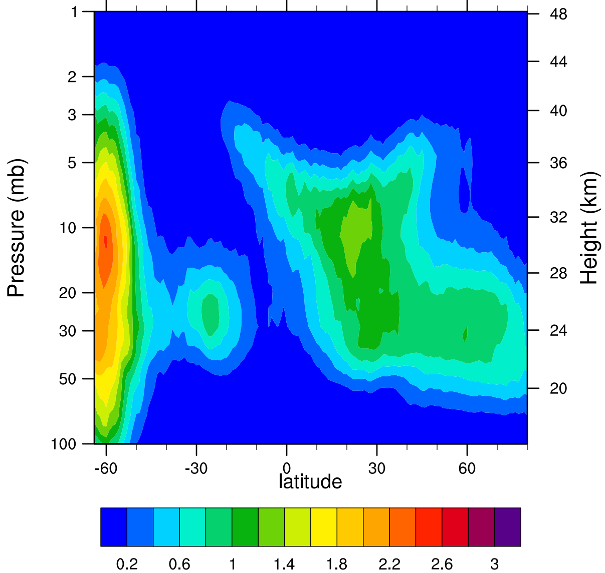
HIRDLSv6 2005d147 ClONO2_Ascending (ppbv)
