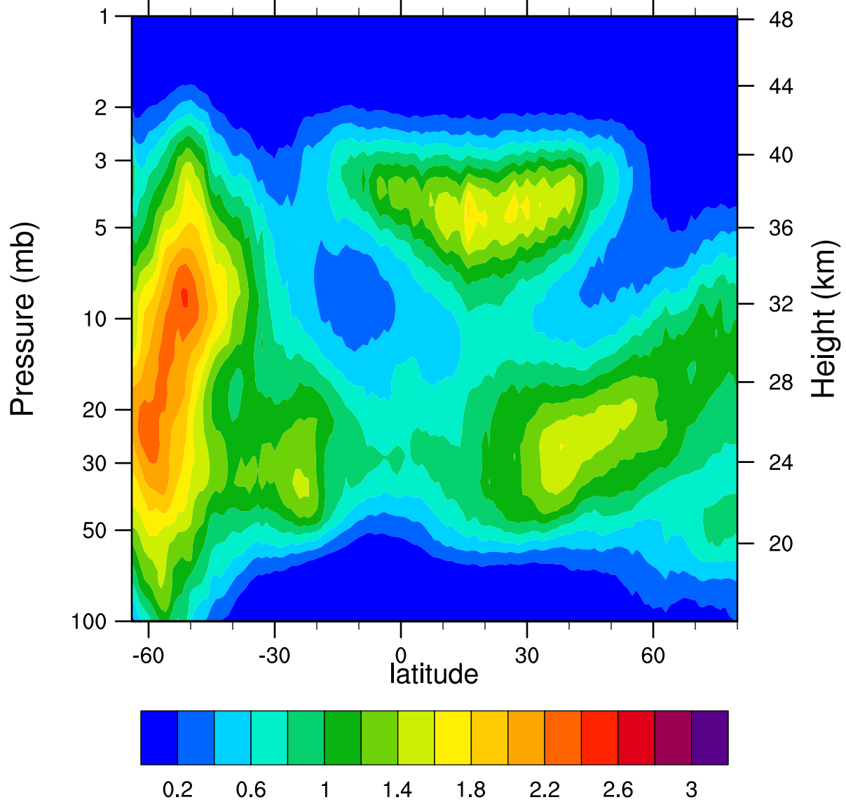
HIRDLSv6 2007d234 ClONO2_Ascending (ppbv)
