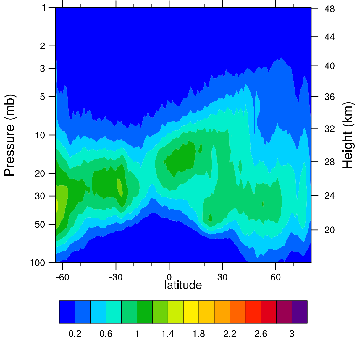
HIRDLSv6 2005d340 ClONO2_Ascending (ppbv)
