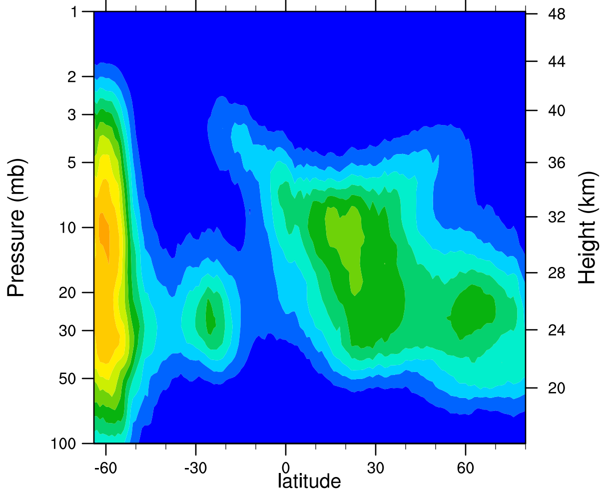
HIRDLSv6 2005d164 ClONO2_Ascending (ppbv)
