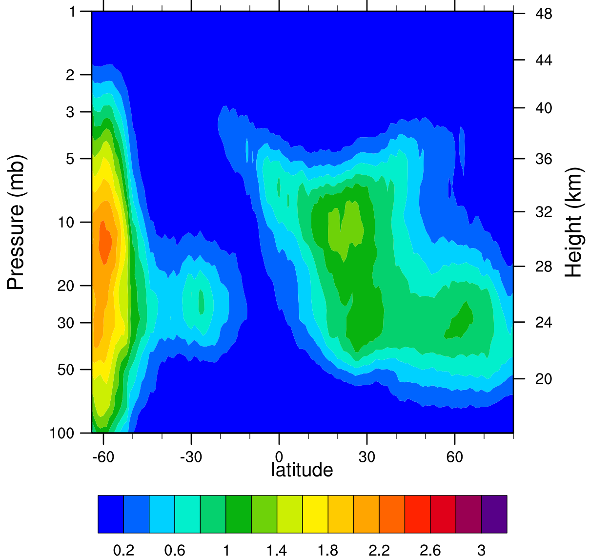
HIRDLSv6 2005d137 ClONO2_Ascending (ppbv)
