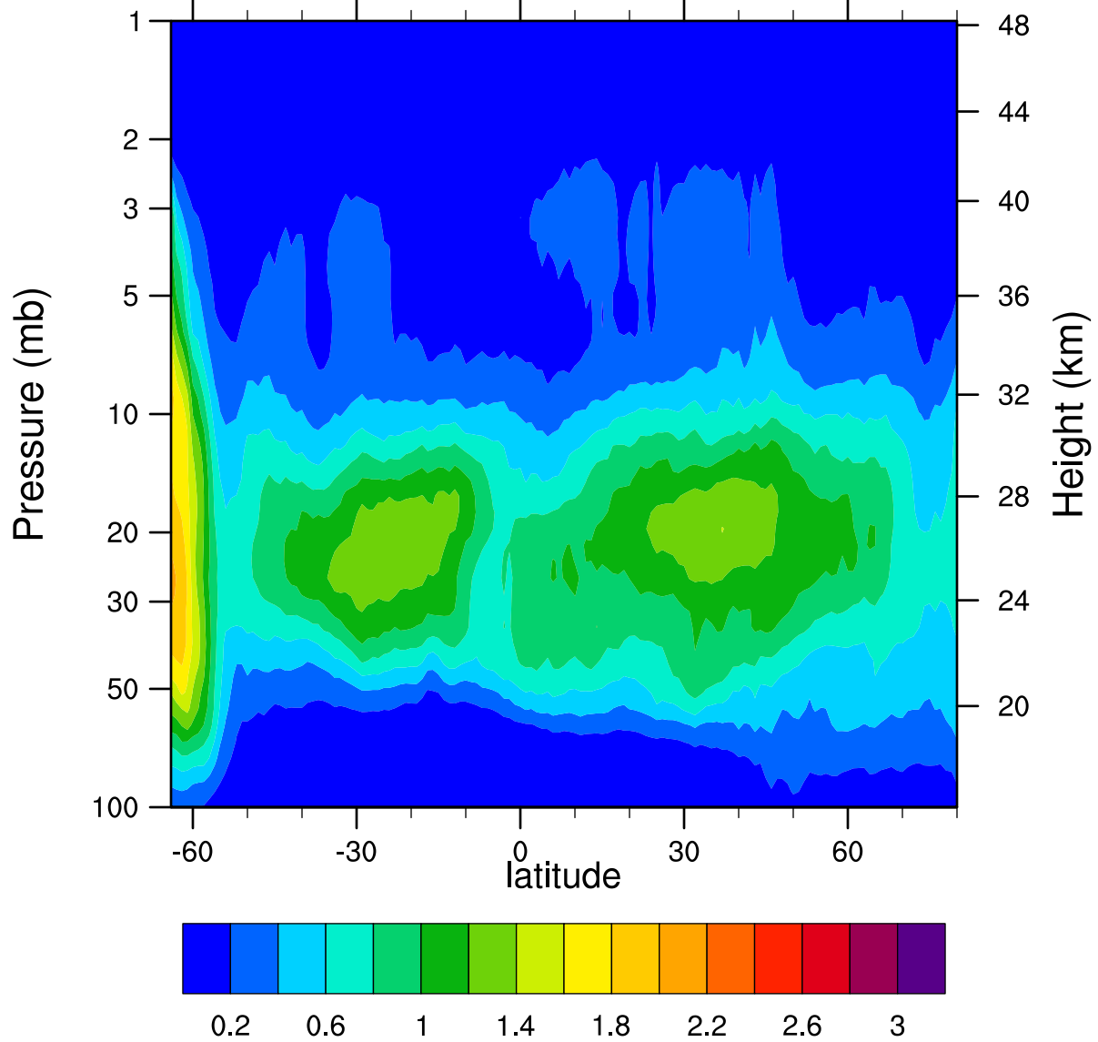
HIRDLSv6 2006d261 ClONO2_Ascending (ppbv)
