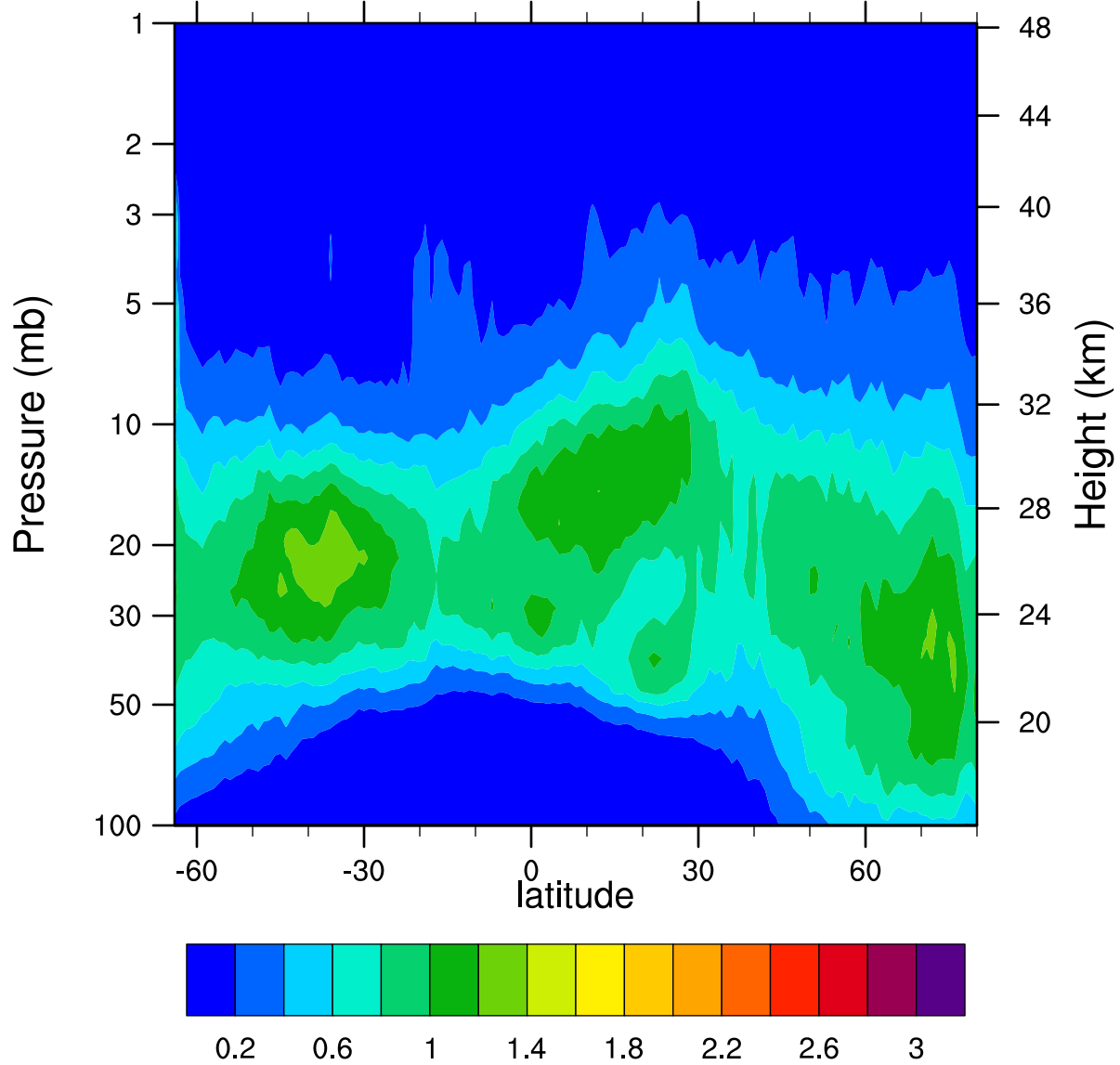
HIRDLSv6 2006d057 ClONO2_Ascending (ppbv)
