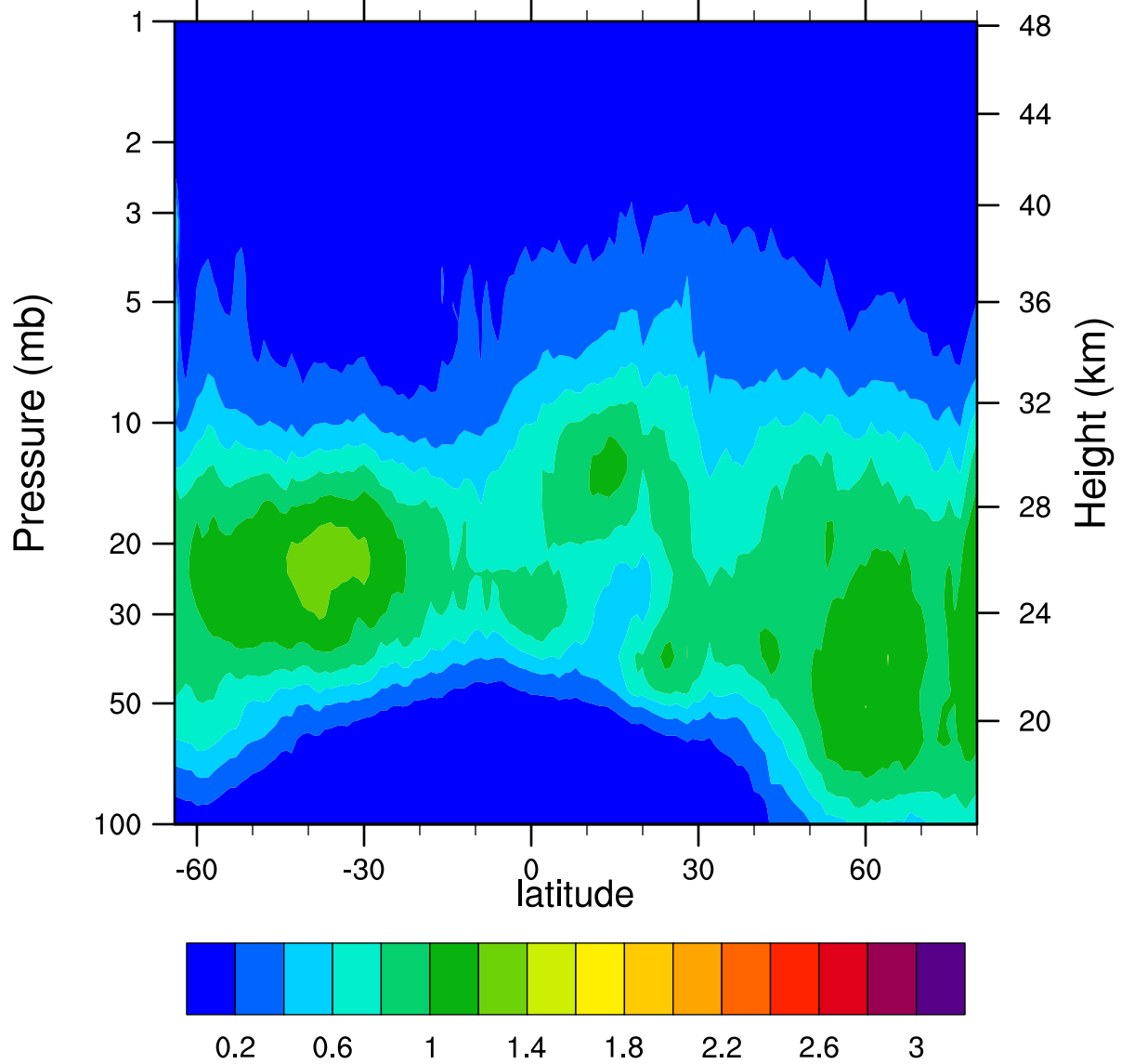
HIRDLSv6 2006d037 ClONO2_Ascending (ppbv)
