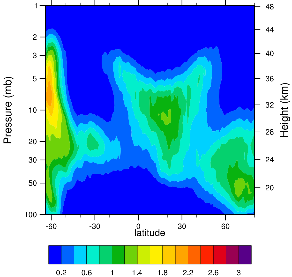
HIRDLSv6 2005d077 ClONO2_Ascending (ppbv)
