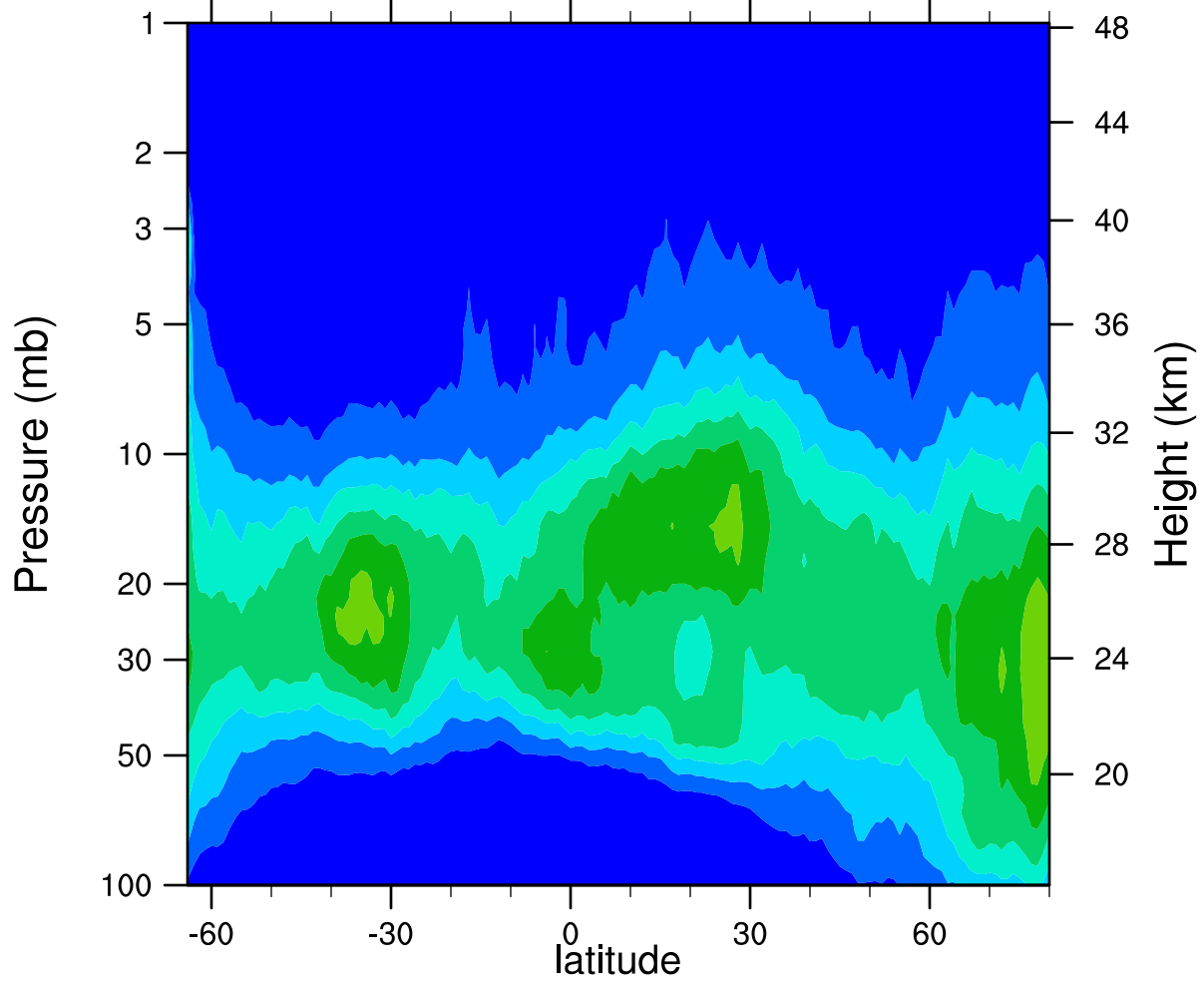
HIRDLSv6 2006d077 ClONO2_Ascending (ppbv)
