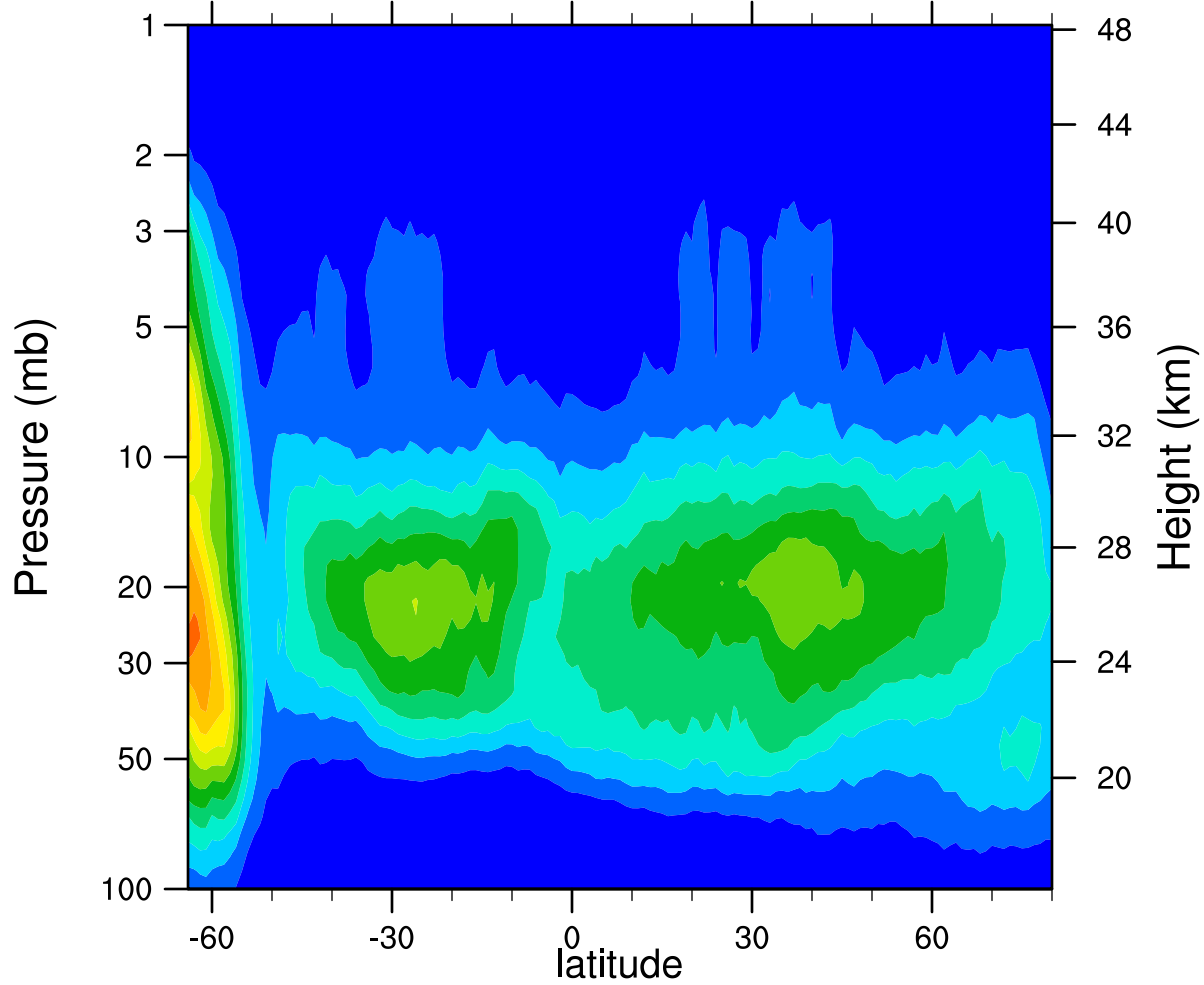
HIRDLSv6 2006d239 ClONO2_Ascending (ppbv)
