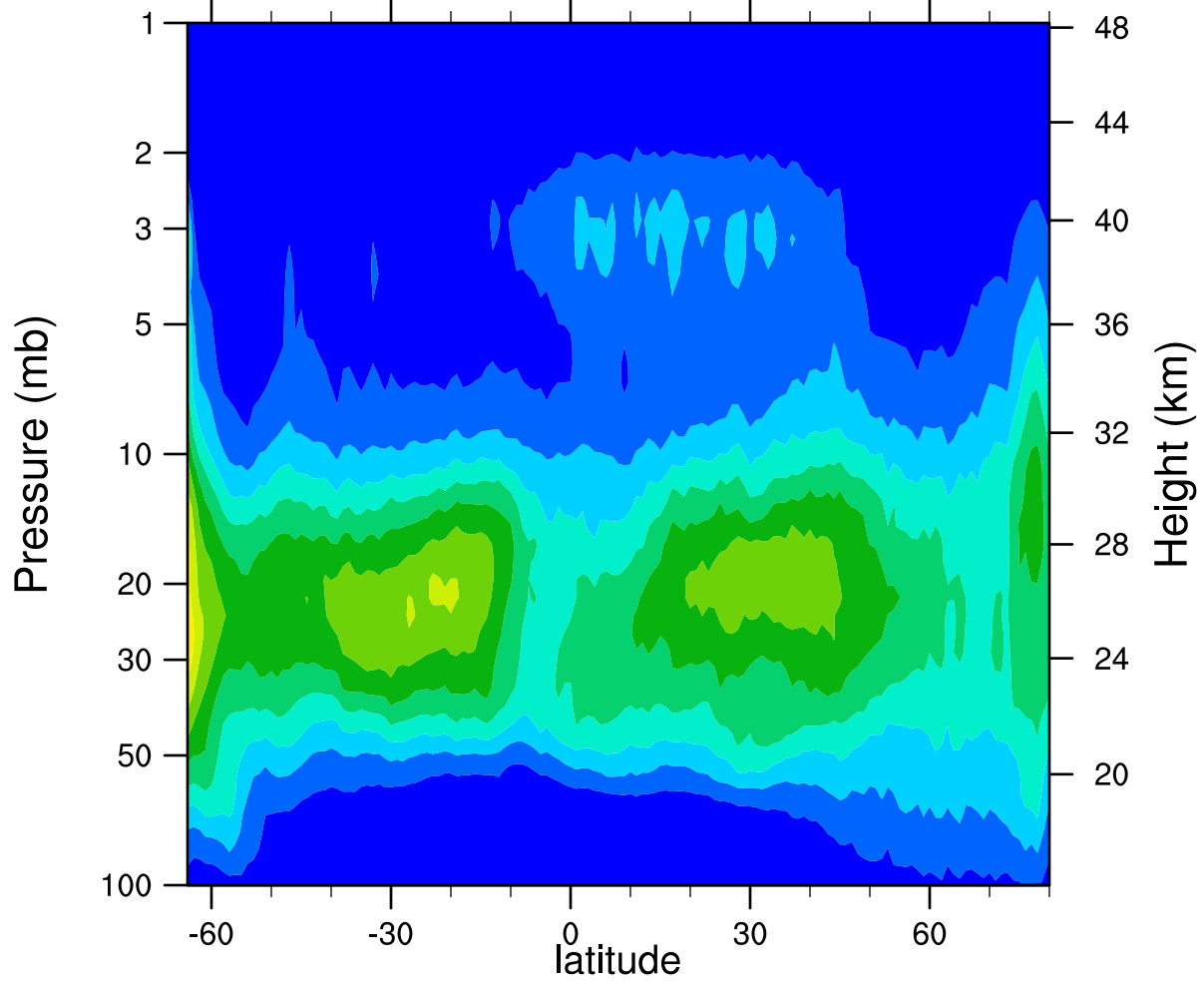
HIRDLSv6 2006d287 ClONO2_Ascending (ppbv)
