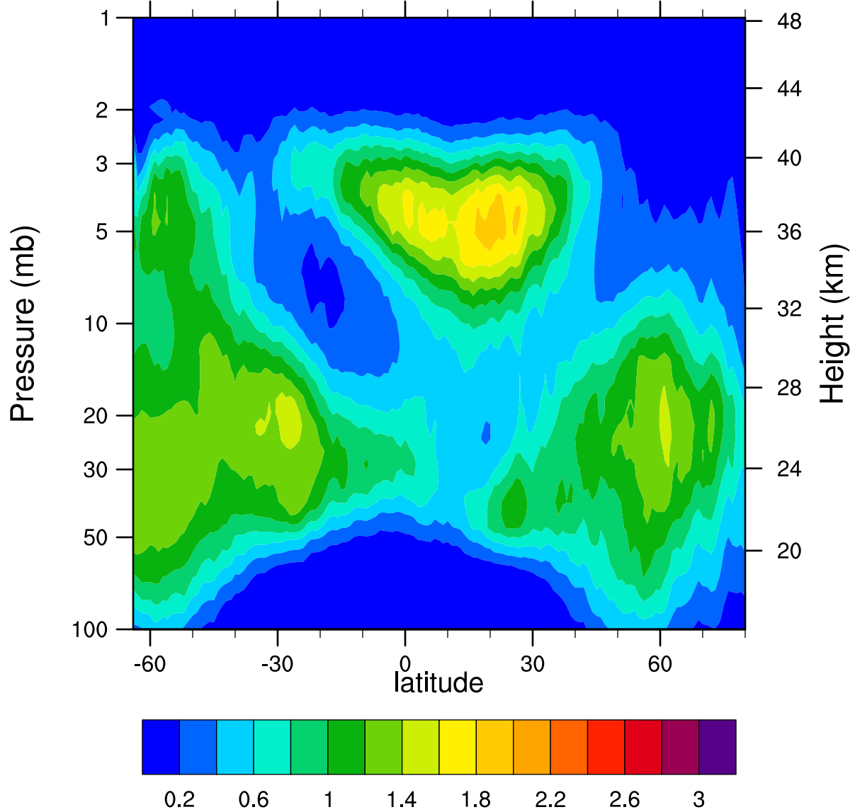
HIRDLSv6 2007d357 ClONO2_Ascending (ppbv)
