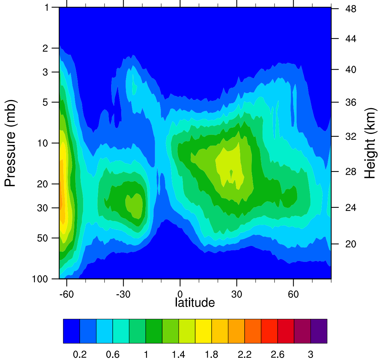
HIRDLSv6 2005d263 ClONO2_Ascending (ppbv)
