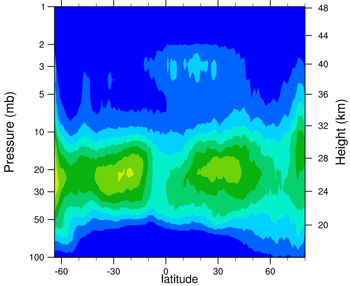
HIRDLSv6 2006d289 ClONO2_Ascending (ppbv)
