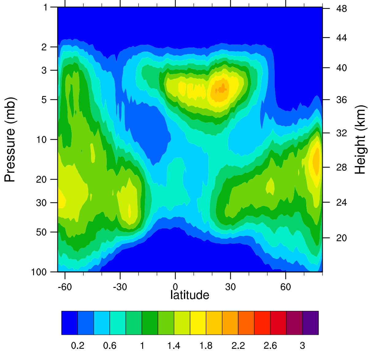
HIRDLSv6 2007d289 ClONO2_Ascending (ppbv)
