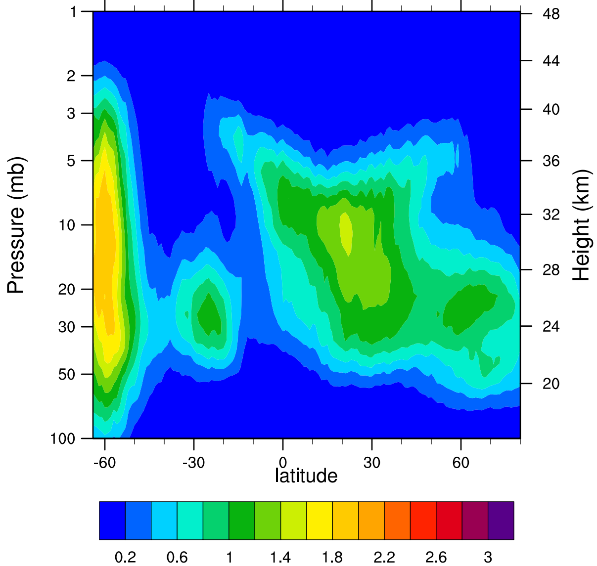
HIRDLSv6 2005d176 ClONO2_Ascending (ppbv)
