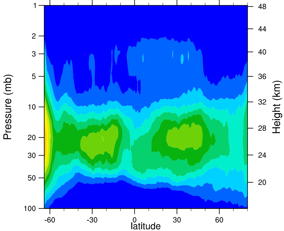
HIRDLSv6 2006d274 ClONO2_Ascending (ppbv)
