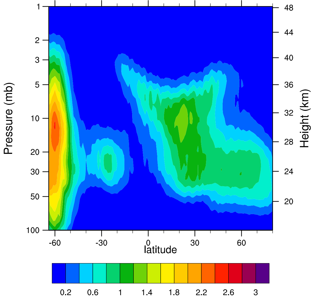
HIRDLSv6 2005d145 ClONO2_Ascending (ppbv)
