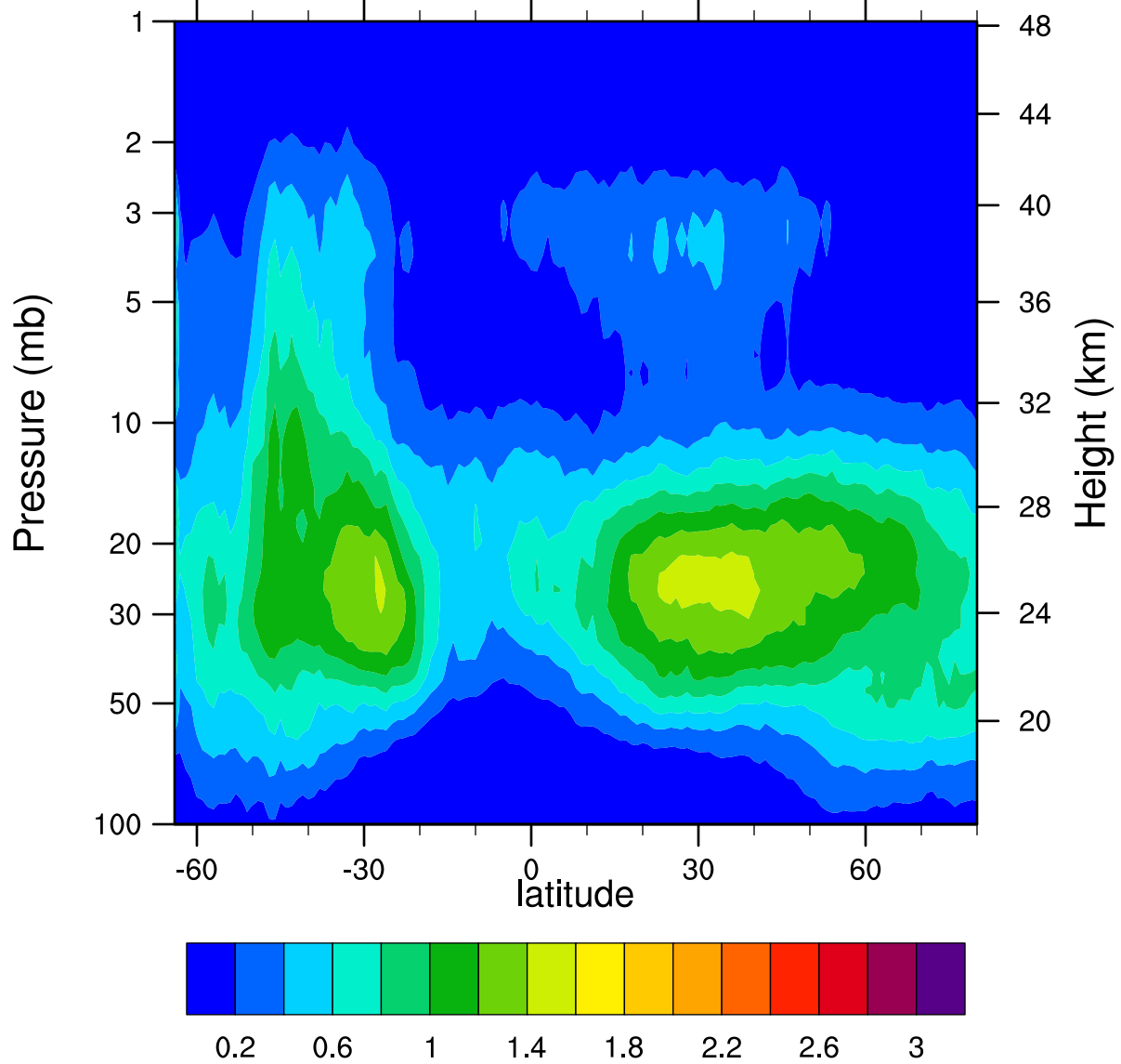
HIRDLSv6 2007d177 ClONO2_Ascending (ppbv)
