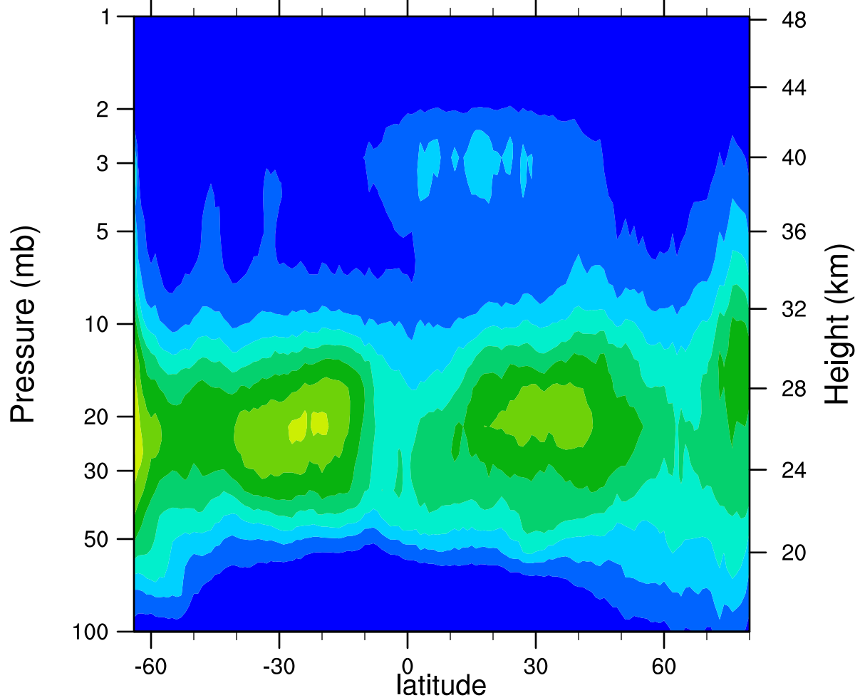
HIRDLSv6 2006d290 ClONO2_Ascending (ppbv)
