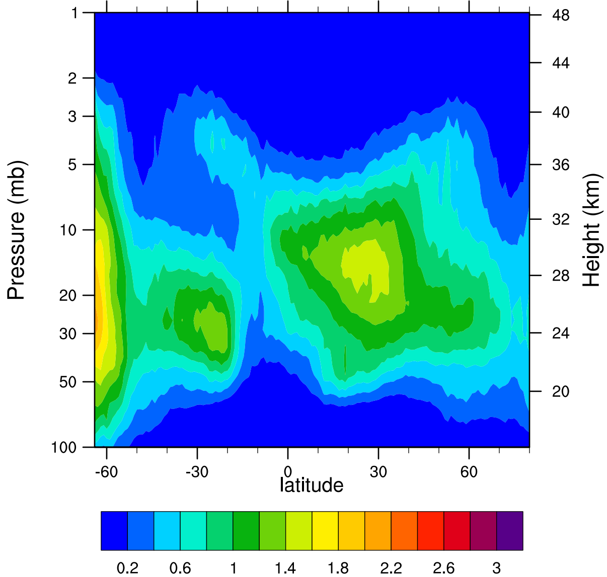
HIRDLSv6 2005d267 ClONO2_Ascending (ppbv)
