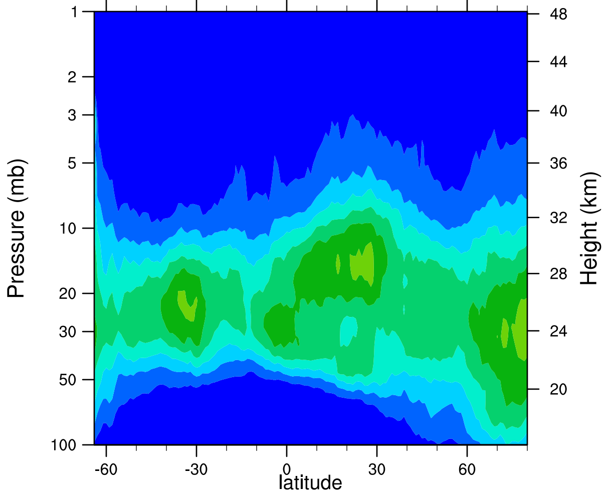
HIRDLSv6 2006d079 ClONO2_Ascending (ppbv)
