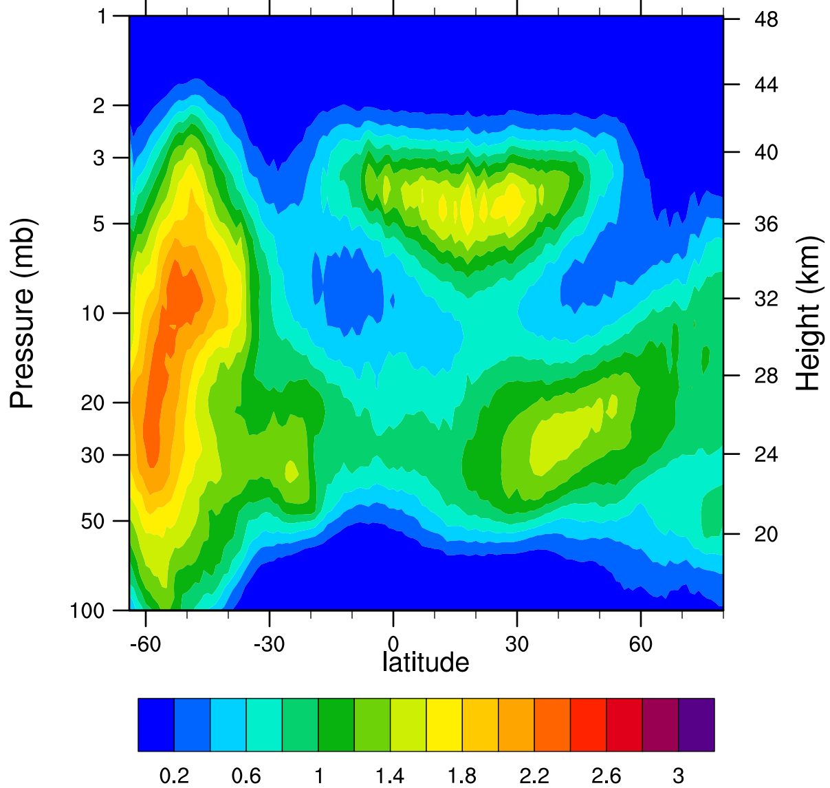
HIRDLSv6 2007d228 ClONO2_Ascending (ppbv)
