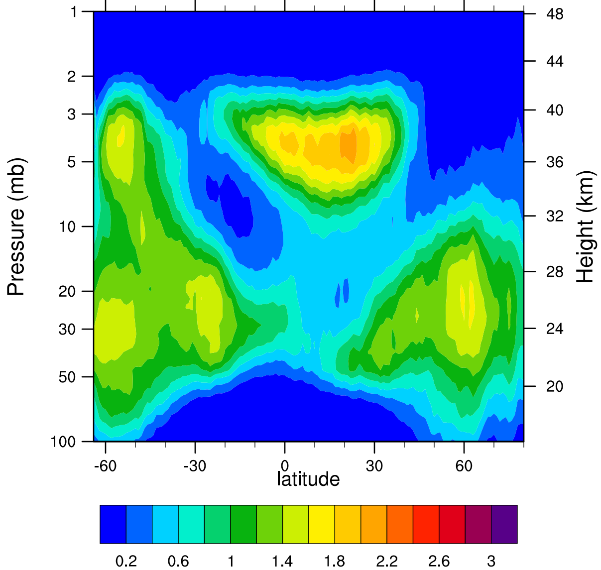
HIRDLSv6 2007d335 ClONO2_Ascending (ppbv)
