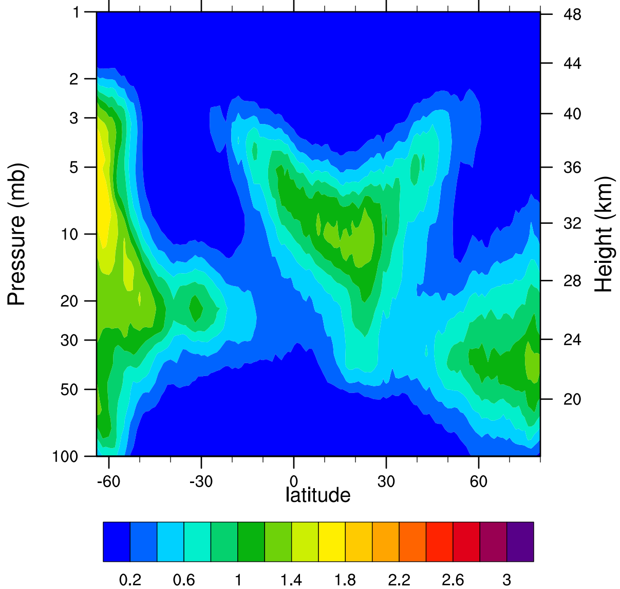
HIRDLSv6 2005d058 ClONO2_Ascending (ppbv)
