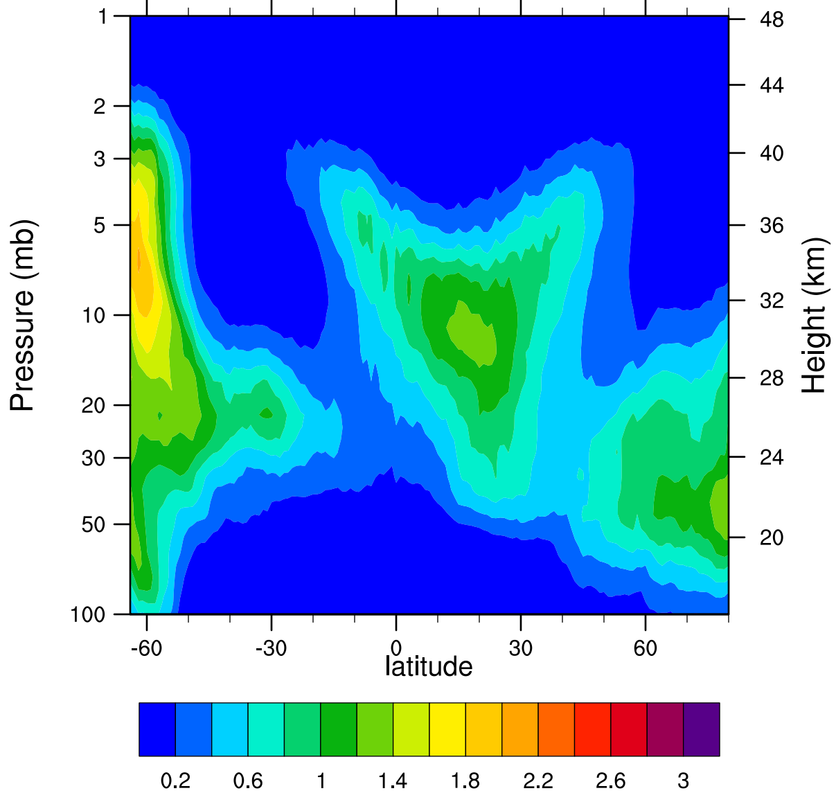
HIRDLSv6 2005d070 ClONO2_Ascending (ppbv)
