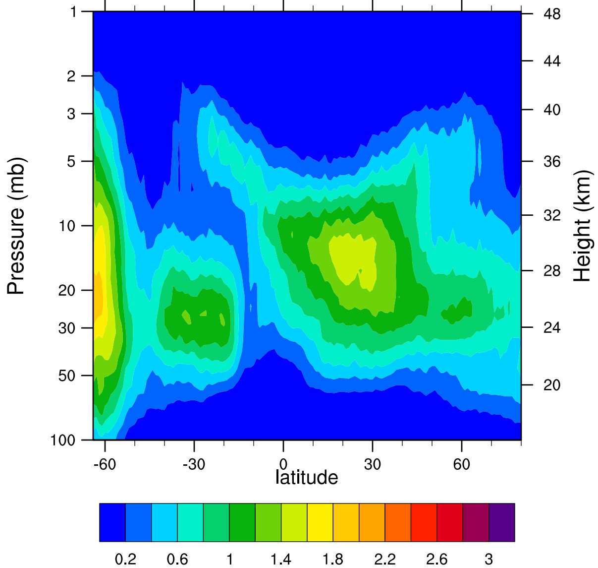
HIRDLSv6 2005d249 ClONO2_Ascending (ppbv)
