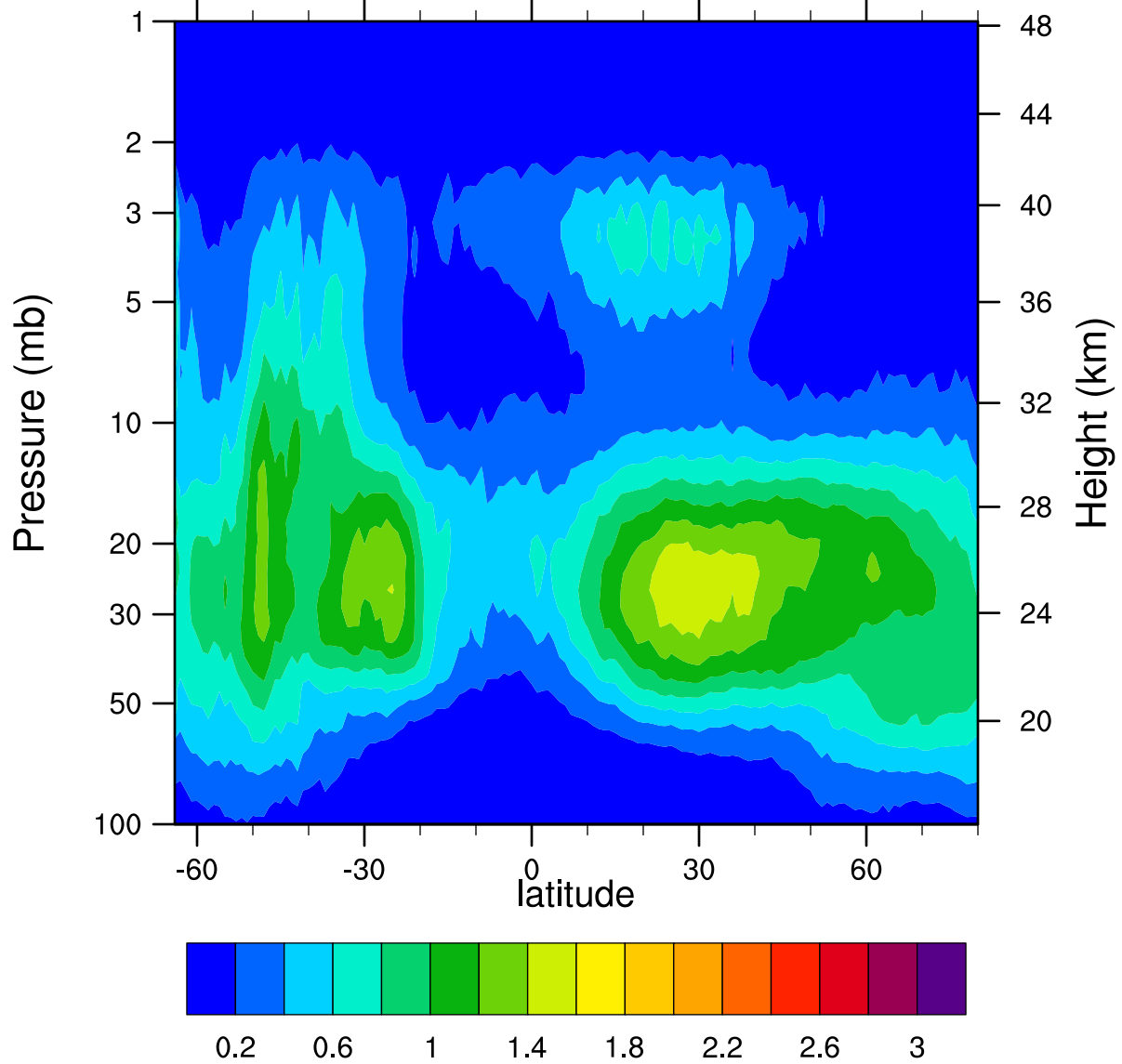
HIRDLSv6 2007d163 ClONO2_Ascending (ppbv)
