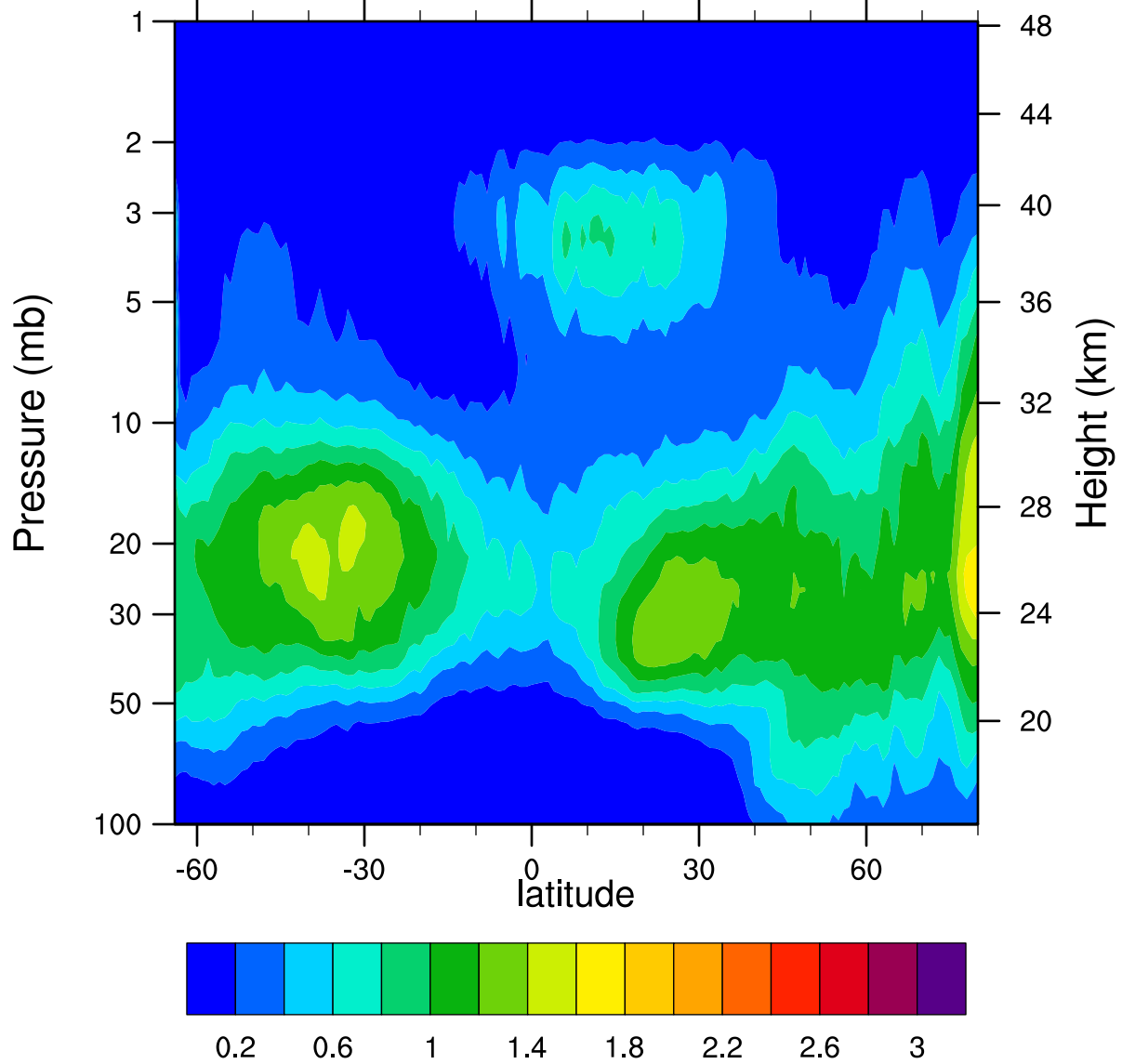
HIRDLSv6 2007d032 ClONO2_Ascending (ppbv)
