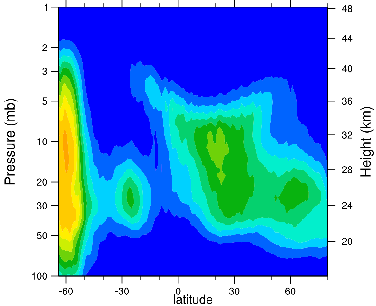
HIRDLSv6 2005d161 ClONO2_Ascending (ppbv)
