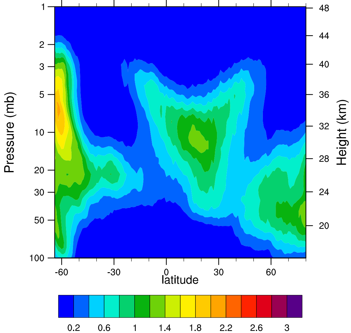
HIRDLSv6 2005d071 ClONO2_Ascending (ppbv)
