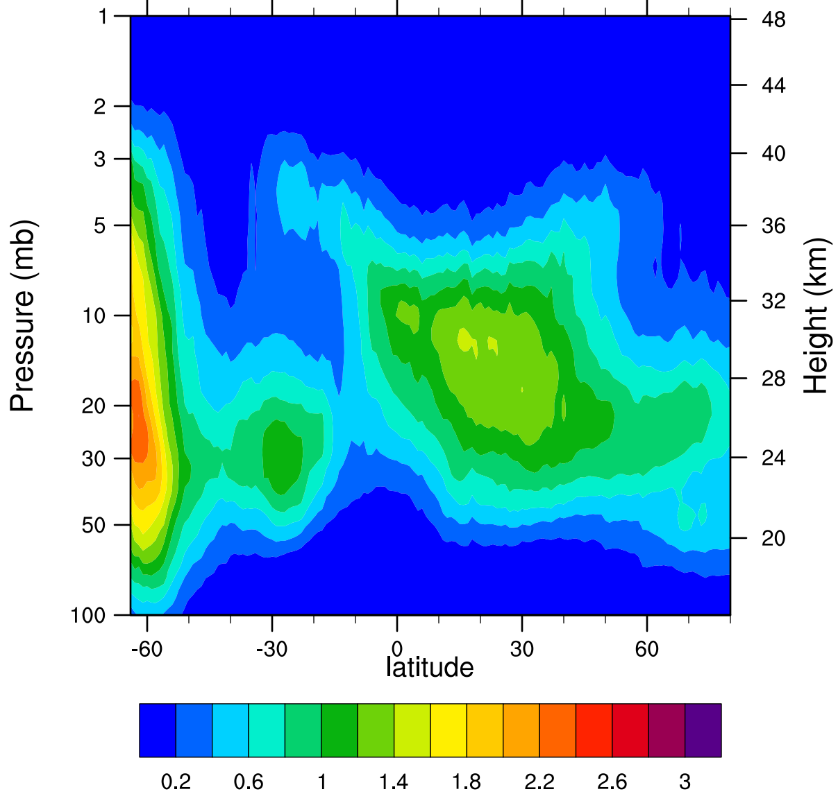
HIRDLSv6 2005d215 ClONO2_Ascending (ppbv)
