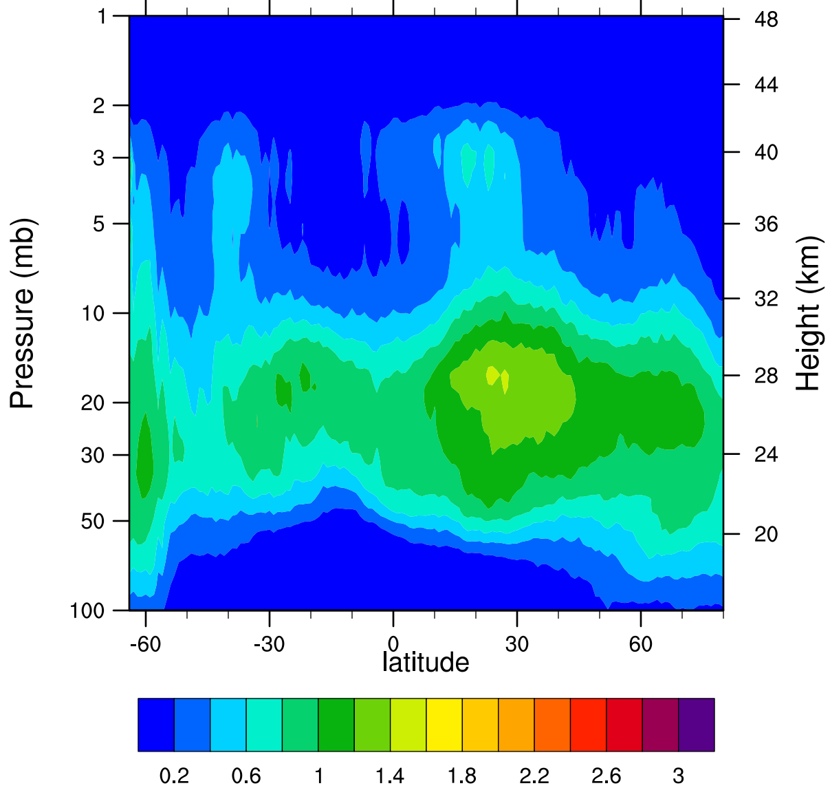
HIRDLSv6 2006d139 ClONO2_Ascending (ppbv)
