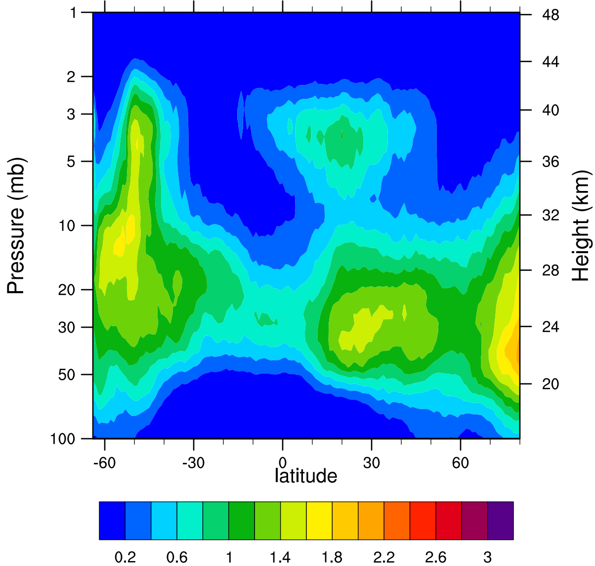
HIRDLSv6 2007d096 ClONO2_Ascending (ppbv)
