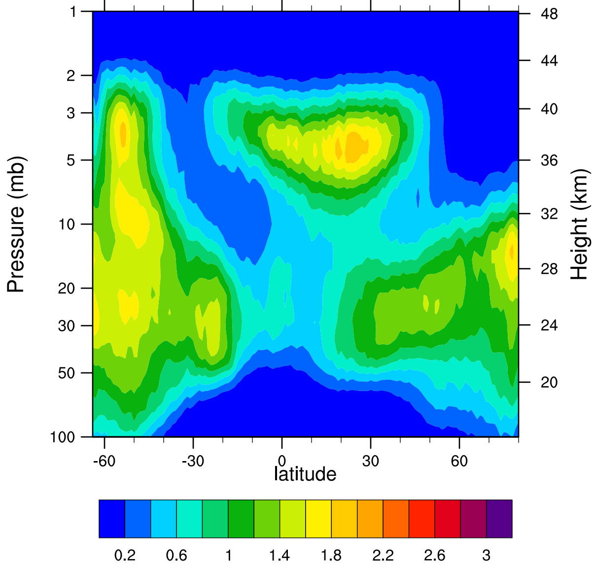
HIRDLSv6 2007d282 ClONO2_Ascending (ppbv)
