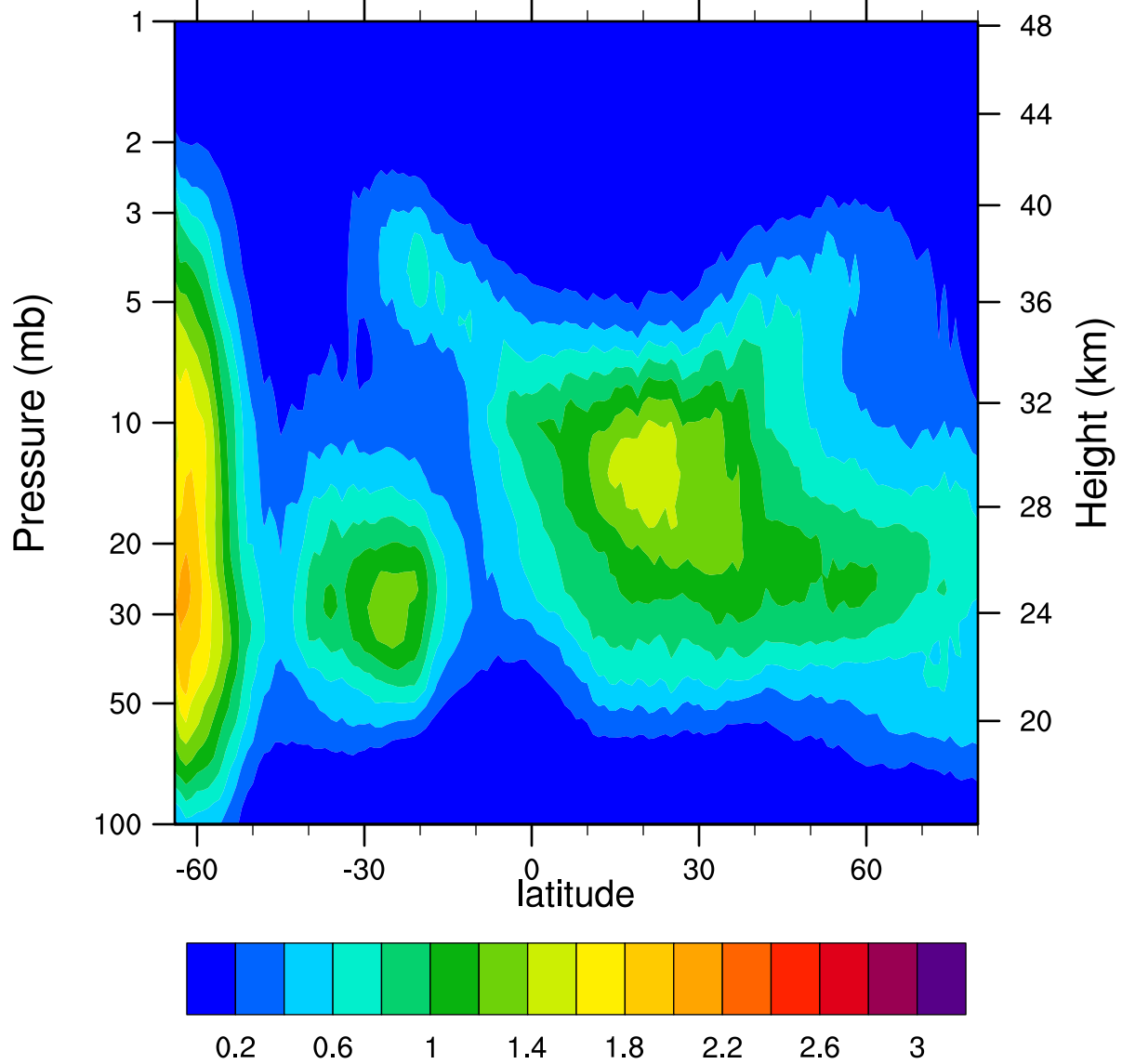
HIRDLSv6 2005d235 ClONO2_Ascending (ppbv)
