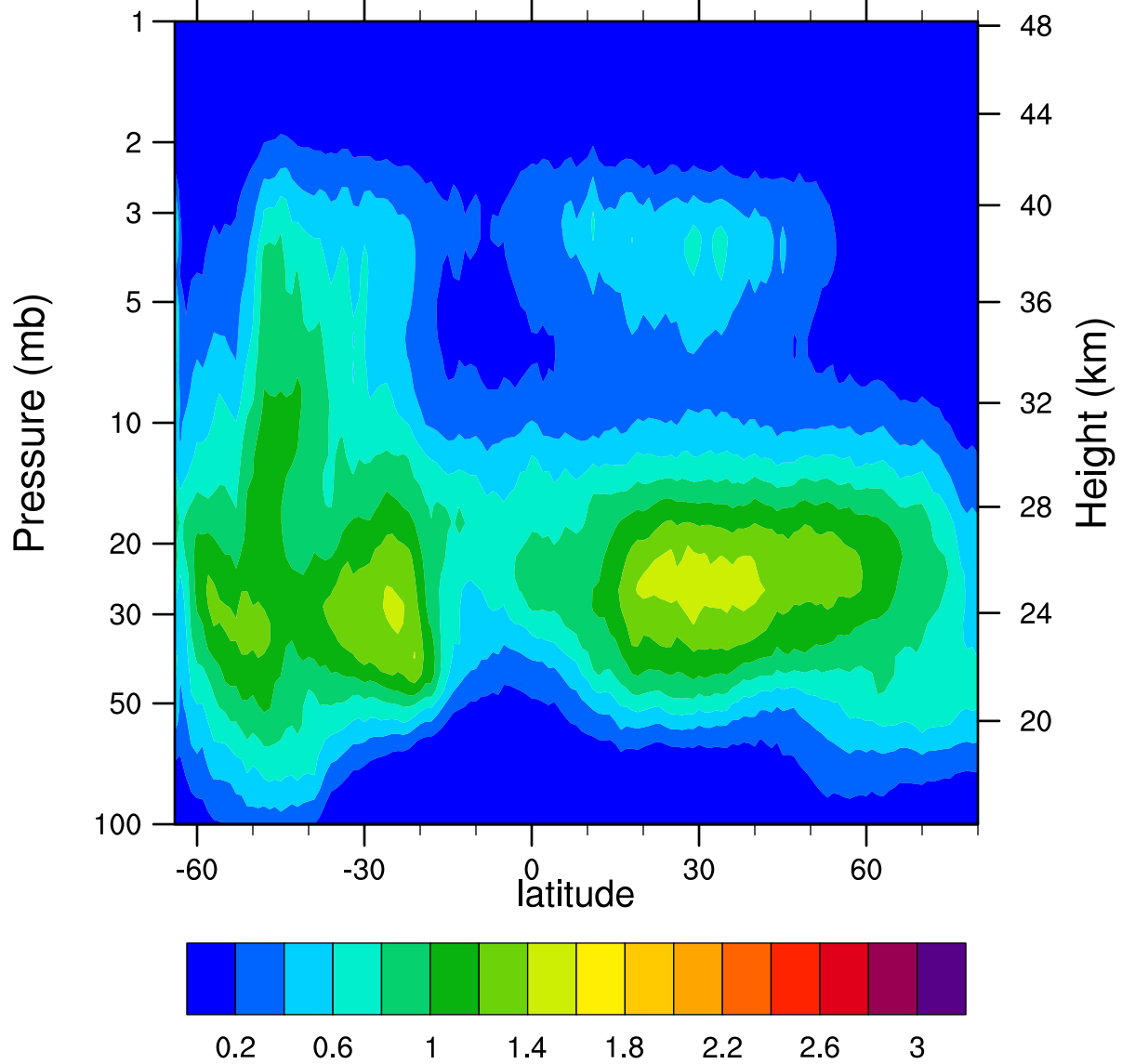
HIRDLSv6 2007d190 ClONO2_Ascending (ppbv)
