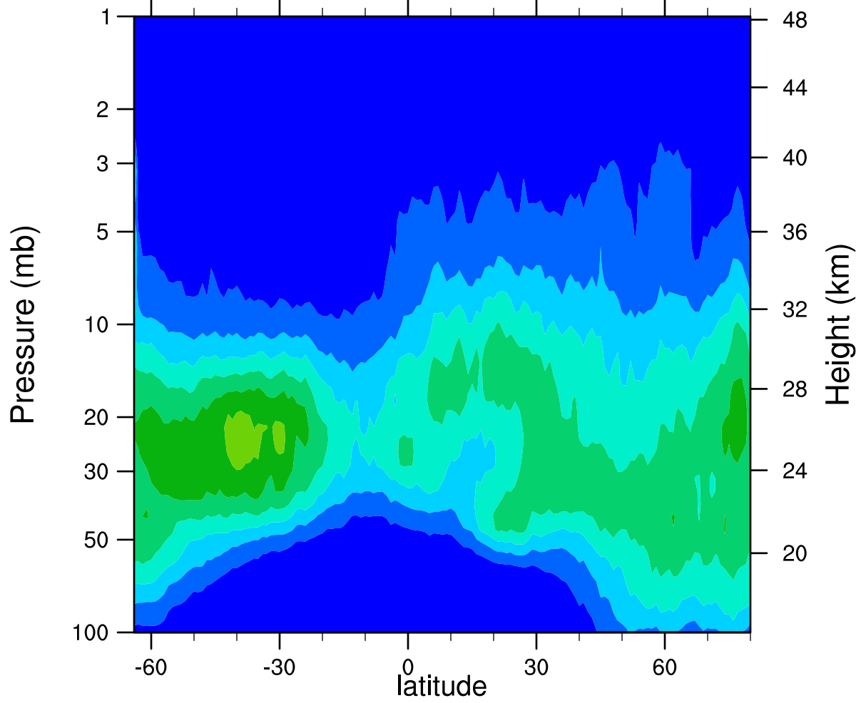
HIRDLSv6 2006d013 ClONO2_Ascending (ppbv)
