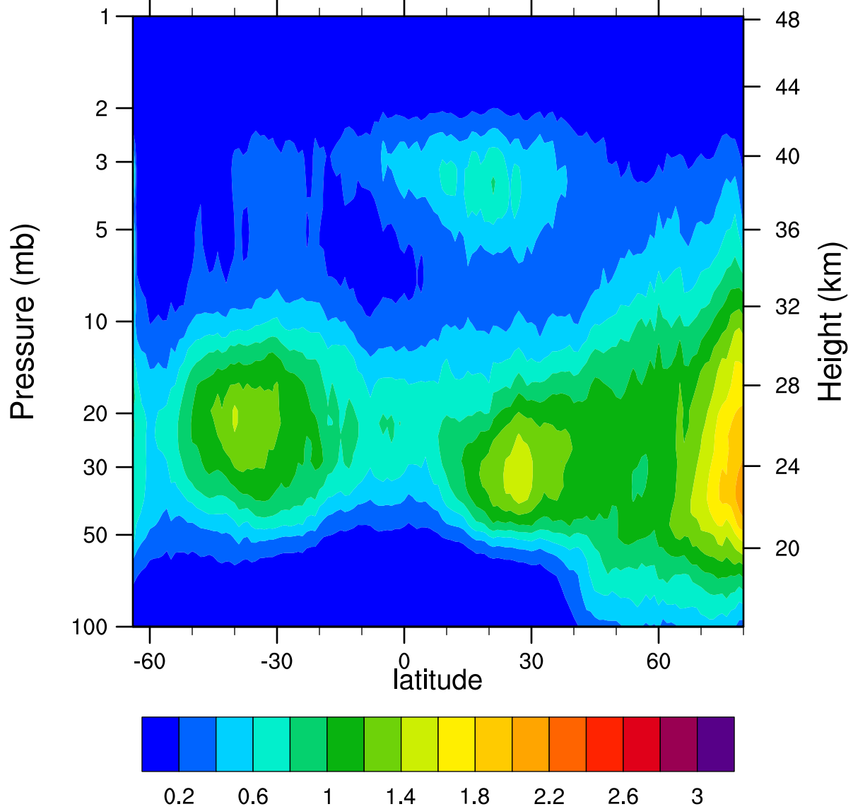
HIRDLSv6 2007d066 ClONO2_Ascending (ppbv)
