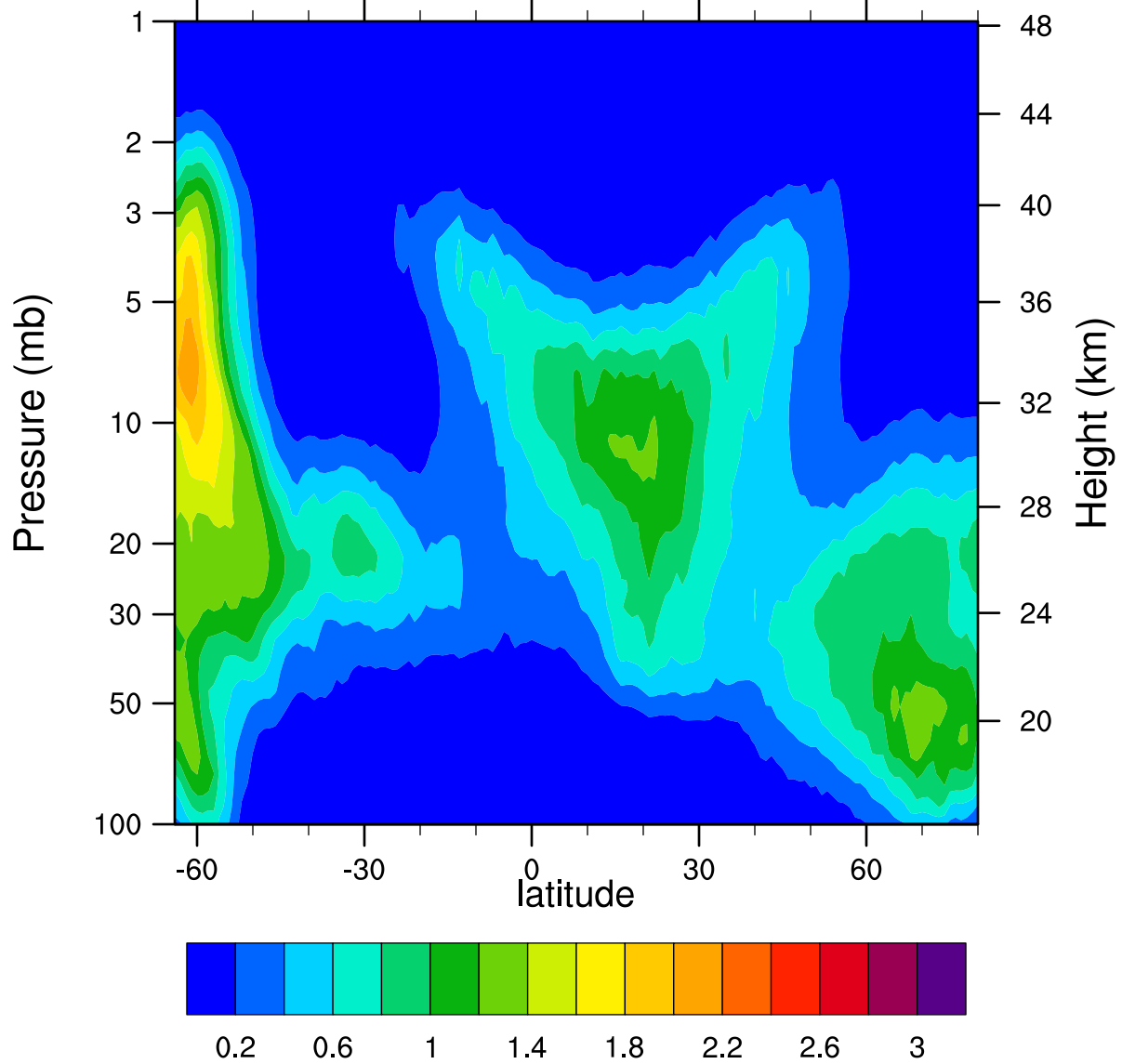
HIRDLSv6 2005d076 ClONO2_Ascending (ppbv)
