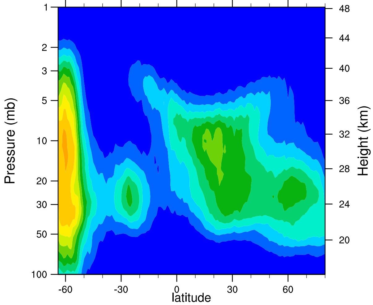
HIRDLSv6 2005d162 ClONO2_Ascending (ppbv)
