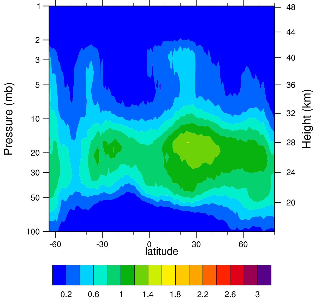
HIRDLSv6 2006d144 ClONO2_Ascending (ppbv)
