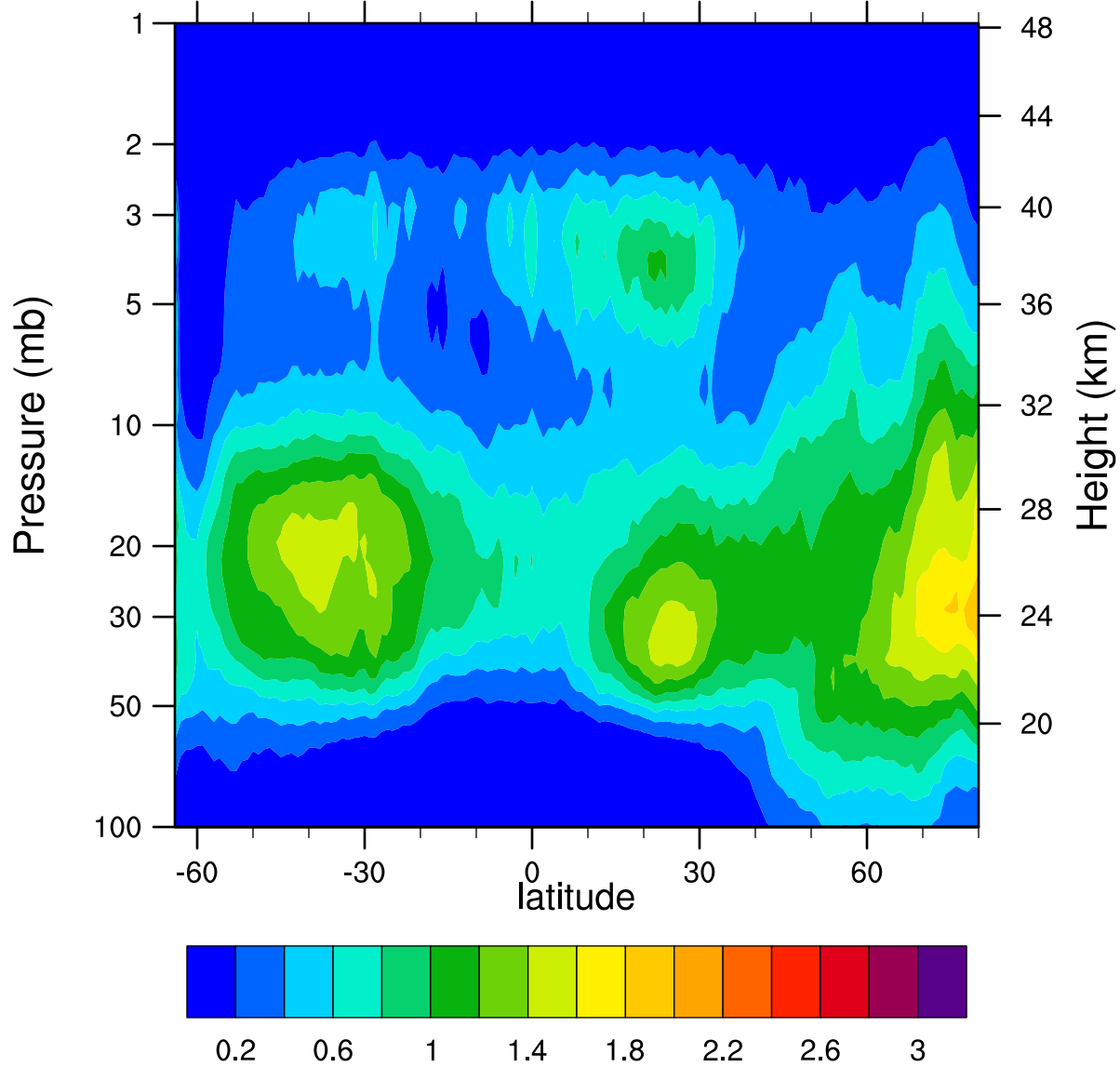
HIRDLSv6 2007d050 ClONO2_Ascending (ppbv)
