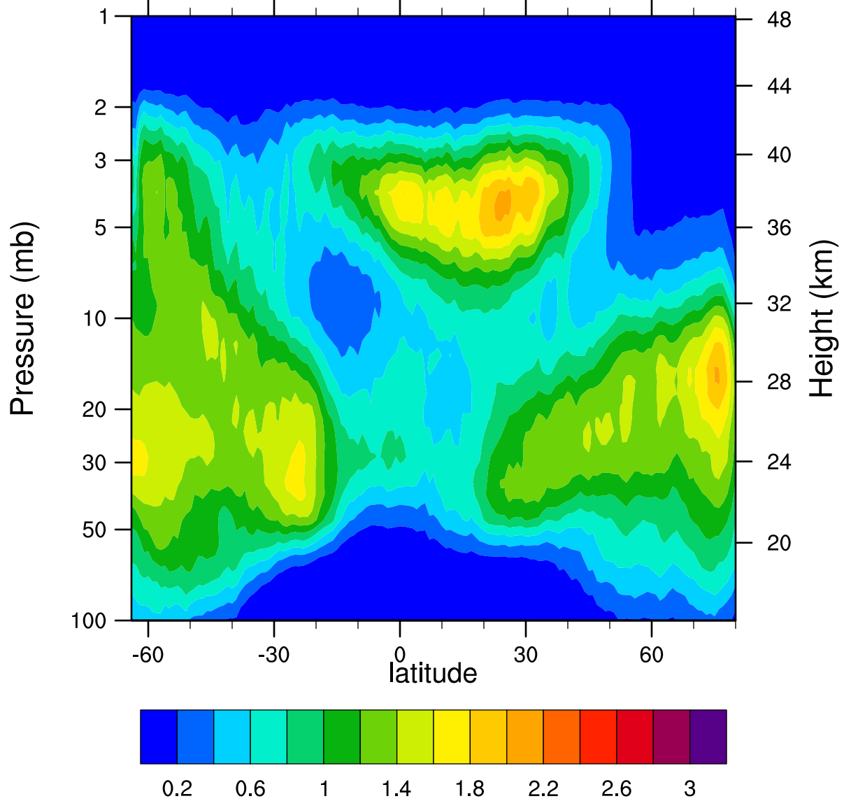
HIRDLSv6 2007d293 ClONO2_Ascending (ppbv)
