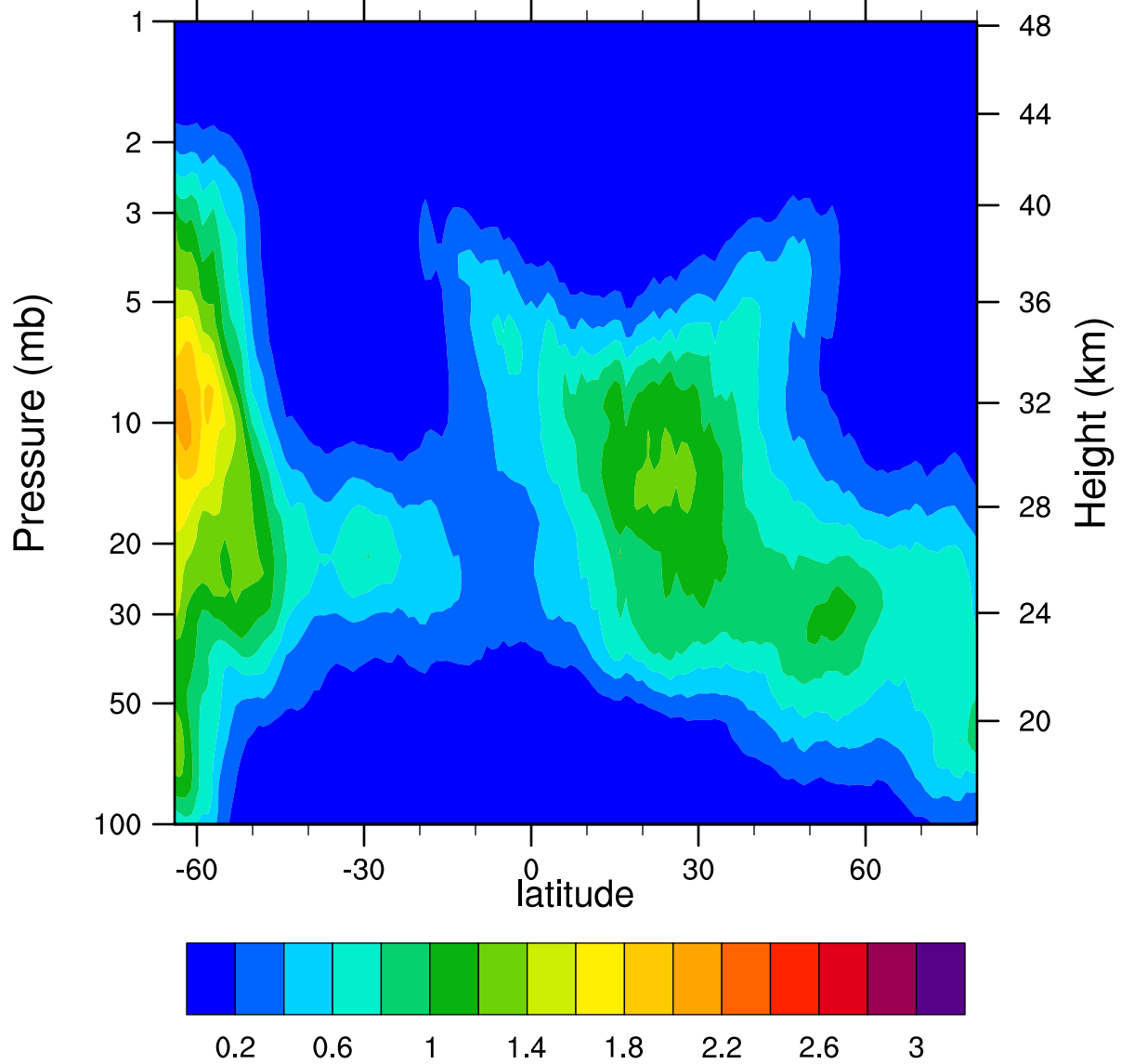
HIRDLSv6 2005d104 ClONO2_Ascending (ppbv)
