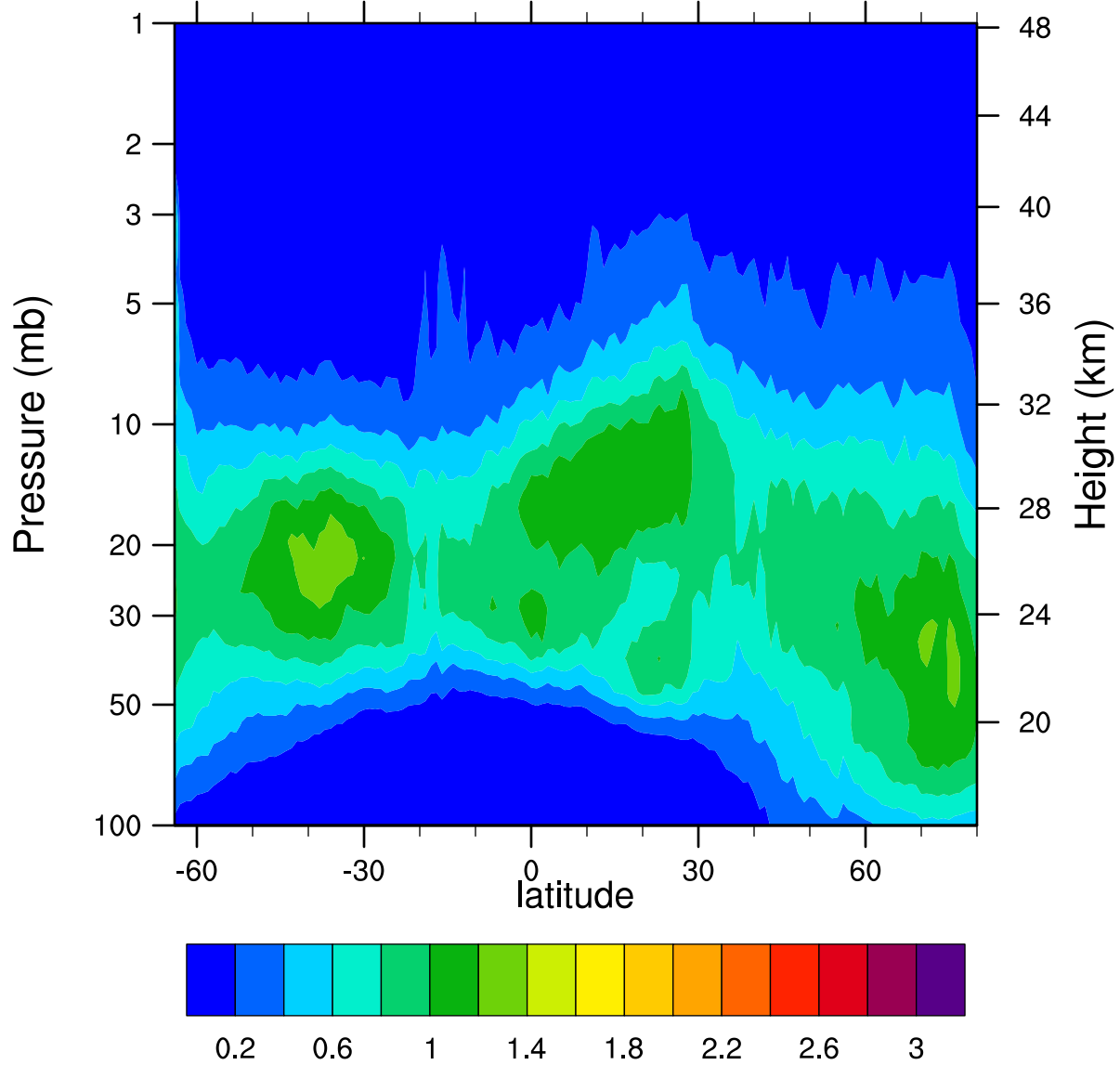
HIRDLSv6 2006d059 ClONO2_Ascending (ppbv)
