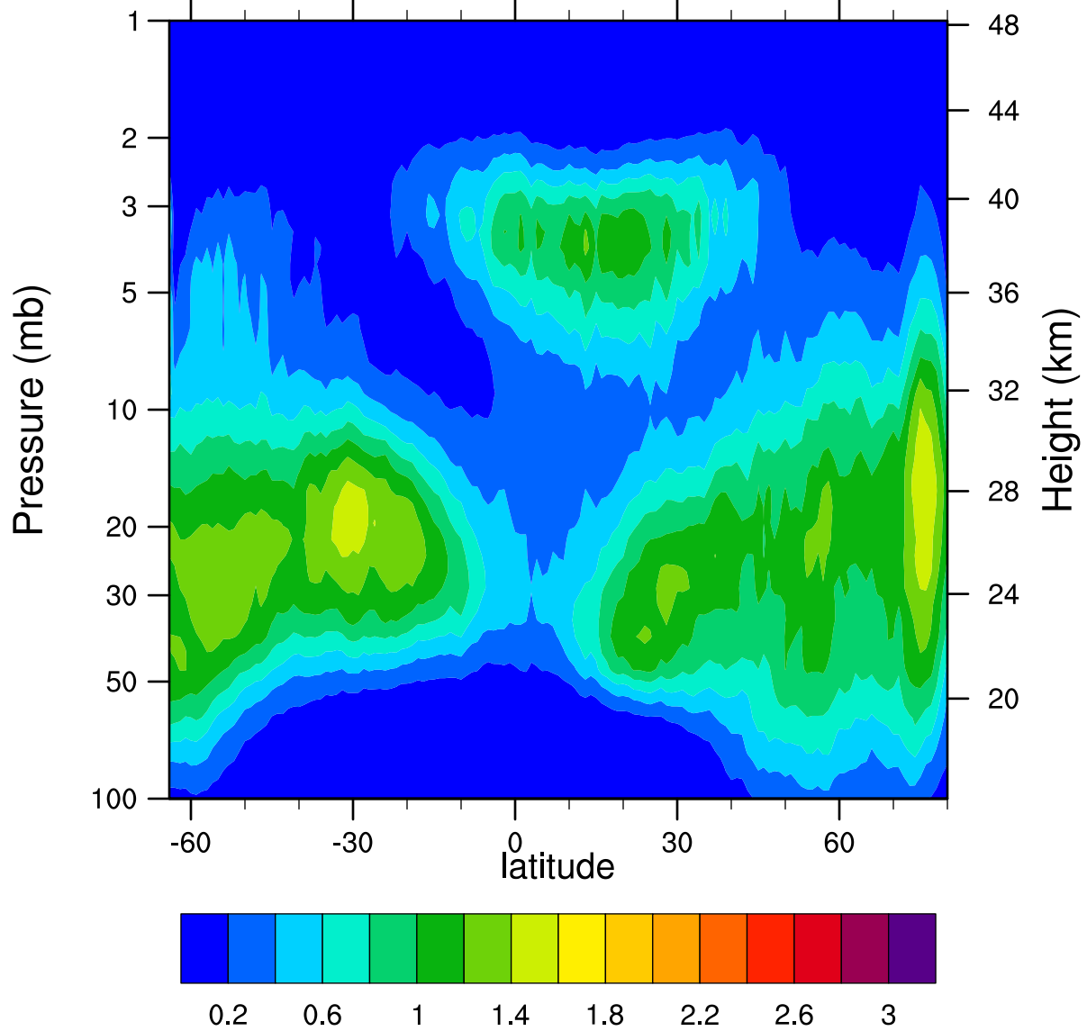
HIRDLSv6 2006d358 ClONO2_Ascending (ppbv)
