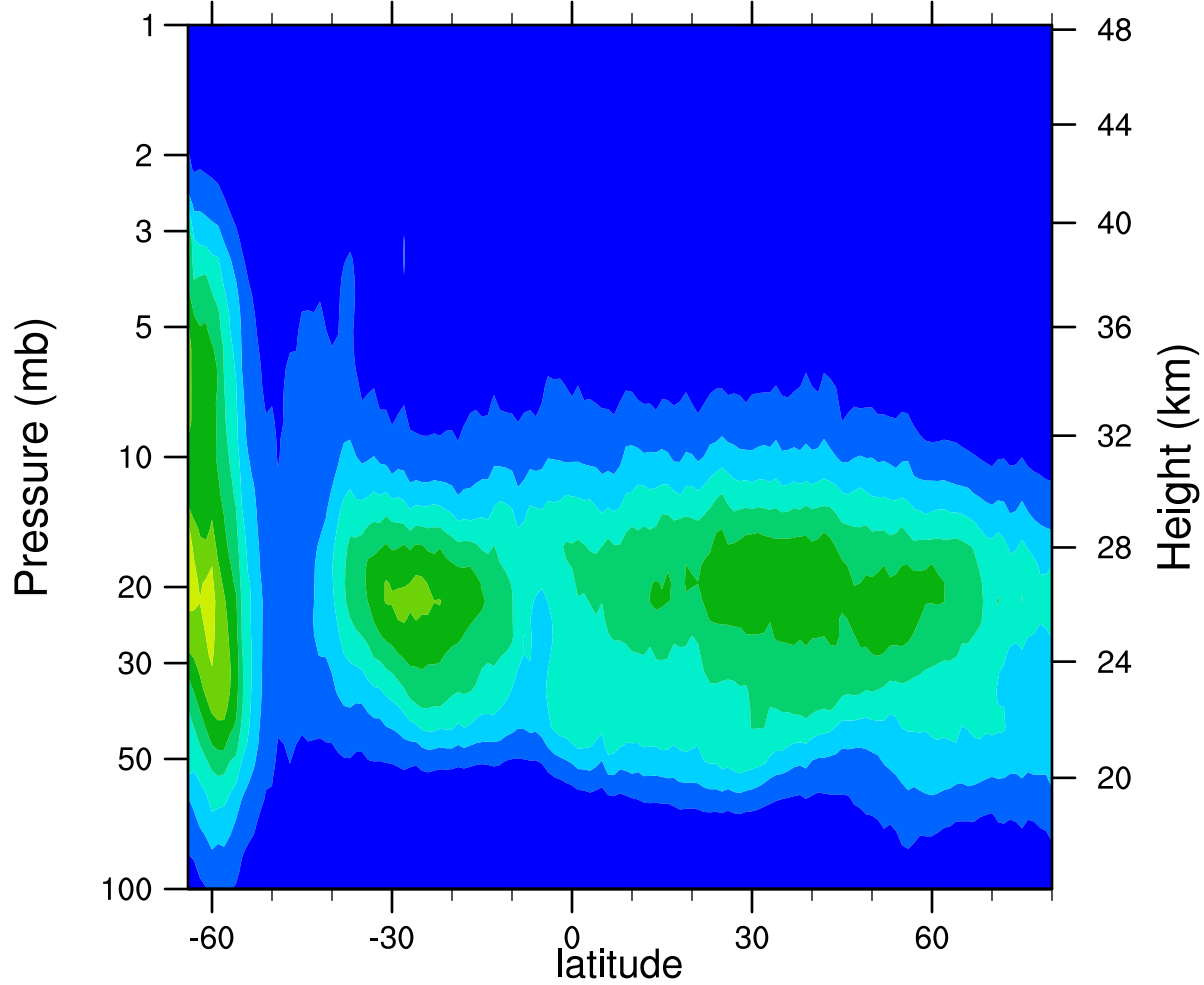
HIRDLSv6 2006d193 ClONO2_Ascending (ppbv)
