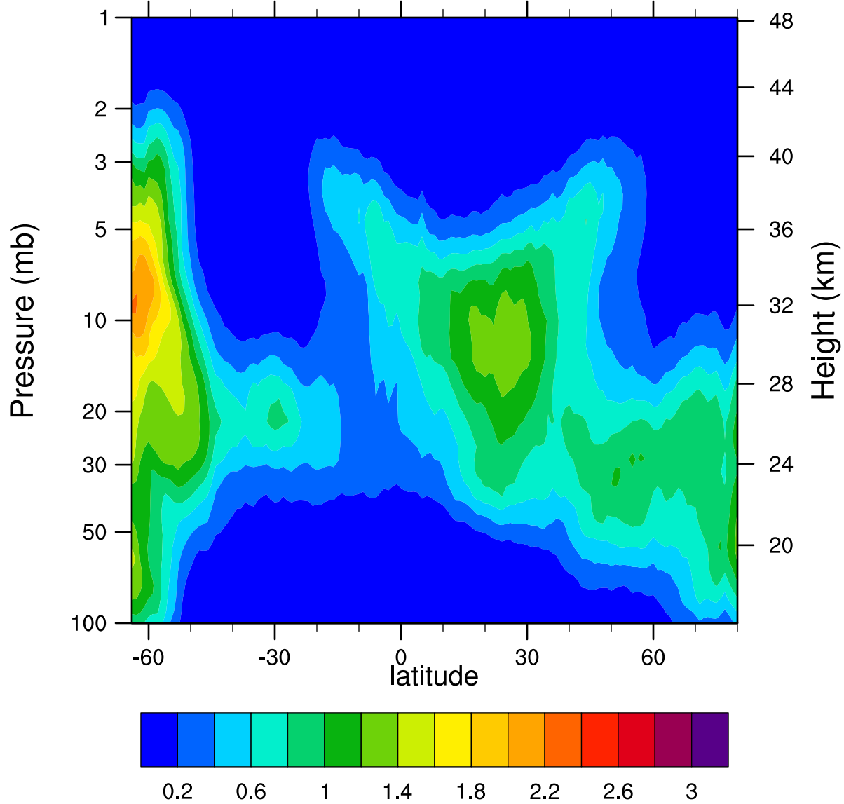
HIRDLSv6 2005d090 ClONO2_Ascending (ppbv)
