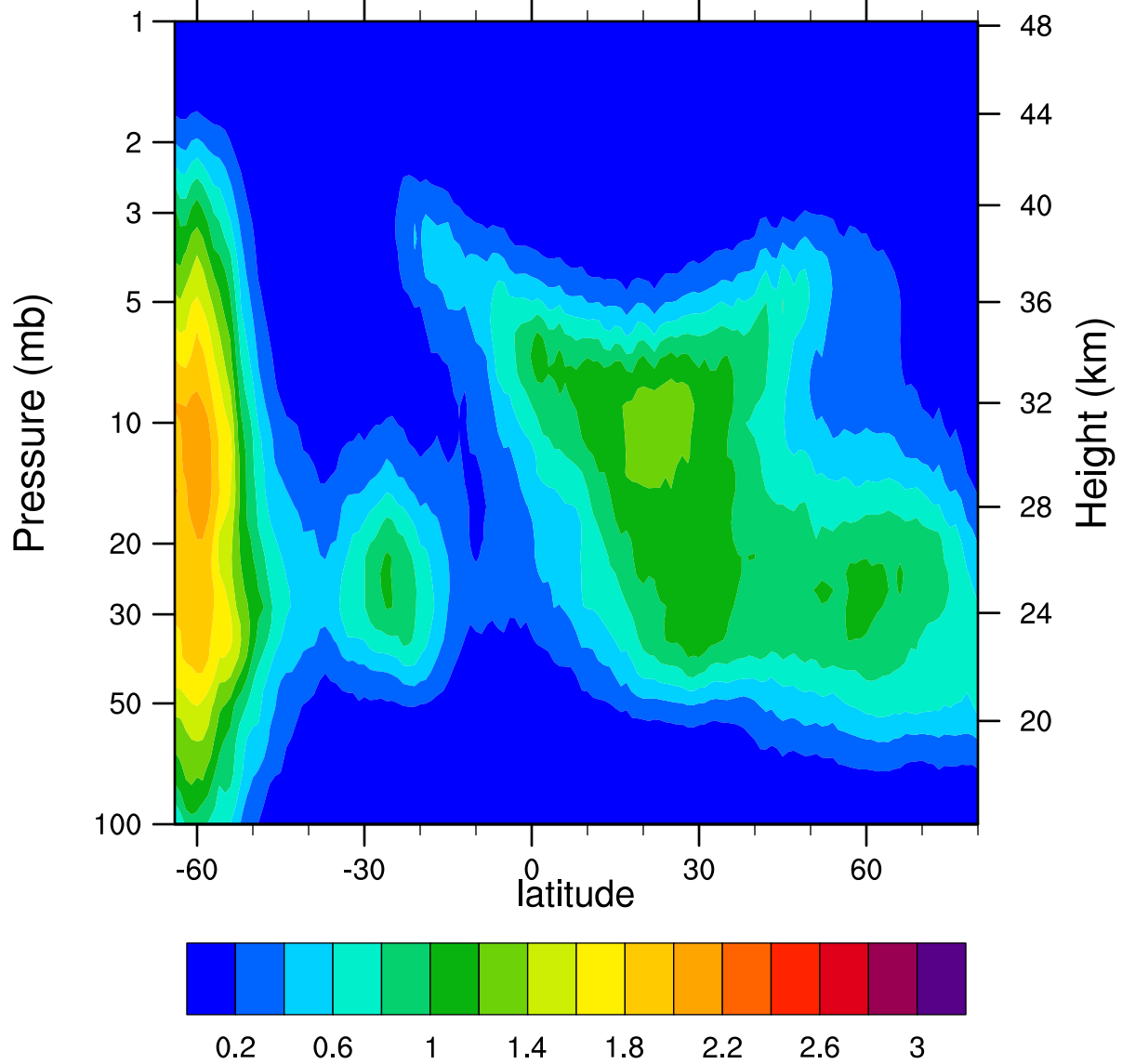
HIRDLSv6 2005d154 ClONO2_Ascending (ppbv)
