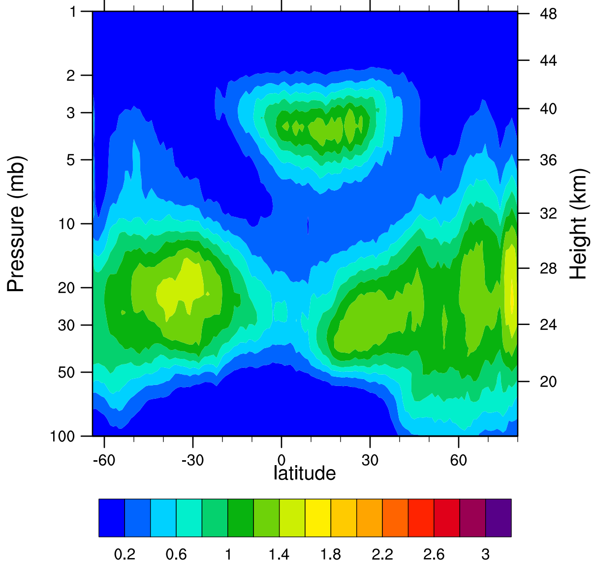
HIRDLSv6 2007d026 ClONO2_Ascending (ppbv)
