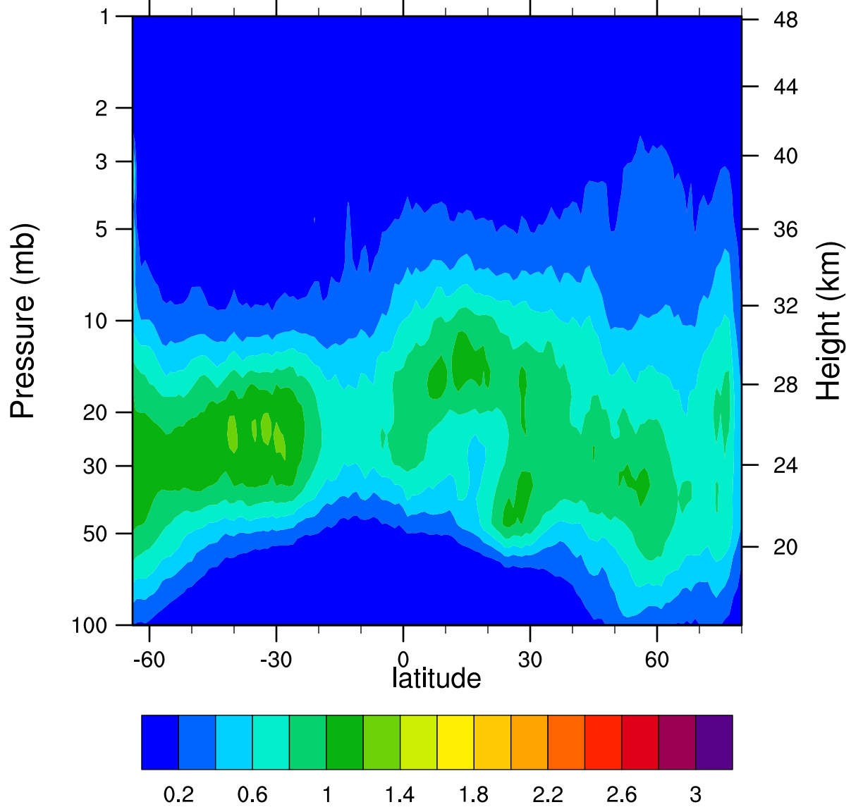
HIRDLSv6 2005d365 ClONO2_Ascending (ppbv)
