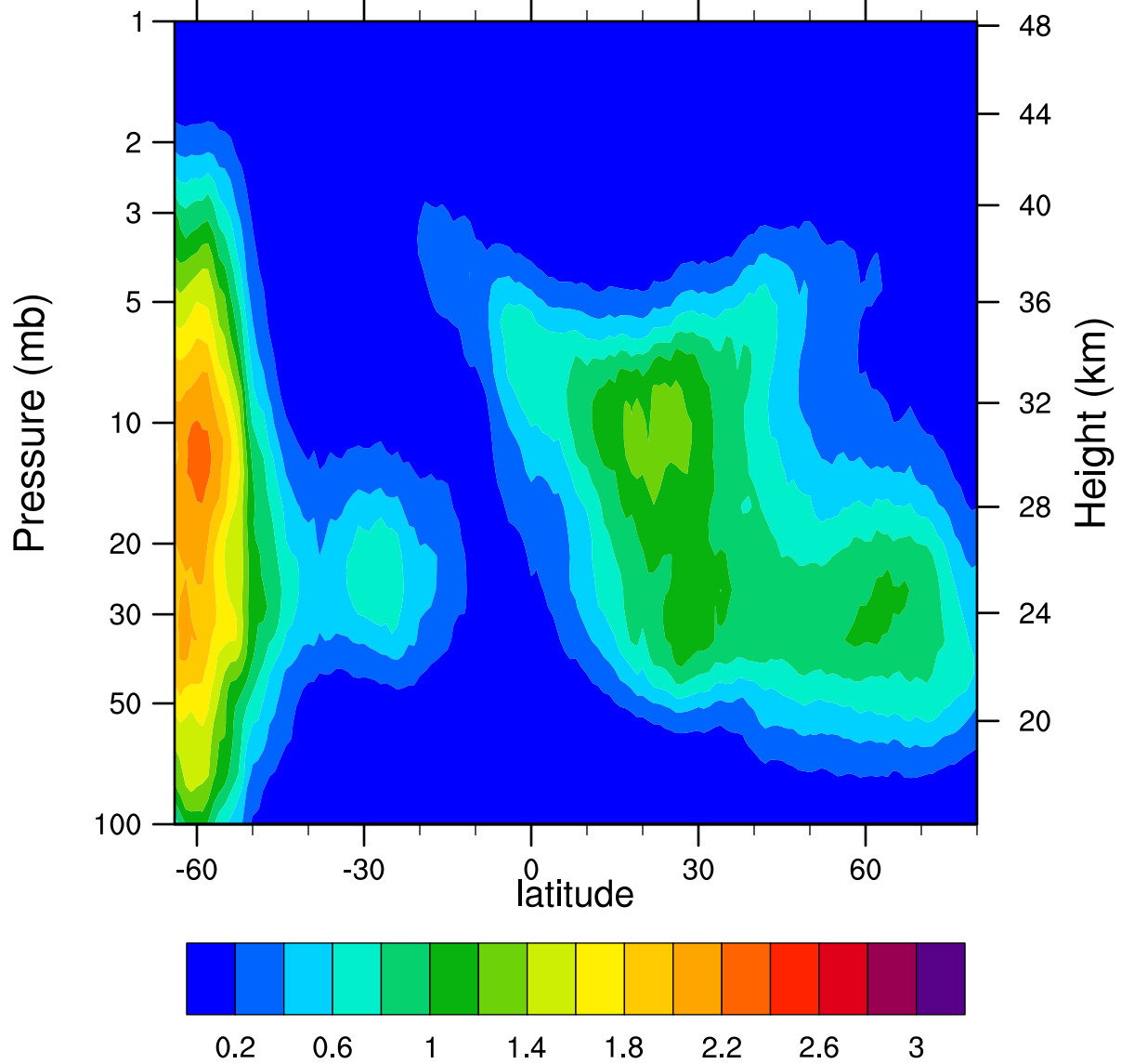
HIRDLSv6 2005d136 ClONO2_Ascending (ppbv)
