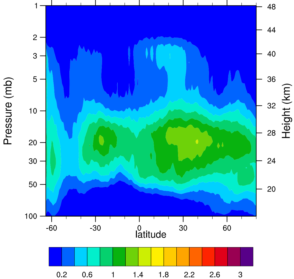
HIRDLSv6 2006d155 ClONO2_Ascending (ppbv)
