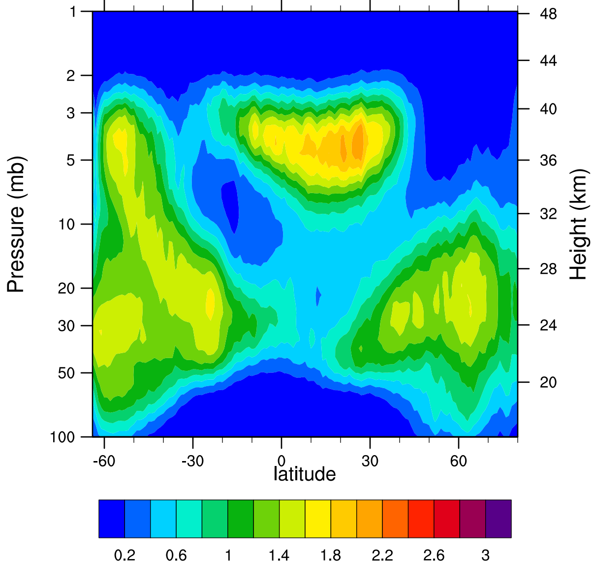
HIRDLSv6 2007d325 ClONO2_Ascending (ppbv)
