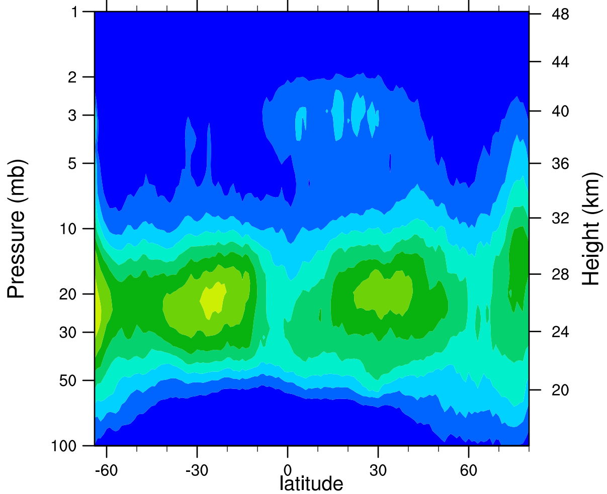
HIRDLSv6 2006d294 ClONO2_Ascending (ppbv)
