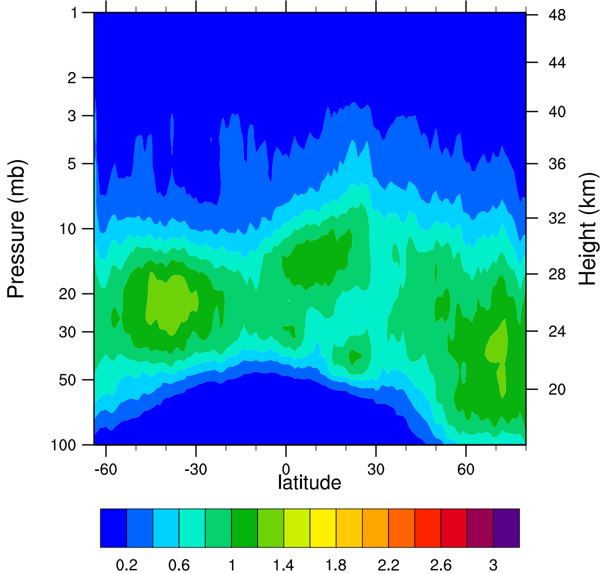
HIRDLSv6 2006d050 ClONO2_Ascending (ppbv)
