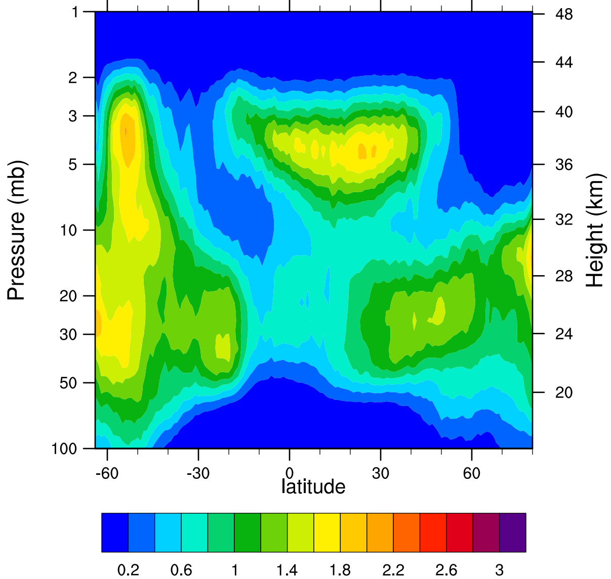
HIRDLSv6 2007d275 ClONO2_Ascending (ppbv)
