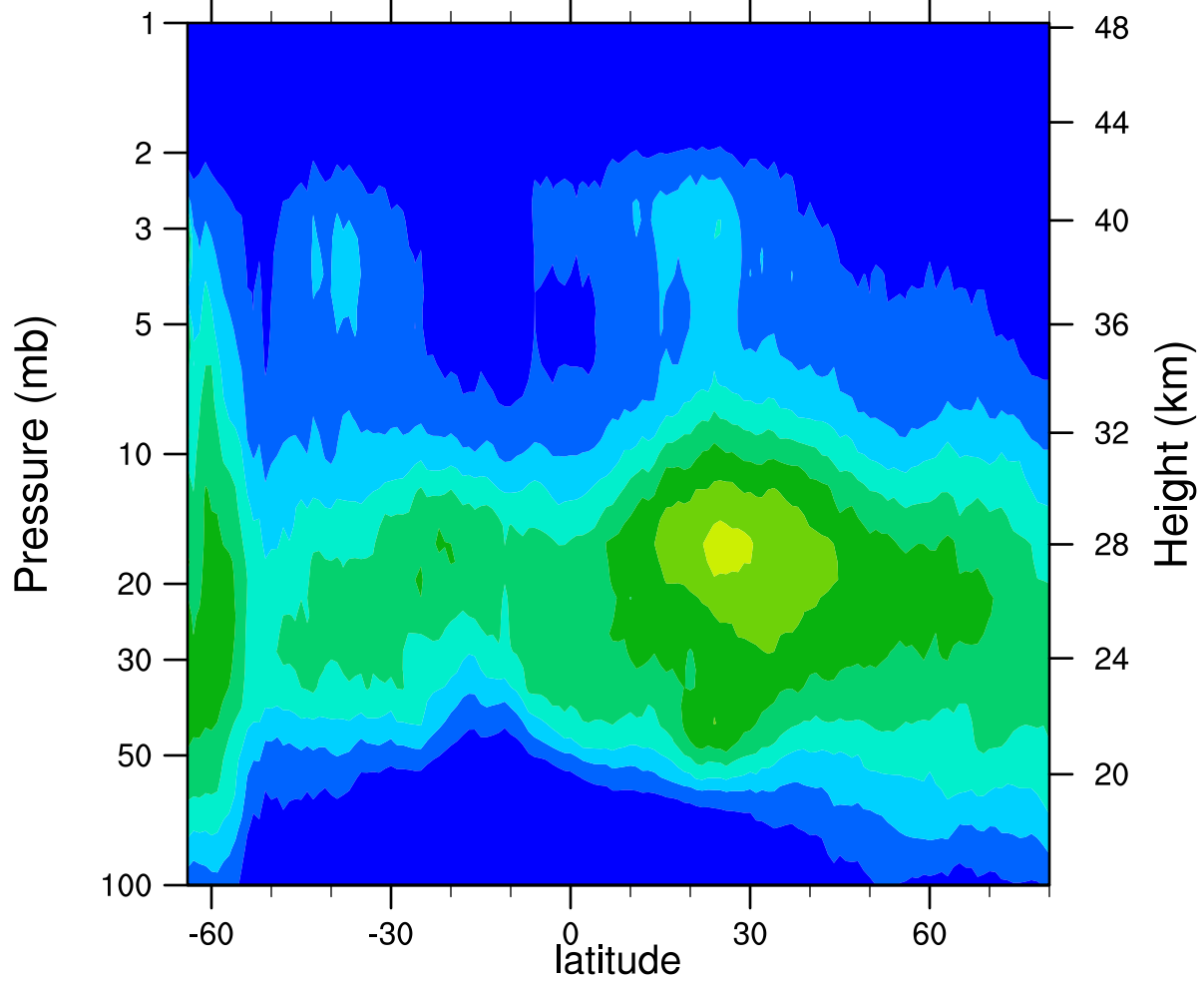
HIRDLSv6 2006d131 ClONO2_Ascending (ppbv)
