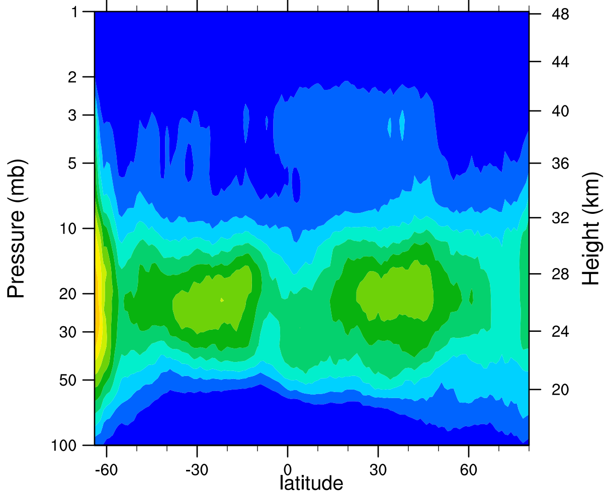
HIRDLSv6 2006d271 ClONO2_Ascending (ppbv)
