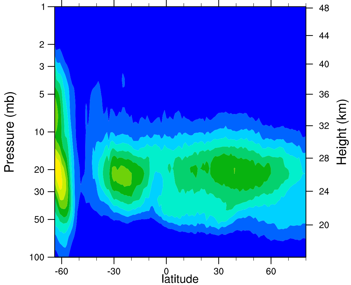
HIRDLSv6 2006d206 ClONO2_Ascending (ppbv)
