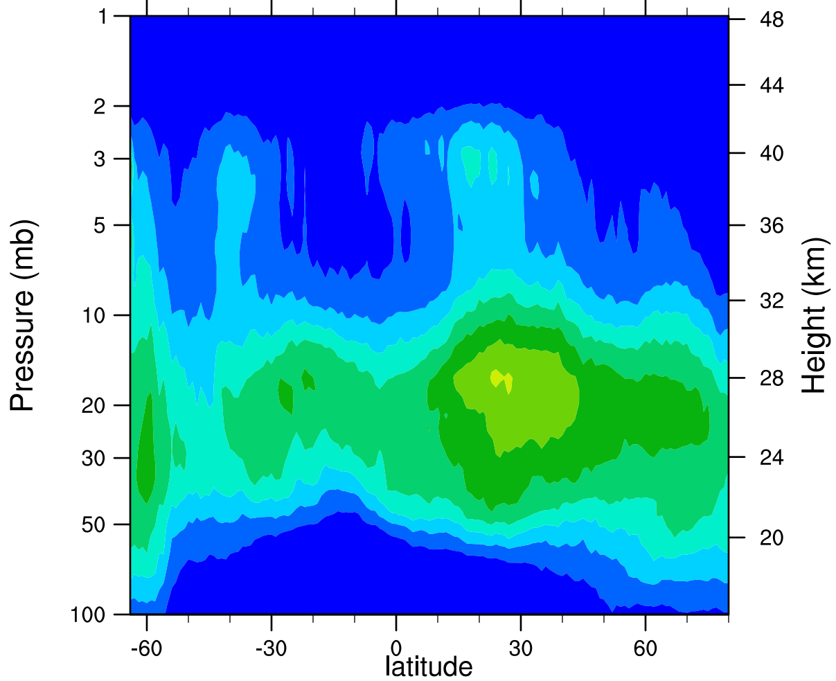
HIRDLSv6 2006d138 ClONO2_Ascending (ppbv)
