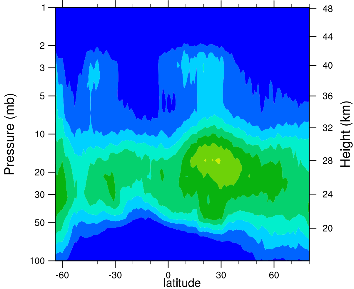
HIRDLSv6 2006d122 ClONO2_Ascending (ppbv)
