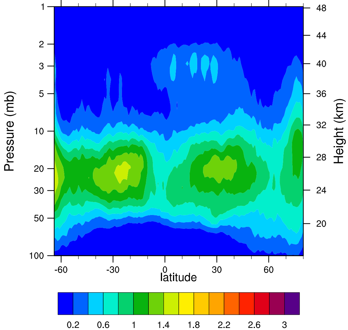
HIRDLSv6 2006d295 ClONO2_Ascending (ppbv)
