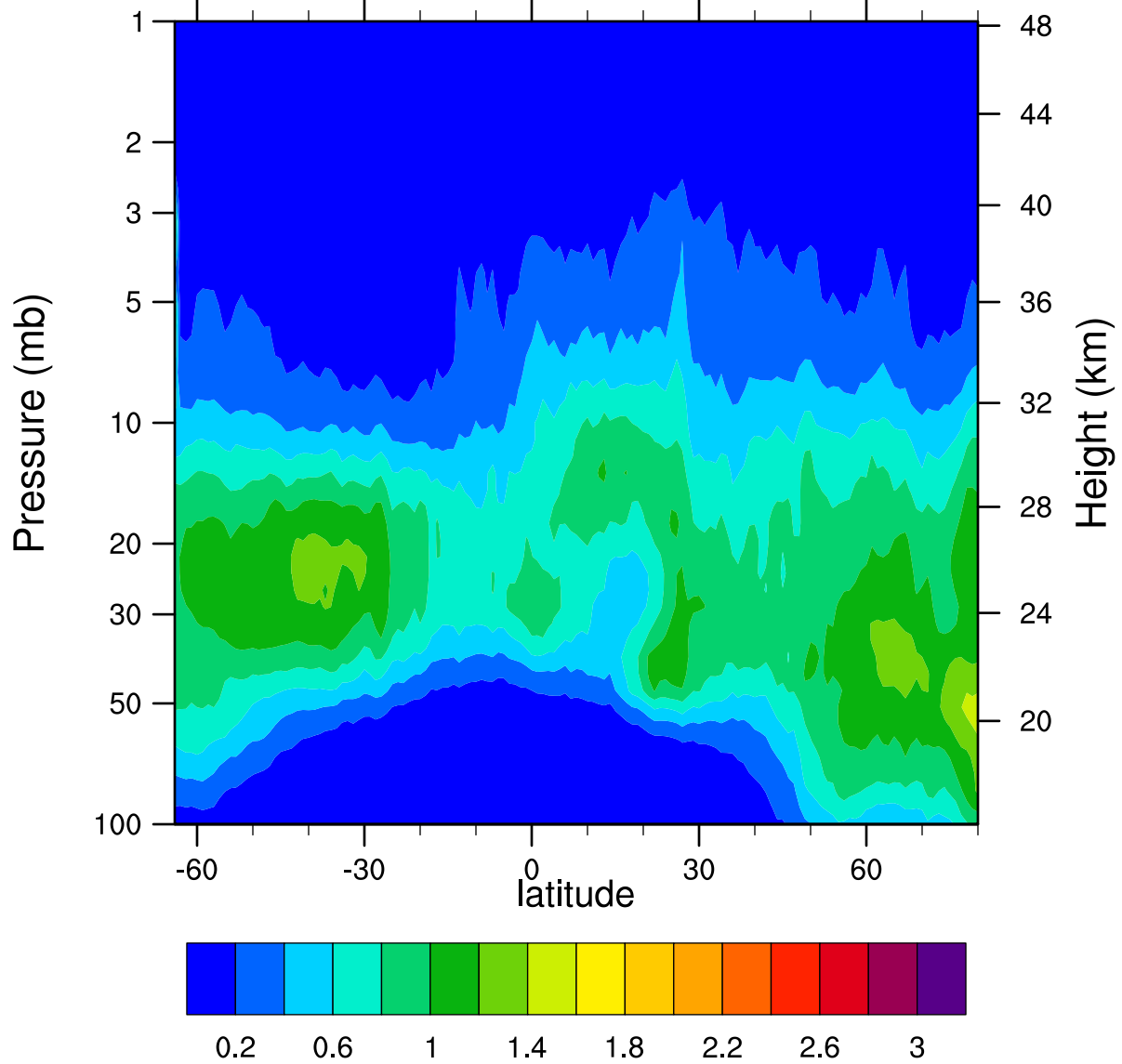
HIRDLSv6 2006d030 ClONO2_Ascending (ppbv)
