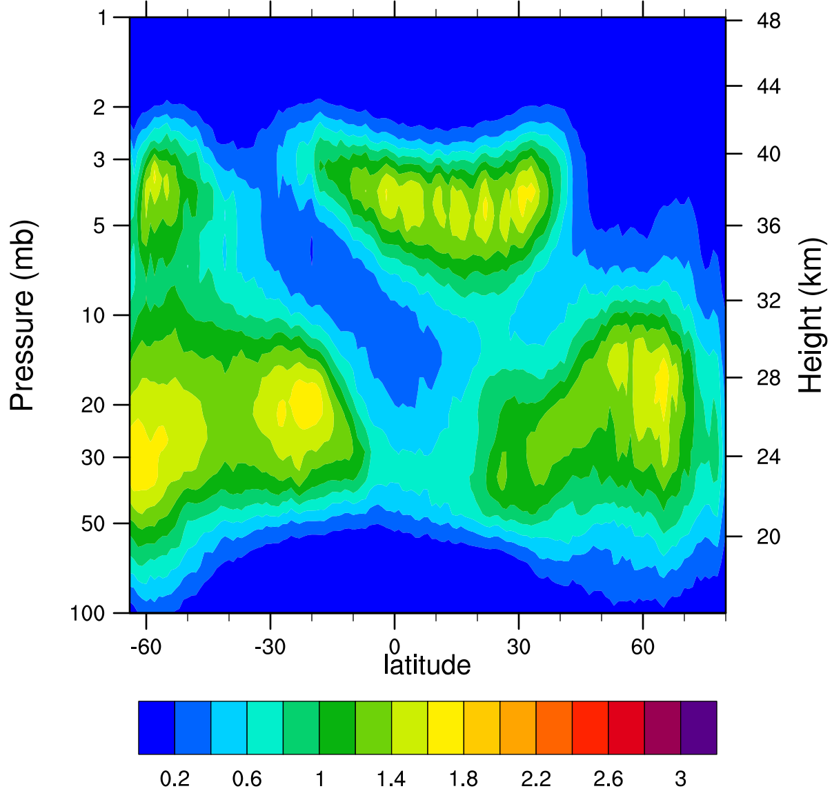
HIRDLSv6 2006d328 ClONO2_Ascending (ppbv)
