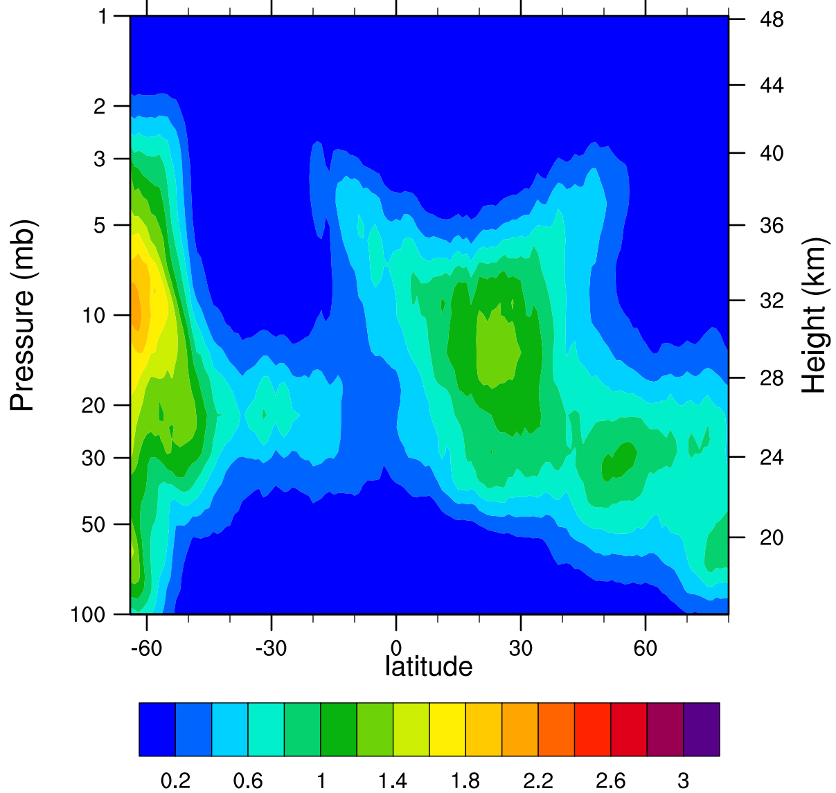
HIRDLSv6 2005d101 ClONO2_Ascending (ppbv)
