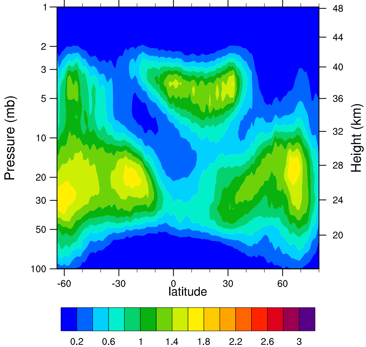
HIRDLSv6 2006d319 ClONO2_Ascending (ppbv)
