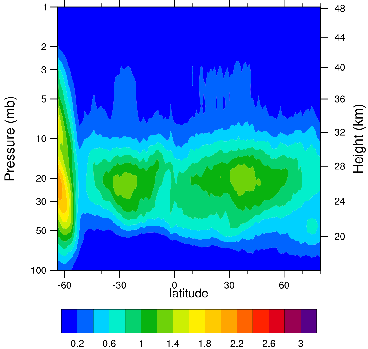
HIRDLSv6 2006d234 ClONO2_Ascending (ppbv)
