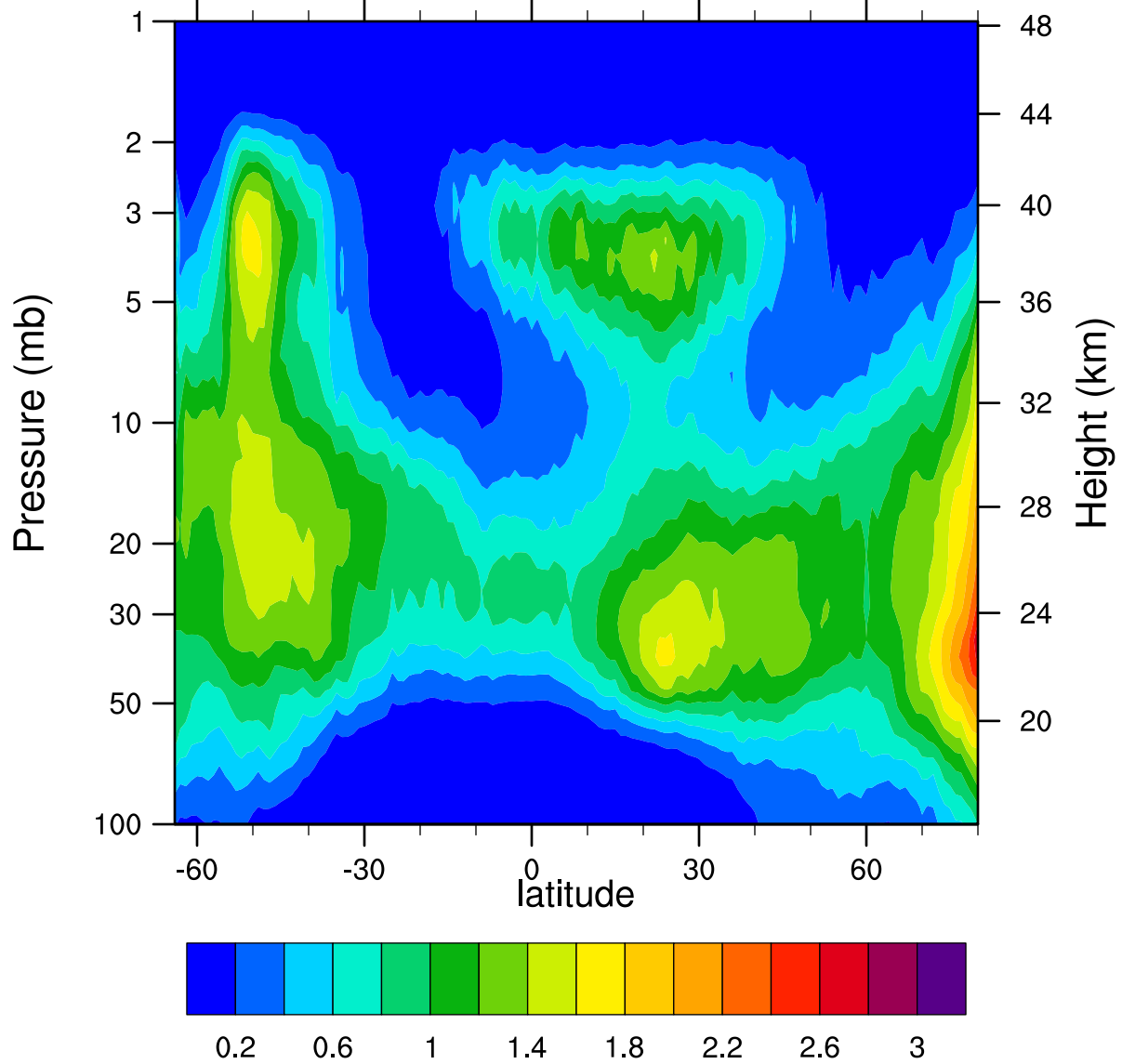
HIRDLSv6 2007d084 ClONO2_Ascending (ppbv)
