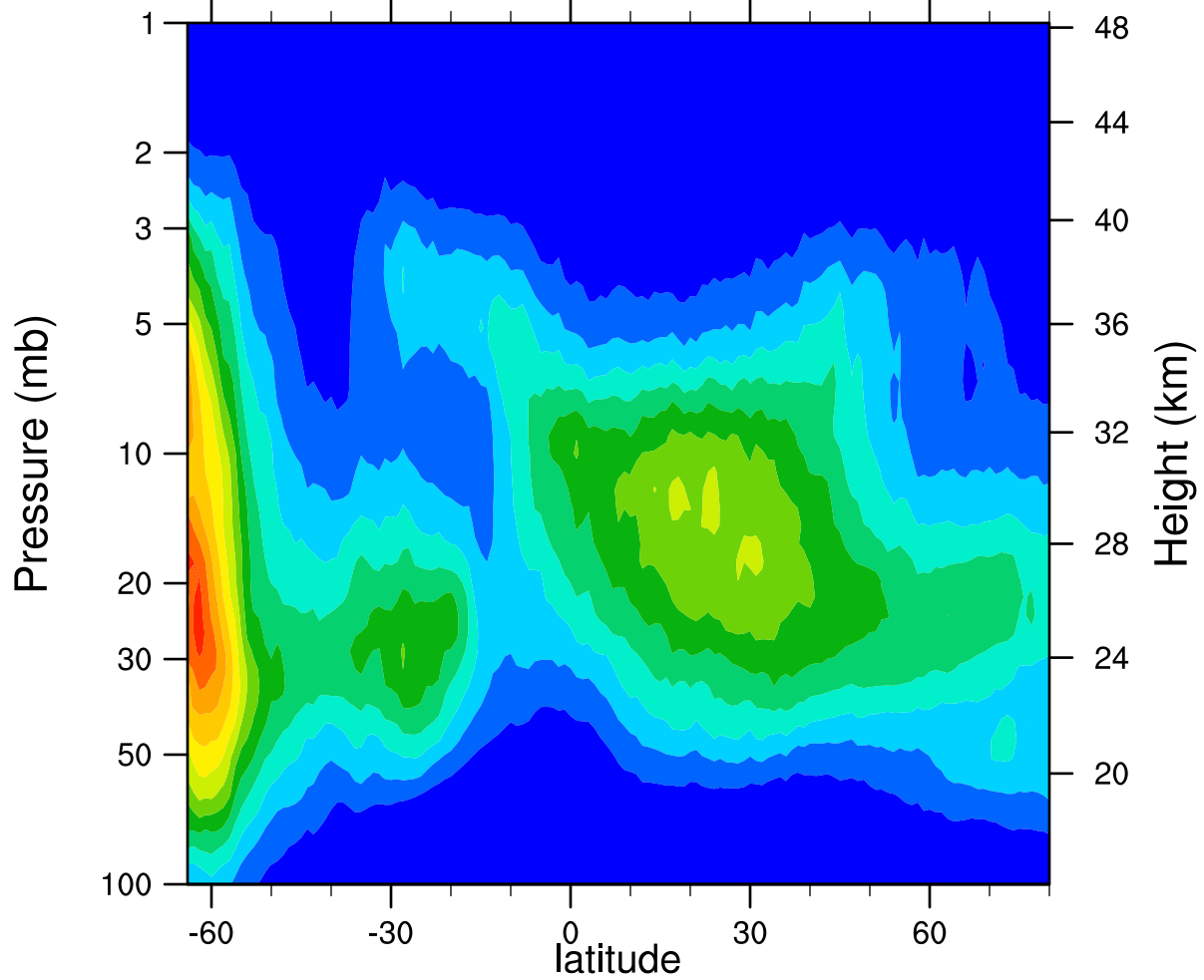
HIRDLSv6 2005d220 ClONO2_Ascending (ppbv)
