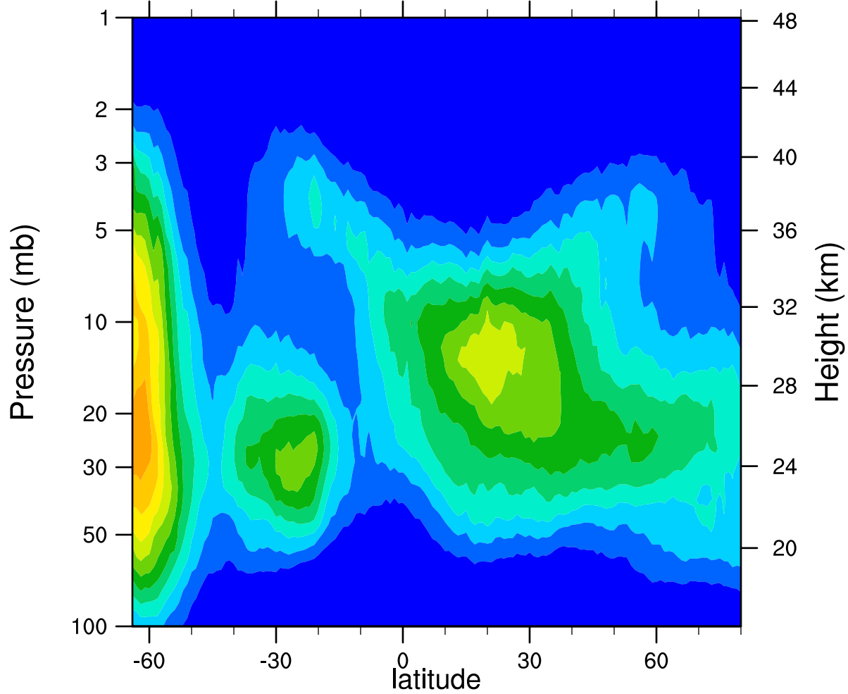
HIRDLSv6 2005d231 ClONO2_Ascending (ppbv)
