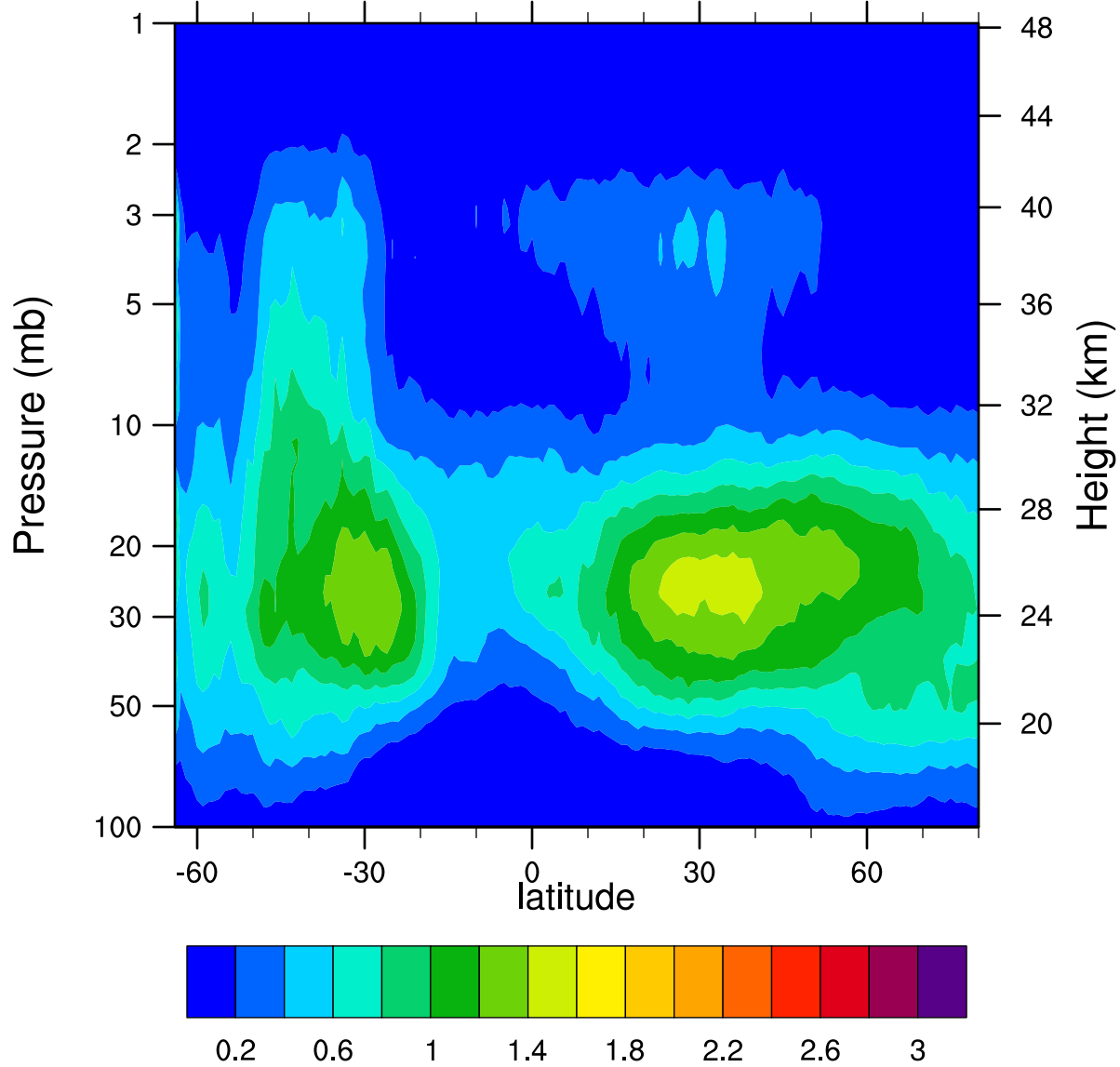
HIRDLSv6 2007d175 ClONO2_Ascending (ppbv)
