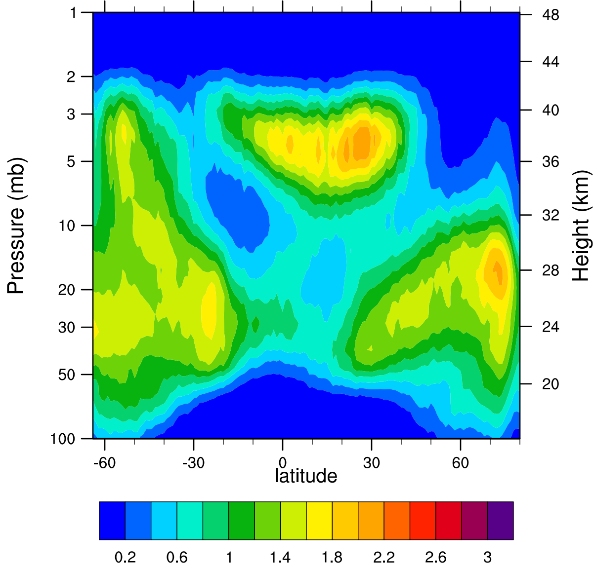
HIRDLSv6 2007d304 ClONO2_Ascending (ppbv)
