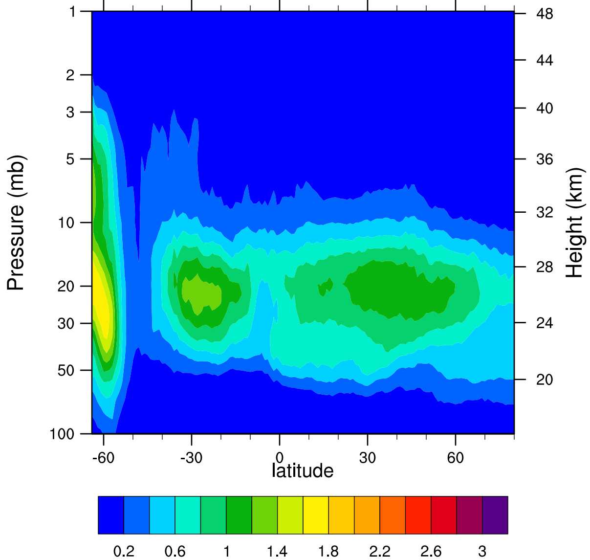
HIRDLSv6 2006d201 ClONO2_Ascending (ppbv)
