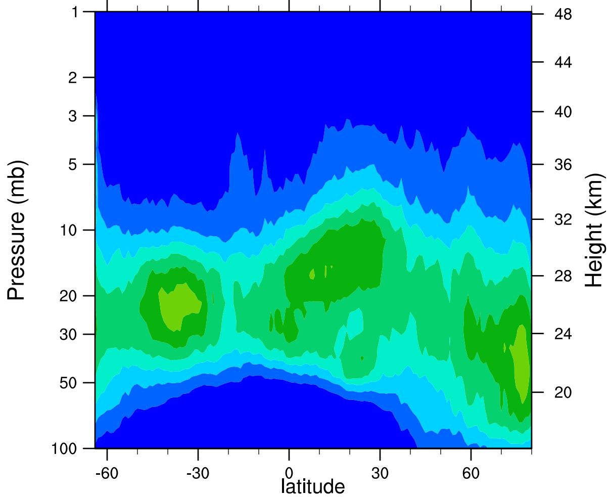
HIRDLSv6 2006d062 ClONO2_Ascending (ppbv)
