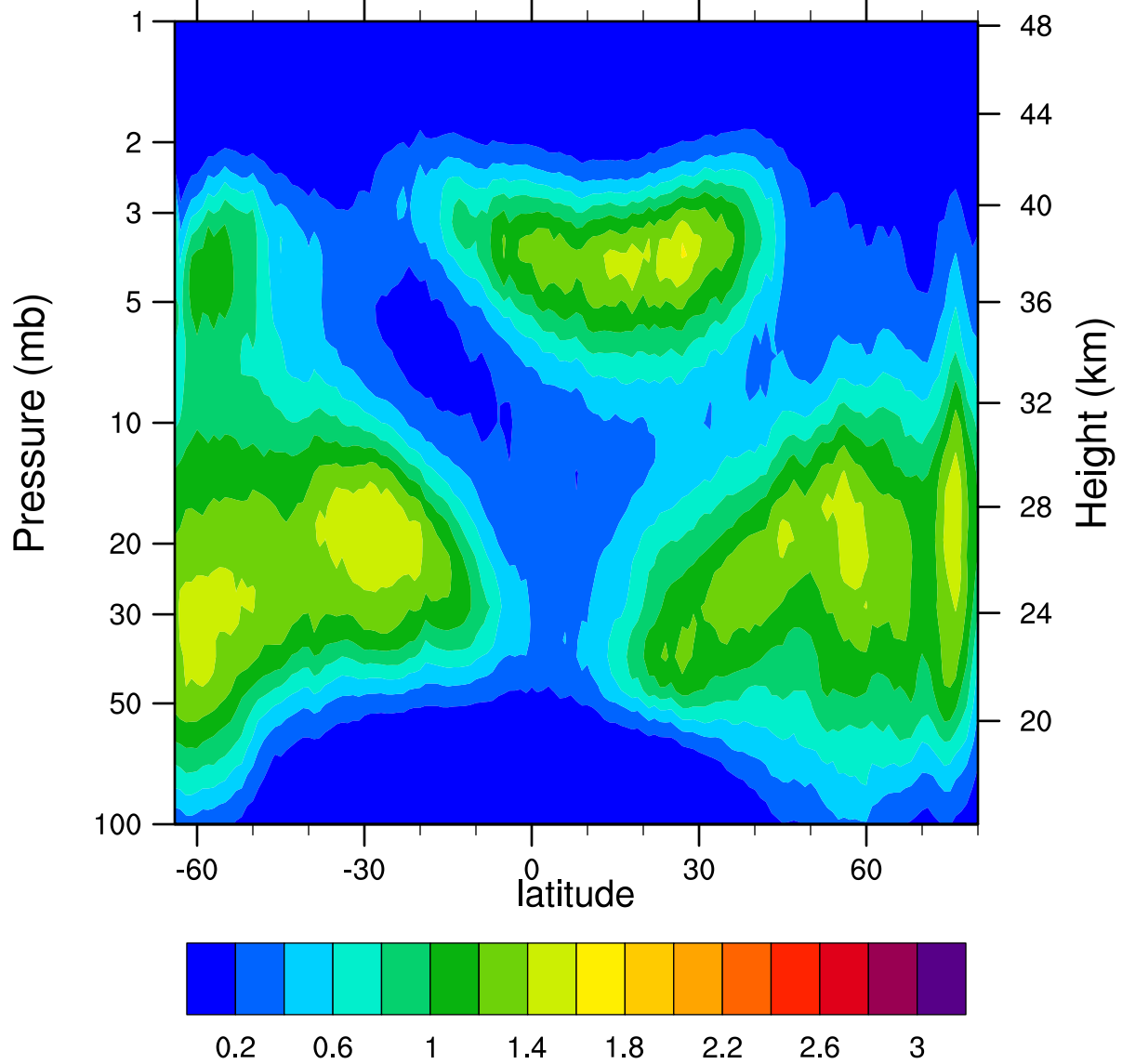
HIRDLSv6 2006d351 ClONO2_Ascending (ppbv)
