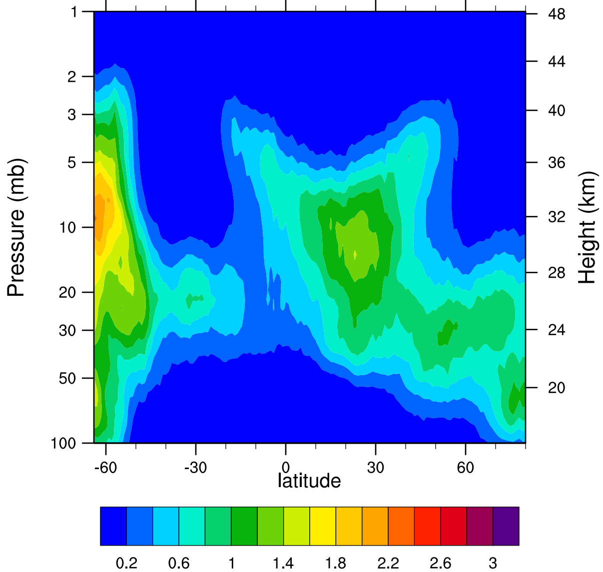
HIRDLSv6 2005d095 ClONO2_Ascending (ppbv)
