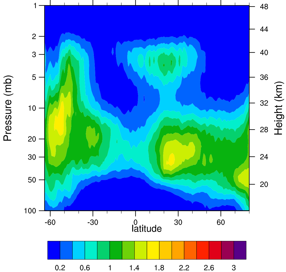
HIRDLSv6 2007d1115 ClONO2_Ascending (ppbv)
