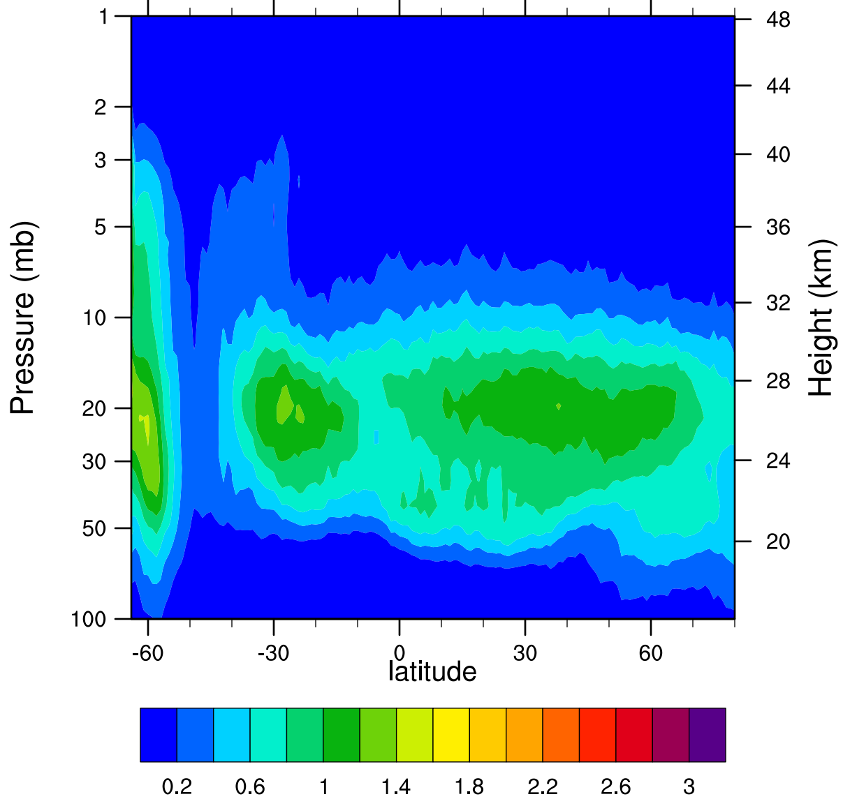
HIRDLSv6 2006d188 ClONO2_Ascending (ppbv)
