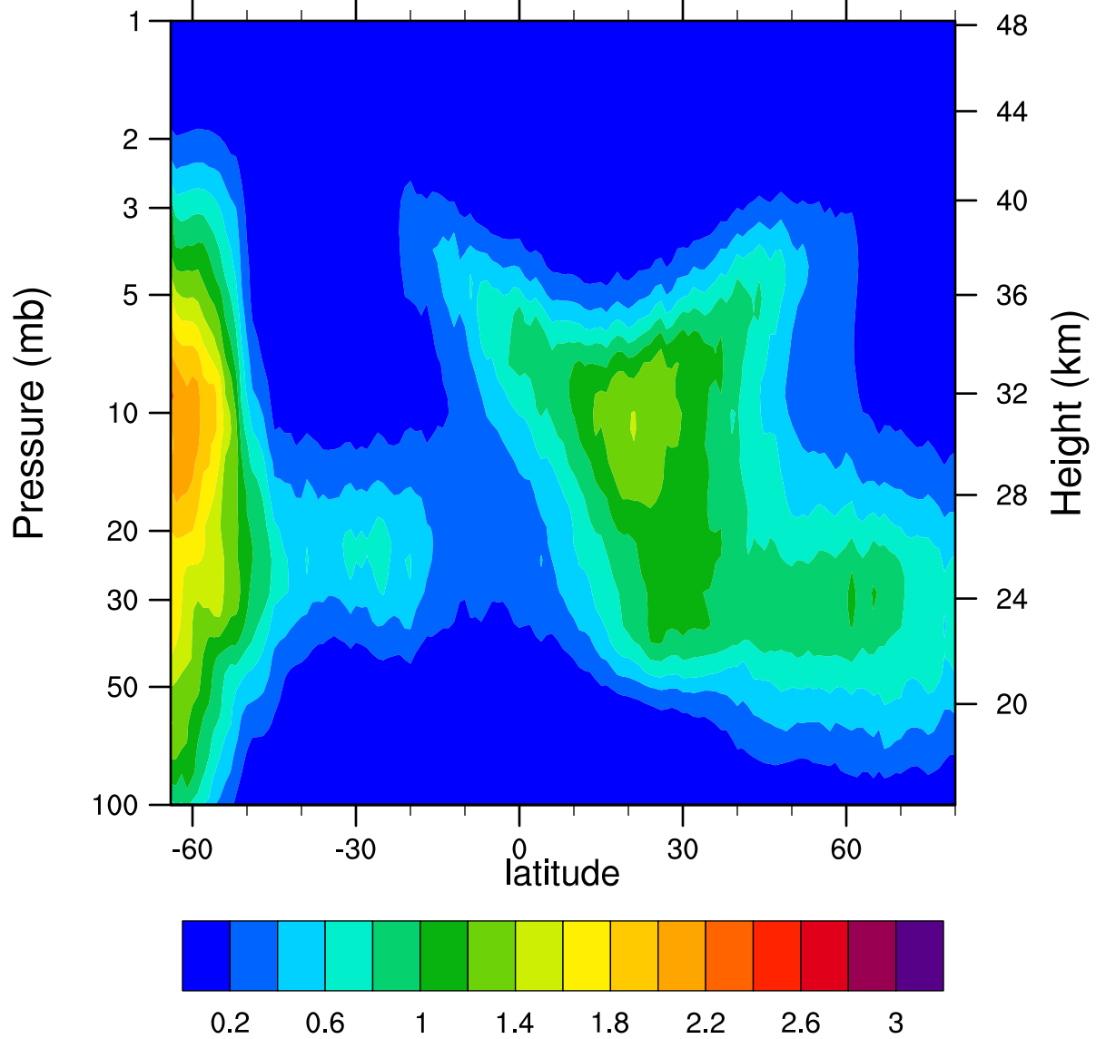
HIRDLSv6 2005d119 ClONO2_Ascending (ppbv)
