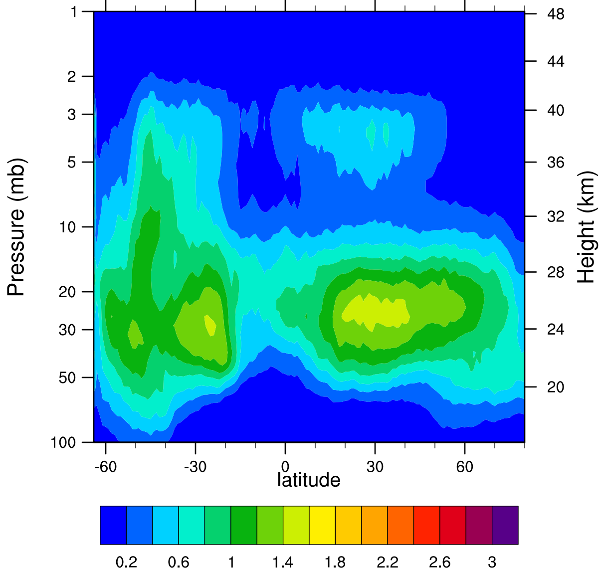
HIRDLSv6 2007d189 ClONO2_Ascending (ppbv)
