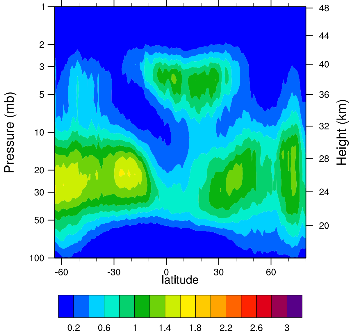
HIRDLSv6 2006d313 ClONO2_Ascending (ppbv)
