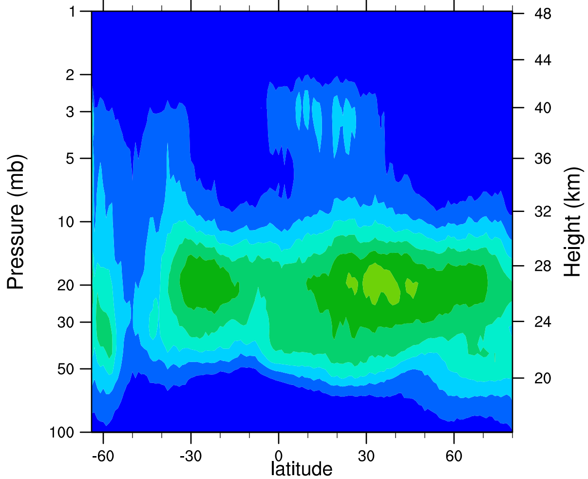
HIRDLSv6 2006d175 ClONO2_Ascending (ppbv)
