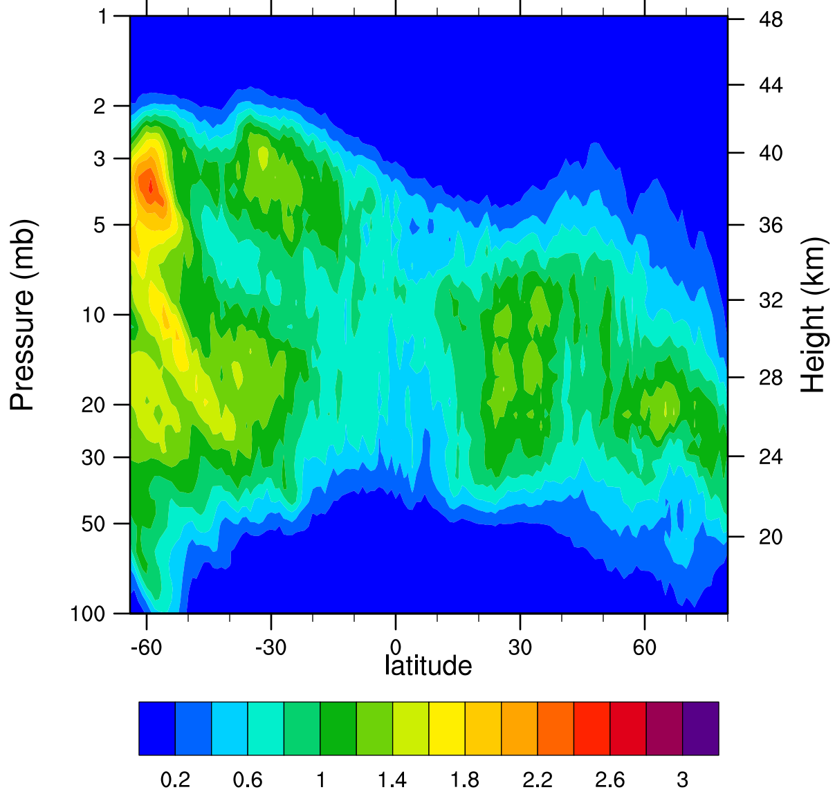
HIRDLSv6 2005d025 ClONO2_Ascending (ppbv)
