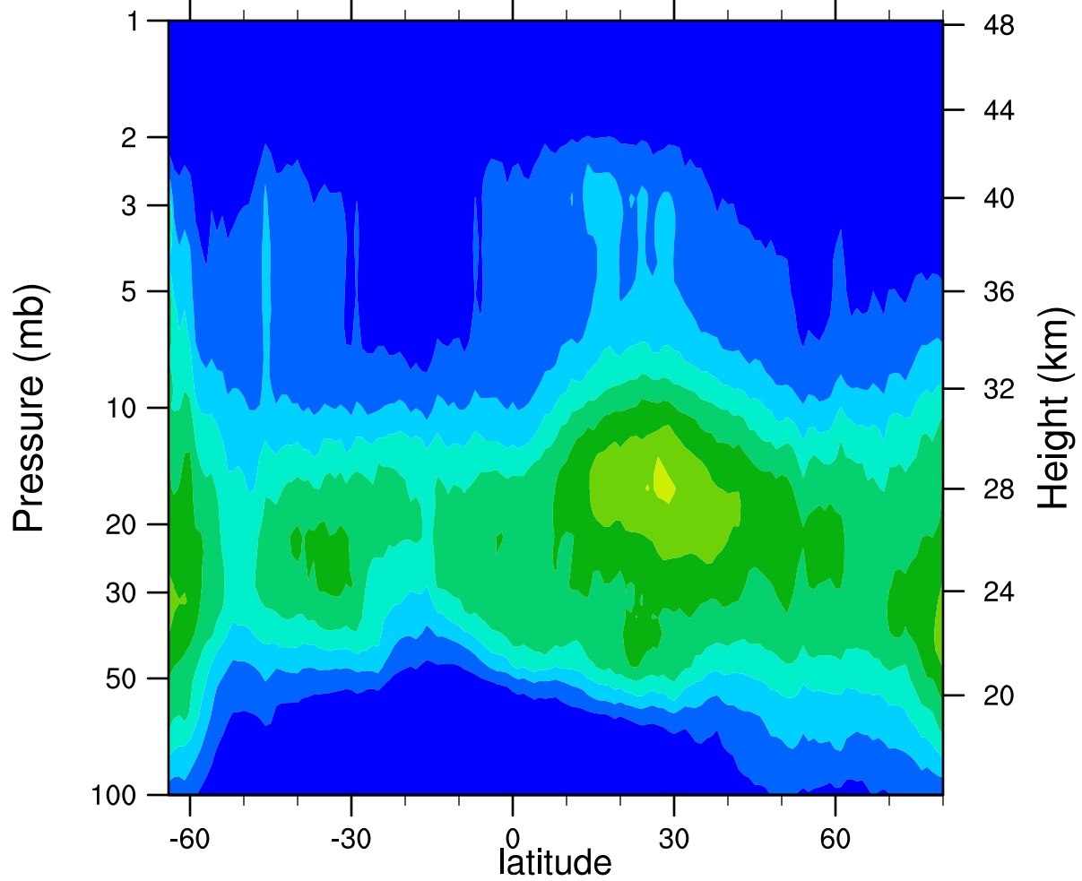
HIRDLSv6 2006d115 ClONO2_Ascending (ppbv)
