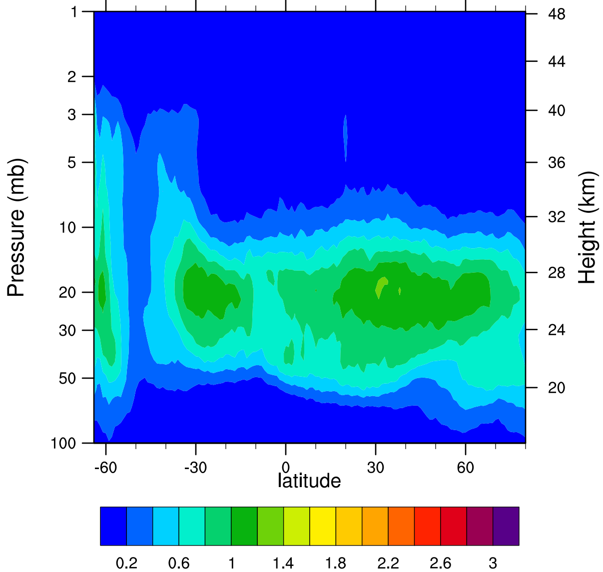
HIRDLSv6 2006d179 ClONO2_Ascending (ppbv)
