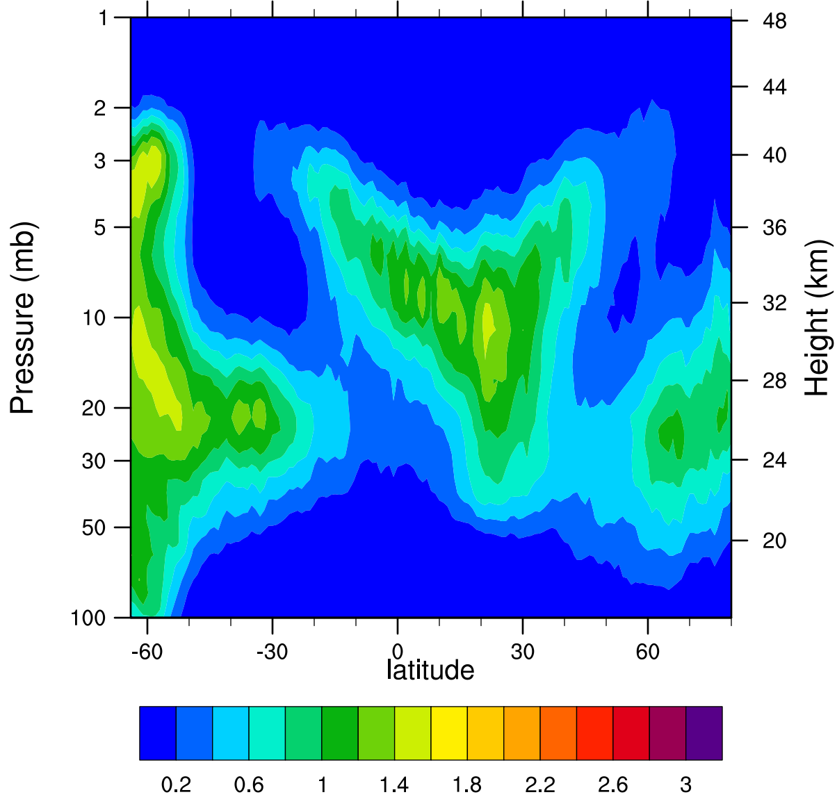
HIRDLSv6 2005d031 ClONO2_Ascending (ppbv)
