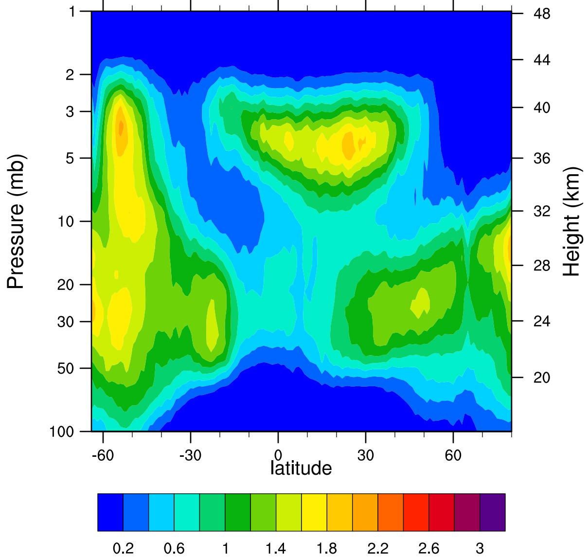
HIRDLSv6 2007d278 ClONO2_Ascending (ppbv)
