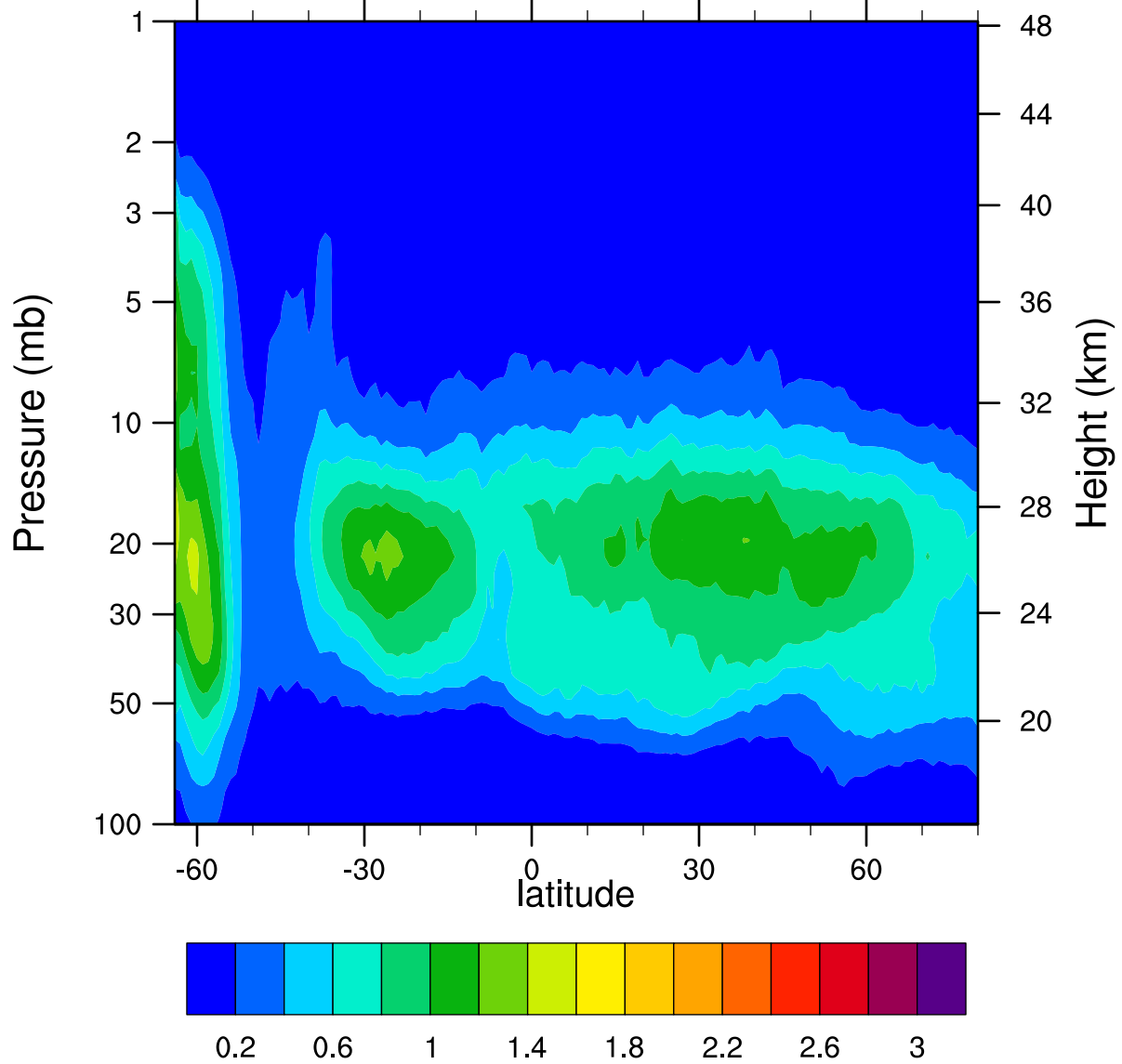
HIRDLSv6 2006d192 ClONO2_Ascending (ppbv)
