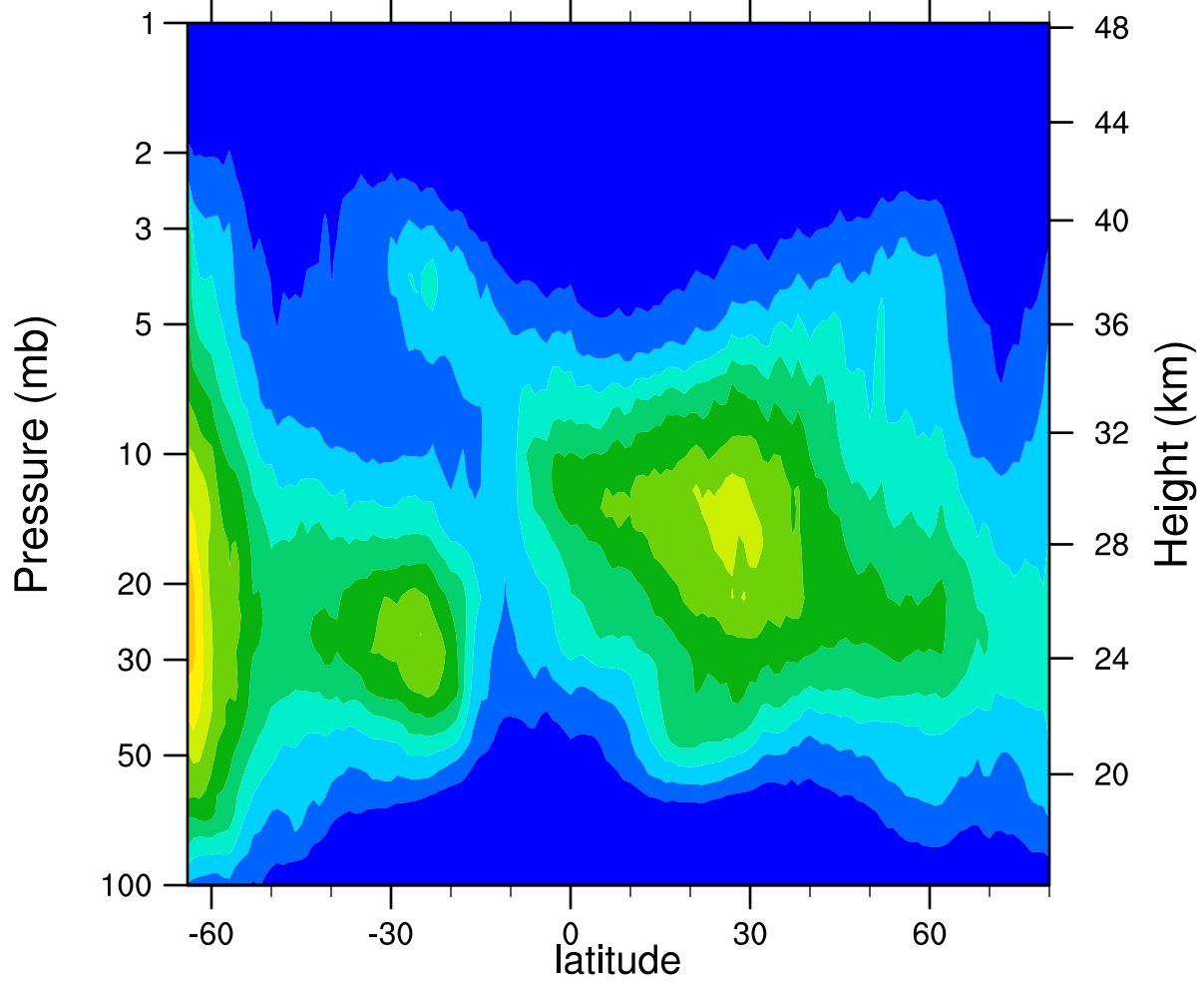
HIRDLSv6 2005d272 ClONO2_Ascending (ppbv)
