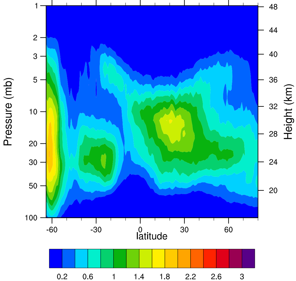
HIRDLSv6 2005d240 ClONO2_Ascending (ppbv)
