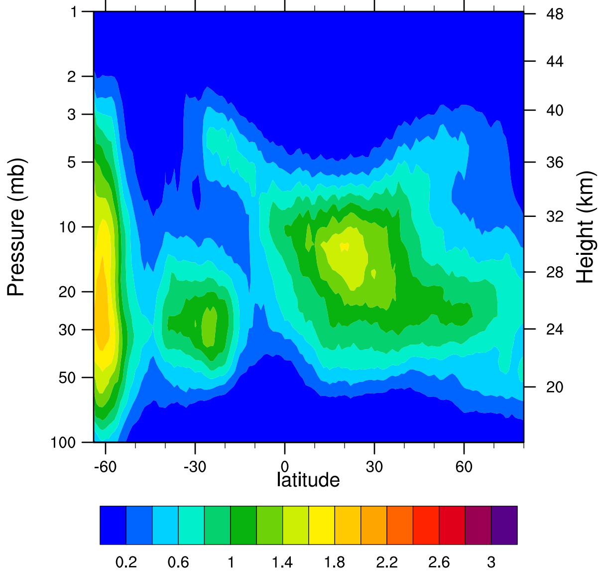
HIRDLSv6 2005d238 ClONO2_Ascending (ppbv)
