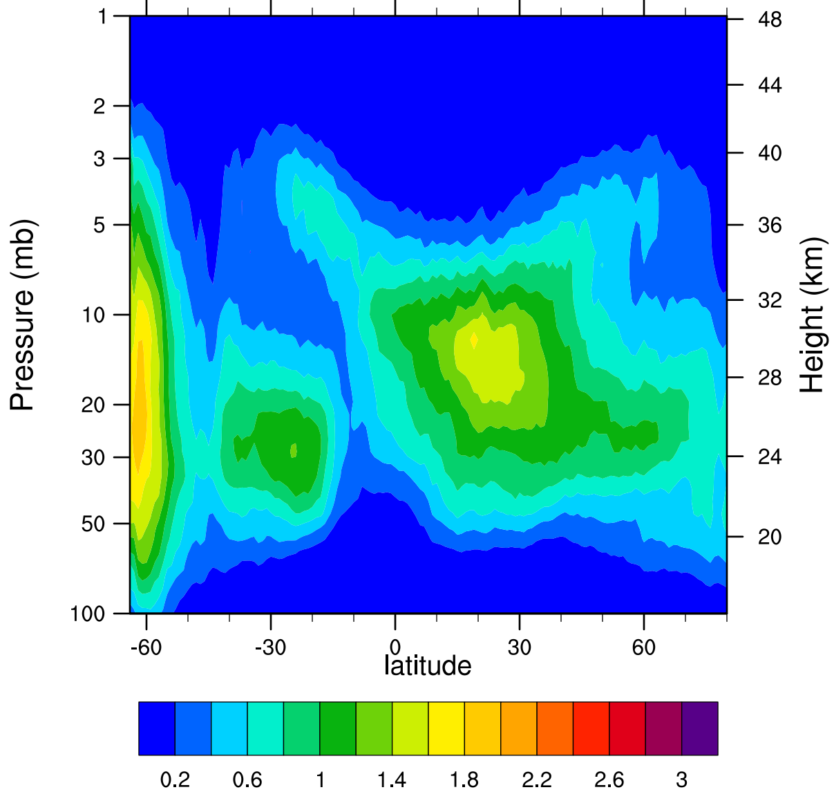
HIRDLSv6 2005d242 ClONO2_Ascending (ppbv)
