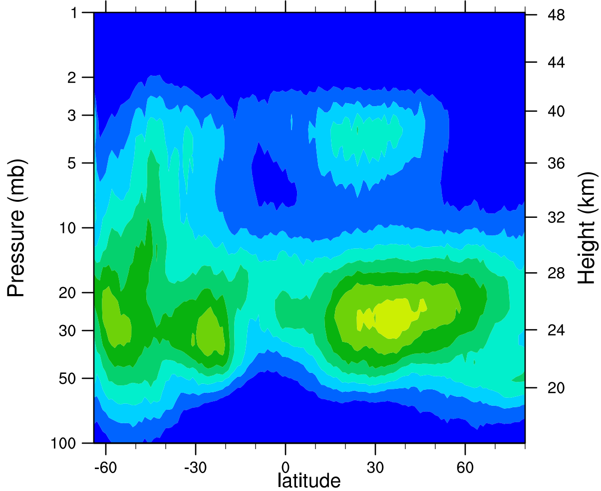
HIRDLSv6 2007d197 ClONO2_Ascending (ppbv)
