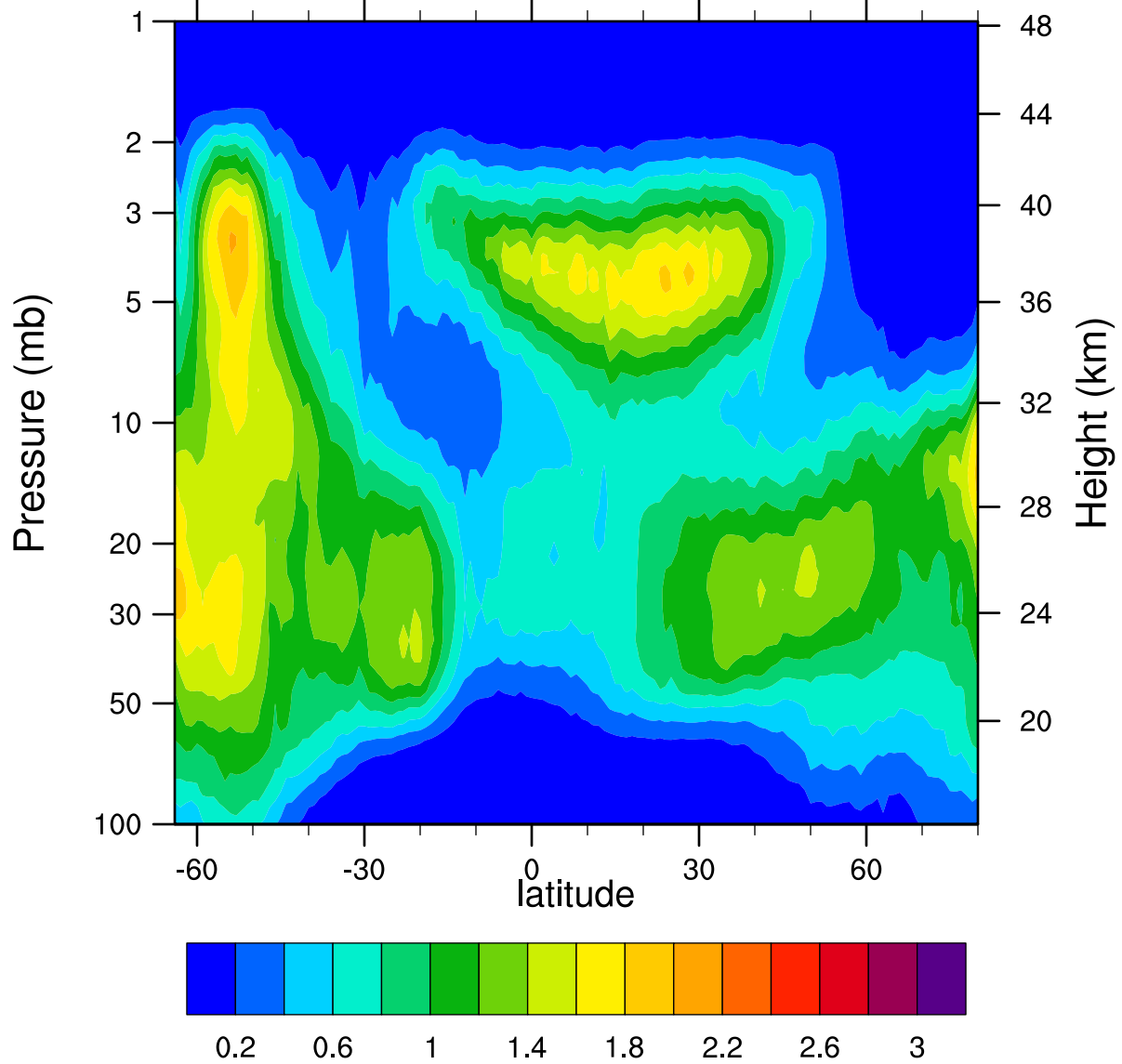
HIRDLSv6 2007d274 ClONO2_Ascending (ppbv)
