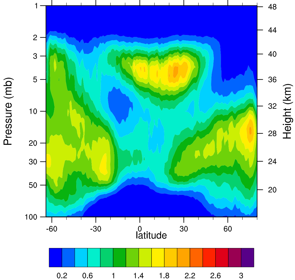
HIRDLSv6 2007d294 ClONO2_Ascending (ppbv)
