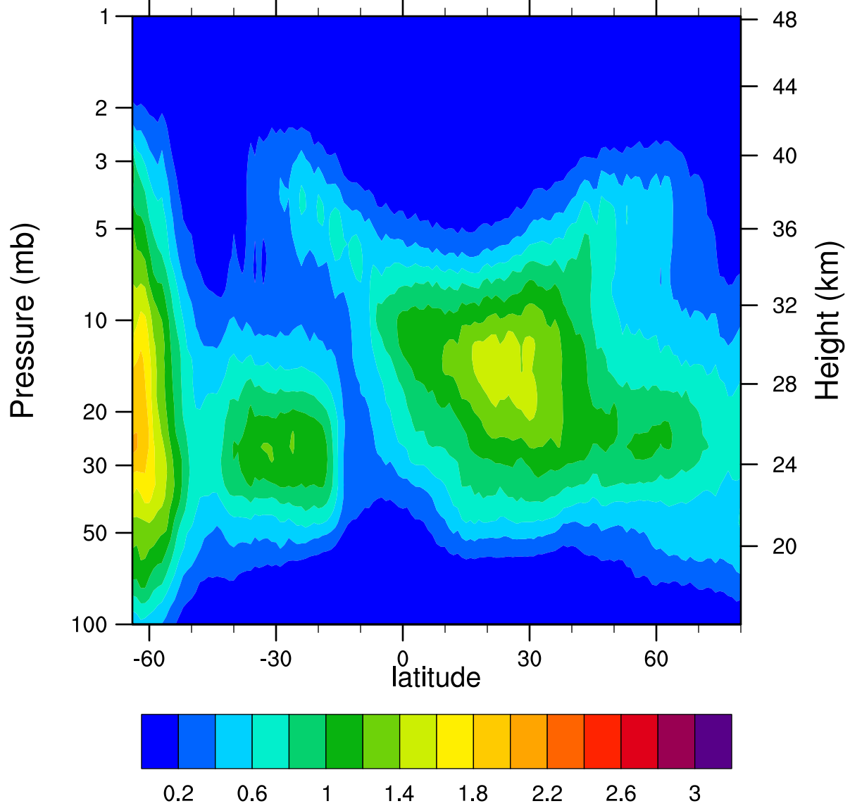
HIRDLSv6 2005d251 ClONO2_Ascending (ppbv)
