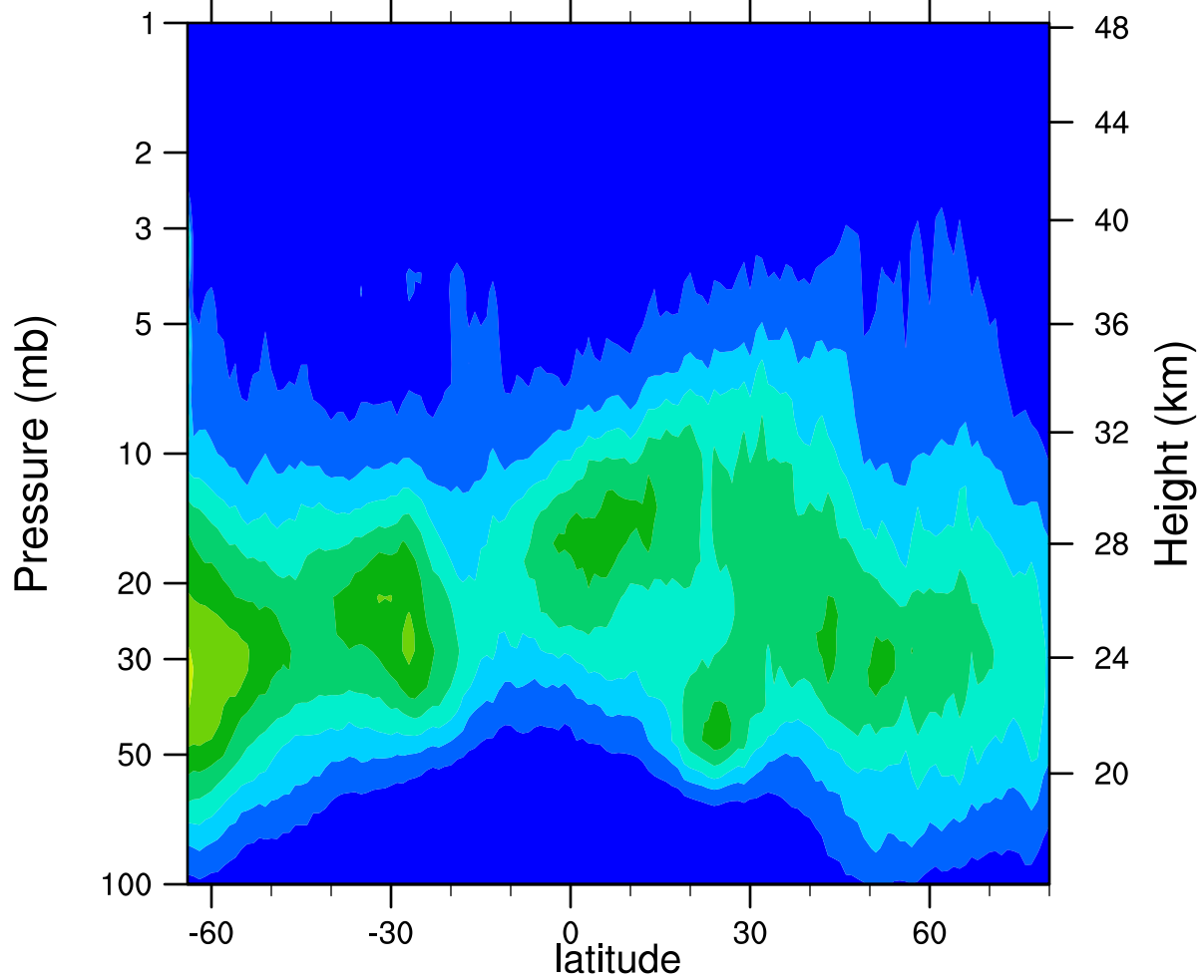
HIRDLSv6 2005d331 ClONO2_Ascending (ppbv)
