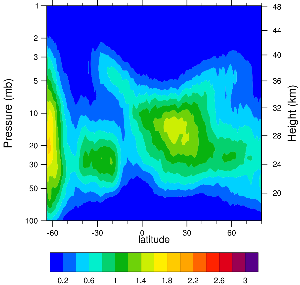
HIRDLSv6 2005d247 ClONO2_Ascending (ppbv)
