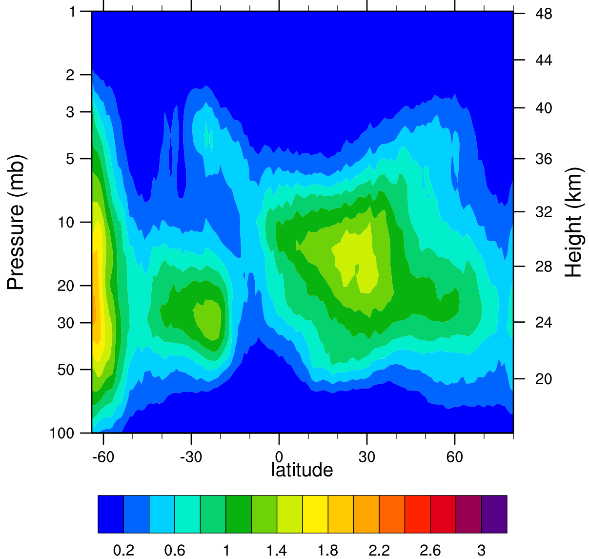
HIRDLSv6 2005d264 ClONO2_Ascending (ppbv)
