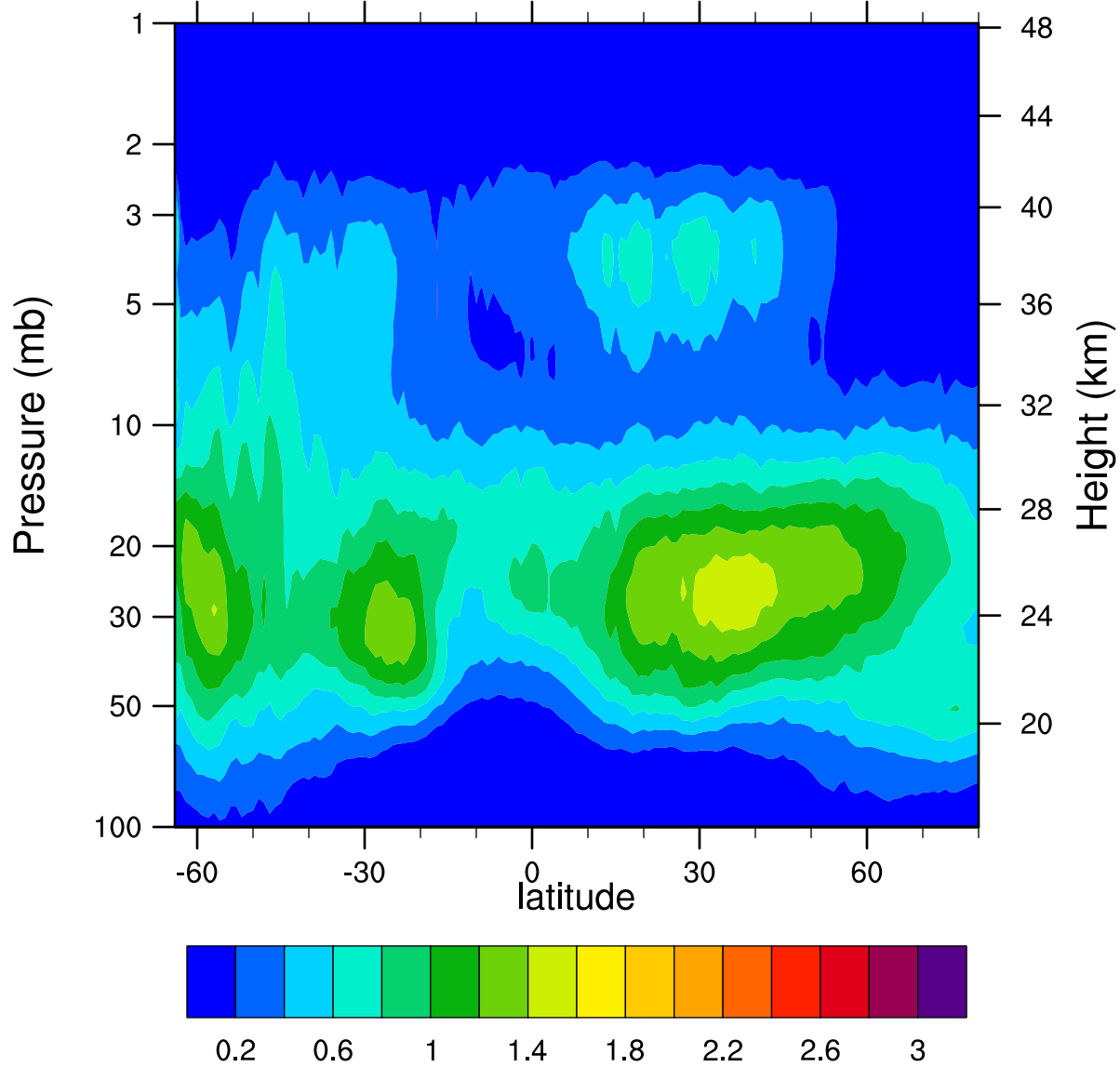
HIRDLSv6 2007d202 ClONO2_Ascending (ppbv)
