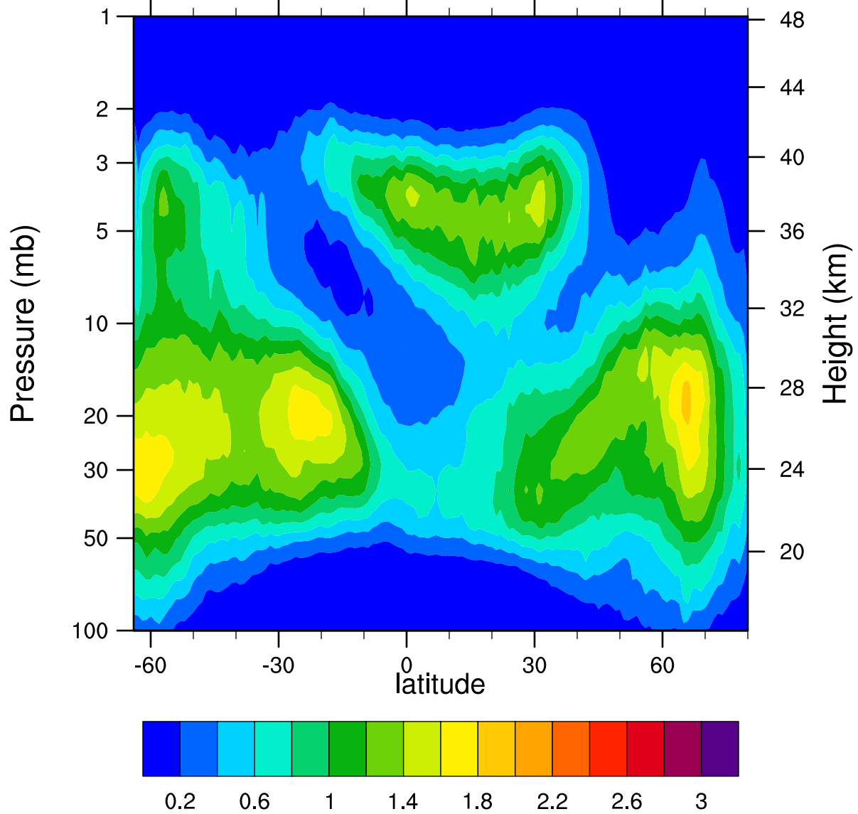
HIRDLSv6 2006d321 ClONO2_Ascending (ppbv)
