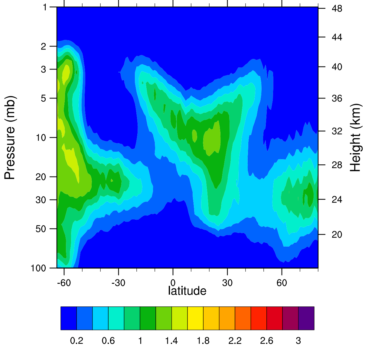
HIRDLSv6 2005d045 ClONO2_Ascending (ppbv)
