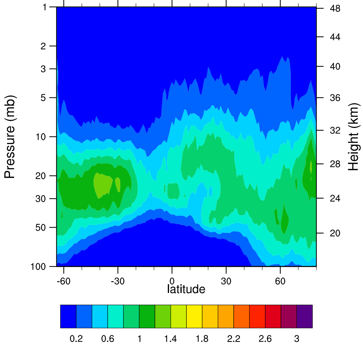
HIRDLSv6 2006d015 ClONO2_Ascending (ppbv)
