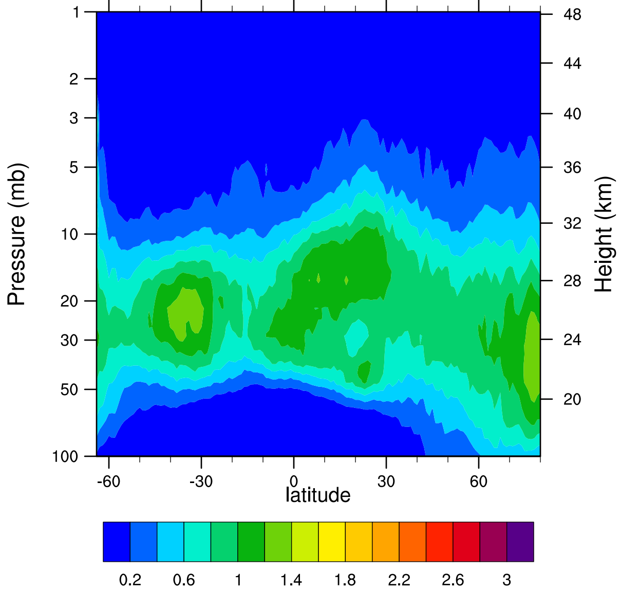
HIRDLSv6 2006d069 ClONO2_Ascending (ppbv)
