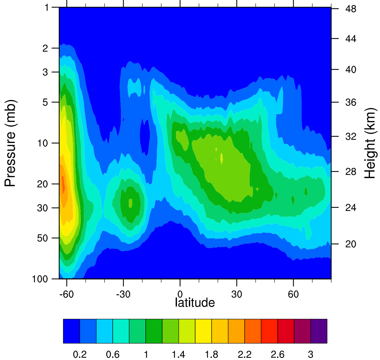
HIRDLSv6 2005d206 ClONO2_Ascending (ppbv)
