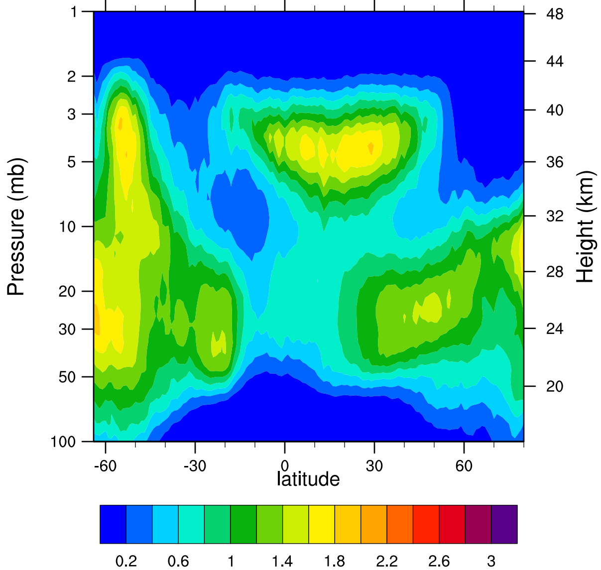
HIRDLSv6 2007d271 ClONO2_Ascending (ppbv)
