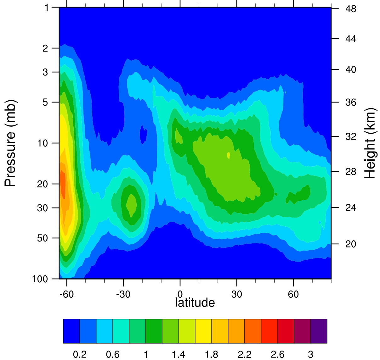
HIRDLSv6 2005d203 ClONO2_Ascending (ppbv)
