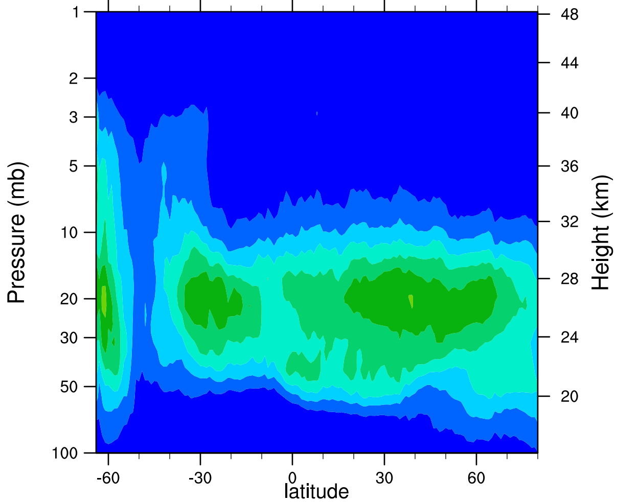
HIRDLSv6 2006d184 ClONO2_Ascending (ppbv)
