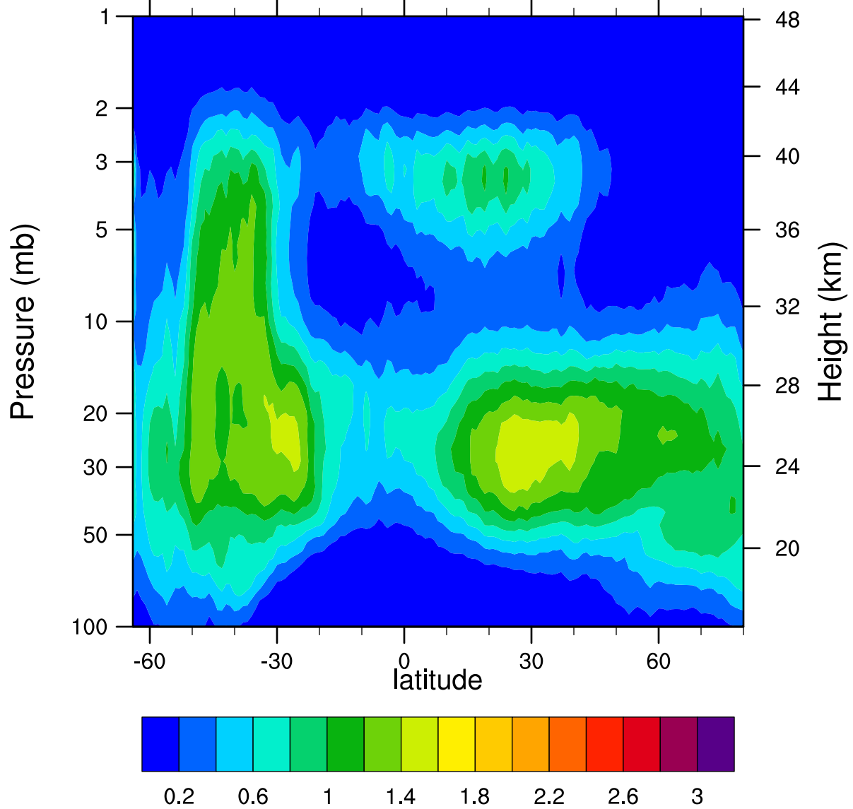
HIRDLSv6 2007d159 ClONO2_Ascending (ppbv)
