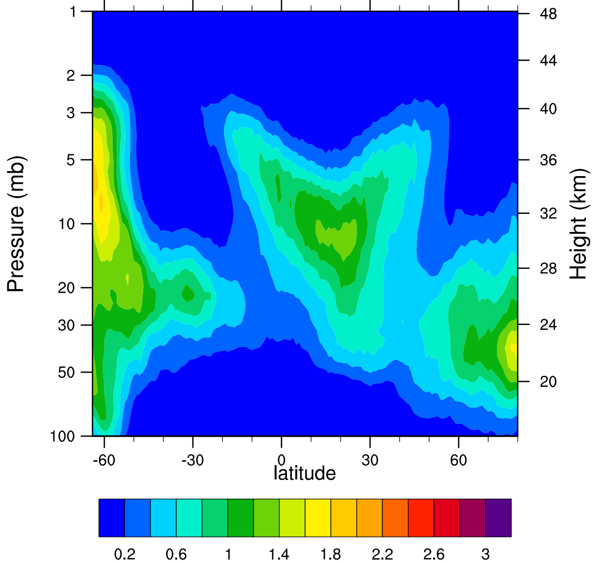
HIRDLSv6 2005d065 ClONO2_Ascending (ppbv)
