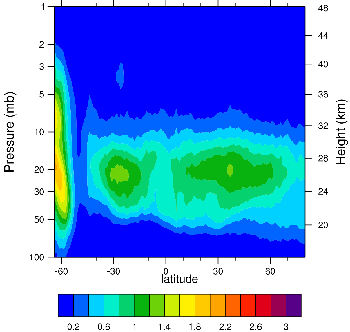
HIRDLSv6 2006d219 ClONO2_Ascending (ppbv)
