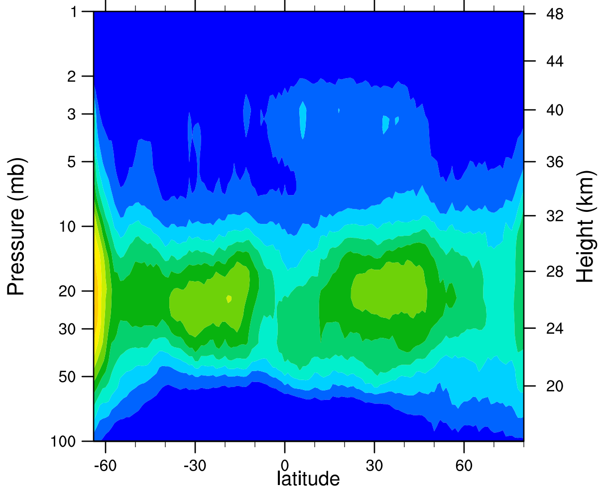
HIRDLSv6 2006d275 ClONO2_Ascending (ppbv)
