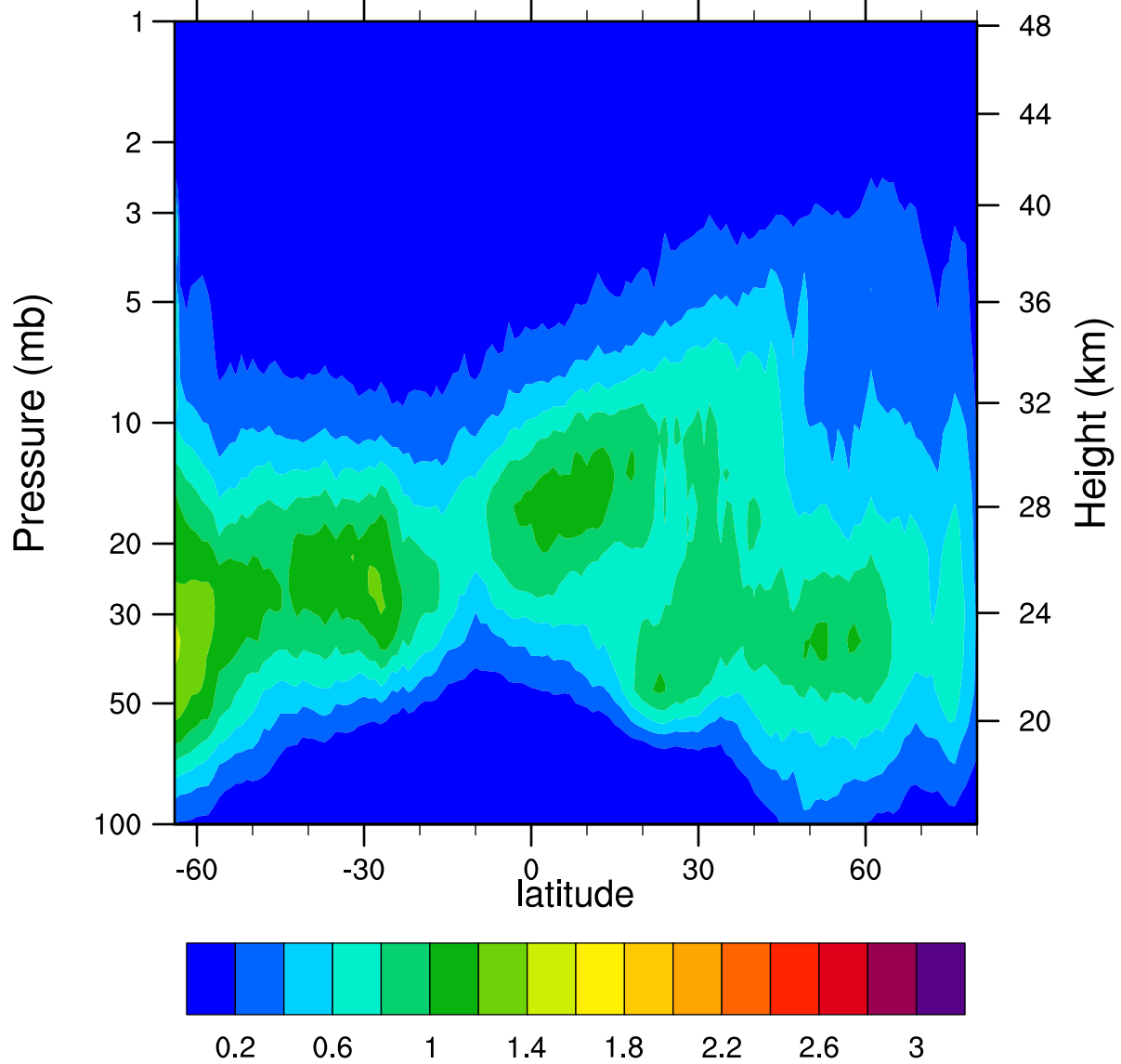
HIRDLSv6 2005d341 ClONO2_Ascending (ppbv)
