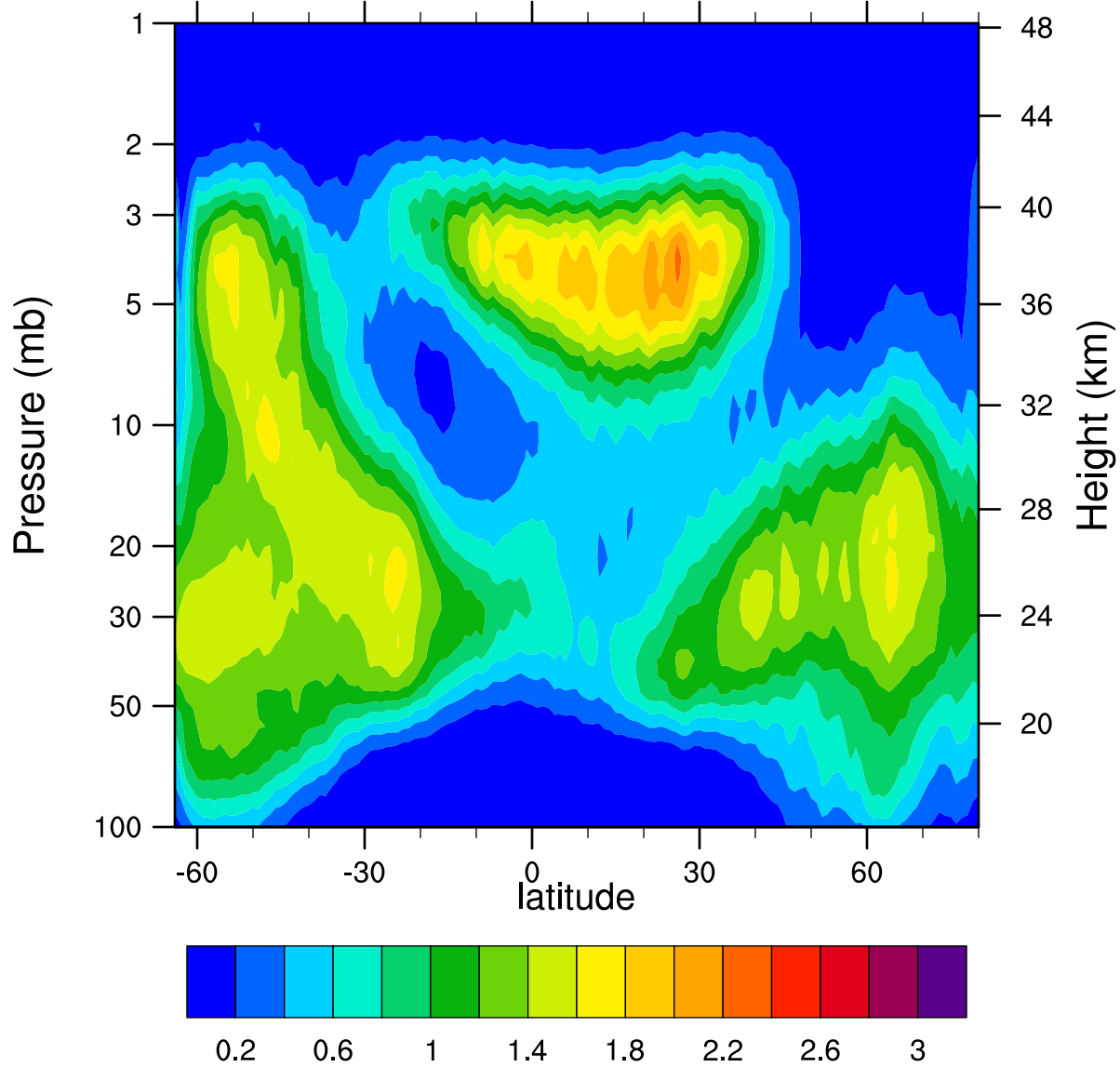
HIRDLSv6 2007d323 ClONO2_Ascending (ppbv)
