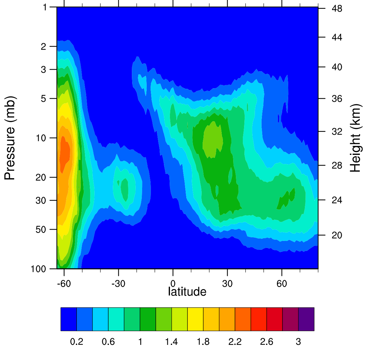
HIRDLSv6 2005d140 ClONO2_Ascending (ppbv)
