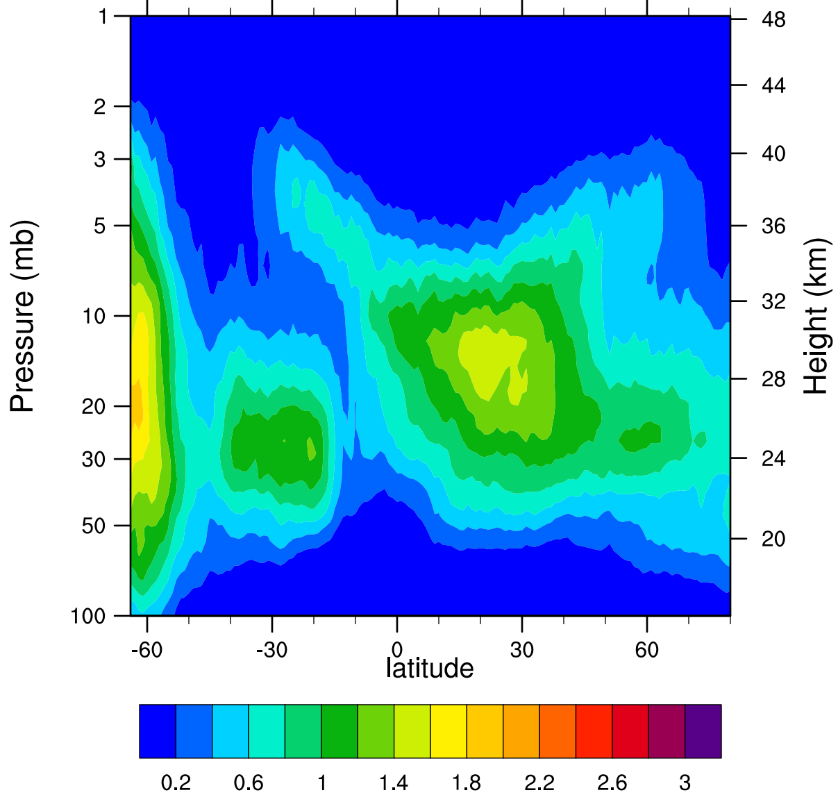
HIRDLSv6 2005d248 ClONO2_Ascending (ppbv)
