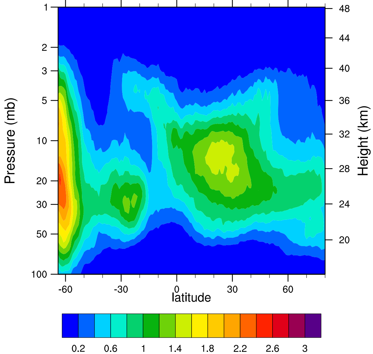
HIRDLSv6 2005d226 ClONO2_Ascending (ppbv)
