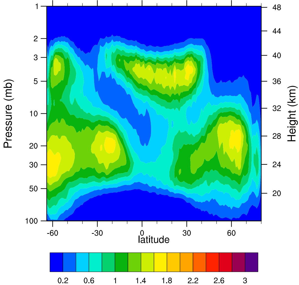
HIRDLSv6 2006d330 ClONO2_Ascending (ppbv)
