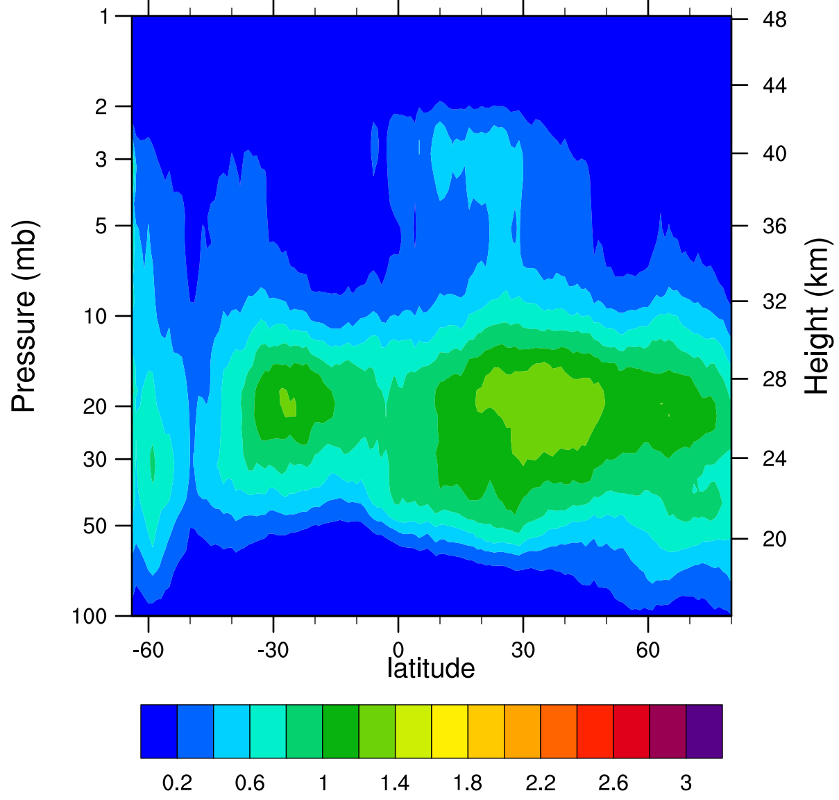
HIRDLSv6 2006d163 ClONO2_Ascending (ppbv)
