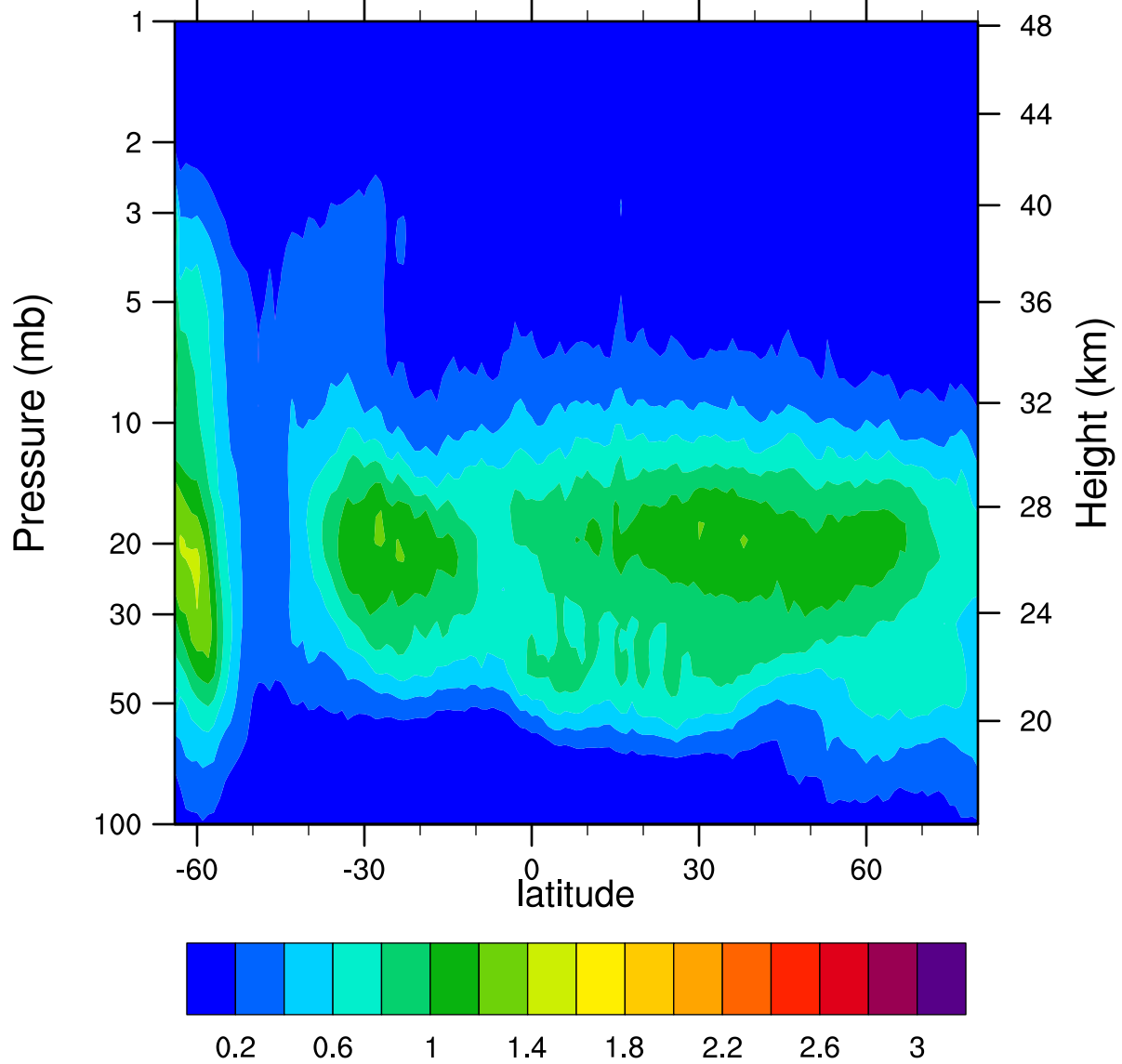
HIRDLSv6 2006d187 ClONO2_Ascending (ppbv)
