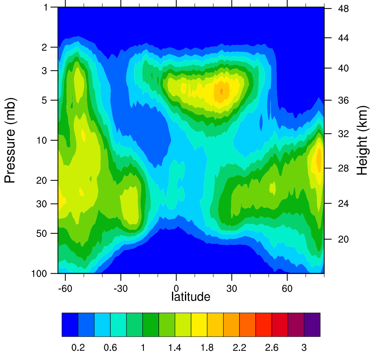
HIRDLSv6 2007d286 ClONO2_Ascending (ppbv)
