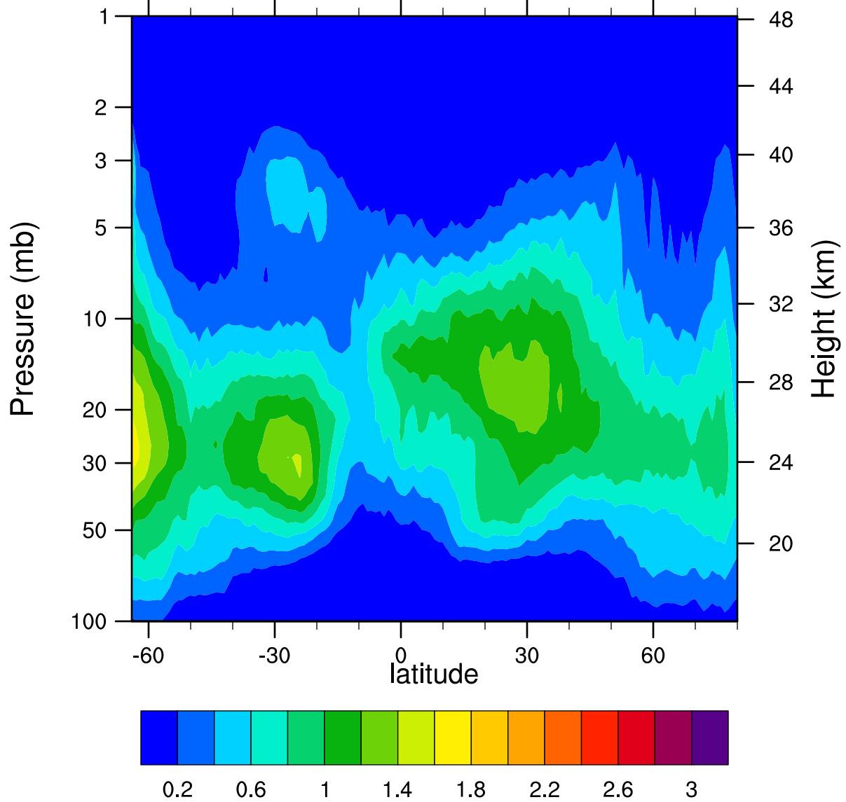
HIRDLSv6 2005d292 ClONO2_Ascending (ppbv)
