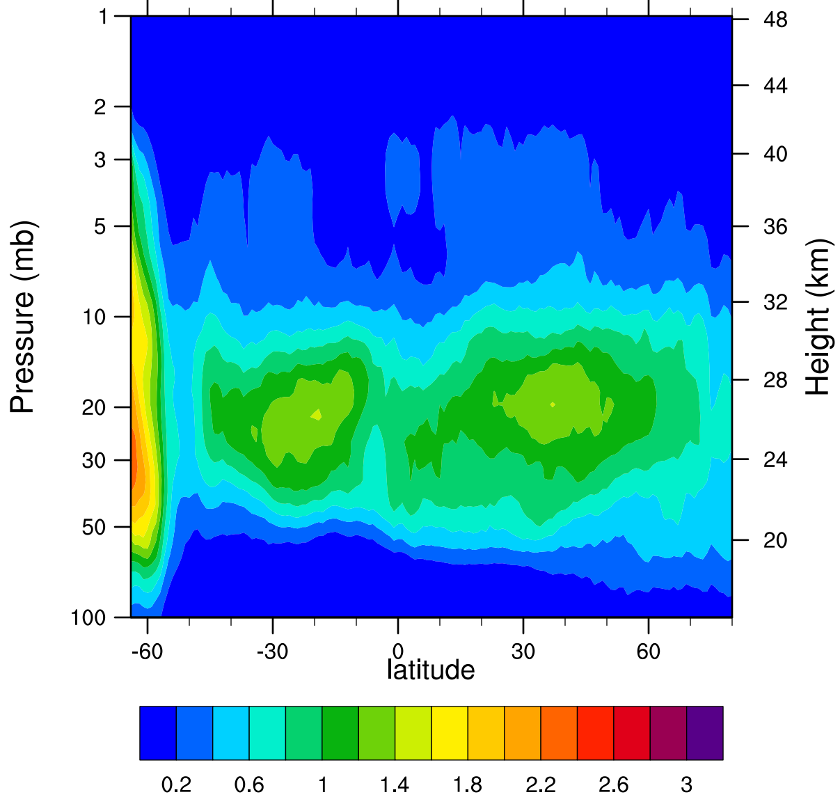
HIRDLSv6 2006d252 ClONO2_Ascending (ppbv)
