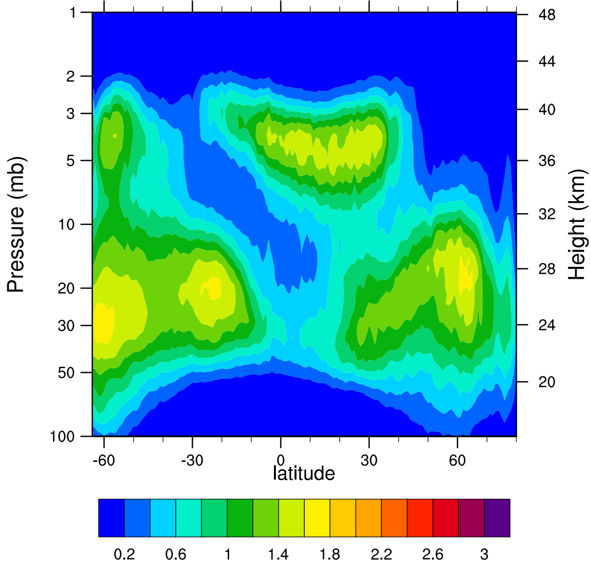
HIRDLSv6 2006d334 ClONO2_Ascending (ppbv)
