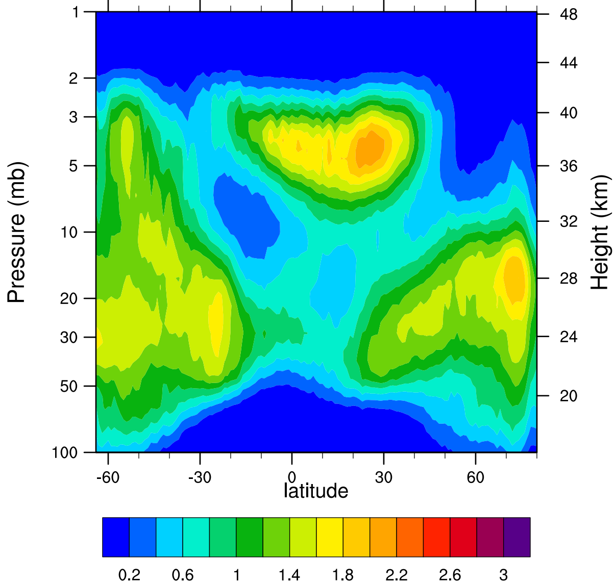
HIRDLSv6 2007d302 ClONO2_Ascending (ppbv)
