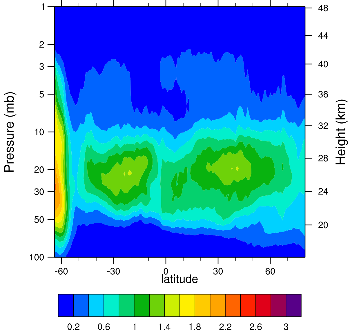
HIRDLSv6 2006d255 ClONO2_Ascending (ppbv)
