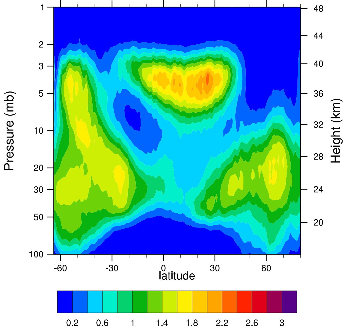
HIRDLSv6 2007d321 ClONO2_Ascending (ppbv)
