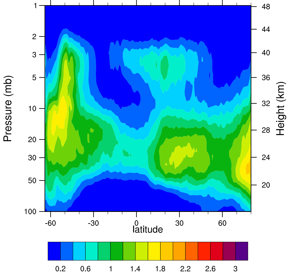
HIRDLSv6 2007d100 ClONO2_Ascending (ppbv)
