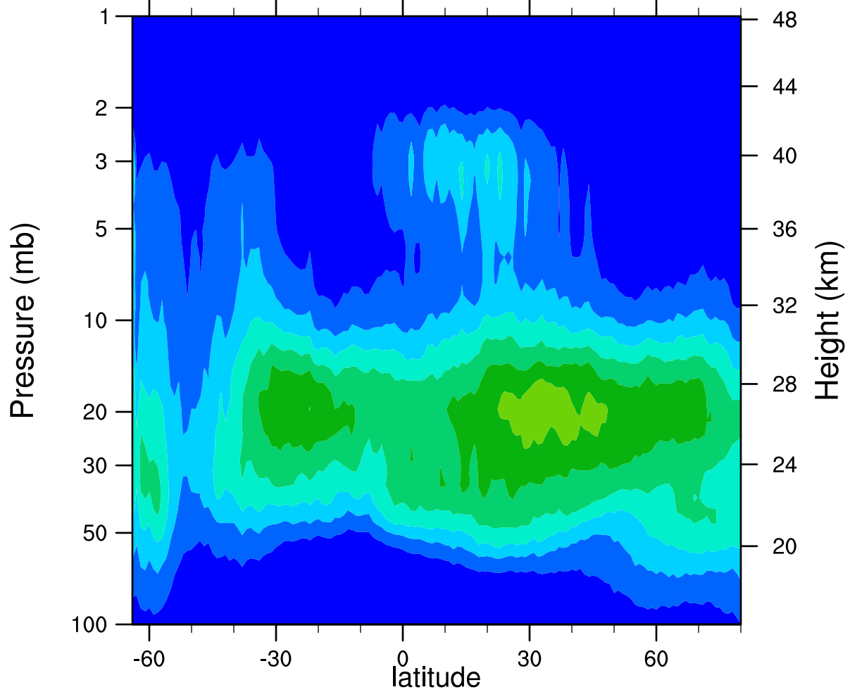
HIRDLSv6 2006d174 ClONO2_Ascending (ppbv)
