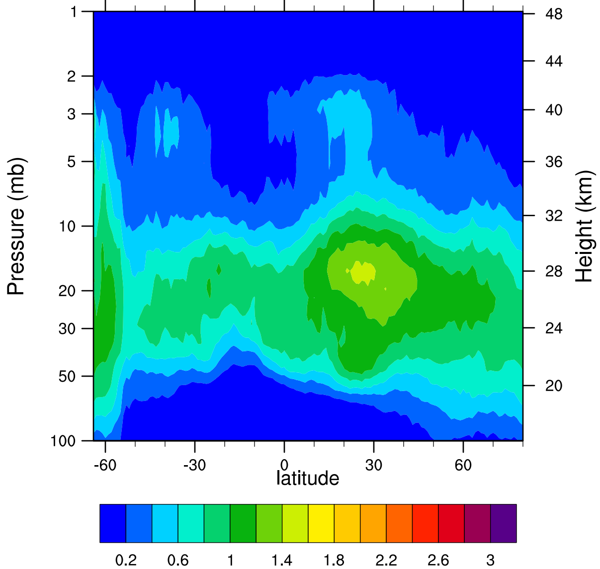
HIRDLSv6 2006d130 ClONO2_Ascending (ppbv)
