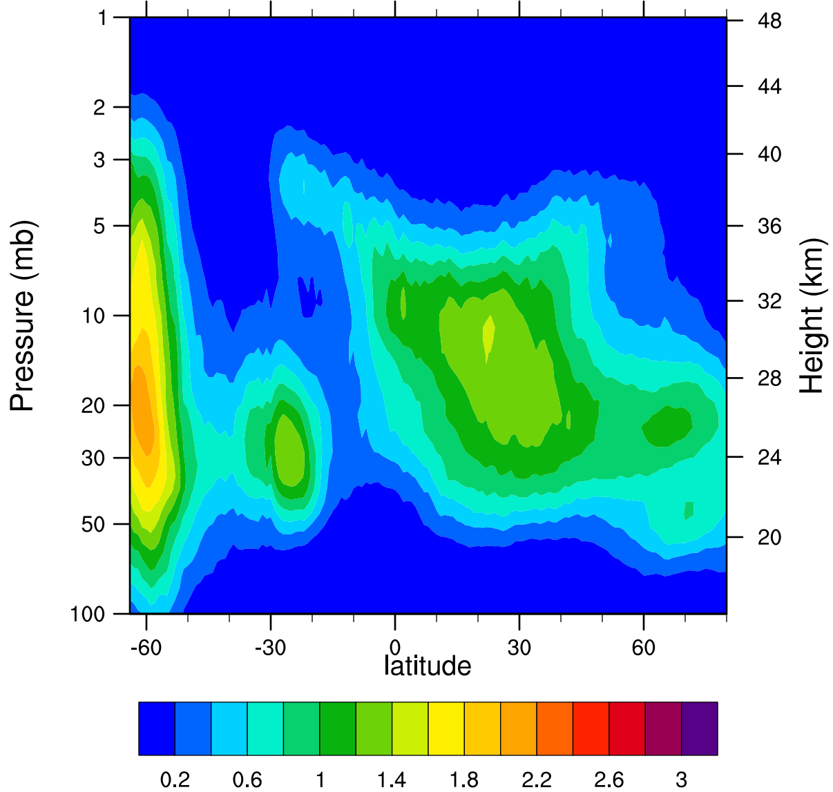
HIRDLSv6 2005d193 ClONO2_Ascending (ppbv)
