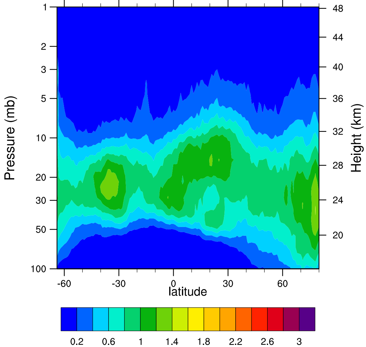
HIRDLSv6 2006d074 ClONO2_Ascending (ppbv)
