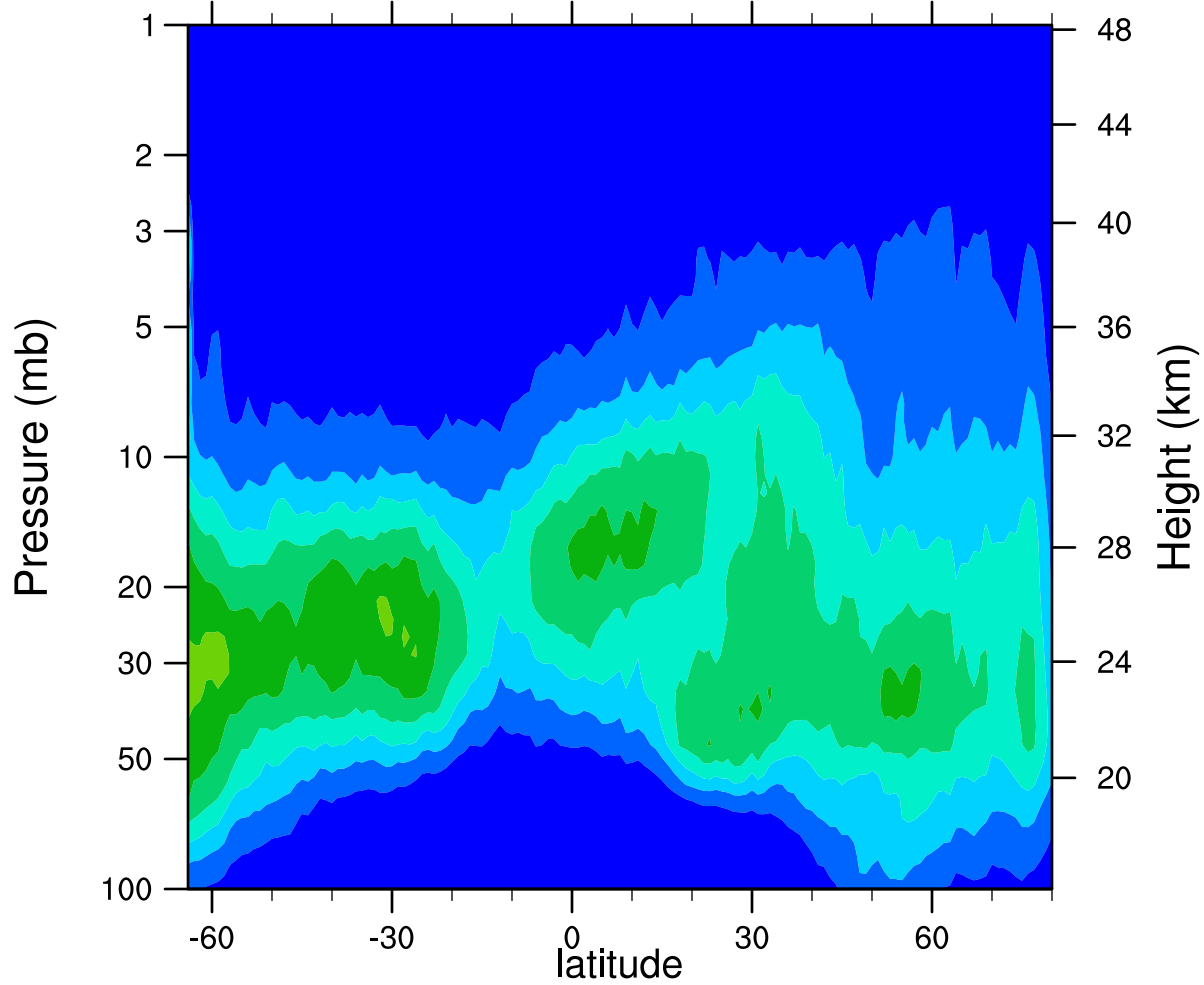
HIRDLSv6 2005d346 ClONO2_Ascending (ppbv)
