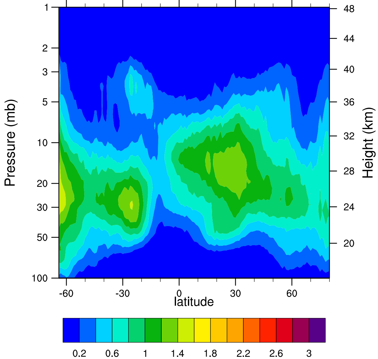
HIRDLSv6 2005d286 ClONO2_Ascending (ppbv)
