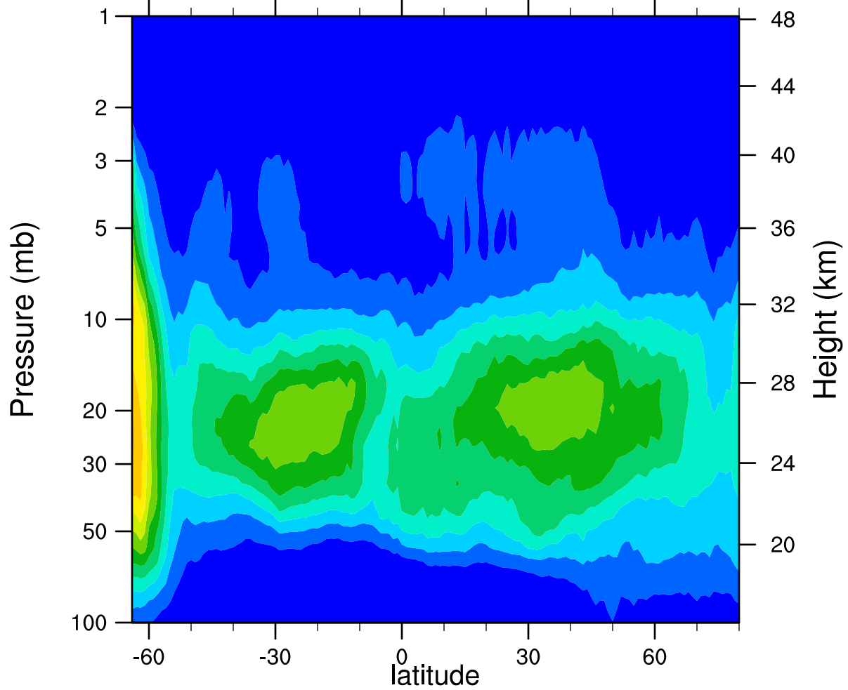
HIRDLSv6 2006d263 ClONO2_Ascending (ppbv)
