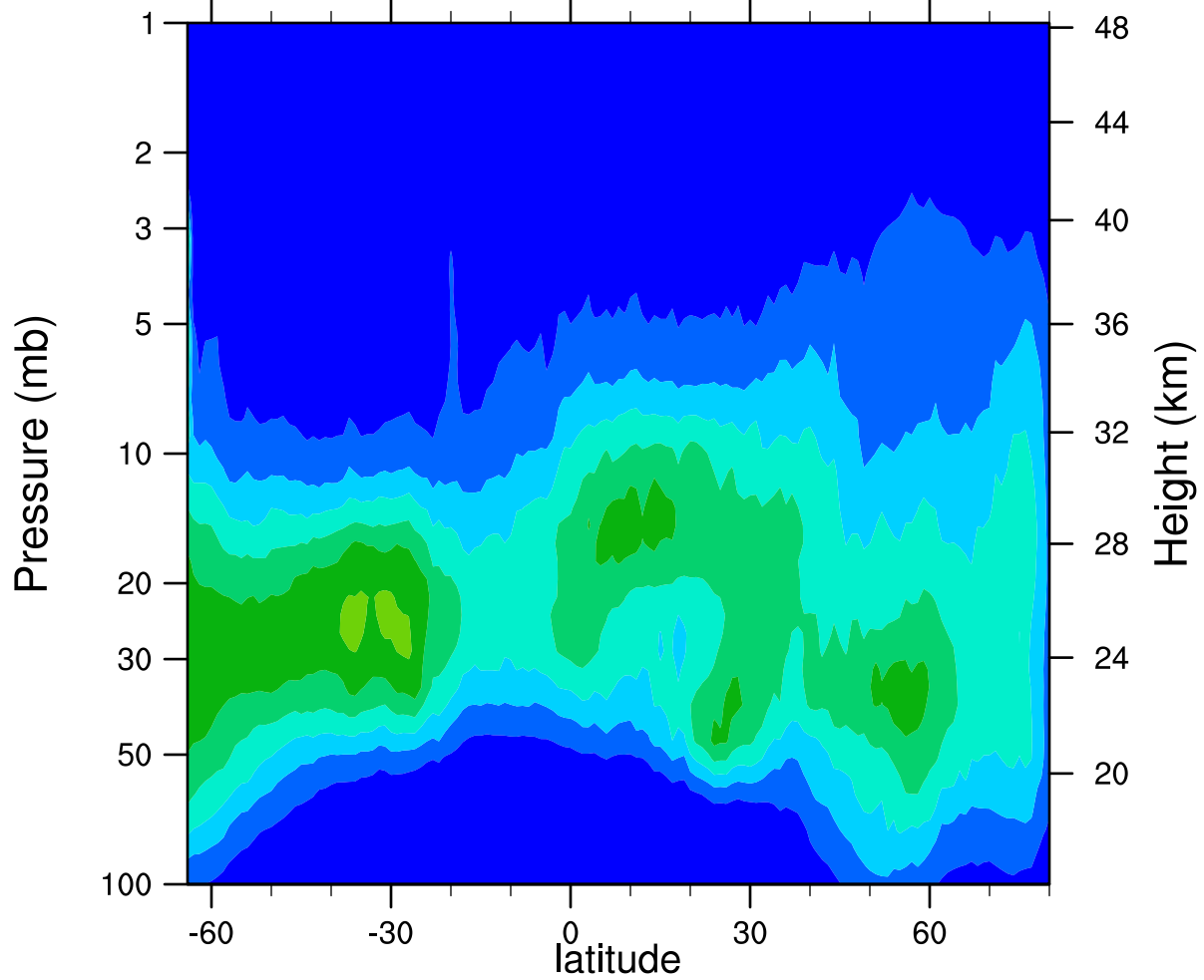
HIRDLSv6 2005d360 ClONO2_Ascending (ppbv)
