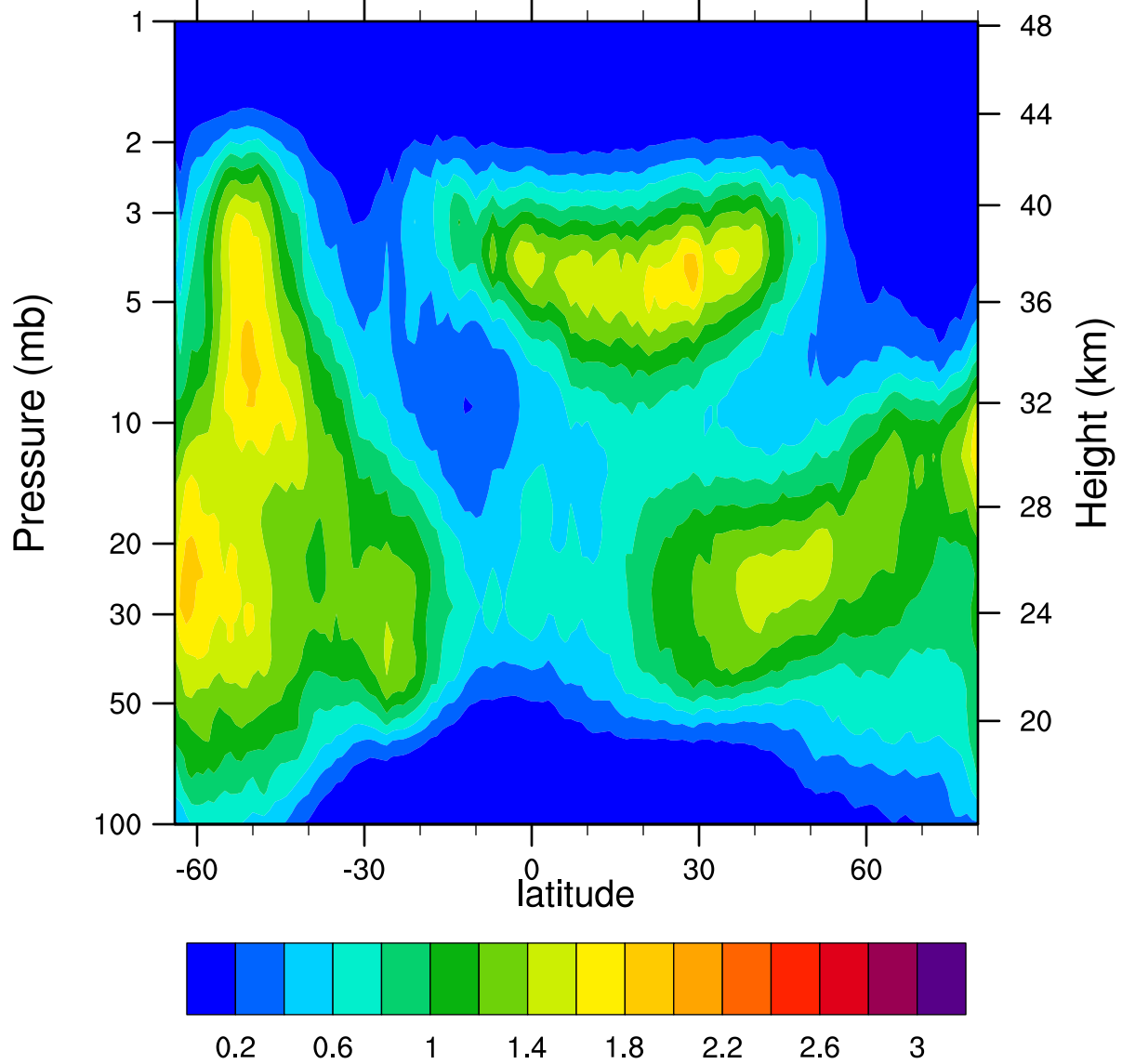
HIRDLSv6 2007d261 ClONO2_Ascending (ppbv)
