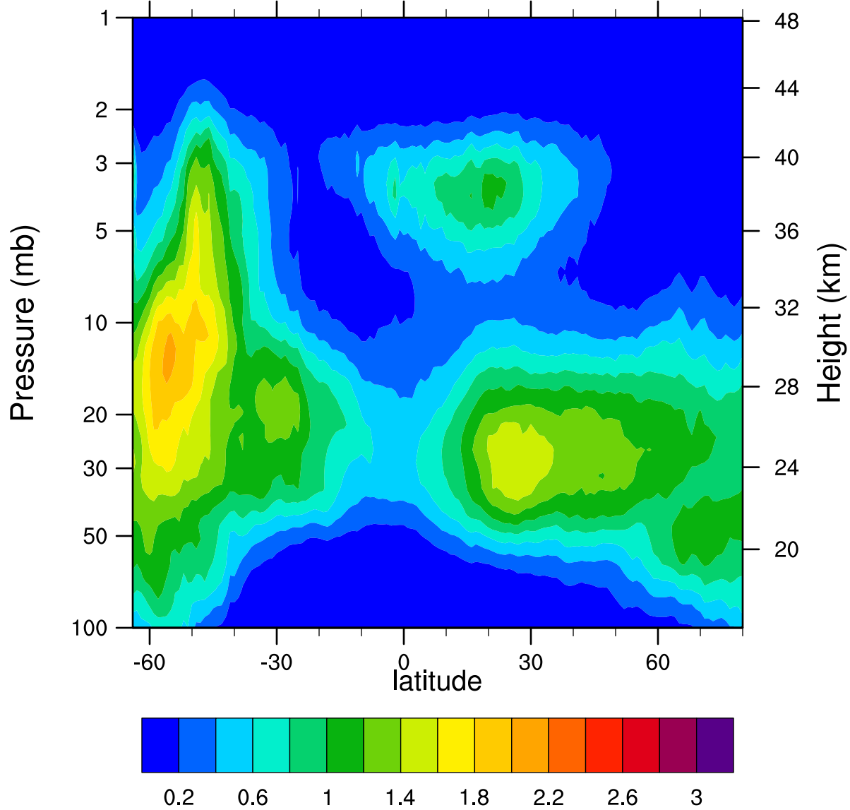
HIRDLSv6 2007d131 ClONO2_Ascending (ppbv)
