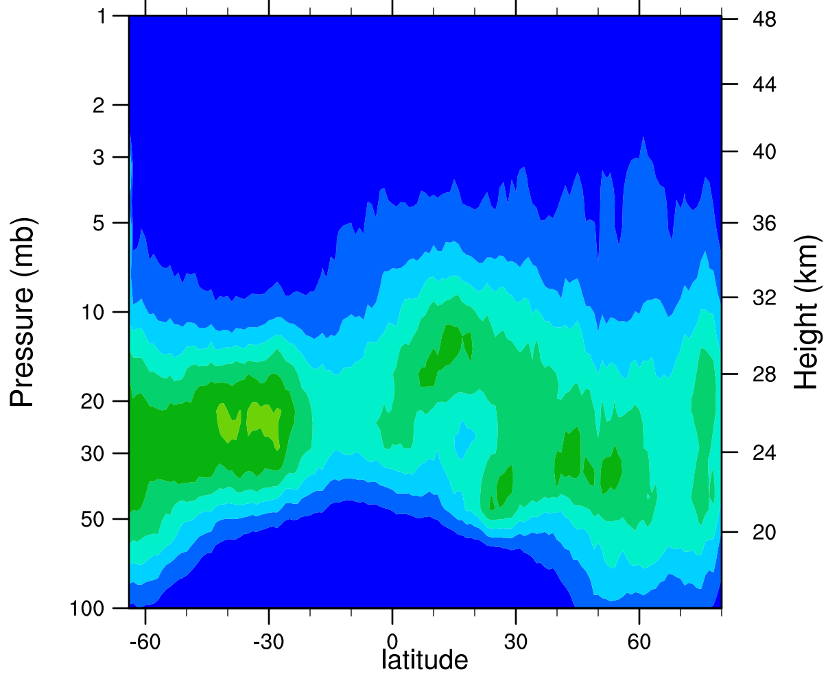
HIRDLSv6 2006d004 ClONO2_Ascending (ppbv)
