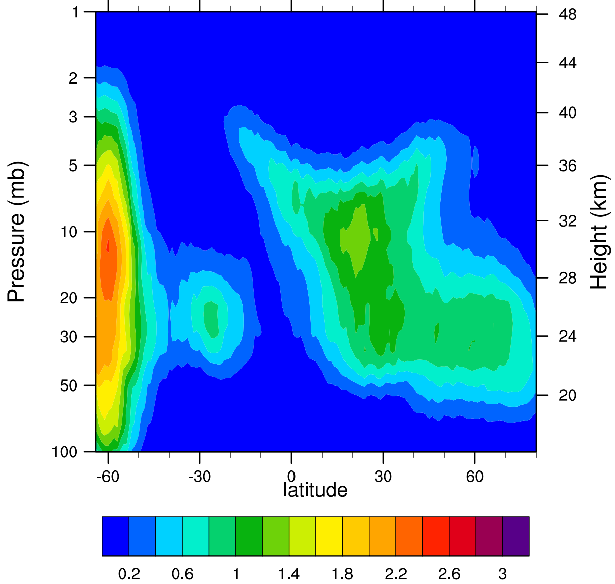
HIRDLSv6 2005d144 ClONO2_Ascending (ppbv)
