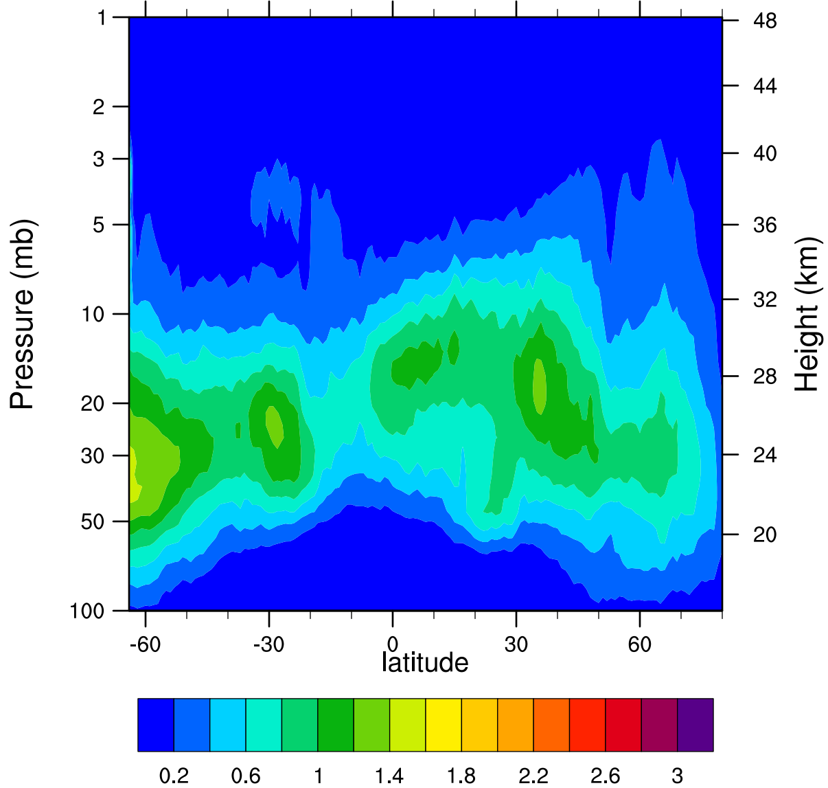
HIRDLSv6 2005d324 ClONO2_Ascending (ppbv)
