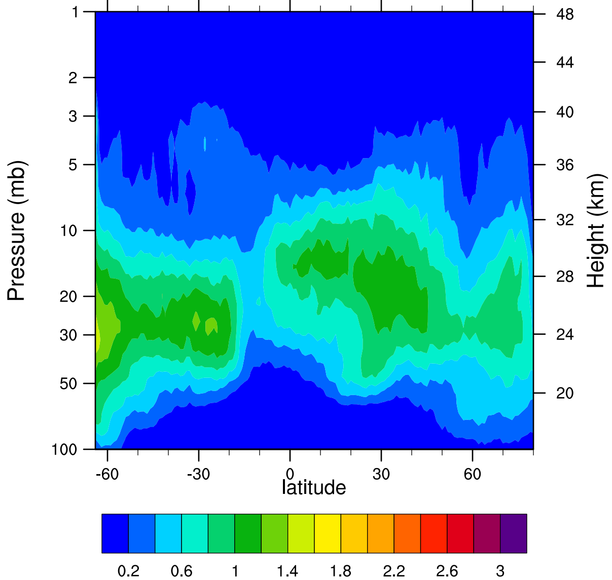
HIRDLSv6 2005d304 ClONO2_Ascending (ppbv)
