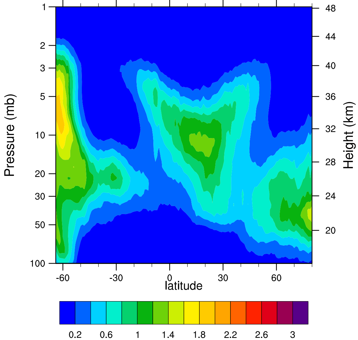
HIRDLSv6 2005d068 ClONO2_Ascending (ppbv)
