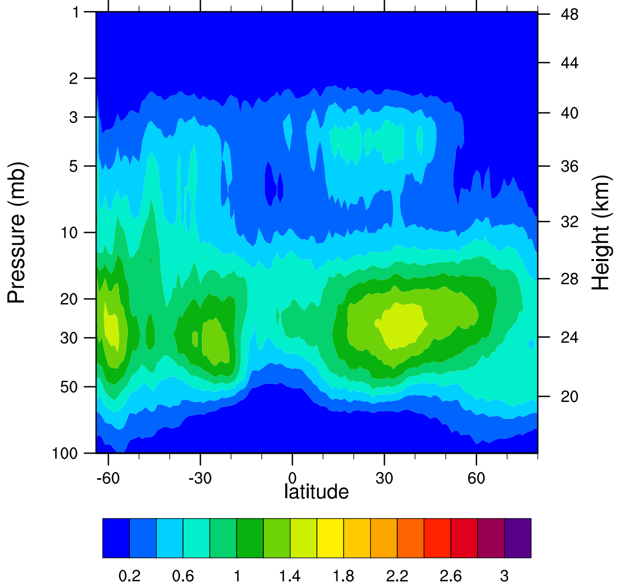
HIRDLSv6 2007d206 ClONO2_Ascending (ppbv)
