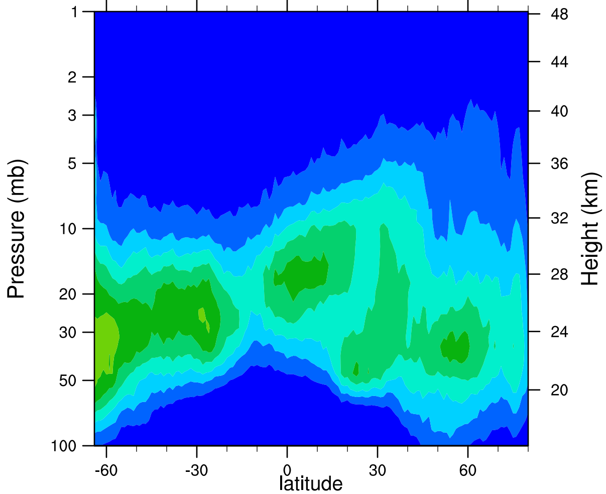
HIRDLSv6 2005d343 ClONO2_Ascending (ppbv)
