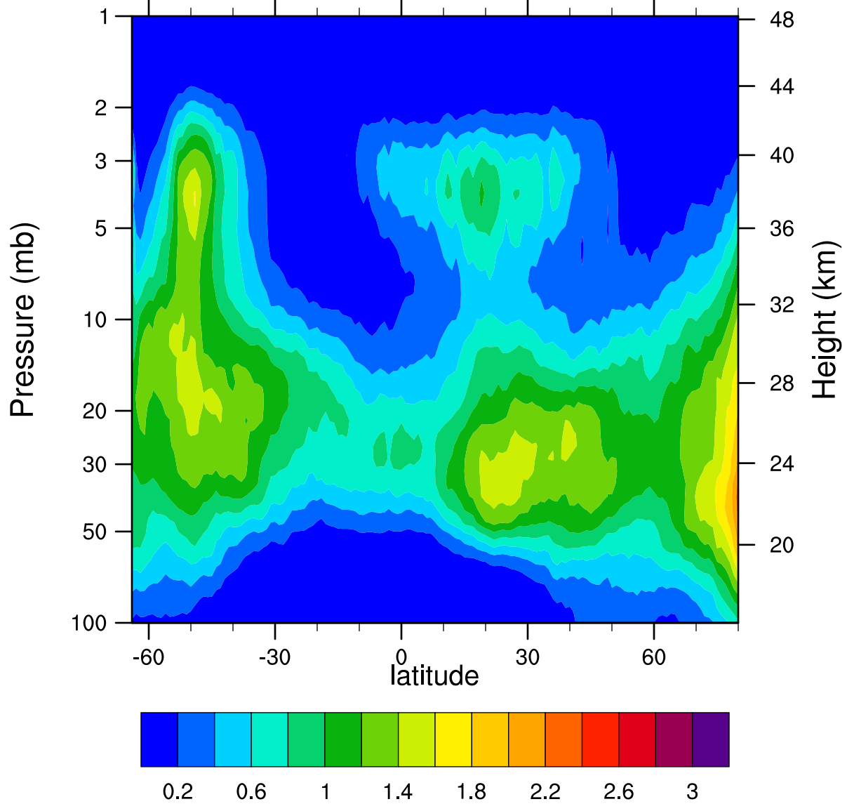
HIRDLSv6 2007d088 ClONO2_Ascending (ppbv)
