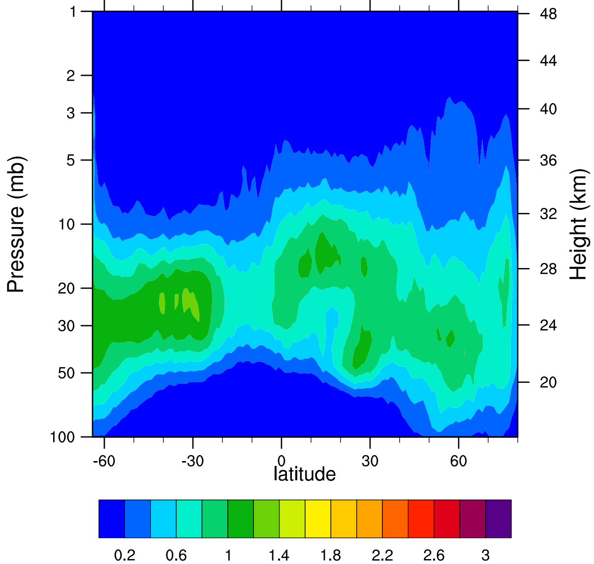
HIRDLSv6 2005d364 ClONO2_Ascending (ppbv)
