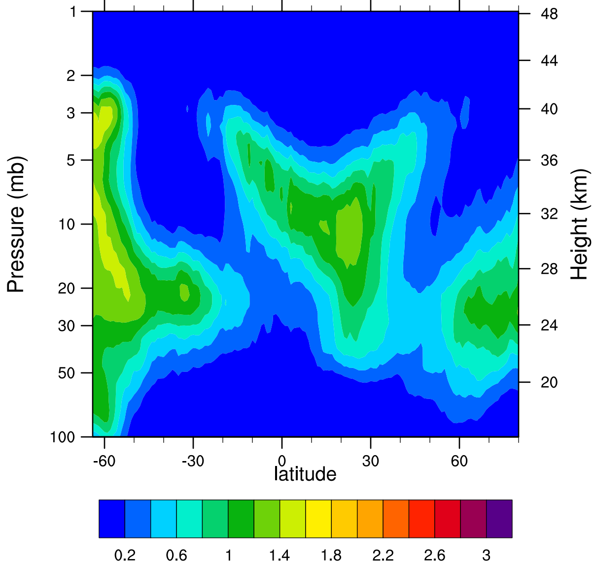
HIRDLSv6 2005d039 ClONO2_Ascending (ppbv)
