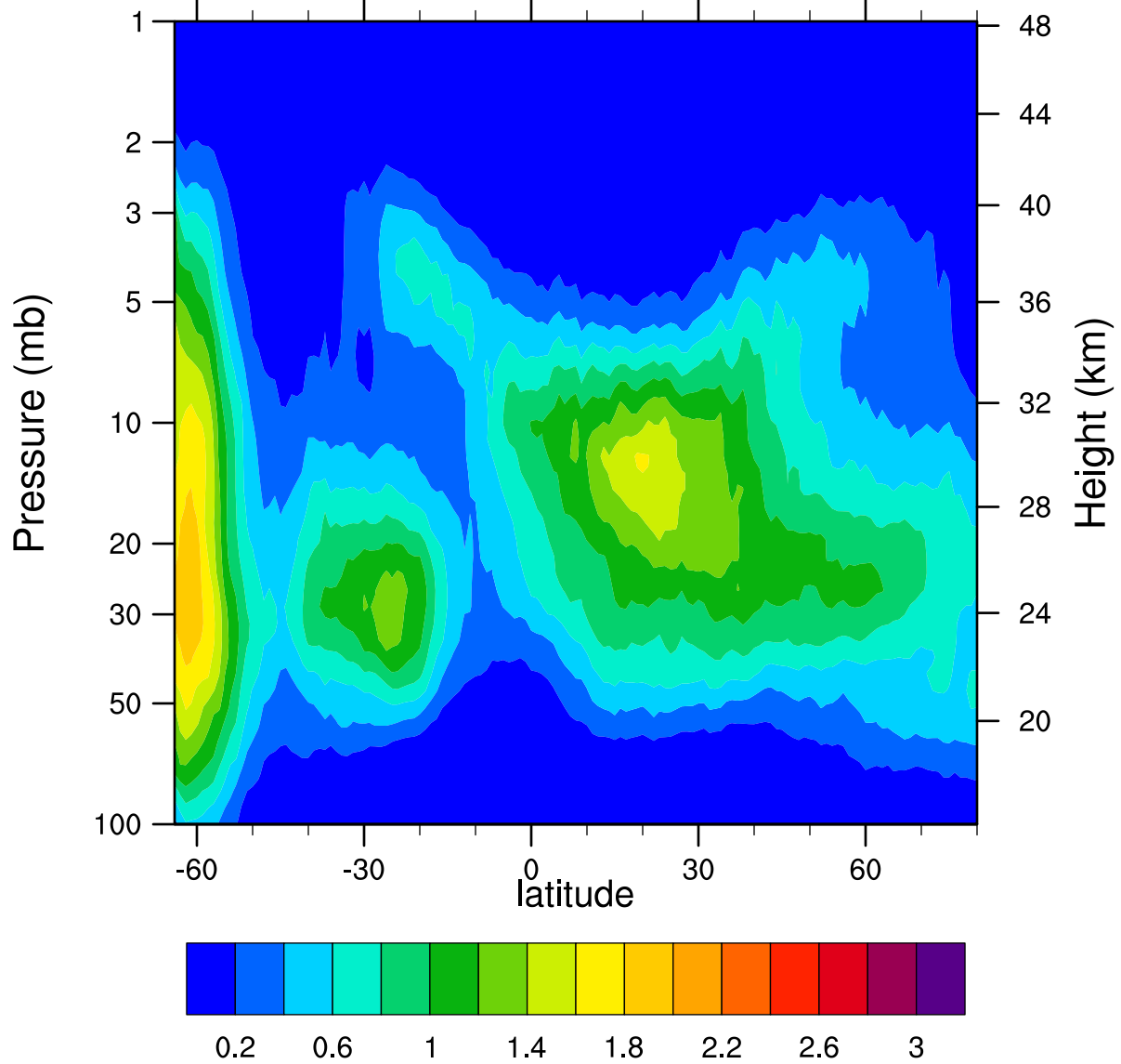
HIRDLSv6 2005d237 ClONO2_Ascending (ppbv)
