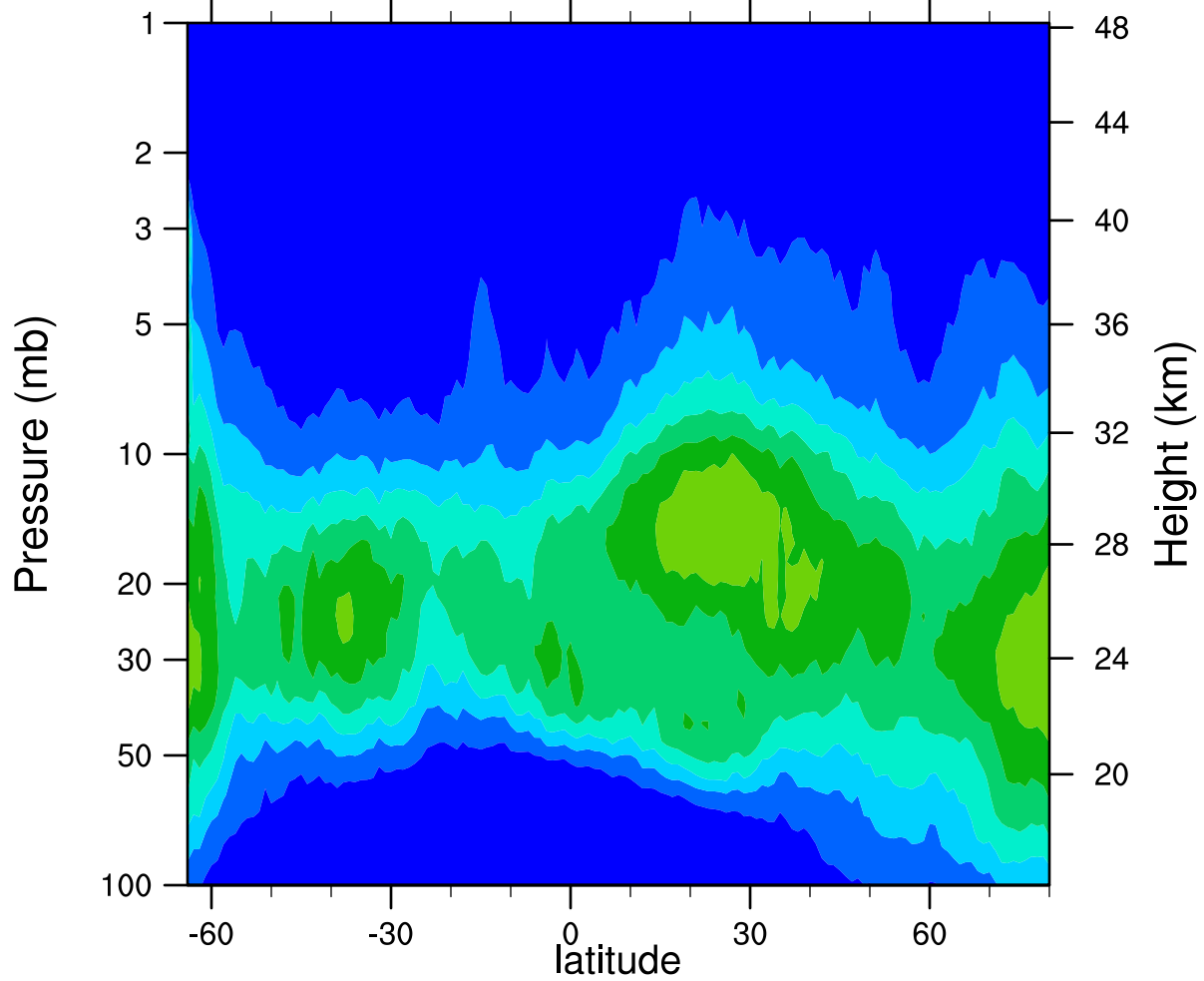
HIRDLSv6 2006d097 ClONO2_Ascending (ppbv)
