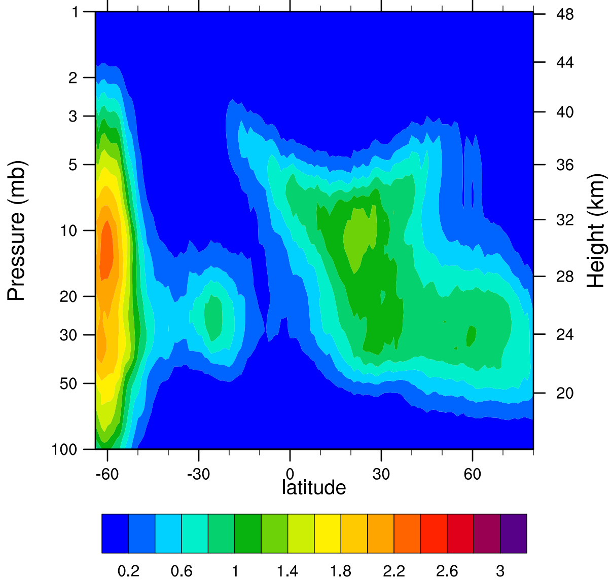
HIRDLSv6 2005d149 ClONO2_Ascending (ppbv)
