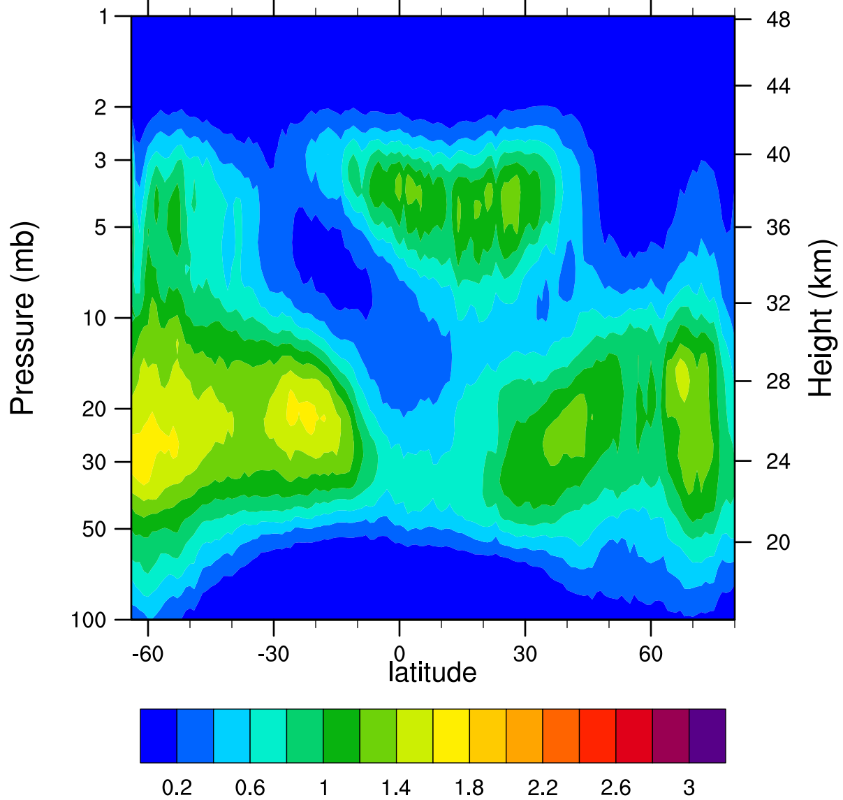
HIRDLSv6 2006d315 ClONO2_Ascending (ppbv)
