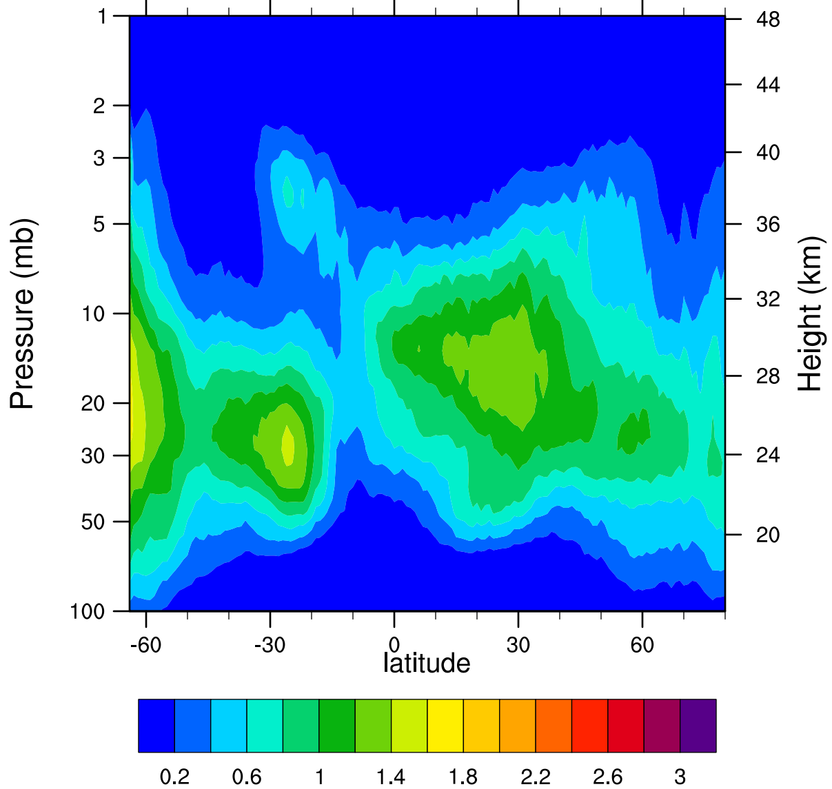
HIRDLSv6 2005d282 ClONO2_Ascending (ppbv)
