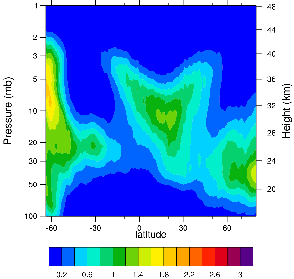
HIRDLSv6 2005d066 ClONO2_Ascending (ppbv)
