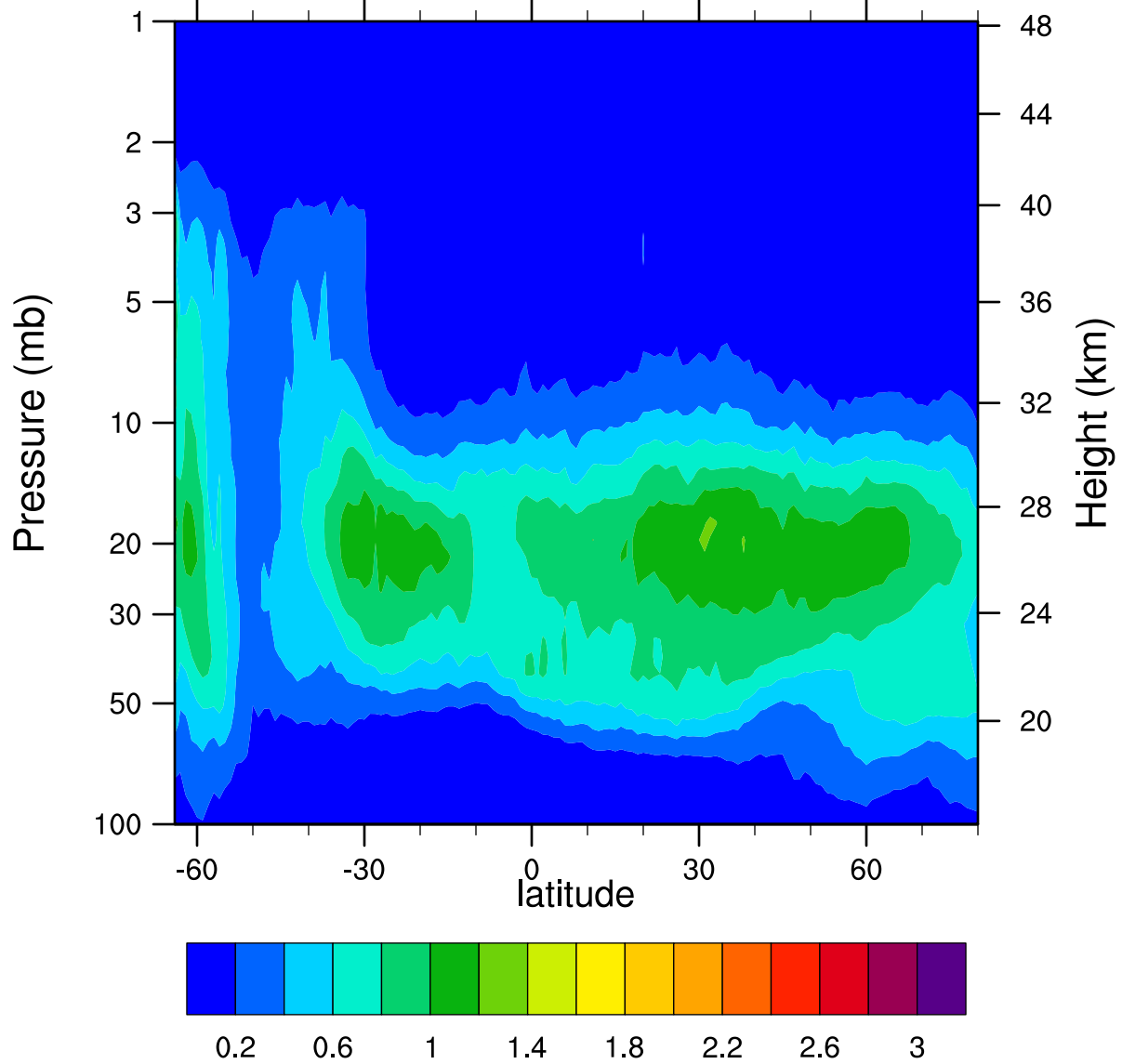
HIRDLSv6 2006d180 ClONO2_Ascending (ppbv)
