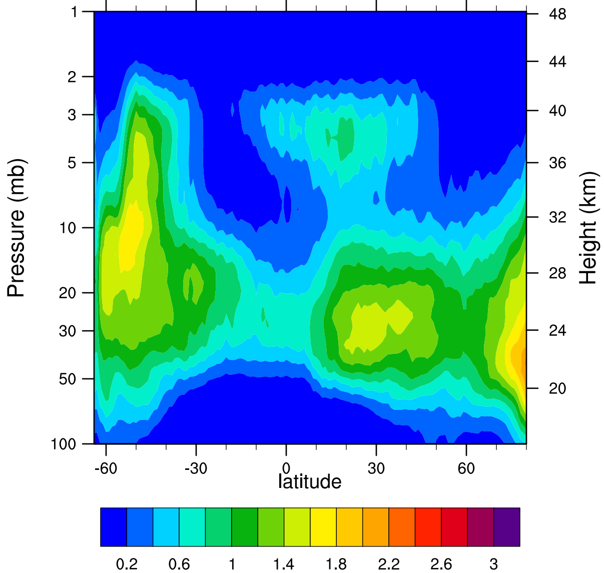
HIRDLSv6 2007d103 ClONO2_Ascending (ppbv)
