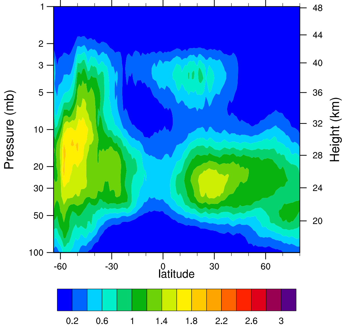
HIRDLSv6 2007d140 ClONO2_Ascending (ppbv)
