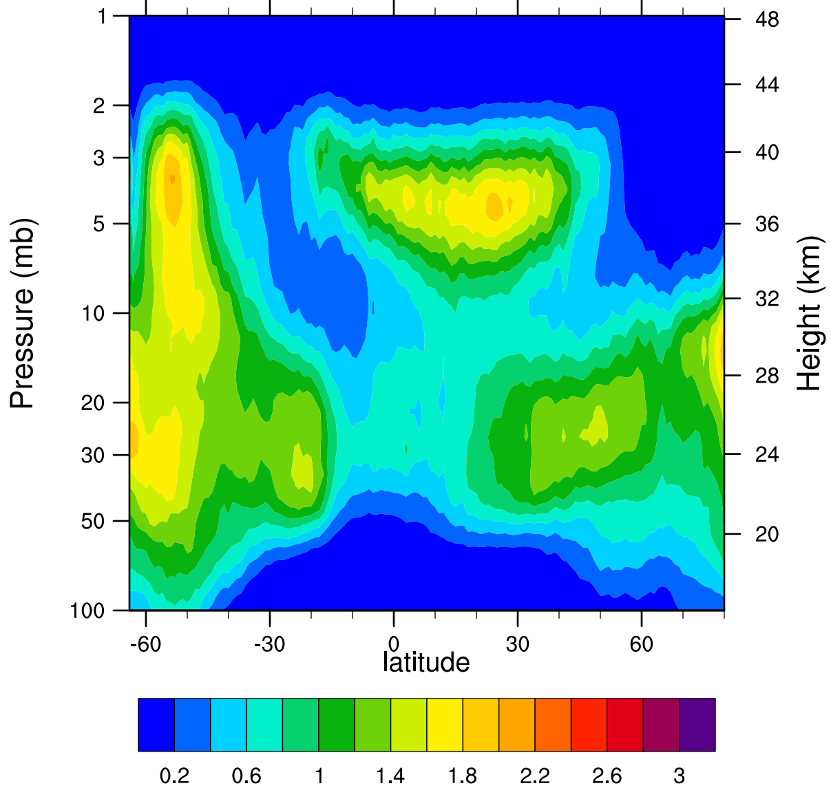
HIRDLSv6 2007d276 ClONO2_Ascending (ppbv)
