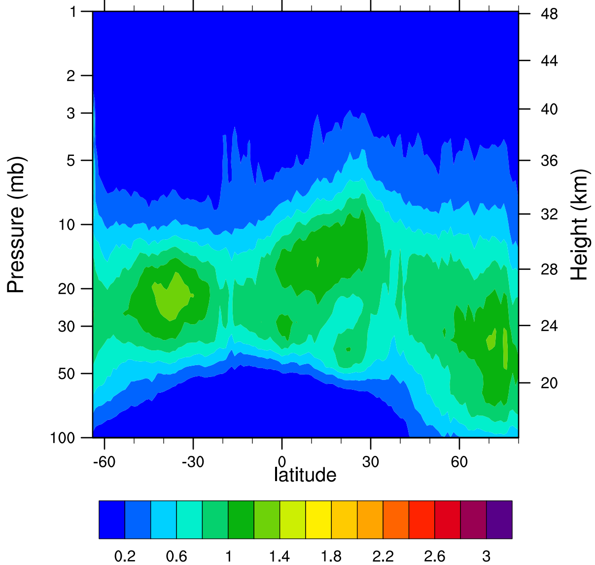
HIRDLSv6 2006d058 ClONO2_Ascending (ppbv)
