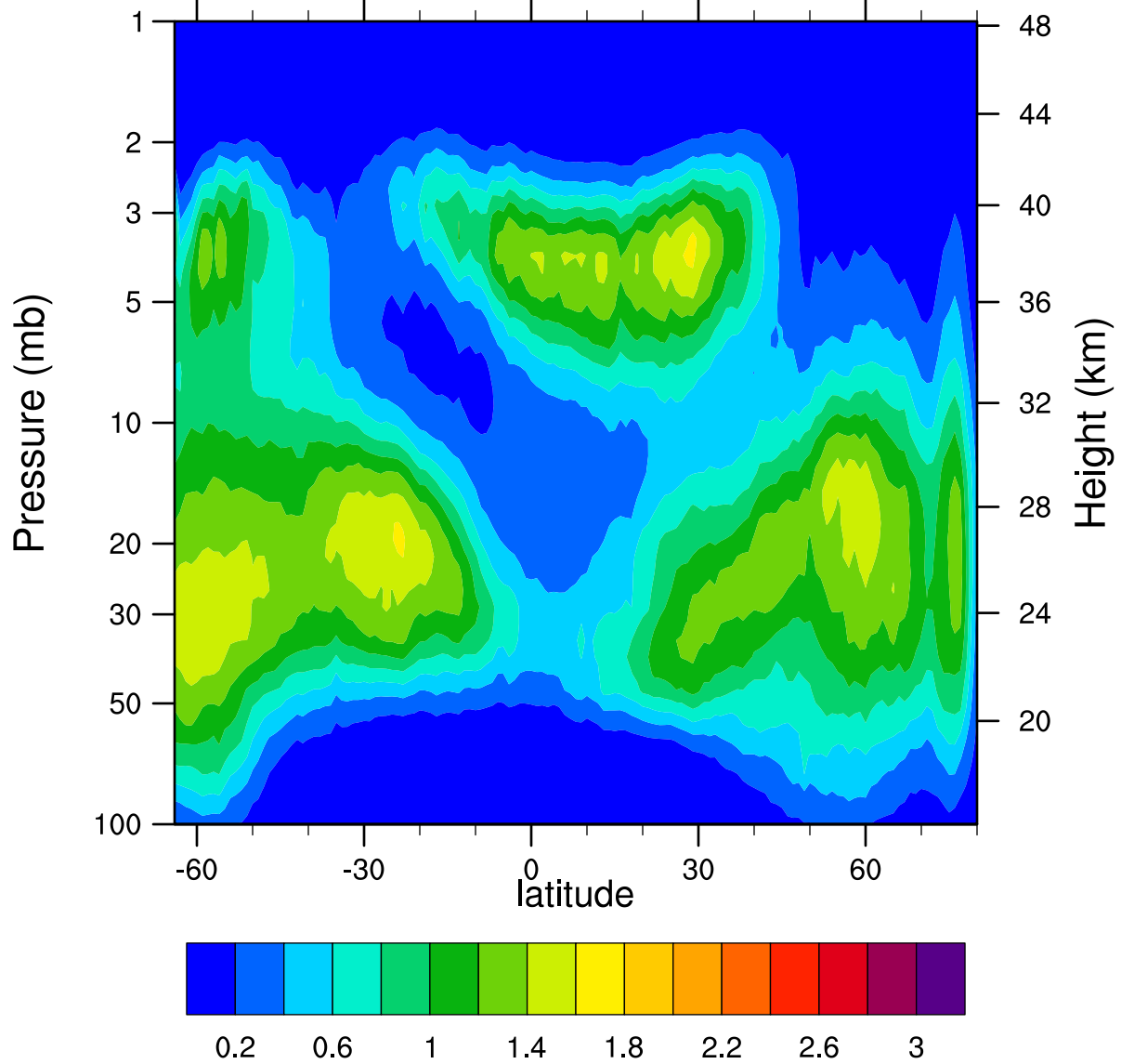
HIRDLSv6 2006d344 ClONO2_Ascending (ppbv)
