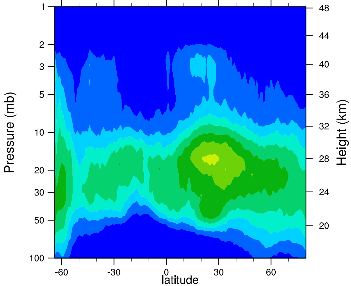
HIRDLSv6 2006d128 ClONO2_Ascending (ppbv)
