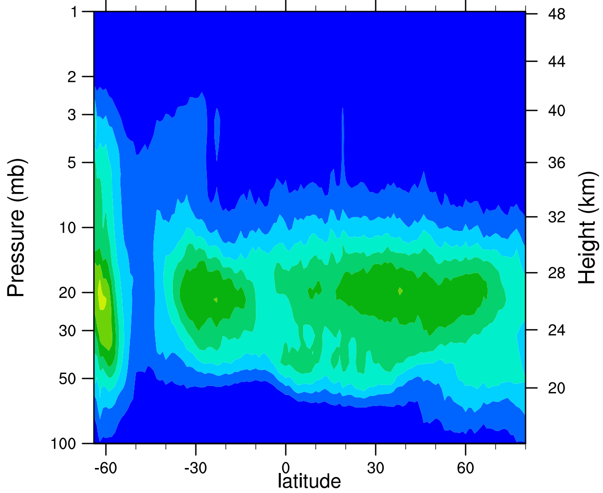
HIRDLSv6 2006d186 ClONO2_Ascending (ppbv)
