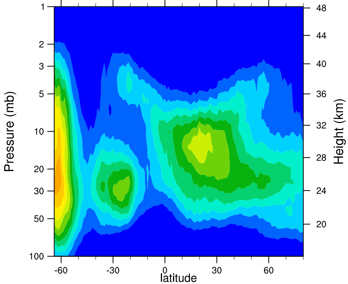
HIRDLSv6 2005d232 ClONO2_Ascending (ppbv)
