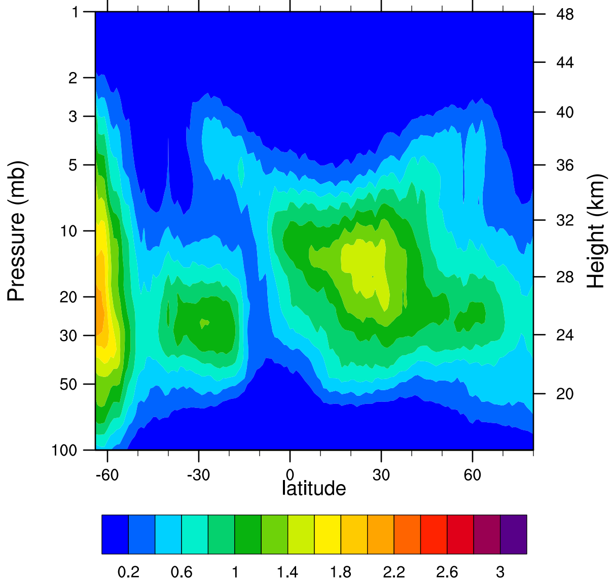
HIRDLSv6 2005d254 ClONO2_Ascending (ppbv)
