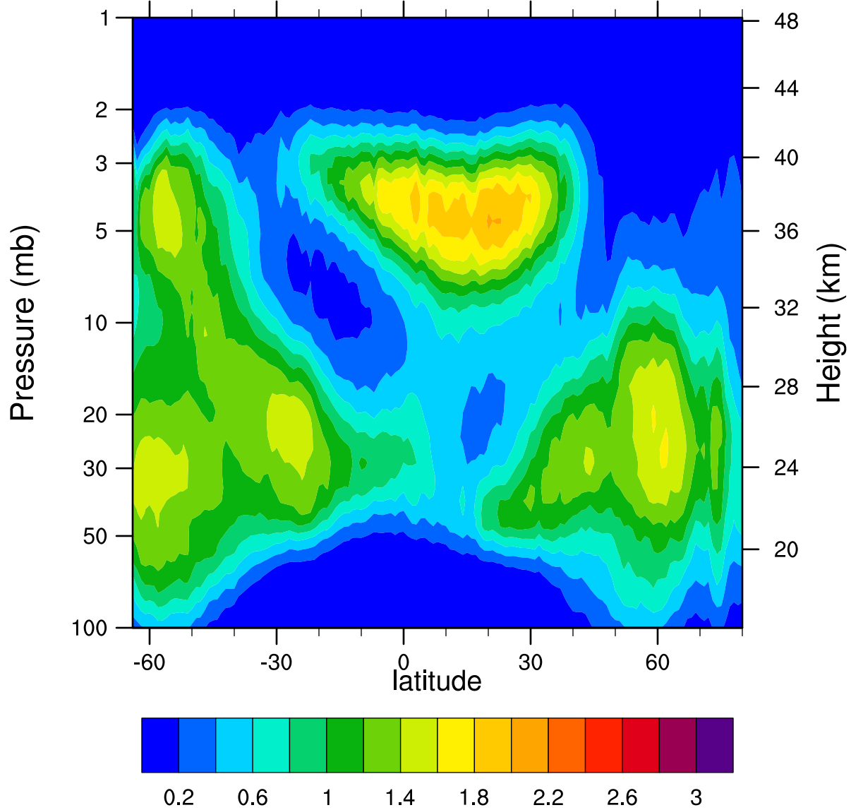
HIRDLSv6 2007d339 ClONO2_Ascending (ppbv)
