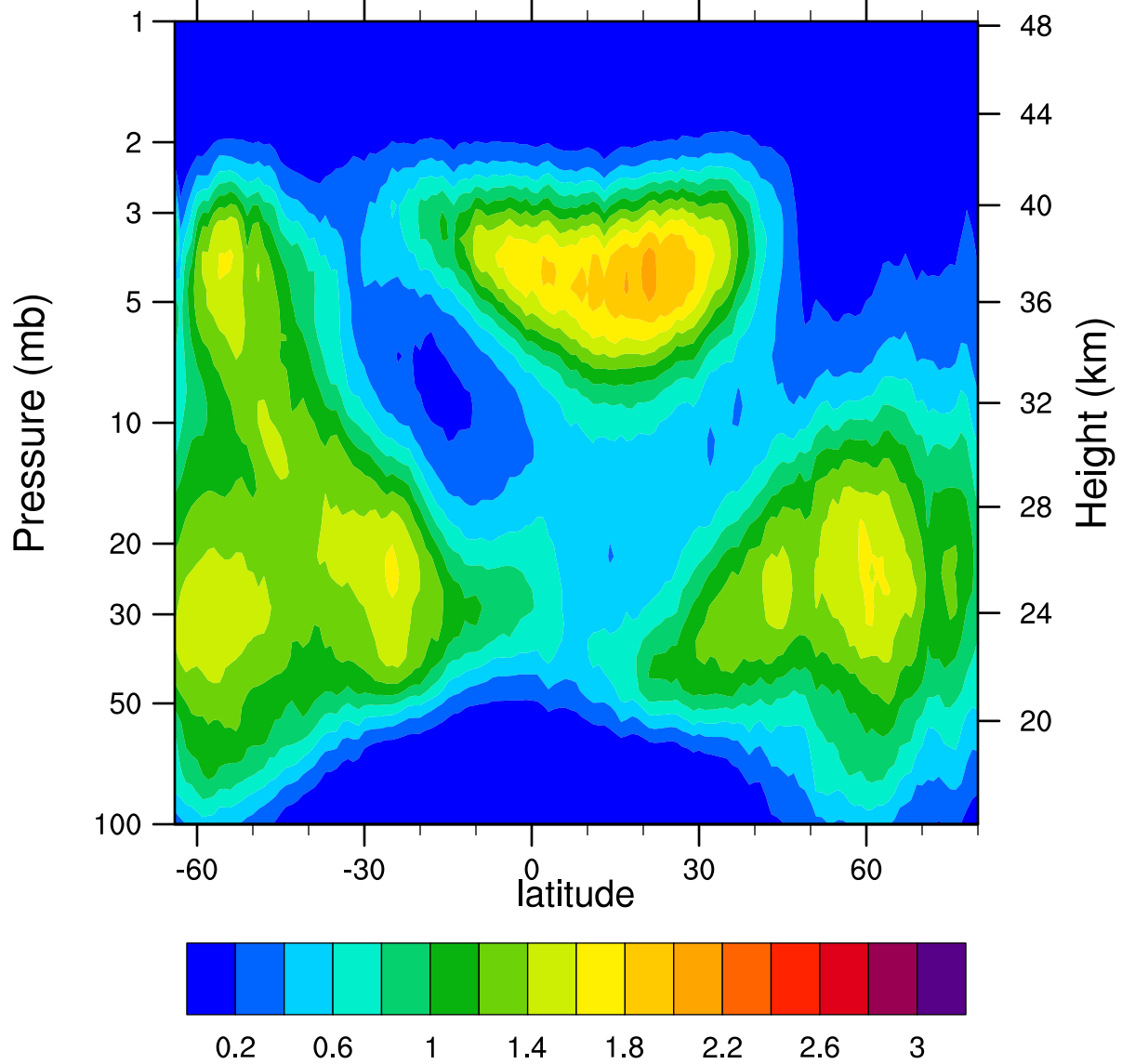
HIRDLSv6 2007d331 ClONO2_Ascending (ppbv)
