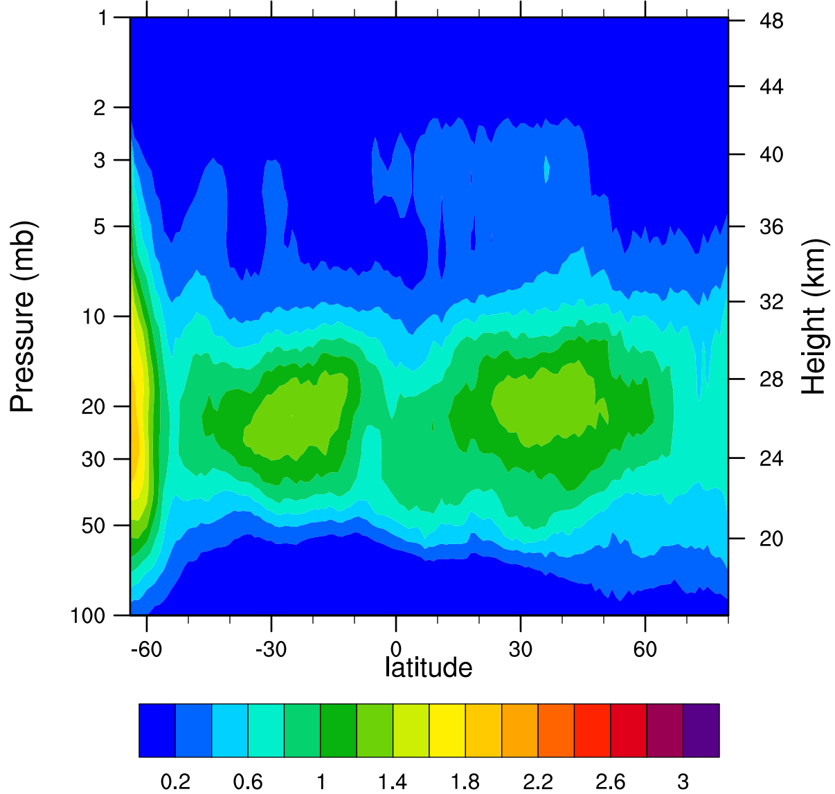
HIRDLSv6 2006d266 ClONO2_Ascending (ppbv)
