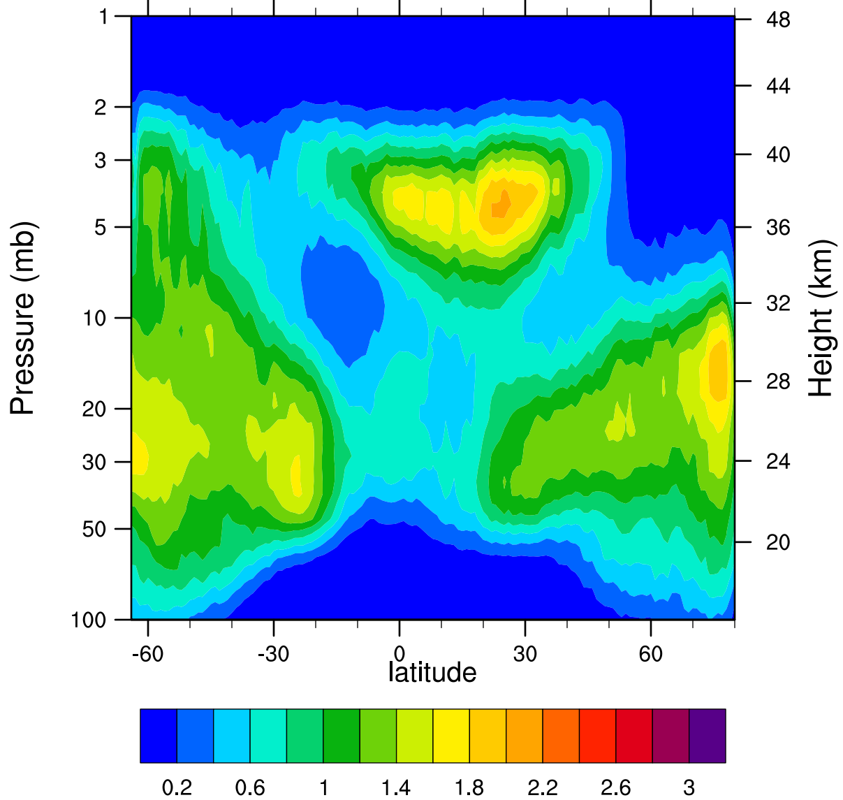
HIRDLSv6 2007d291 ClONO2_Ascending (ppbv)
