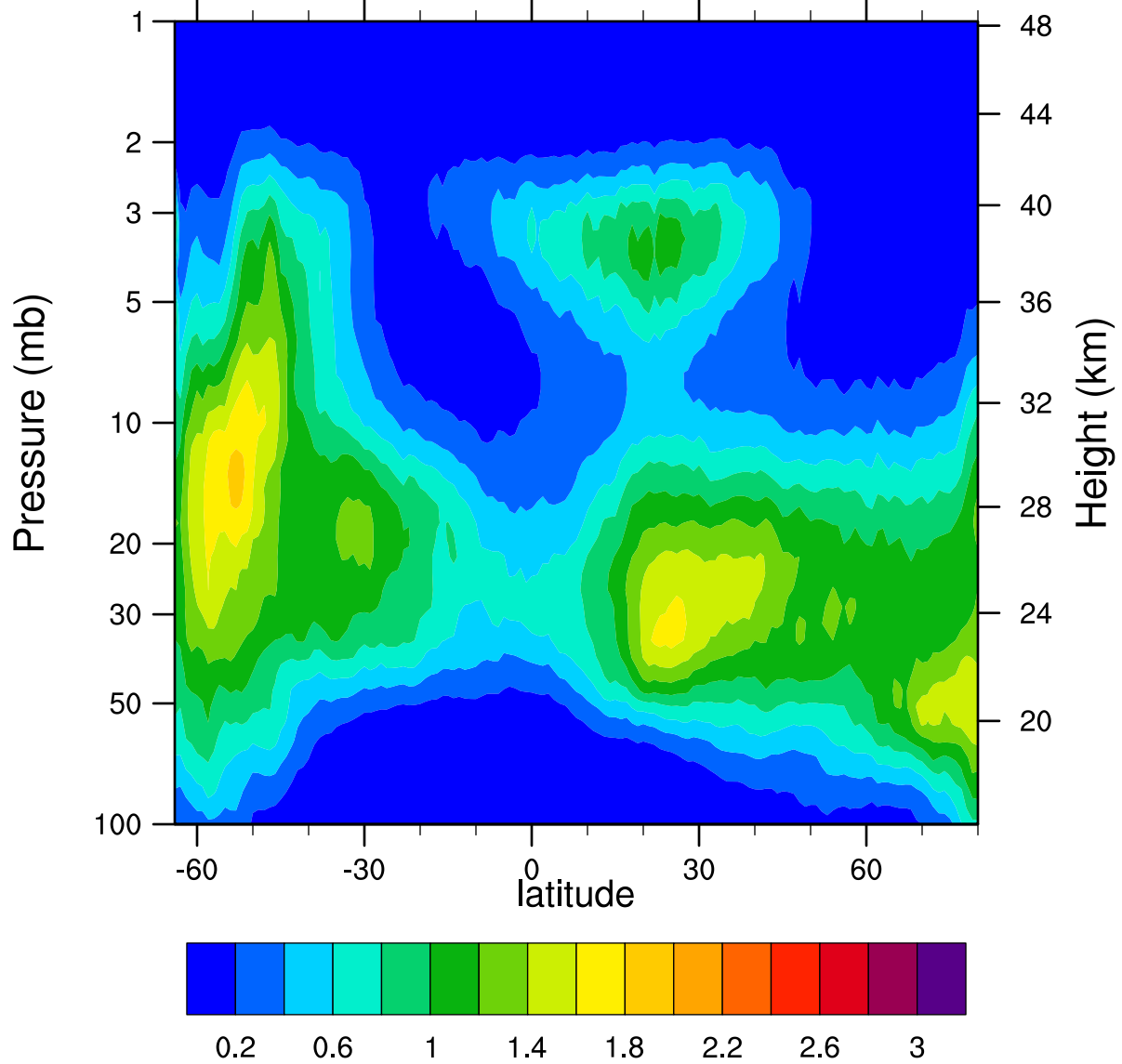
HIRDLSv6 2007d117 ClONO2_Ascending (ppbv)
