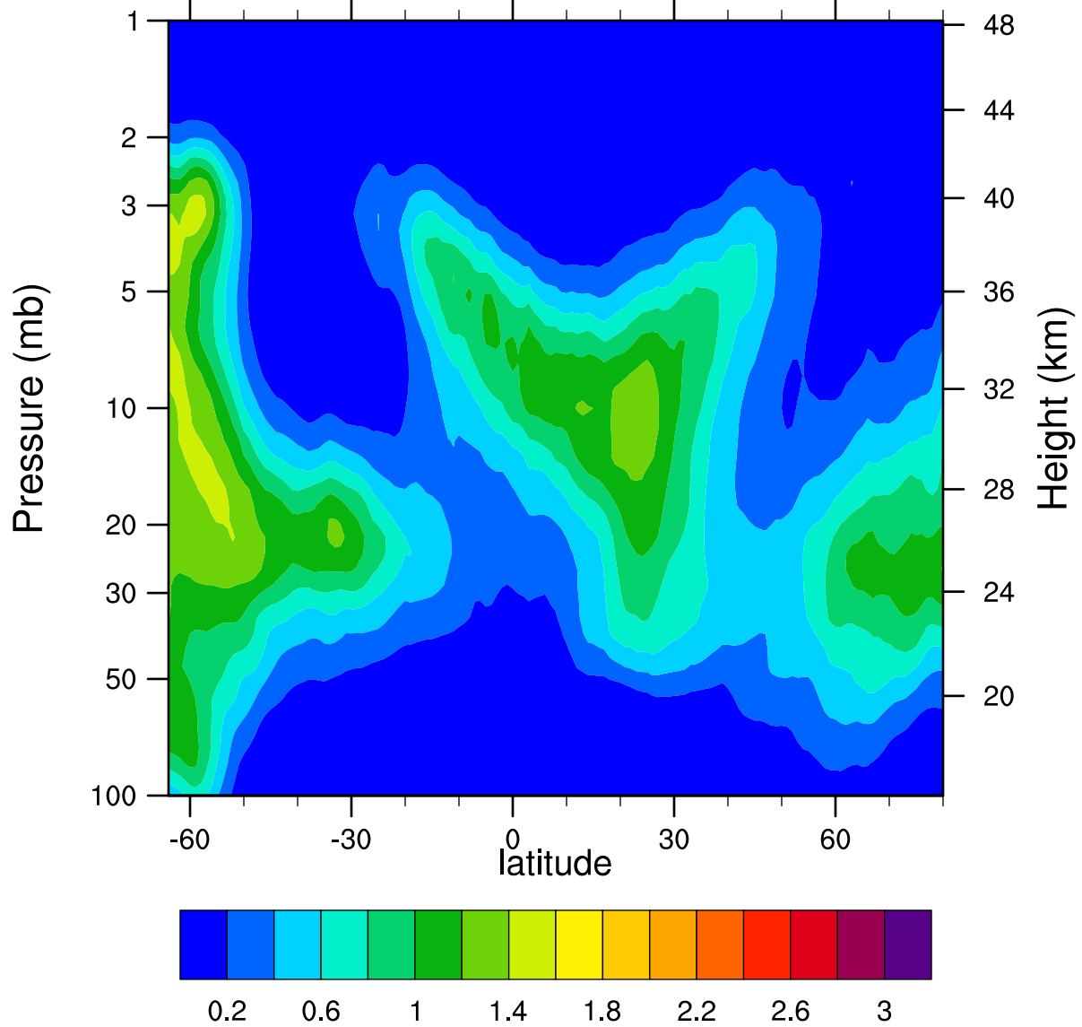
HIRDLSv6 2005d040 ClONO2_Ascending (ppbv)
