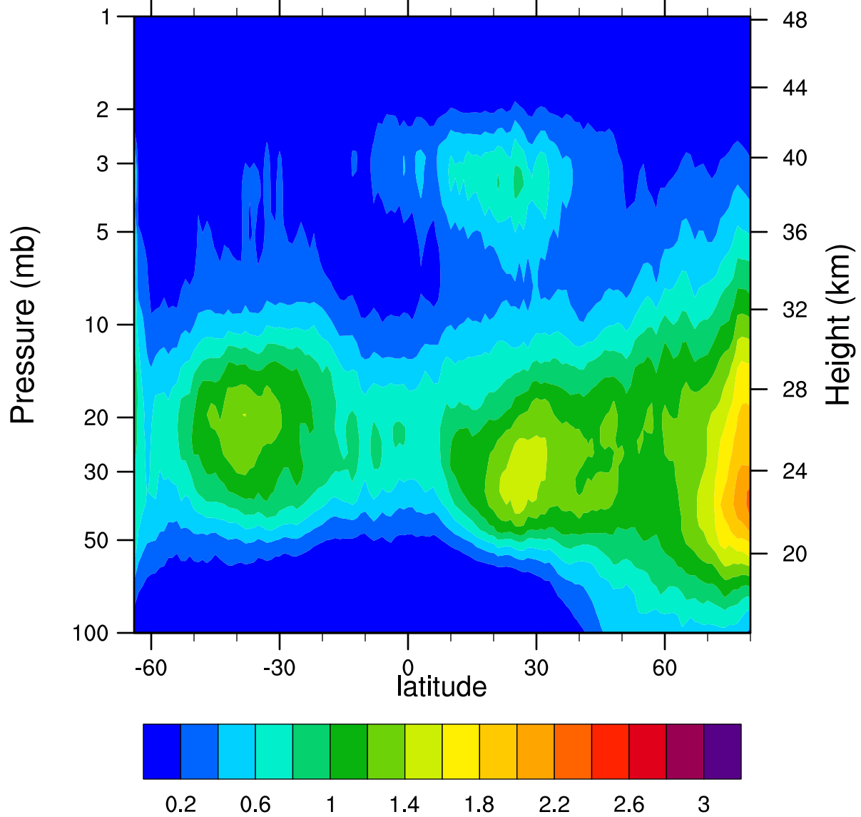
HIRDLSv6 2007d072 ClONO2_Ascending (ppbv)
