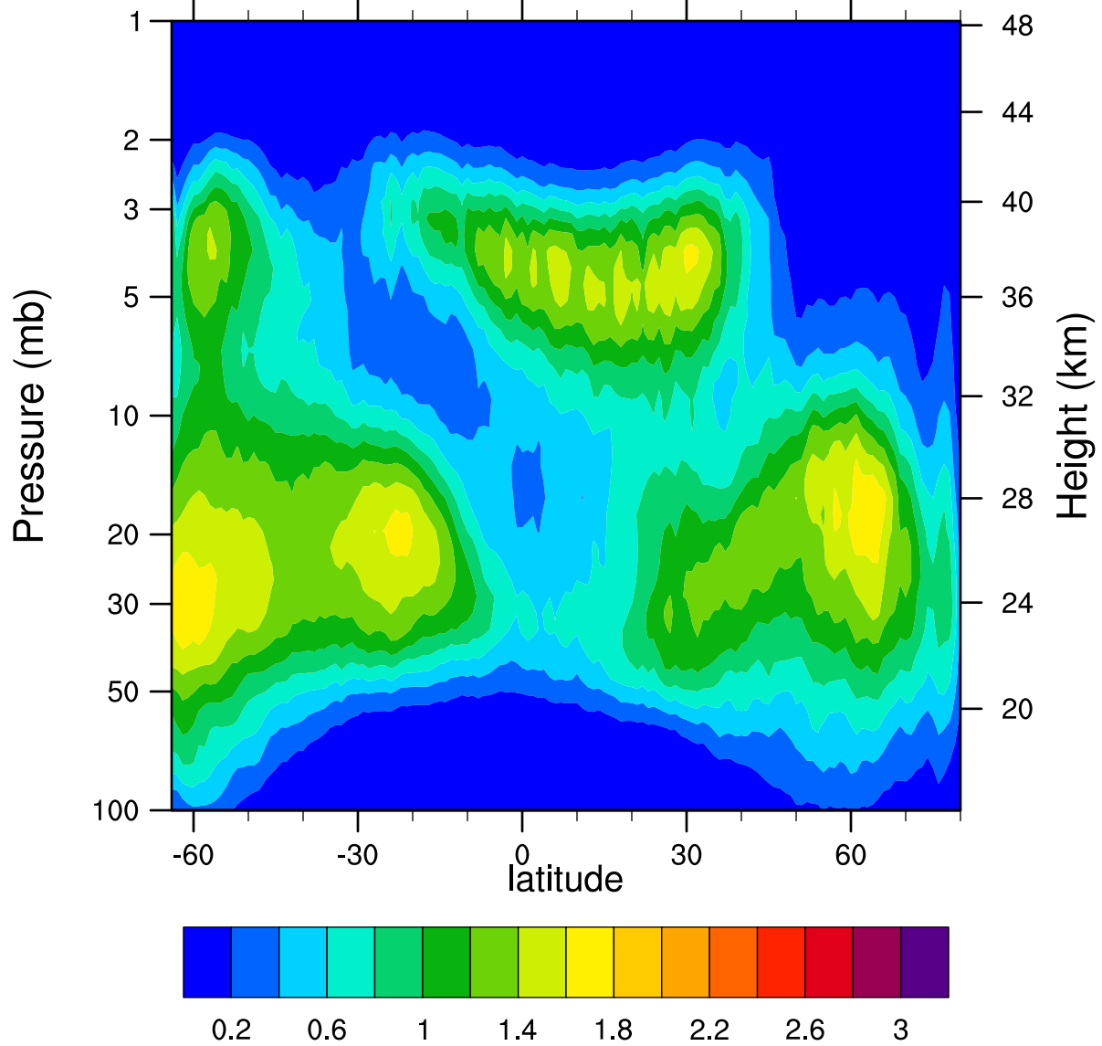
HIRDLSv6 2006d333 ClONO2_Ascending (ppbv)
