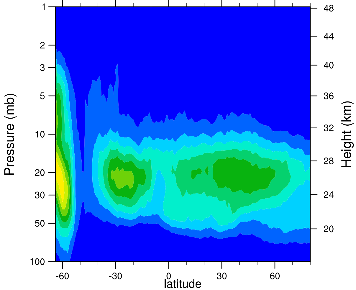
HIRDLSv6 2006d203 ClONO2_Ascending (ppbv)
