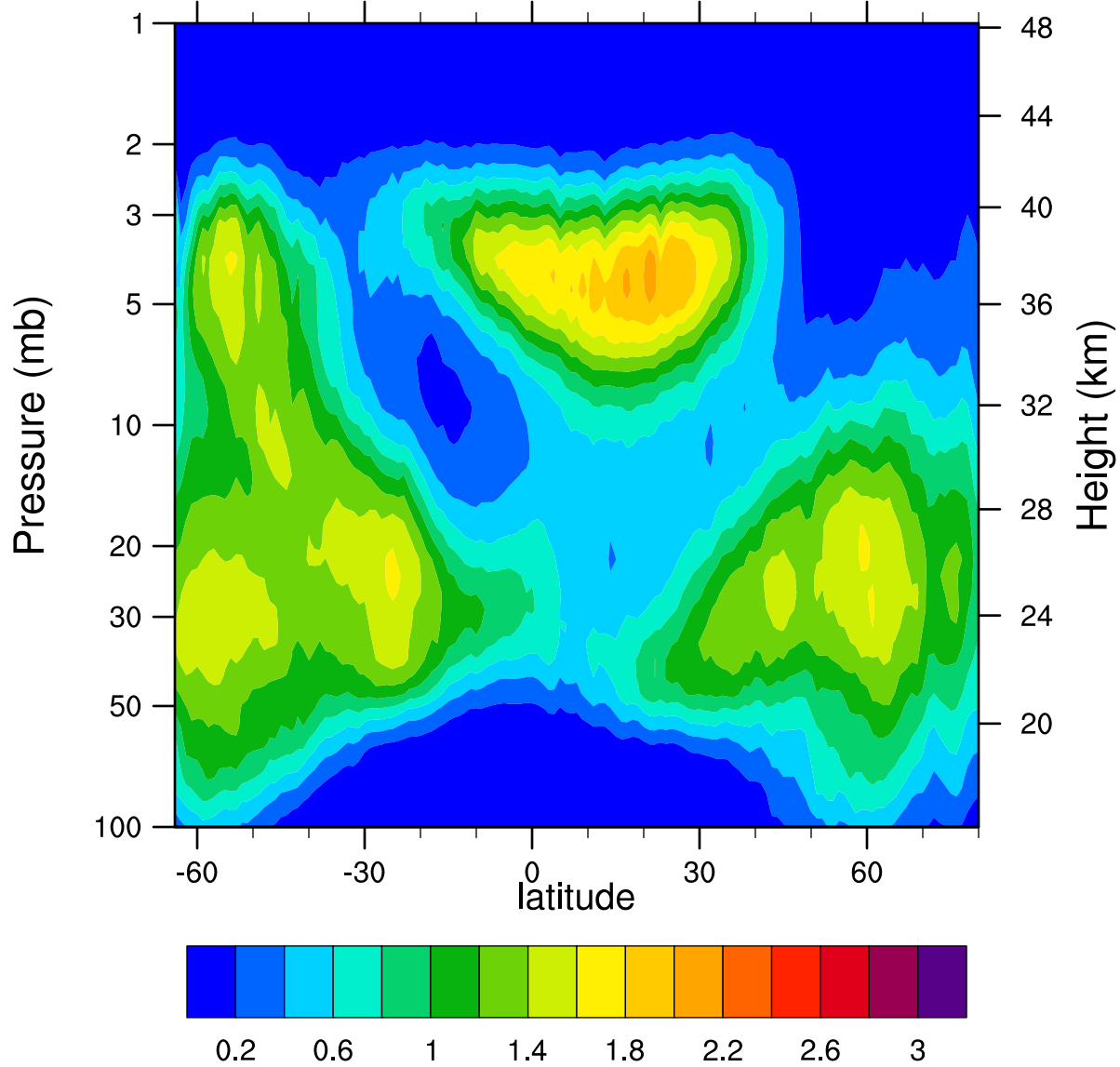
HIRDLSv6 2007d330 ClONO2_Ascending (ppbv)
