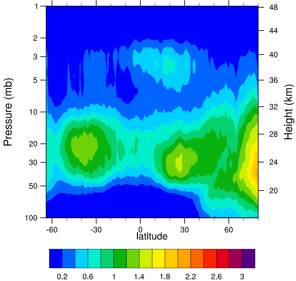
HIRDLSv6 2007d062 ClONO2_Ascending (ppbv)
