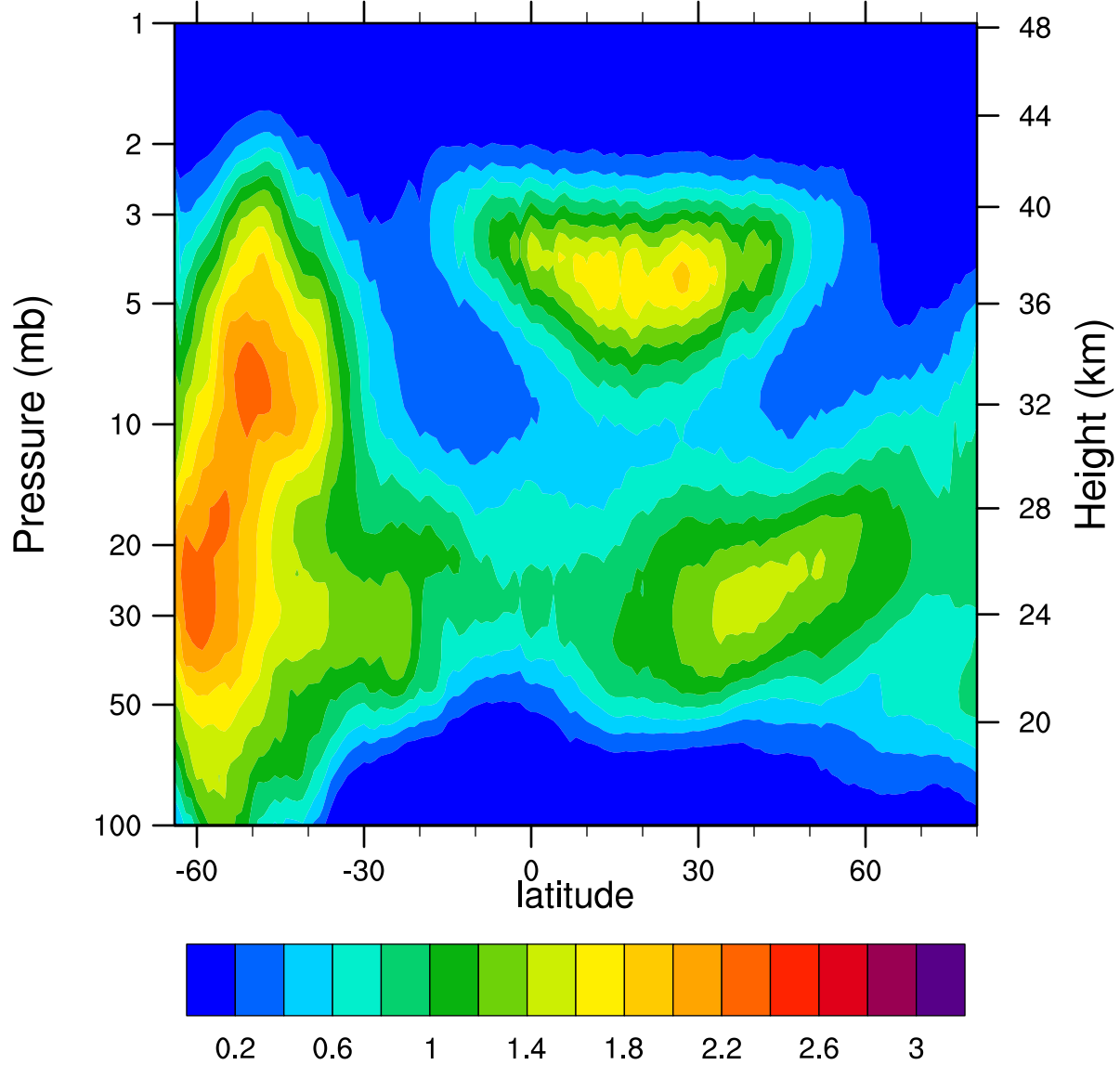
HIRDLSv6 2007d222 ClONO2_Ascending (ppbv)
