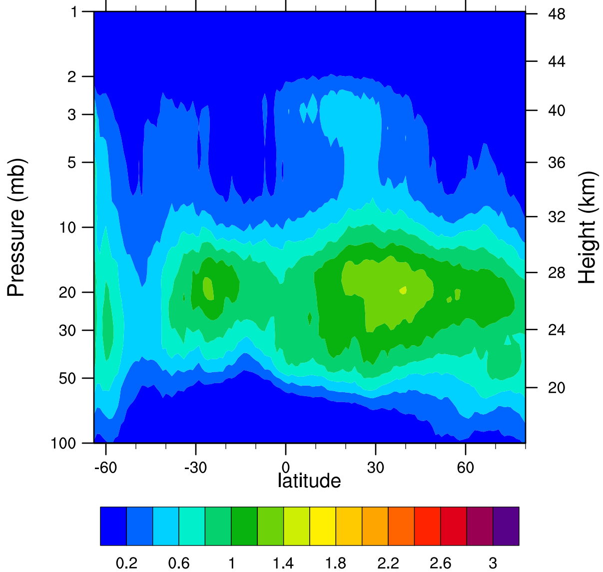
HIRDLSv6 2006d156 ClONO2_Ascending (ppbv)
