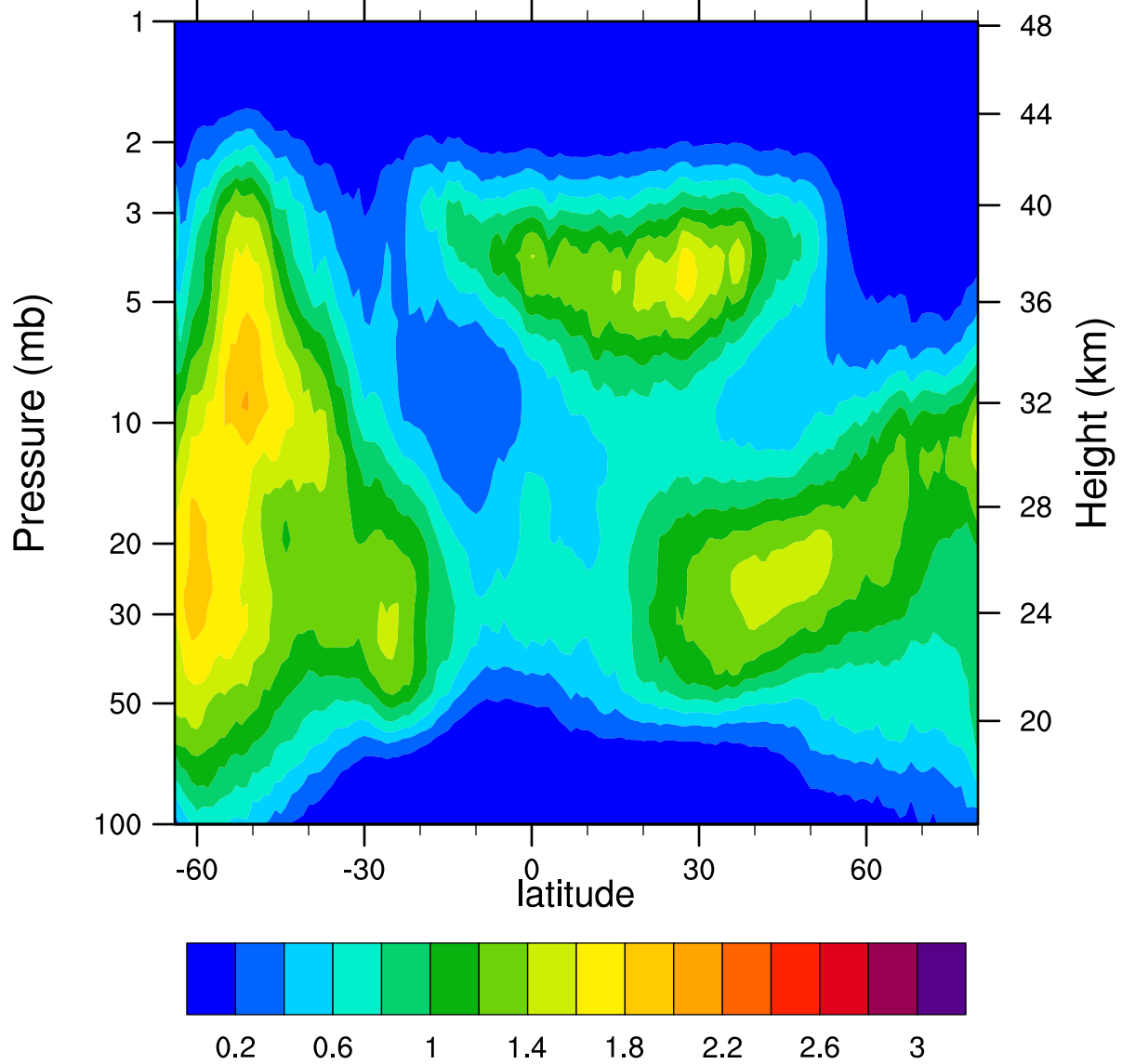
HIRDLSv6 2007d257 ClONO2_Ascending (ppbv)
