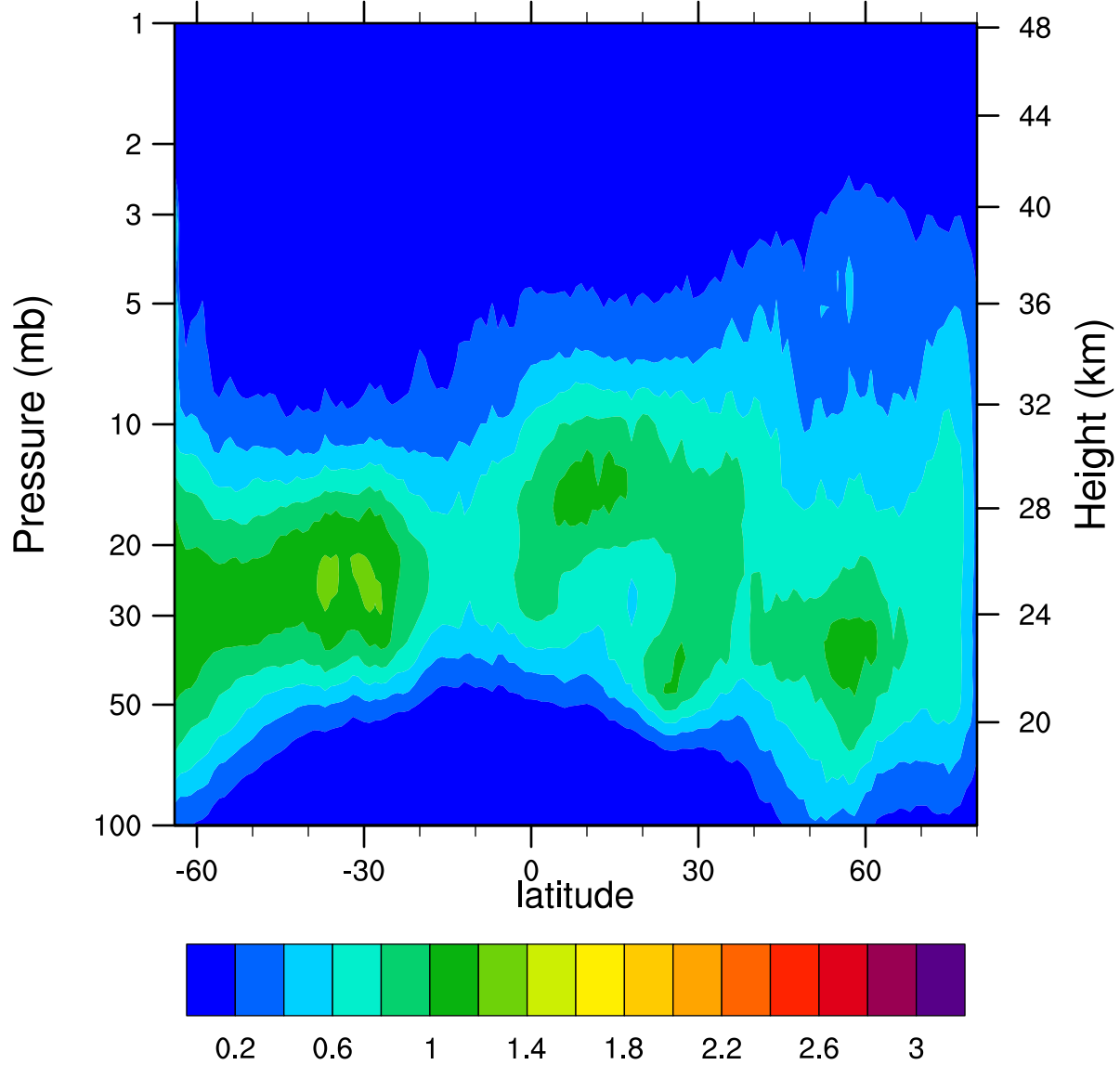
HIRDLSv6 2005d359 ClONO2_Ascending (ppbv)
