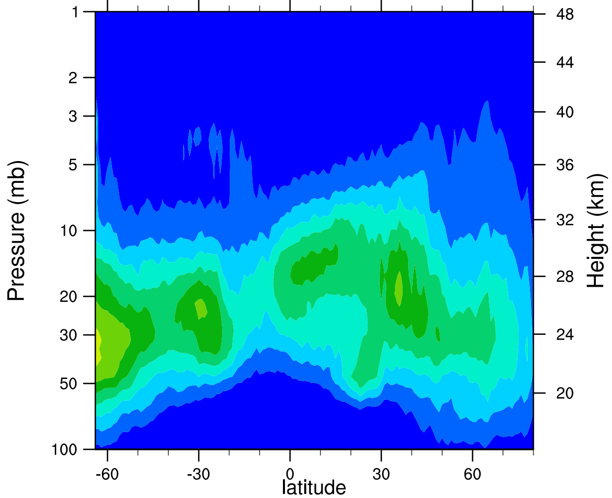
HIRDLSv6 2005d326 ClONO2_Ascending (ppbv)
