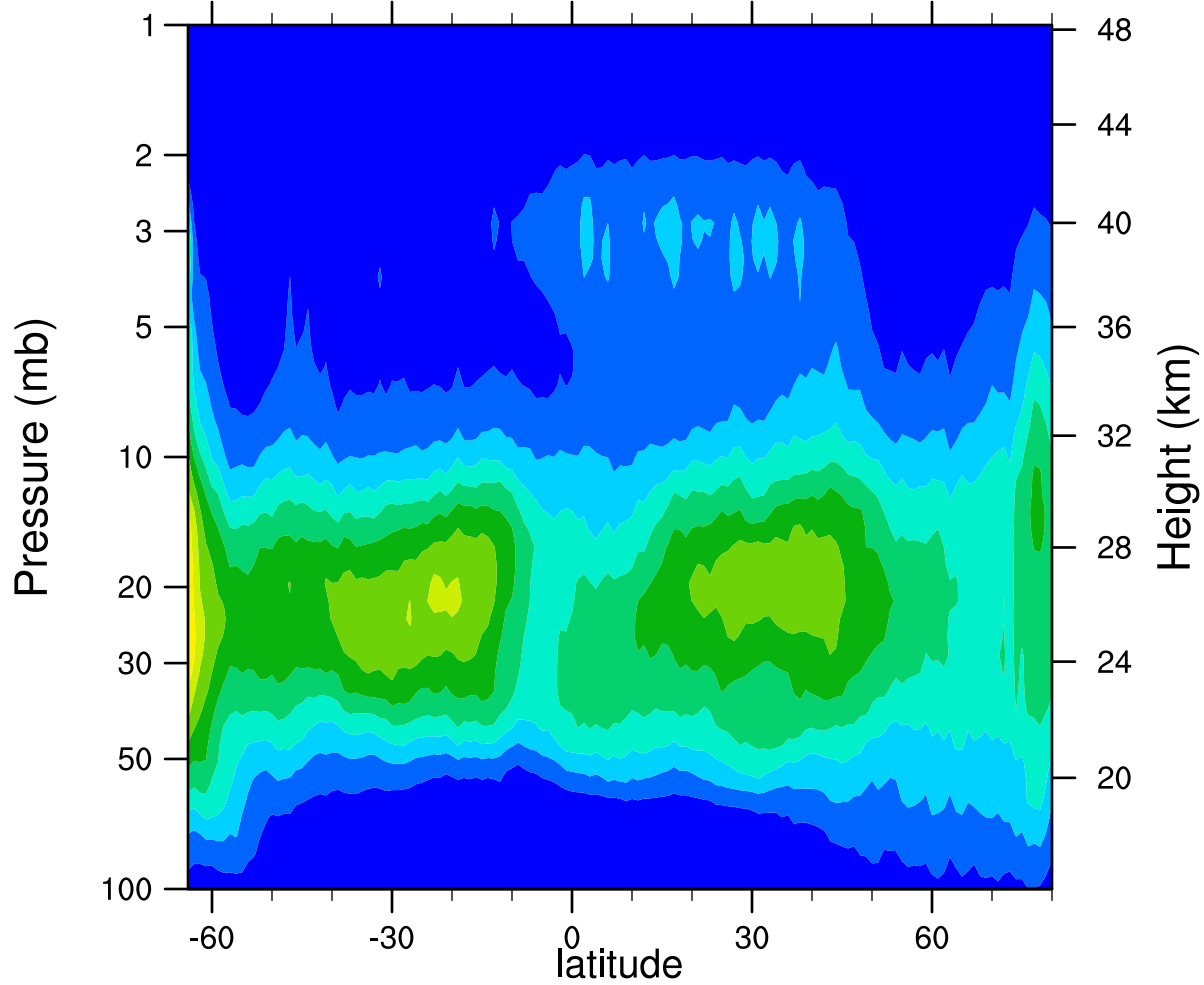
HIRDLSv6 2006d286 ClONO2_Ascending (ppbv)
