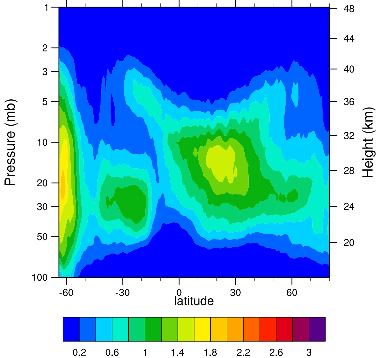
HIRDLSv6 2005d244 ClONO2_Ascending (ppbv)
