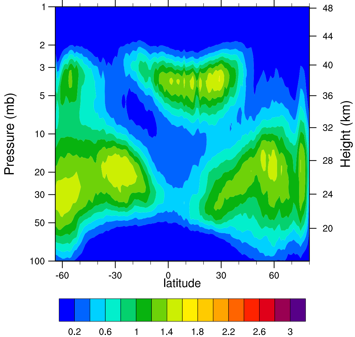
HIRDLSv6 2006d346 ClONO2_Ascending (ppbv)
