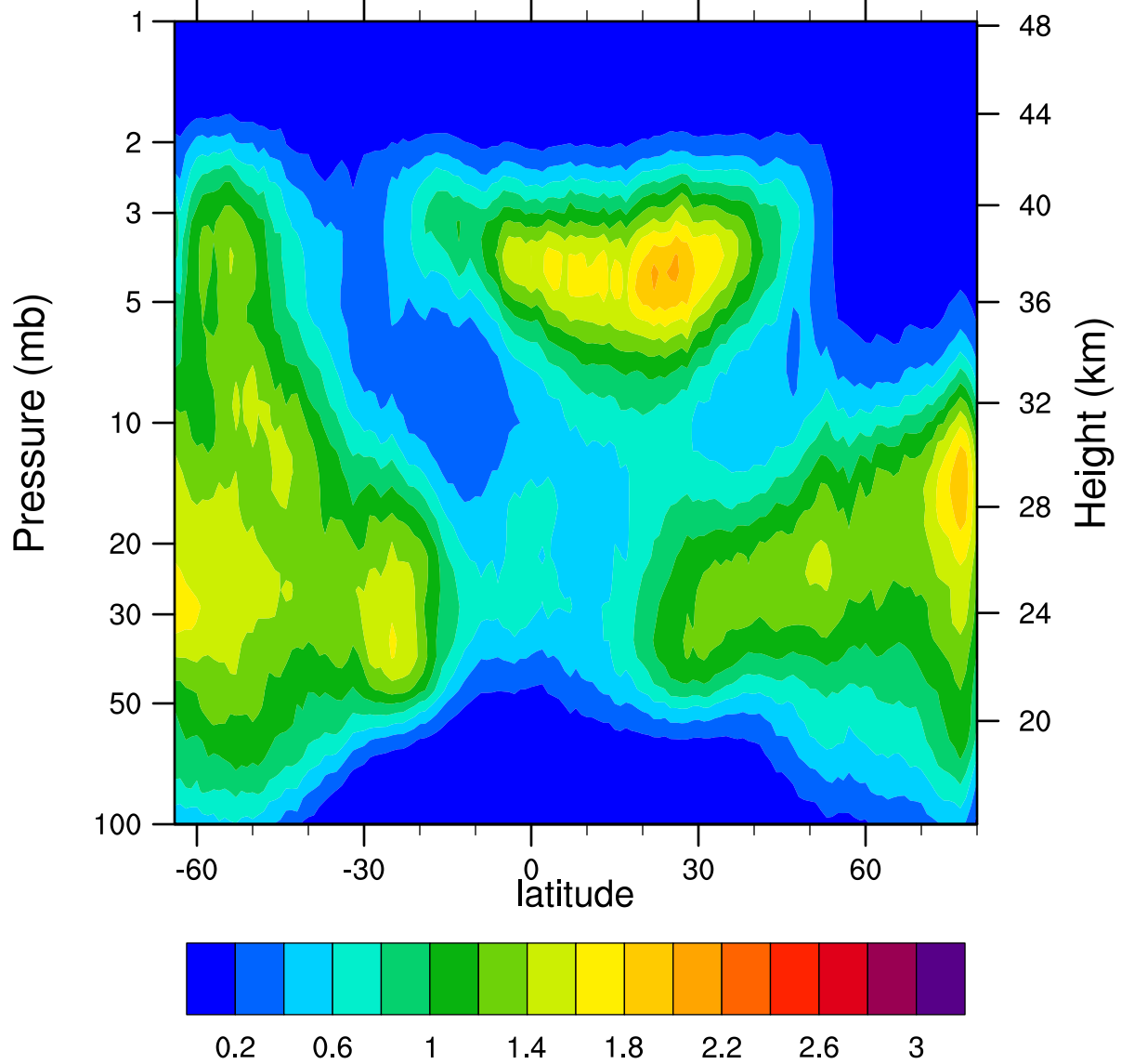
HIRDLSv6 2007d288 ClONO2_Ascending (ppbv)
