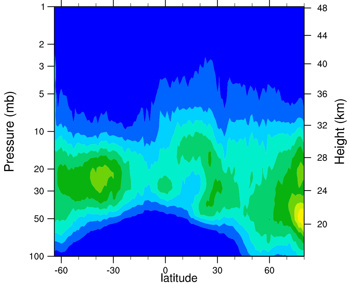
HIRDLSv6 2006d025 ClONO2_Ascending (ppbv)
