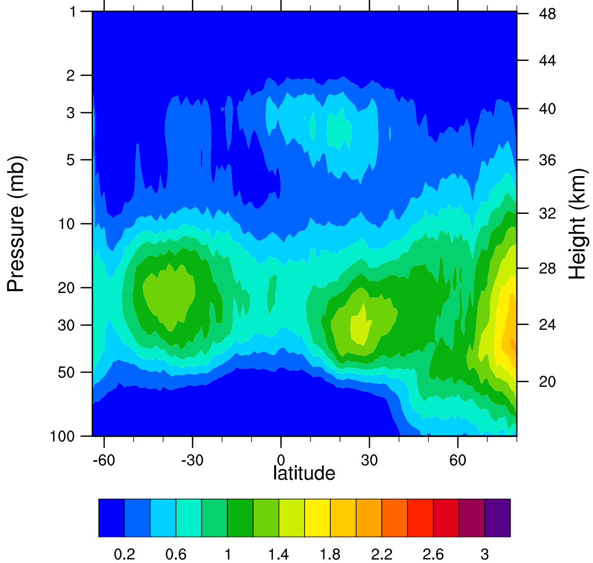
HIRDLSv6 2007d063 ClONO2_Ascending (ppbv)
