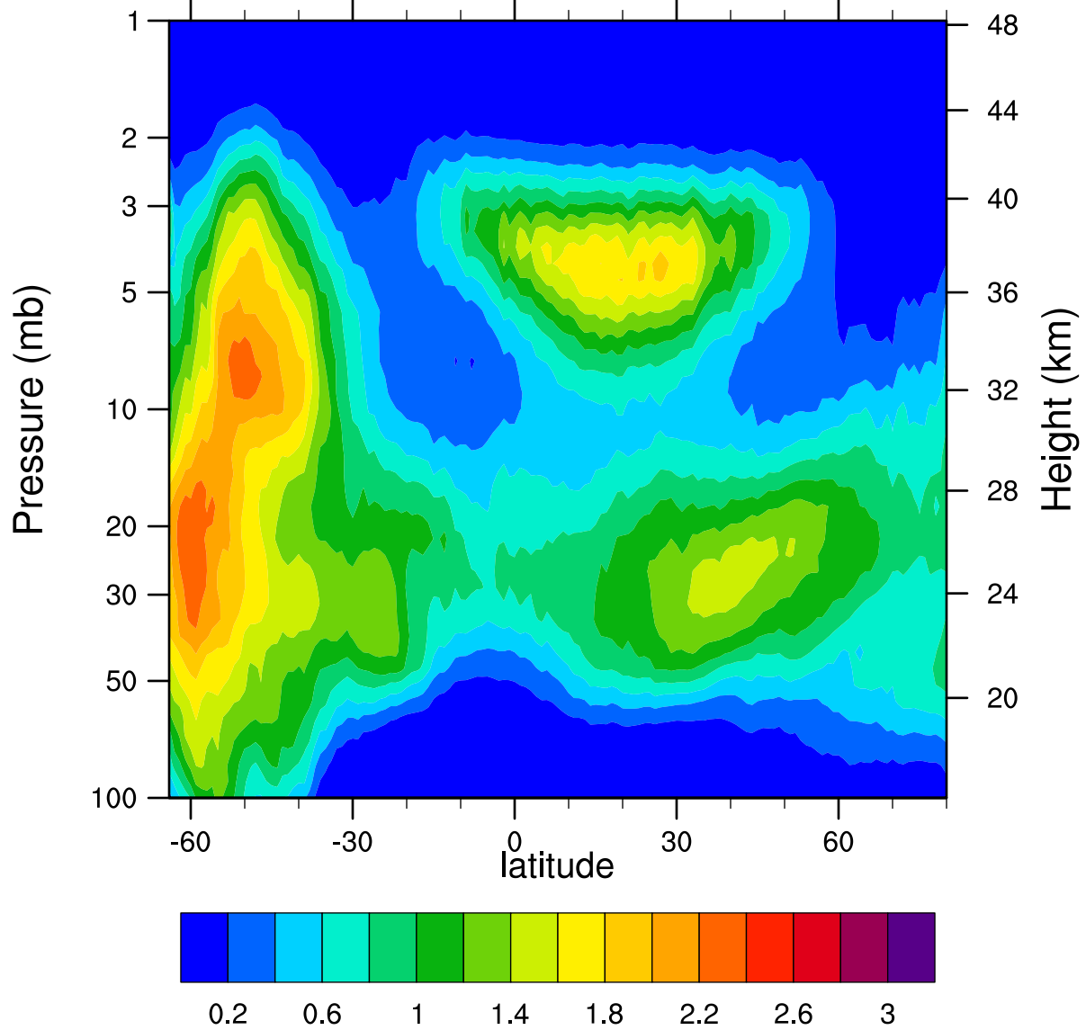
HIRDLSv6 2007d219 ClONO2_Ascending (ppbv)
