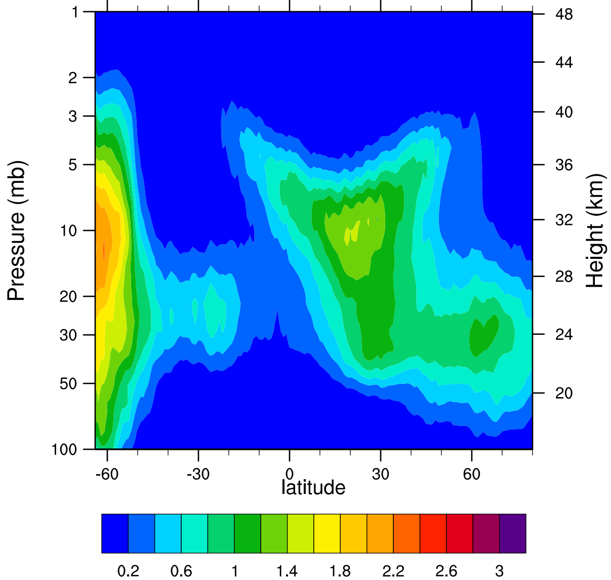
HIRDLSv6 2005d121 ClONO2_Ascending (ppbv)
