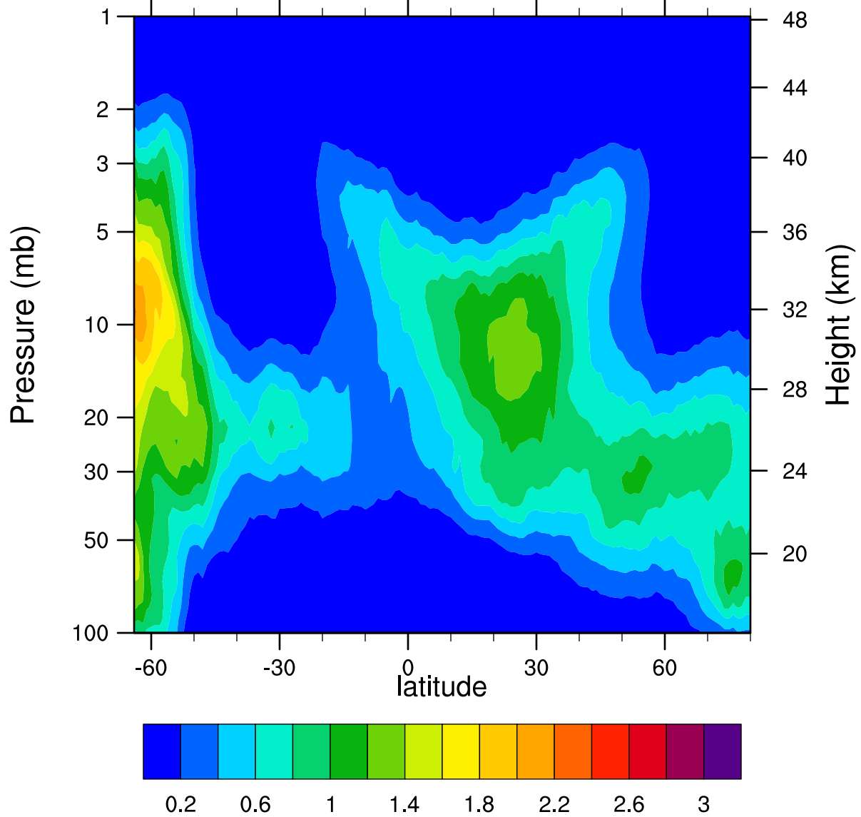
HIRDLSv6 2005d097 ClONO2_Ascending (ppbv)
