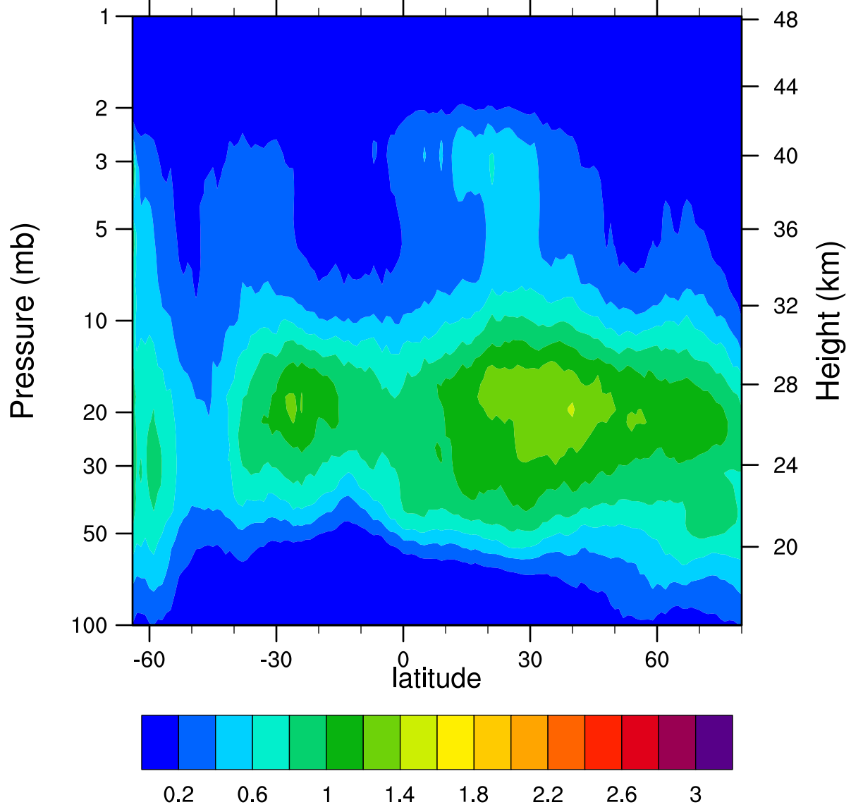
HIRDLSv6 2006d154 ClONO2_Ascending (ppbv)
