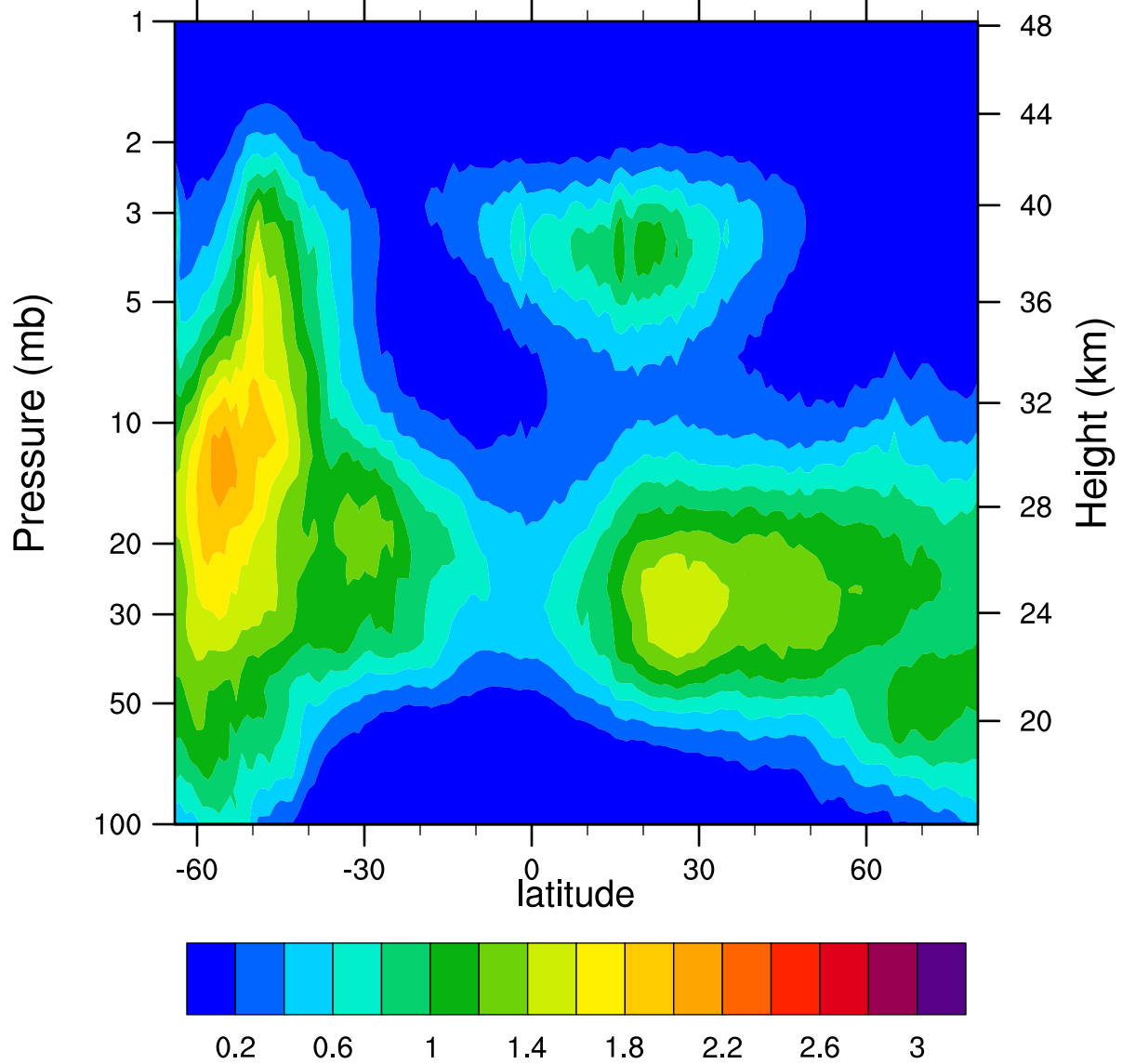
HIRDLSv6 2007d130 ClONO2_Ascending (ppbv)
