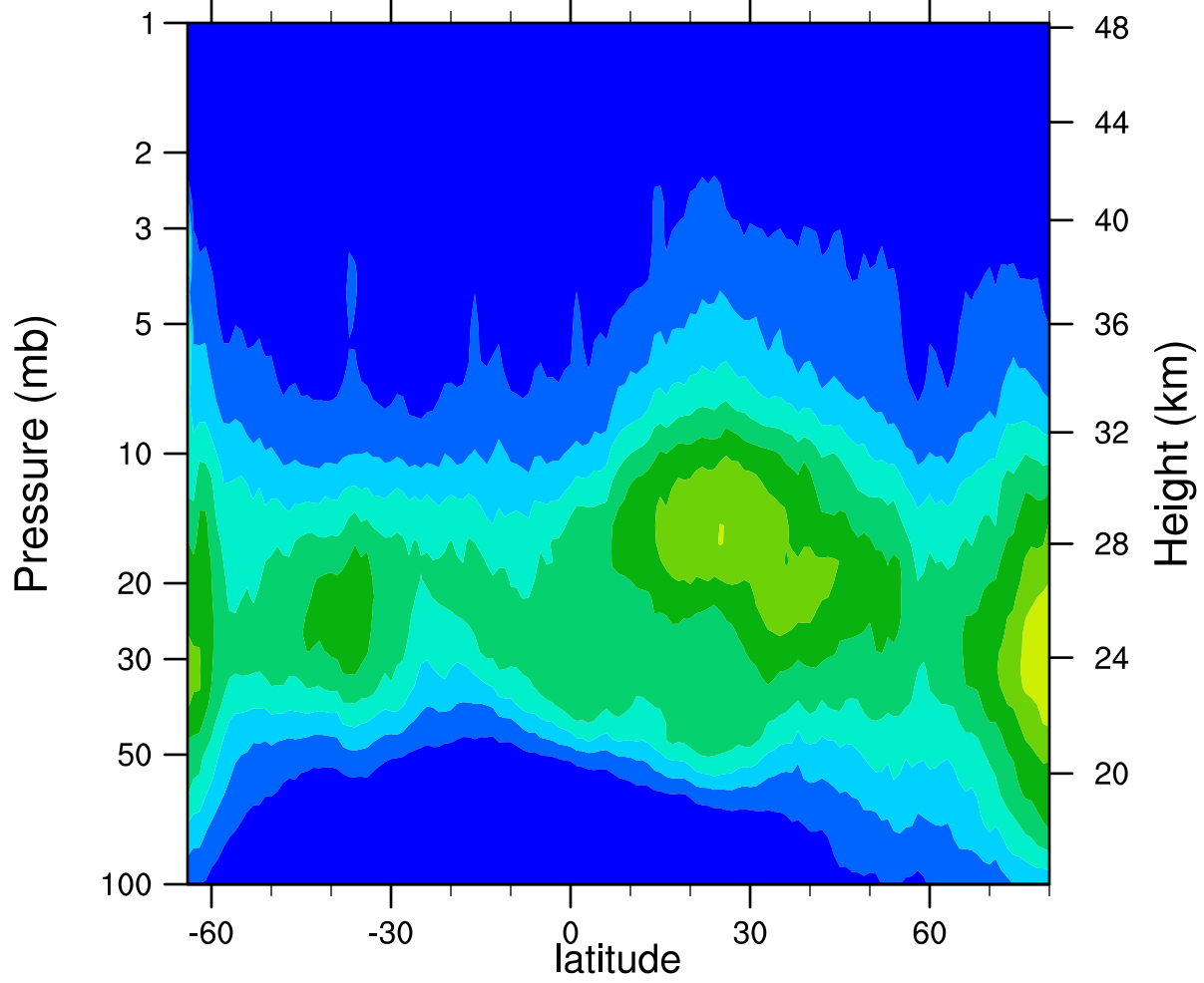
HIRDLSv6 2006d101 ClONO2_Ascending (ppbv)
