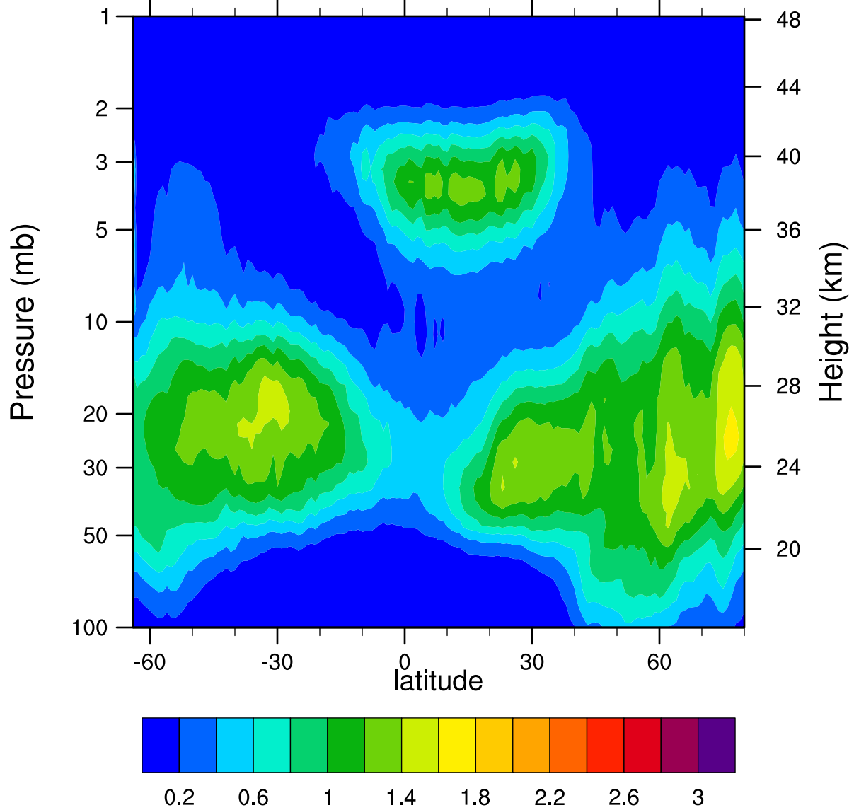
HIRDLSv6 2007d021 ClONO2_Ascending (ppbv)
