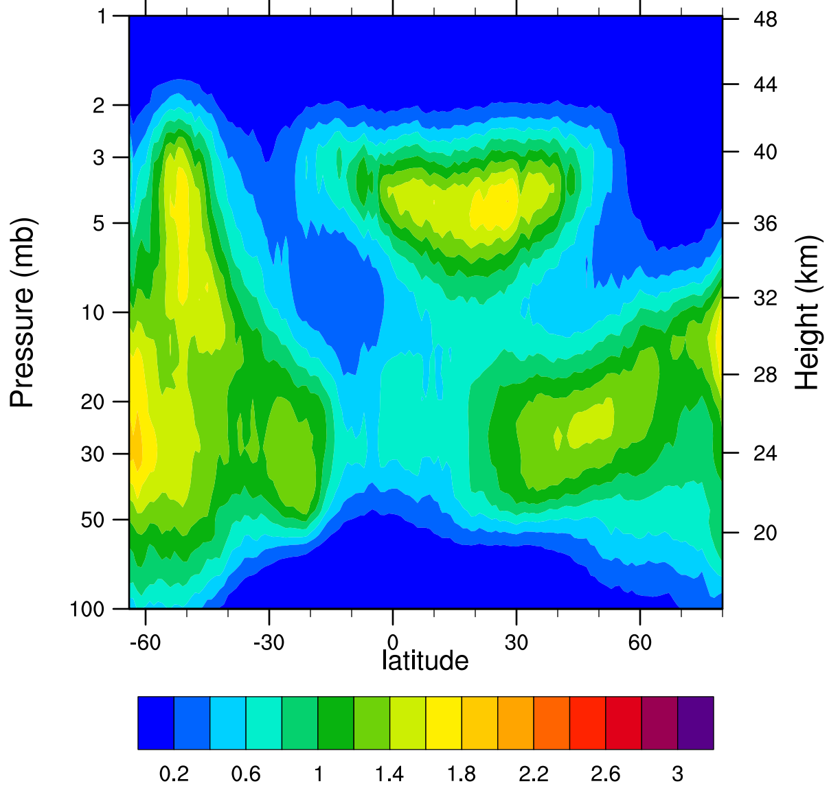
HIRDLSv6 2007d267 ClONO2_Ascending (ppbv)
