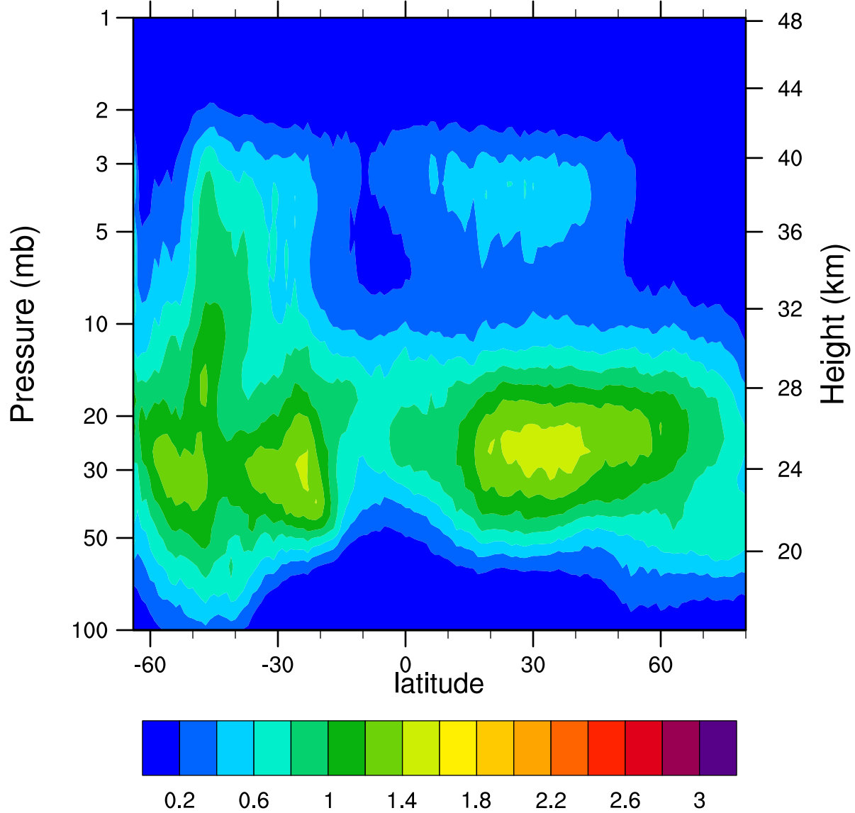
HIRDLSv6 2007d193 ClONO2_Ascending (ppbv)
