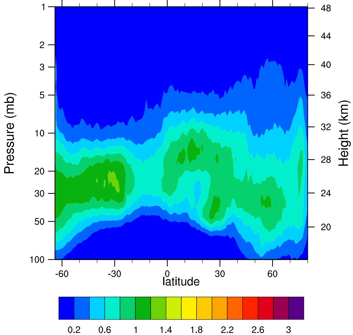
HIRDLSv6 2005d363 ClONO2_Ascending (ppbv)
