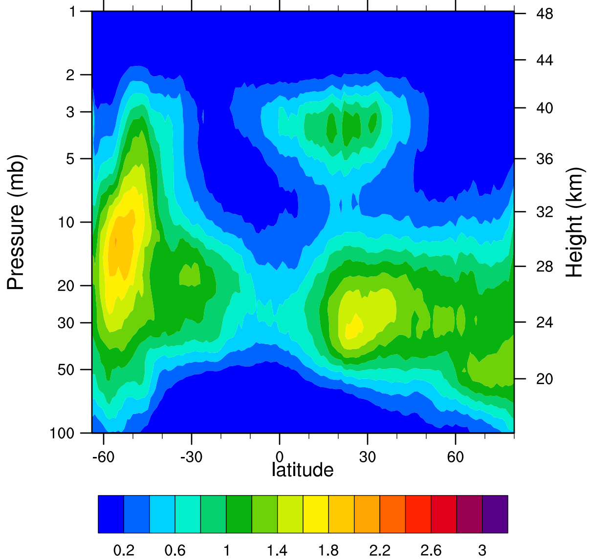
HIRDLSv6 2007d120 ClONO2_Ascending (ppbv)
