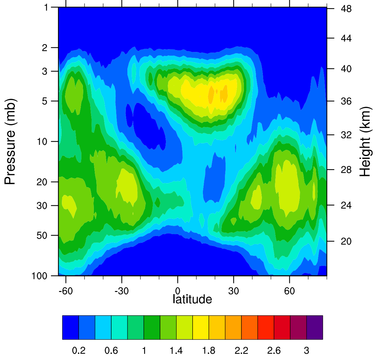
HIRDLSv6 2007d345 ClONO2_Ascending (ppbv)
