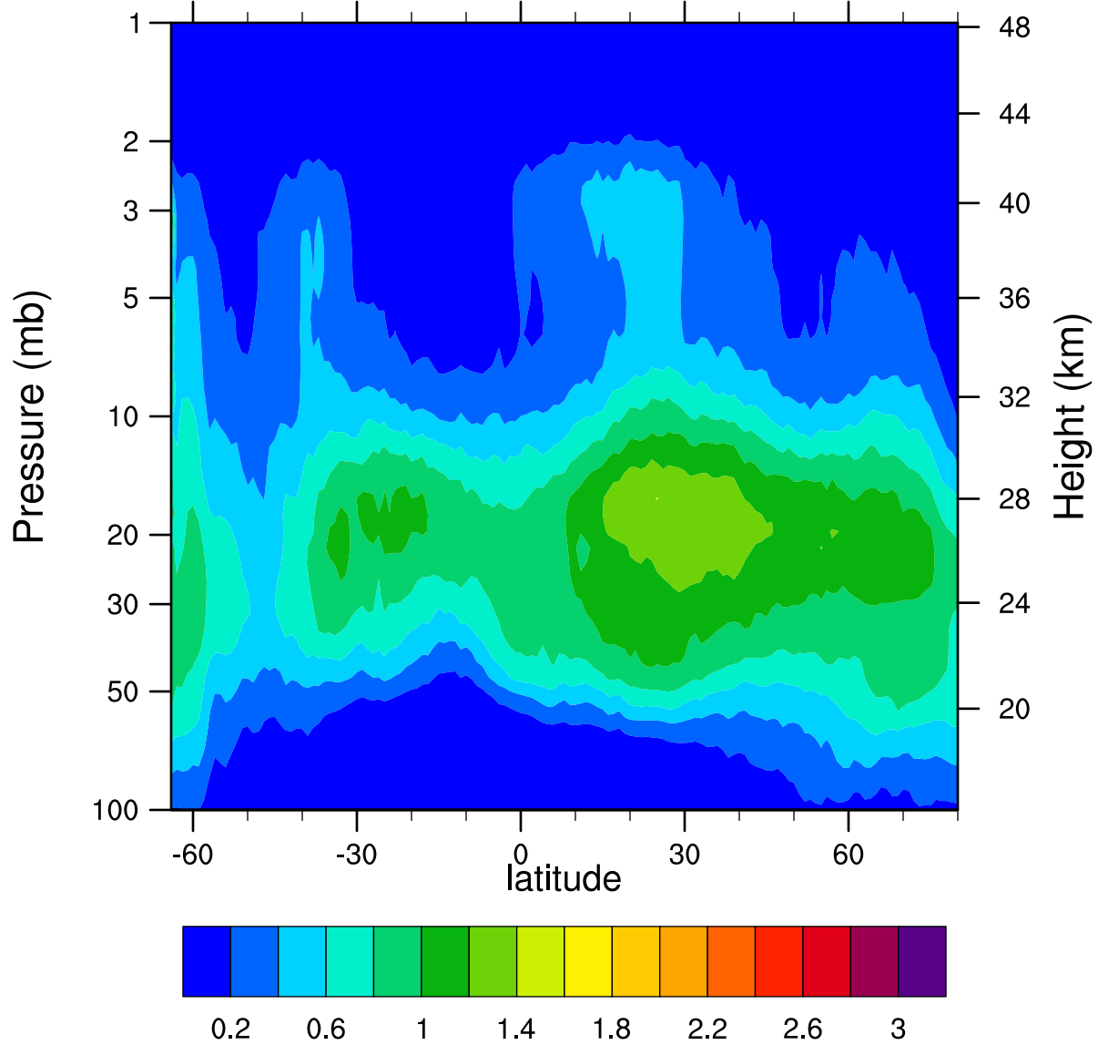
HIRDLSv6 2006d145 ClONO2_Ascending (ppbv)
