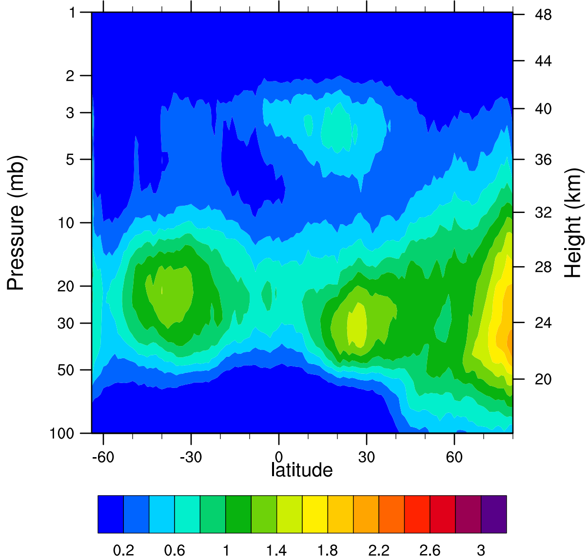
HIRDLSv6 2007d065 ClONO2_Ascending (ppbv)
