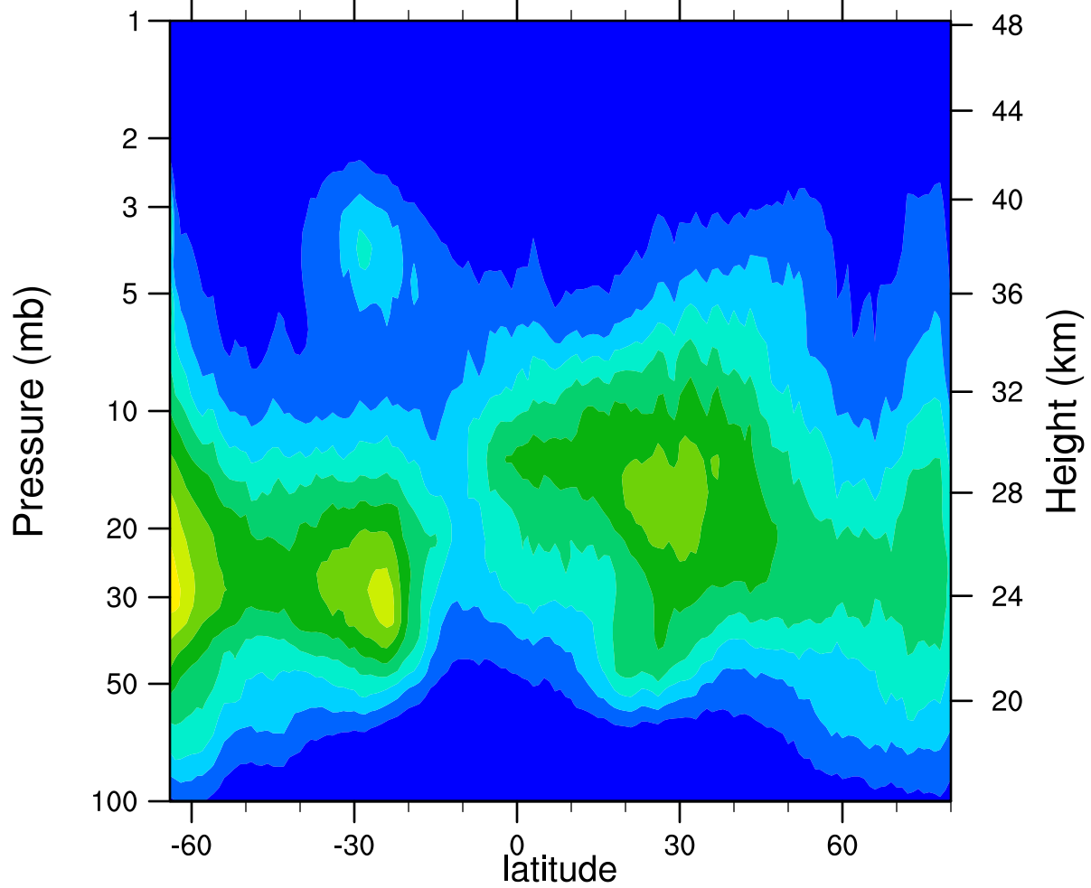
HIRDLSv6 2005d295 ClONO2_Ascending (ppbv)
