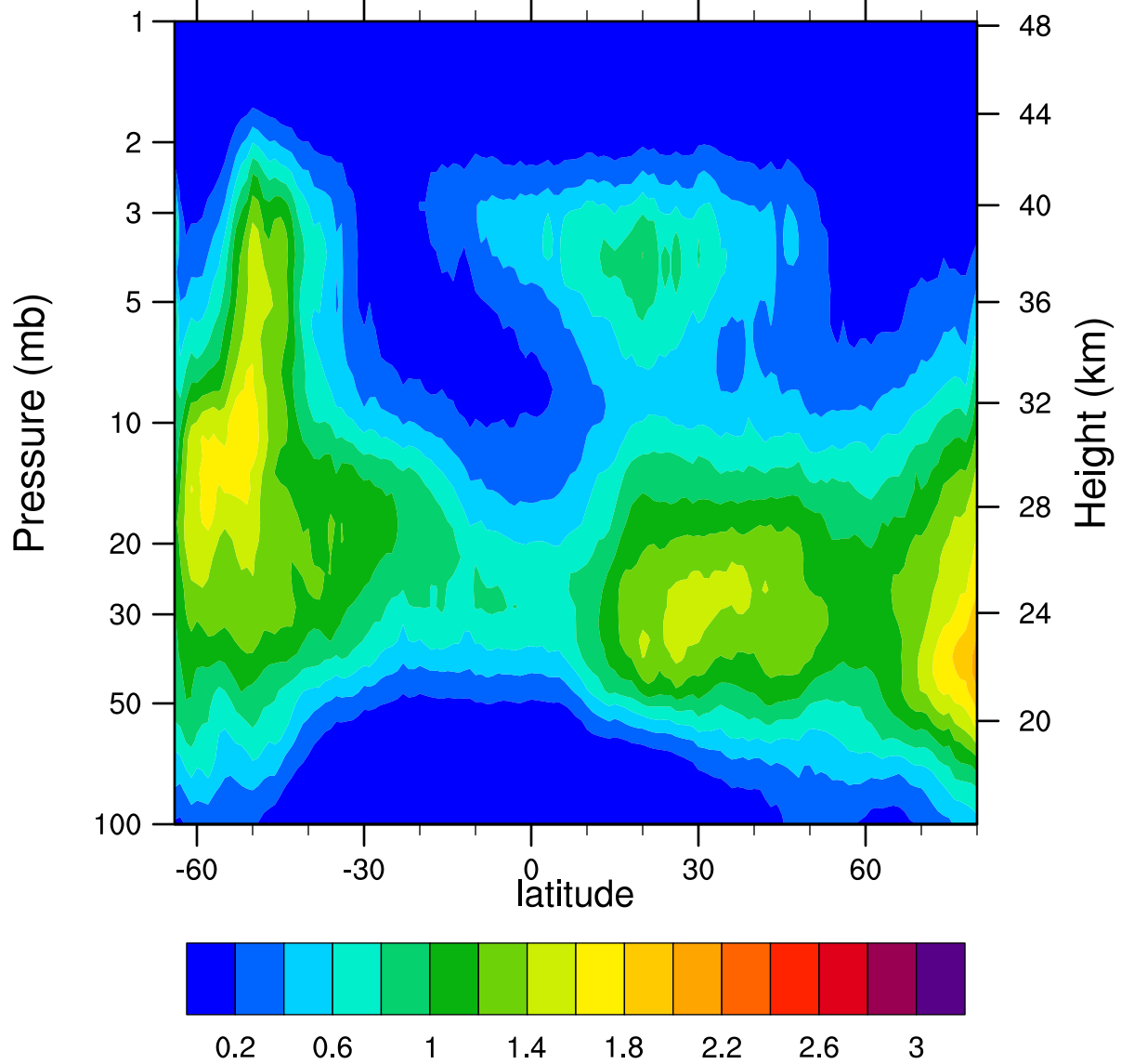
HIRDLSv6 2007d098 ClONO2_Ascending (ppbv)
