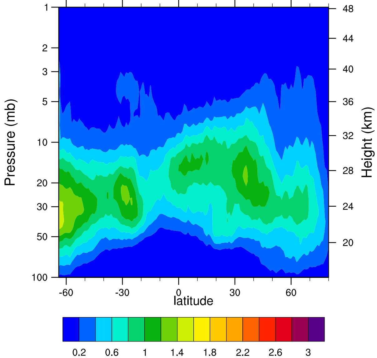
HIRDLSv6 2005d322 ClONO2_Ascending (ppbv)
