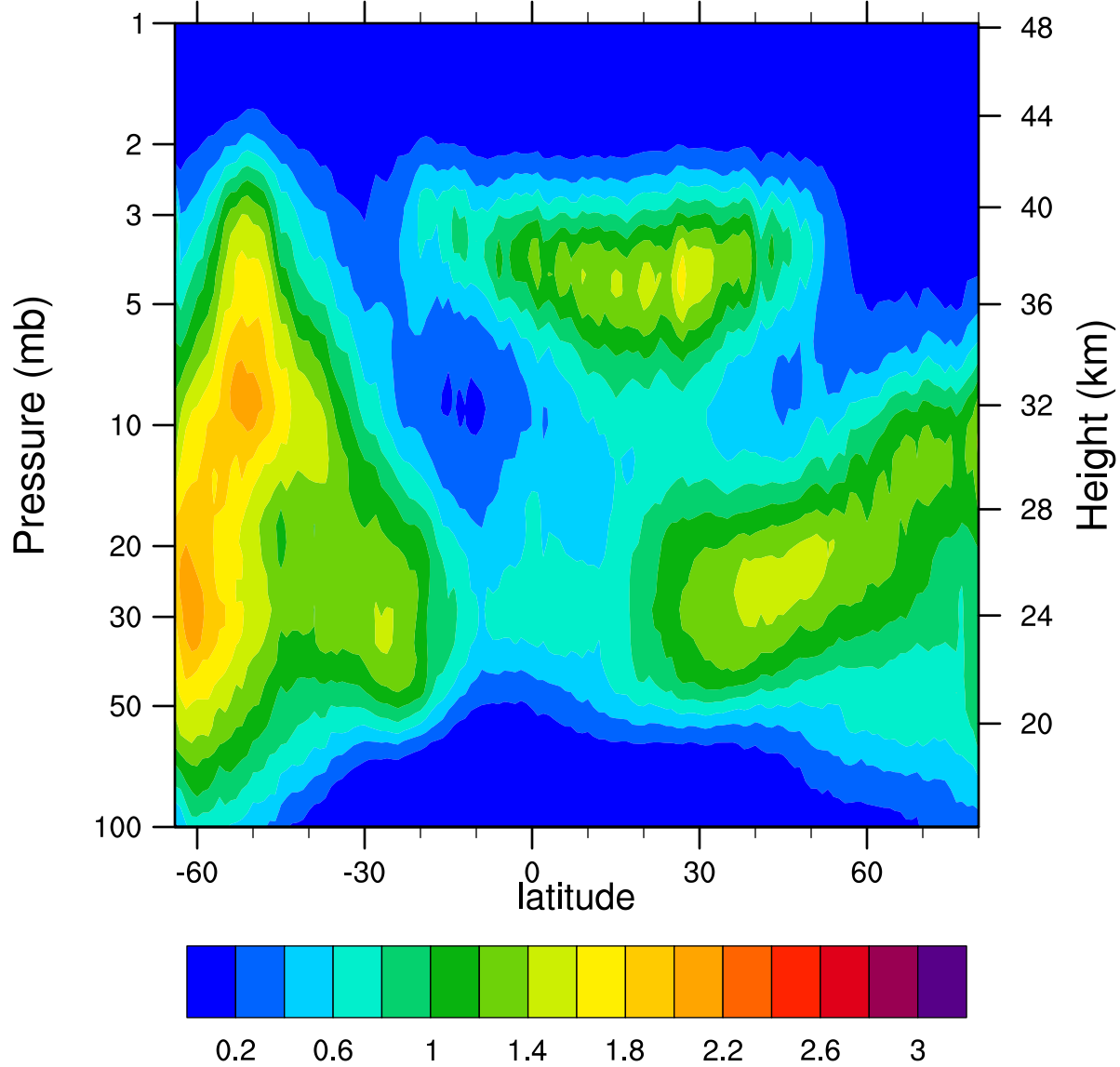
HIRDLSv6 2007d254 ClONO2_Ascending (ppbv)
