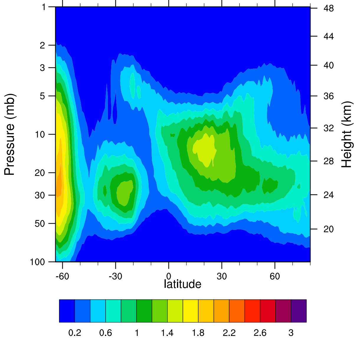
HIRDLSv6 2005d234 ClONO2_Ascending (ppbv)
