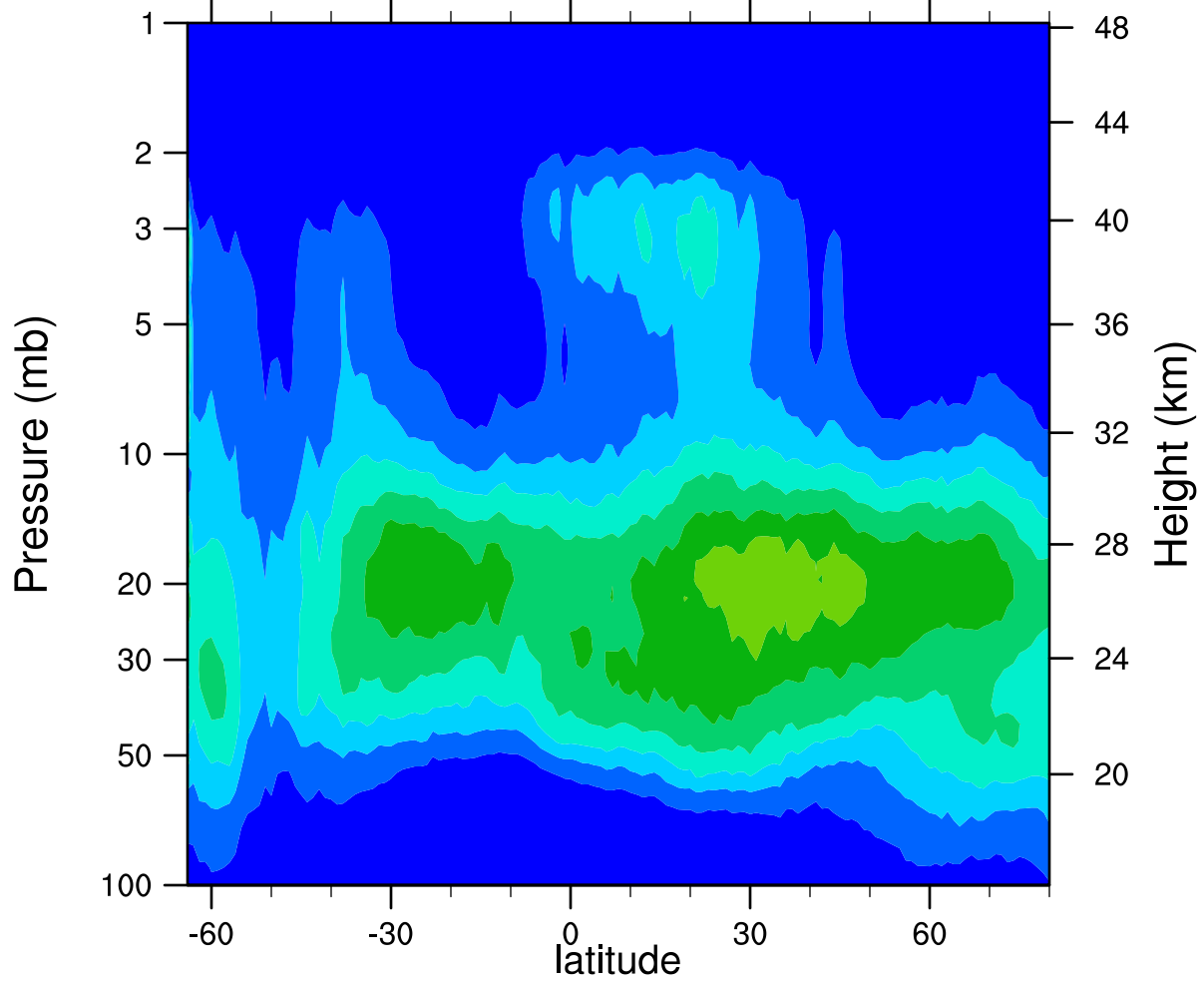
HIRDLSv6 2006d172 ClONO2_Ascending (ppbv)
