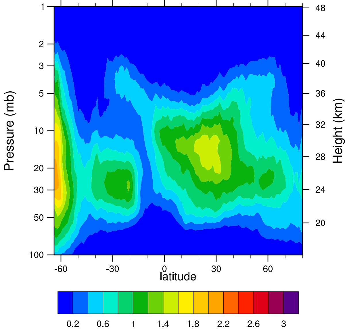
HIRDLSv6 2005d257 ClONO2_Ascending (ppbv)
