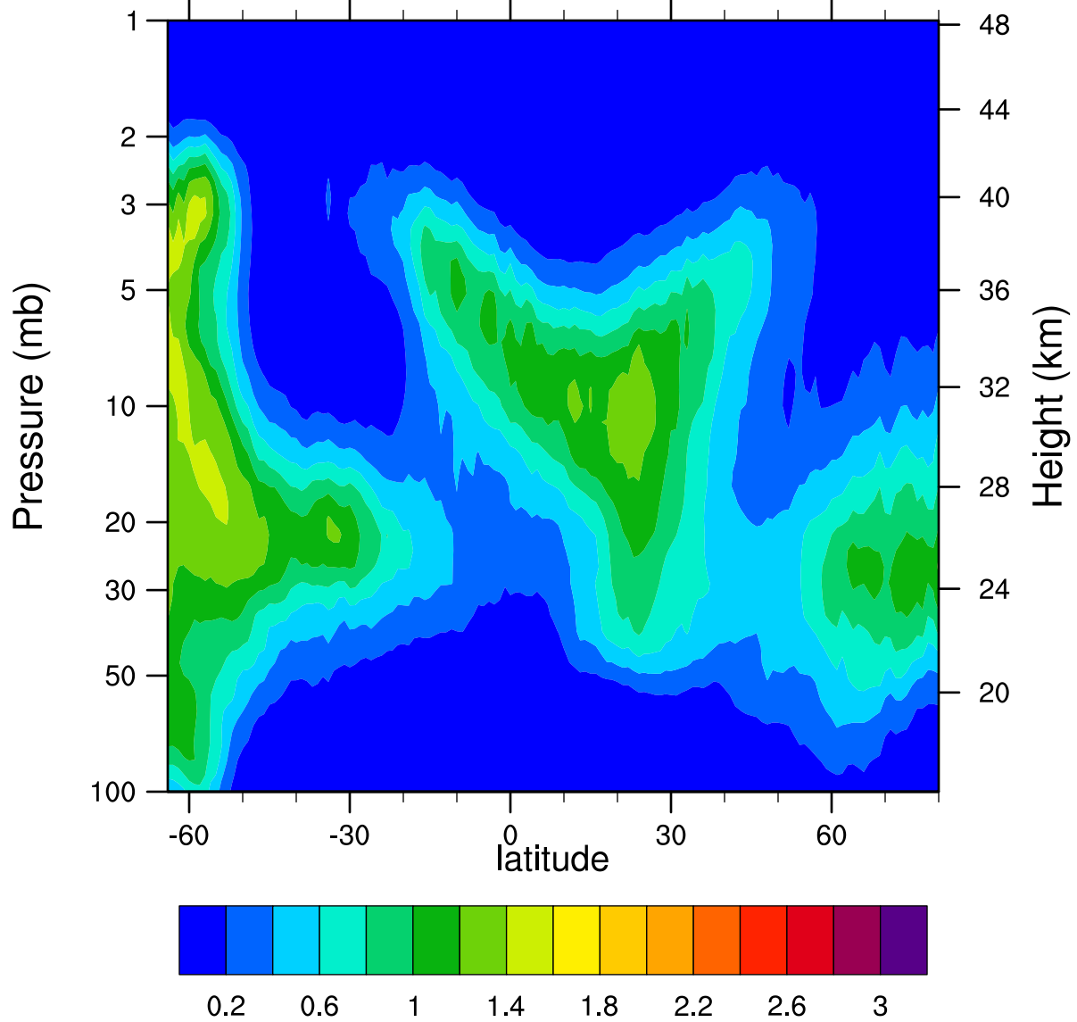
HIRDLSv6 2005d042 ClONO2_Ascending (ppbv)
