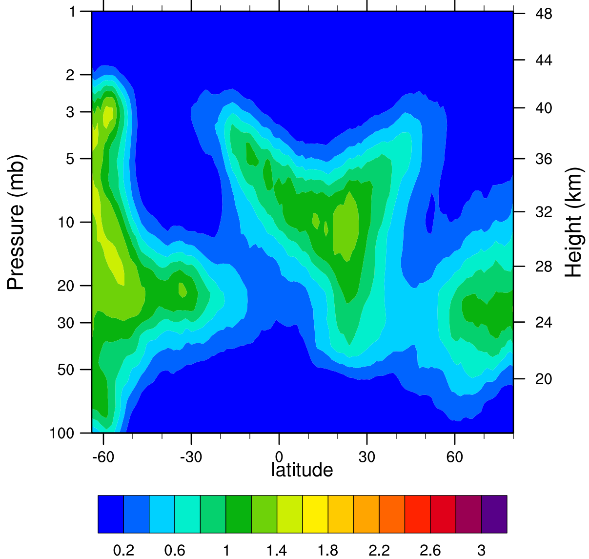
HIRDLSv6 2005d041 ClONO2_Ascending (ppbv)
