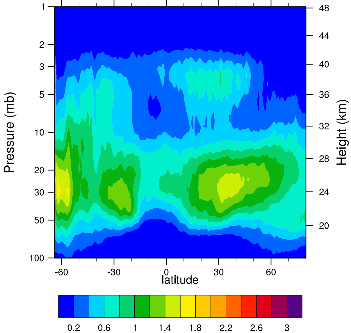
HIRDLSv6 2007d208 ClONO2_Ascending (ppbv)
