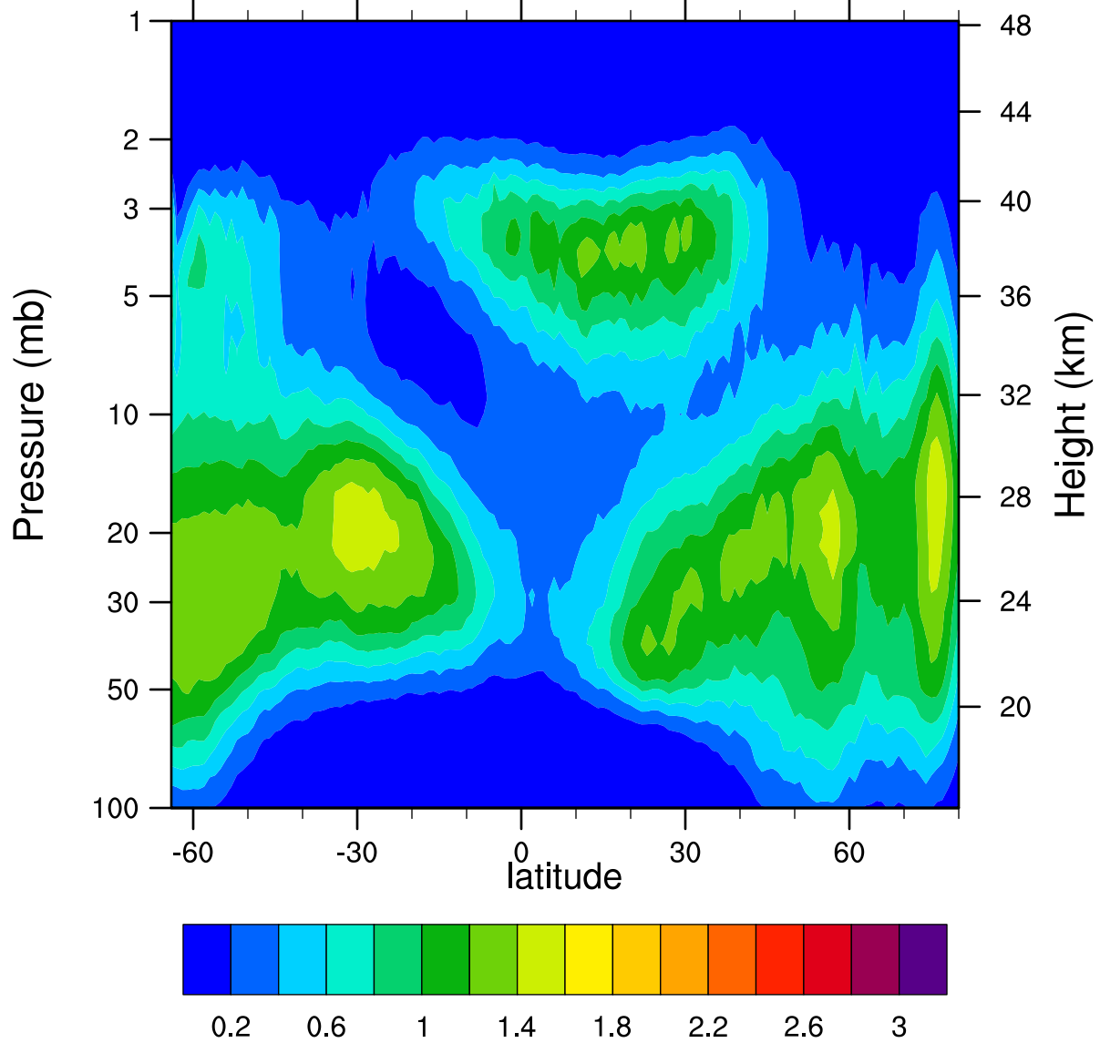
HIRDLSv6 2006d355 ClONO2_Ascending (ppbv)
