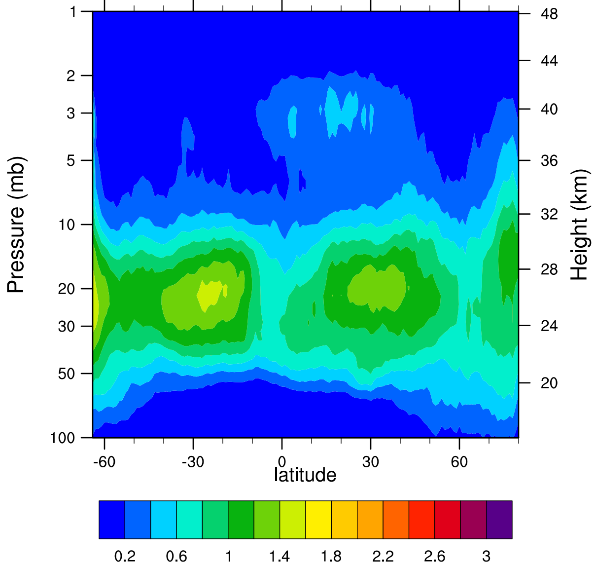
HIRDLSv6 2006d293 ClONO2_Ascending (ppbv)
