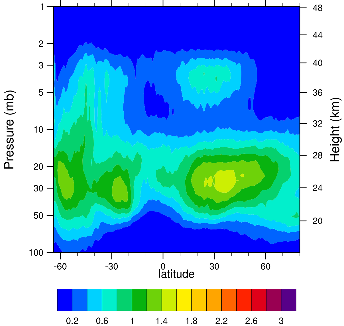
HIRDLSv6 2007d198 ClONO2_Ascending (ppbv)
