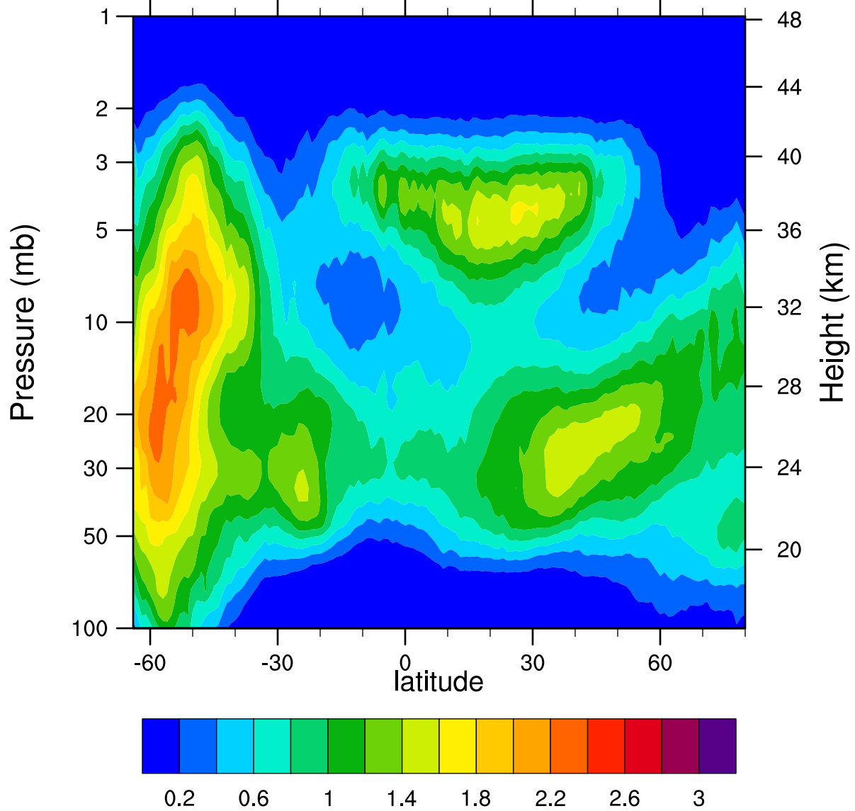
HIRDLSv6 2007d231 ClONO2_Ascending (ppbv)
