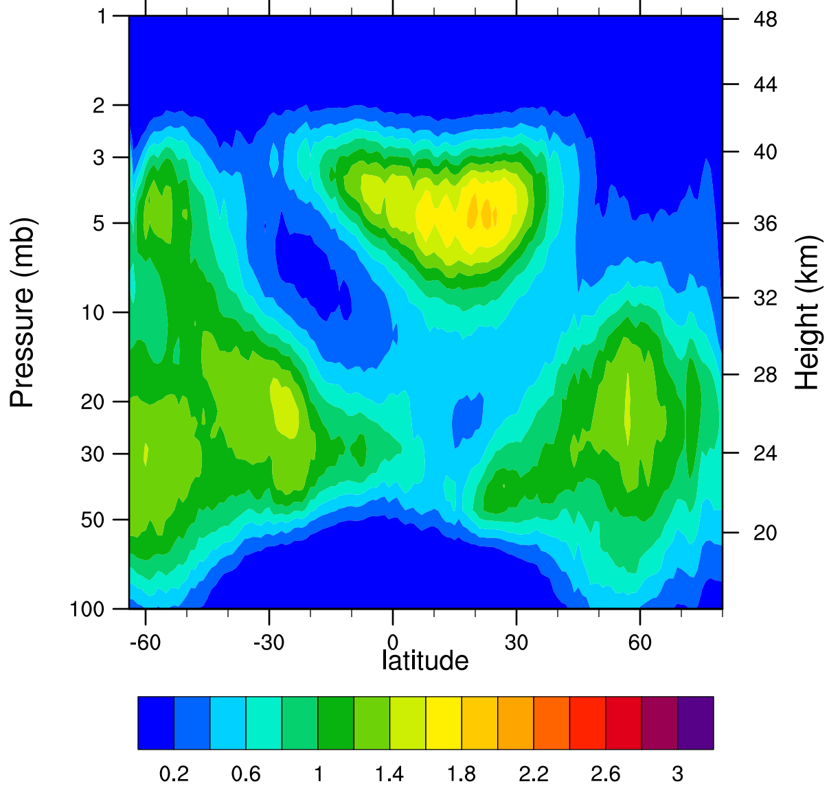
HIRDLSv6 2007d353 ClONO2_Ascending (ppbv)
