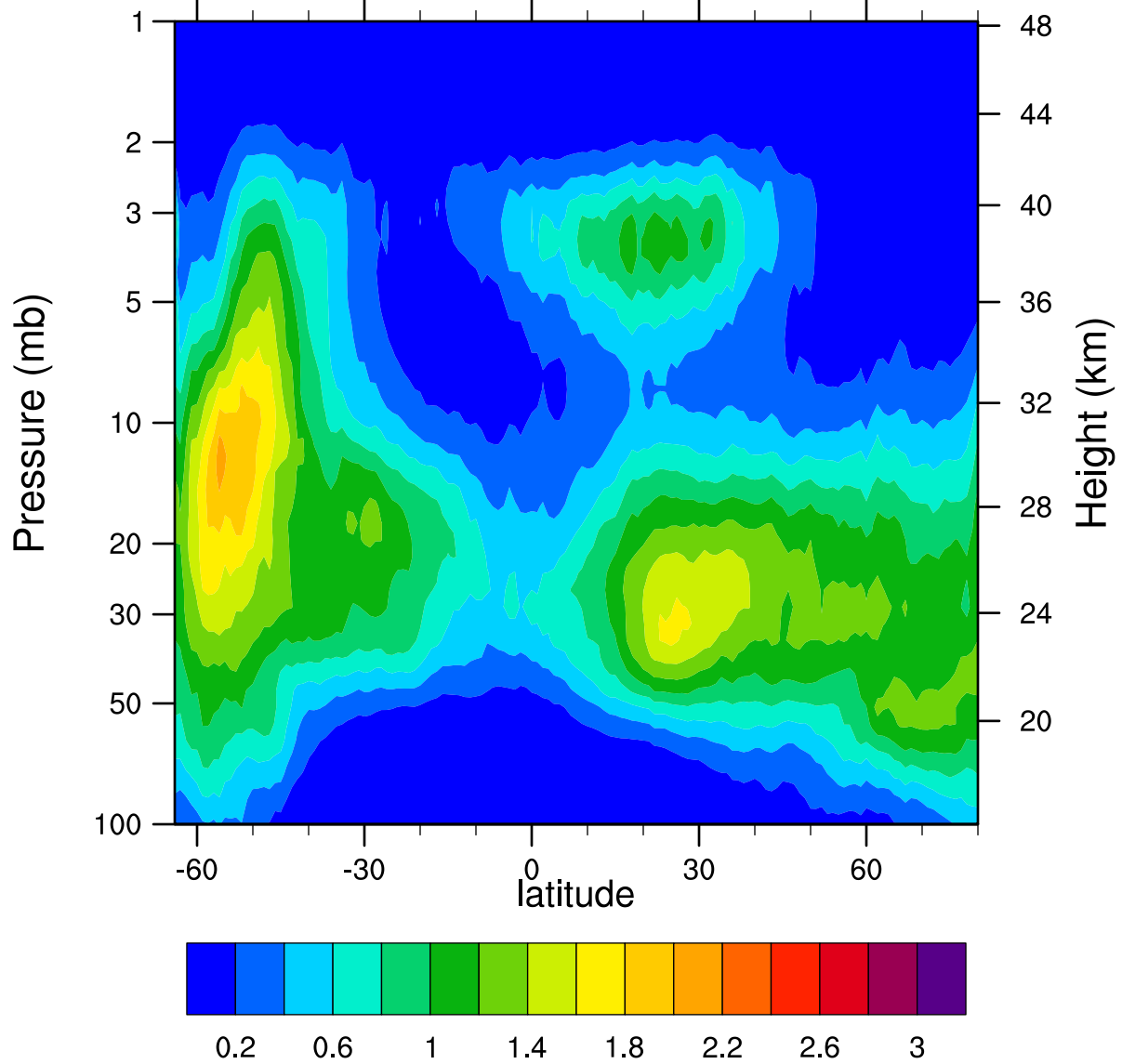
HIRDLSv6 2007d121 ClONO2_Ascending (ppbv)
