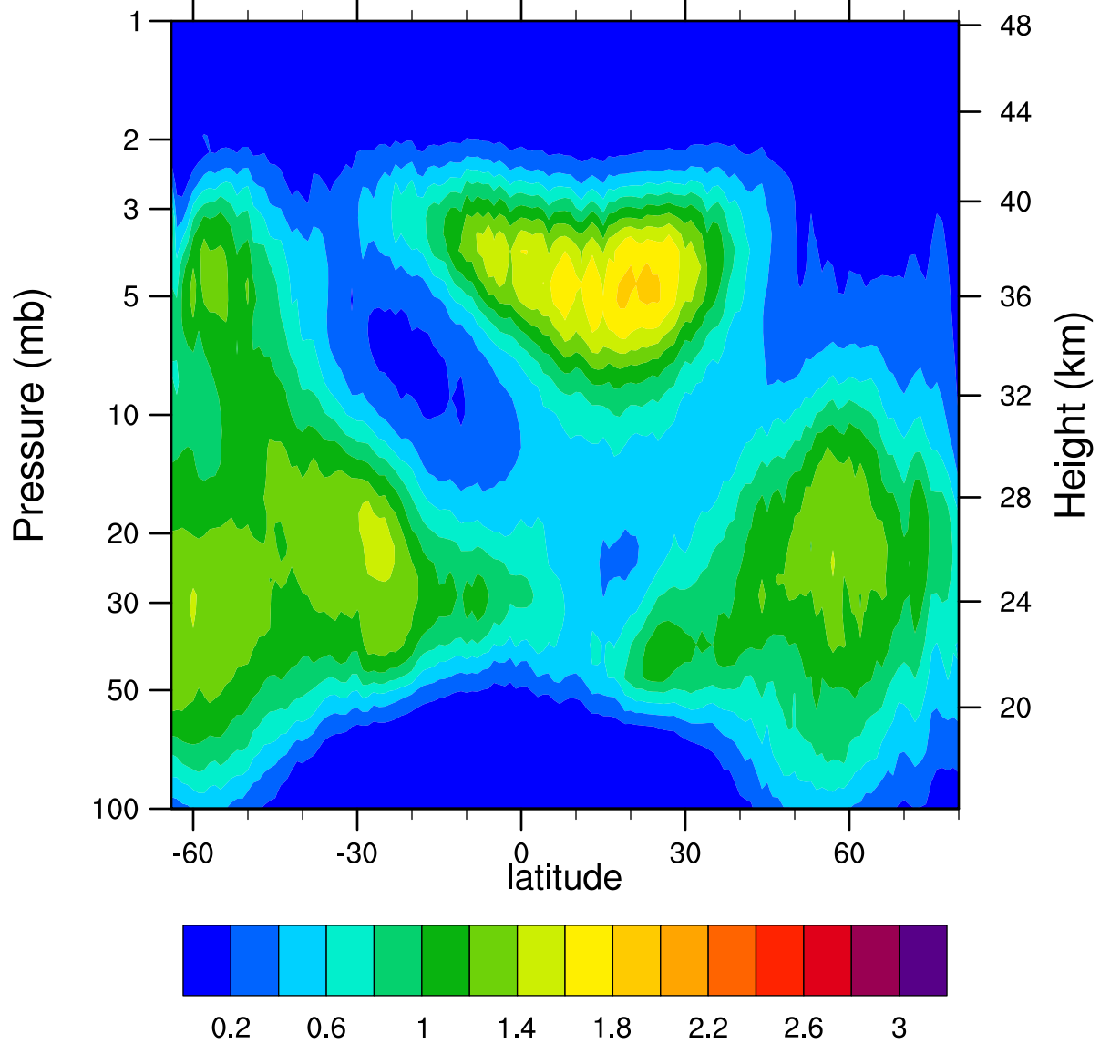
HIRDLSv6 2007d354 ClONO2_Ascending (ppbv)
