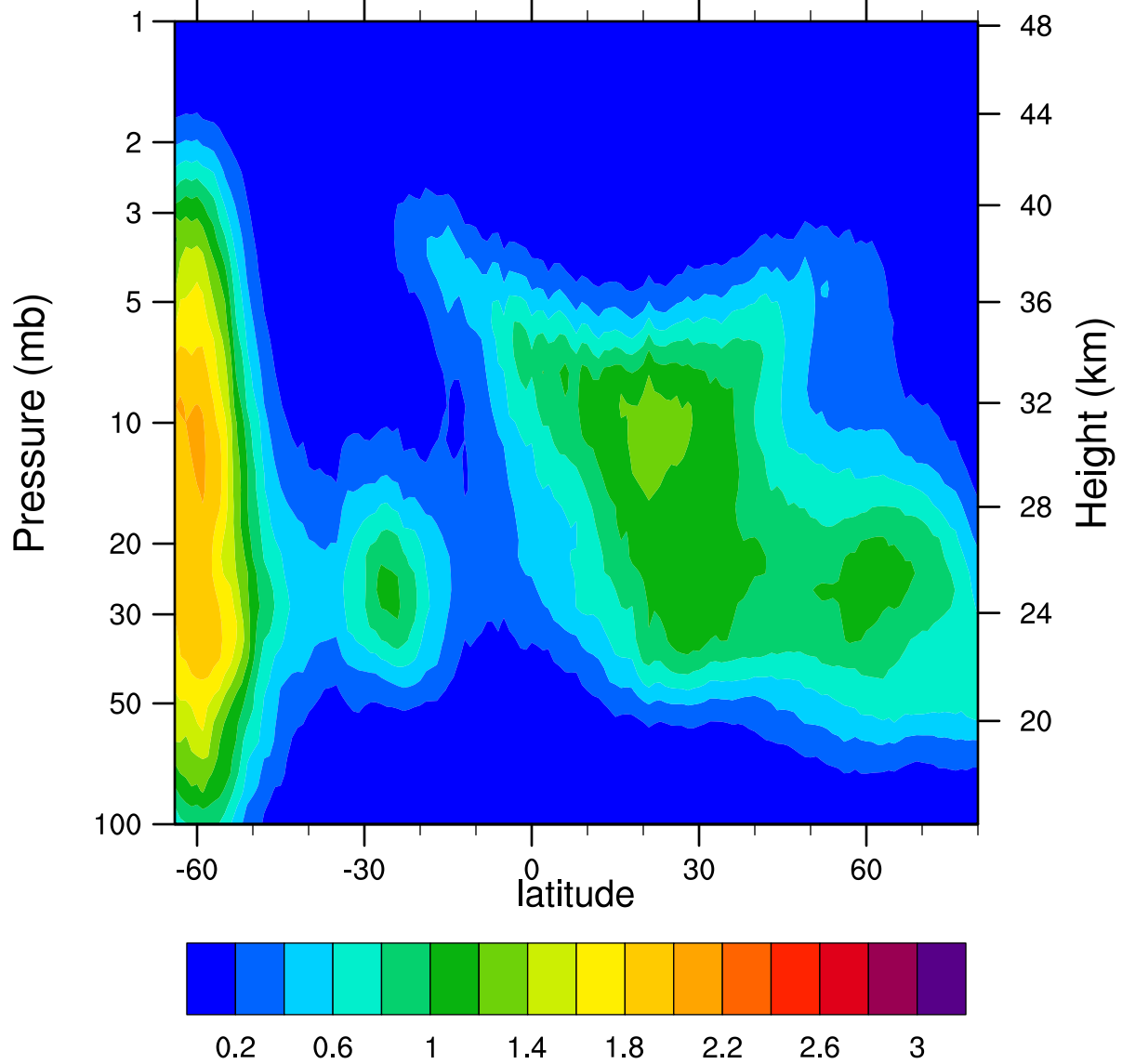
HIRDLSv6 2005d158 ClONO2_Ascending (ppbv)
