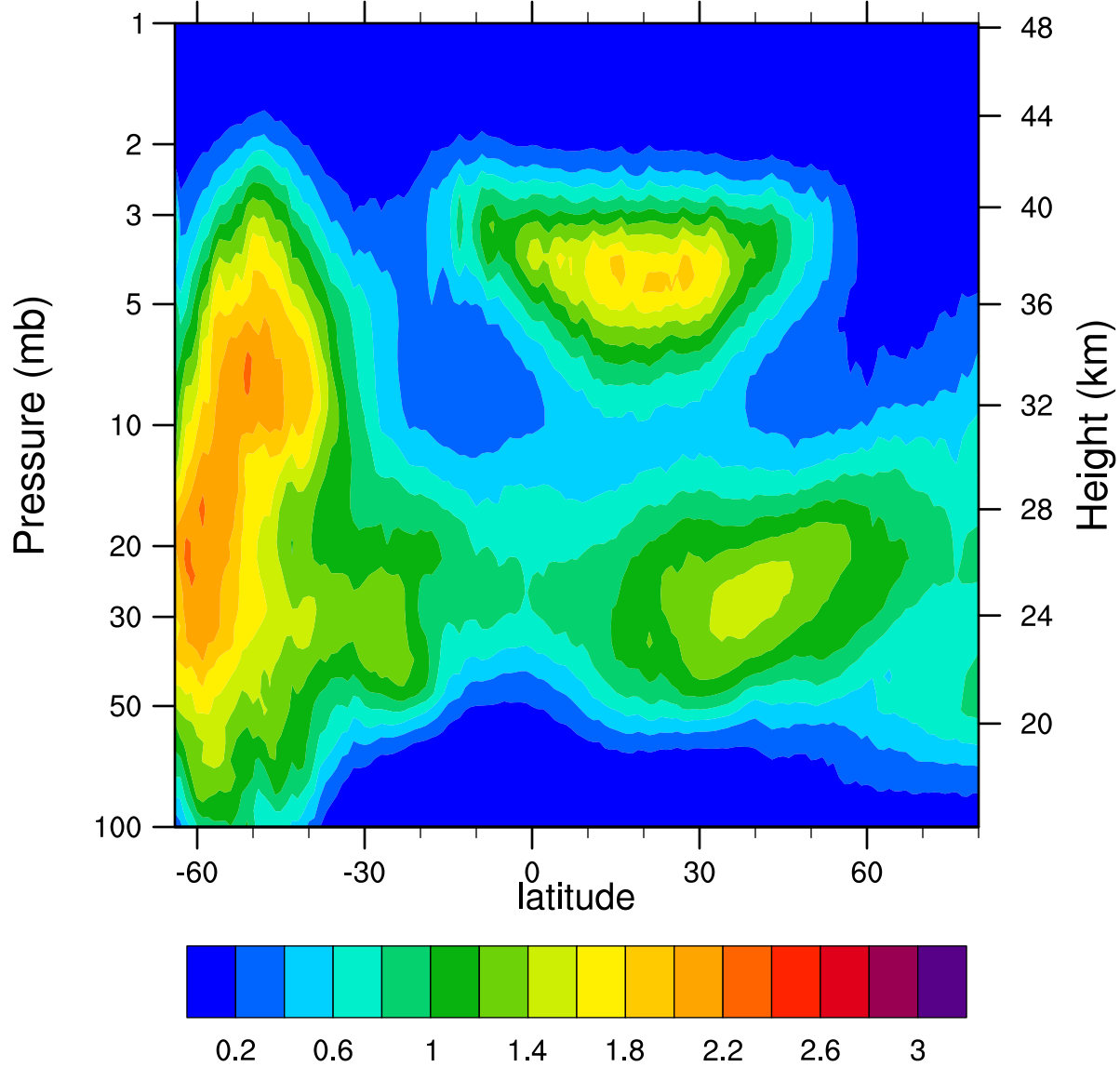
HIRDLSv6 2007d216 ClONO2_Ascending (ppbv)
