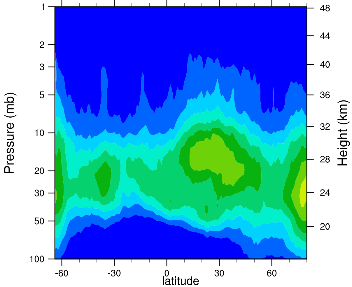
HIRDLSv6 2006d106 ClONO2_Ascending (ppbv)
