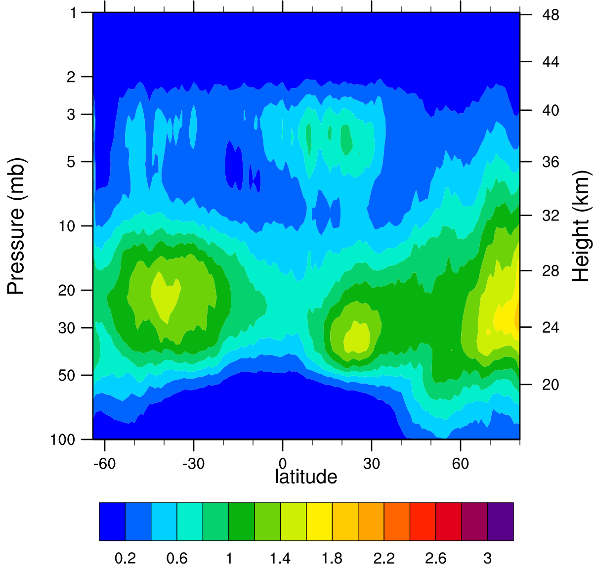
HIRDLSv6 2007d046 ClONO2_Ascending (ppbv)
