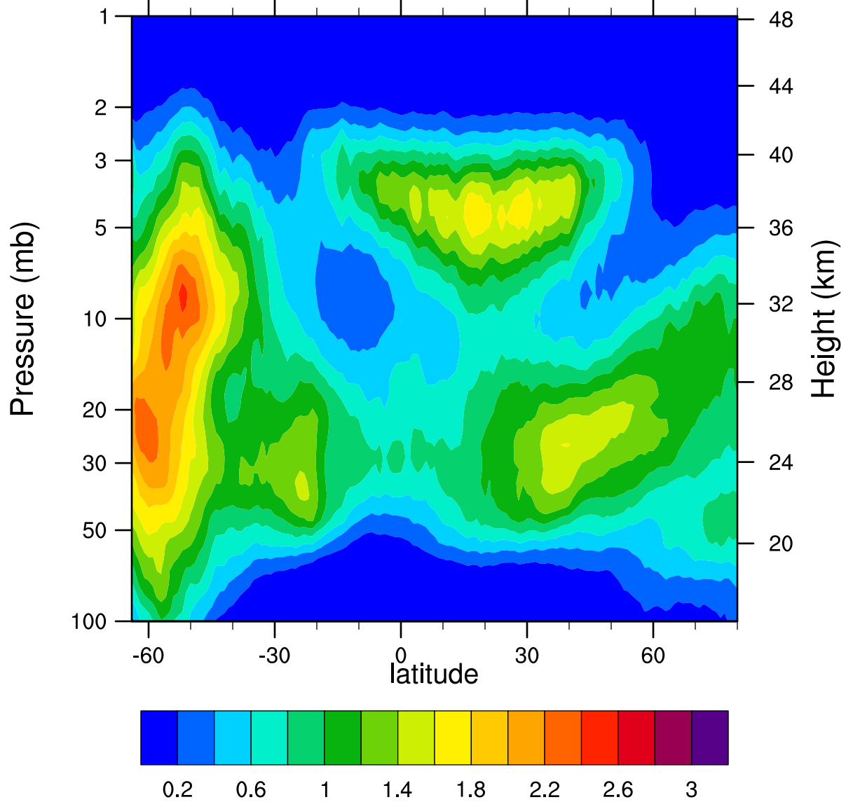
HIRDLSv6 2007d236 ClONO2_Ascending (ppbv)
