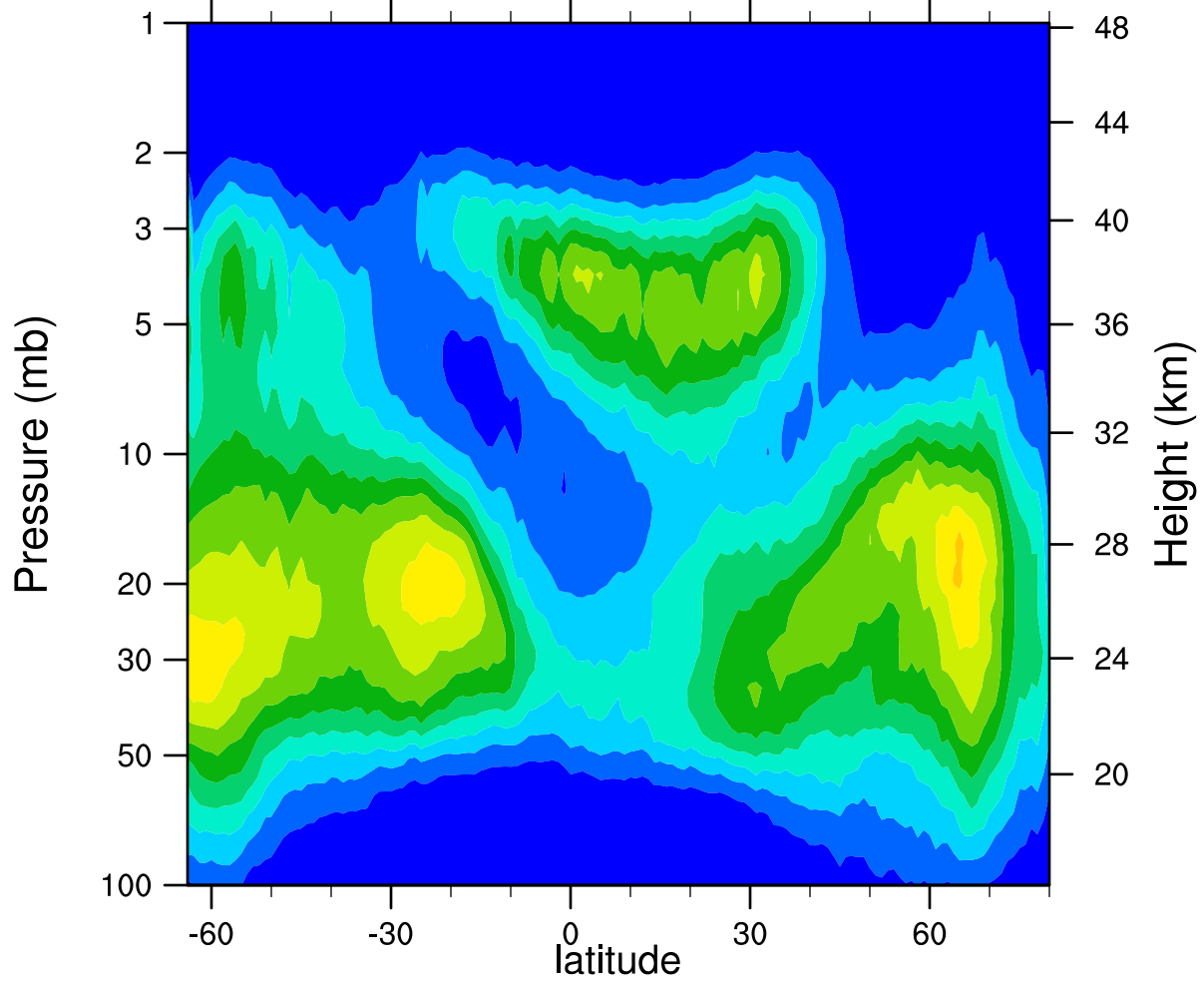
HIRDLSv6 2006d323 ClONO2_Ascending (ppbv)
