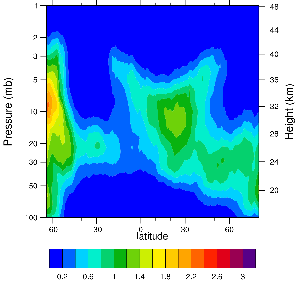
HIRDLSv6 2005d092 ClONO2_Ascending (ppbv)
