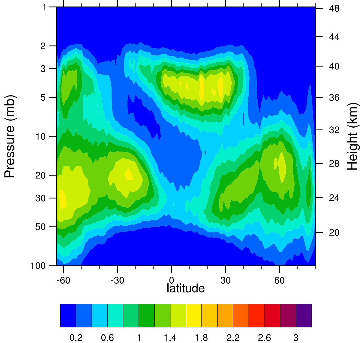
HIRDLSv6 2006d338 ClONO2_Ascending (ppbv)
