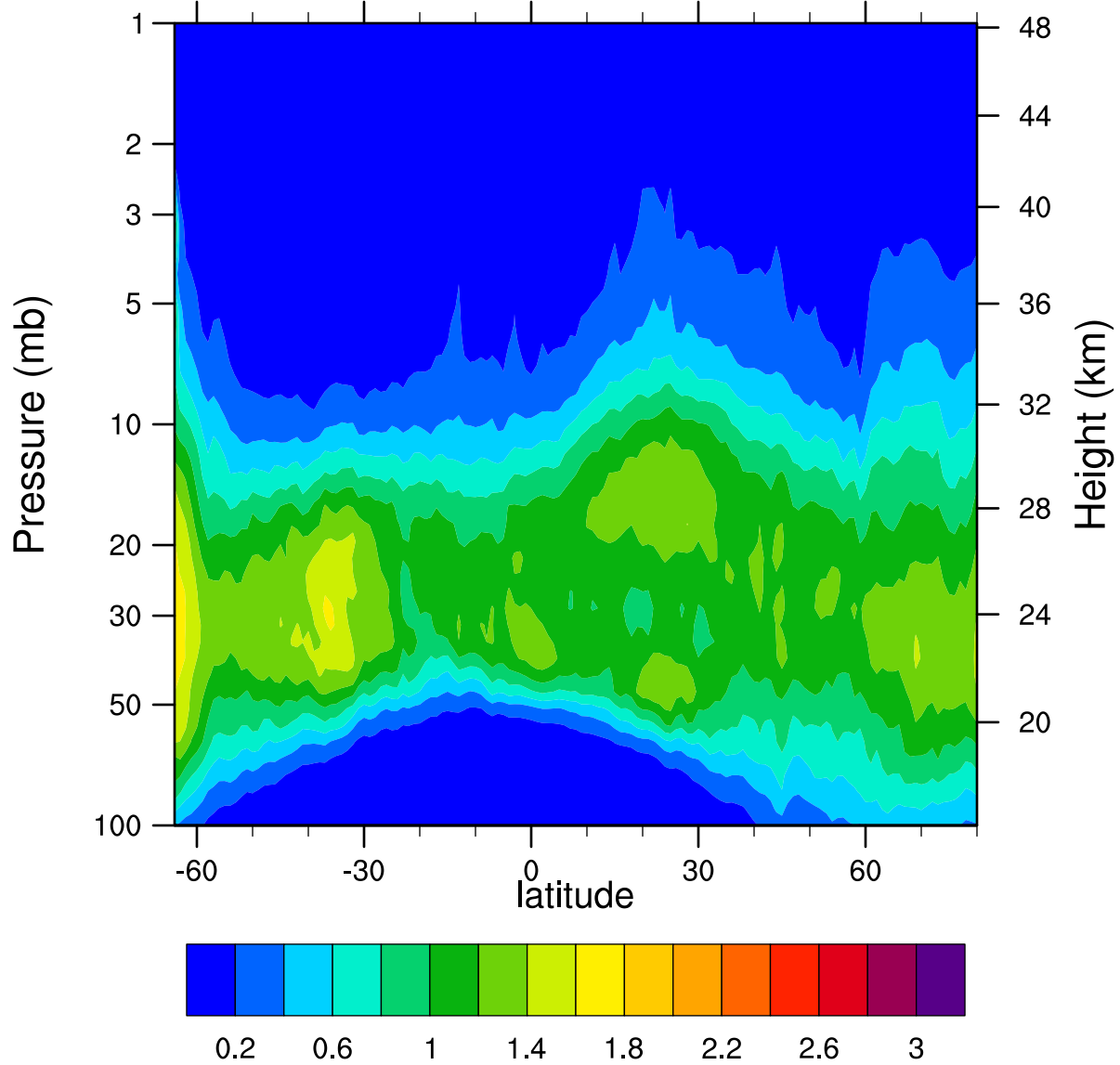
HIRDLSv6 2006d089 ClONO2_Ascending (ppbv)
