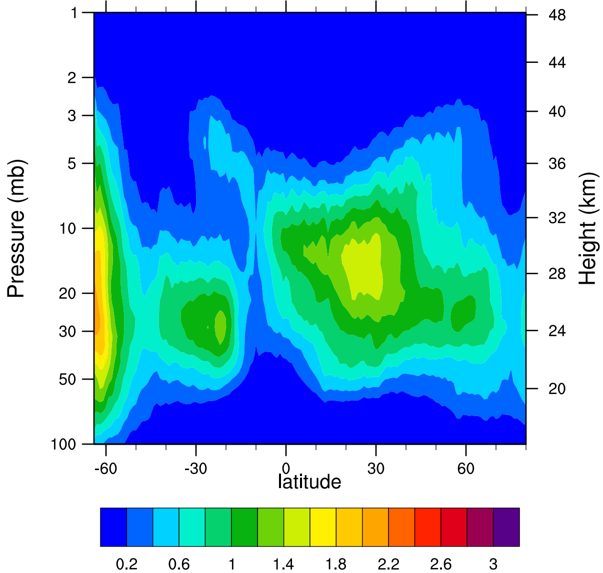
HIRDLSv6 2005d260 ClONO2_Ascending (ppbv)
