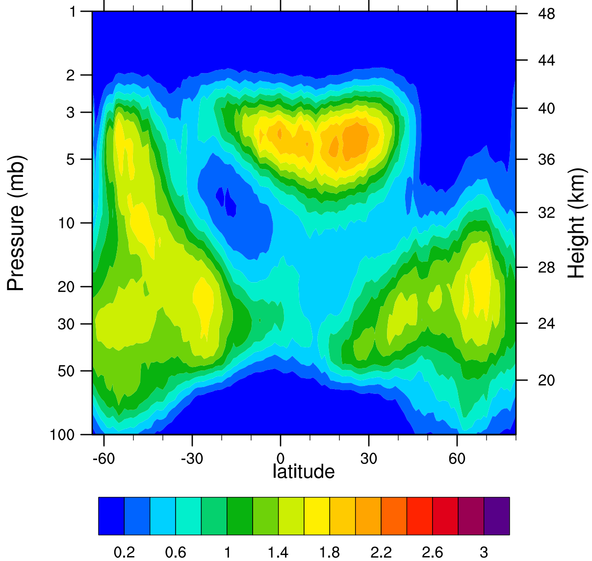
HIRDLSv6 2007d319 ClONO2_Ascending (ppbv)
