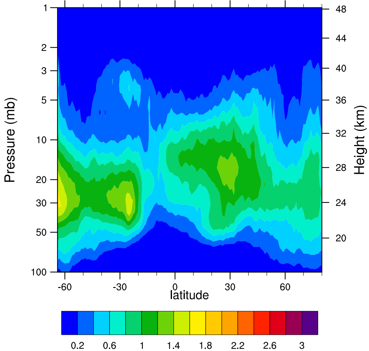
HIRDLSv6 2005d298 ClONO2_Ascending (ppbv)
