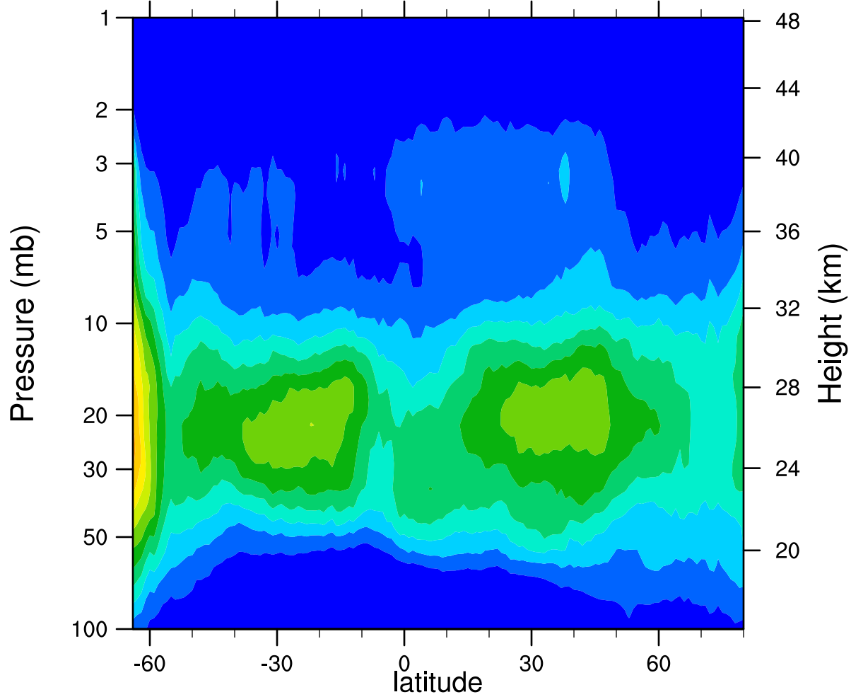
HIRDLSv6 2006d270 ClONO2_Ascending (ppbv)
