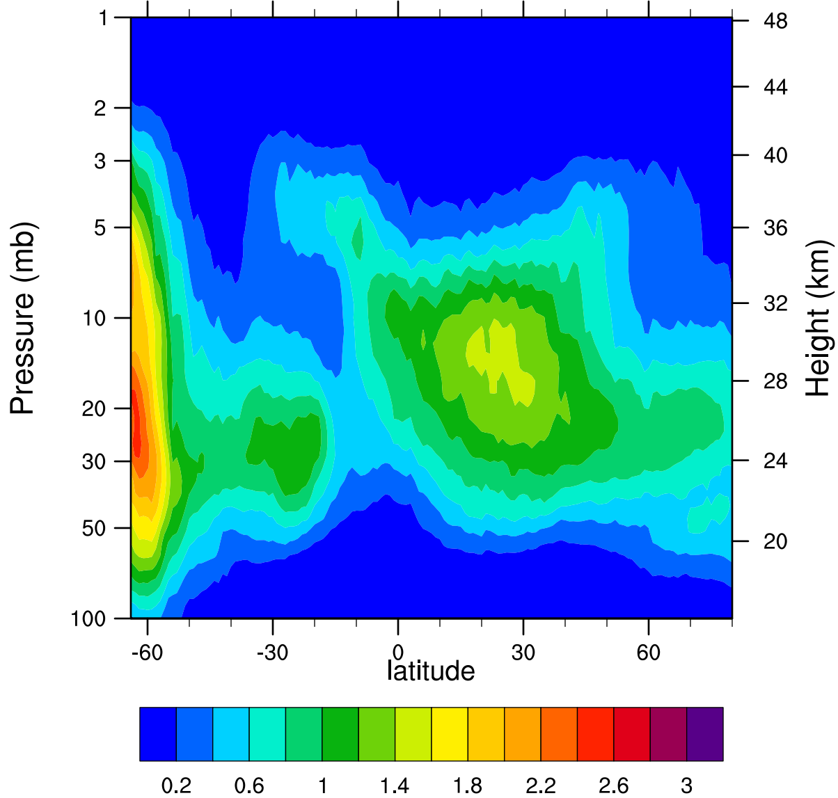
HIRDLSv6 2005d223 ClONO2_Ascending (ppbv)
