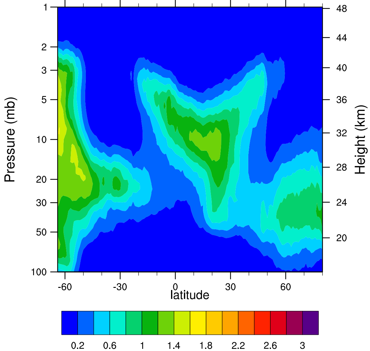
HIRDLSv6 2005d053 ClONO2_Ascending (ppbv)
