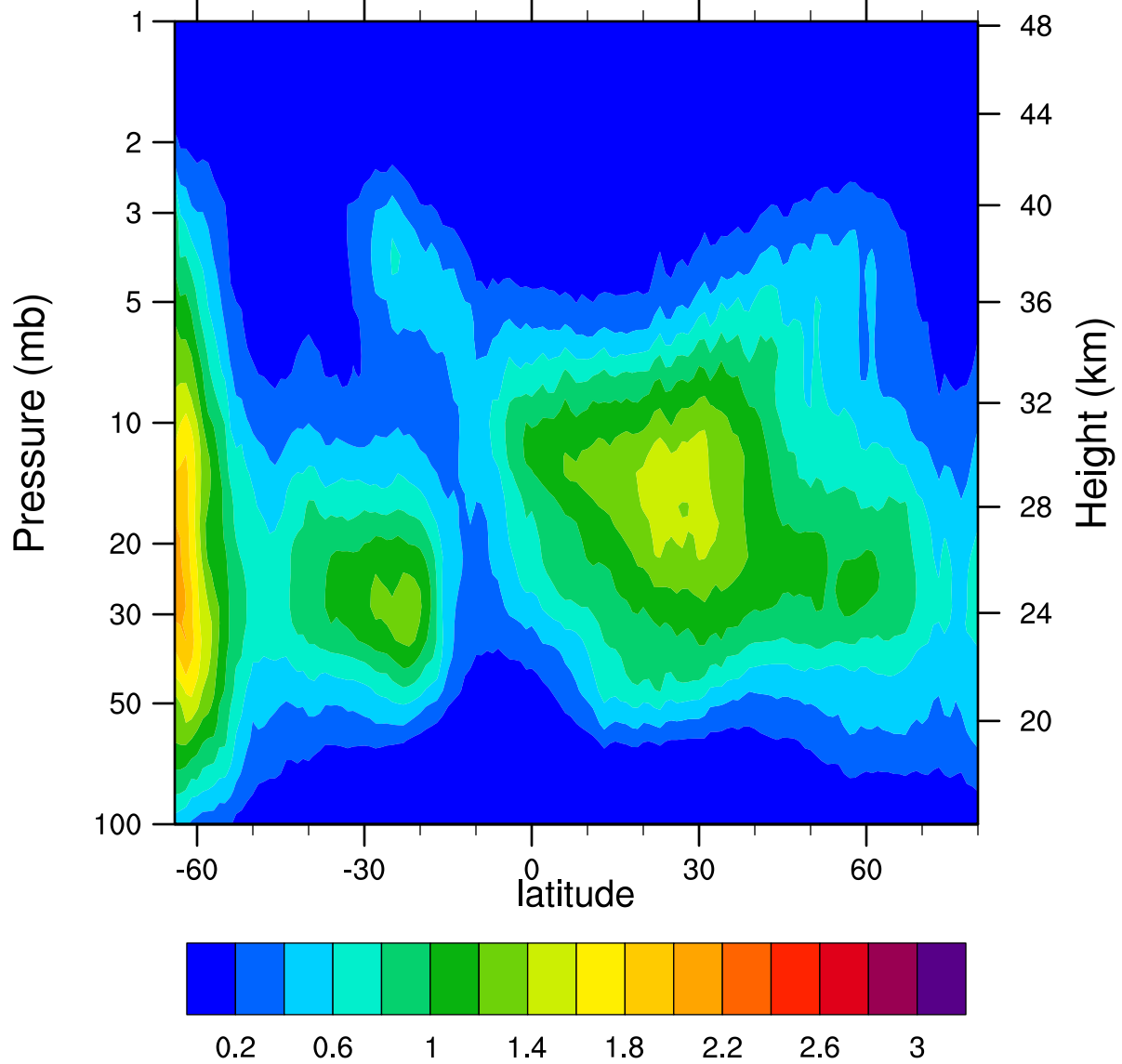
HIRDLSv6 2005d262 ClONO2_Ascending (ppbv)
