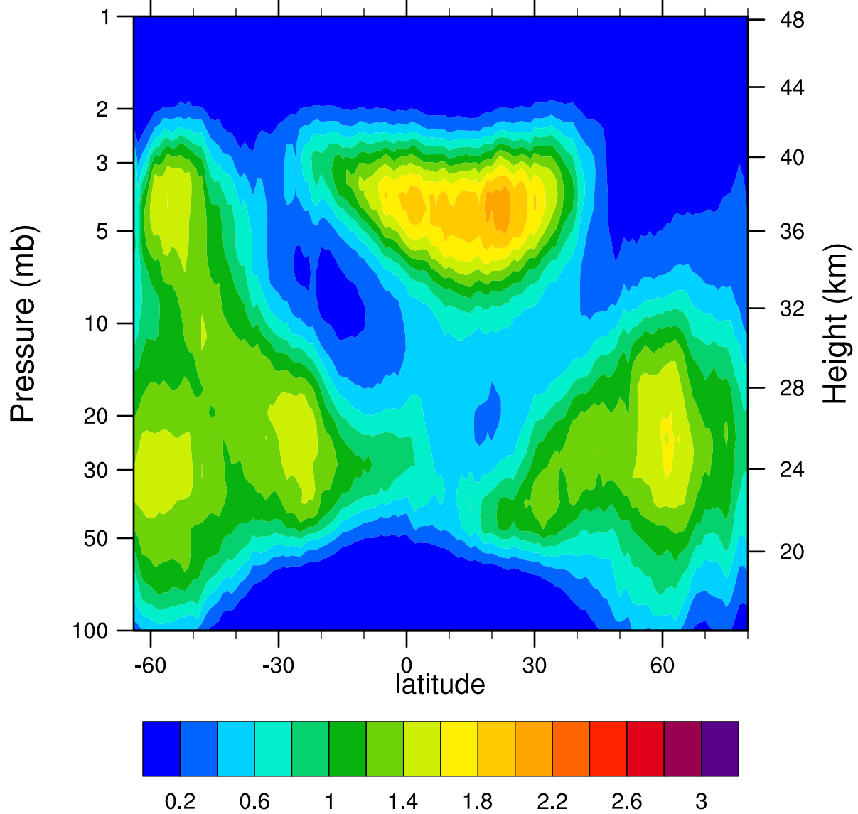
HIRDLSv6 2007d336 ClONO2_Ascending (ppbv)
