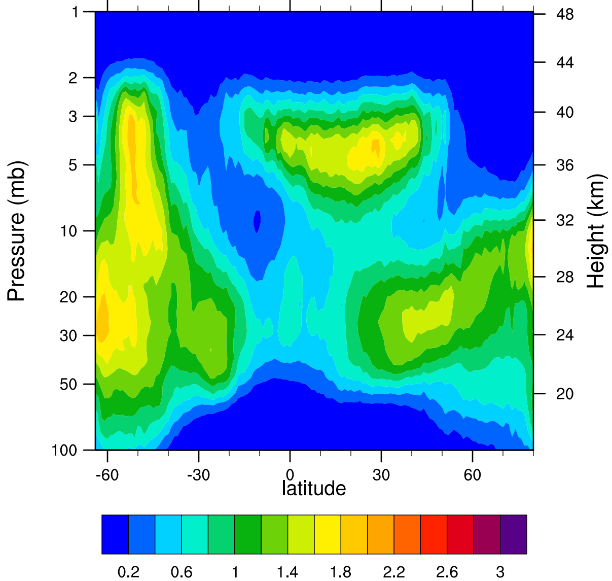
HIRDLSv6 2007d263 ClONO2_Ascending (ppbv)
