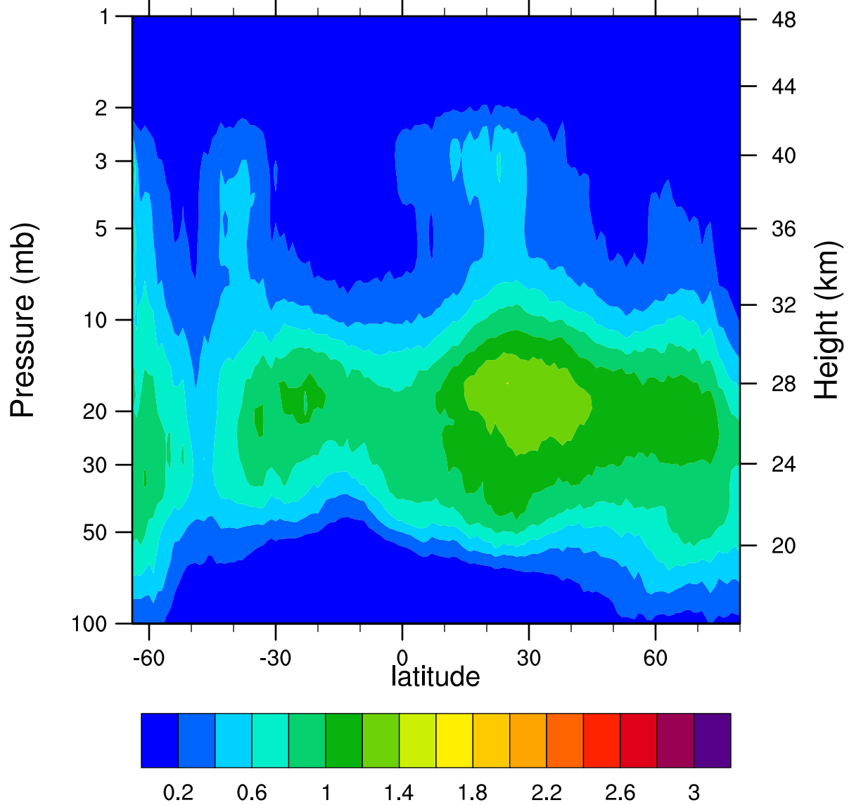
HIRDLSv6 2006d143 ClONO2_Ascending (ppbv)
