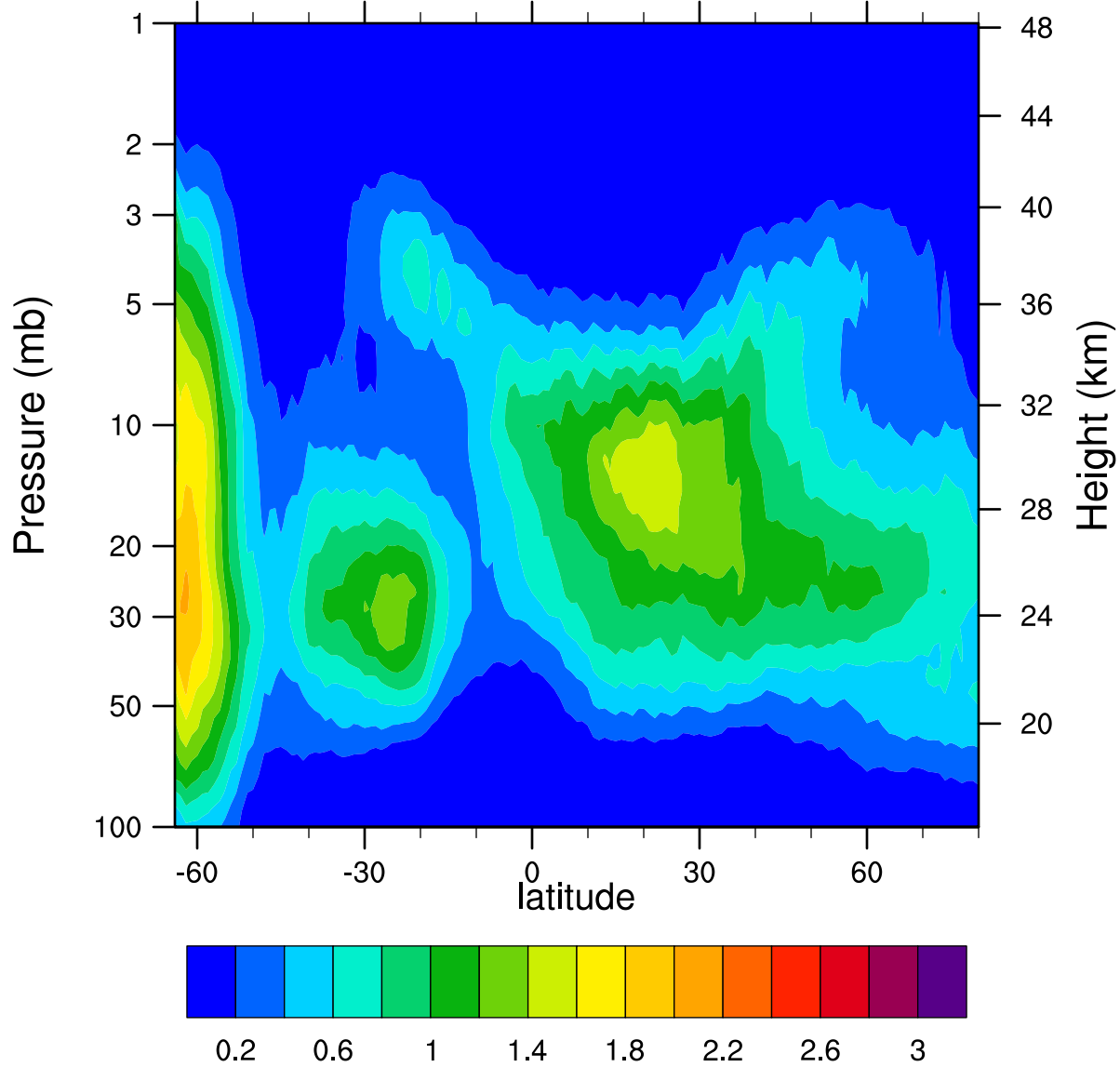
HIRDLSv6 2005d236 ClONO2_Ascending (ppbv)
