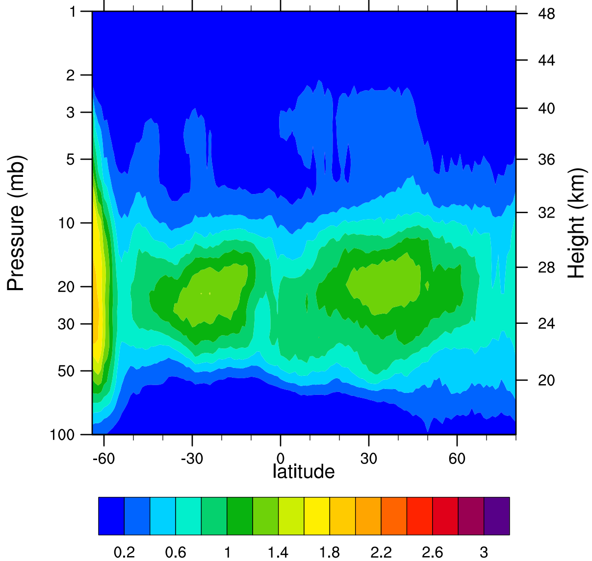
HIRDLSv6 2006d264 ClONO2_Ascending (ppbv)
