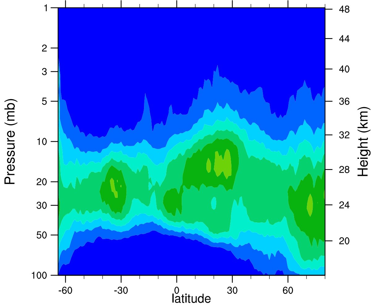
HIRDLSv6 2006d081 ClONO2_Ascending (ppbv)
