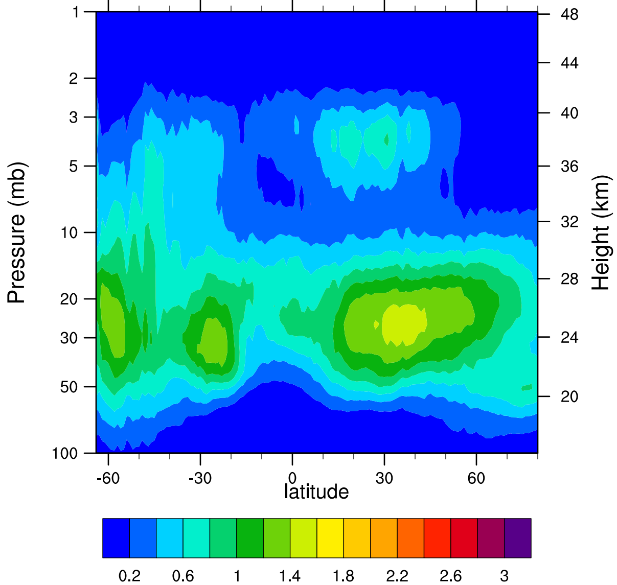
HIRDLSv6 2007d201 ClONO2_Ascending (ppbv)
