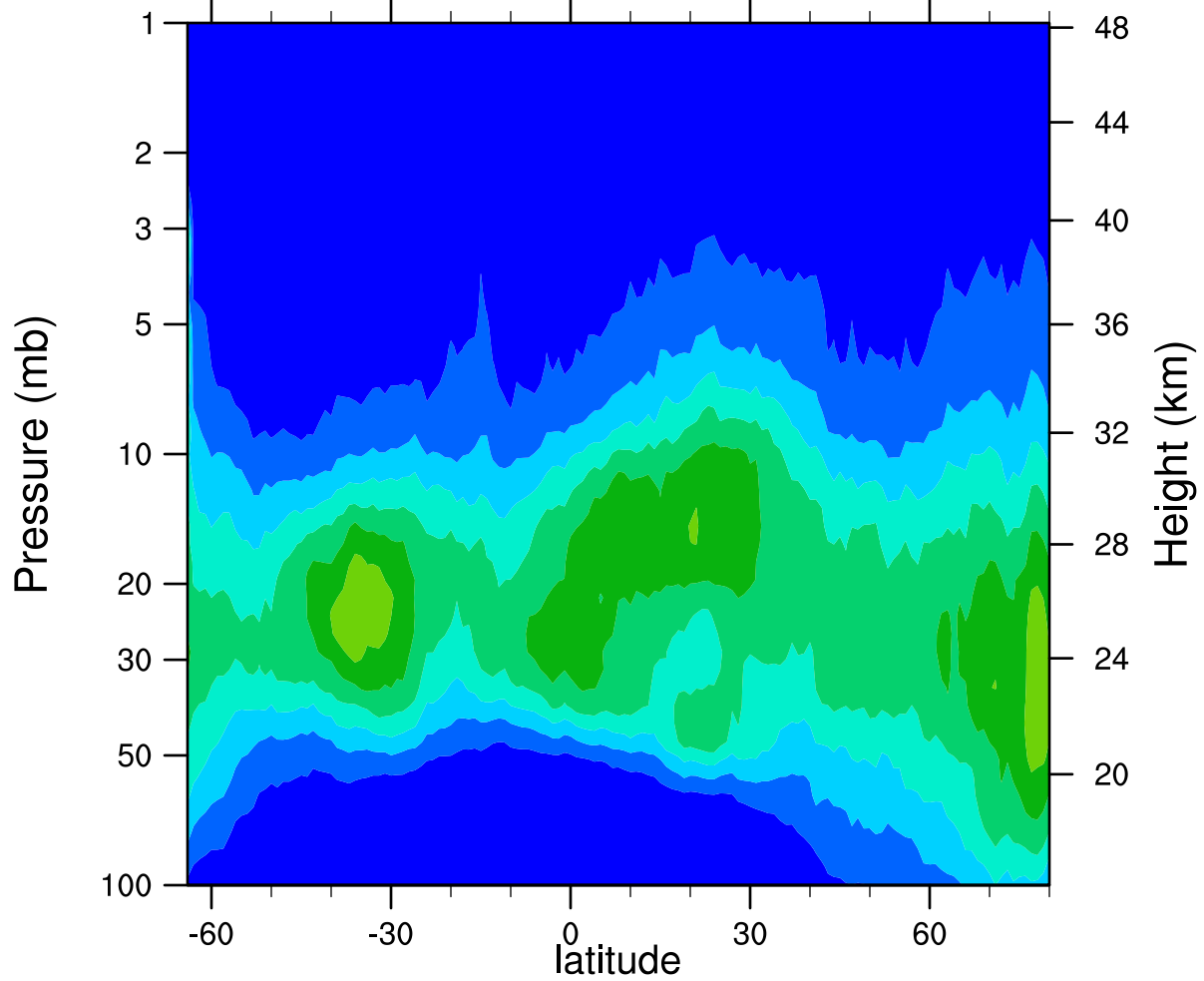
HIRDLSv6 2006d073 ClONO2_Ascending (ppbv)
