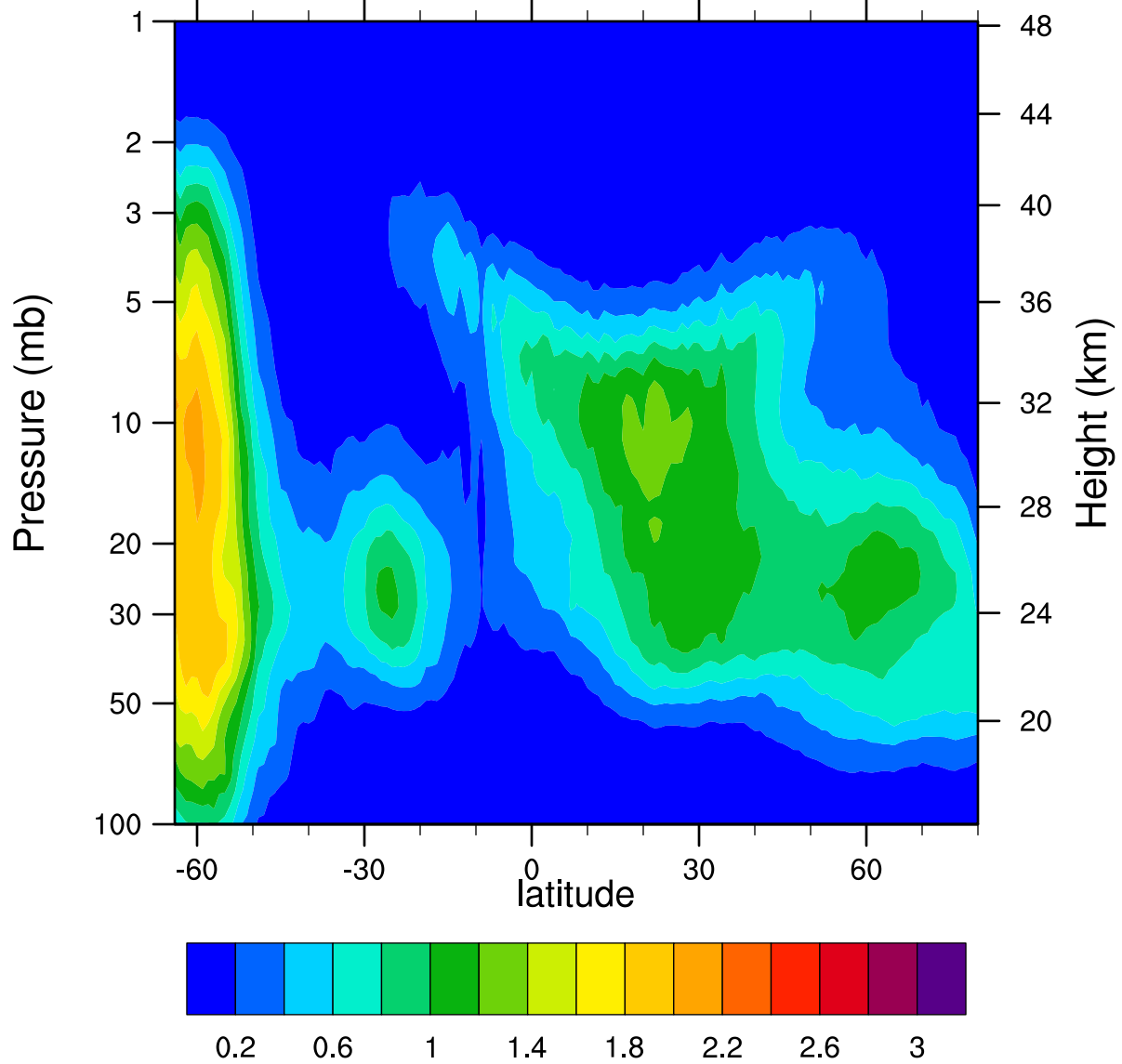
HIRDLSv6 2005d160 ClONO2_Ascending (ppbv)
