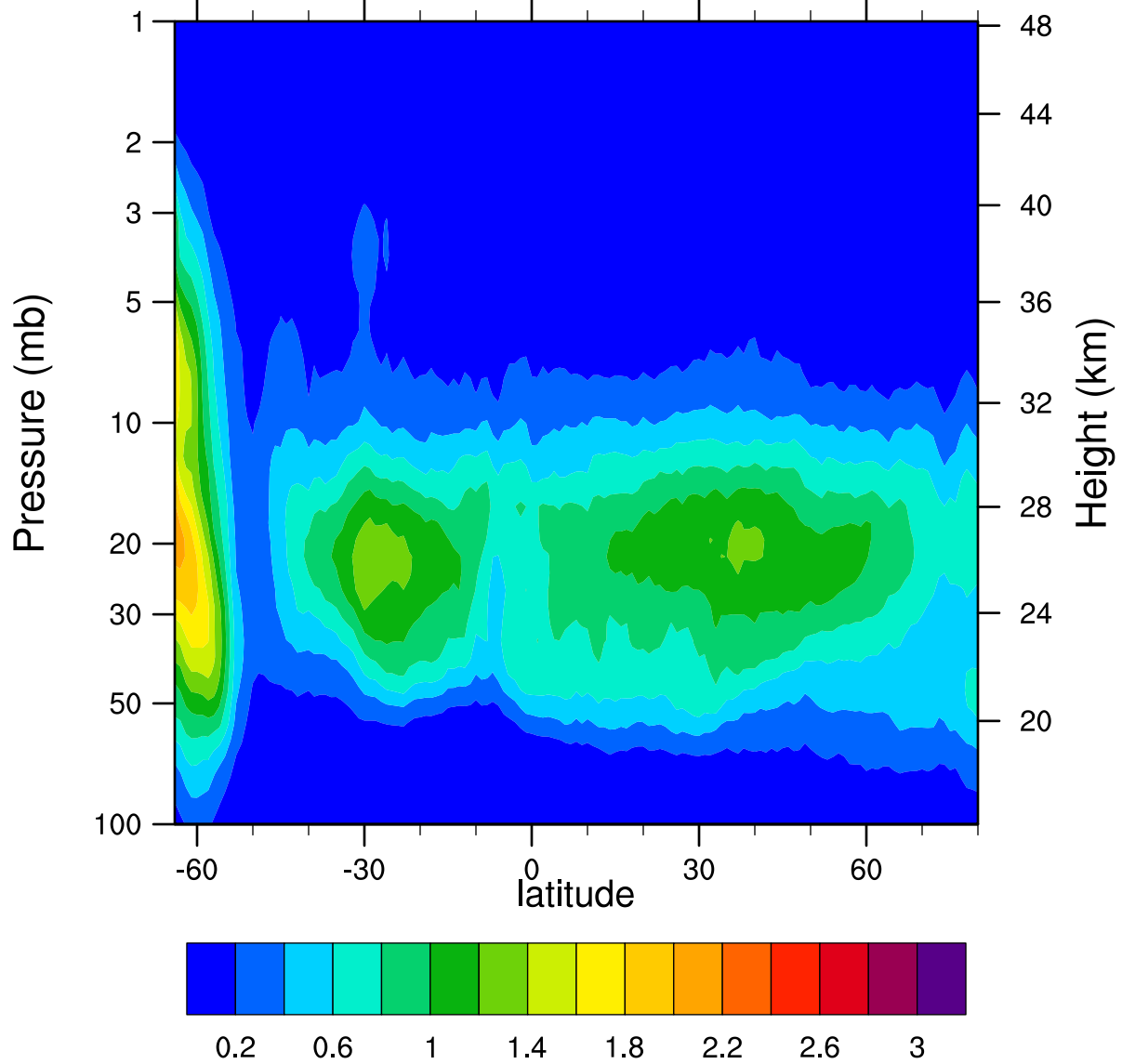
HIRDLSv6 2006d223 ClONO2_Ascending (ppbv)
