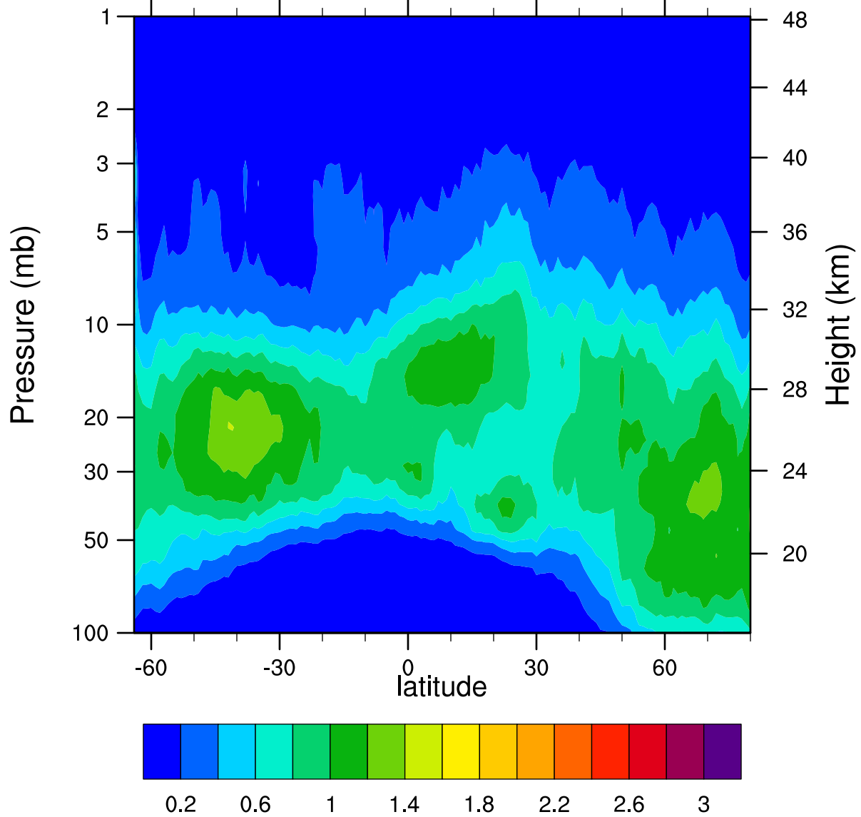
HIRDLSv6 2006d049 ClONO2_Ascending (ppbv)
