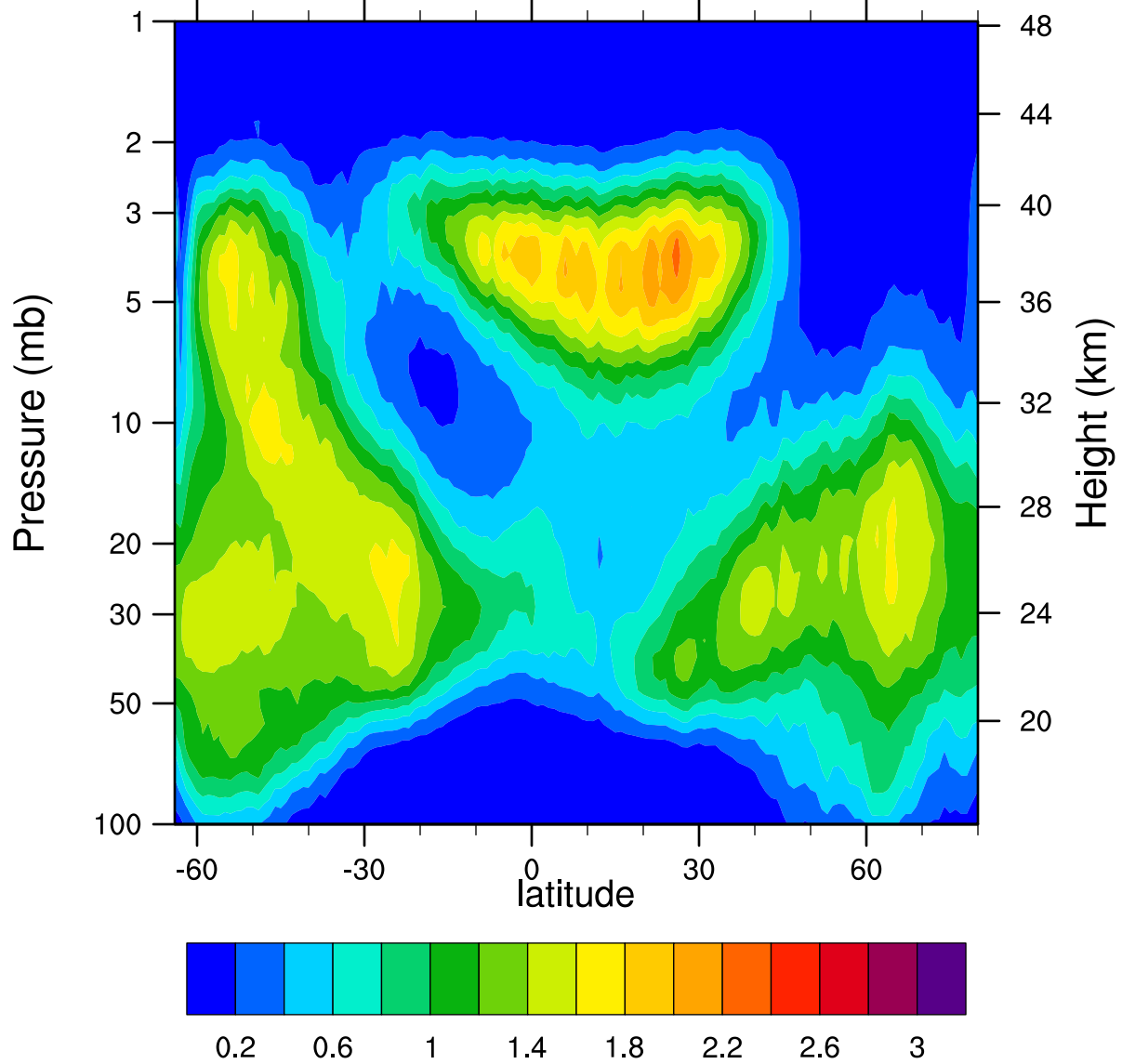
HIRDLSv6 2007d322 ClONO2_Ascending (ppbv)
