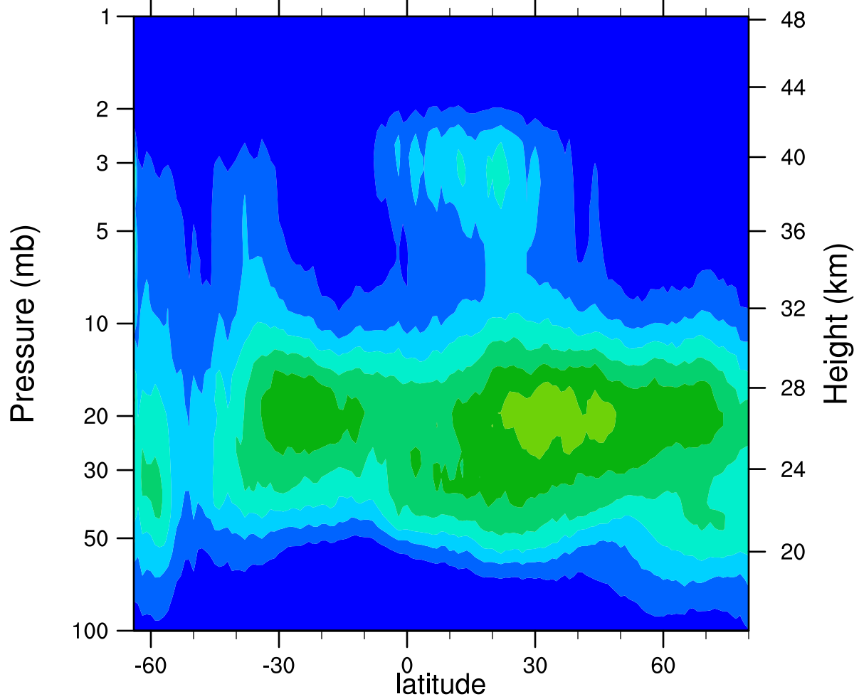
HIRDLSv6 2006d173 ClONO2_Ascending (ppbv)
