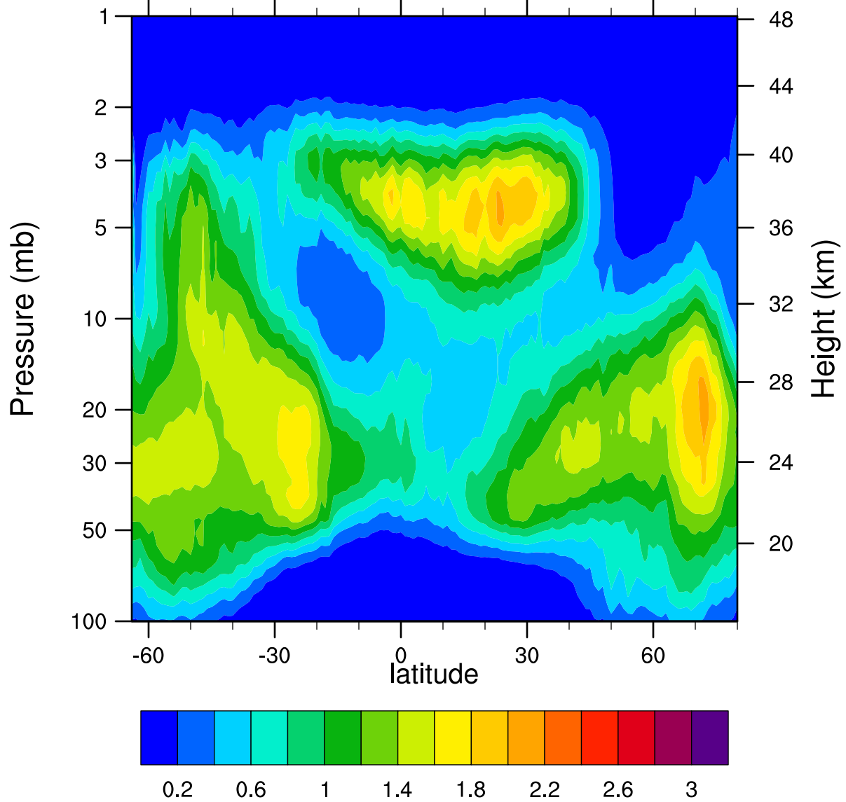
HIRDLSv6 2007d314 ClONO2_Ascending (ppbv)
