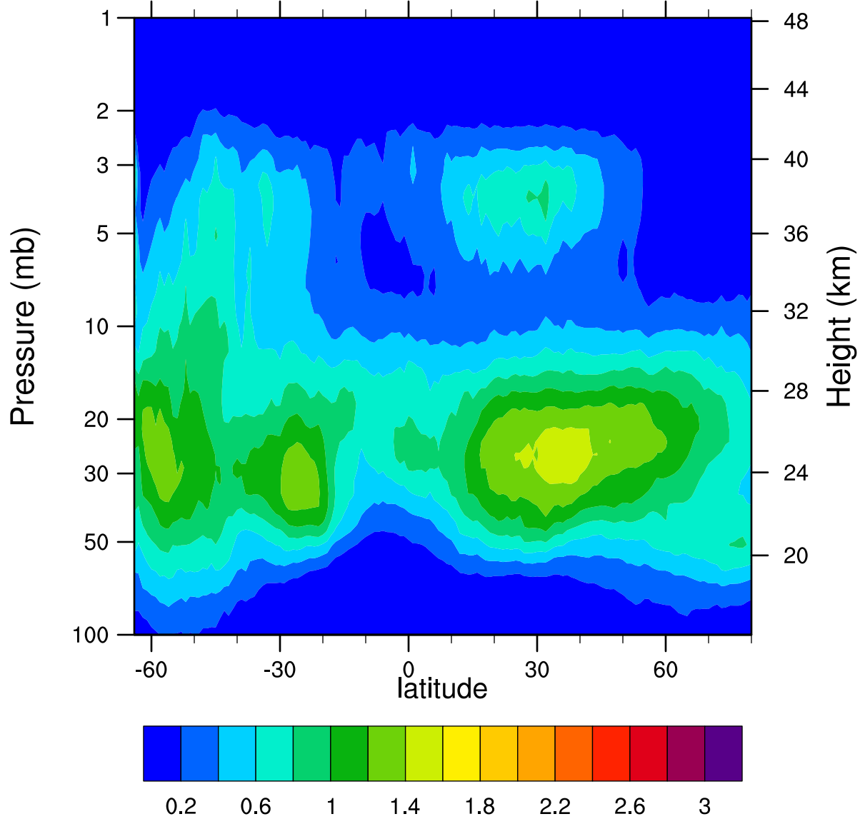
HIRDLSv6 2007d199 ClONO2_Ascending (ppbv)
