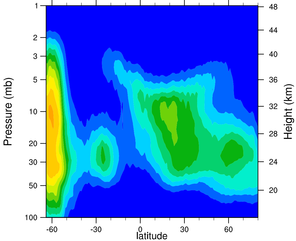
HIRDLSv6 2005d163 ClONO2_Ascending (ppbv)
