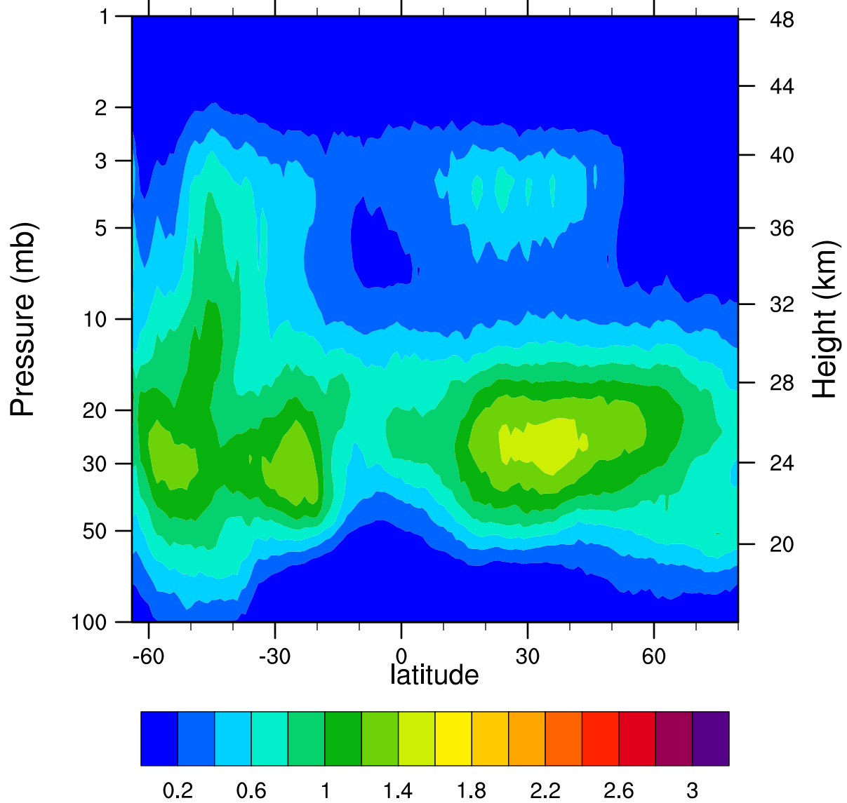
HIRDLSv6 2007d195 ClONO2_Ascending (ppbv)
