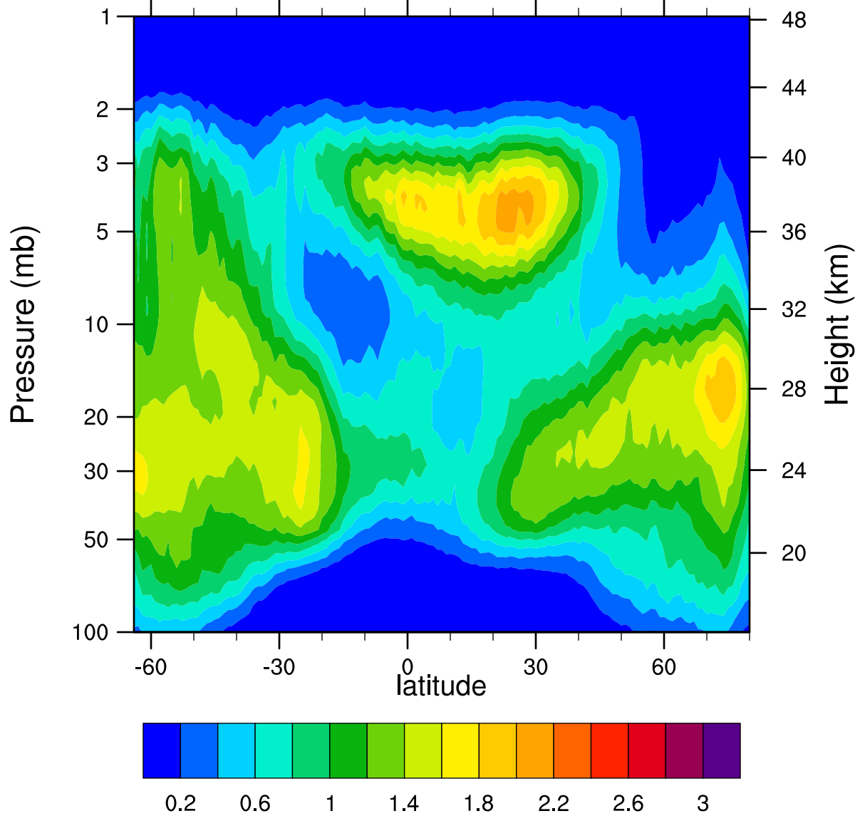
HIRDLSv6 2007d298 ClONO2_Ascending (ppbv)
