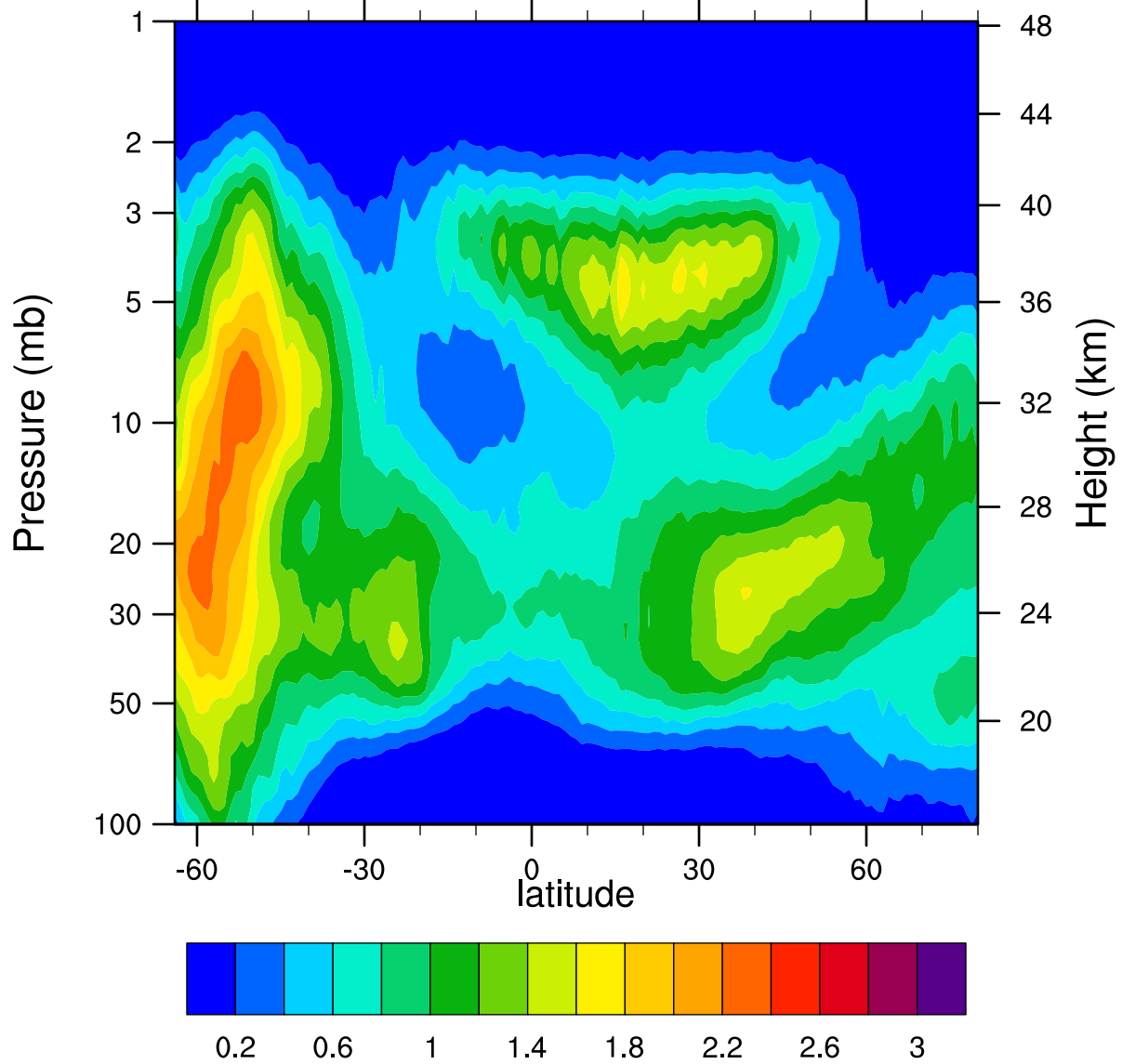
HIRDLSv6 2007d233 ClONO2_Ascending (ppbv)
