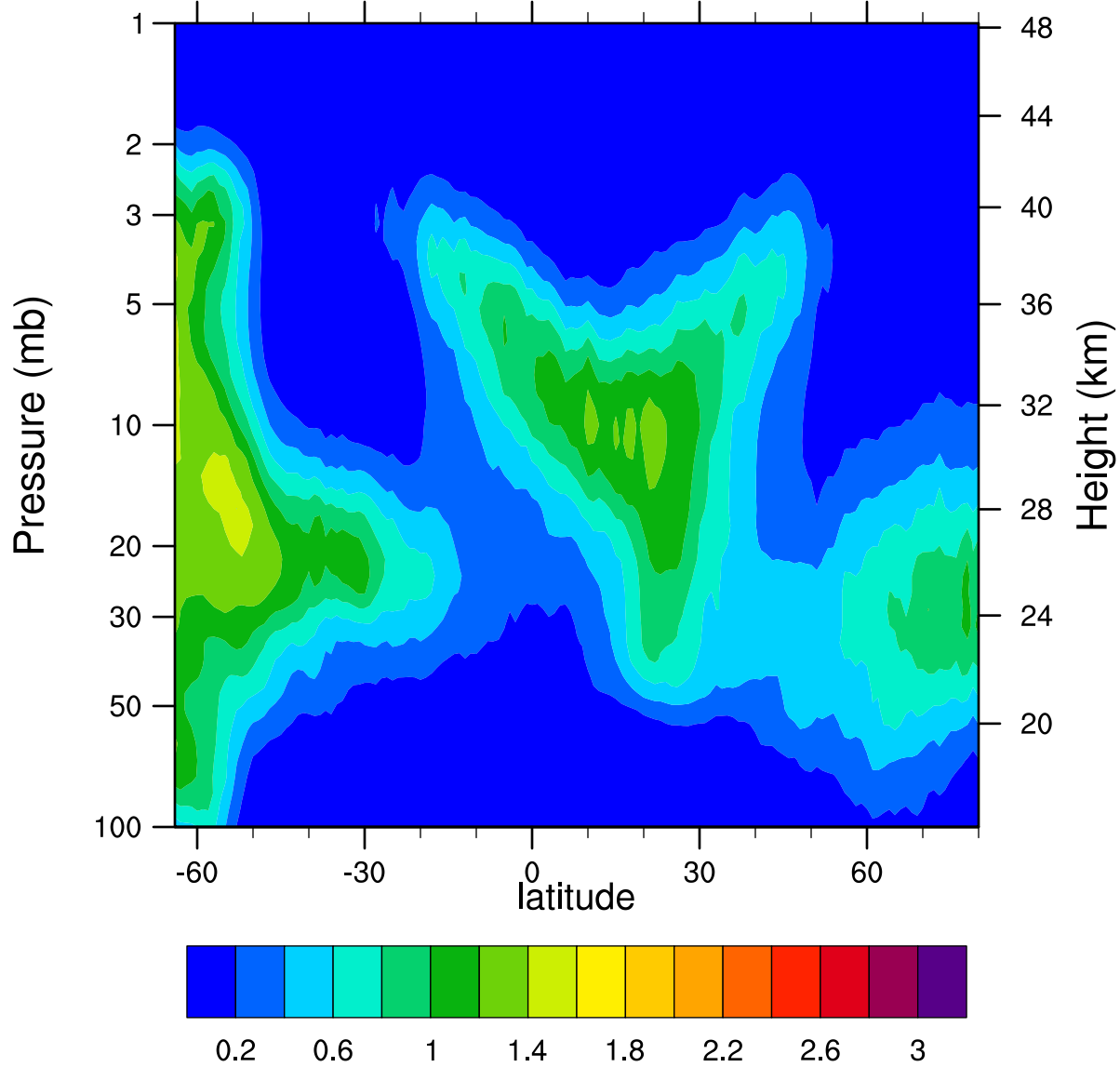
HIRDLSv6 2005d049 ClONO2_Ascending (ppbv)
