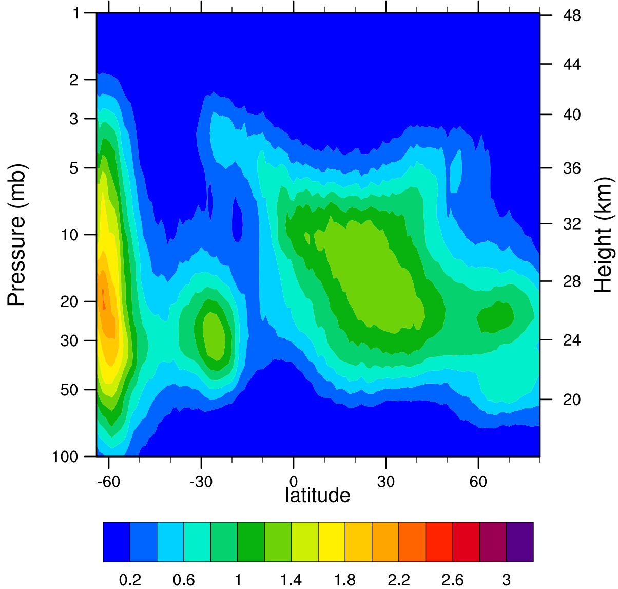
HIRDLSv6 2005d196 ClONO2_Ascending (ppbv)
