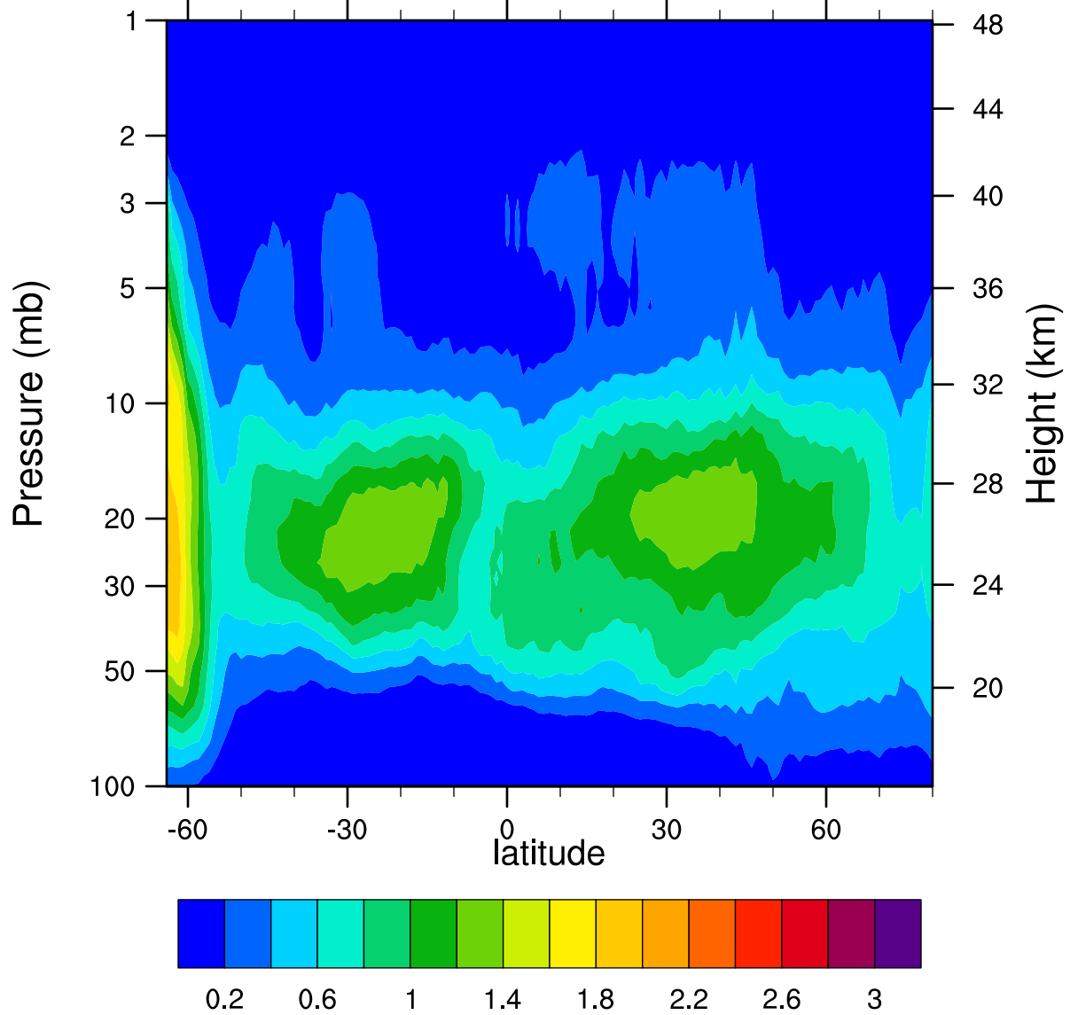
HIRDLSv6 2006d262 ClONO2_Ascending (ppbv)
