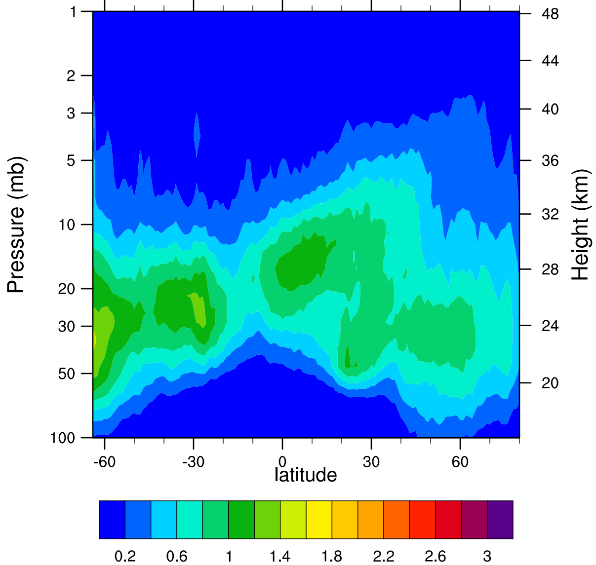
HIRDLSv6 2005d338 ClONO2_Ascending (ppbv)
