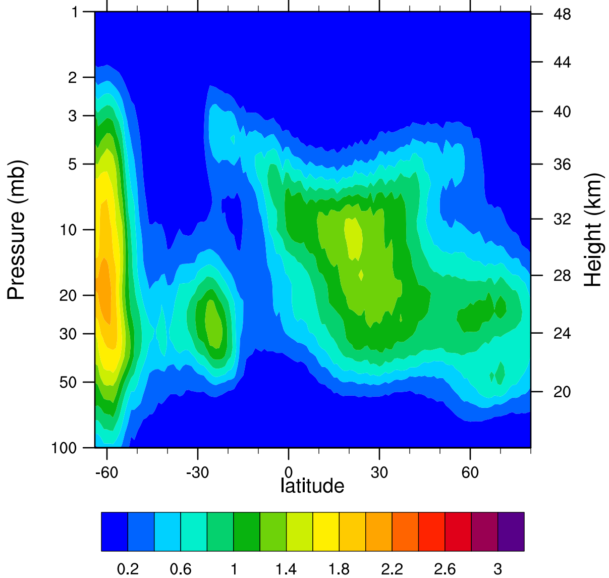
HIRDLSv6 2005d182 ClONO2_Ascending (ppbv)
