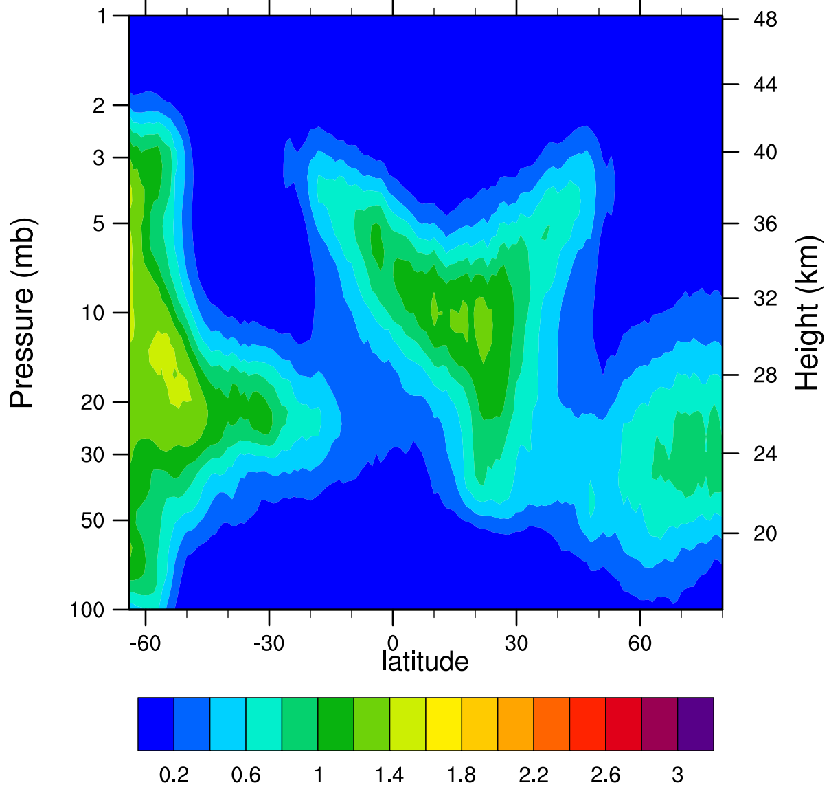
HIRDLSv6 2005d050 ClONO2_Ascending (ppbv)
