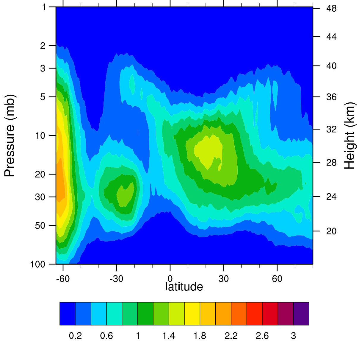
HIRDLSv6 2005d230 ClONO2_Ascending (ppbv)
