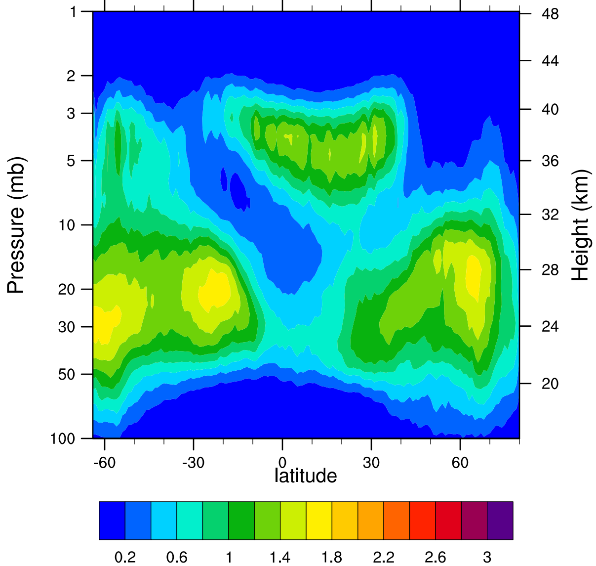
HIRDLSv6 2006d325 ClONO2_Ascending (ppbv)
