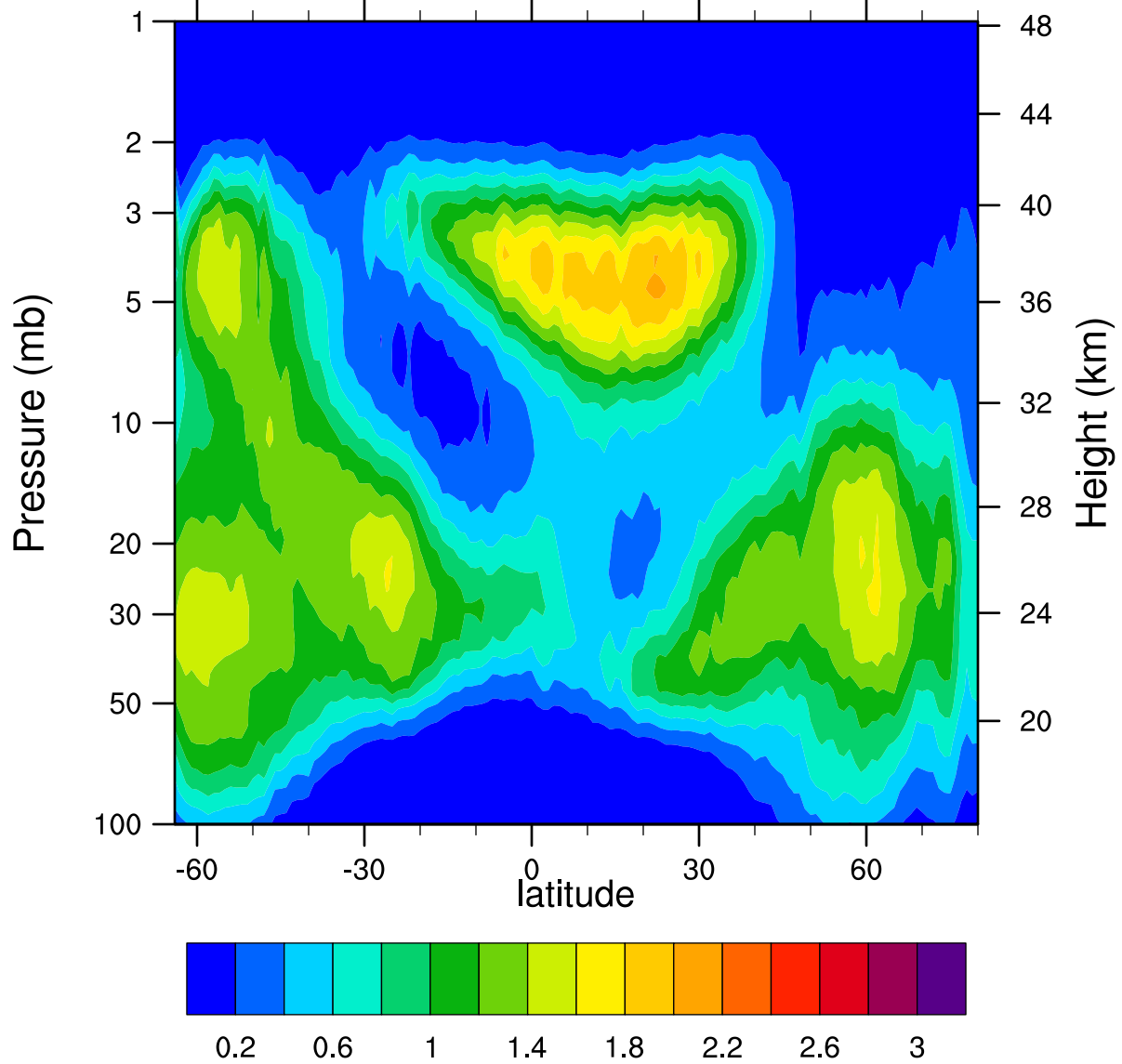
HIRDLSv6 2007d338 ClONO2_Ascending (ppbv)
