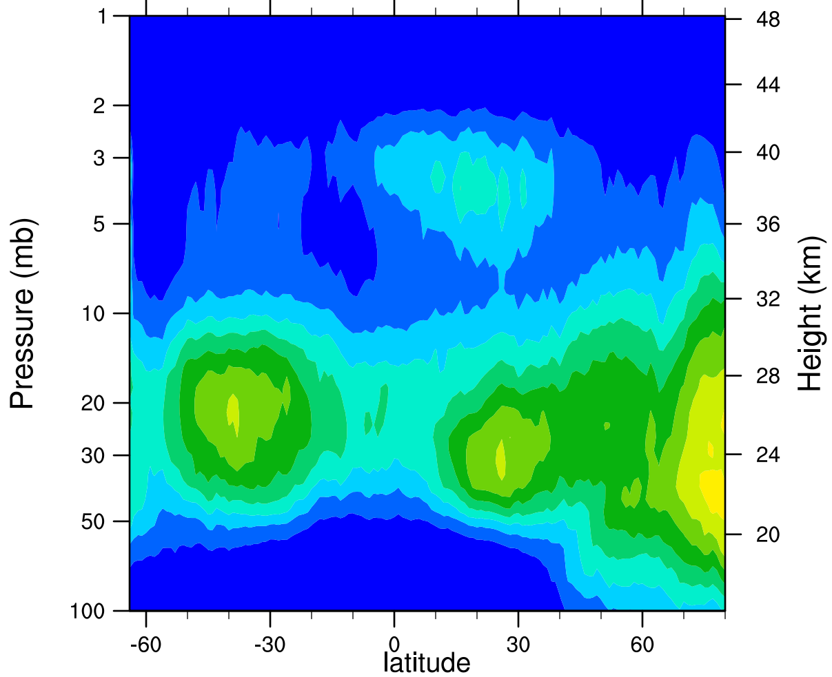
HIRDLSv6 2007d059 ClONO2_Ascending (ppbv)
