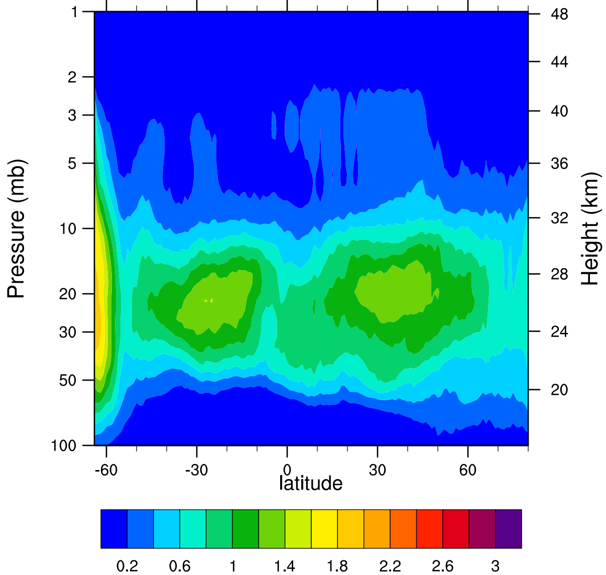
HIRDLSv6 2006d265 ClONO2_Ascending (ppbv)
