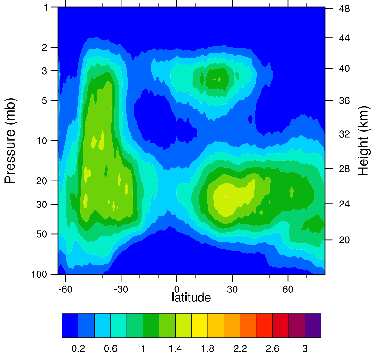
HIRDLSv6 2007d151 ClONO2_Ascending (ppbv)
