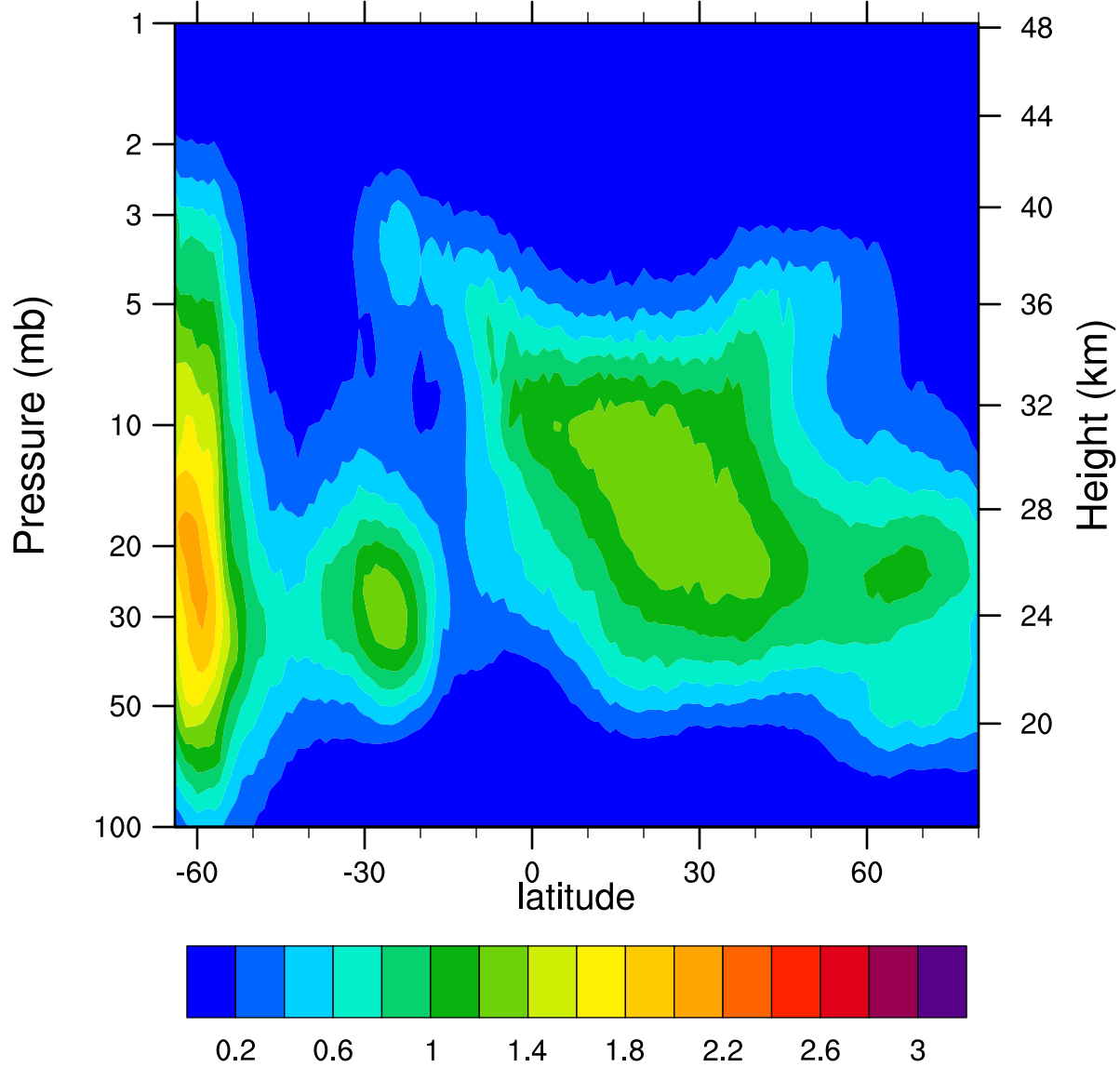
HIRDLSv6 2005d199 ClONO2_Ascending (ppbv)
