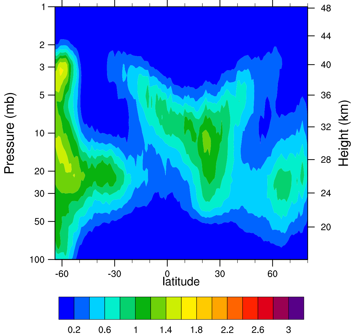
HIRDLSv6 2005d029 ClONO2_Ascending (ppbv)
