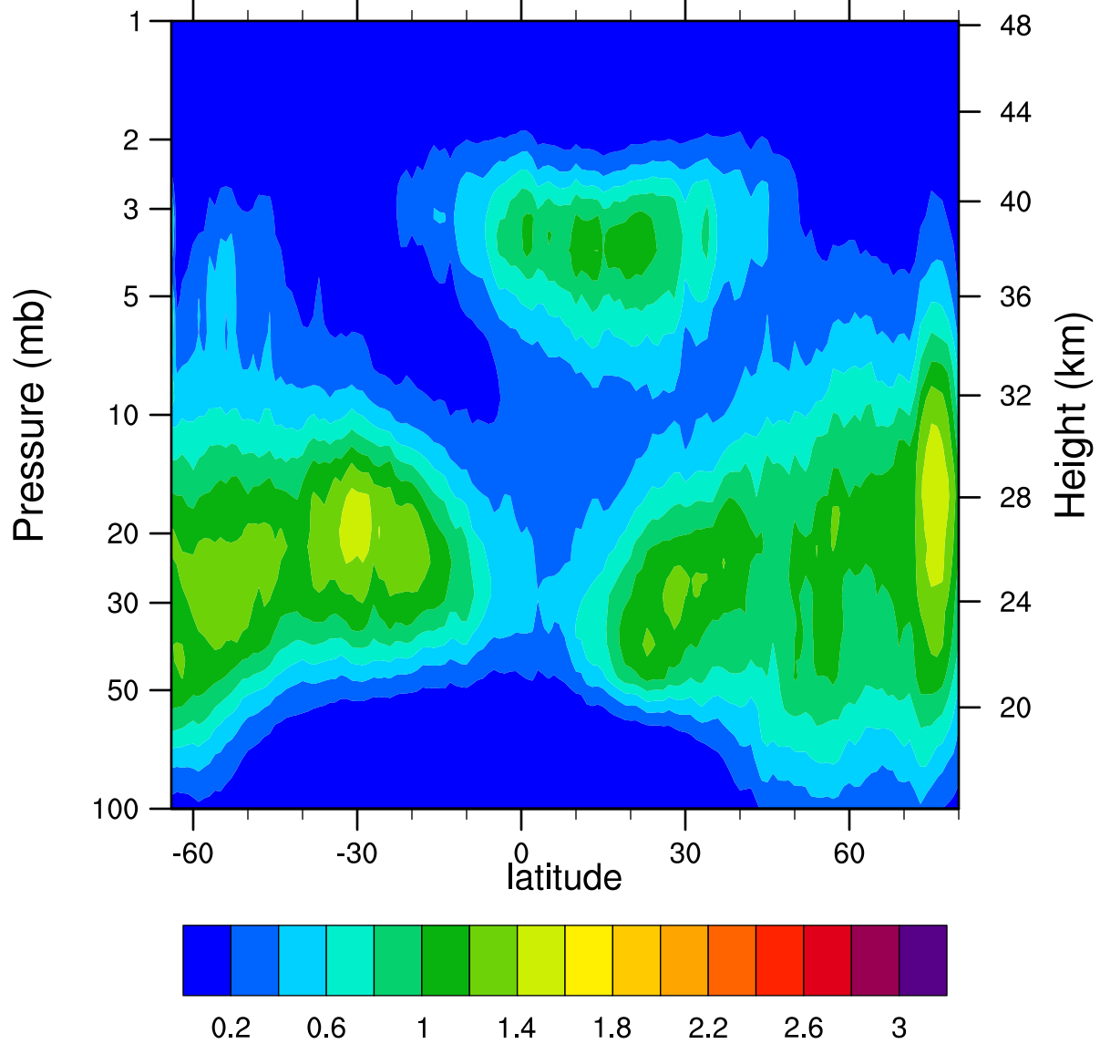
HIRDLSv6 2006d359 ClONO2_Ascending (ppbv)
