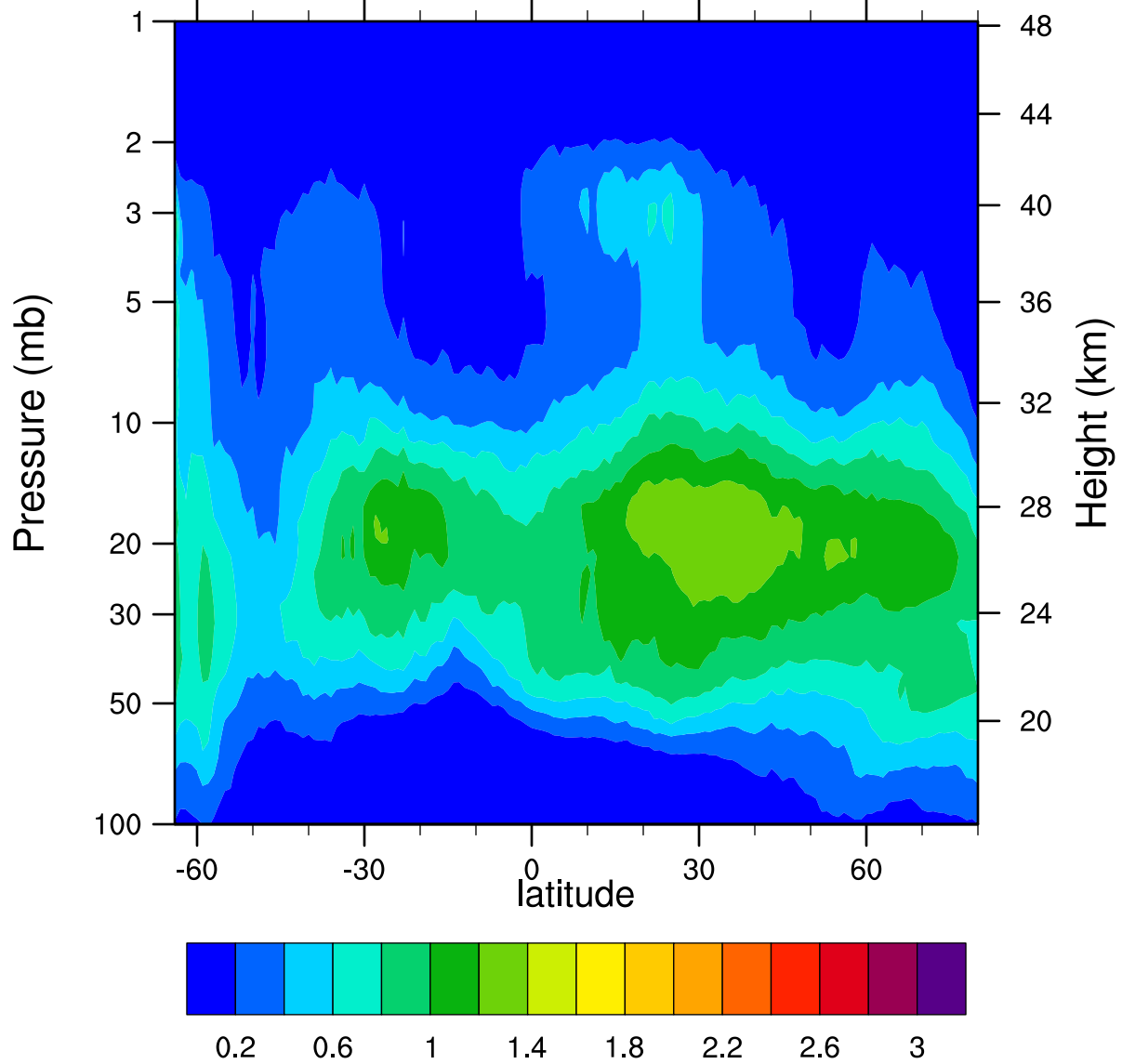
HIRDLSv6 2006d152 ClONO2_Ascending (ppbv)
