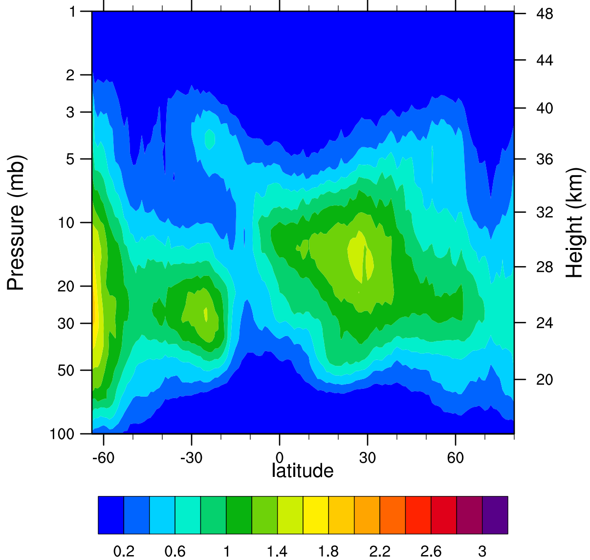
HIRDLSv6 2005d273 ClONO2_Ascending (ppbv)
