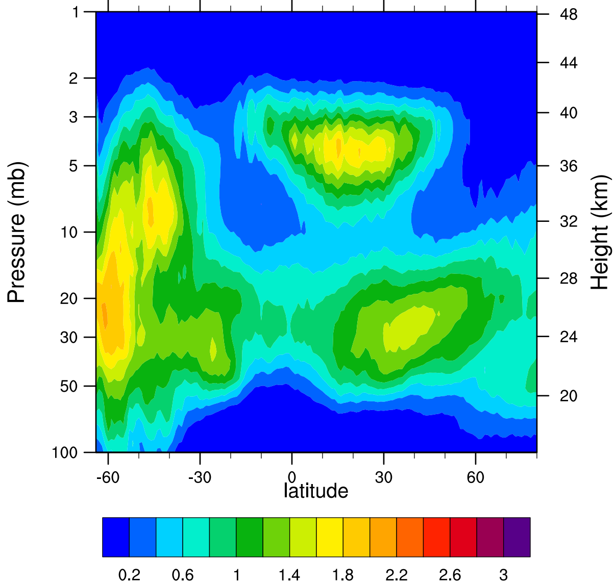
HIRDLSv6 2007d214 ClONO2_Ascending (ppbv)
