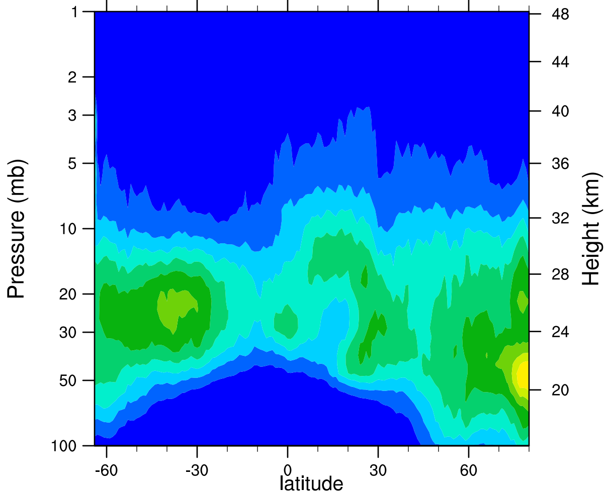
HIRDLSv6 2006d026 ClONO2_Ascending (ppbv)
