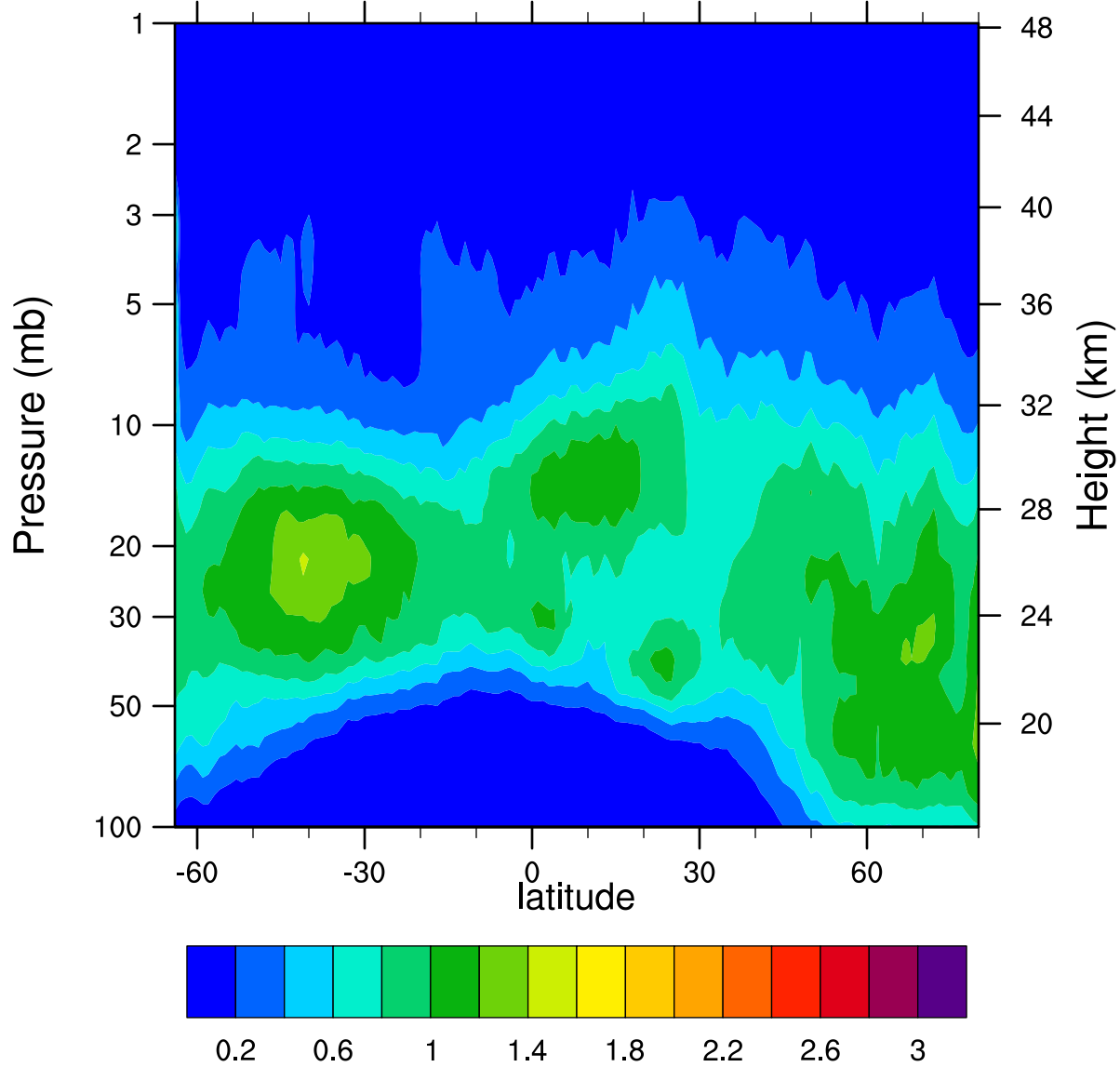
HIRDLSv6 2006d047 ClONO2_Ascending (ppbv)
