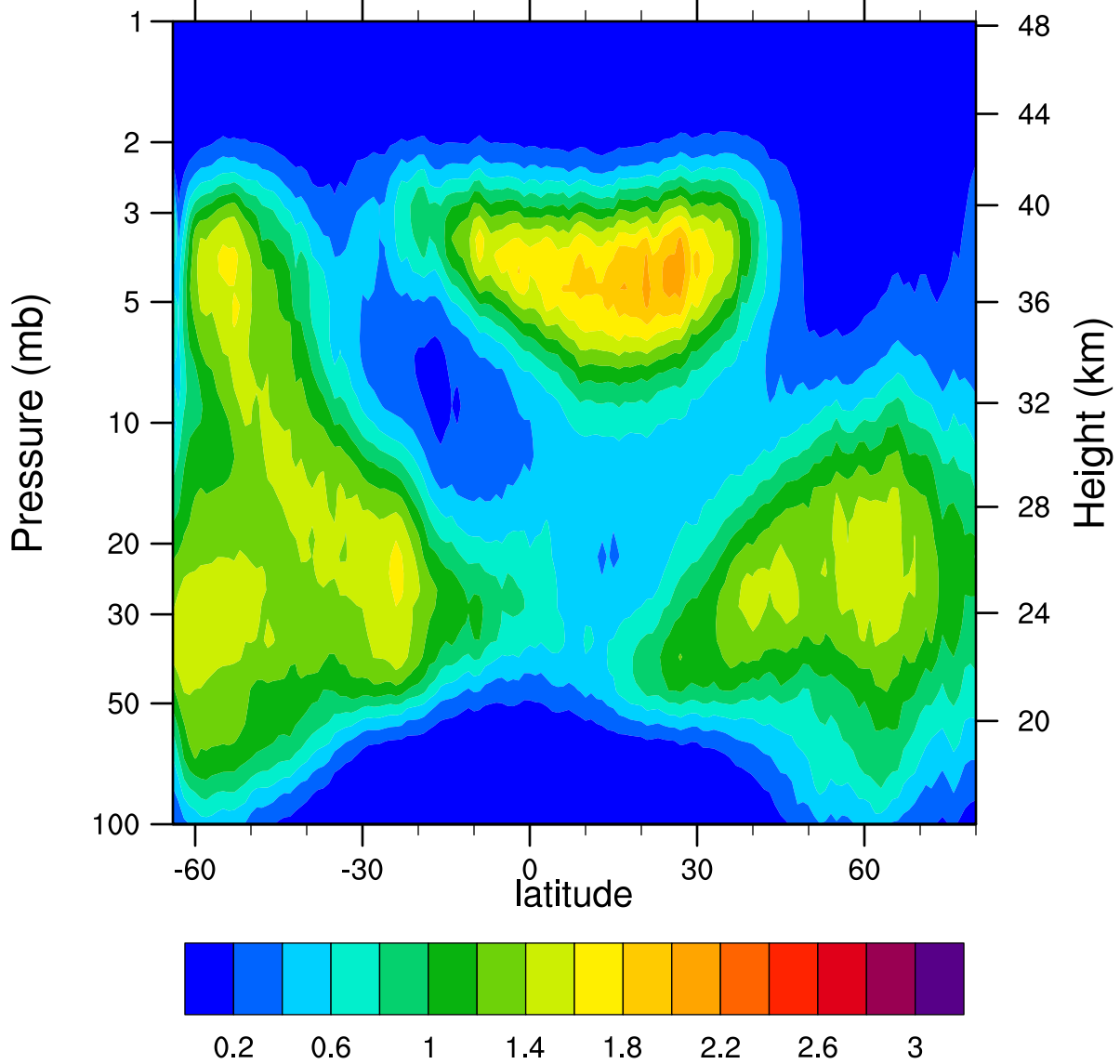
HIRDLSv6 2007d326 ClONO2_Ascending (ppbv)
