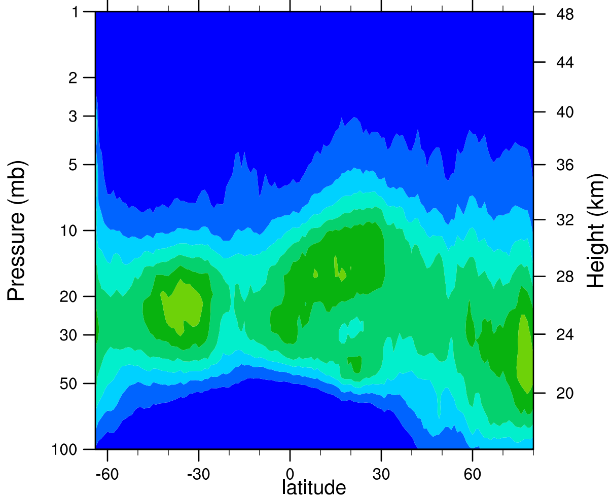
HIRDLSv6 2006d065 ClONO2_Ascending (ppbv)
