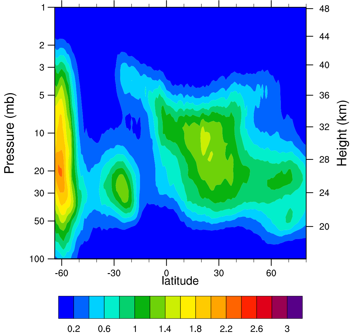
HIRDLSv6 2005d185 ClONO2_Ascending (ppbv)
