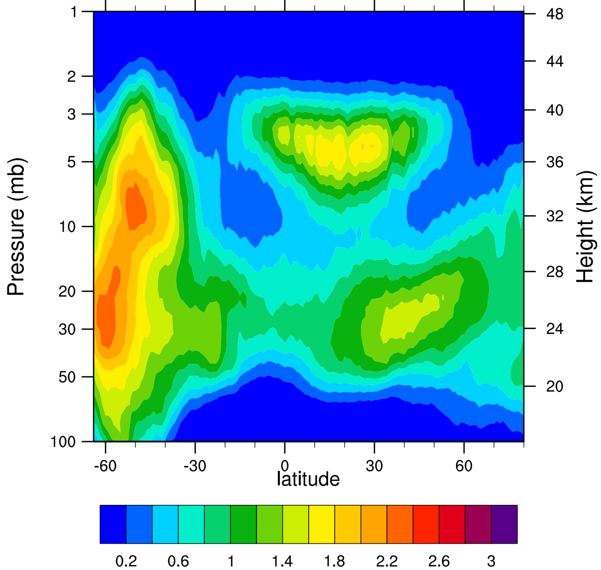
HIRDLSv6 2007d224 ClONO2_Ascending (ppbv)
