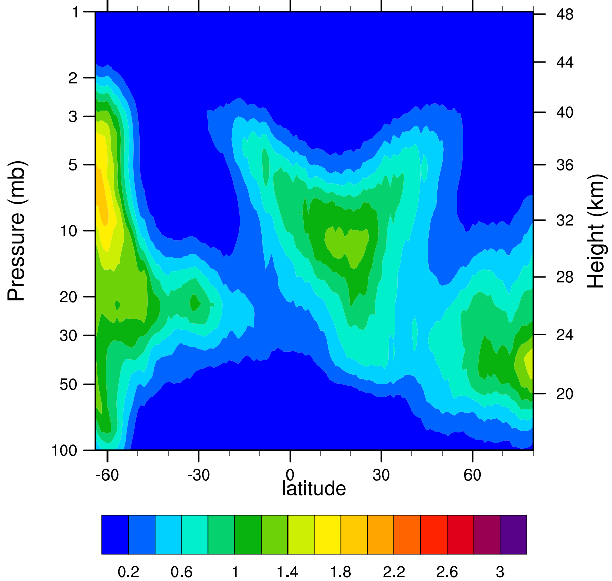
HIRDLSv6 2005d067 ClONO2_Ascending (ppbv)
