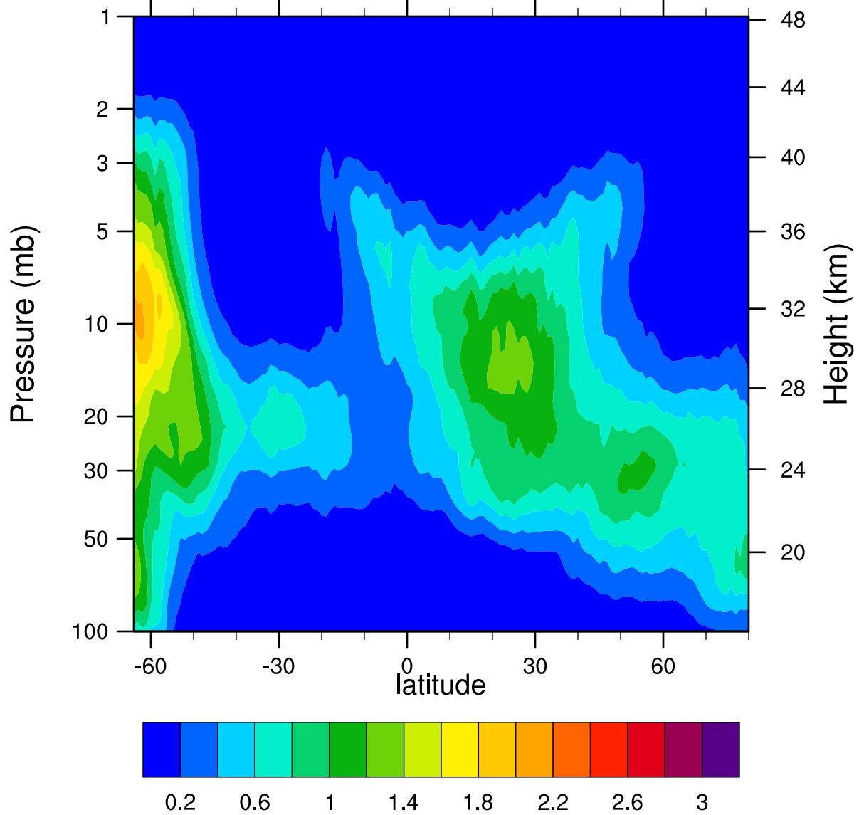
HIRDLSv6 2005d103 ClONO2_Ascending (ppbv)
