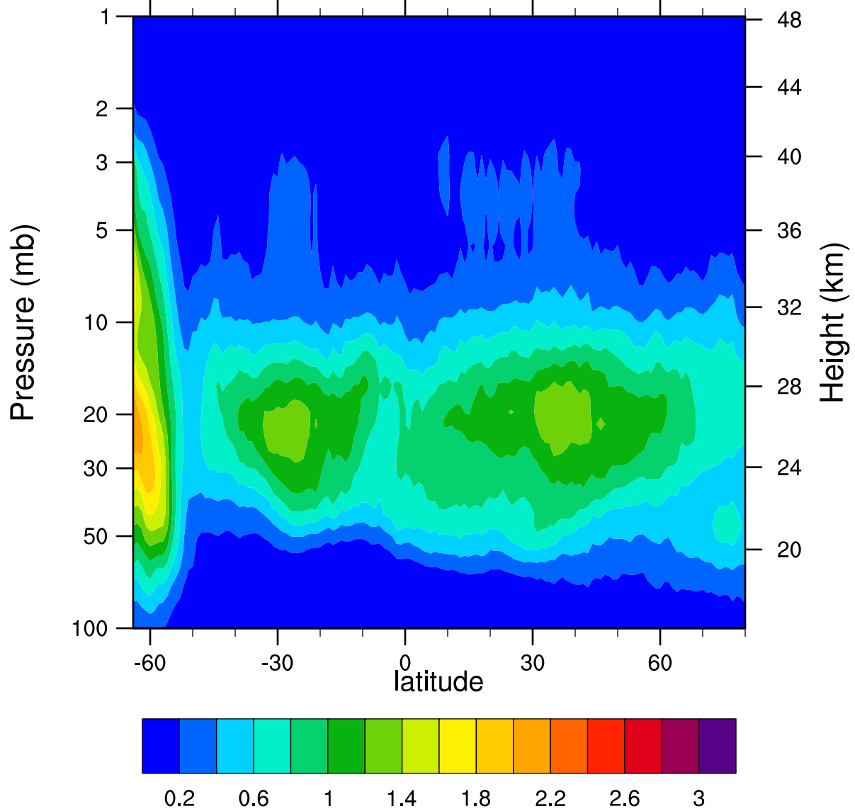
HIRDLSv6 2006d233 ClONO2_Ascending (ppbv)
