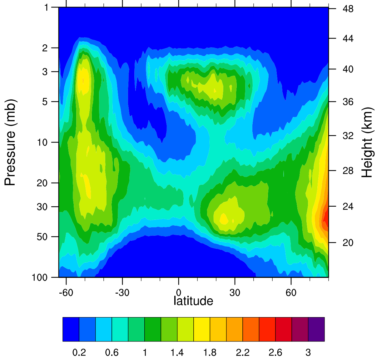
HIRDLSv6 2007d081 ClONO2_Ascending (ppbv)
