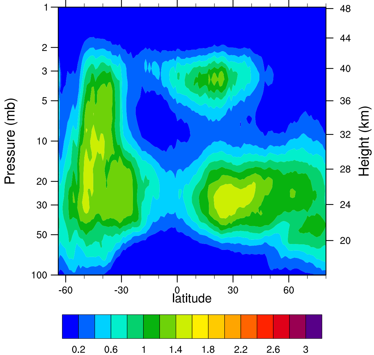
HIRDLSv6 2007d149 ClONO2_Ascending (ppbv)
