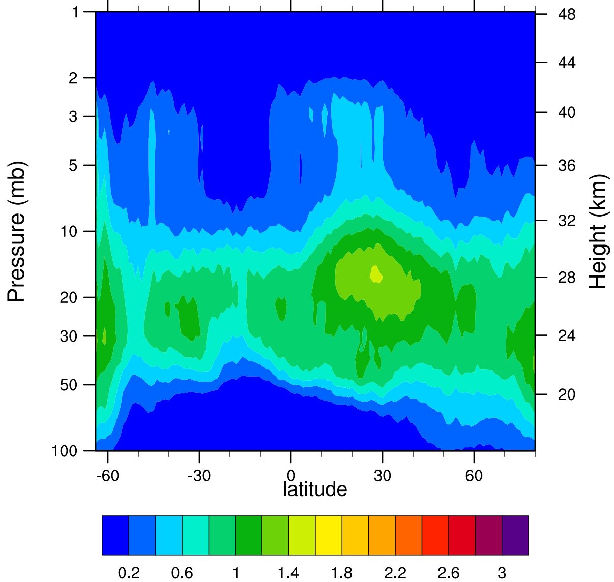
HIRDLSv6 2006d116 ClONO2_Ascending (ppbv)
