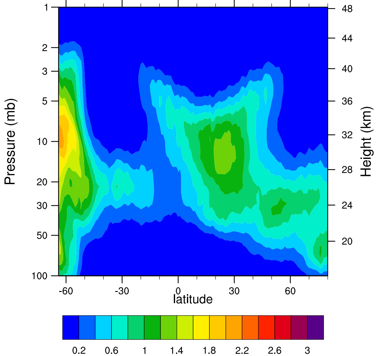
HIRDLSv6 2005d099 ClONO2_Ascending (ppbv)
