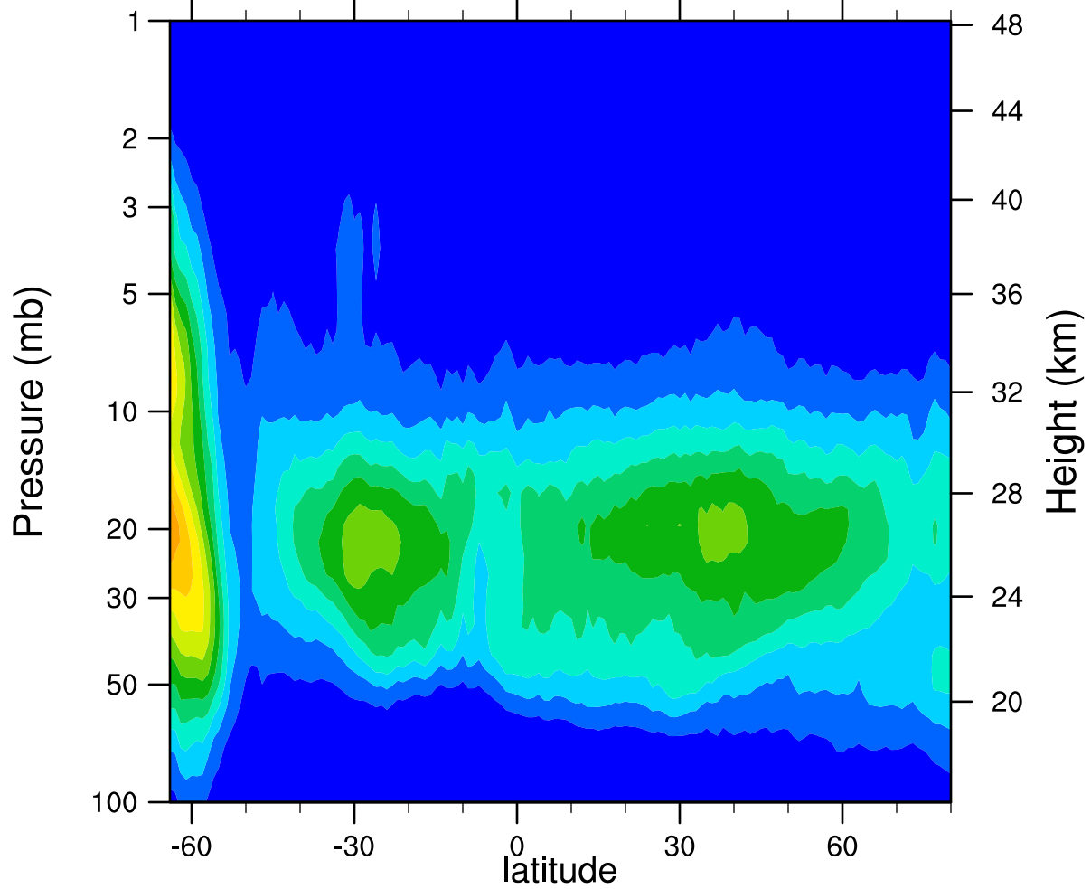
HIRDLSv6 2006d225 ClONO2_Ascending (ppbv)
