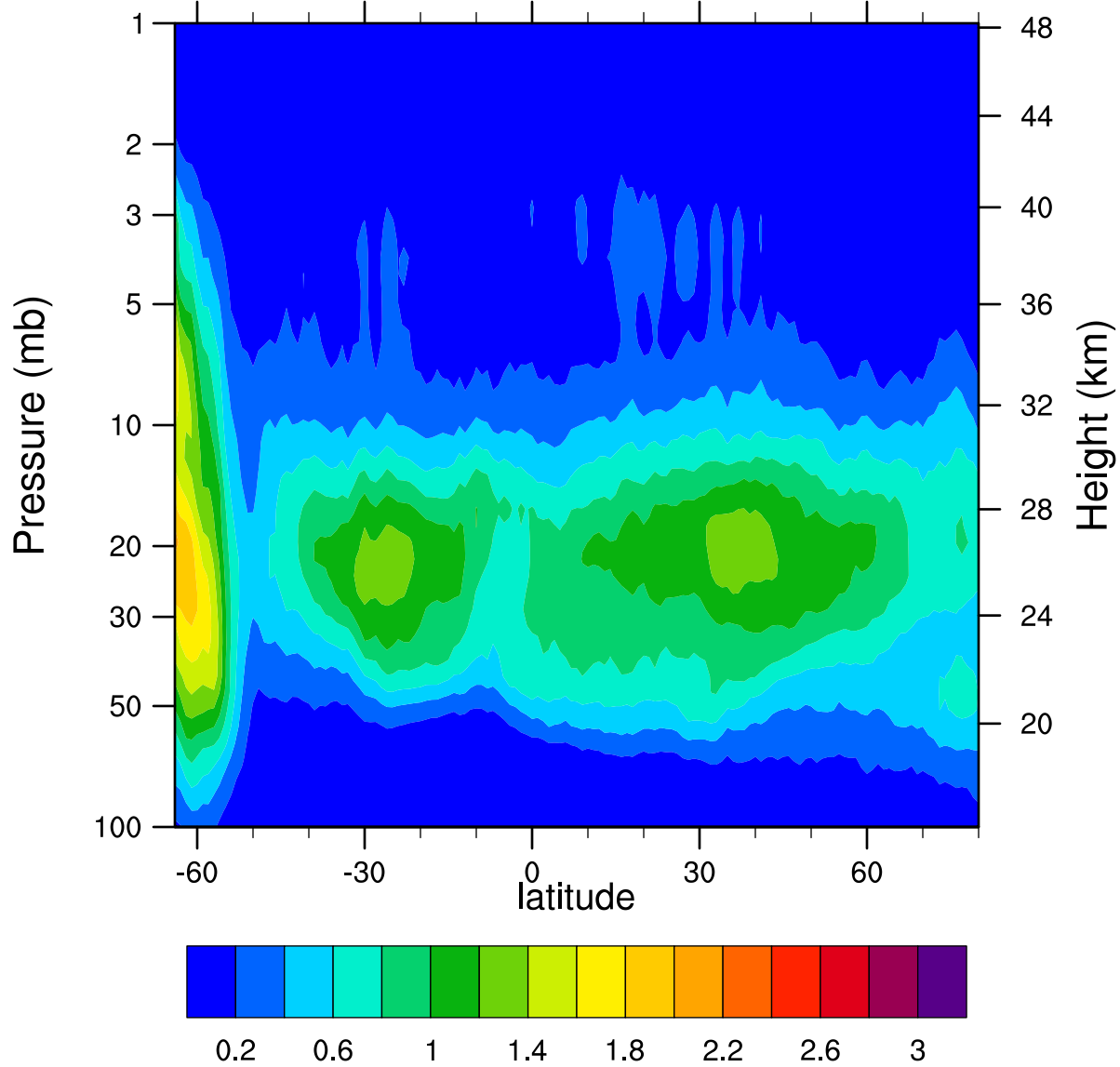
HIRDLSv6 2006d230 ClONO2_Ascending (ppbv)
