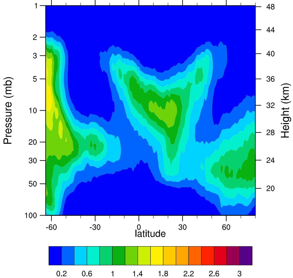
HIRDLSv6 2005d056 ClONO2_Ascending (ppbv)
