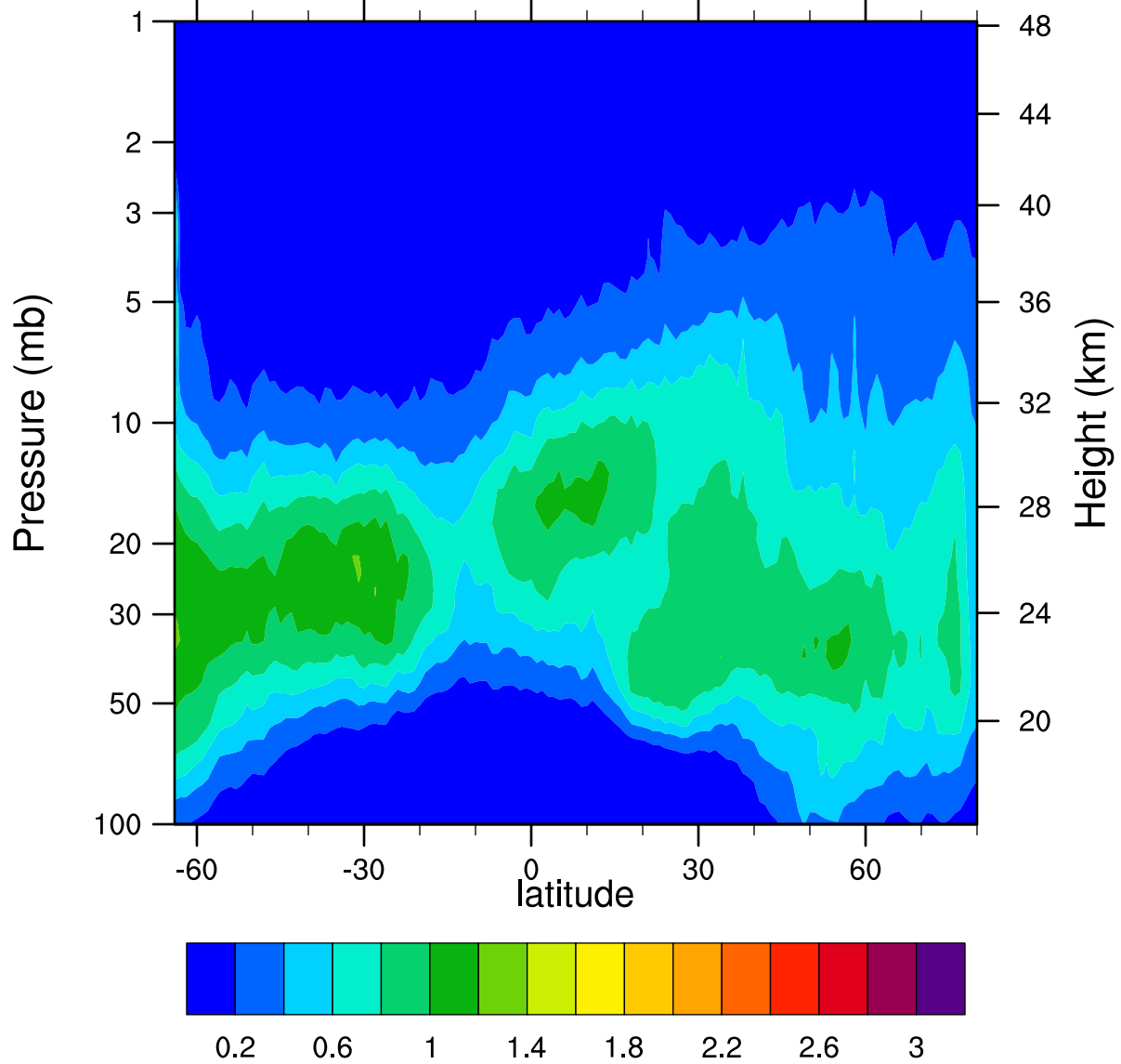
HIRDLSv6 2005d348 ClONO2_Ascending (ppbv)
