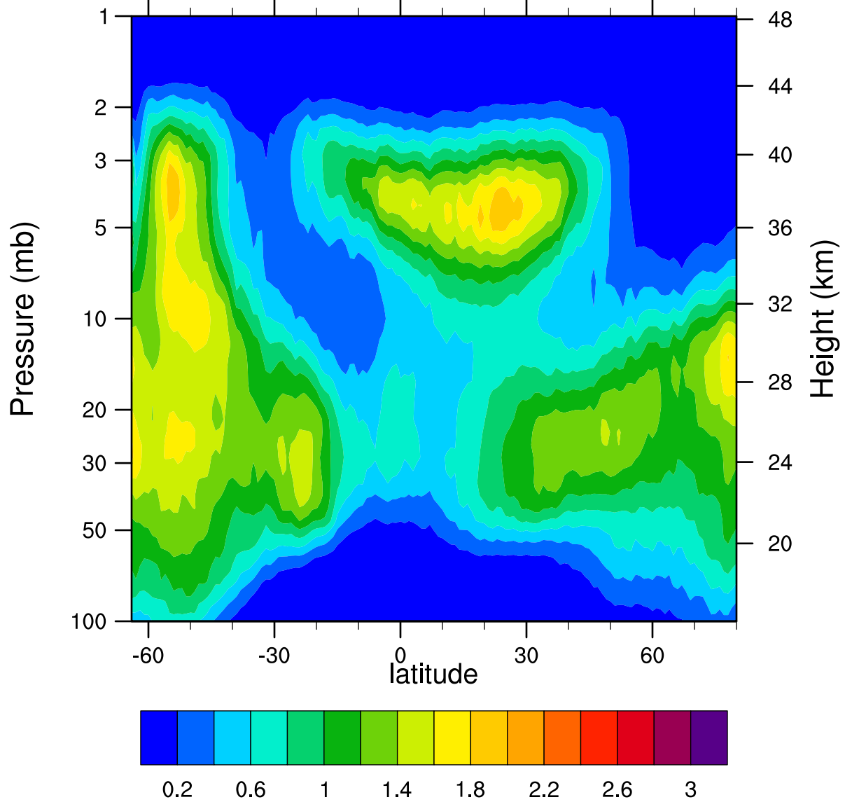
HIRDLSv6 2007d281 ClONO2_Ascending (ppbv)
