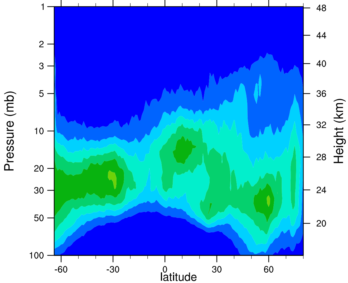
HIRDLSv6 2005d356 ClONO2_Ascending (ppbv)
