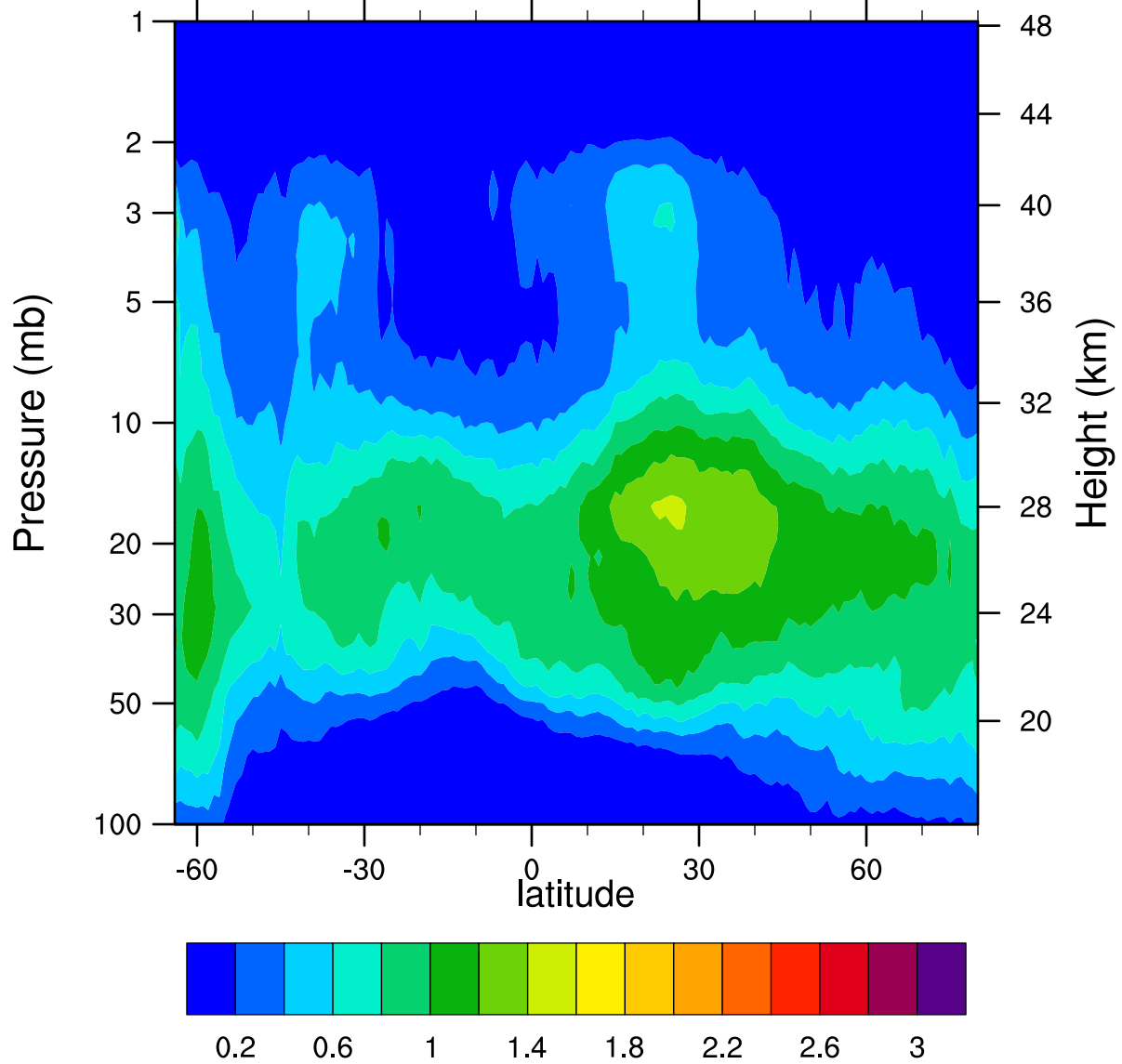
HIRDLSv6 2006d136 ClONO2_Ascending (ppbv)
