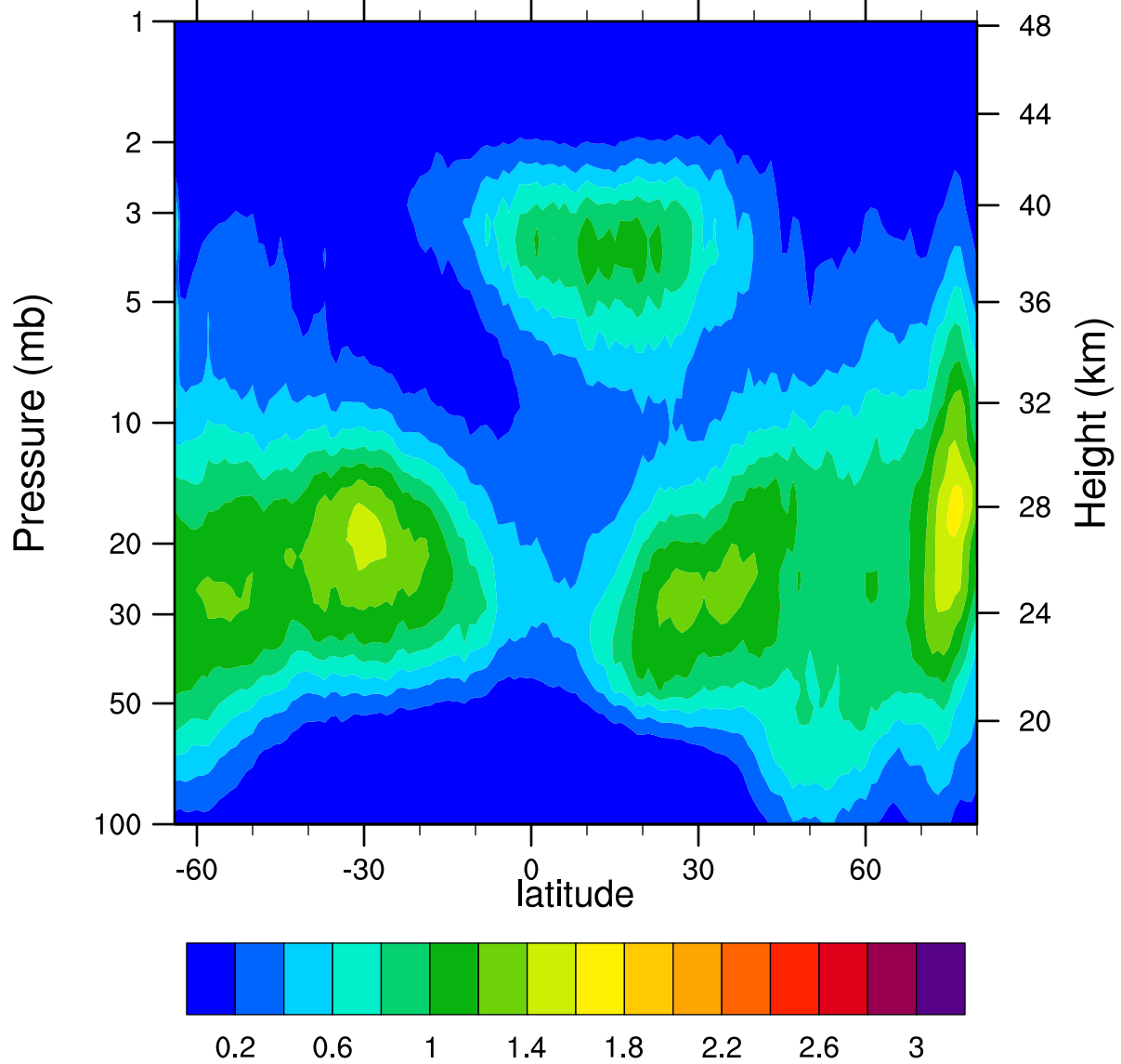
HIRDLSv6 2006d365 ClONO2_Ascending (ppbv)
