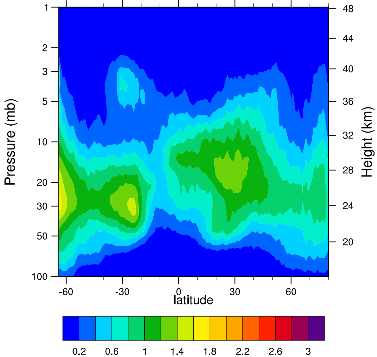
HIRDLSv6 2005d294 ClONO2_Ascending (ppbv)
