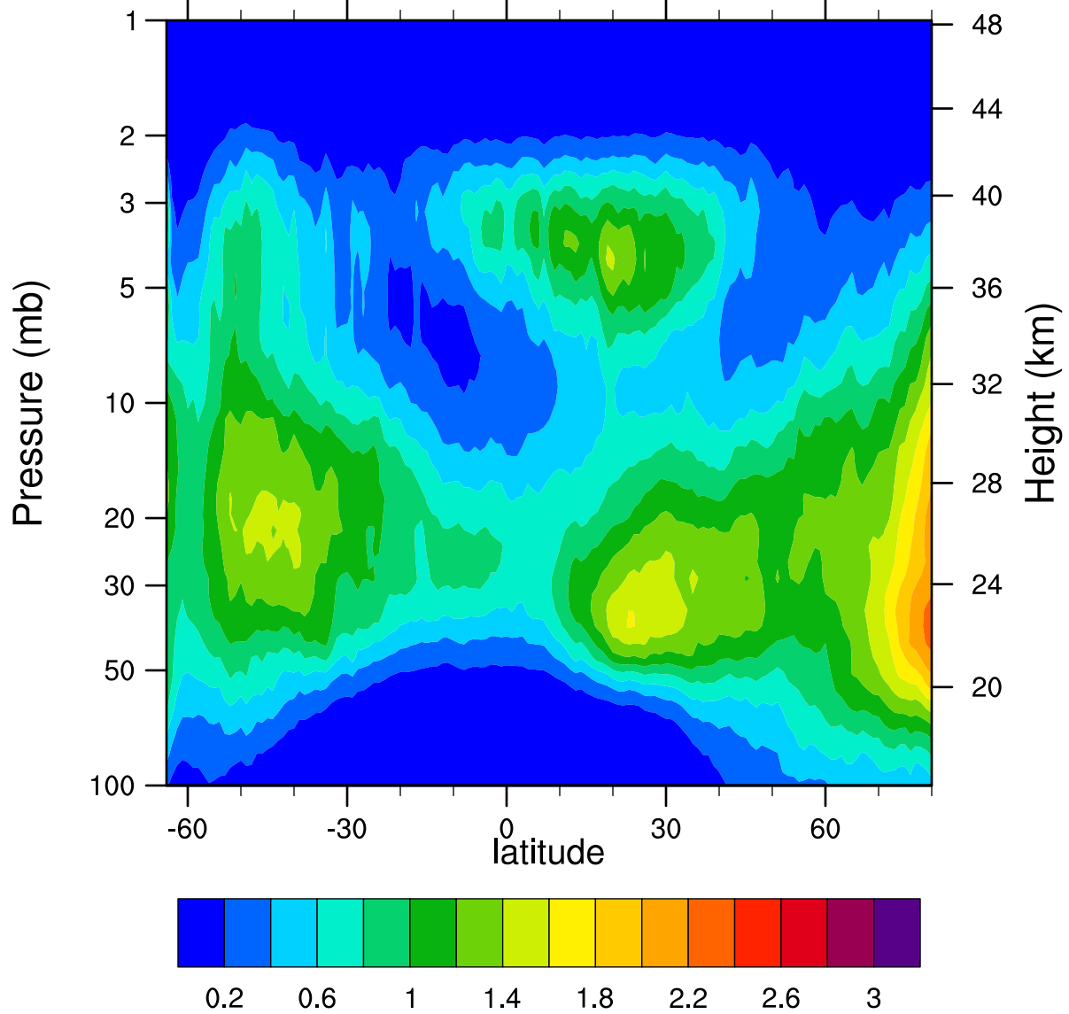
HIRDLSv6 2007d077 ClONO2_Ascending (ppbv)
