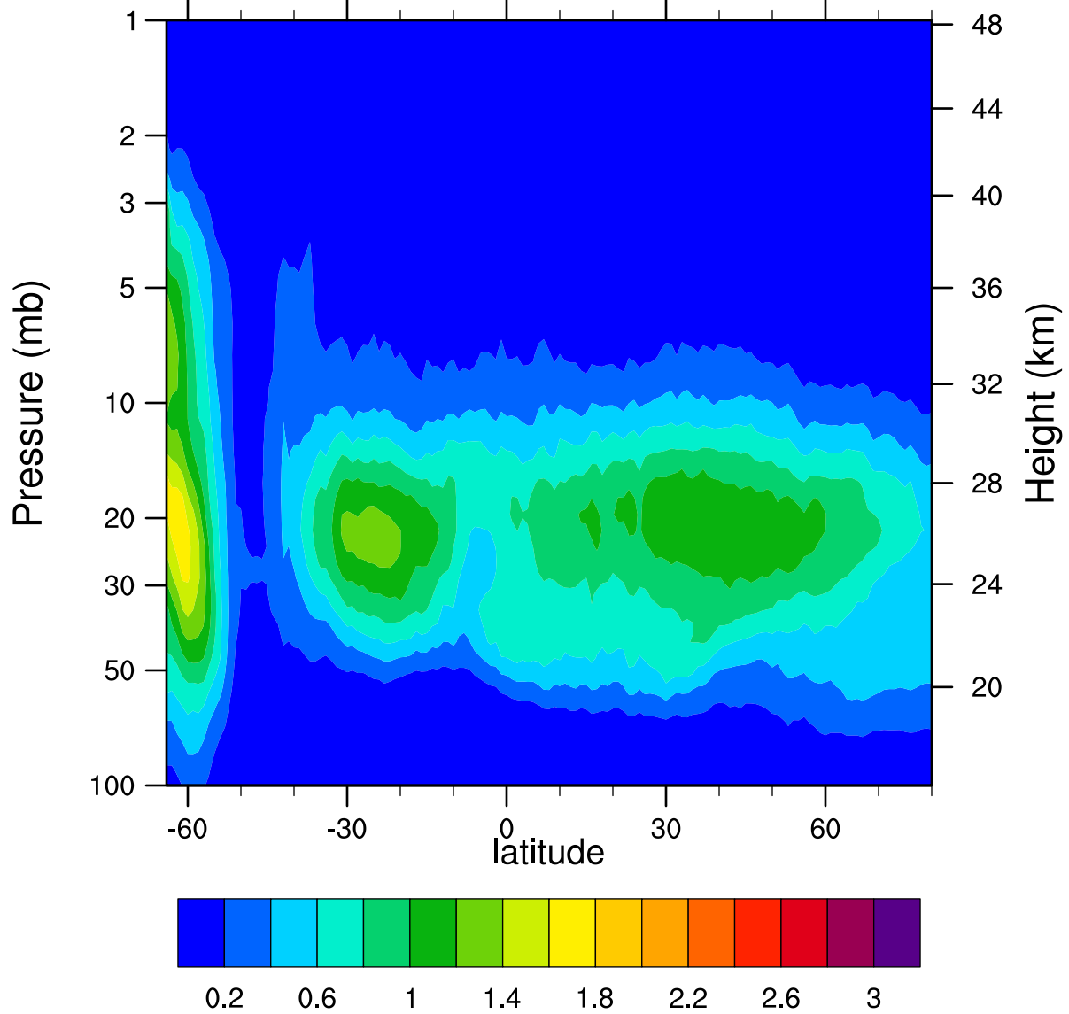
HIRDLSv6 2006d207 ClONO2_Ascending (ppbv)
