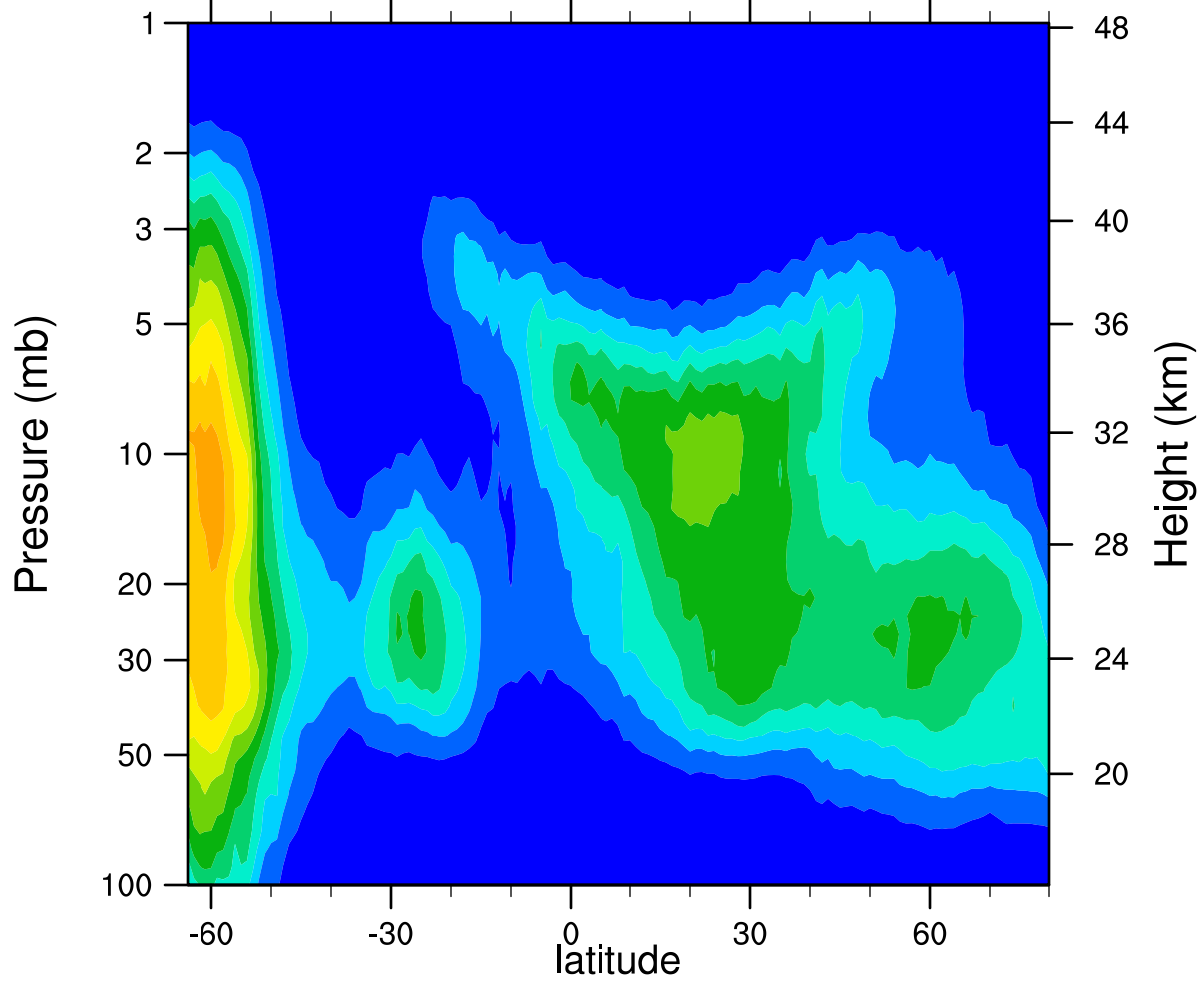
HIRDLSv6 2005d155 ClONO2_Ascending (ppbv)
