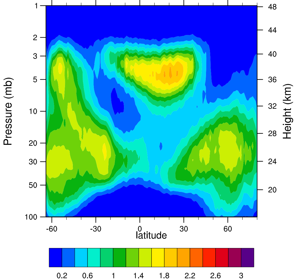
HIRDLSv6 2007d328 ClONO2_Ascending (ppbv)
