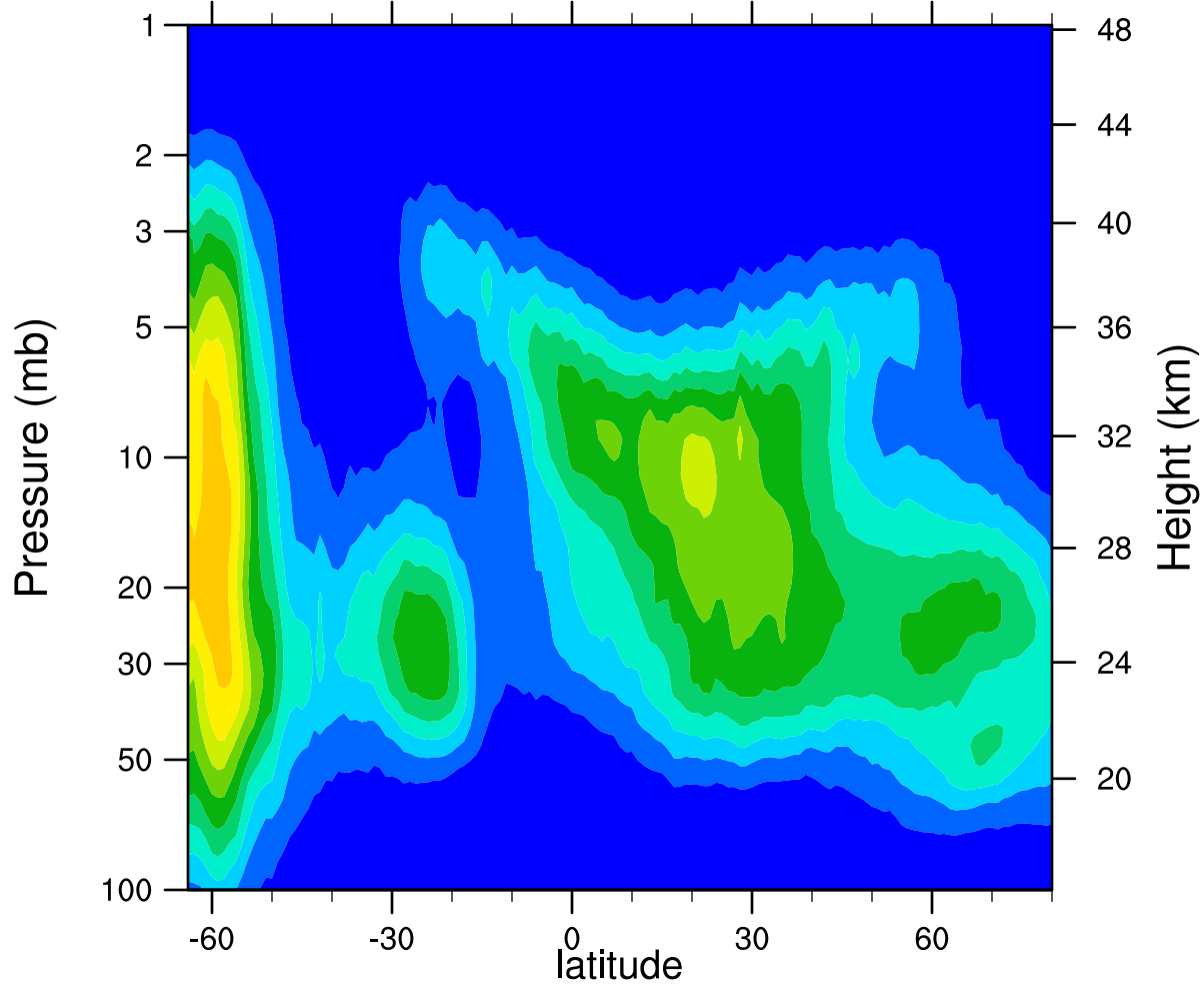
HIRDLSv6 2005d179 ClONO2_Ascending (ppbv)
