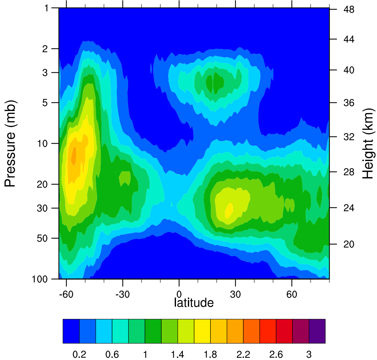
HIRDLSv6 2007d124 ClONO2_Ascending (ppbv)
