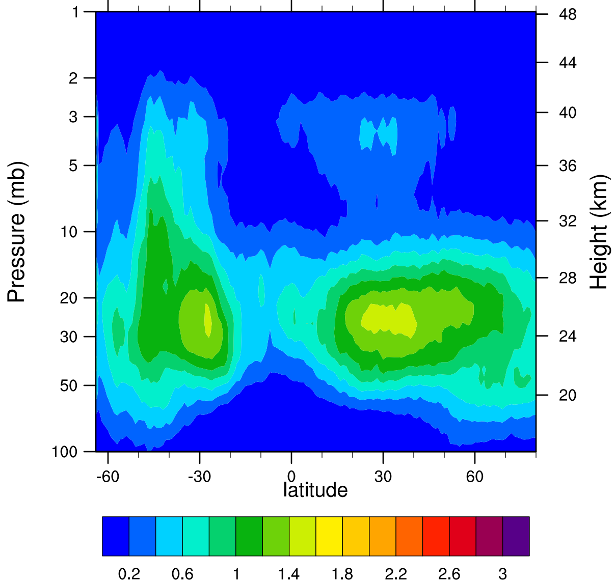
HIRDLSv6 2007d178 ClONO2_Ascending (ppbv)
