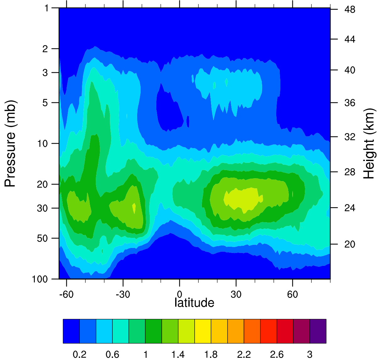
HIRDLSv6 2007d194 ClONO2_Ascending (ppbv)
