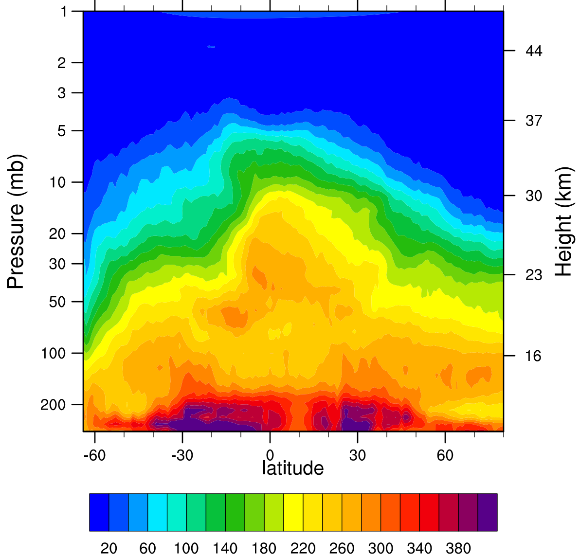
HIRDLSv6 2006d272 N2O_Combined (ppbv)
