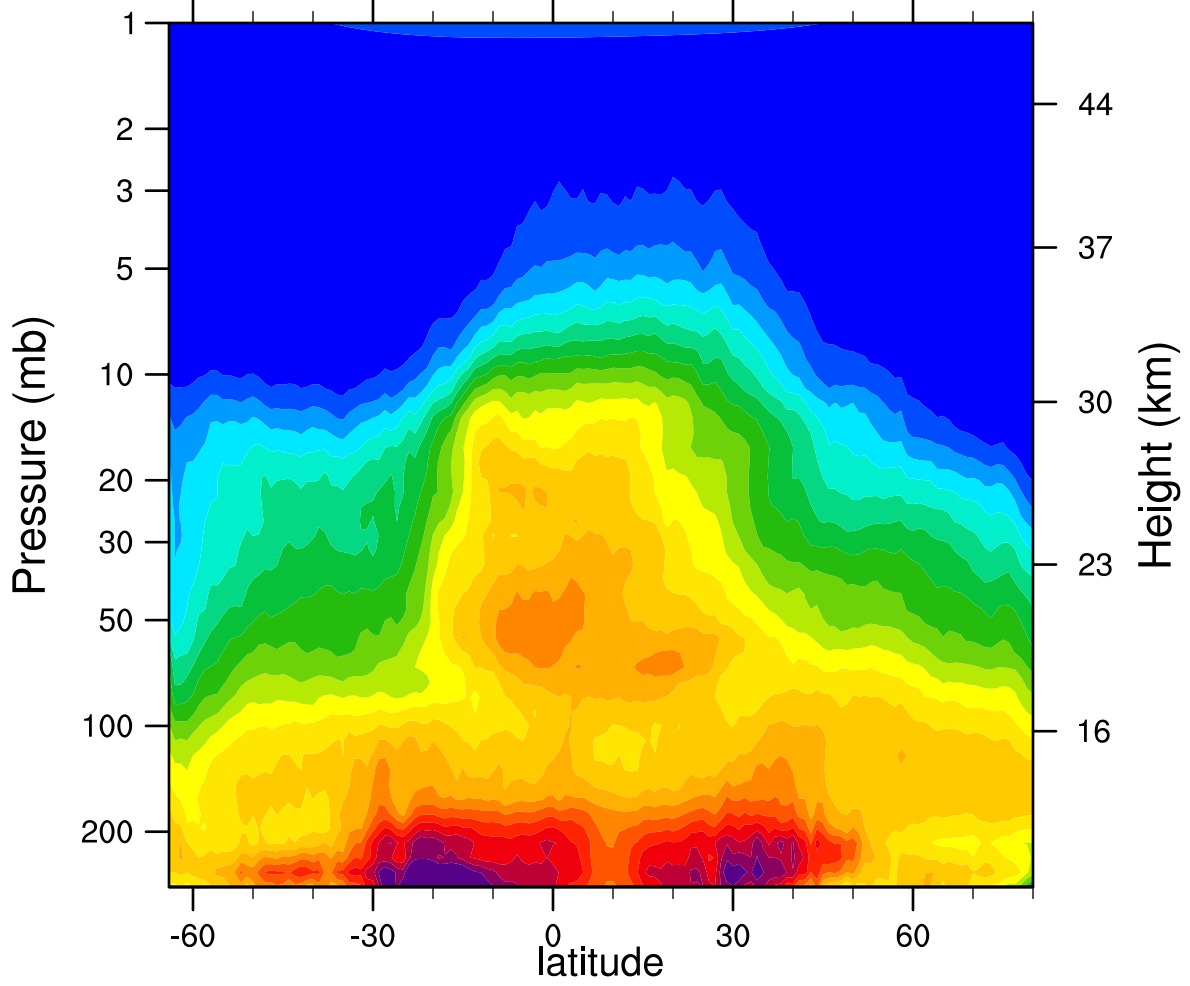
HIRDLSv6 2007d262 N2O_Combined (ppbv)
