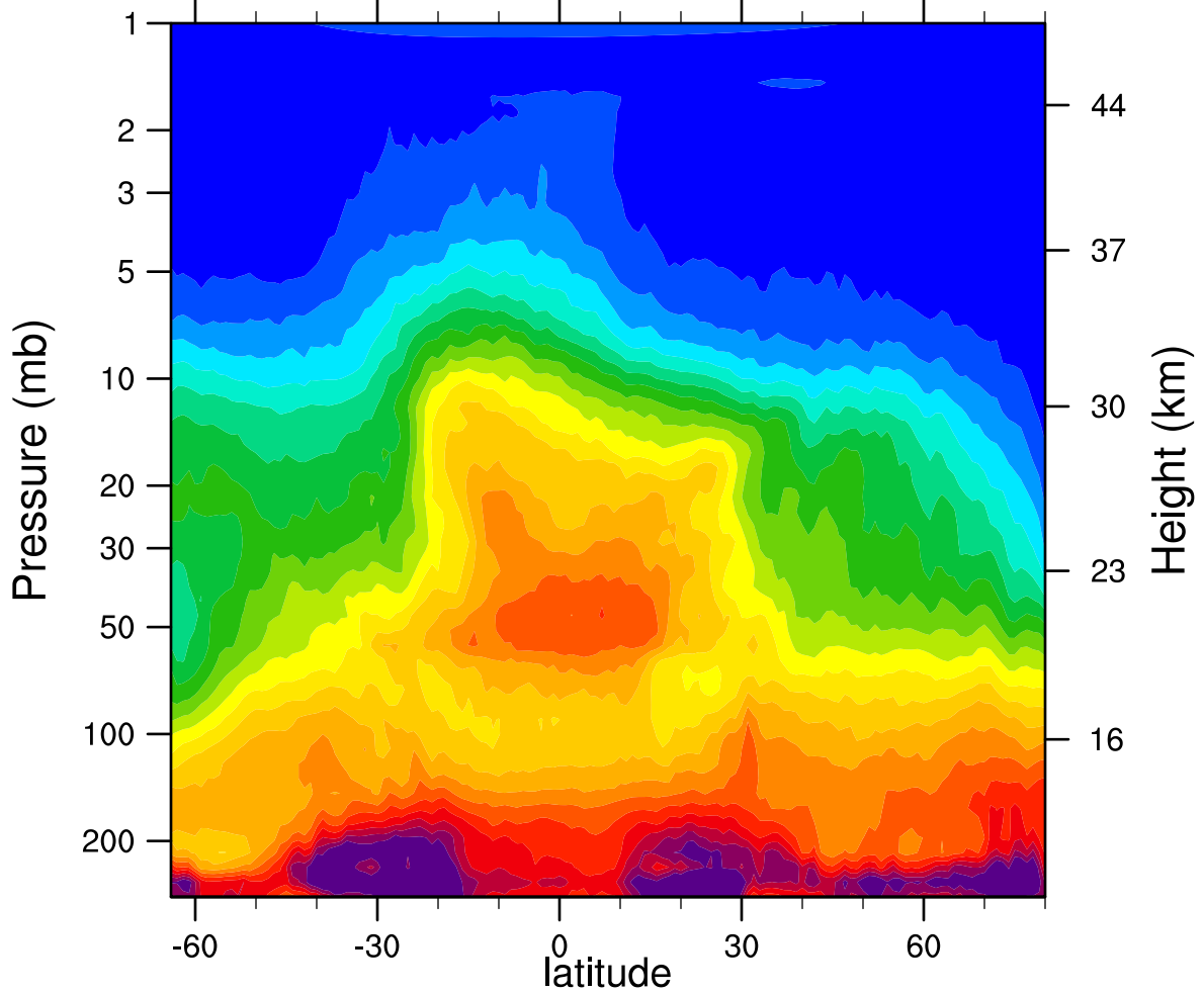
HIRDLSv6 2005d341 N2O_Combined (ppbv)
