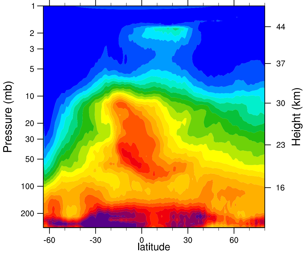
HIRDLSv6 2005d207 N2O_Combined (ppbv)
