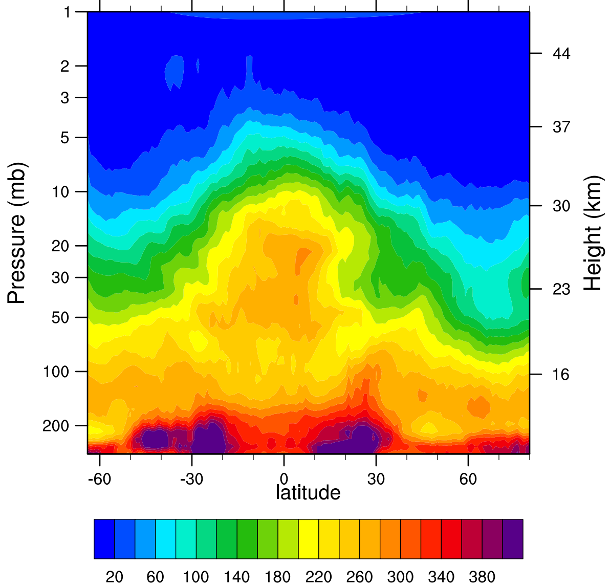
HIRDLSv6 2007d055 N2O_Combined (ppbv)
