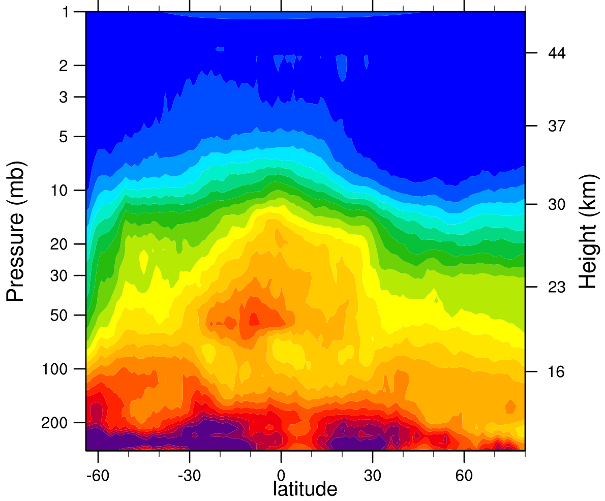
HIRDLSv6 2006d161 N2O_Combined (ppbv)
