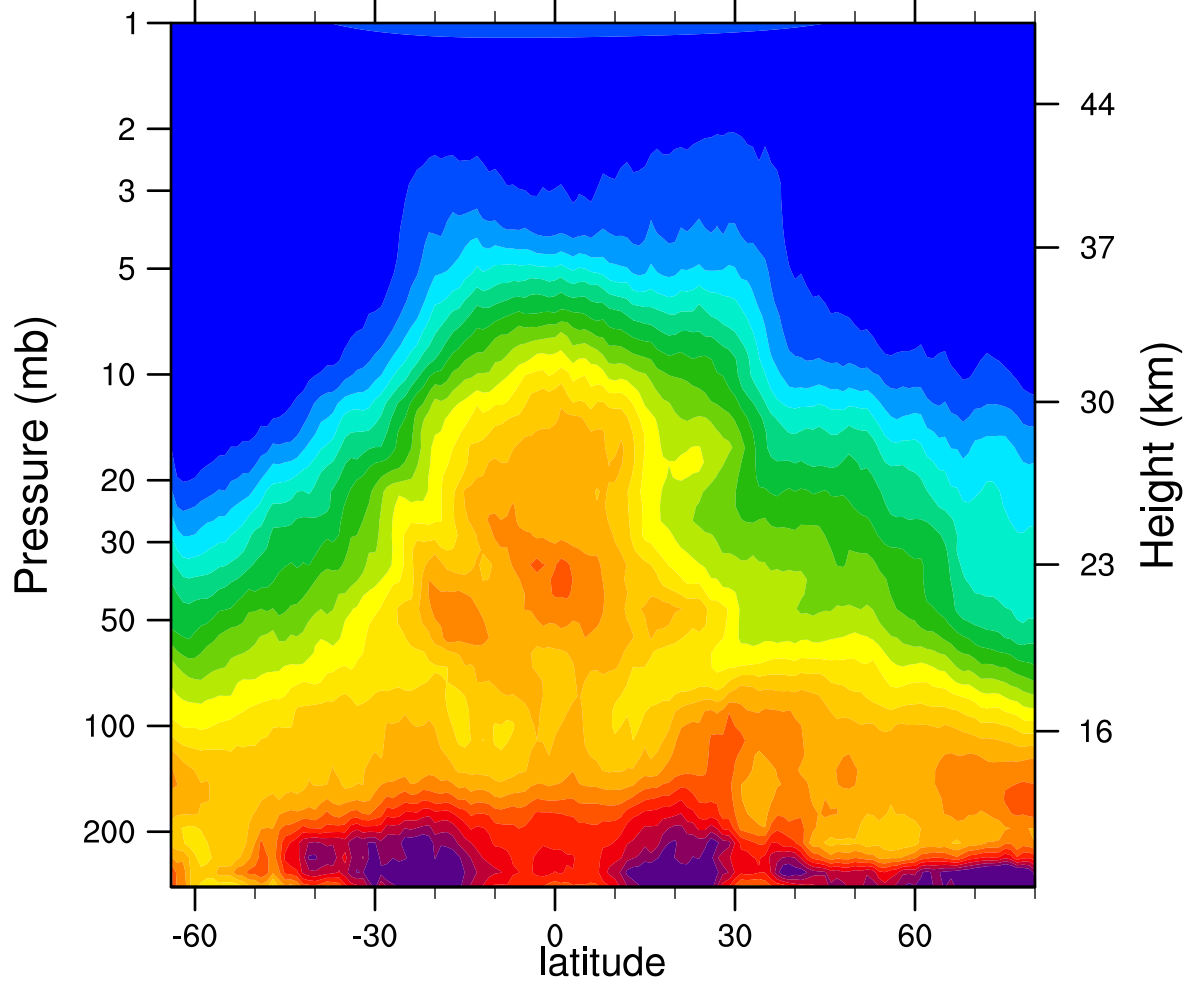
HIRDLSv6 2007d101 N2O_Combined (ppbv)
