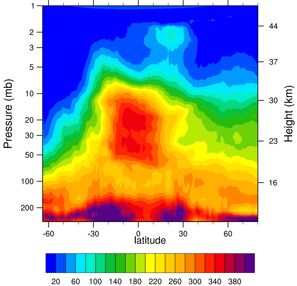
HIRDLSv6 2005d149 N2O_Combined (ppbv)
