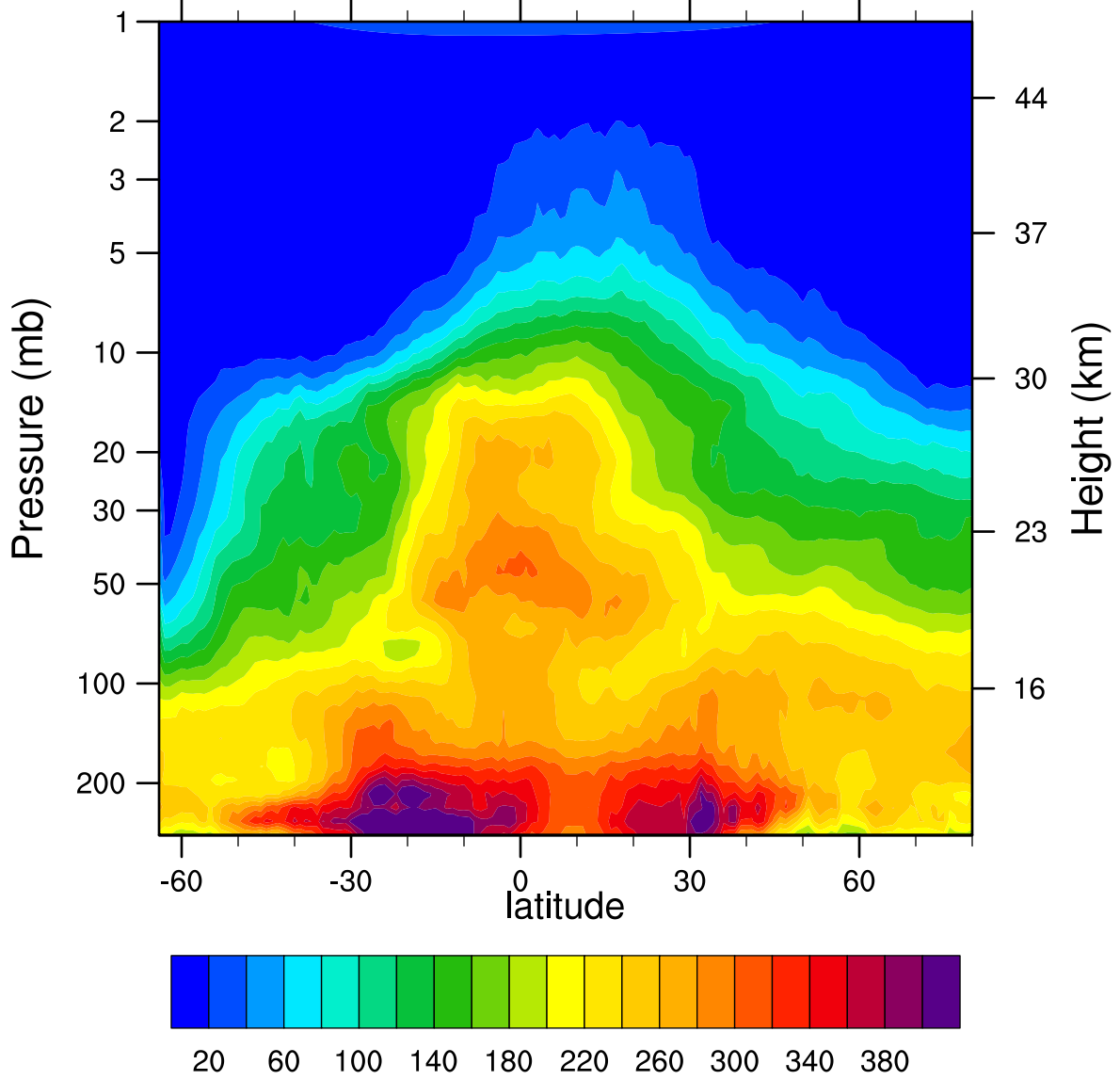
HIRDLSv6 2007d232 N2O_Combined (ppbv)
