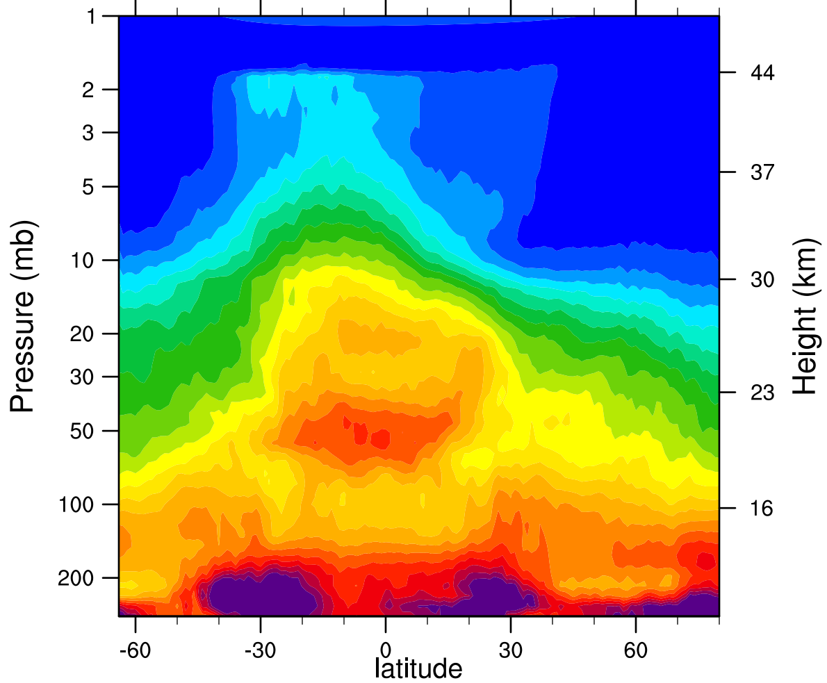
HIRDLSv6 2006d075 N2O_Combined (ppbv)
