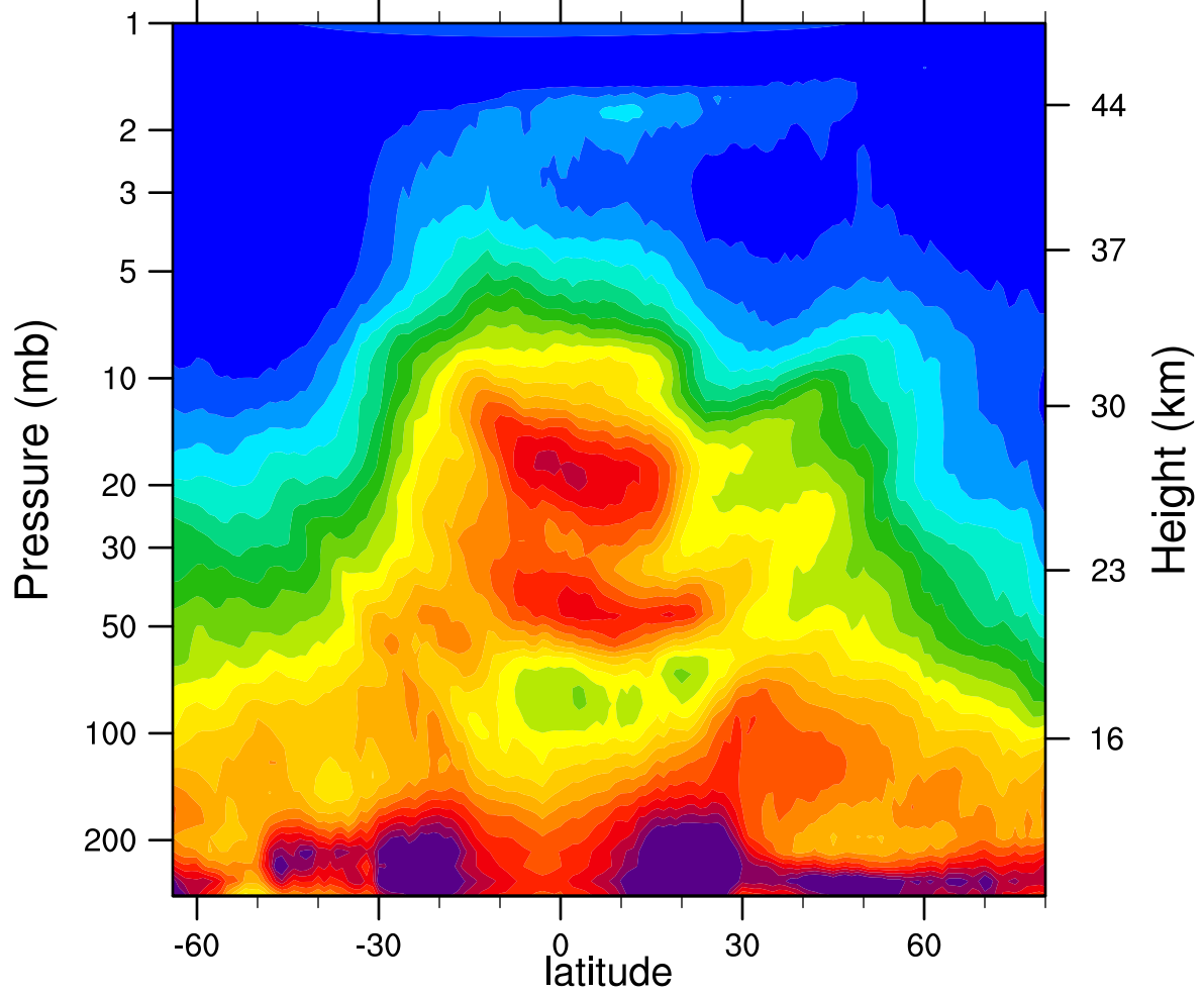
HIRDLSv6 2005d051 N2O_Combined (ppbv)
