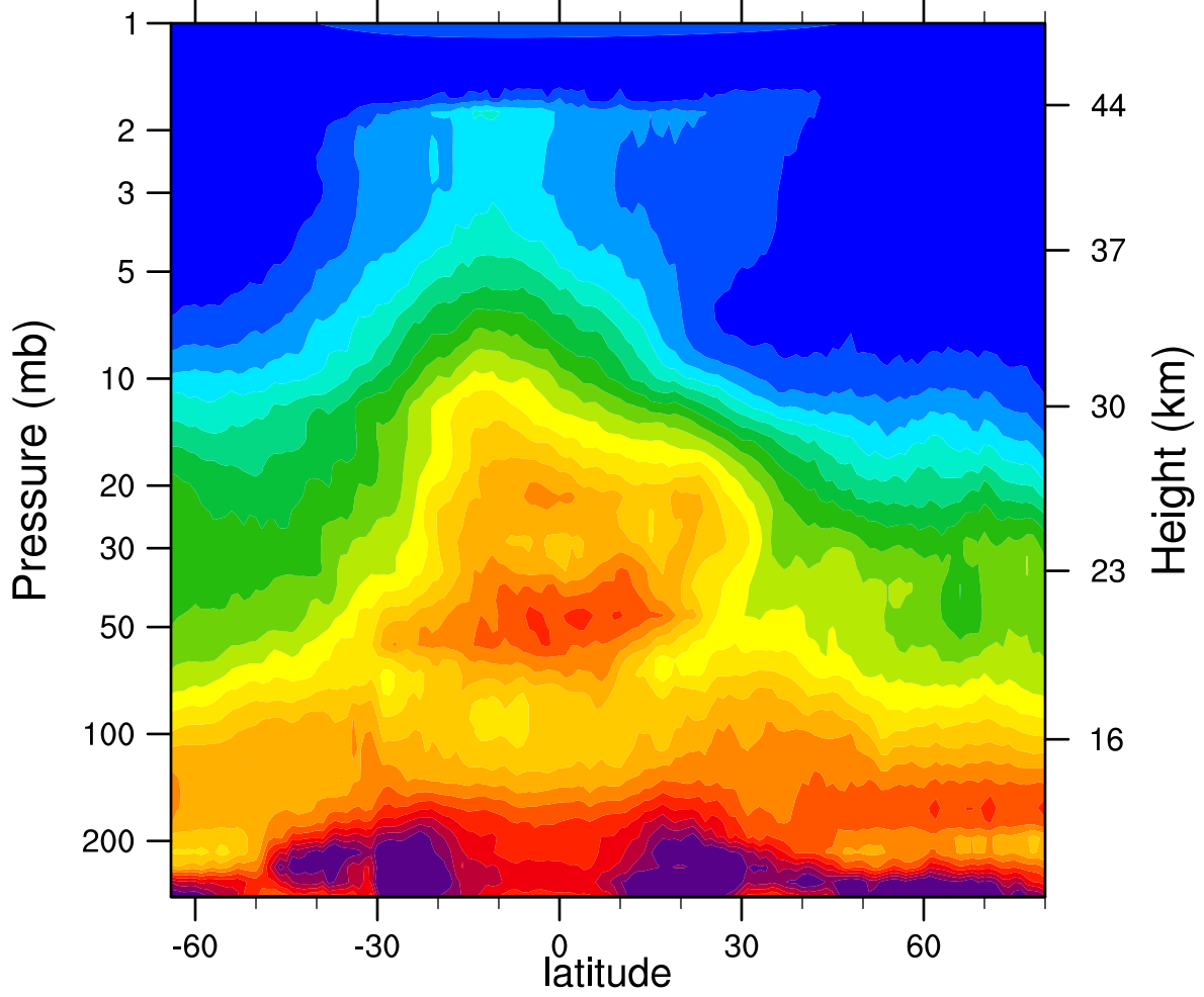
HIRDLSv6 2006d048 N2O_Combined (ppbv)
