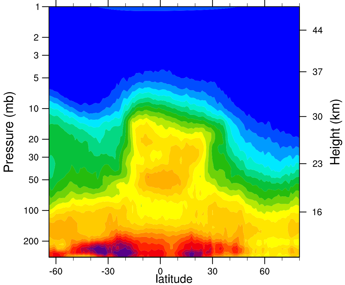
HIRDLSv6 2007d333 N2O_Combined (ppbv)
