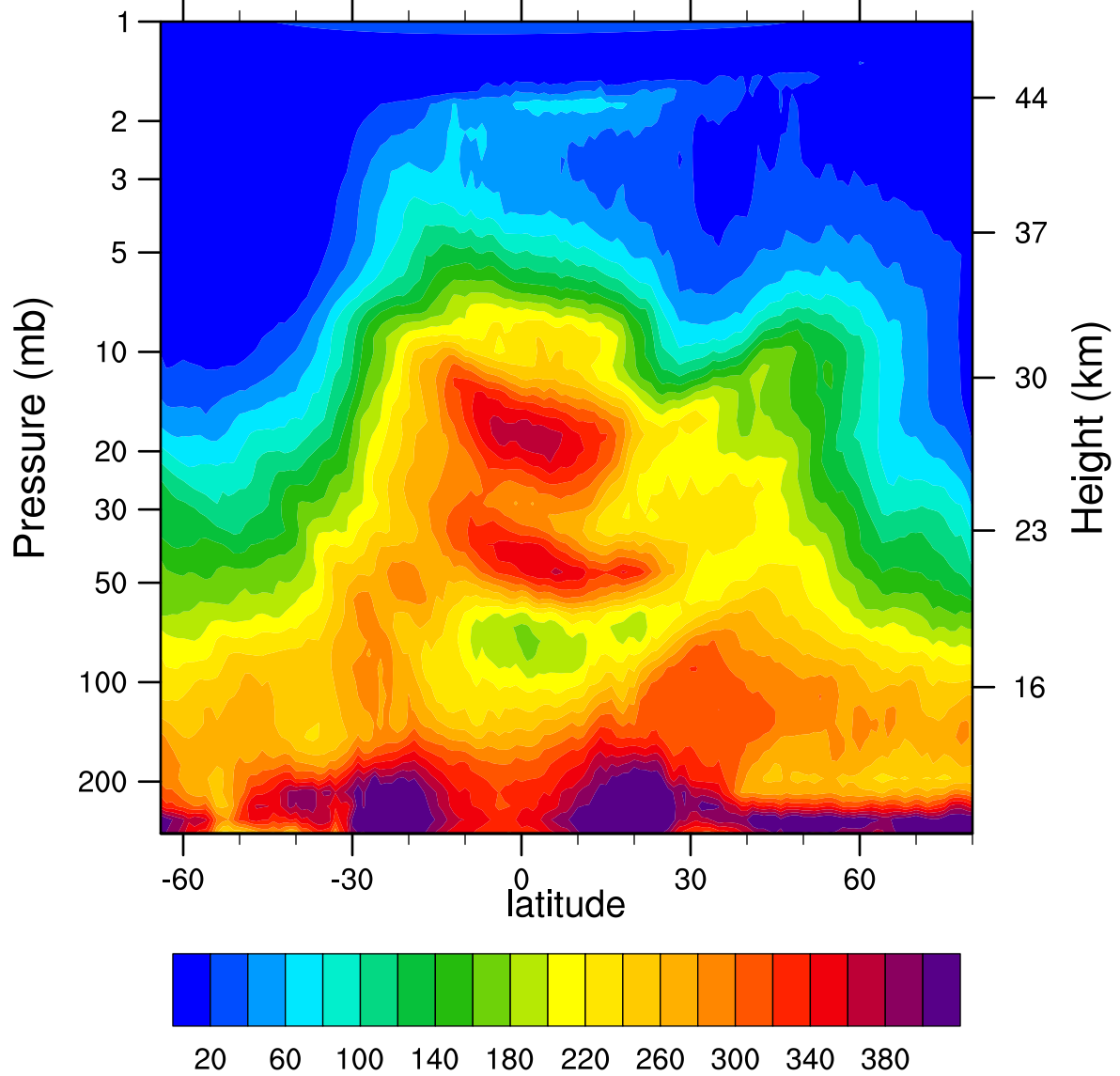
HIRDLSv6 2005d065 N2O_Combined (ppbv)
