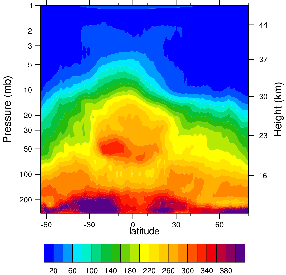
HIRDLSv6 2006d117 N2O_Combined (ppbv)
