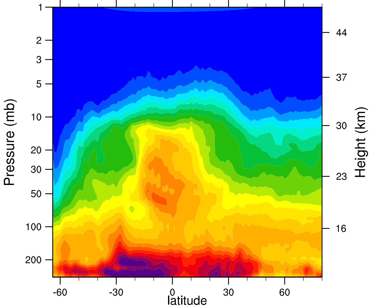
HIRDLSv6 2007d187 N2O_Combined (ppbv)
