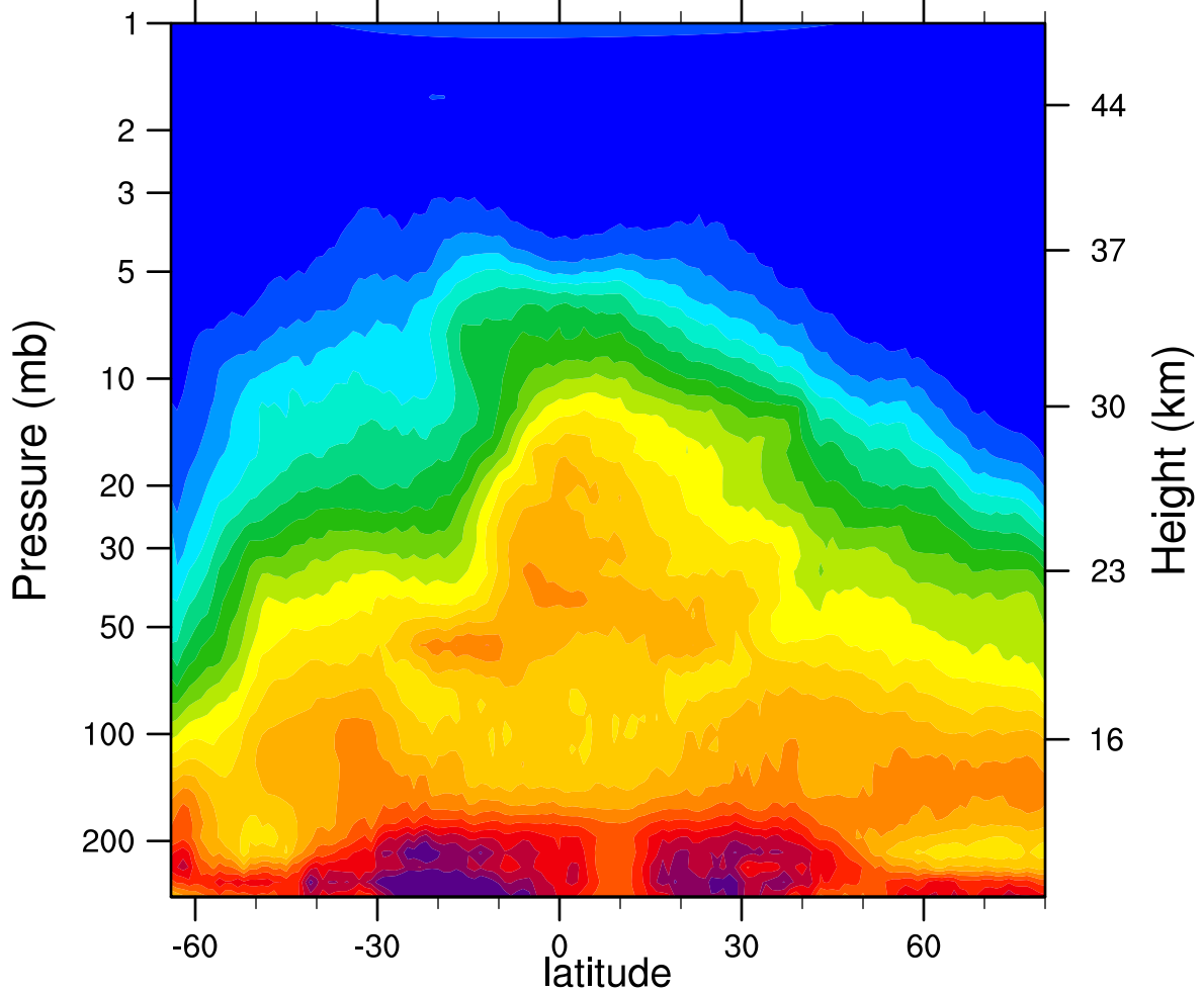
HIRDLSv6 2006d280 N2O_Combined (ppbv)
