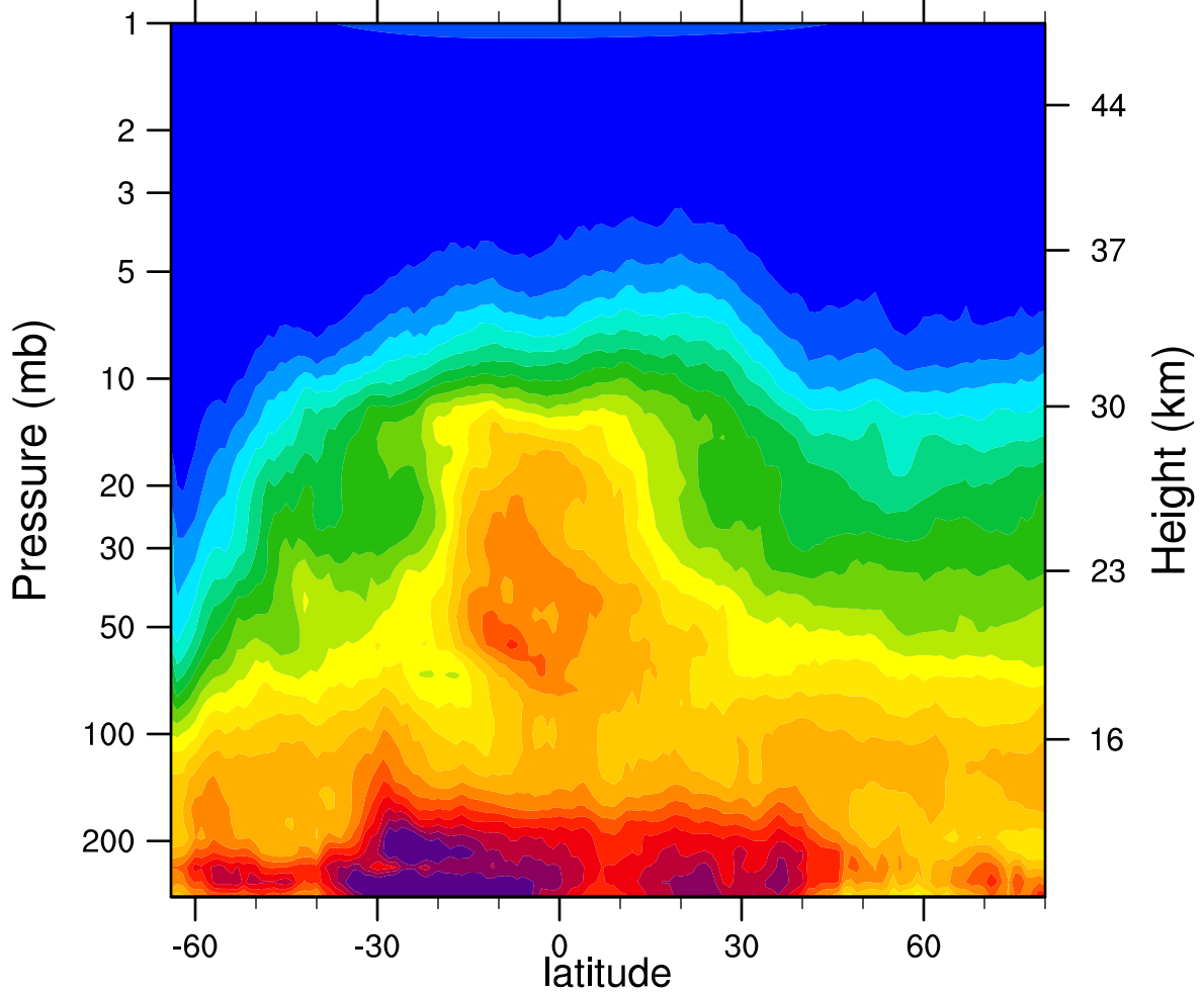
HIRDLSv6 2007d185 N2O_Combined (ppbv)
