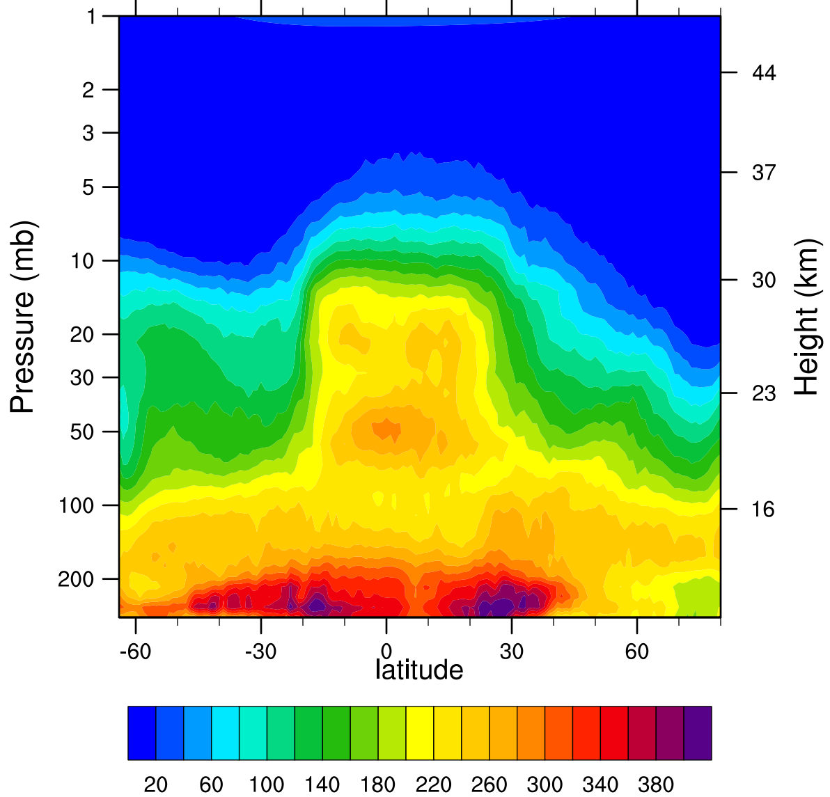
HIRDLSv6 2007d306 N2O_Combined (ppbv)
