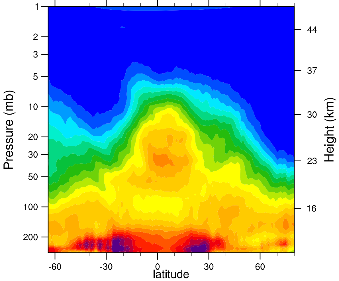
HIRDLSv6 2006d340 N2O_Combined (ppbv)
