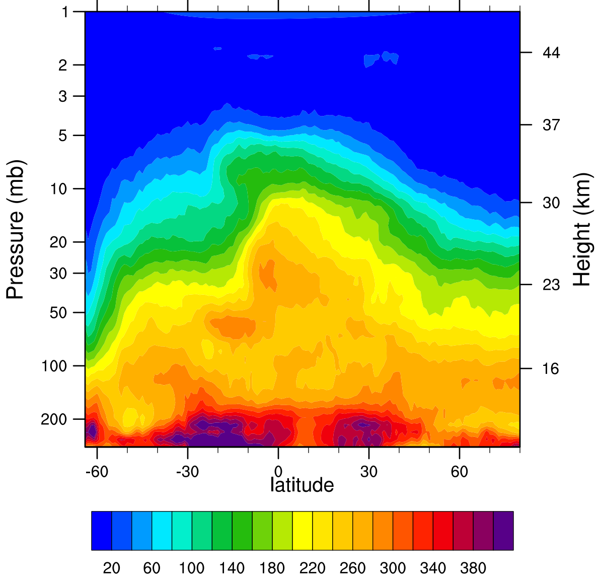
HIRDLSv6 2006d262 N2O_Combined (ppbv)
