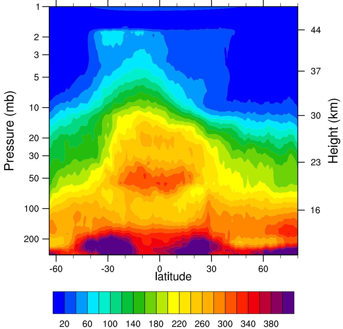
HIRDLSv6 2006d084 N2O_Combined (ppbv)
