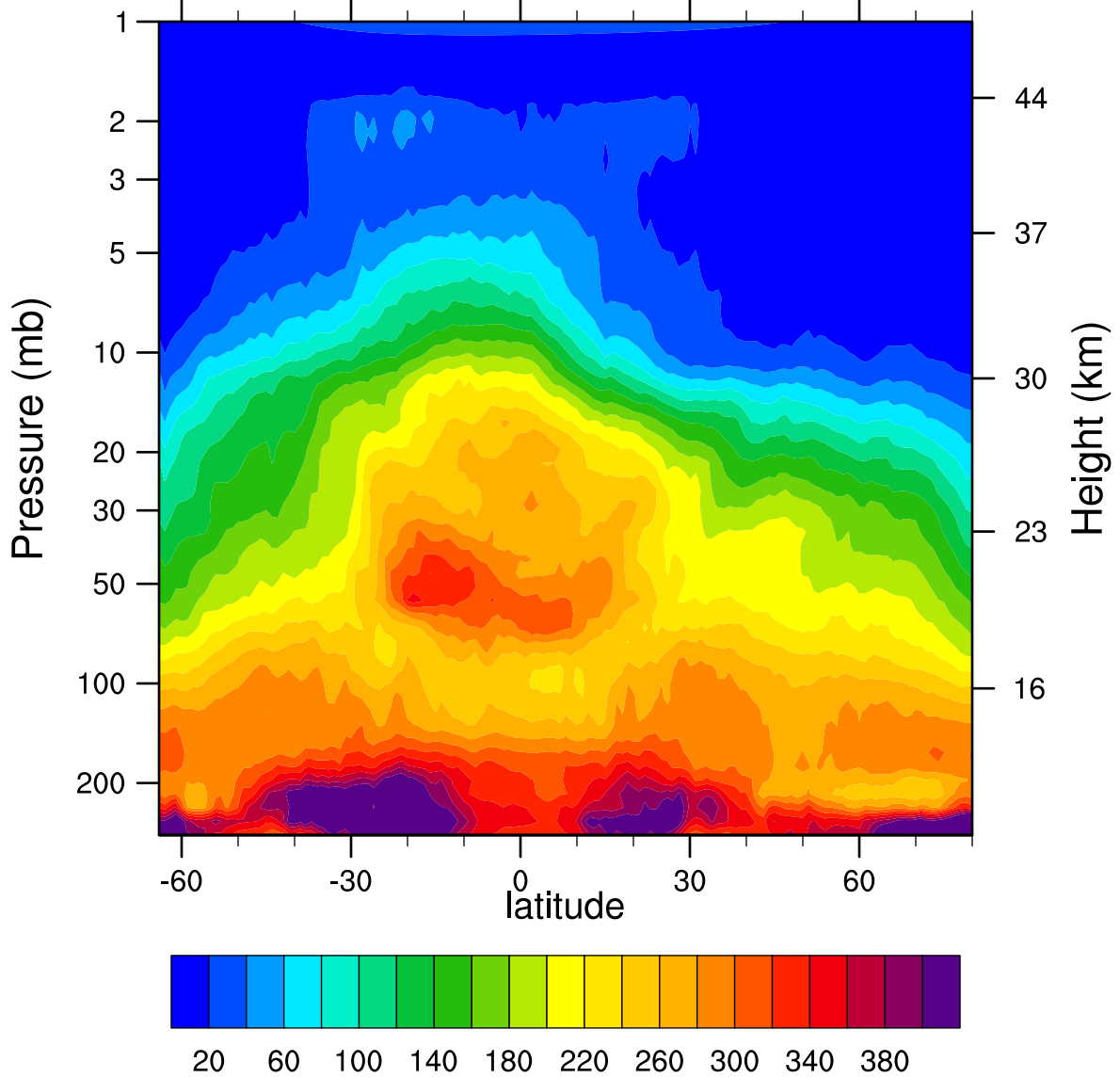
HIRDLSv6 2006d113 N2O_Combined (ppbv)
