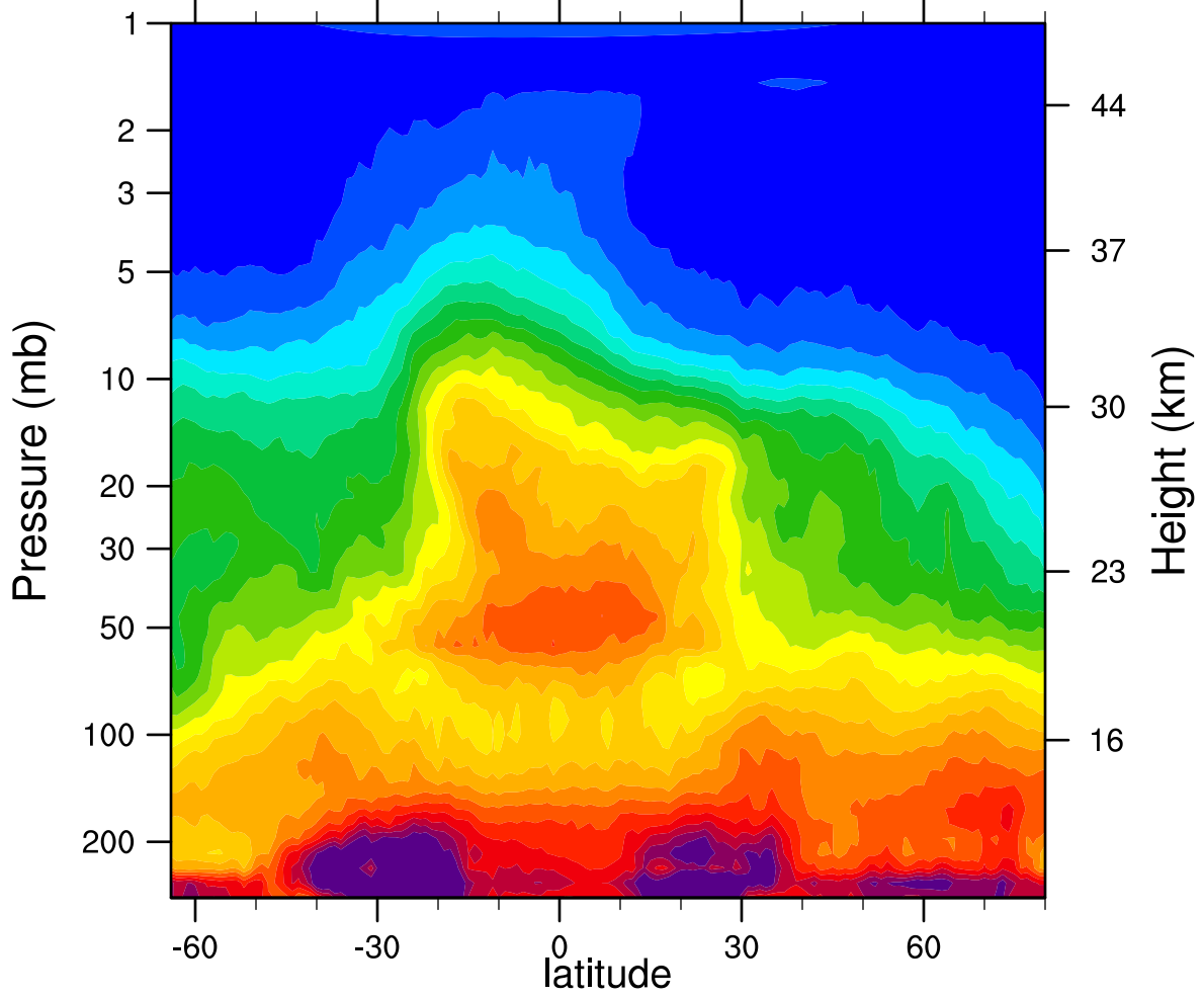
HIRDLSv6 2005d346 N2O_Combined (ppbv)
