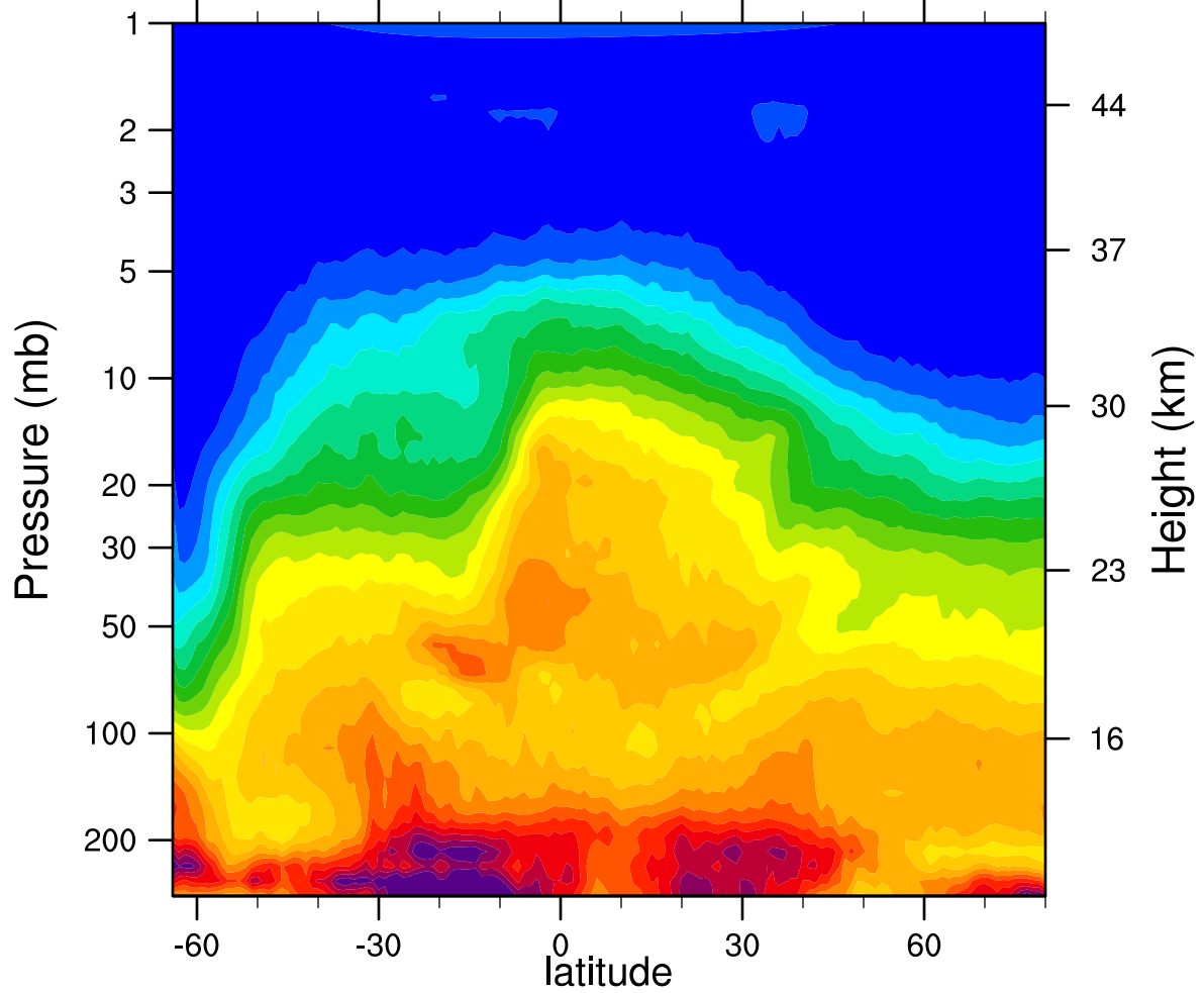
HIRDLSv6 2006d245 N2O_Combined (ppbv)
