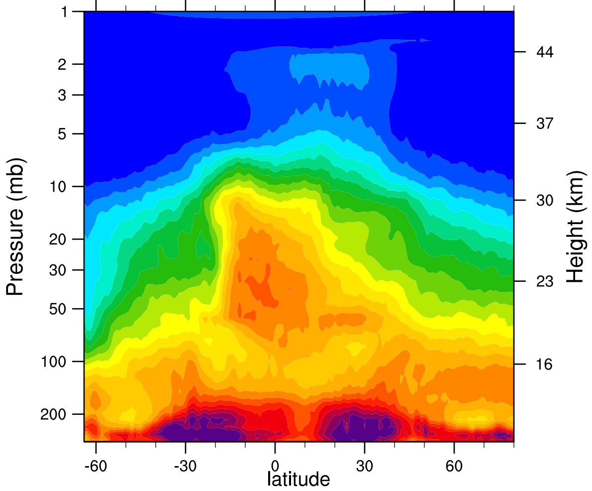
HIRDLSv6 2005d268 N2O_Combined (ppbv)
