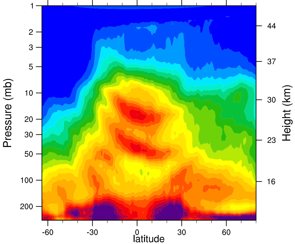
HIRDLSv6 2005d090 N2O_Combined (ppbv)
