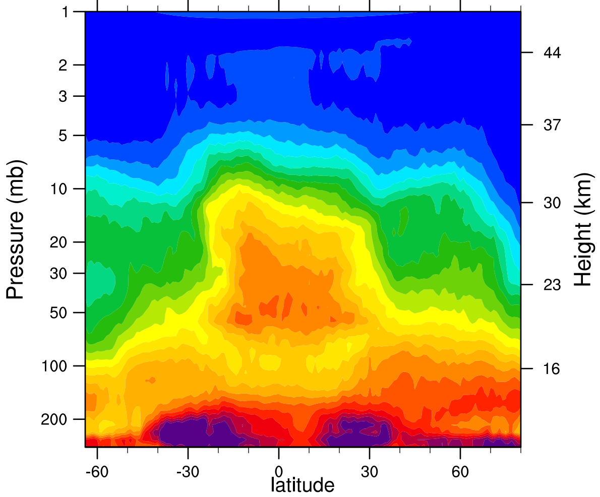
HIRDLSv6 2005d316 N2O_Combined (ppbv)
