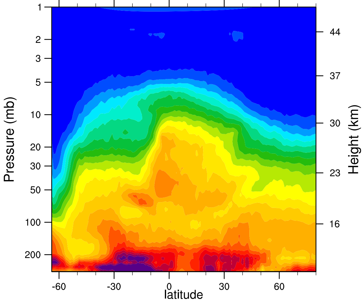
HIRDLSv6 2006d247 N2O_Combined (ppbv)
