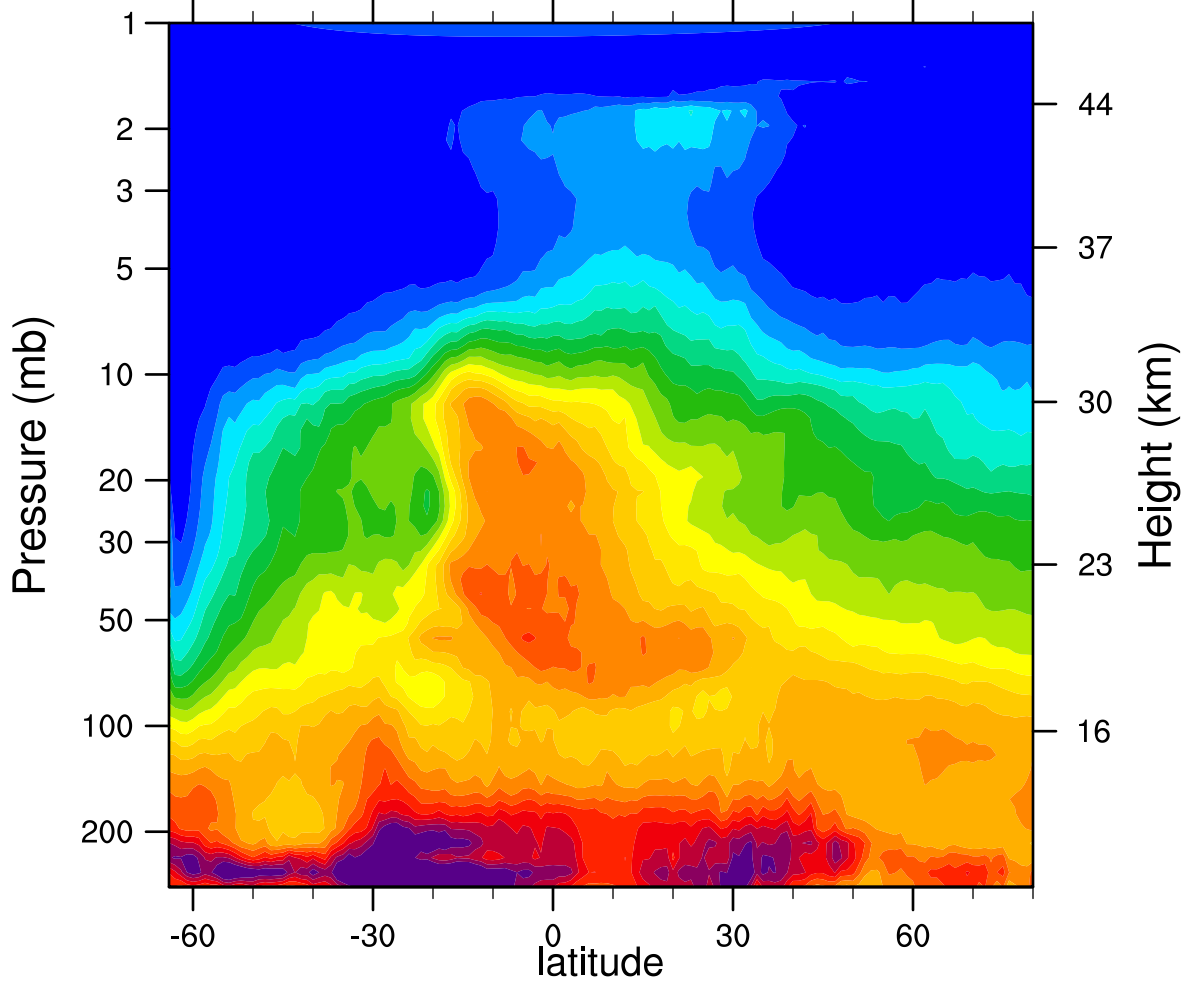
HIRDLSv6 2005d230 N2O_Combined (ppbv)
