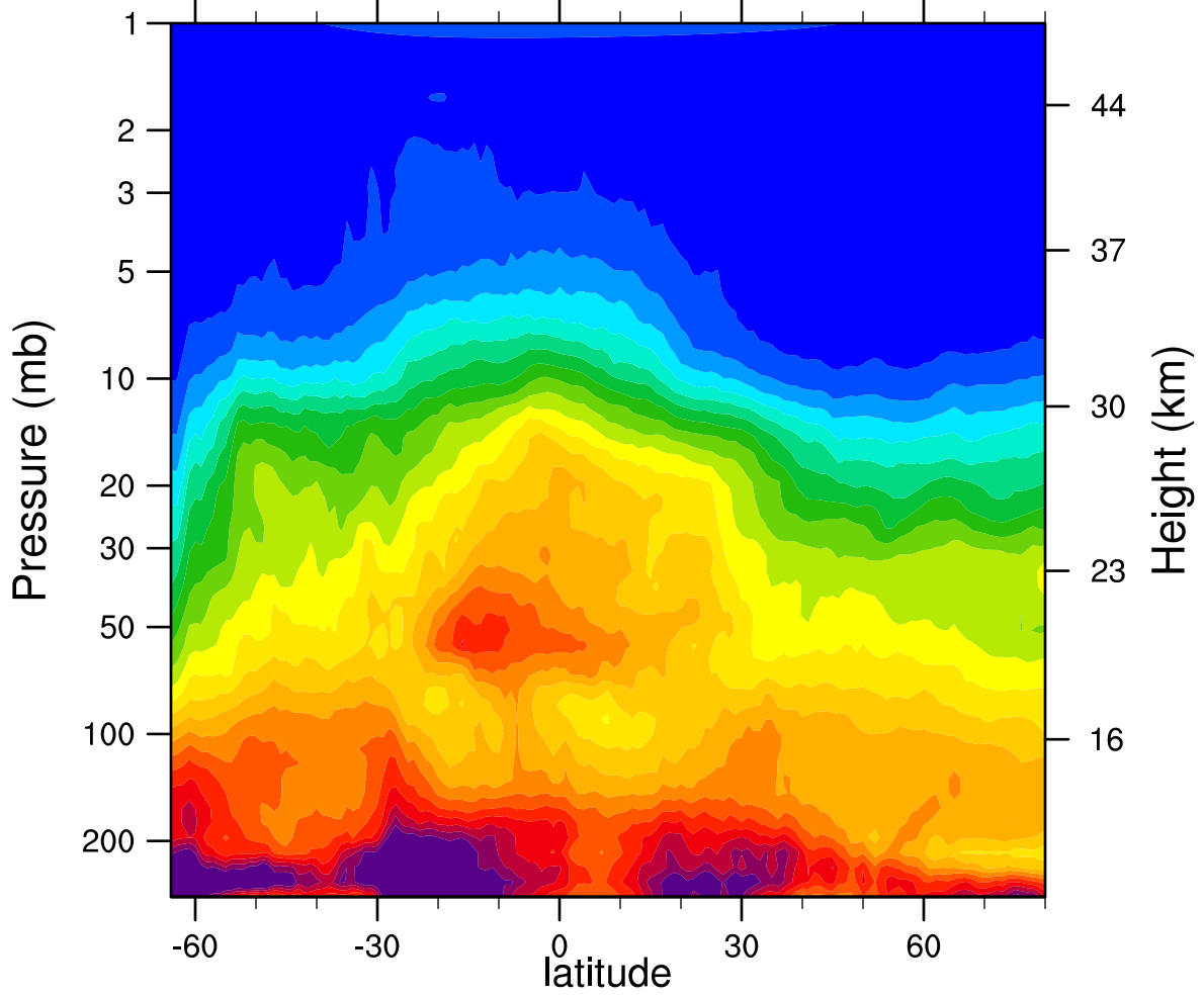
HIRDLSv6 2006d153 N2O_Combined (ppbv)
