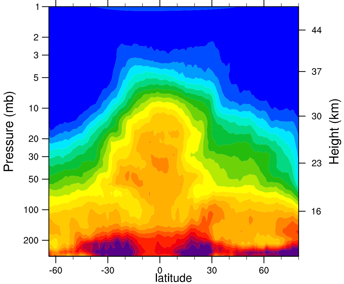
HIRDLSv6 2007d089 N2O_Combined (ppbv)
