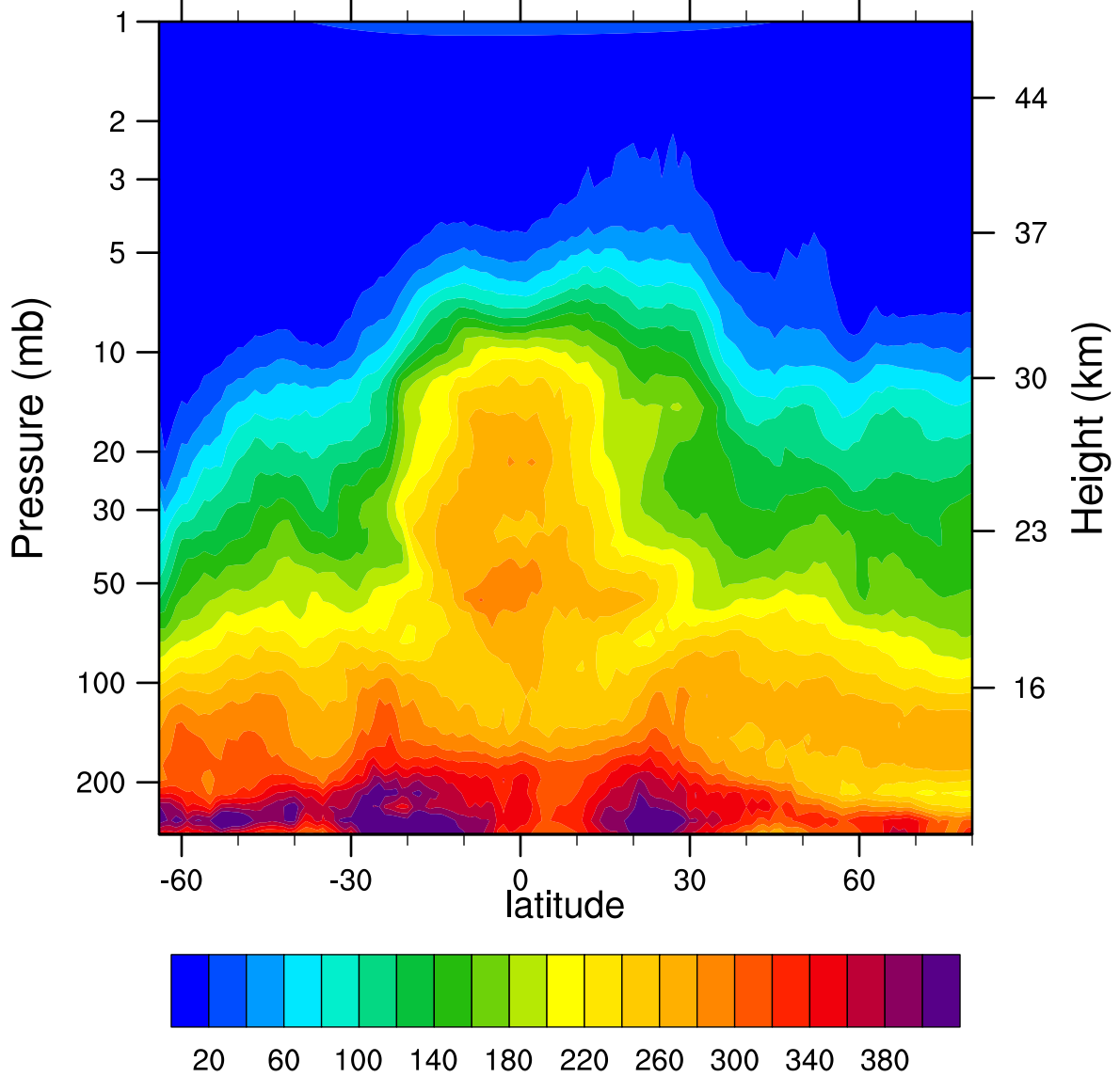
HIRDLSv6 2007d147 N2O_Combined (ppbv)
