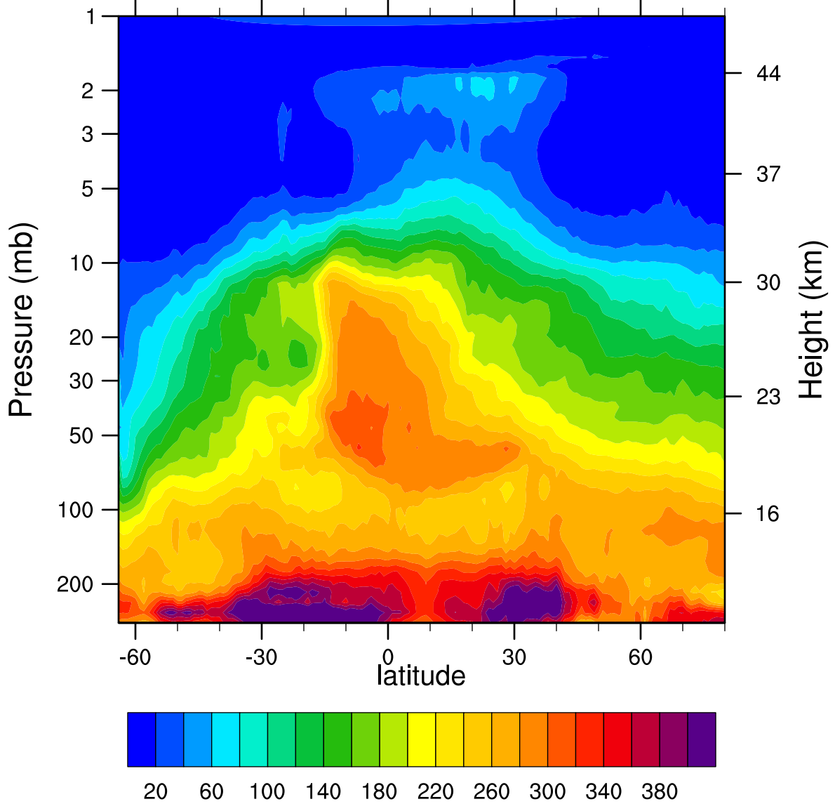
HIRDLSv6 2005d245 N2O_Combined (ppbv)
