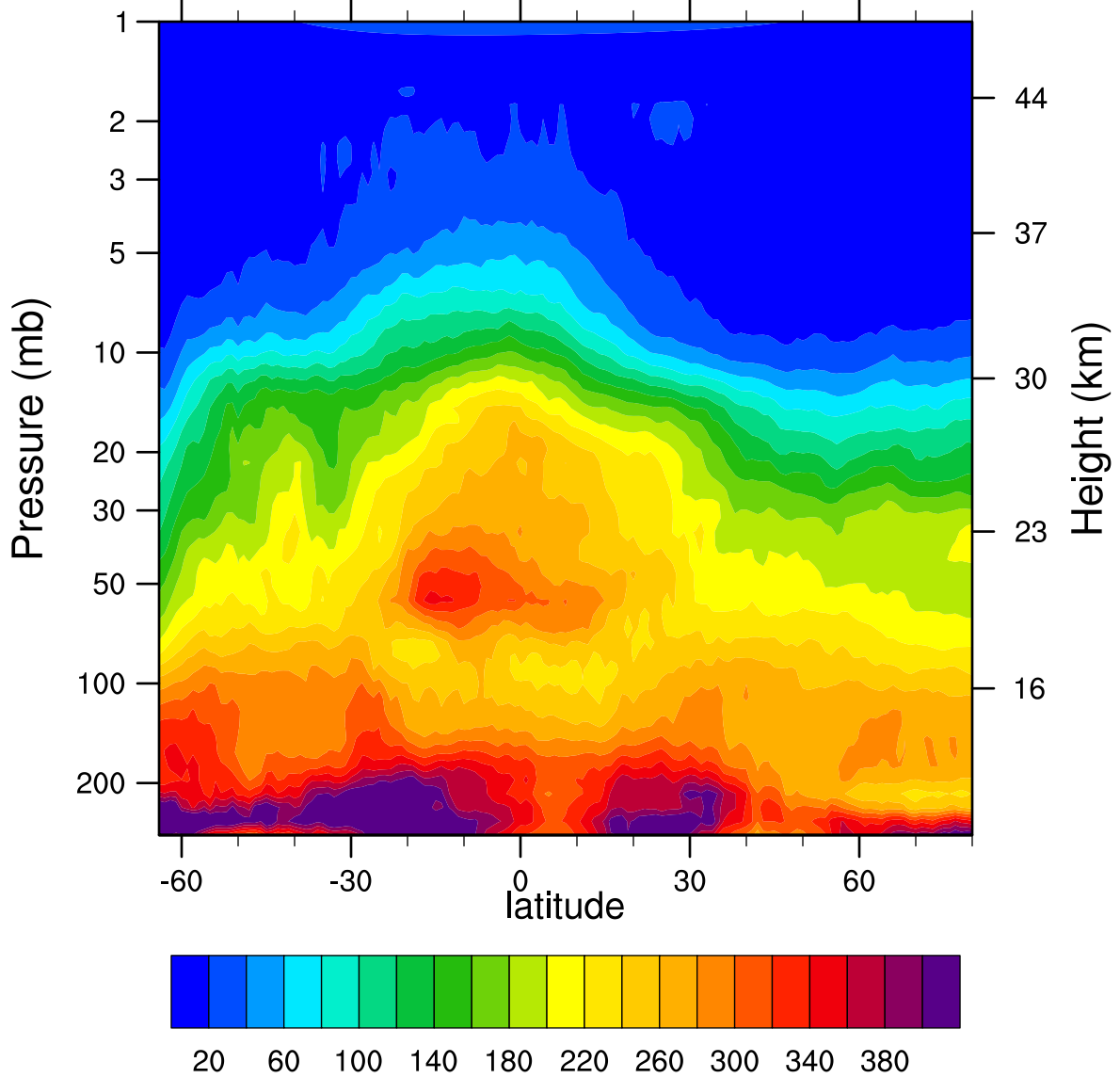
HIRDLSv6 2006d146 N2O_Combined (ppbv)
