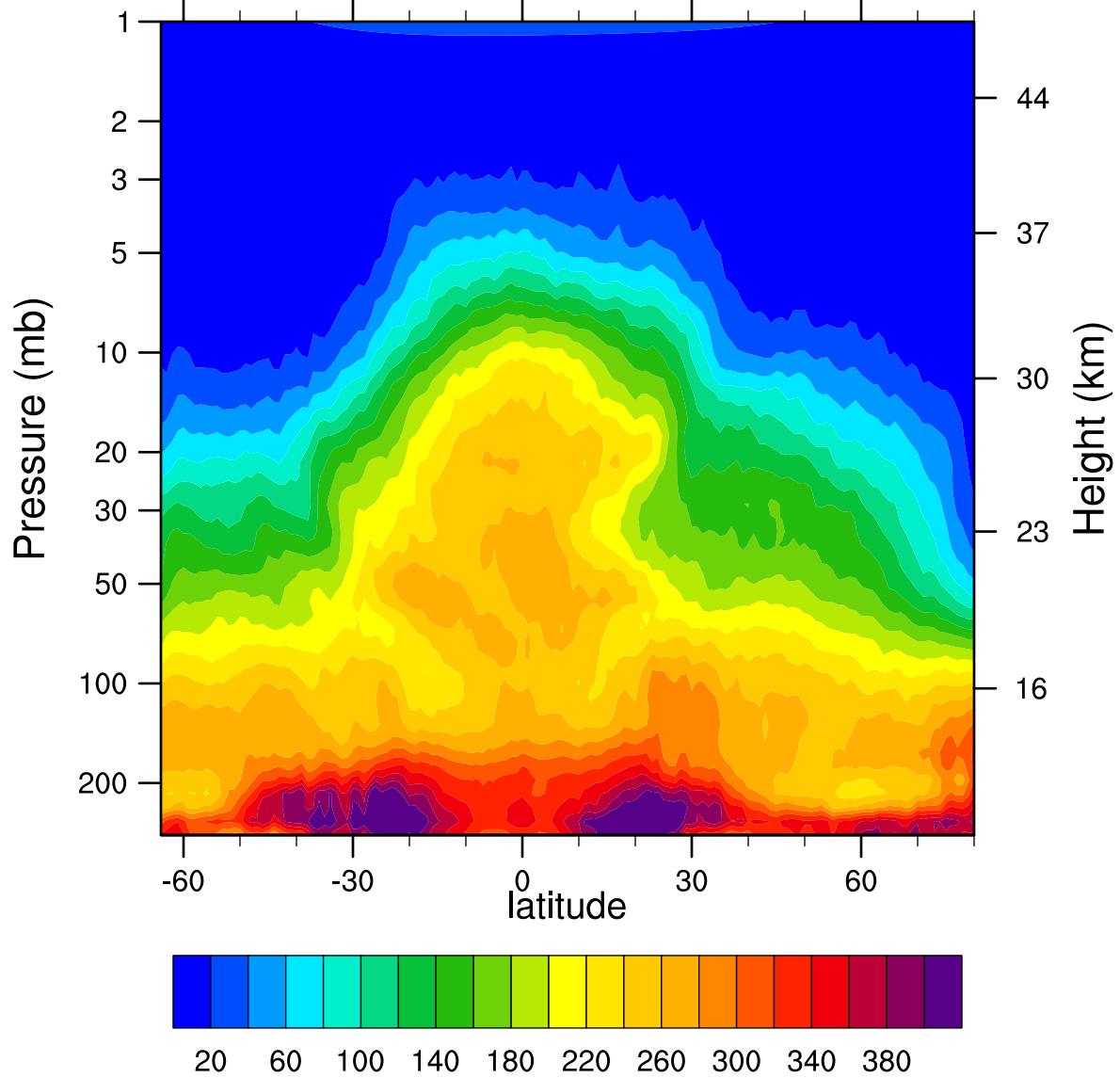
HIRDLSv6 2007d077 N2O_Combined (ppbv)
