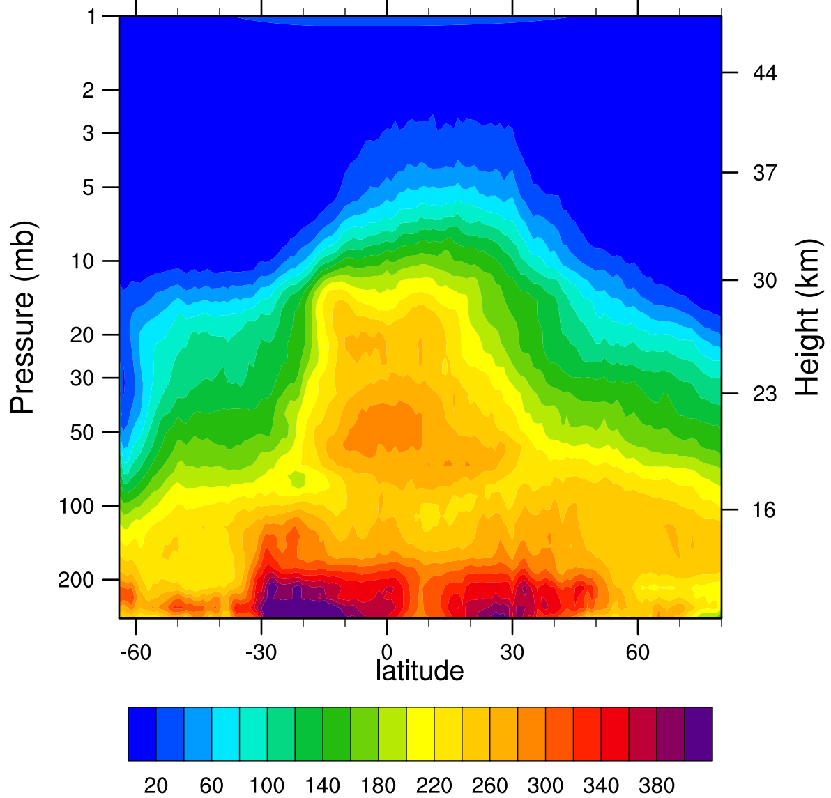
HIRDLSv6 2007d253 N2O_Combined (ppbv)
