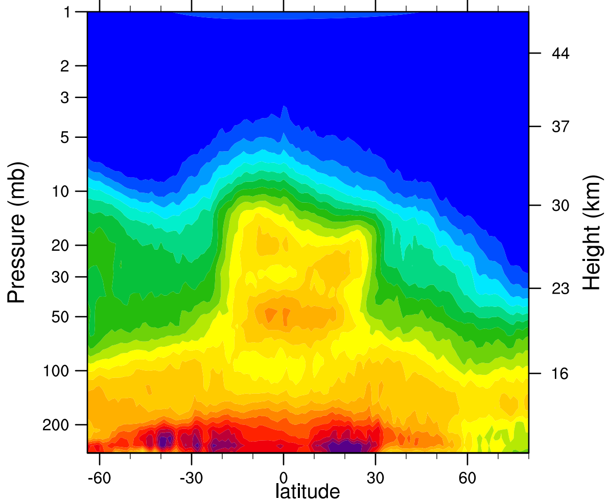
HIRDLSv6 2007d343 N2O_Combined (ppbv)
