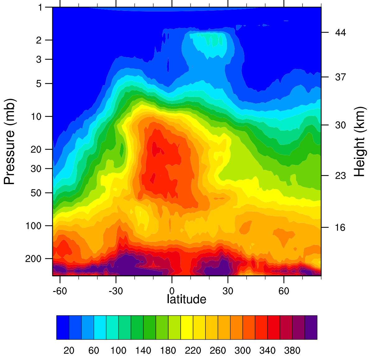
HIRDLSv6 2005d162 N2O_Combined (ppbv)
