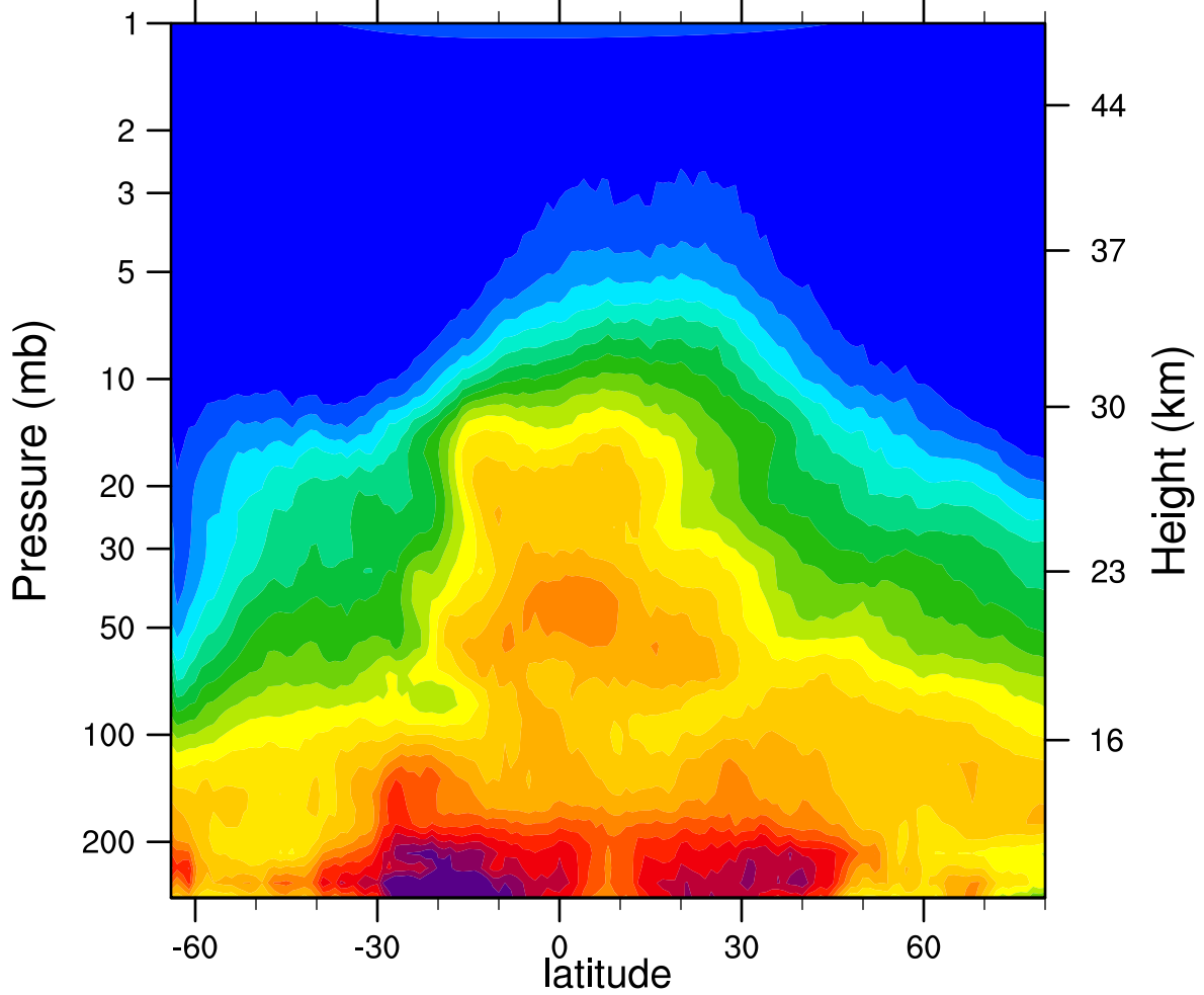
HIRDLSv6 2007d248 N2O_Combined (ppbv)
