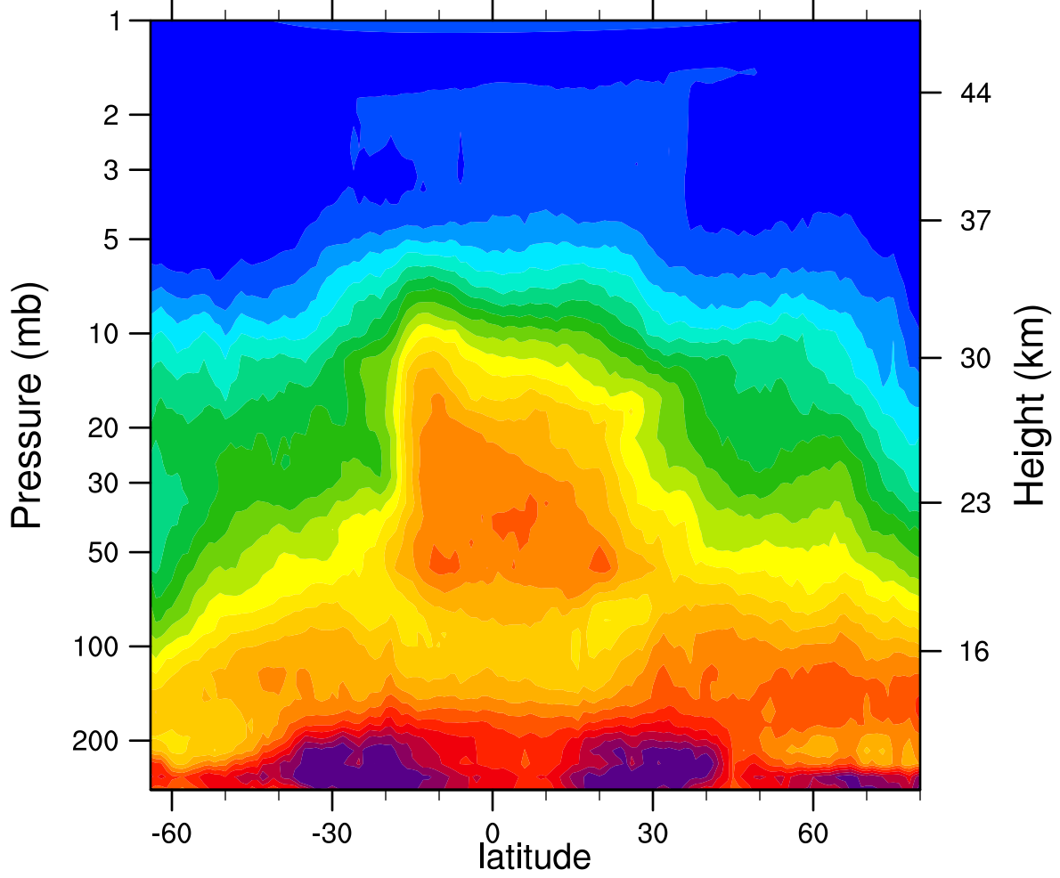
HIRDLSv6 2005d305 N2O_Combined (ppbv)
