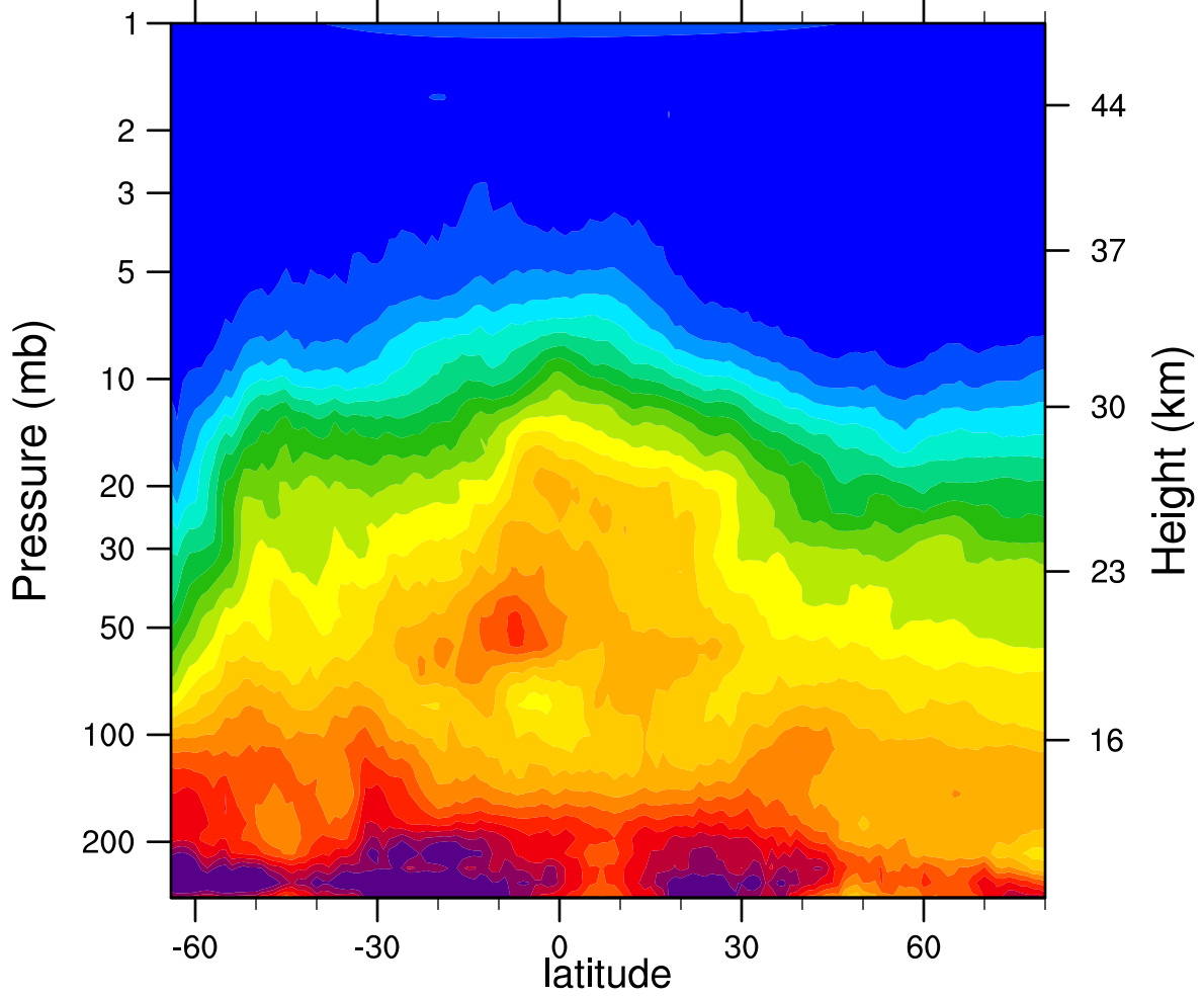
HIRDLSv6 2006d172 N2O_Combined (ppbv)
