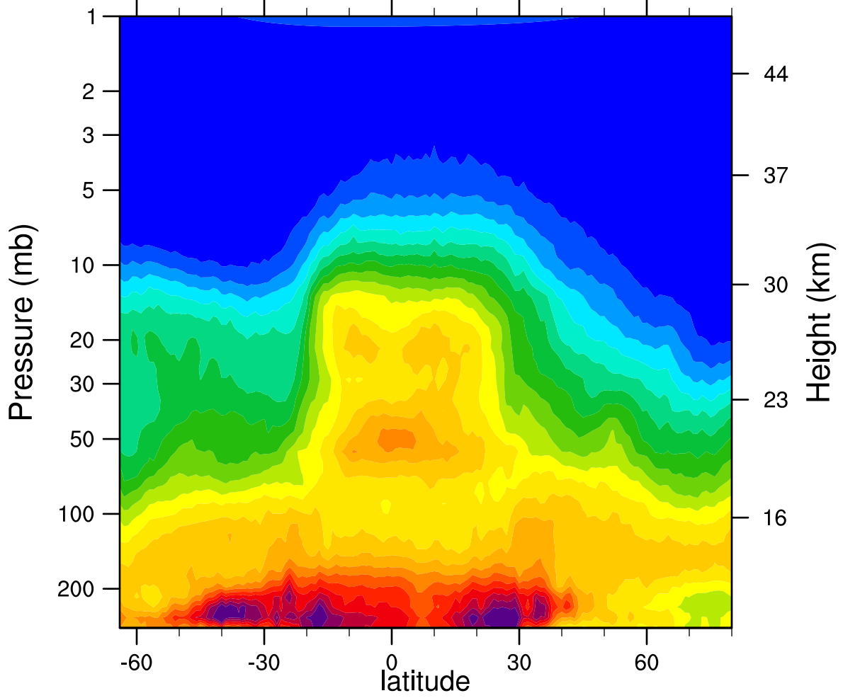
HIRDLSv6 2007d302 N2O_Combined (ppbv)
