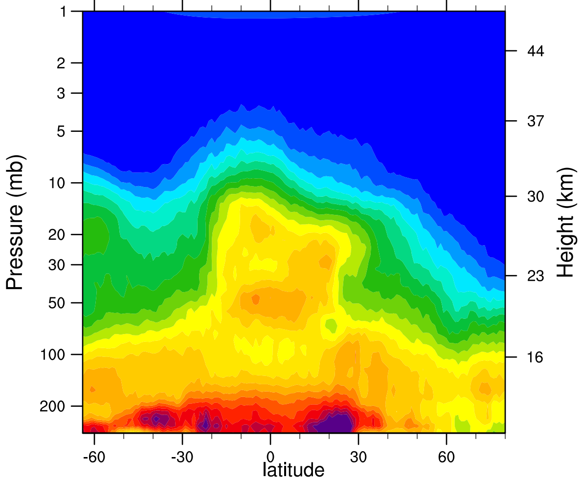
HIRDLSv6 2007d352 N2O_Combined (ppbv)
