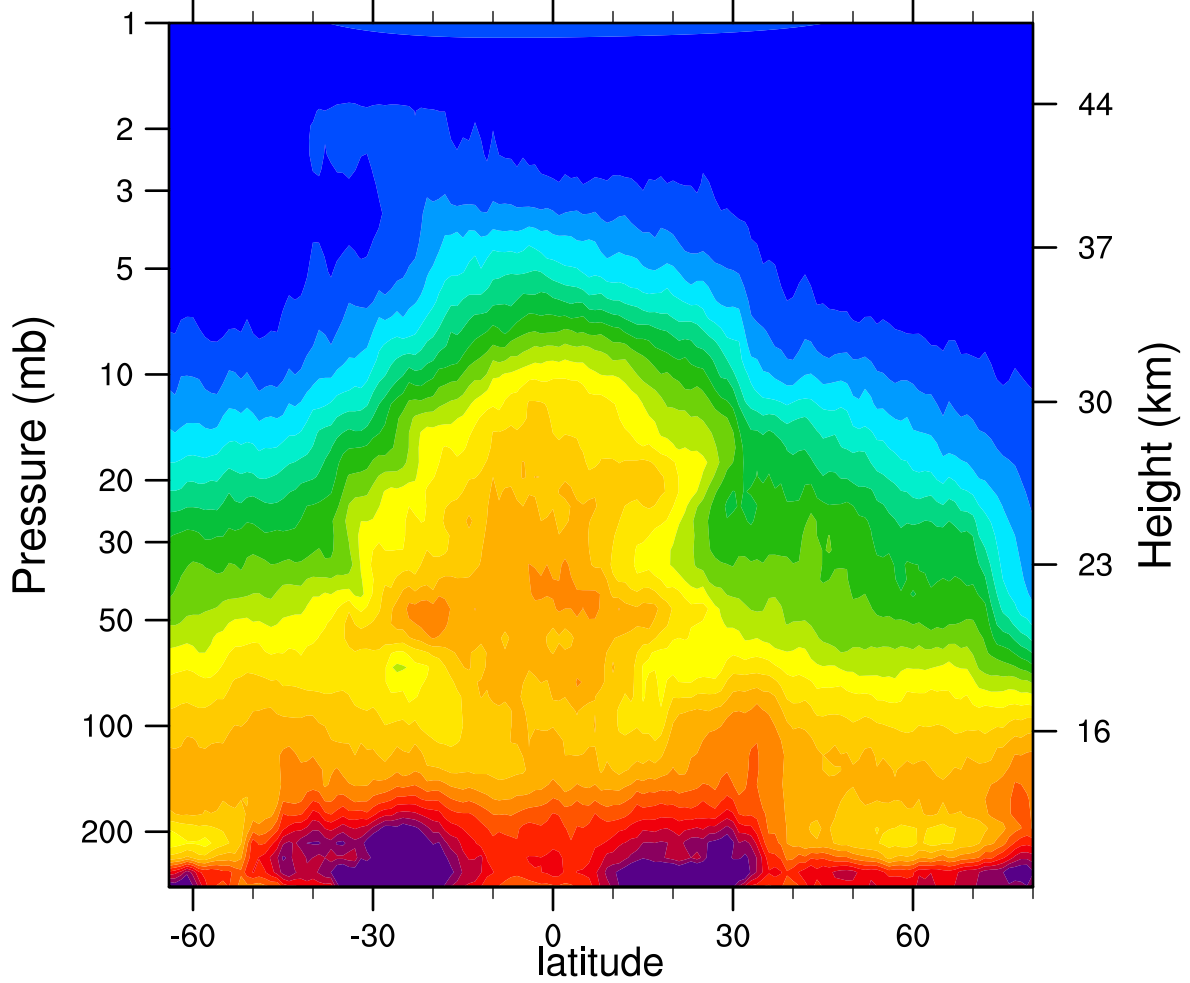
HIRDLSv6 2007d069 N2O_Combined (ppbv)
