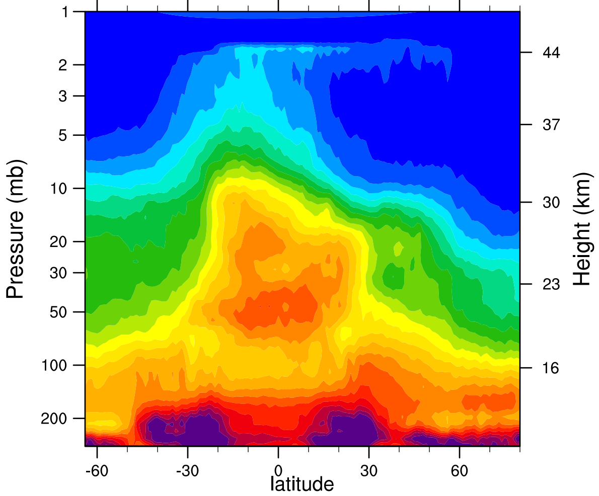
HIRDLSv6 2006d011 N2O_Combined (ppbv)
