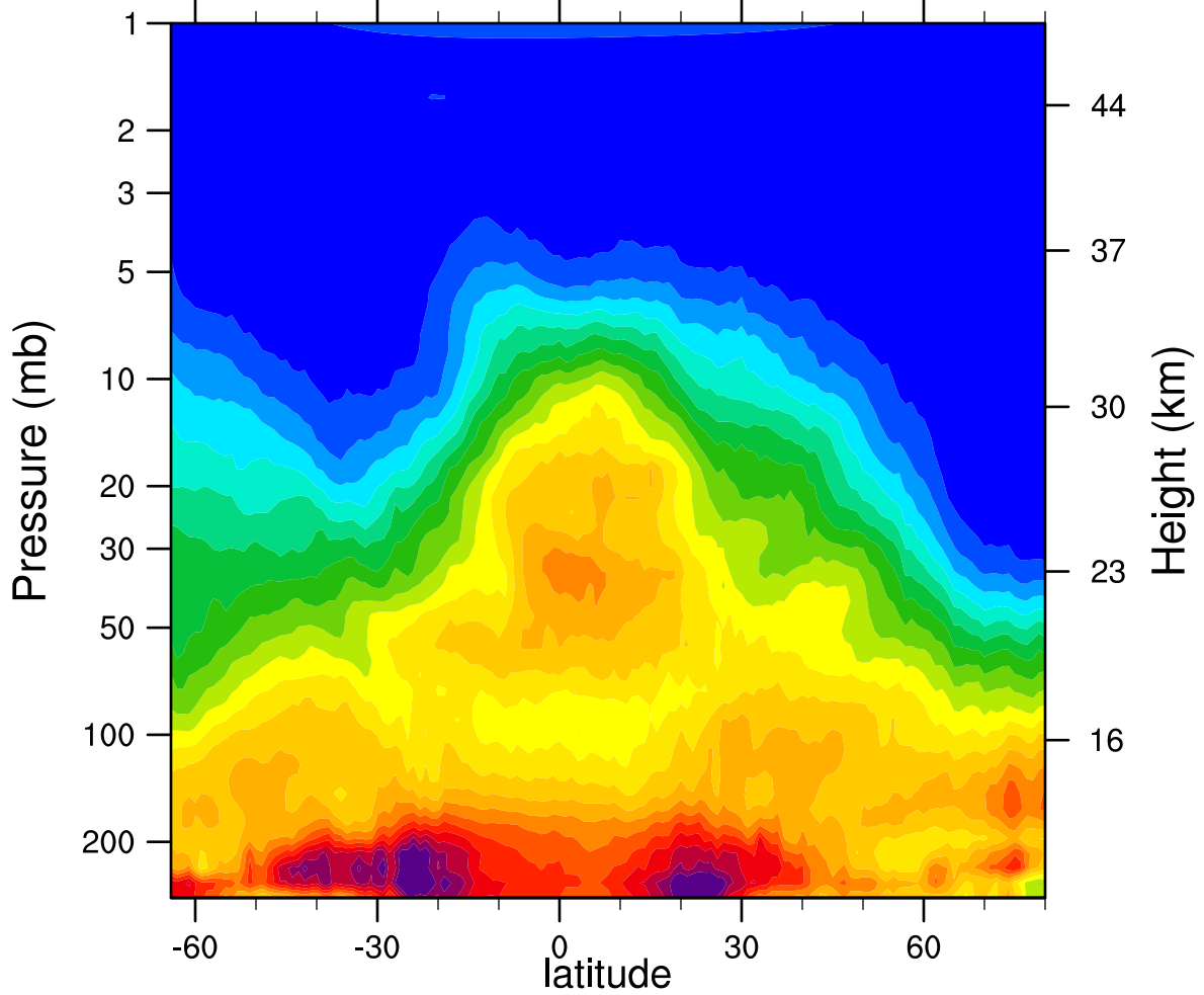
HIRDLSv6 2006d342 N2O_Combined (ppbv)
