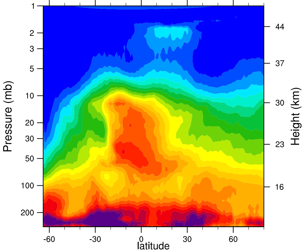
HIRDLSv6 2005d191 N2O_Combined (ppbv)
