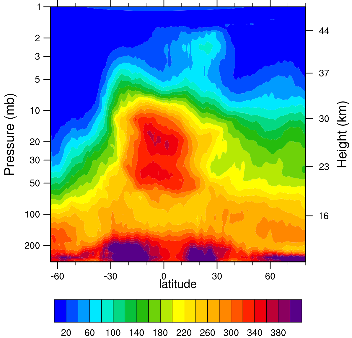
HIRDLSv6 2005d140 N2O_Combined (ppbv)
