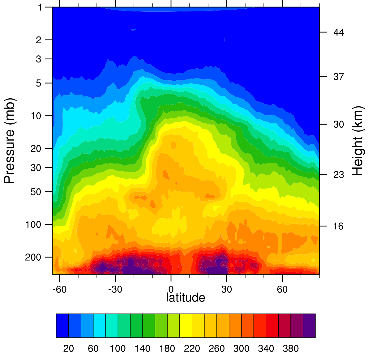
HIRDLSv6 2006d287 N2O_Combined (ppbv)
