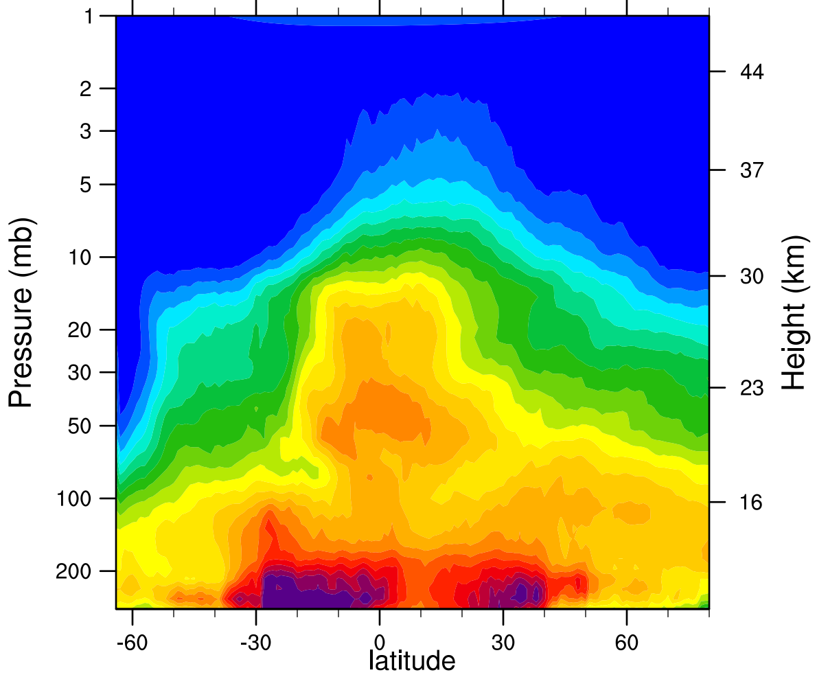
HIRDLSv6 2007d225 N2O_Combined (ppbv)
