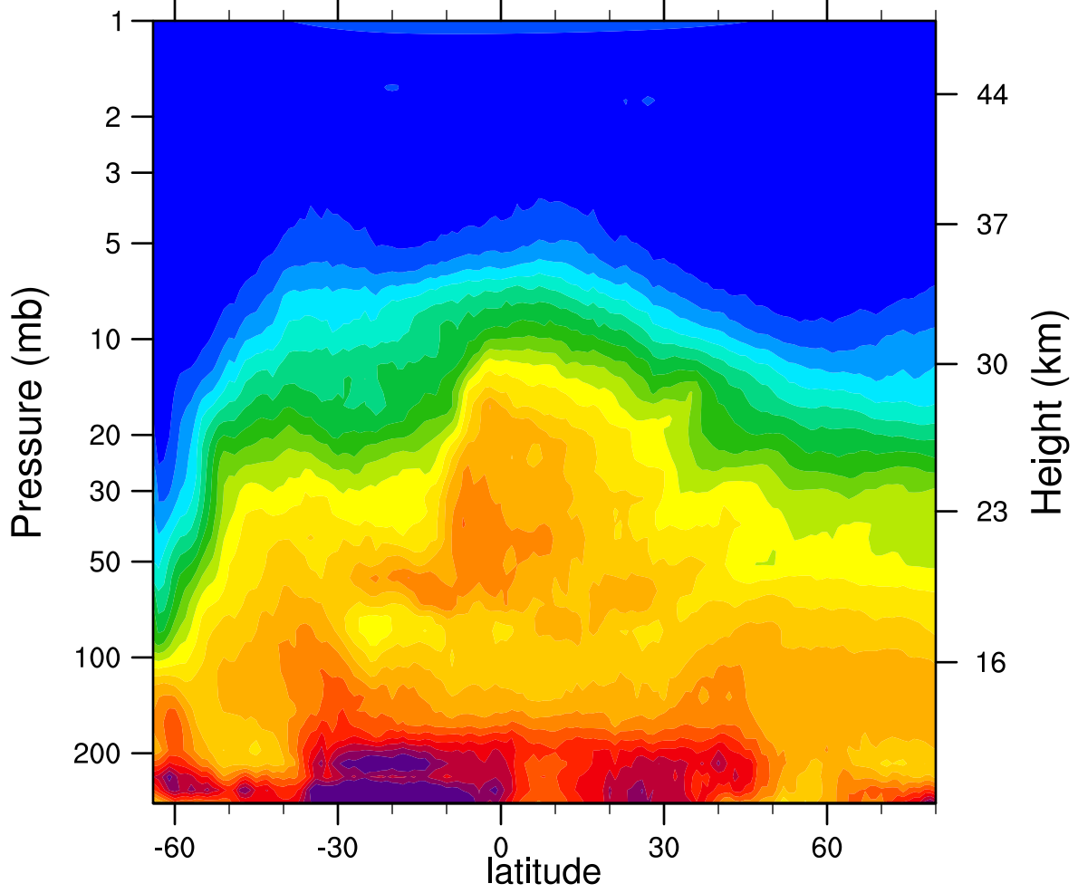
HIRDLSv6 2006d222 N2O_Combined (ppbv)
