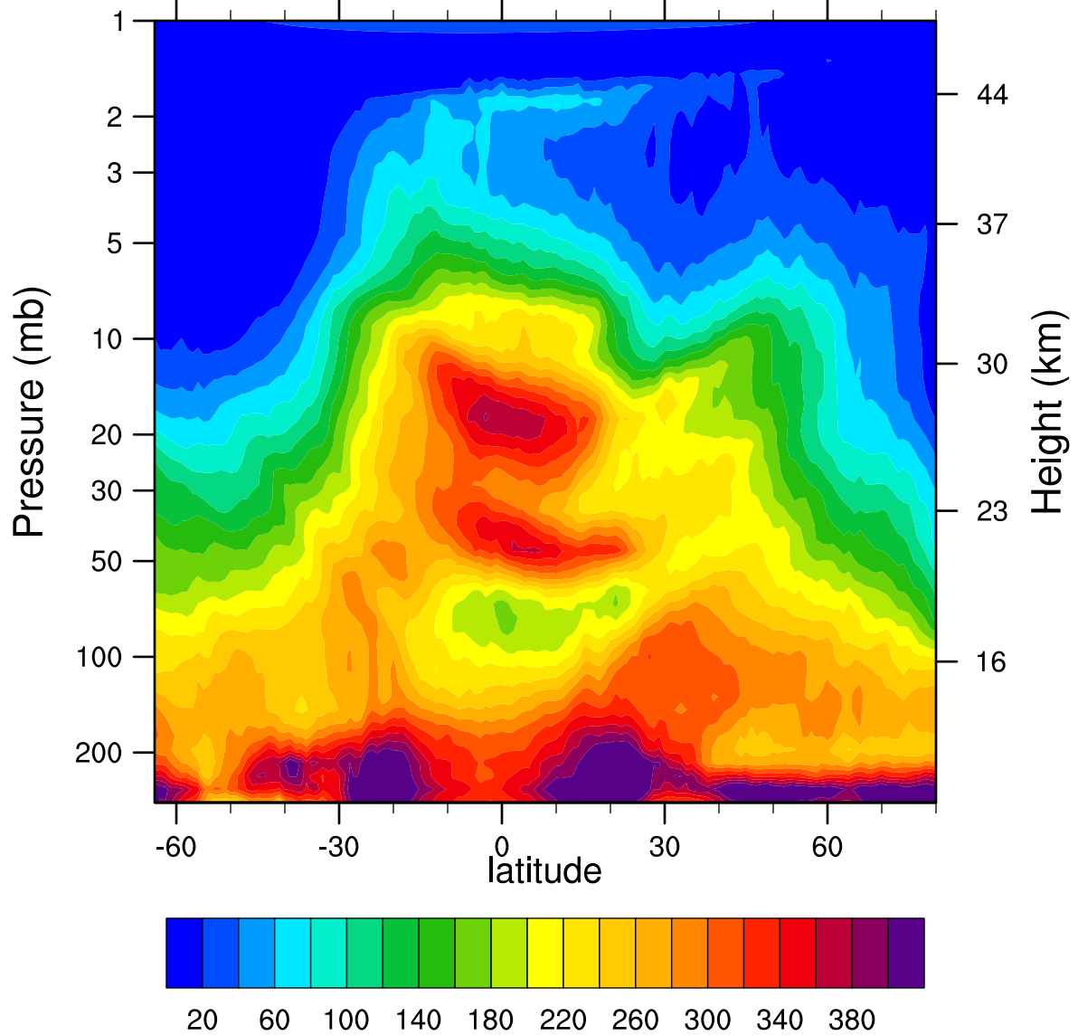
HIRDLSv6 2005d063 N2O_Combined (ppbv)
