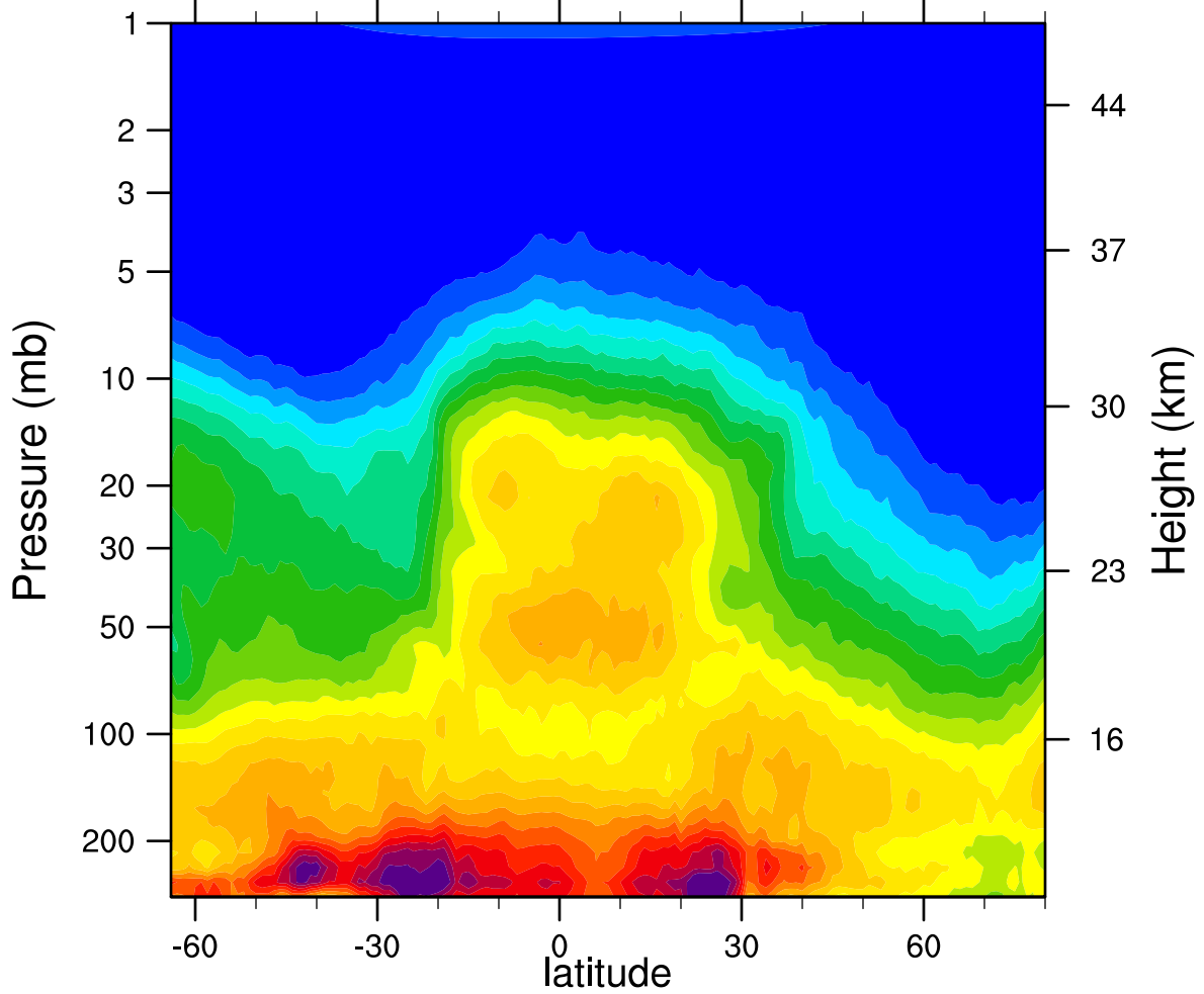
HIRDLSv6 2007d322 N2O_Combined (ppbv)
