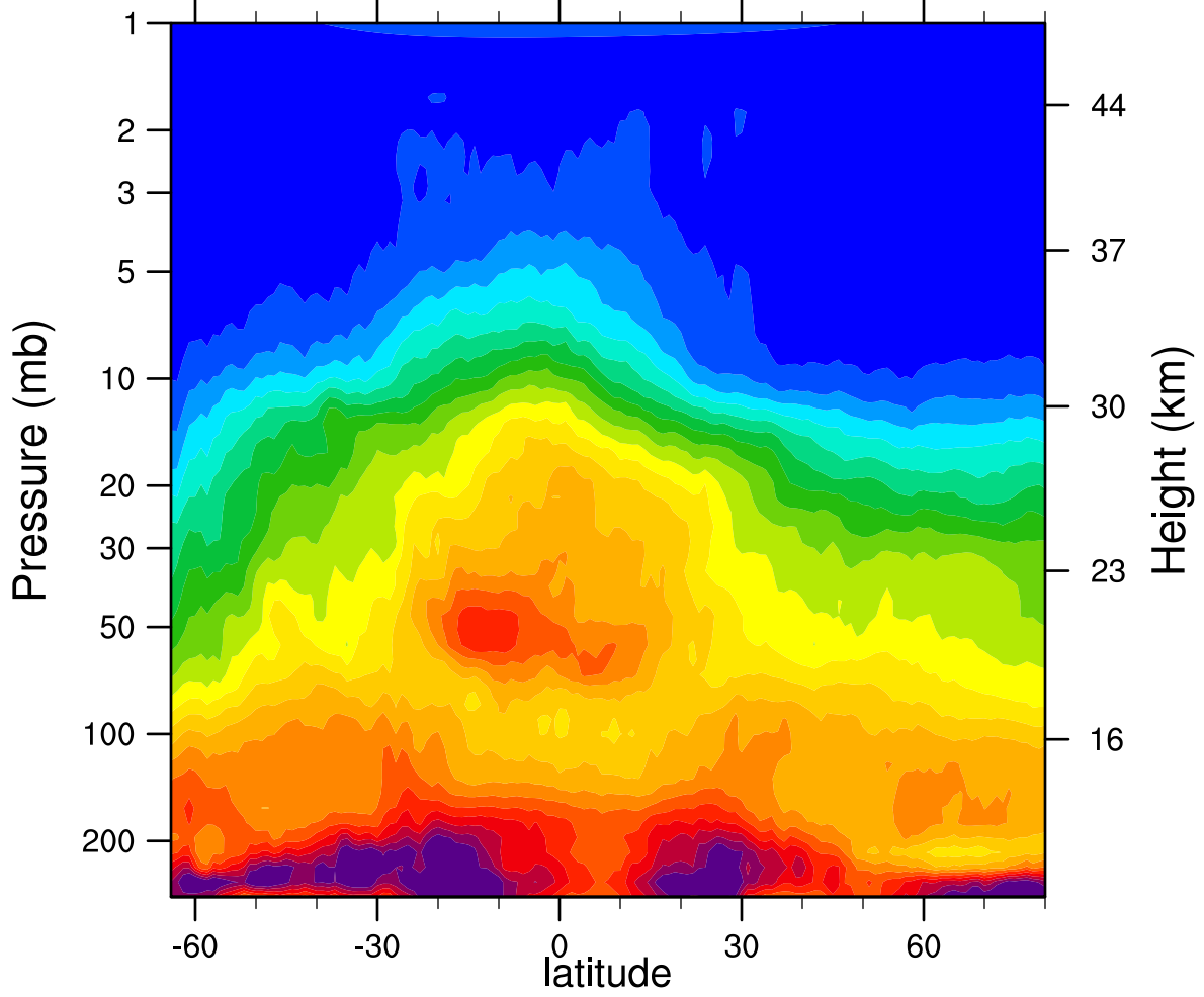
HIRDLSv6 2006d136 N2O_Combined (ppbv)
