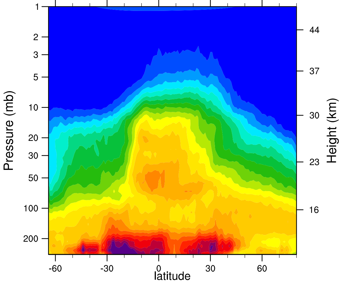
HIRDLSv6 2007d270 N2O_Combined (ppbv)
