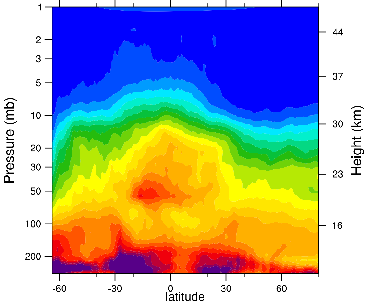
HIRDLSv6 2006d154 N2O_Combined (ppbv)
