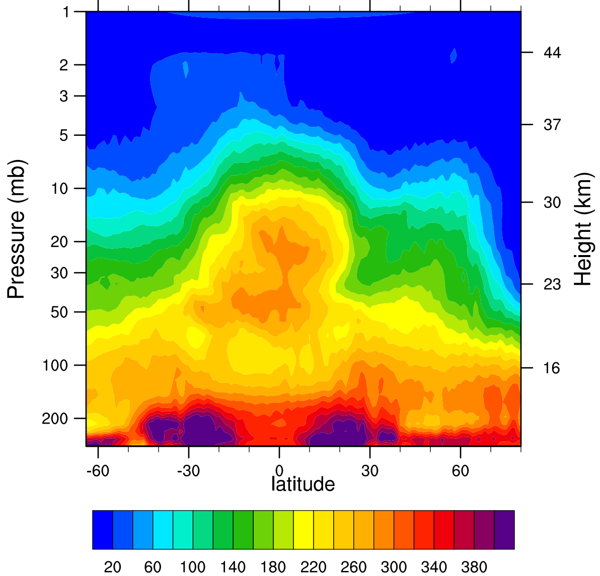
HIRDLSv6 2007d033 N2O_Combined (ppbv)
