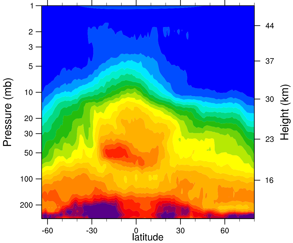
HIRDLSv6 2006d120 N2O_Combined (ppbv)
