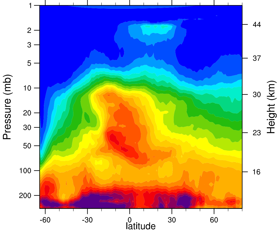
HIRDLSv6 2005d201 N2O_Combined (ppbv)
