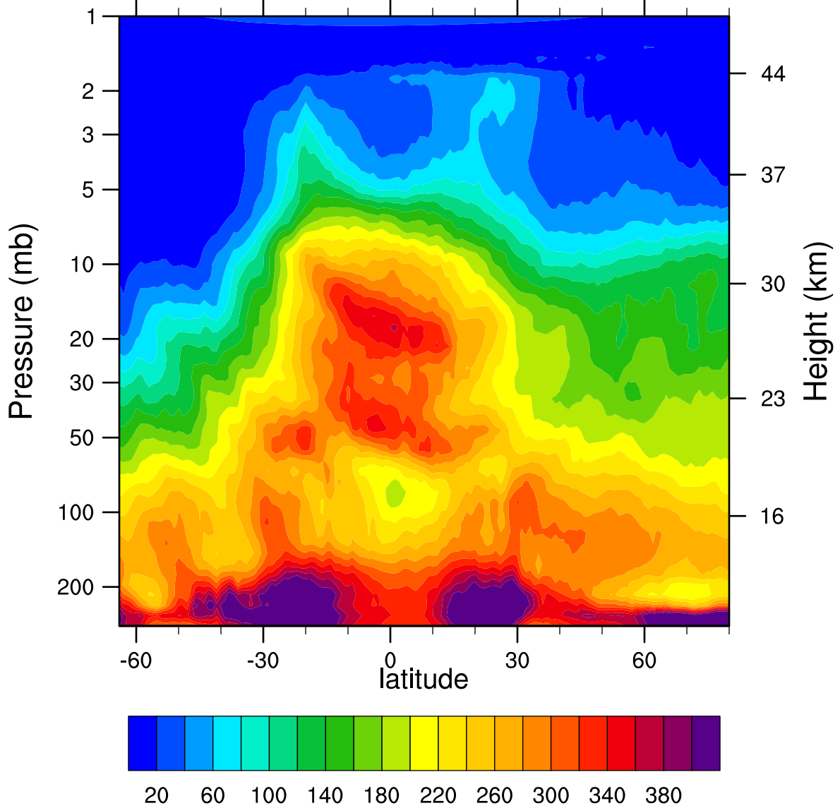
HIRDLSv6 2005d107 N2O_Combined (ppbv)
