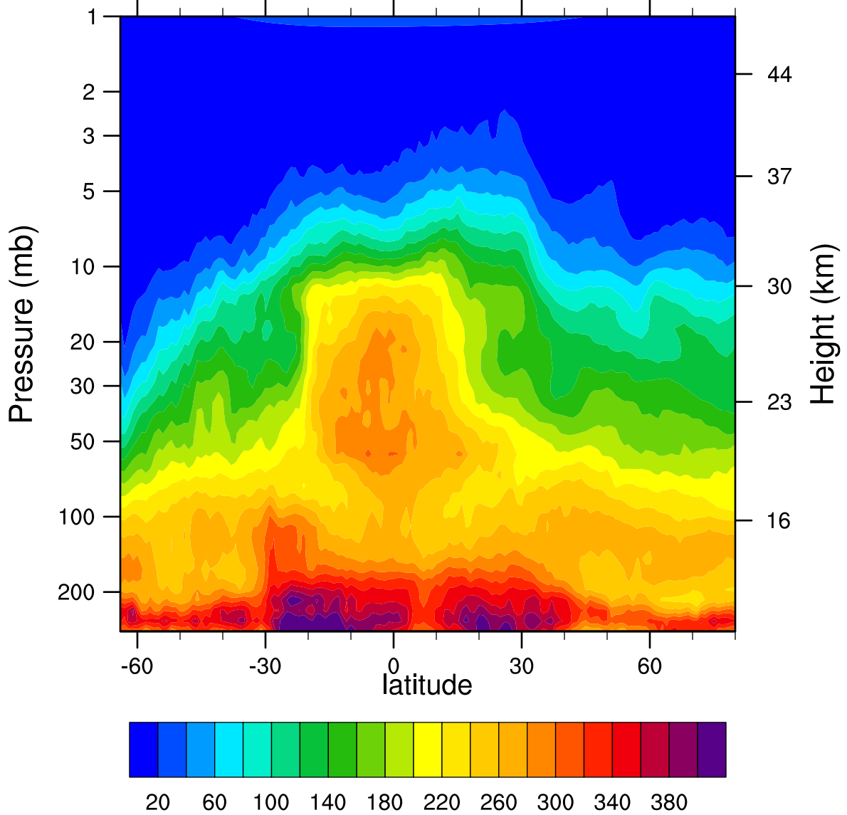
HIRDLSv6 2007d163 N2O_Combined (ppbv)
