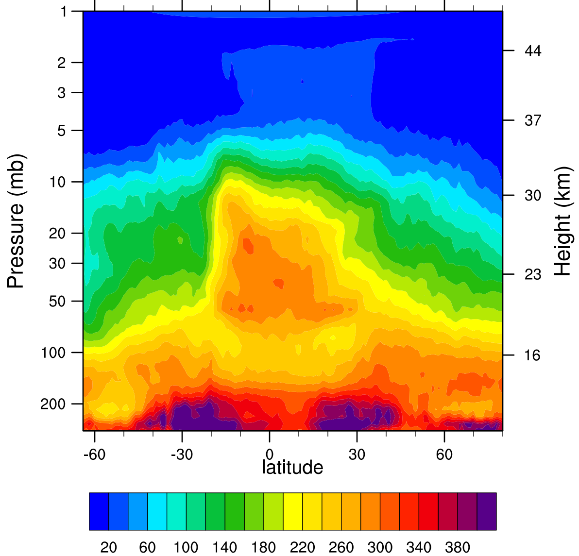
HIRDLSv6 2005d297 N2O_Combined (ppbv)
