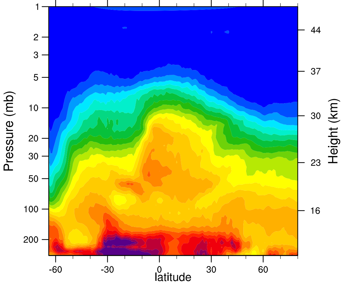
HIRDLSv6 2006d232 N2O_Combined (ppbv)
