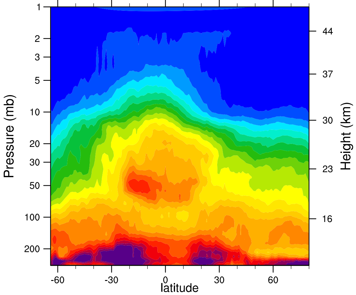
HIRDLSv6 2006d128 N2O_Combined (ppbv)
