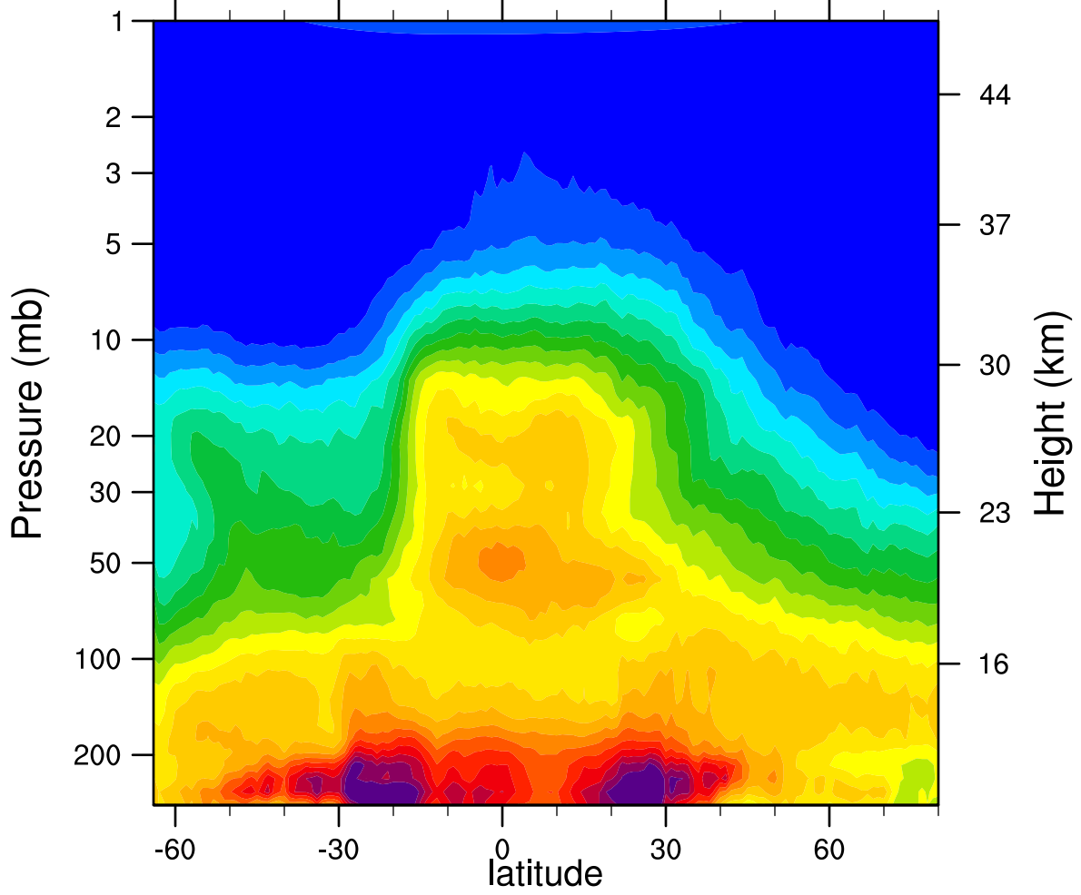
HIRDLSv6 2007d294 N2O_Combined (ppbv)
