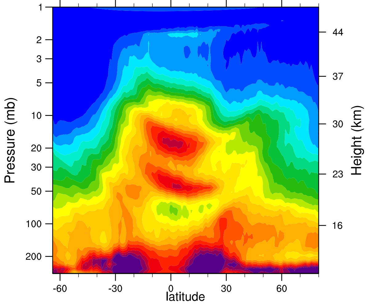
HIRDLSv6 2005d070 N2O_Combined (ppbv)
