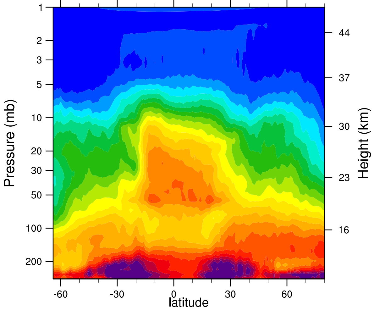
HIRDLSv6 2005d308 N2O_Combined (ppbv)
