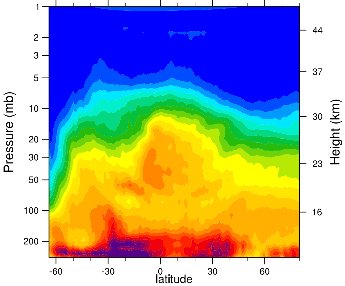
HIRDLSv6 2006d215 N2O_Combined (ppbv)
