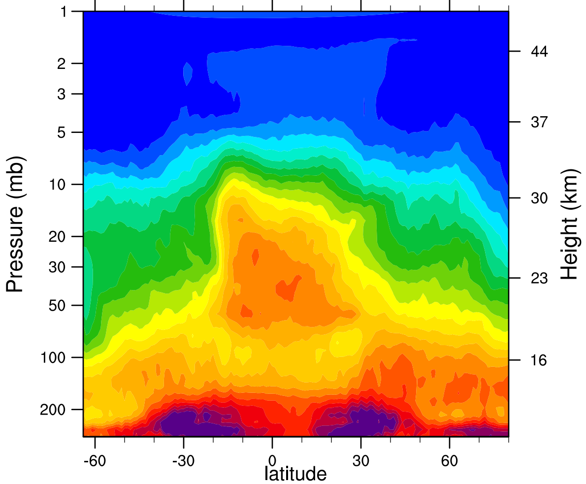
HIRDLSv6 2005d301 N2O_Combined (ppbv)
