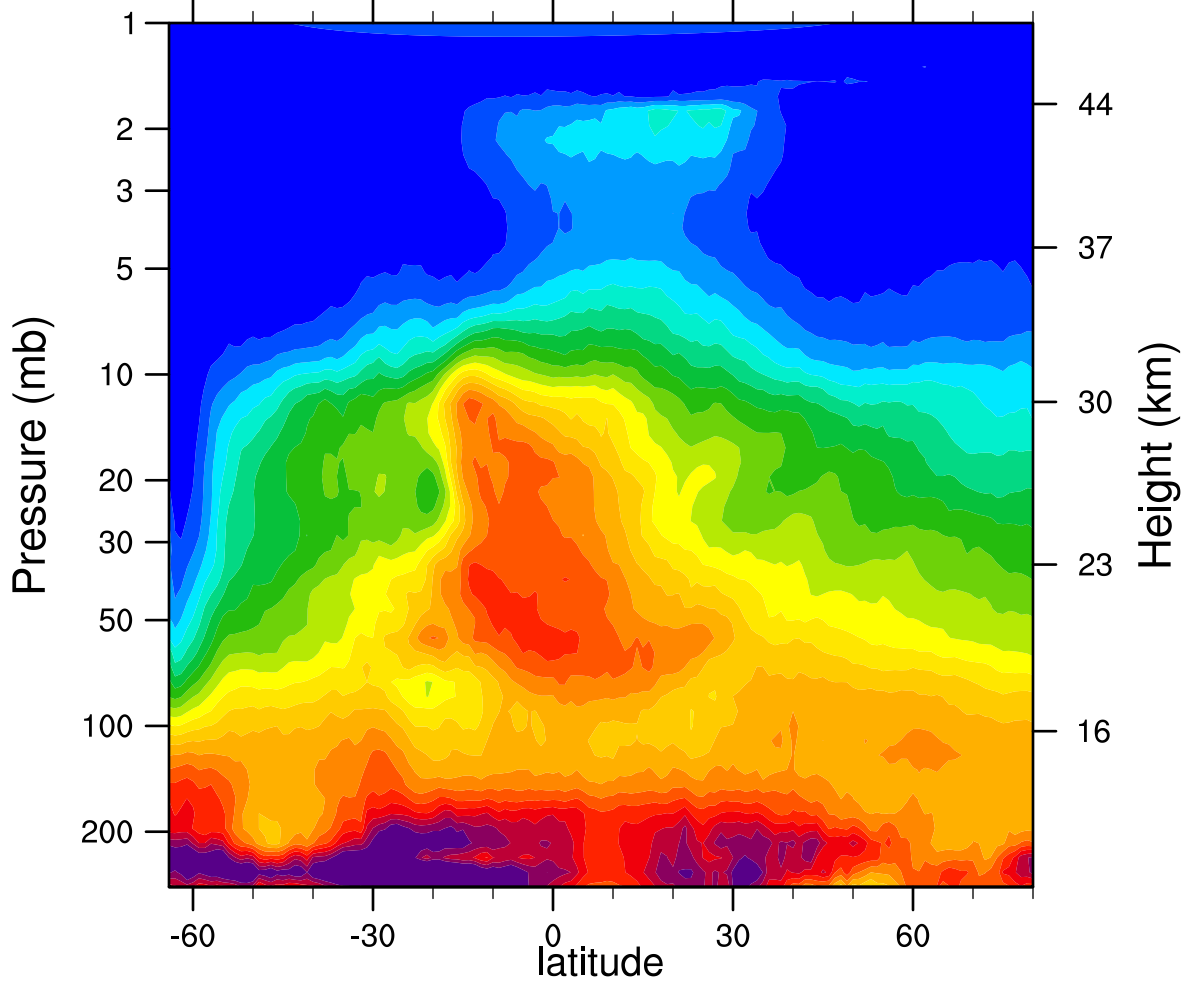
HIRDLSv6 2005d220 N2O_Combined (ppbv)
