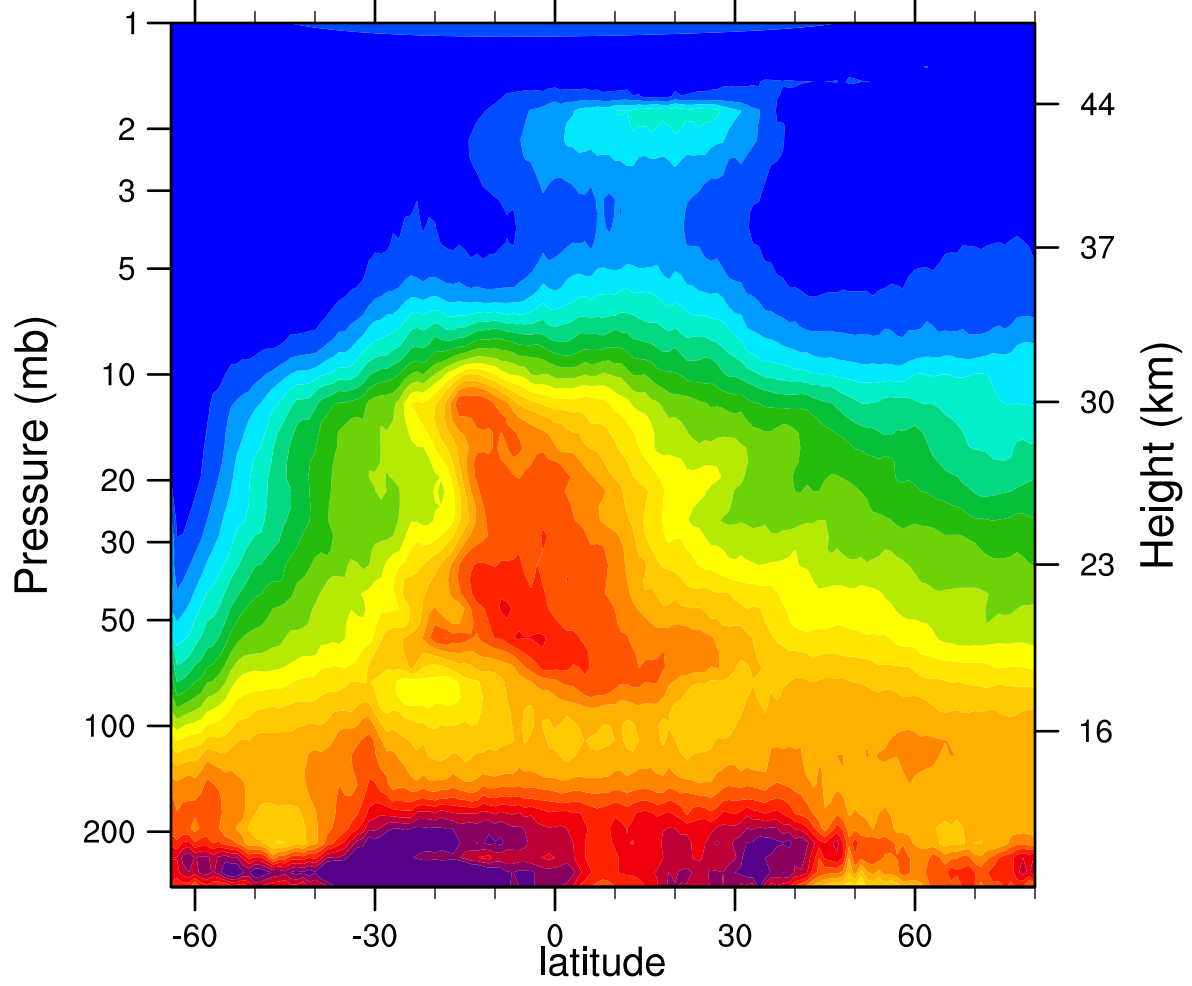
HIRDLSv6 2005d211 N2O_Combined (ppbv)
