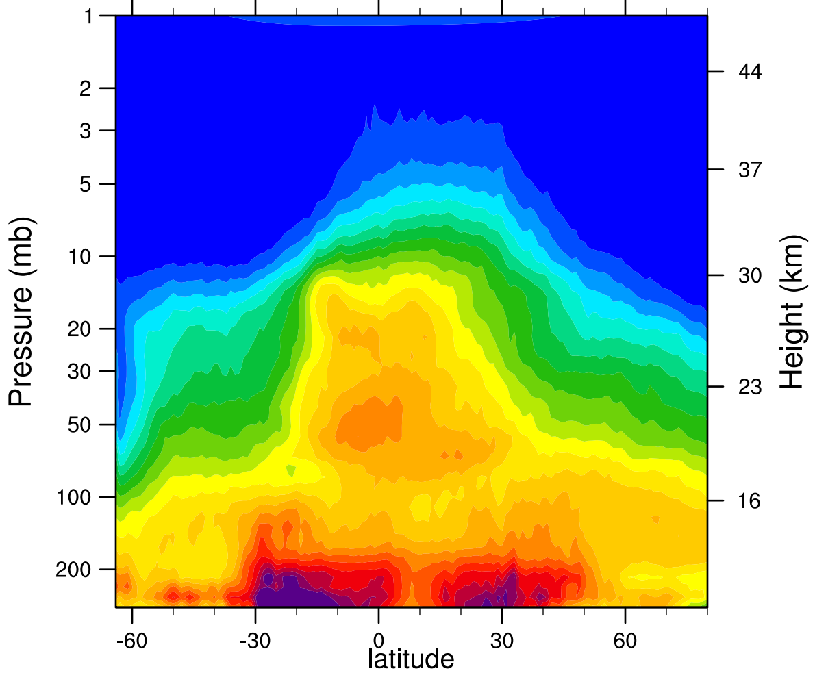
HIRDLSv6 2007d254 N2O_Combined (ppbv)
