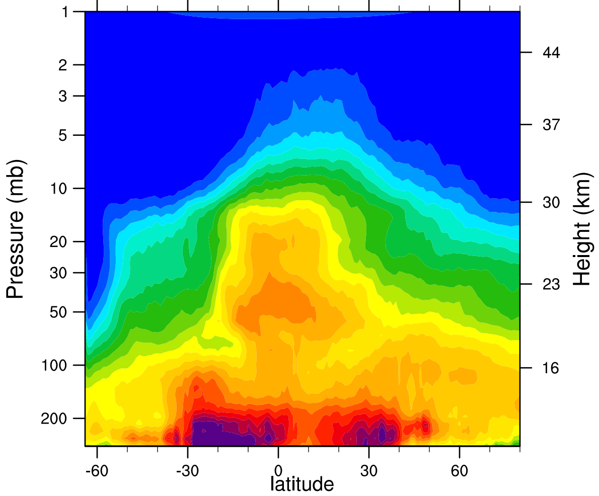
HIRDLSv6 2007d226 N2O_Combined (ppbv)
