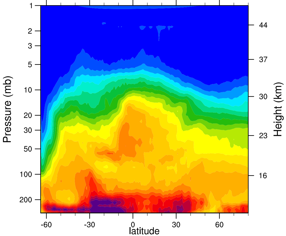
HIRDLSv6 2006d216 N2O_Combined (ppbv)
