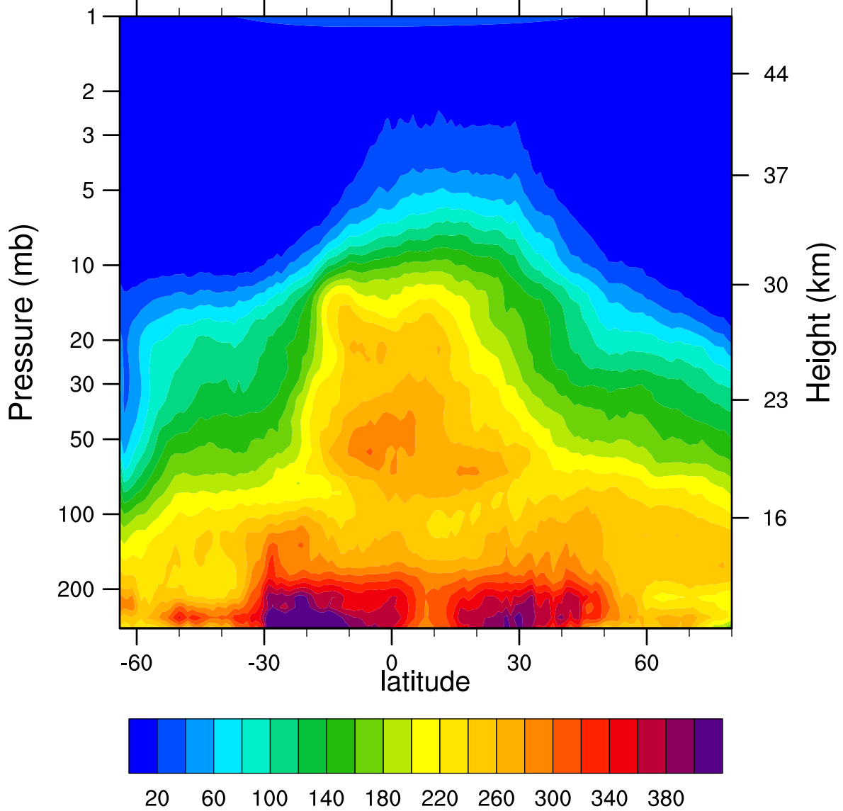
HIRDLSv6 2007d255 N2O_Combined (ppbv)
