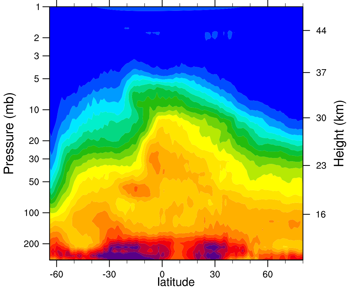
HIRDLSv6 2006d265 N2O_Combined (ppbv)
