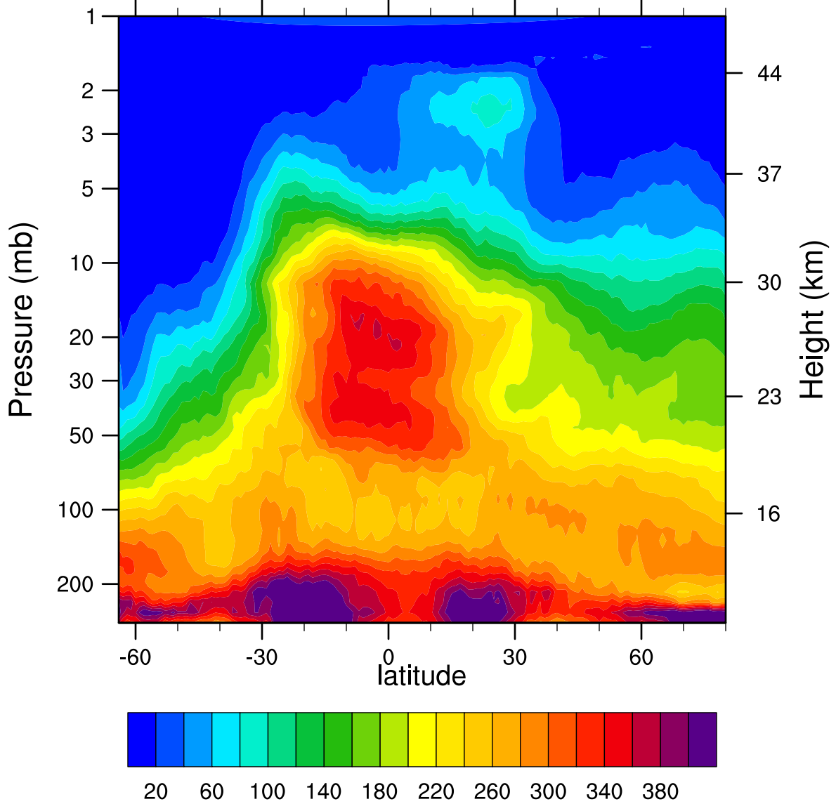
HIRDLSv6 2005d143 N2O_Combined (ppbv)
