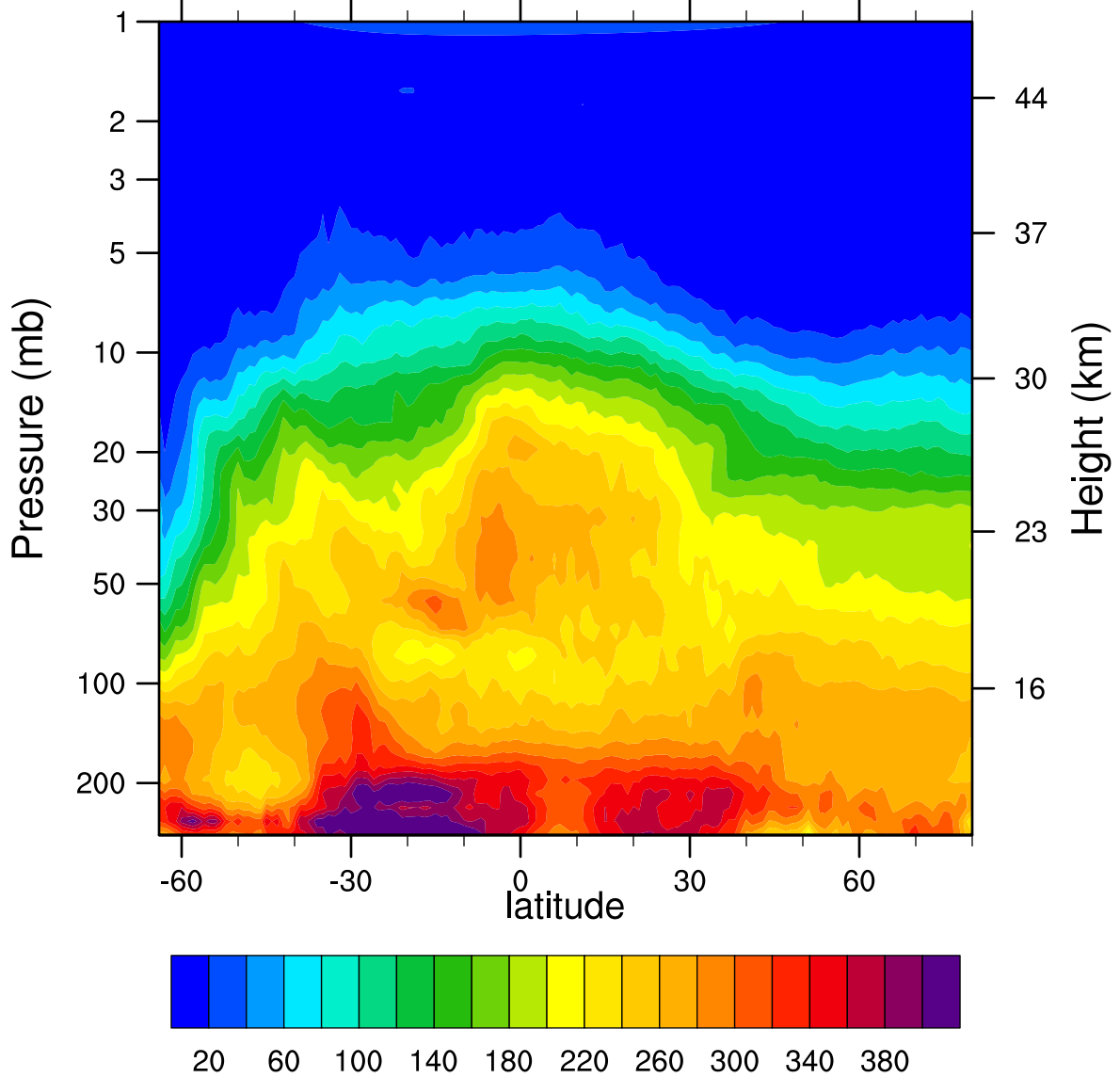
HIRDLSv6 2006d188 N2O_Combined (ppbv)
