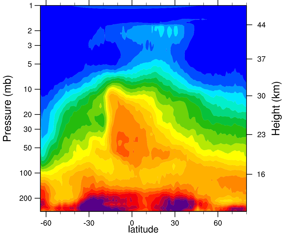
HIRDLSv6 2005d257 N2O_Combined (ppbv)
