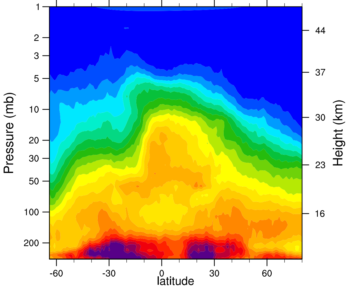
HIRDLSv6 2006d294 N2O_Combined (ppbv)
