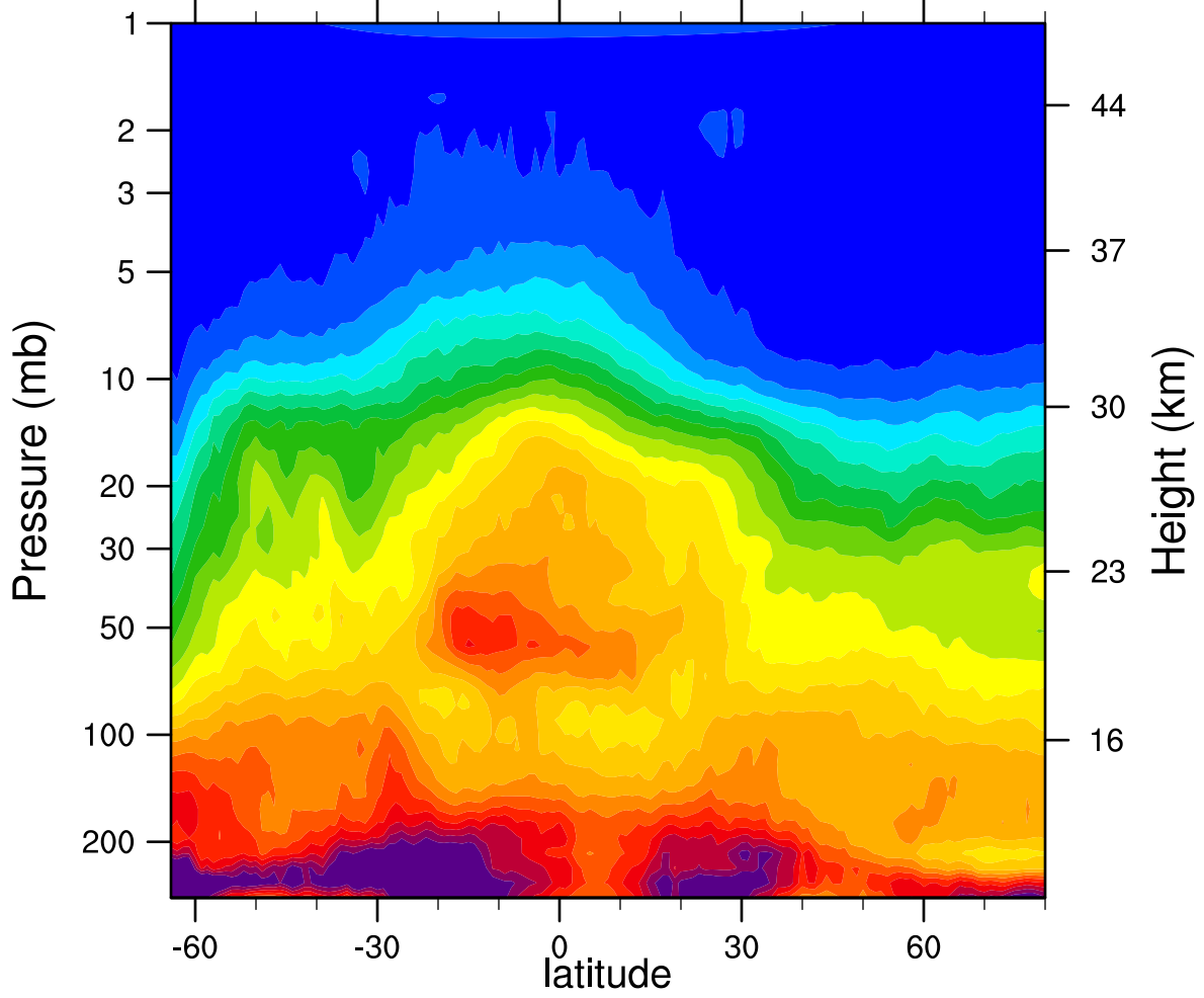
HIRDLSv6 2006d148 N2O_Combined (ppbv)
