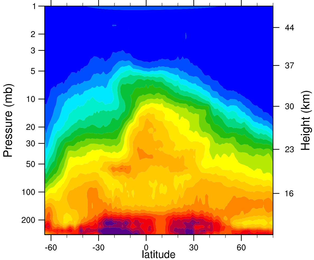
HIRDLSv6 2006d279 N2O_Combined (ppbv)
