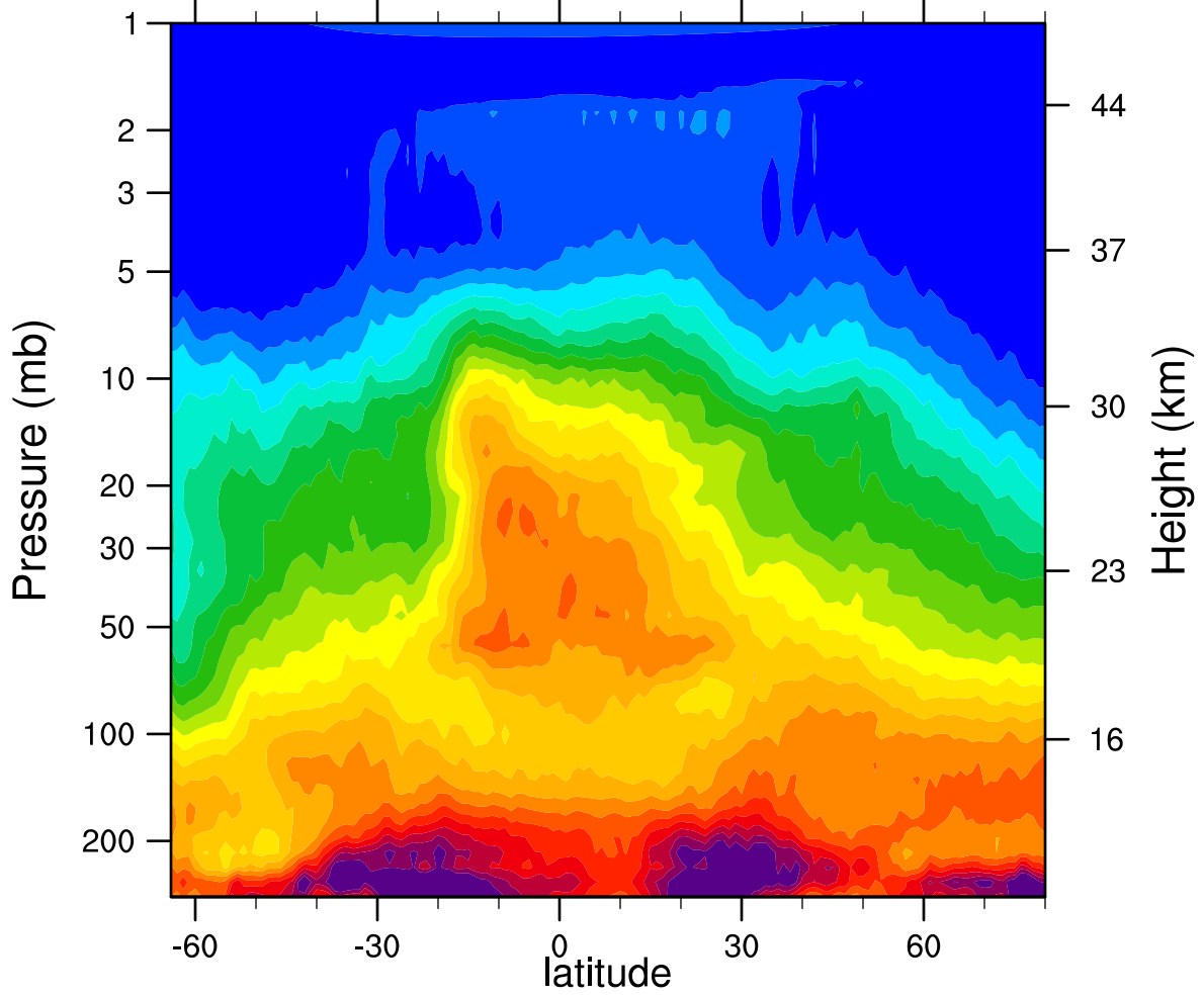
HIRDLSv6 2005d289 N2O_Combined (ppbv)
