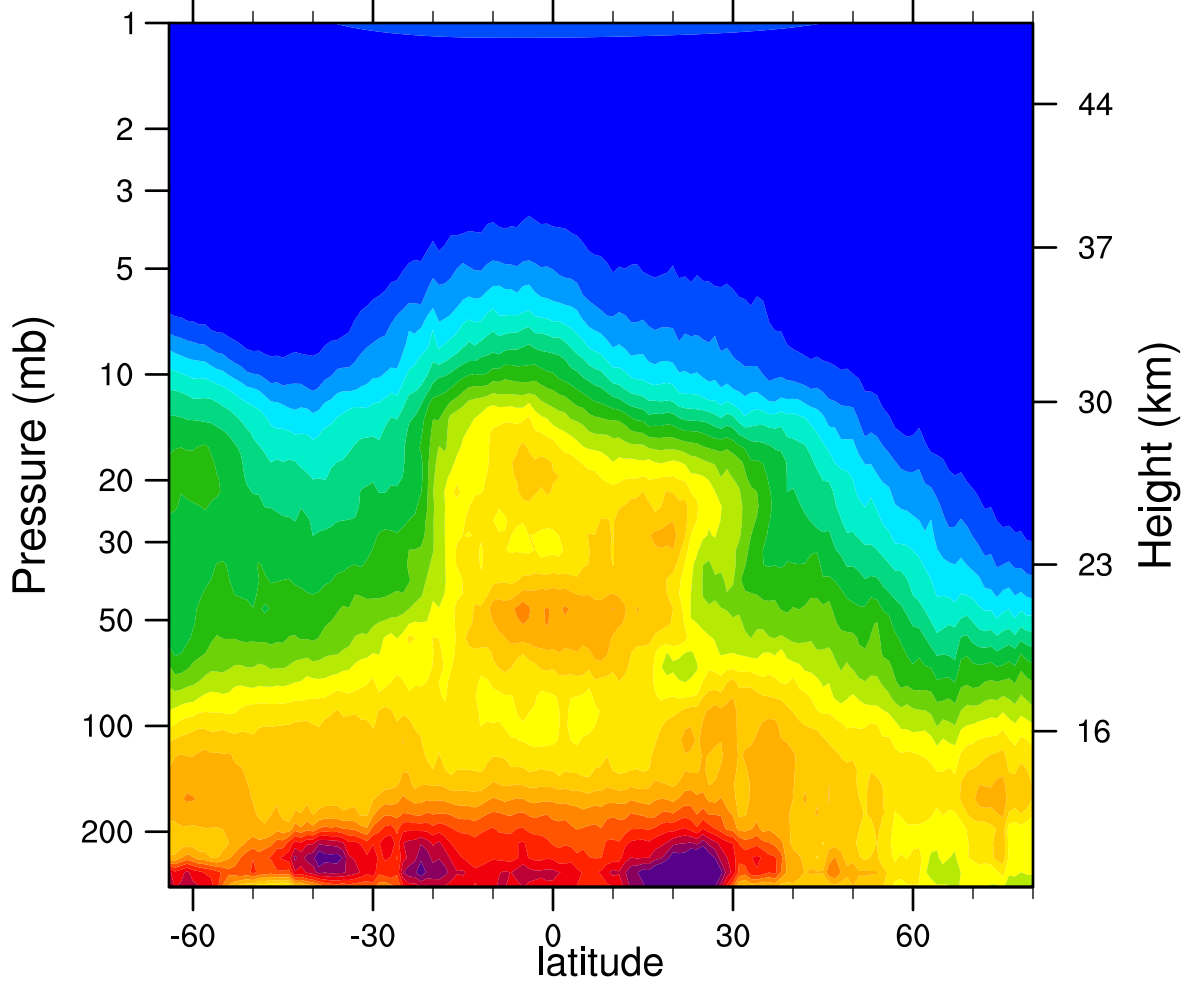
HIRDLSv6 2007d351 N2O_Combined (ppbv)
