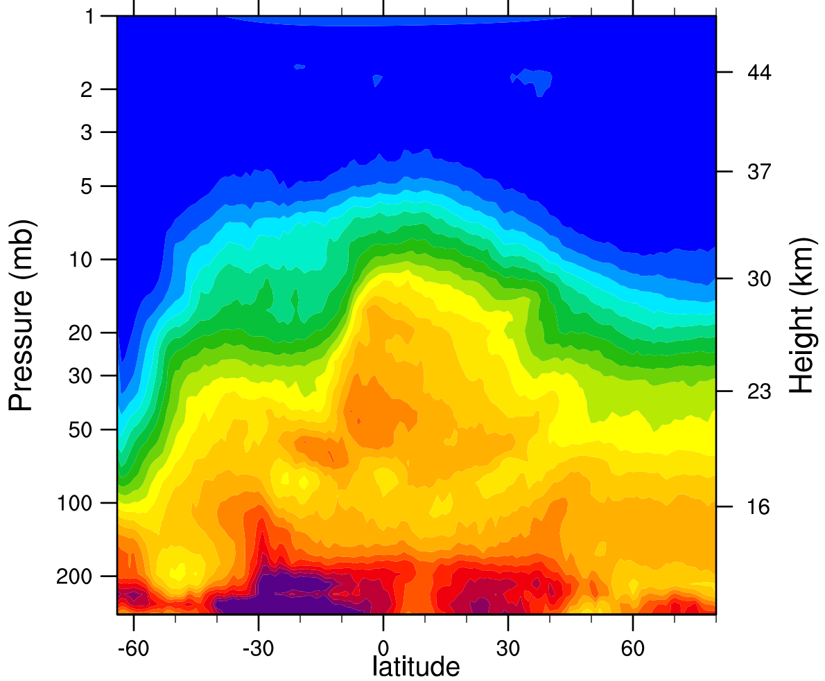
HIRDLSv6 2006d238 N2O_Combined (ppbv)
