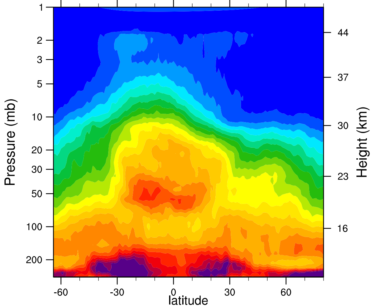
HIRDLSv6 2006d106 N2O_Combined (ppbv)
