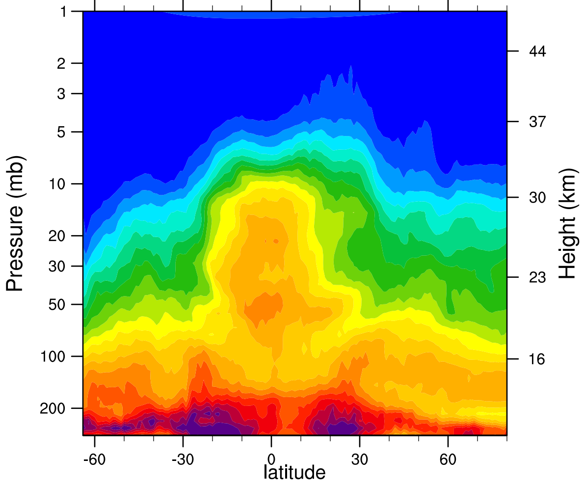
HIRDLSv6 2007d146 N2O_Combined (ppbv)
