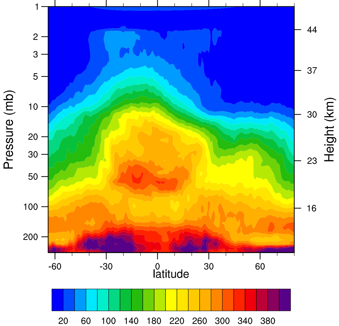
HIRDLSv6 2006d104 N2O_Combined (ppbv)
