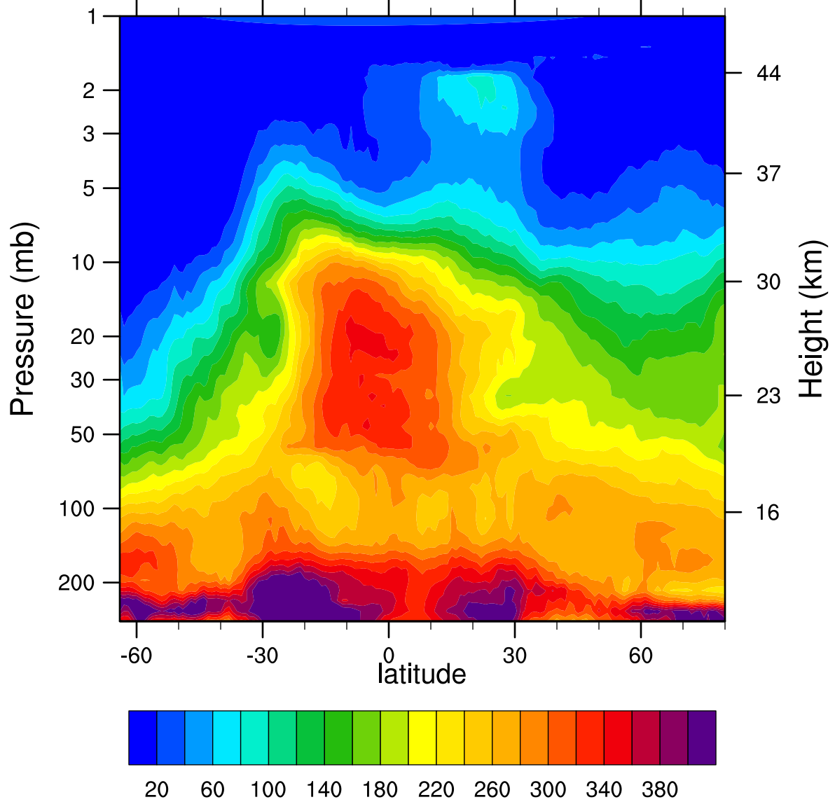
HIRDLSv6 2005d156 N2O_Combined (ppbv)
