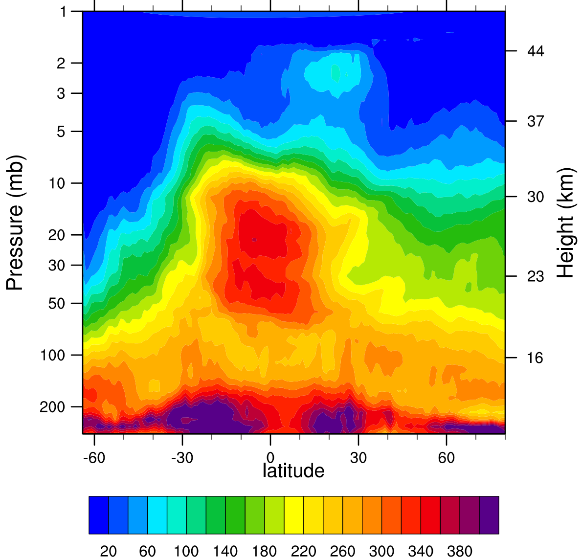
HIRDLSv6 2005d147 N2O_Combined (ppbv)
