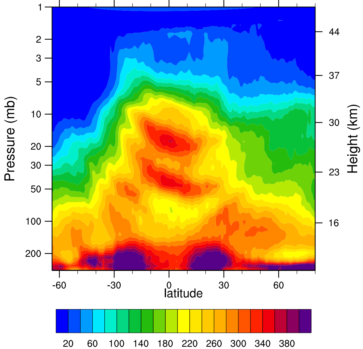
HIRDLSv6 2005d092 N2O_Combined (ppbv)
