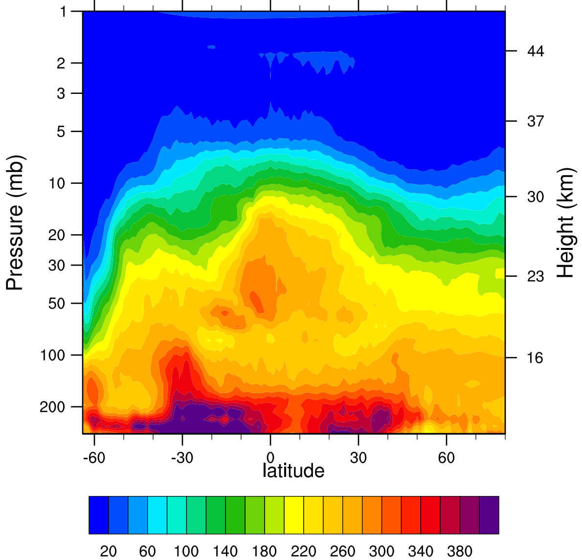
HIRDLSv6 2006d204 N2O_Combined (ppbv)
