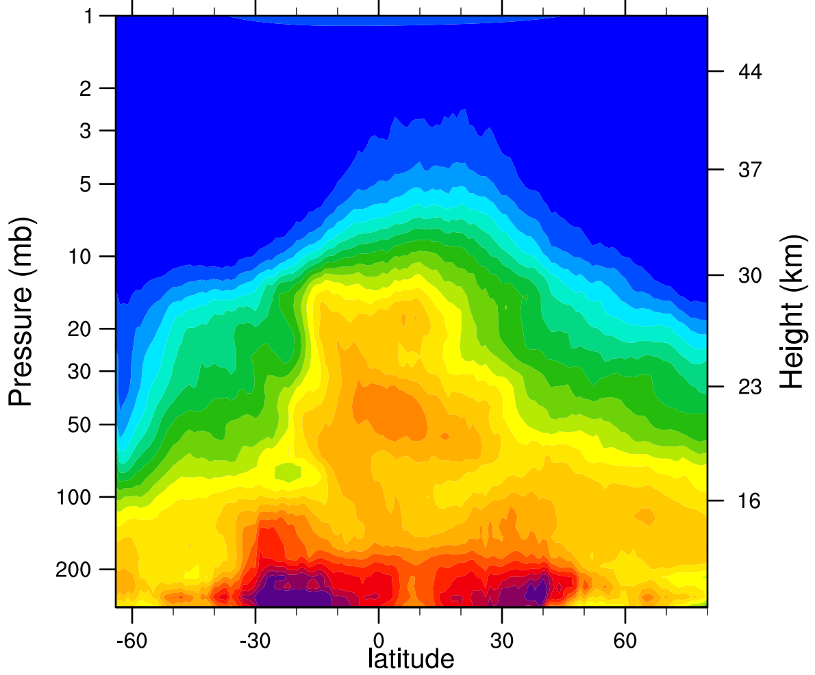
HIRDLSv6 2007d243 N2O_Combined (ppbv)
