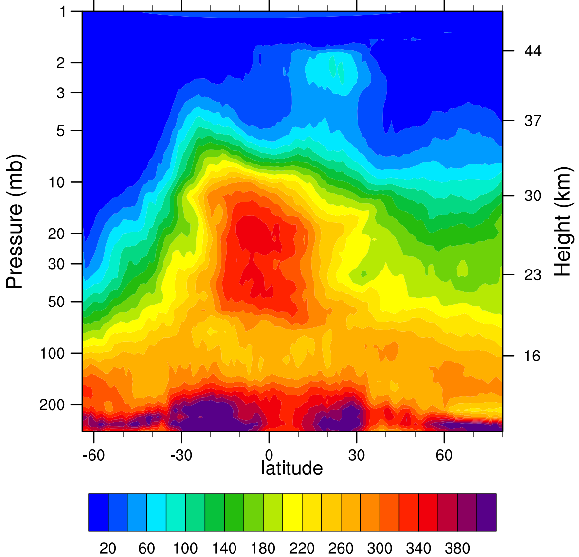
HIRDLSv6 2005d151 N2O_Combined (ppbv)
