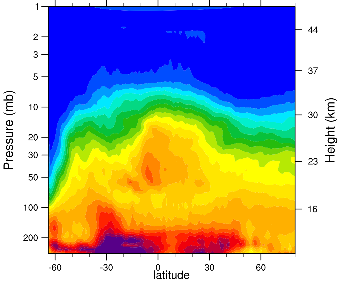
HIRDLSv6 2006d201 N2O_Combined (ppbv)
