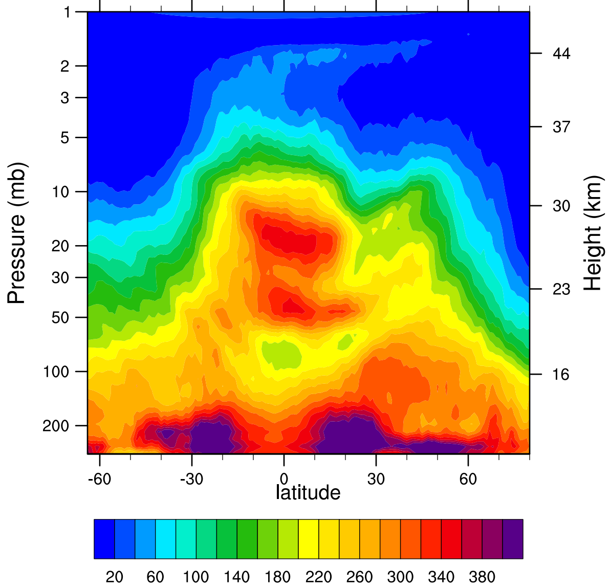
HIRDLSv6 2005d044 N2O_Combined (ppbv)
