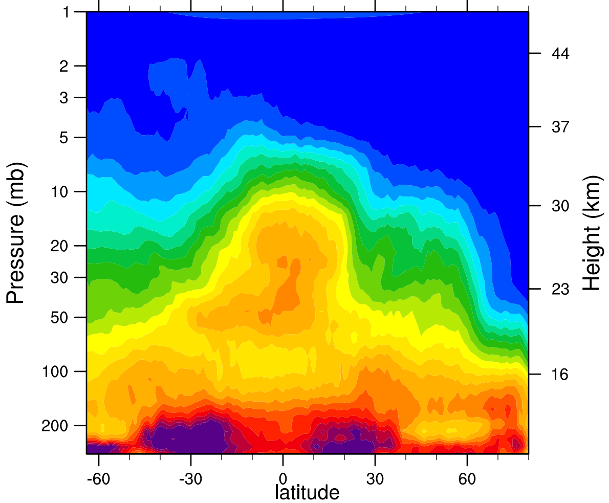
HIRDLSv6 2007d013 N2O_Combined (ppbv)
