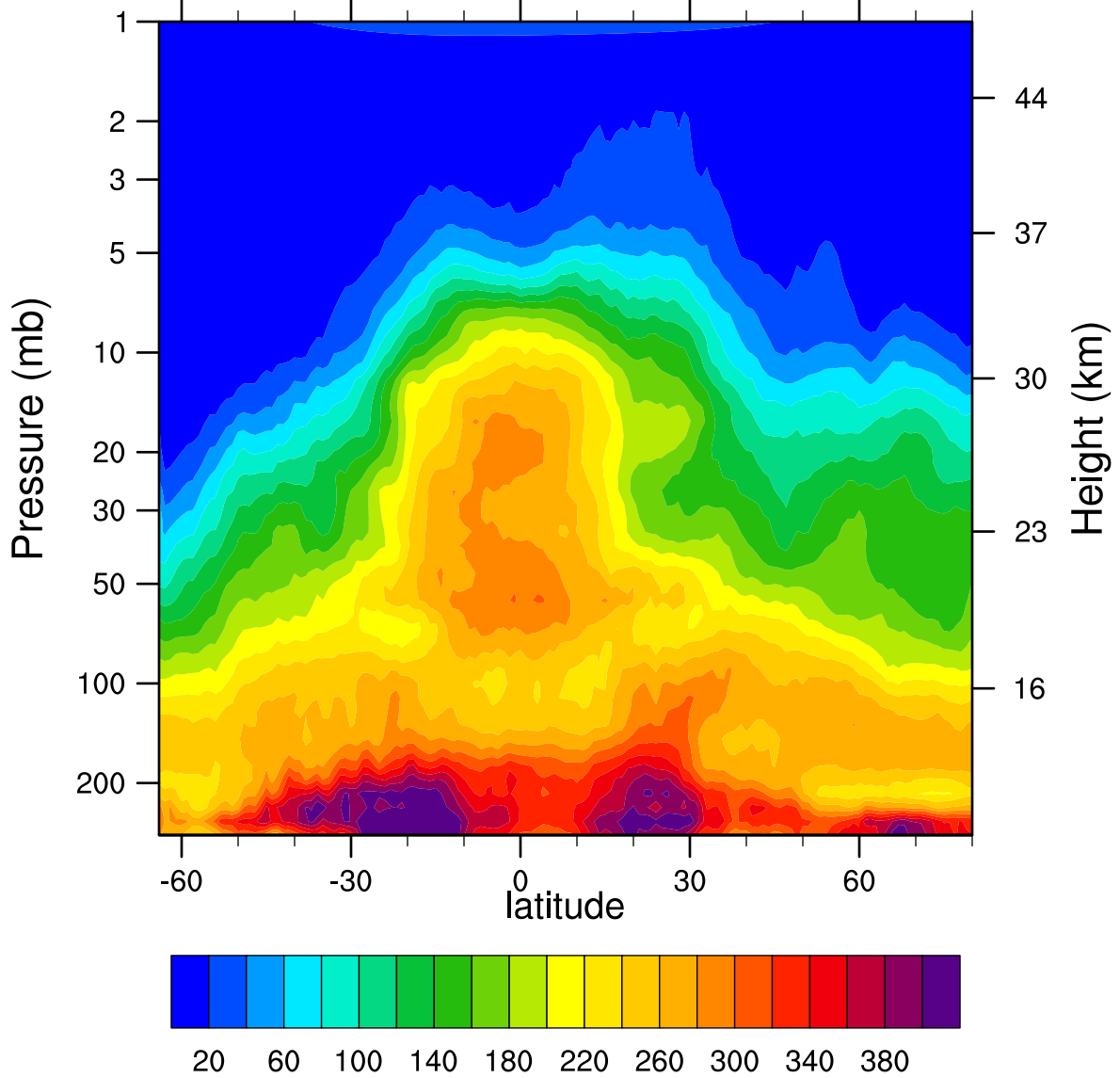
HIRDLSv6 2007d128 N2O_Combined (ppbv)
