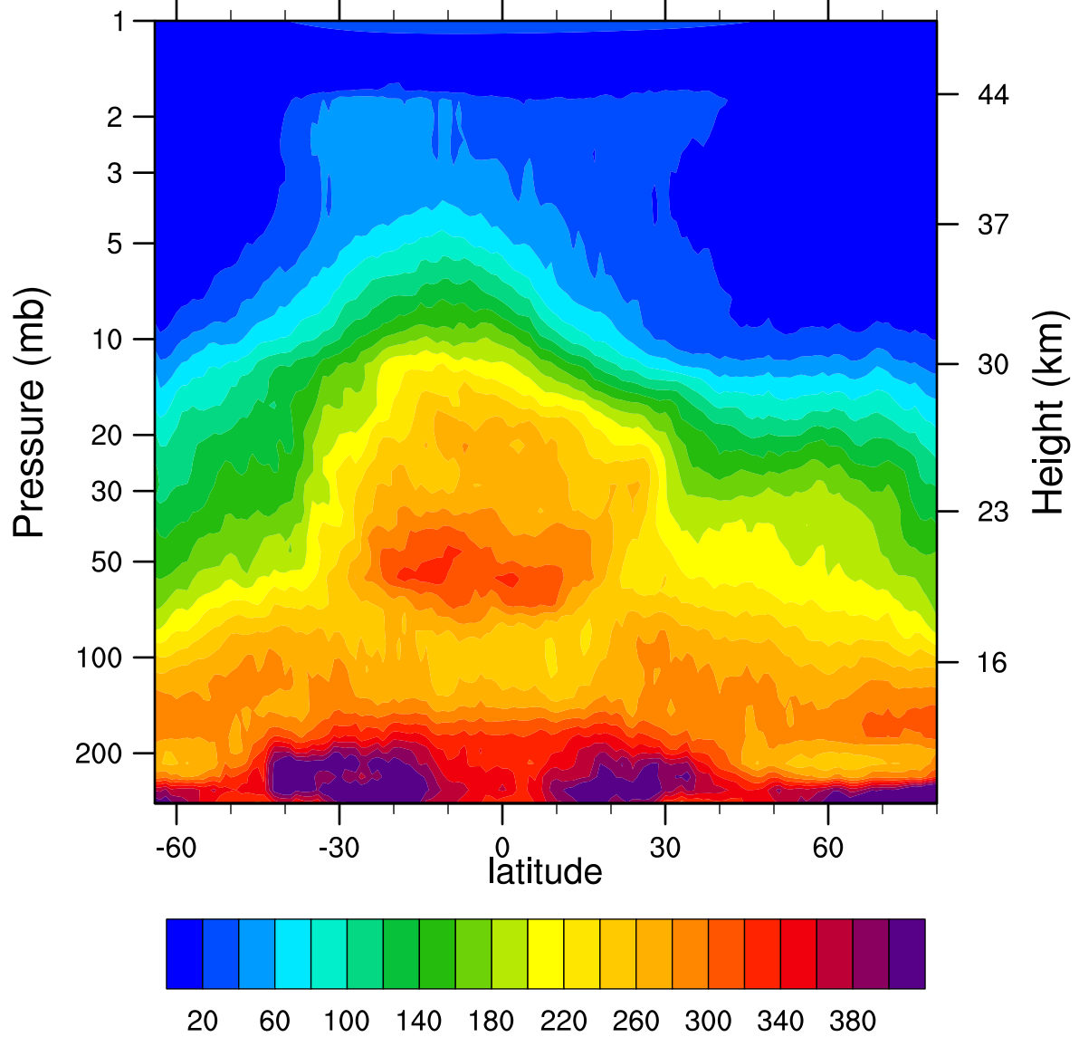
HIRDLSv6 2006d099 N2O_Combined (ppbv)
