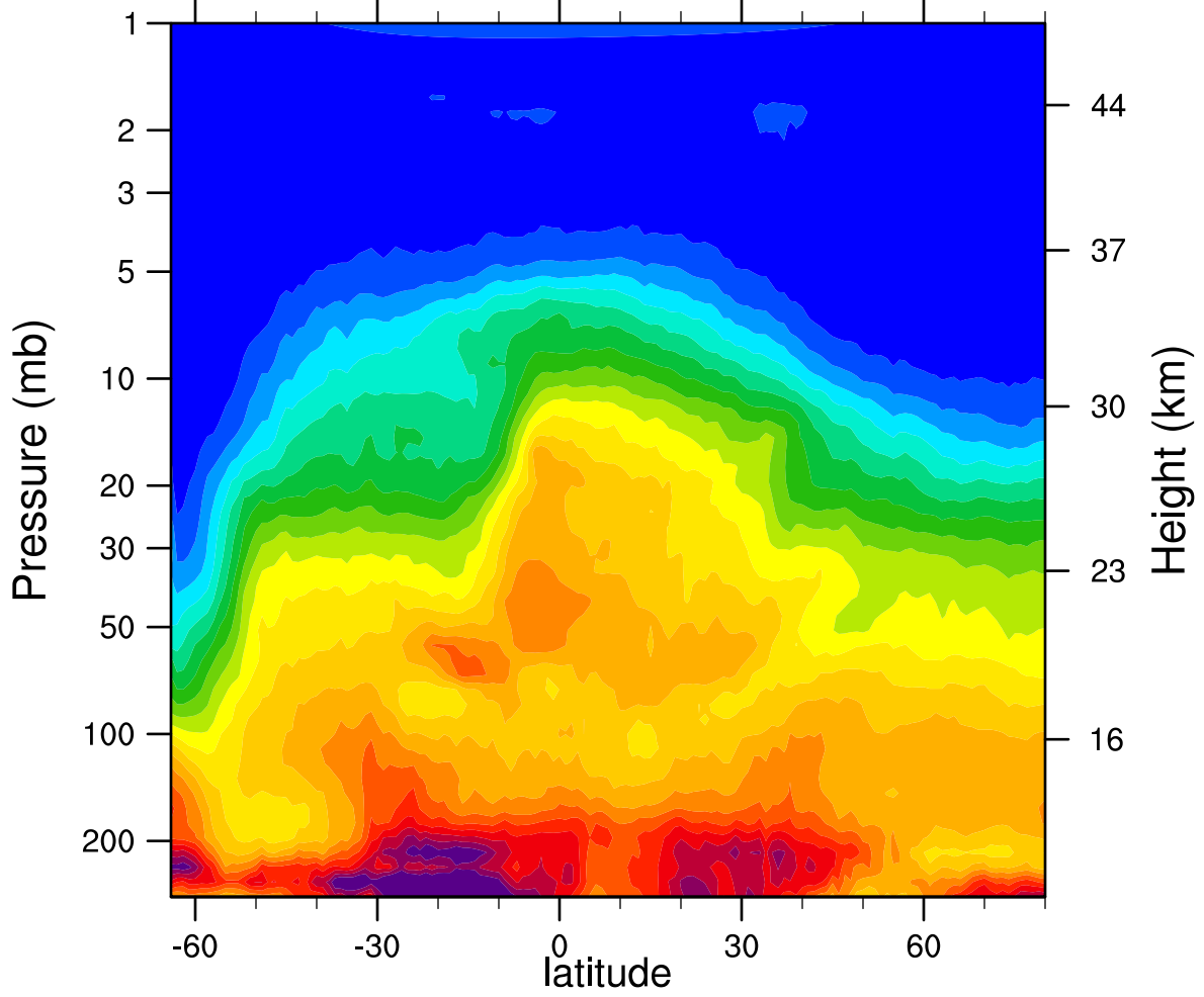
HIRDLSv6 2006d246 N2O_Combined (ppbv)
