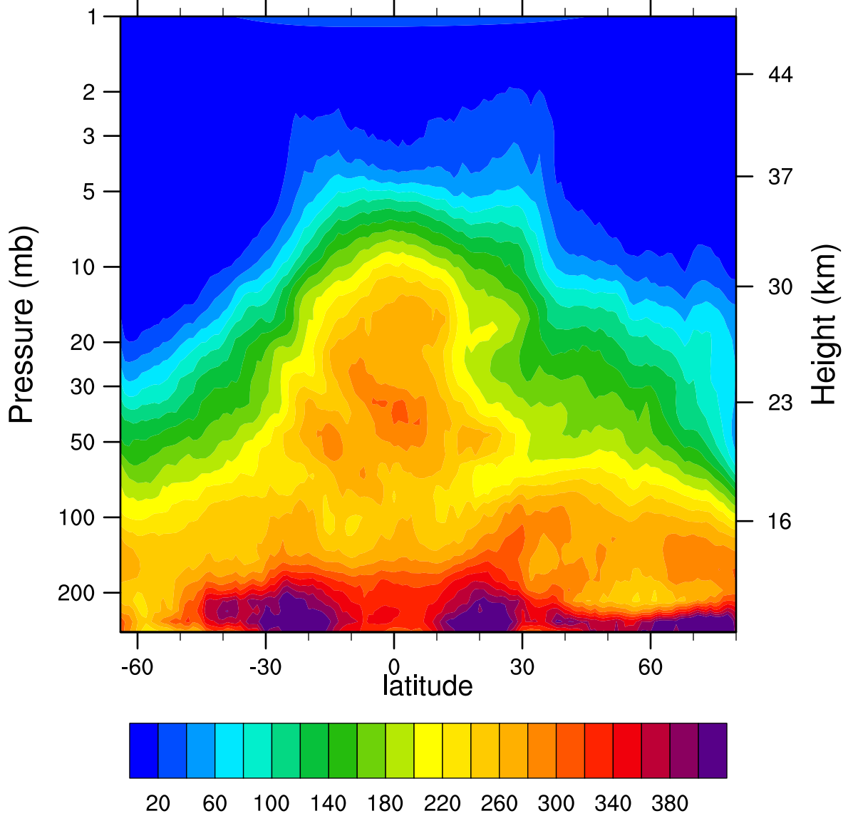
HIRDLSv6 2007d103 N2O_Combined (ppbv)
