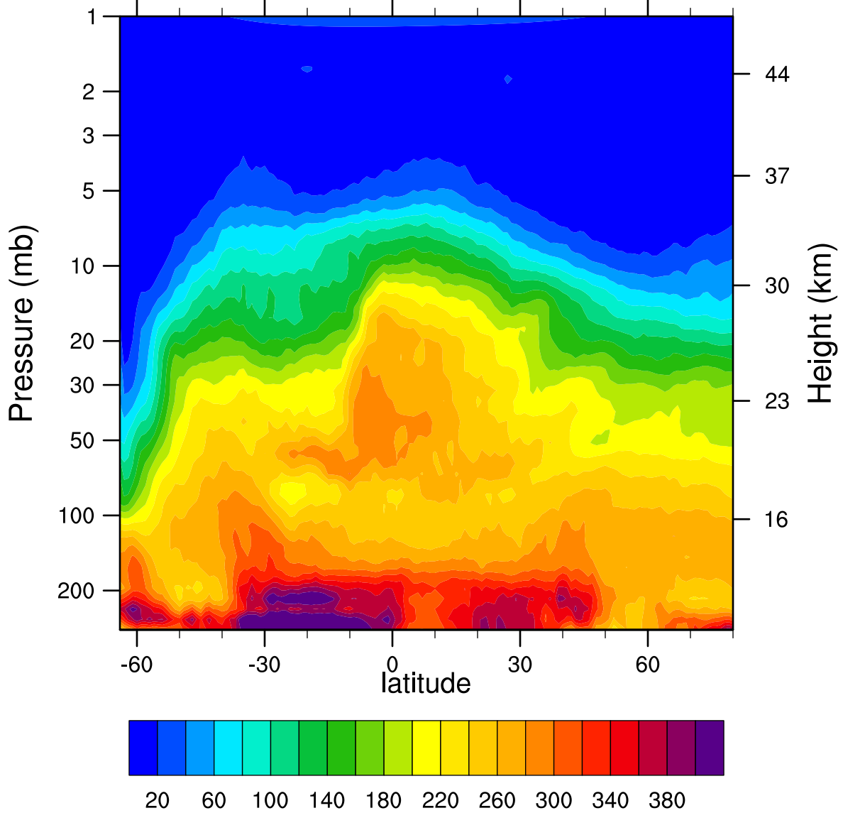
HIRDLSv6 2006d223 N2O_Combined (ppbv)
