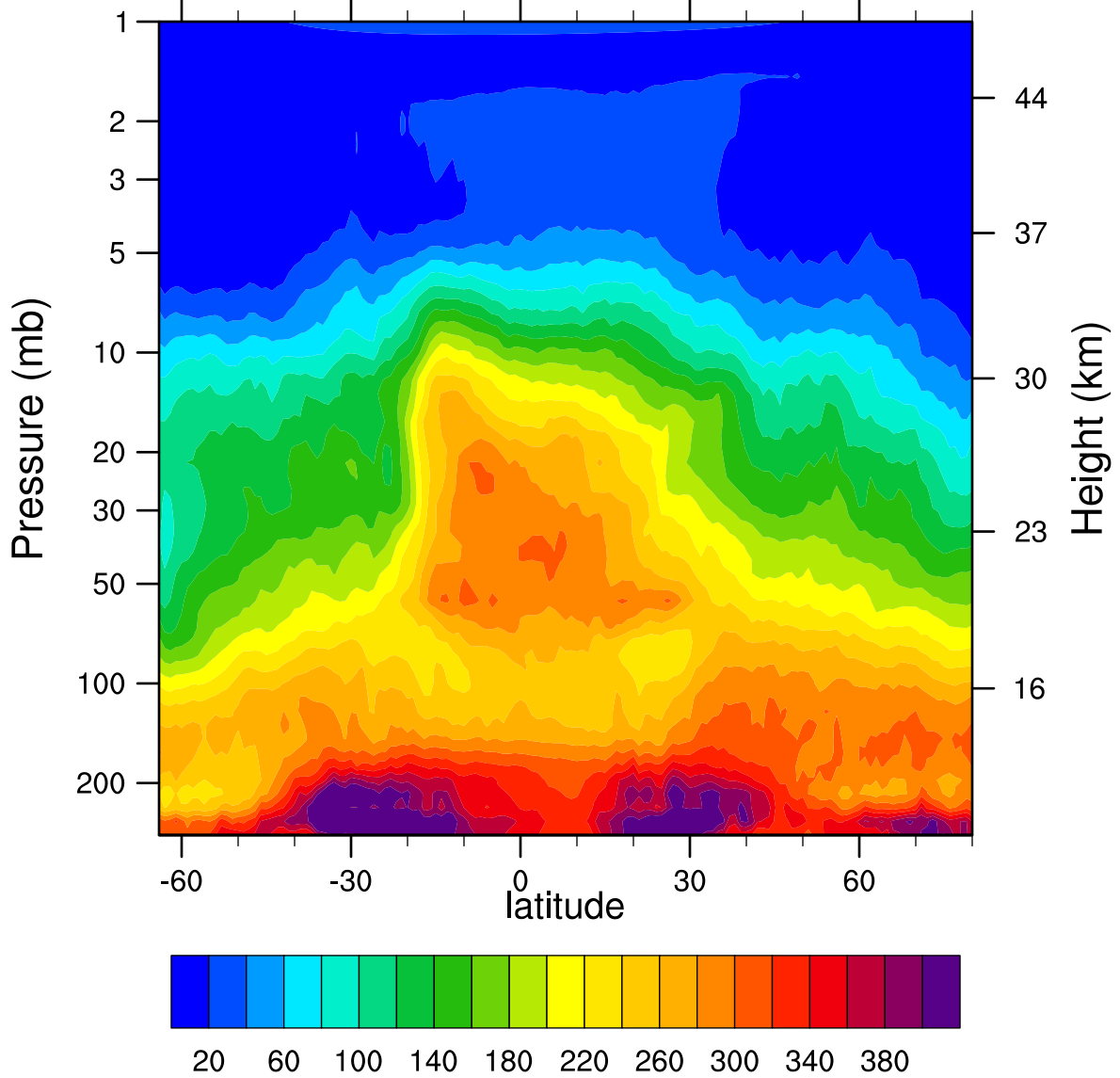
HIRDLSv6 2005d299 N2O_Combined (ppbv)
