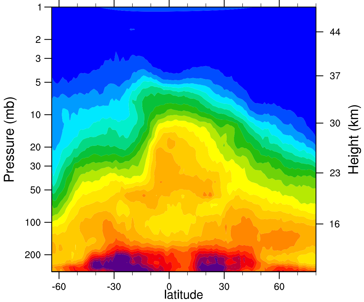
HIRDLSv6 2006d293 N2O_Combined (ppbv)
