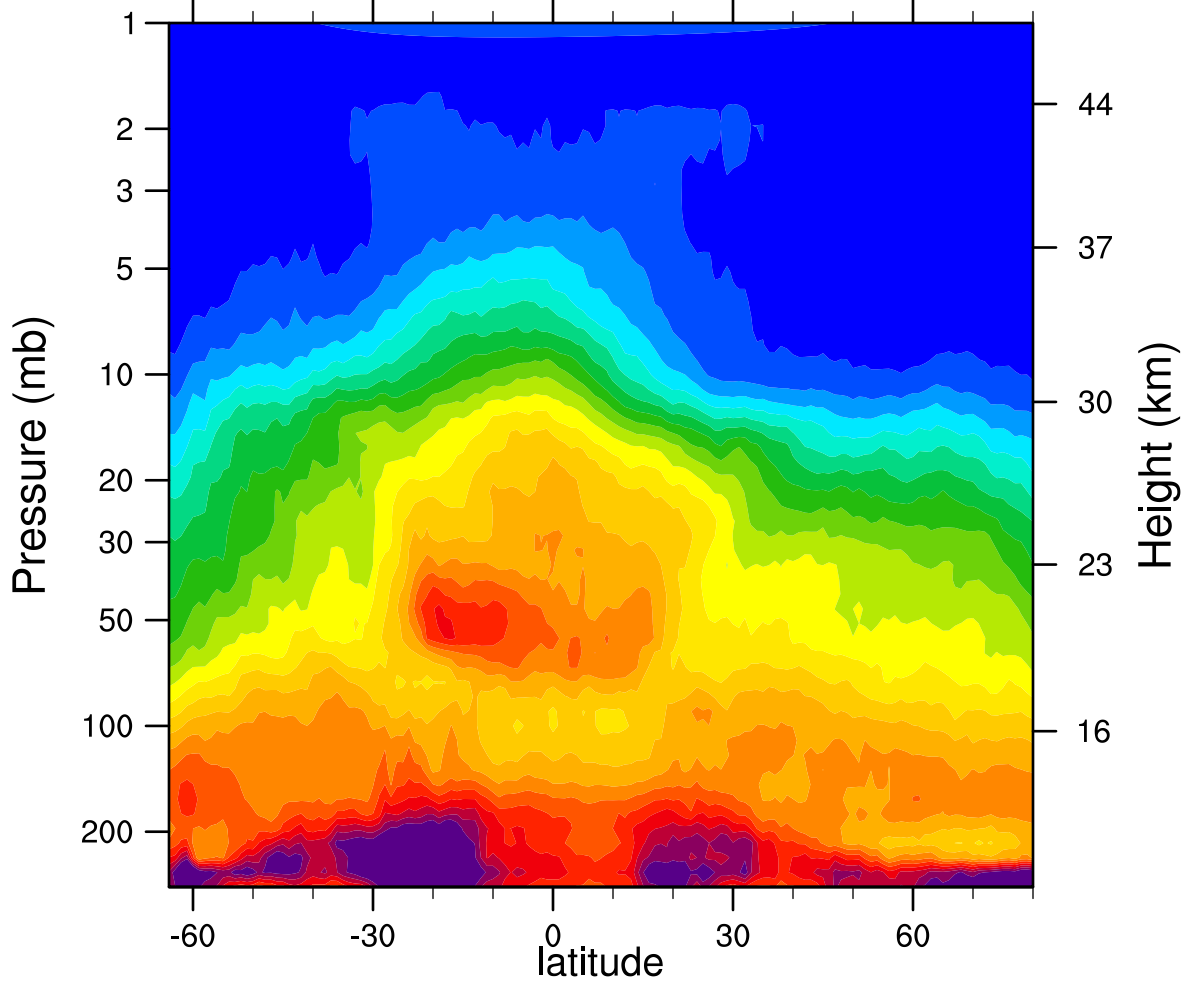
HIRDLSv6 2006d124 N2O_Combined (ppbv)
