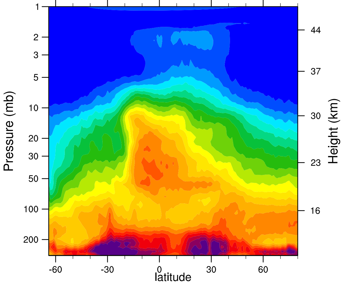
HIRDLSv6 2005d270 N2O_Combined (ppbv)
