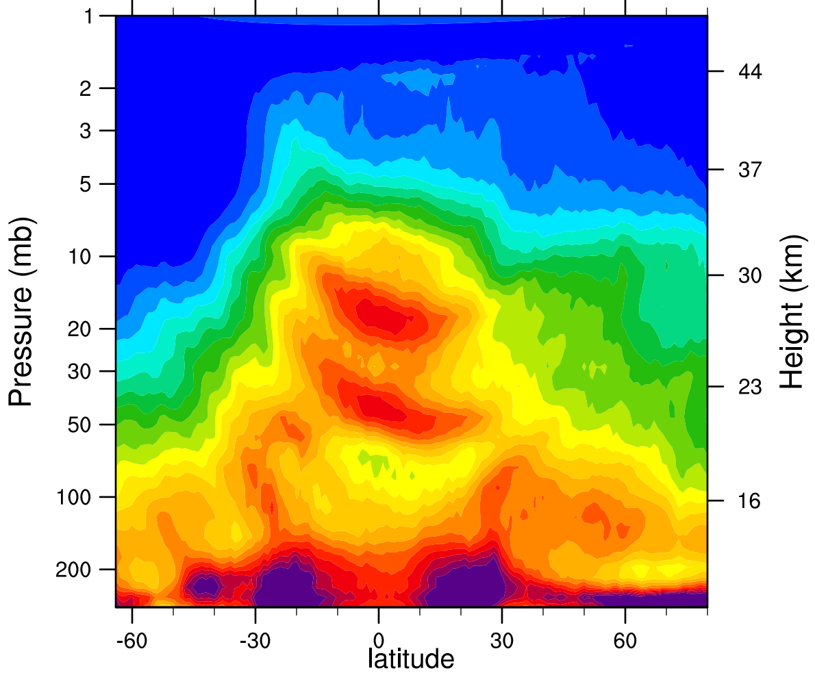
HIRDLSv6 2005d086 N2O_Combined (ppbv)
