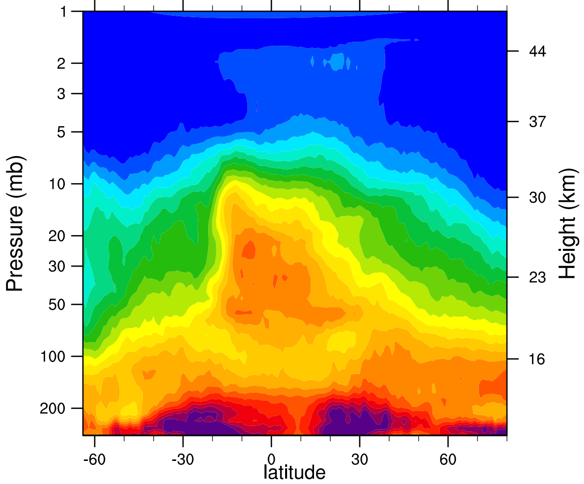
HIRDLSv6 2005d286 N2O_Combined (ppbv)
