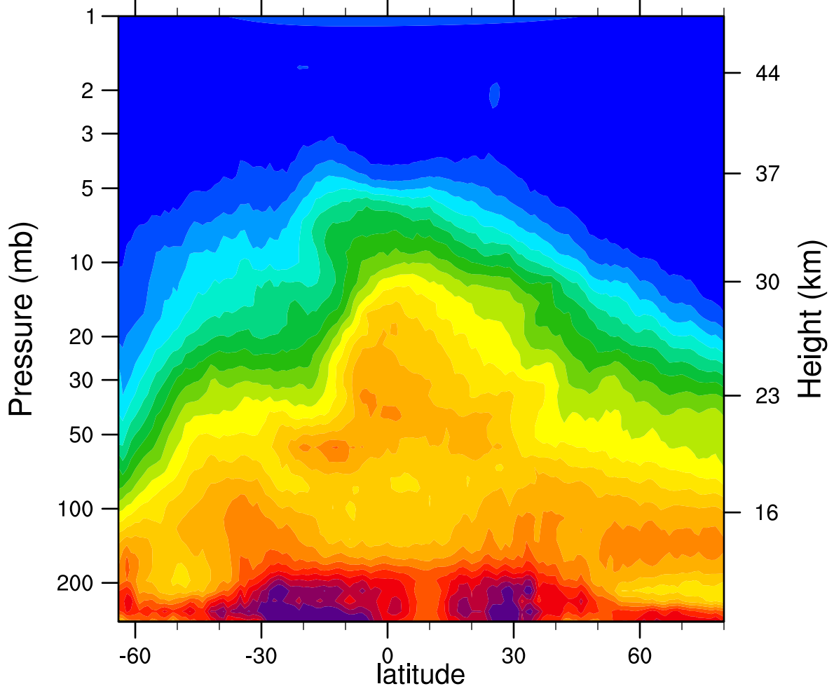
HIRDLSv6 2006d276 N2O_Combined (ppbv)
