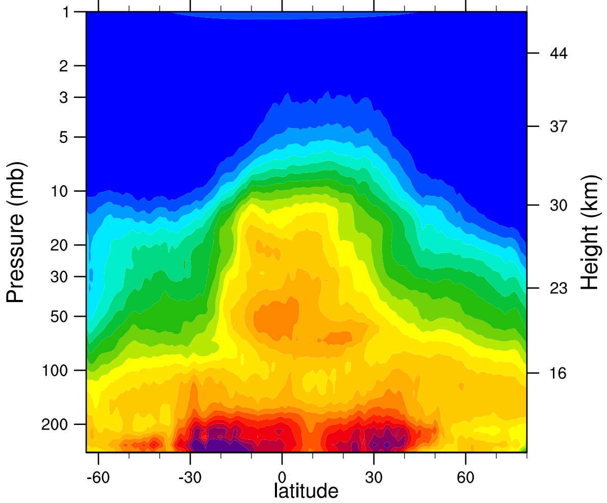
HIRDLSv6 2007d263 N2O_Combined (ppbv)
