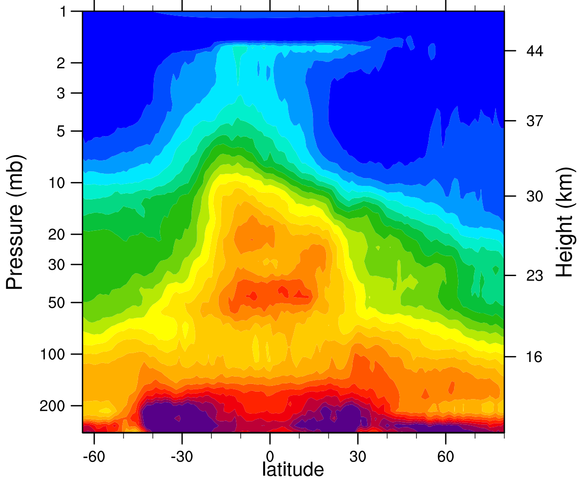
HIRDLSv6 2006d021 N2O_Combined (ppbv)
