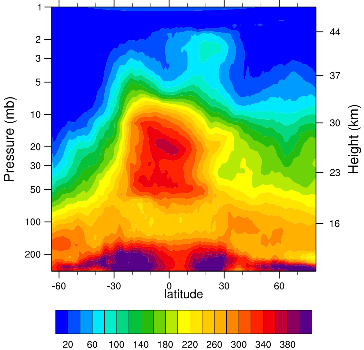
HIRDLSv6 2005d132 N2O_Combined (ppbv)
