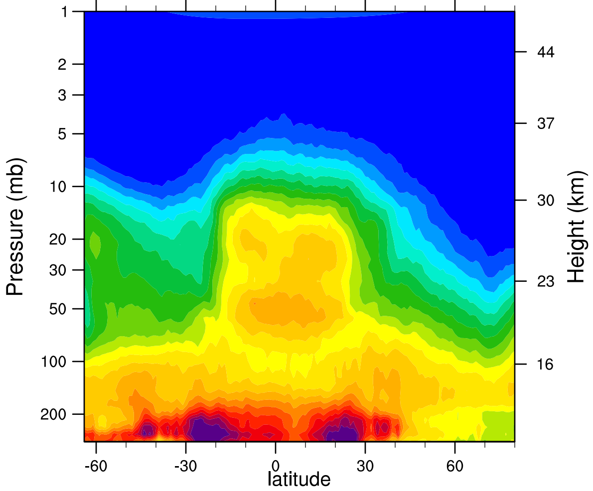
HIRDLSv6 2007d319 N2O_Combined (ppbv)
