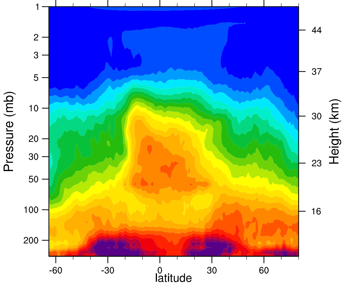
HIRDLSv6 2005d300 N2O_Combined (ppbv)
