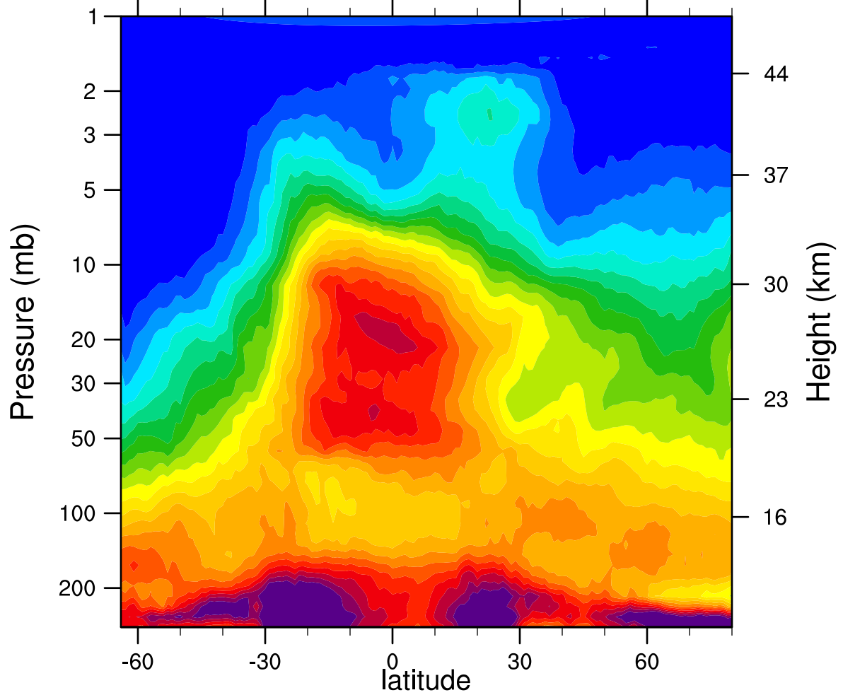
HIRDLSv6 2005d127 N2O_Combined (ppbv)
