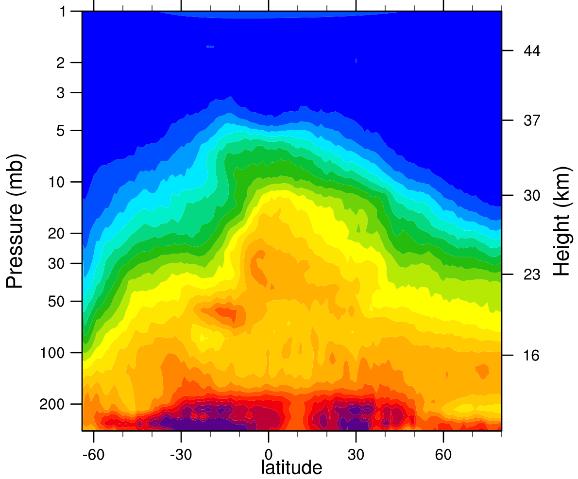
HIRDLSv6 2006d269 N2O_Combined (ppbv)
