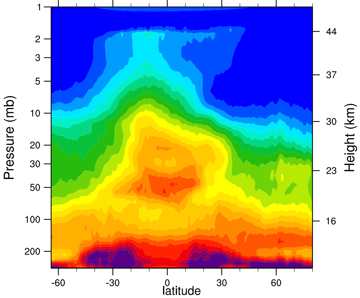
HIRDLSv6 2006d045 N2O_Combined (ppbv)
