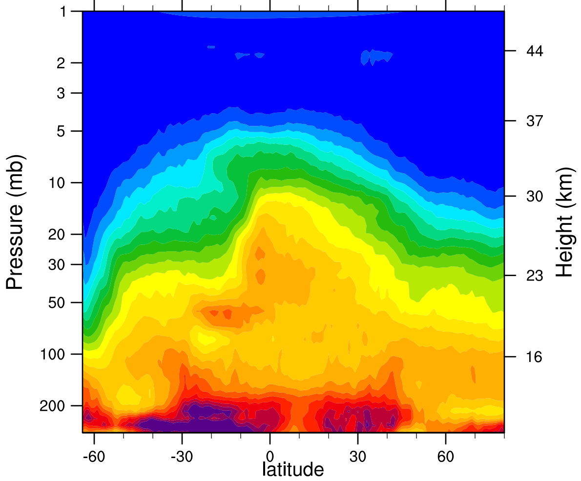
HIRDLSv6 2006d255 N2O_Combined (ppbv)
