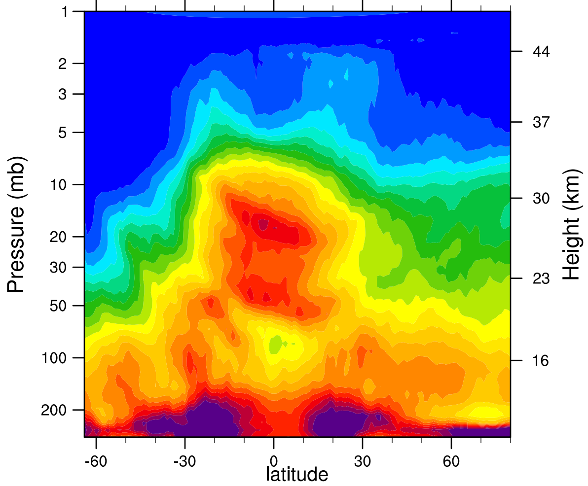
HIRDLSv6 2005d111 N2O_Combined (ppbv)
