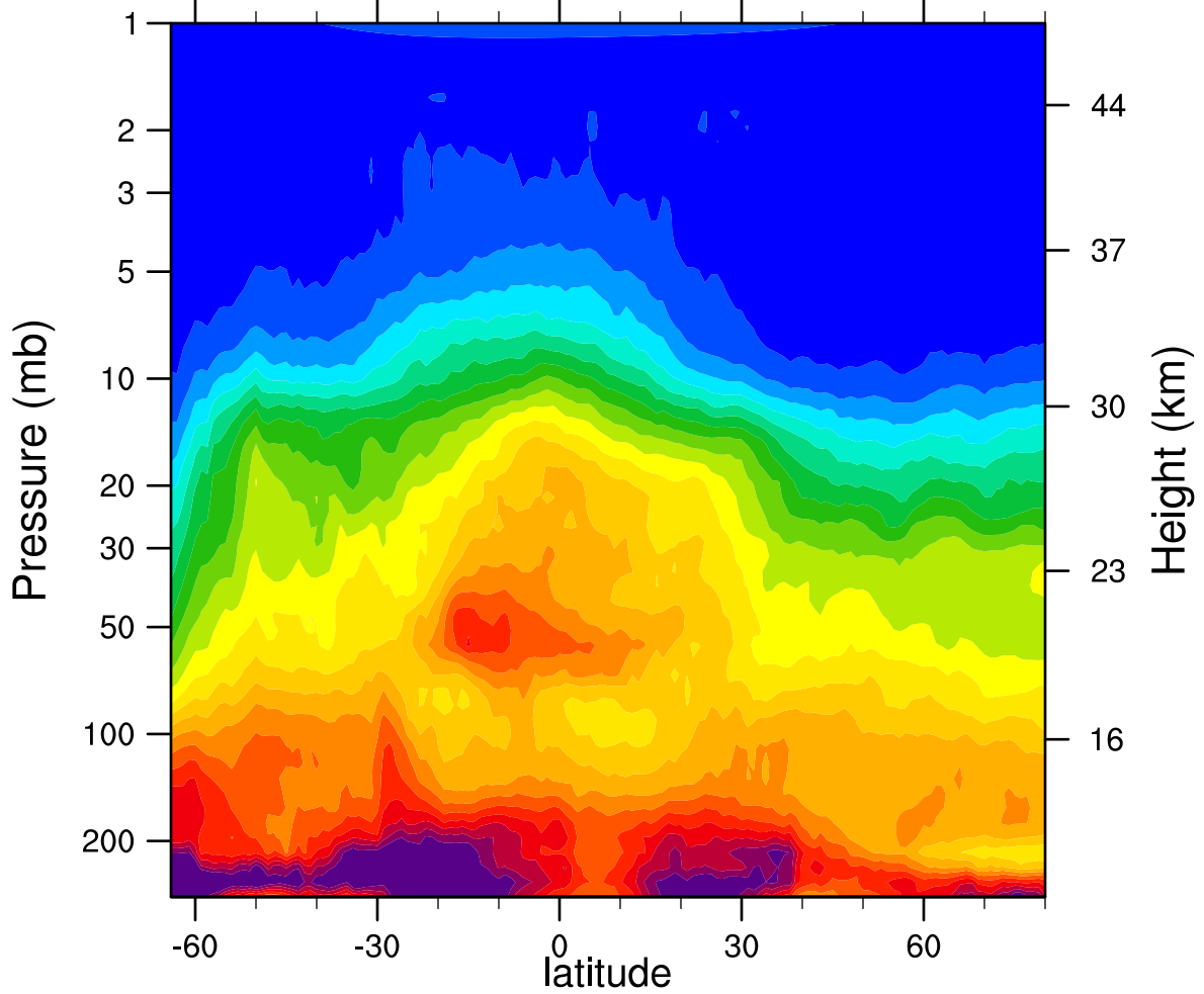
HIRDLSv6 2006d150 N2O_Combined (ppbv)
