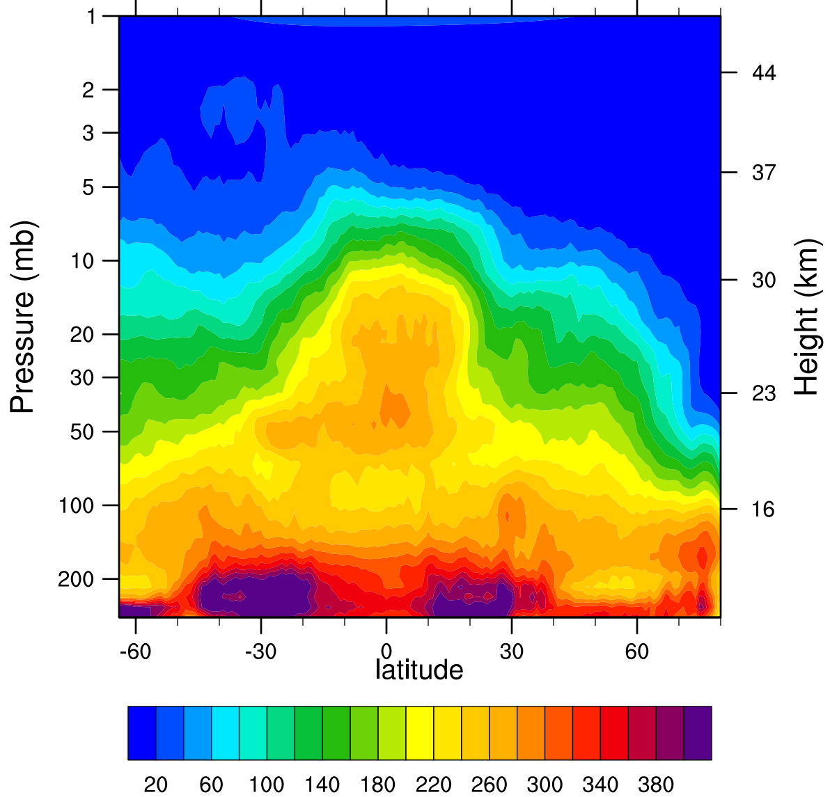
HIRDLSv6 2007d009 N2O_Combined (ppbv)
