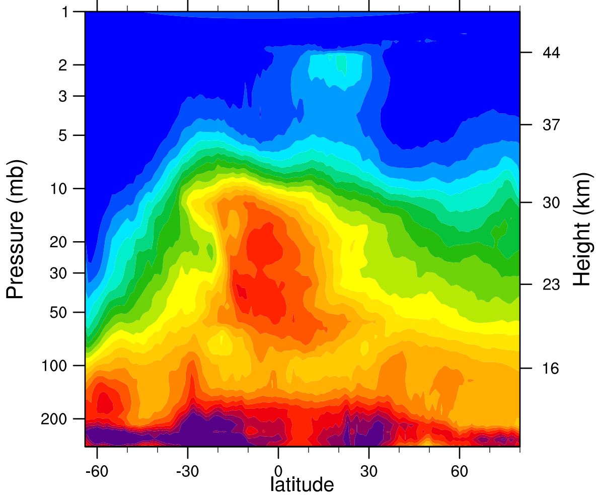
HIRDLSv6 2005d179 N2O_Combined (ppbv)
