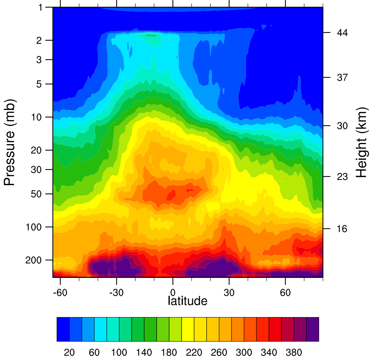
HIRDLSv6 2006d063 N2O_Combined (ppbv)
