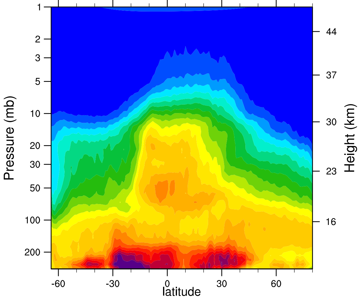
HIRDLSv6 2007d269 N2O_Combined (ppbv)
