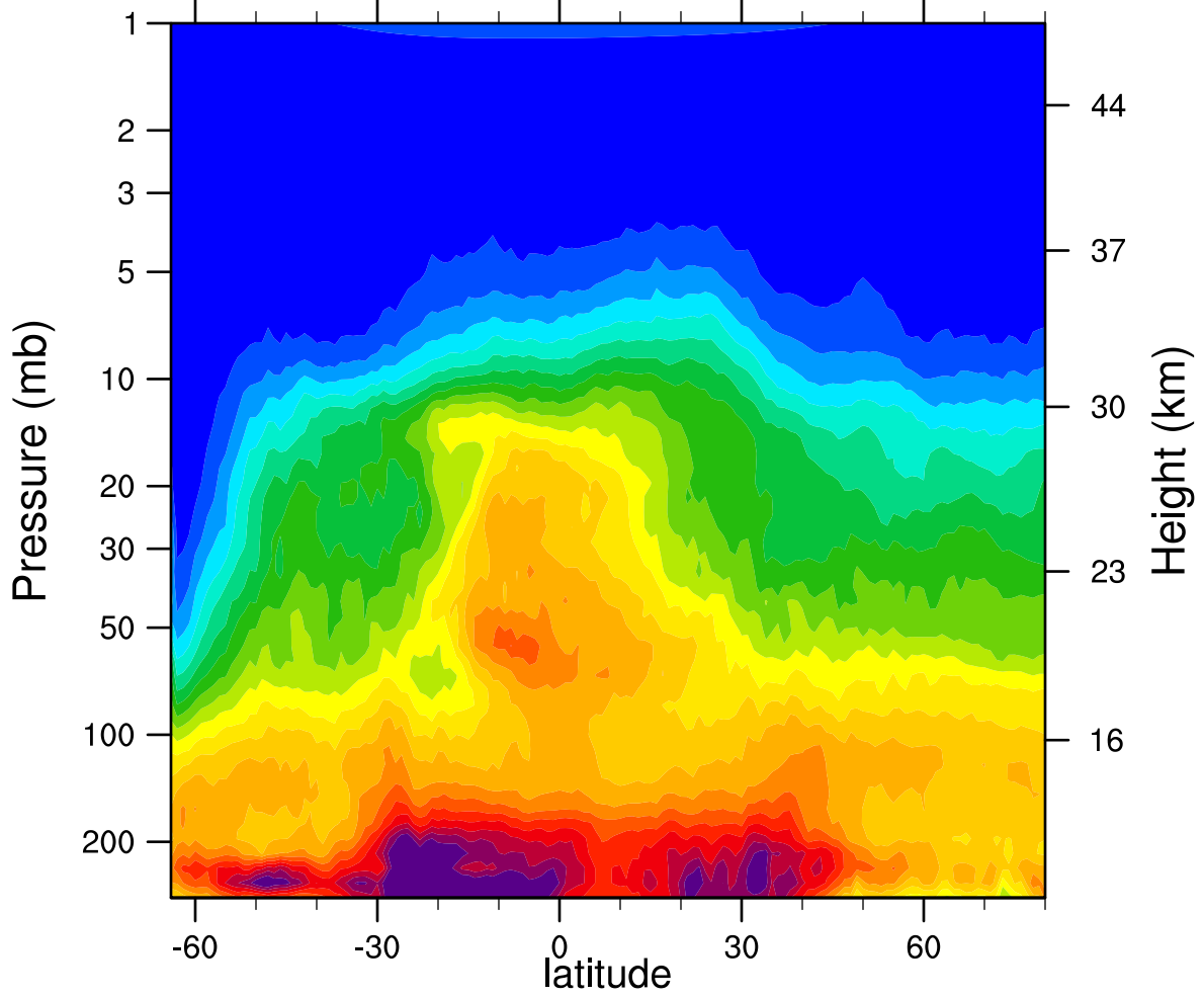
HIRDLSv6 2007d194 N2O_Combined (ppbv)
