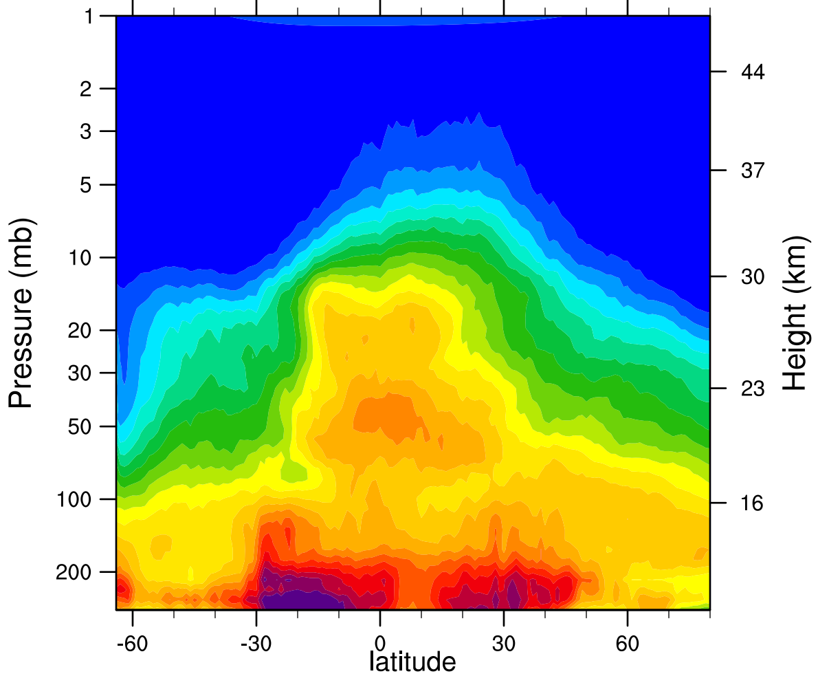
HIRDLSv6 2007d250 N2O_Combined (ppbv)
