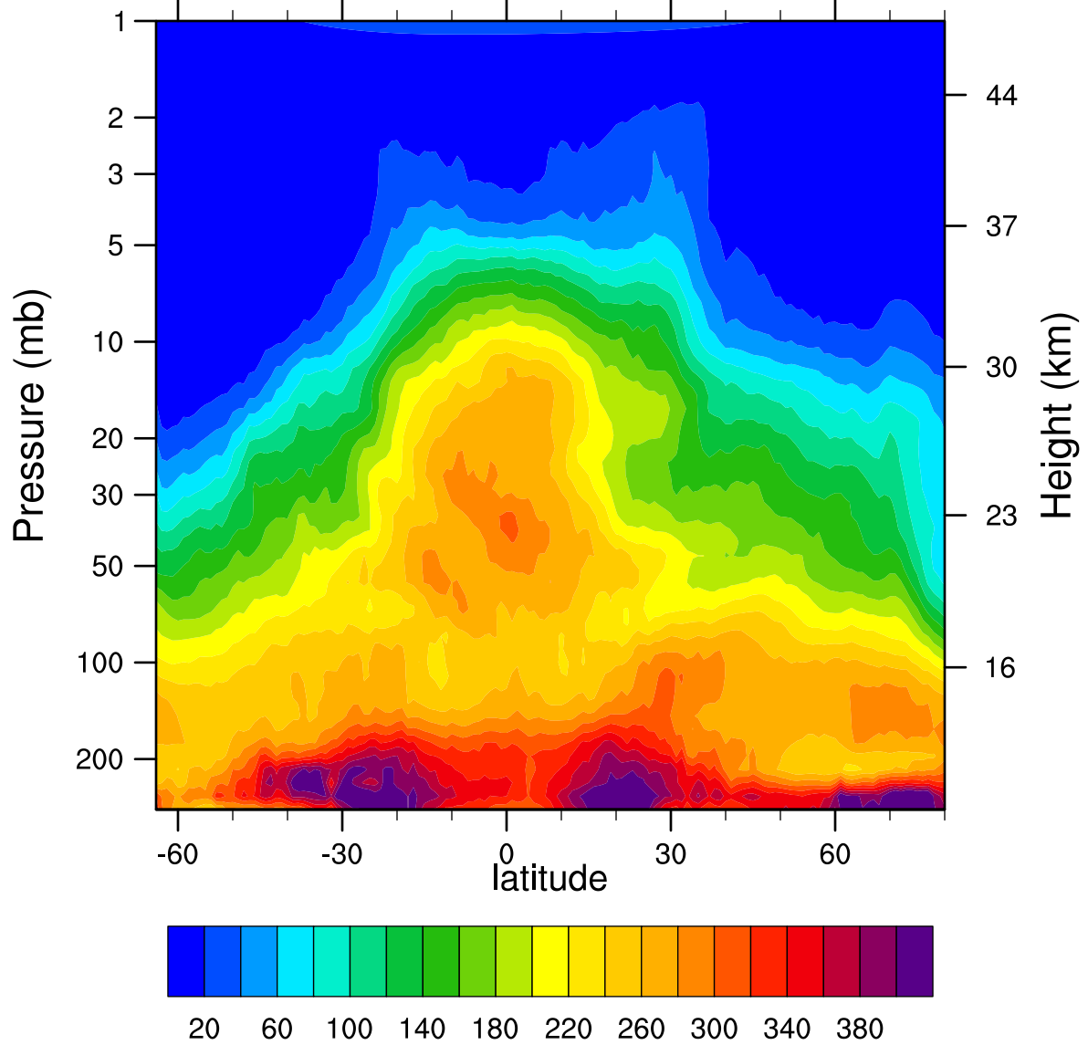
HIRDLSv6 2007d107 N2O_Combined (ppbv)
