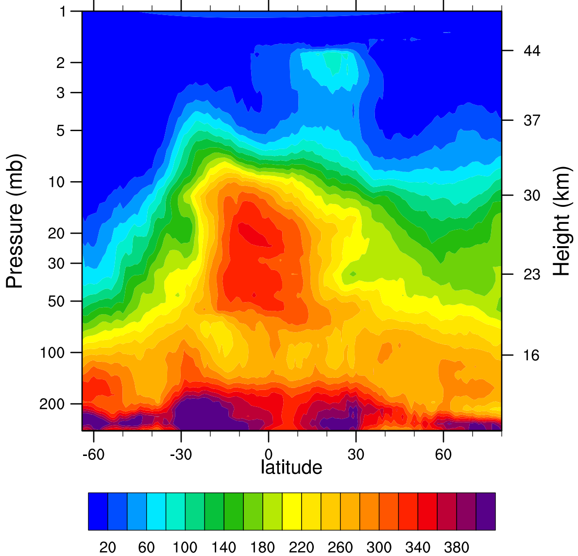
HIRDLSv6 2005d157 N2O_Combined (ppbv)
