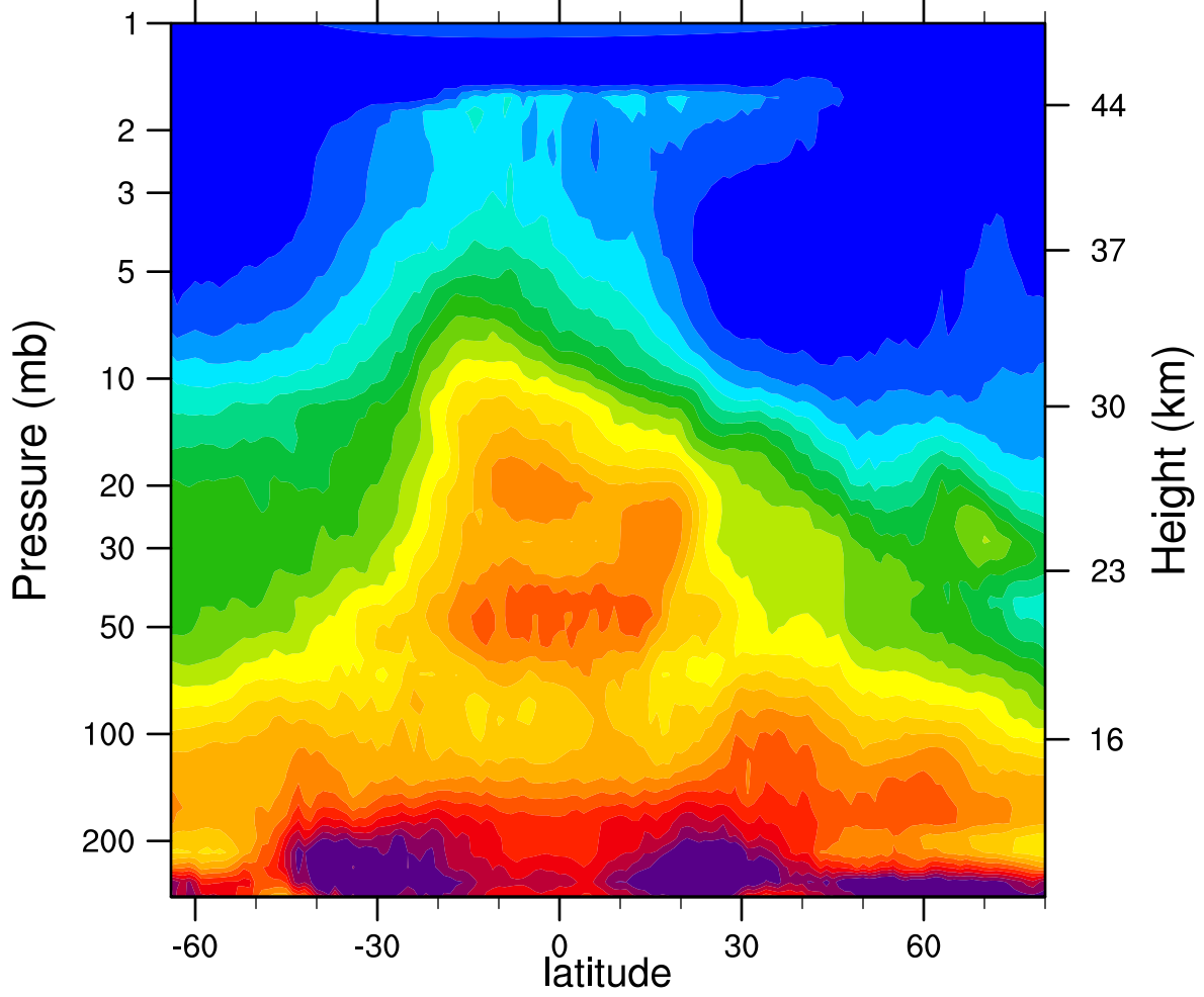
HIRDLSv6 2006d027 N2O_Combined (ppbv)
