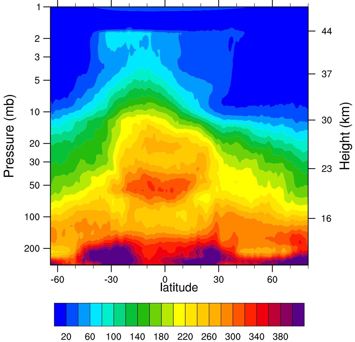
HIRDLSv6 2006d078 N2O_Combined (ppbv)
