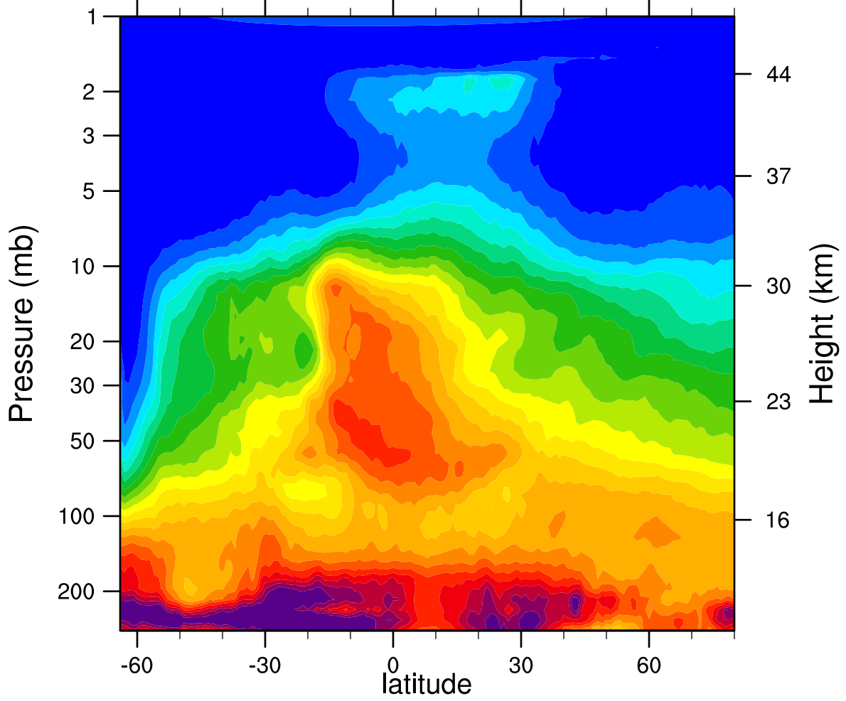
HIRDLSv6 2005d221 N2O_Combined (ppbv)
