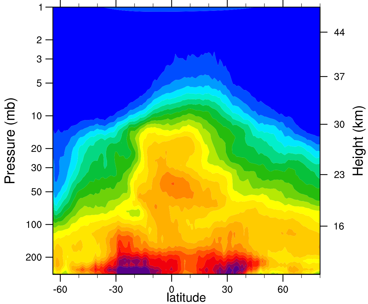
HIRDLSv6 2007d240 N2O_Combined (ppbv)
