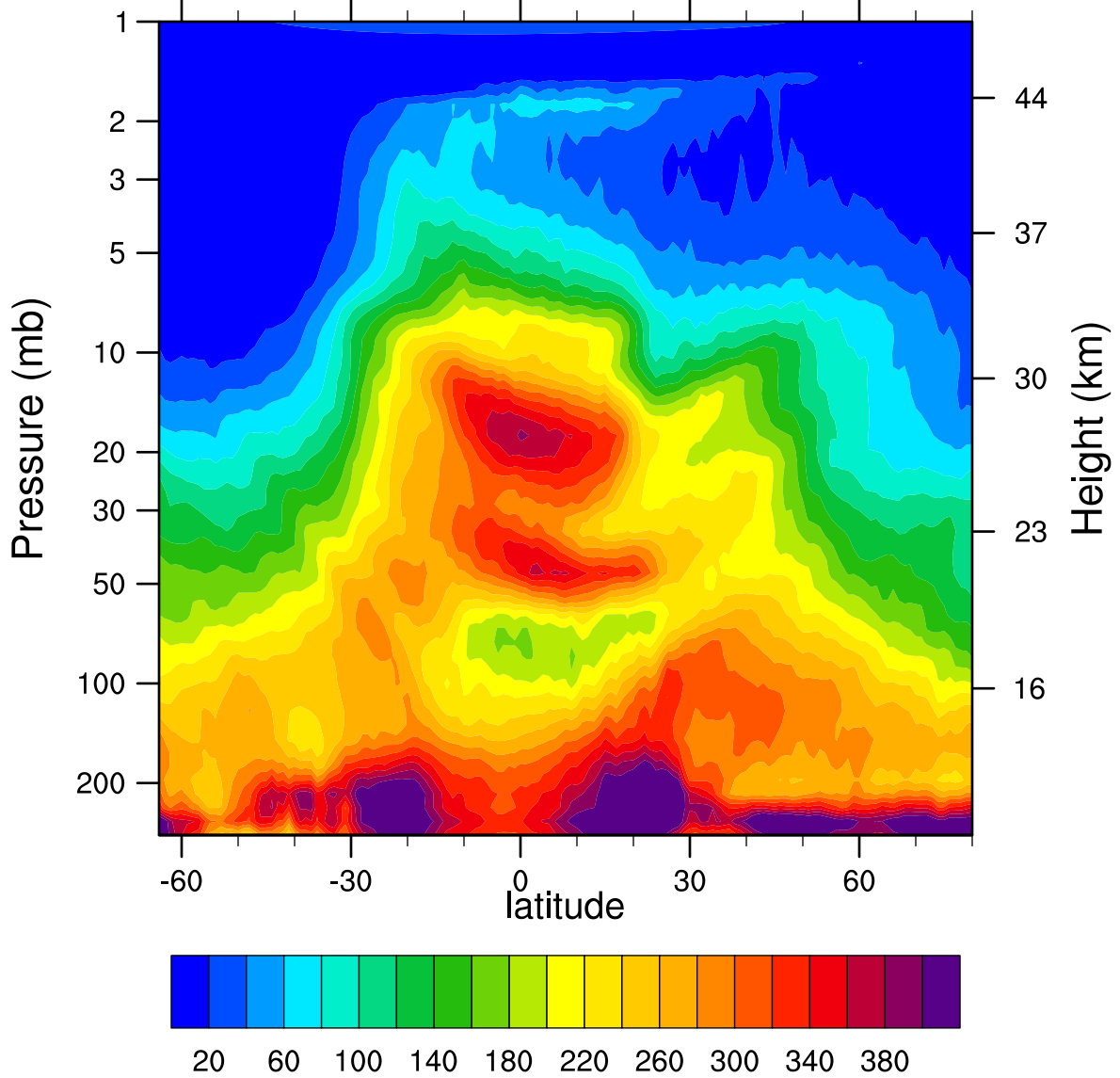
HIRDLSv6 2005d060 N2O_Combined (ppbv)
