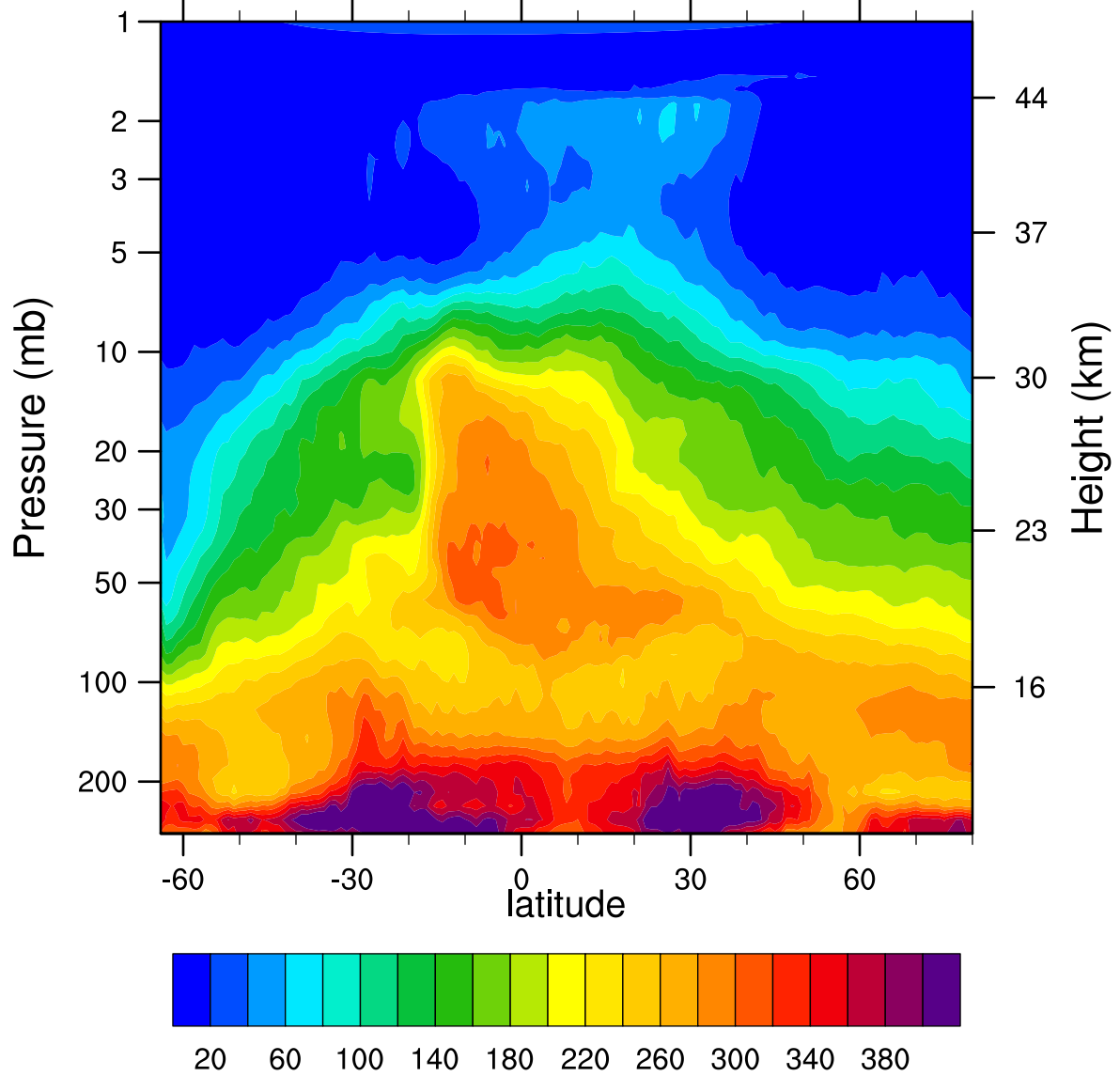
HIRDLSv6 2005d252 N2O_Combined (ppbv)
