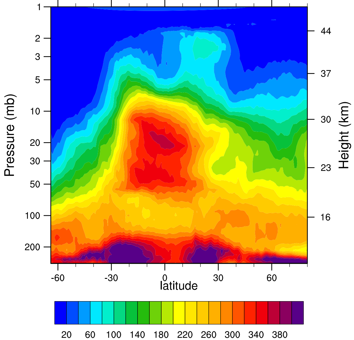
HIRDLSv6 2005d129 N2O_Combined (ppbv)
