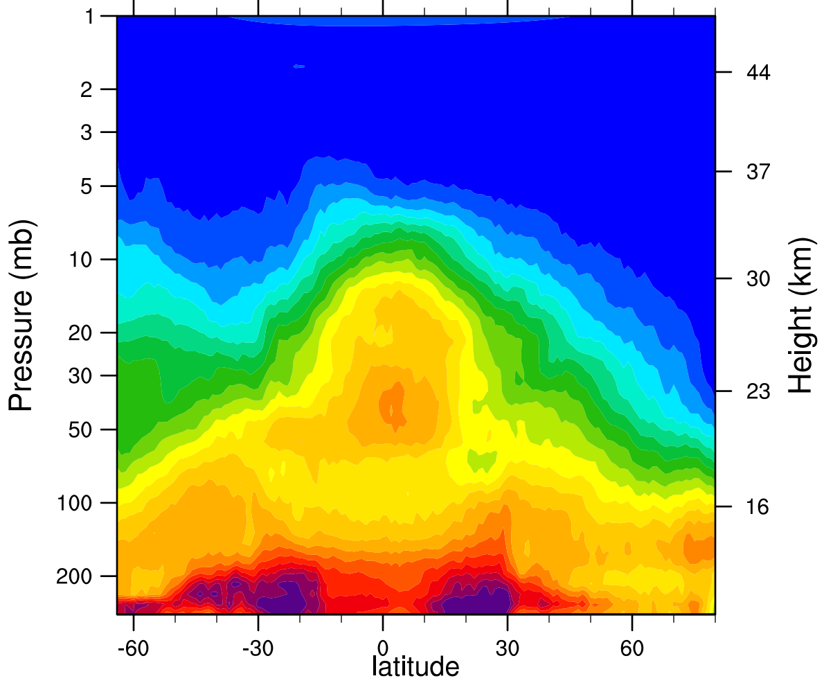
HIRDLSv6 2006d355 N2O_Combined (ppbv)
