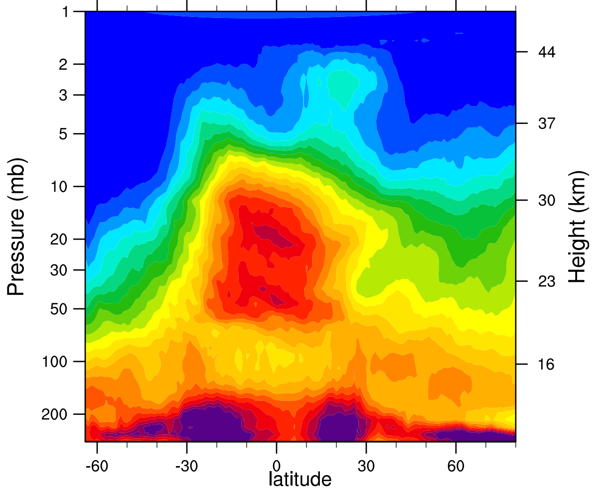
HIRDLSv6 2005d122 N2O_Combined (ppbv)
