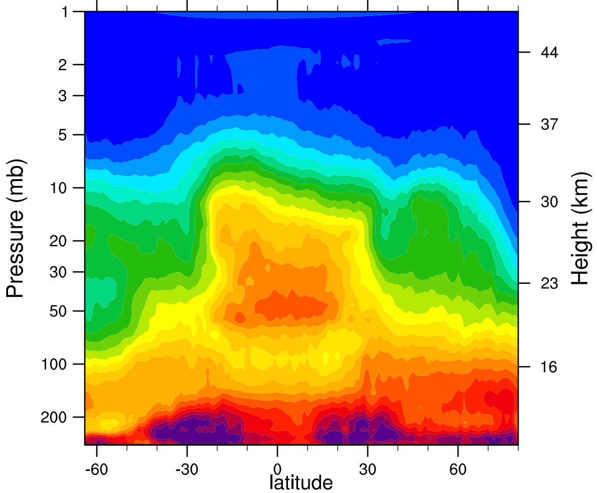
HIRDLSv6 2005d325 N2O_Combined (ppbv)
