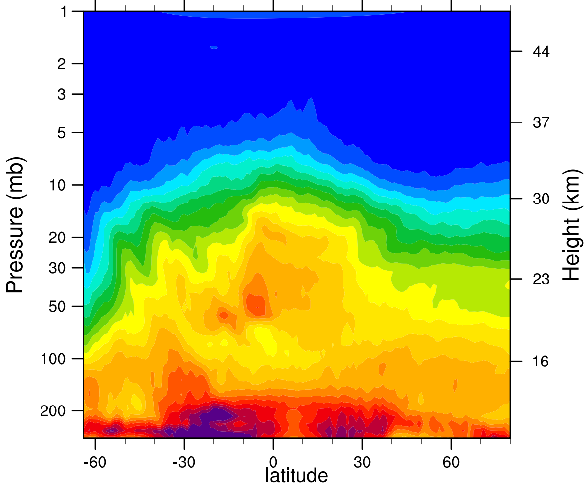
HIRDLSv6 2006d180 N2O_Combined (ppbv)
