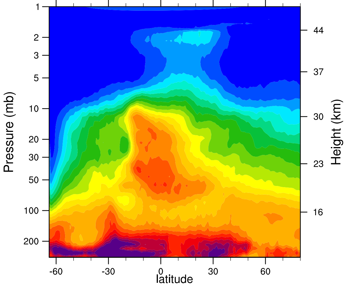
HIRDLSv6 2005d228 N2O_Combined (ppbv)
