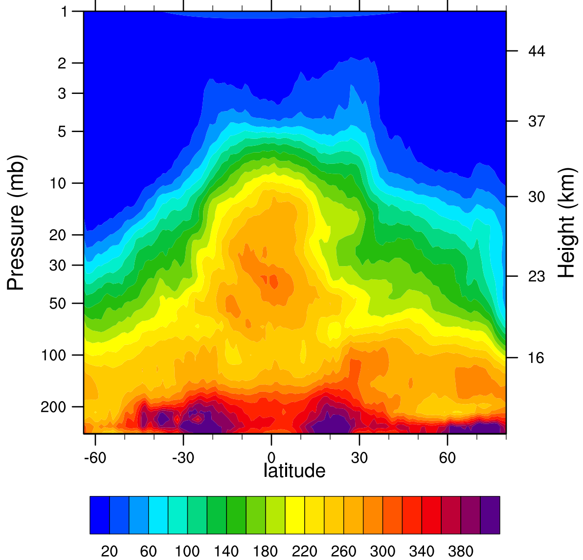
HIRDLSv6 2007d106 N2O_Combined (ppbv)
