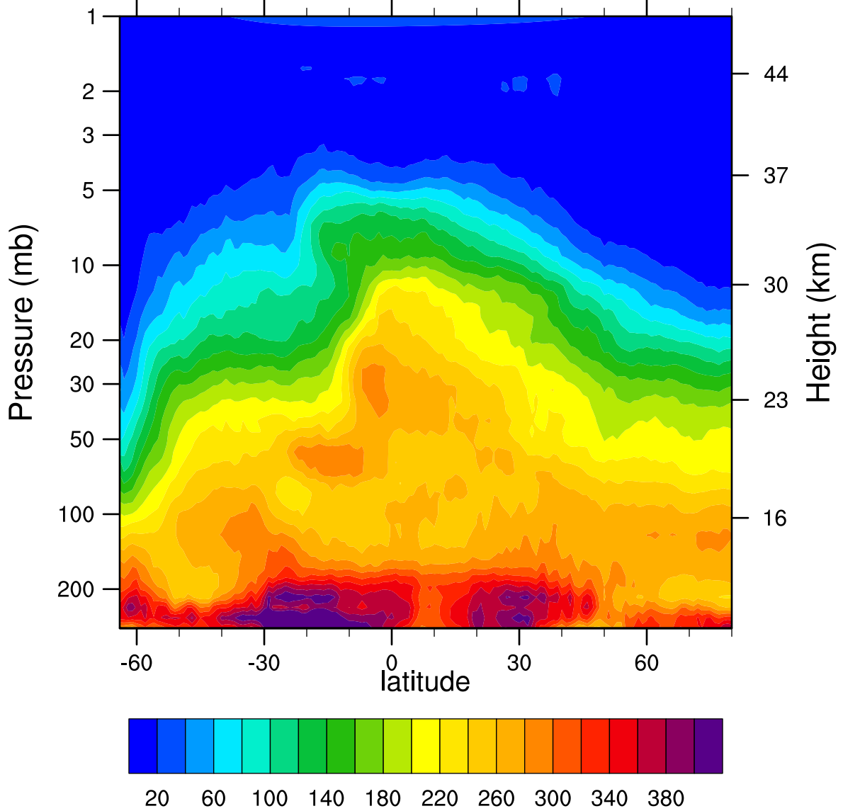
HIRDLSv6 2006d264 N2O_Combined (ppbv)
