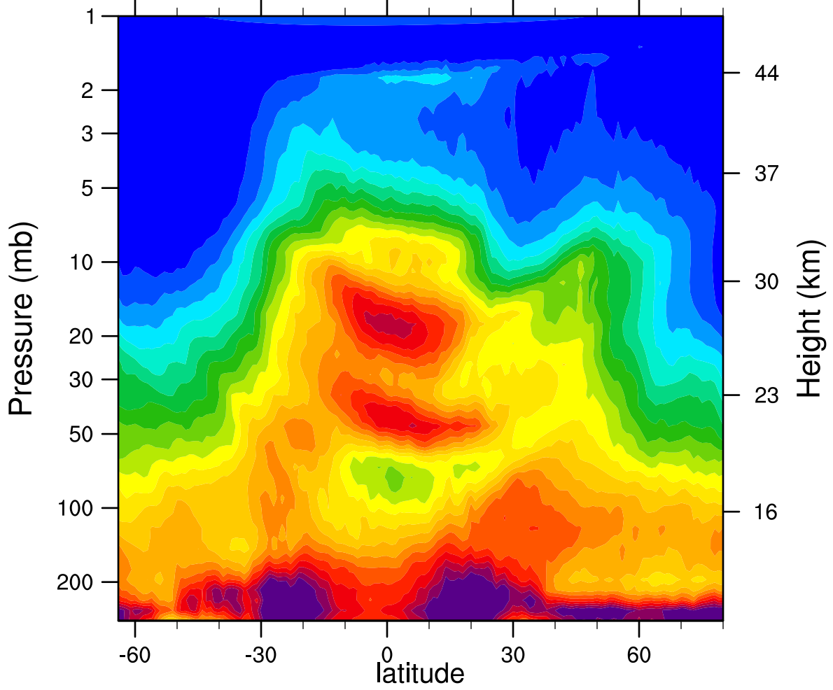
HIRDLSv6 2005d067 N2O_Combined (ppbv)
