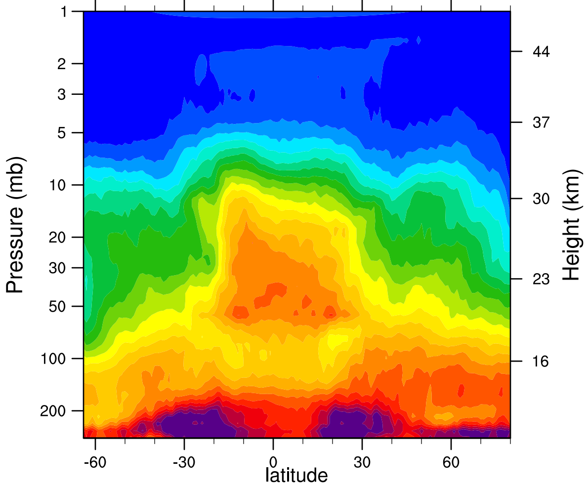
HIRDLSv6 2005d310 N2O_Combined (ppbv)
