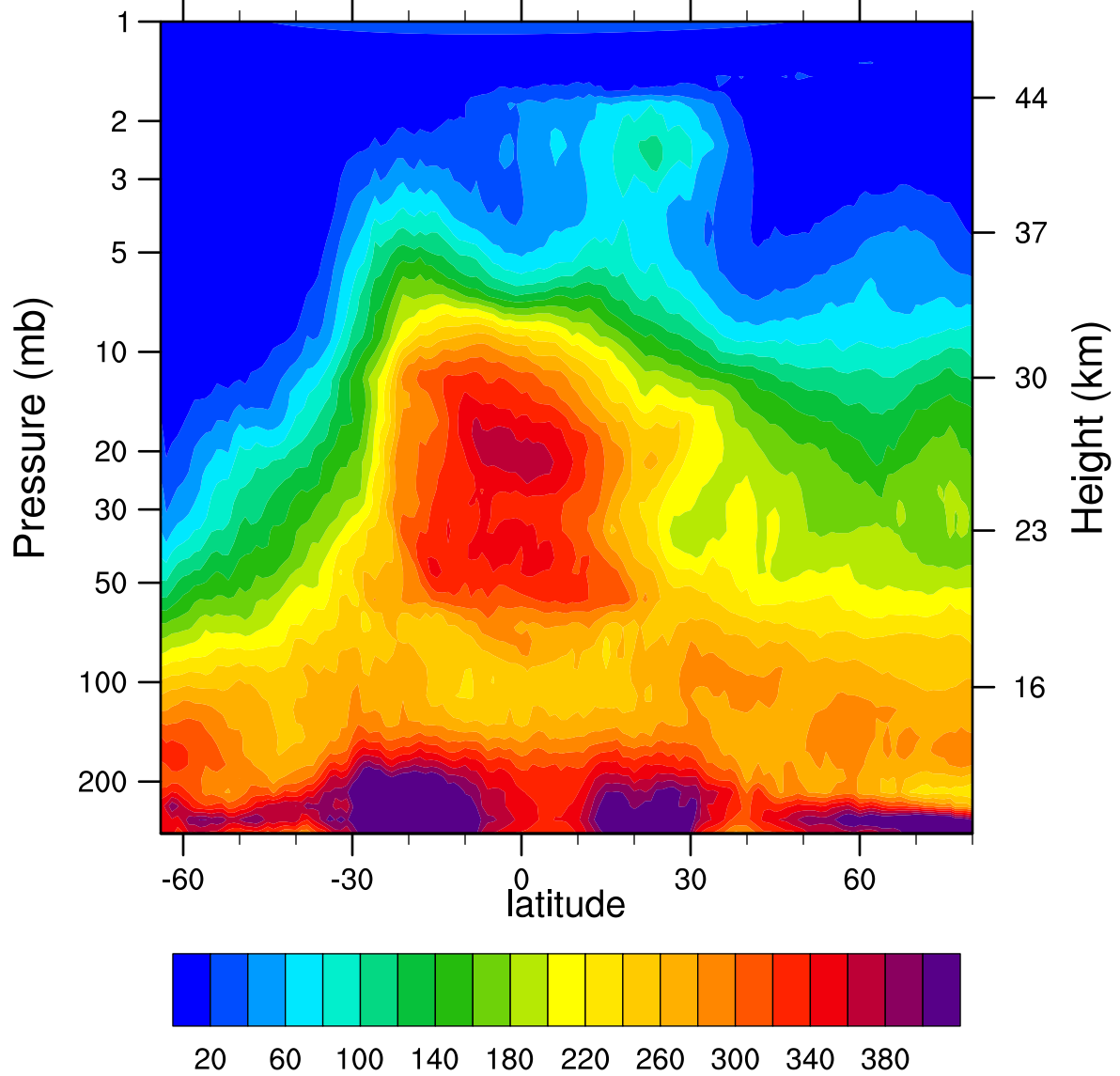
HIRDLSv6 2005d136 N2O_Combined (ppbv)
