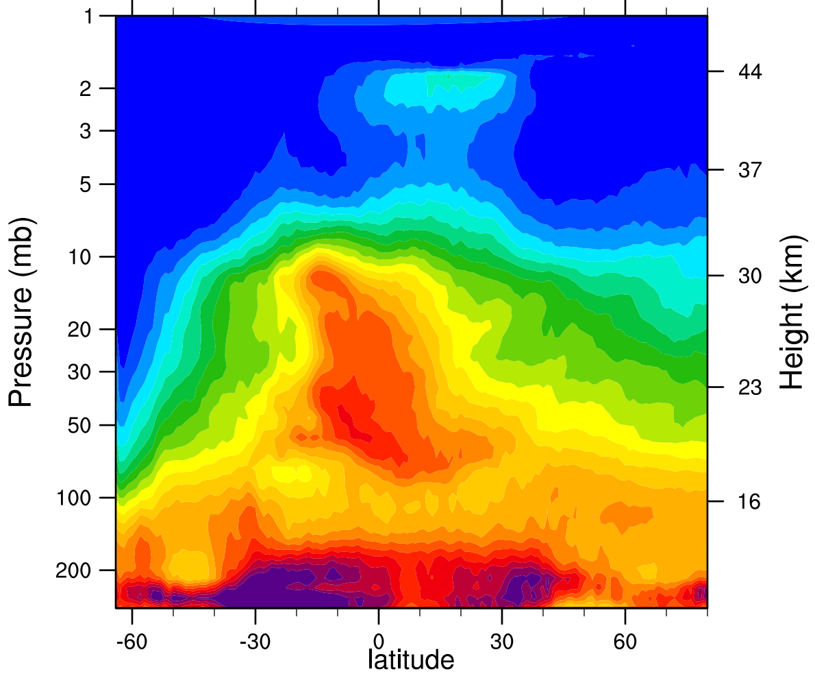
HIRDLSv6 2005d210 N2O_Combined (ppbv)
