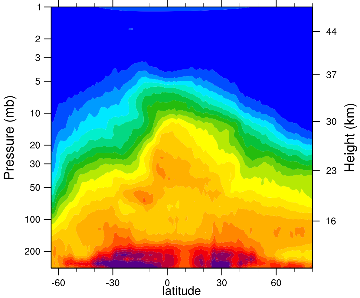
HIRDLSv6 2006d271 N2O_Combined (ppbv)
