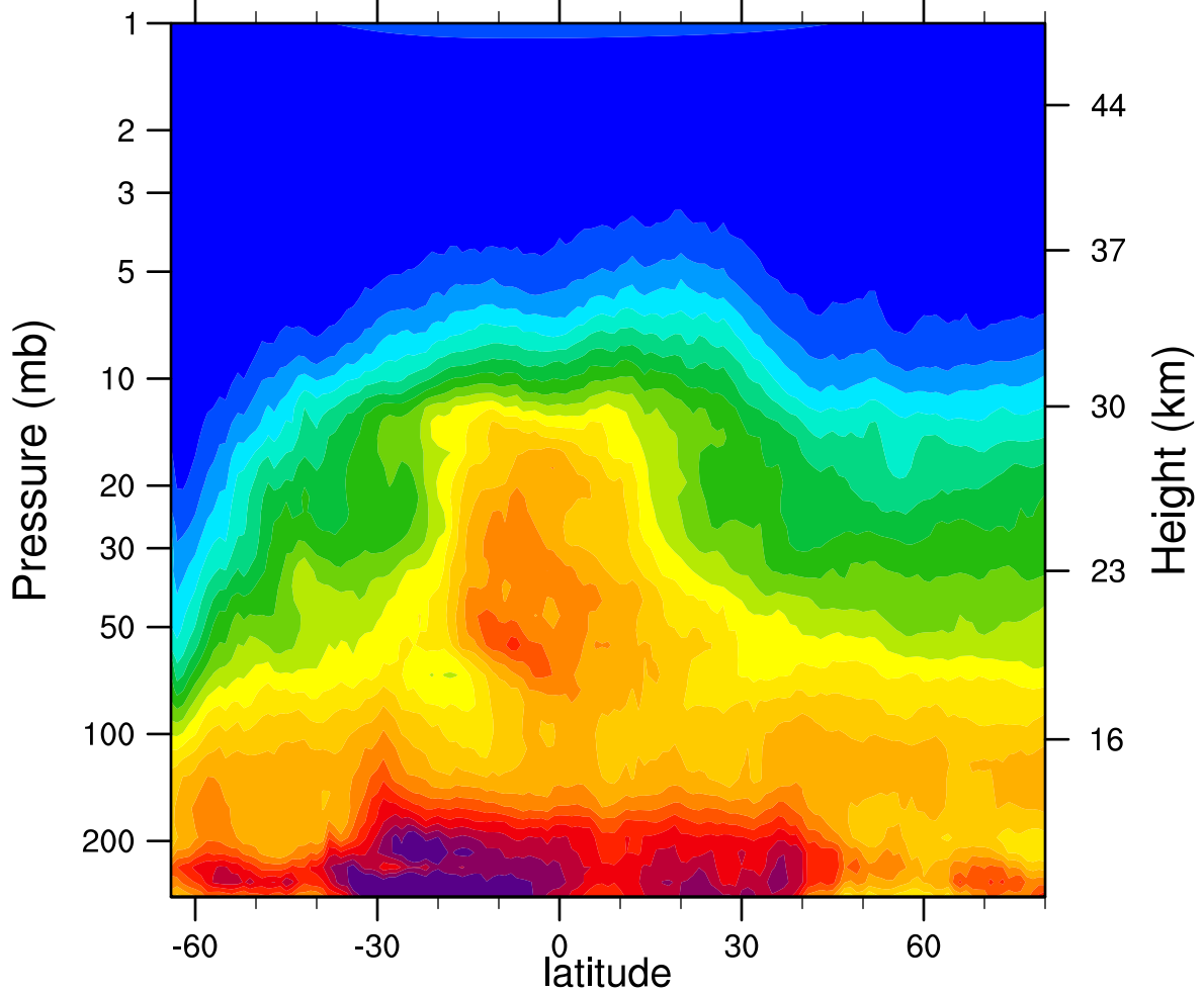
HIRDLSv6 2007d184 N2O_Combined (ppbv)
