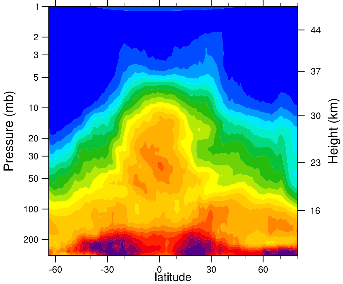
HIRDLSv6 2007d108 N2O_Combined (ppbv)
