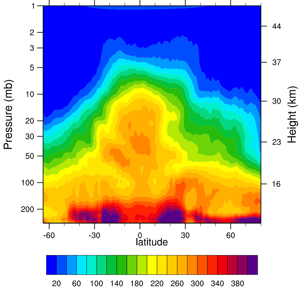
HIRDLSv6 2007d096 N2O_Combined (ppbv)
