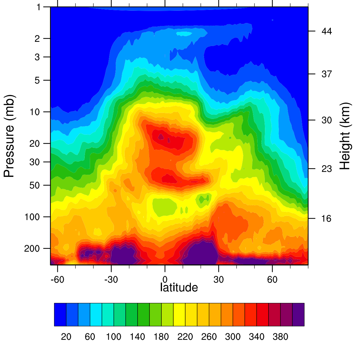
HIRDLSv6 2005d049 N2O_Combined (ppbv)
