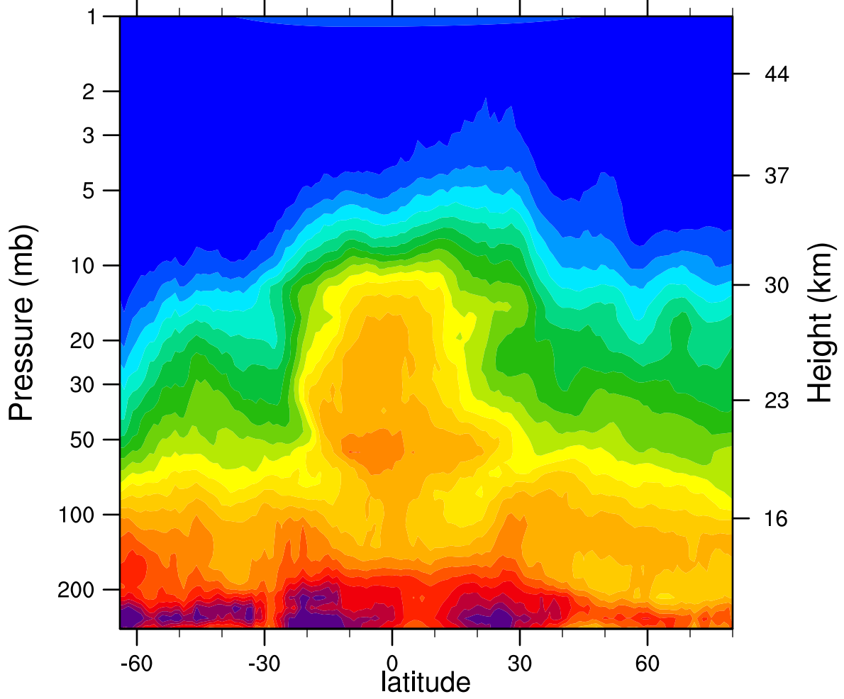
HIRDLSv6 2007d158 N2O_Combined (ppbv)
