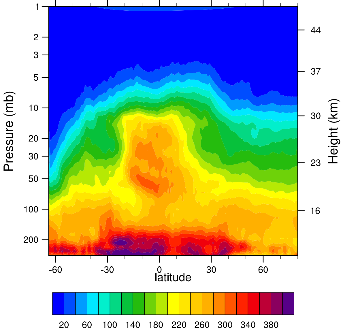
HIRDLSv6 2007d178 N2O_Combined (ppbv)
