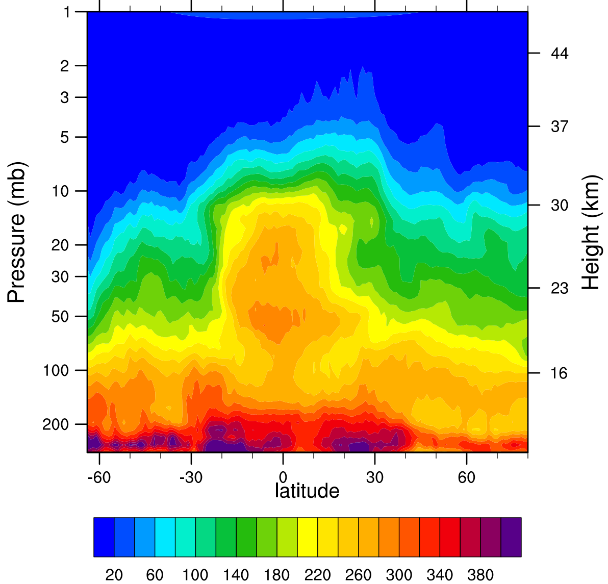
HIRDLSv6 2007d161 N2O_Combined (ppbv)
