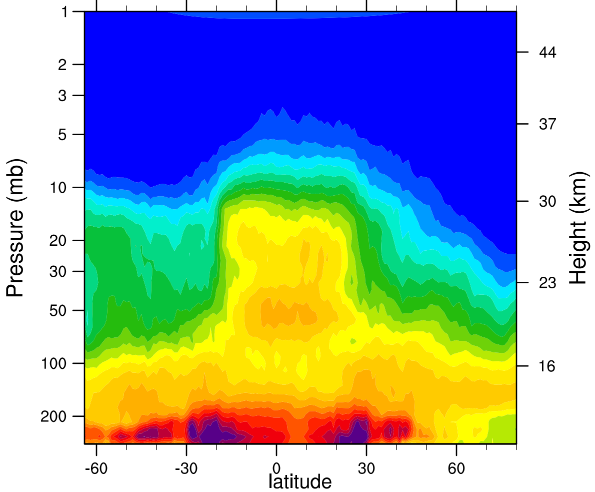
HIRDLSv6 2007d310 N2O_Combined (ppbv)
