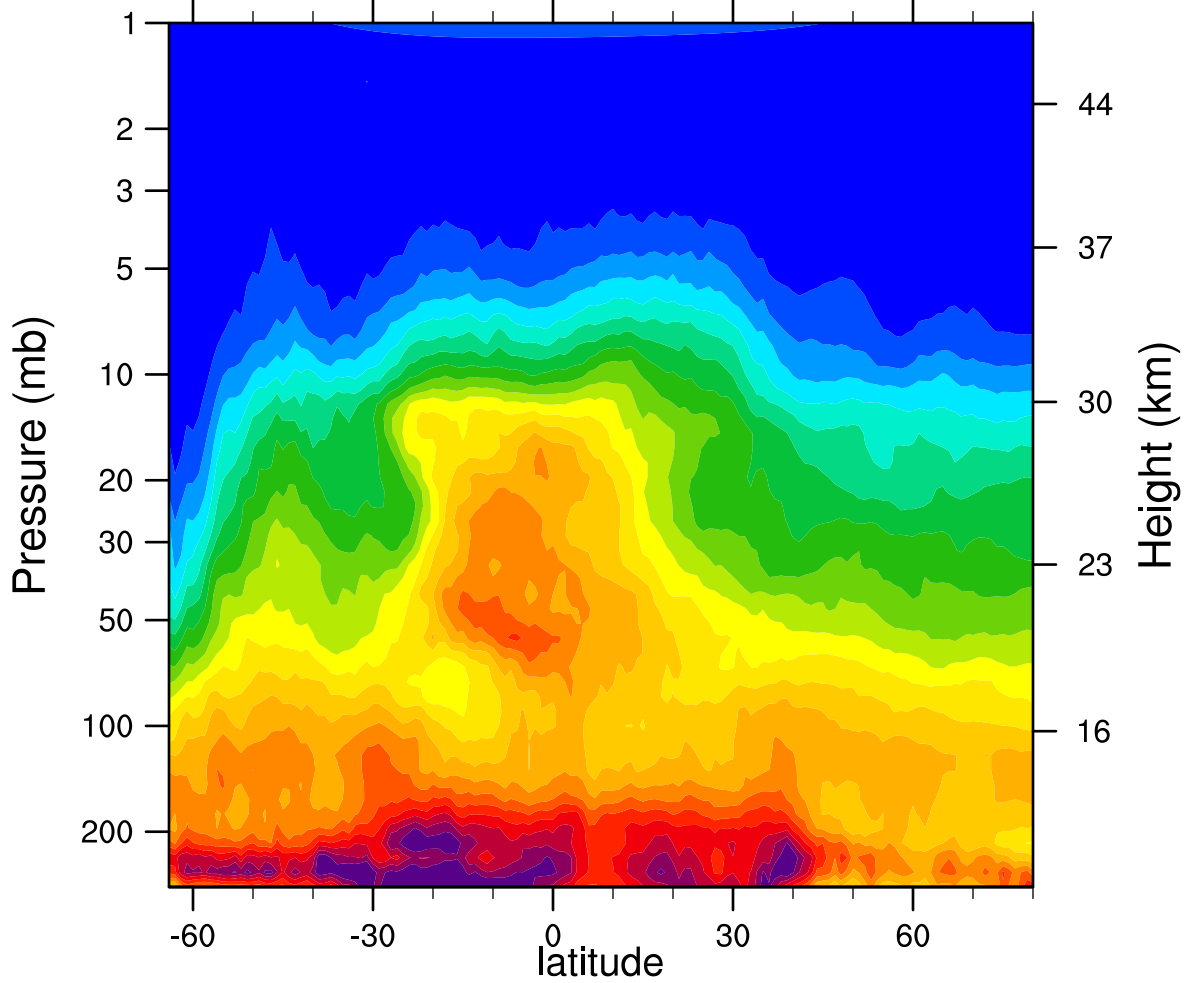
HIRDLSv6 2007d174 N2O_Combined (ppbv)
