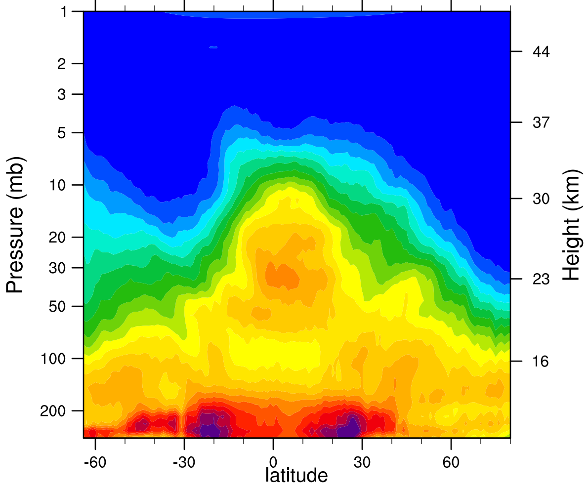
HIRDLSv6 2006d337 N2O_Combined (ppbv)
