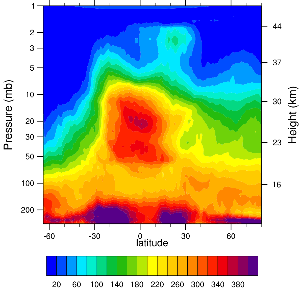
HIRDLSv6 2005d137 N2O_Combined (ppbv)
