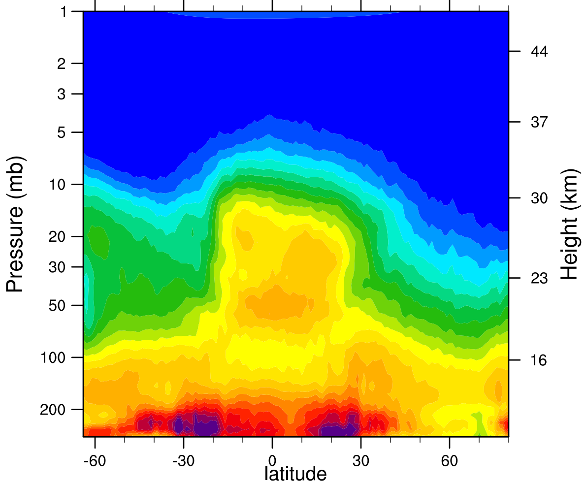
HIRDLSv6 2007d326 N2O_Combined (ppbv)
