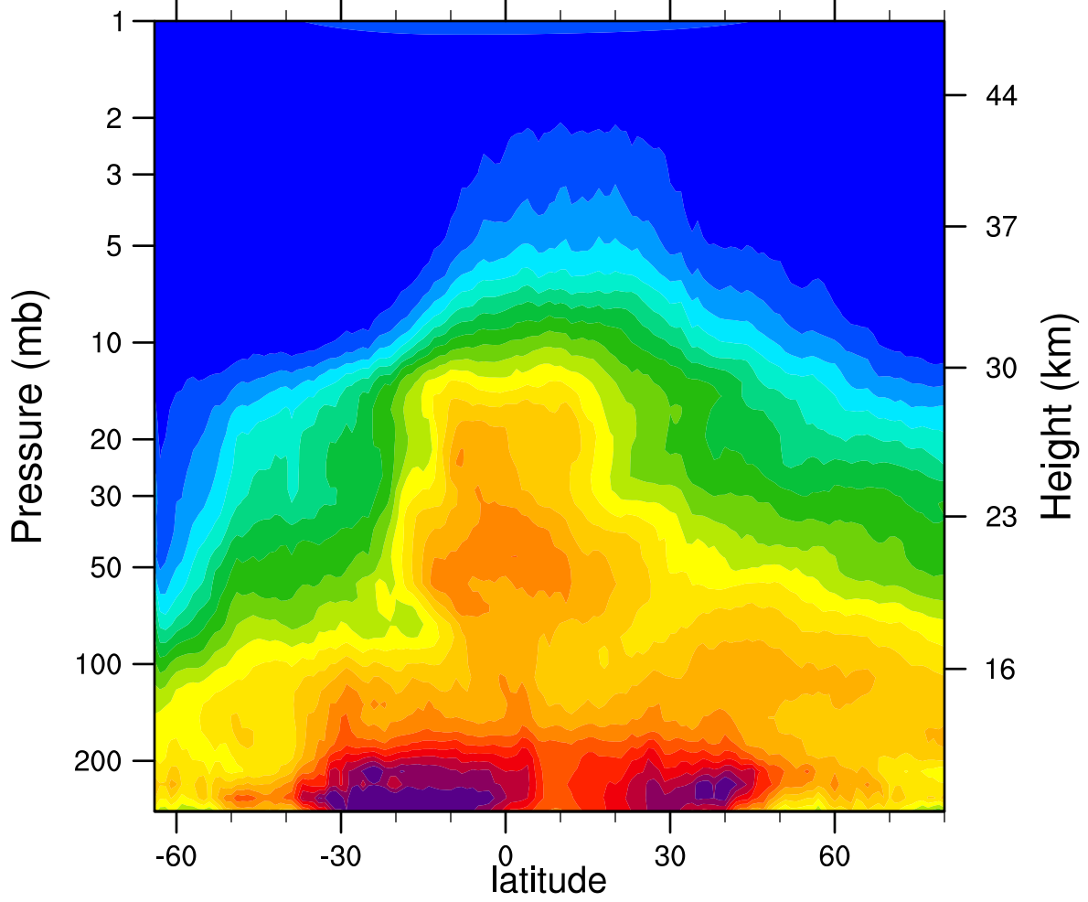
HIRDLSv6 2007d221 N2O_Combined (ppbv)
