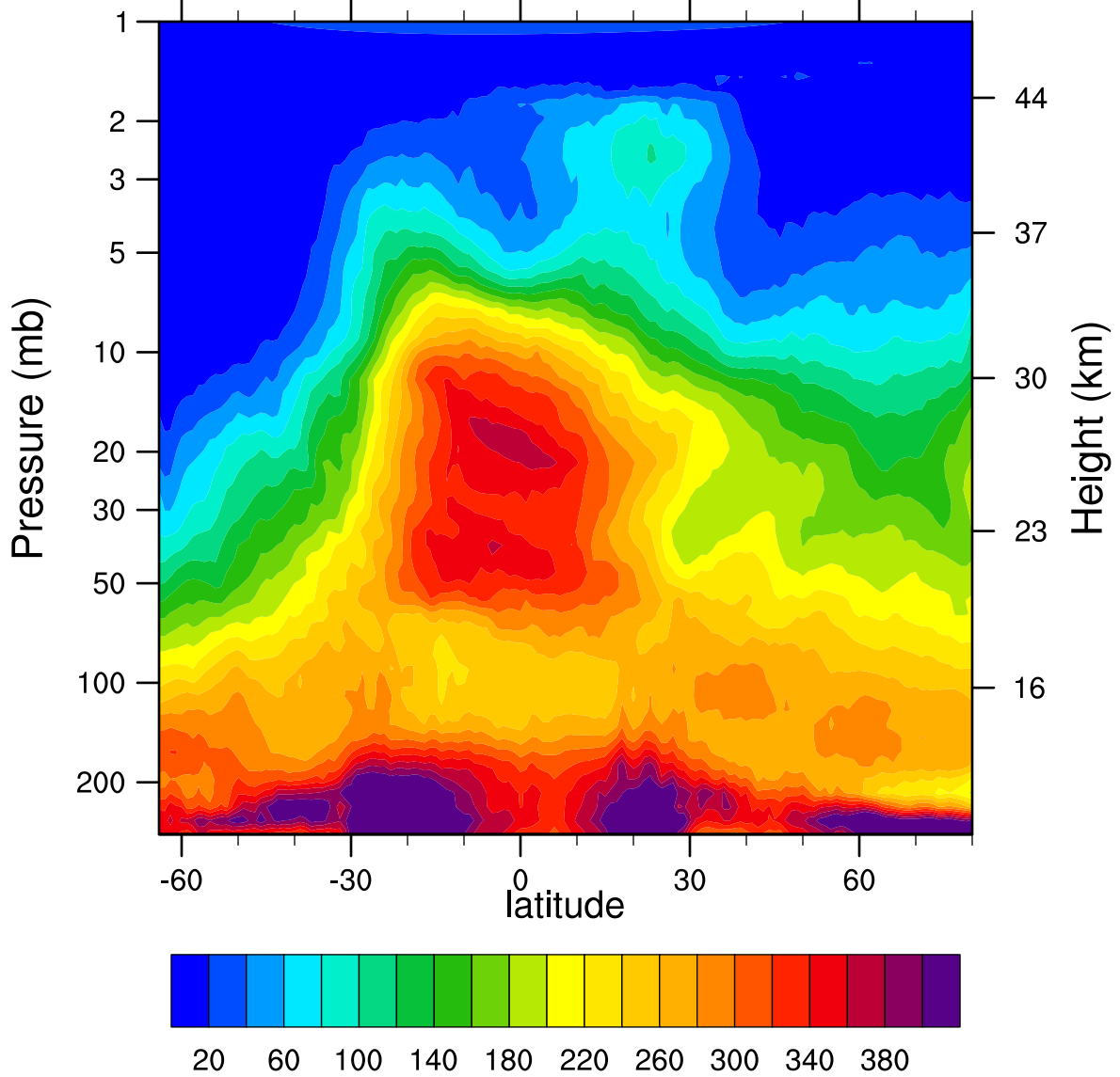
HIRDLSv6 2005d126 N2O_Combined (ppbv)
