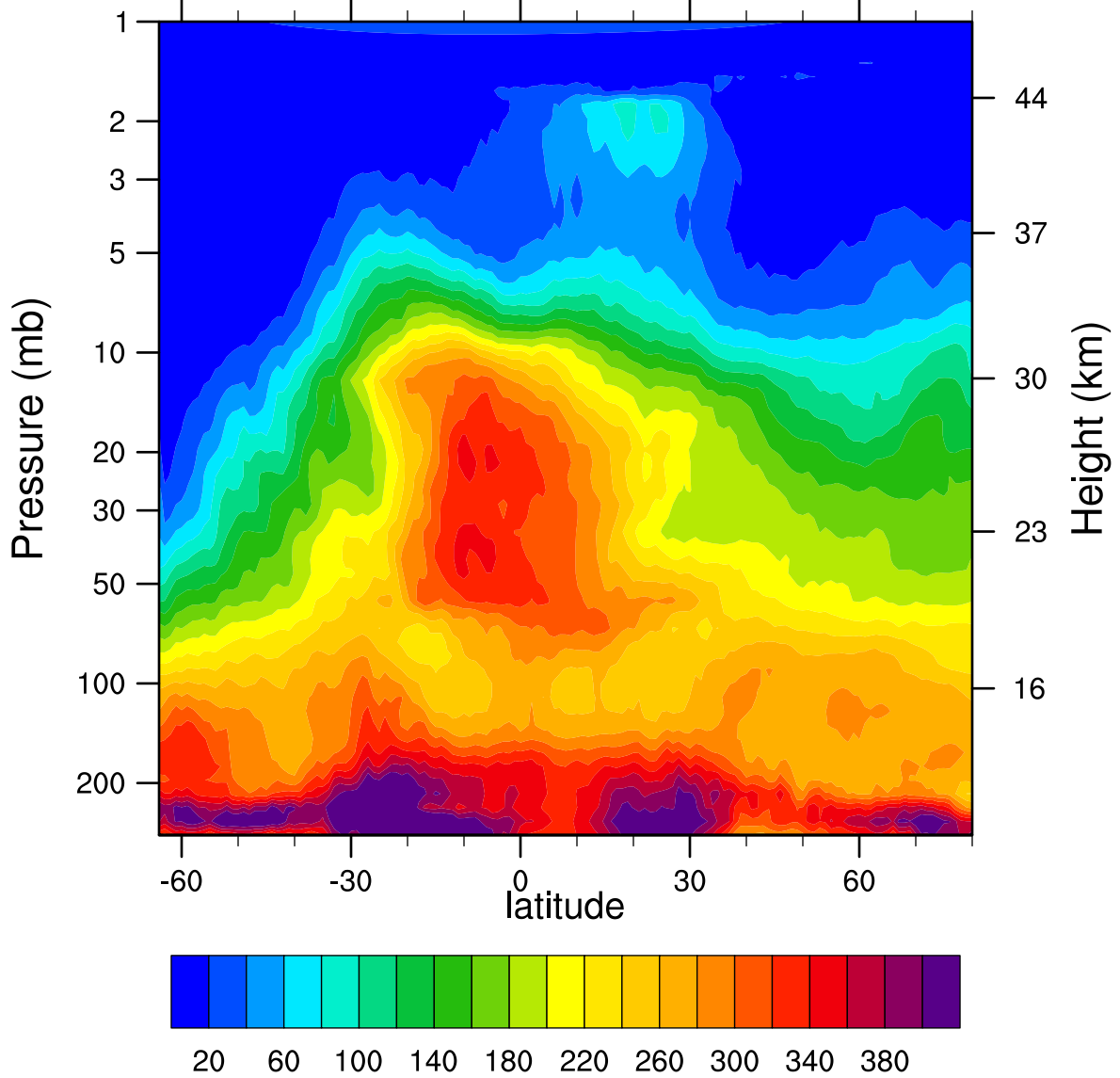
HIRDLSv6 2005d166 N2O_Combined (ppbv)
