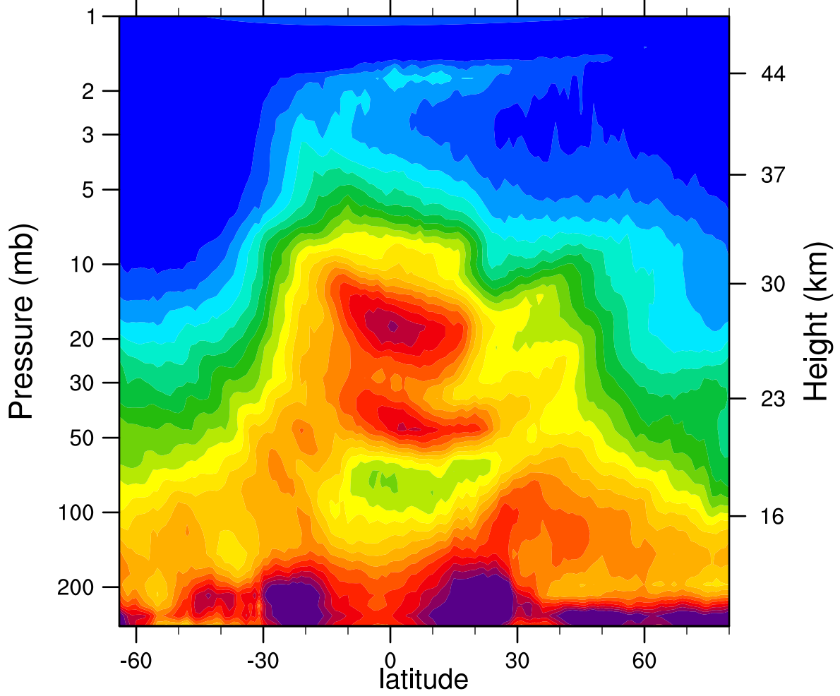
HIRDLSv6 2005d059 N2O_Combined (ppbv)
