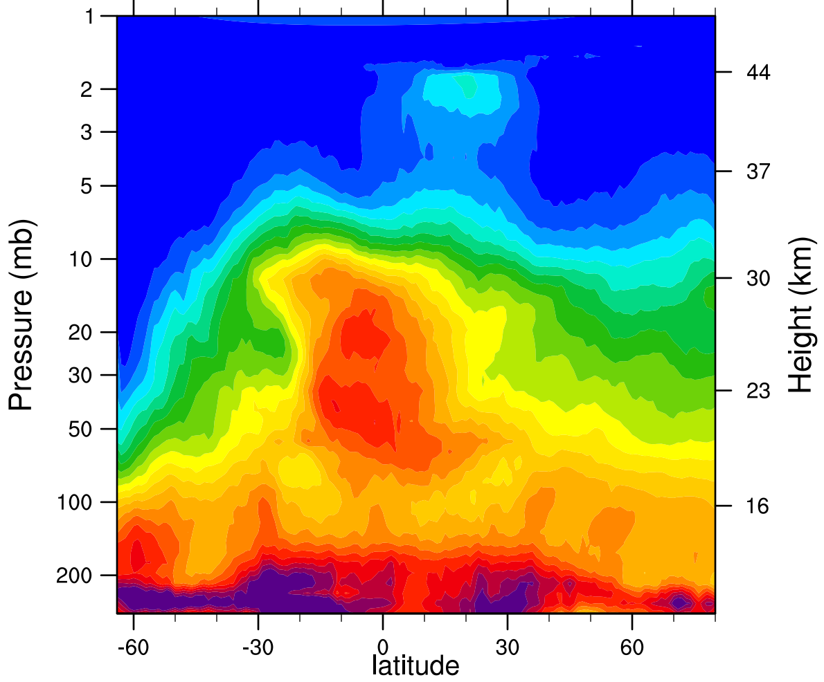
HIRDLSv6 2005d182 N2O_Combined (ppbv)
