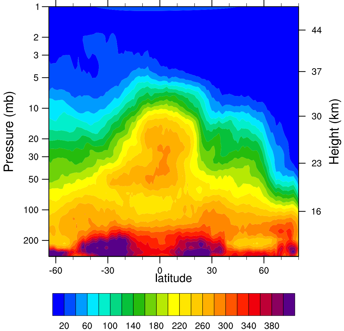
HIRDLSv6 2007d014 N2O_Combined (ppbv)
