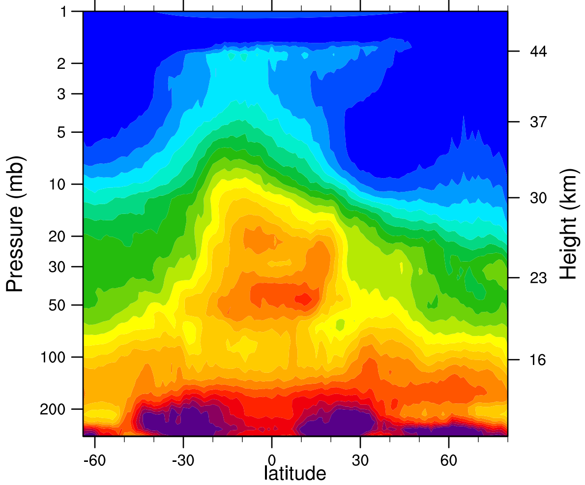
HIRDLSv6 2006d033 N2O_Combined (ppbv)
