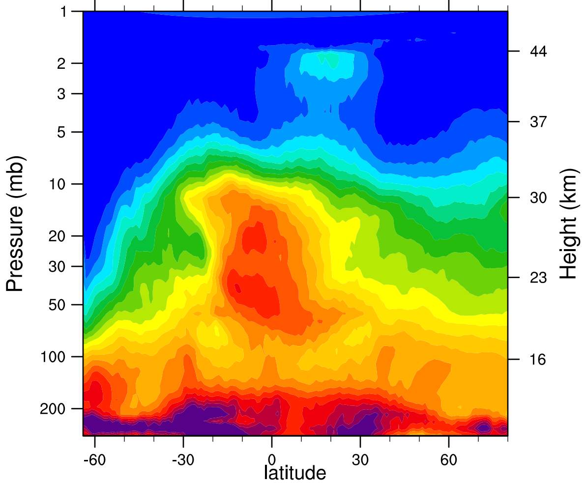
HIRDLSv6 2005d183 N2O_Combined (ppbv)
