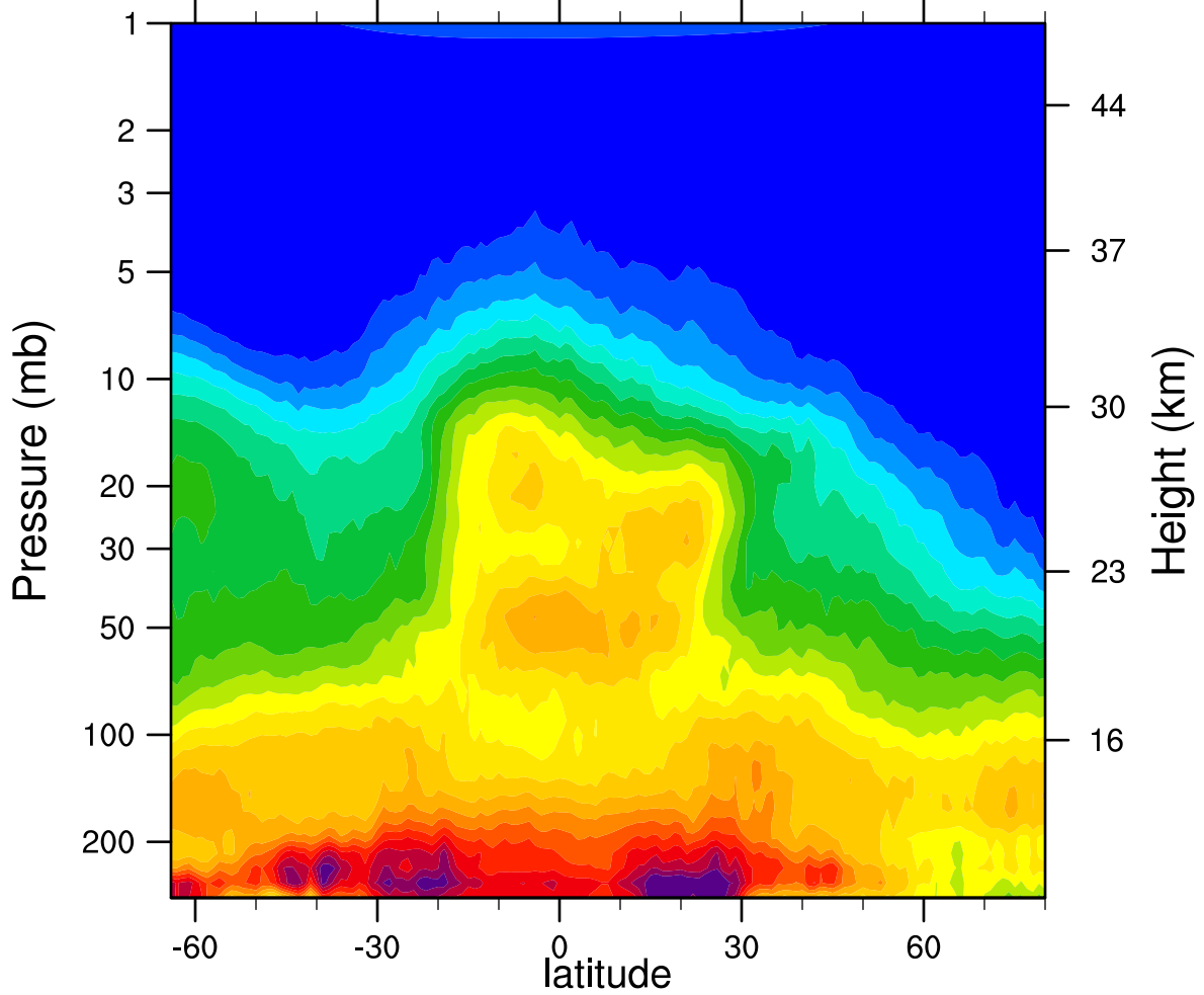
HIRDLSv6 2007d346 N2O_Combined (ppbv)
