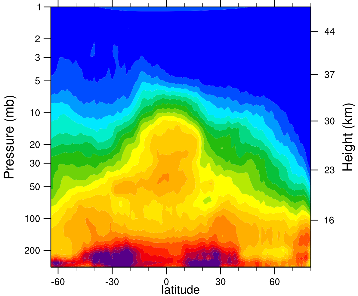
HIRDLSv6 2006d363 N2O_Combined (ppbv)
