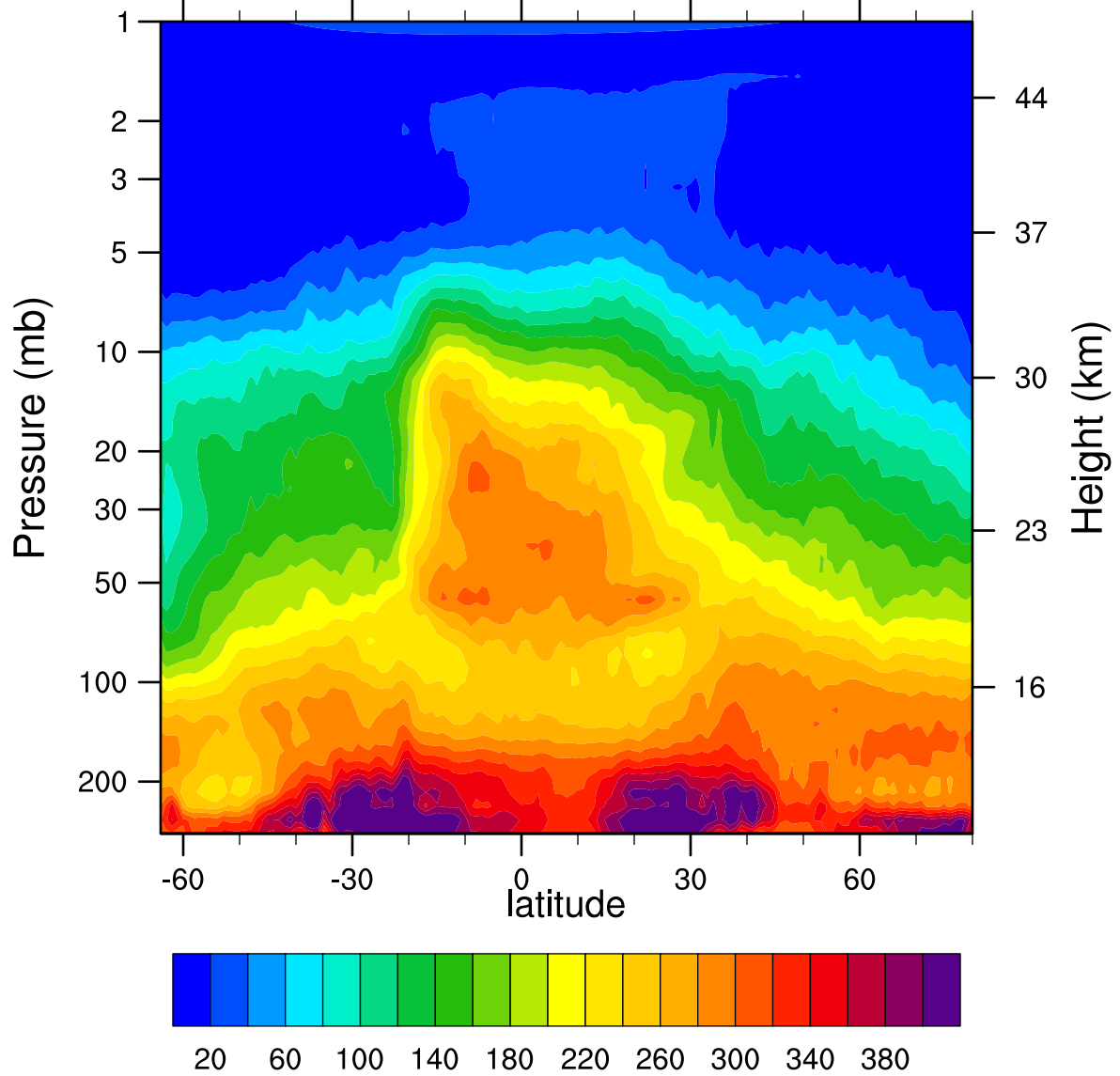
HIRDLSv6 2005d296 N2O_Combined (ppbv)
