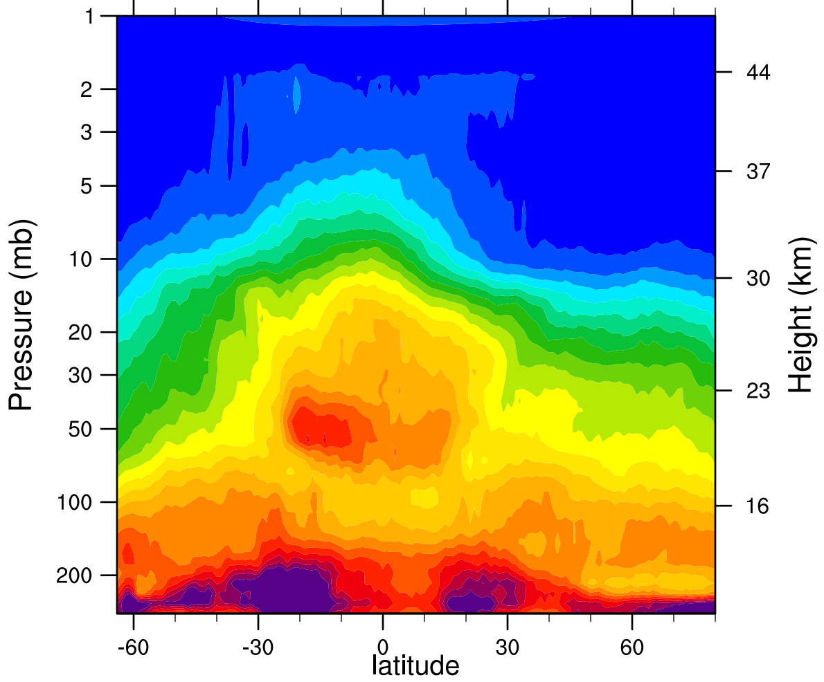
HIRDLSv6 2006d126 N2O_Combined (ppbv)
