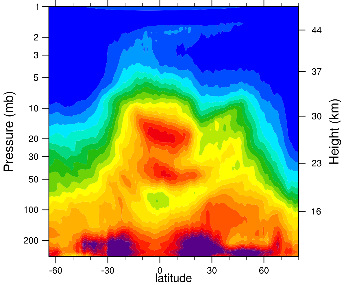
HIRDLSv6 2005d042 N2O_Combined (ppbv)
