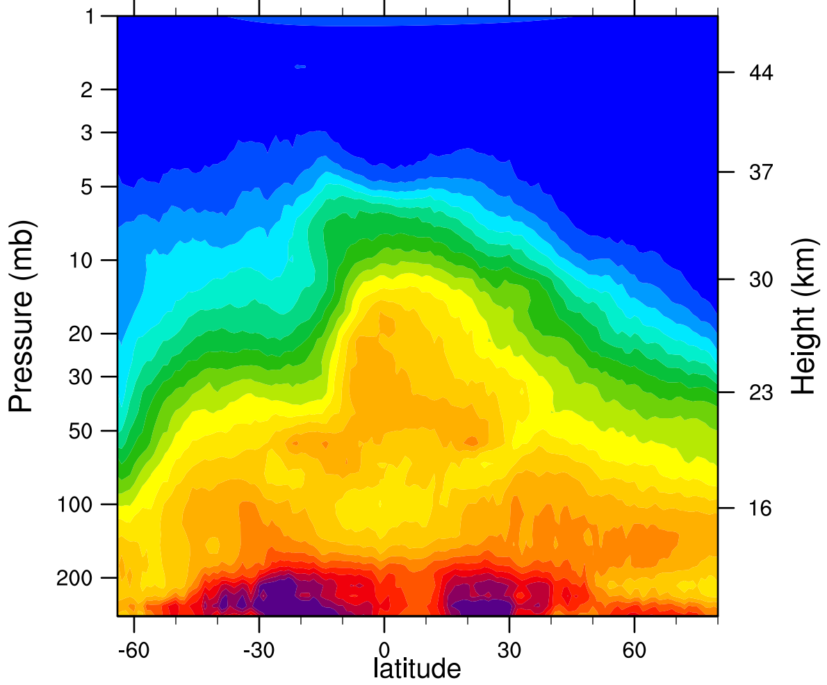
HIRDLSv6 2006d291 N2O_Combined (ppbv)
