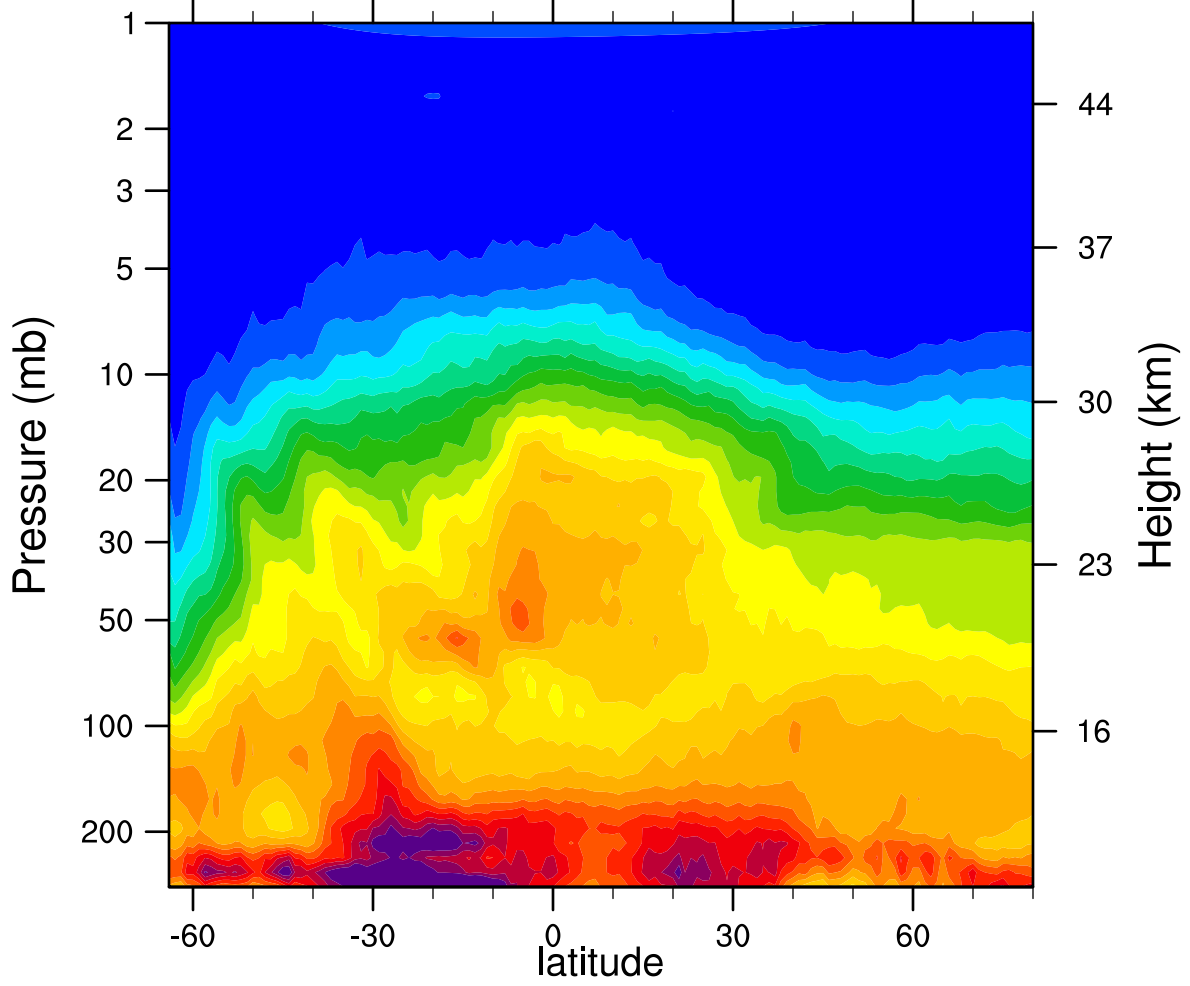
HIRDLSv6 2006d184 N2O_Combined (ppbv)
