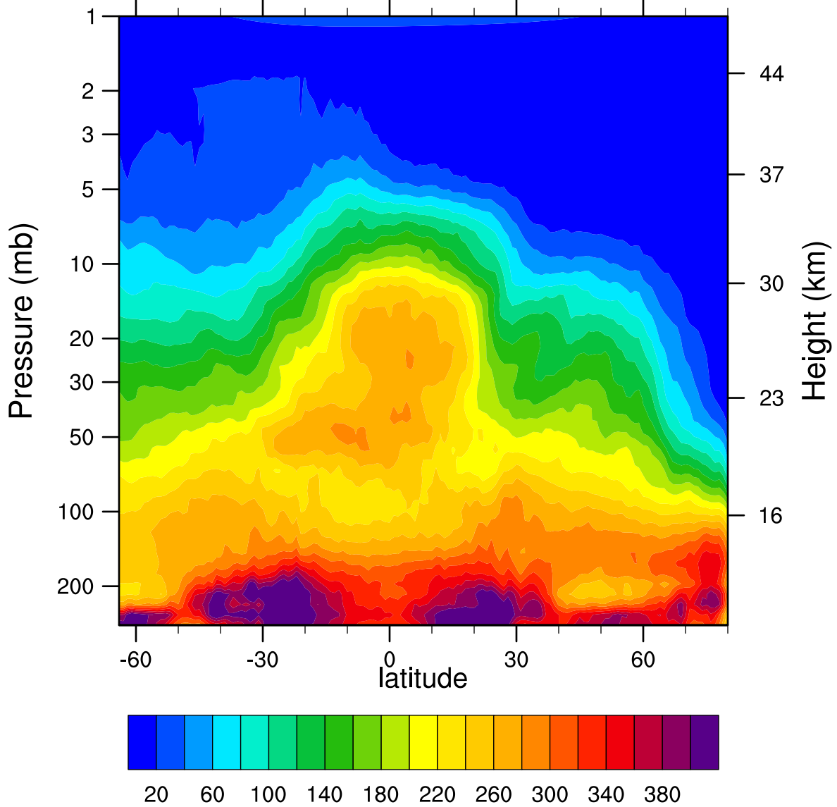
HIRDLSv6 2007d020 N2O_Combined (ppbv)
