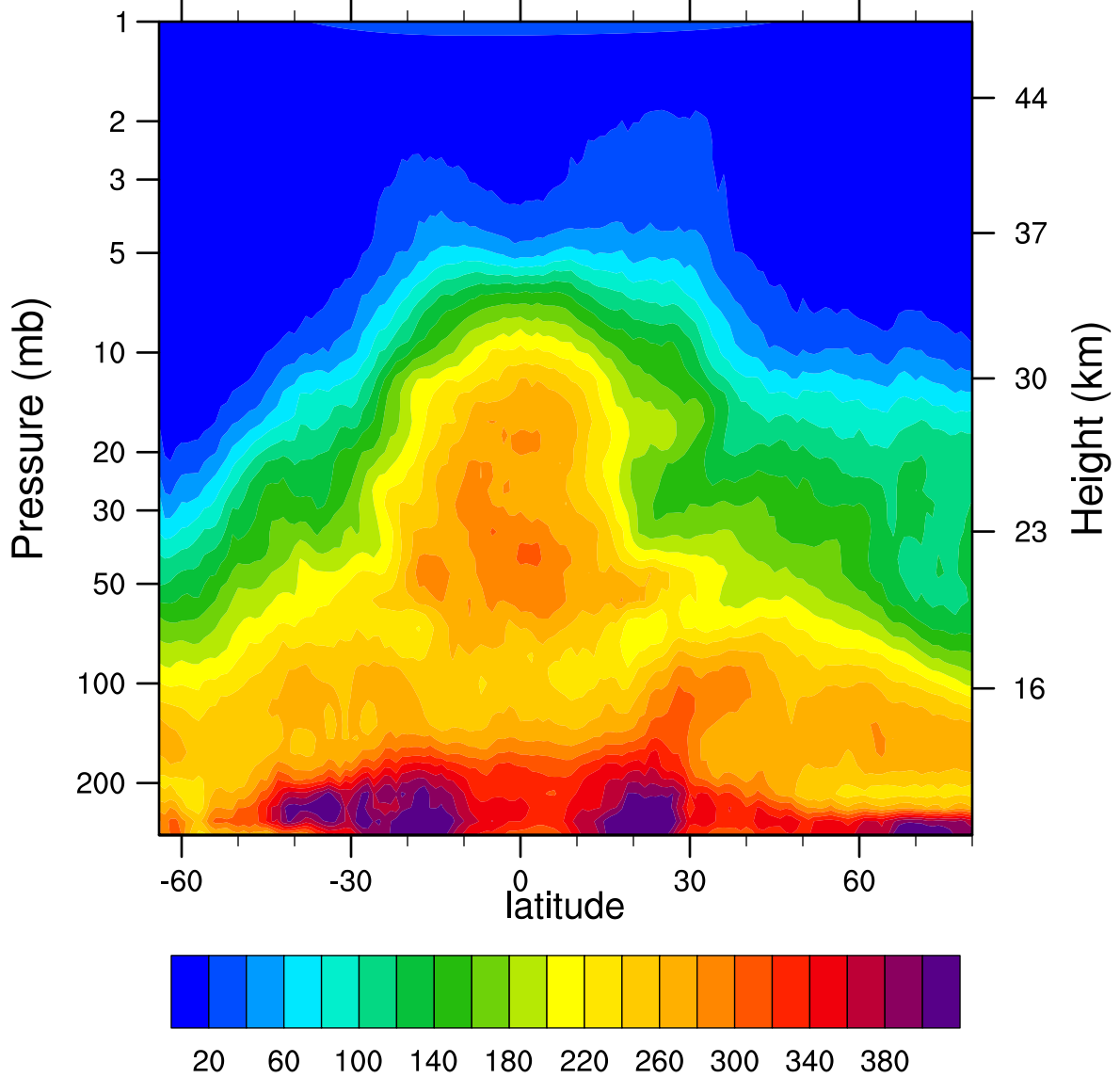
HIRDLSv6 2007d116 N2O_Combined (ppbv)
