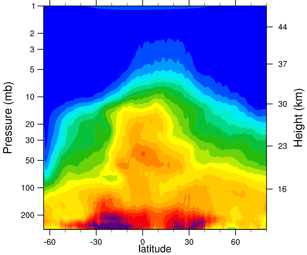
HIRDLSv6 2007d236 N2O_Combined (ppbv)
