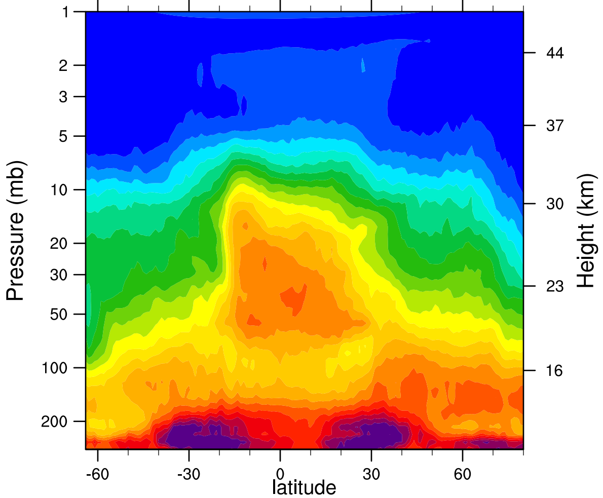
HIRDLSv6 2005d302 N2O_Combined (ppbv)
