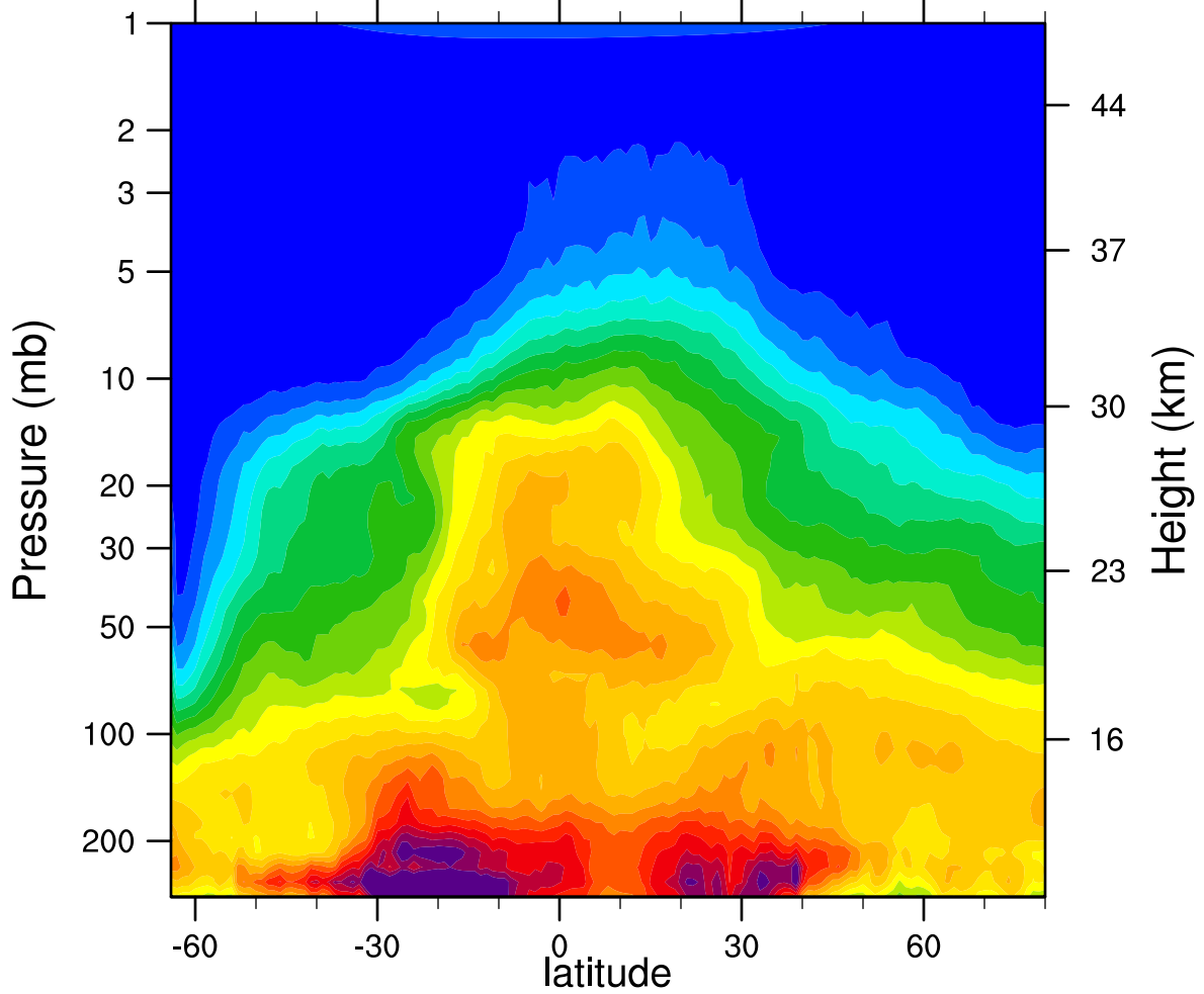
HIRDLSv6 2007d235 N2O_Combined (ppbv)
