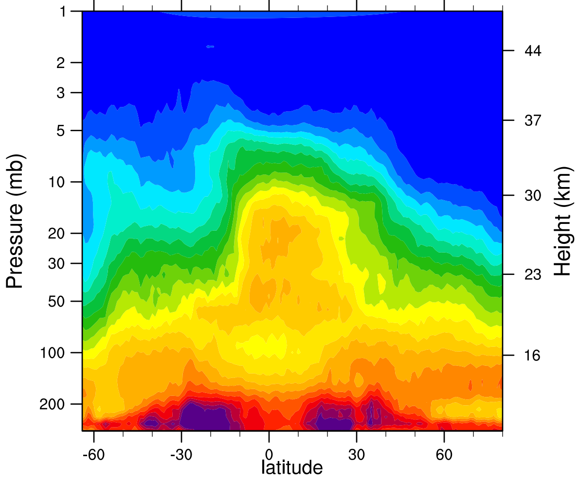
HIRDLSv6 2006d307 N2O_Combined (ppbv)
