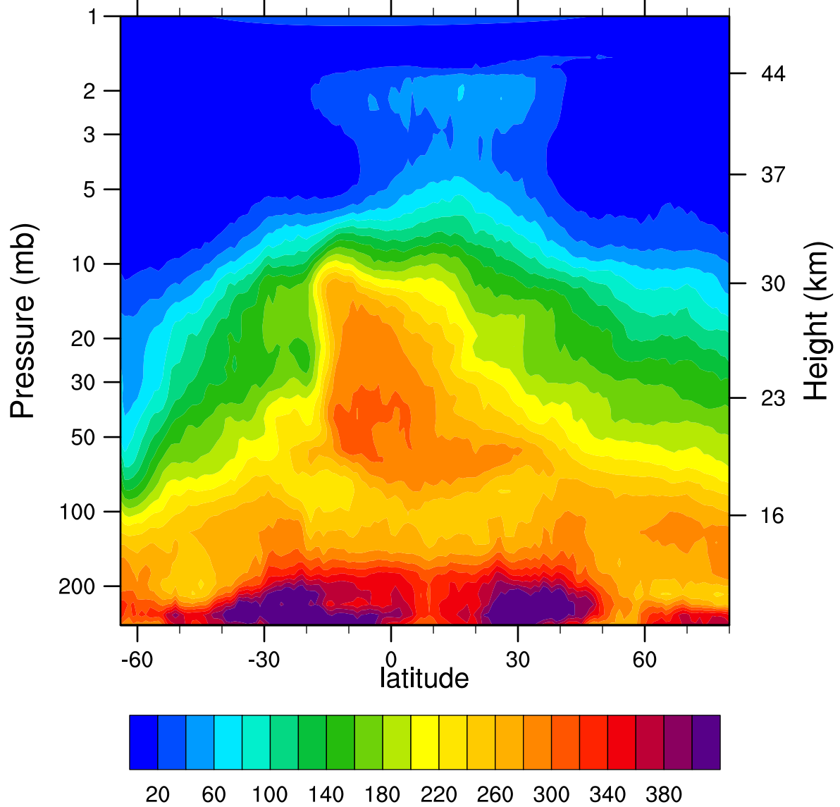
HIRDLSv6 2005d250 N2O_Combined (ppbv)
