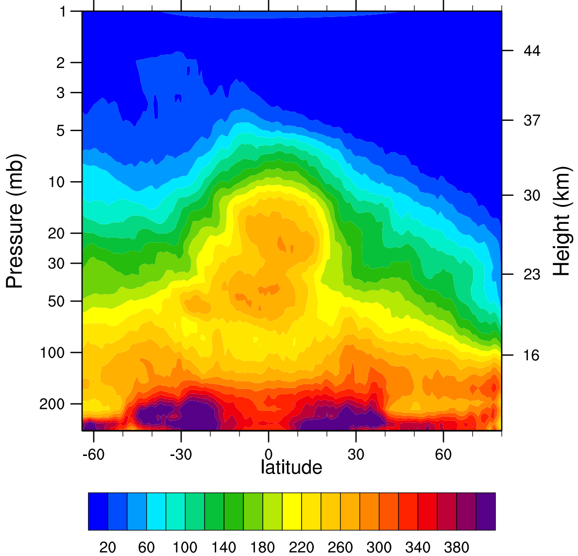
HIRDLSv6 2007d026 N2O_Combined (ppbv)
