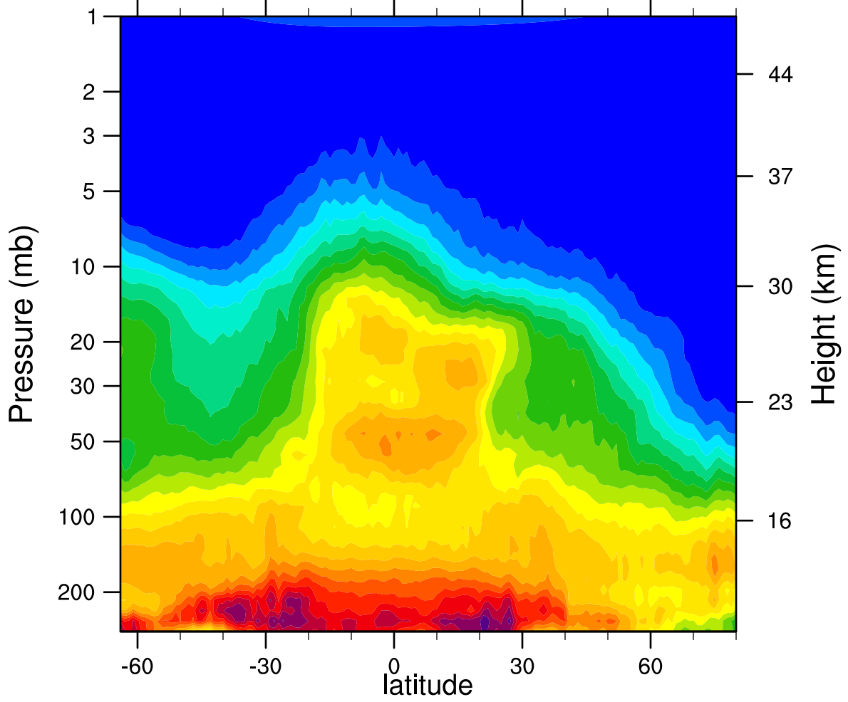
HIRDLSv6 2007d364 N2O_Combined (ppbv)
