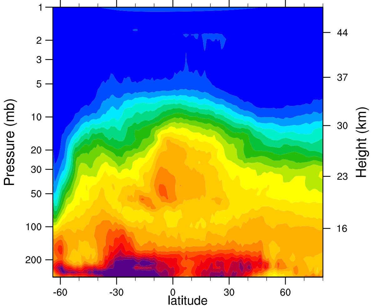
HIRDLSv6 2006d200 N2O_Combined (ppbv)
