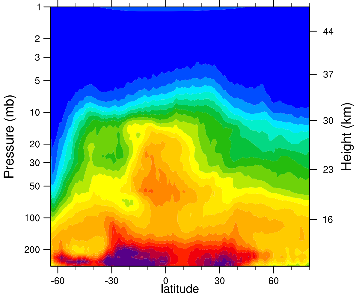
HIRDLSv6 2007d199 N2O_Combined (ppbv)
