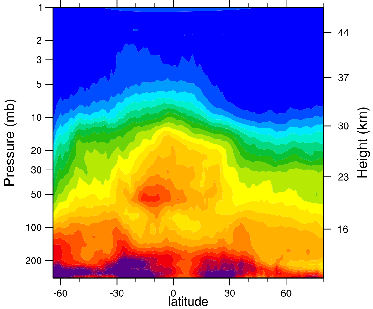
HIRDLSv6 2006d156 N2O_Combined (ppbv)
