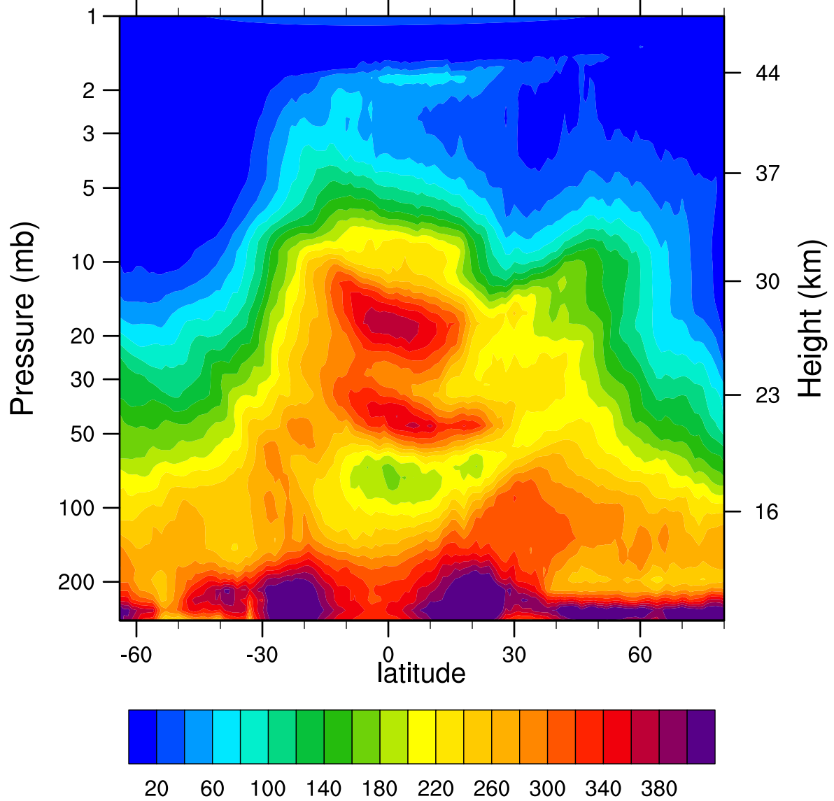
HIRDLSv6 2005d064 N2O_Combined (ppbv)
