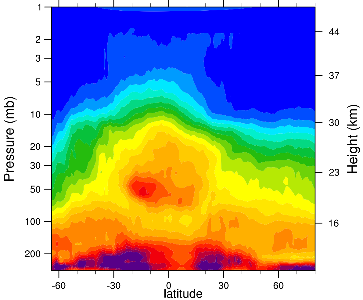
HIRDLSv6 2006d132 N2O_Combined (ppbv)
