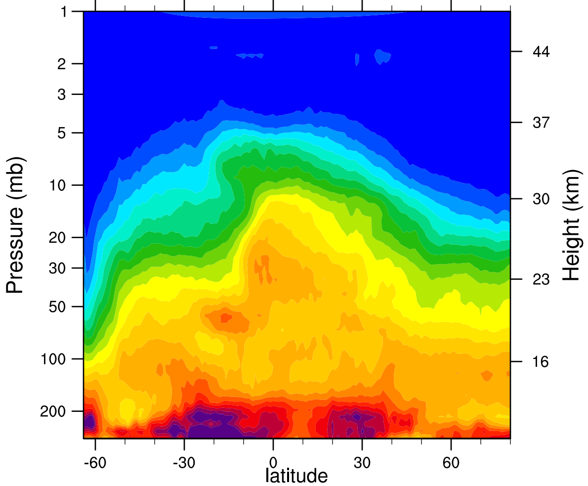
HIRDLSv6 2006d261 N2O_Combined (ppbv)
