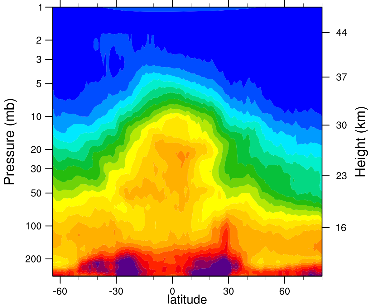
HIRDLSv6 2007d059 N2O_Combined (ppbv)
