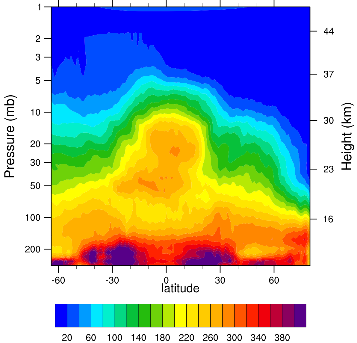
HIRDLSv6 2007d022 N2O_Combined (ppbv)
