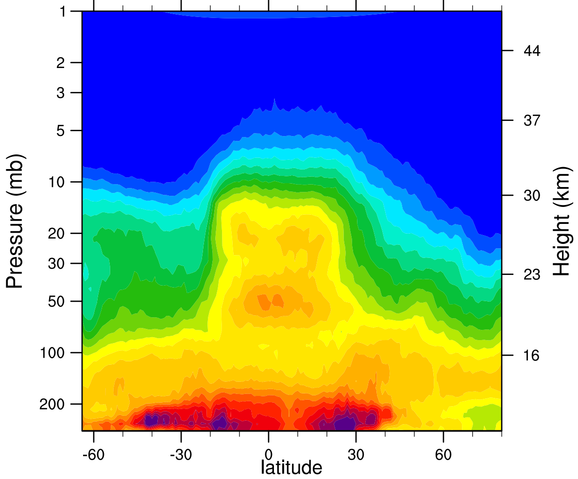
HIRDLSv6 2007d304 N2O_Combined (ppbv)
