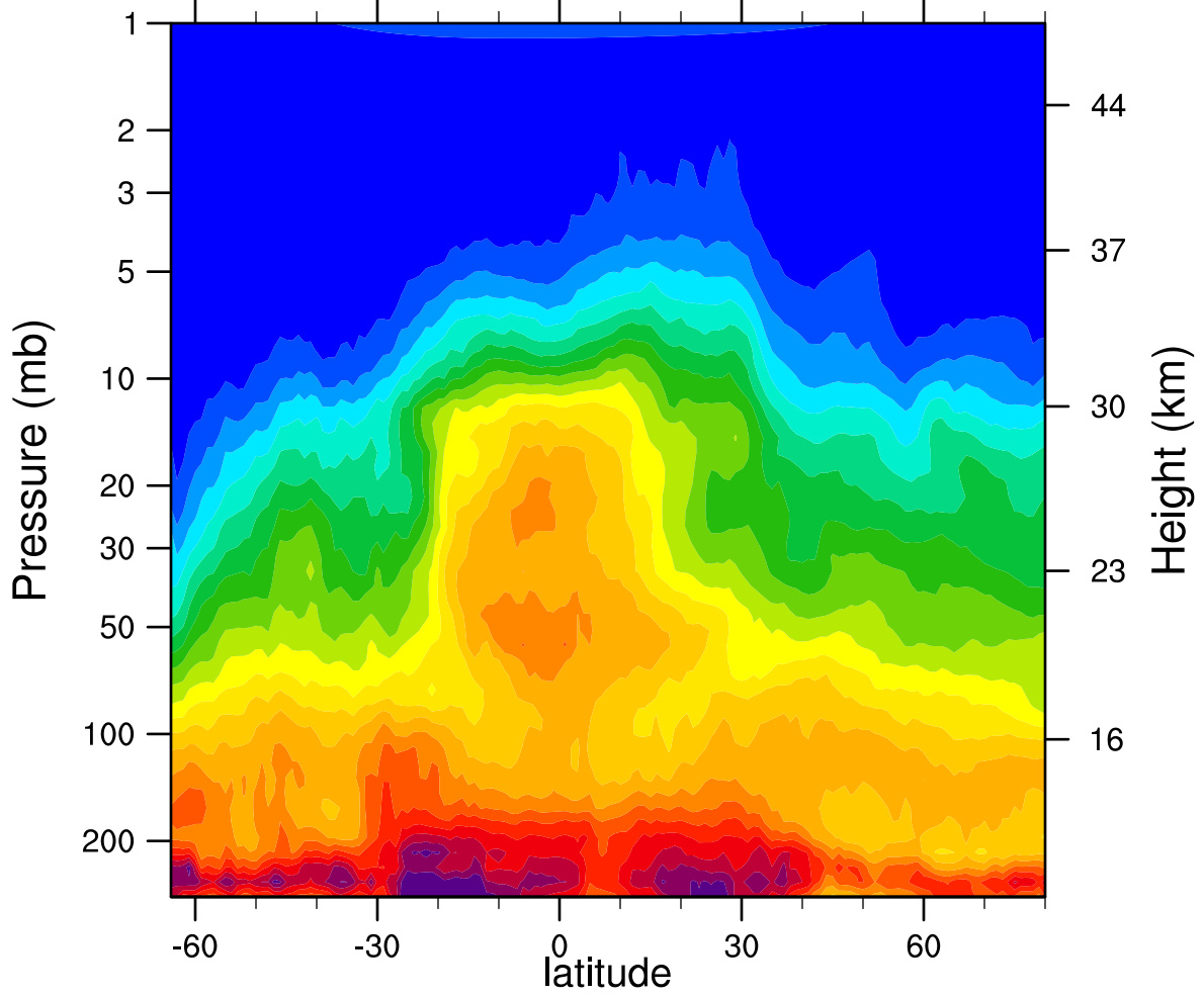
HIRDLSv6 2007d162 N2O_Combined (ppbv)
