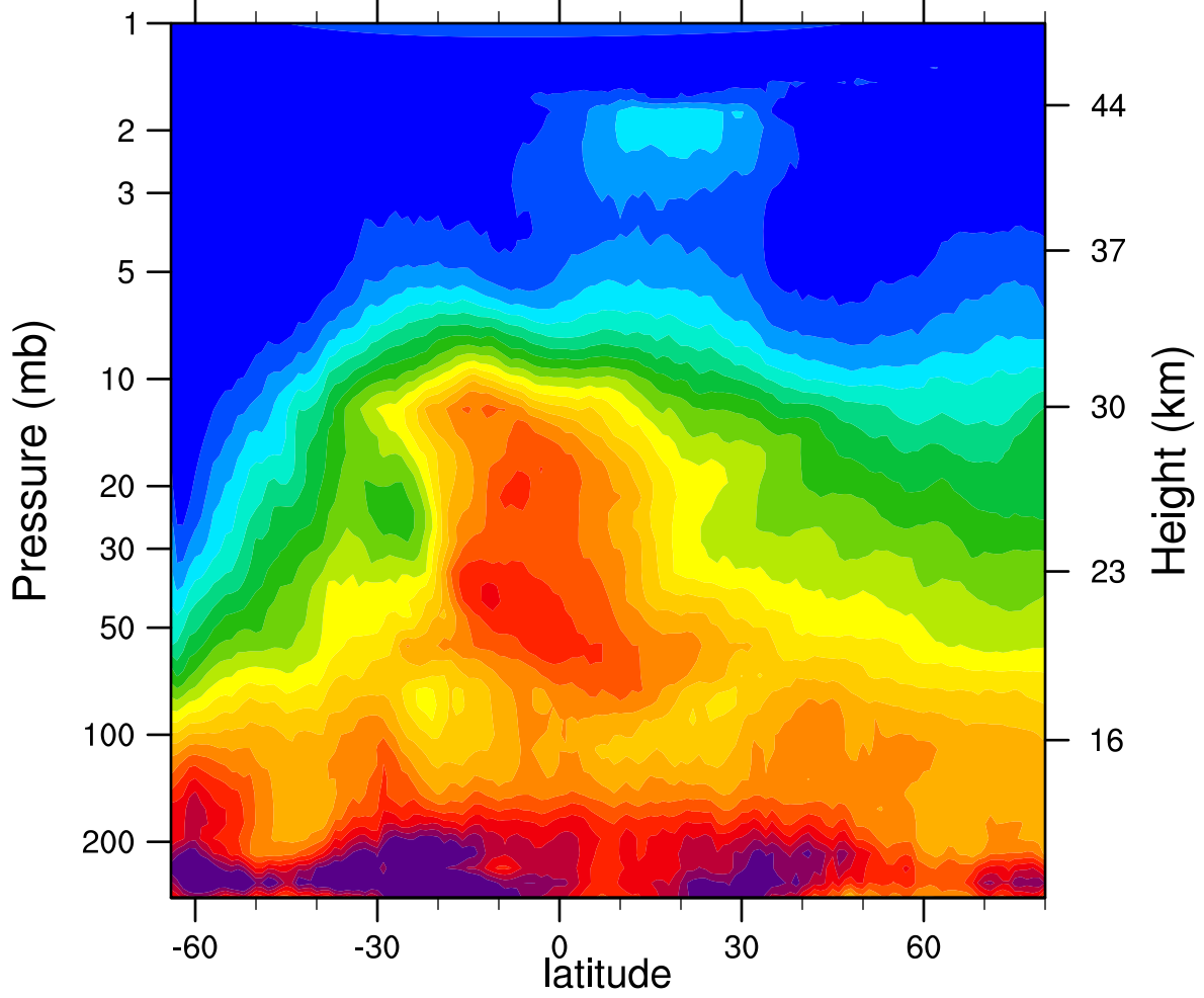
HIRDLSv6 2005d189 N2O_Combined (ppbv)
