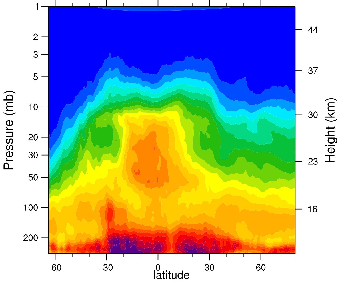
HIRDLSv6 2007d165 N2O_Combined (ppbv)
