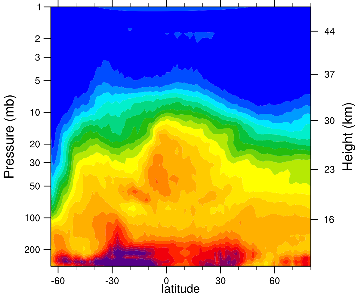
HIRDLSv6 2006d214 N2O_Combined (ppbv)
