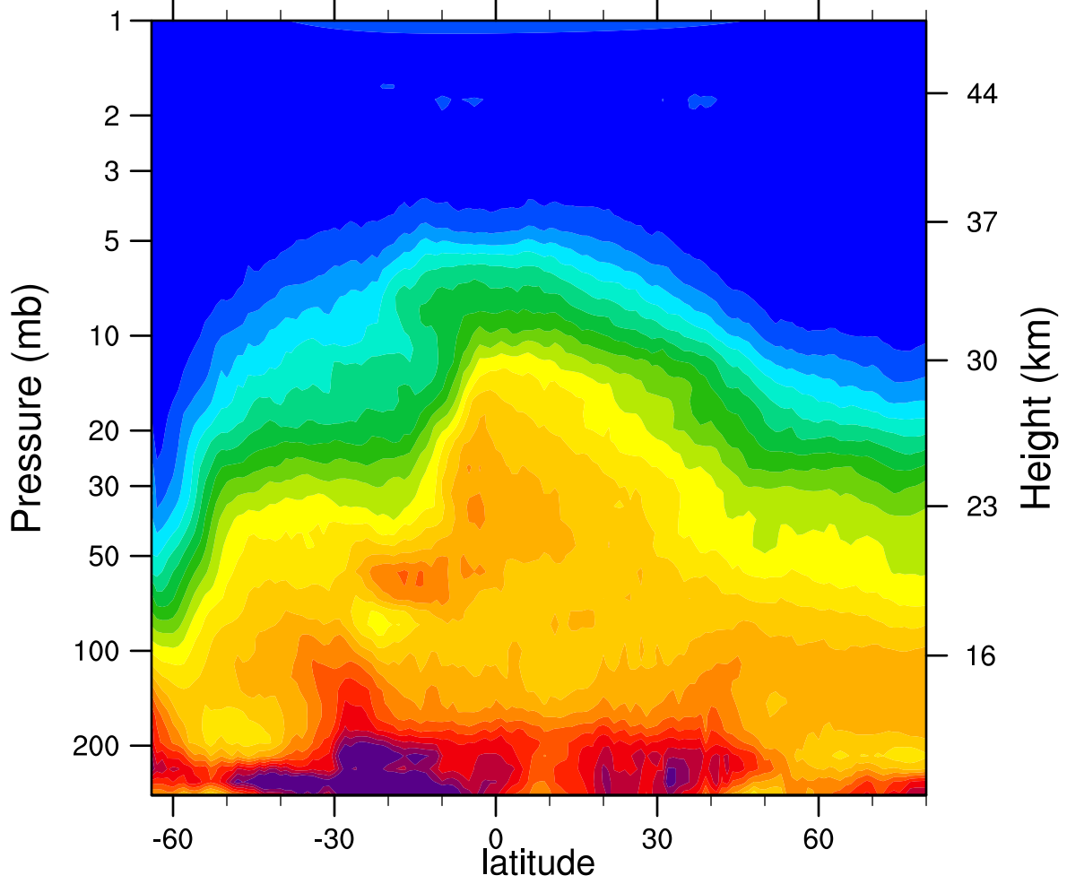
HIRDLSv6 2006d253 N2O_Combined (ppbv)
