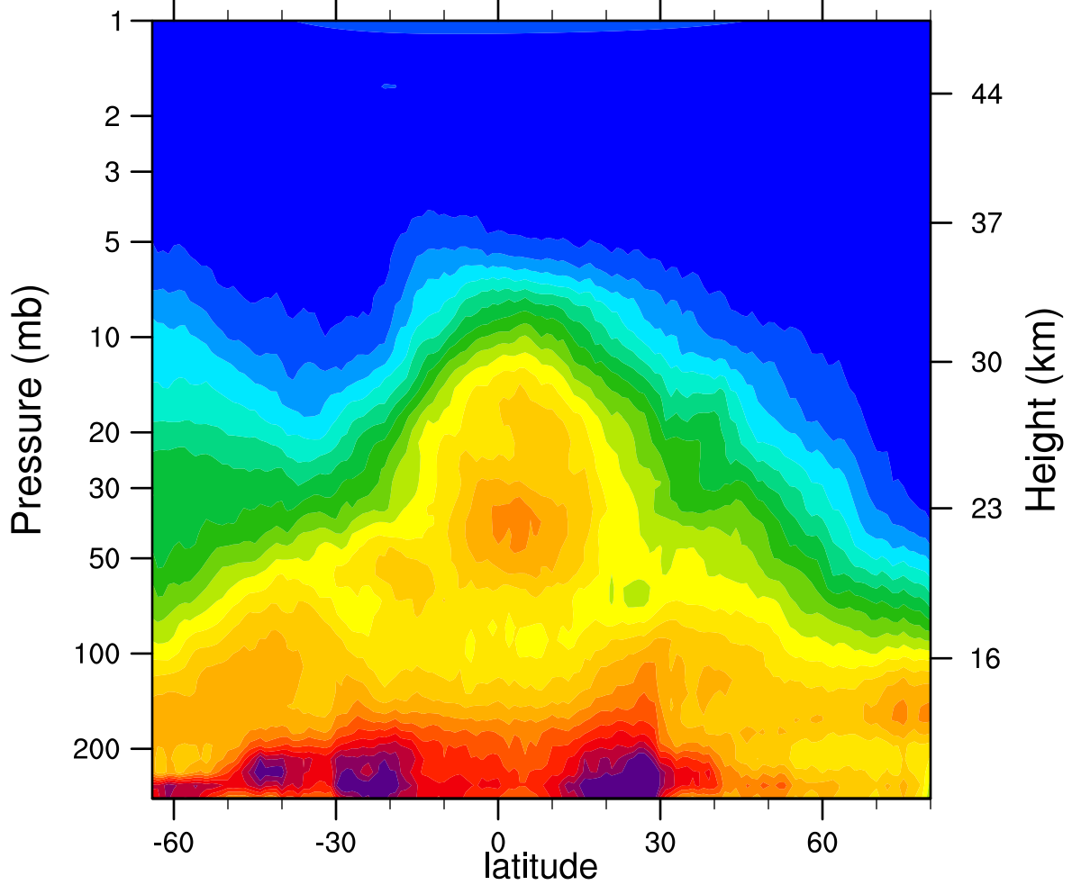
HIRDLSv6 2006d352 N2O_Combined (ppbv)
