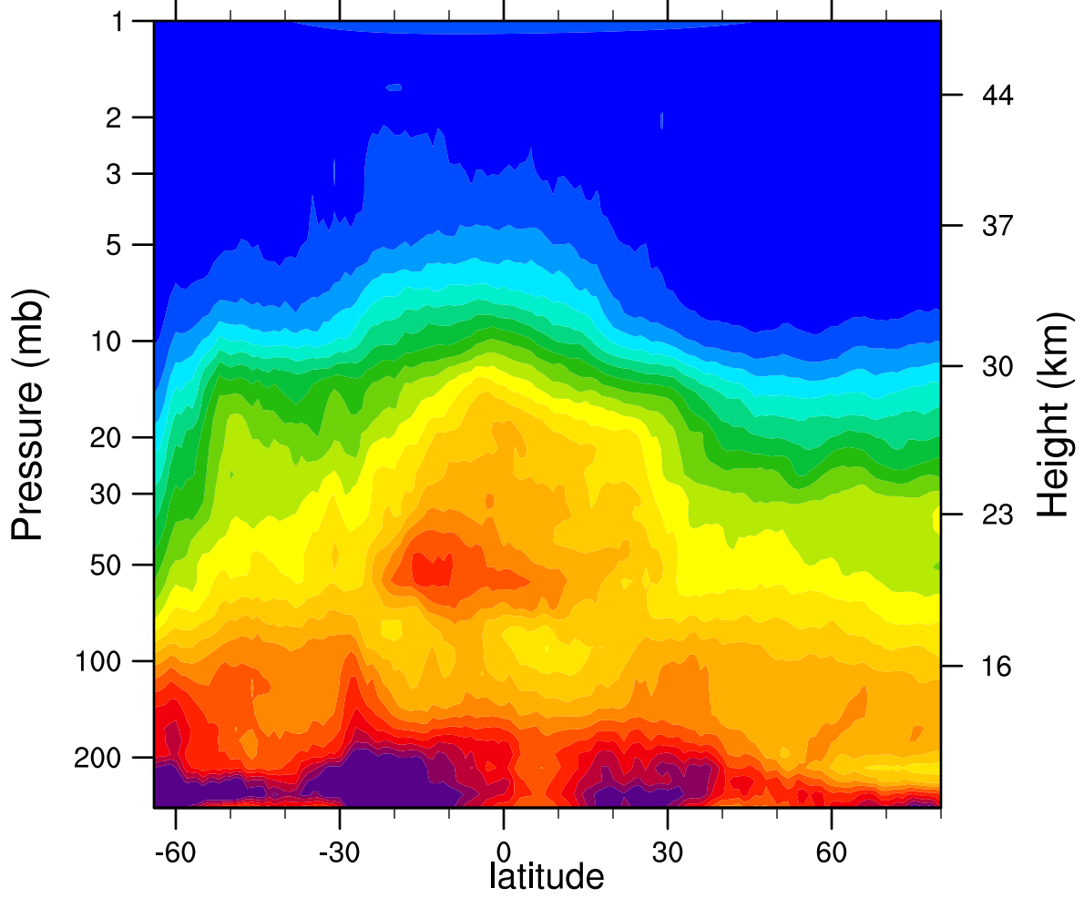
HIRDLSv6 2006d152 N2O_Combined (ppbv)
