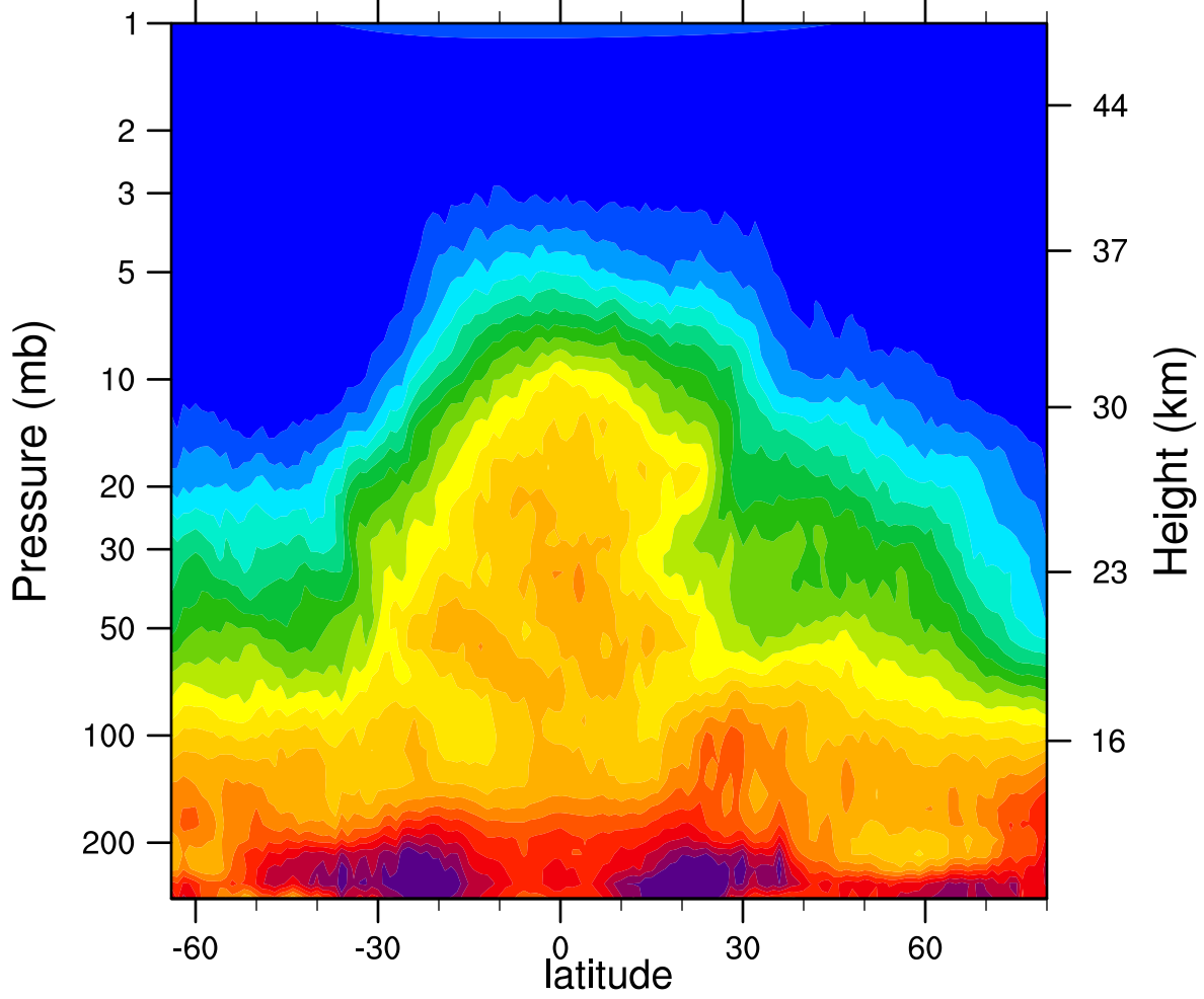
HIRDLSv6 2007d079 N2O_Combined (ppbv)
