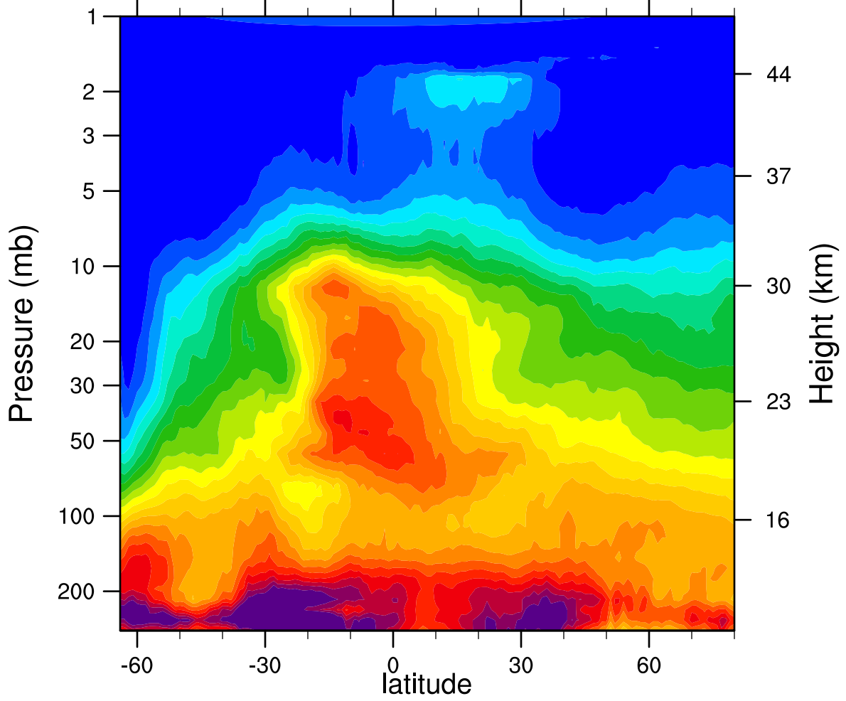
HIRDLSv6 2005d196 N2O_Combined (ppbv)
