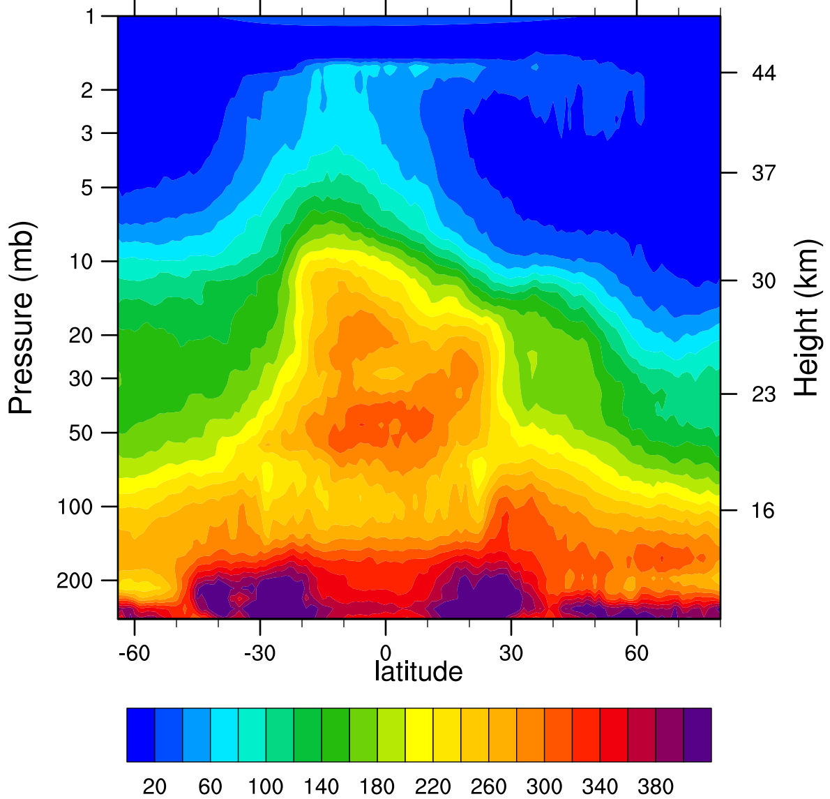
HIRDLSv6 2006d014 N2O_Combined (ppbv)
