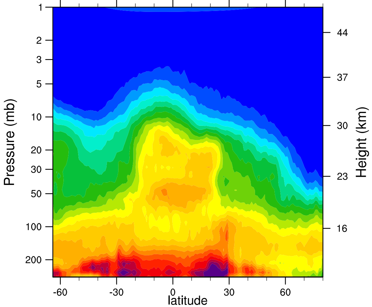
HIRDLSv6 2007d359 N2O_Combined (ppbv)
