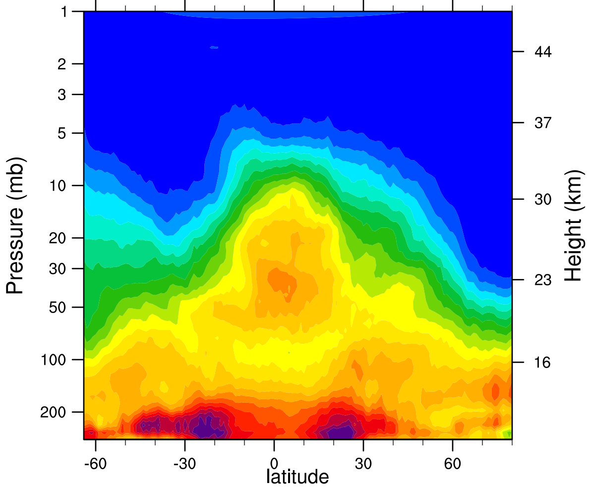
HIRDLSv6 2006d343 N2O_Combined (ppbv)
