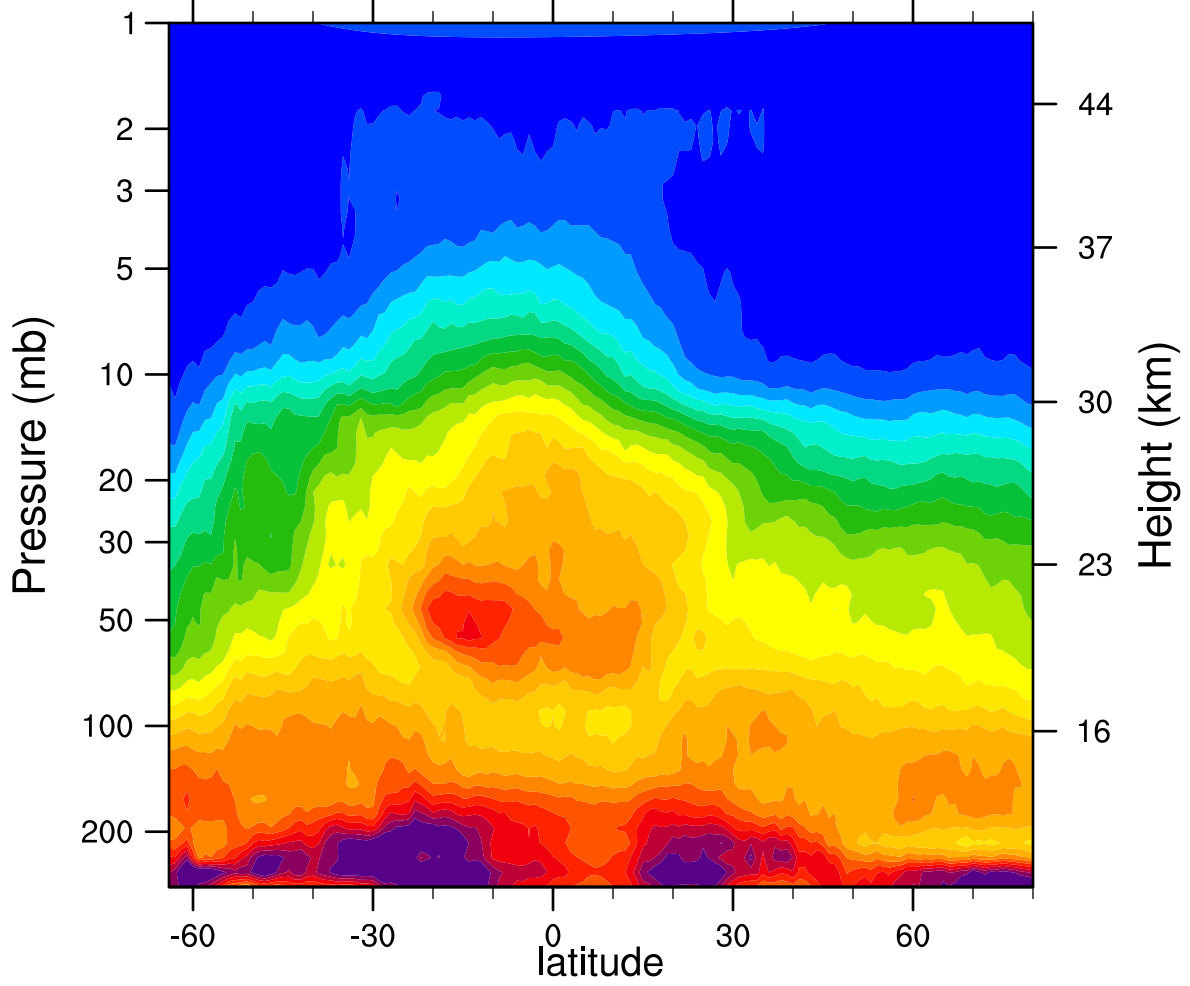
HIRDLSv6 2006d131 N2O_Combined (ppbv)
