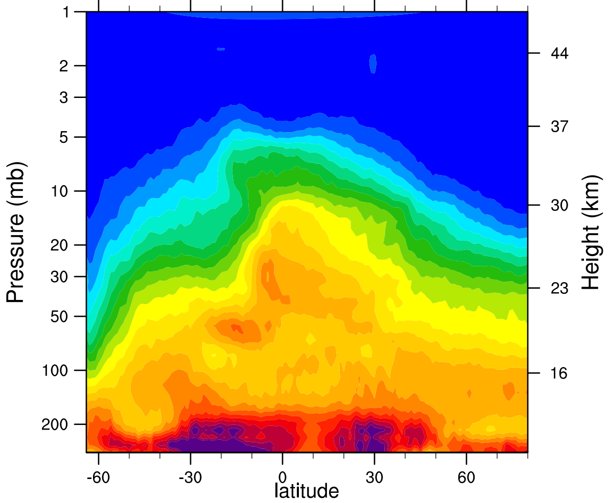
HIRDLSv6 2006d267 N2O_Combined (ppbv)
