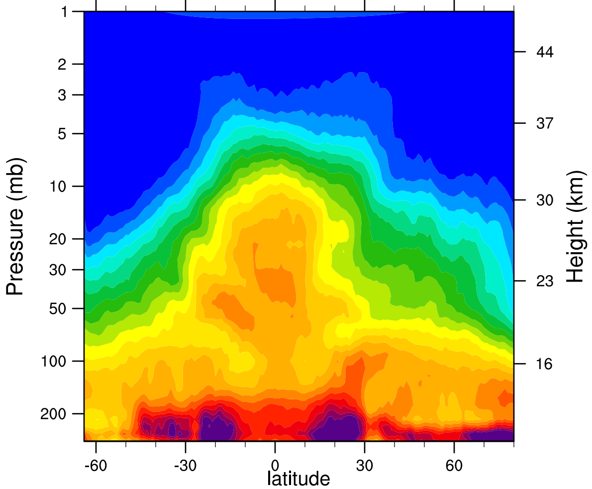
HIRDLSv6 2007d095 N2O_Combined (ppbv)
