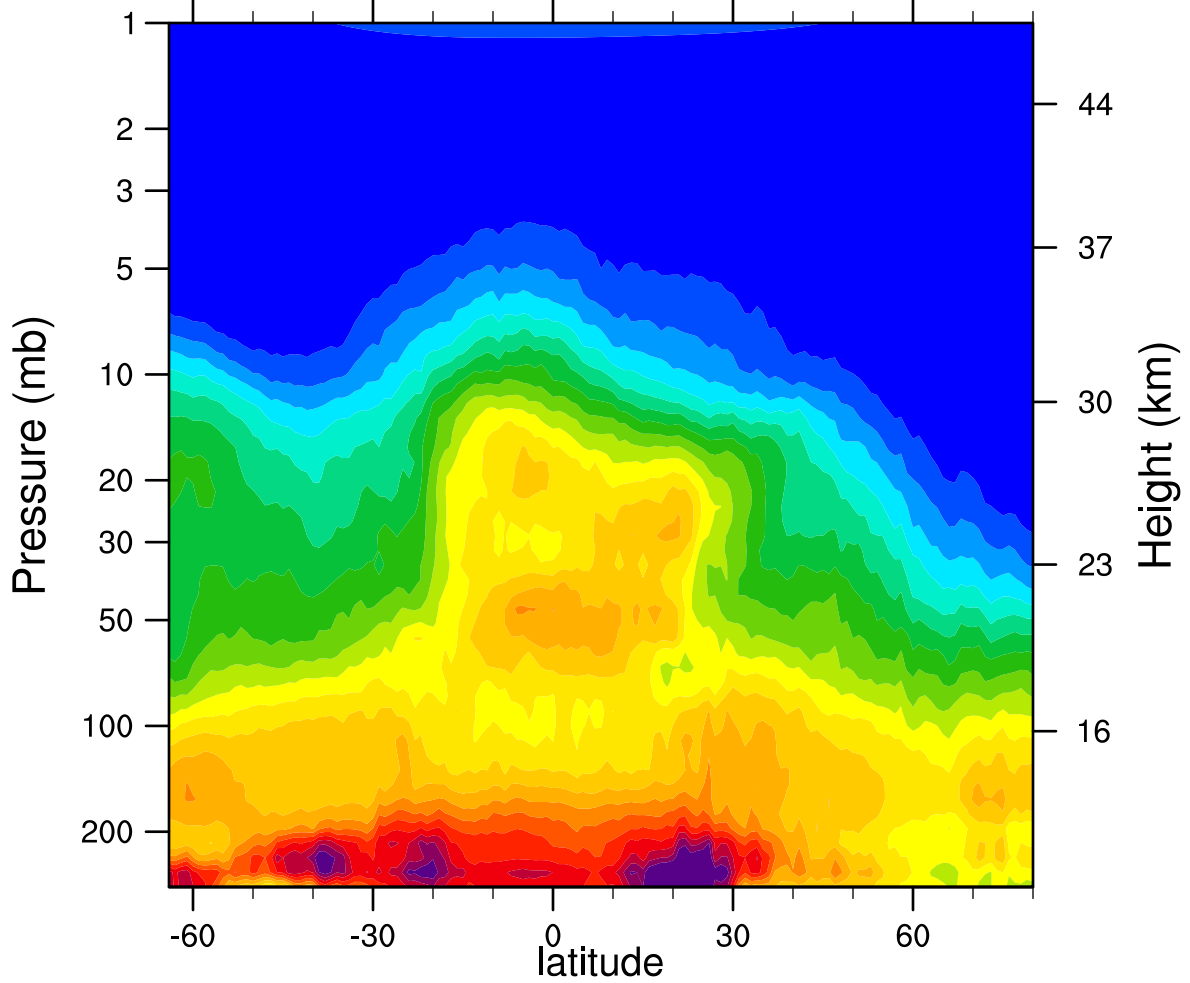
HIRDLSv6 2007d349 N2O_Combined (ppbv)
