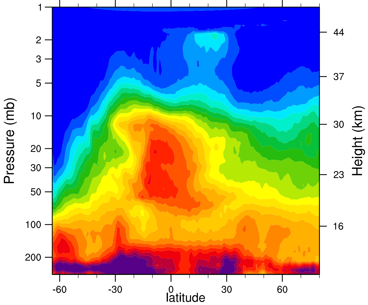
HIRDLSv6 2005d175 N2O_Combined (ppbv)
