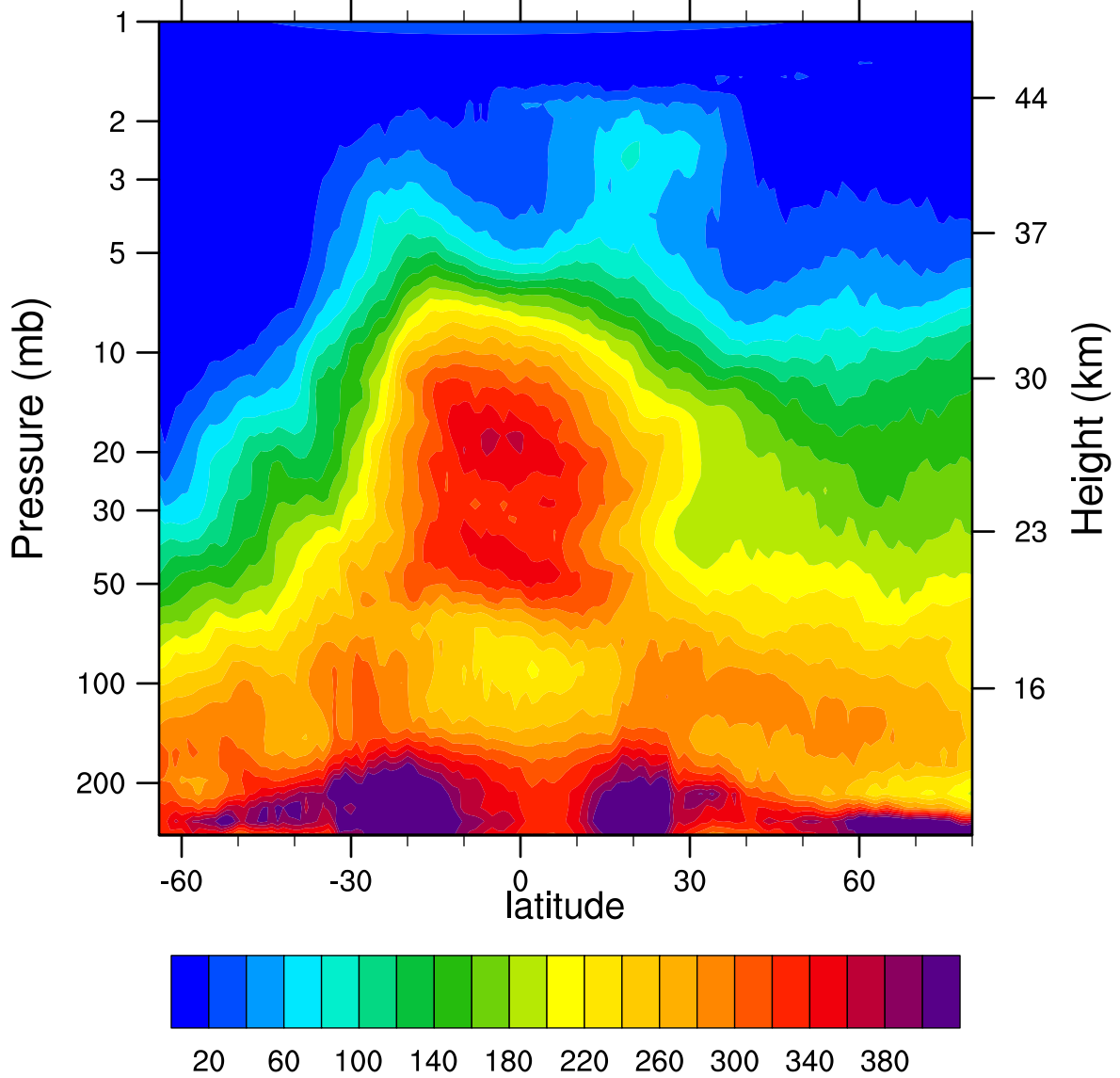
HIRDLSv6 2005d118 N2O_Combined (ppbv)
