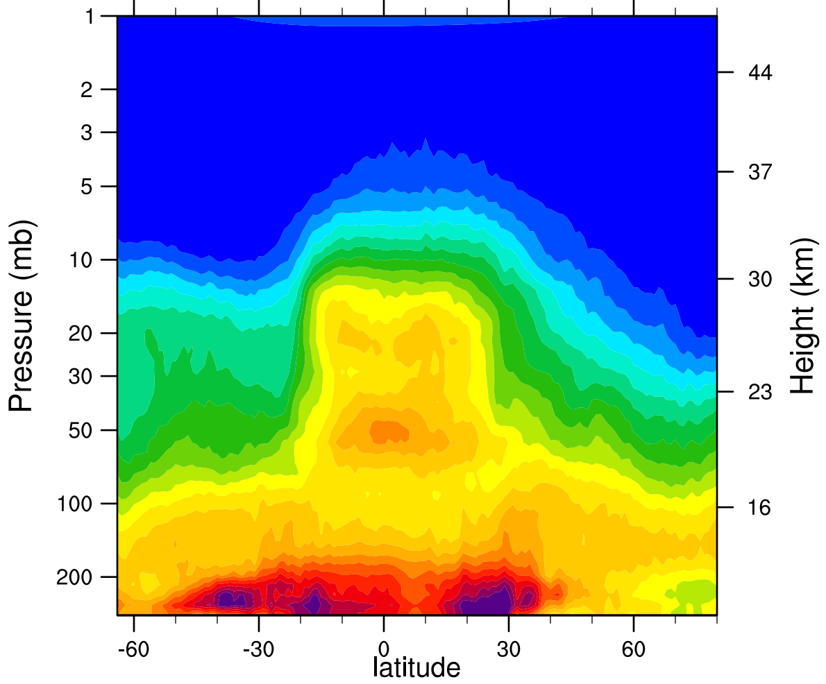
HIRDLSv6 2007d301 N2O_Combined (ppbv)
