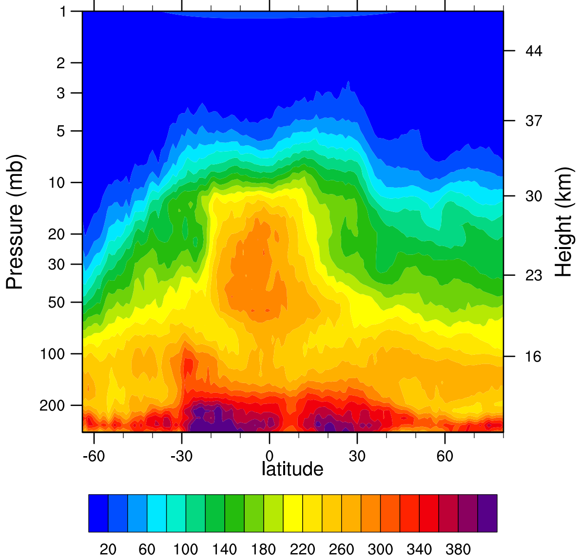
HIRDLSv6 2007d164 N2O_Combined (ppbv)
