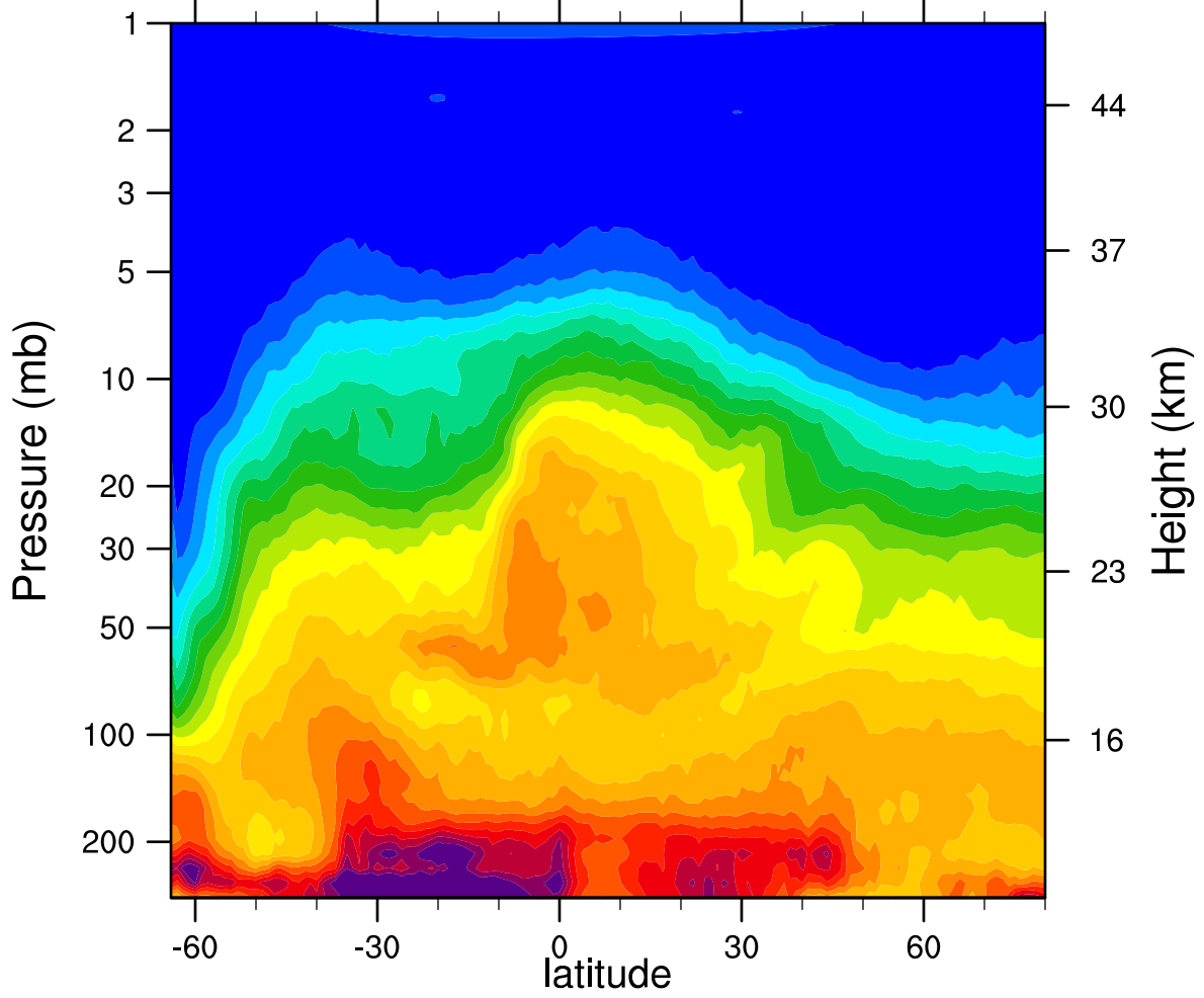
HIRDLSv6 2006d226 N2O_Combined (ppbv)
