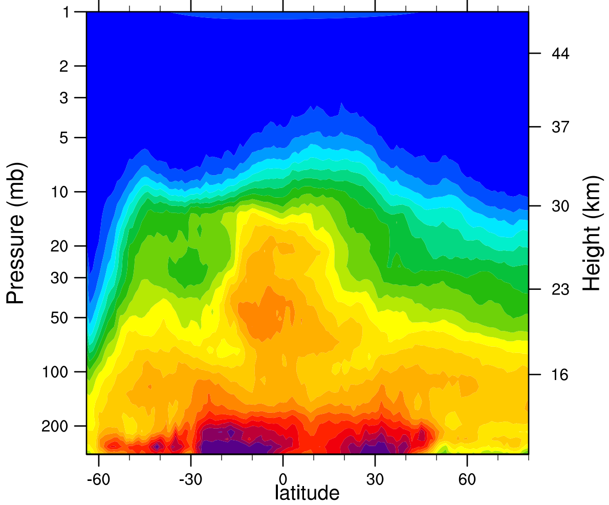
HIRDLSv6 2007d209 N2O_Combined (ppbv)
