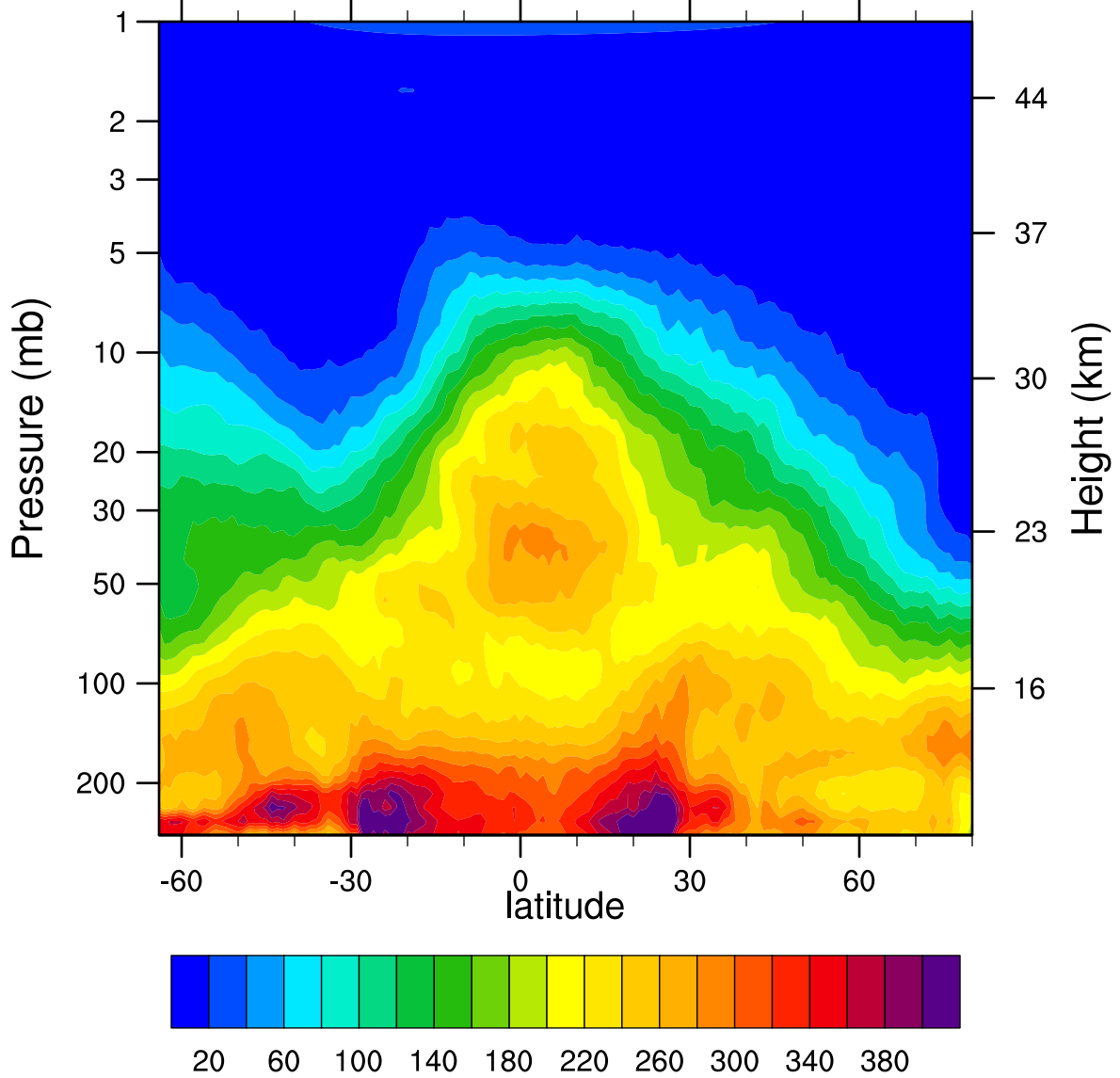
HIRDLSv6 2006d348 N2O_Combined (ppbv)
