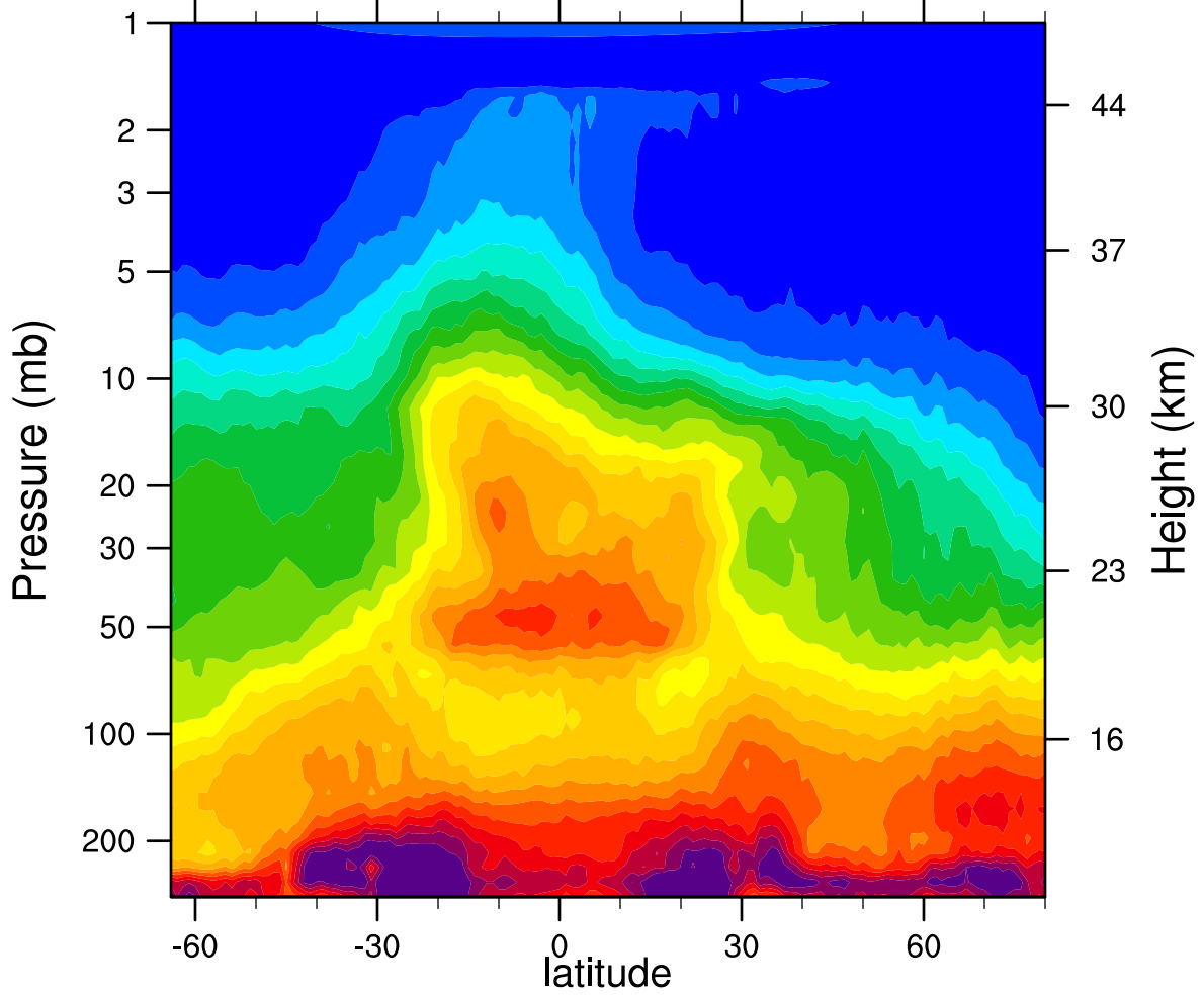
HIRDLSv6 2005d354 N2O_Combined (ppbv)
