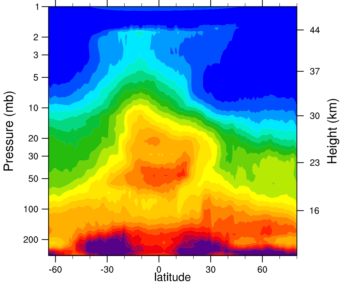
HIRDLSv6 2006d042 N2O_Combined (ppbv)
