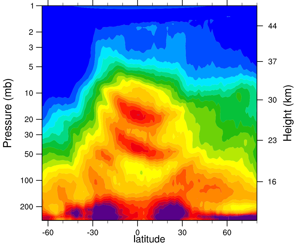
HIRDLSv6 2005d091 N2O_Combined (ppbv)
