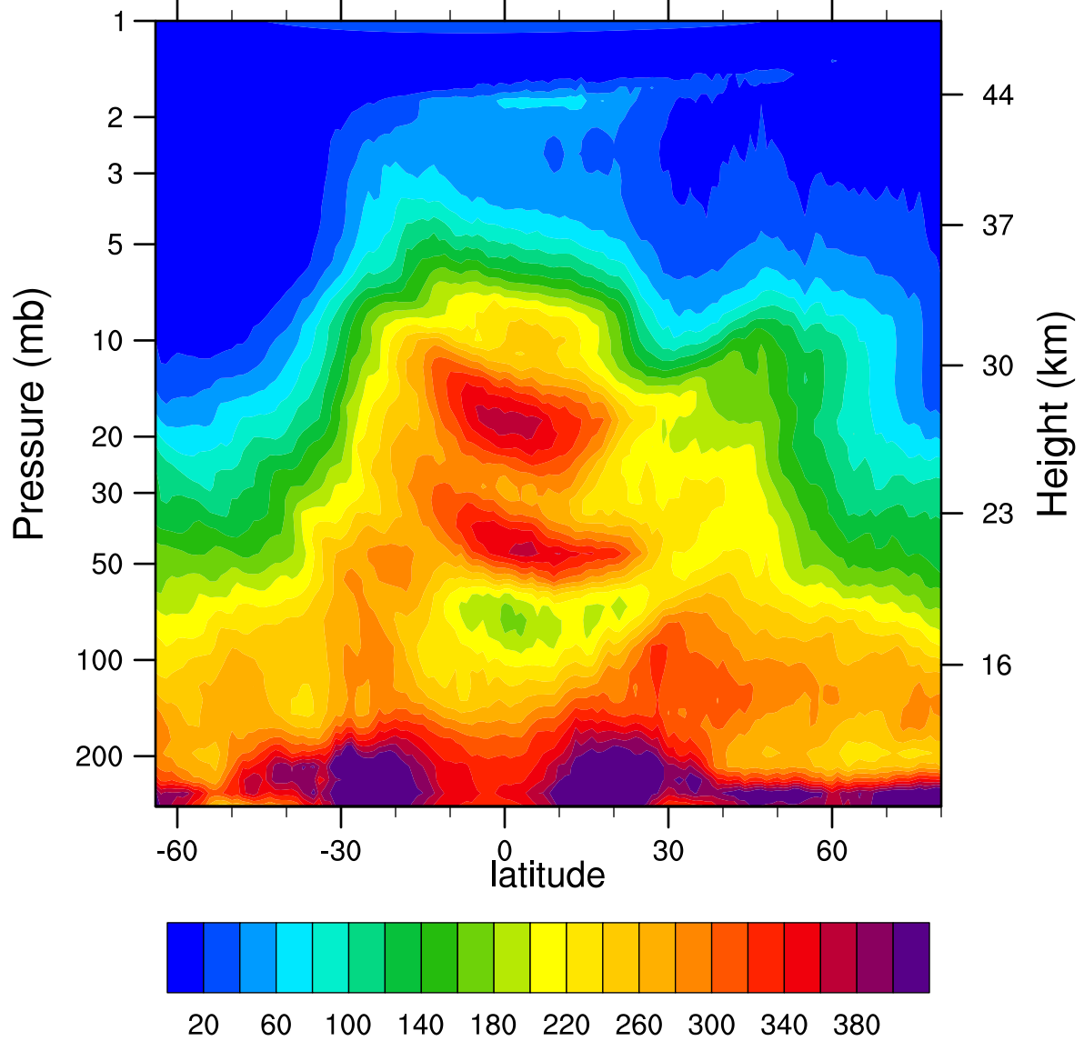
HIRDLSv6 2005d069 N2O_Combined (ppbv)
