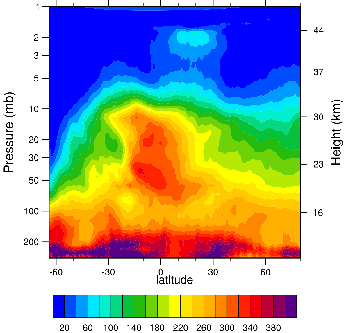
HIRDLSv6 2005d186 N2O_Combined (ppbv)
