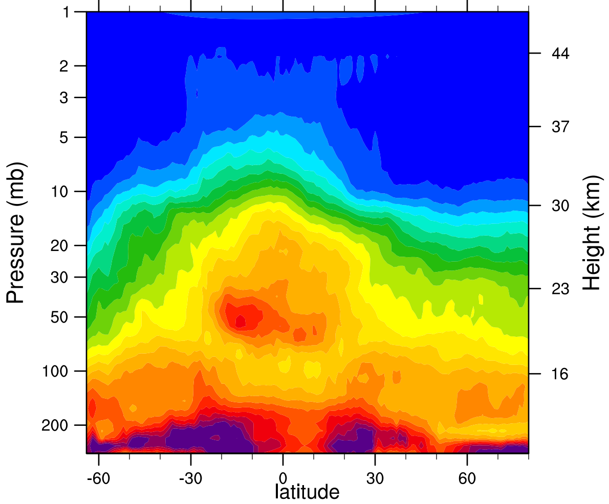
HIRDLSv6 2006d134 N2O_Combined (ppbv)
