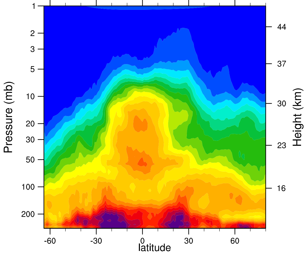
HIRDLSv6 2007d132 N2O_Combined (ppbv)
