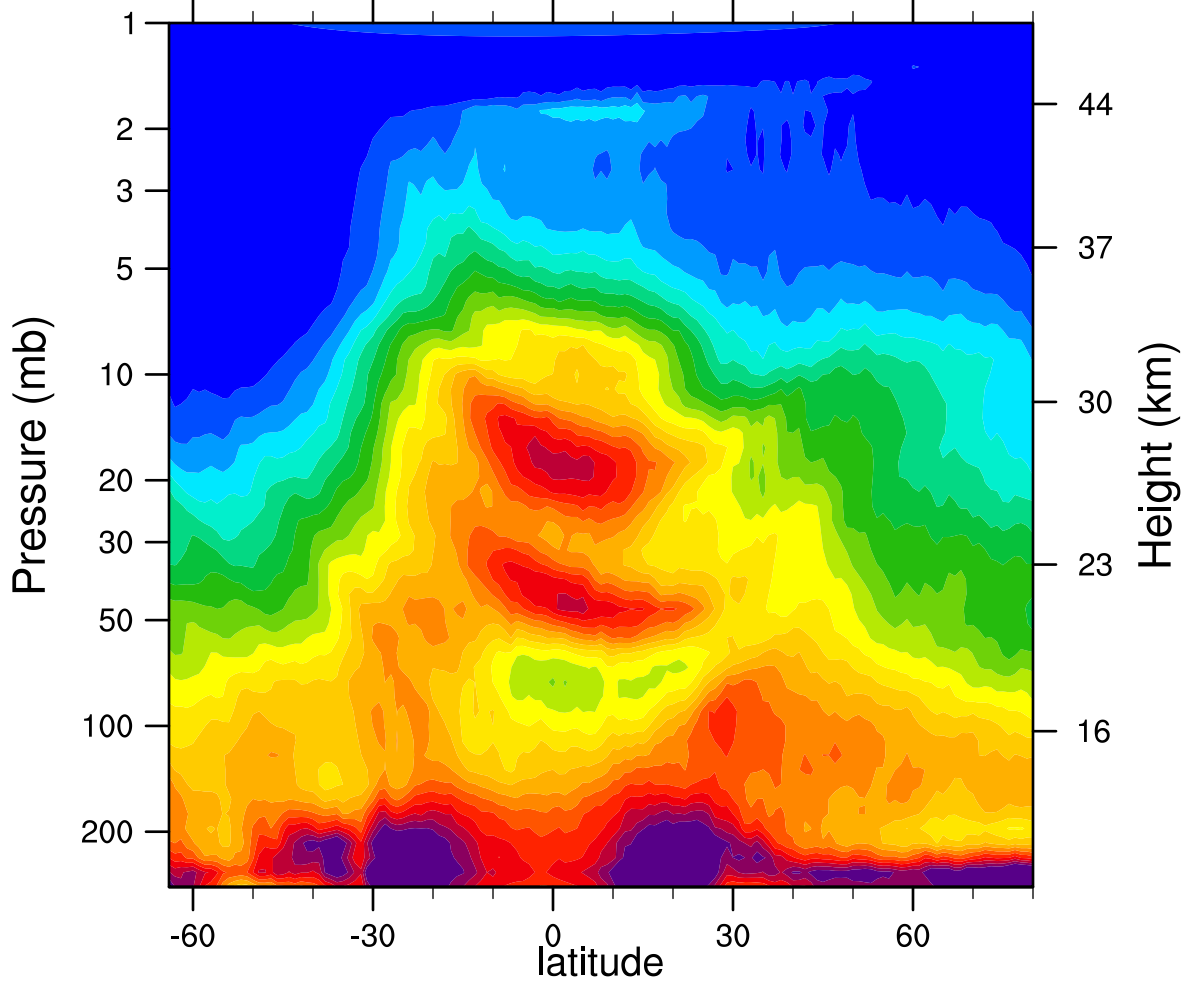
HIRDLSv6 2005d072 N2O_Combined (ppbv)
