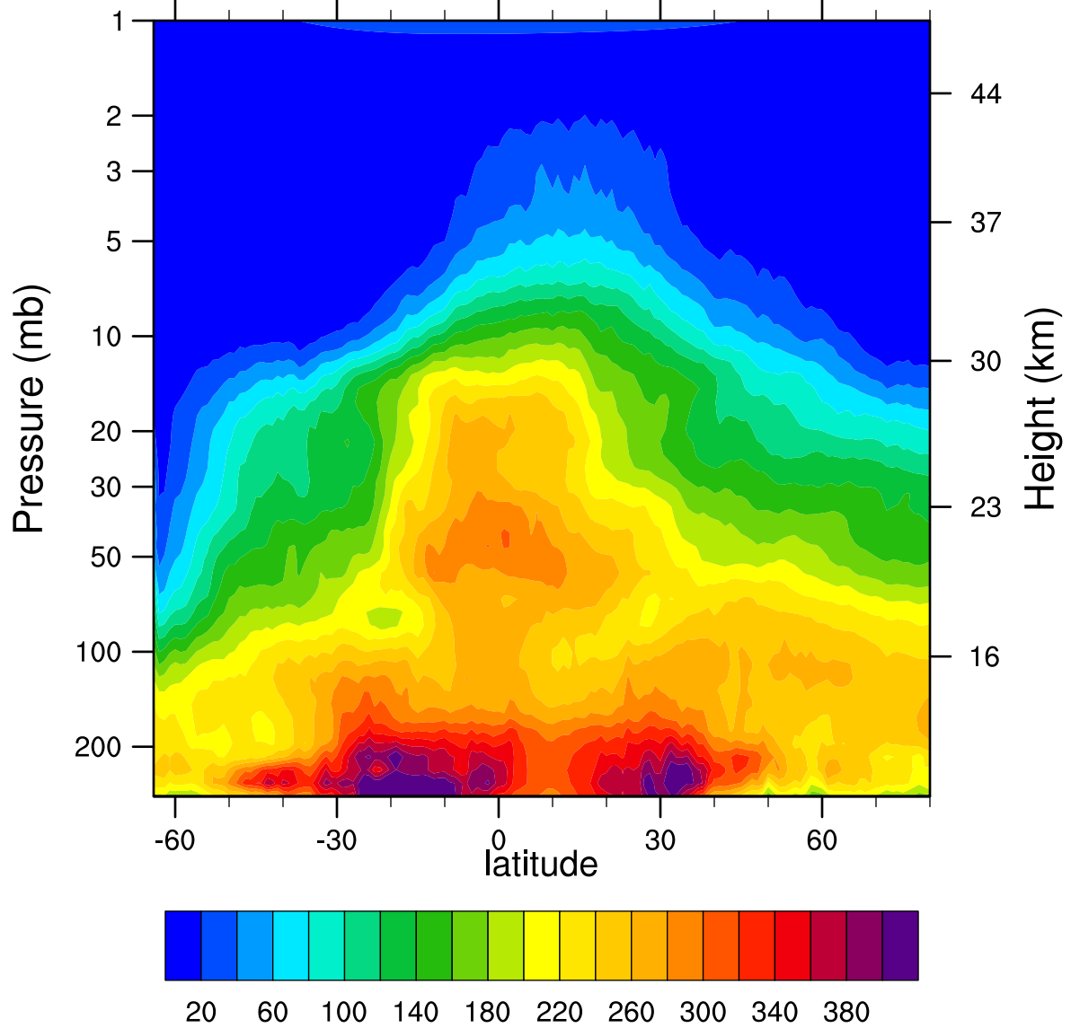
HIRDLSv6 2007d230 N2O_Combined (ppbv)
