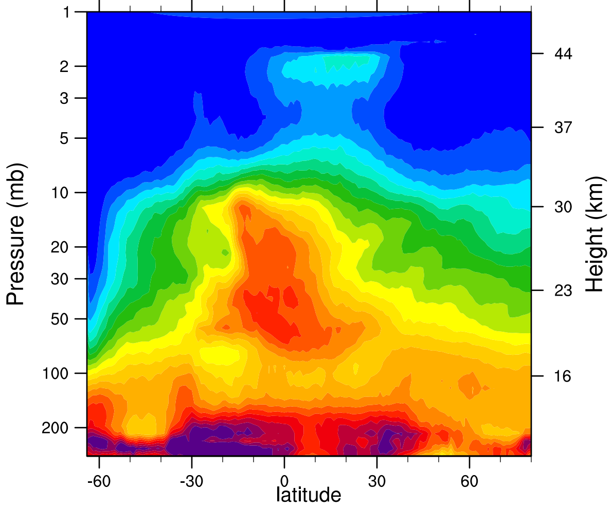
HIRDLSv6 2005d215 N2O_Combined (ppbv)
