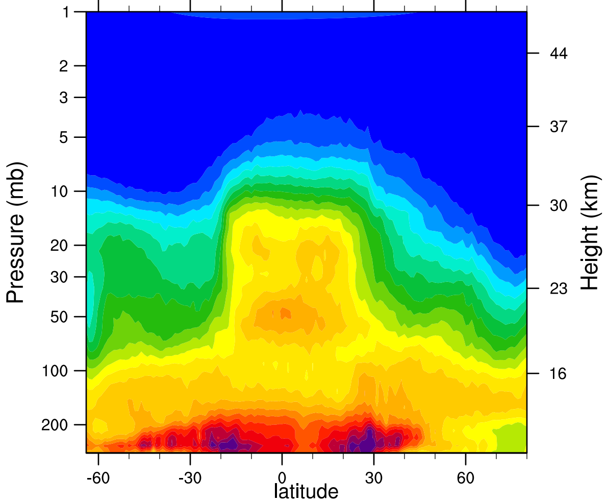
HIRDLSv6 2007d307 N2O_Combined (ppbv)
