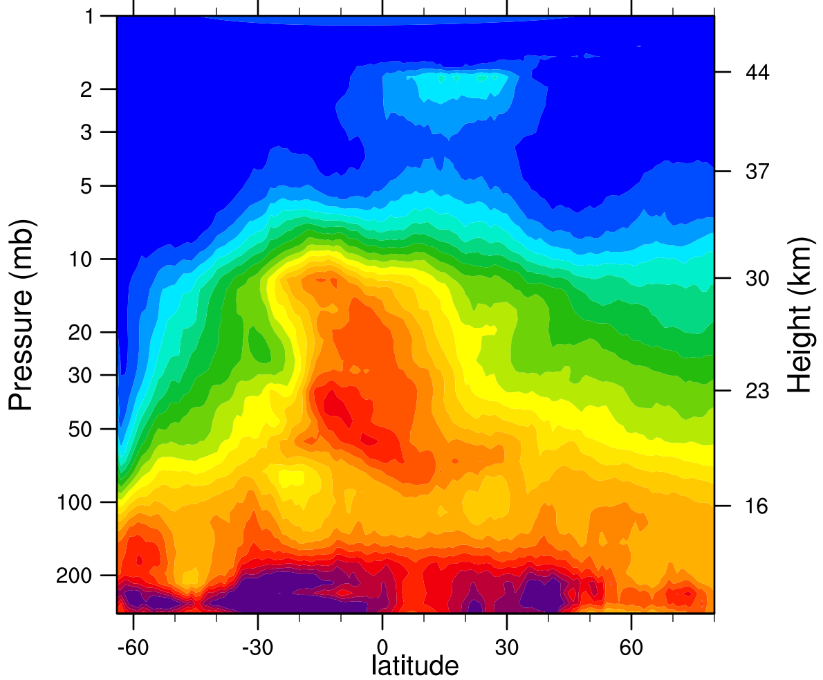
HIRDLSv6 2005d200 N2O_Combined (ppbv)
