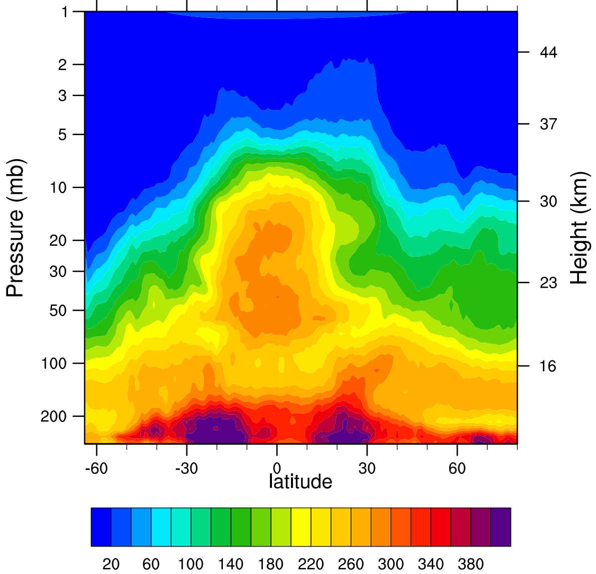
HIRDLSv6 2007d125 N2O_Combined (ppbv)
