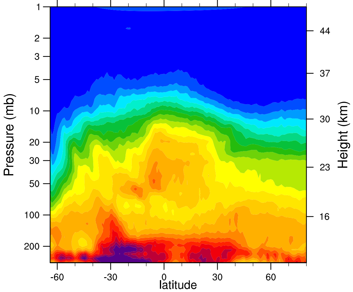
HIRDLSv6 2006d185 N2O_Combined (ppbv)
