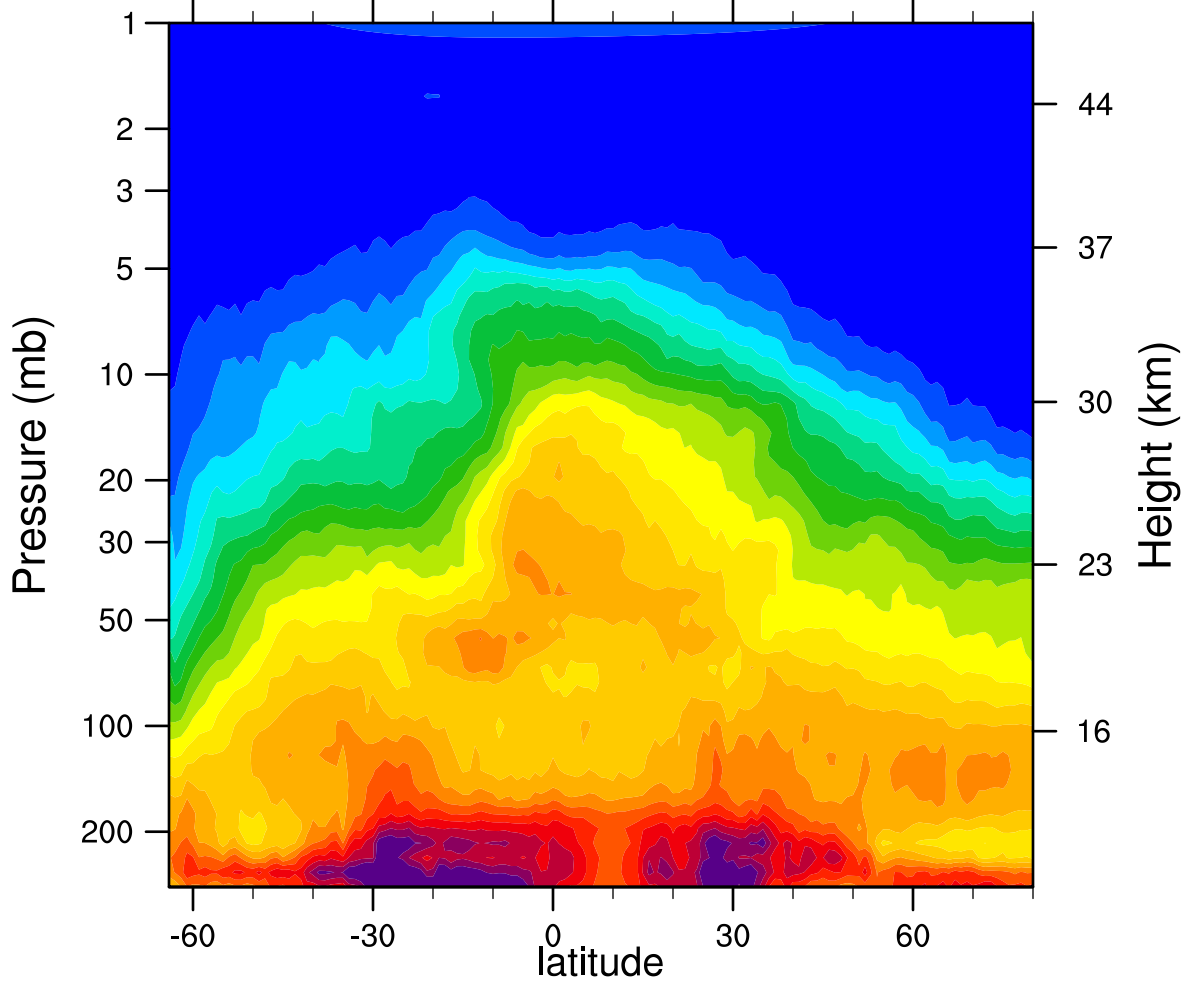
HIRDLSv6 2006d273 N2O_Combined (ppbv)
