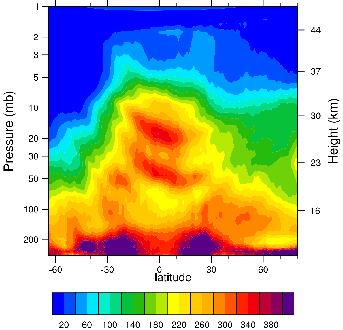
HIRDLSv6 2005d095 N2O_Combined (ppbv)
