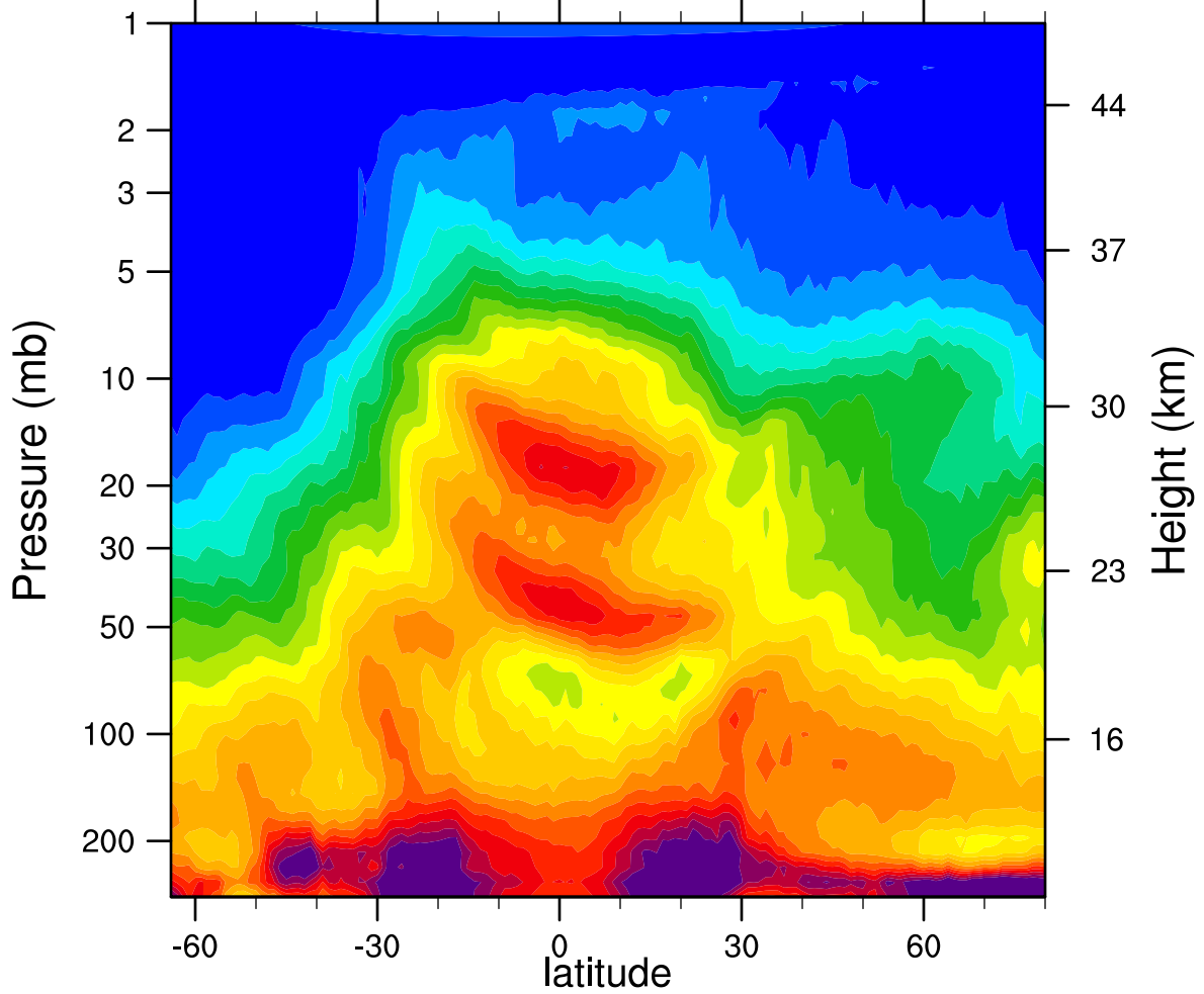
HIRDLSv6 2005d083 N2O_Combined (ppbv)
