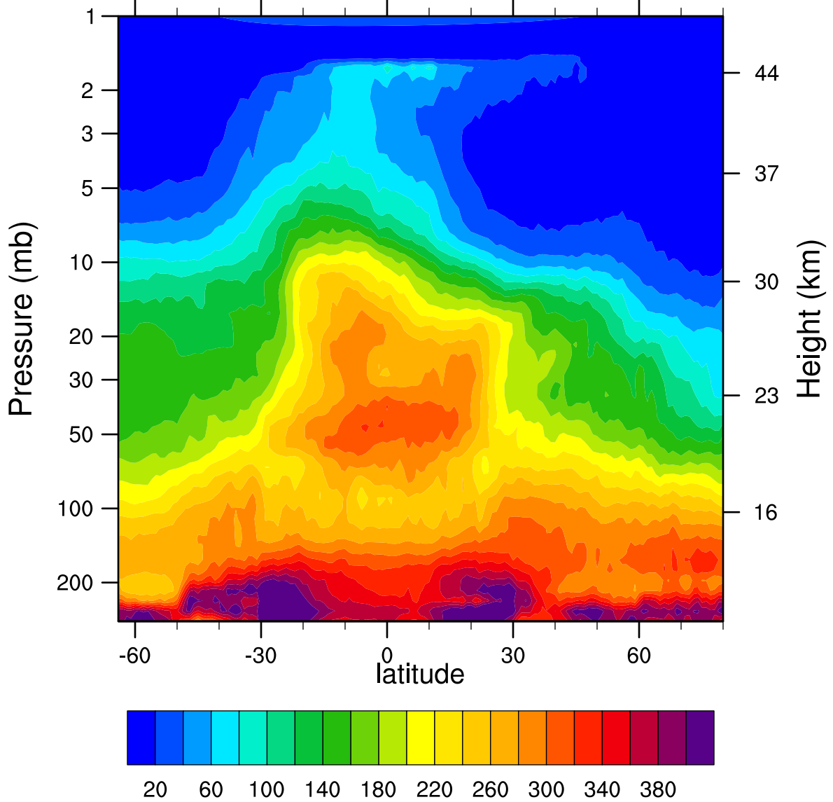
HIRDLSv6 2006d004 N2O_Combined (ppbv)
