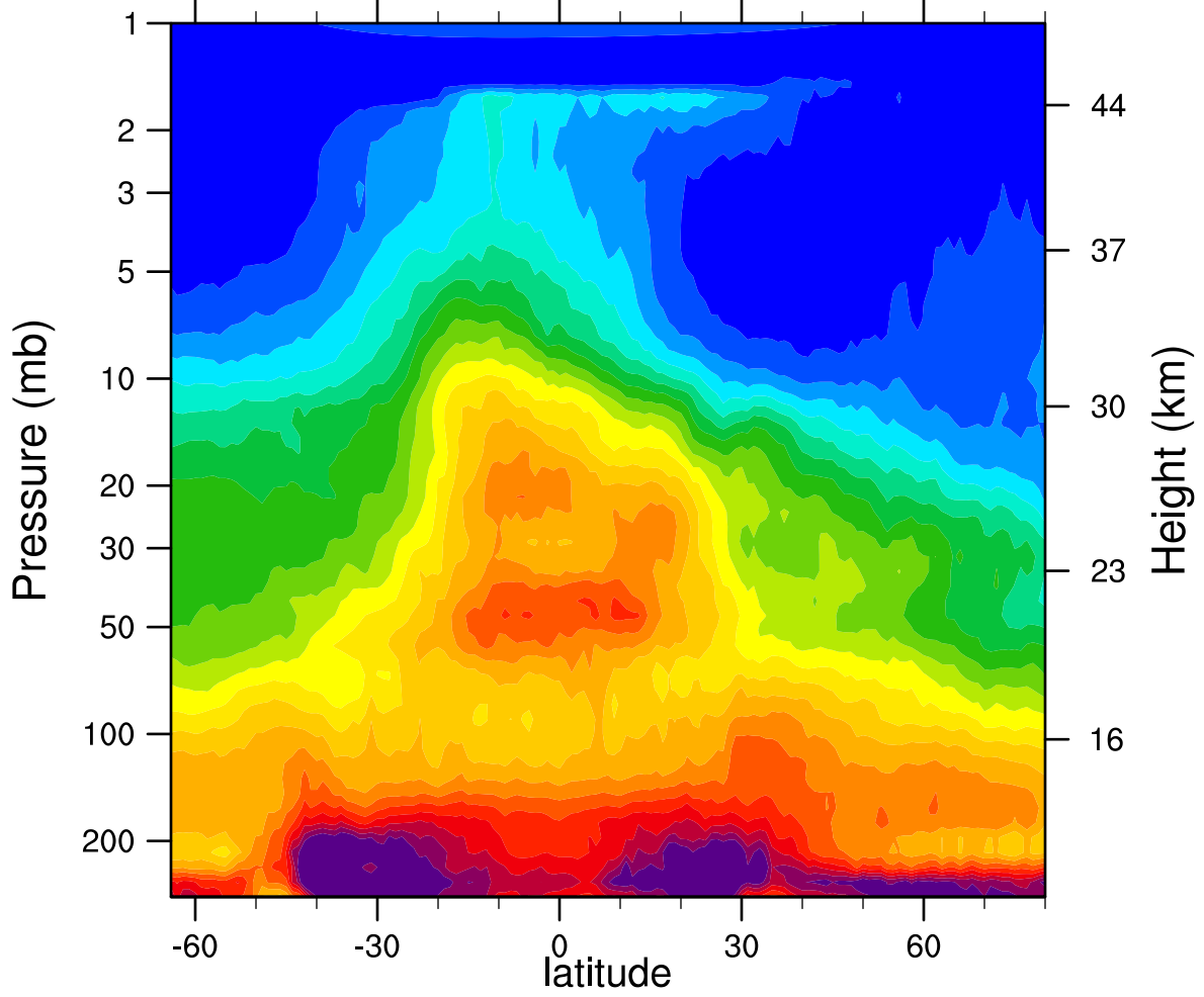
HIRDLSv6 2006d022 N2O_Combined (ppbv)
