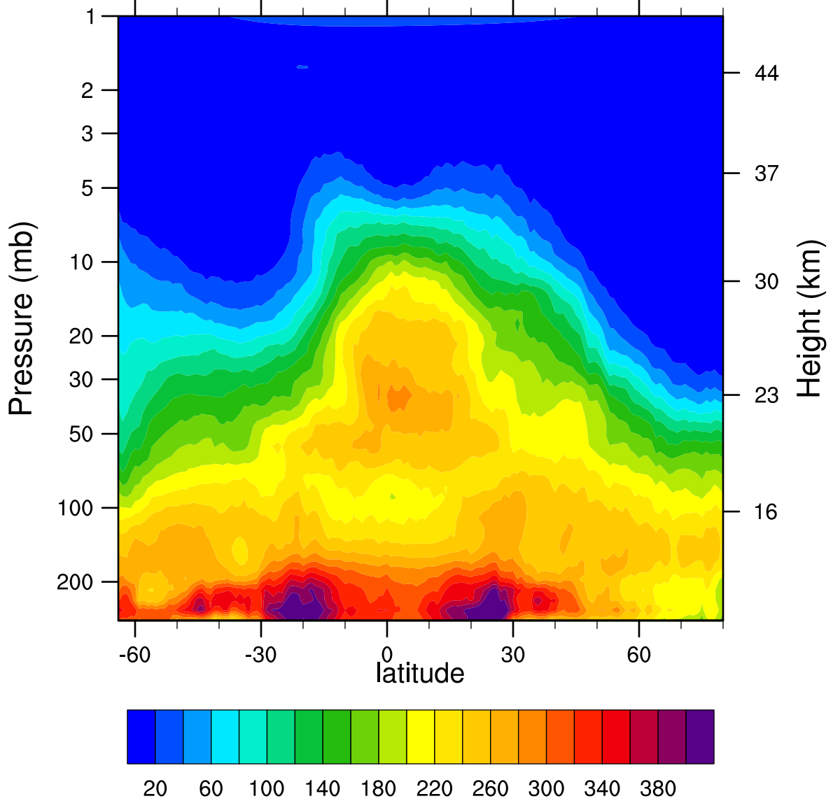
HIRDLSv6 2006d331 N2O_Combined (ppbv)
