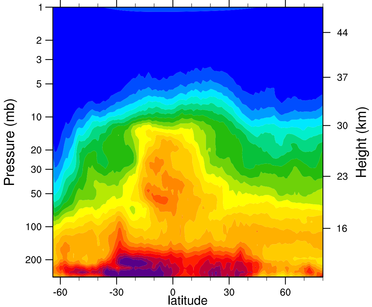
HIRDLSv6 2007d188 N2O_Combined (ppbv)
