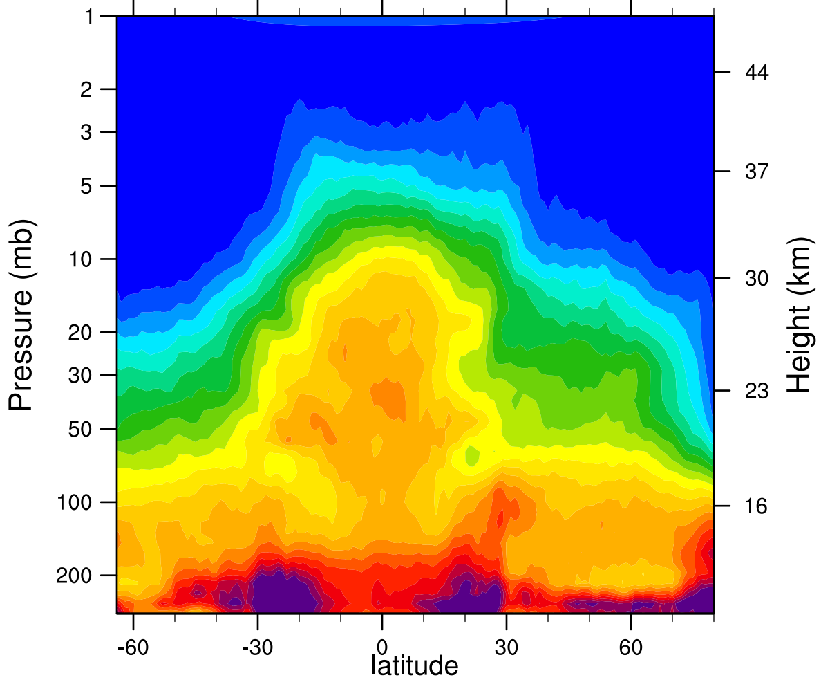
HIRDLSv6 2007d086 N2O_Combined (ppbv)
