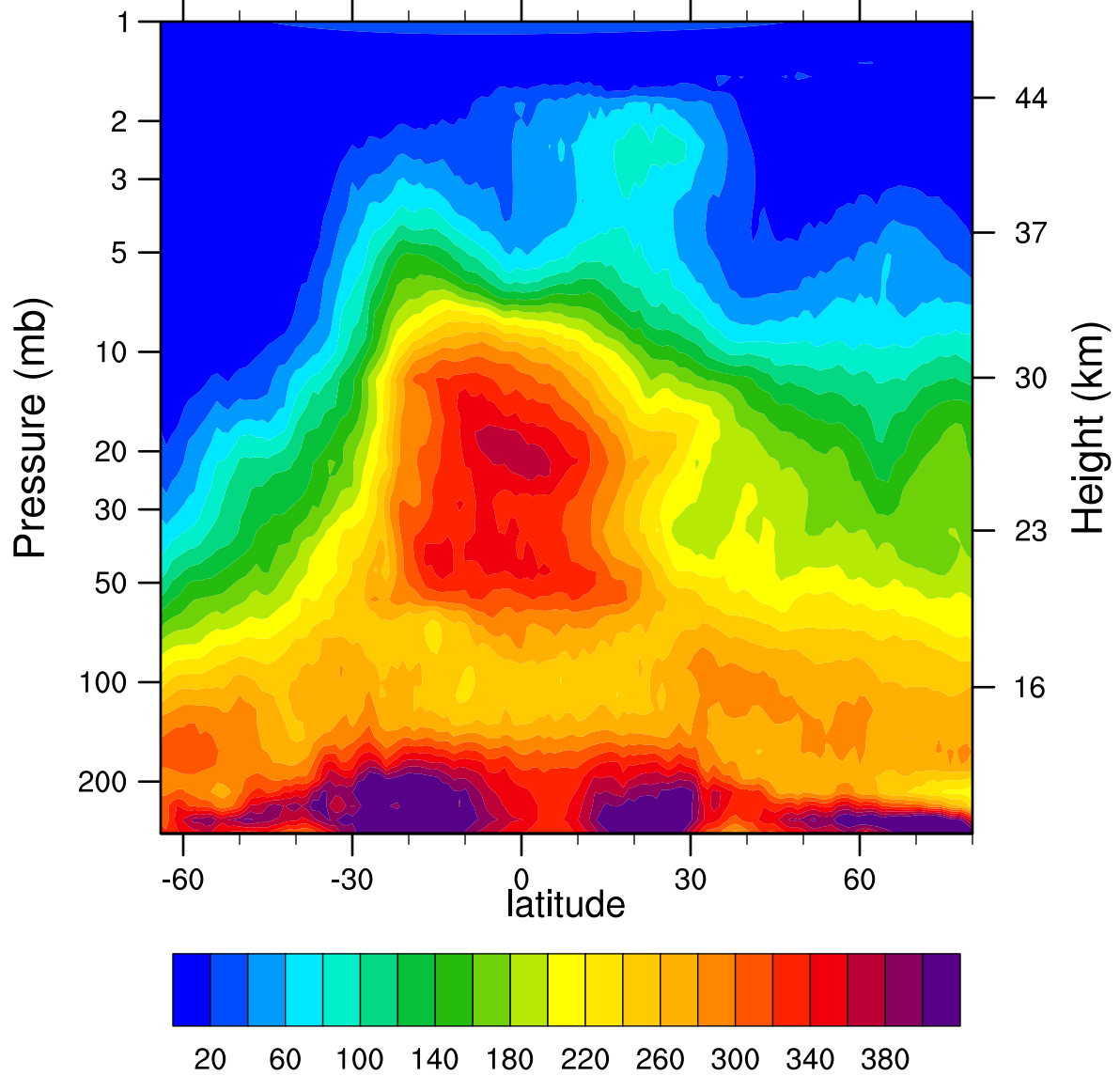
HIRDLSv6 2005d133 N2O_Combined (ppbv)
