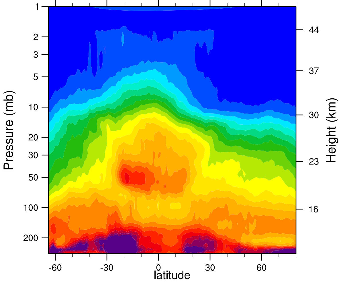
HIRDLSv6 2006d125 N2O_Combined (ppbv)
