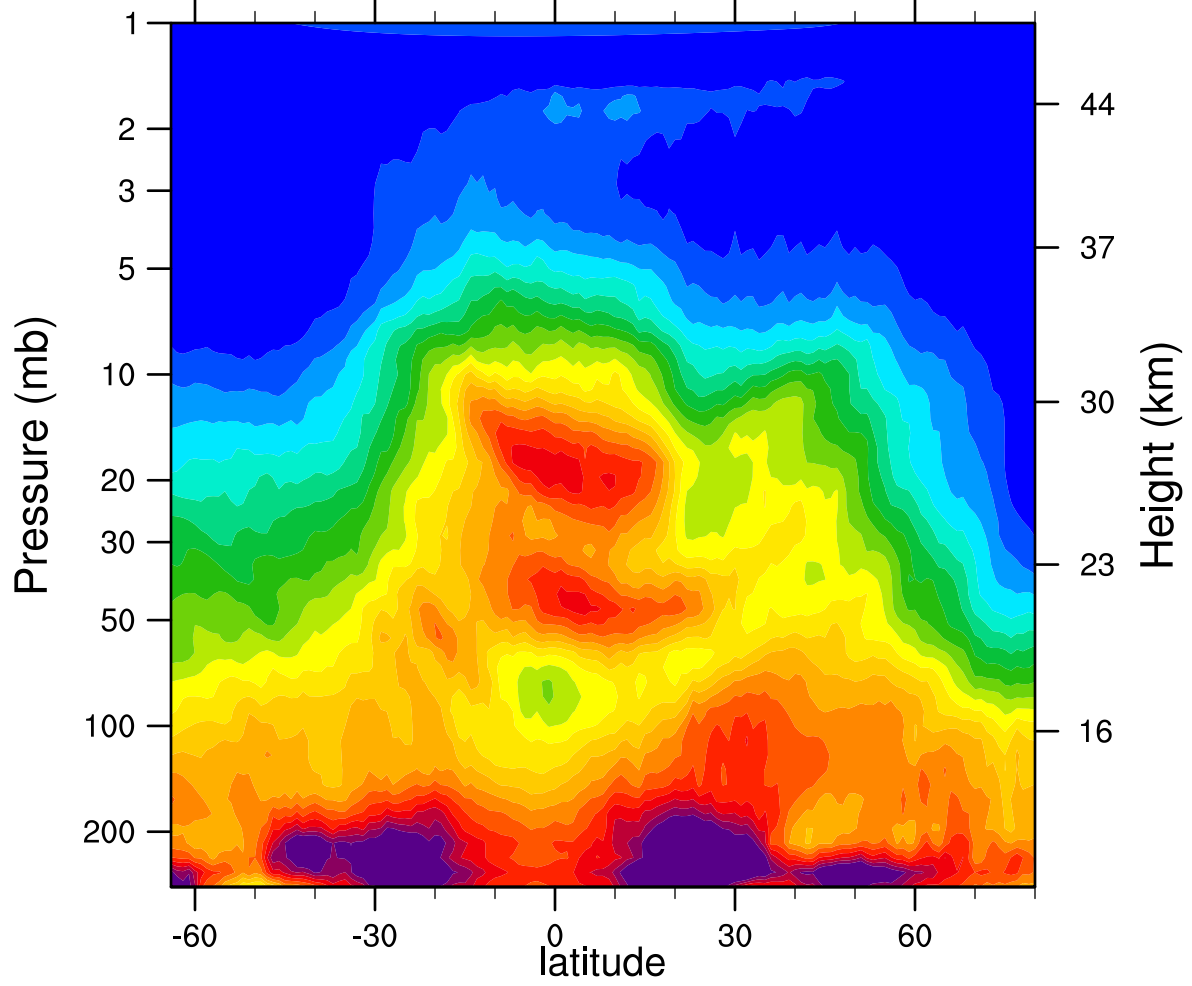
HIRDLSv6 2005d038 N2O_Combined (ppbv)
