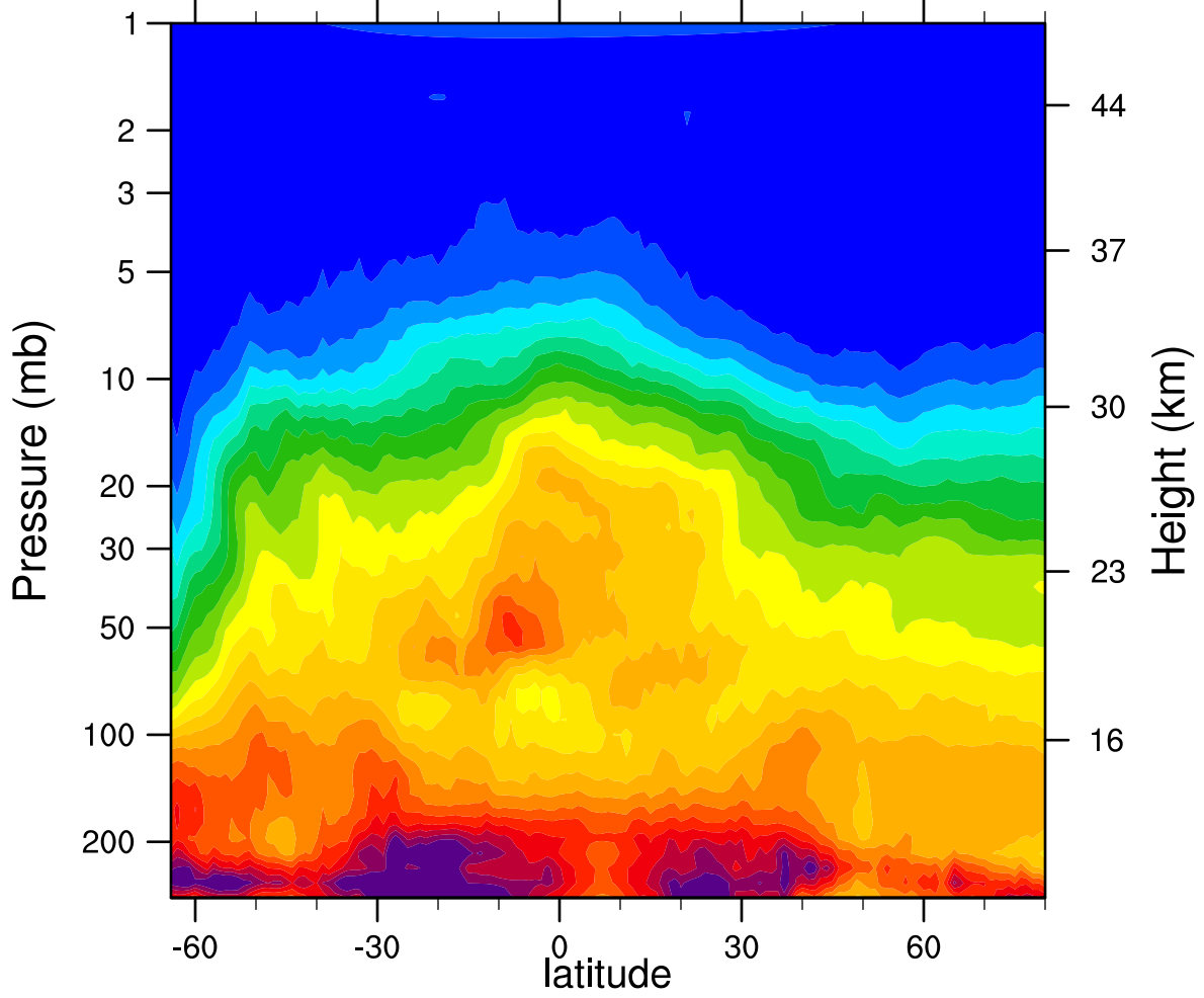
HIRDLSv6 2006d175 N2O_Combined (ppbv)
