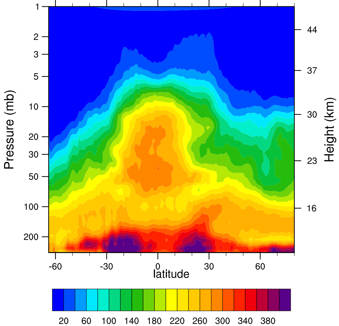
HIRDLSv6 2007d121 N2O_Combined (ppbv)
