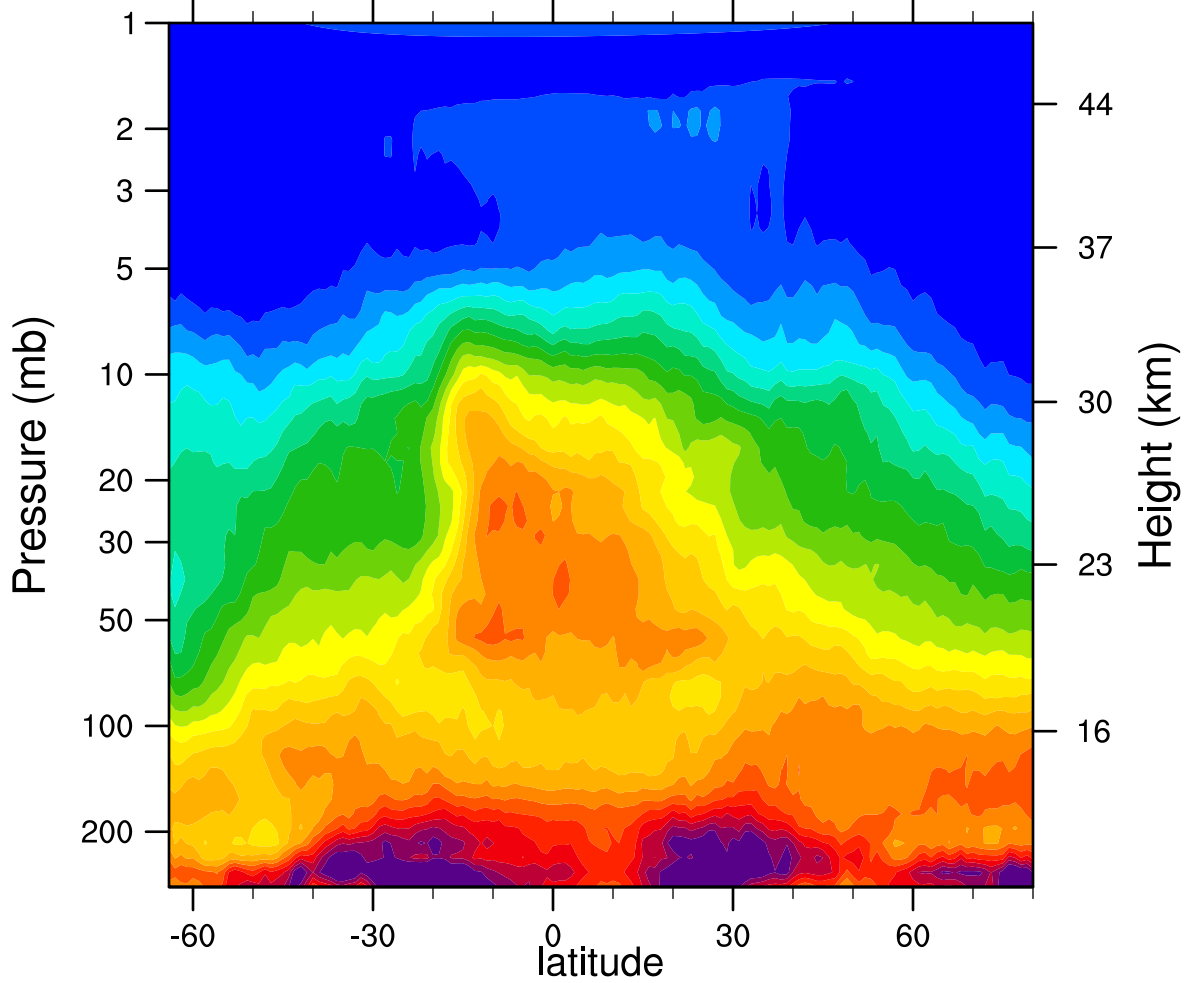
HIRDLSv6 2005d288 N2O_Combined (ppbv)
