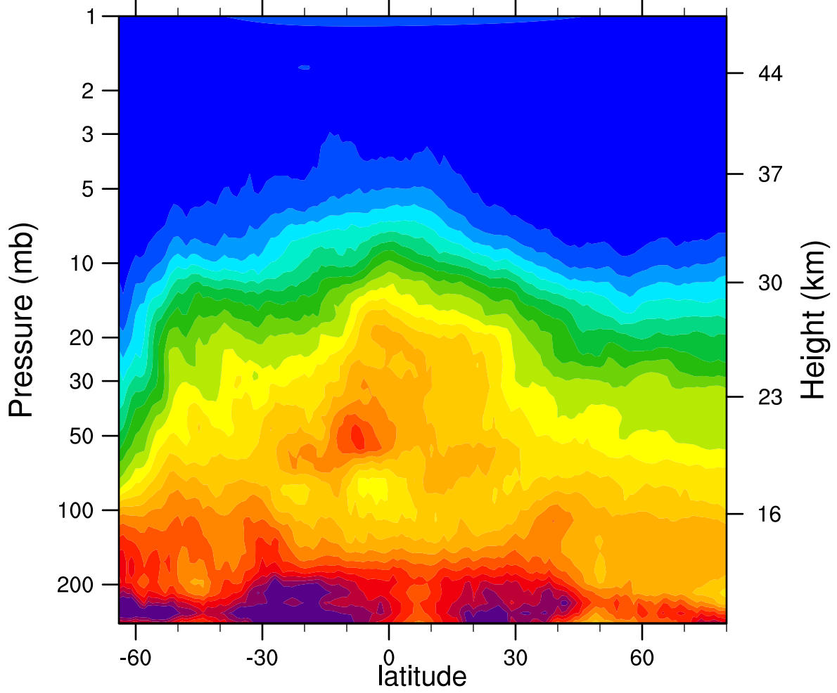
HIRDLSv6 2006d174 N2O_Combined (ppbv)
