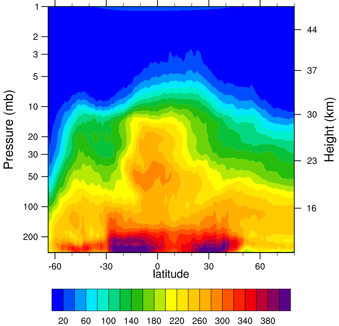
HIRDLSv6 2007d212 N2O_Combined (ppbv)
