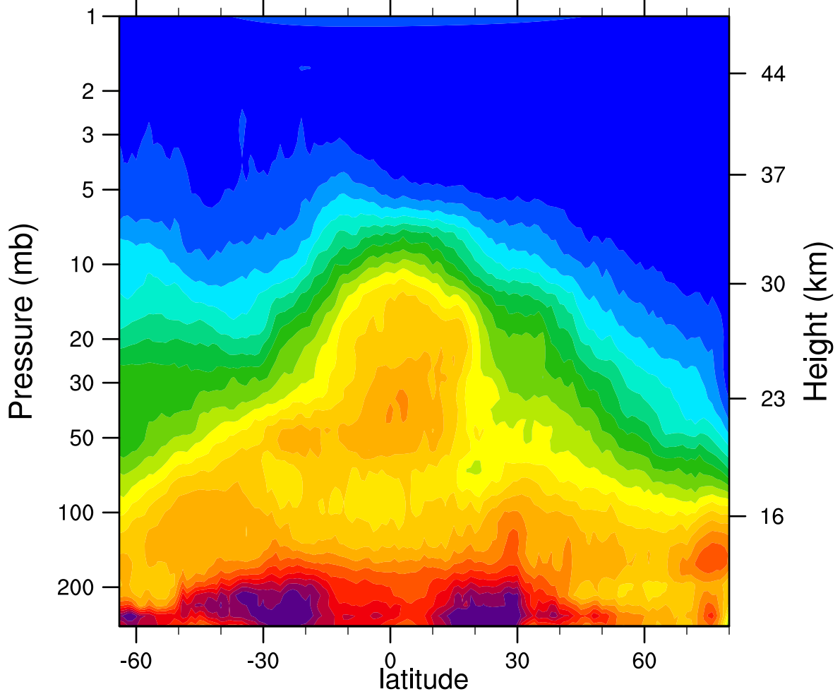
HIRDLSv6 2006d358 N2O_Combined (ppbv)
