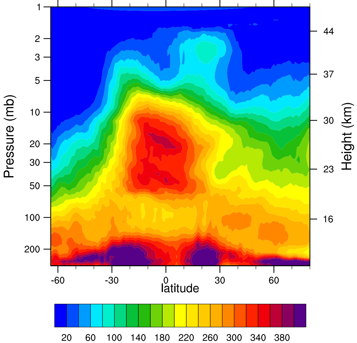
HIRDLSv6 2005d124 N2O_Combined (ppbv)
