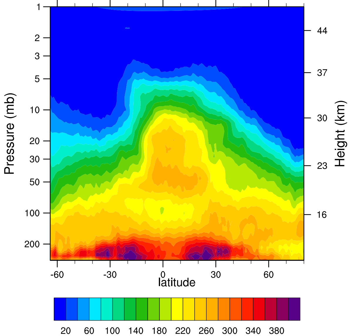
HIRDLSv6 2006d315 N2O_Combined (ppbv)
