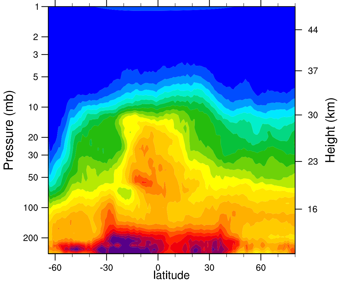
HIRDLSv6 2007d191 N2O_Combined (ppbv)
