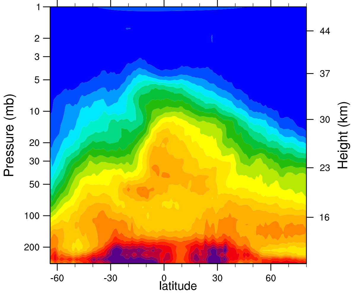
HIRDLSv6 2006d275 N2O_Combined (ppbv)
