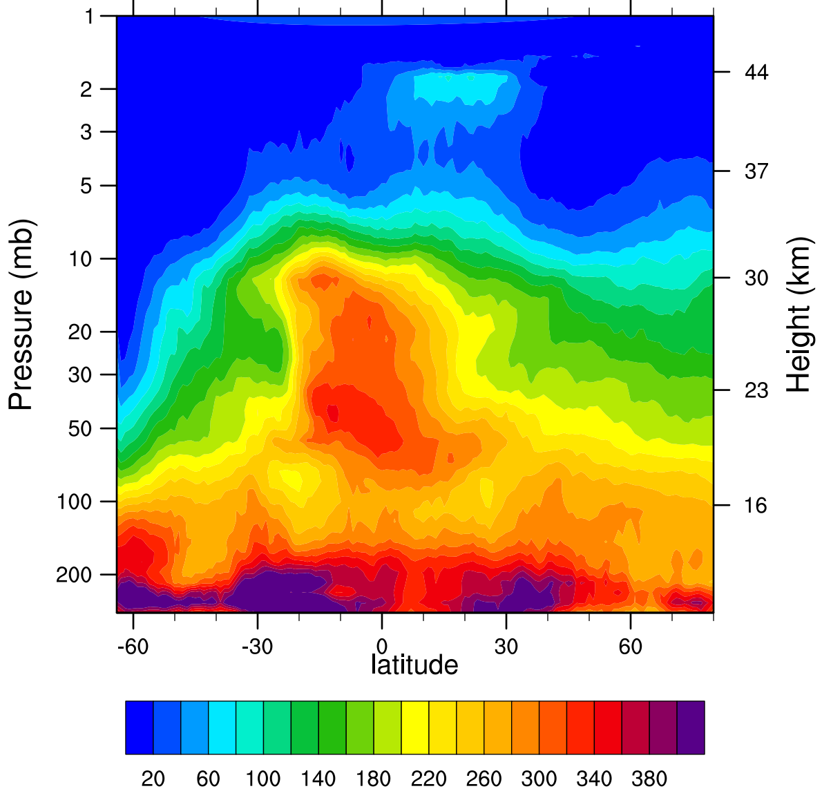
HIRDLSv6 2005d192 N2O_Combined (ppbv)
