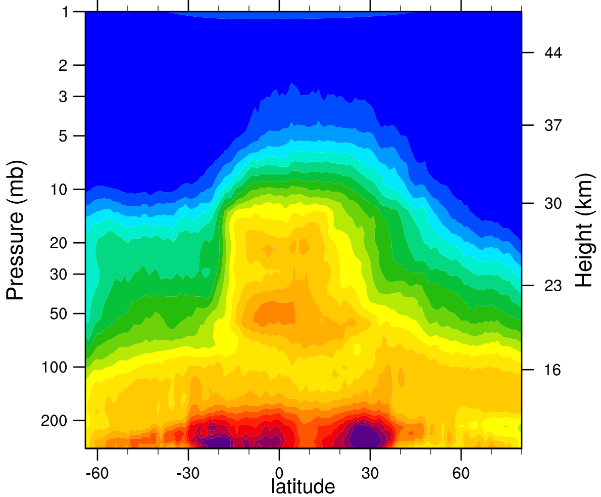
HIRDLSv6 2007d281 N2O_Combined (ppbv)
