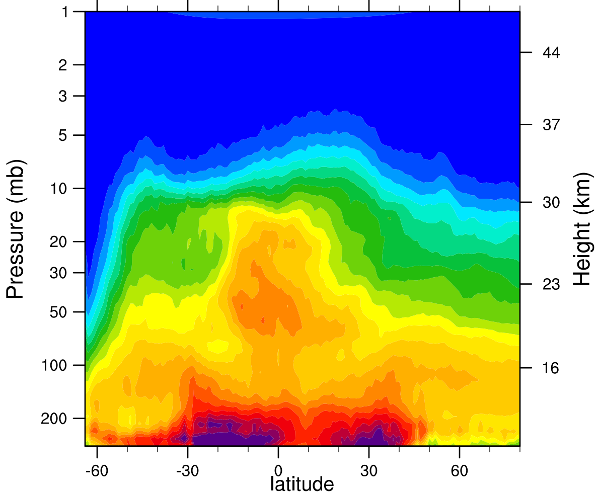
HIRDLSv6 2007d206 N2O_Combined (ppbv)
