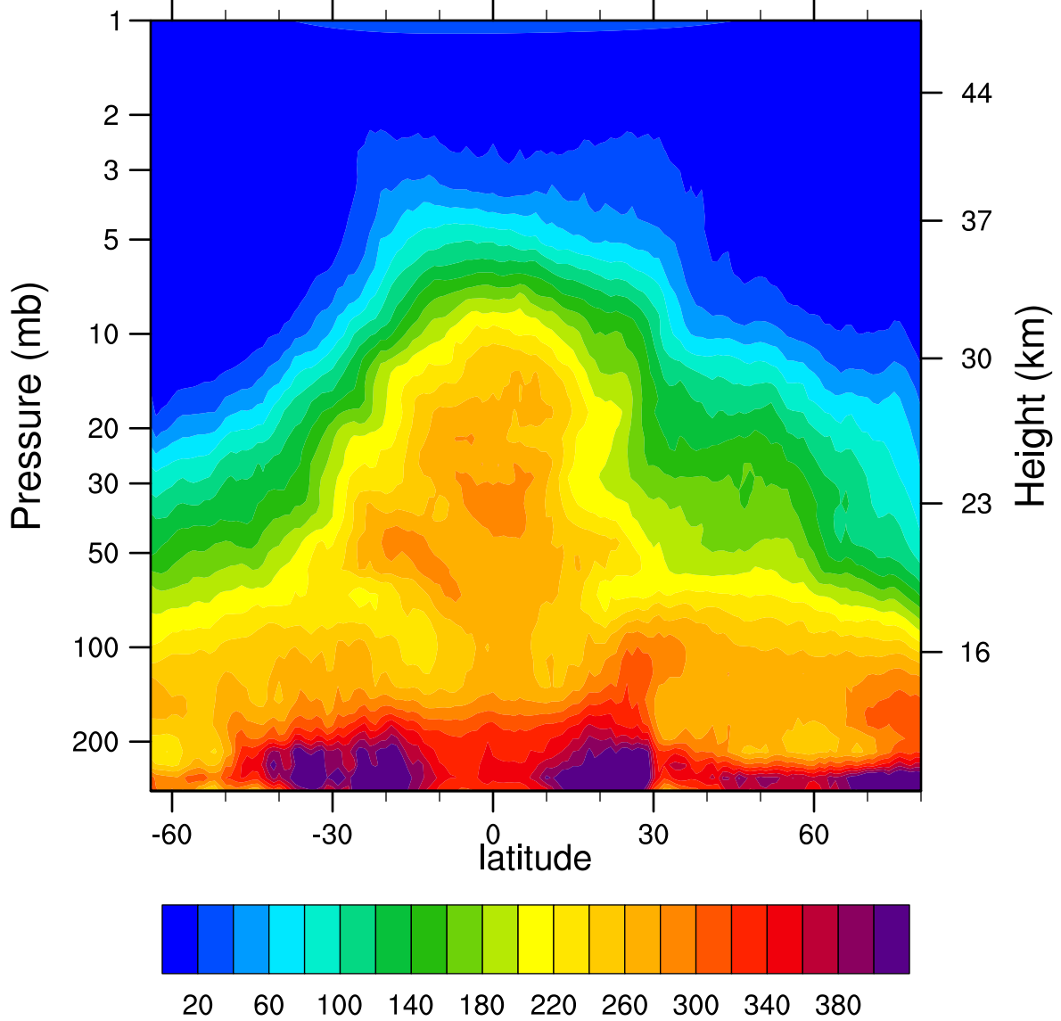
HIRDLSv6 2007d091 N2O_Combined (ppbv)
