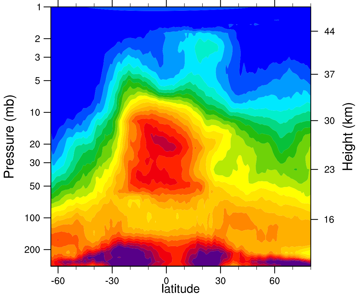
HIRDLSv6 2005d131 N2O_Combined (ppbv)
