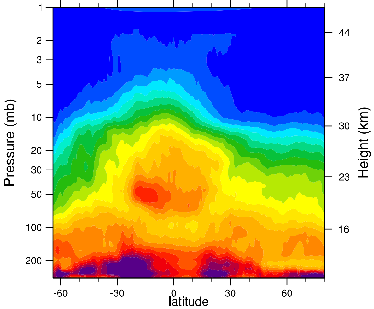
HIRDLSv6 2006d129 N2O_Combined (ppbv)
