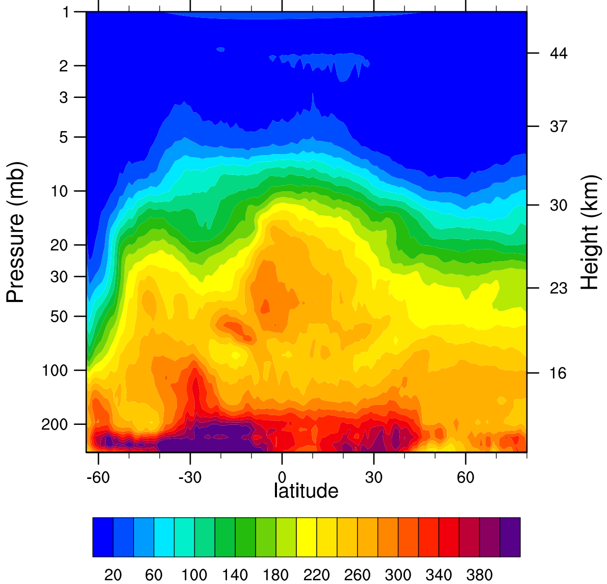
HIRDLSv6 2006d209 N2O_Combined (ppbv)
