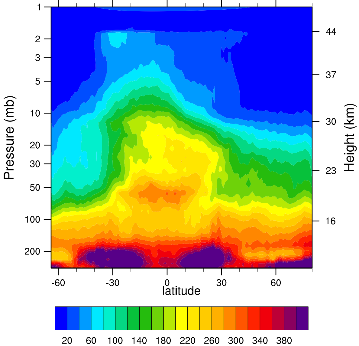
HIRDLSv6 2006d089 N2O_Combined (ppbv)
