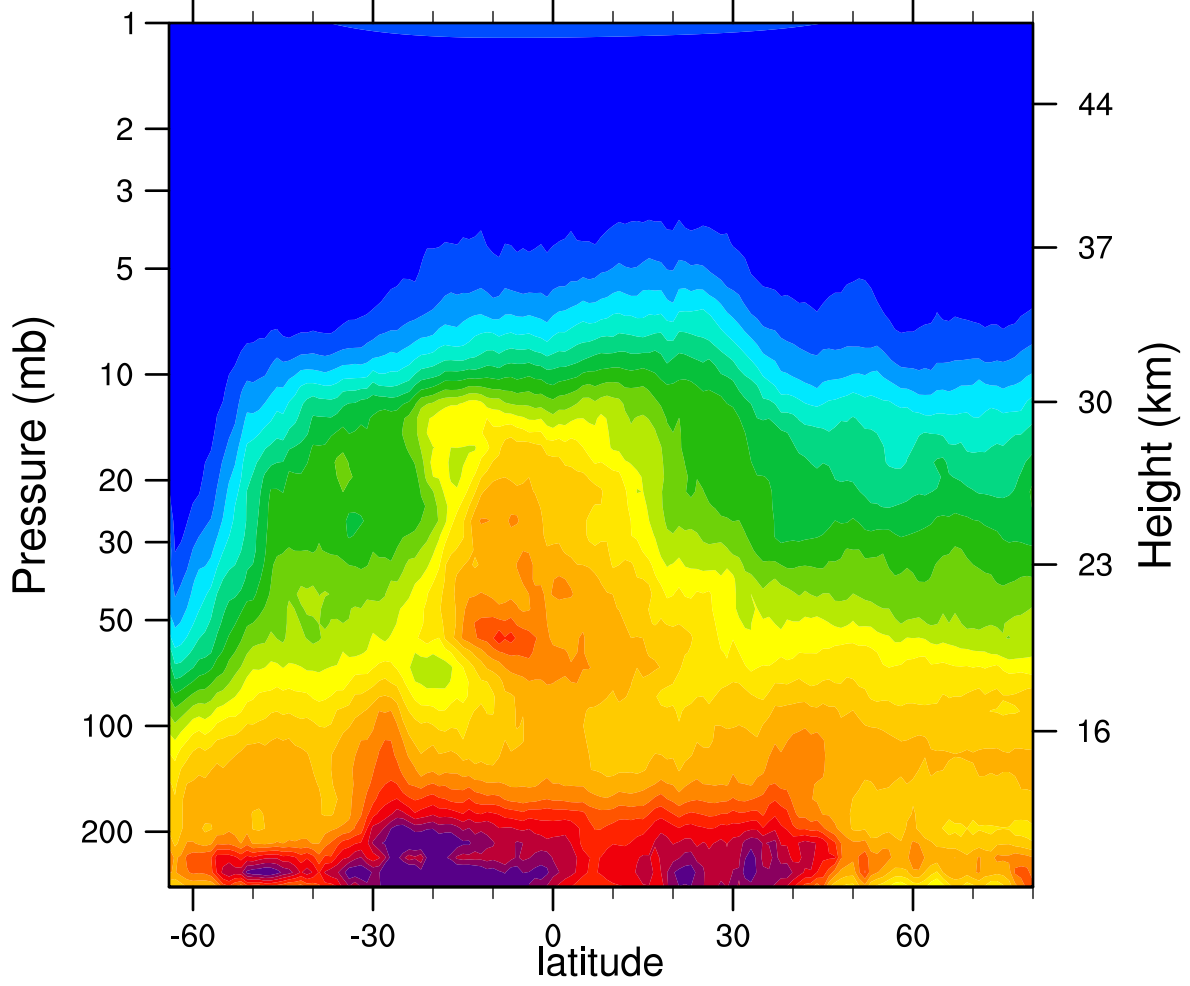
HIRDLSv6 2007d192 N2O_Combined (ppbv)
