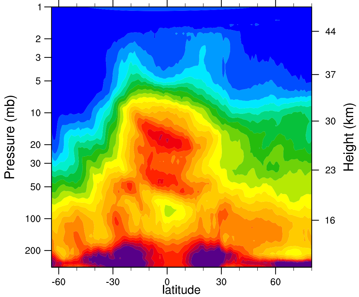
HIRDLSv6 2005d109 N2O_Combined (ppbv)
