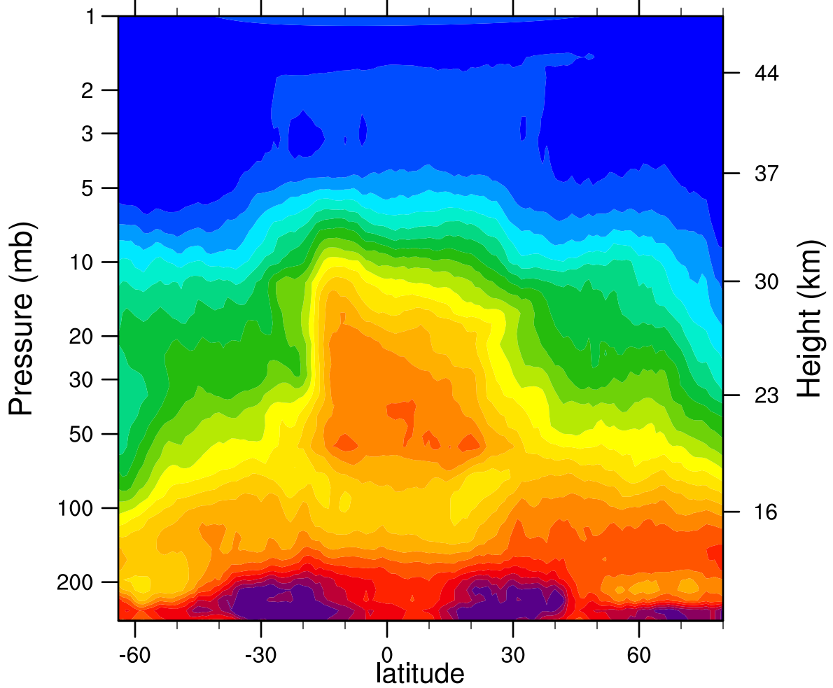
HIRDLSv6 2005d306 N2O_Combined (ppbv)
