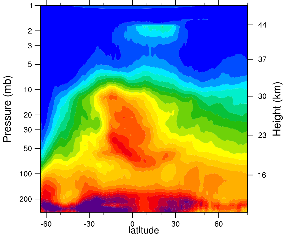
HIRDLSv6 2005d204 N2O_Combined (ppbv)
