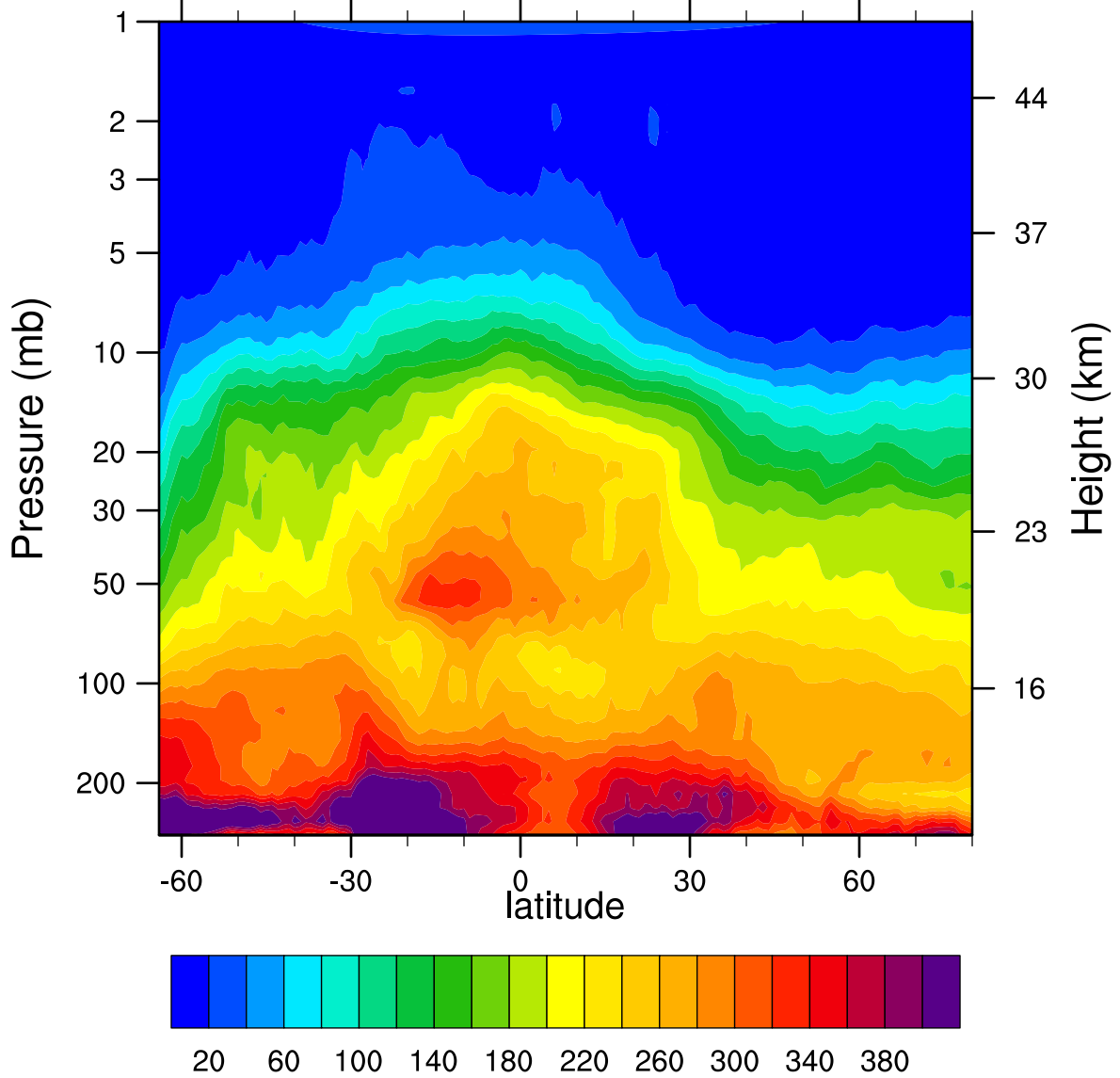
HIRDLSv6 2006d155 N2O_Combined (ppbv)
