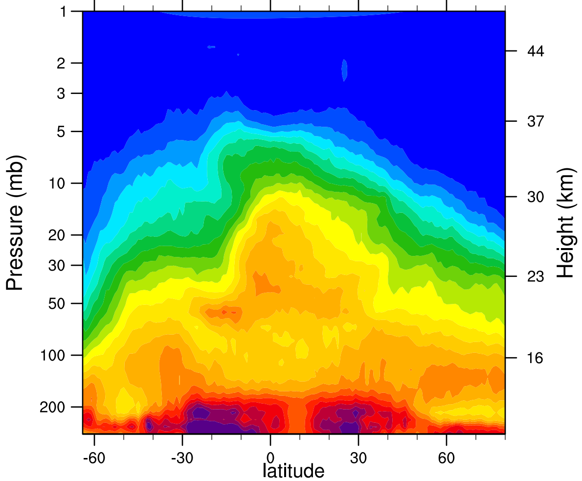
HIRDLSv6 2006d278 N2O_Combined (ppbv)
