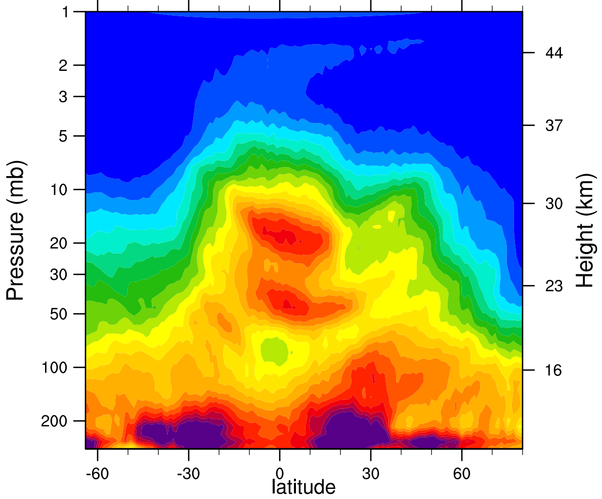
HIRDLSv6 2005d035 N2O_Combined (ppbv)
