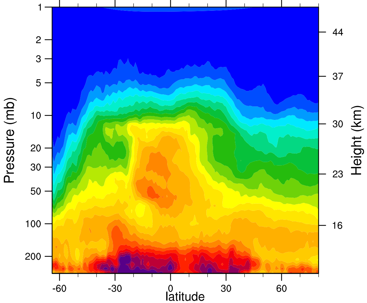
HIRDLSv6 2007d170 N2O_Combined (ppbv)
