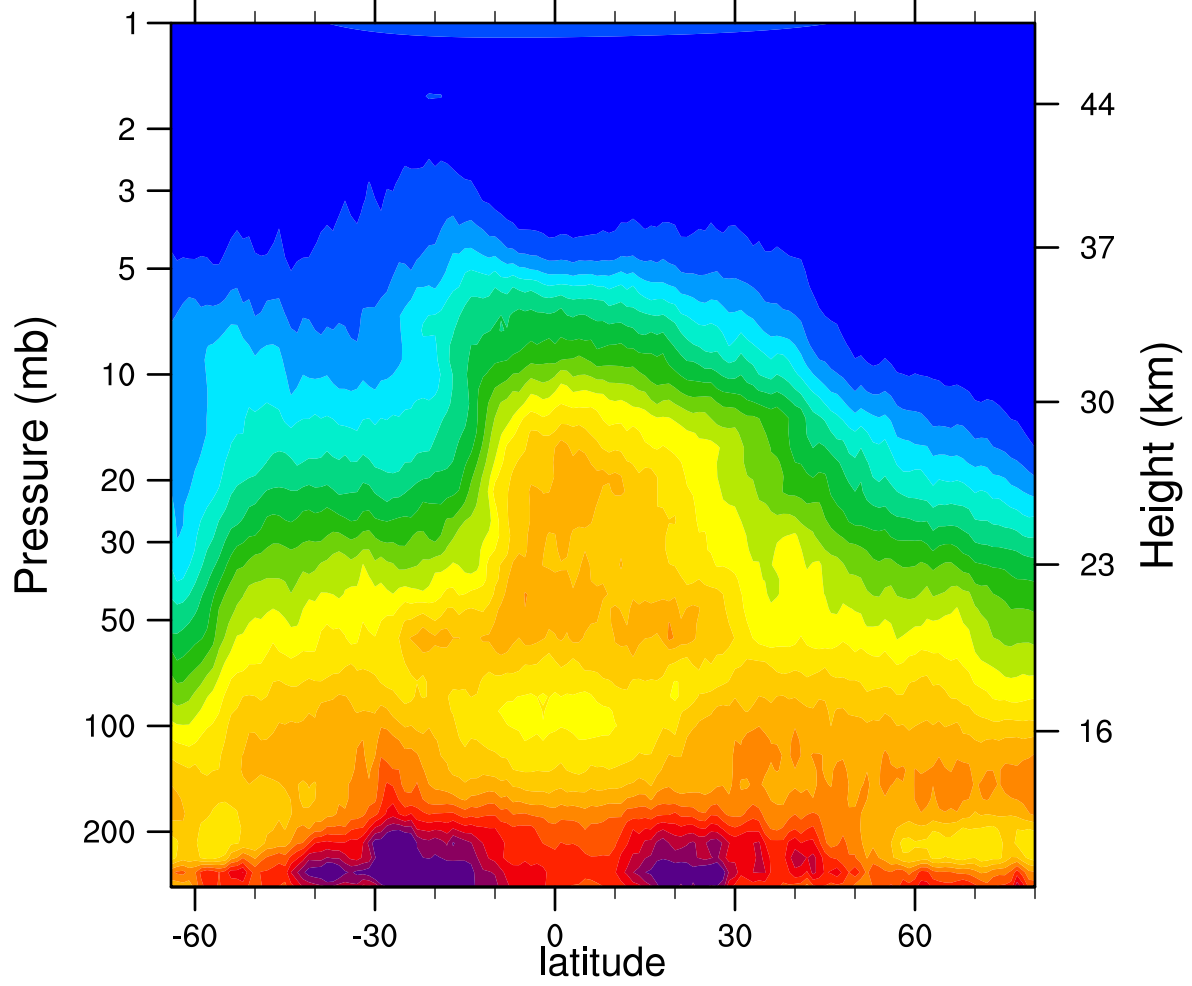
HIRDLSv6 2006d305 N2O_Combined (ppbv)
