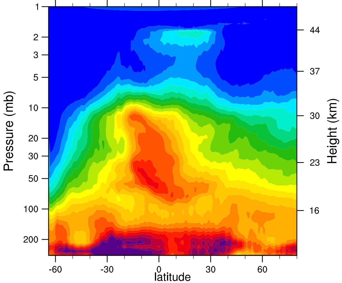
HIRDLSv6 2005d208 N2O_Combined (ppbv)
