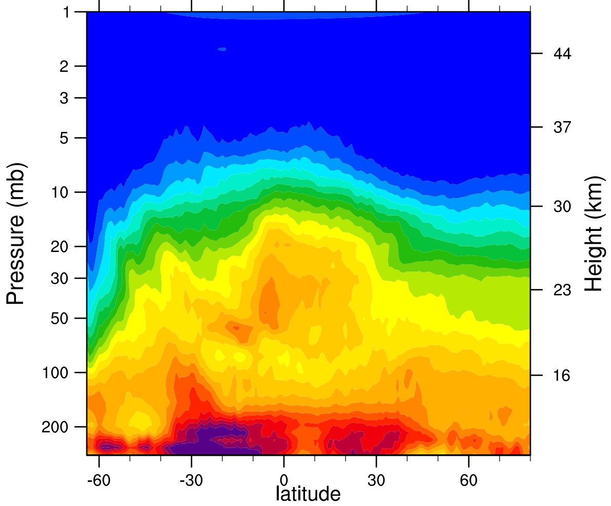
HIRDLSv6 2006d186 N2O_Combined (ppbv)
