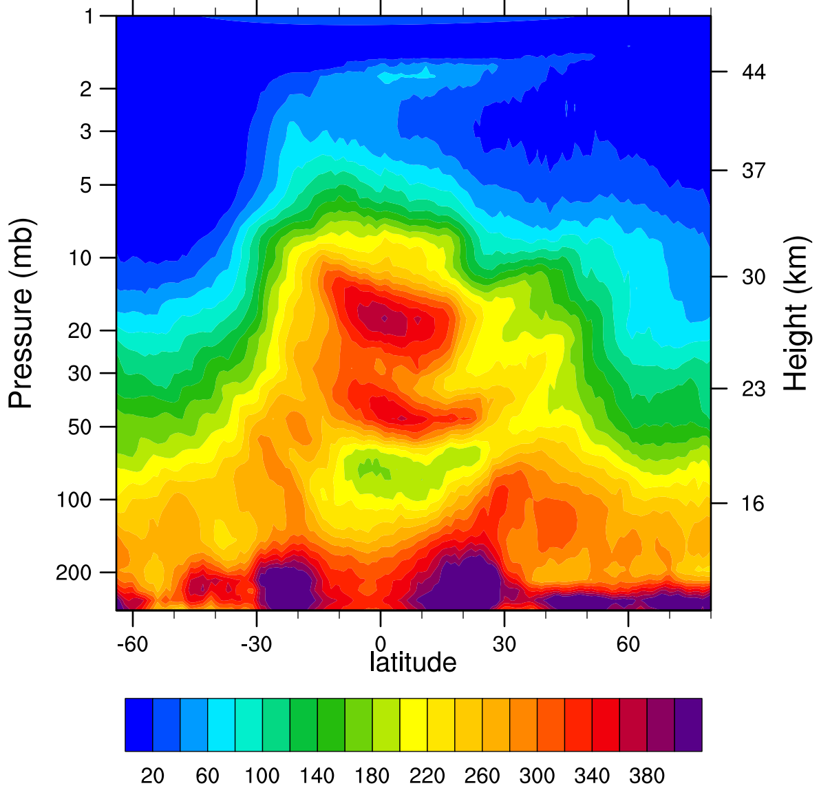
HIRDLSv6 2005d057 N2O_Combined (ppbv)
