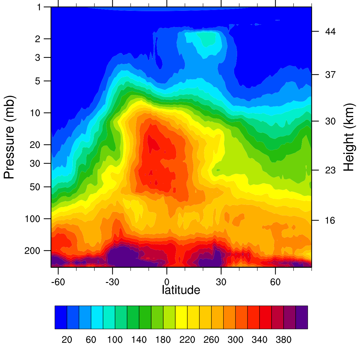
HIRDLSv6 2005d159 N2O_Combined (ppbv)
