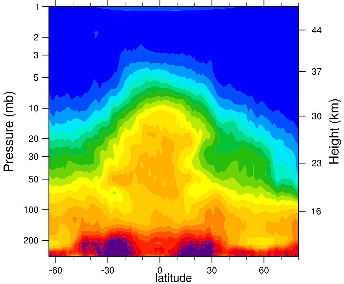
HIRDLSv6 2007d066 N2O_Combined (ppbv)
