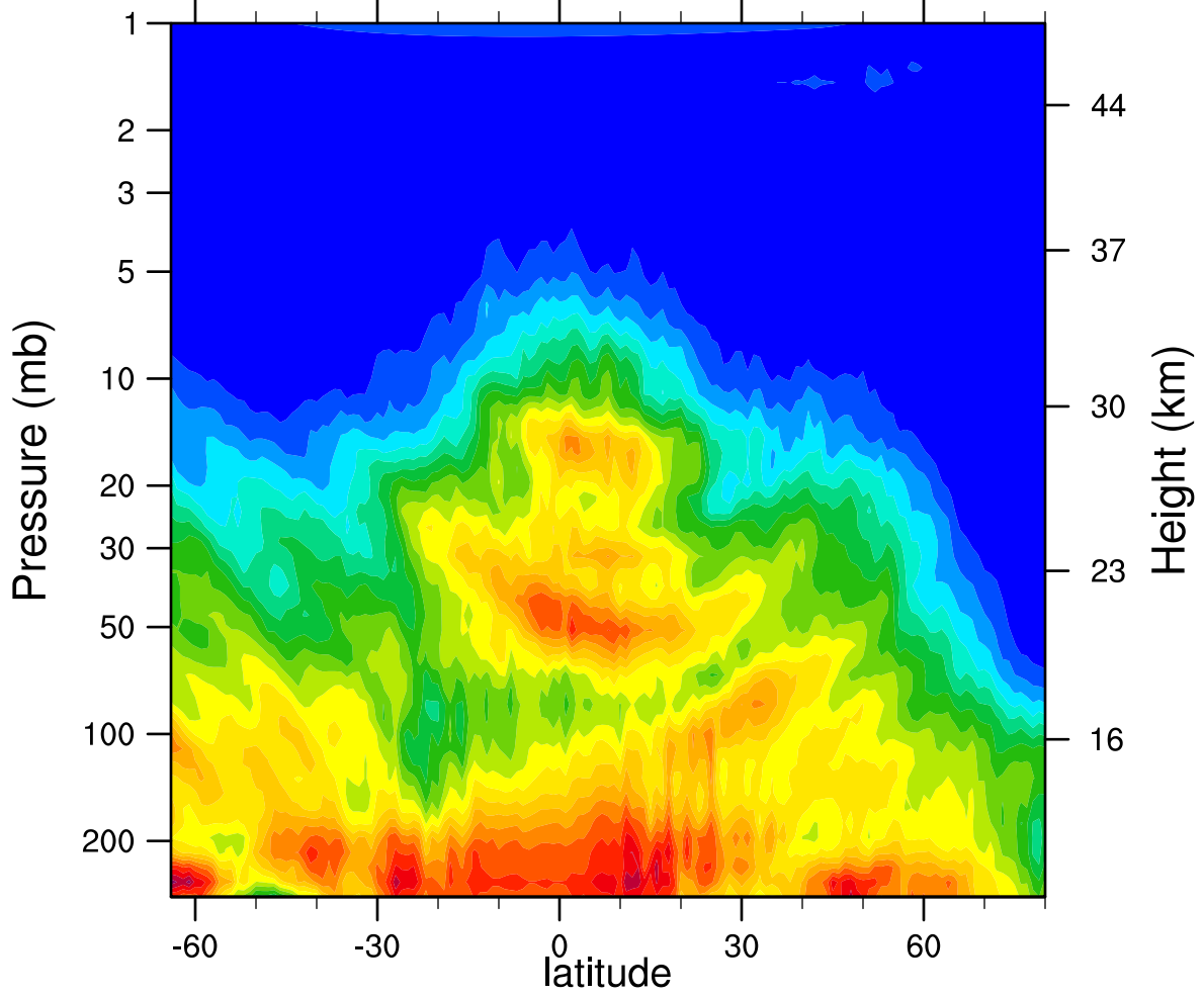
HIRDLSv6 2005d024 N2O_Combined (ppbv)
