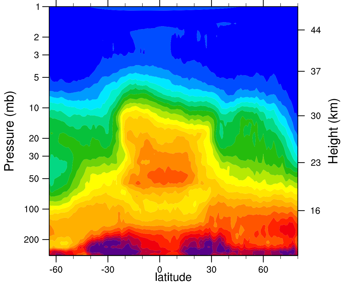
HIRDLSv6 2005d326 N2O_Combined (ppbv)
