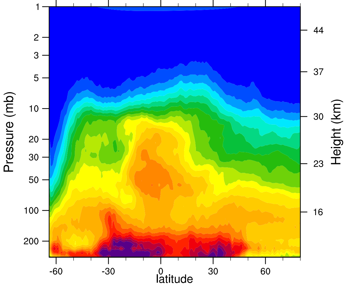
HIRDLSv6 2007d202 N2O_Combined (ppbv)
