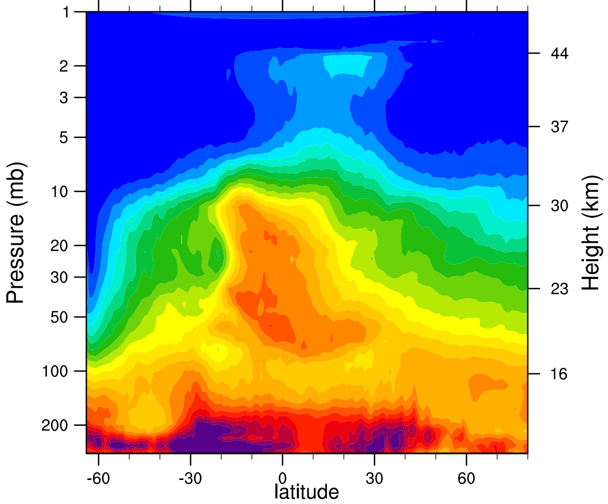
HIRDLSv6 2005d231 N2O_Combined (ppbv)
