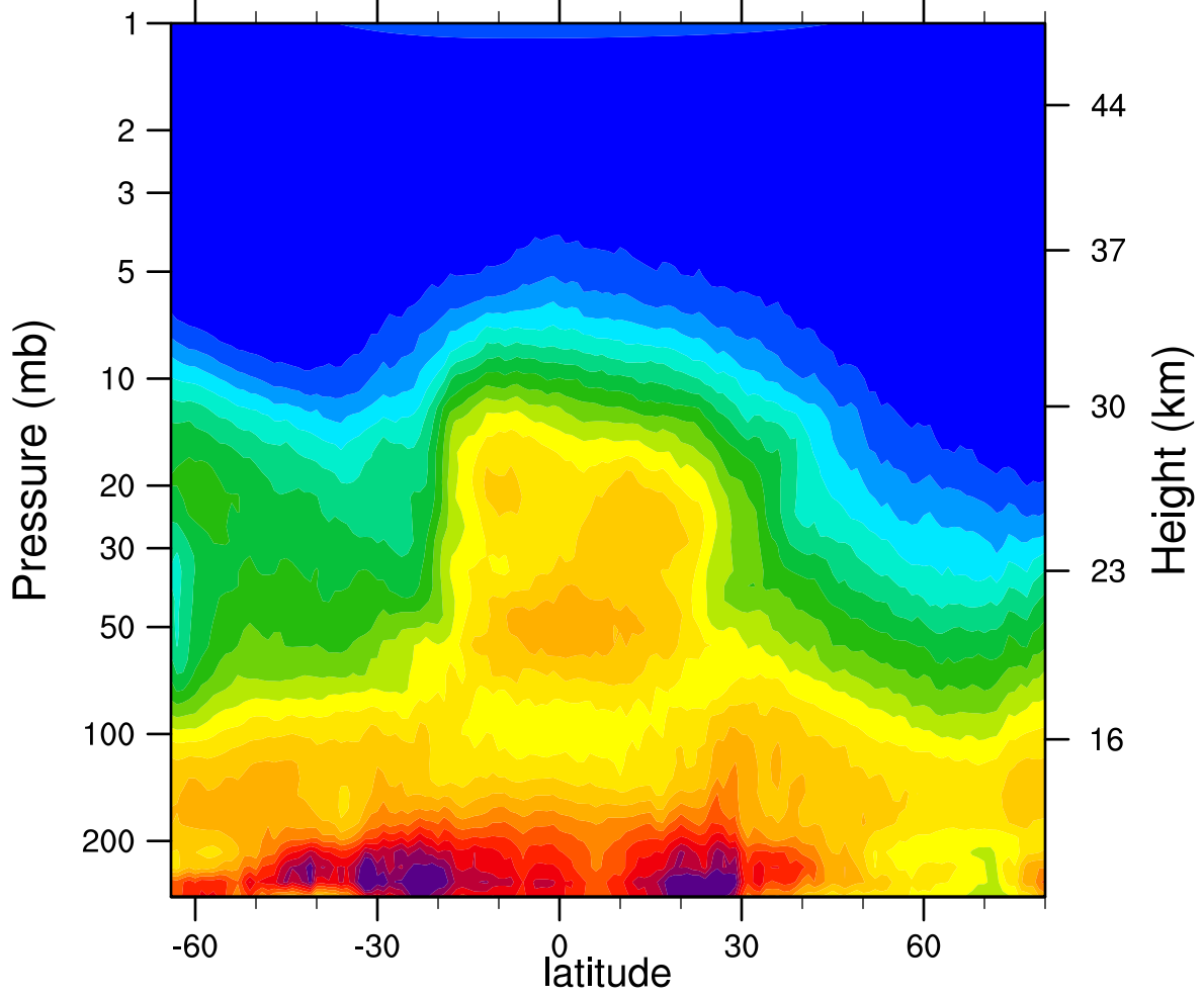
HIRDLSv6 2007d325 N2O_Combined (ppbv)
