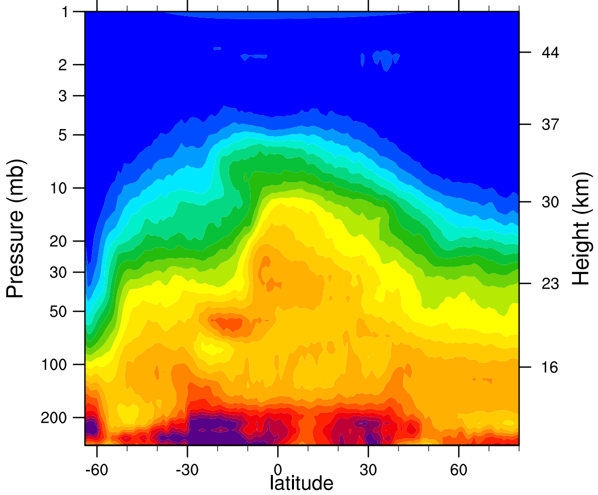
HIRDLSv6 2006d259 N2O_Combined (ppbv)
