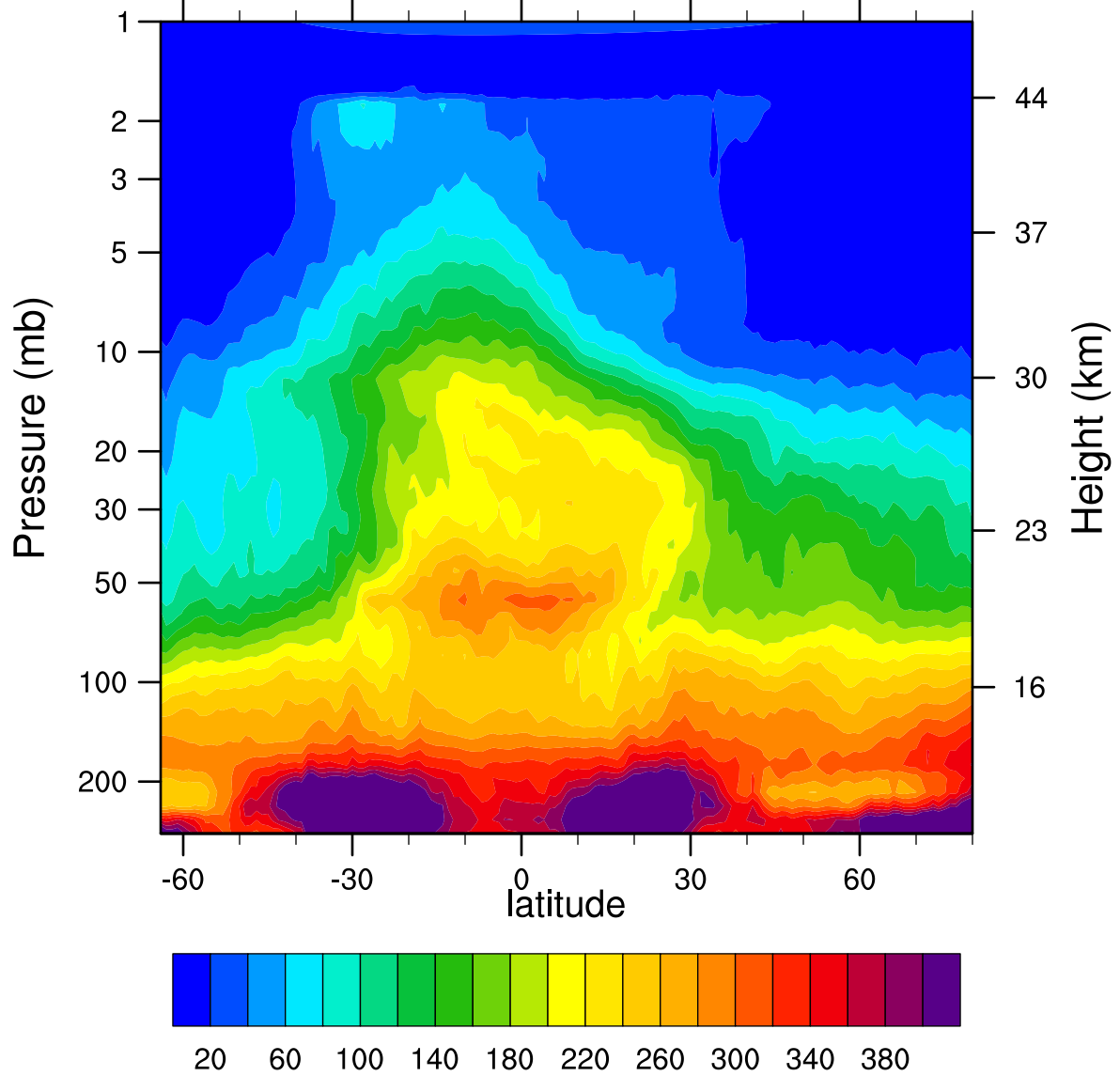
HIRDLSv6 2006d087 N2O_Combined (ppbv)
