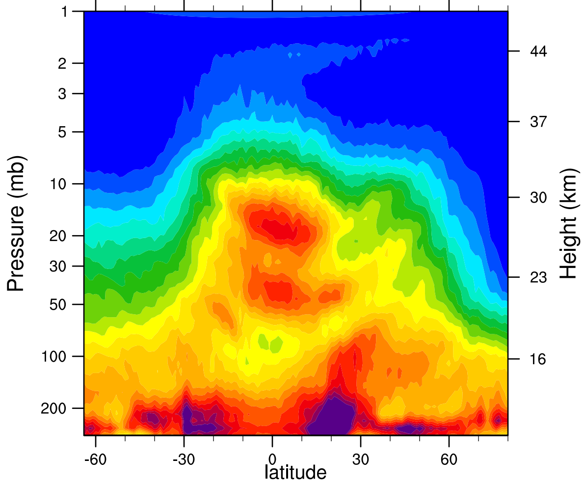
HIRDLSv6 2005d029 N2O_Combined (ppbv)
