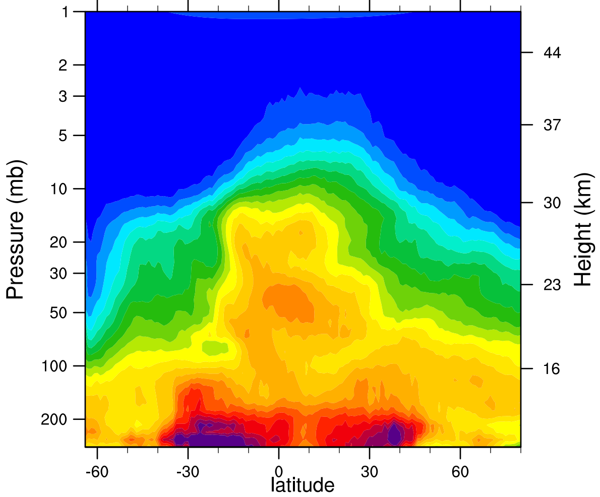
HIRDLSv6 2007d245 N2O_Combined (ppbv)
