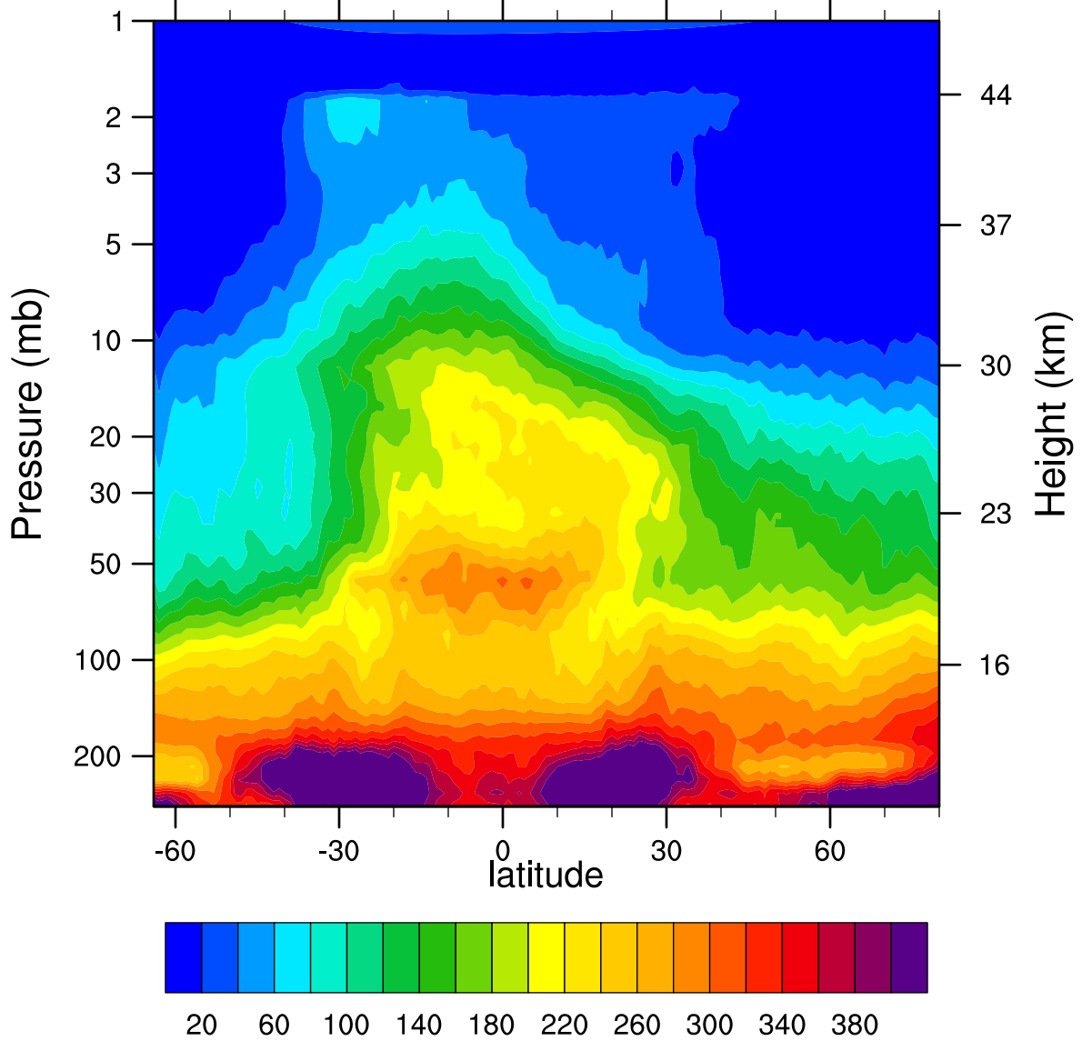
HIRDLSv6 2006d088 N2O_Combined (ppbv)
