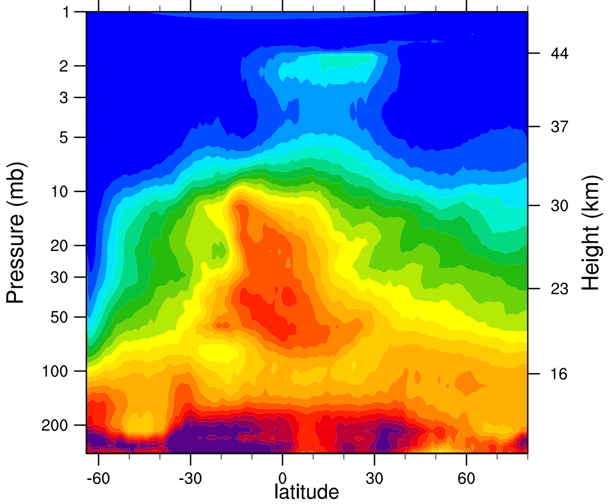
HIRDLSv6 2005d216 N2O_Combined (ppbv)
