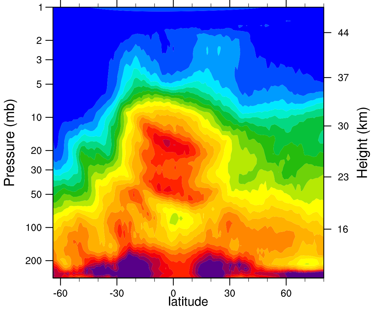
HIRDLSv6 2005d112 N2O_Combined (ppbv)
