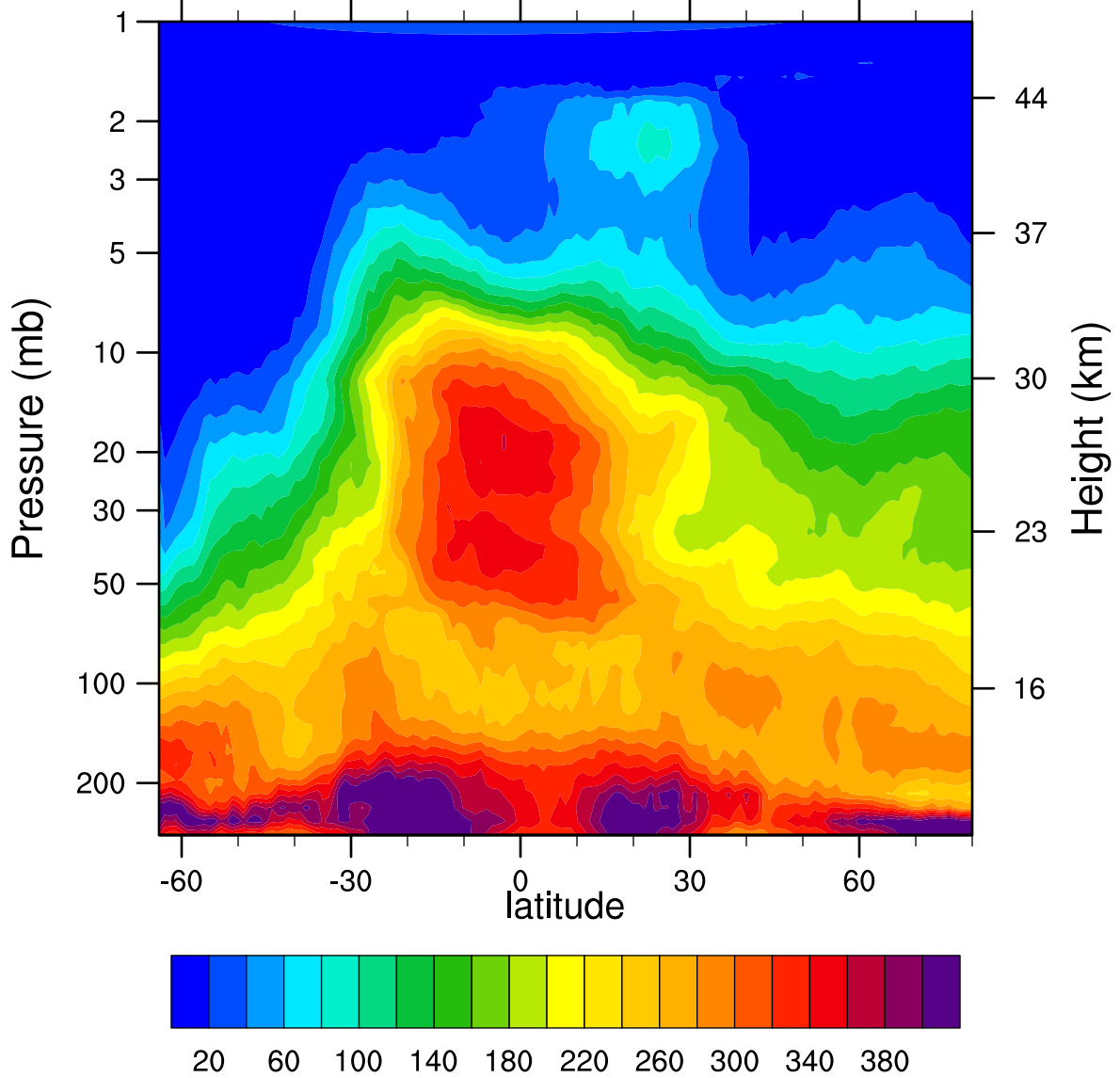
HIRDLSv6 2005d145 N2O_Combined (ppbv)
