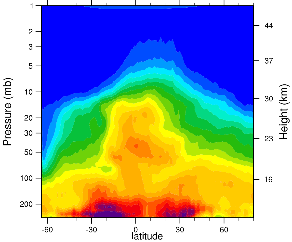
HIRDLSv6 2007d237 N2O_Combined (ppbv)
