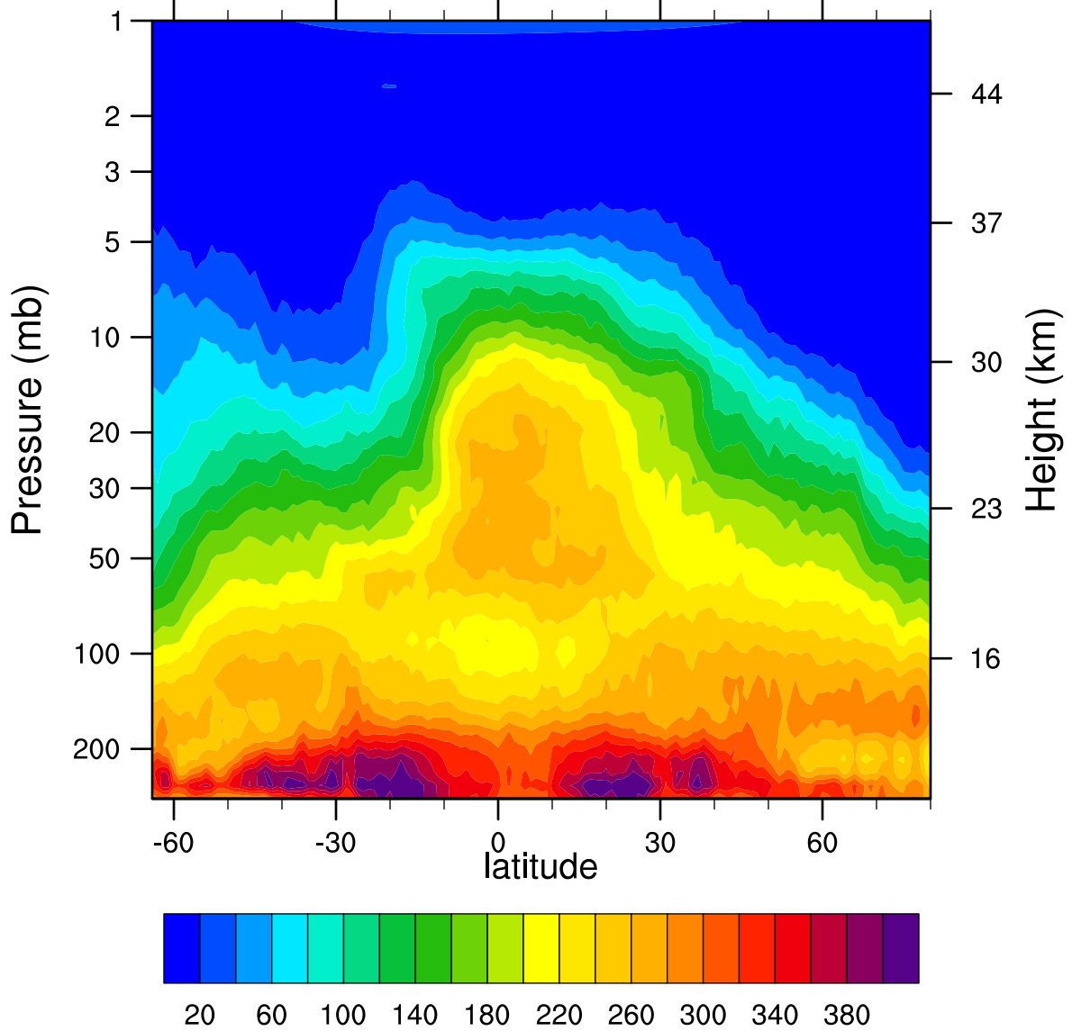
HIRDLSv6 2006d312 N2O_Combined (ppbv)
