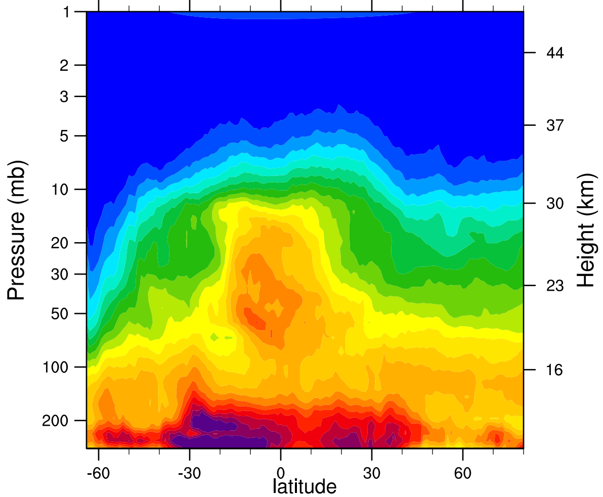
HIRDLSv6 2007d186 N2O_Combined (ppbv)
