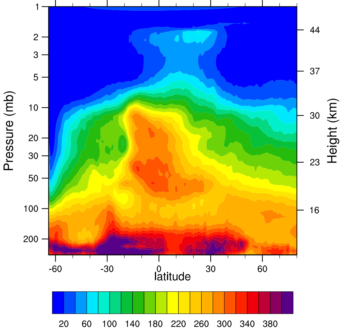
HIRDLSv6 2005d229 N2O_Combined (ppbv)
