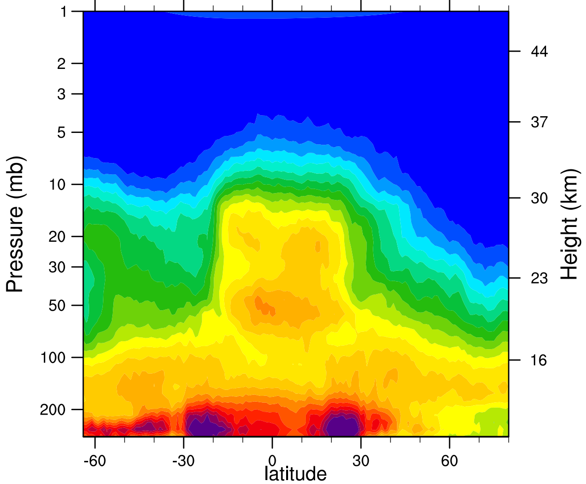
HIRDLSv6 2007d314 N2O_Combined (ppbv)
