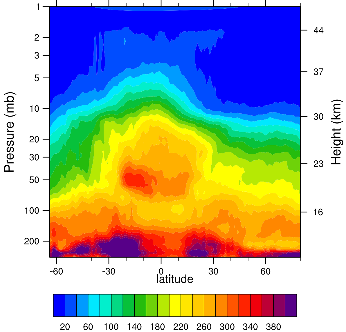
HIRDLSv6 2006d127 N2O_Combined (ppbv)
