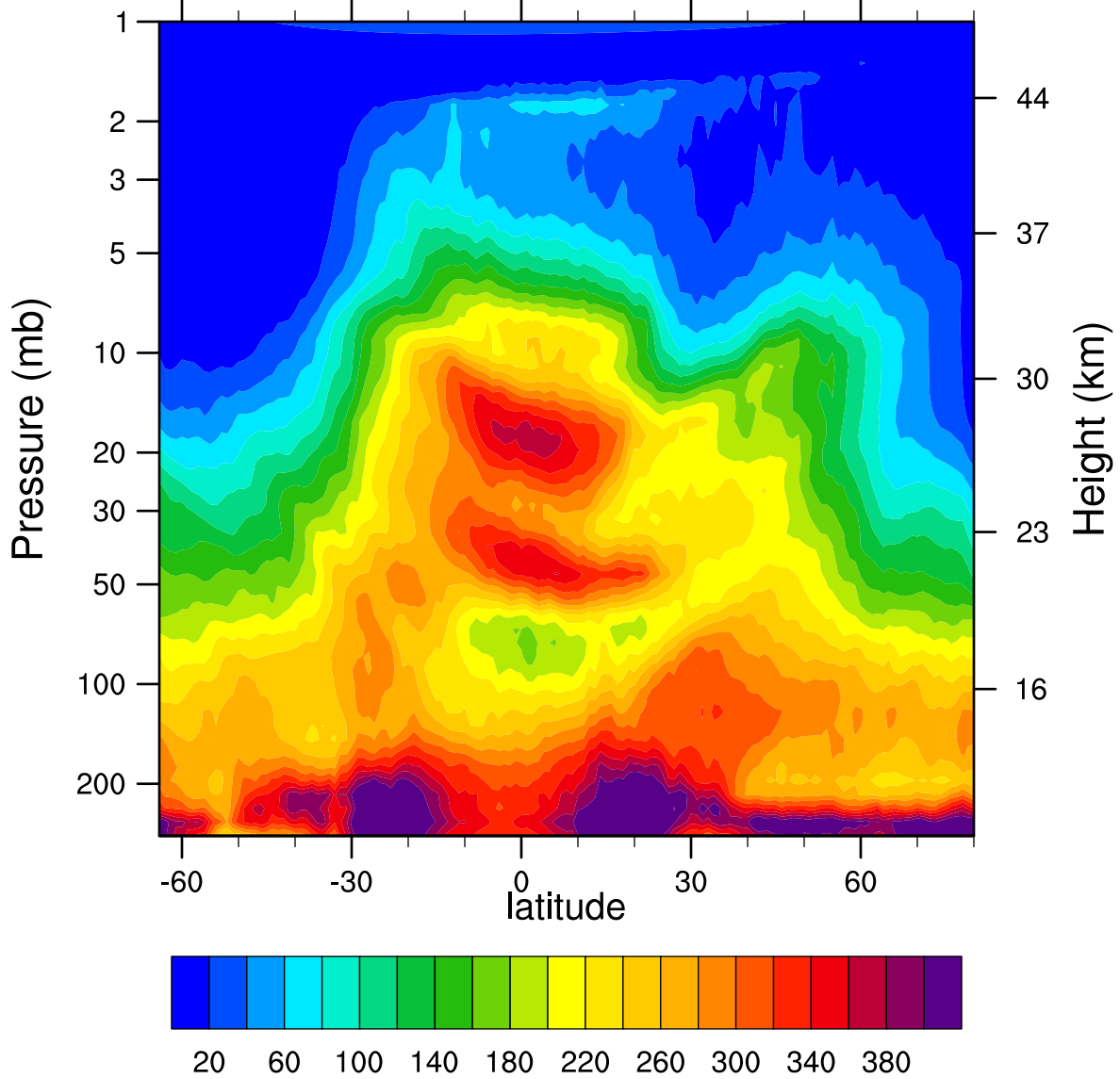
HIRDLSv6 2005d066 N2O_Combined (ppbv)
