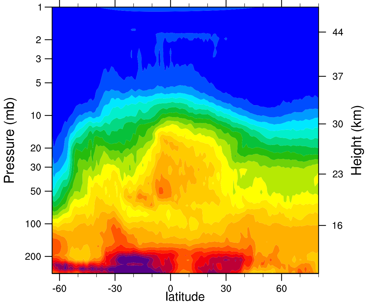
HIRDLSv6 2006d191 N2O_Combined (ppbv)
