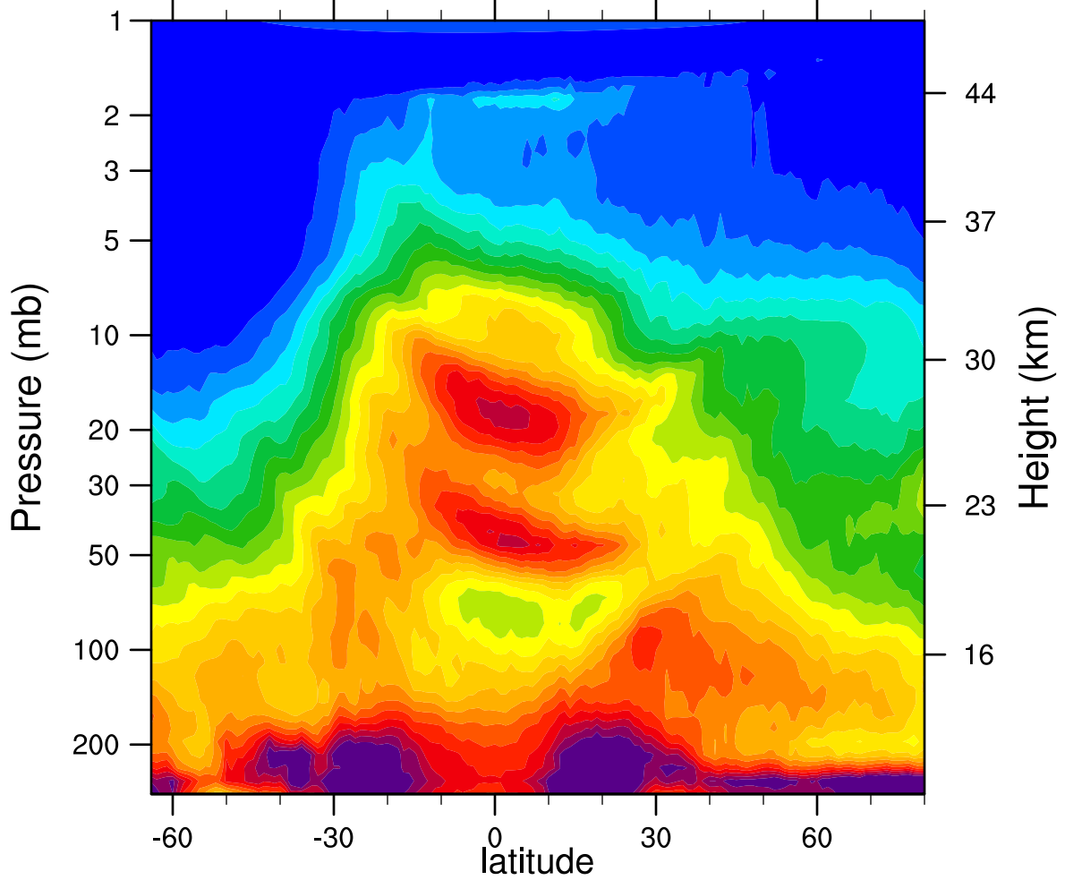
HIRDLSv6 2005d074 N2O_Combined (ppbv)
