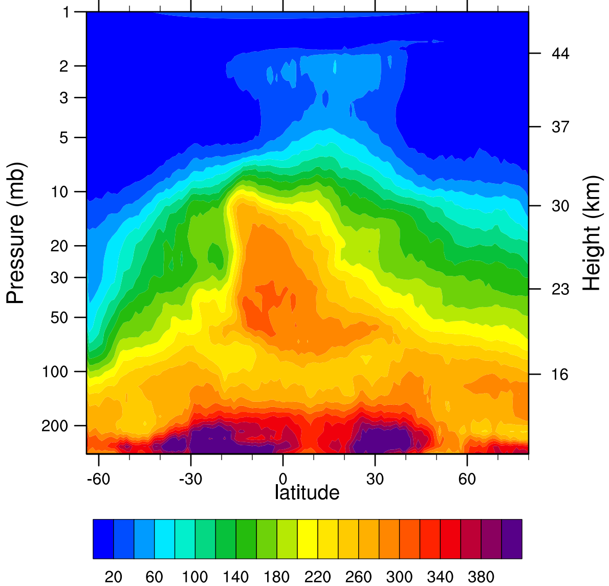
HIRDLSv6 2005d249 N2O_Combined (ppbv)
