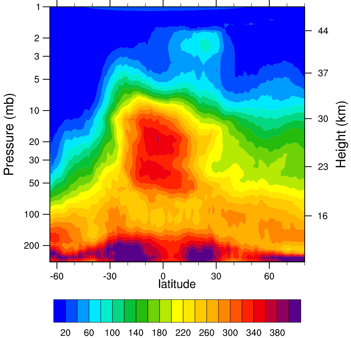
HIRDLSv6 2005d144 N2O_Combined (ppbv)
