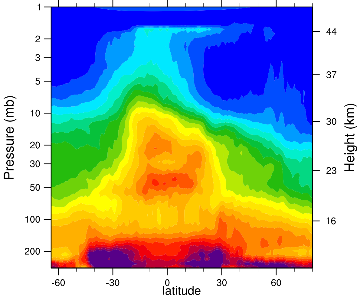
HIRDLSv6 2006d020 N2O_Combined (ppbv)
