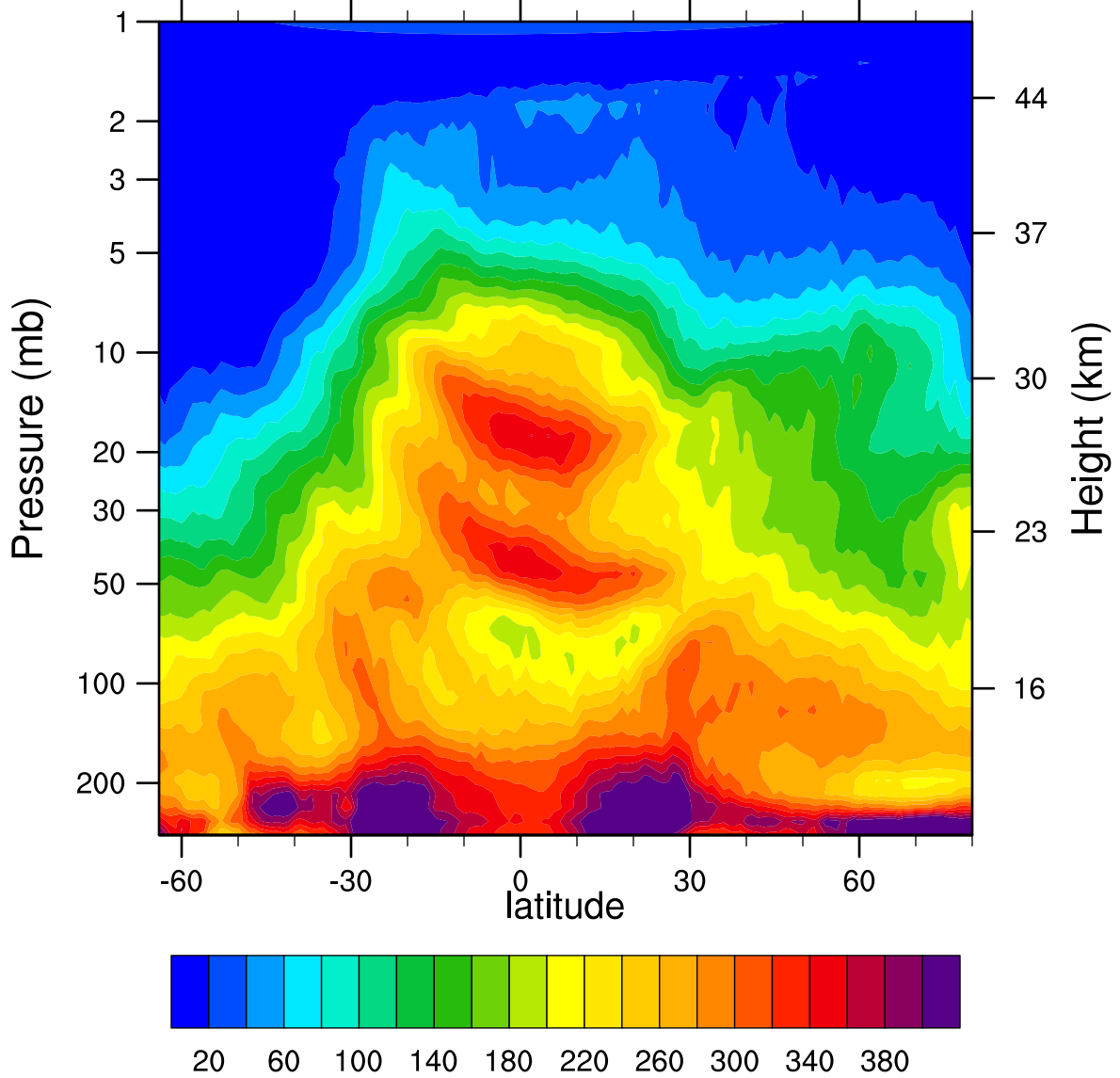
HIRDLSv6 2005d084 N2O_Combined (ppbv)
