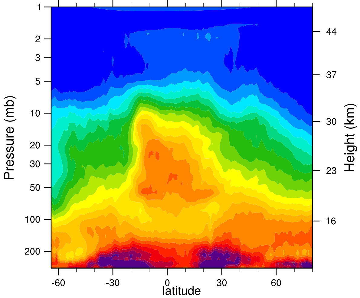
HIRDLSv6 2005d290 N2O_Combined (ppbv)
