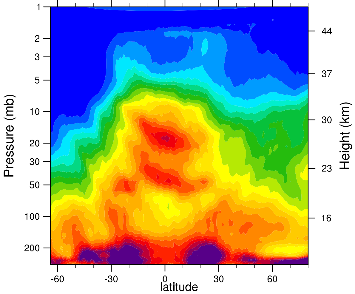
HIRDLSv6 2005d099 N2O_Combined (ppbv)
