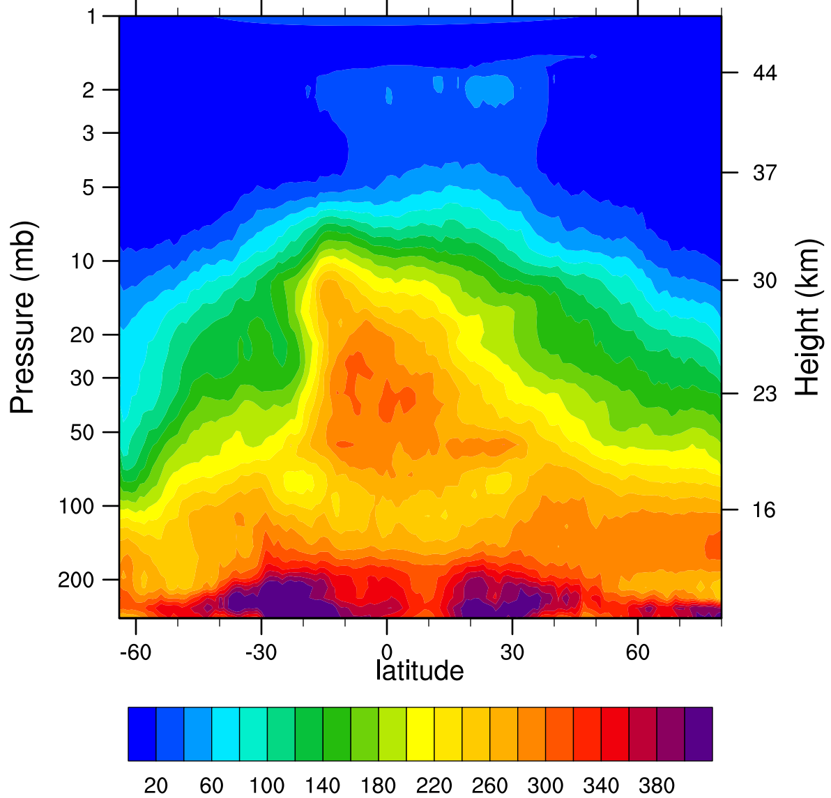
HIRDLSv6 2005d279 N2O_Combined (ppbv)
