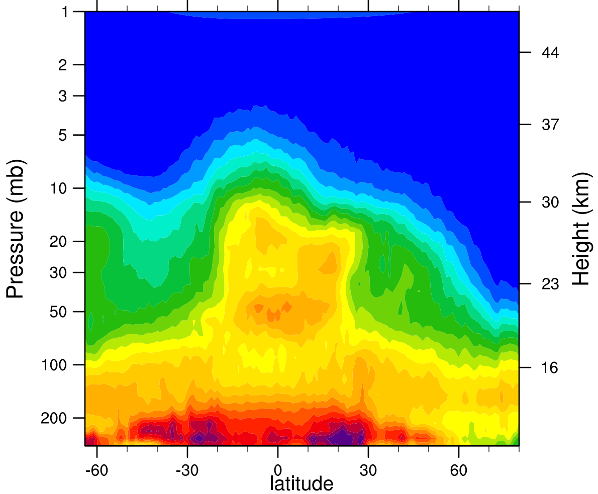
HIRDLSv6 2007d361 N2O_Combined (ppbv)
