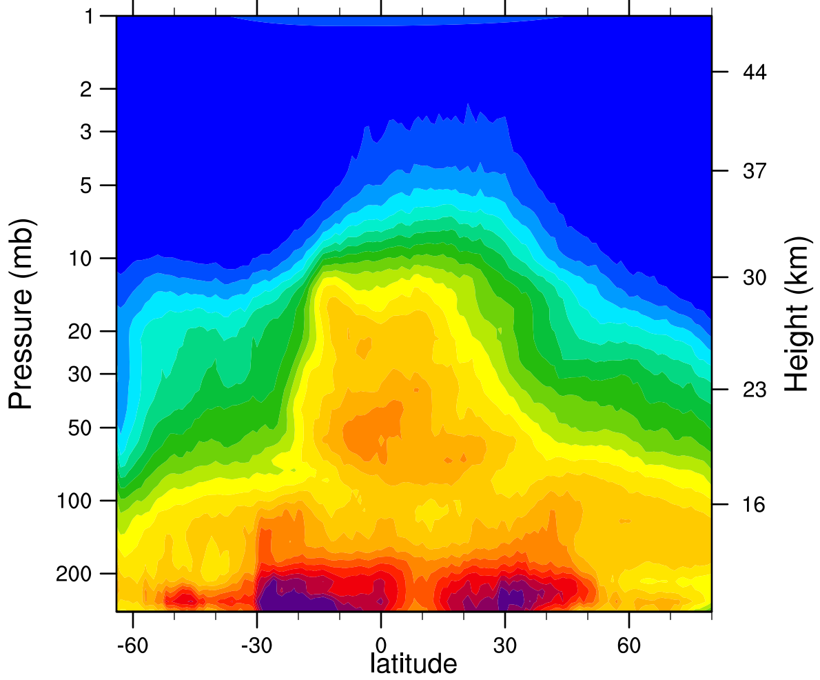
HIRDLSv6 2007d258 N2O_Combined (ppbv)
