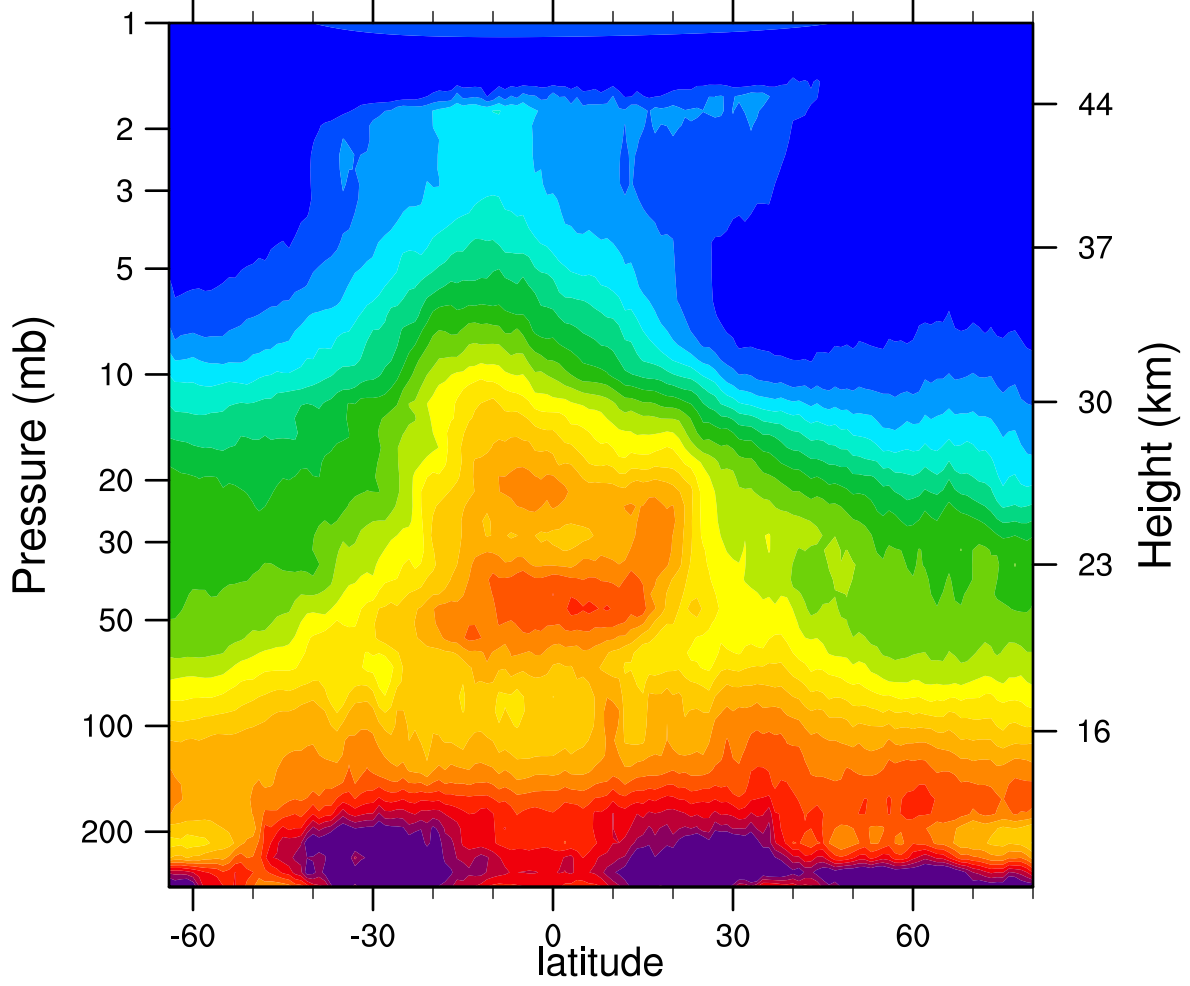
HIRDLSv6 2006d037 N2O_Combined (ppbv)
