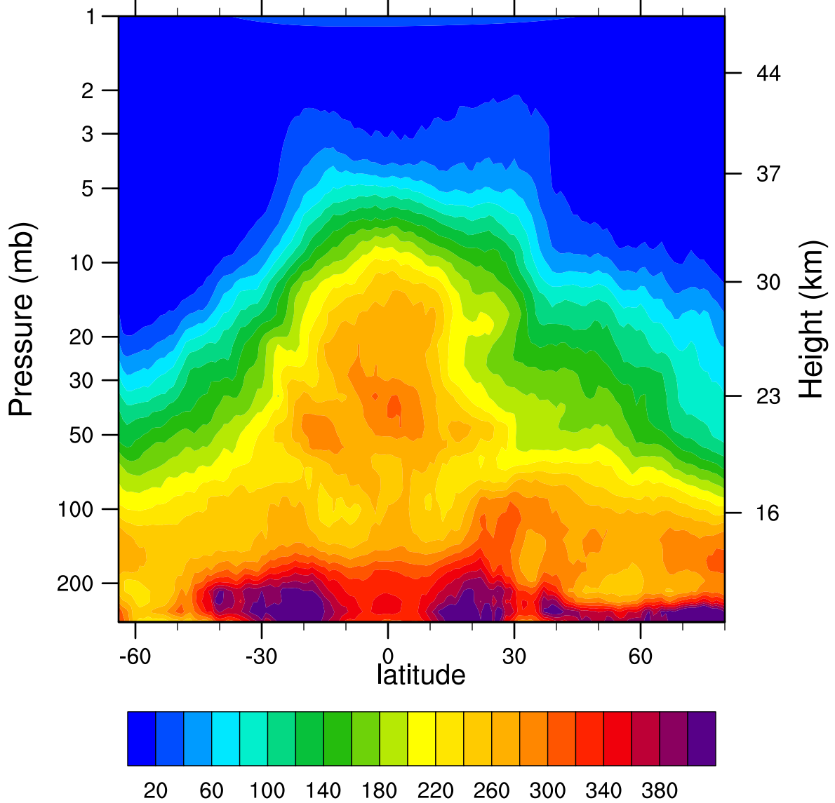
HIRDLSv6 2007d100 N2O_Combined (ppbv)
