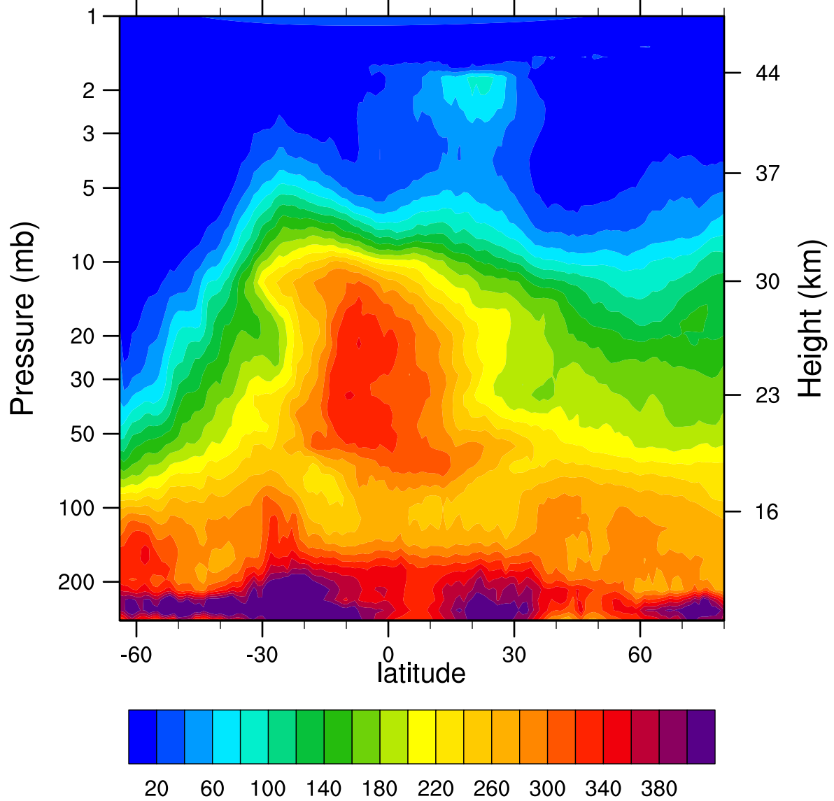
HIRDLSv6 2005d170 N2O_Combined (ppbv)
