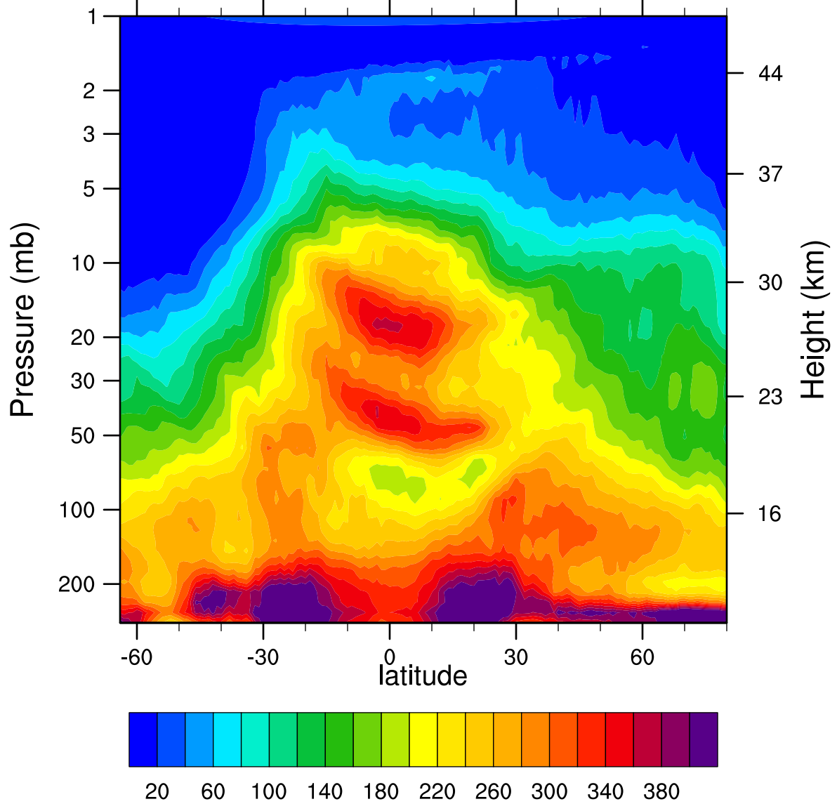
HIRDLSv6 2005d079 N2O_Combined (ppbv)
