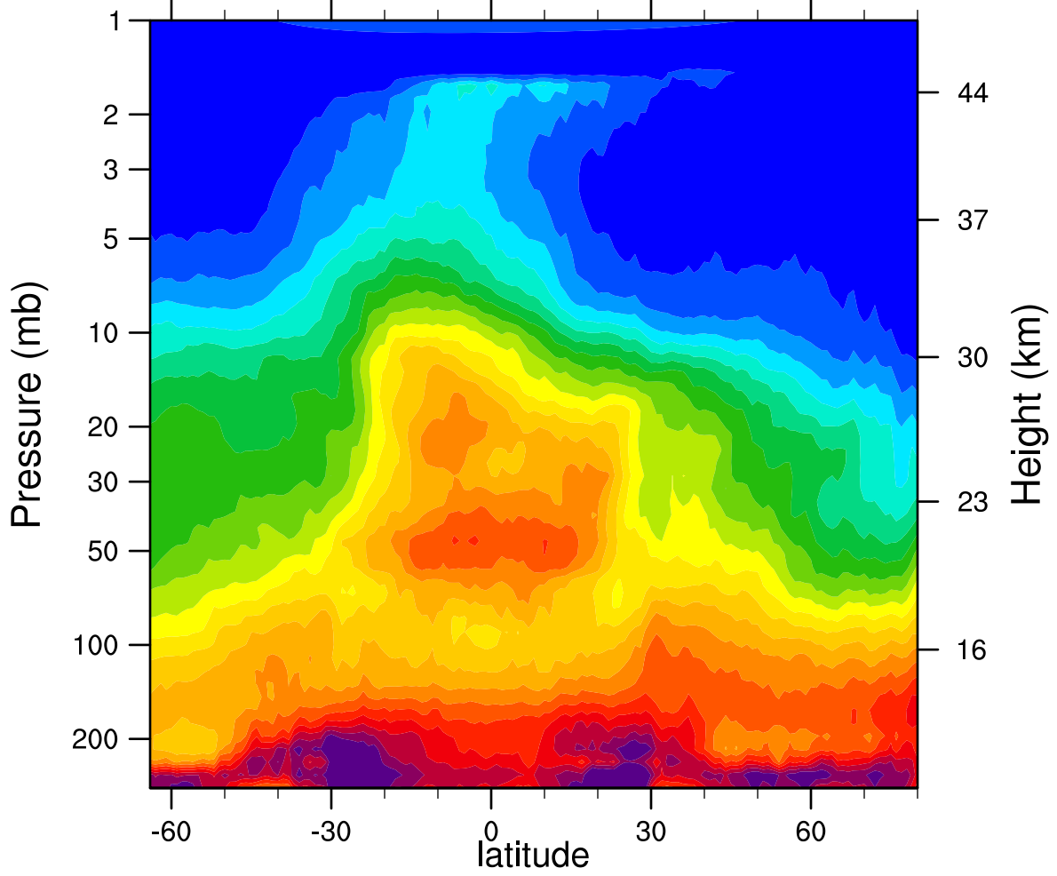
HIRDLSv6 2005d365 N2O_Combined (ppbv)
