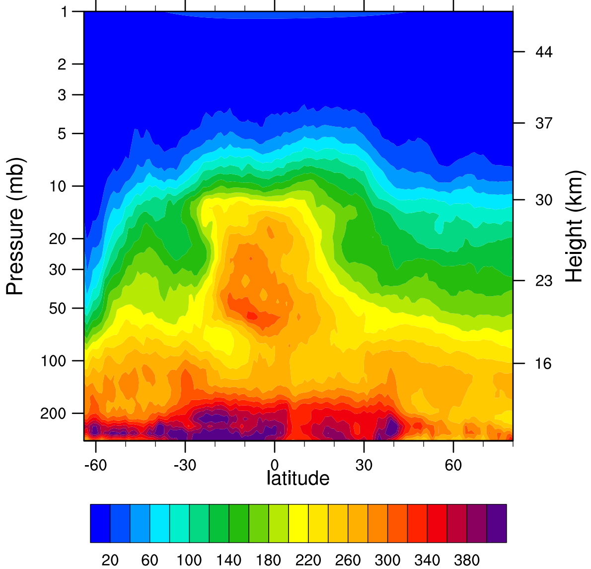
HIRDLSv6 2007d175 N2O_Combined (ppbv)
