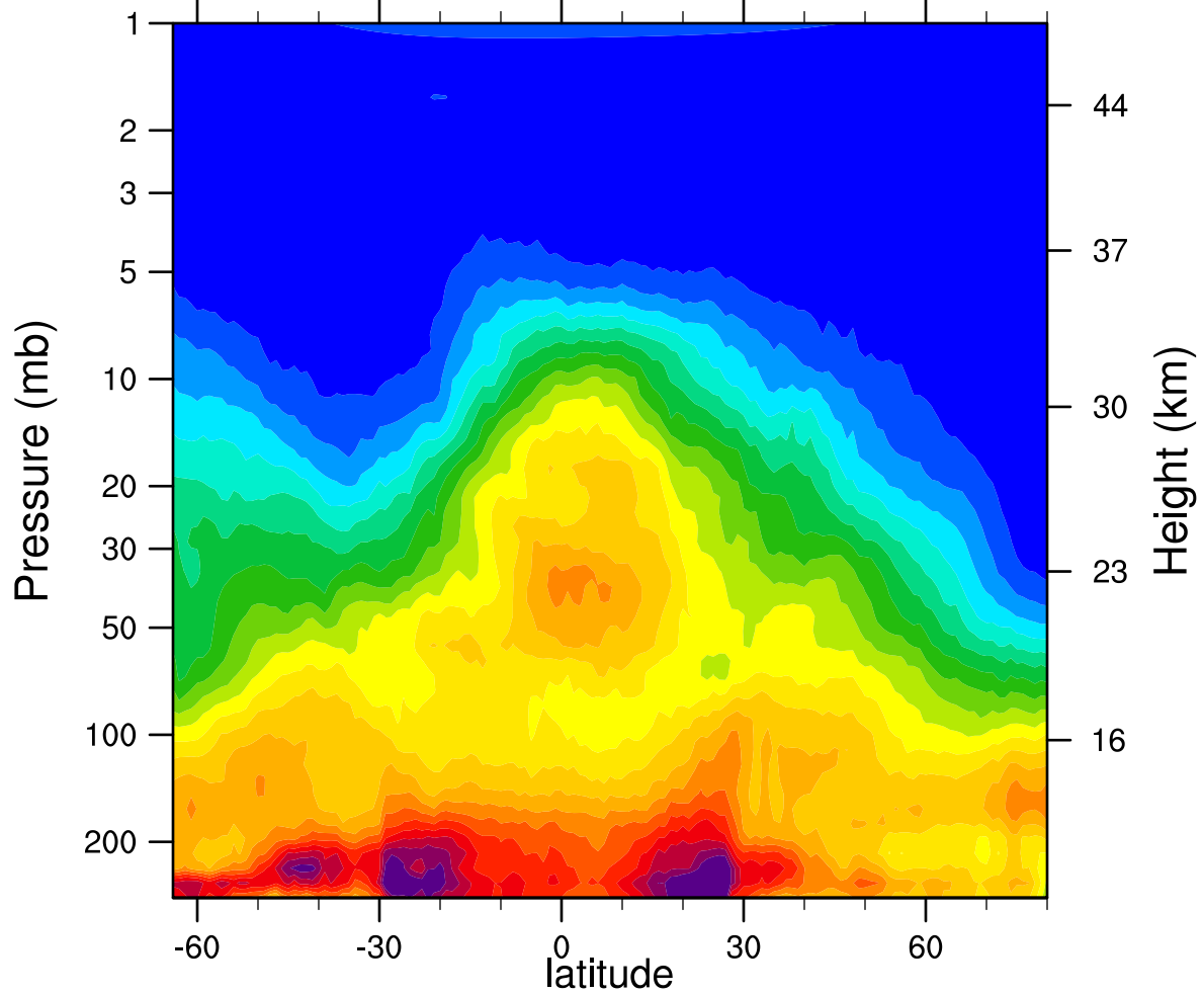
HIRDLSv6 2006d350 N2O_Combined (ppbv)
