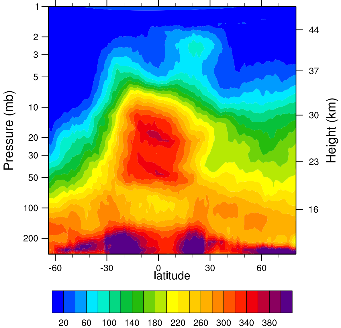
HIRDLSv6 2005d120 N2O_Combined (ppbv)
