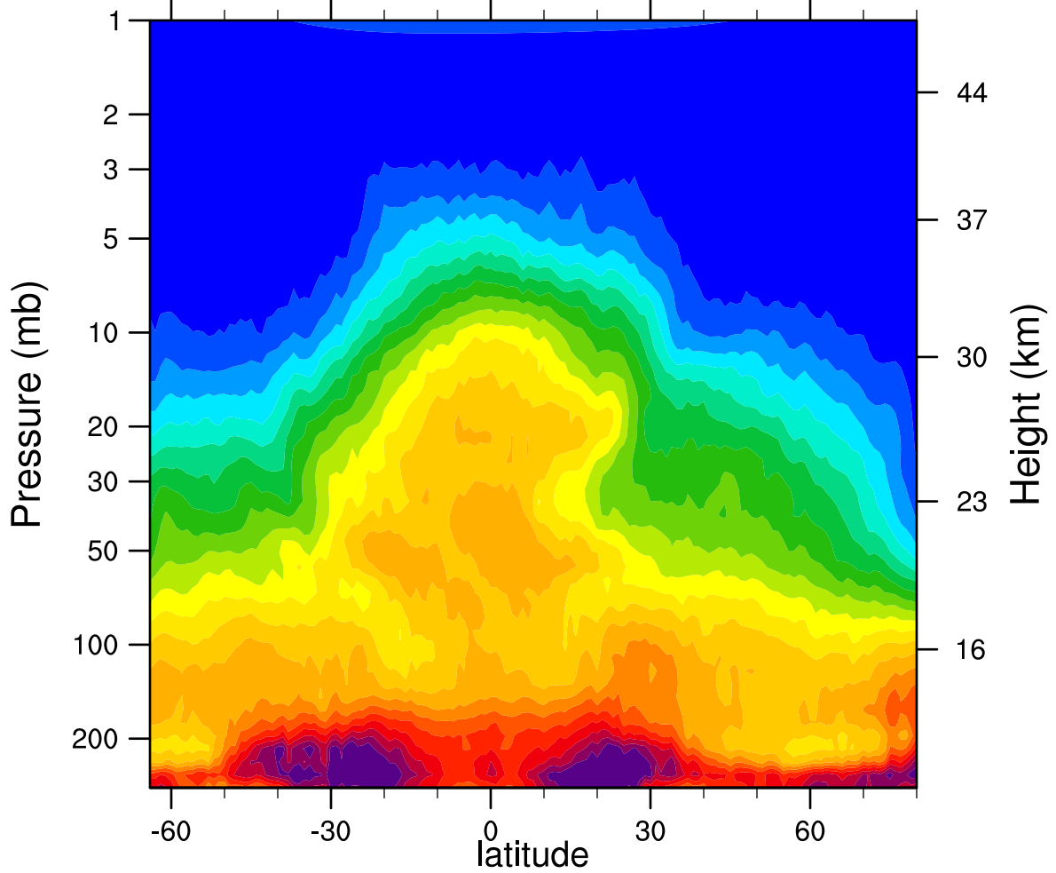
HIRDLSv6 2007d076 N2O_Combined (ppbv)
