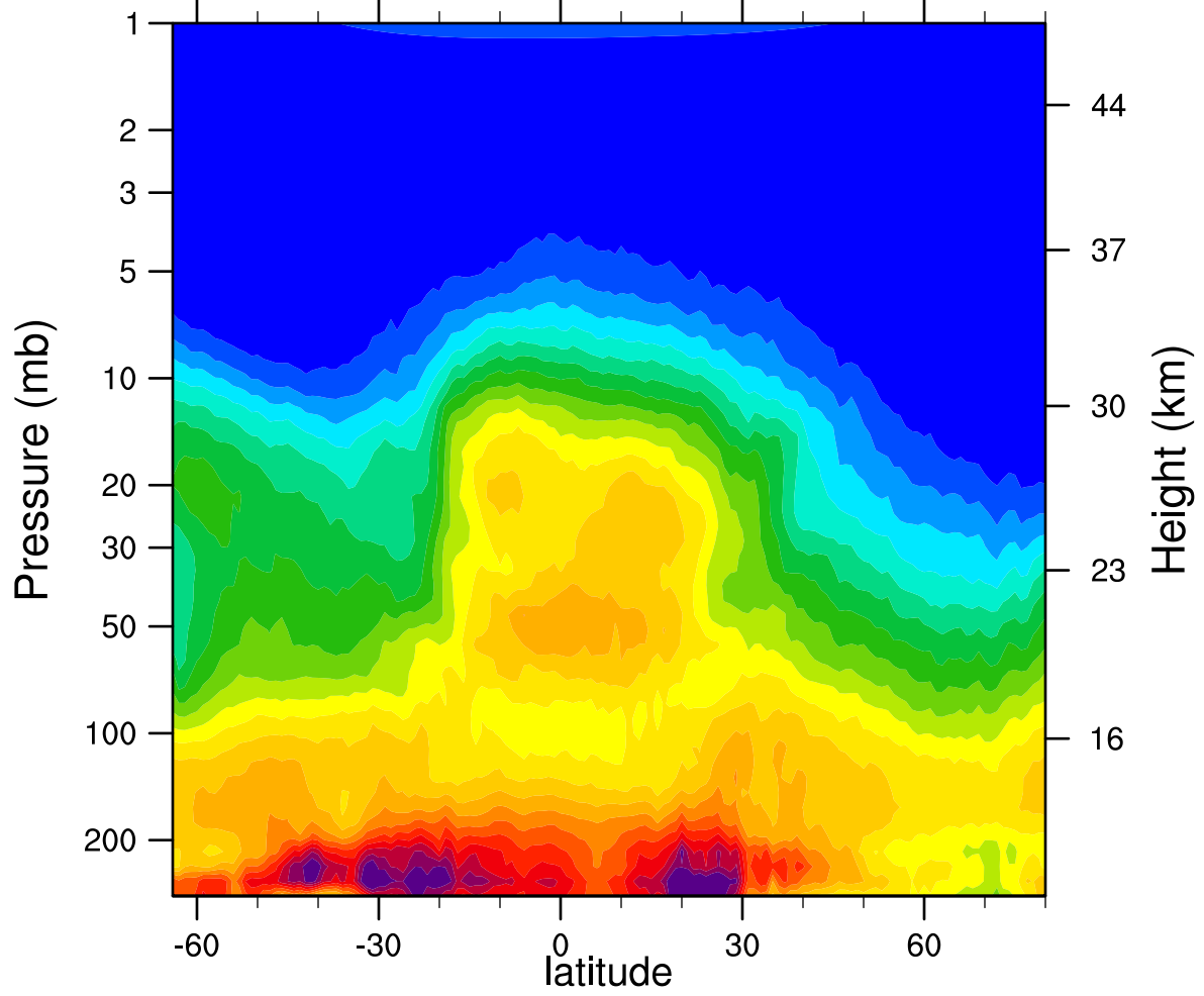
HIRDLSv6 2007d324 N2O_Combined (ppbv)
