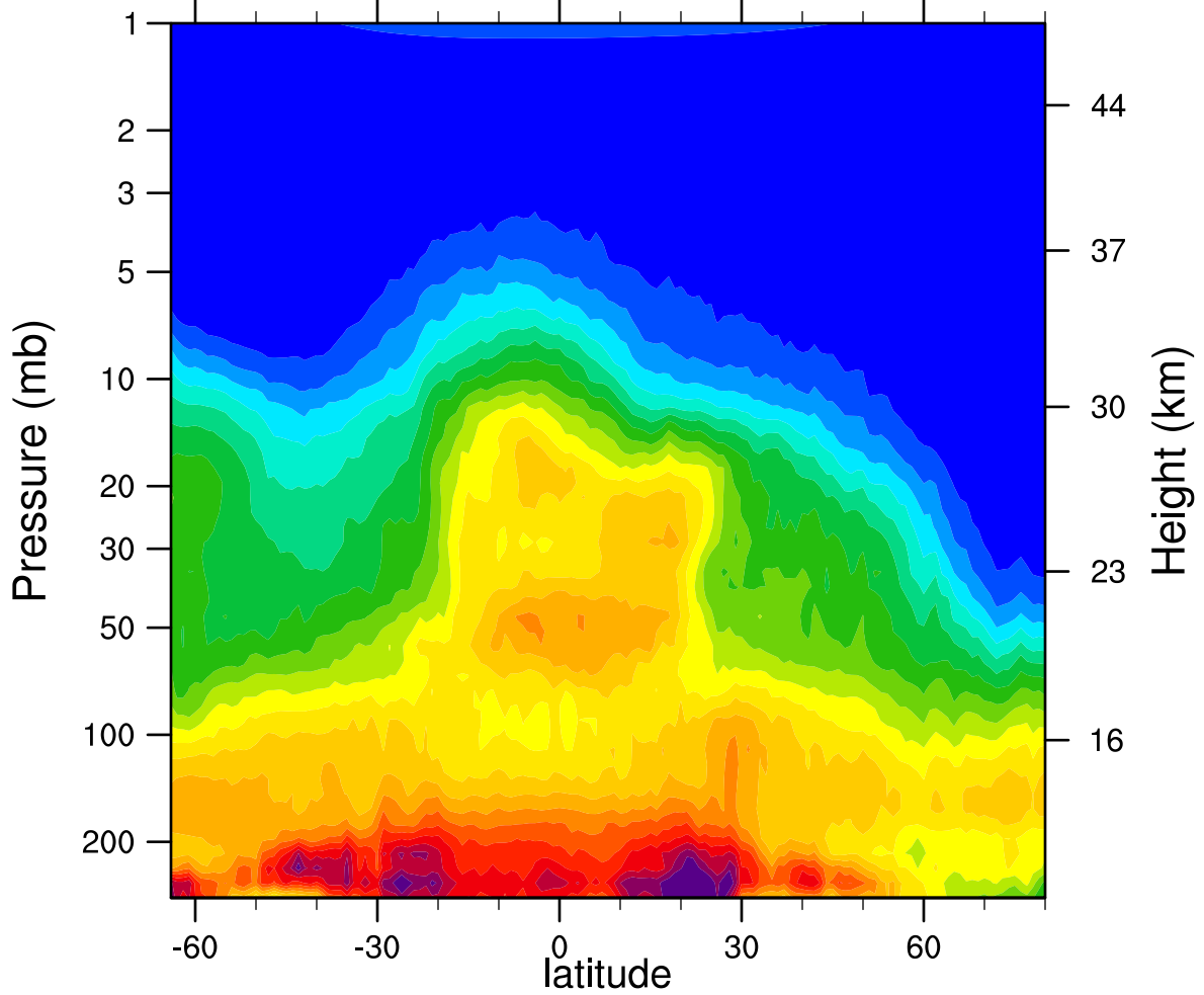
HIRDLSv6 2007d360 N2O_Combined (ppbv)
