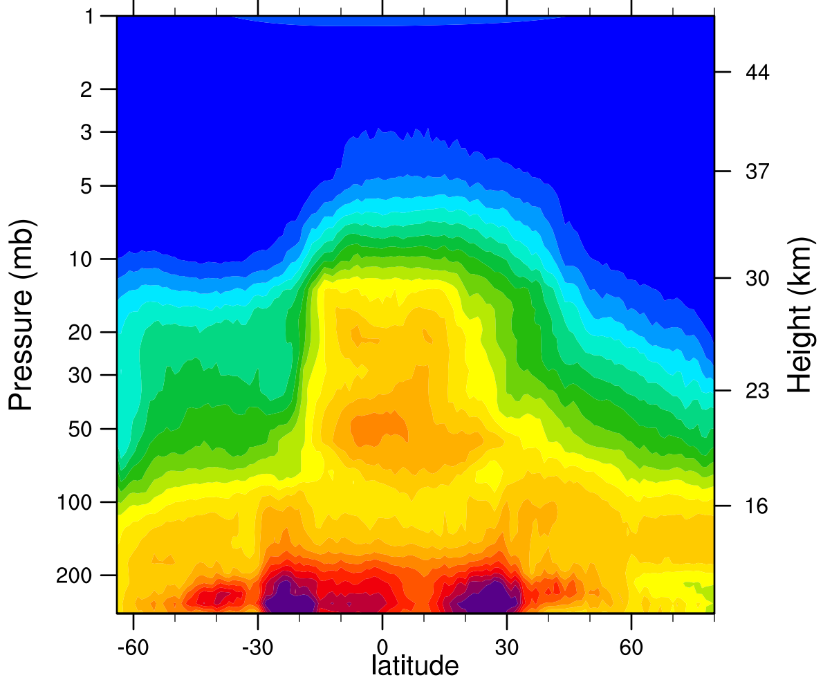
HIRDLSv6 2007d287 N2O_Combined (ppbv)
