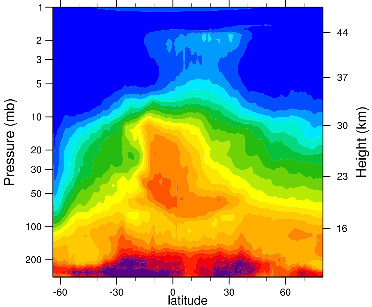
HIRDLSv6 2005d241 N2O_Combined (ppbv)
