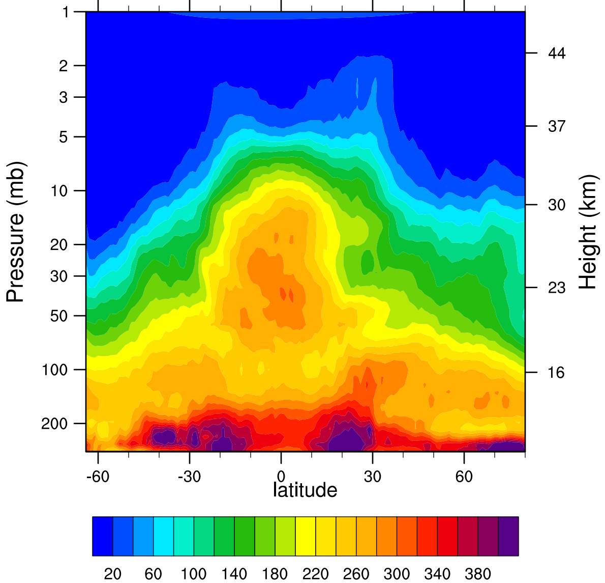
HIRDLSv6 2007d111 N2O_Combined (ppbv)
