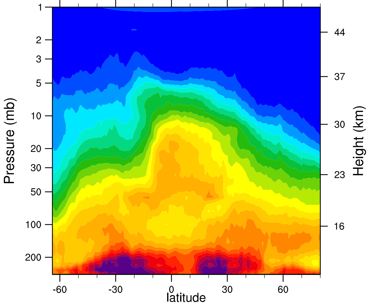
HIRDLSv6 2006d295 N2O_Combined (ppbv)
