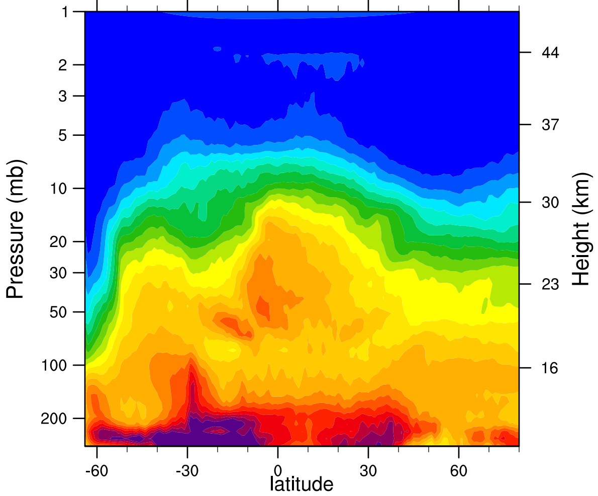
HIRDLSv6 2006d211 N2O_Combined (ppbv)
