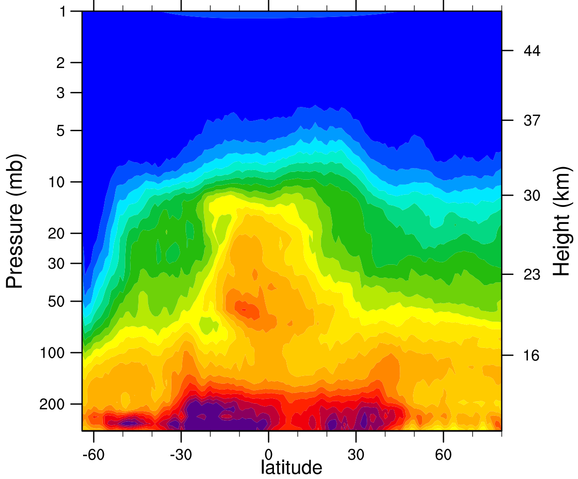
HIRDLSv6 2007d193 N2O_Combined (ppbv)
