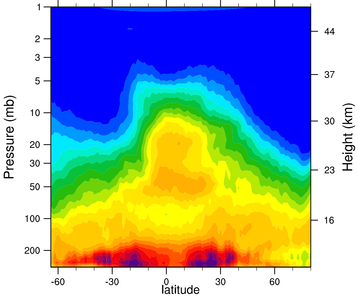
HIRDLSv6 2006d318 N2O_Combined (ppbv)
