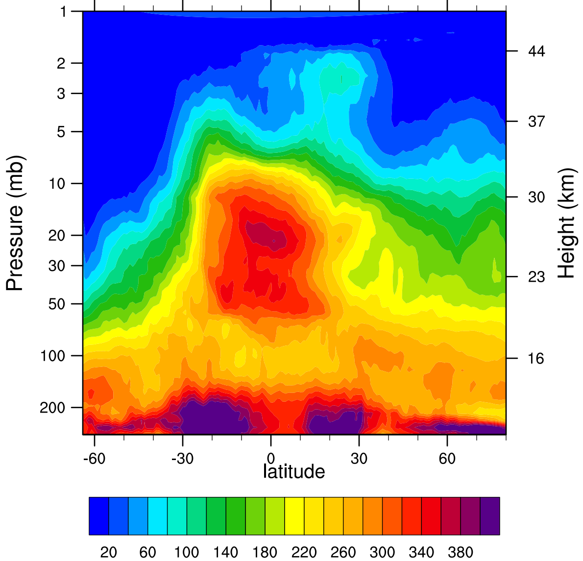
HIRDLSv6 2005d135 N2O_Combined (ppbv)
