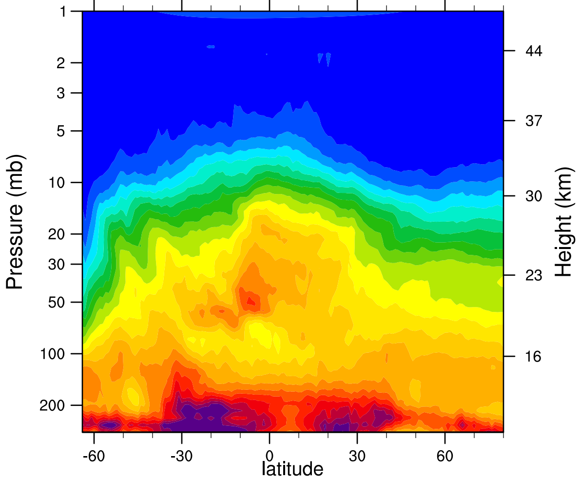
HIRDLSv6 2006d177 N2O_Combined (ppbv)
