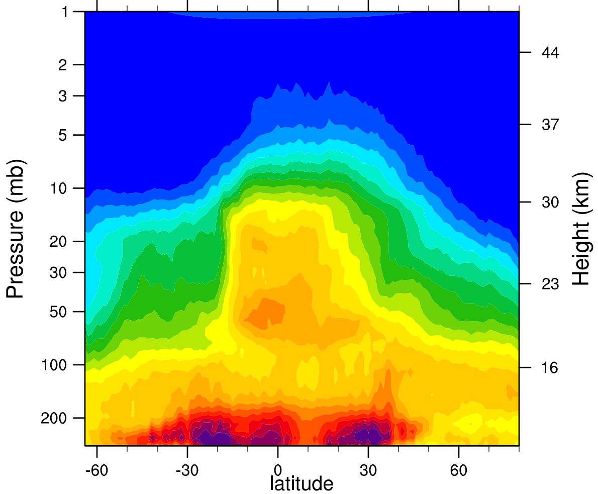
HIRDLSv6 2007d276 N2O_Combined (ppbv)
