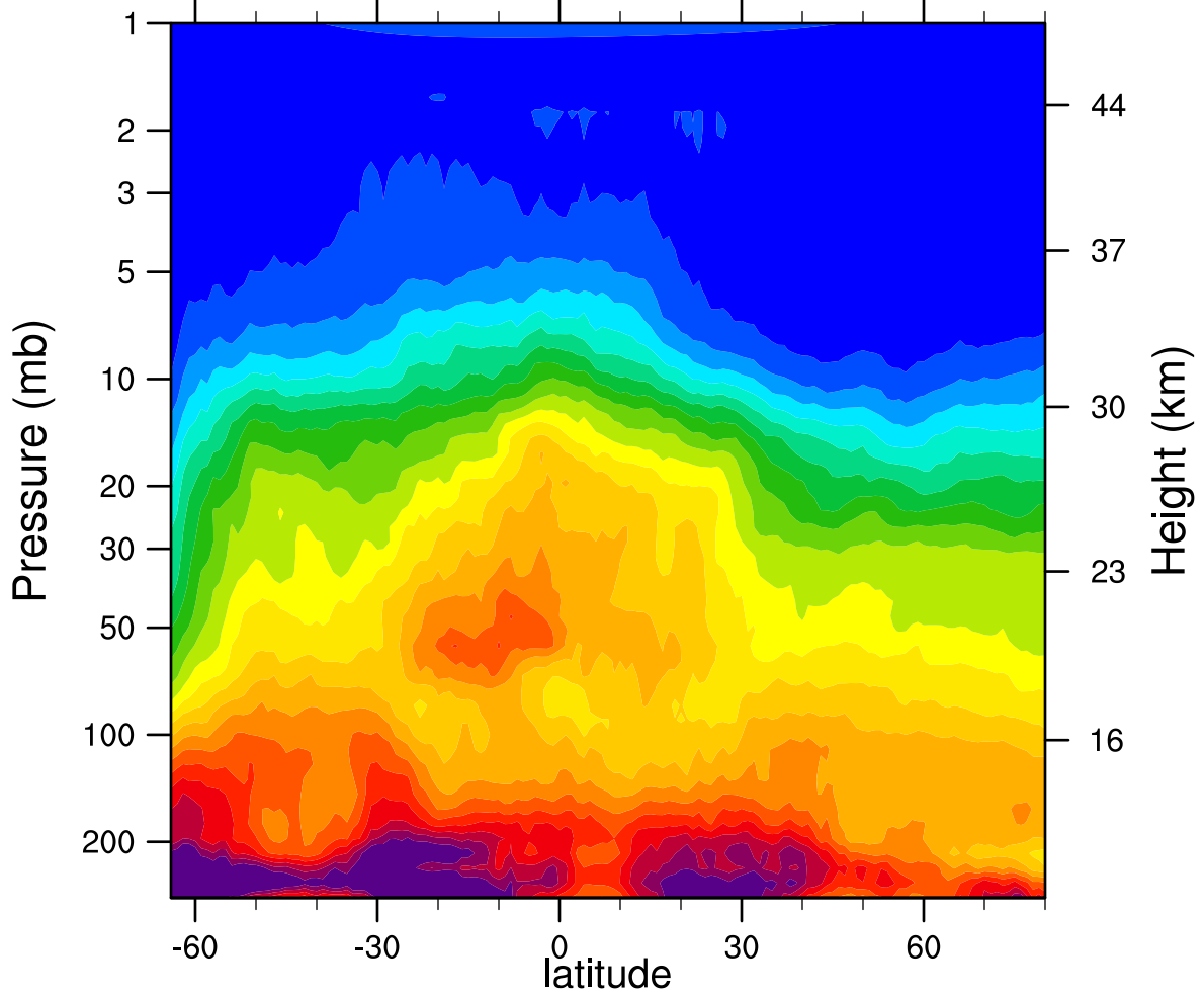
HIRDLSv6 2006d164 N2O_Combined (ppbv)
