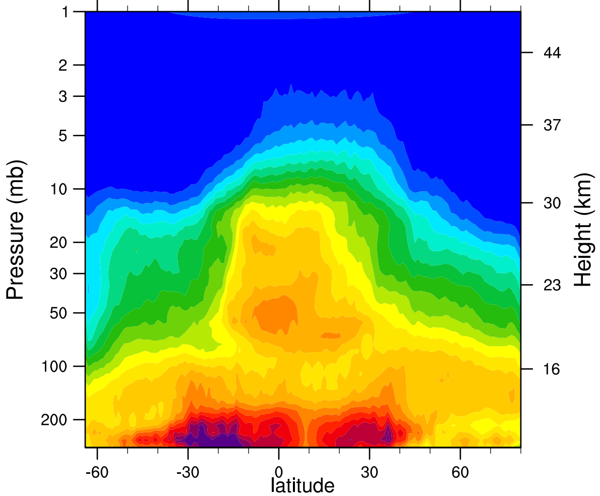
HIRDLSv6 2007d266 N2O_Combined (ppbv)
