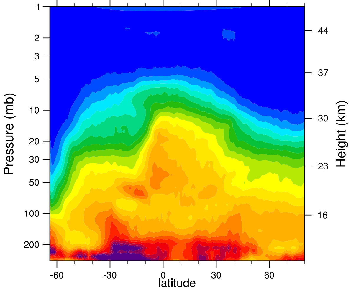
HIRDLSv6 2006d249 N2O_Combined (ppbv)
