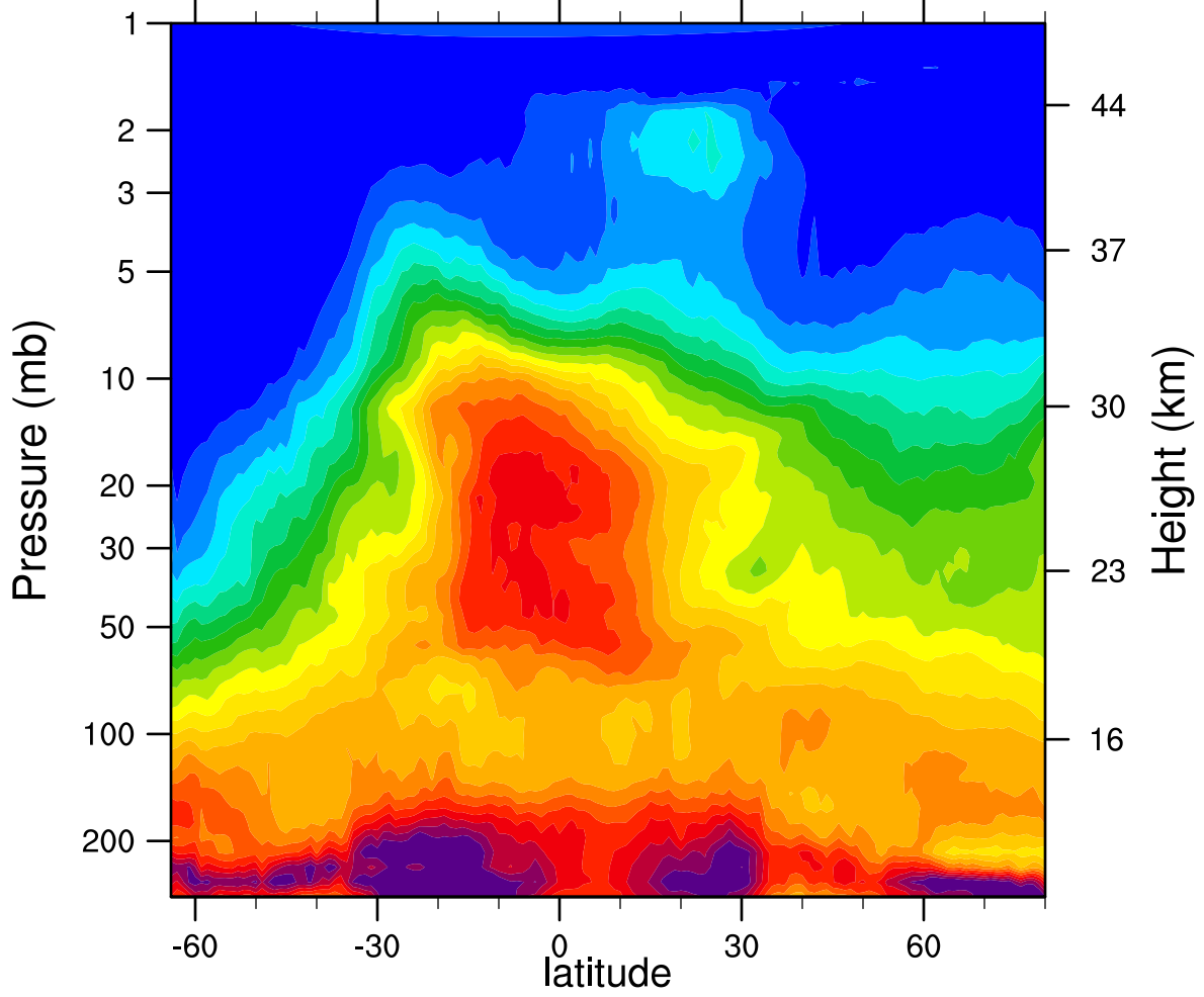
HIRDLSv6 2005d152 N2O_Combined (ppbv)
