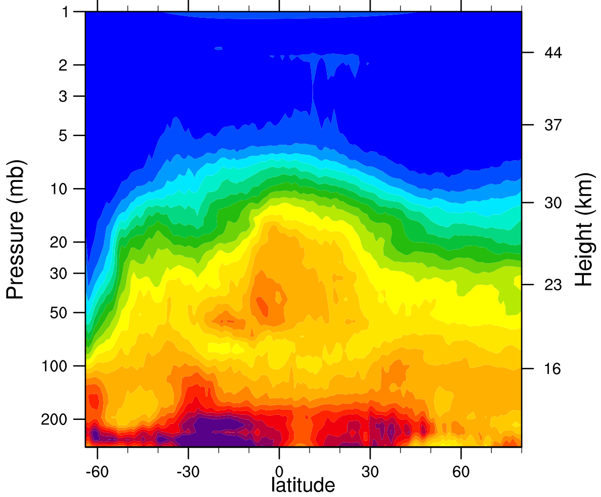
HIRDLSv6 2006d197 N2O_Combined (ppbv)
