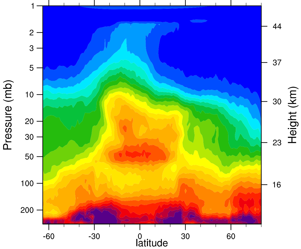
HIRDLSv6 2005d356 N2O_Combined (ppbv)
