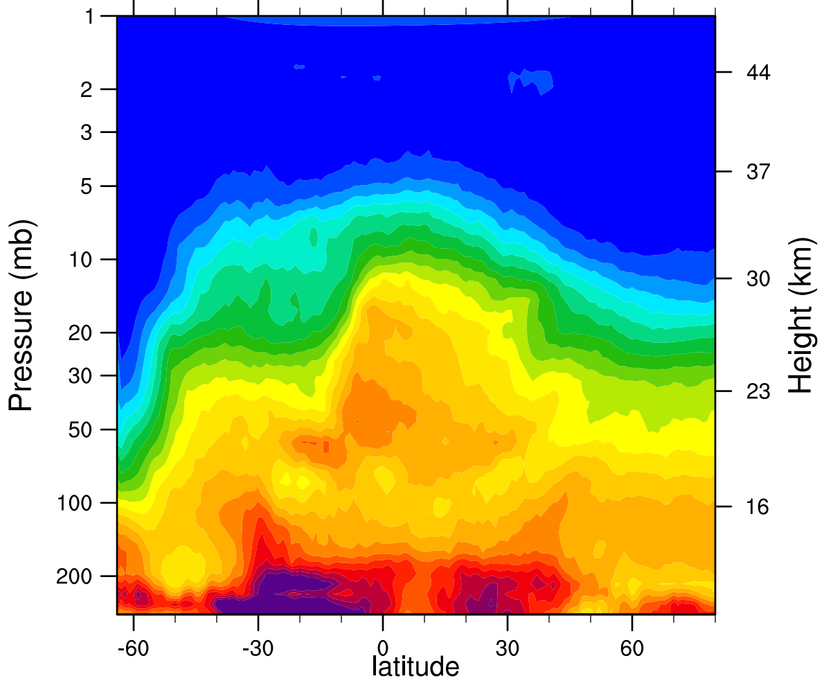
HIRDLSv6 2006d239 N2O_Combined (ppbv)
