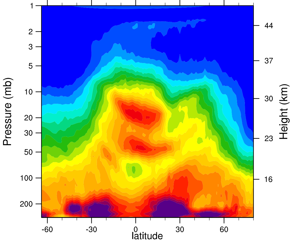
HIRDLSv6 2005d039 N2O_Combined (ppbv)
