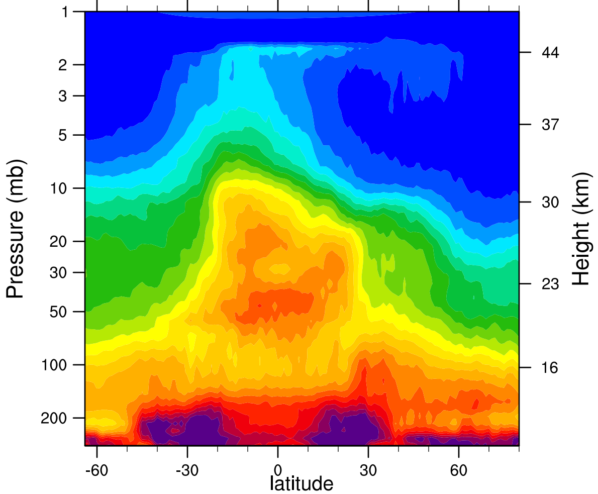
HIRDLSv6 2006d015 N2O_Combined (ppbv)
