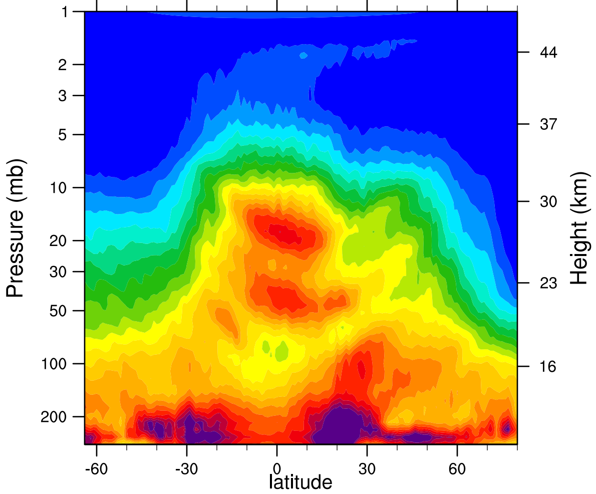
HIRDLSv6 2005d030 N2O_Combined (ppbv)
