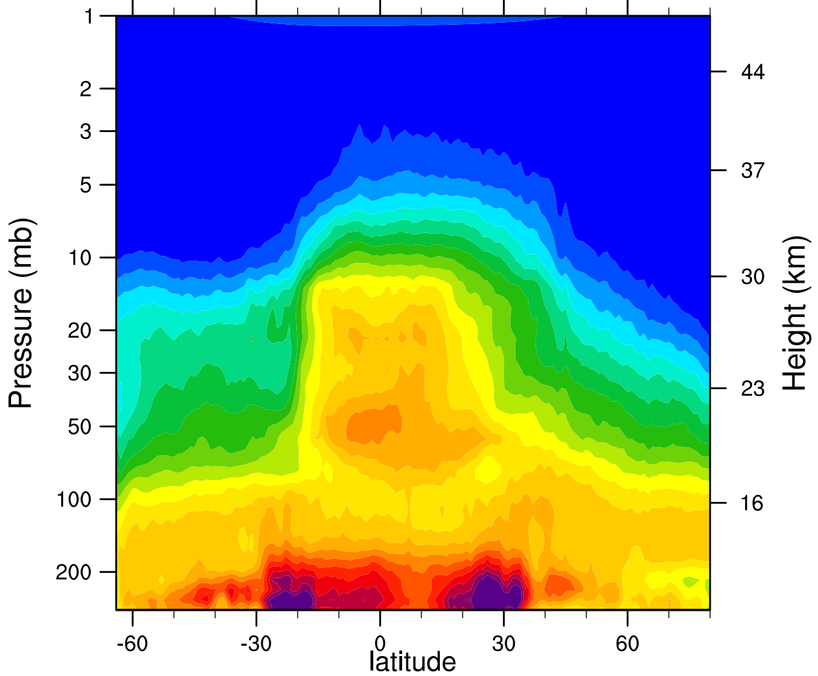
HIRDLSv6 2007d285 N2O_Combined (ppbv)
