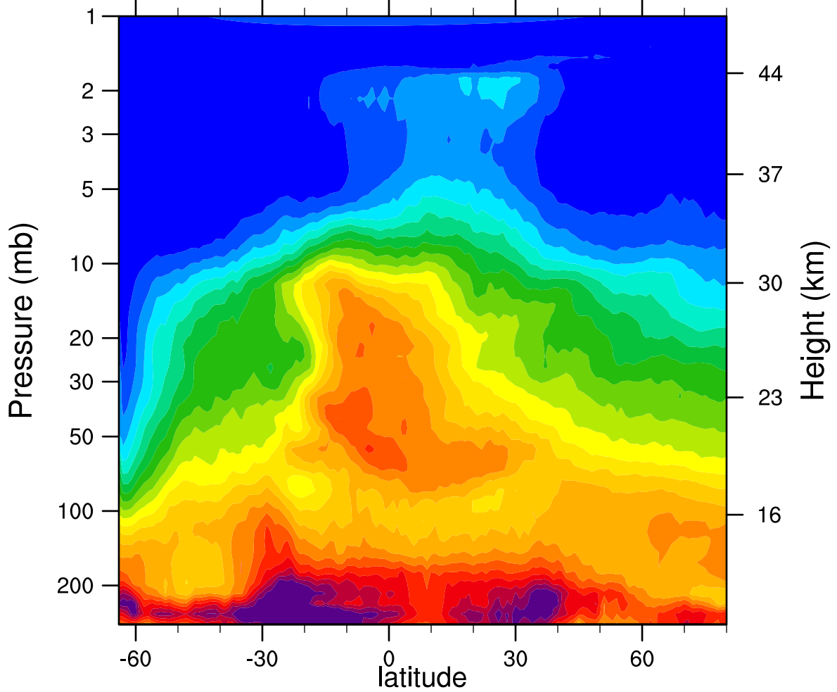
HIRDLSv6 2005d235 N2O_Combined (ppbv)
