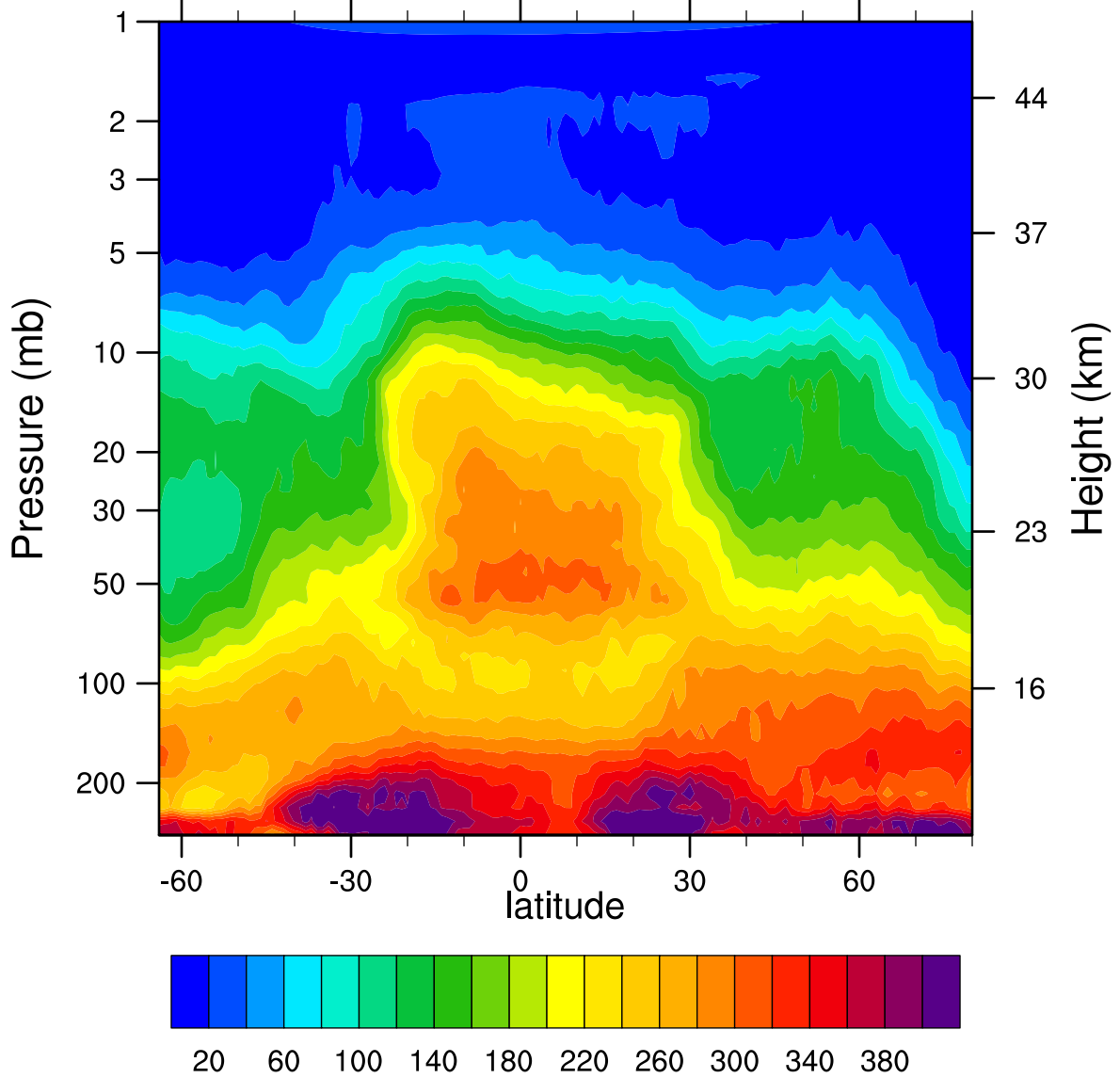
HIRDLSv6 2005d319 N2O_Combined (ppbv)
