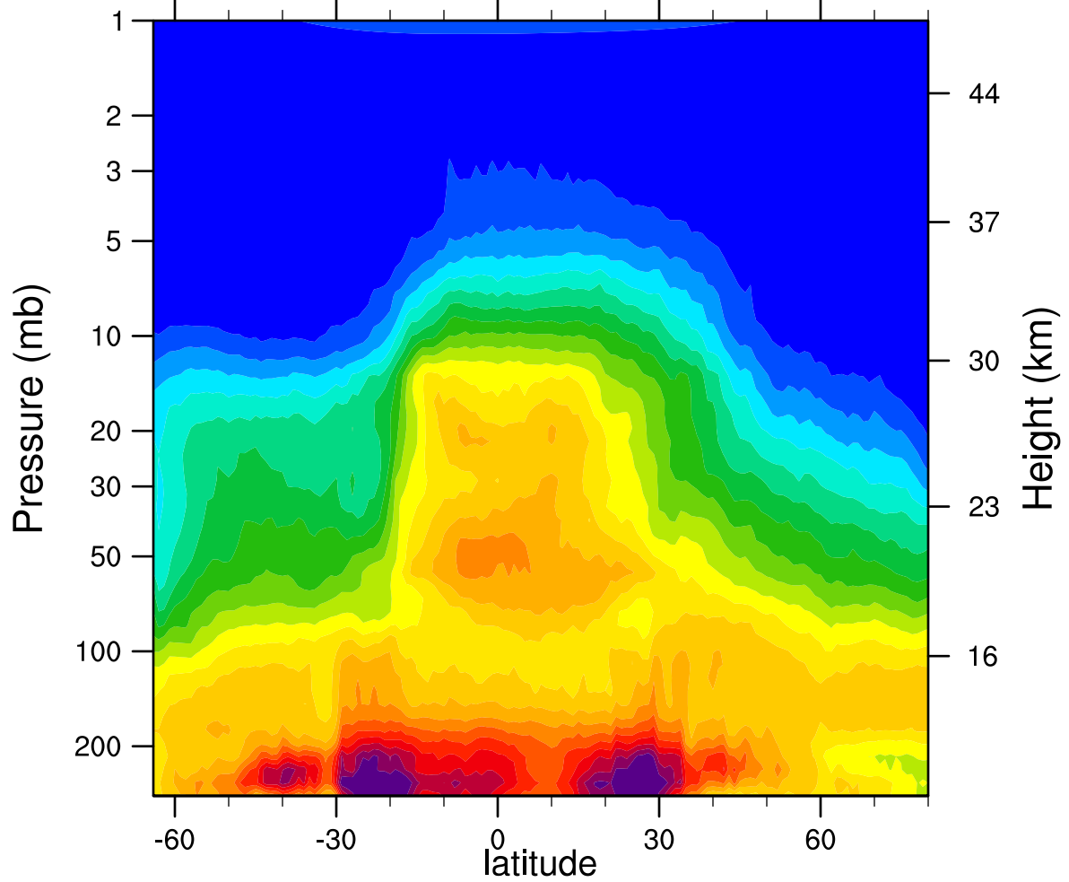
HIRDLSv6 2007d288 N2O_Combined (ppbv)
