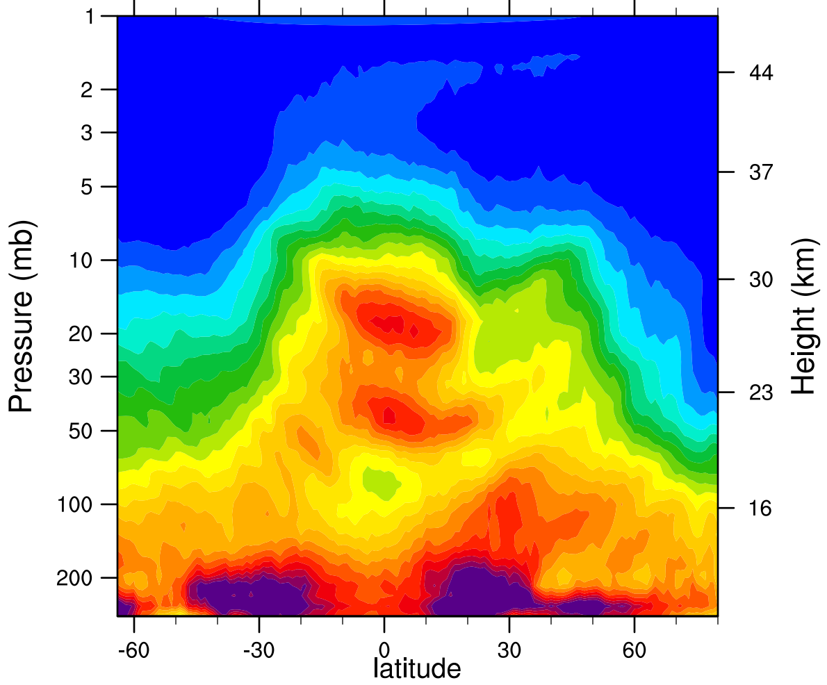
HIRDLSv6 2005d033 N2O_Combined (ppbv)
