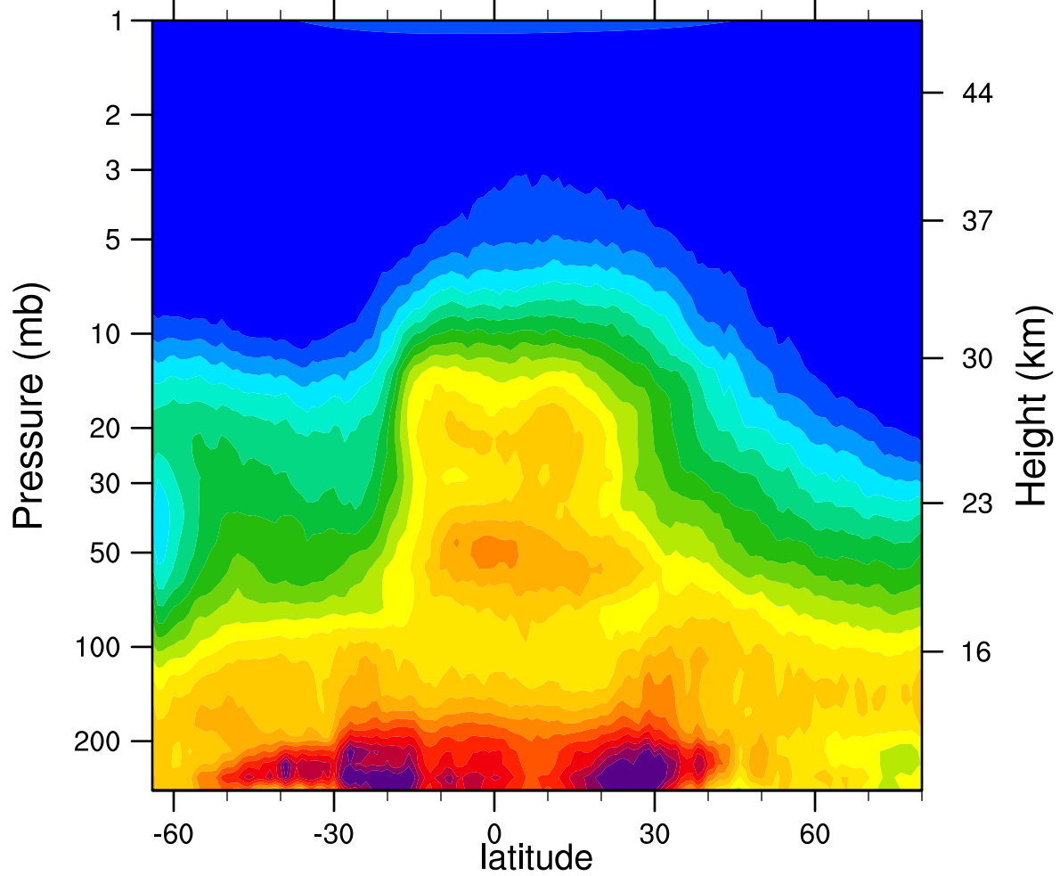
HIRDLSv6 2007d296 N2O_Combined (ppbv)
