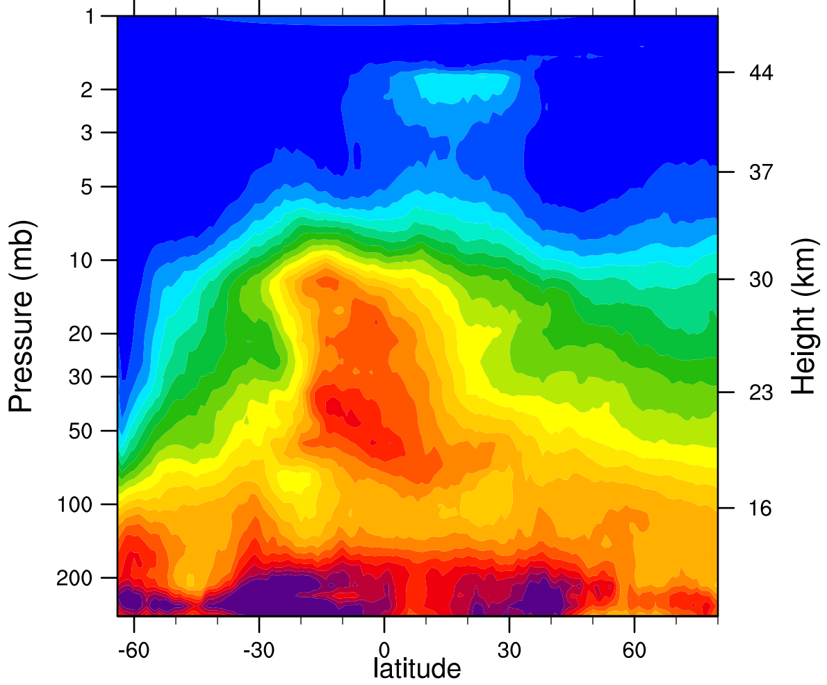
HIRDLSv6 2005d198 N2O_Combined (ppbv)
