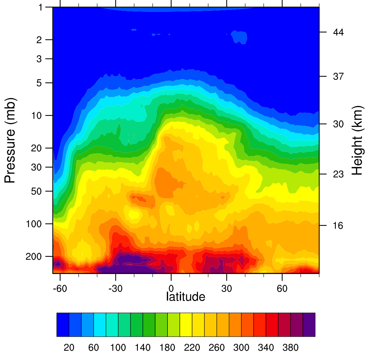
HIRDLSv6 2006d241 N2O_Combined (ppbv)
