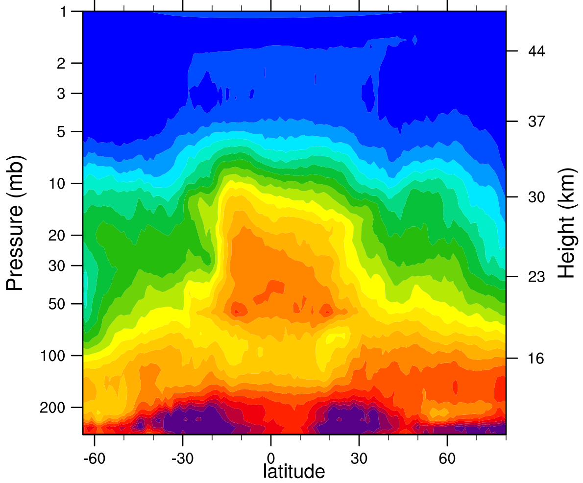
HIRDLSv6 2005d309 N2O_Combined (ppbv)
