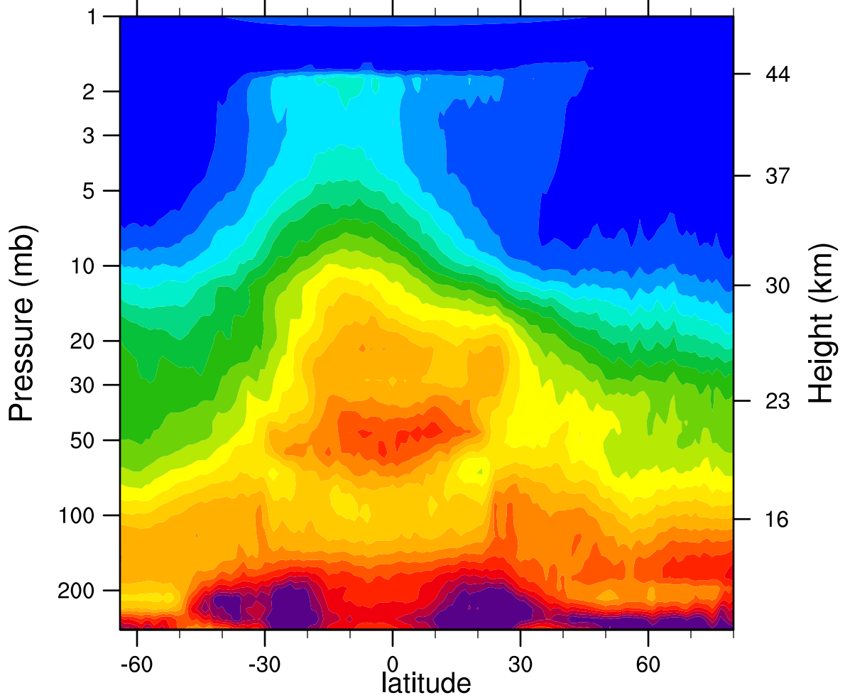
HIRDLSv6 2006d055 N2O_Combined (ppbv)
