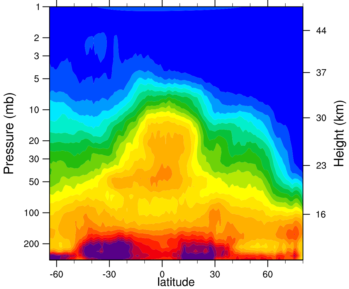
HIRDLSv6 2007d010 N2O_Combined (ppbv)
