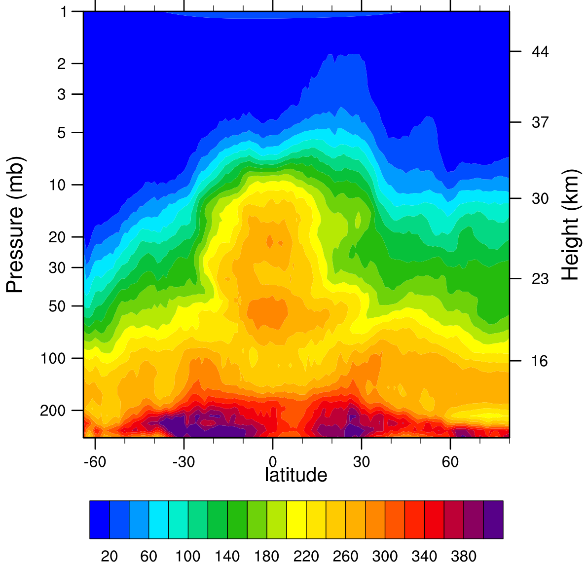
HIRDLSv6 2007d141 N2O_Combined (ppbv)
