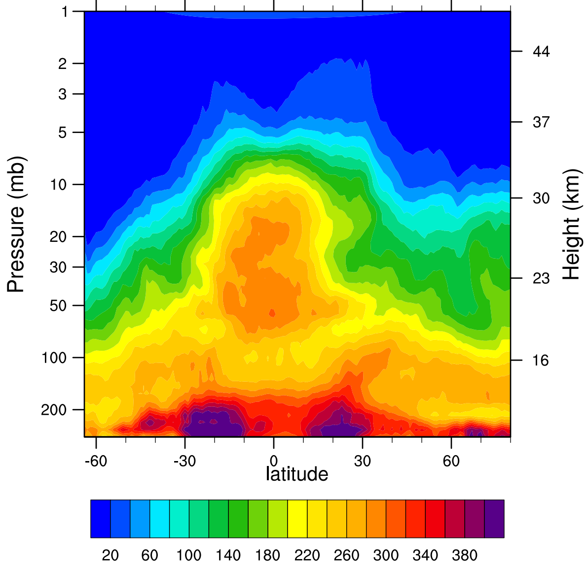
HIRDLSv6 2007d123 N2O_Combined (ppbv)
