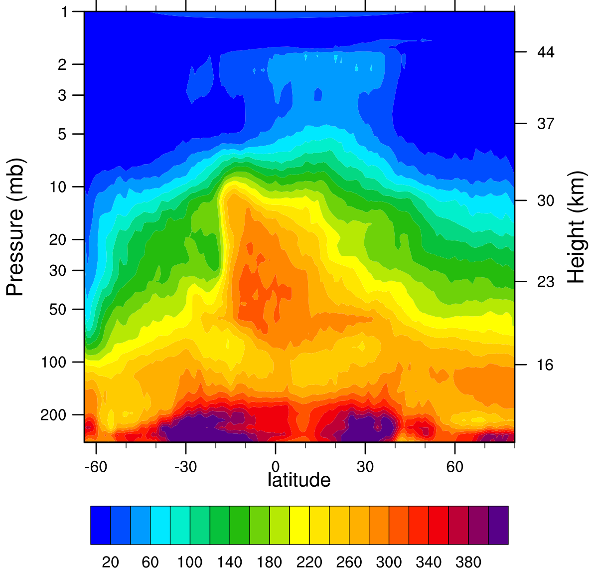
HIRDLSv6 2005d260 N2O_Combined (ppbv)
