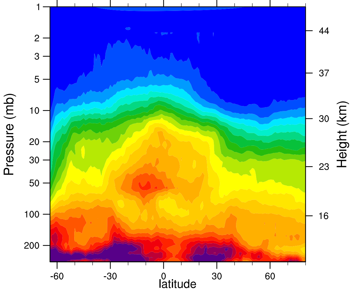
HIRDLSv6 2006d159 N2O_Combined (ppbv)
