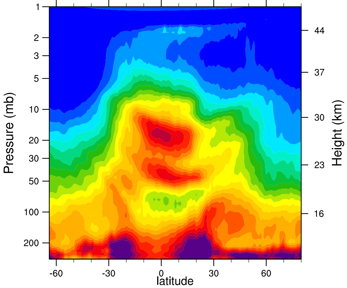
HIRDLSv6 2005d055 N2O_Combined (ppbv)
