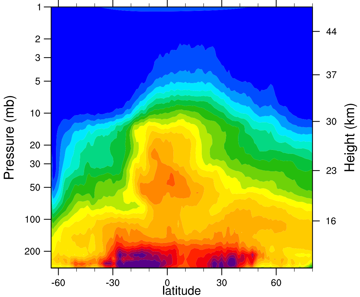
HIRDLSv6 2007d217 N2O_Combined (ppbv)
