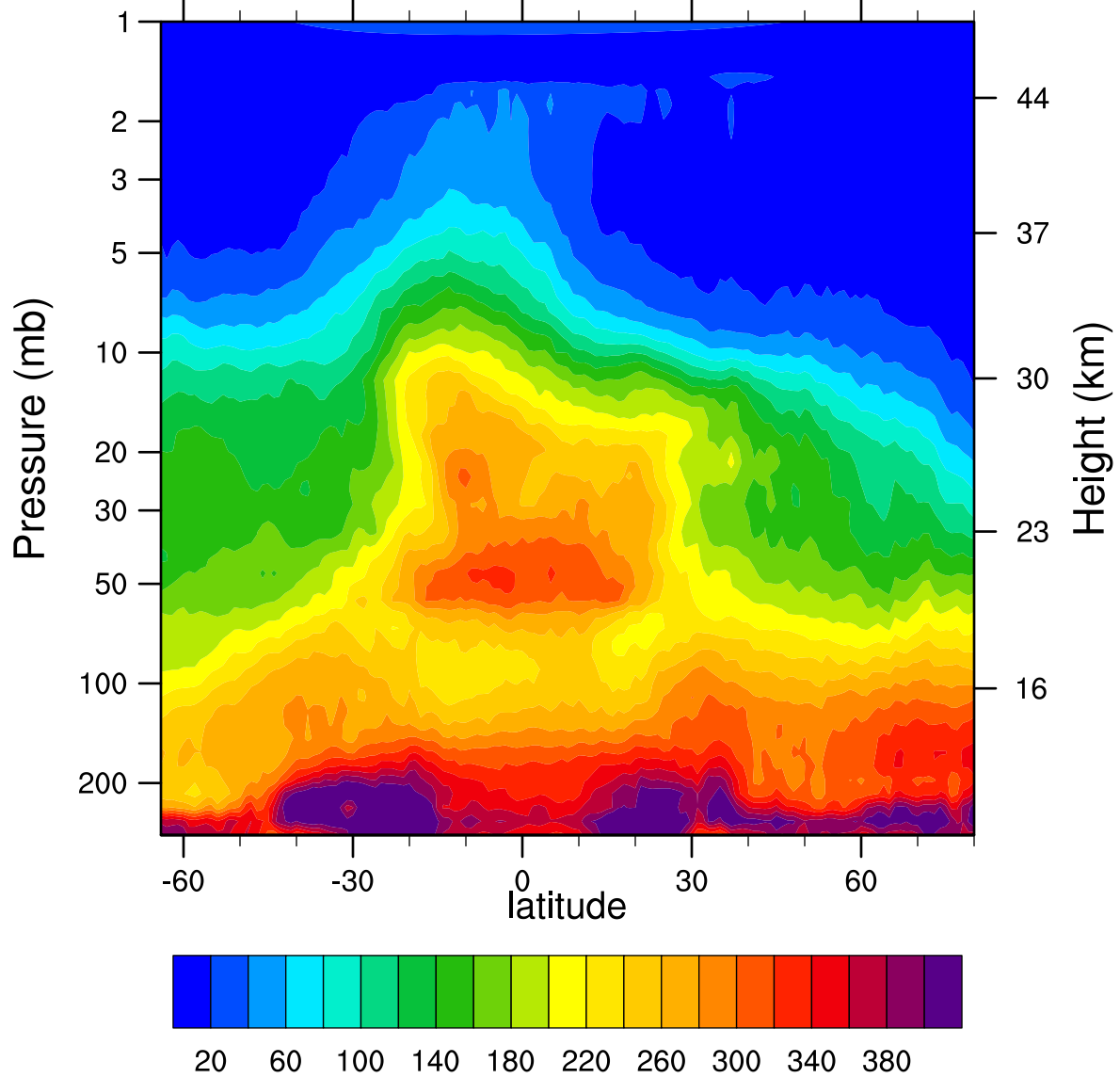
HIRDLSv6 2005d353 N2O_Combined (ppbv)
