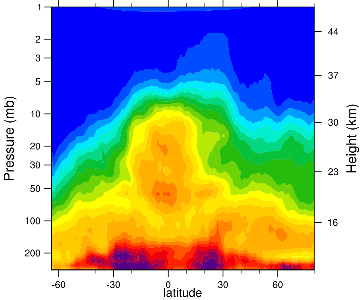
HIRDLSv6 2007d135 N2O_Combined (ppbv)
