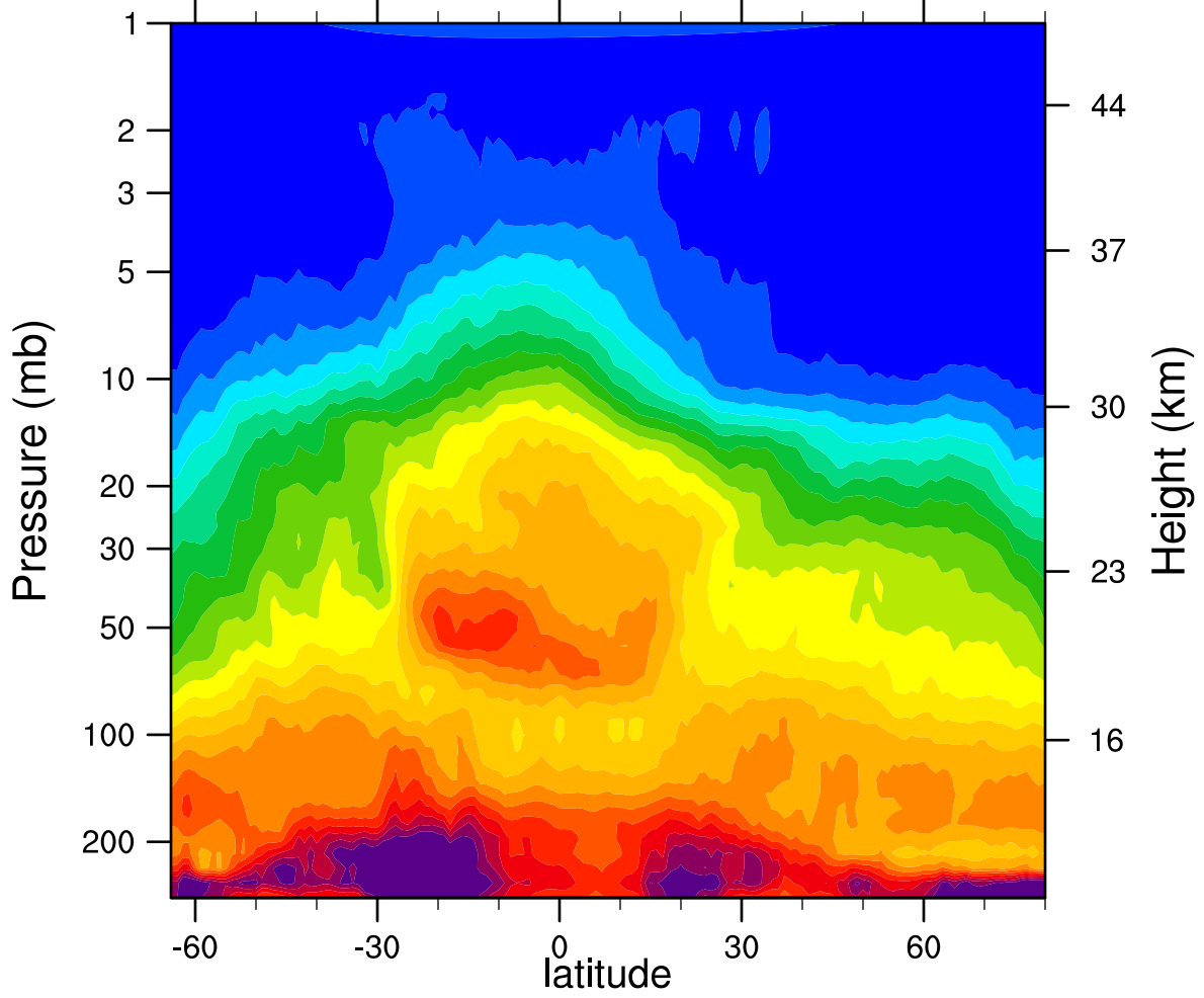
HIRDLSv6 2006d122 N2O_Combined (ppbv)
