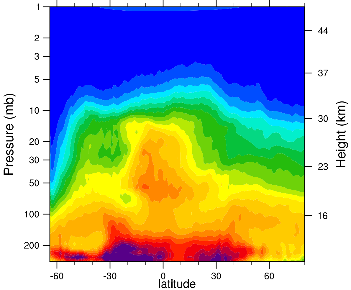
HIRDLSv6 2007d198 N2O_Combined (ppbv)
