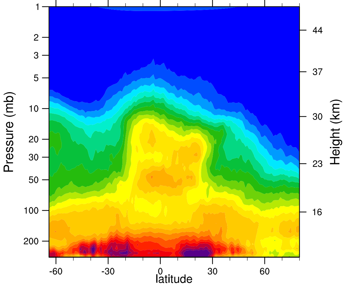
HIRDLSv6 2007d347 N2O_Combined (ppbv)
