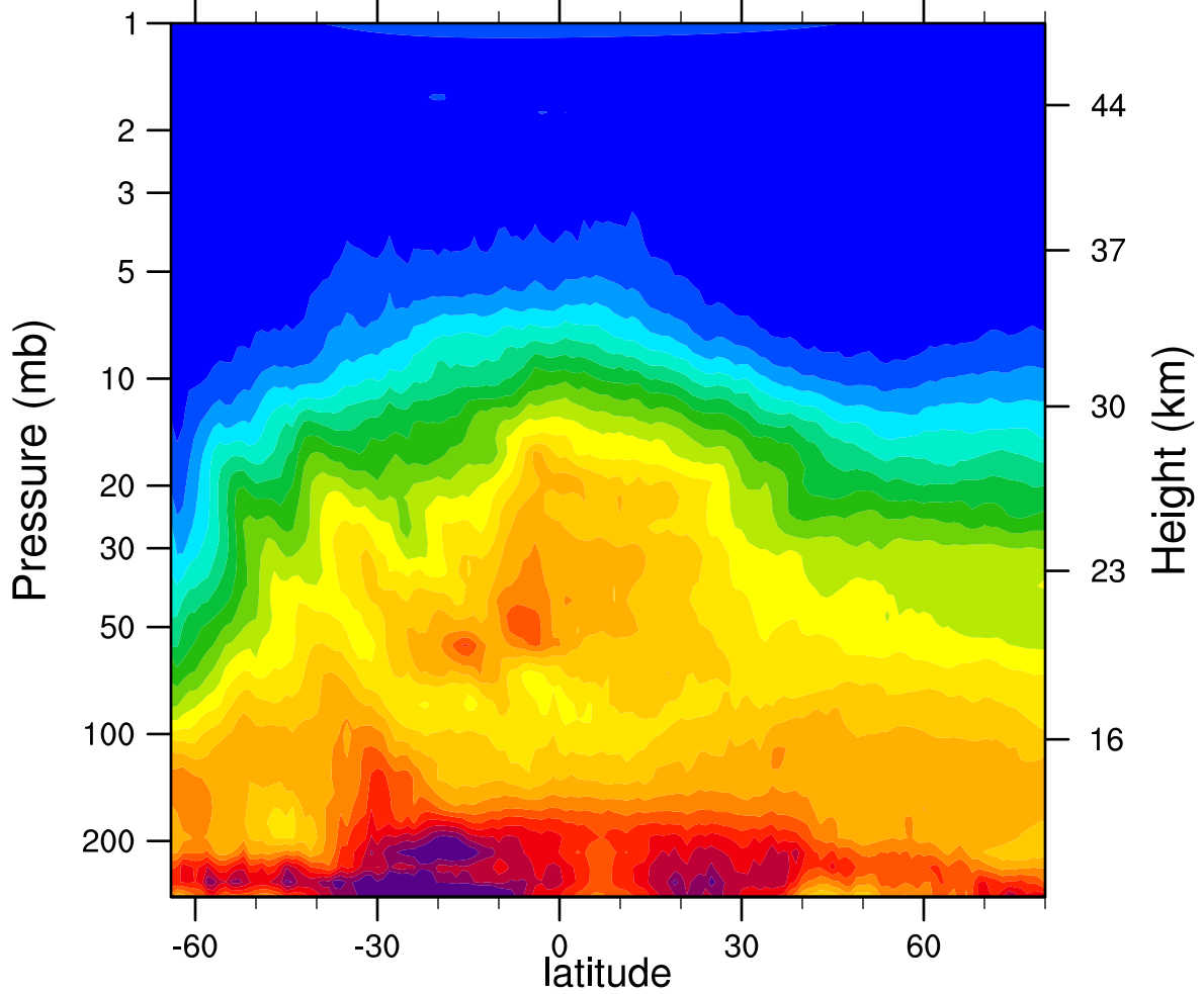
HIRDLSv6 2006d182 N2O_Combined (ppbv)
