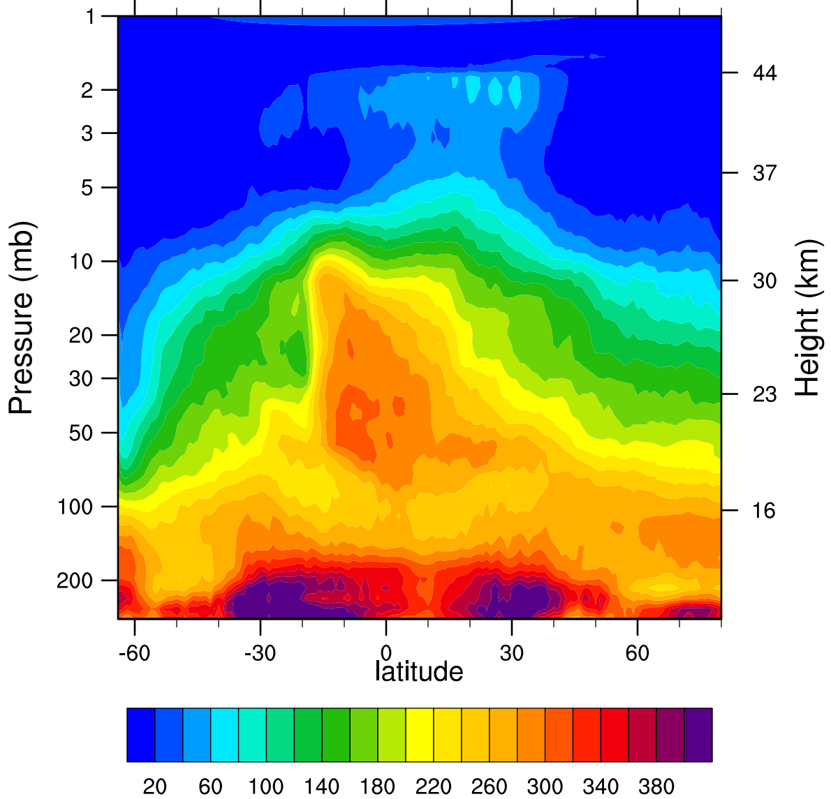
HIRDLSv6 2005d258 N2O_Combined (ppbv)
