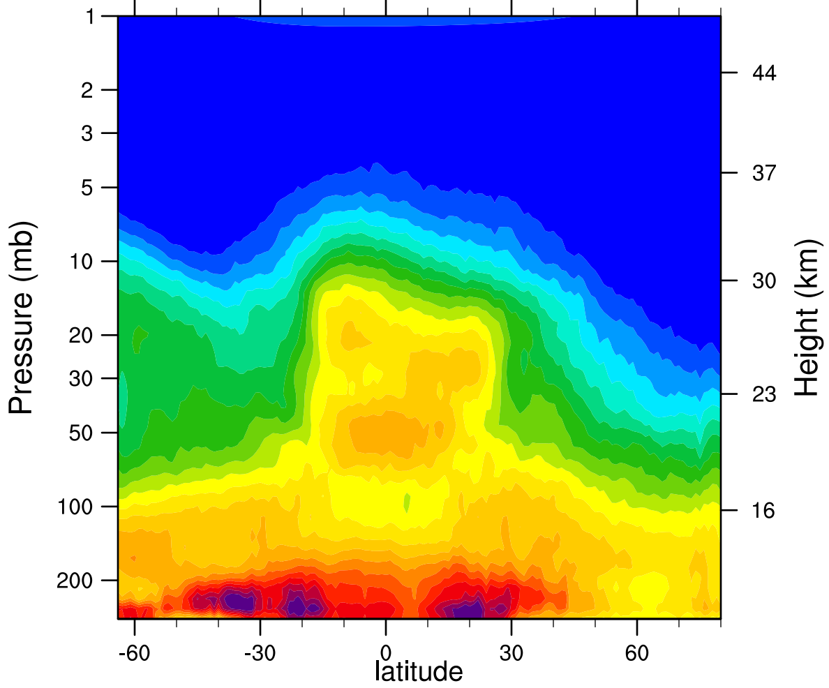
HIRDLSv6 2007d336 N2O_Combined (ppbv)
