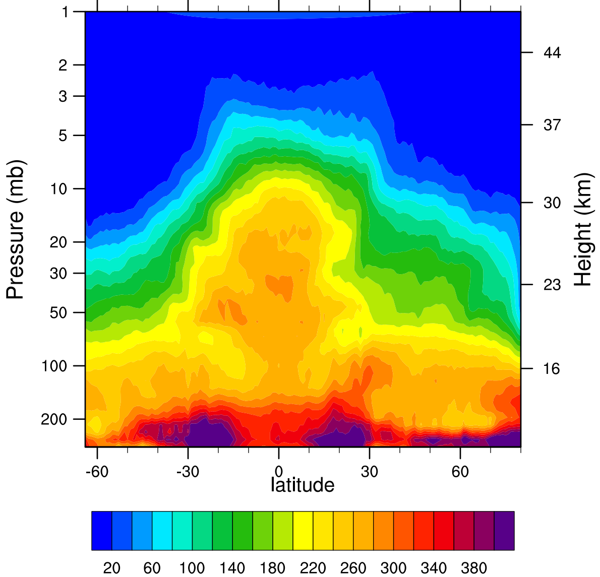
HIRDLSv6 2007d088 N2O_Combined (ppbv)
