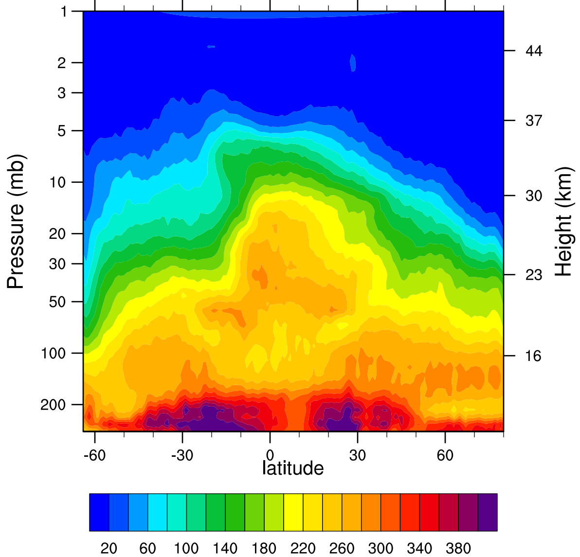
HIRDLSv6 2006d285 N2O_Combined (ppbv)
