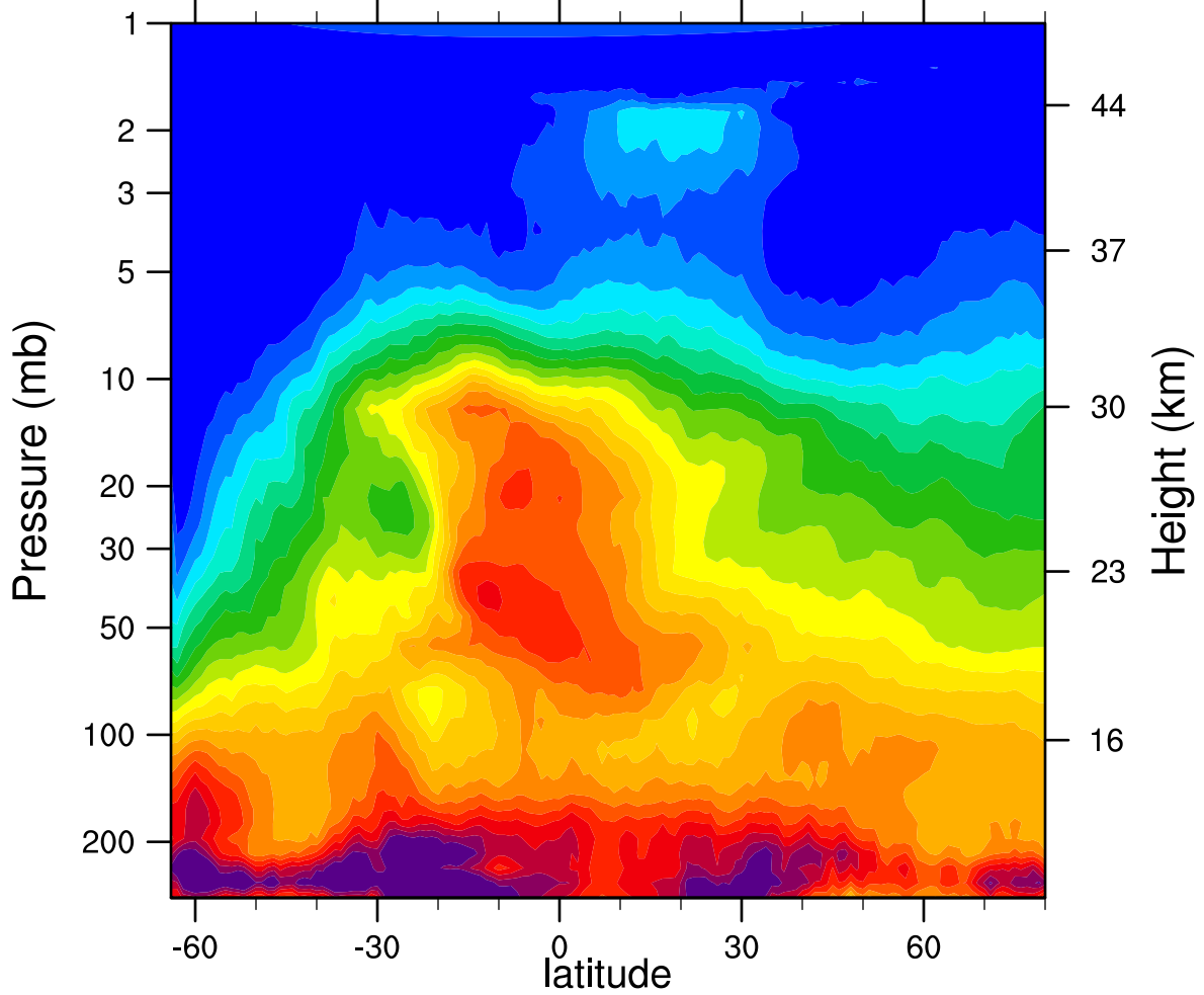
HIRDLSv6 2005d188 N2O_Combined (ppbv)
