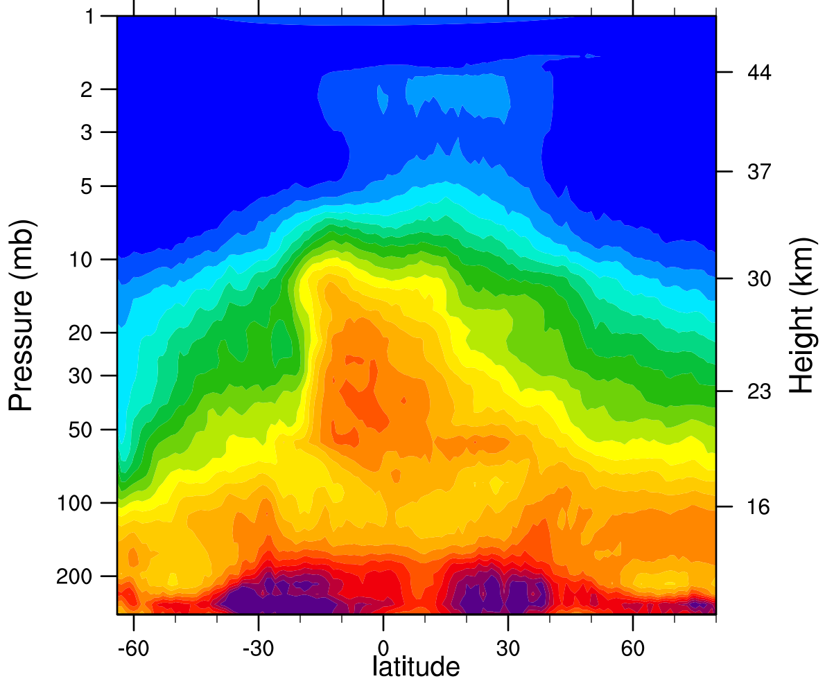
HIRDLSv6 2005d269 N2O_Combined (ppbv)
