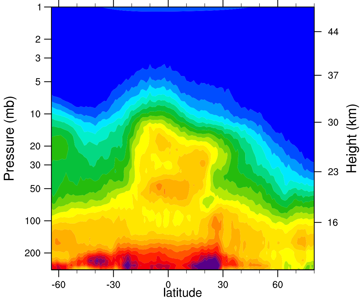
HIRDLSv6 2007d353 N2O_Combined (ppbv)
