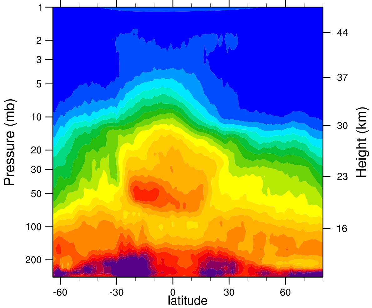
HIRDLSv6 2006d123 N2O_Combined (ppbv)
