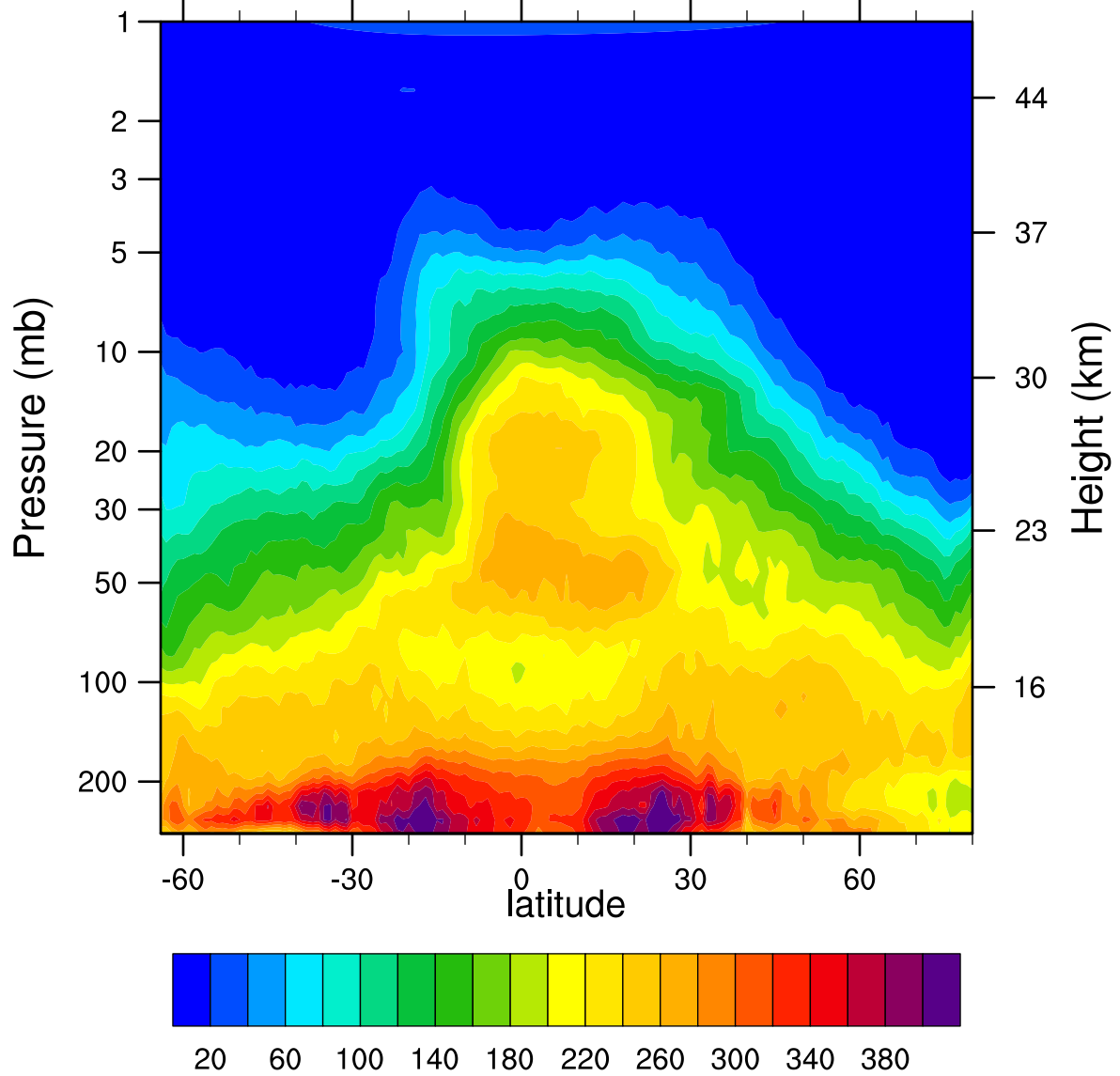
HIRDLSv6 2006d317 N2O_Combined (ppbv)
