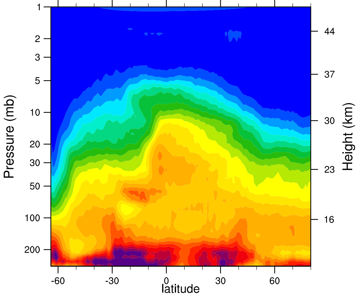
HIRDLSv6 2006d257 N2O_Combined (ppbv)
