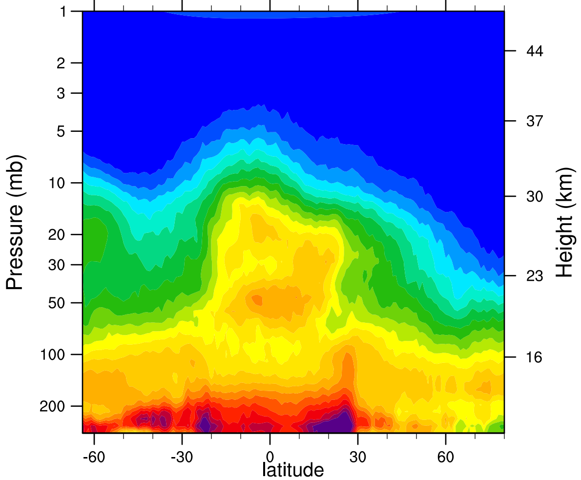
HIRDLSv6 2007d355 N2O_Combined (ppbv)
