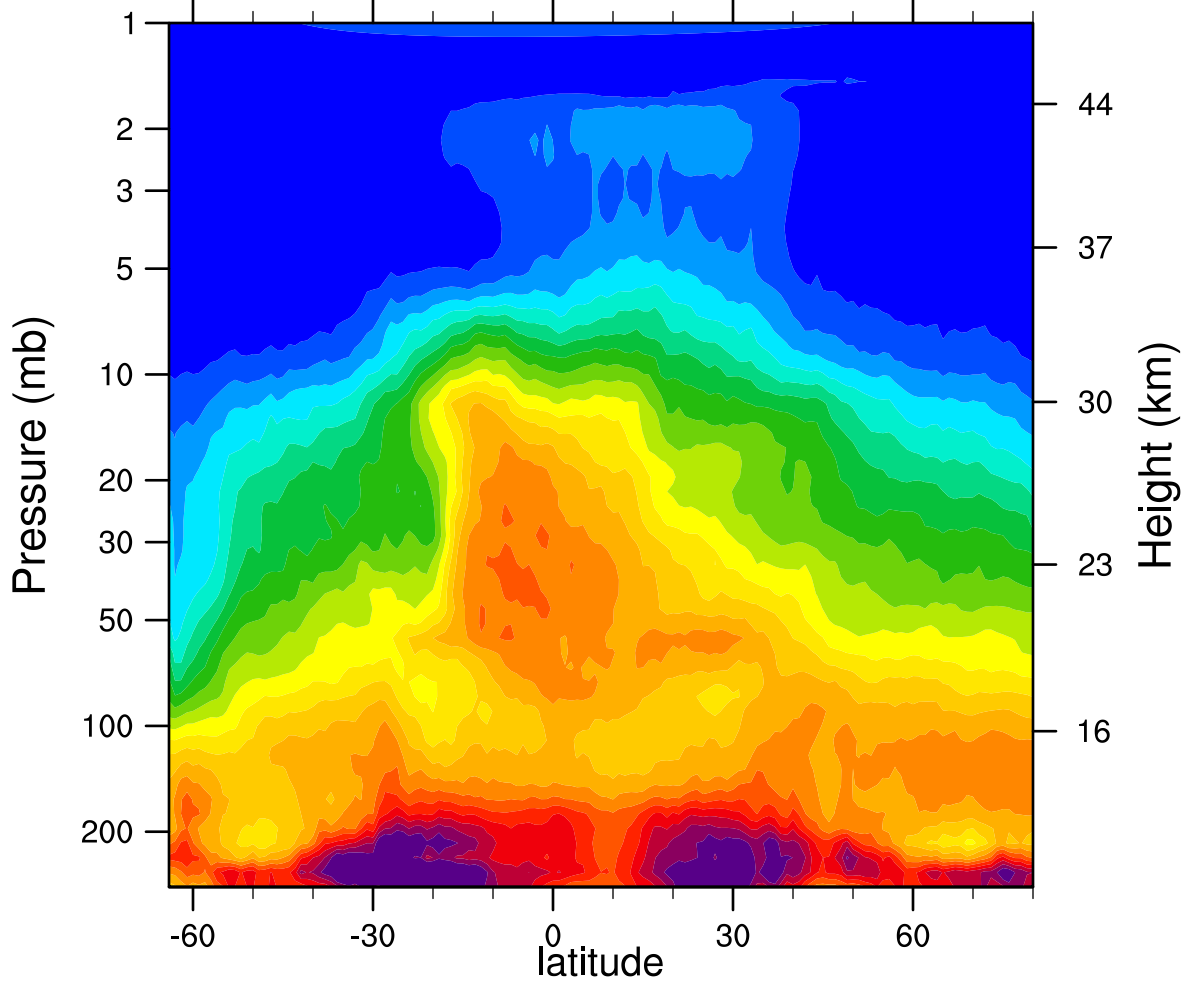
HIRDLSv6 2005d266 N2O_Combined (ppbv)
