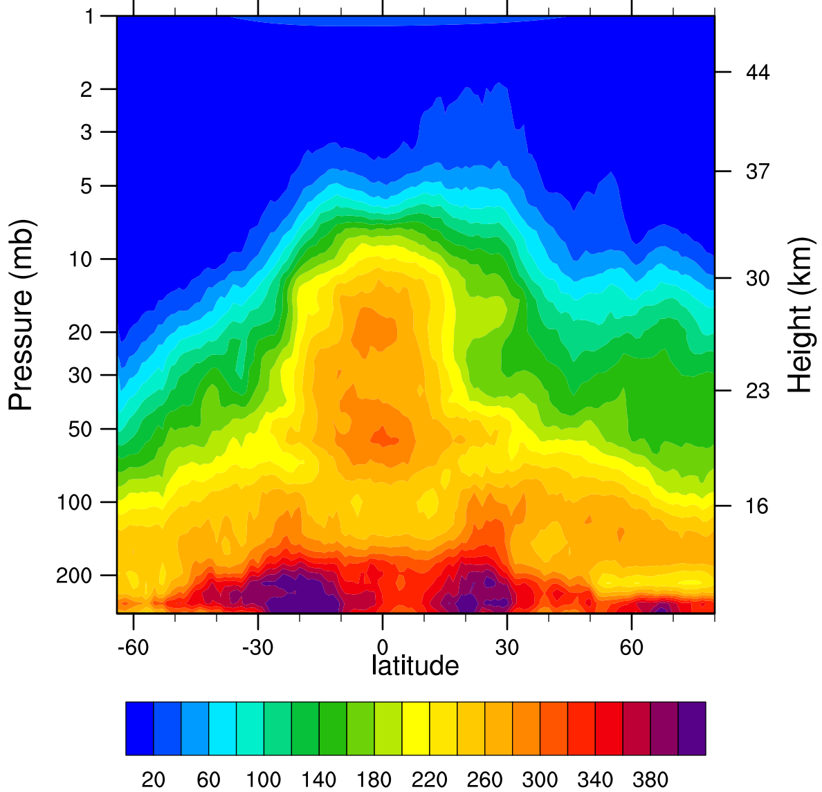
HIRDLSv6 2007d130 N2O_Combined (ppbv)
