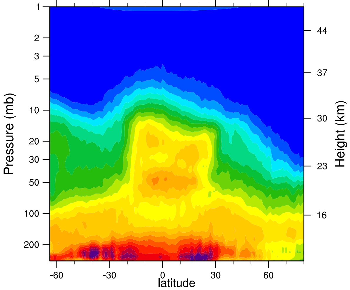
HIRDLSv6 2007d342 N2O_Combined (ppbv)
