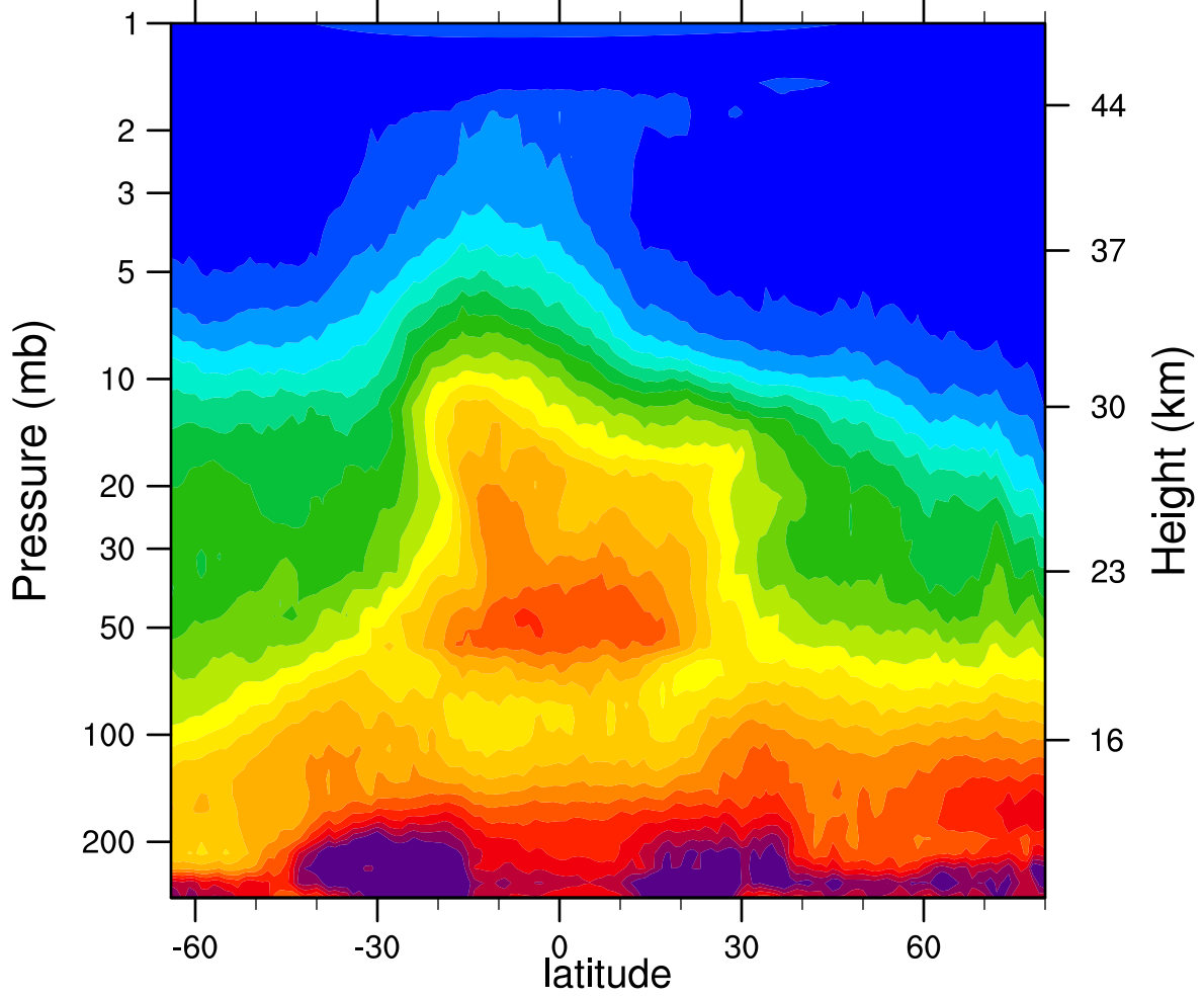
HIRDLSv6 2005d351 N2O_Combined (ppbv)
