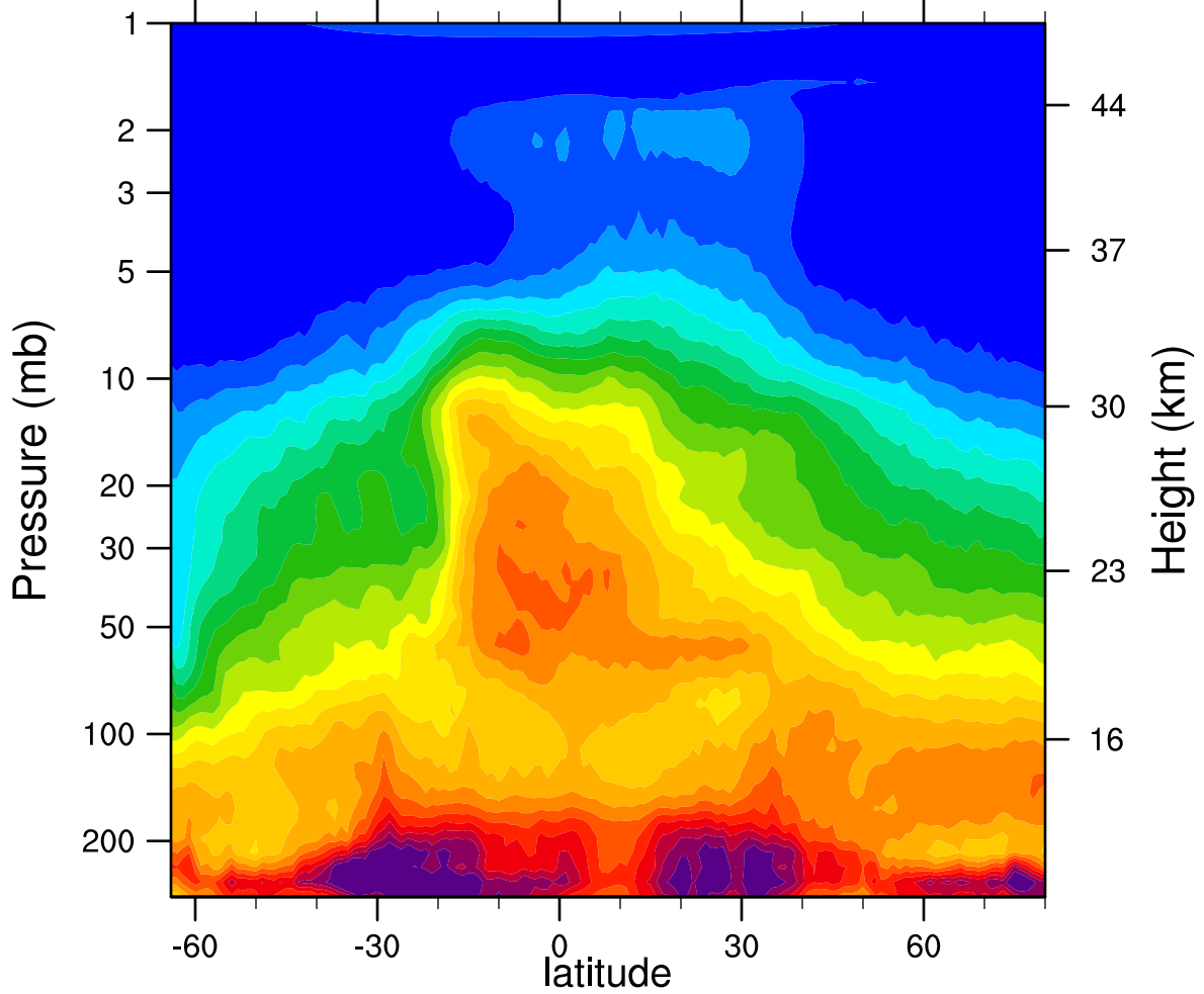
HIRDLSv6 2005d271 N2O_Combined (ppbv)
