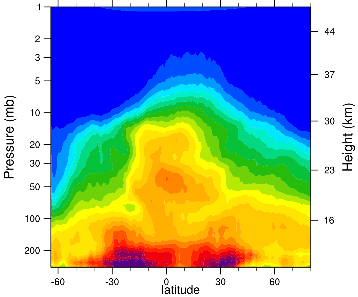
HIRDLSv6 2007d239 N2O_Combined (ppbv)
