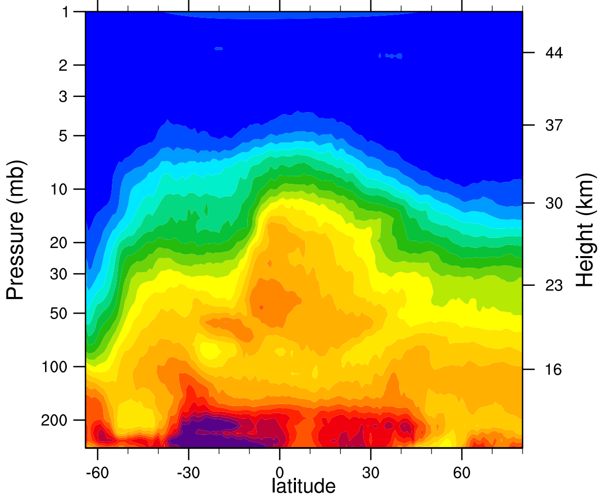
HIRDLSv6 2006d233 N2O_Combined (ppbv)
