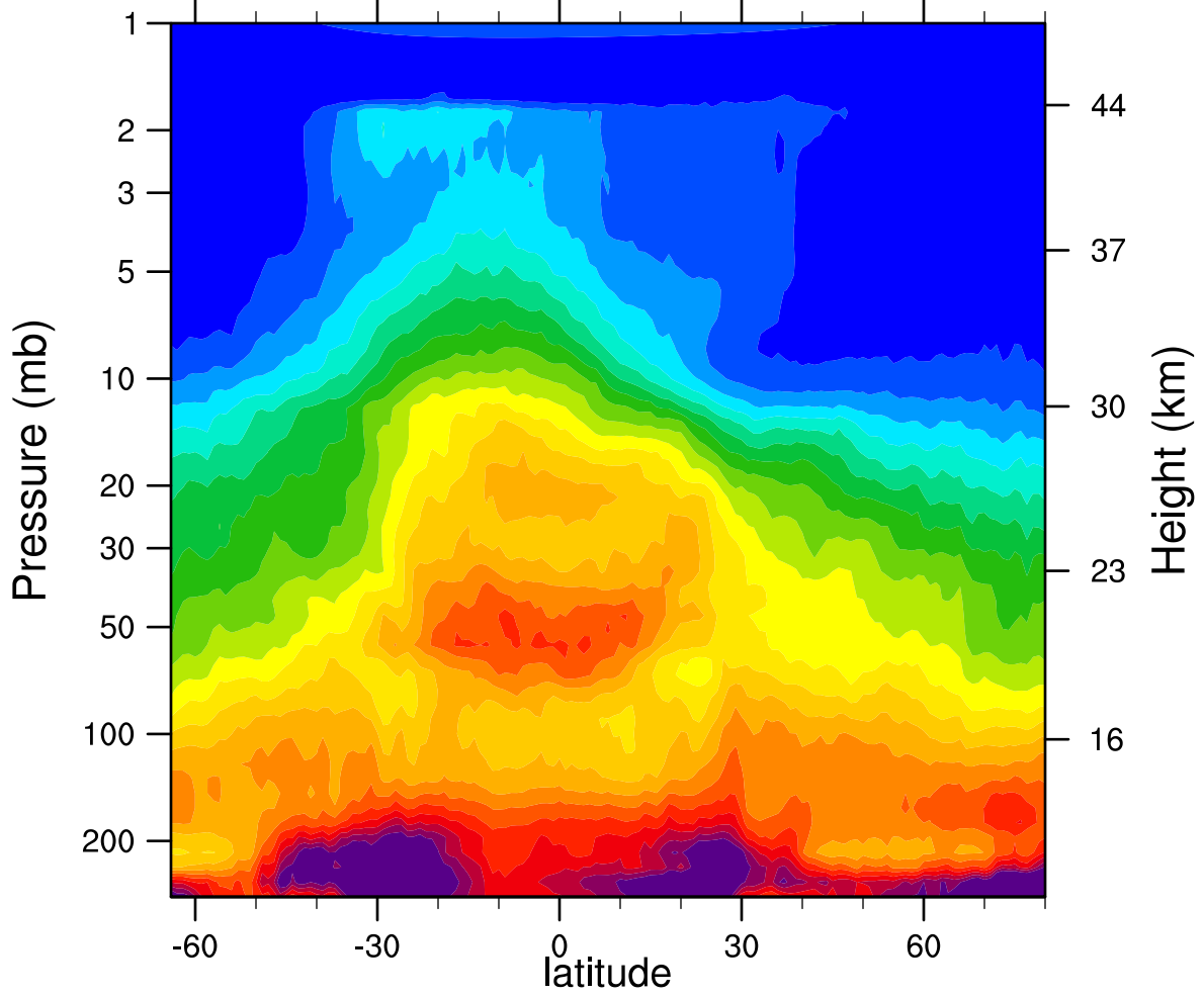
HIRDLSv6 2006d079 N2O_Combined (ppbv)
