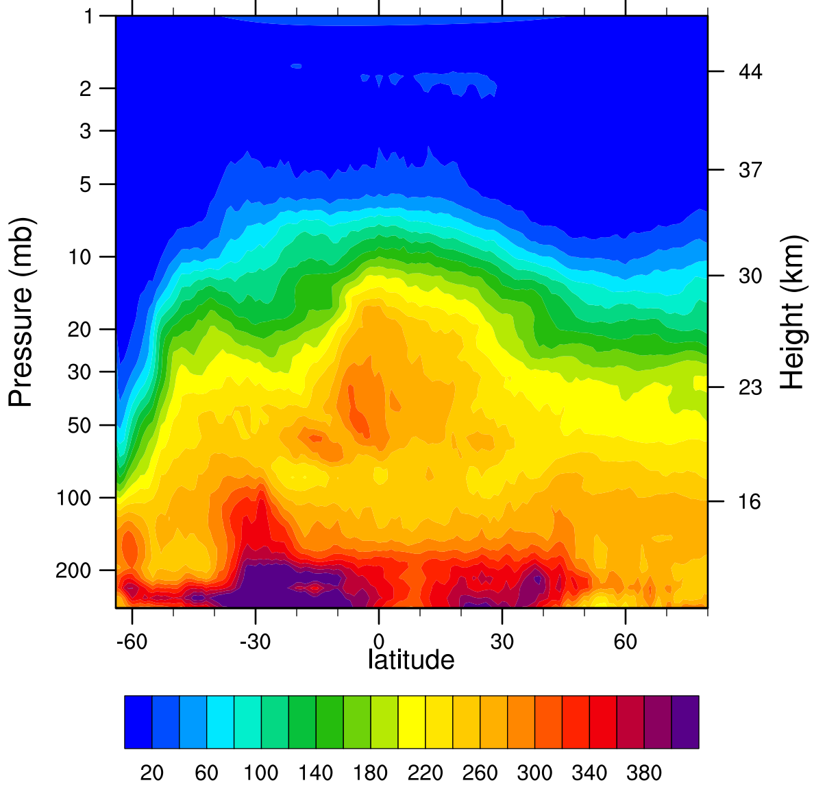
HIRDLSv6 2006d203 N2O_Combined (ppbv)
