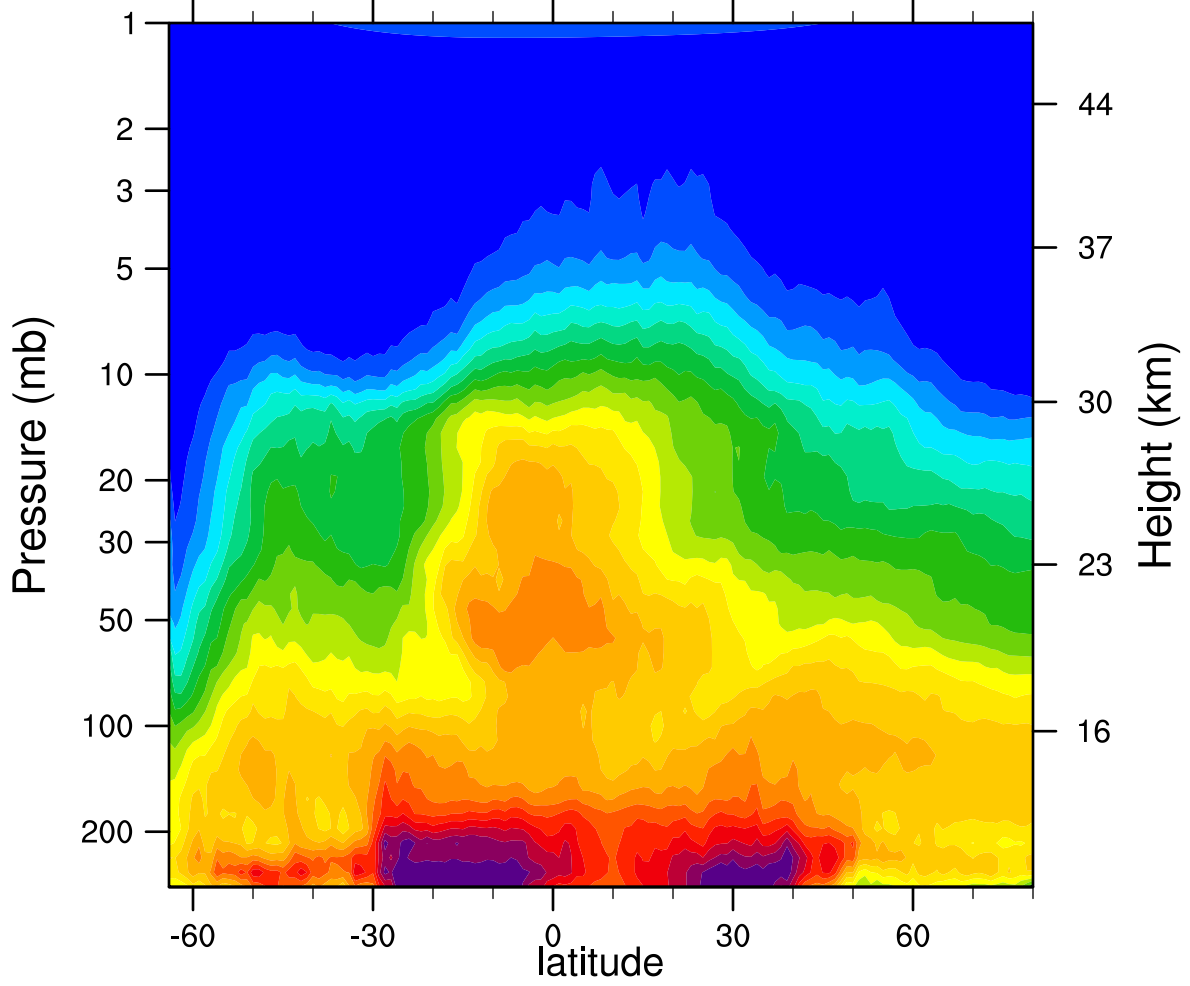
HIRDLSv6 2007d213 N2O_Combined (ppbv)
