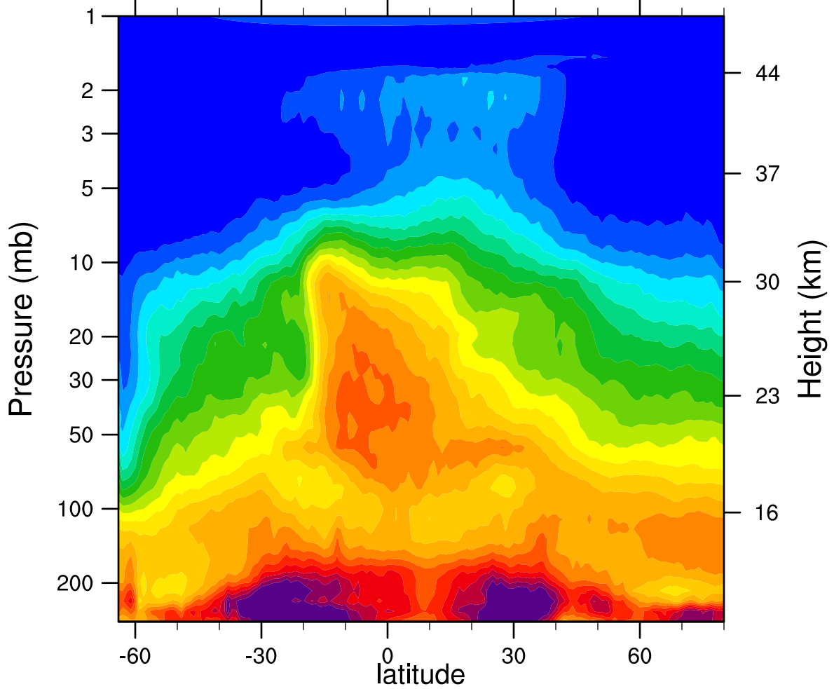
HIRDLSv6 2005d262 N2O_Combined (ppbv)
