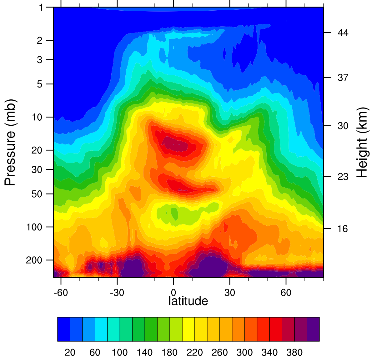
HIRDLSv6 2005d062 N2O_Combined (ppbv)
