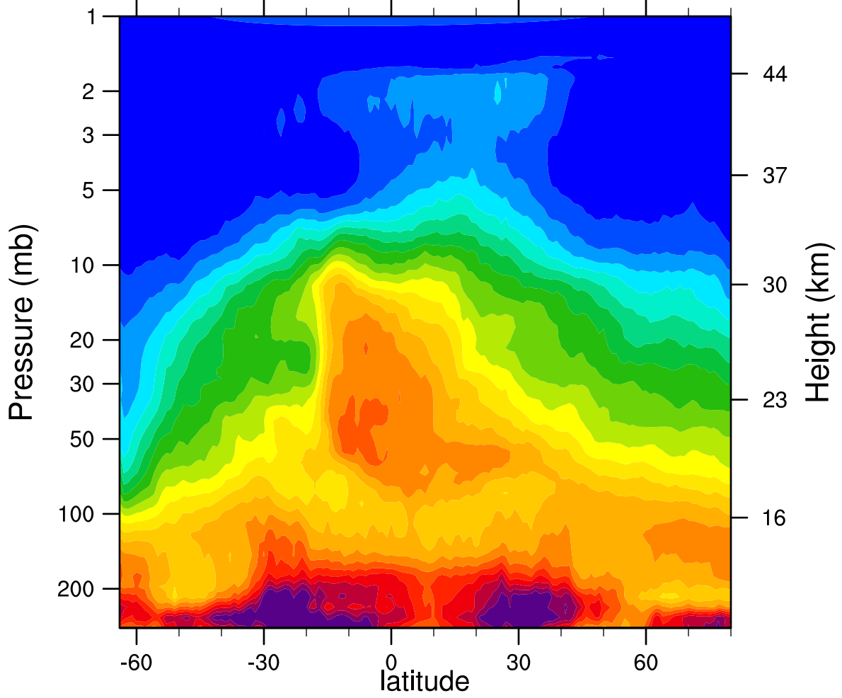
HIRDLSv6 2005d253 N2O_Combined (ppbv)
