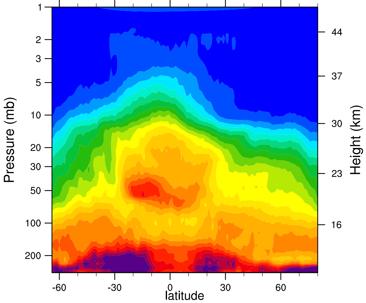
HIRDLSv6 2006d119 N2O_Combined (ppbv)
