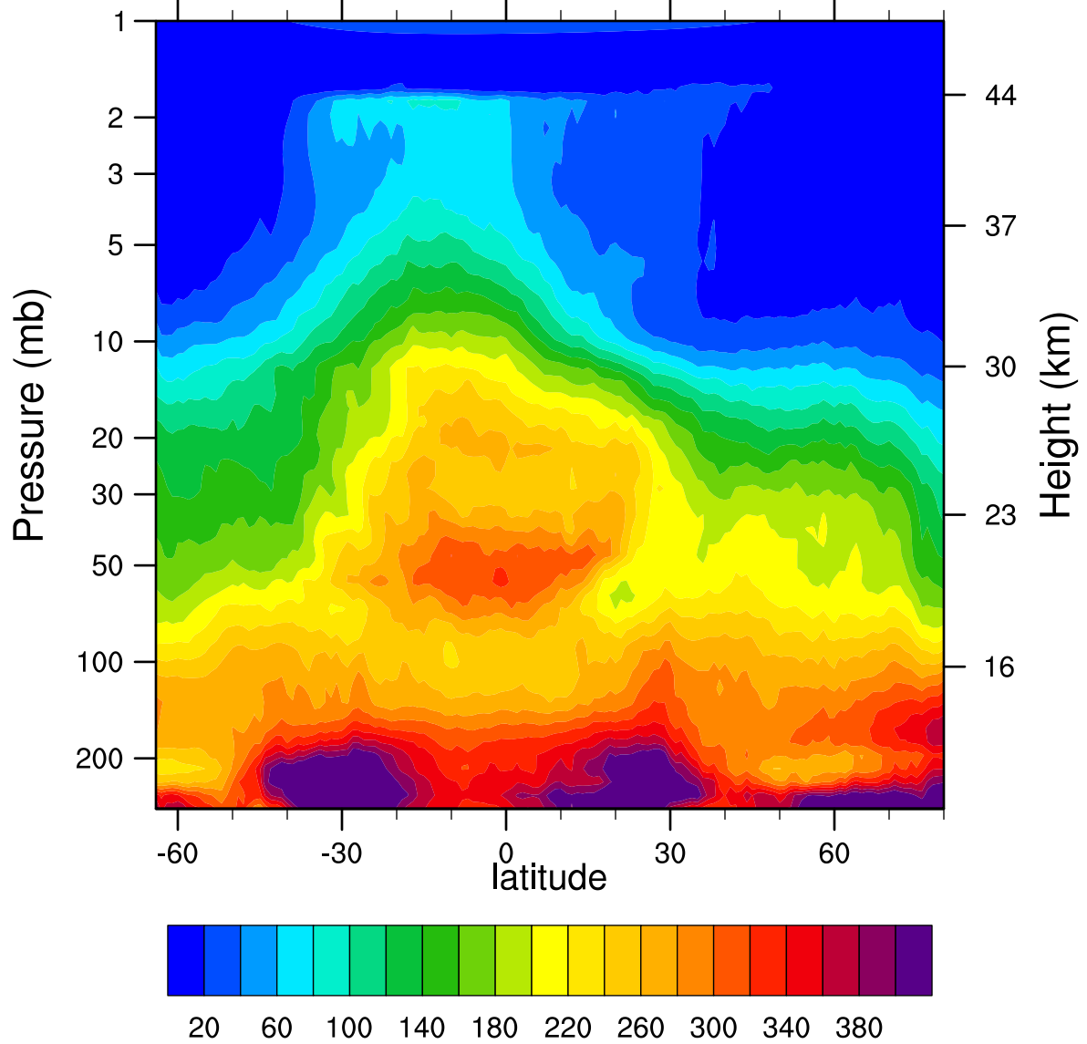
HIRDLSv6 2006d068 N2O_Combined (ppbv)
