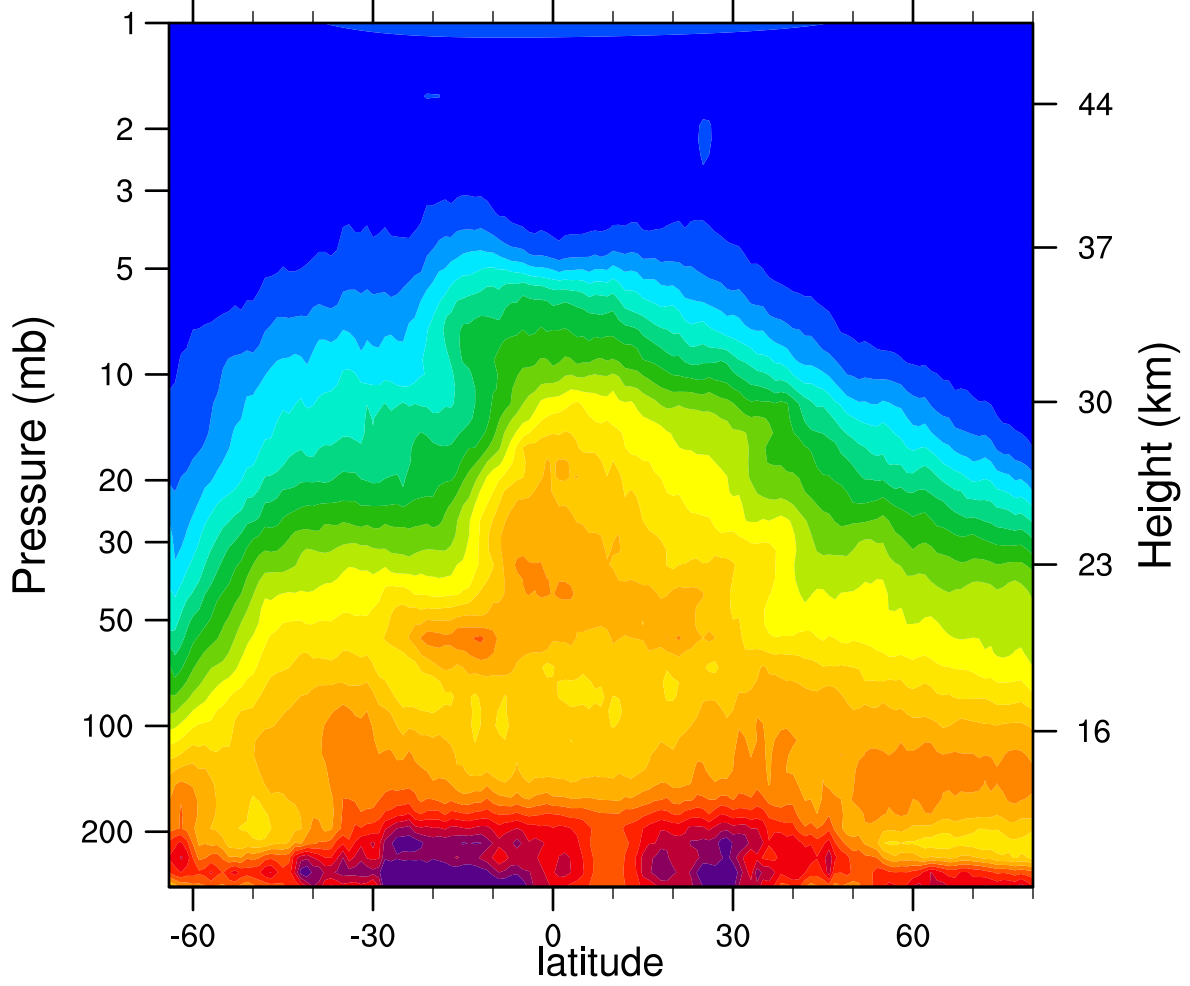
HIRDLSv6 2006d277 N2O_Combined (ppbv)
