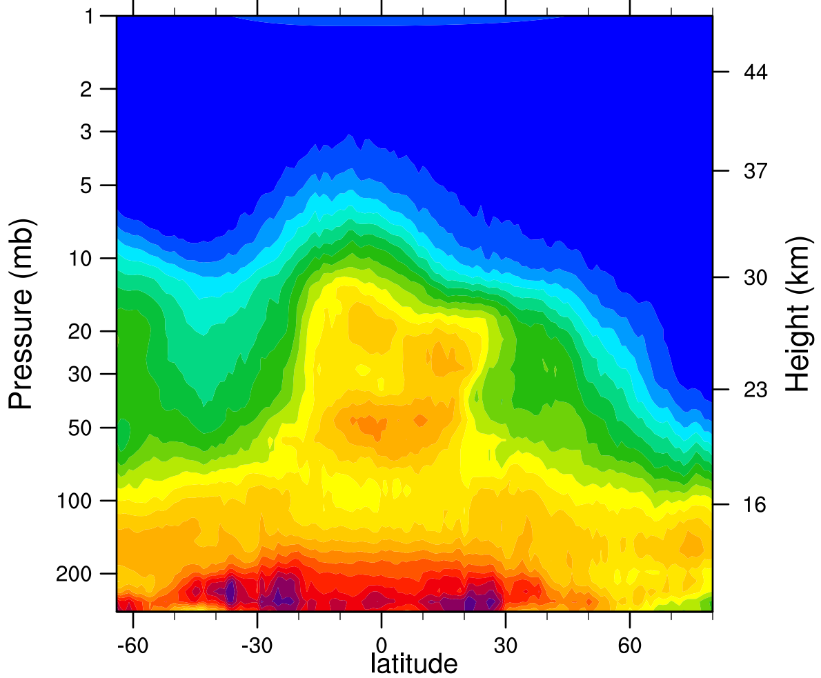
HIRDLSv6 2007d365 N2O_Combined (ppbv)
