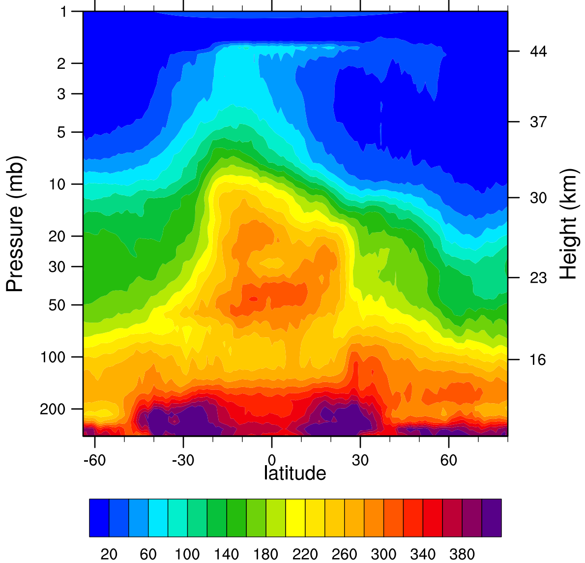
HIRDLSv6 2006d016 N2O_Combined (ppbv)
