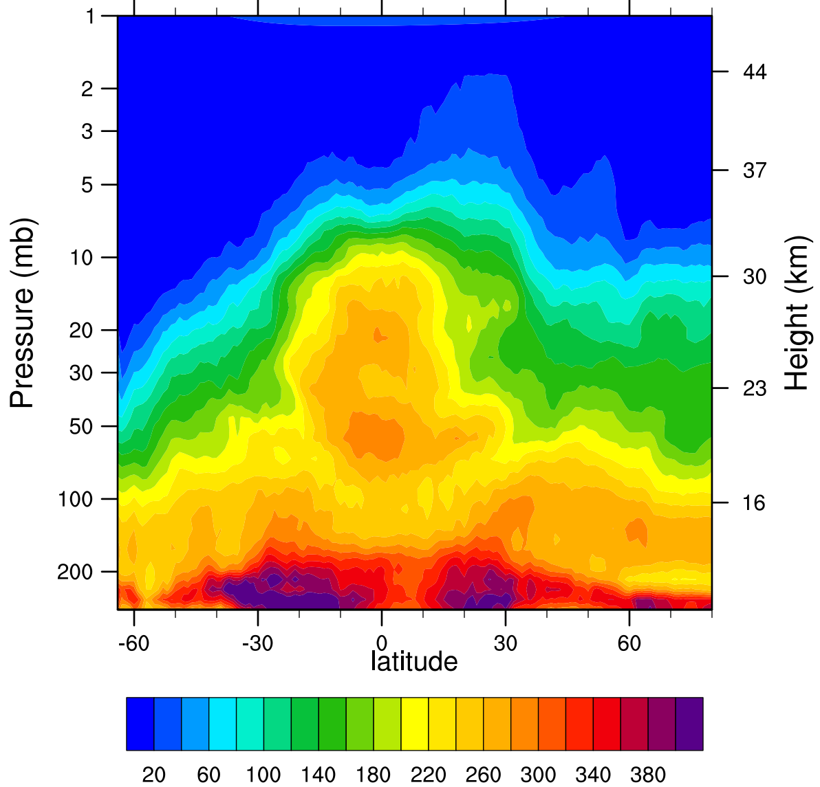
HIRDLSv6 2007d139 N2O_Combined (ppbv)
