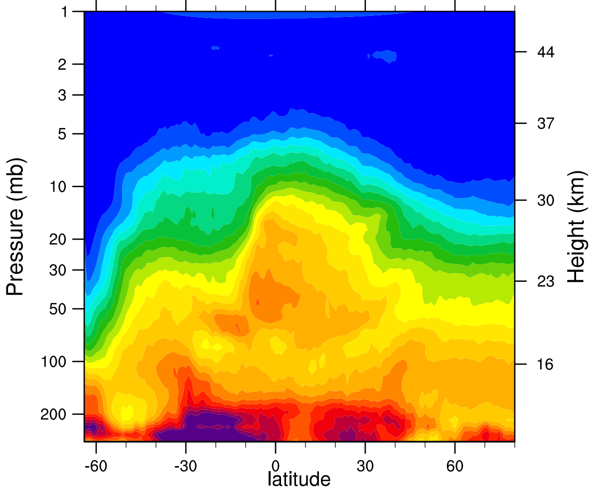
HIRDLSv6 2006d237 N2O_Combined (ppbv)
