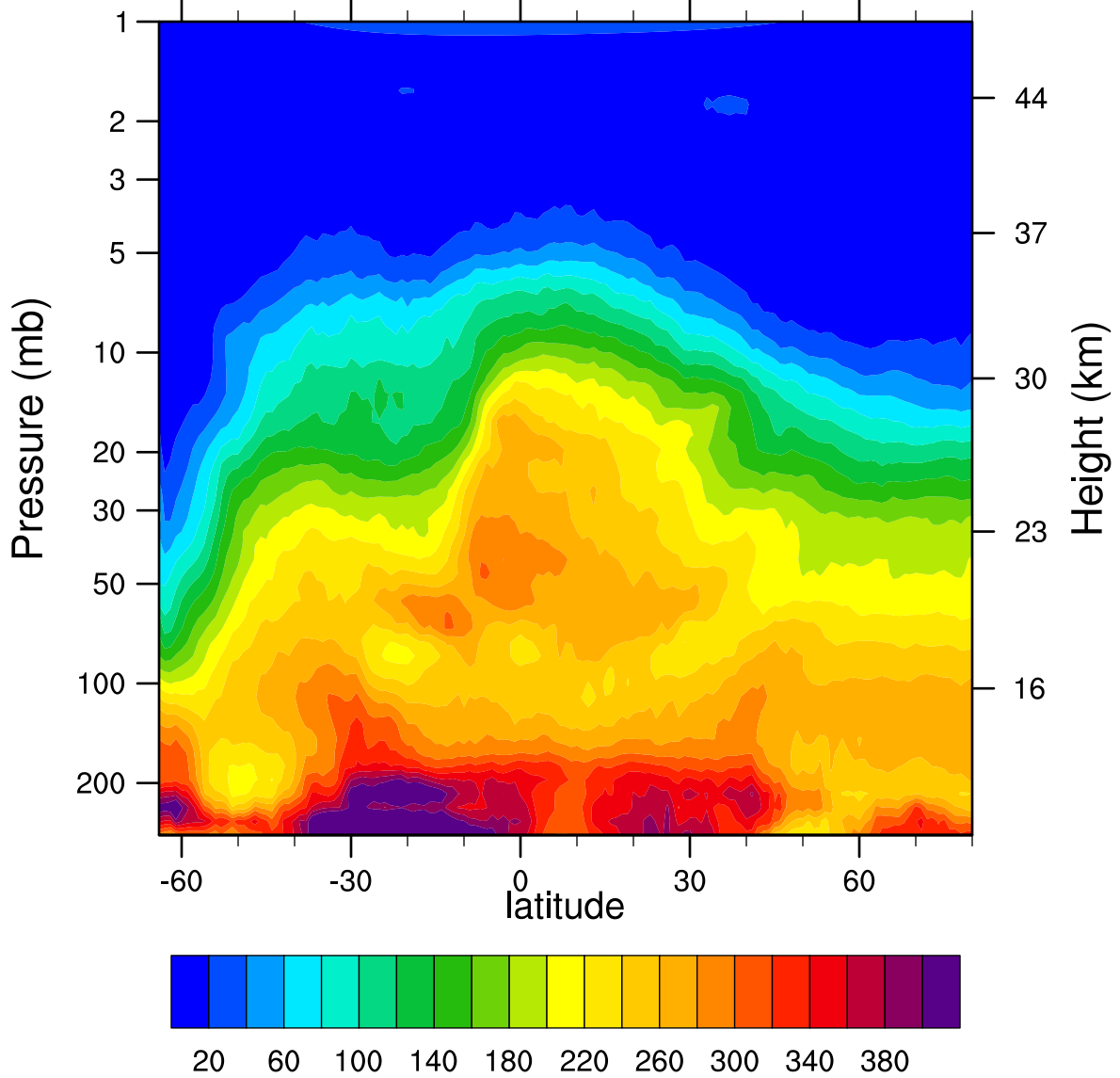
HIRDLSv6 2006d236 N2O_Combined (ppbv)
