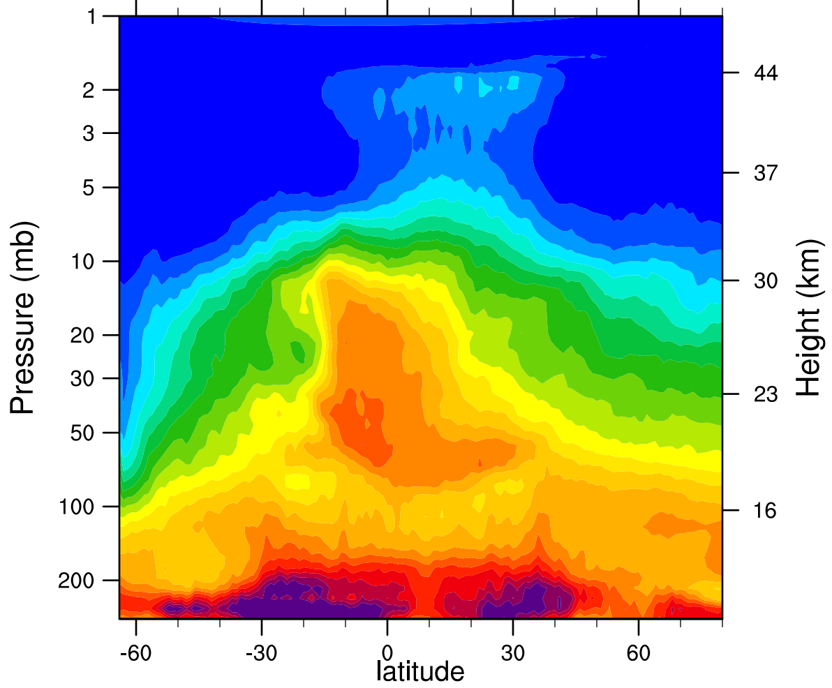
HIRDLSv6 2005d242 N2O_Combined (ppbv)
