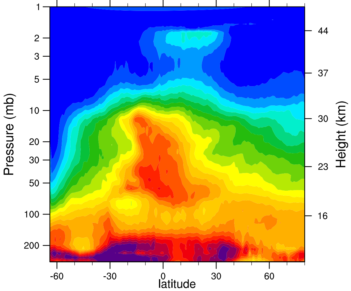
HIRDLSv6 2005d212 N2O_Combined (ppbv)
