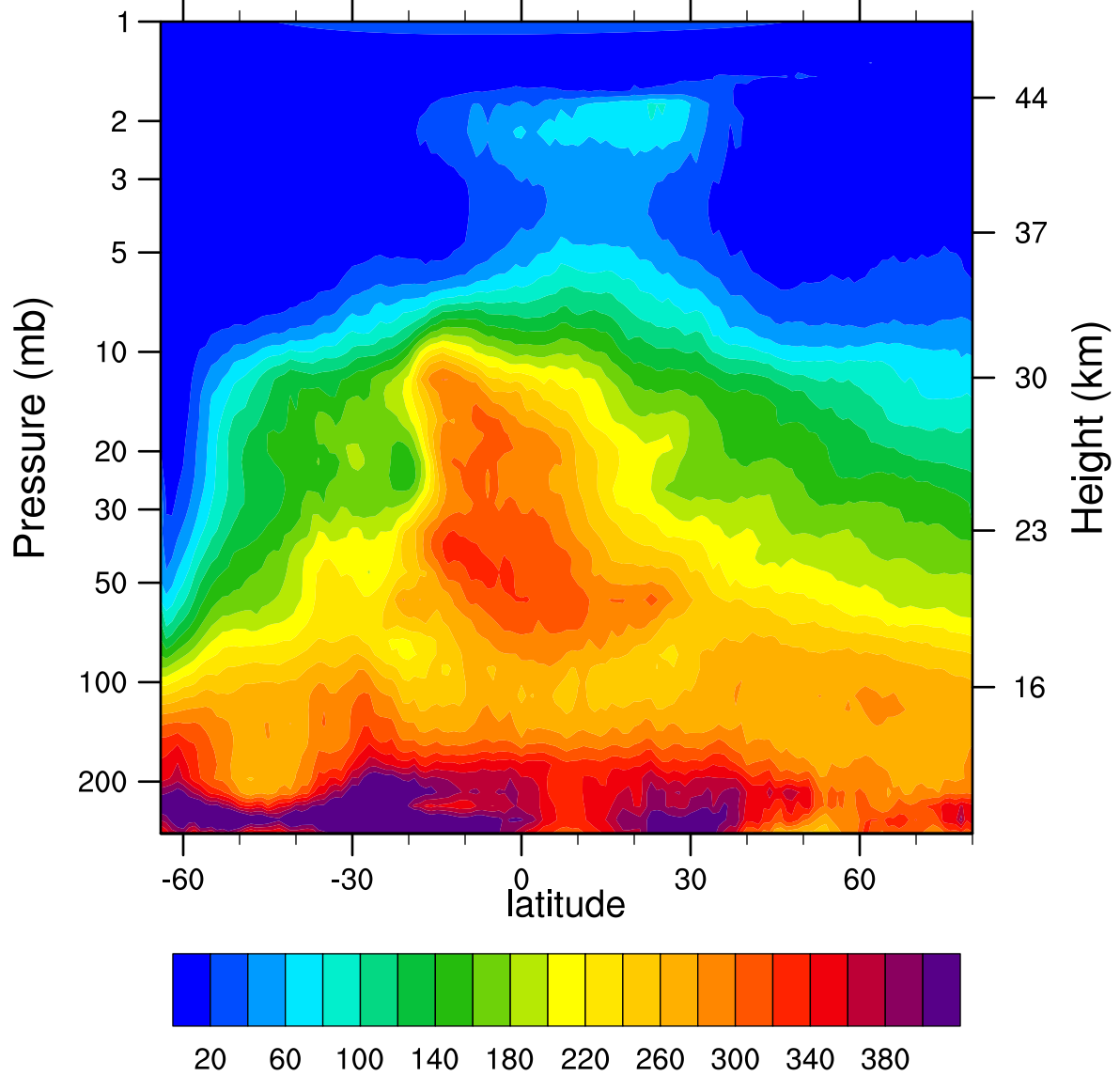
HIRDLSv6 2005d225 N2O_Combined (ppbv)
