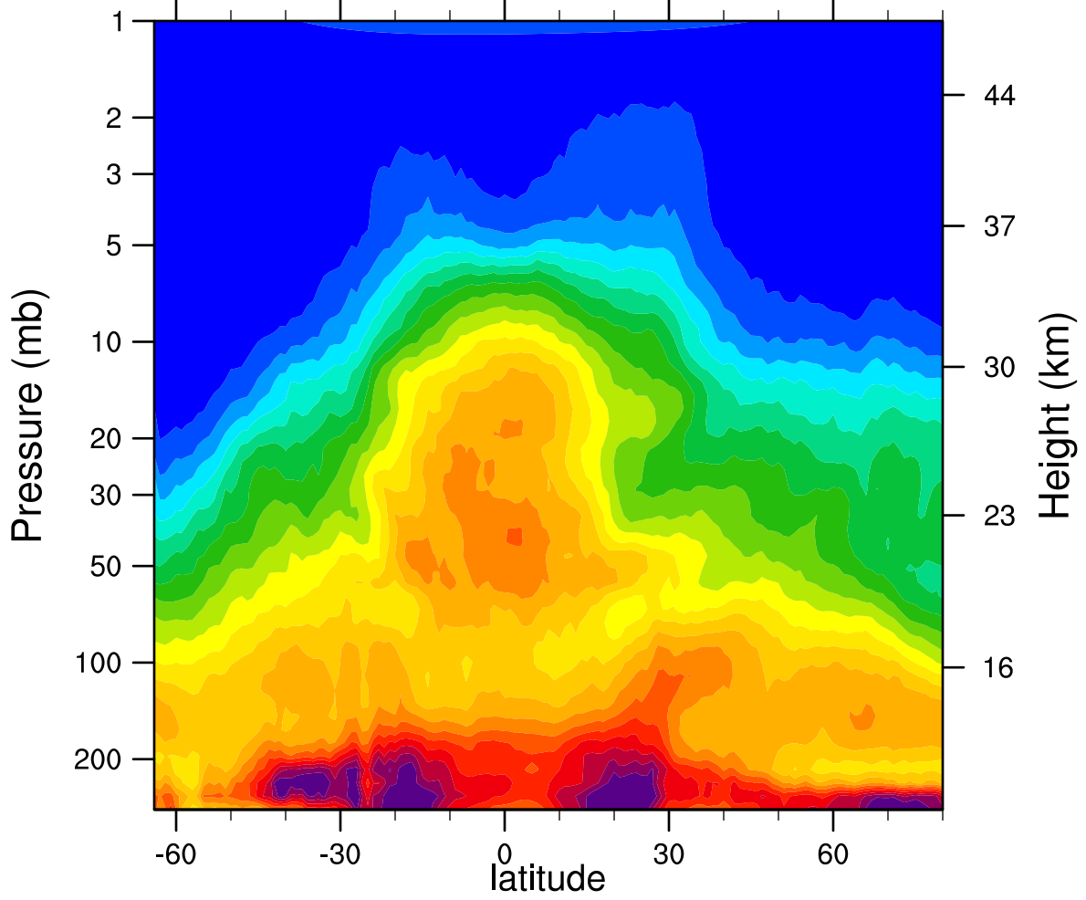
HIRDLSv6 2007d115 N2O_Combined (ppbv)
