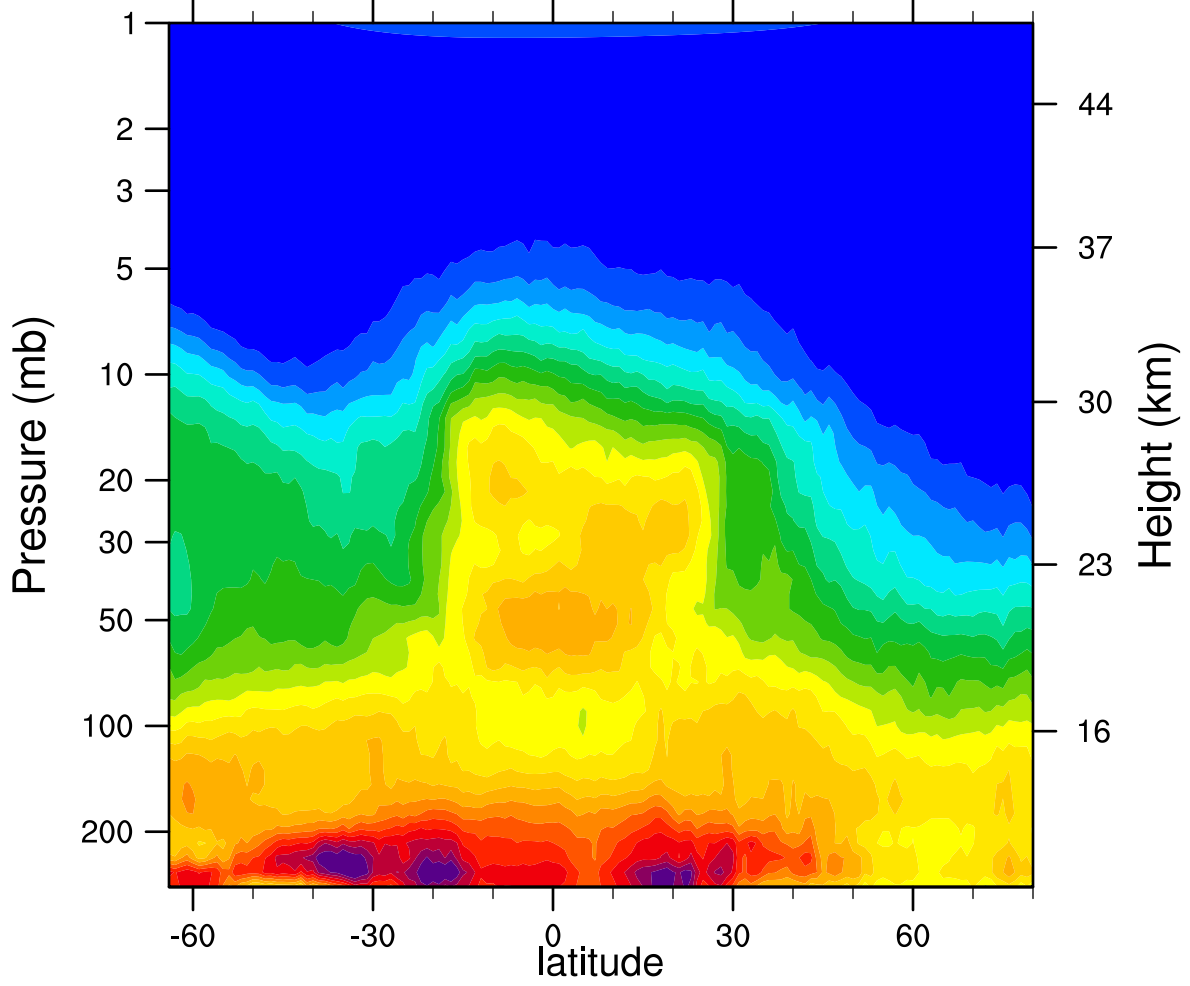
HIRDLSv6 2007d335 N2O_Combined (ppbv)
