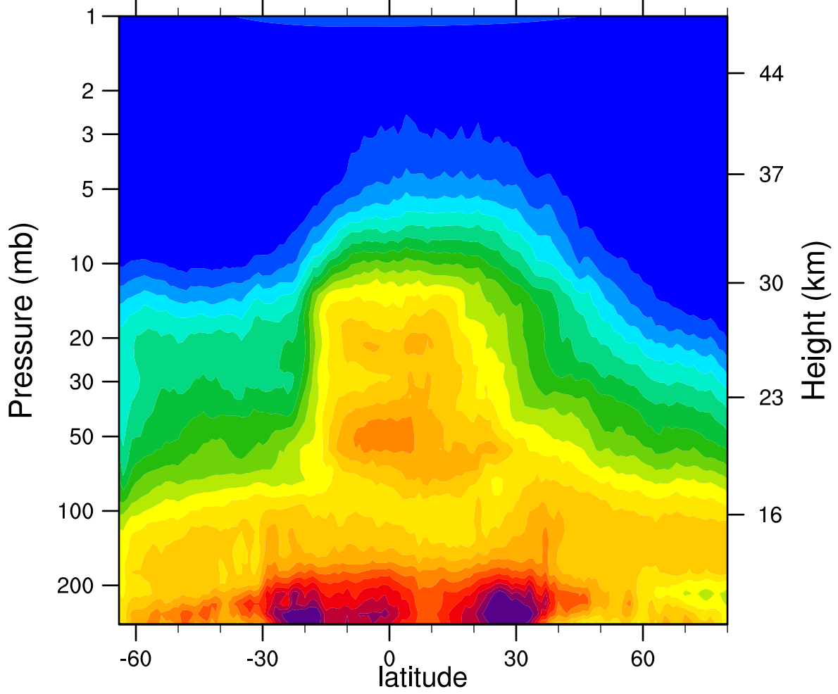
HIRDLSv6 2007d282 N2O_Combined (ppbv)
