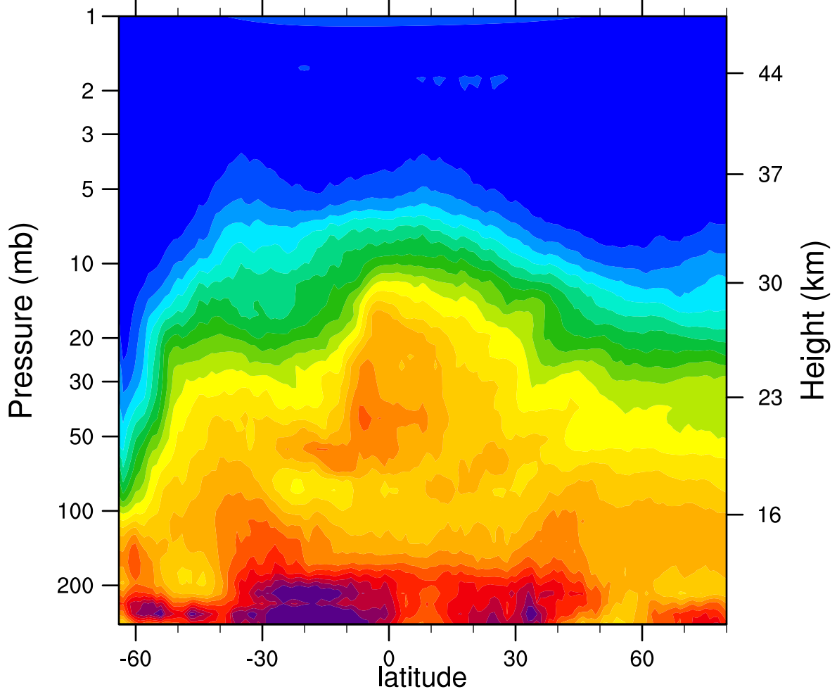
HIRDLSv6 2006d219 N2O_Combined (ppbv)
