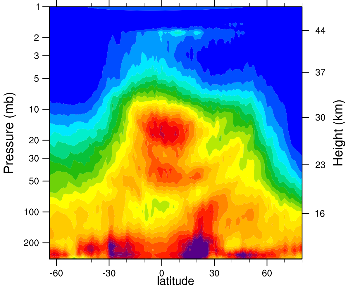
HIRDLSv6 2005d028 N2O_Combined (ppbv)
