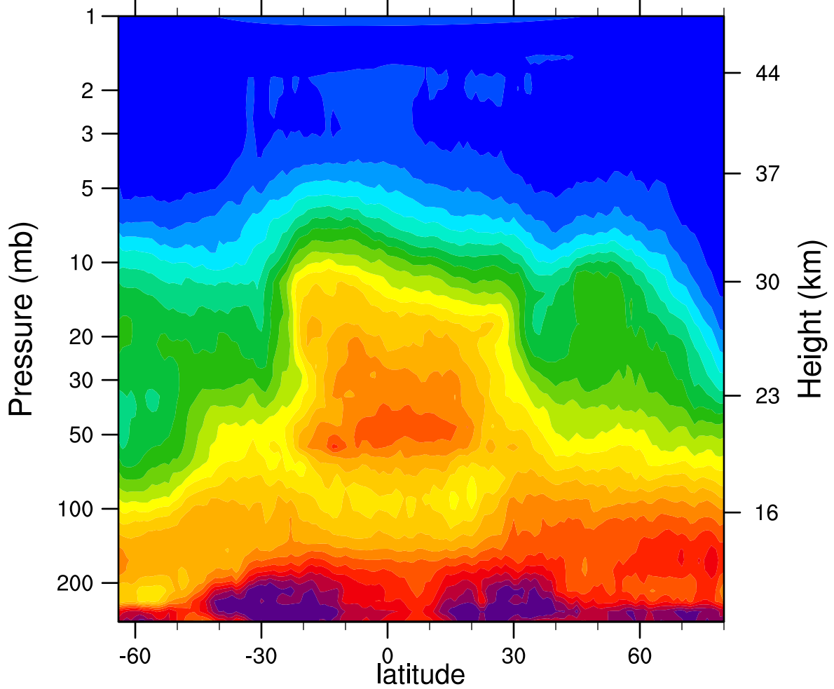
HIRDLSv6 2005d324 N2O_Combined (ppbv)
