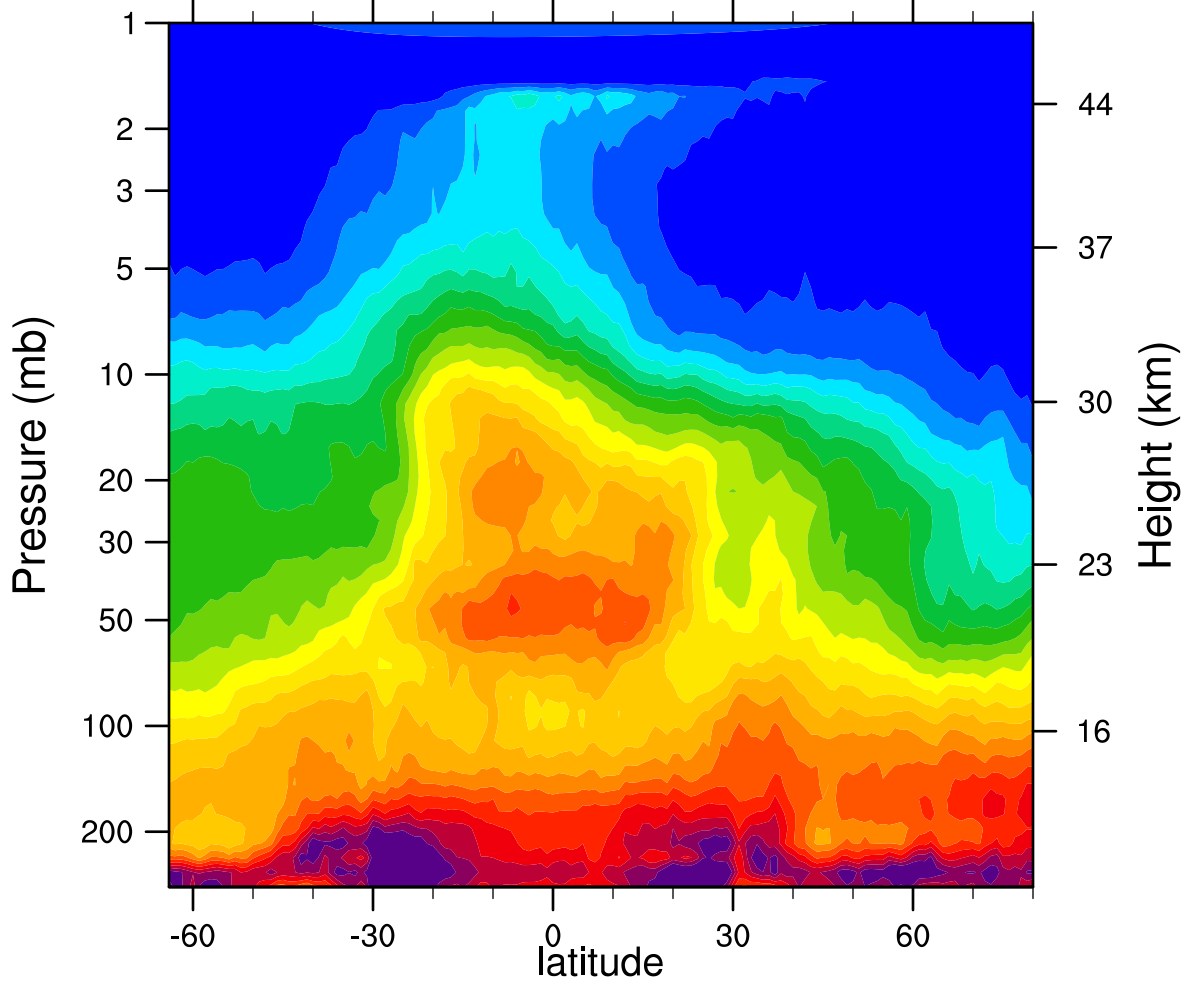
HIRDLSv6 2005d363 N2O_Combined (ppbv)
