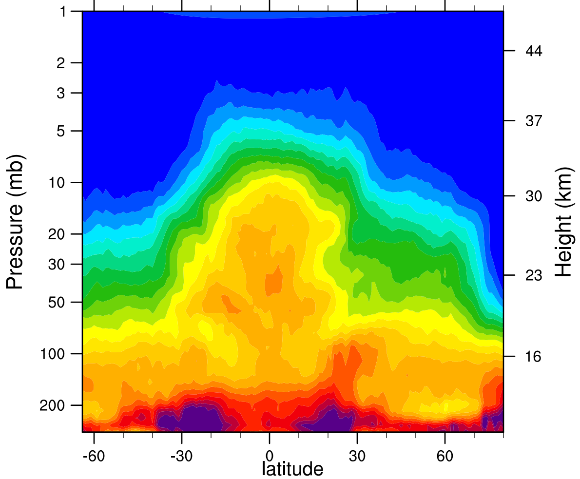
HIRDLSv6 2007d083 N2O_Combined (ppbv)
