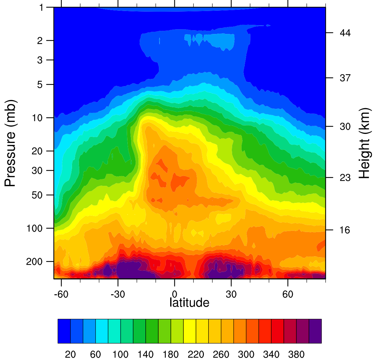
HIRDLSv6 2005d277 N2O_Combined (ppbv)
