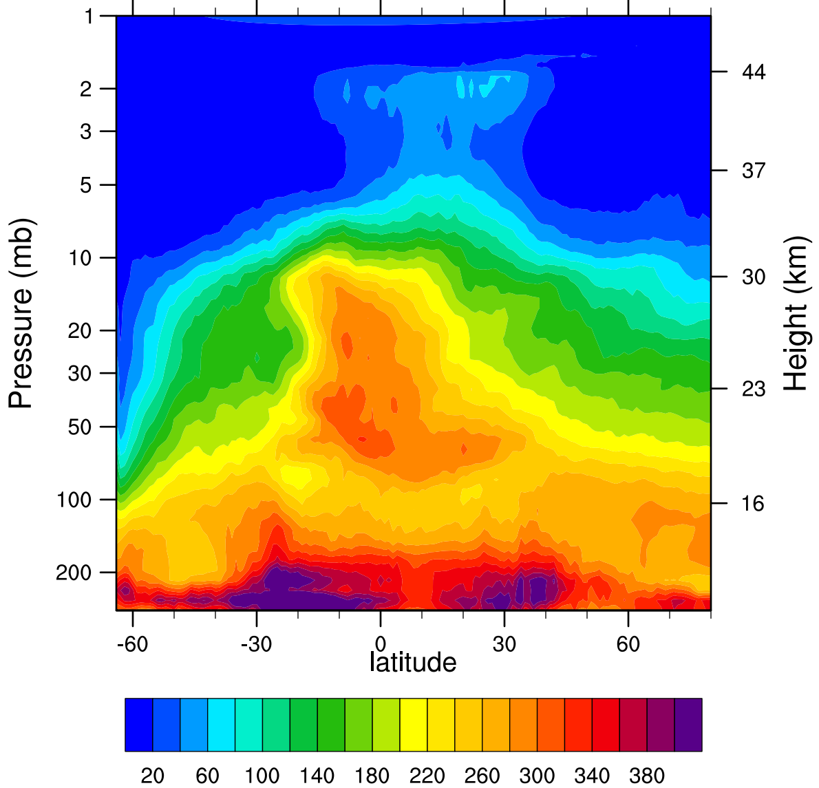
HIRDLSv6 2005d237 N2O_Combined (ppbv)
