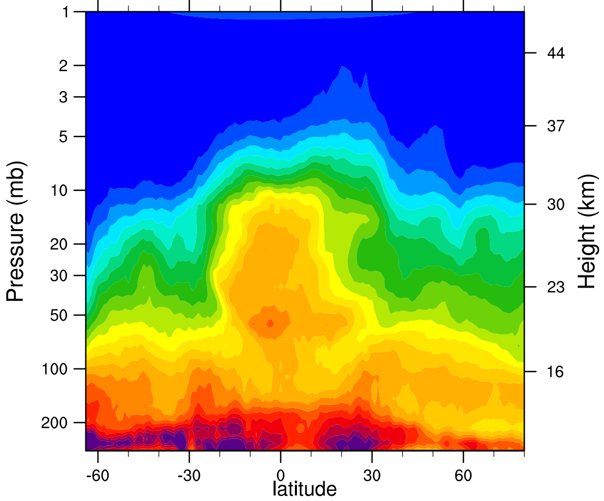
HIRDLSv6 2007d154 N2O_Combined (ppbv)
