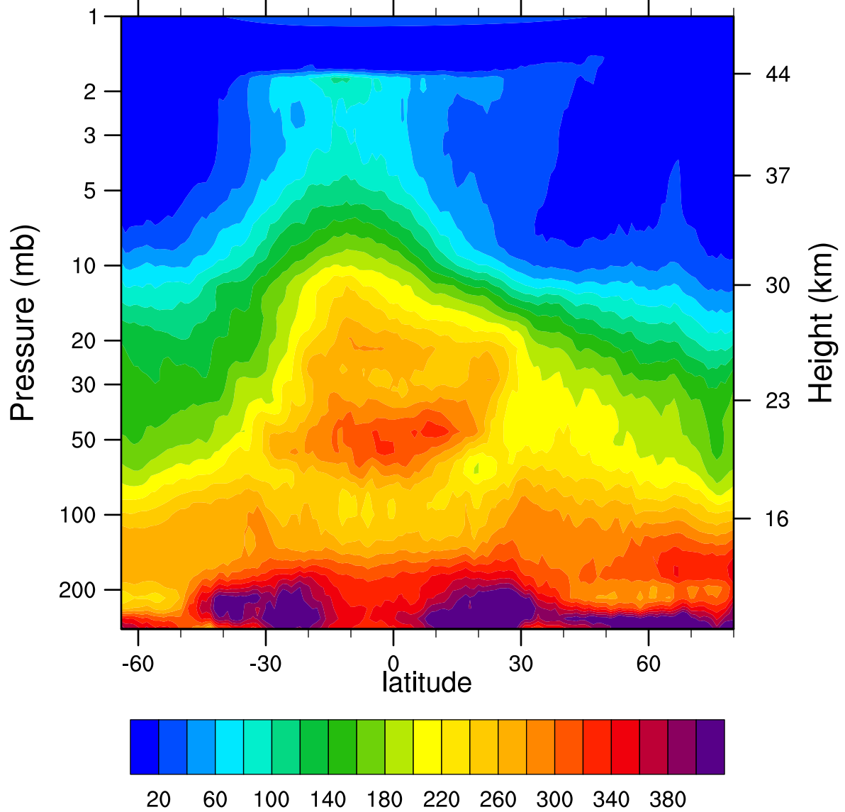
HIRDLSv6 2006d059 N2O_Combined (ppbv)
