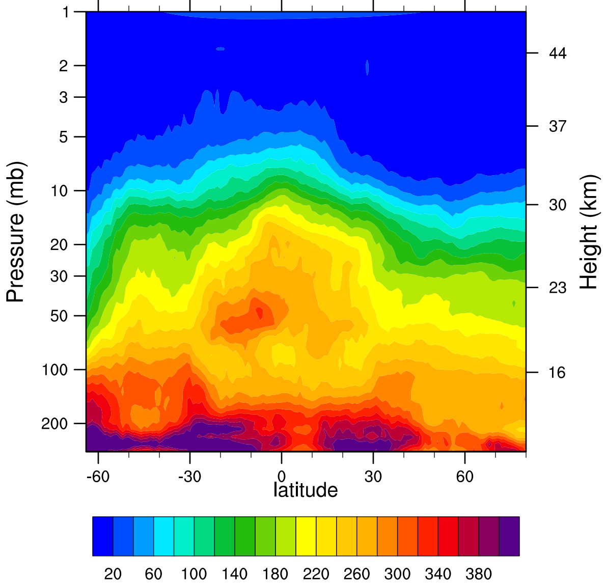
HIRDLSv6 2006d167 N2O_Combined (ppbv)
