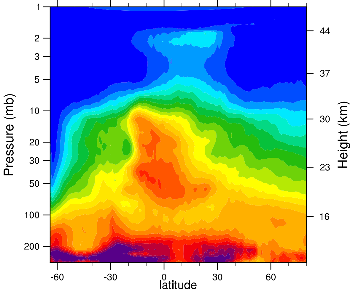
HIRDLSv6 2005d226 N2O_Combined (ppbv)
