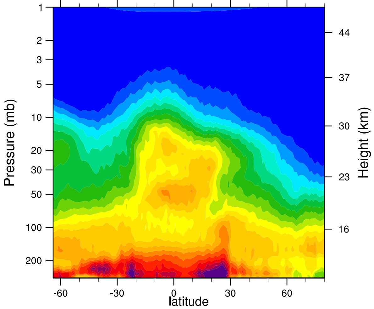
HIRDLSv6 2007d354 N2O_Combined (ppbv)
