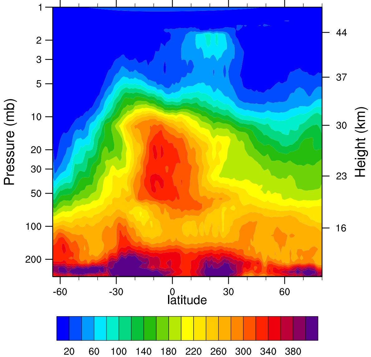
HIRDLSv6 2005d167 N2O_Combined (ppbv)
