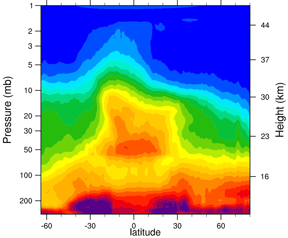
HIRDLSv6 2005d350 N2O_Combined (ppbv)
