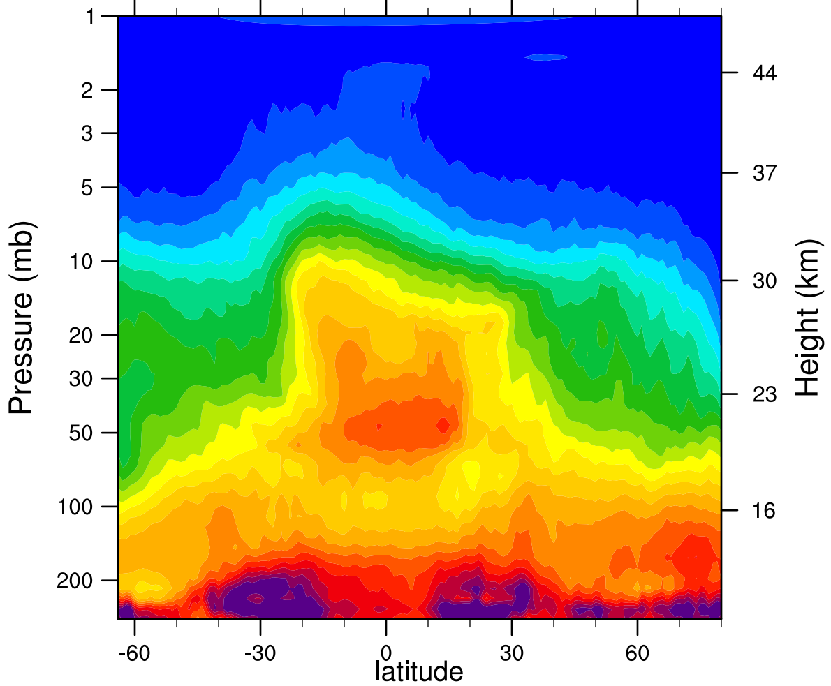
HIRDLSv6 2005d336 N2O_Combined (ppbv)
