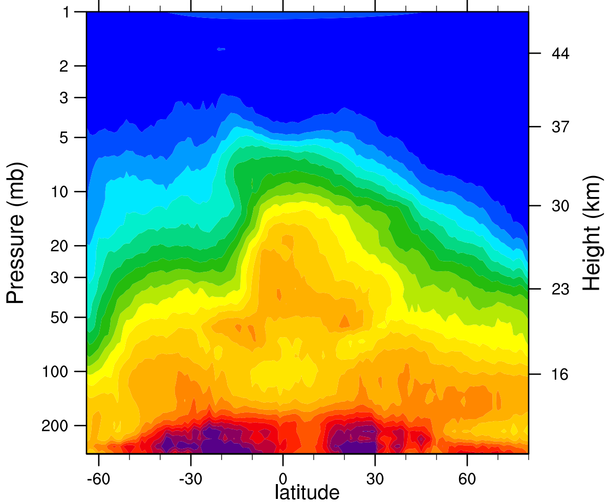
HIRDLSv6 2006d289 N2O_Combined (ppbv)
