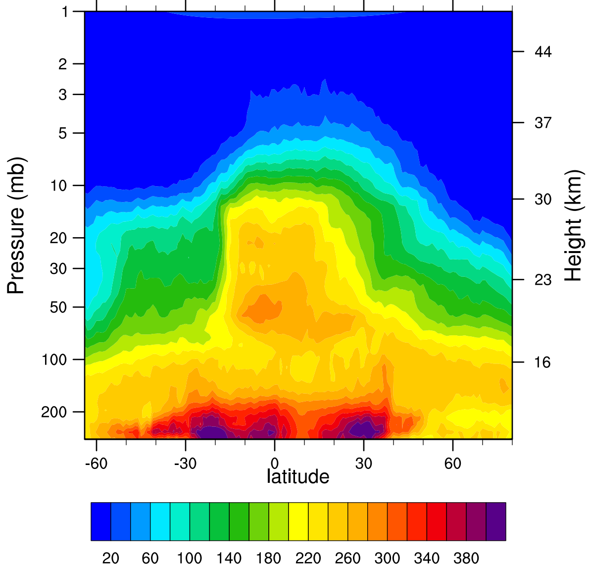
HIRDLSv6 2007d277 N2O_Combined (ppbv)
