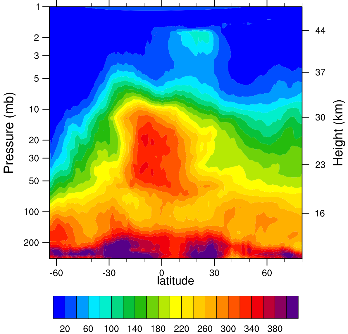
HIRDLSv6 2005d164 N2O_Combined (ppbv)
