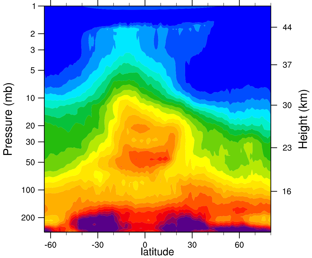
HIRDLSv6 2006d039 N2O_Combined (ppbv)
