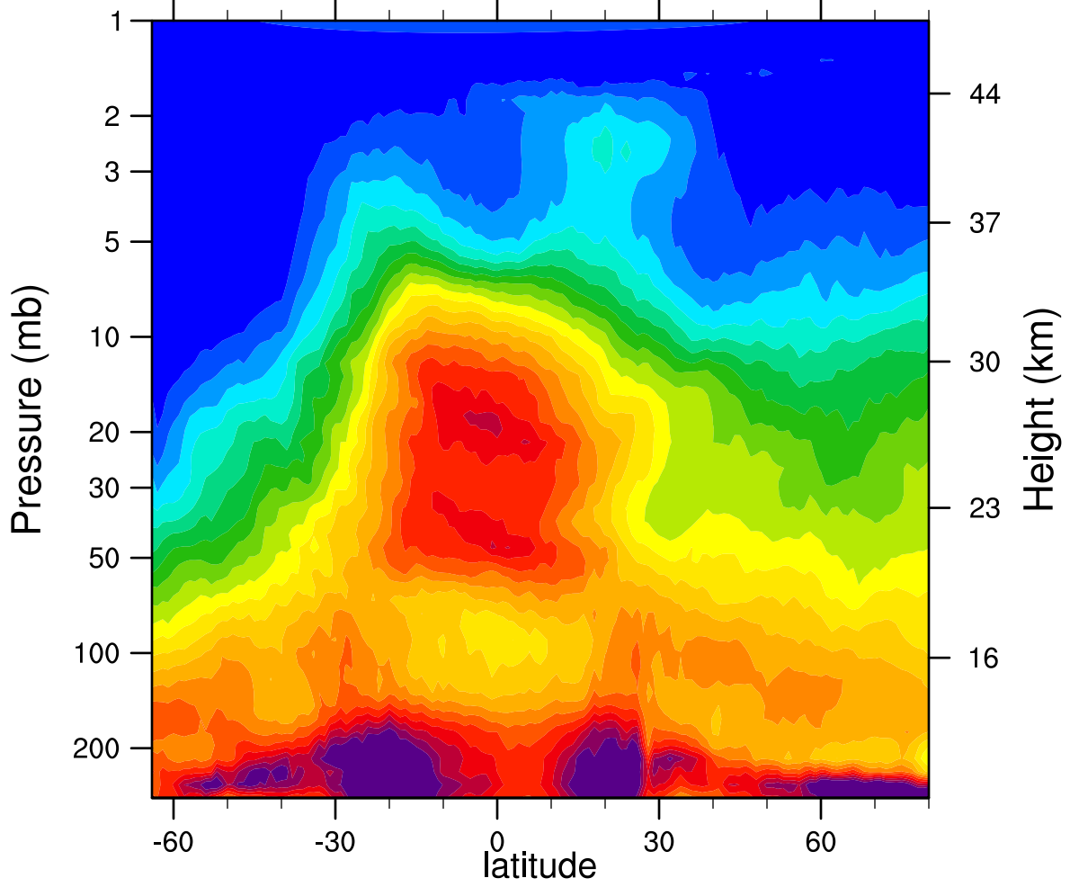
HIRDLSv6 2005d119 N2O_Combined (ppbv)
