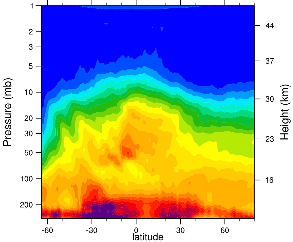
HIRDLSv6 2006d178 N2O_Combined (ppbv)
