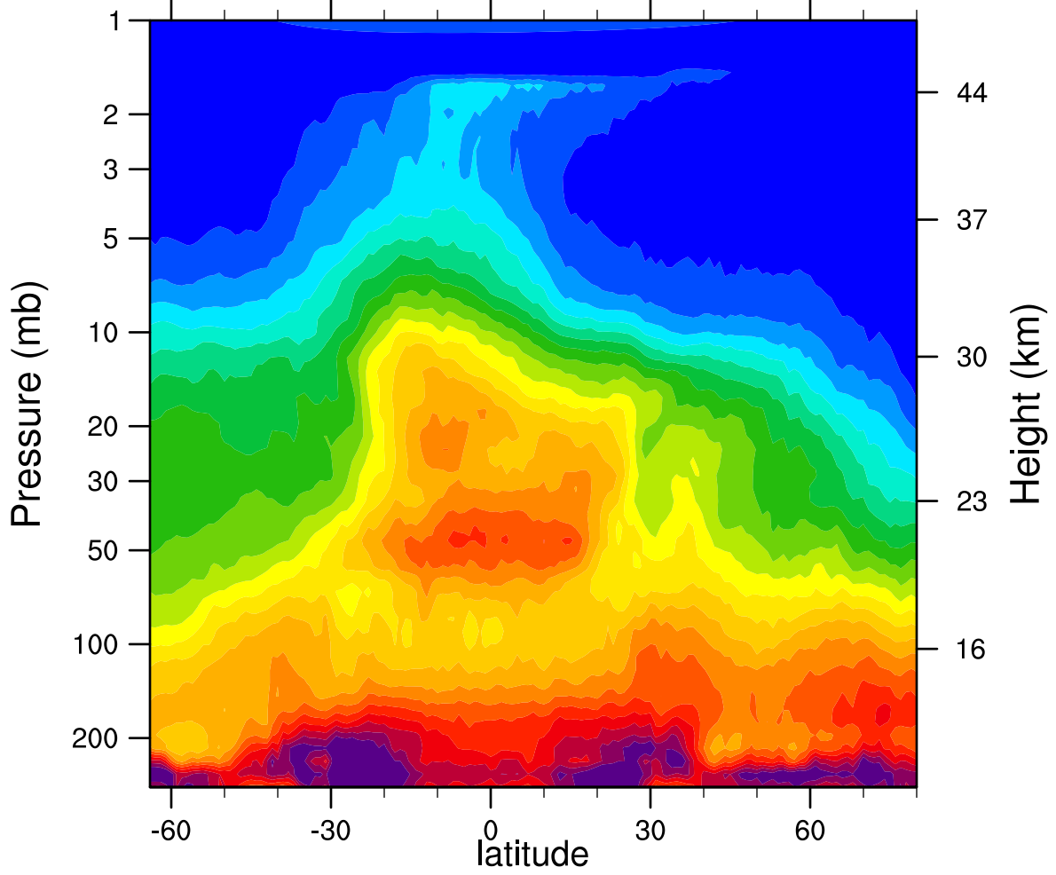
HIRDLSv6 2005d360 N2O_Combined (ppbv)
