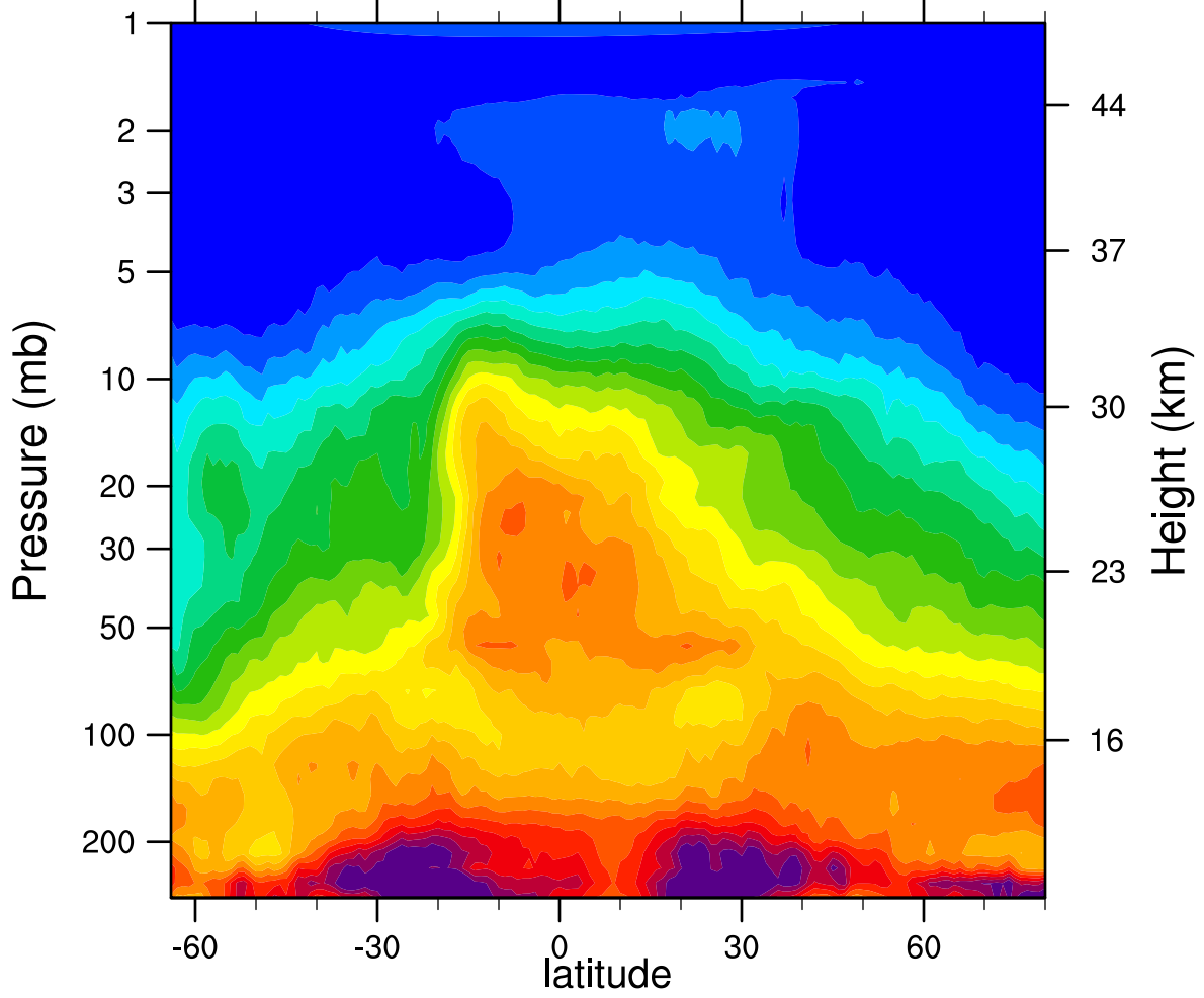
HIRDLSv6 2005d285 N2O_Combined (ppbv)
