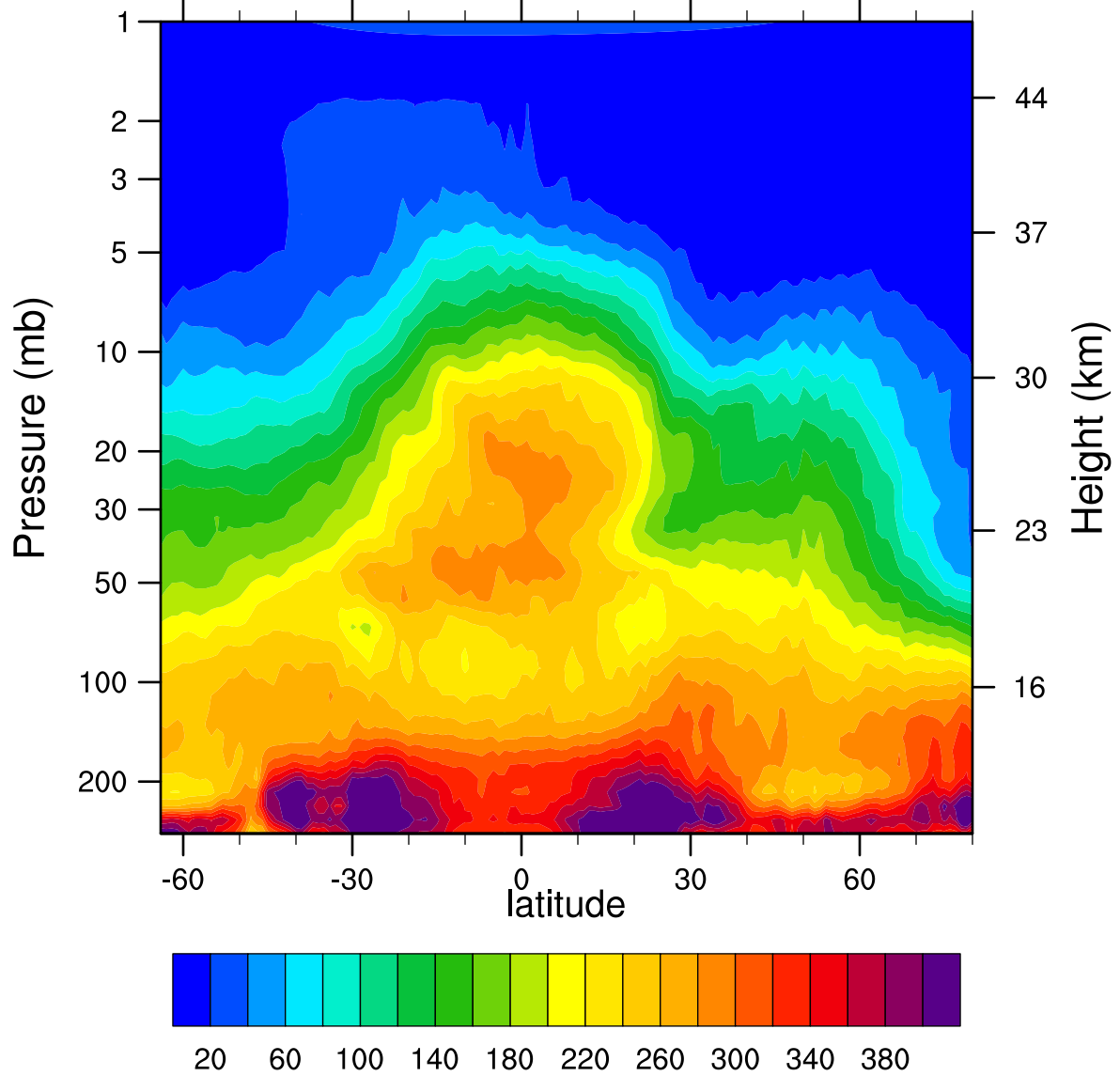
HIRDLSv6 2007d035 N2O_Combined (ppbv)
