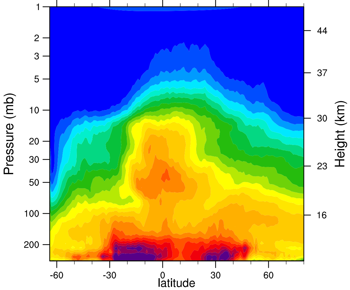
HIRDLSv6 2007d216 N2O_Combined (ppbv)
