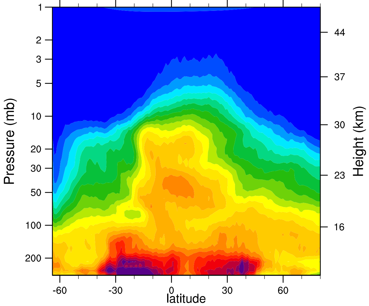
HIRDLSv6 2007d246 N2O_Combined (ppbv)
