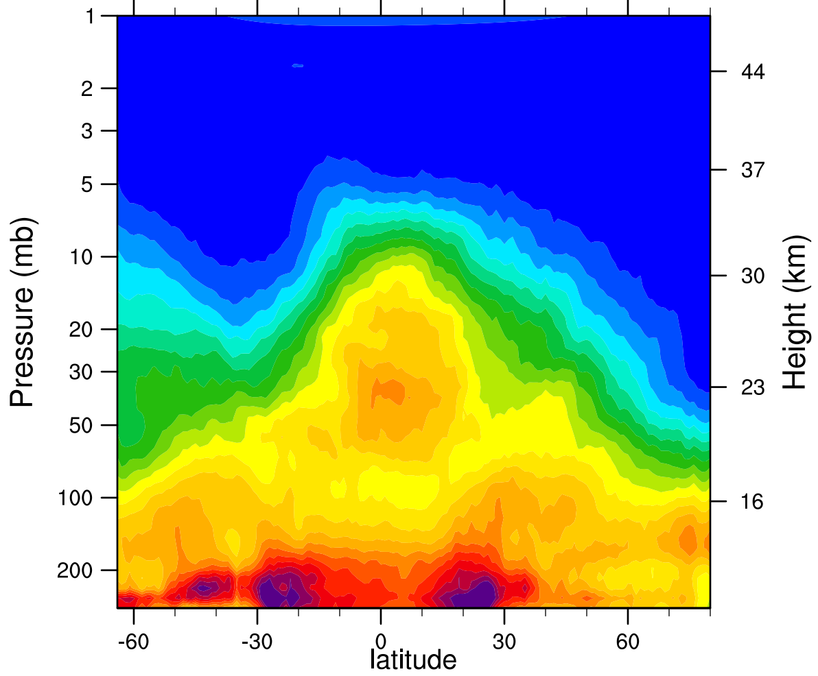
HIRDLSv6 2006d347 N2O_Combined (ppbv)
