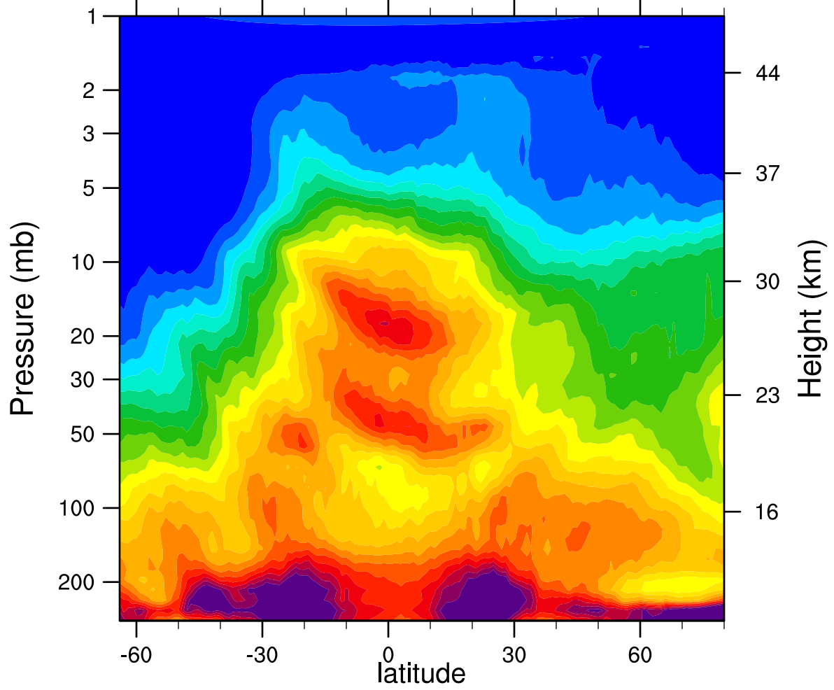
HIRDLSv6 2005d097 N2O_Combined (ppbv)
