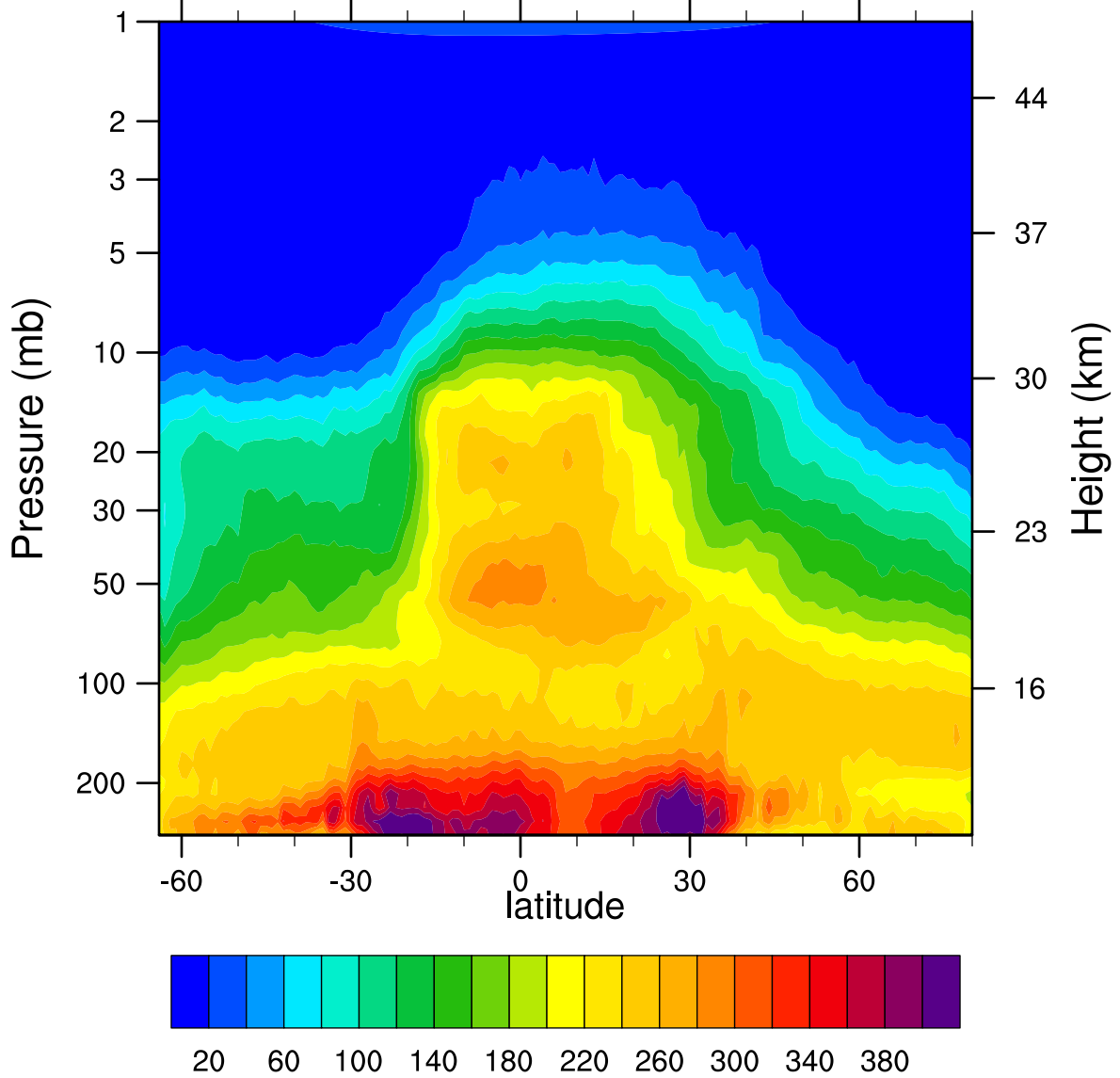
HIRDLSv6 2007d280 N2O_Combined (ppbv)
