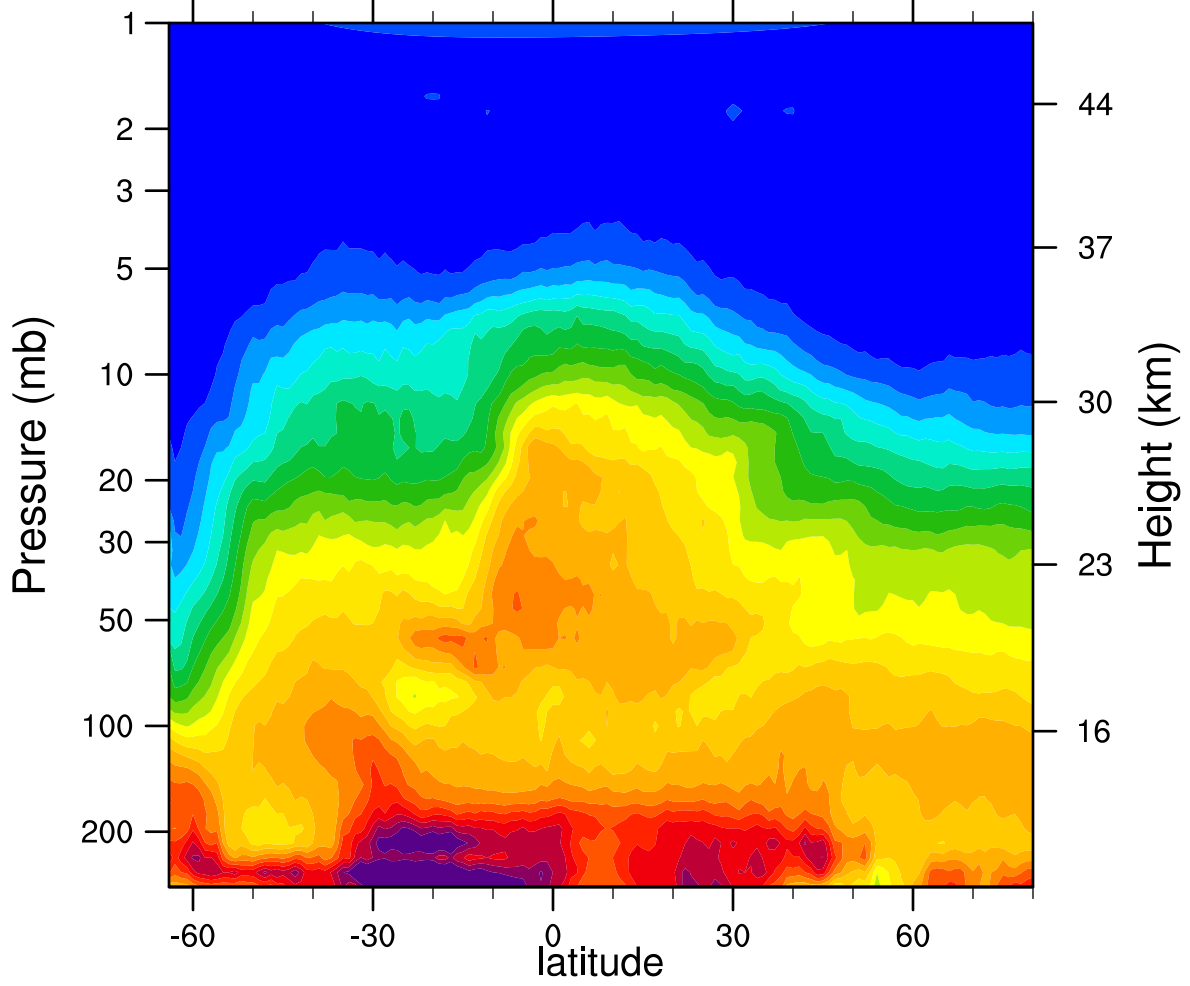
HIRDLSv6 2006d231 N2O_Combined (ppbv)
