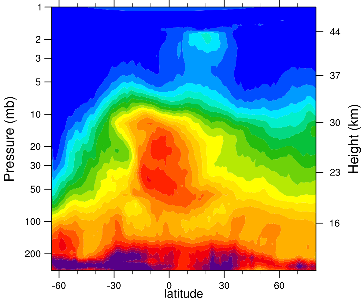
HIRDLSv6 2005d181 N2O_Combined (ppbv)
