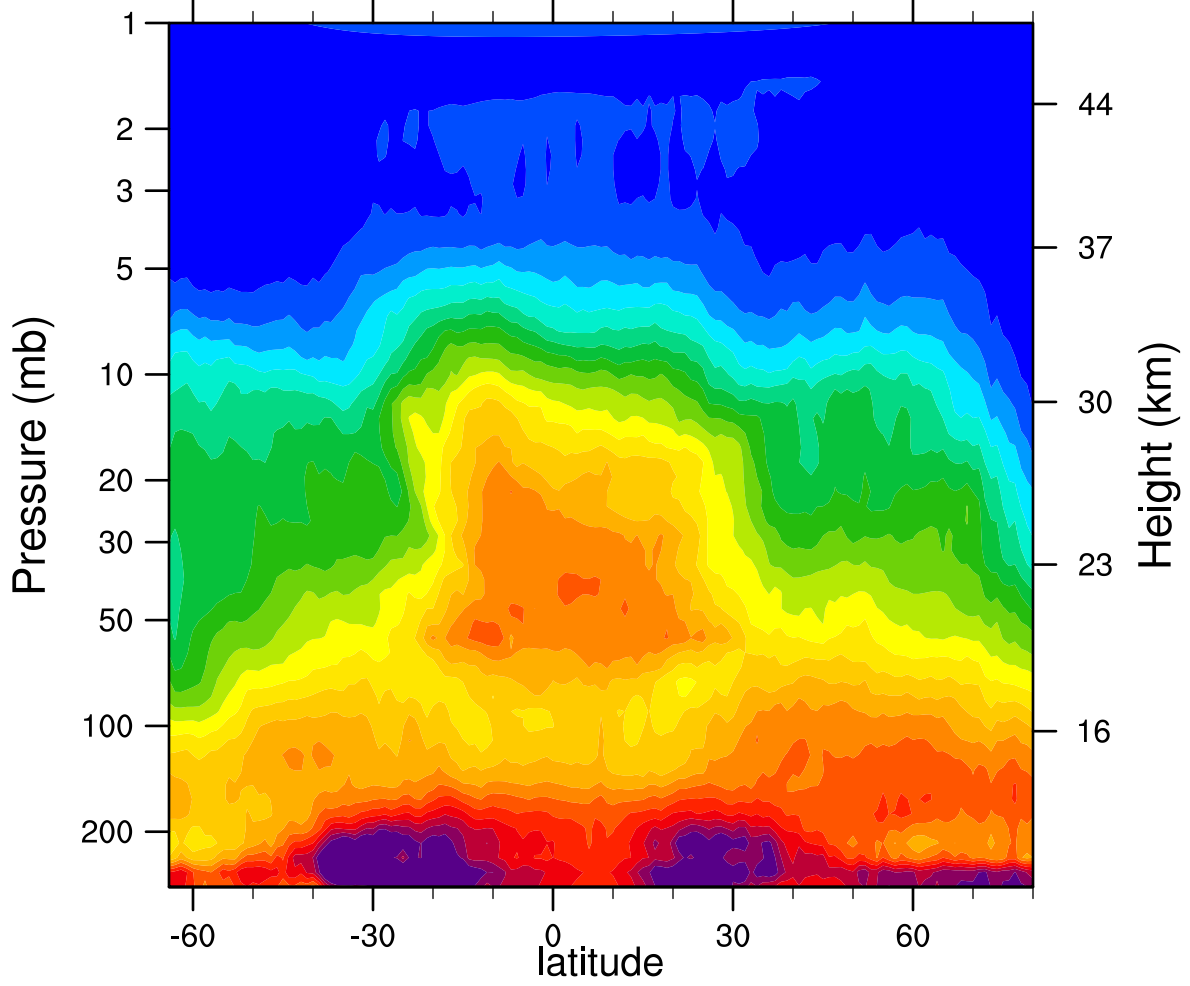
HIRDLSv6 2005d313 N2O_Combined (ppbv)
