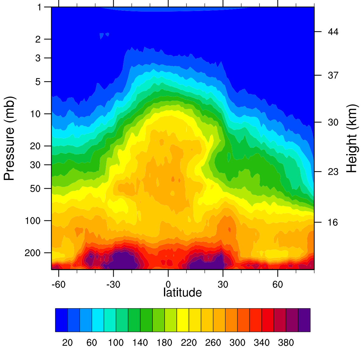
HIRDLSv6 2007d067 N2O_Combined (ppbv)
