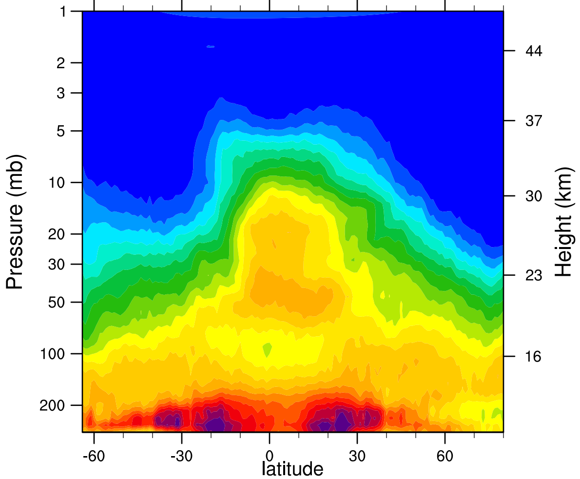
HIRDLSv6 2006d316 N2O_Combined (ppbv)
