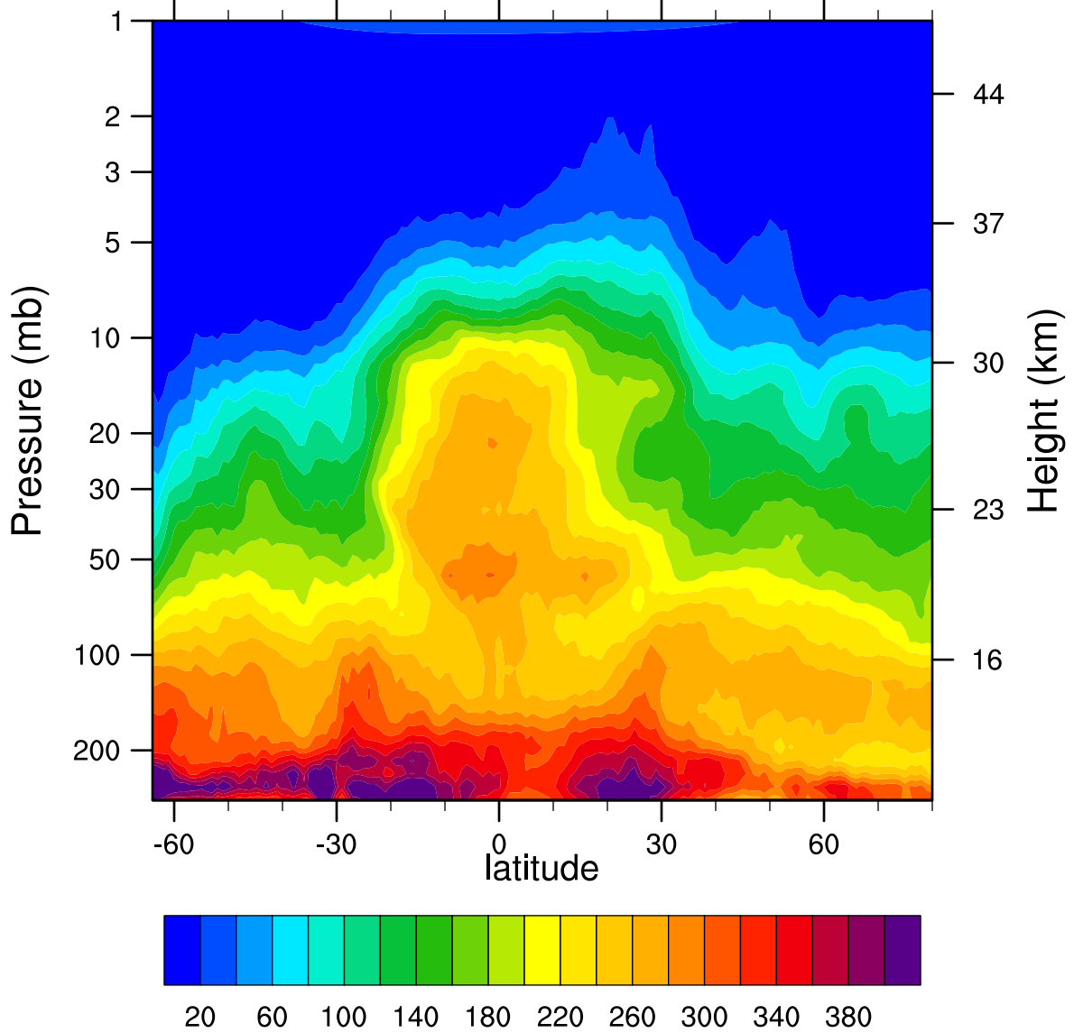
HIRDLSv6 2007d153 N2O_Combined (ppbv)
