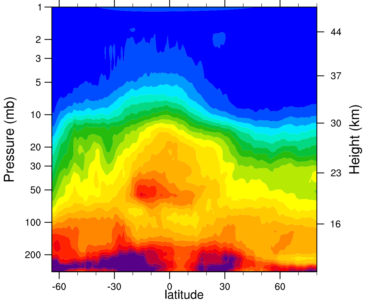
HIRDLSv6 2006d147 N2O_Combined (ppbv)
