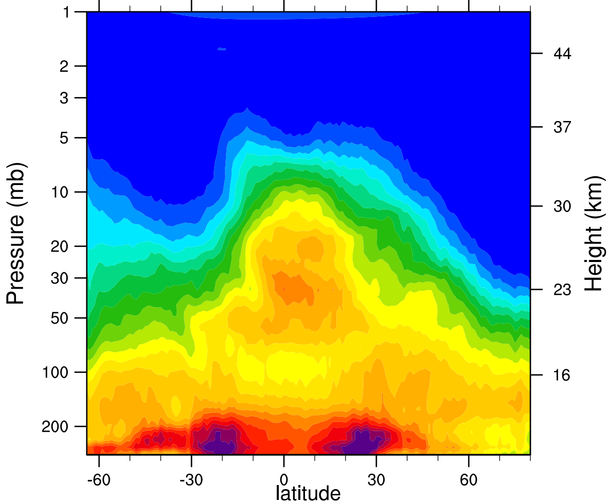
HIRDLSv6 2006d334 N2O_Combined (ppbv)
