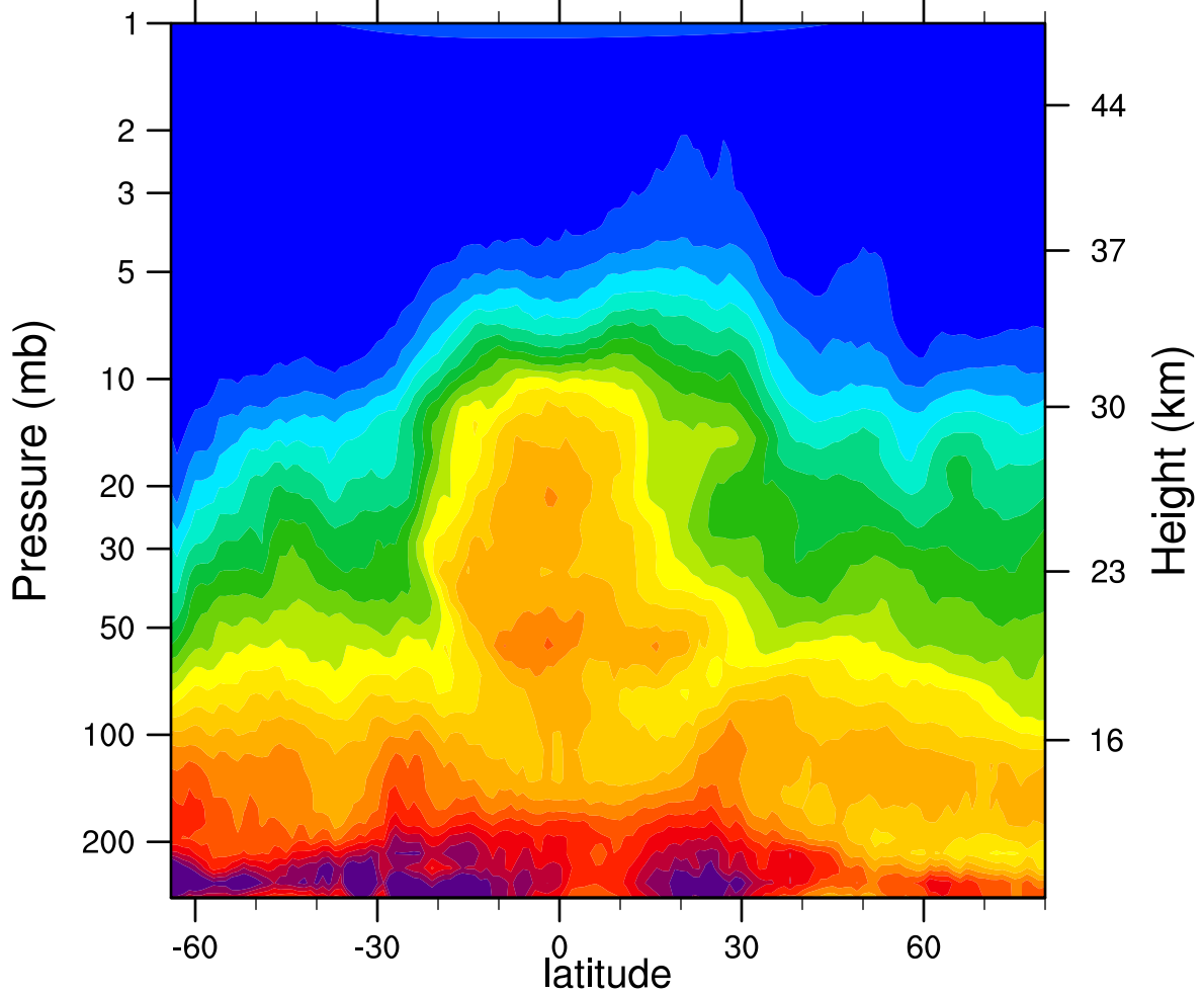
HIRDLSv6 2007d152 N2O_Combined (ppbv)
