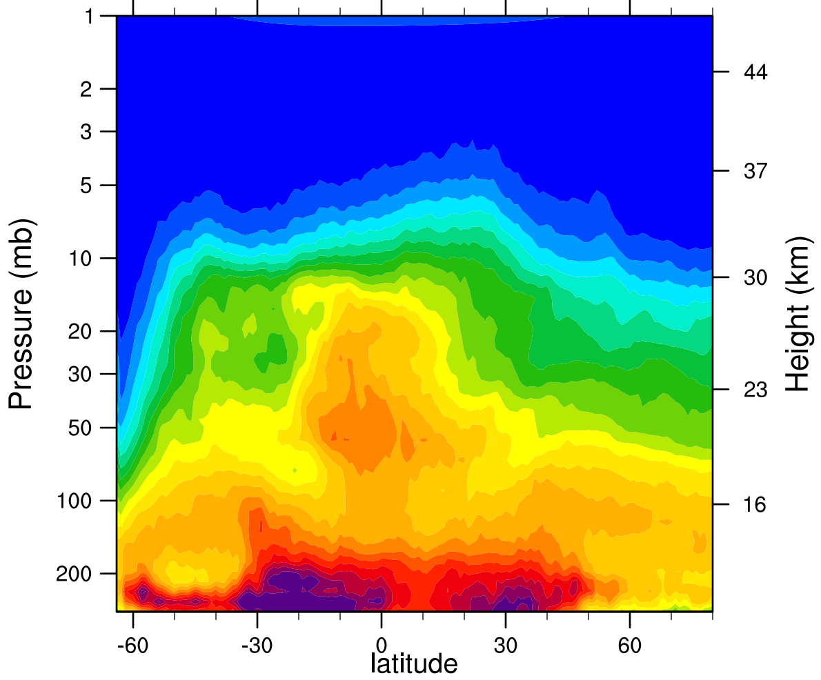
HIRDLSv6 2007d200 N2O_Combined (ppbv)
