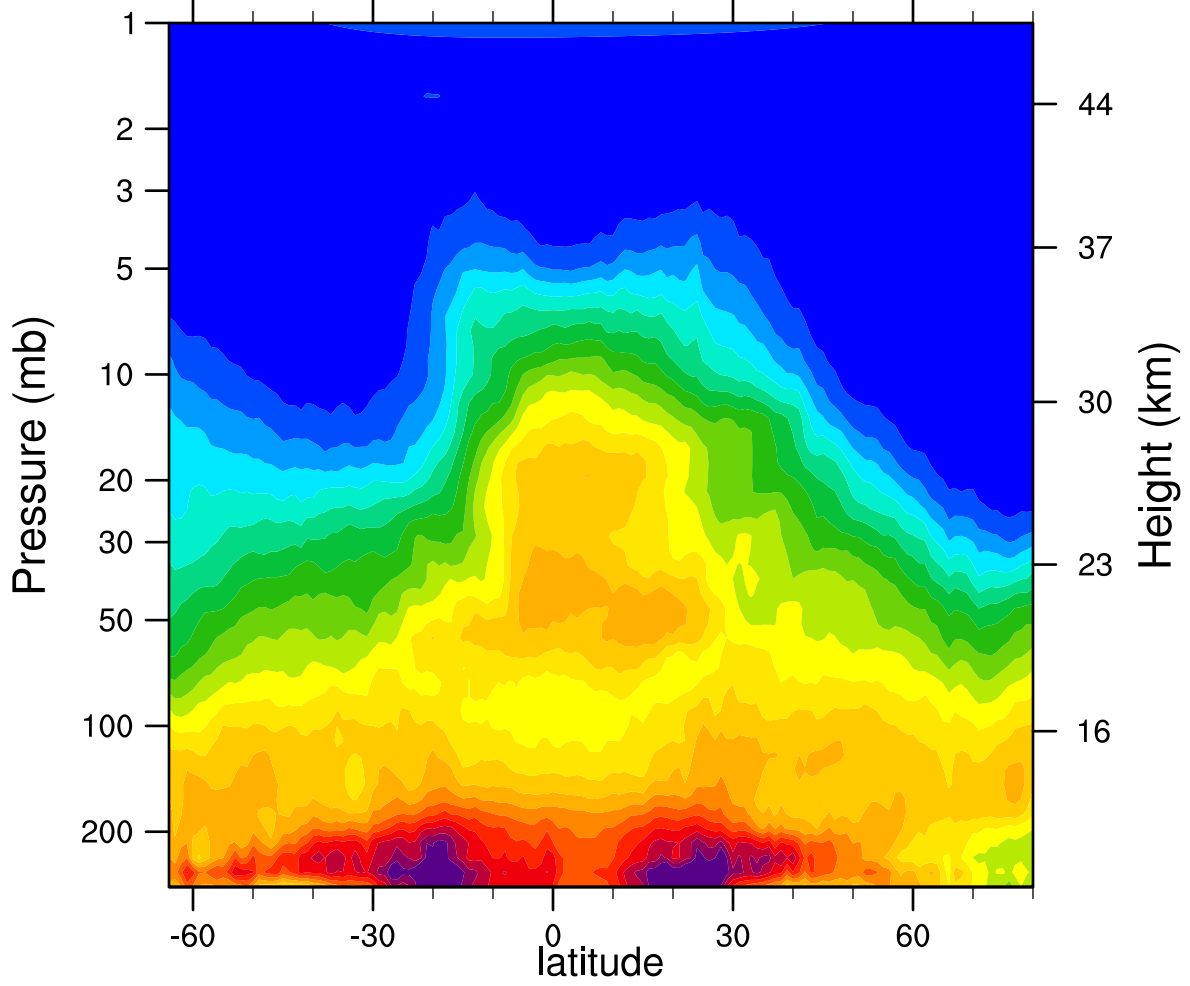
HIRDLSv6 2006d321 N2O_Combined (ppbv)
