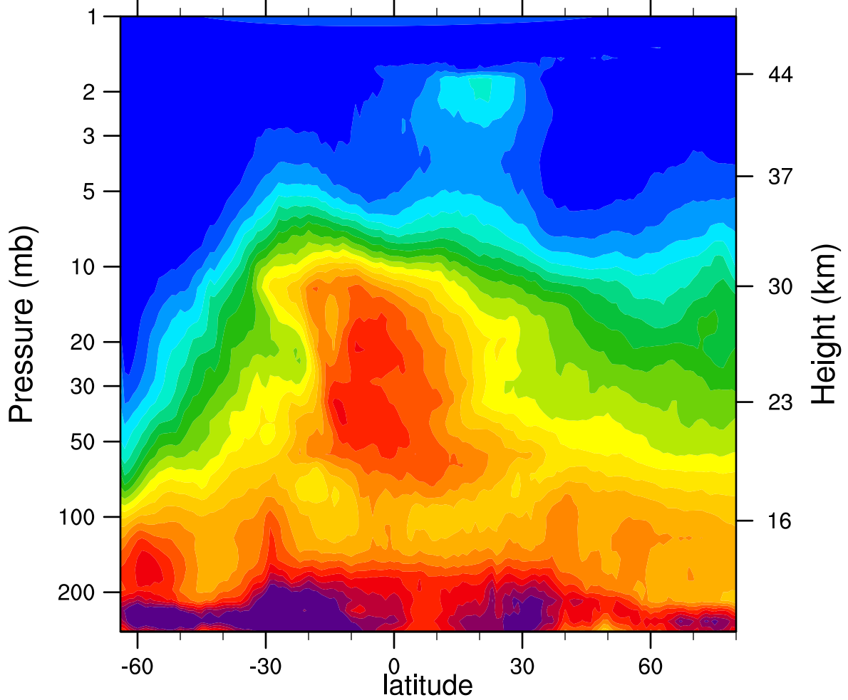
HIRDLSv6 2005d178 N2O_Combined (ppbv)
