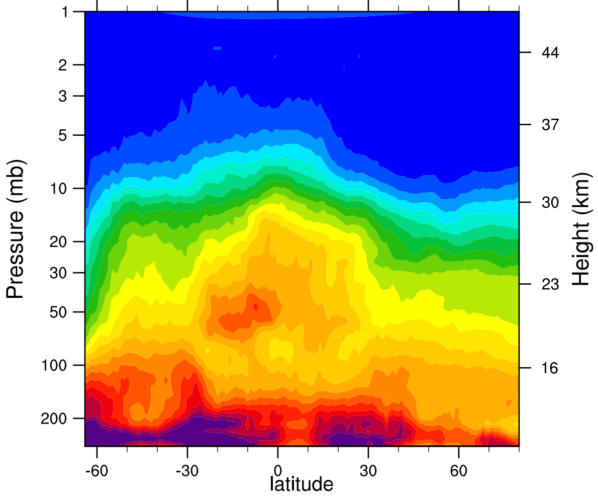
HIRDLSv6 2006d166 N2O_Combined (ppbv)
