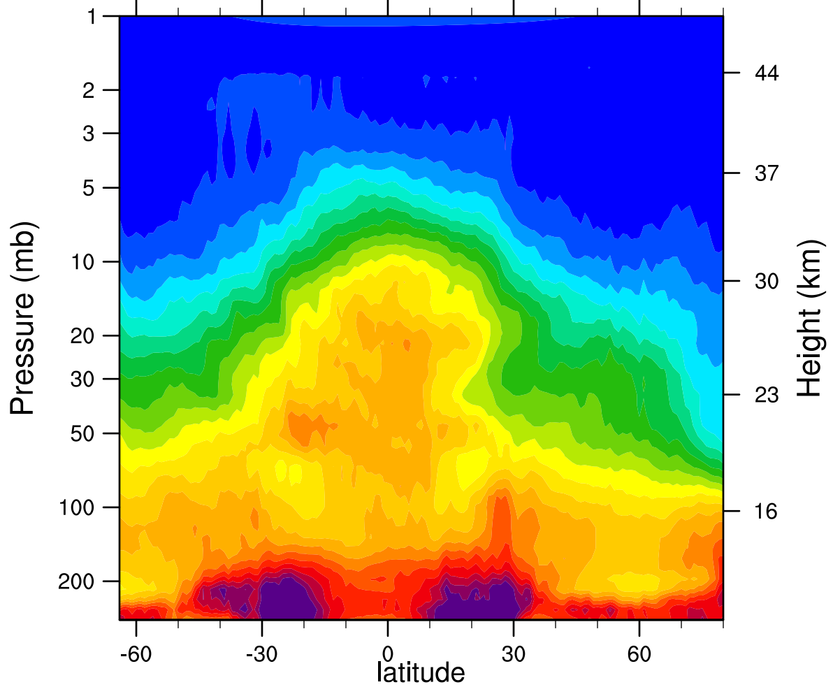
HIRDLSv6 2007d063 N2O_Combined (ppbv)
