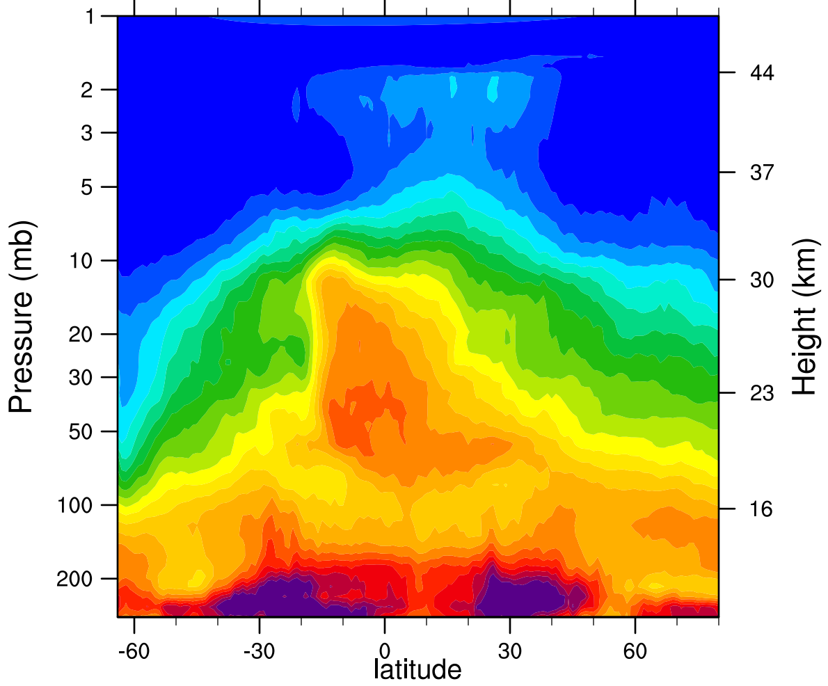
HIRDLSv6 2005d251 N2O_Combined (ppbv)
