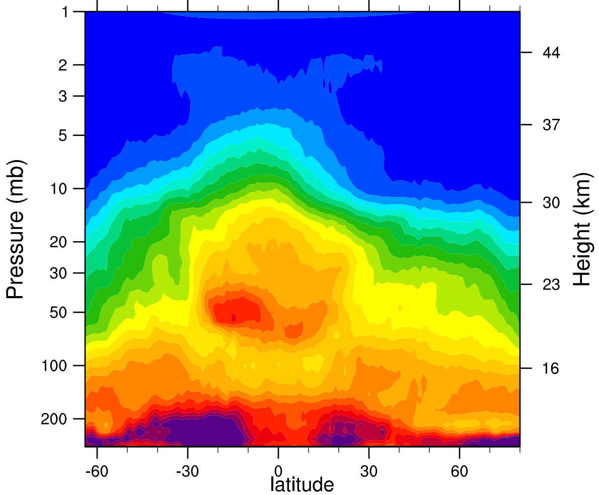
HIRDLSv6 2006d118 N2O_Combined (ppbv)
