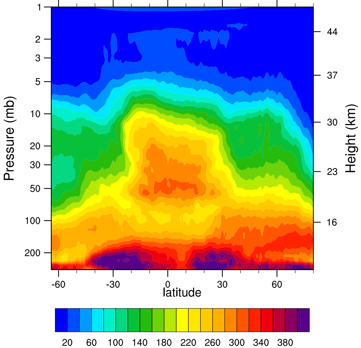
HIRDLSv6 2005d318 N2O_Combined (ppbv)
