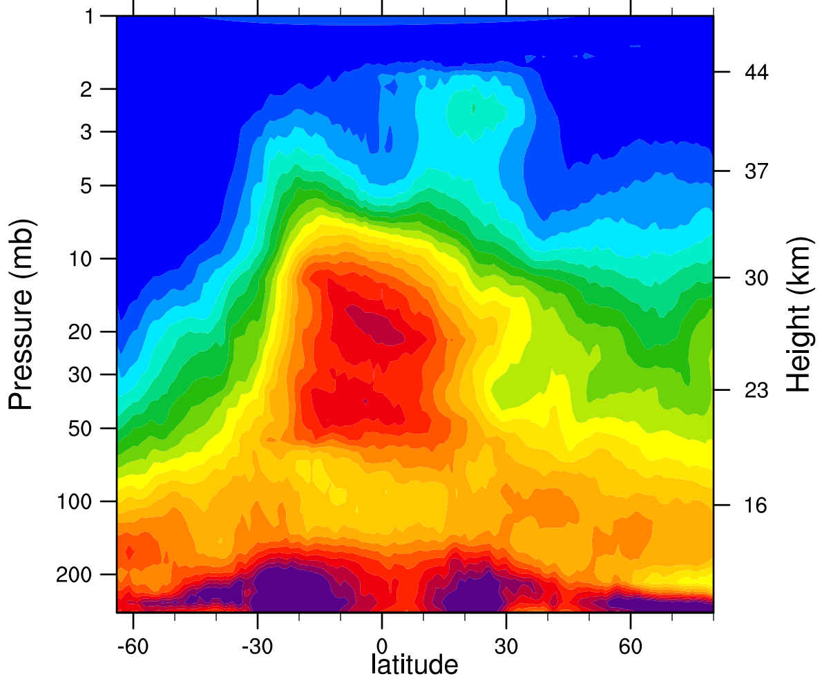
HIRDLSv6 2005d128 N2O_Combined (ppbv)
