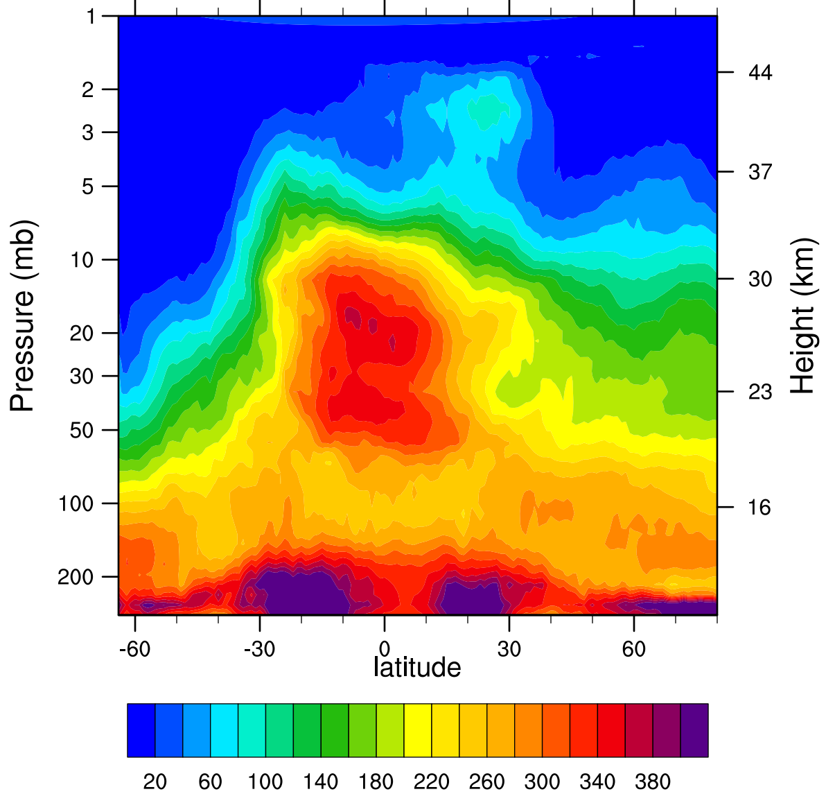
HIRDLSv6 2005d141 N2O_Combined (ppbv)
