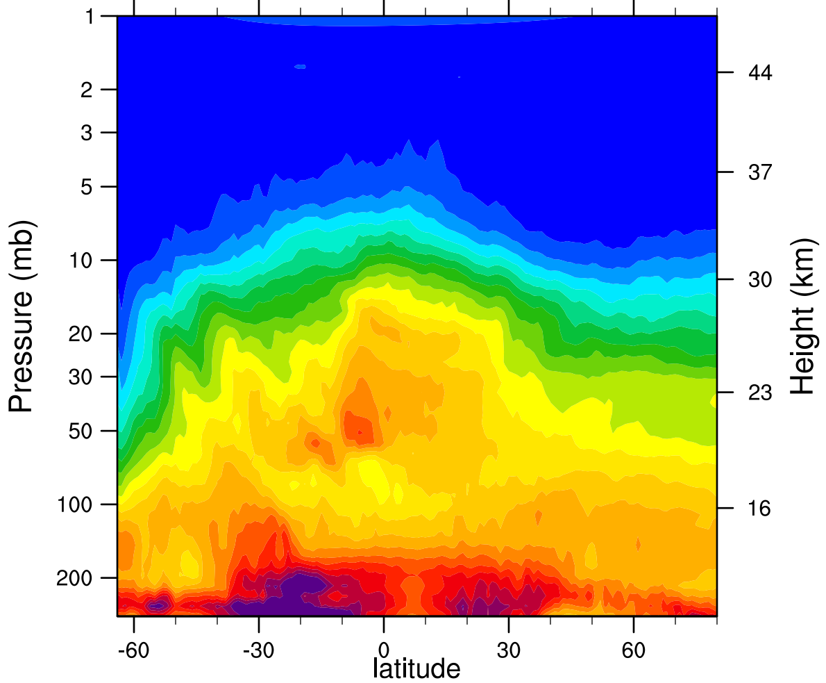
HIRDLSv6 2006d179 N2O_Combined (ppbv)
