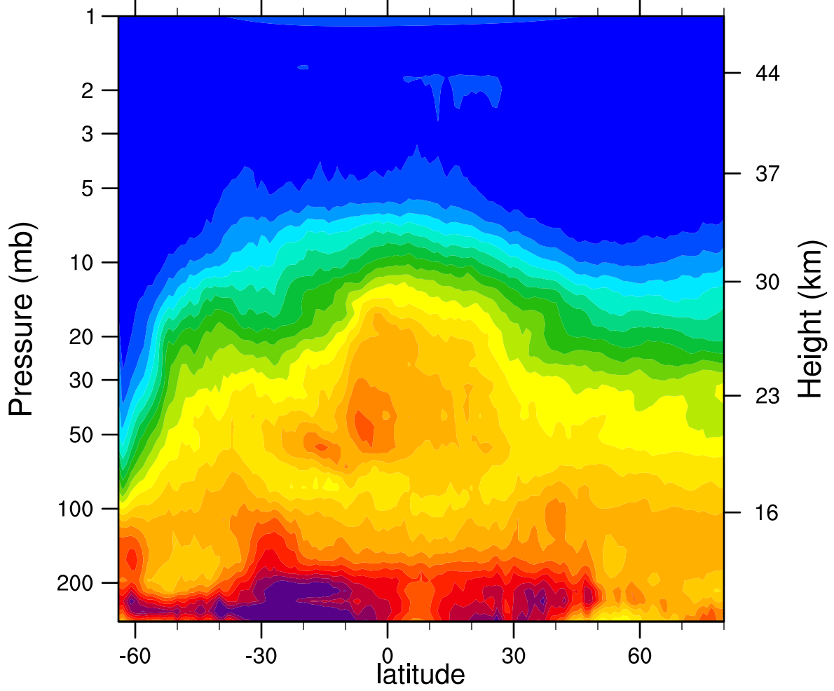
HIRDLSv6 2006d198 N2O_Combined (ppbv)
