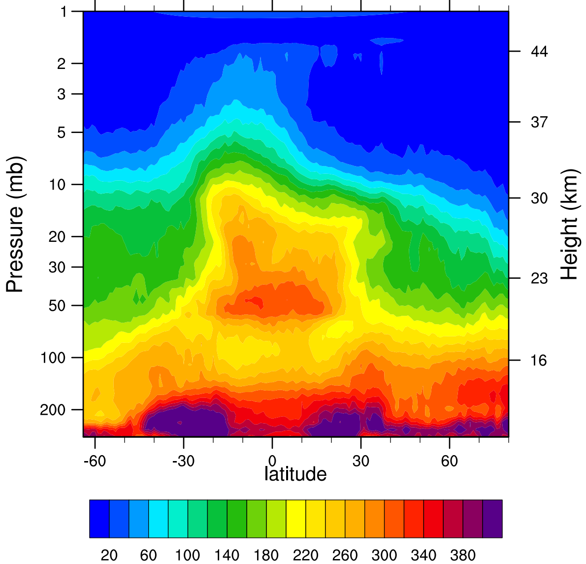
HIRDLSv6 2005d352 N2O_Combined (ppbv)
