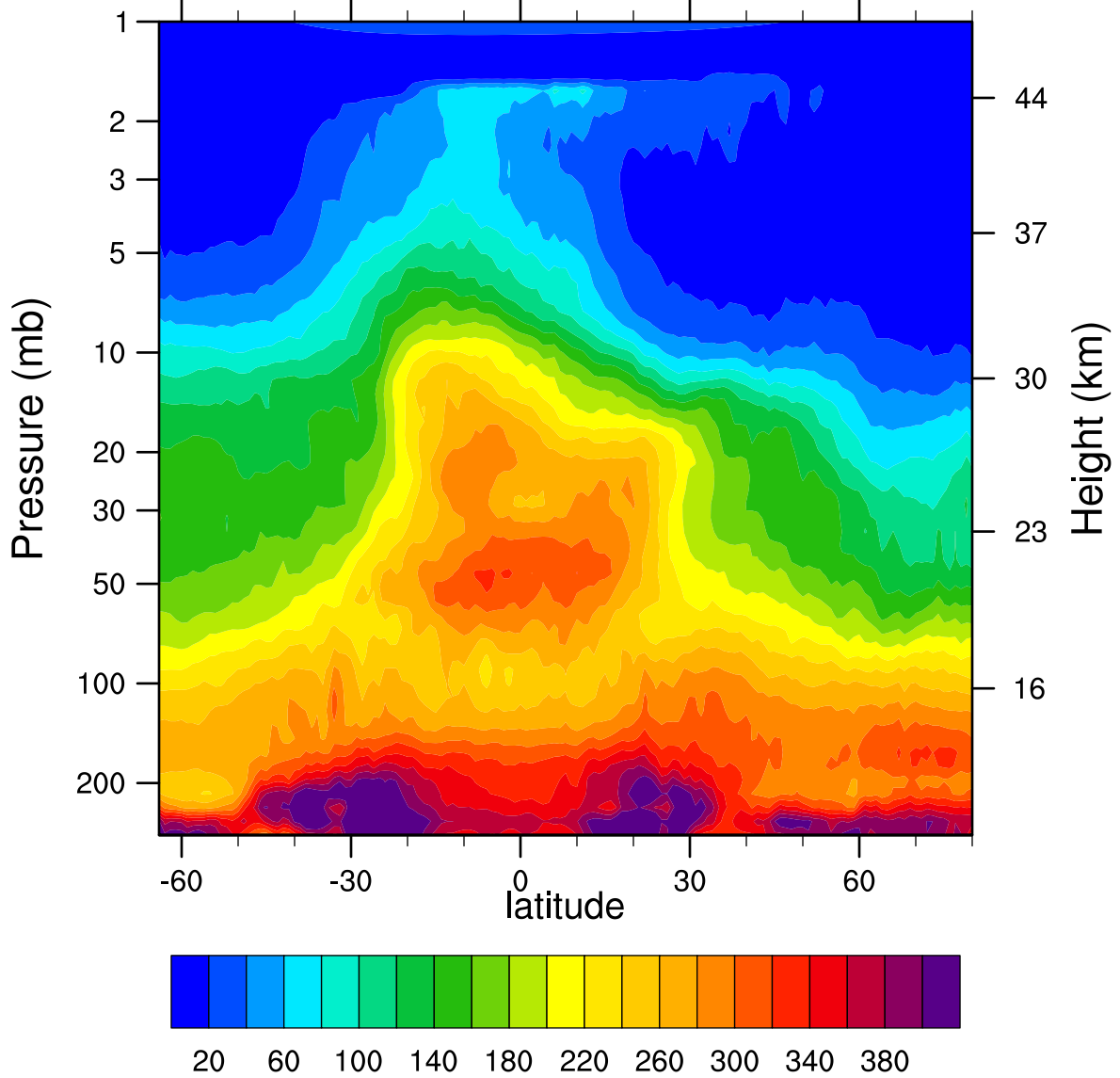
HIRDLSv6 2006d006 N2O_Combined (ppbv)
