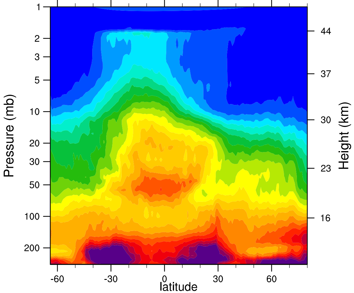
HIRDLSv6 2006d067 N2O_Combined (ppbv)
