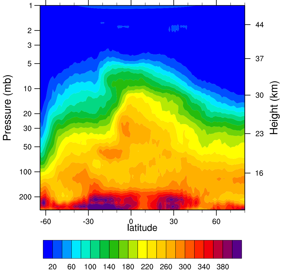
HIRDLSv6 2006d263 N2O_Combined (ppbv)
