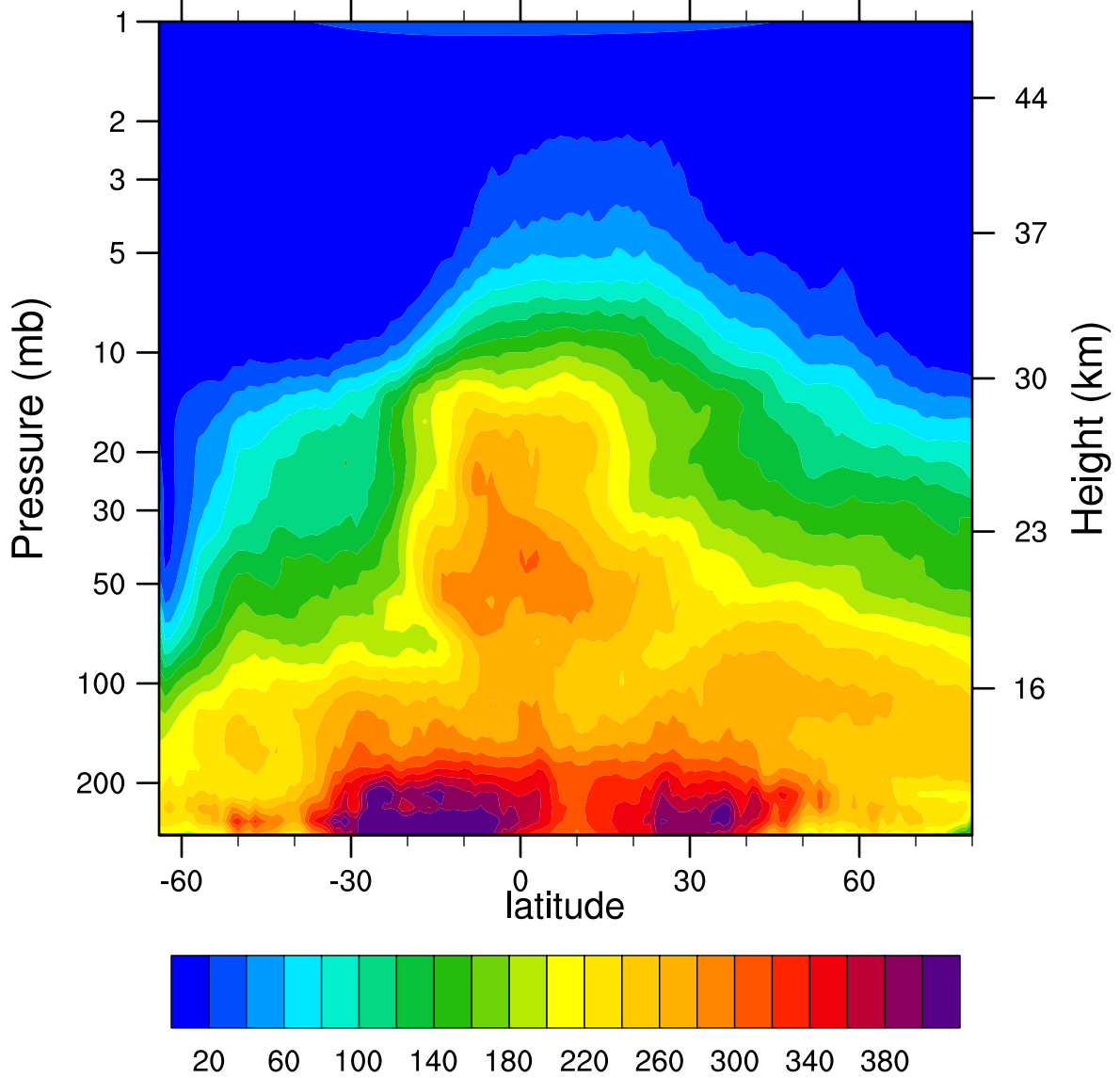
HIRDLSv6 2007d219 N2O_Combined (ppbv)
