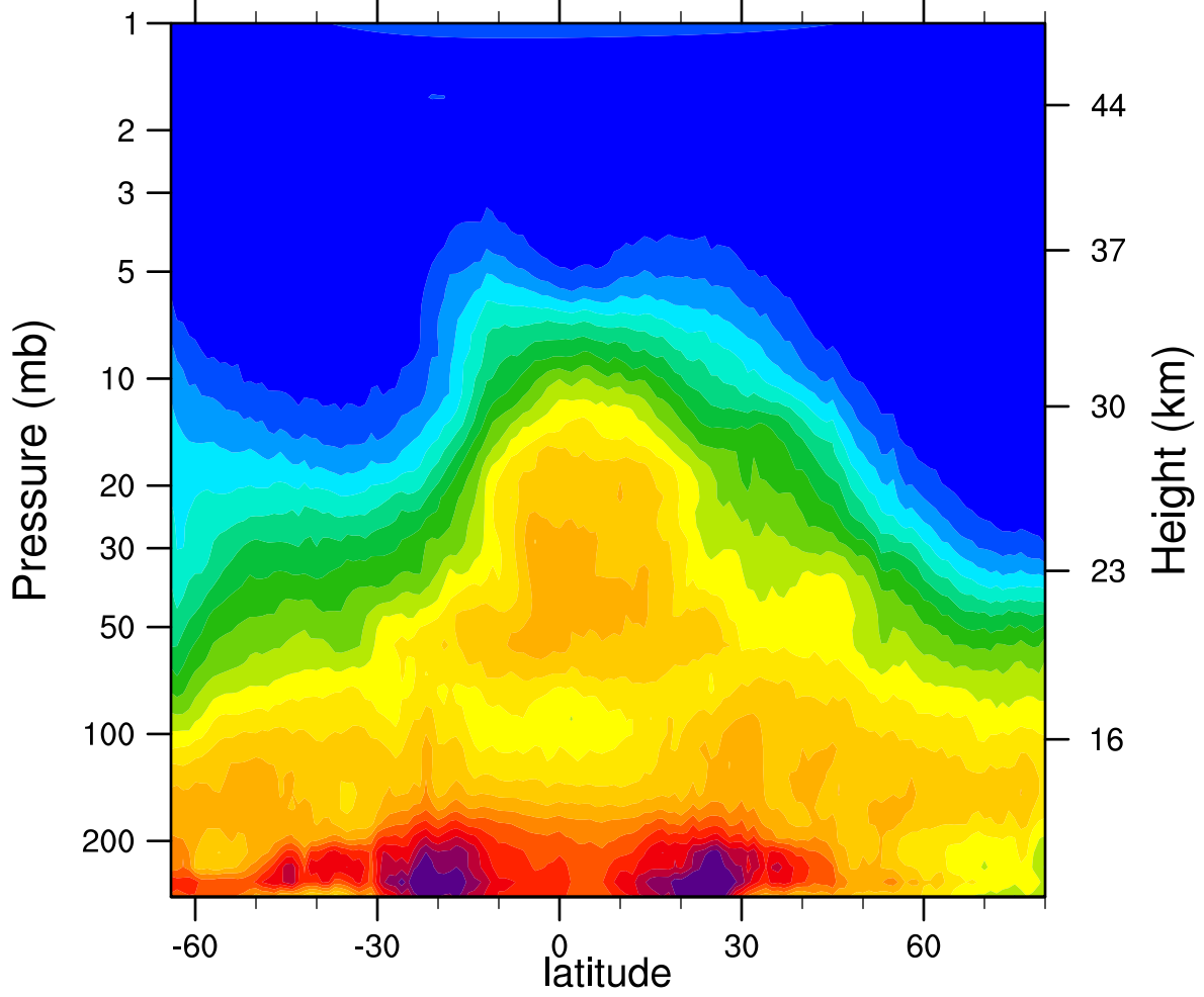
HIRDLSv6 2006d332 N2O_Combined (ppbv)
