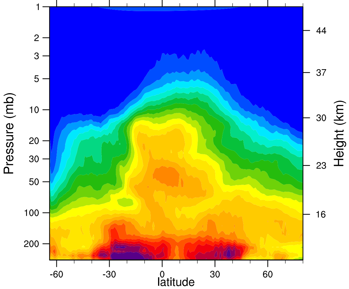
HIRDLSv6 2007d247 N2O_Combined (ppbv)
