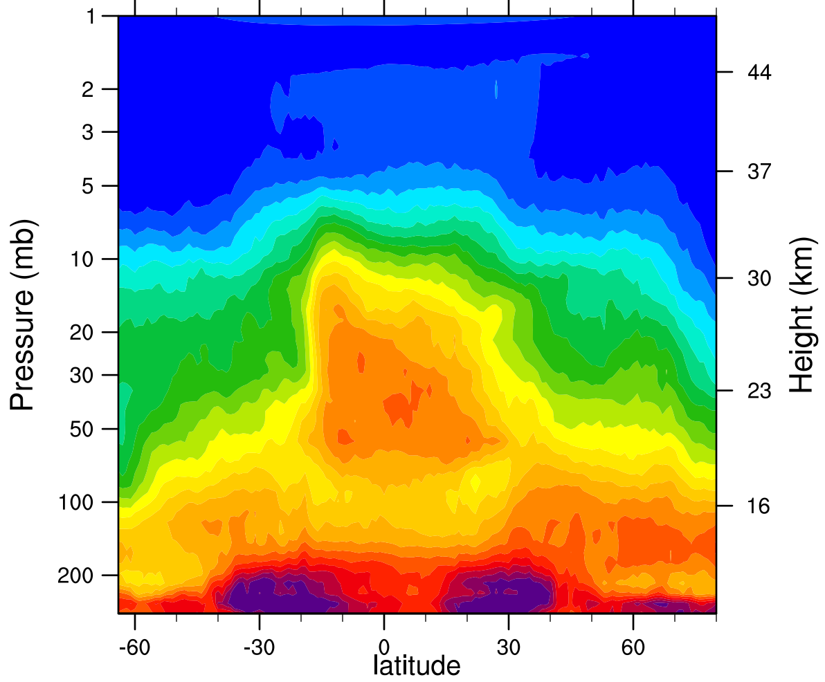
HIRDLSv6 2005d303 N2O_Combined (ppbv)
