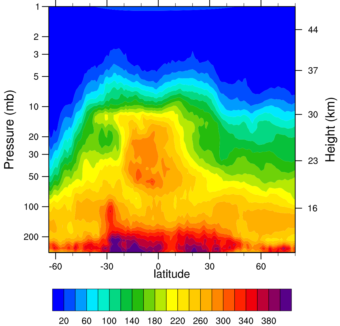
HIRDLSv6 2007d167 N2O_Combined (ppbv)
