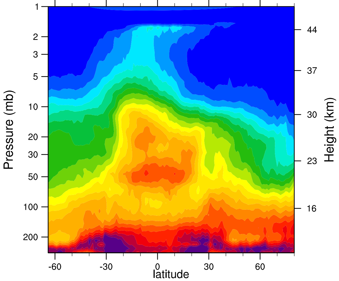
HIRDLSv6 2005d364 N2O_Combined (ppbv)
