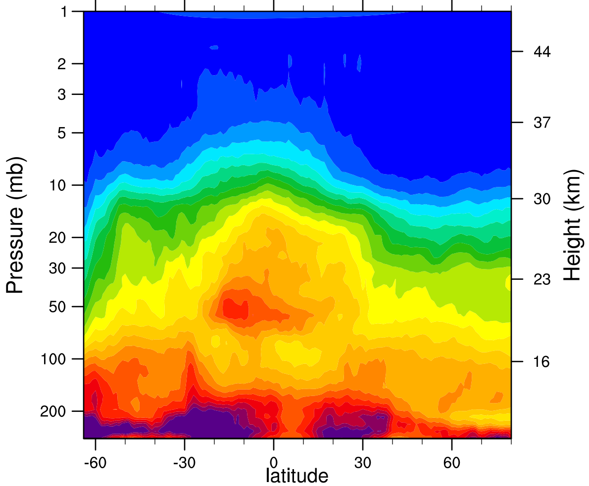
HIRDLSv6 2006d151 N2O_Combined (ppbv)
