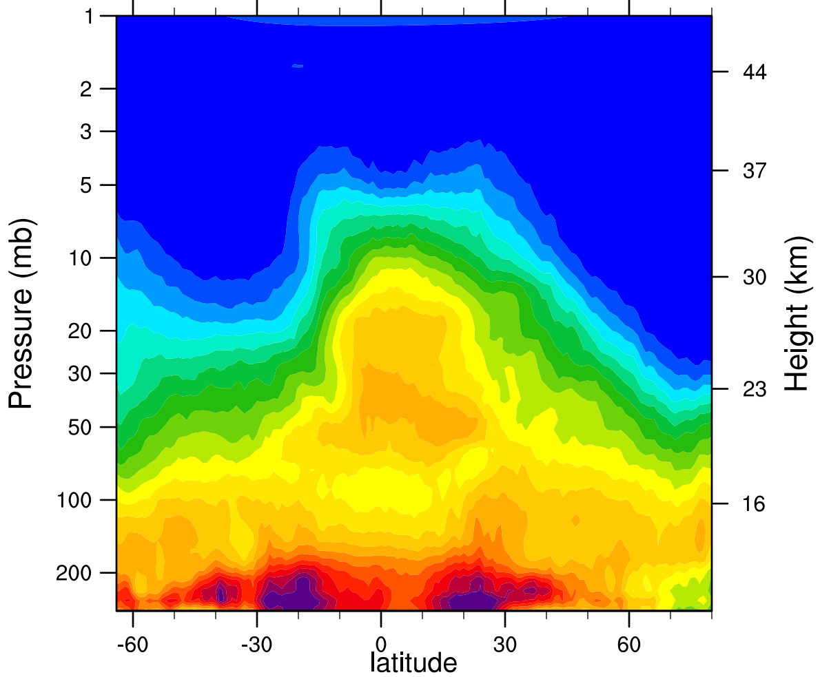
HIRDLSv6 2006d323 N2O_Combined (ppbv)
