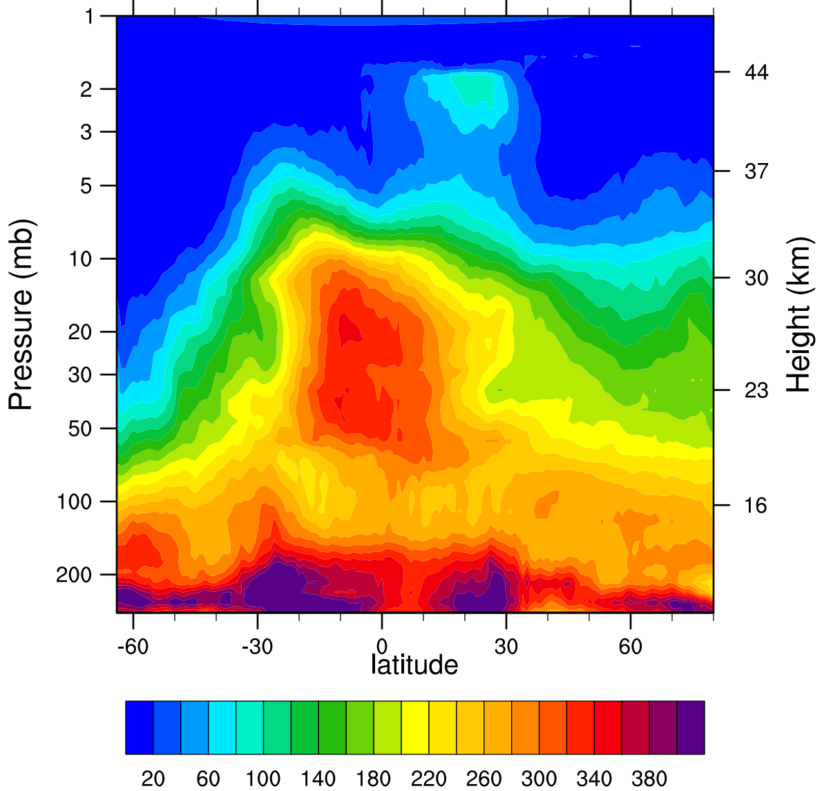
HIRDLSv6 2005d160 N2O_Combined (ppbv)
