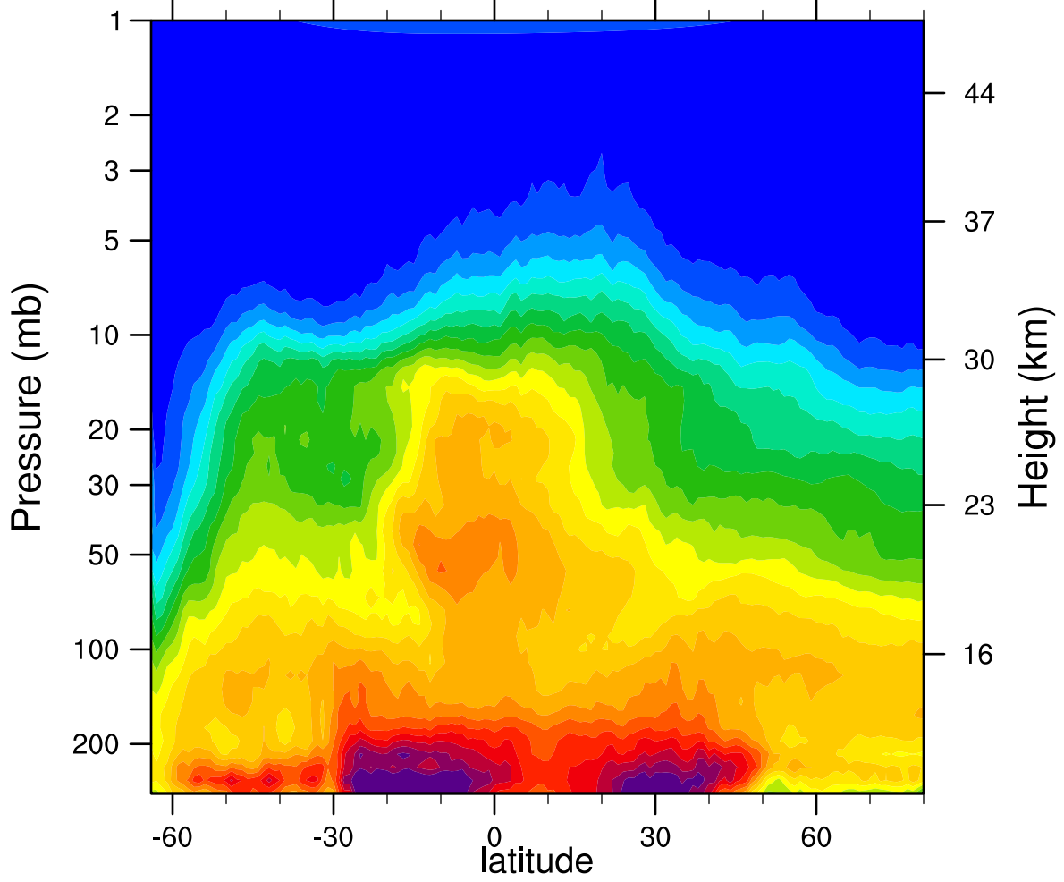
HIRDLSv6 2007d211 N2O_Combined (ppbv)
