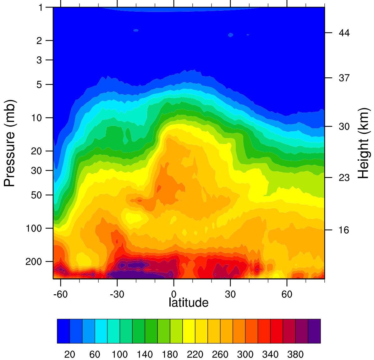
HIRDLSv6 2006d230 N2O_Combined (ppbv)
