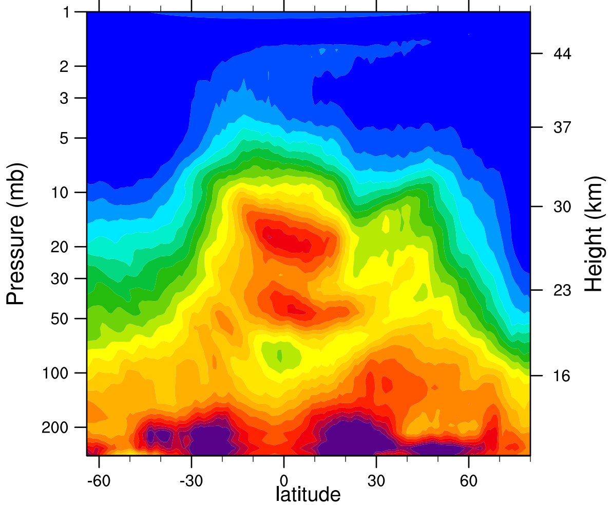
HIRDLSv6 2005d041 N2O_Combined (ppbv)
