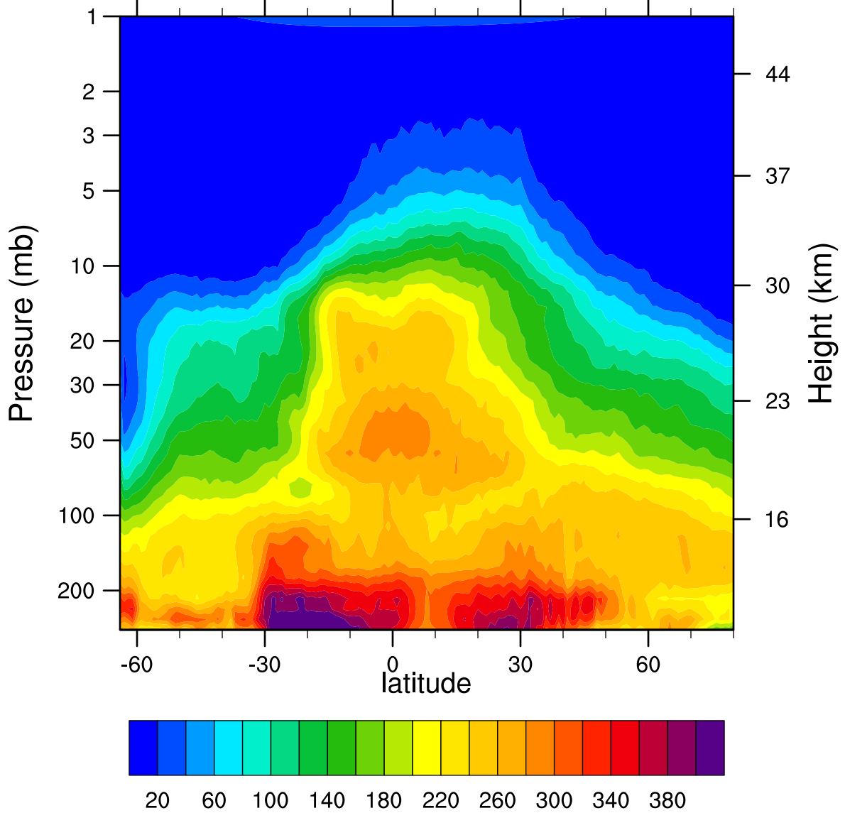
HIRDLSv6 2007d252 N2O_Combined (ppbv)
