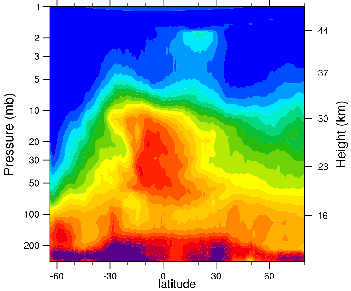
HIRDLSv6 2005d177 N2O_Combined (ppbv)
