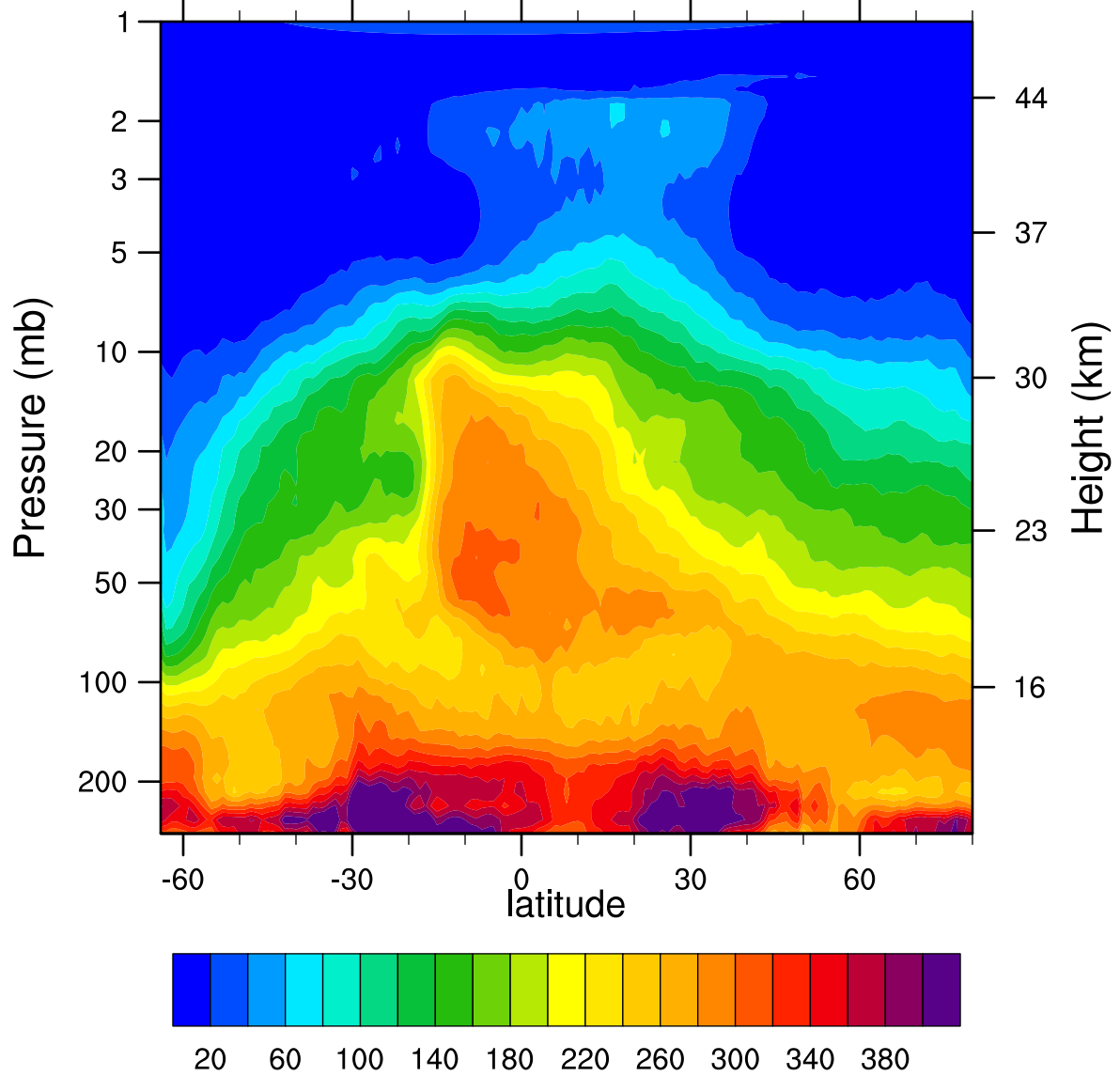
HIRDLSv6 2005d254 N2O_Combined (ppbv)
