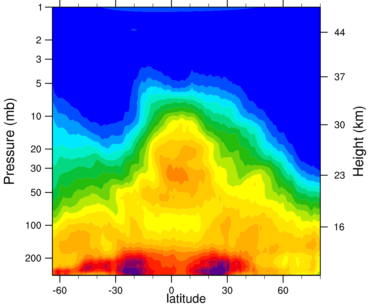
HIRDLSv6 2006d336 N2O_Combined (ppbv)
