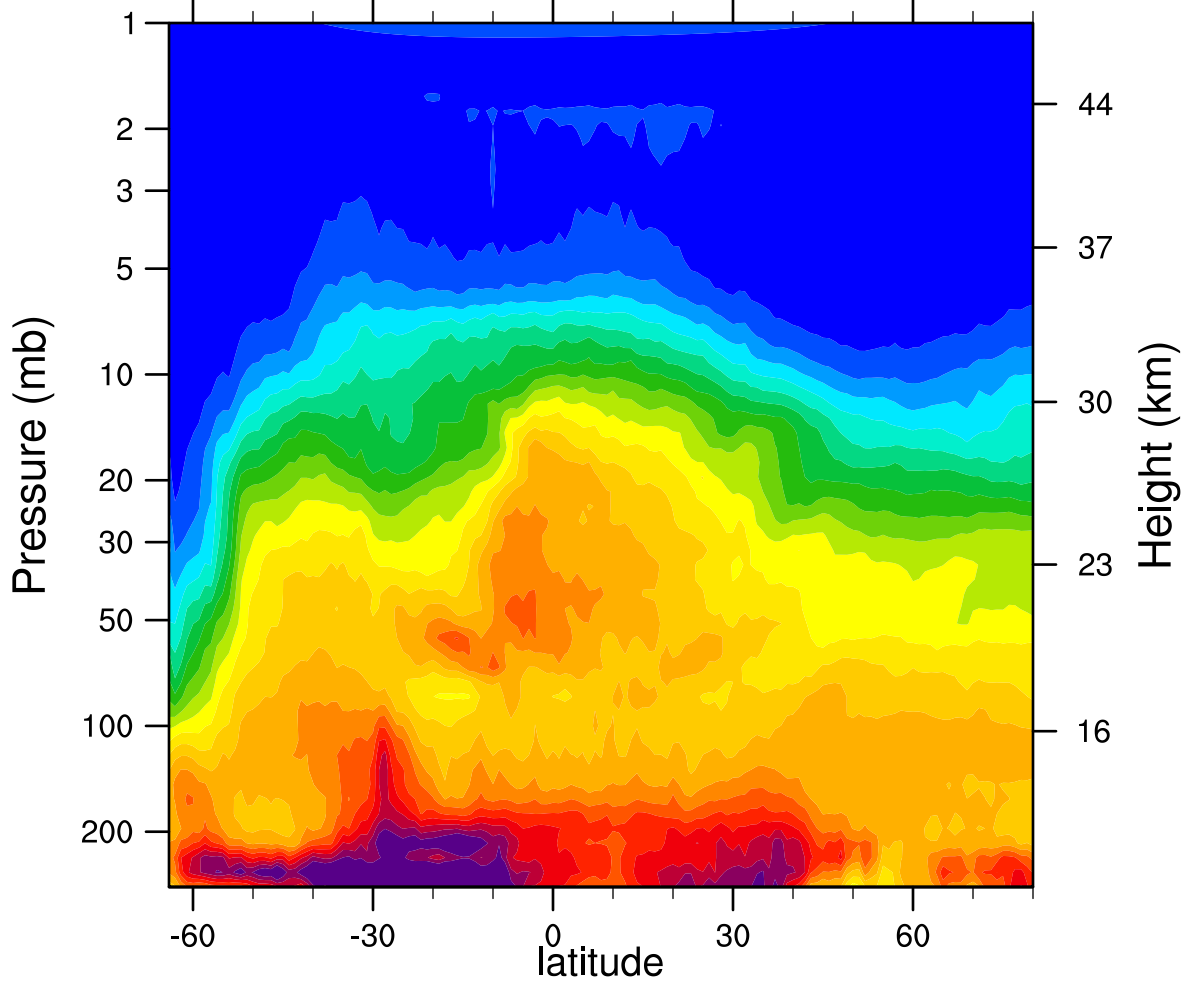
HIRDLSv6 2006d212 N2O_Combined (ppbv)
