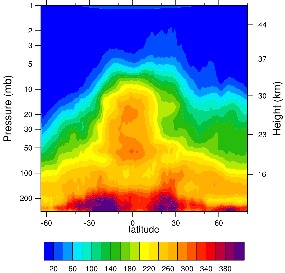
HIRDLSv6 2007d129 N2O_Combined (ppbv)
