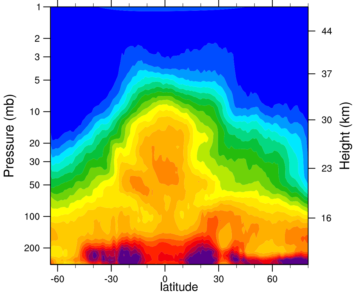
HIRDLSv6 2007d097 N2O_Combined (ppbv)
