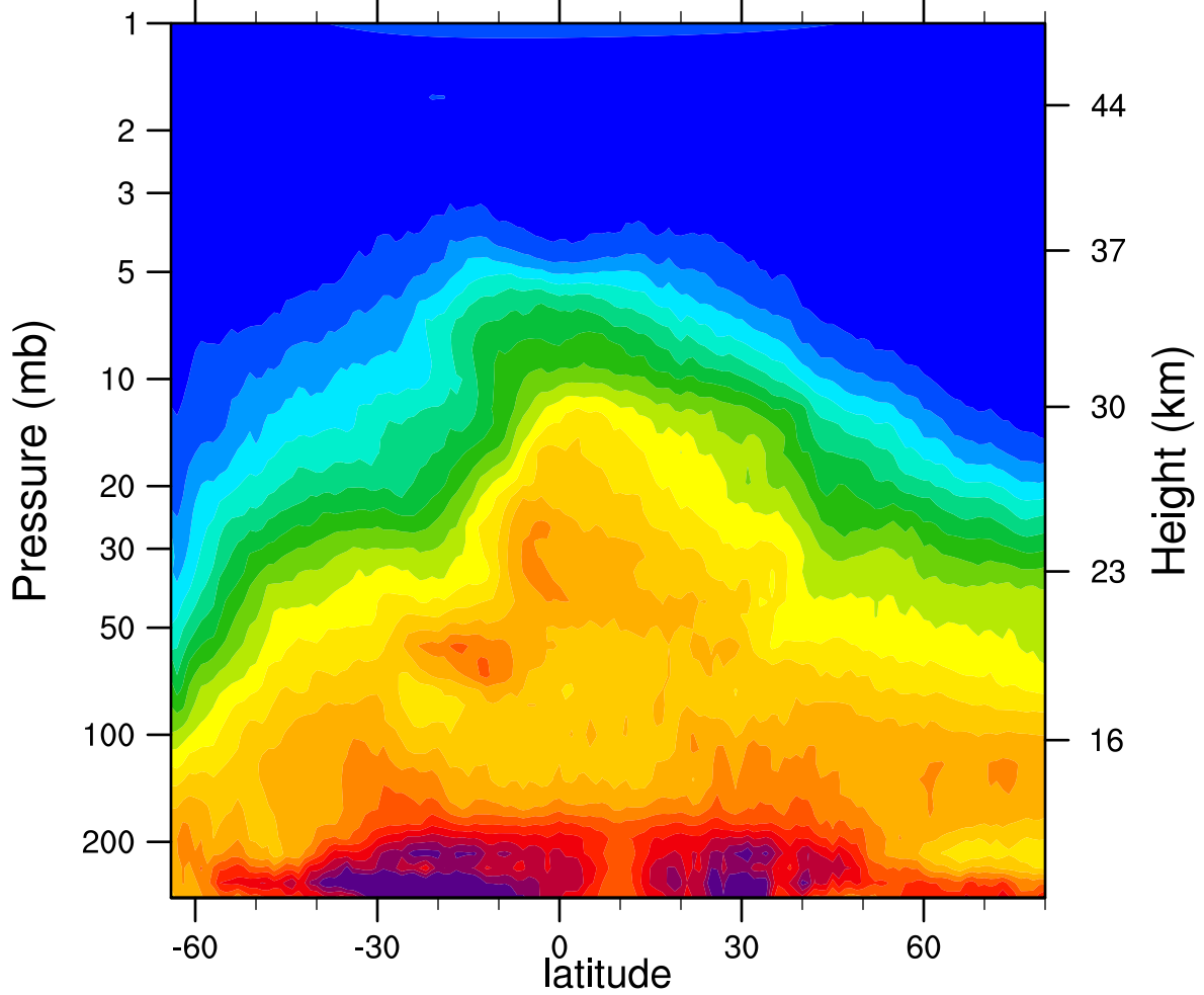
HIRDLSv6 2006d270 N2O_Combined (ppbv)
