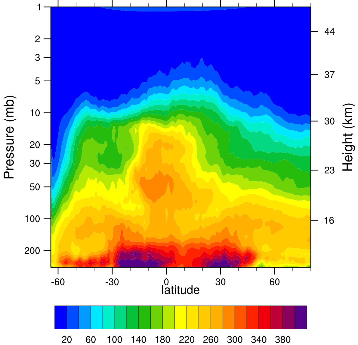
HIRDLSv6 2007d210 N2O_Combined (ppbv)
