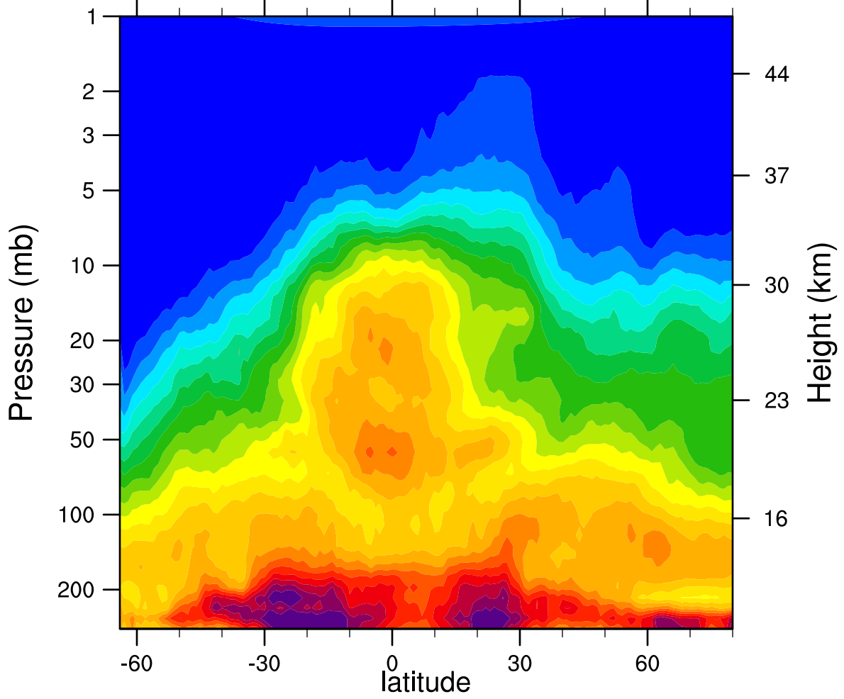
HIRDLSv6 2007d136 N2O_Combined (ppbv)
