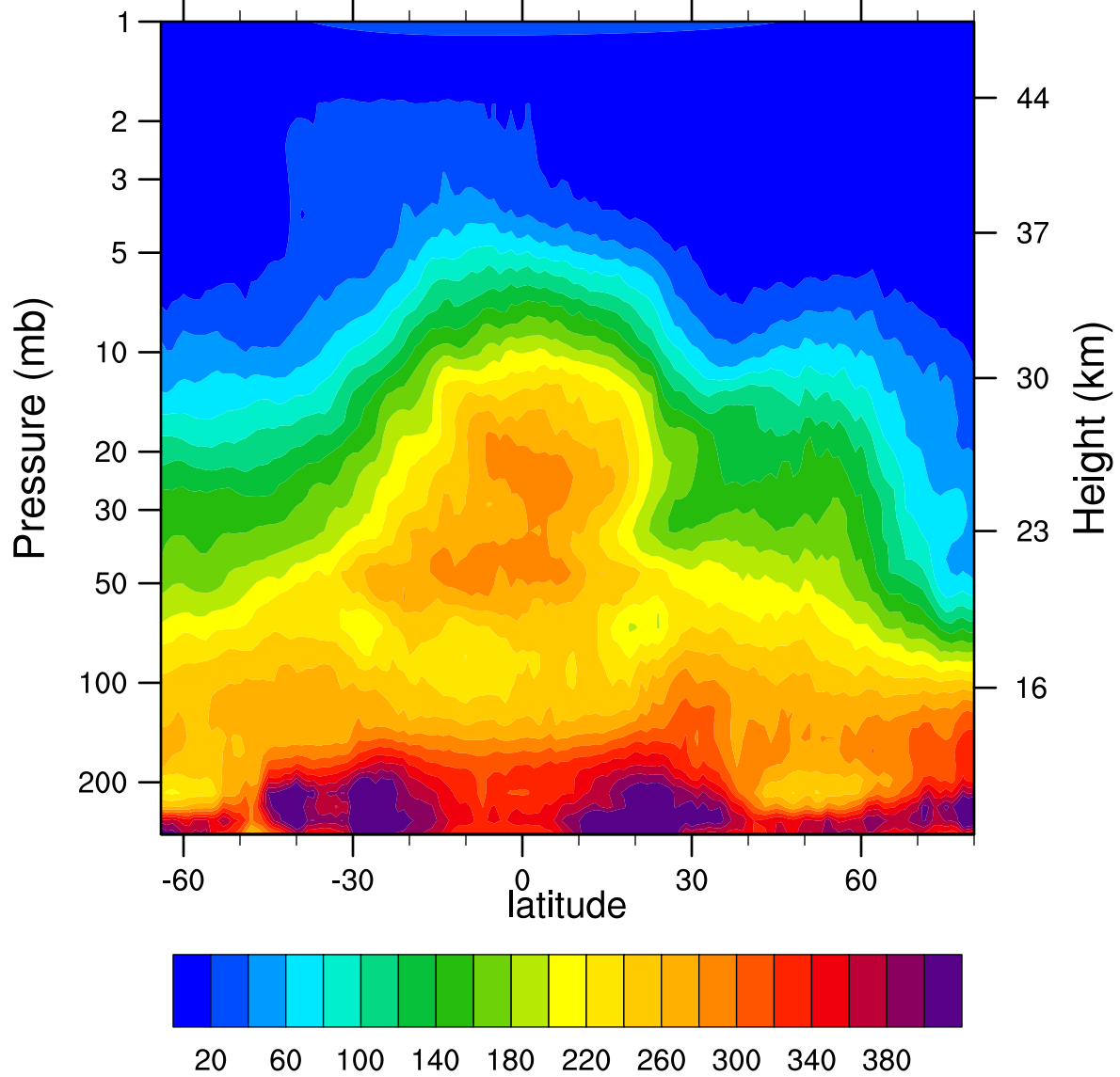
HIRDLSv6 2007d036 N2O_Combined (ppbv)
