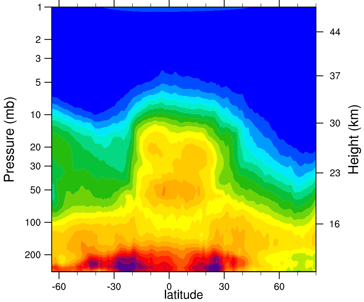
HIRDLSv6 2007d321 N2O_Combined (ppbv)
