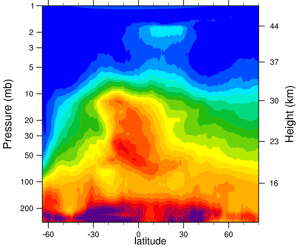
HIRDLSv6 2005d199 N2O_Combined (ppbv)
