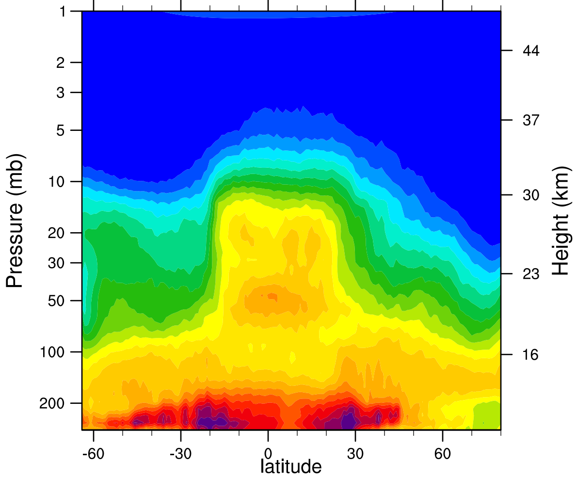
HIRDLSv6 2007d308 N2O_Combined (ppbv)
