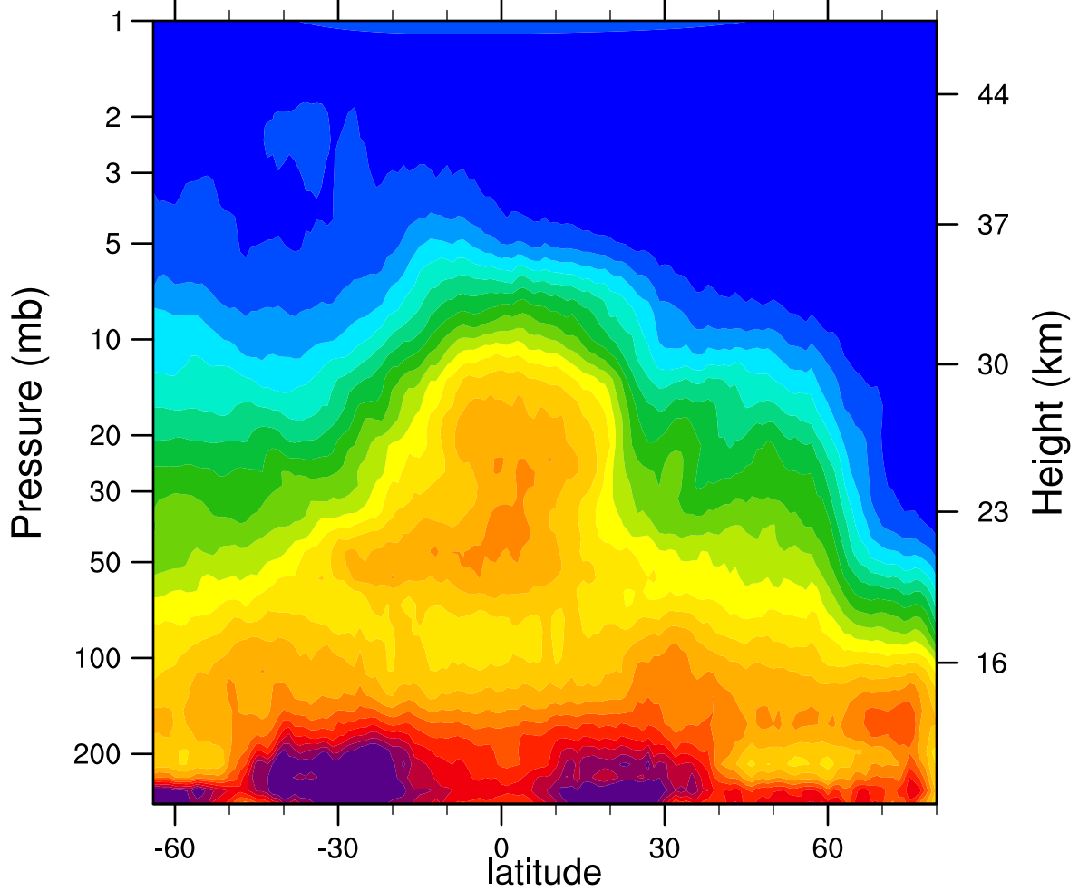
HIRDLSv6 2007d012 N2O_Combined (ppbv)
