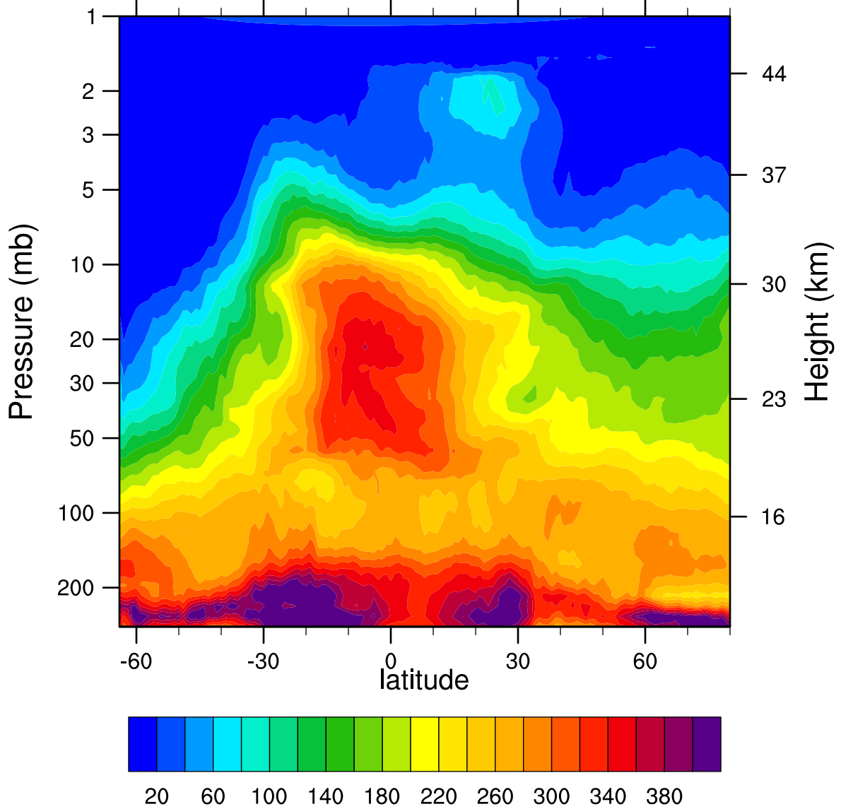
HIRDLSv6 2005d153 N2O_Combined (ppbv)
