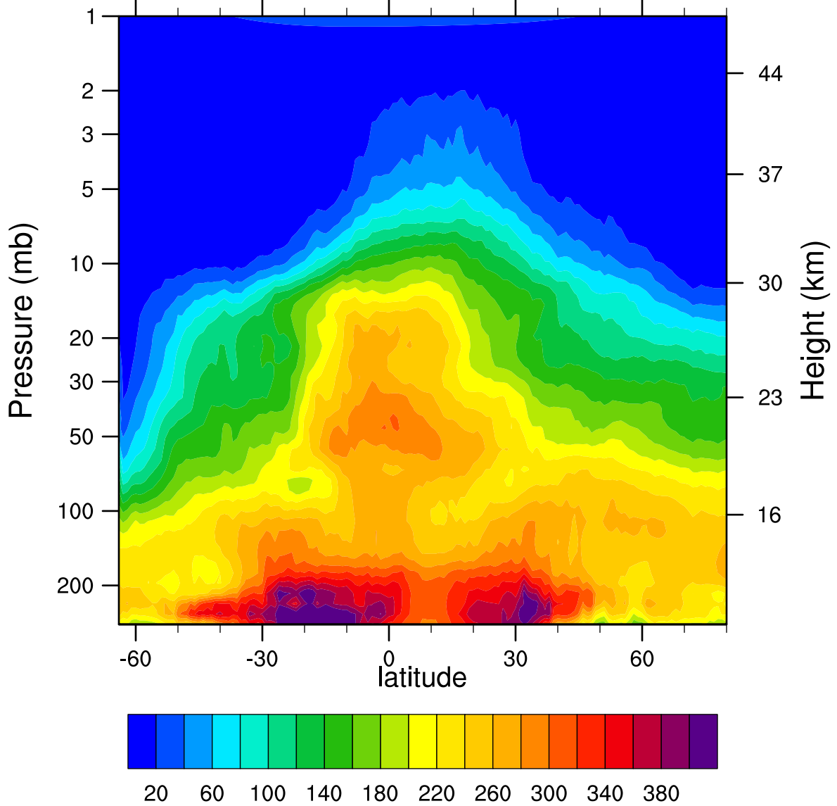
HIRDLSv6 2007d231 N2O_Combined (ppbv)
