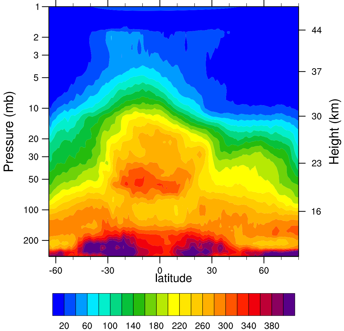
HIRDLSv6 2006d102 N2O_Combined (ppbv)
