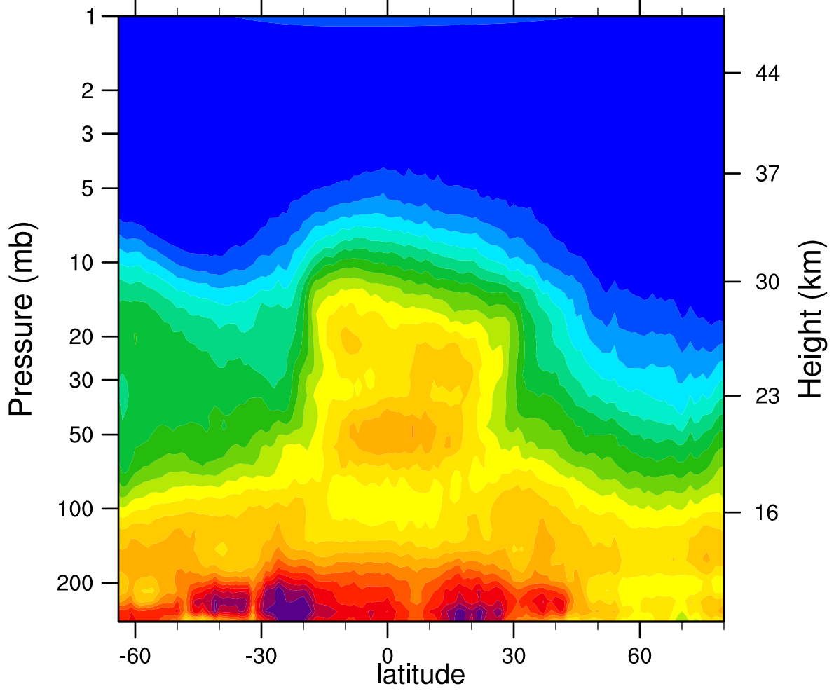
HIRDLSv6 2007d329 N2O_Combined (ppbv)
