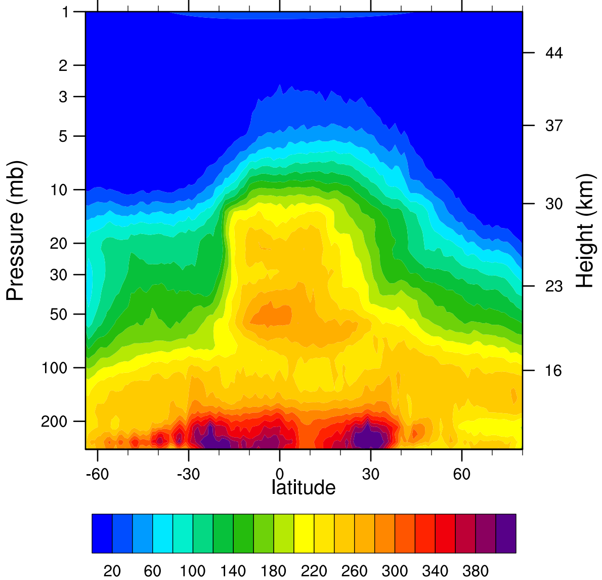
HIRDLSv6 2007d279 N2O_Combined (ppbv)
