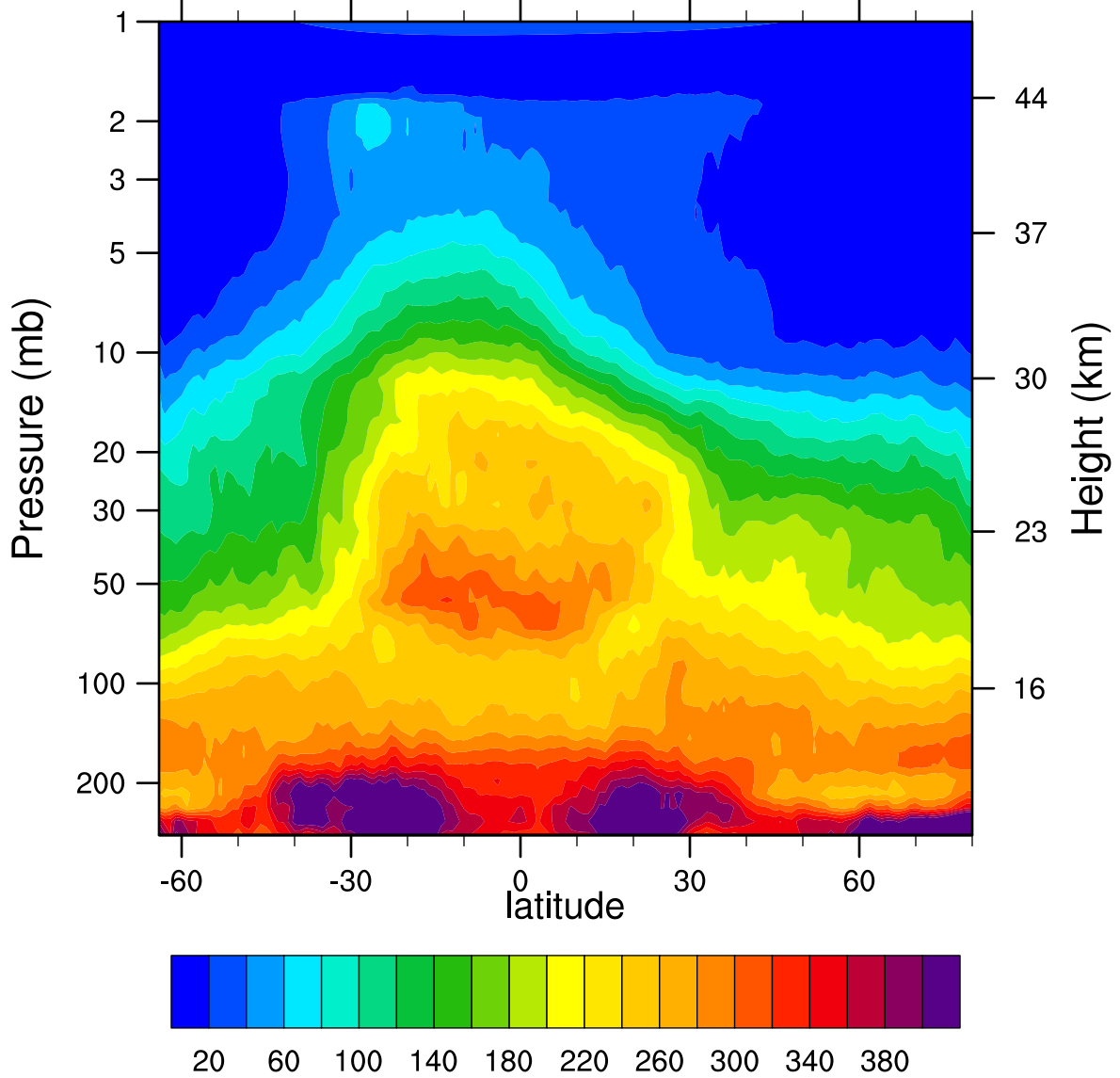
HIRDLSv6 2006d096 N2O_Combined (ppbv)
