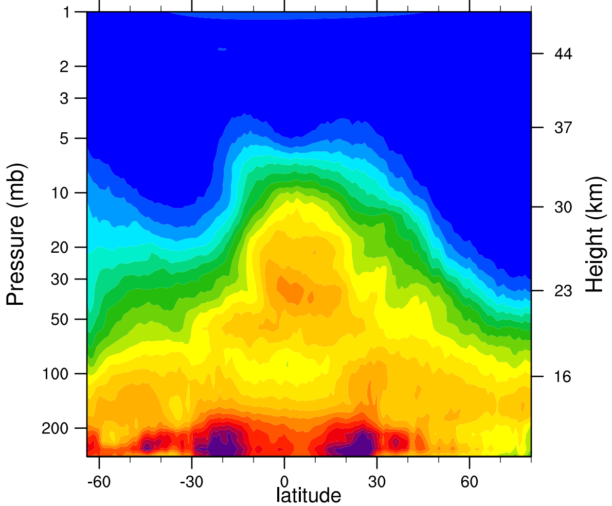
HIRDLSv6 2006d330 N2O_Combined (ppbv)
