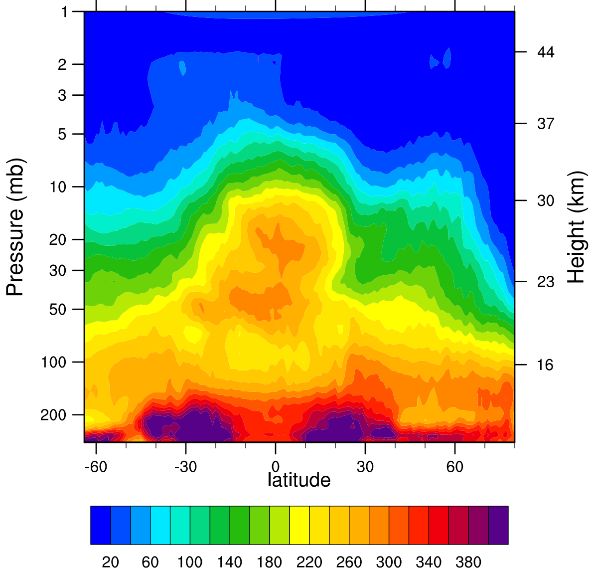
HIRDLSv6 2007d032 N2O_Combined (ppbv)
