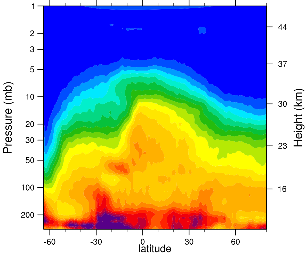
HIRDLSv6 2006d251 N2O_Combined (ppbv)
