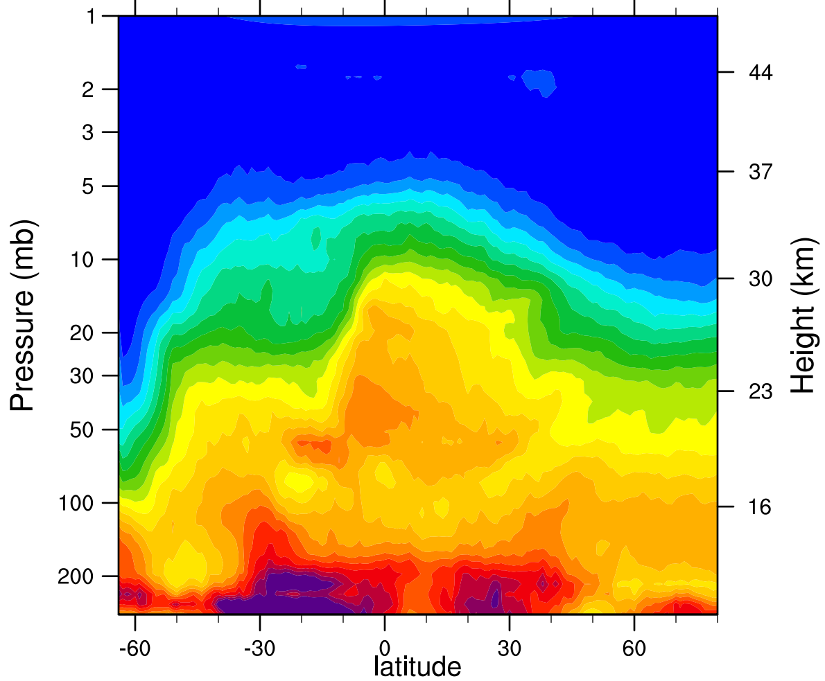
HIRDLSv6 2006d240 N2O_Combined (ppbv)
