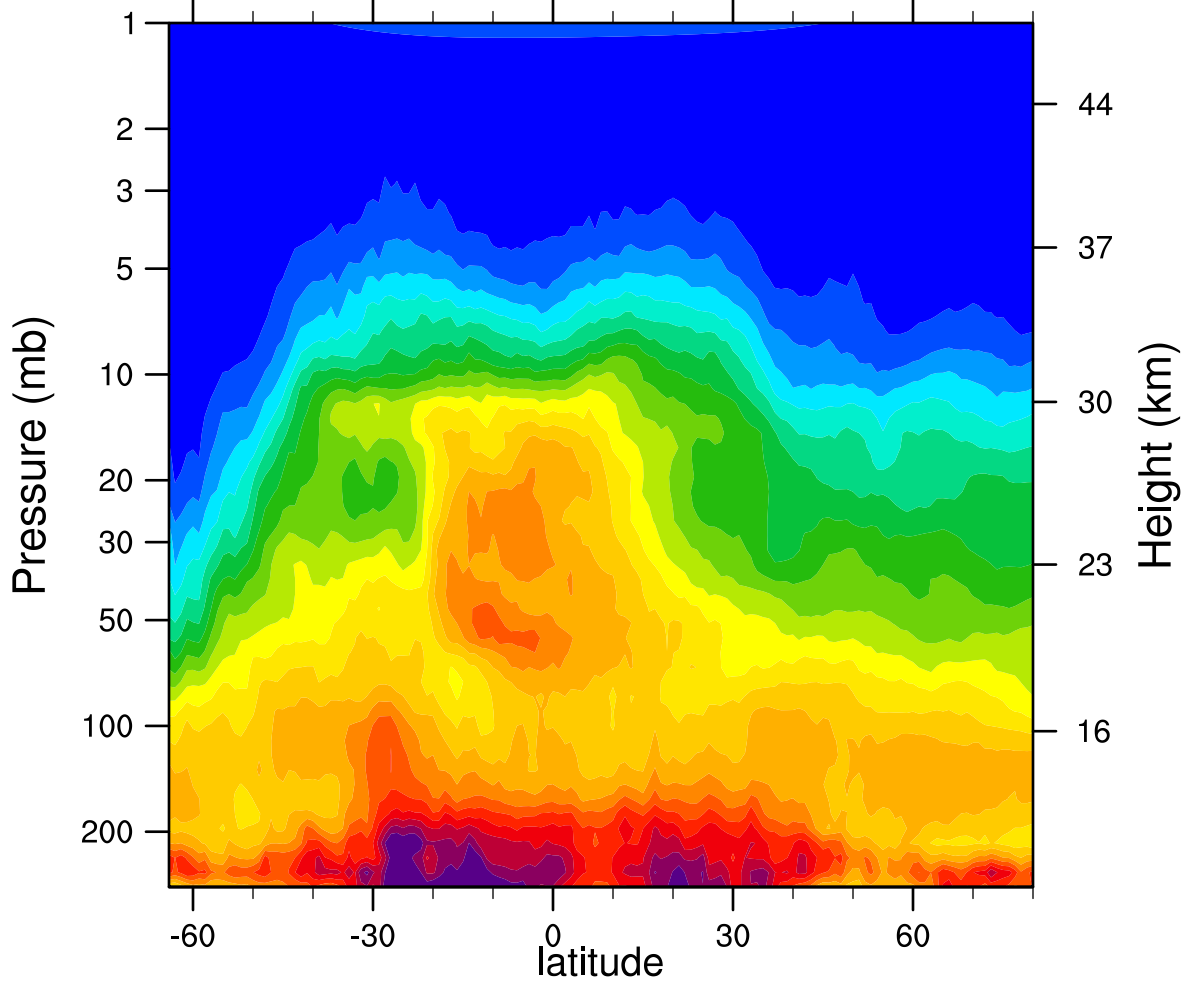
HIRDLSv6 2007d168 N2O_Combined (ppbv)
