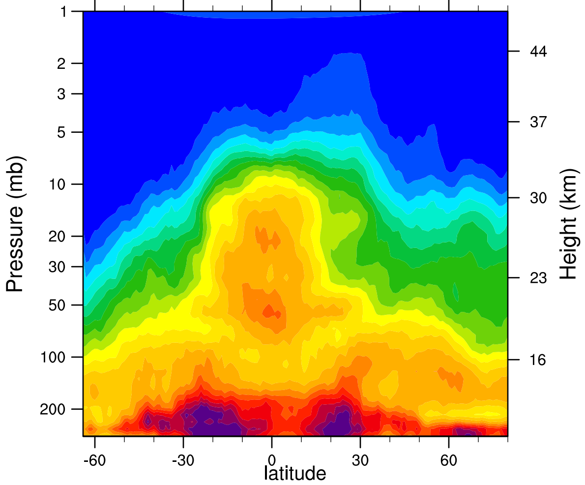
HIRDLSv6 2007d133 N2O_Combined (ppbv)
