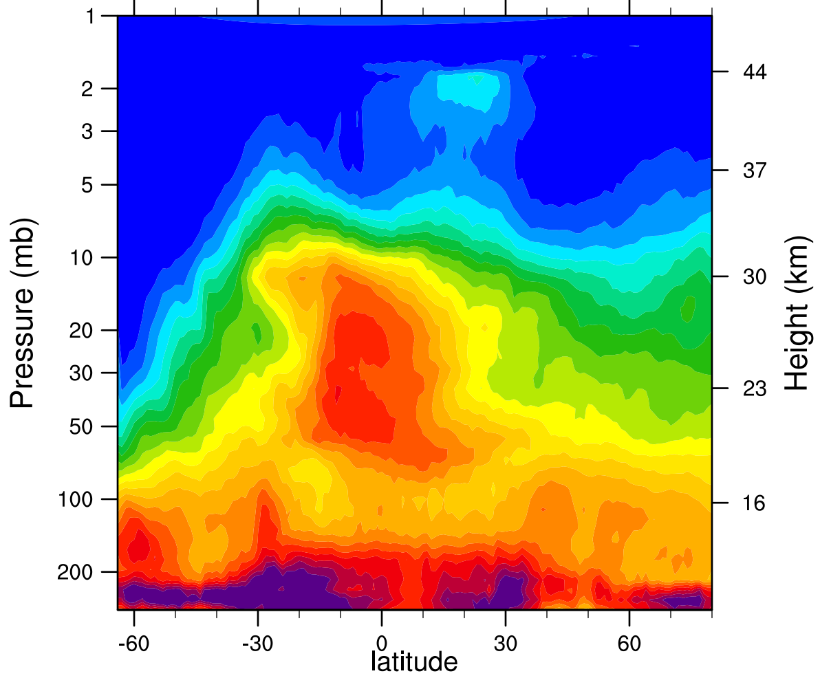
HIRDLSv6 2005d174 N2O_Combined (ppbv)
