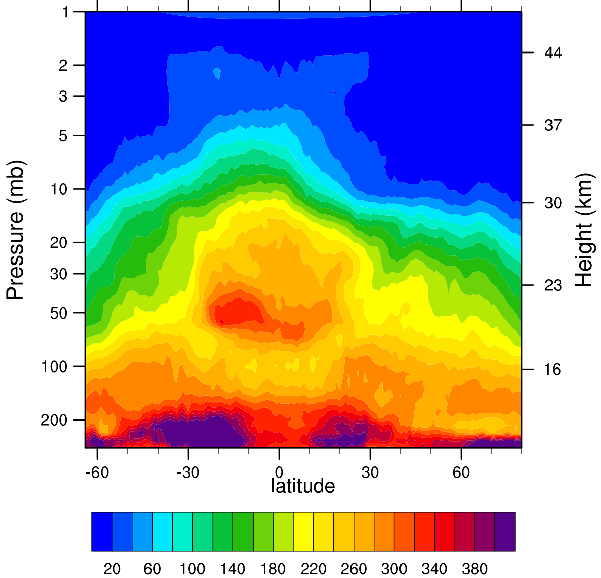
HIRDLSv6 2006d115 N2O_Combined (ppbv)
