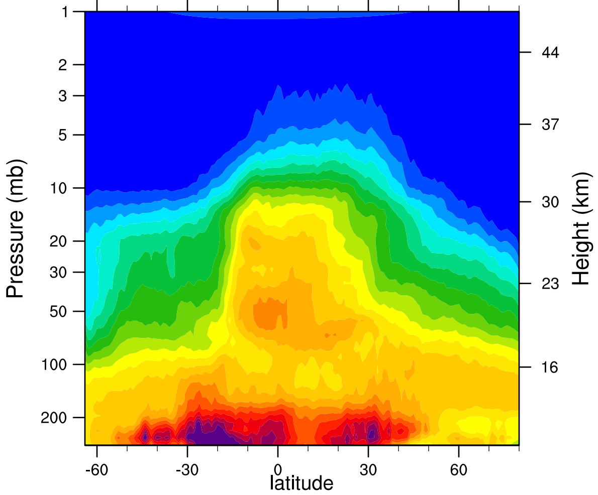
HIRDLSv6 2007d271 N2O_Combined (ppbv)
