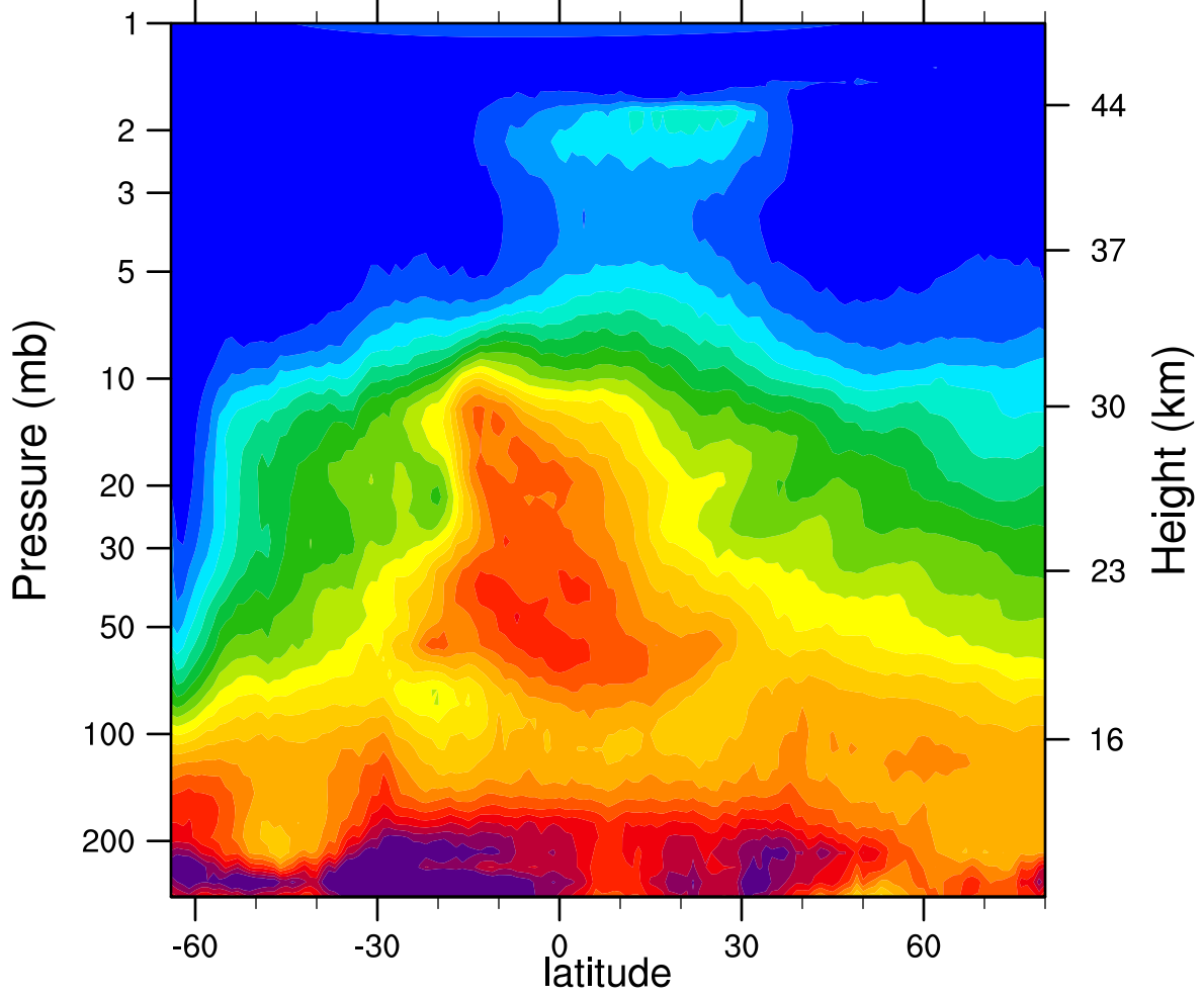
HIRDLSv6 2005d218 N2O_Combined (ppbv)
