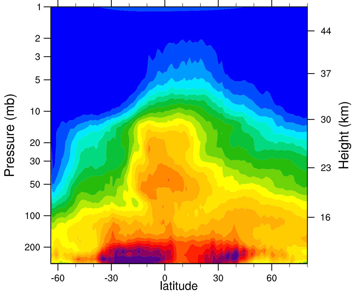
HIRDLSv6 2007d222 N2O_Combined (ppbv)
