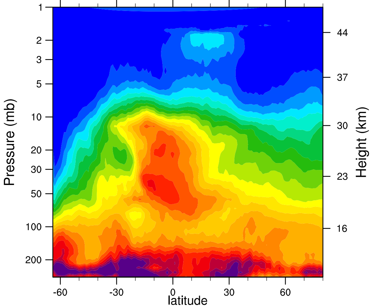
HIRDLSv6 2005d187 N2O_Combined (ppbv)
