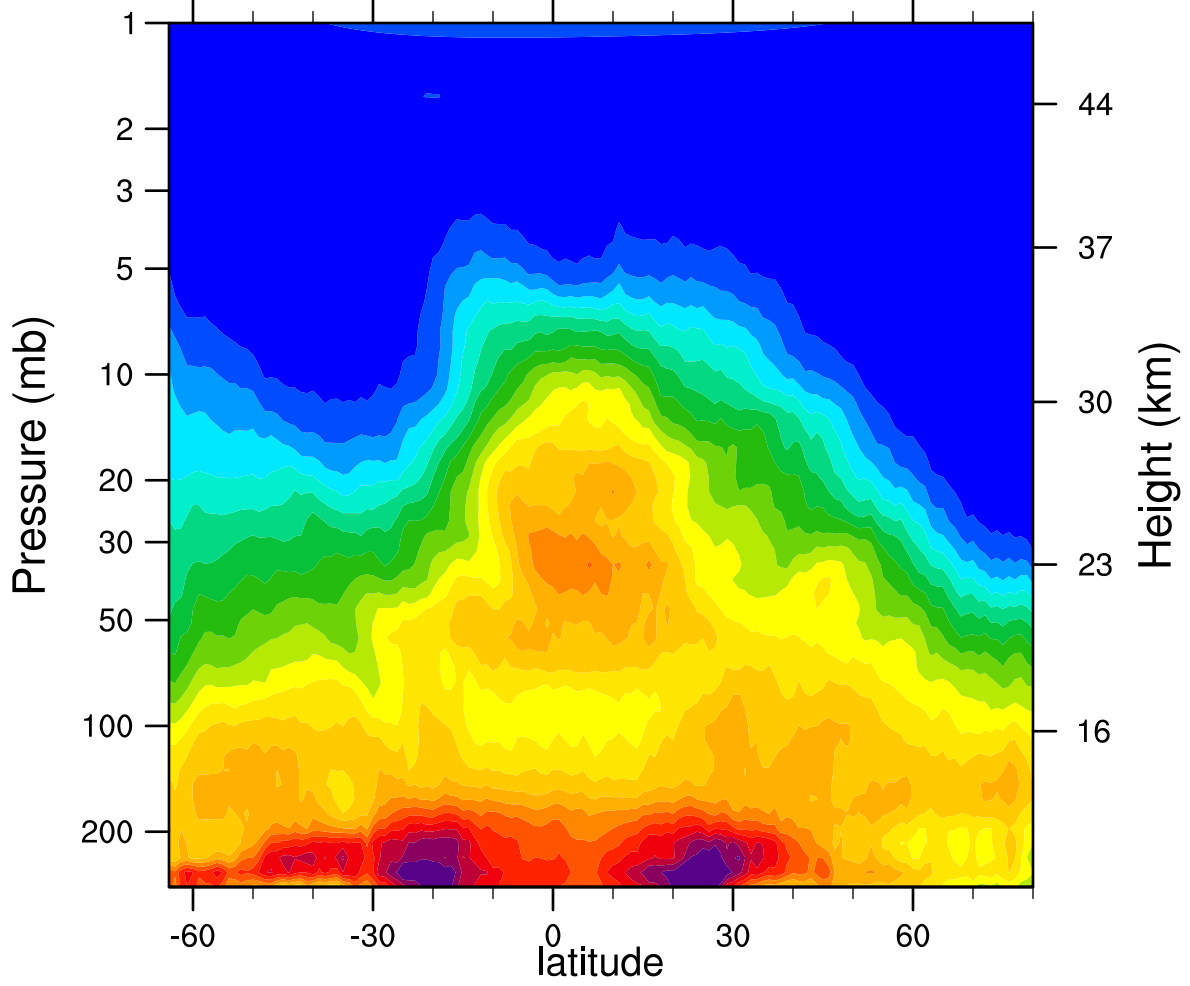
HIRDLSv6 2006d335 N2O_Combined (ppbv)
