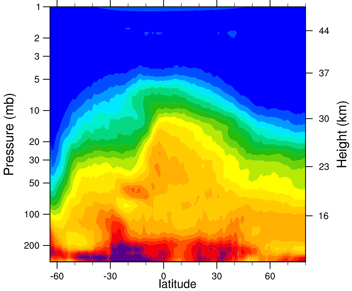
HIRDLSv6 2006d252 N2O_Combined (ppbv)
