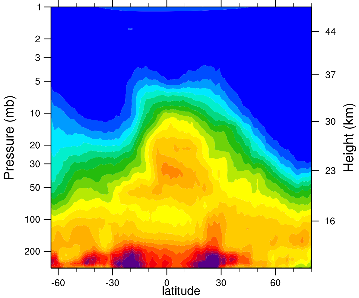
HIRDLSv6 2006d327 N2O_Combined (ppbv)
