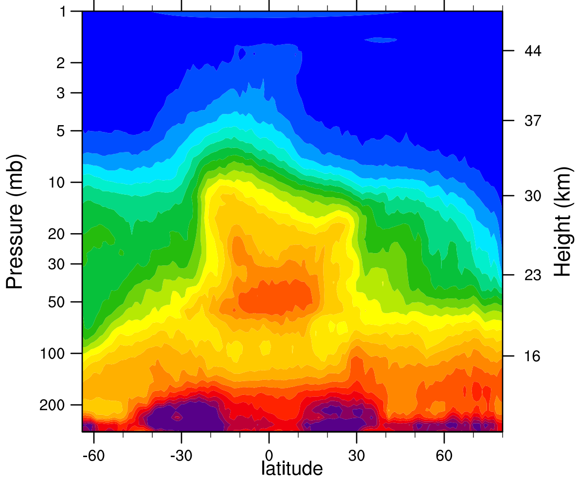
HIRDLSv6 2005d343 N2O_Combined (ppbv)
