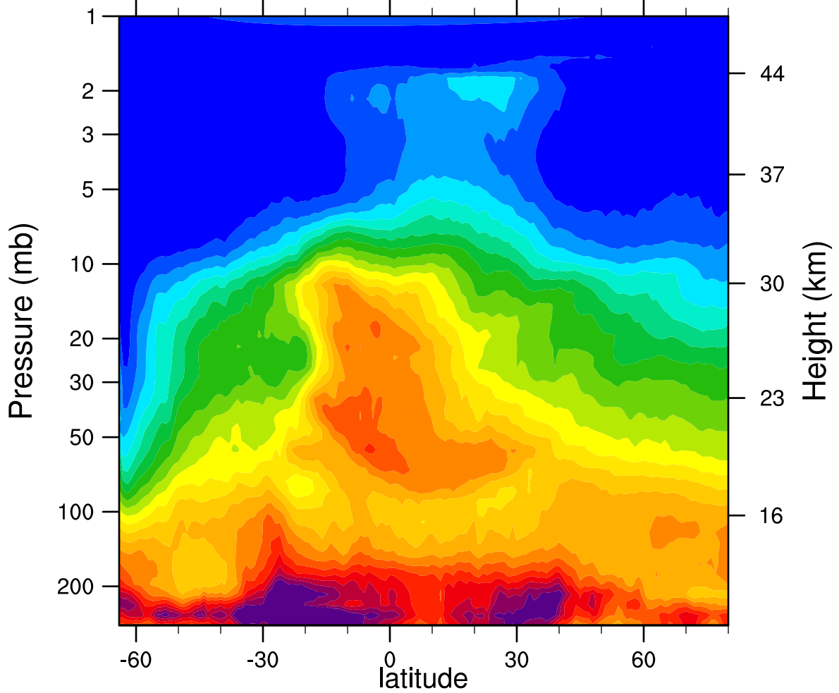
HIRDLSv6 2005d233 N2O_Combined (ppbv)
