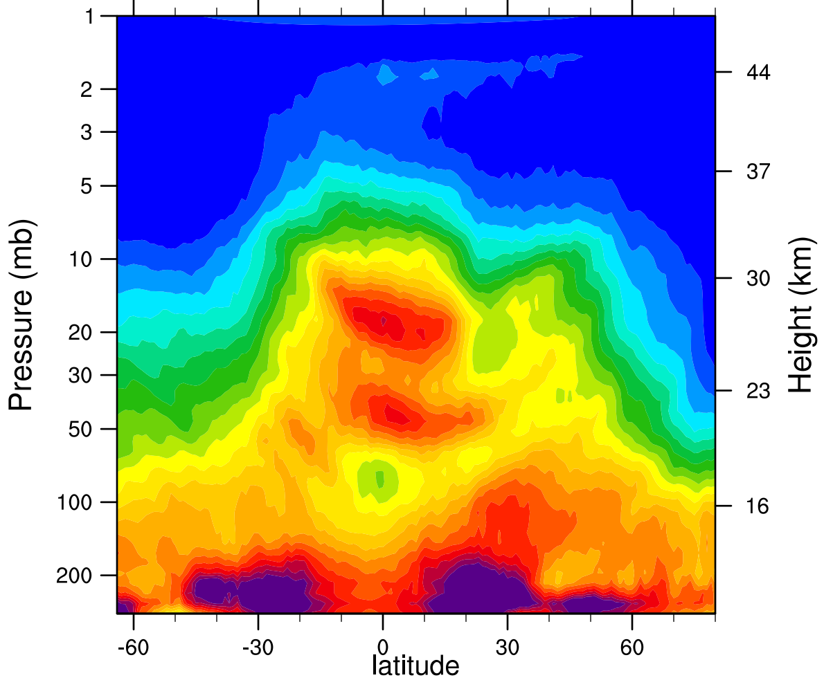
HIRDLSv6 2005d037 N2O_Combined (ppbv)
