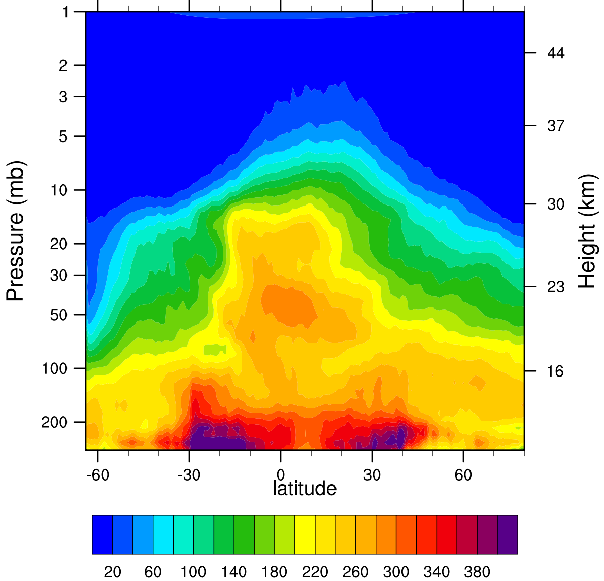
HIRDLSv6 2007d242 N2O_Combined (ppbv)
