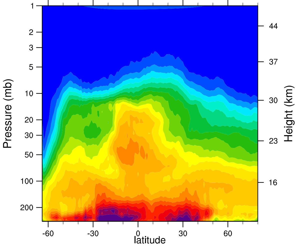
HIRDLSv6 2007d208 N2O_Combined (ppbv)
