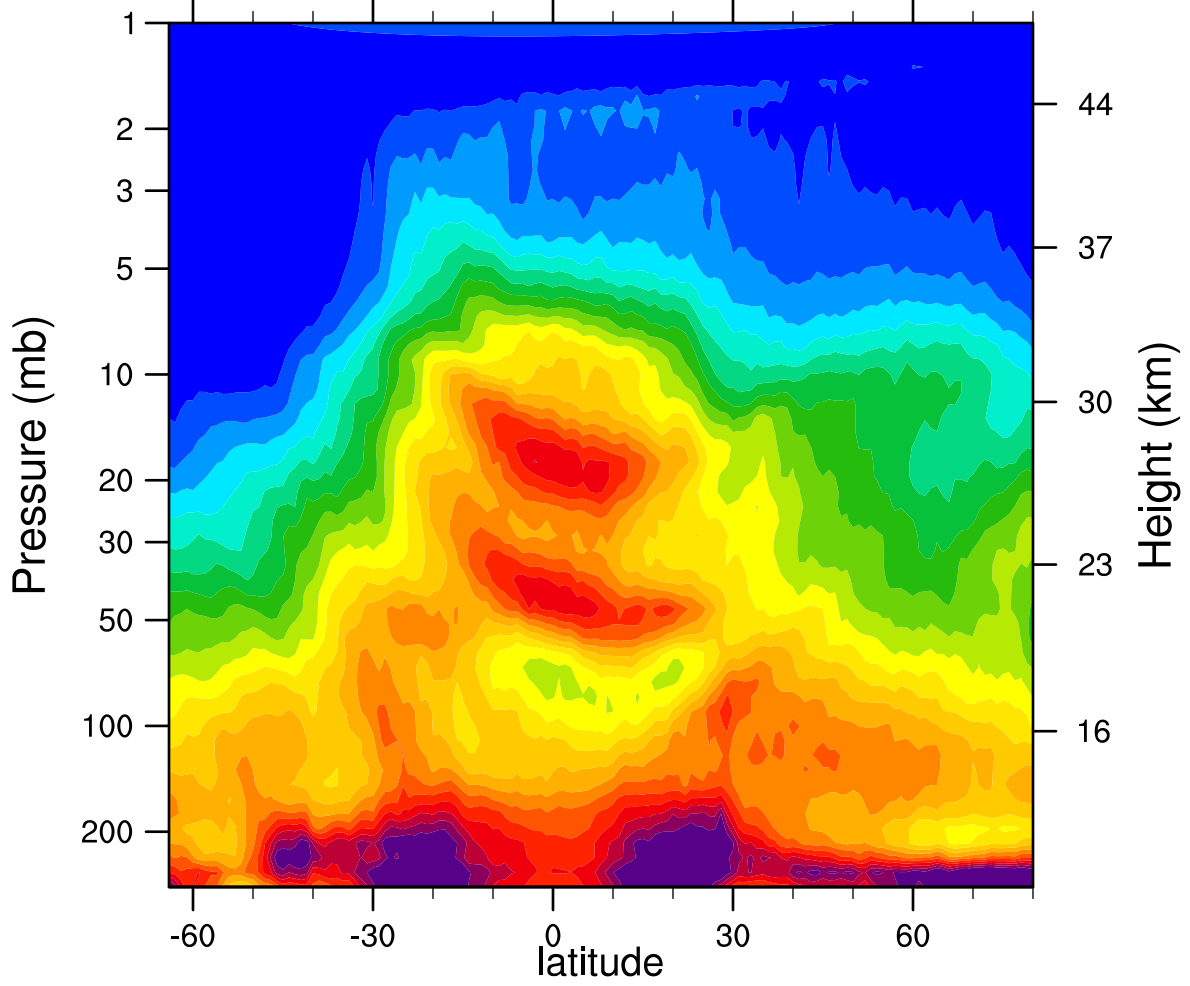
HIRDLSv6 2005d082 N2O_Combined (ppbv)
