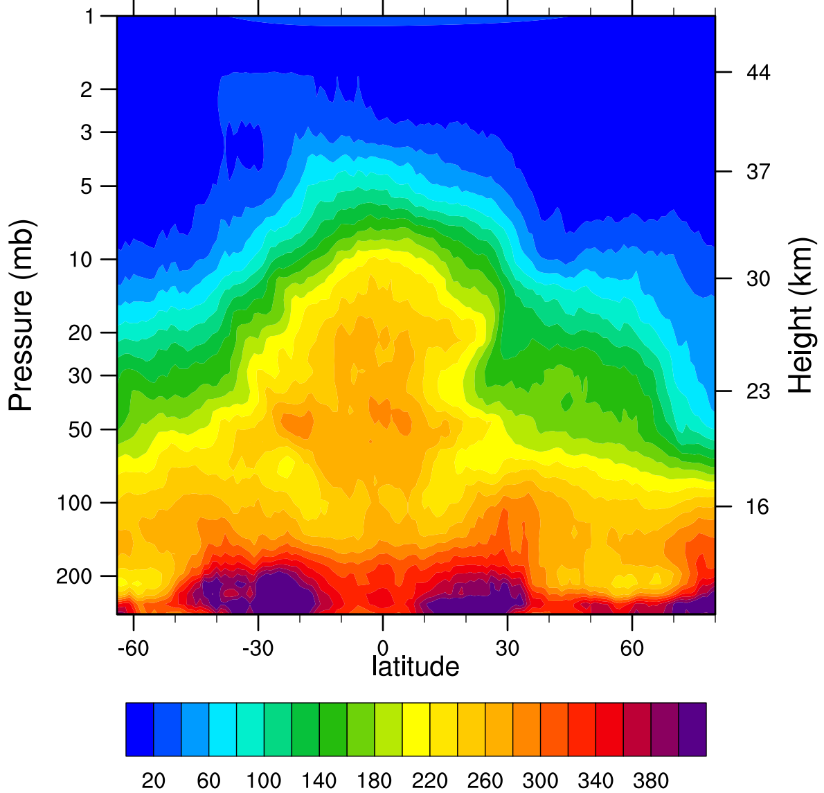
HIRDLSv6 2007d072 N2O_Combined (ppbv)
