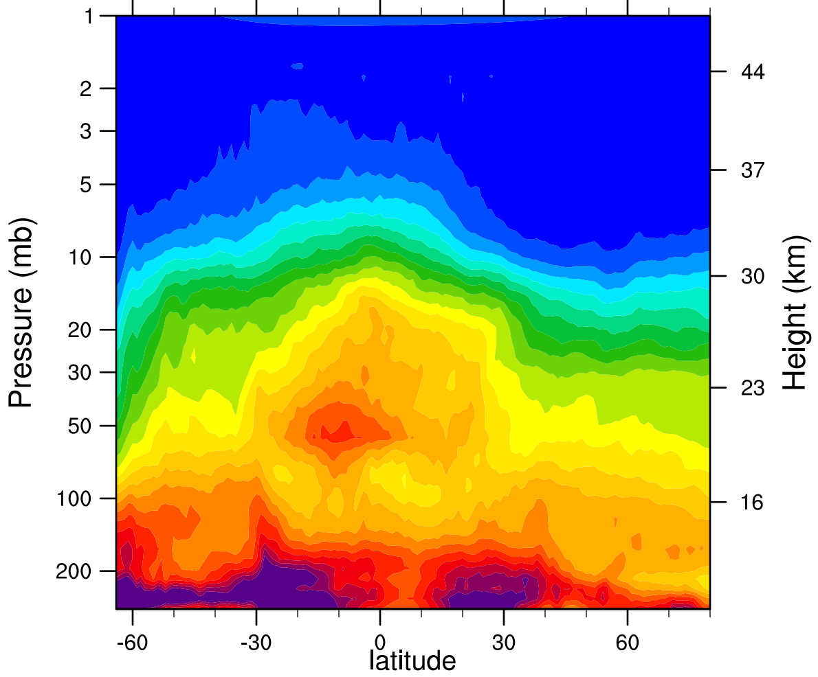
HIRDLSv6 2006d158 N2O_Combined (ppbv)
