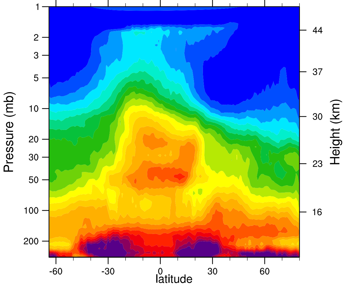
HIRDLSv6 2006d032 N2O_Combined (ppbv)
