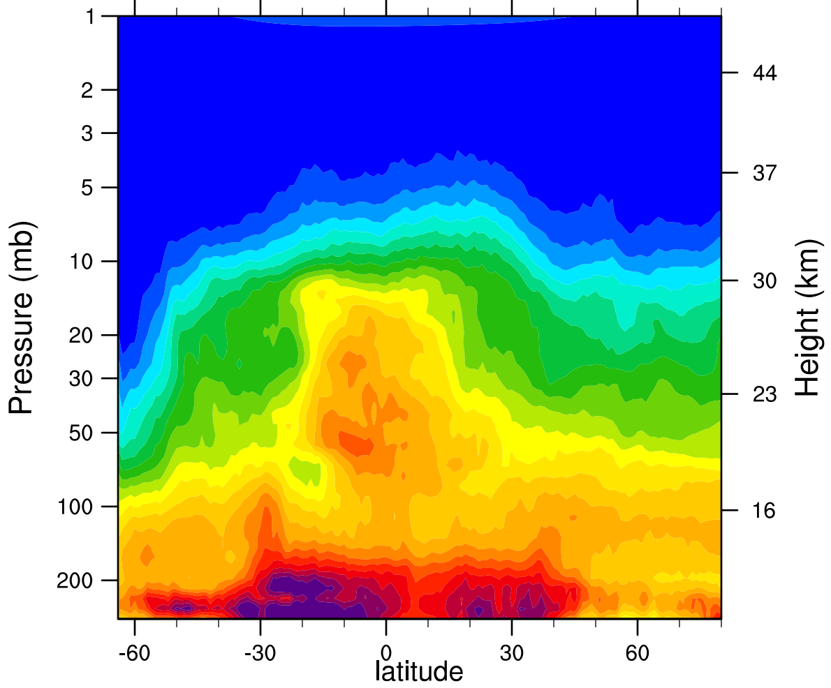
HIRDLSv6 2007d190 N2O_Combined (ppbv)
