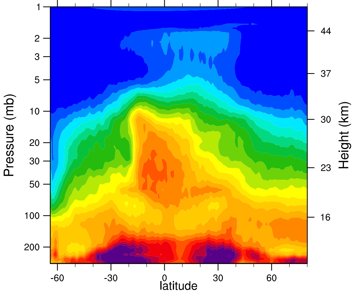
HIRDLSv6 2005d263 N2O_Combined (ppbv)
