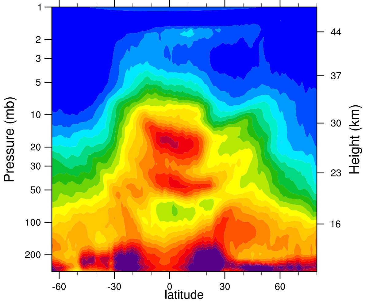
HIRDLSv6 2005d052 N2O_Combined (ppbv)
