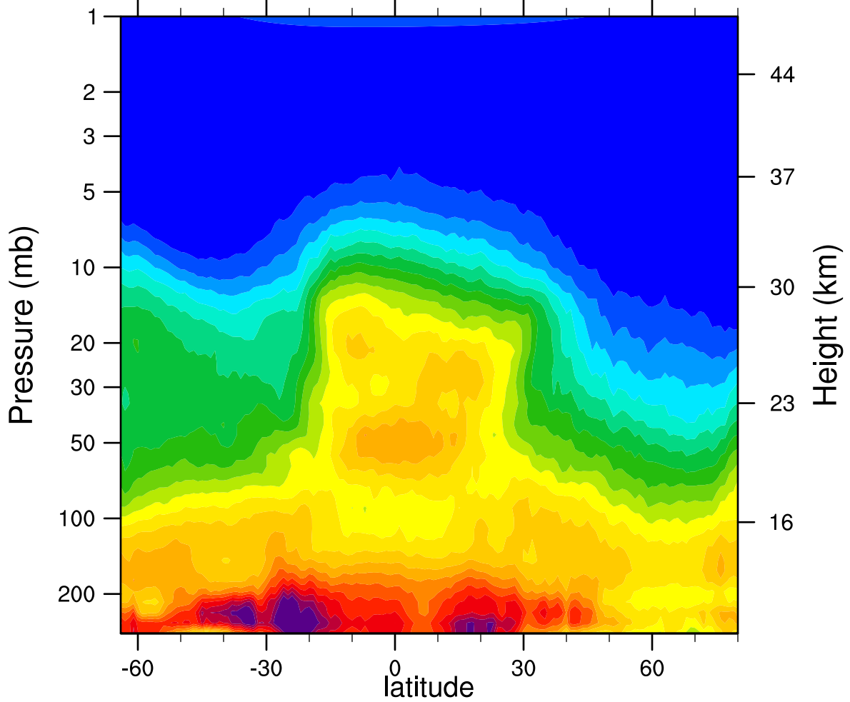
HIRDLSv6 2007d331 N2O_Combined (ppbv)
