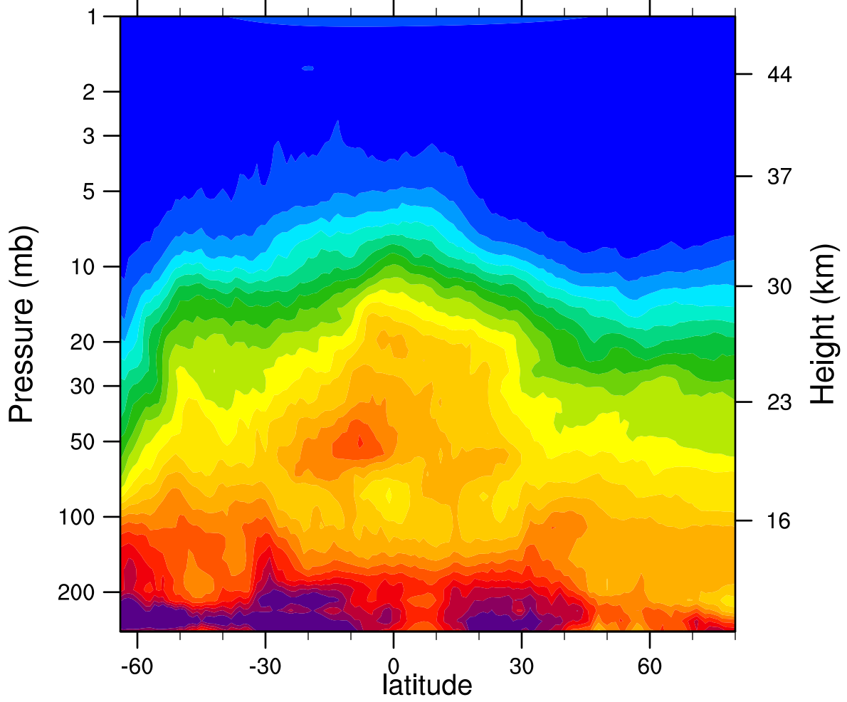
HIRDLSv6 2006d170 N2O_Combined (ppbv)
