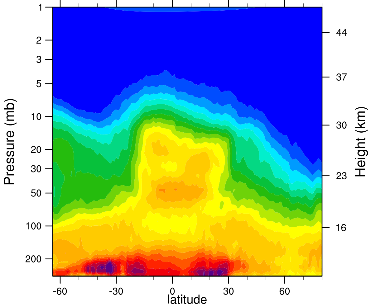
HIRDLSv6 2007d340 N2O_Combined (ppbv)
