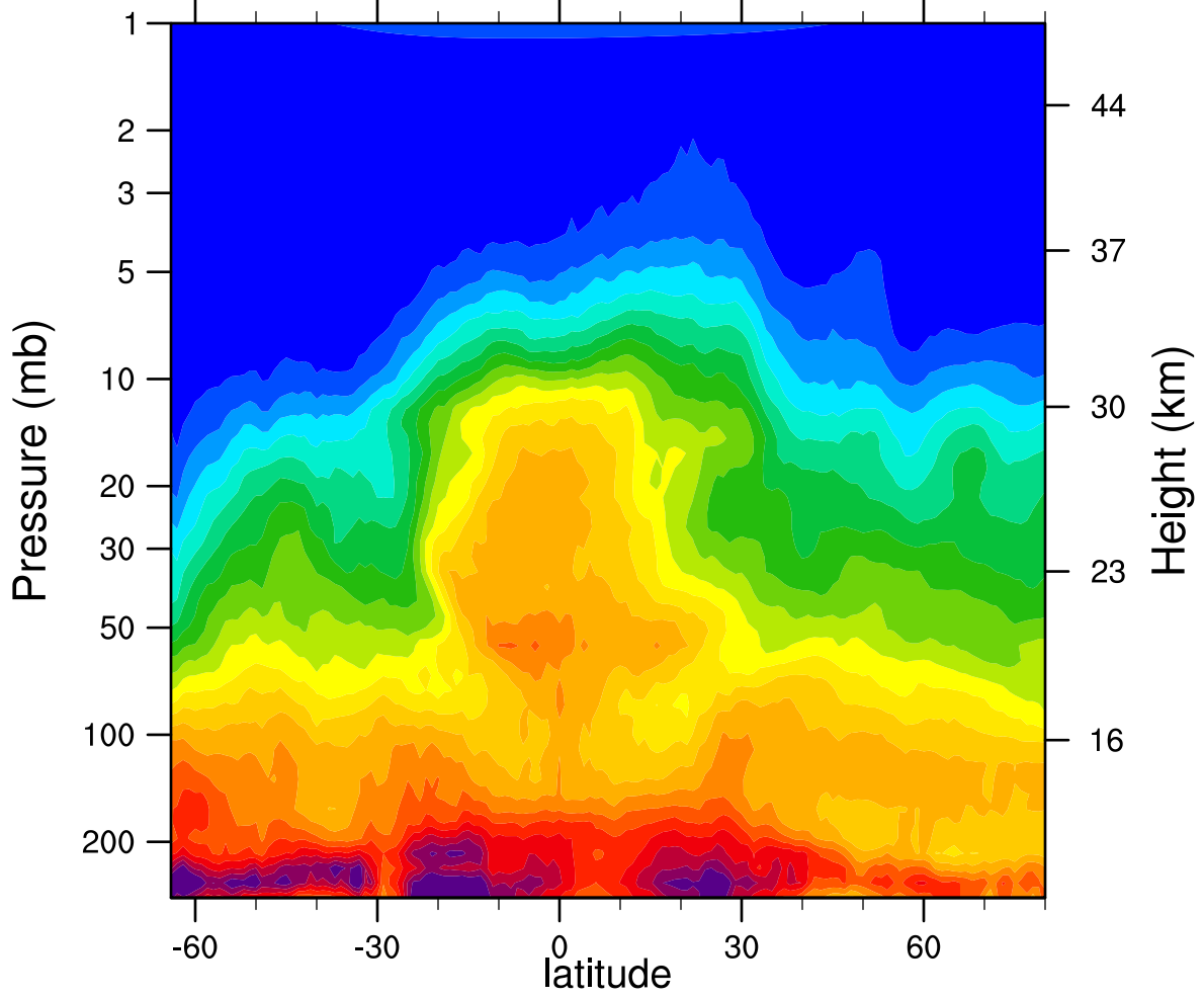
HIRDLSv6 2007d157 N2O_Combined (ppbv)
