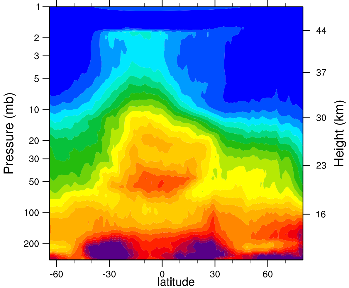
HIRDLSv6 2006d066 N2O_Combined (ppbv)
