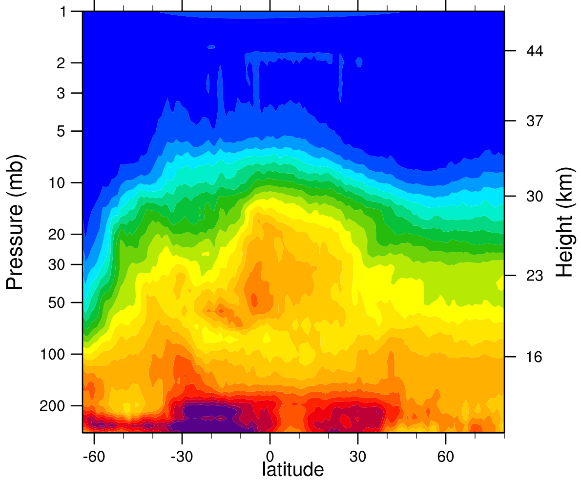
HIRDLSv6 2006d190 N2O_Combined (ppbv)
