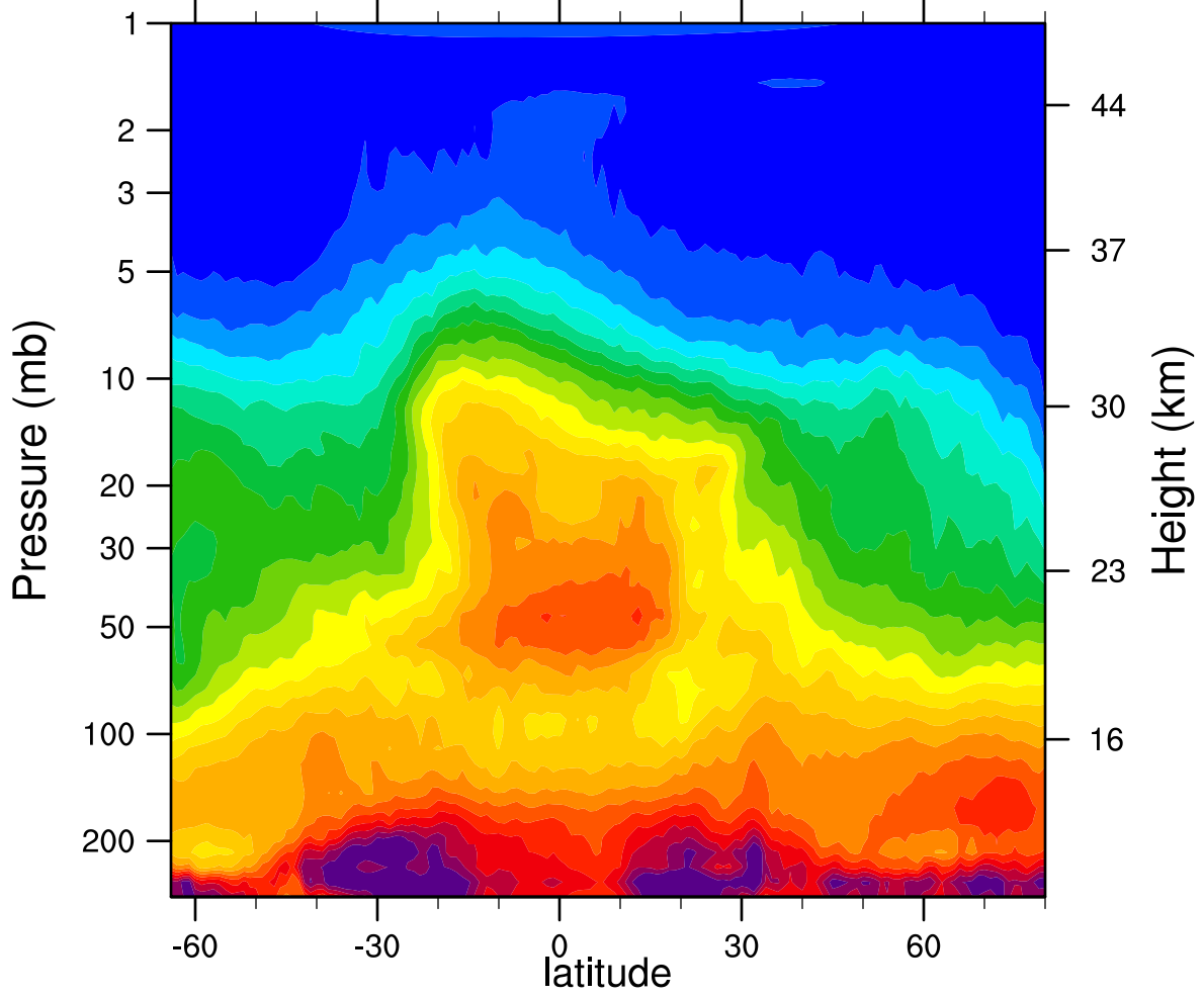
HIRDLSv6 2005d335 N2O_Combined (ppbv)
