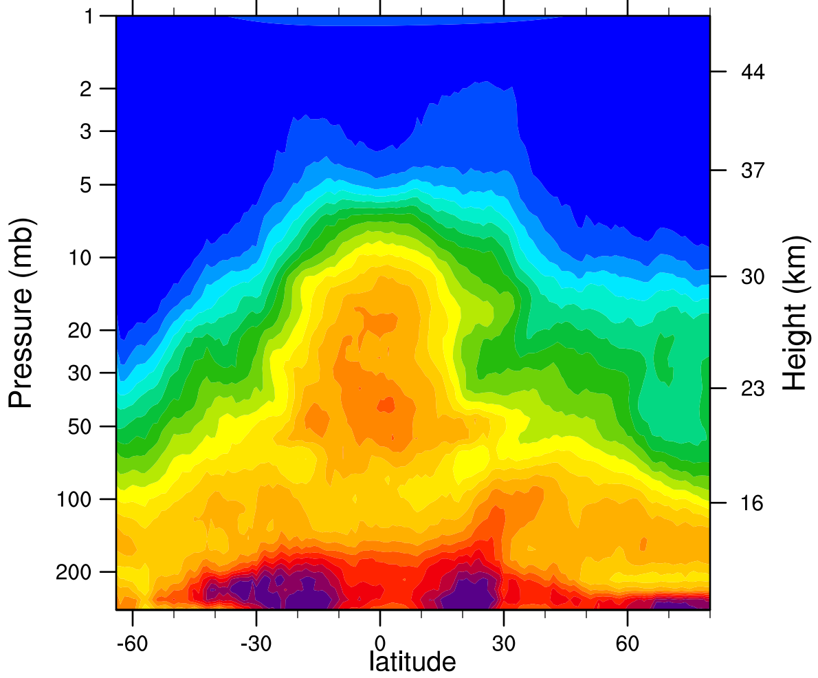
HIRDLSv6 2007d117 N2O_Combined (ppbv)
