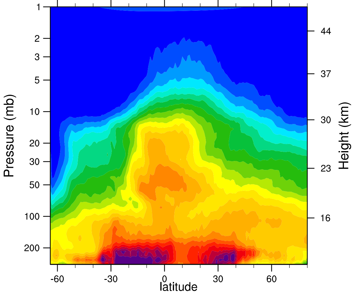
HIRDLSv6 2007d224 N2O_Combined (ppbv)
