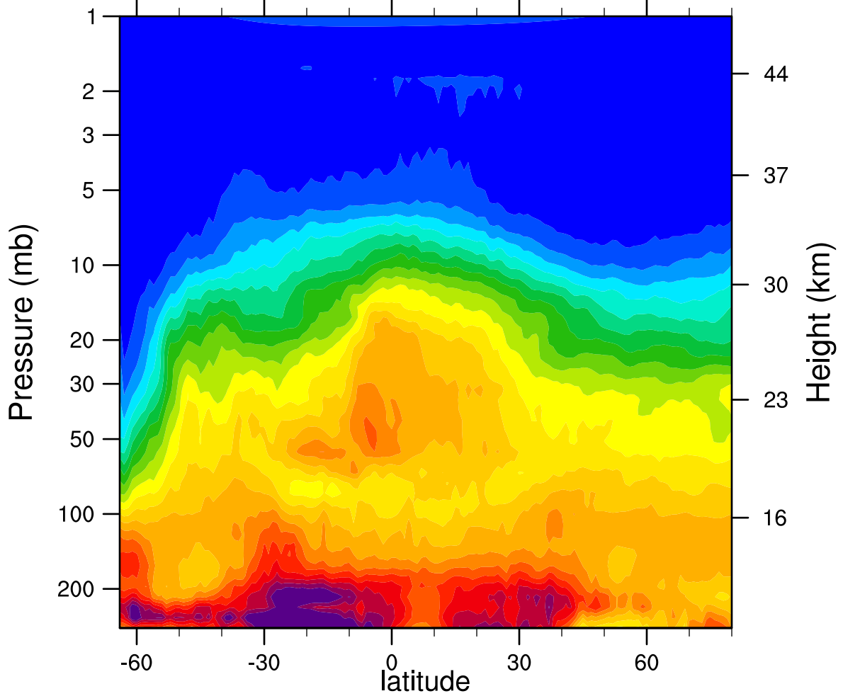
HIRDLSv6 2006d196 N2O_Combined (ppbv)
