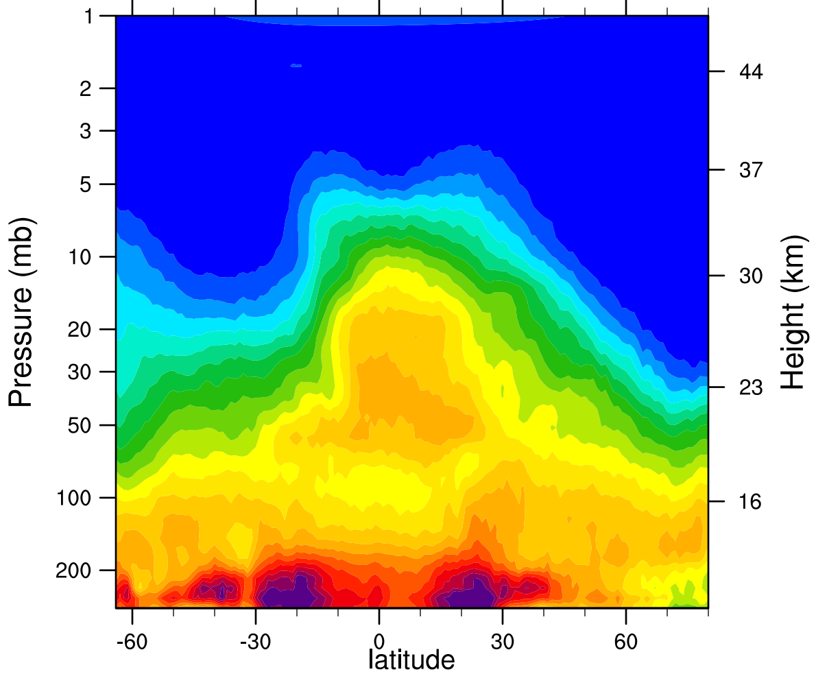
HIRDLSv6 2006d324 N2O_Combined (ppbv)
