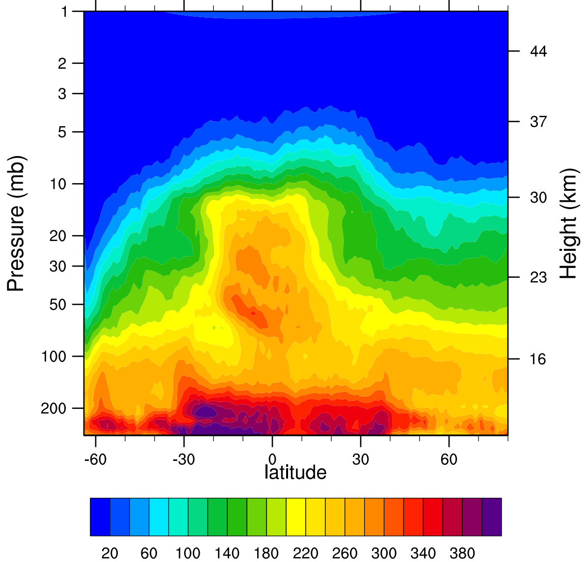
HIRDLSv6 2007d181 N2O_Combined (ppbv)
