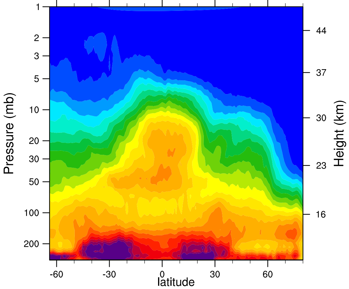
HIRDLSv6 2007d011 N2O_Combined (ppbv)
