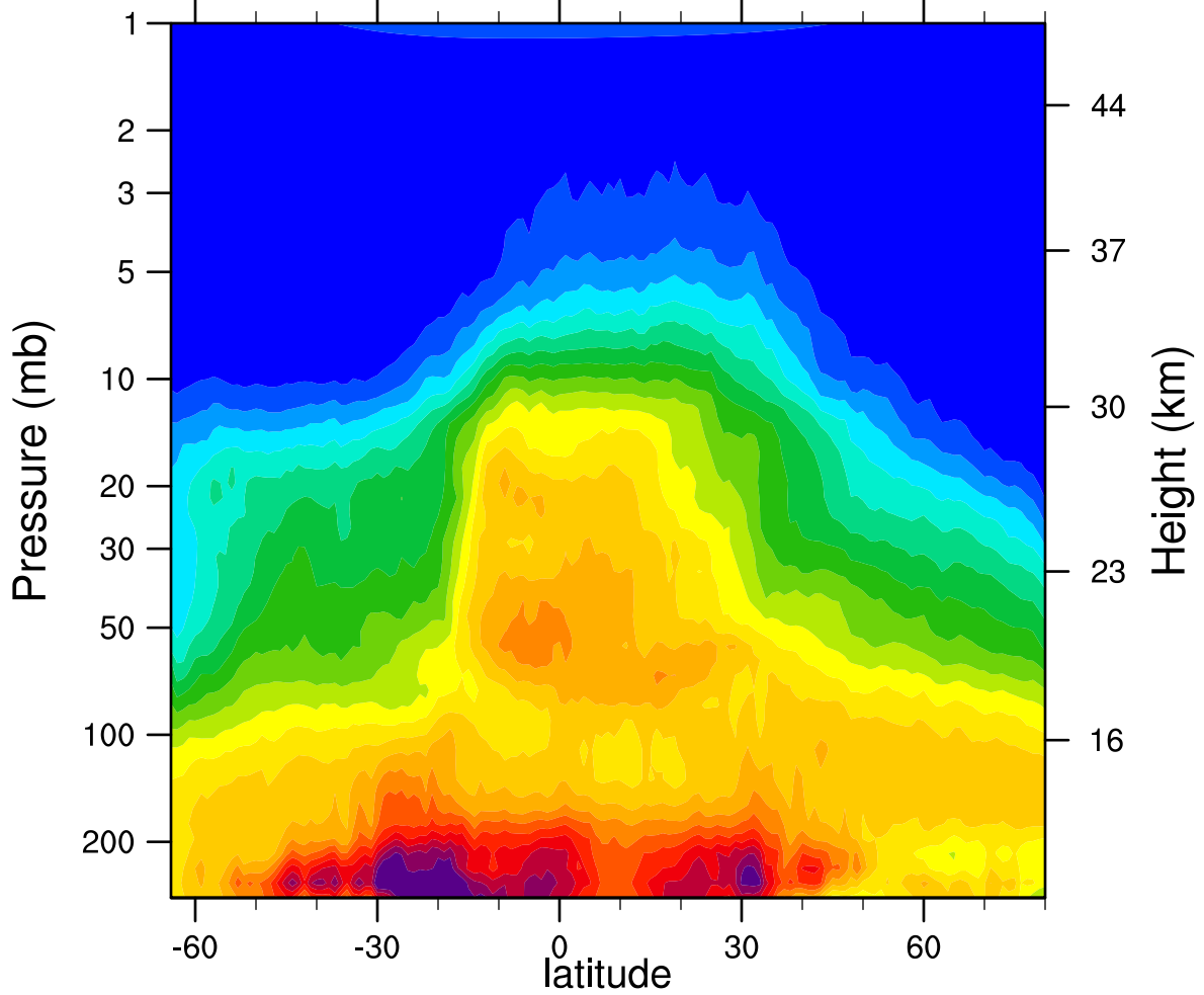
HIRDLSv6 2007d272 N2O_Combined (ppbv)
