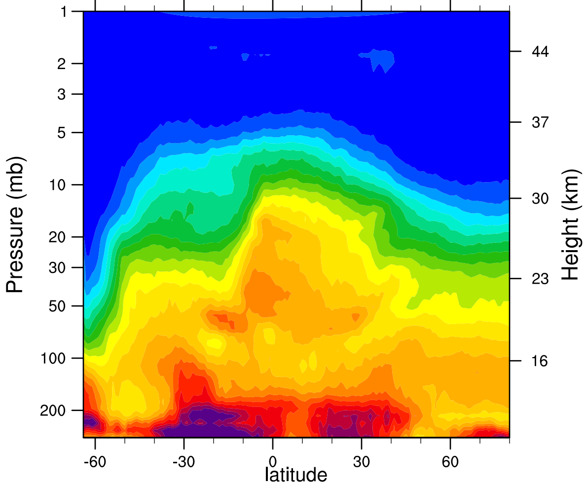
HIRDLSv6 2006d242 N2O_Combined (ppbv)
