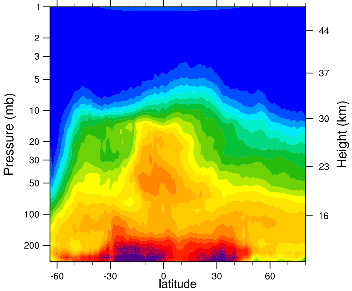
HIRDLSv6 2007d207 N2O_Combined (ppbv)
