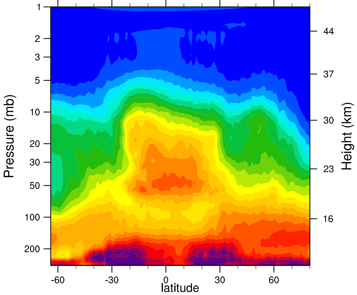
HIRDLSv6 2005d322 N2O_Combined (ppbv)
