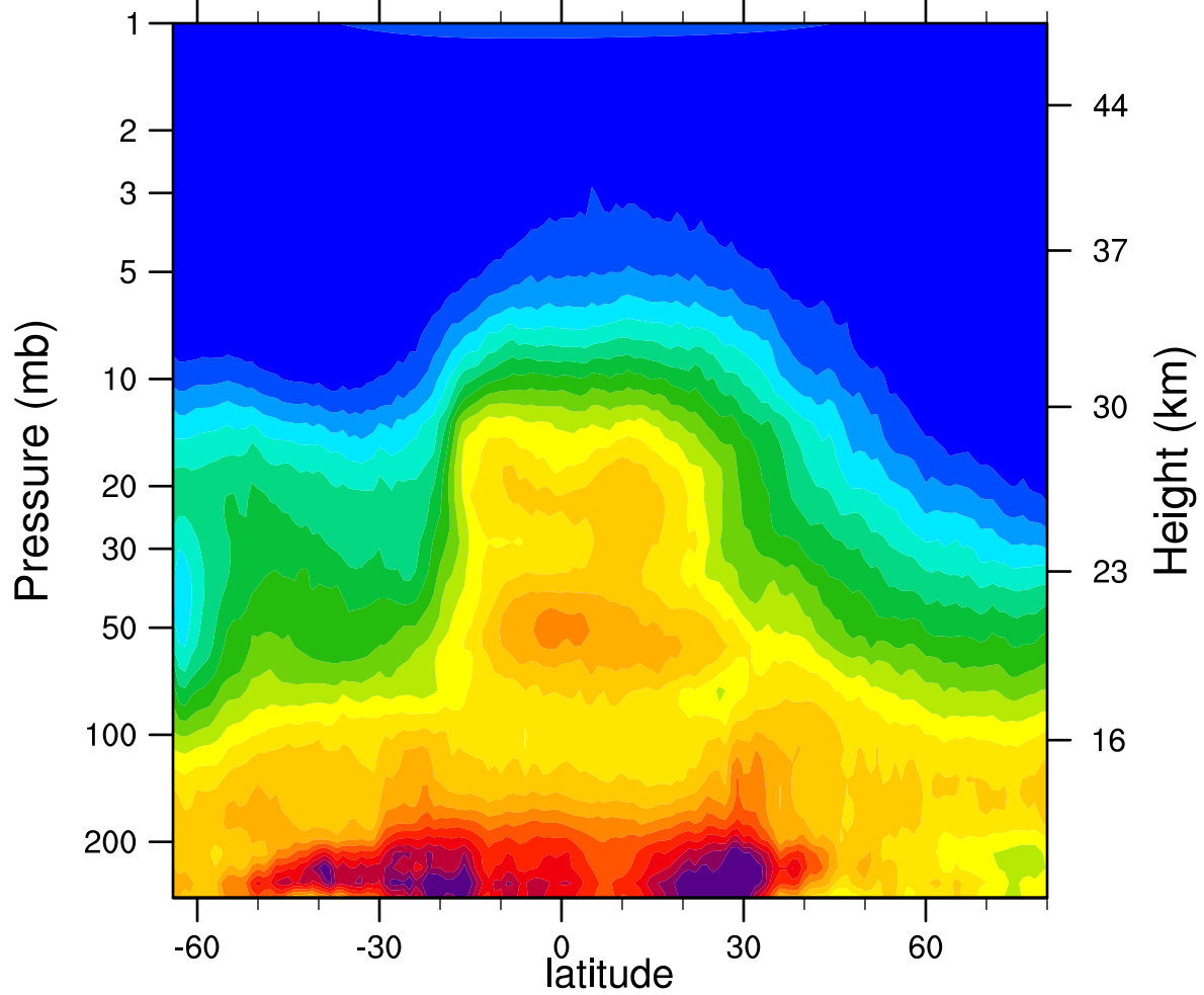
HIRDLSv6 2007d297 N2O_Combined (ppbv)
