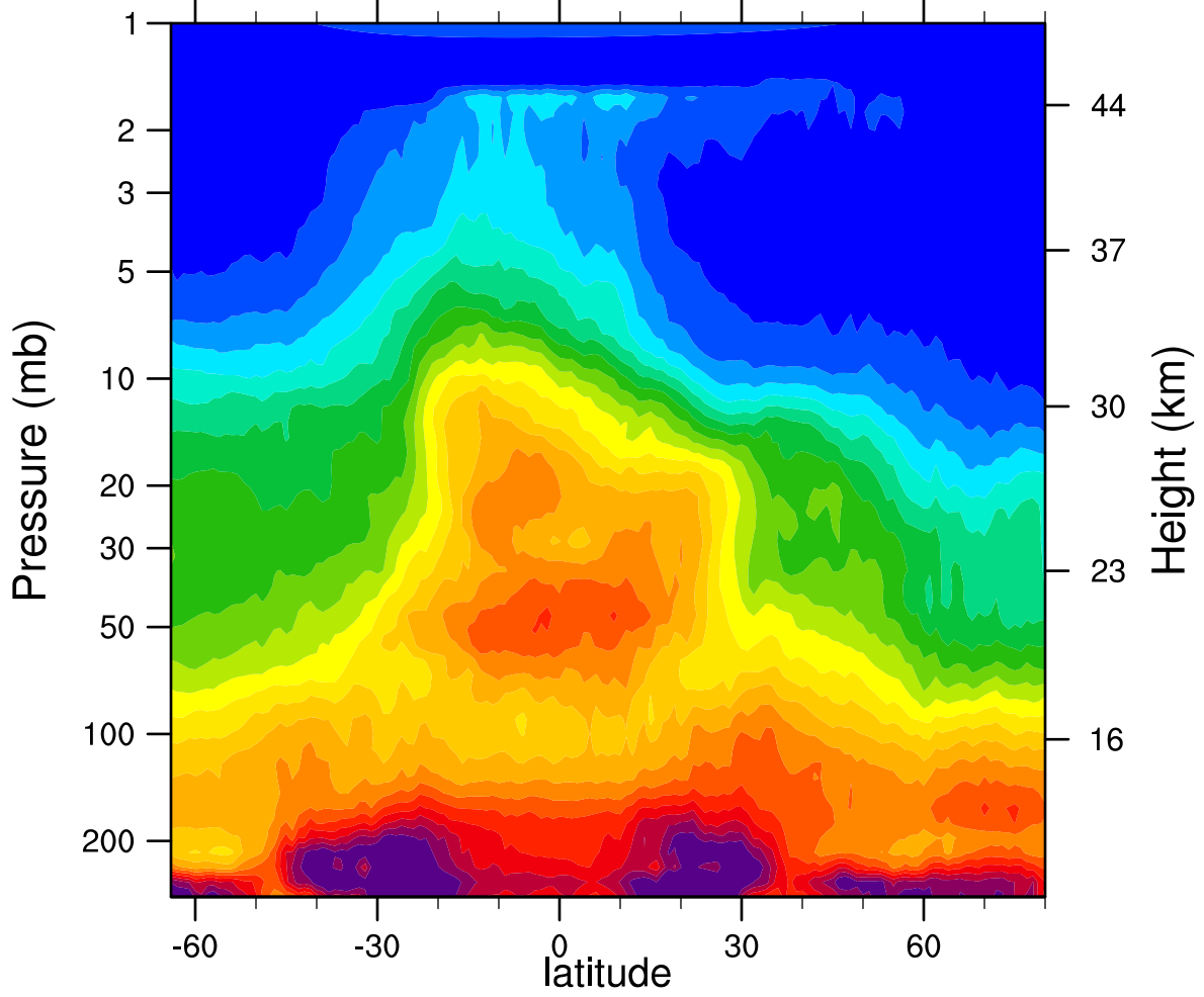
HIRDLSv6 2006d008 N2O_Combined (ppbv)
