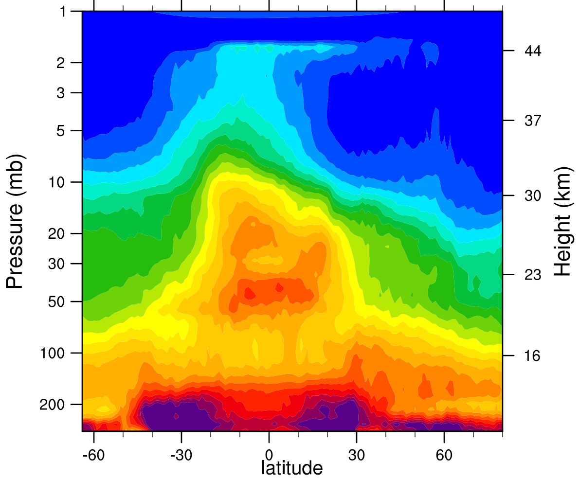
HIRDLSv6 2006d019 N2O_Combined (ppbv)
