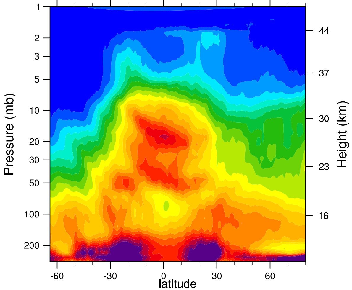
HIRDLSv6 2005d104 N2O_Combined (ppbv)
