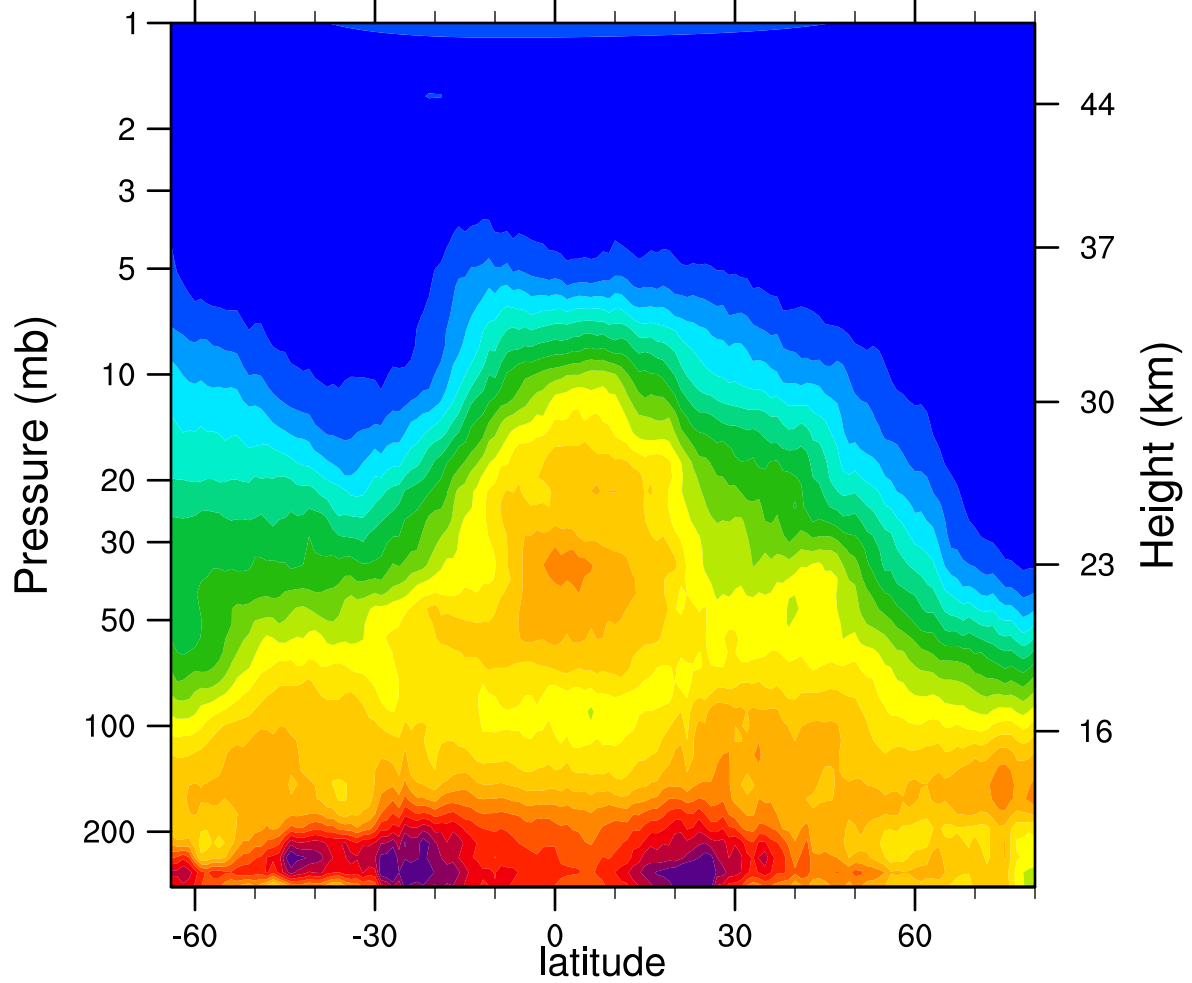
HIRDLSv6 2006d345 N2O_Combined (ppbv)
