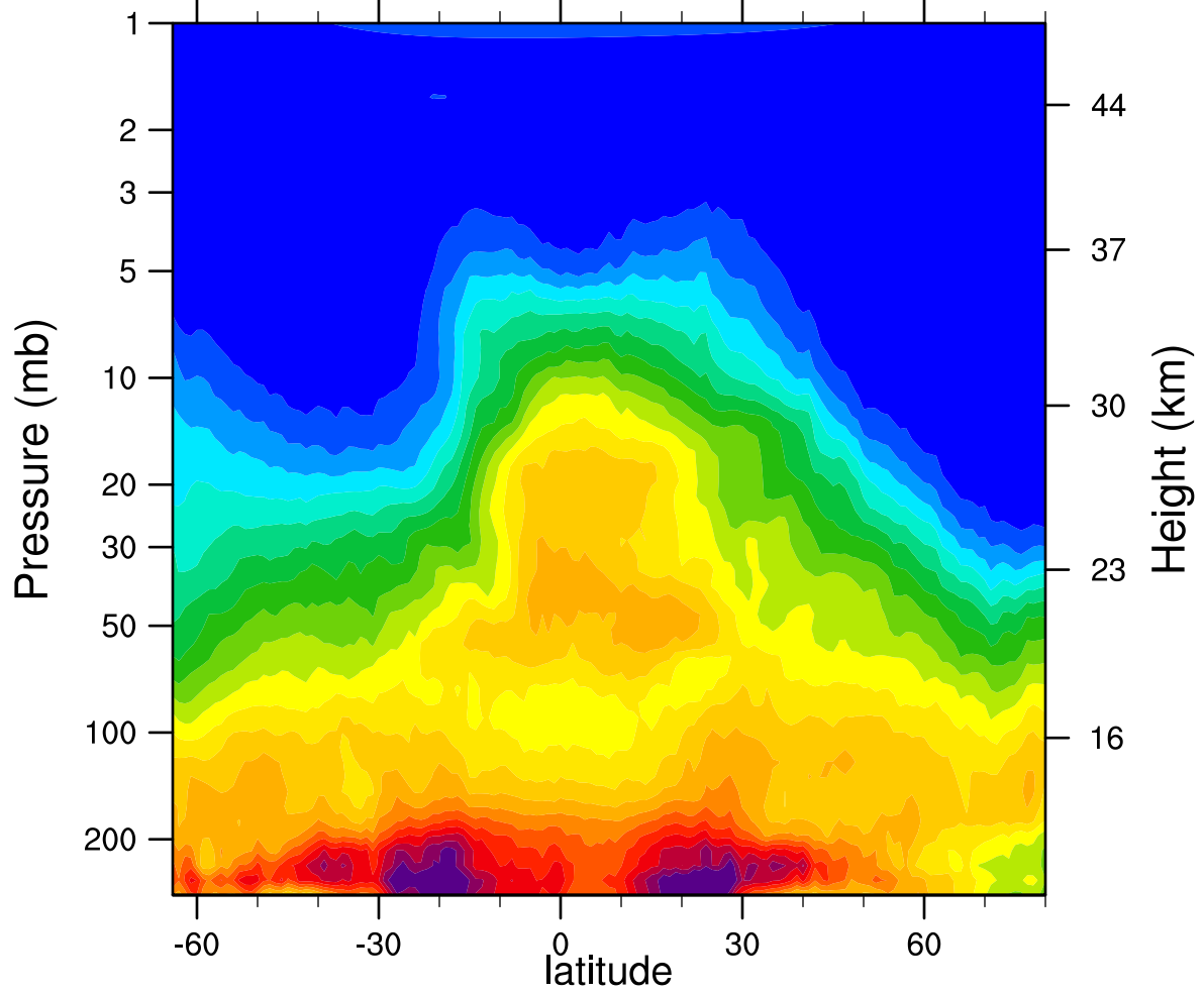
HIRDLSv6 2006d322 N2O_Combined (ppbv)
