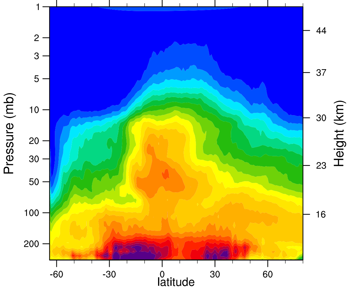
HIRDLSv6 2007d218 N2O_Combined (ppbv)
