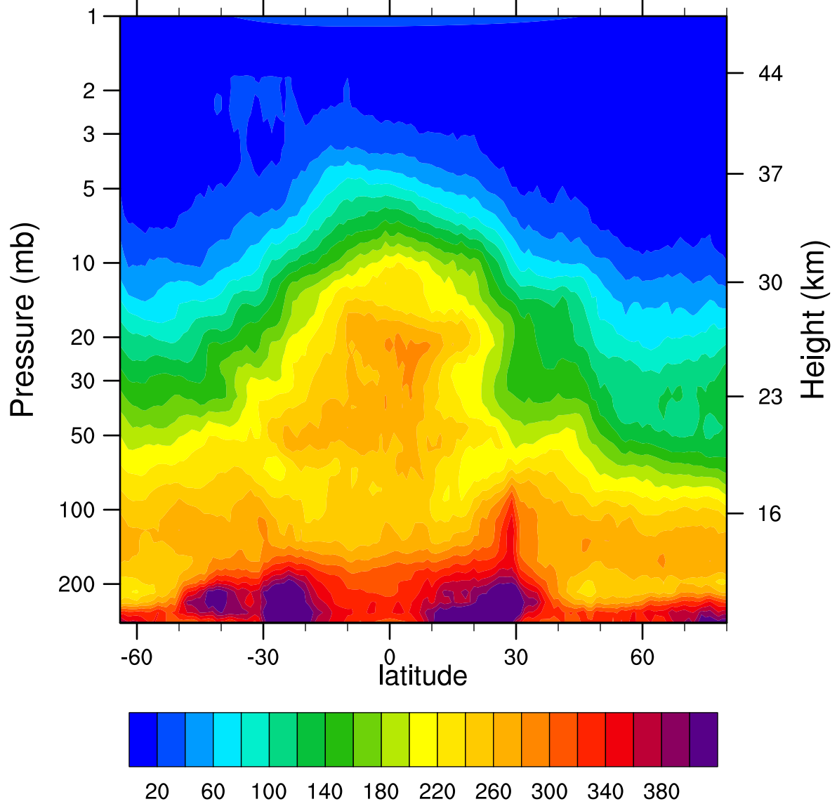
HIRDLSv6 2007d058 N2O_Combined (ppbv)
