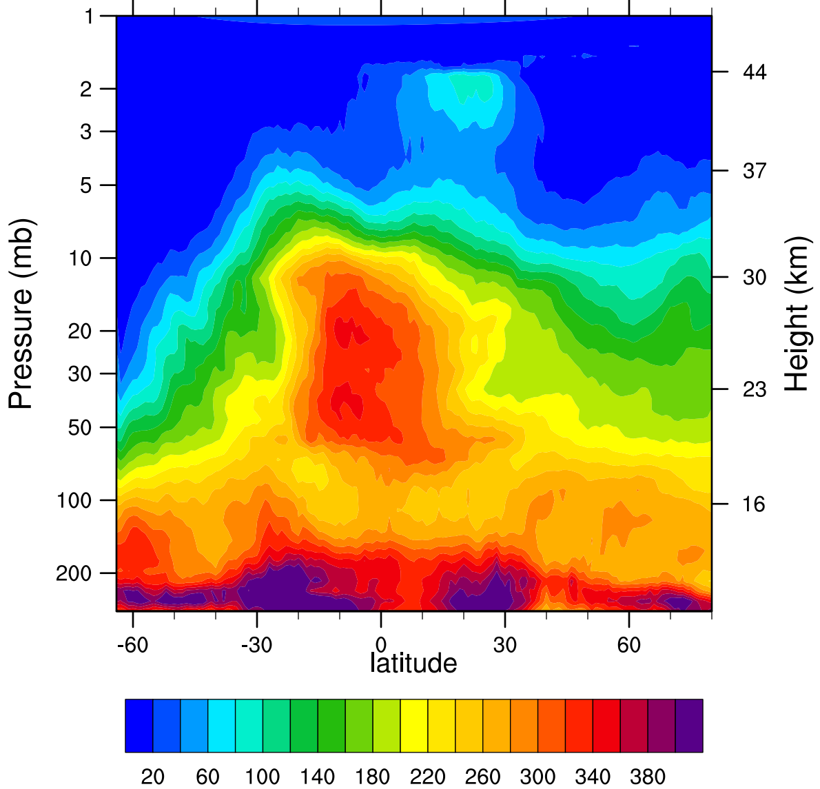
HIRDLSv6 2005d165 N2O_Combined (ppbv)
