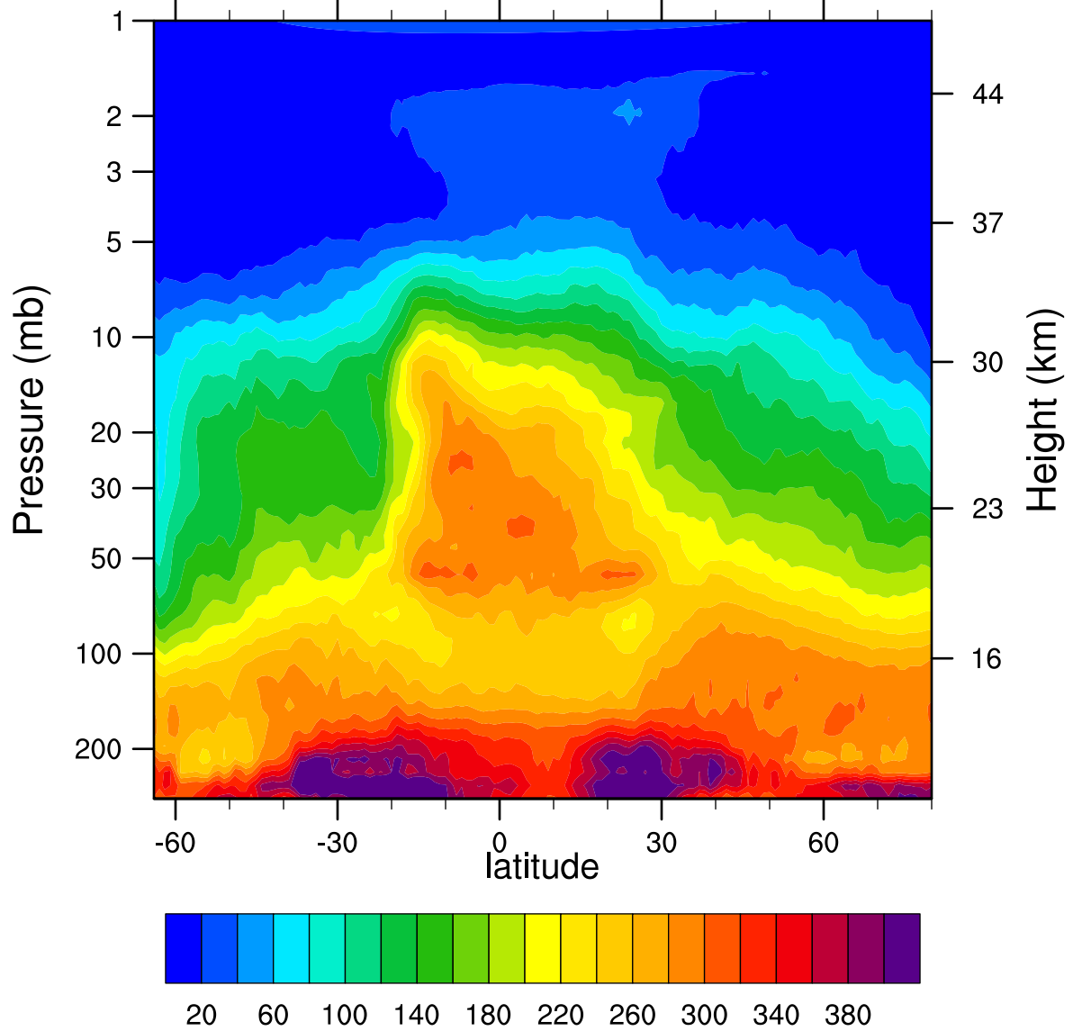
HIRDLSv6 2005d293 N2O_Combined (ppbv)
