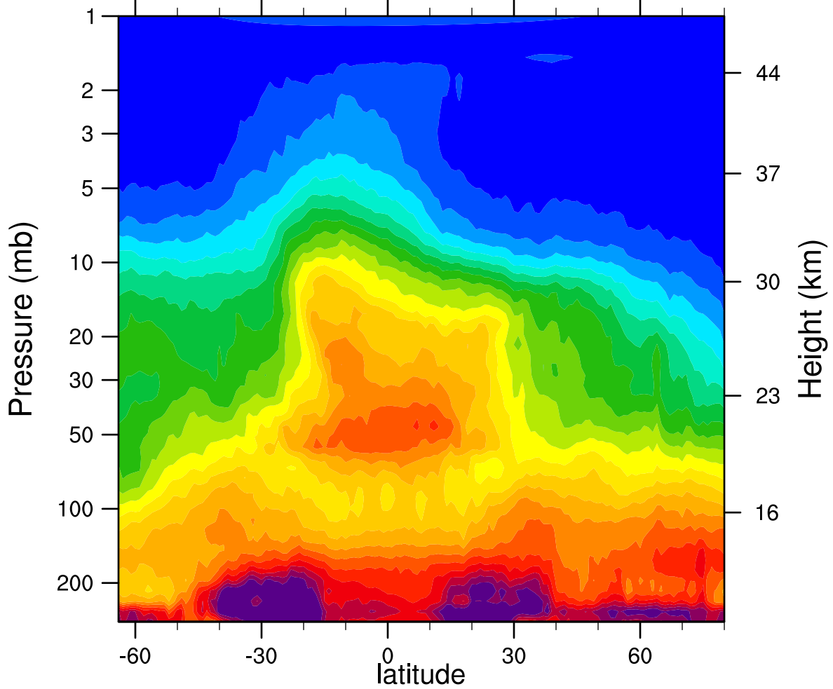
HIRDLSv6 2005d347 N2O_Combined (ppbv)
