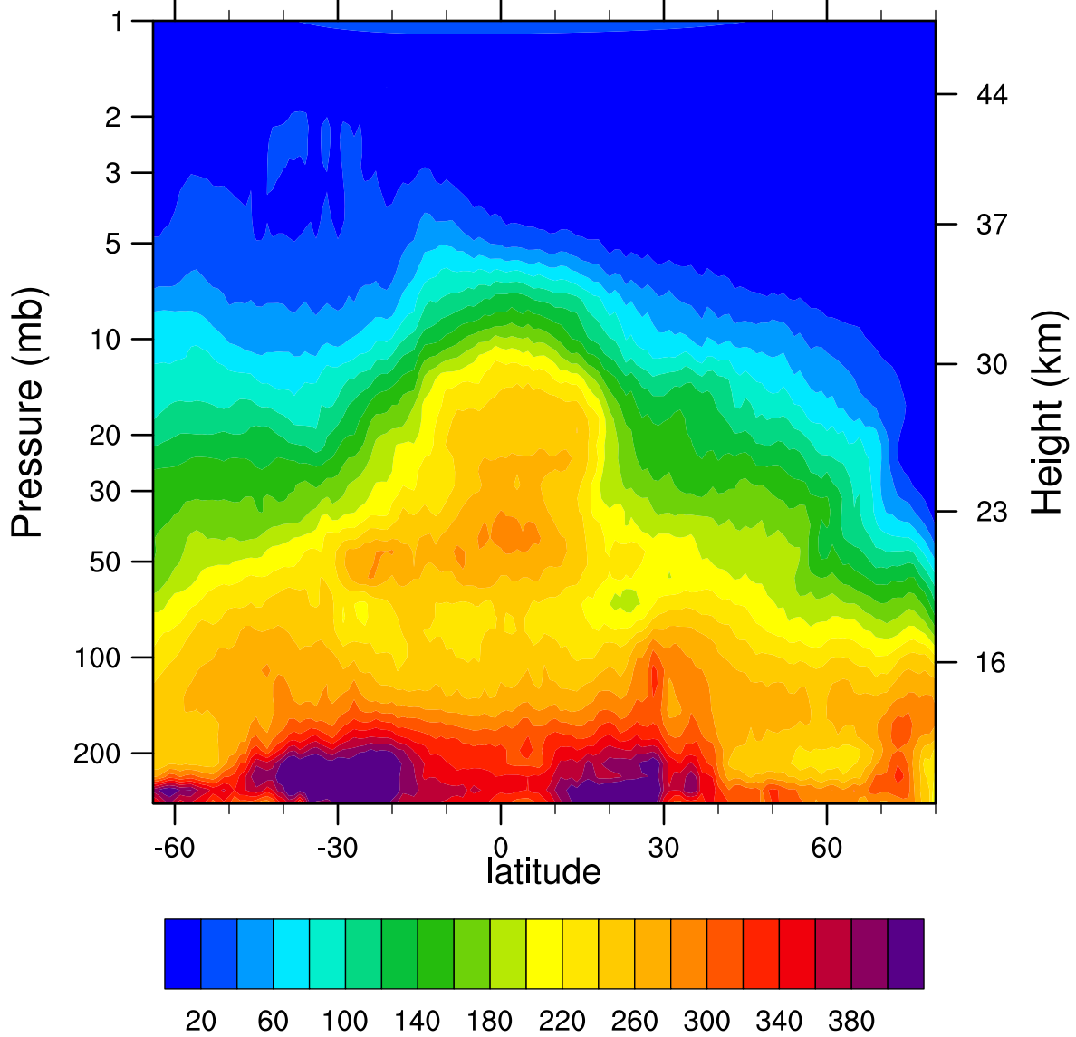
HIRDLSv6 2006d365 N2O_Combined (ppbv)
