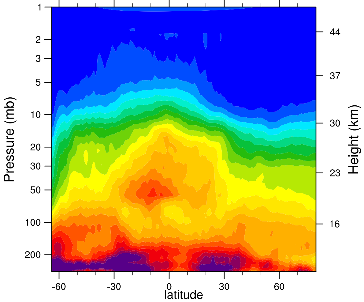
HIRDLSv6 2006d160 N2O_Combined (ppbv)
