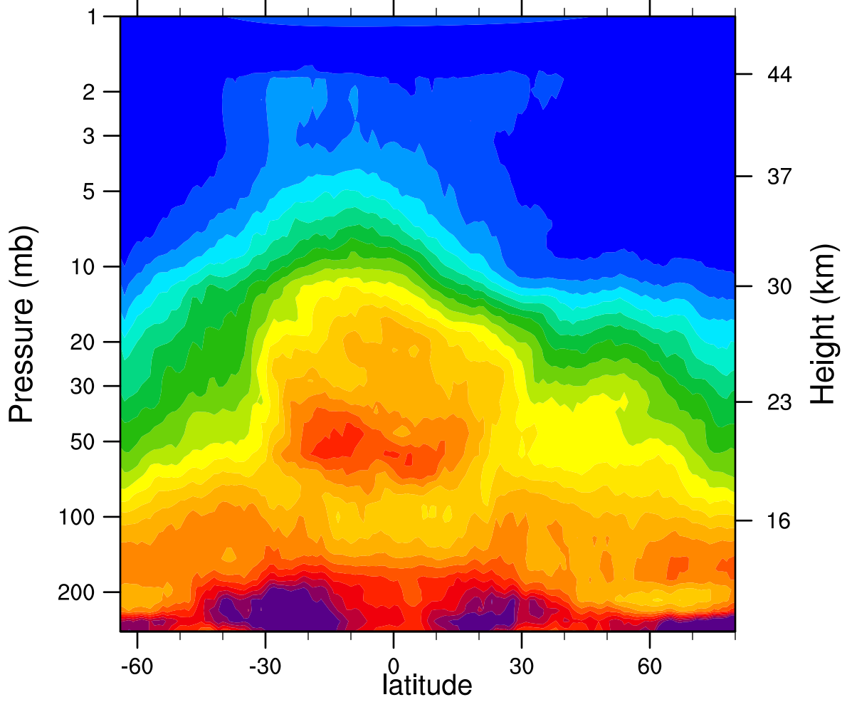
HIRDLSv6 2006d107 N2O_Combined (ppbv)
