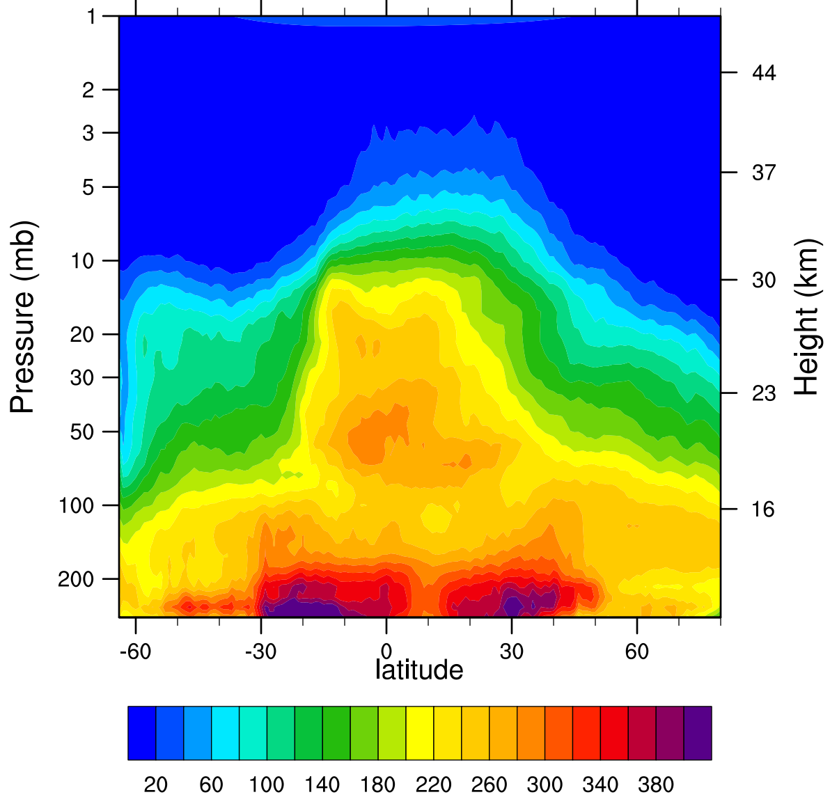
HIRDLSv6 2007d260 N2O_Combined (ppbv)
