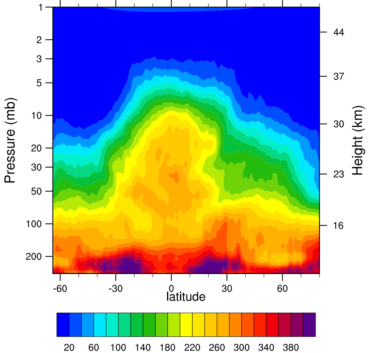
HIRDLSv6 2007d080 N2O_Combined (ppbv)
