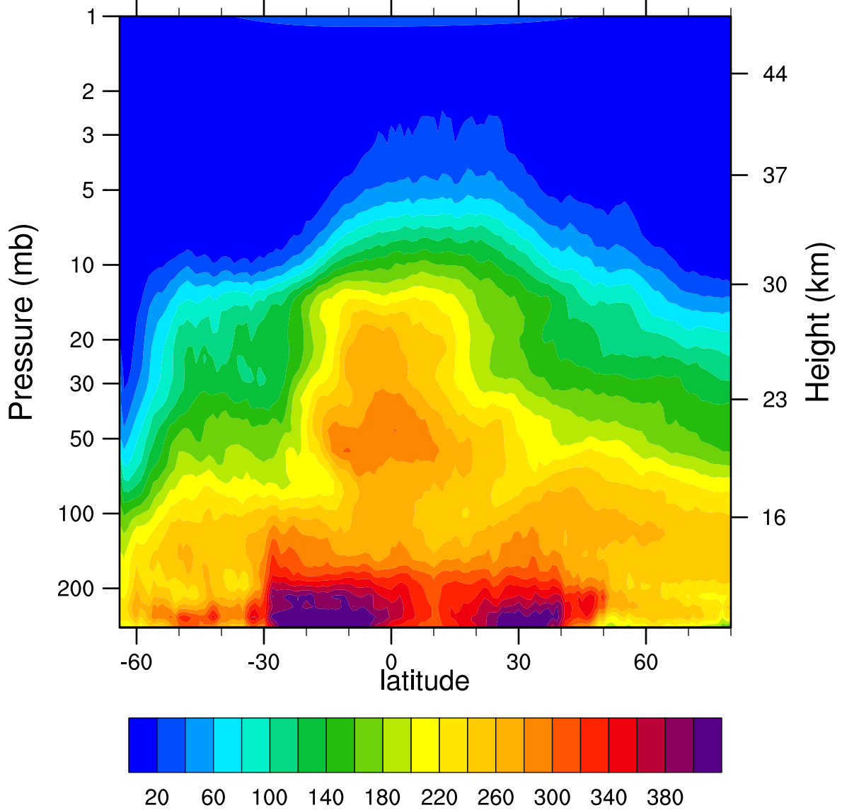
HIRDLSv6 2007d214 N2O_Combined (ppbv)
