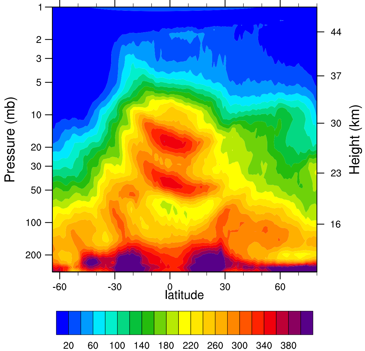
HIRDLSv6 2005d085 N2O_Combined (ppbv)
