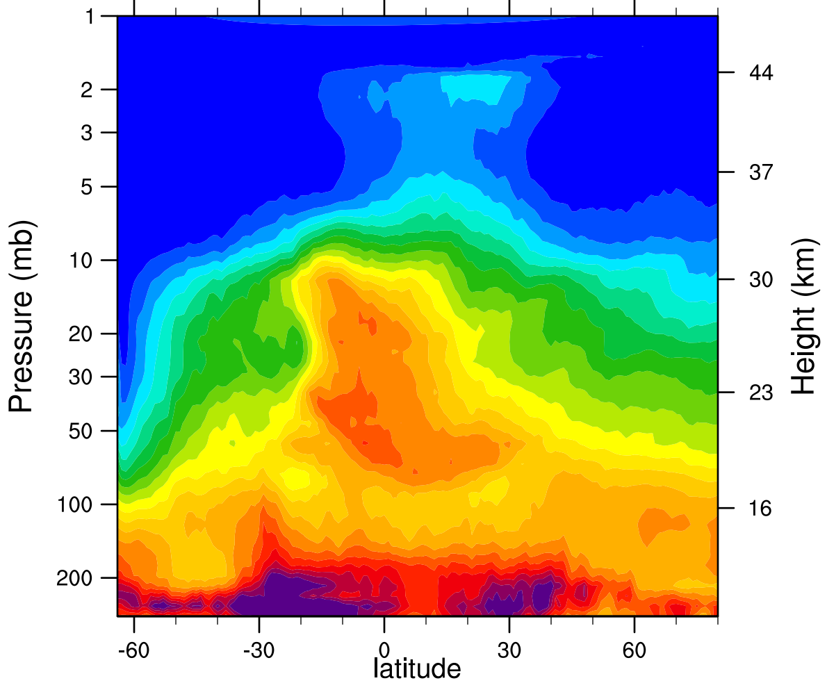
HIRDLSv6 2005d232 N2O_Combined (ppbv)
