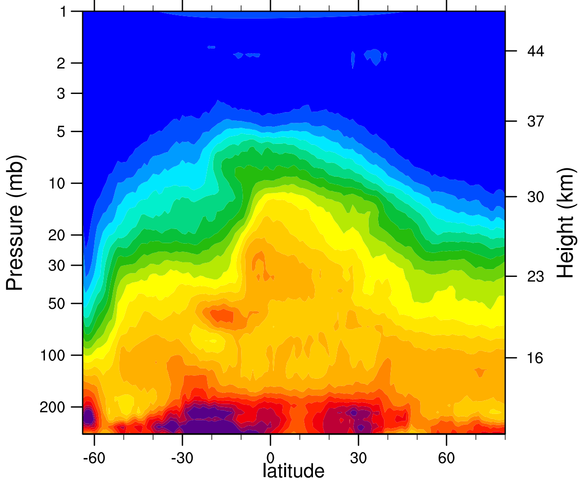
HIRDLSv6 2006d260 N2O_Combined (ppbv)
