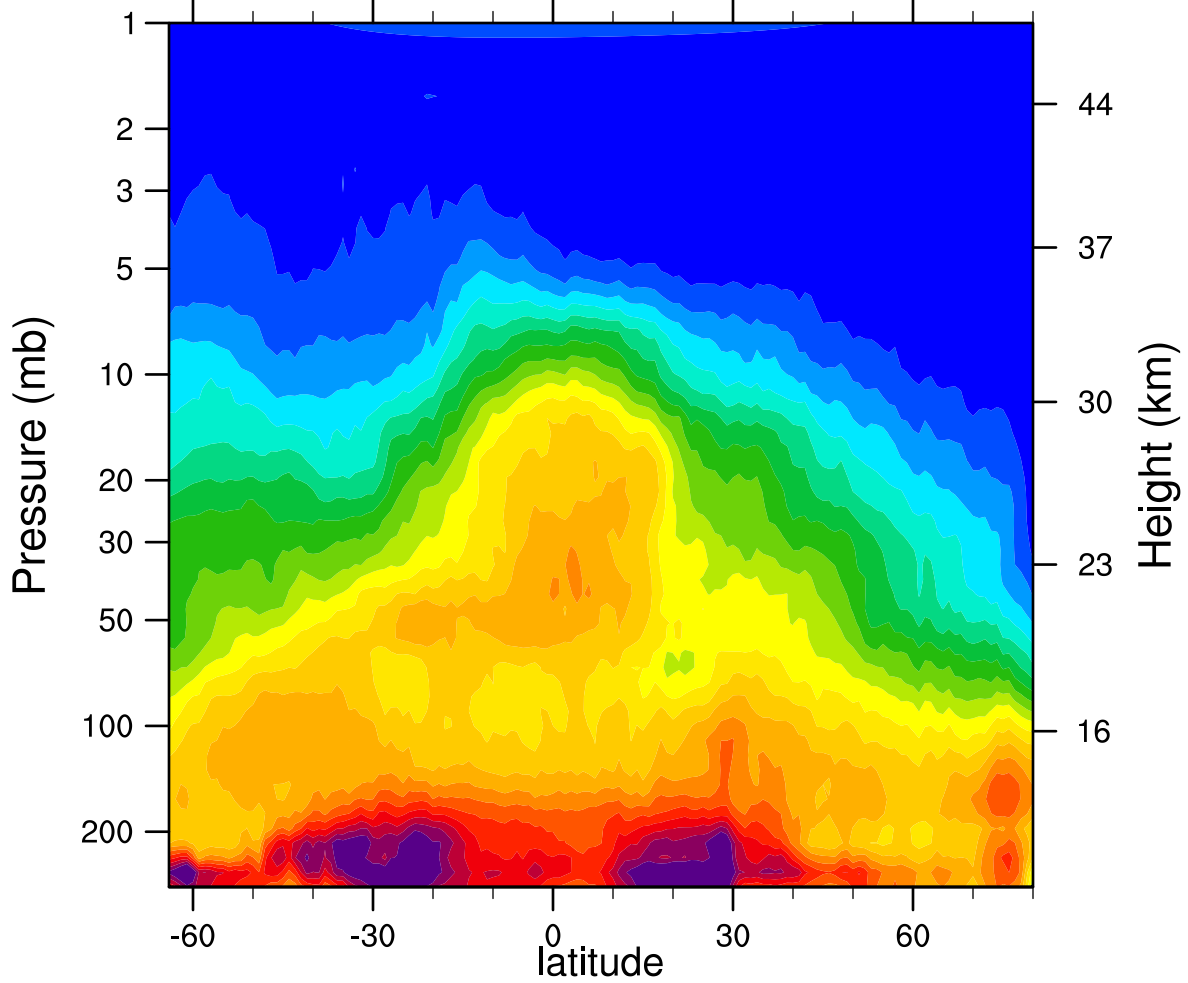
HIRDLSv6 2006d360 N2O_Combined (ppbv)
