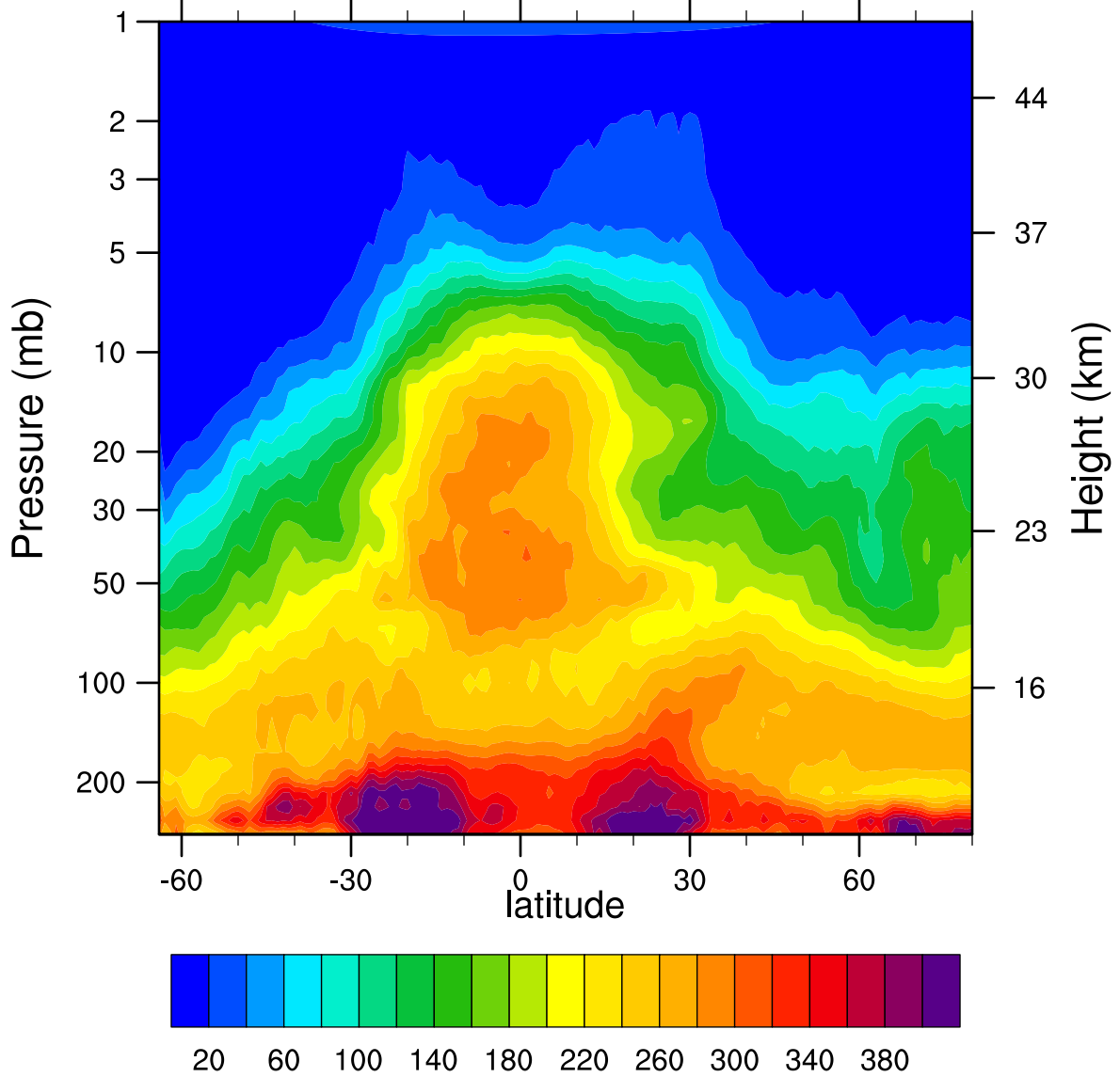
HIRDLSv6 2007d122 N2O_Combined (ppbv)
