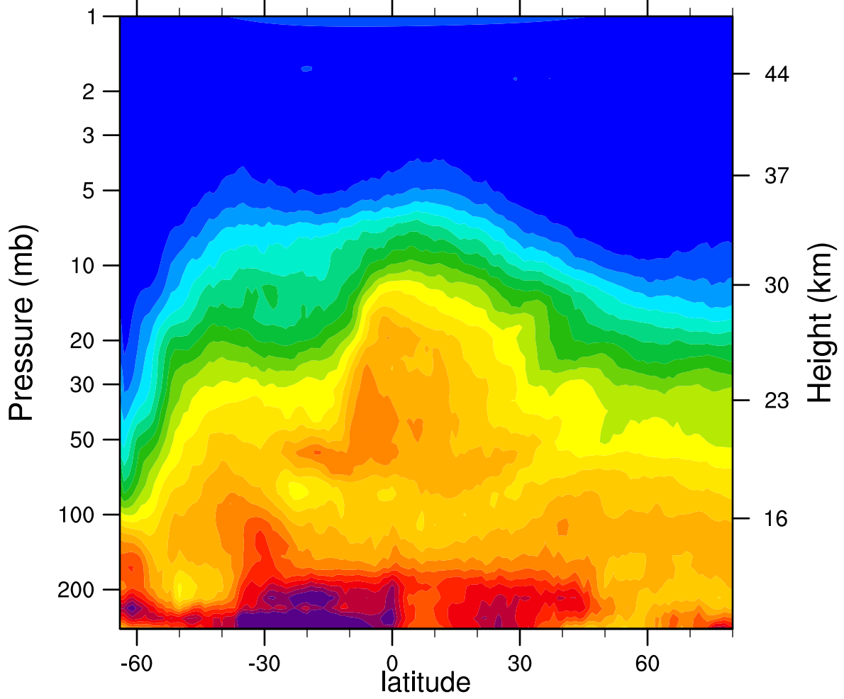
HIRDLSv6 2006d227 N2O_Combined (ppbv)
