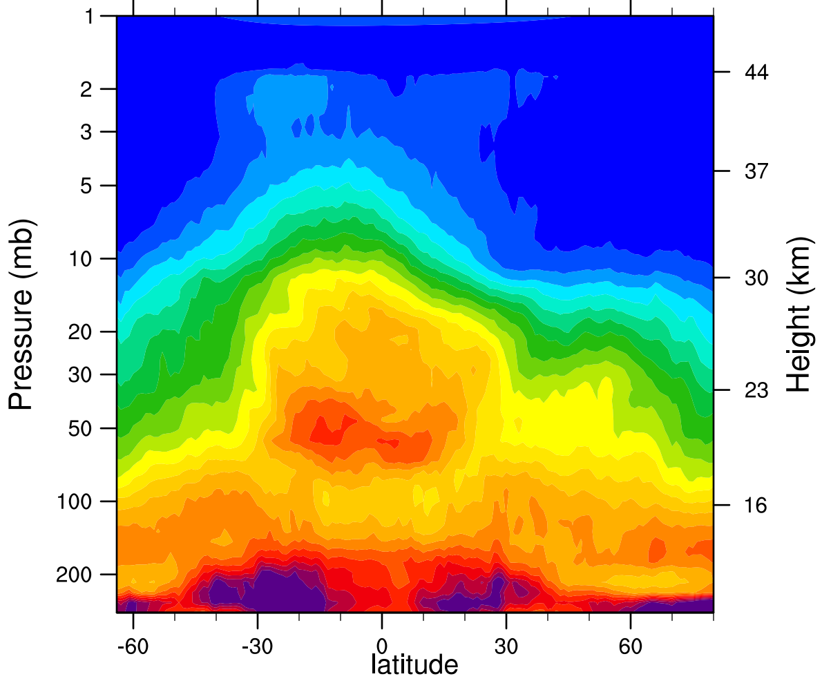
HIRDLSv6 2006d105 N2O_Combined (ppbv)
