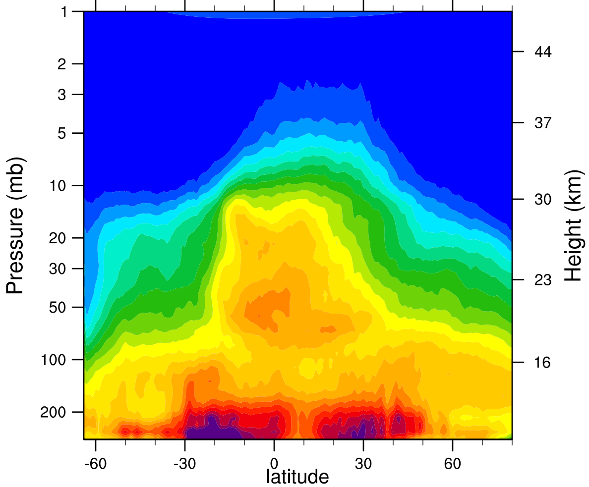
HIRDLSv6 2007d256 N2O_Combined (ppbv)
