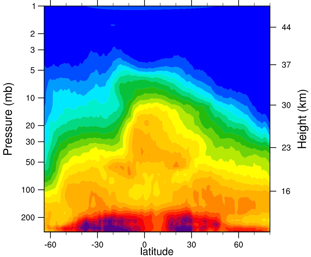
HIRDLSv6 2006d288 N2O_Combined (ppbv)
