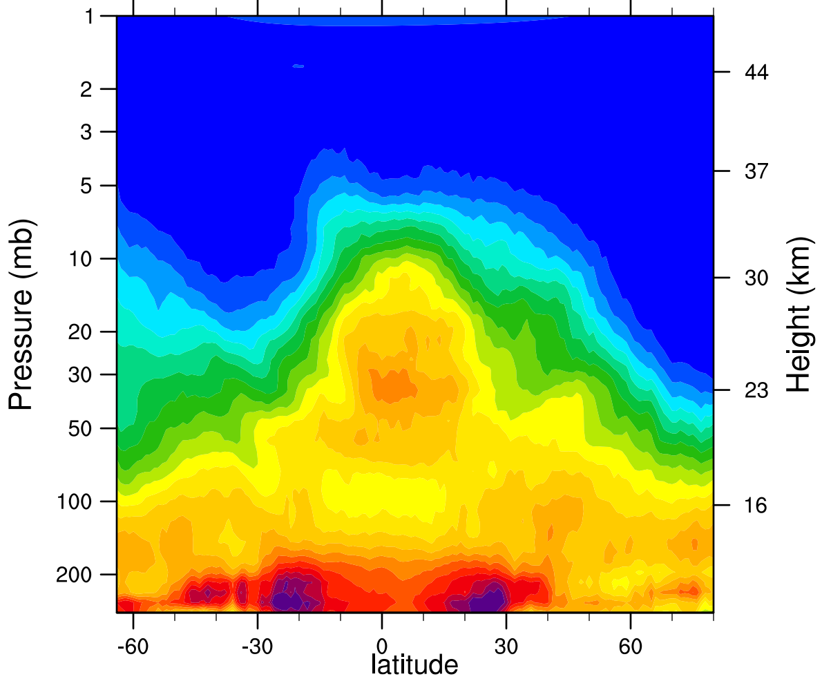
HIRDLSv6 2006d339 N2O_Combined (ppbv)
