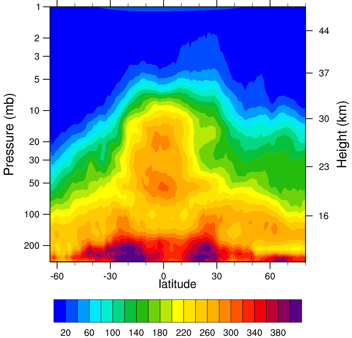
HIRDLSv6 2007d131 N2O_Combined (ppbv)
