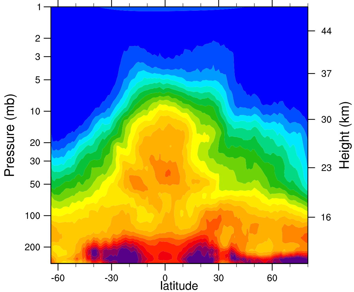
HIRDLSv6 2007d099 N2O_Combined (ppbv)
