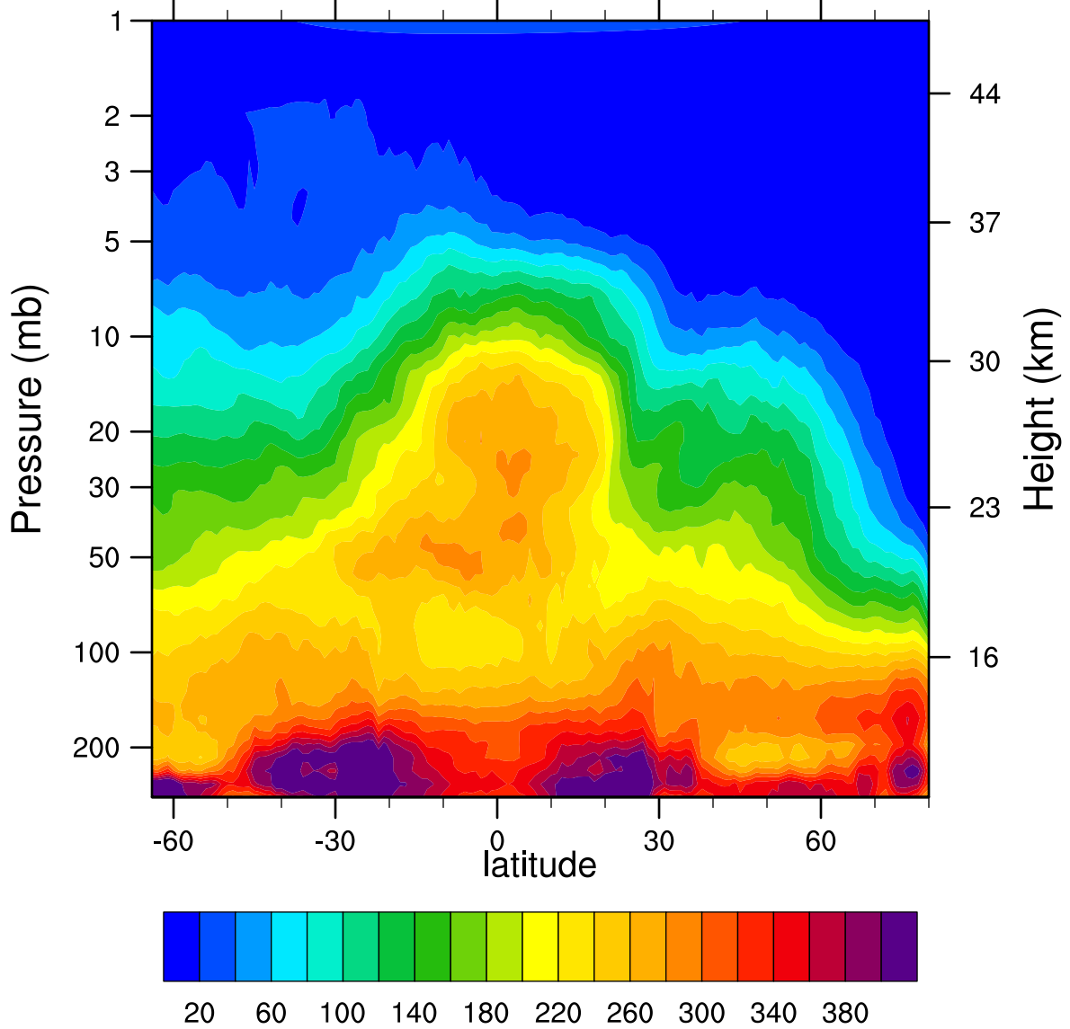
HIRDLSv6 2007d017 N2O_Combined (ppbv)
