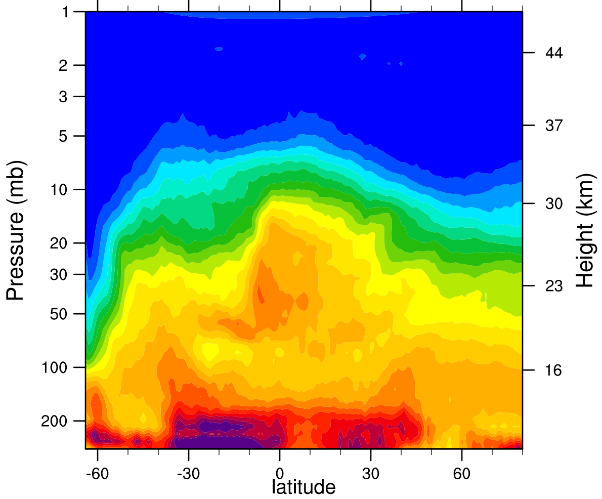
HIRDLSv6 2006d221 N2O_Combined (ppbv)
