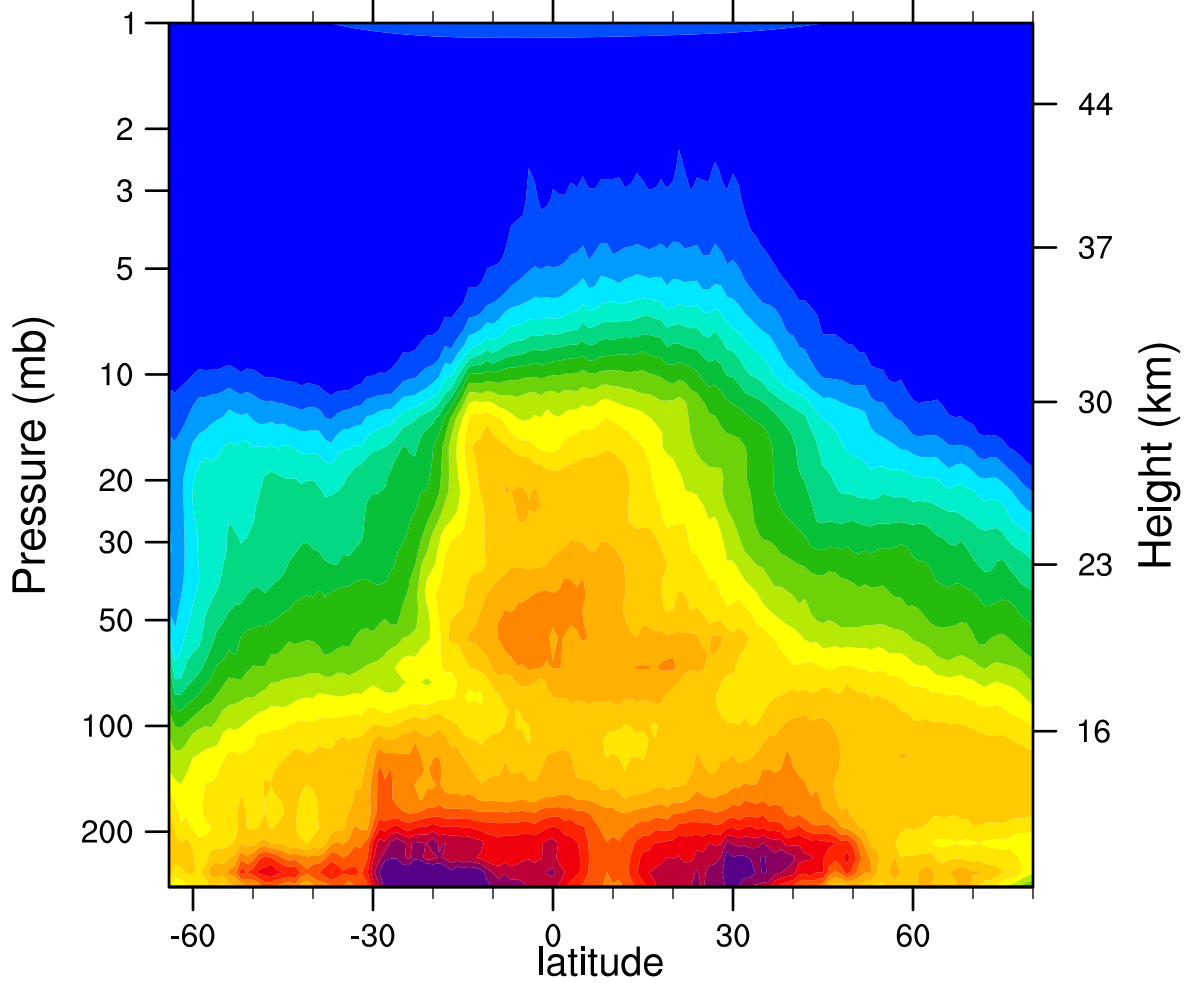
HIRDLSv6 2007d259 N2O_Combined (ppbv)
