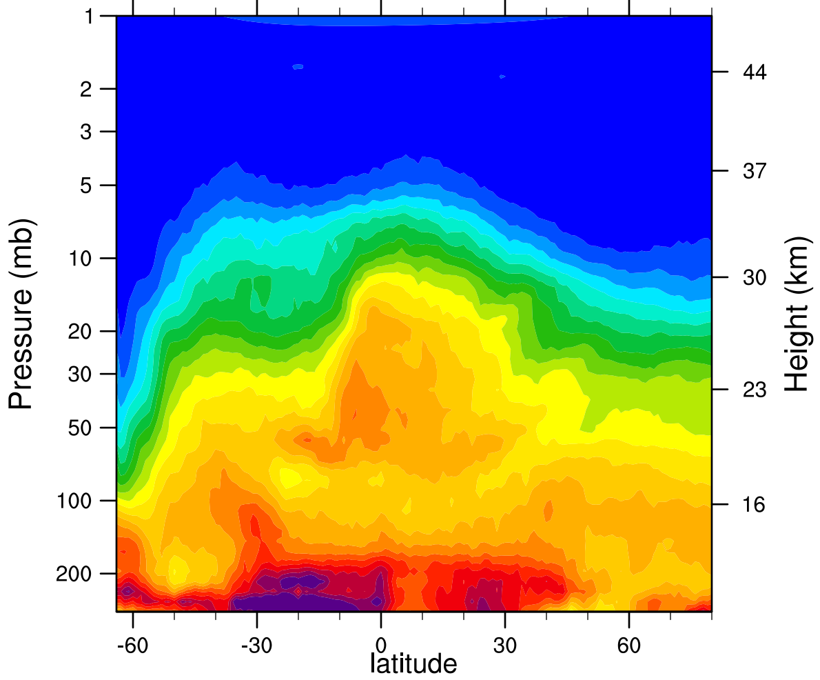
HIRDLSv6 2006d228 N2O_Combined (ppbv)
