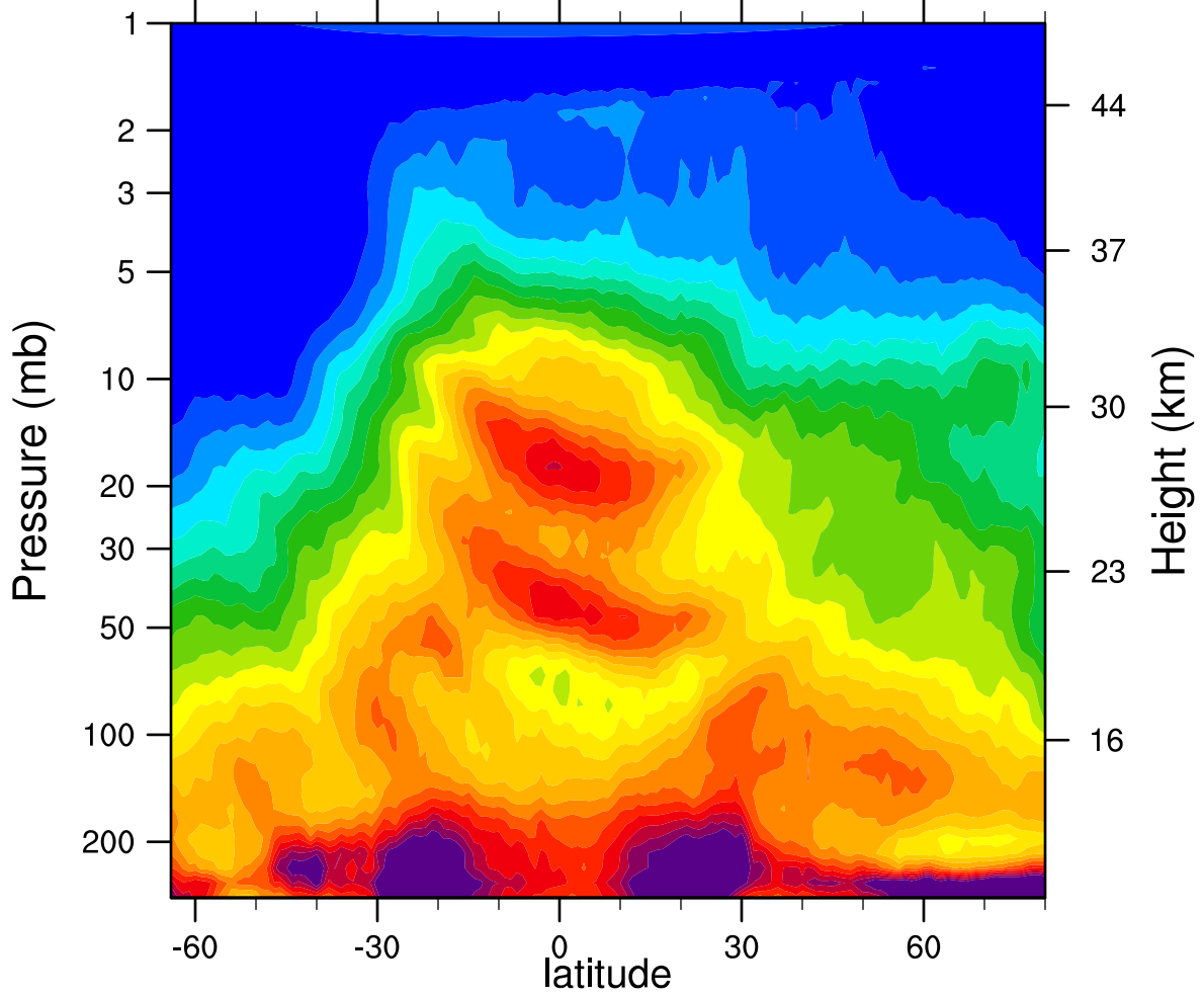
HIRDLSv6 2005d088 N2O_Combined (ppbv)
