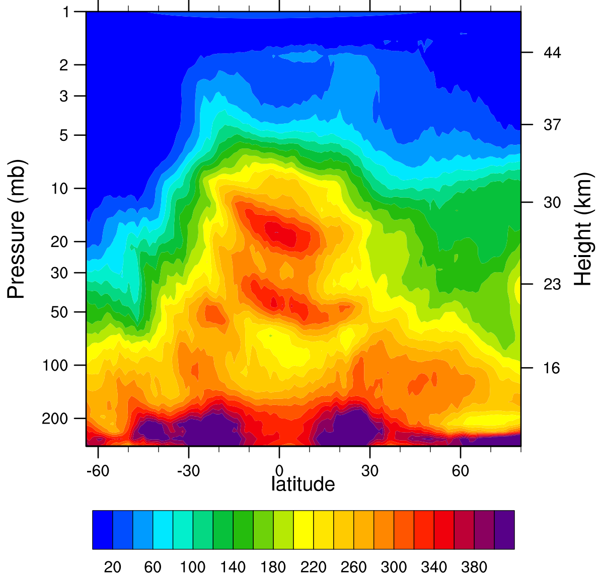
HIRDLSv6 2005d096 N2O_Combined (ppbv)
