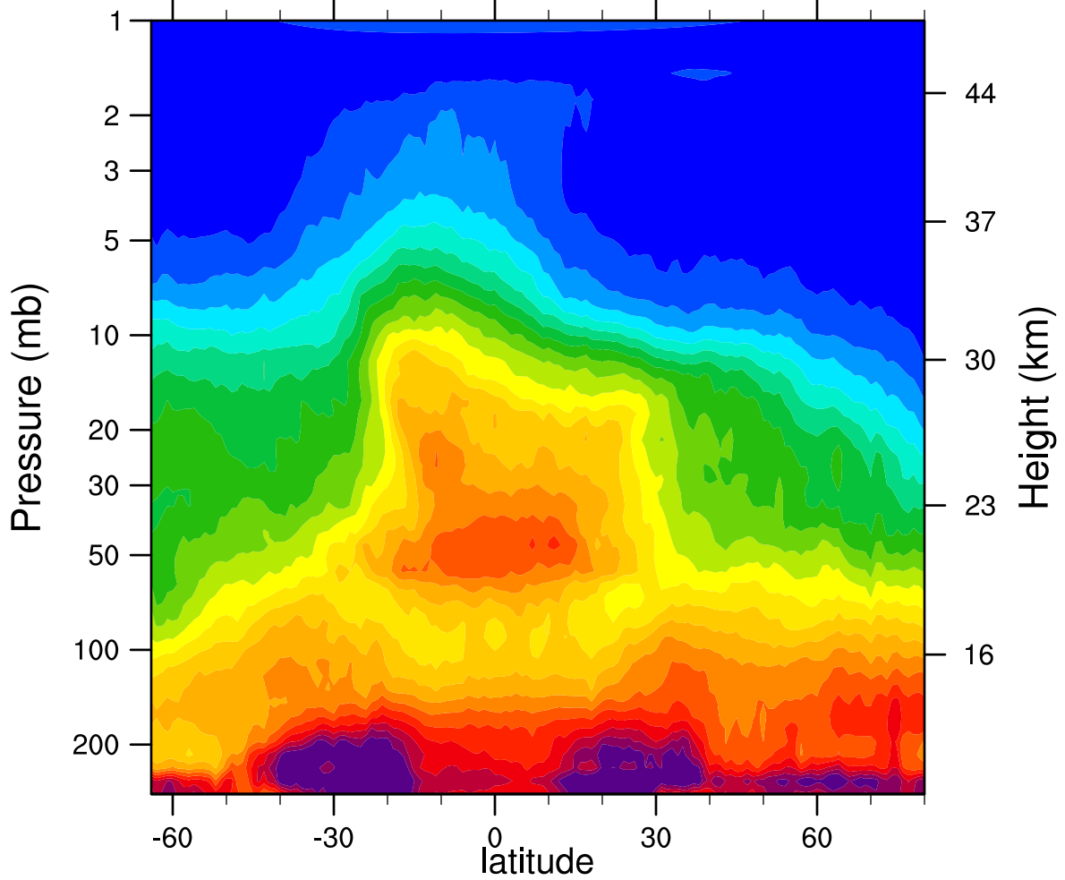
HIRDLSv6 2005d348 N2O_Combined (ppbv)
