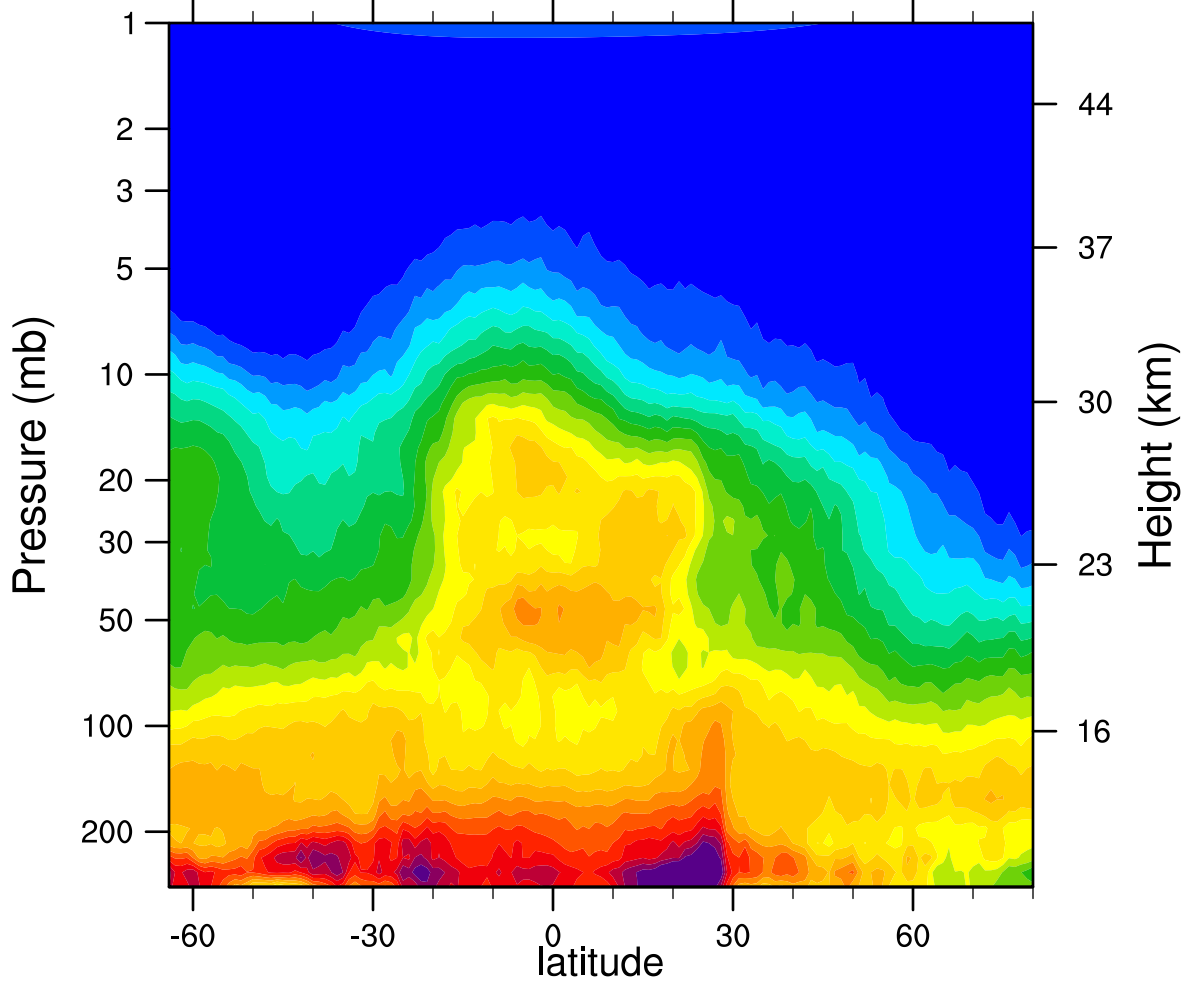
HIRDLSv6 2007d356 N2O_Combined (ppbv)
