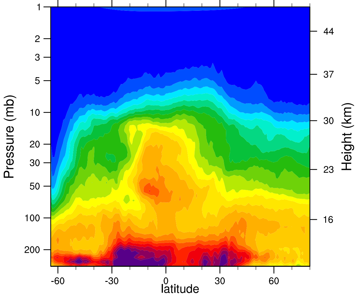
HIRDLSv6 2007d195 N2O_Combined (ppbv)
