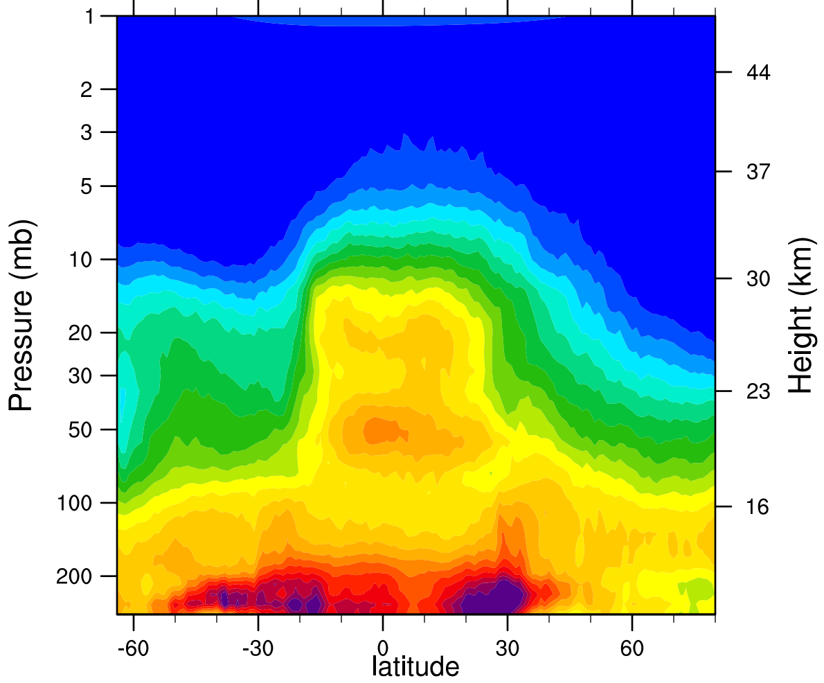
HIRDLSv6 2007d298 N2O_Combined (ppbv)
