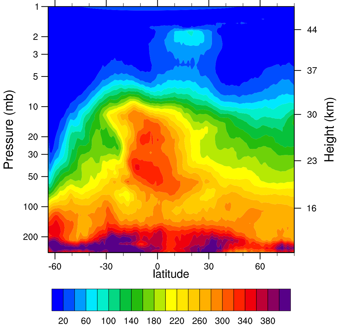
HIRDLSv6 2005d185 N2O_Combined (ppbv)
