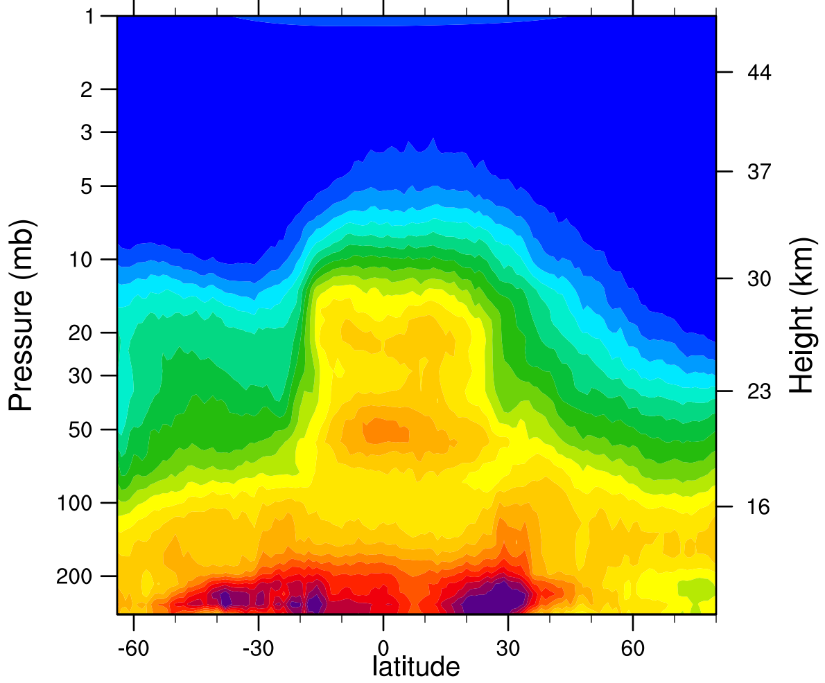
HIRDLSv6 2007d299 N2O_Combined (ppbv)
