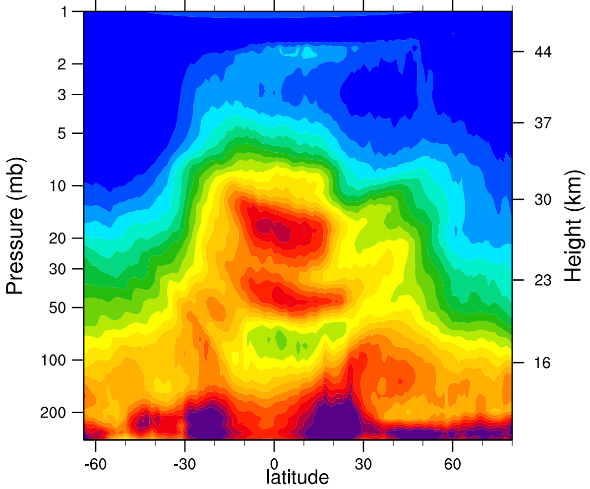
HIRDLSv6 2005d054 N2O_Combined (ppbv)
