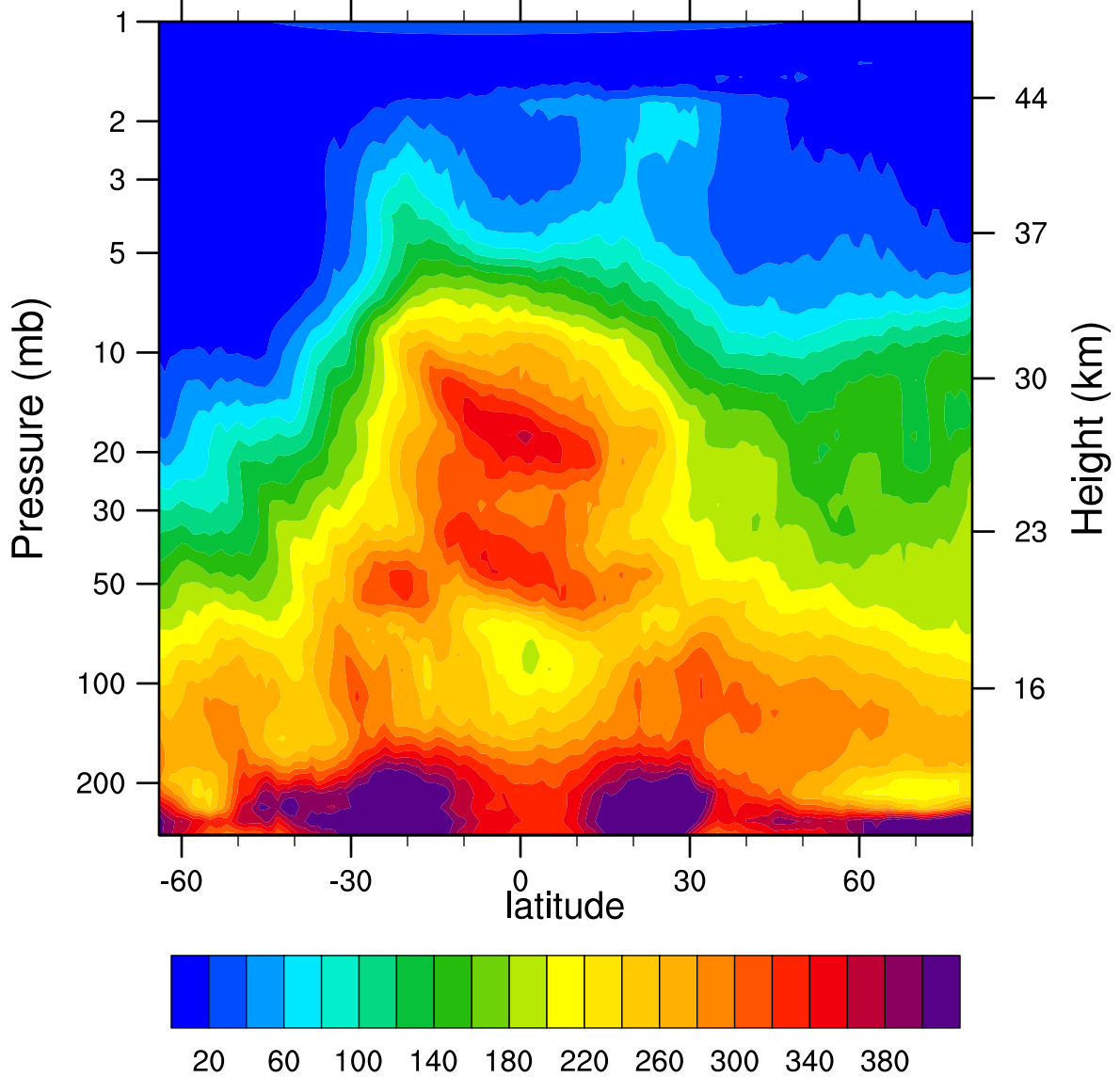
HIRDLSv6 2005d105 N2O_Combined (ppbv)
