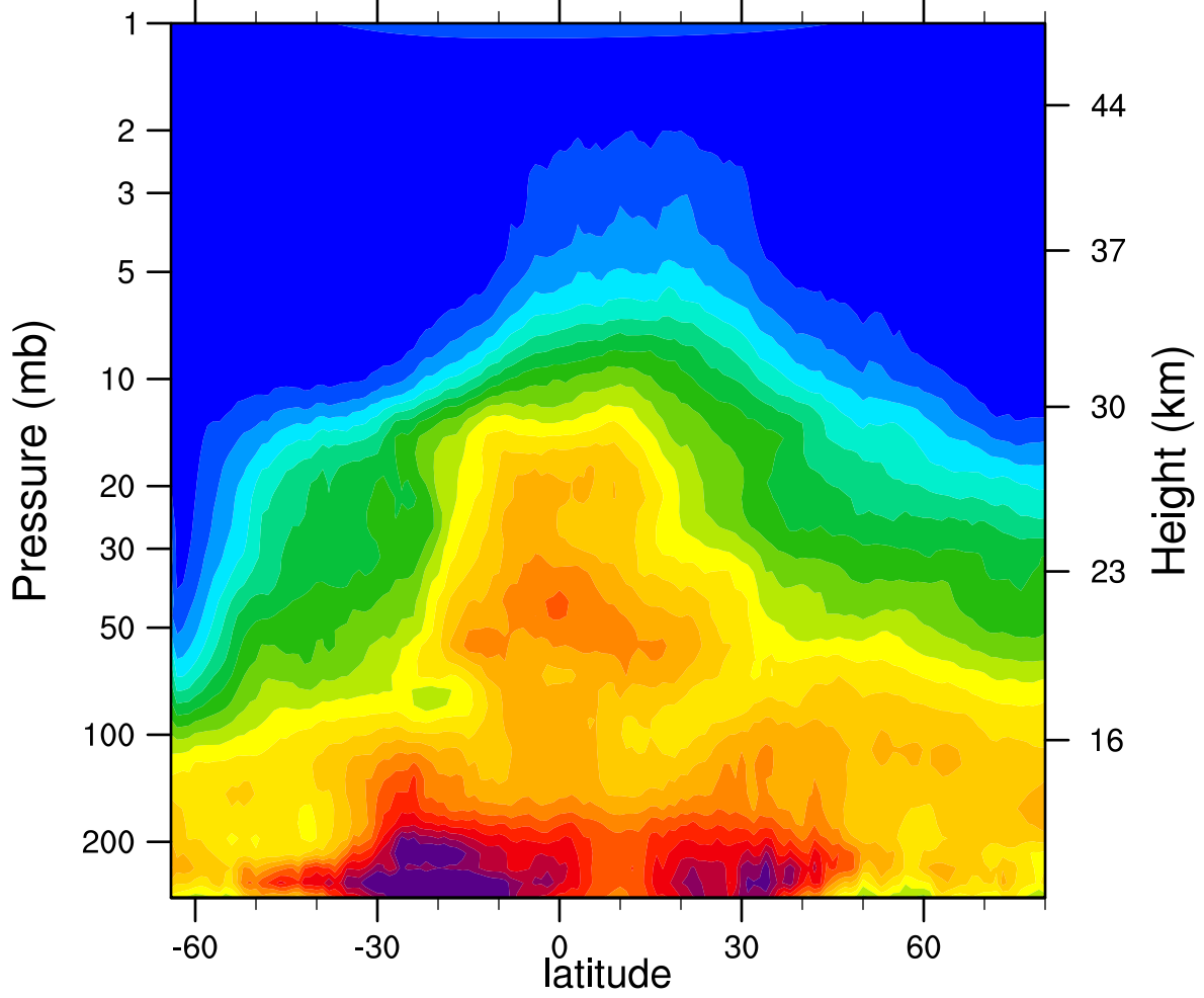
HIRDLSv6 2007d233 N2O_Combined (ppbv)
