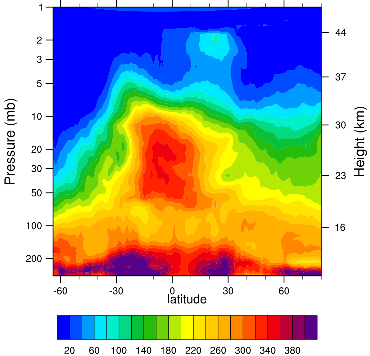
HIRDLSv6 2005d154 N2O_Combined (ppbv)
