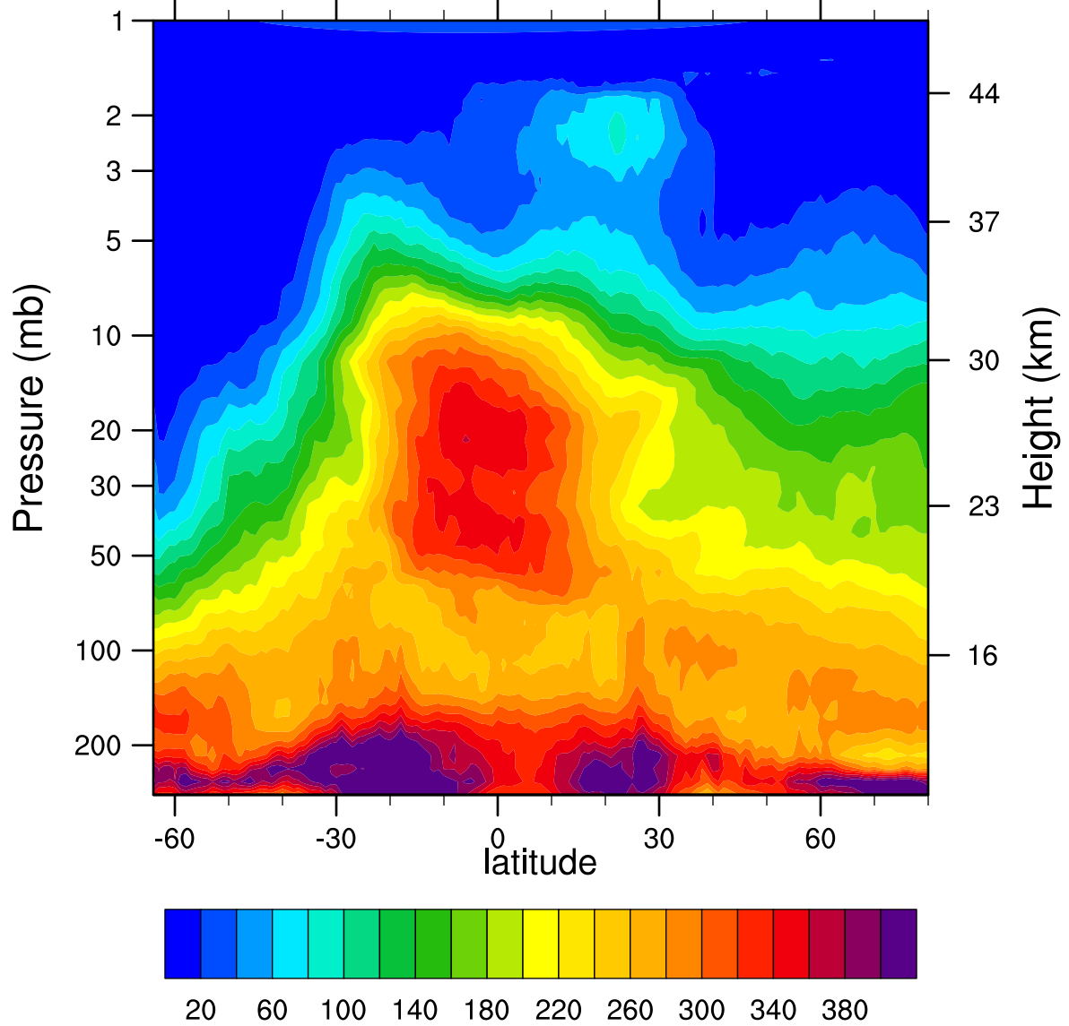
HIRDLSv6 2005d148 N2O_Combined (ppbv)
