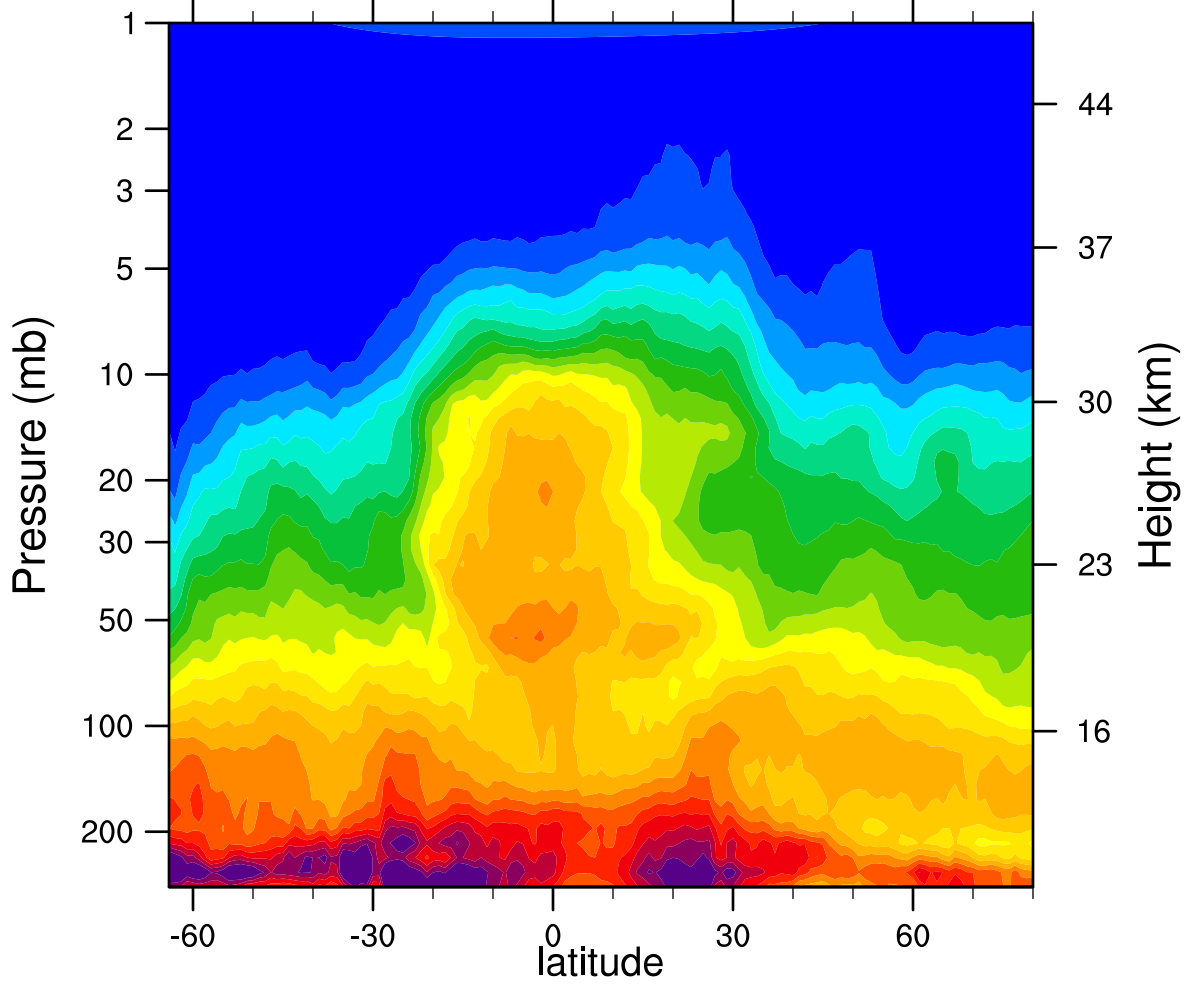
HIRDLSv6 2007d151 N2O_Combined (ppbv)
