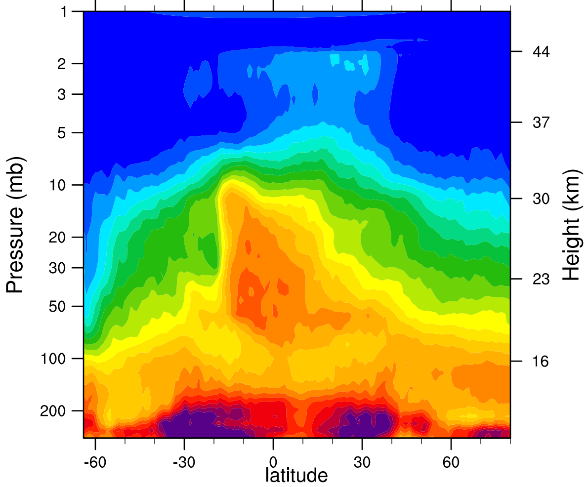
HIRDLSv6 2005d259 N2O_Combined (ppbv)
