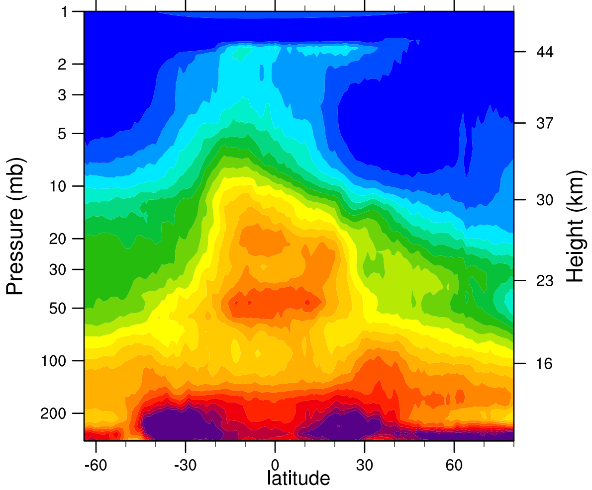
HIRDLSv6 2006d024 N2O_Combined (ppbv)
