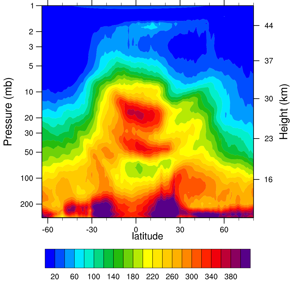
HIRDLSv6 2005d053 N2O_Combined (ppbv)
