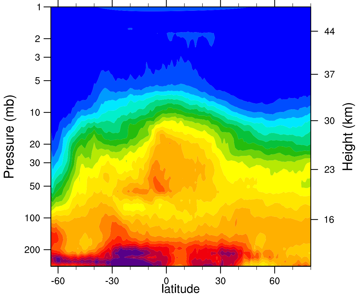
HIRDLSv6 2006d194 N2O_Combined (ppbv)
