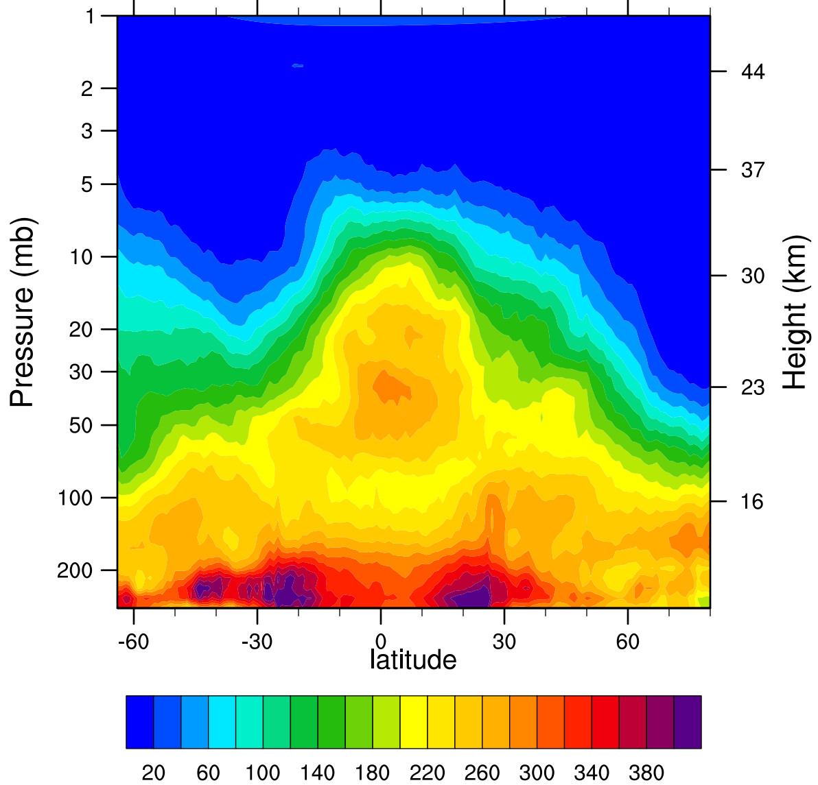
HIRDLSv6 2006d344 N2O_Combined (ppbv)
