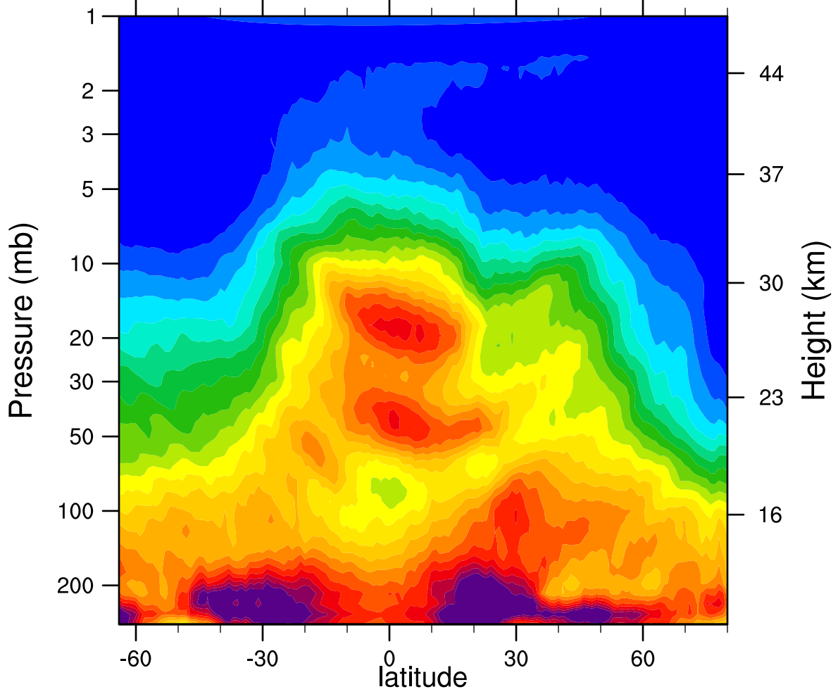
HIRDLSv6 2005d032 N2O_Combined (ppbv)
