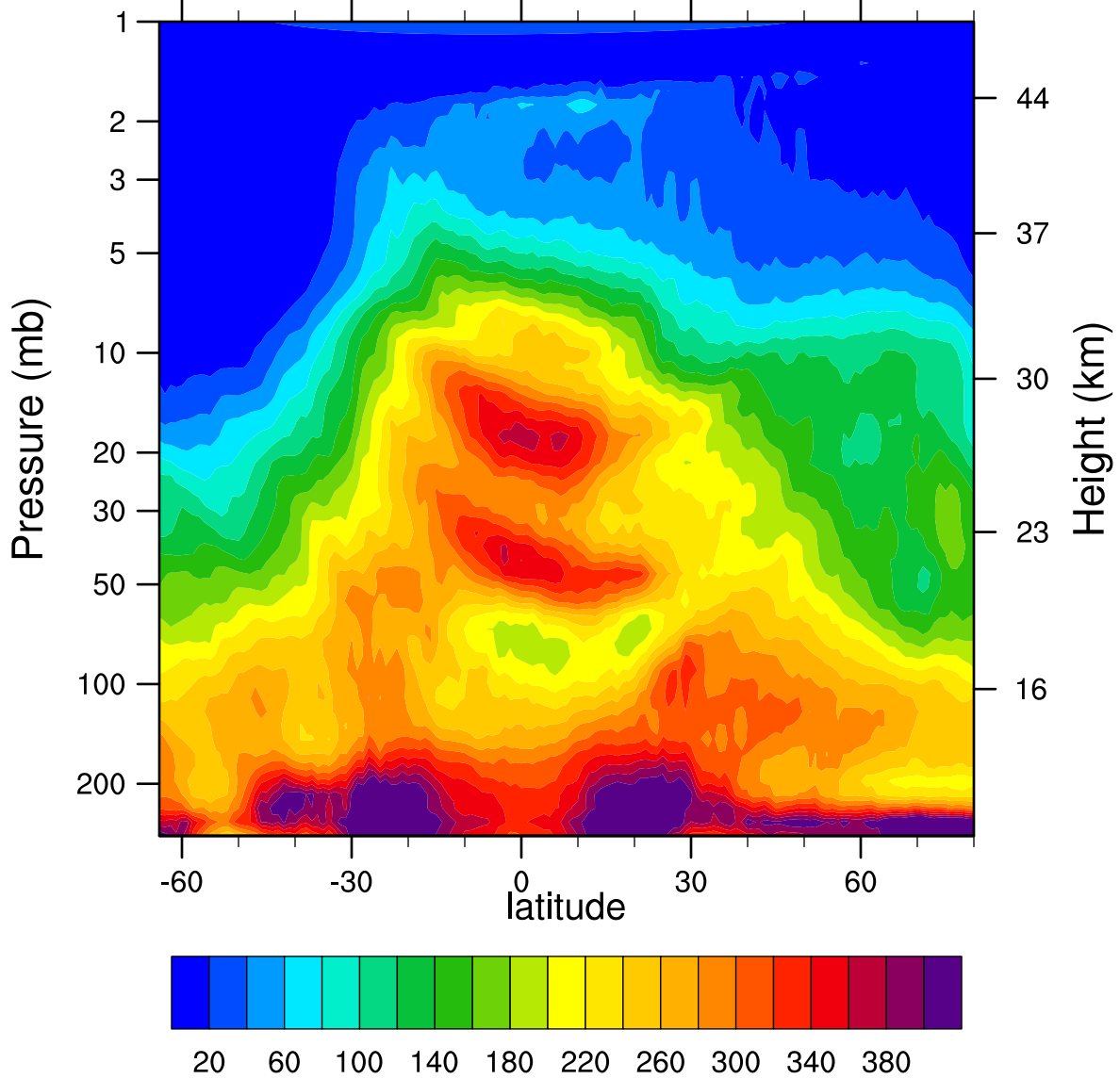
HIRDLSv6 2005d078 N2O_Combined (ppbv)
