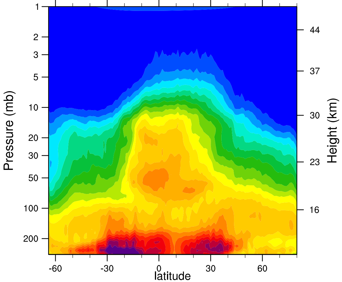
HIRDLSv6 2007d265 N2O_Combined (ppbv)
