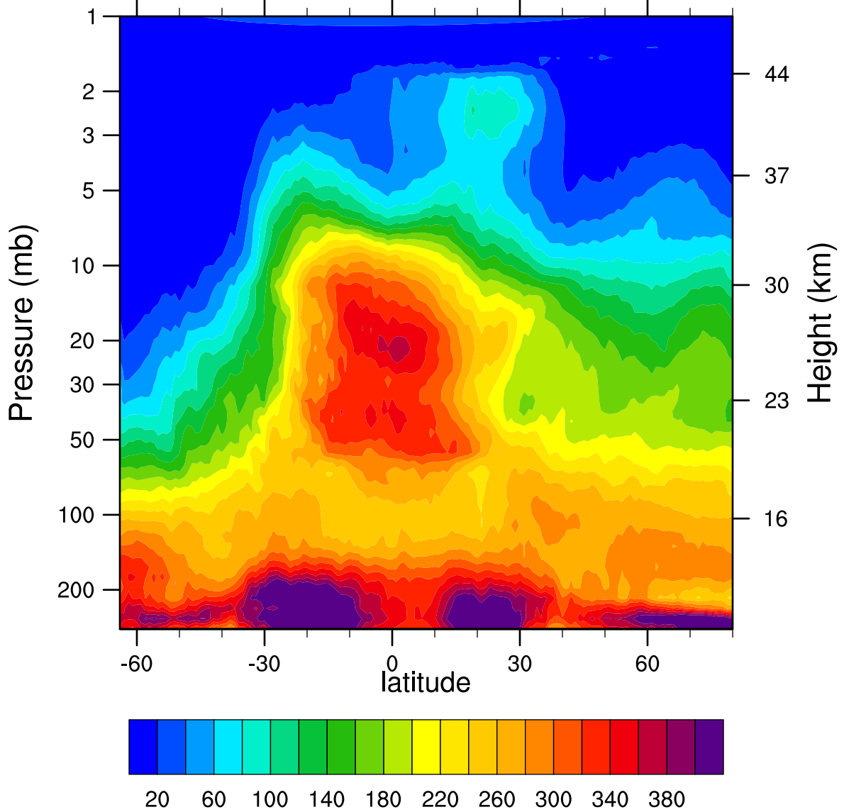
HIRDLSv6 2005d138 N2O_Combined (ppbv)
