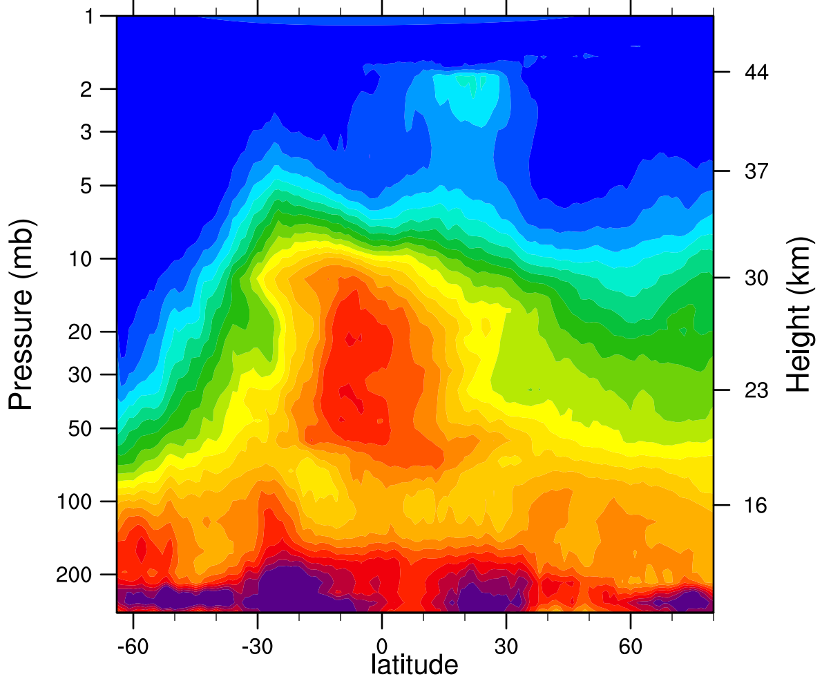
HIRDLSv6 2005d169 N2O_Combined (ppbv)
