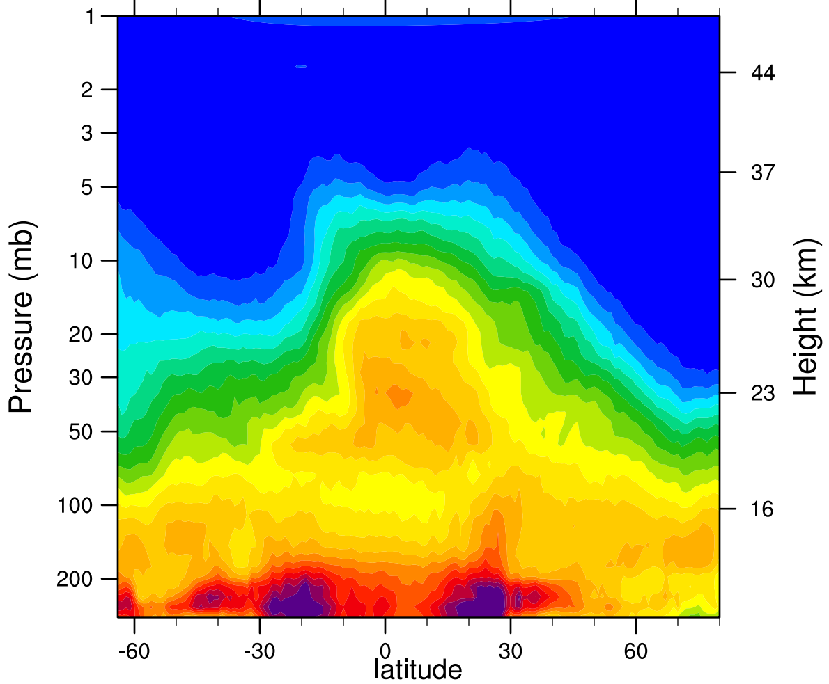
HIRDLSv6 2006d326 N2O_Combined (ppbv)
