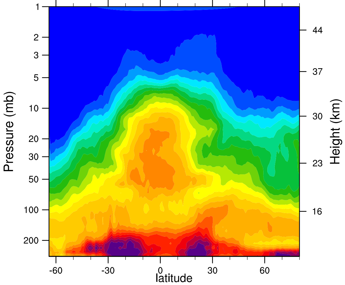
HIRDLSv6 2007d119 N2O_Combined (ppbv)
