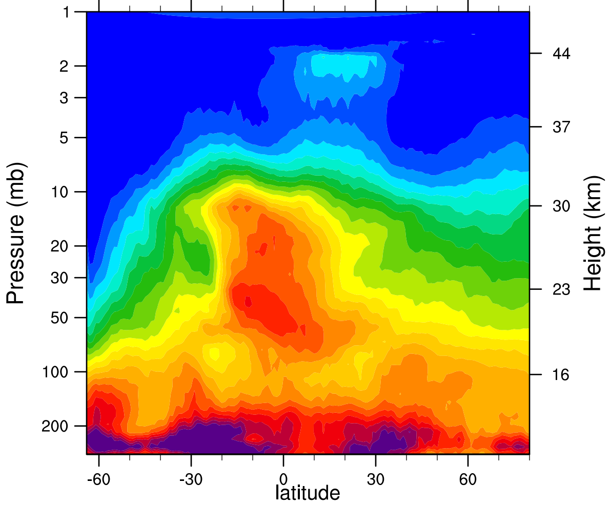
HIRDLSv6 2005d190 N2O_Combined (ppbv)
