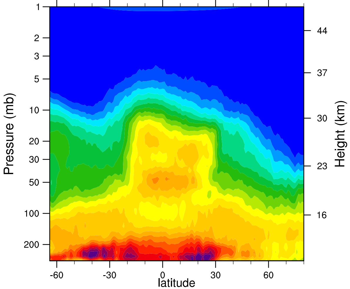
HIRDLSv6 2007d341 N2O_Combined (ppbv)
