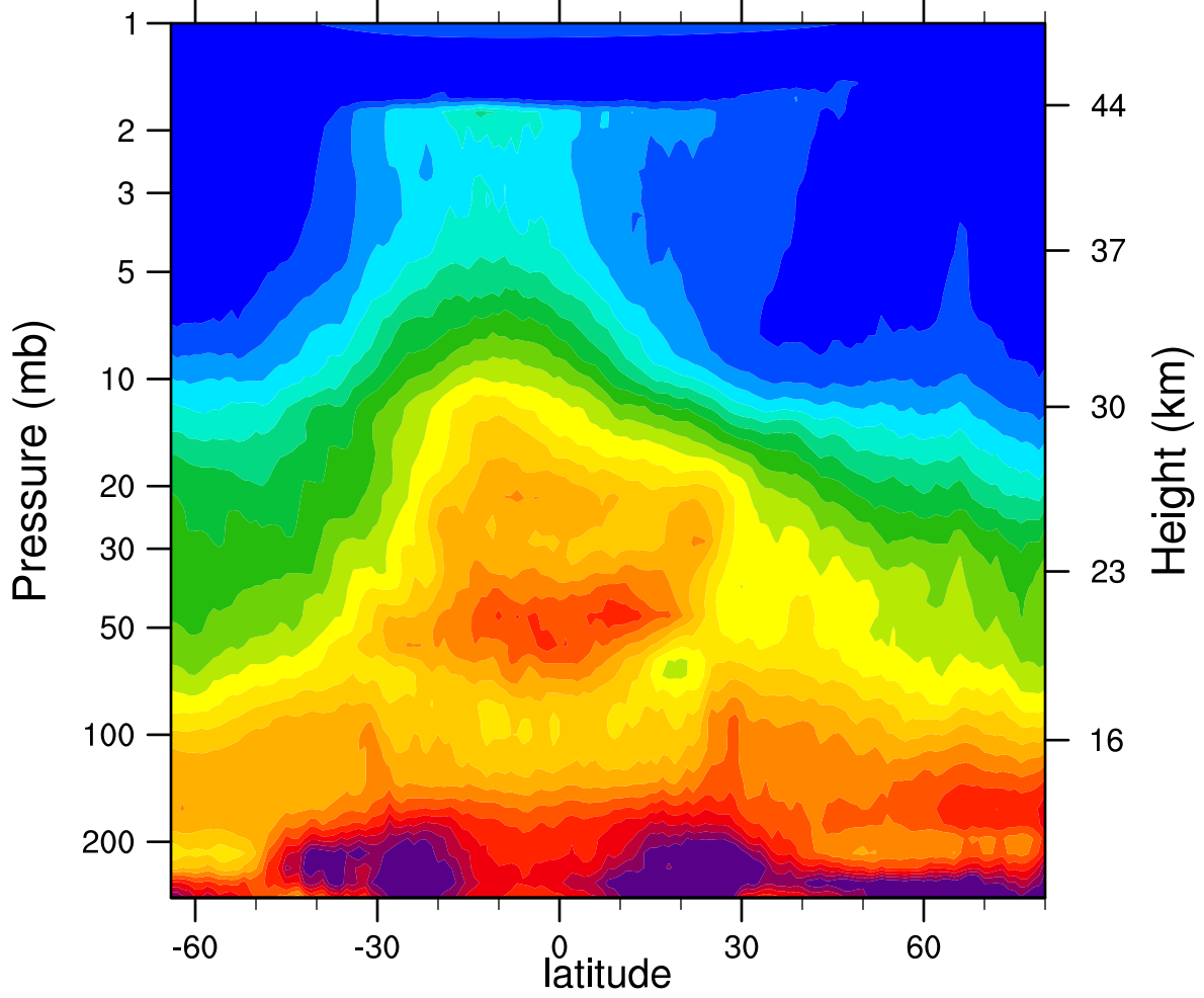
HIRDLSv6 2006d058 N2O_Combined (ppbv)
