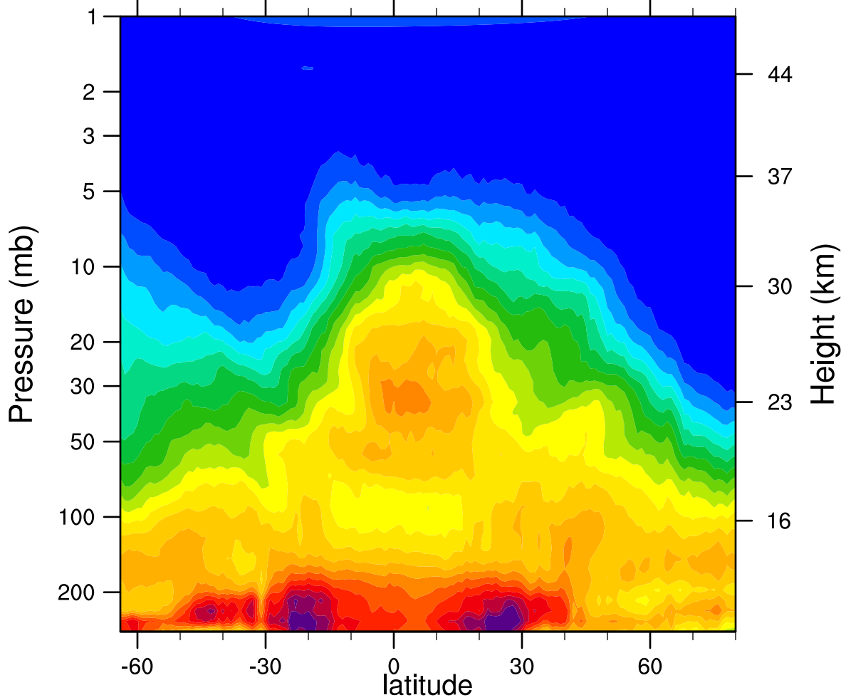
HIRDLSv6 2006d338 N2O_Combined (ppbv)
