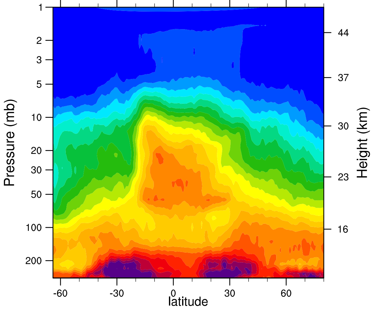
HIRDLSv6 2005d298 N2O_Combined (ppbv)
