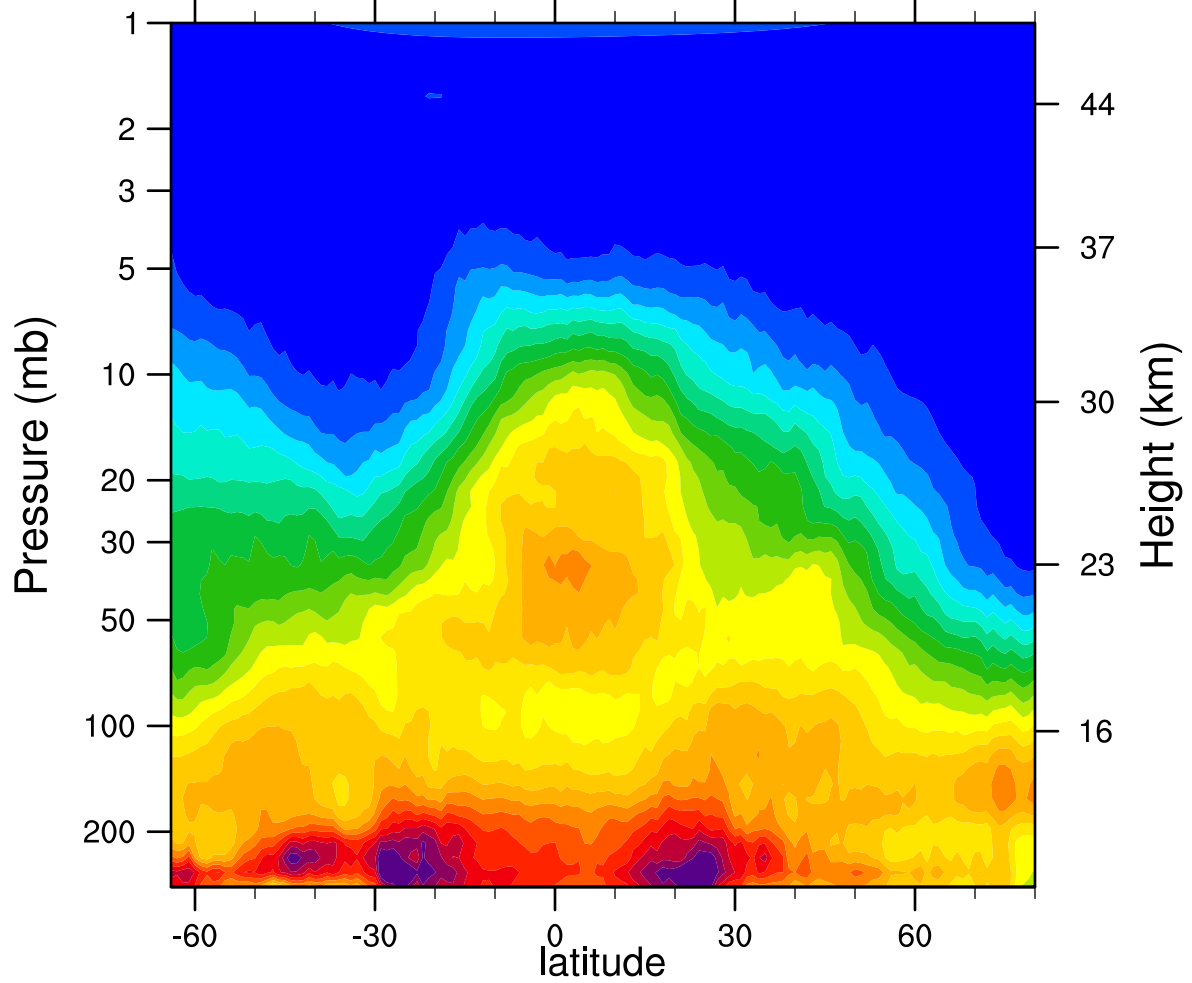
HIRDLSv6 2006d346 N2O_Combined (ppbv)
