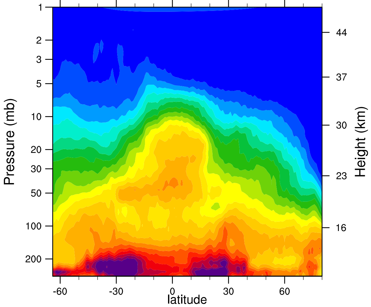
HIRDLSv6 2006d364 N2O_Combined (ppbv)
