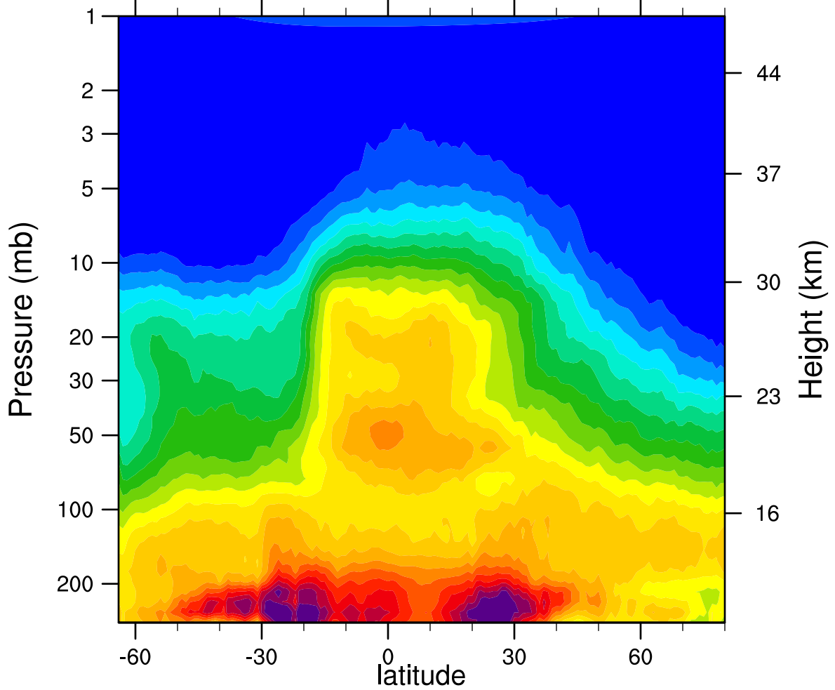
HIRDLSv6 2007d293 N2O_Combined (ppbv)
