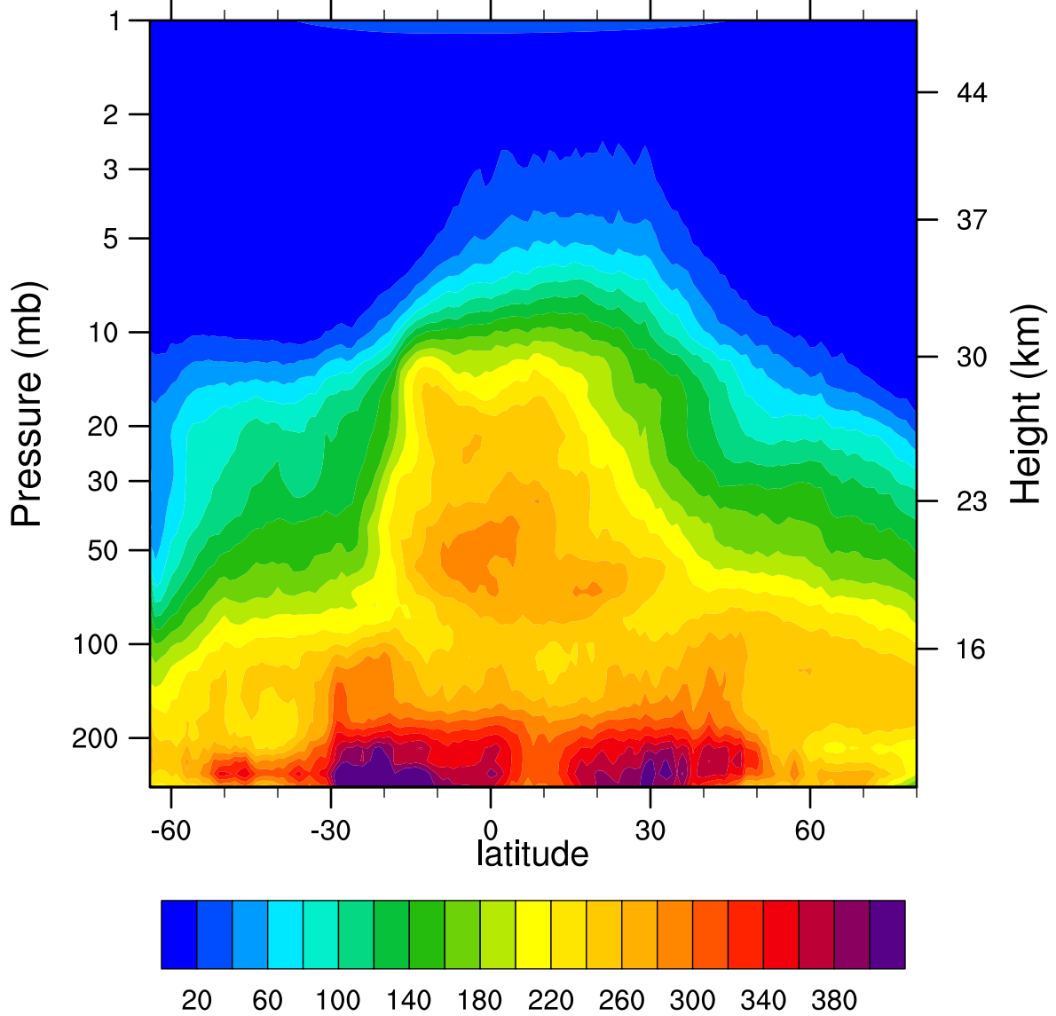
HIRDLSv6 2007d257 N2O_Combined (ppbv)
