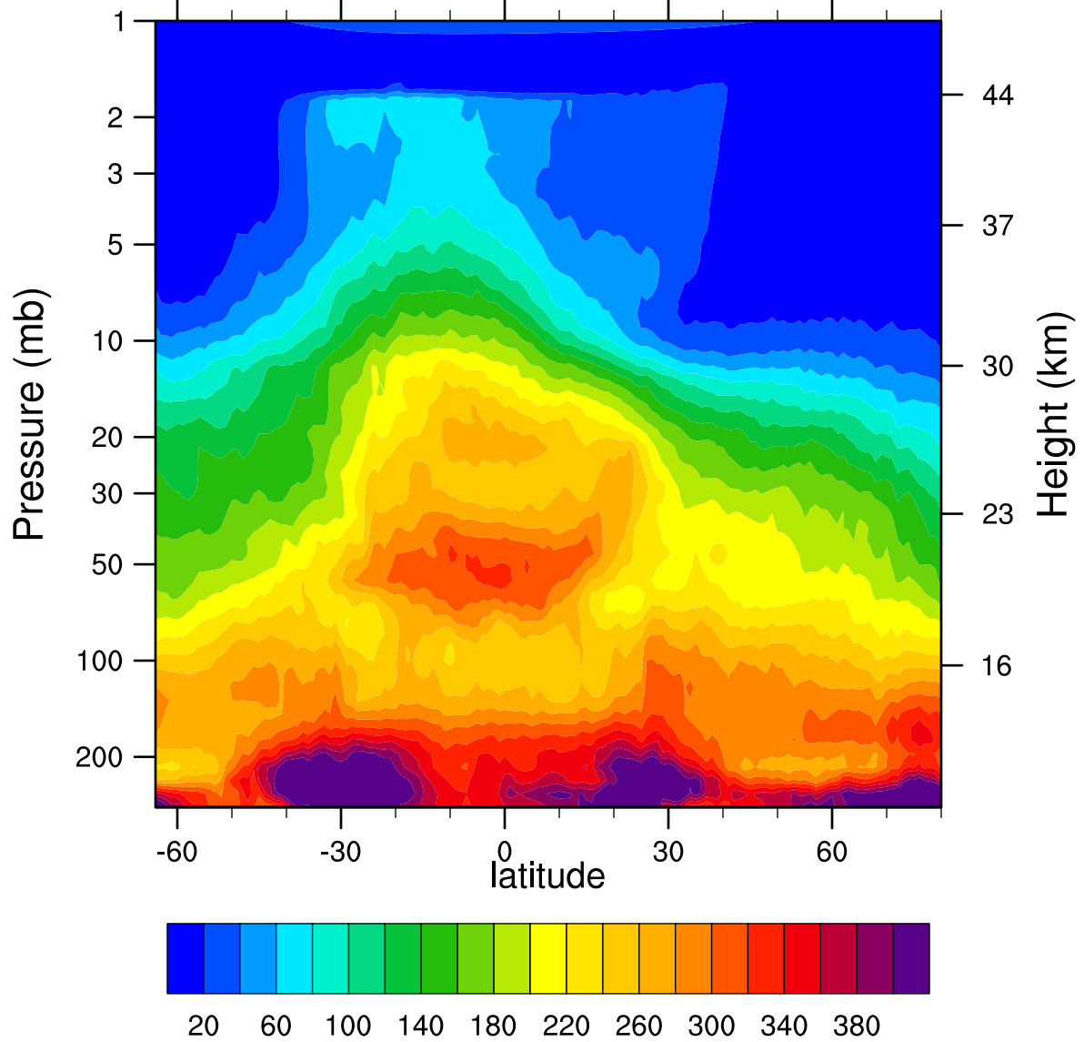
HIRDLSv6 2006d074 N2O_Combined (ppbv)
