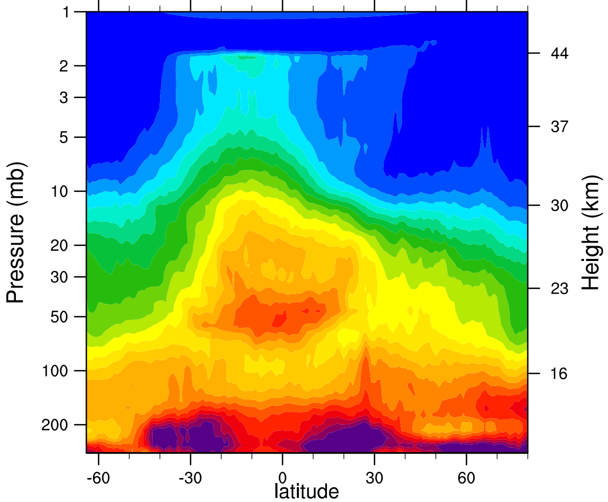
HIRDLSv6 2006d062 N2O_Combined (ppbv)
