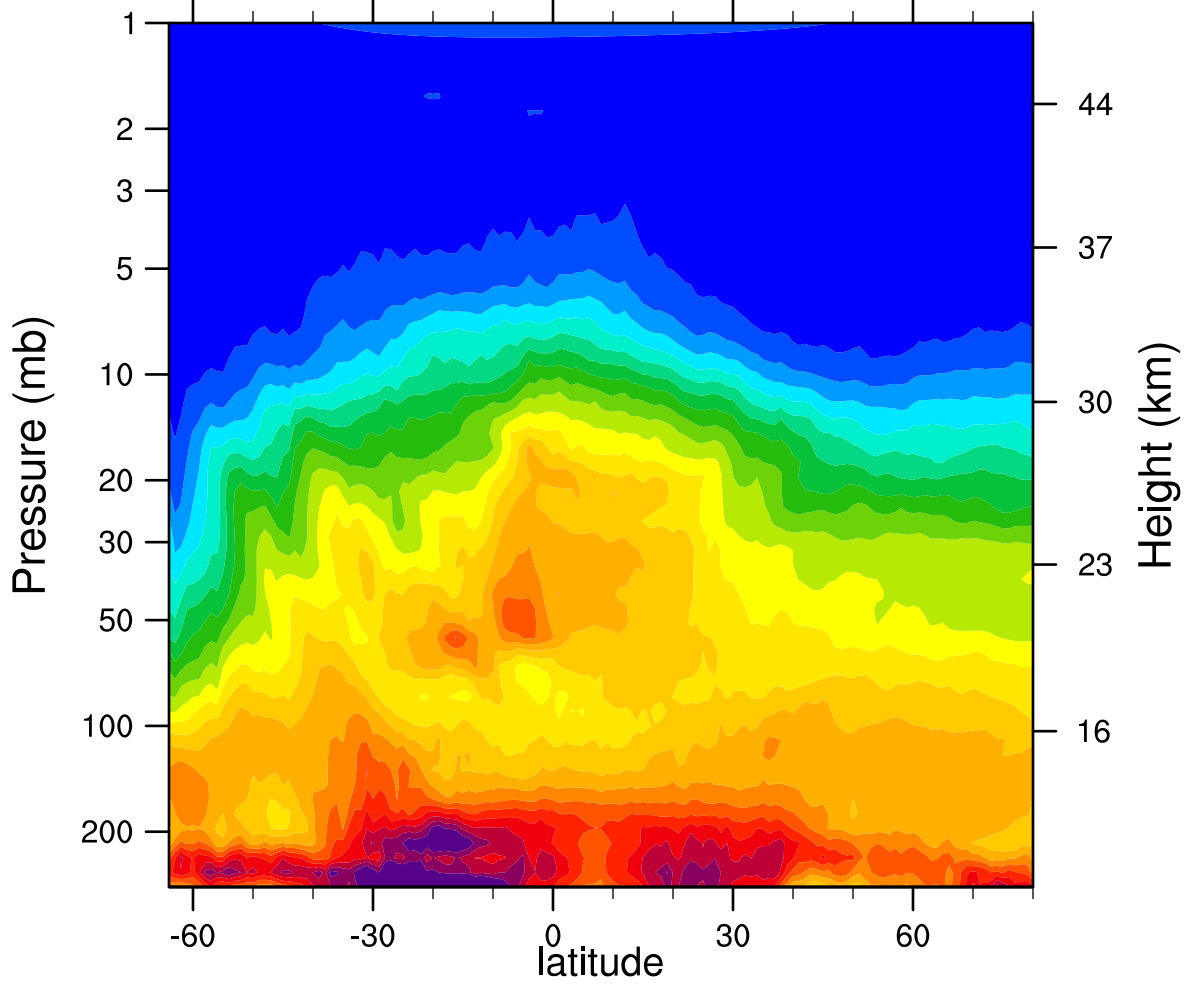
HIRDLSv6 2006d181 N2O_Combined (ppbv)
