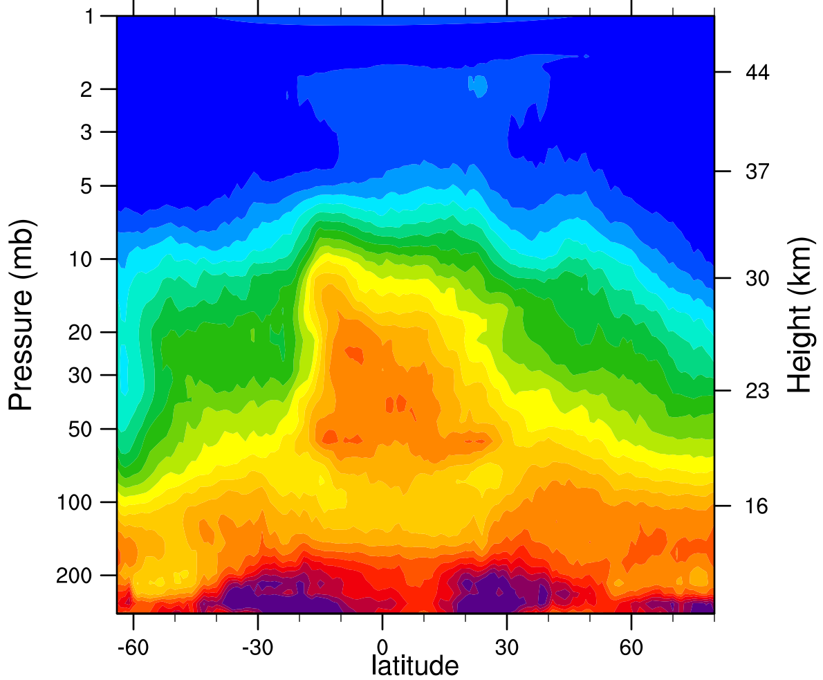
HIRDLSv6 2005d291 N2O_Combined (ppbv)
