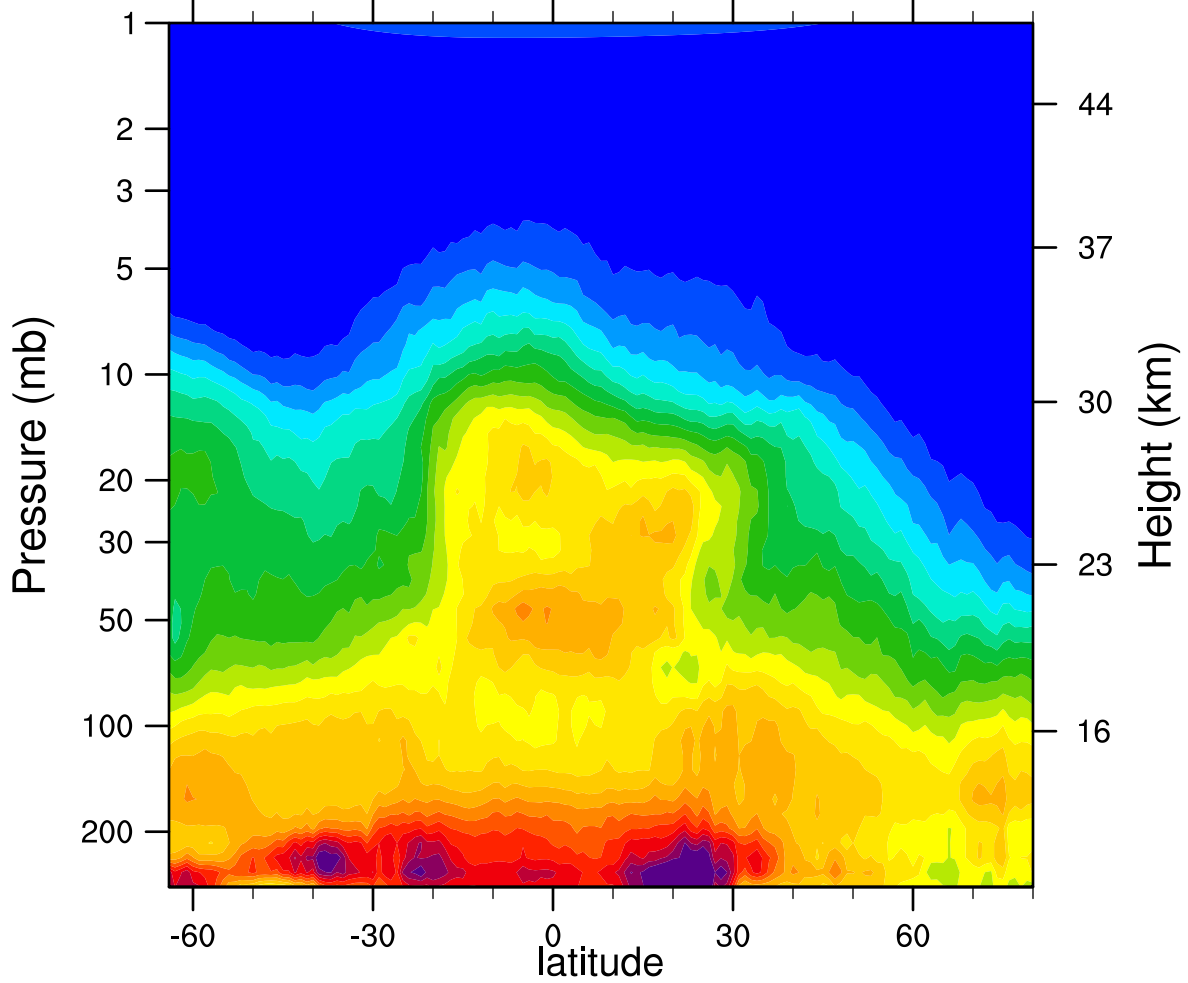
HIRDLSv6 2007d350 N2O_Combined (ppbv)
