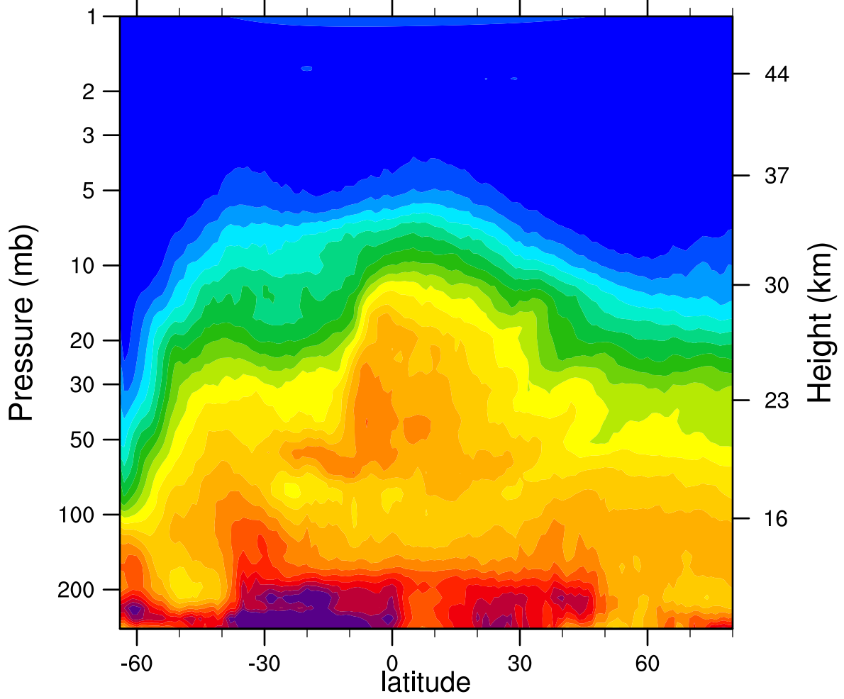
HIRDLSv6 2006d225 N2O_Combined (ppbv)
