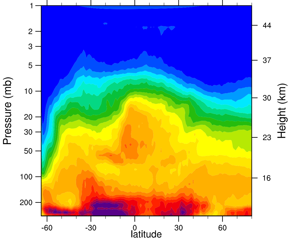
HIRDLSv6 2006d217 N2O_Combined (ppbv)
