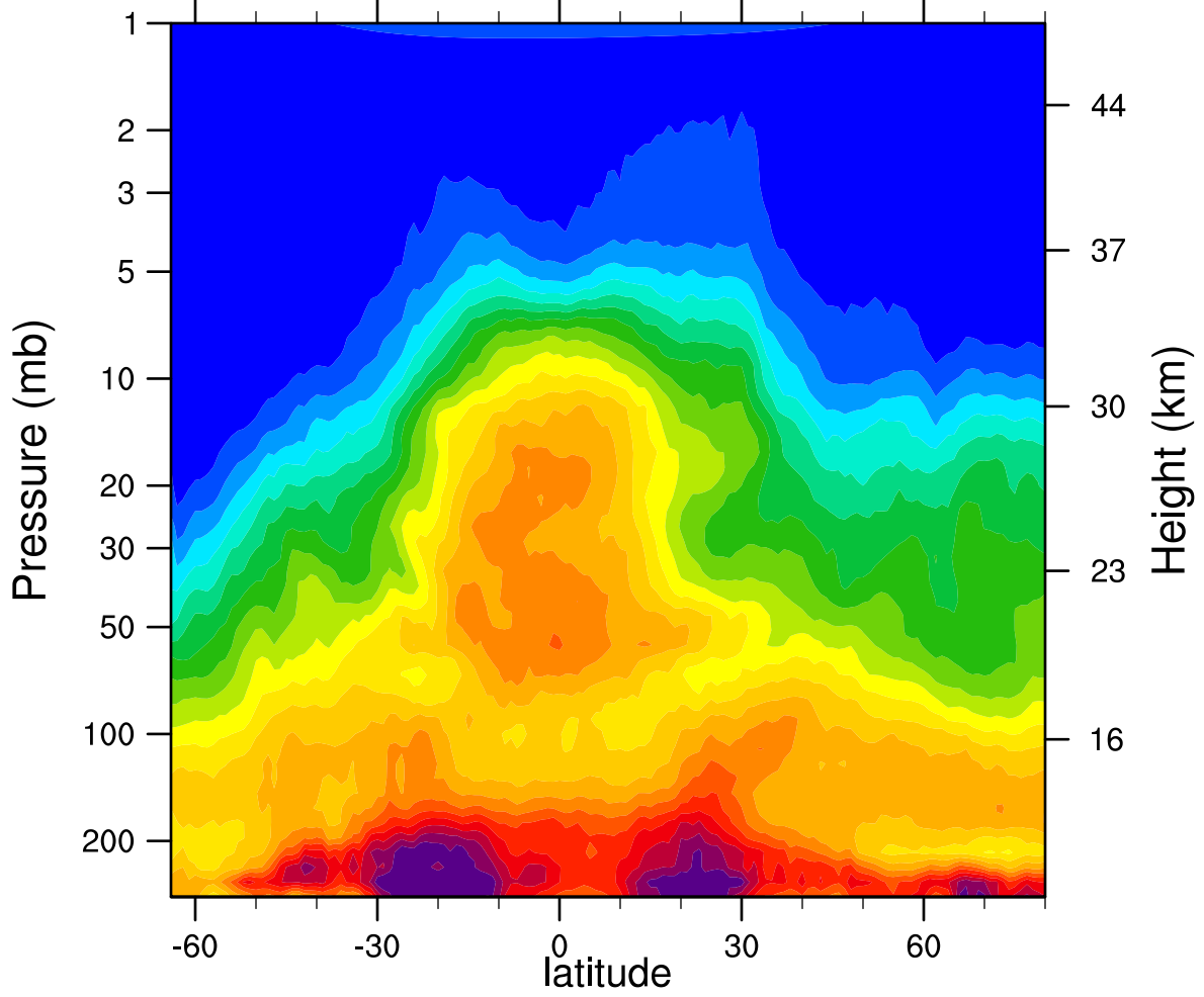
HIRDLSv6 2007d124 N2O_Combined (ppbv)
