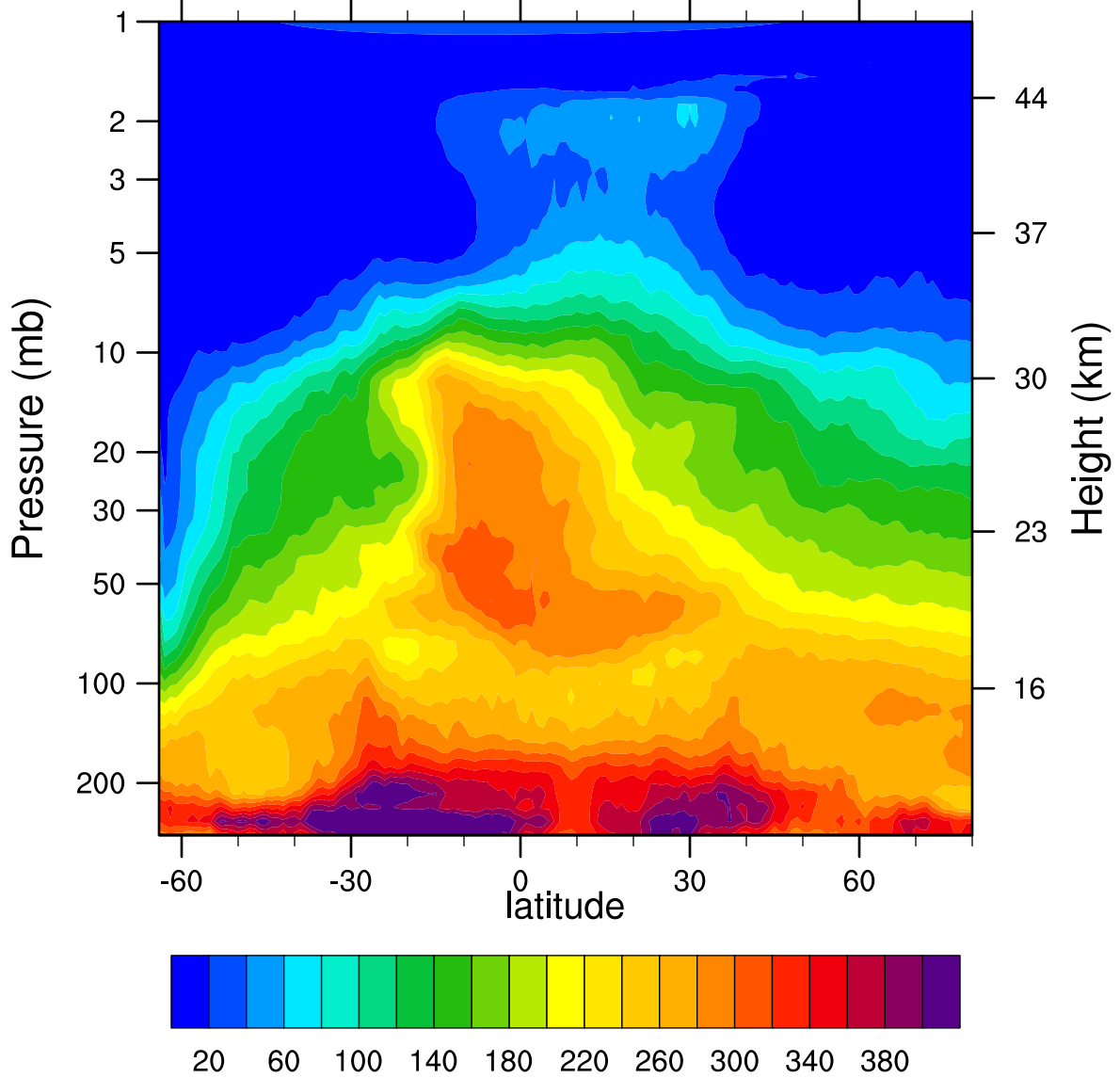
HIRDLSv6 2005d240 N2O_Combined (ppbv)
