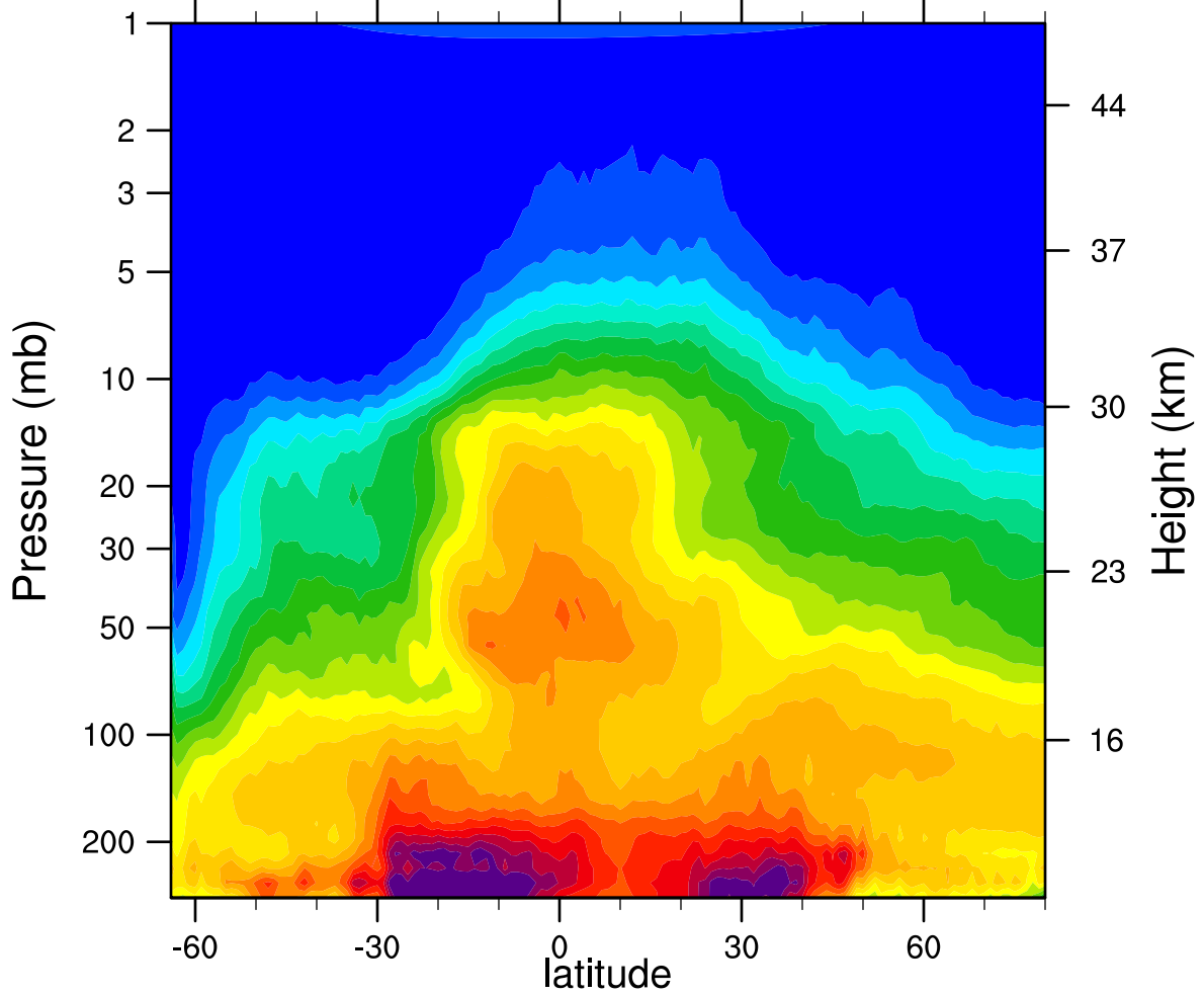
HIRDLSv6 2007d215 N2O_Combined (ppbv)
