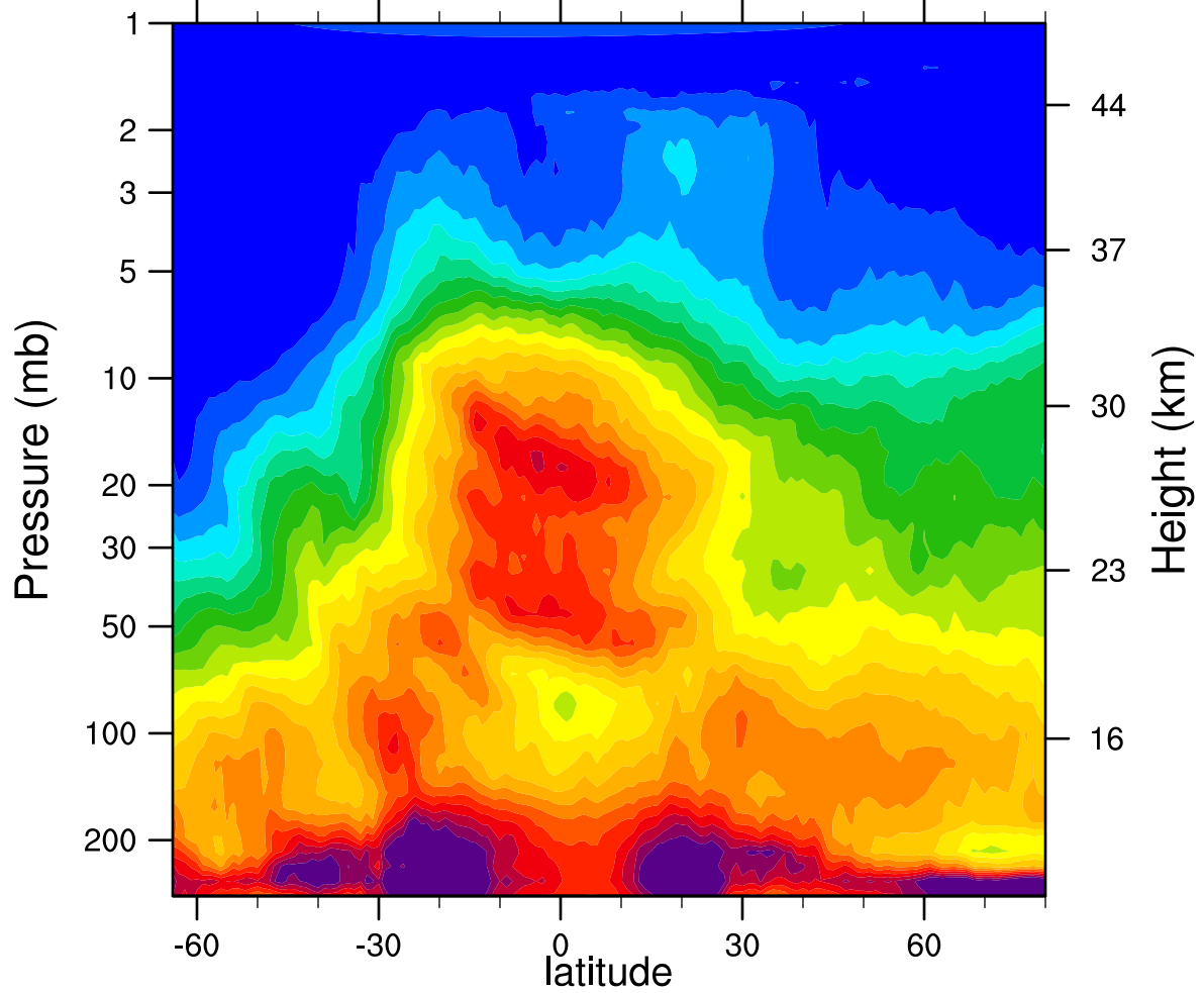
HIRDLSv6 2005d114 N2O_Combined (ppbv)
