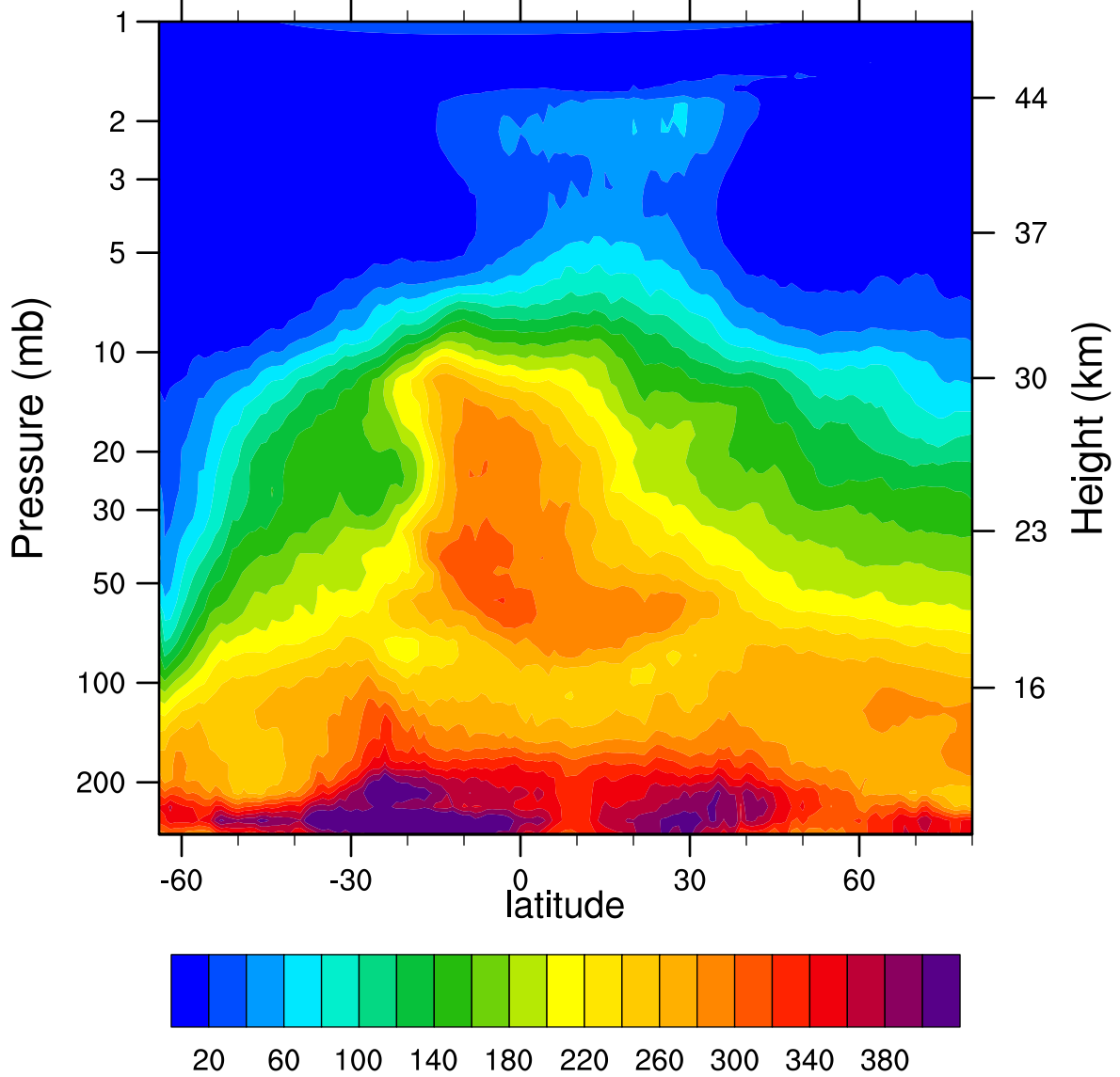
HIRDLSv6 2005d239 N2O_Combined (ppbv)
