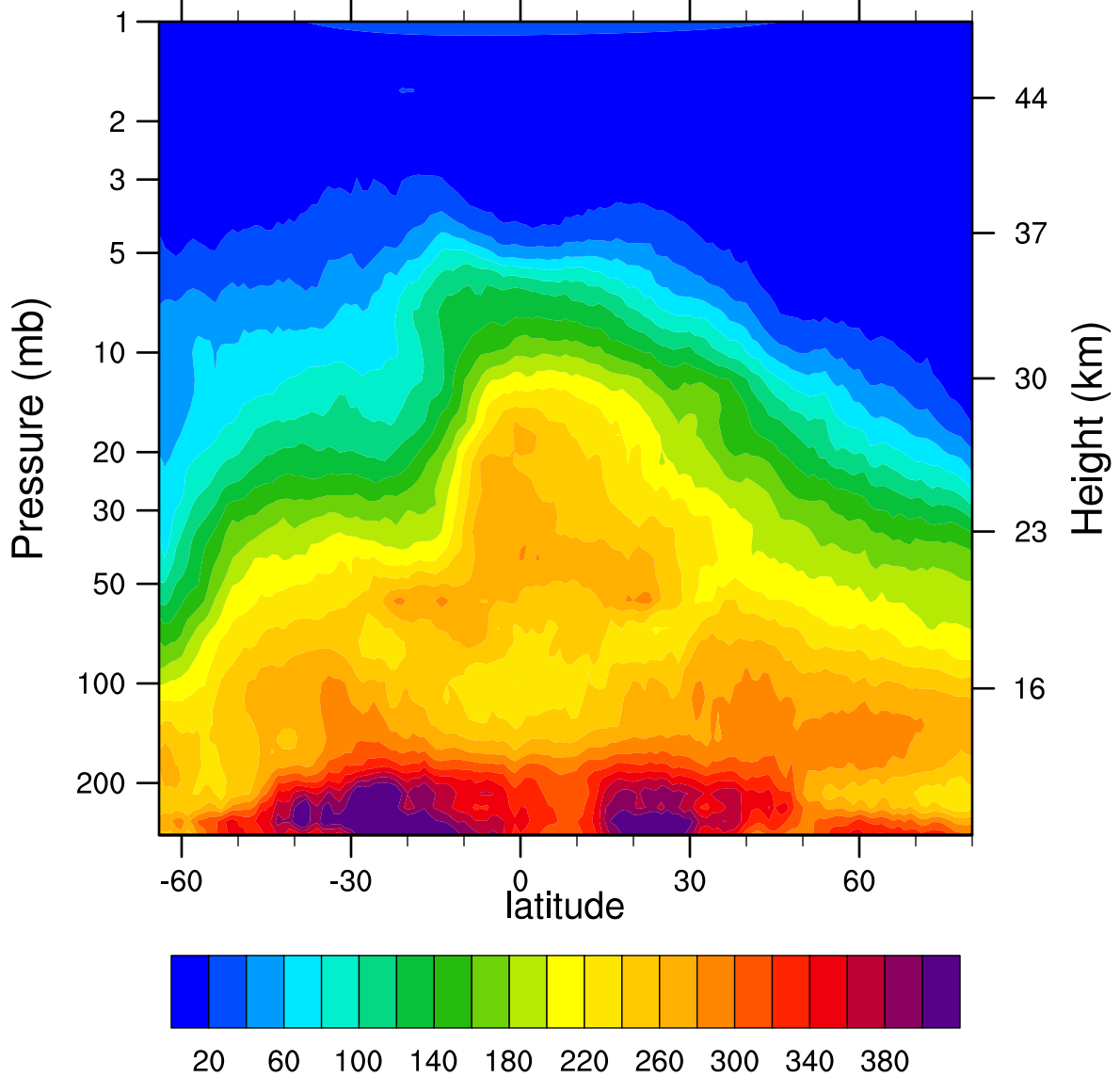
HIRDLSv6 2006d292 N2O_Combined (ppbv)
