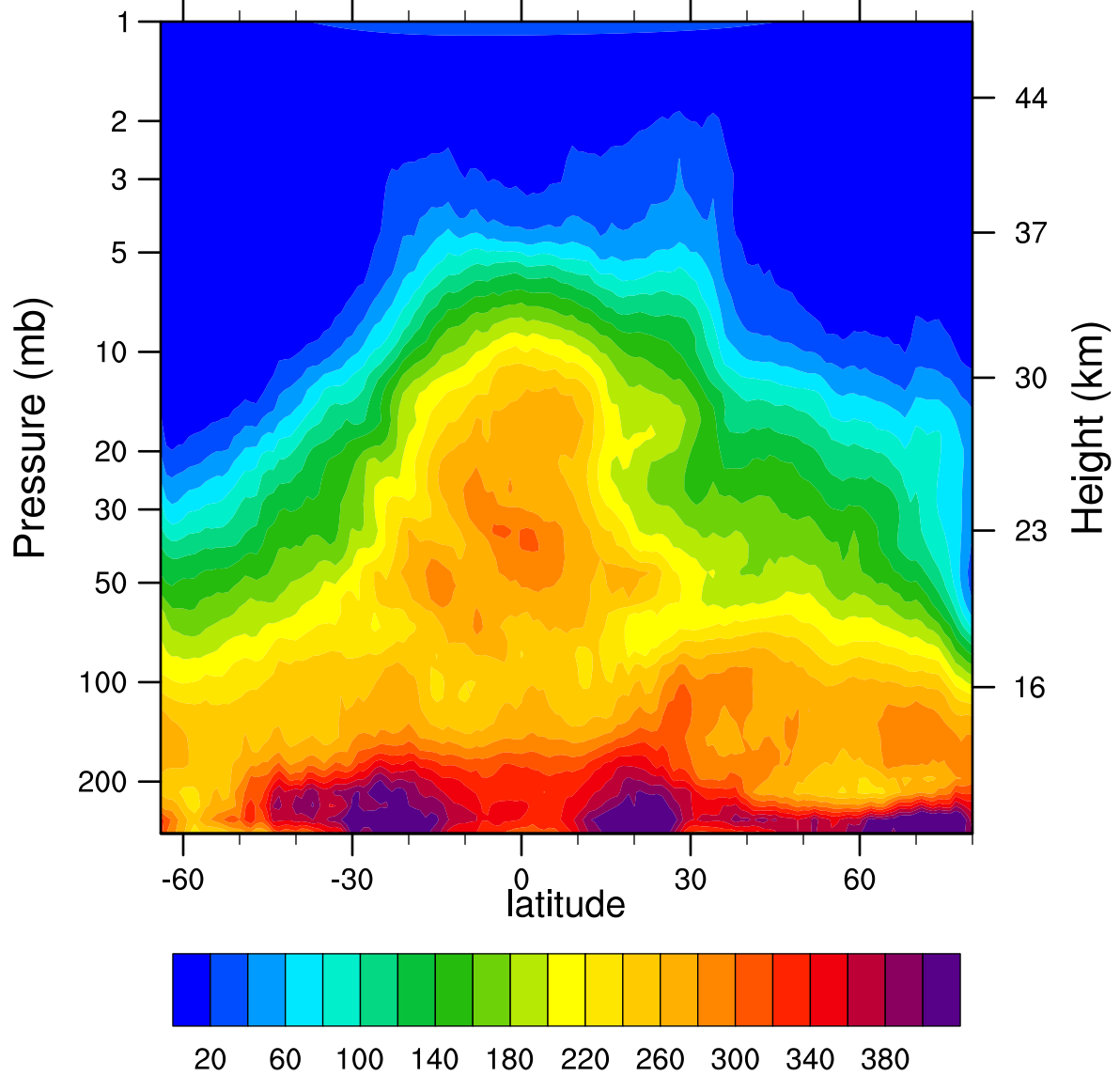
HIRDLSv6 2007d104 N2O_Combined (ppbv)
