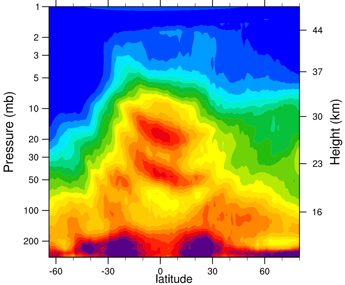
HIRDLSv6 2005d094 N2O_Combined (ppbv)
