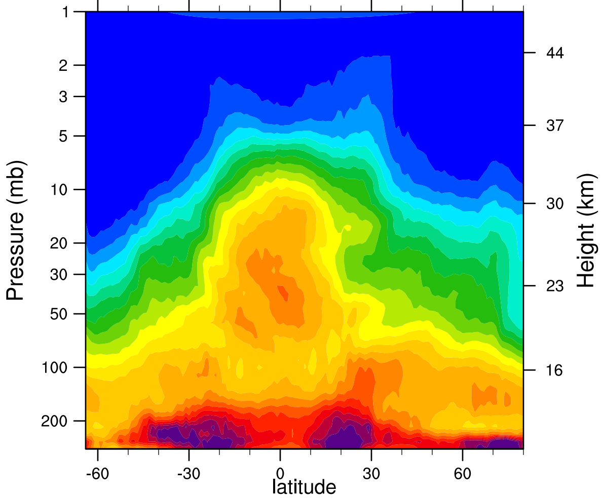
HIRDLSv6 2007d109 N2O_Combined (ppbv)
