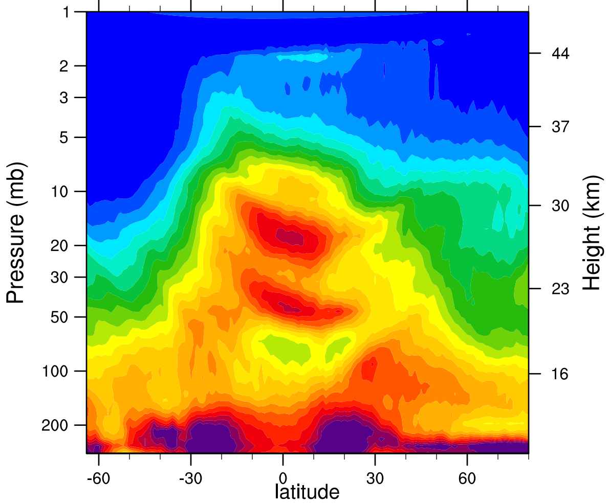
HIRDLSv6 2005d075 N2O_Combined (ppbv)
