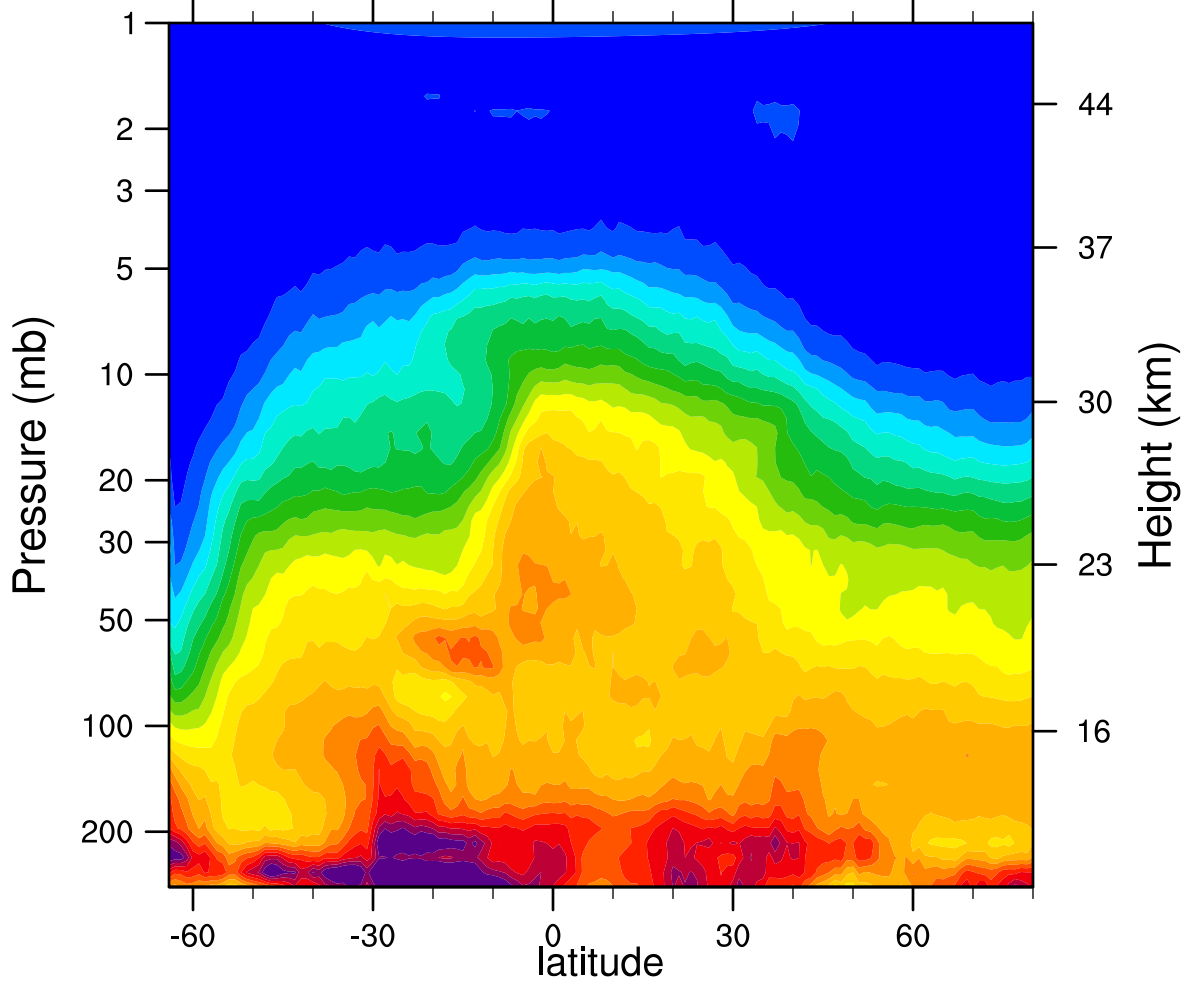
HIRDLSv6 2006d250 N2O_Combined (ppbv)
