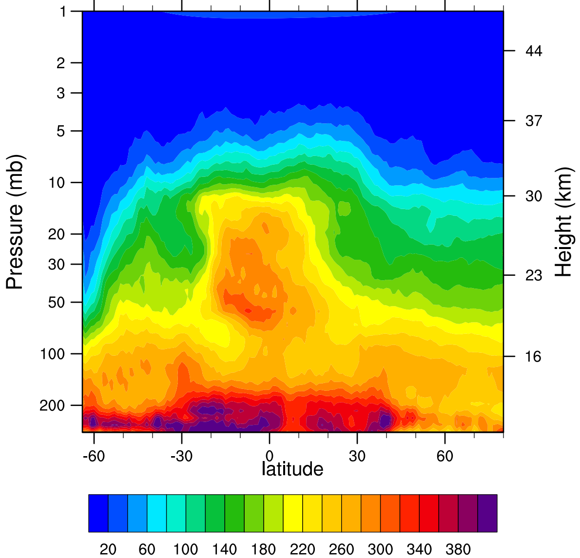
HIRDLSv6 2007d176 N2O_Combined (ppbv)
