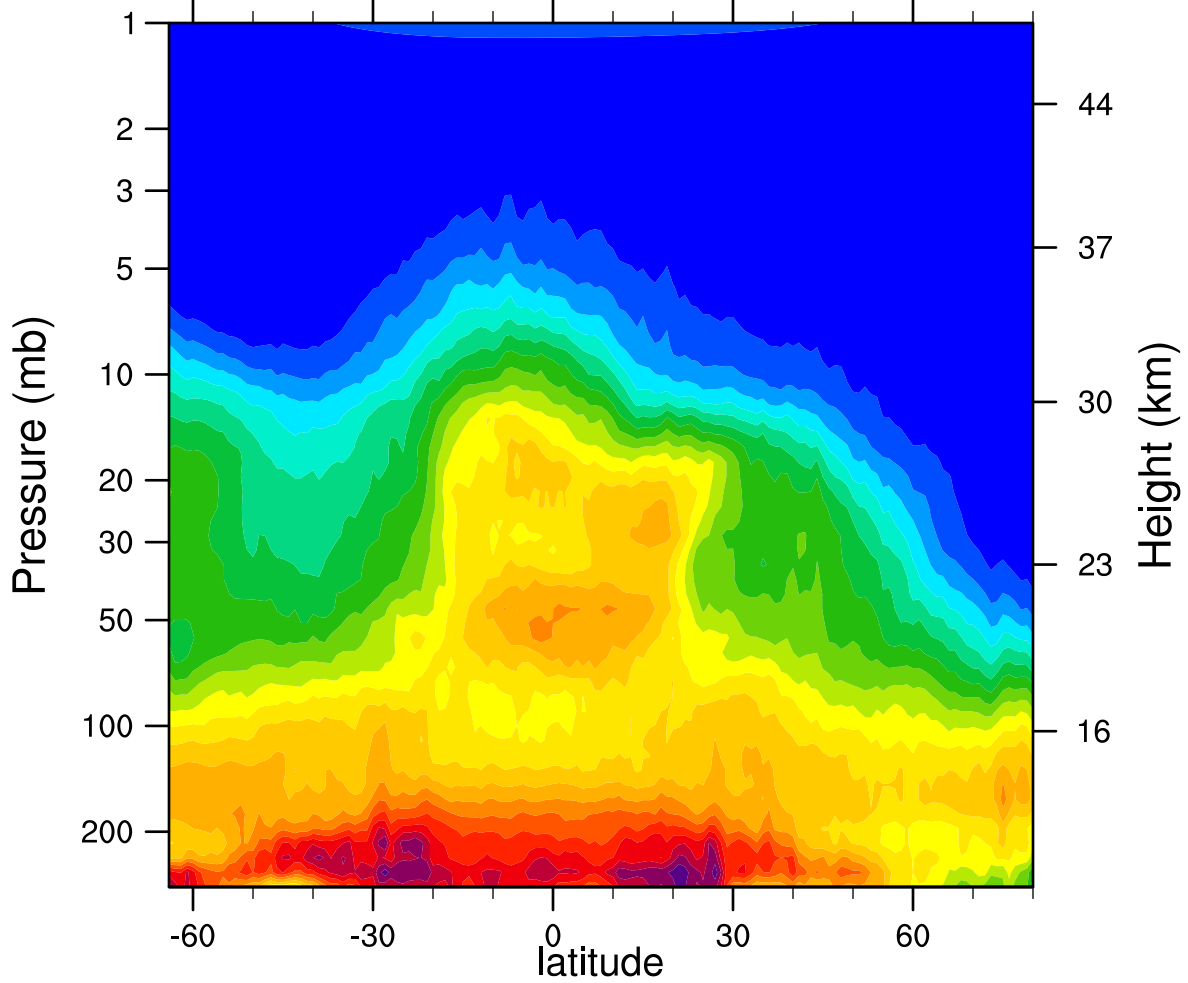
HIRDLSv6 2007d363 N2O_Combined (ppbv)
