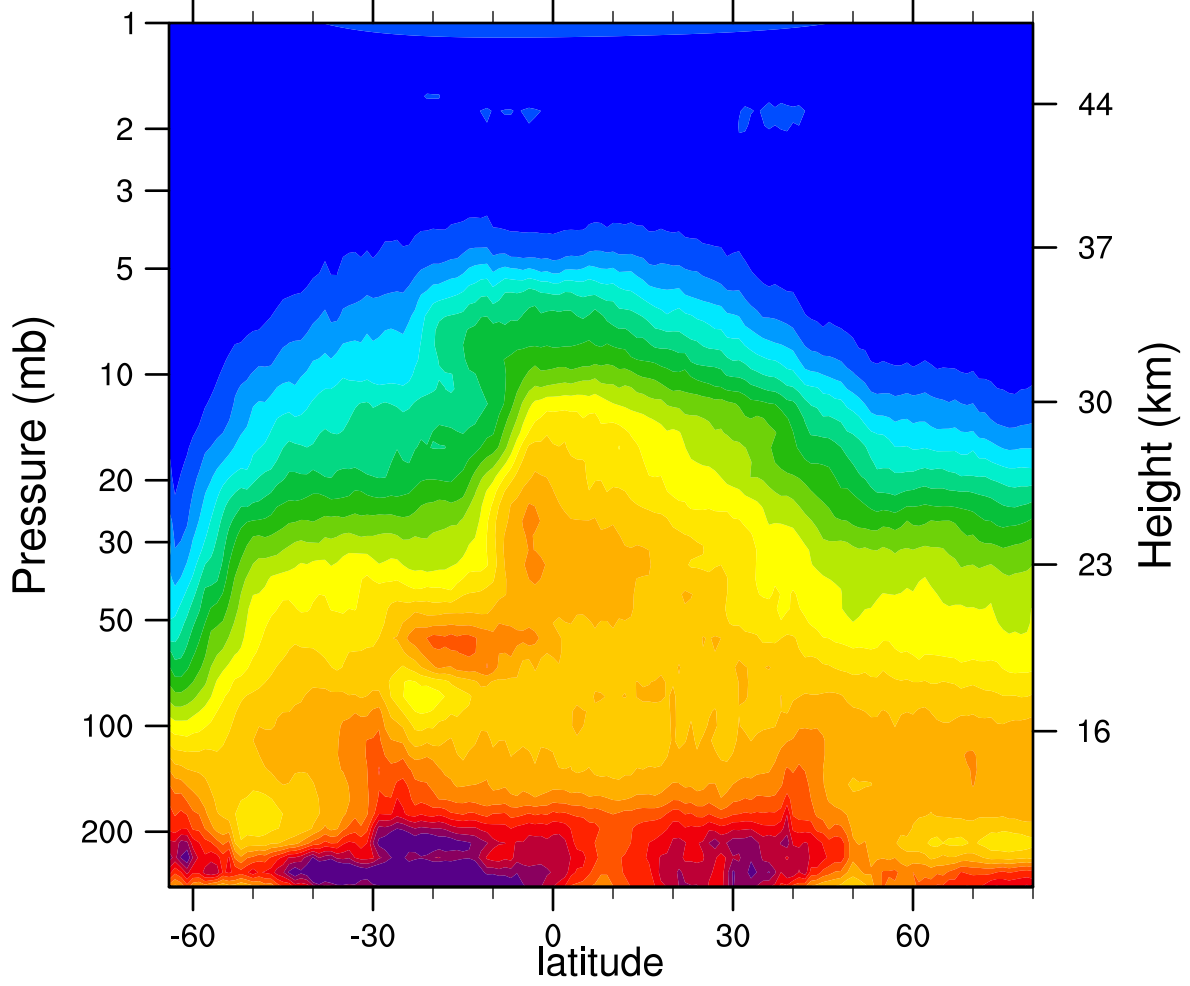
HIRDLSv6 2006d256 N2O_Combined (ppbv)
