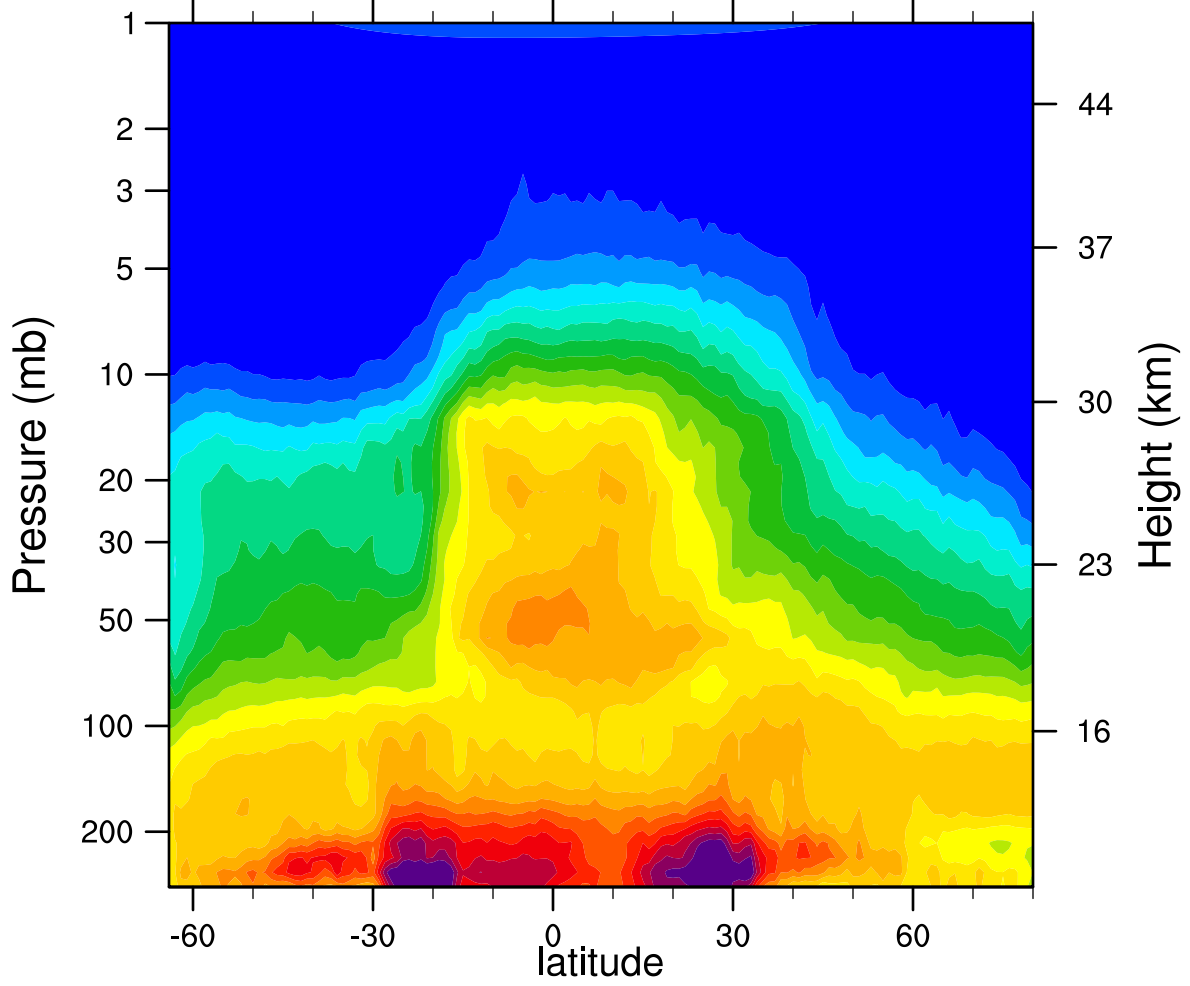
HIRDLSv6 2007d286 N2O_Combined (ppbv)
