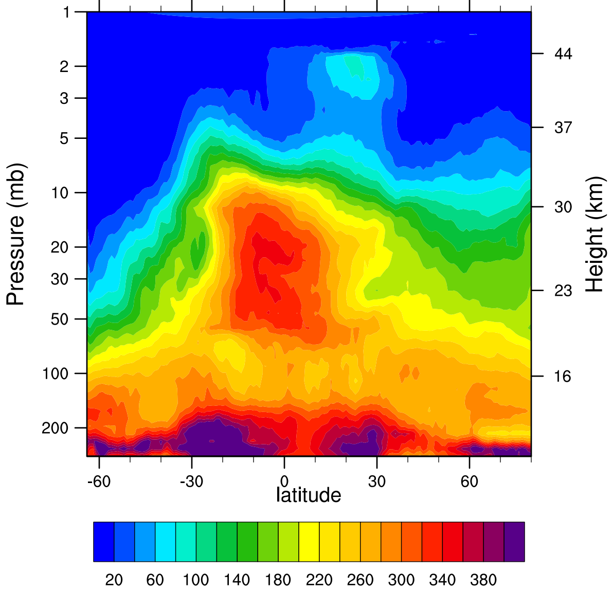
HIRDLSv6 2005d155 N2O_Combined (ppbv)
