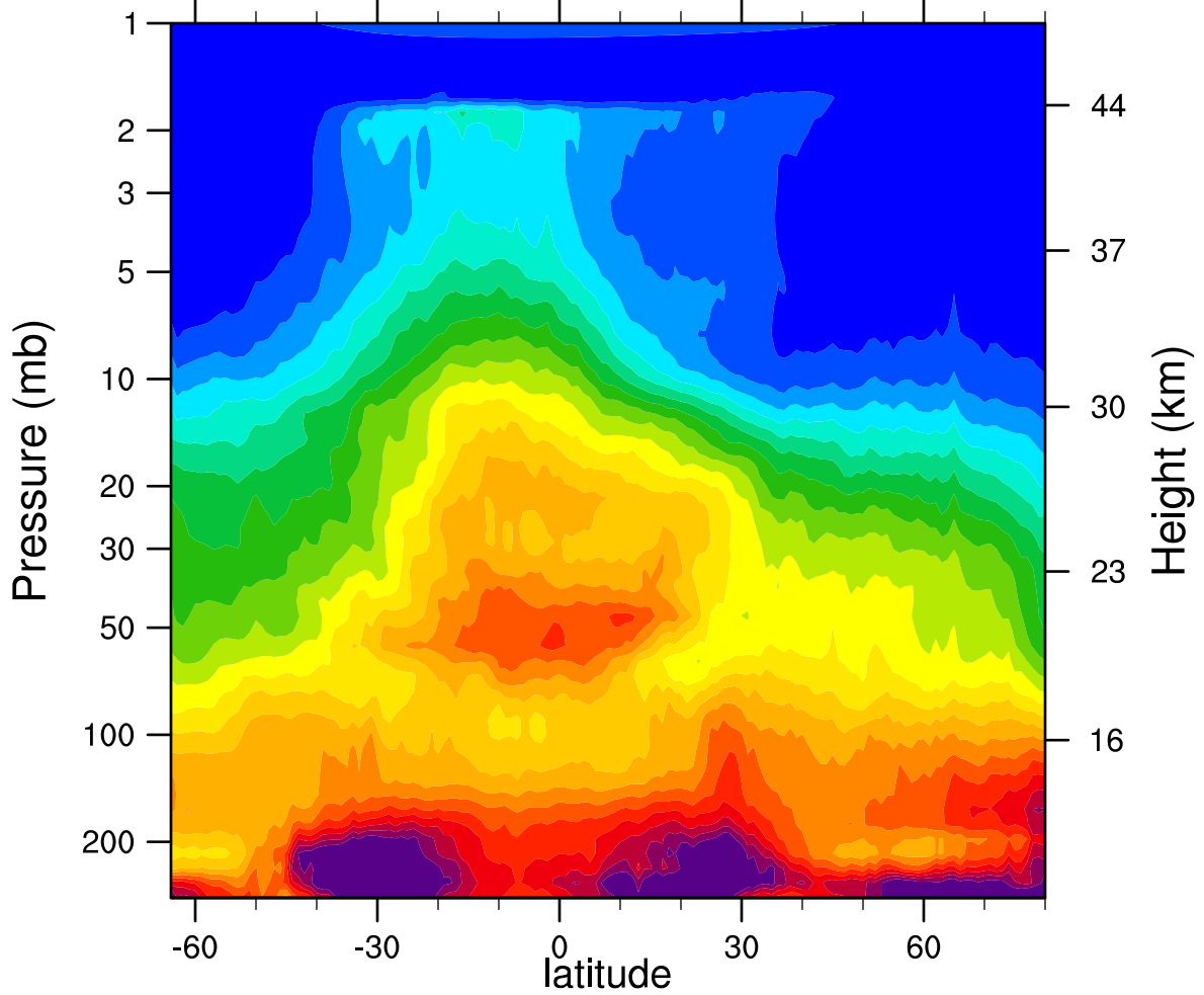
HIRDLSv6 2006d065 N2O_Combined (ppbv)
