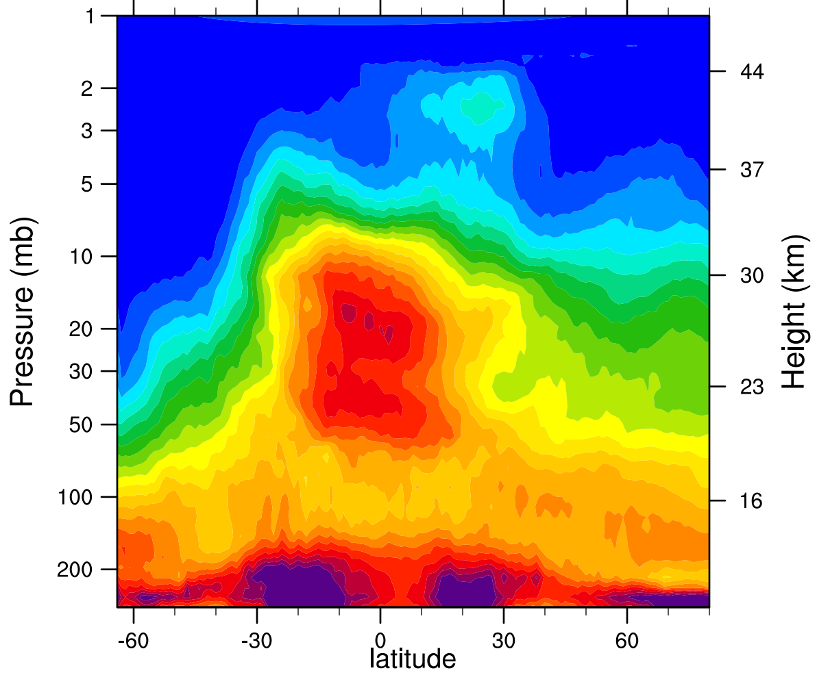
HIRDLSv6 2005d142 N2O_Combined (ppbv)
