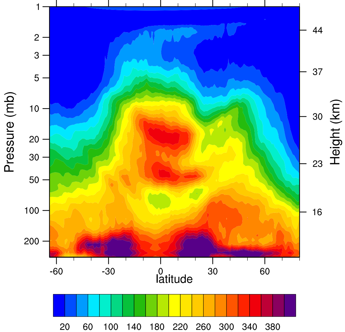
HIRDLSv6 2005d045 N2O_Combined (ppbv)
