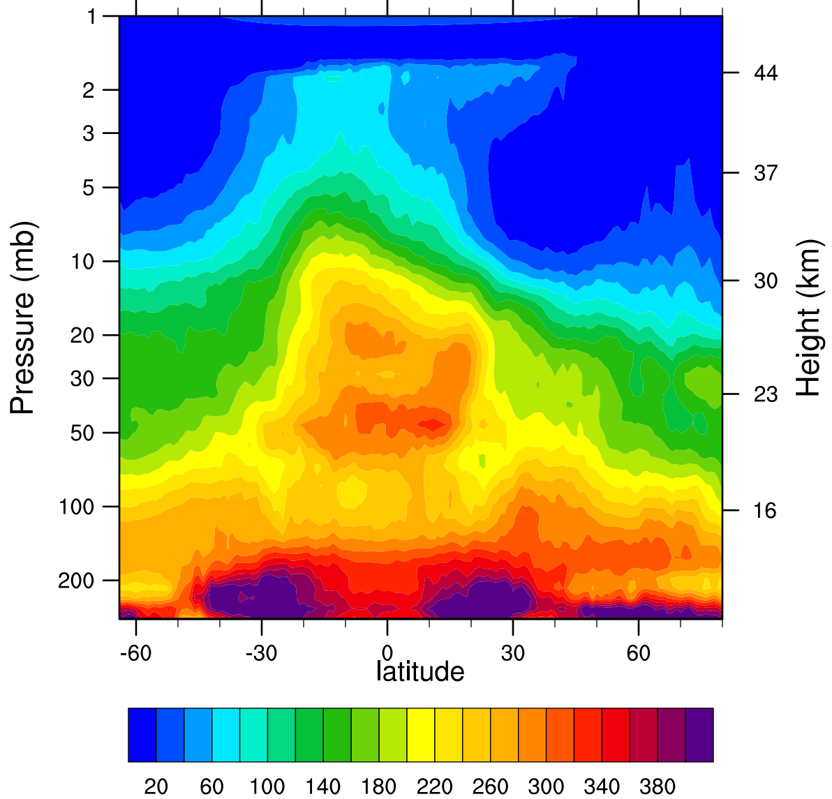
HIRDLSv6 2006d031 N2O_Combined (ppbv)
