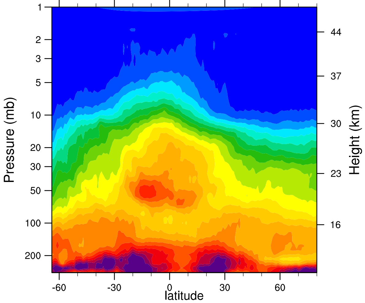
HIRDLSv6 2006d137 N2O_Combined (ppbv)
