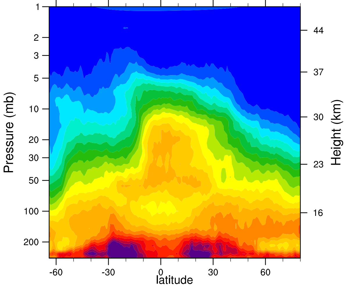
HIRDLSv6 2006d306 N2O_Combined (ppbv)
