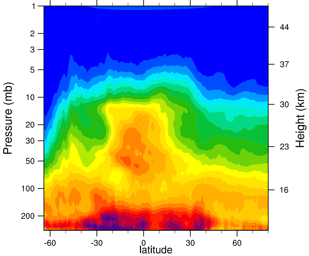
HIRDLSv6 2007d172 N2O_Combined (ppbv)
