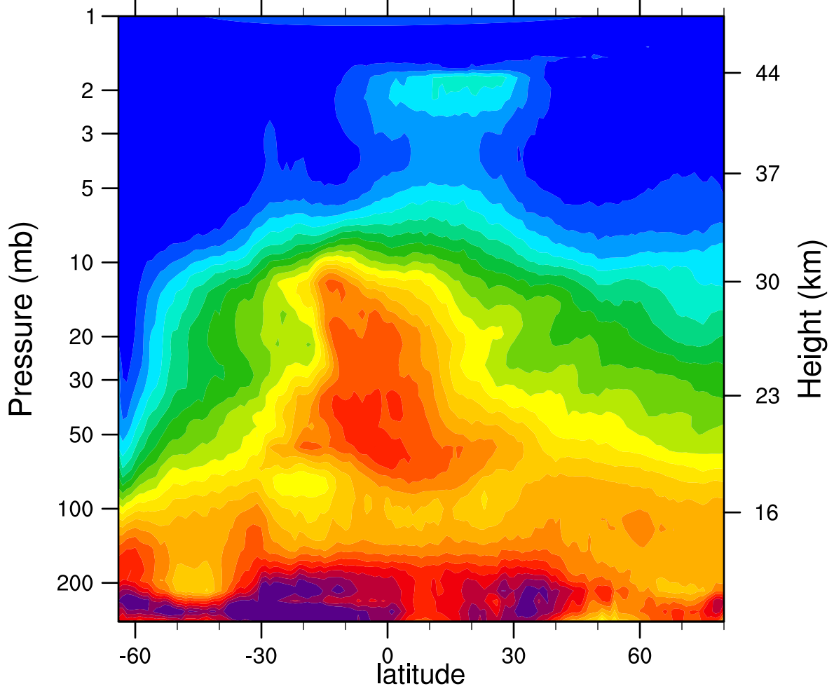
HIRDLSv6 2005d214 N2O_Combined (ppbv)
