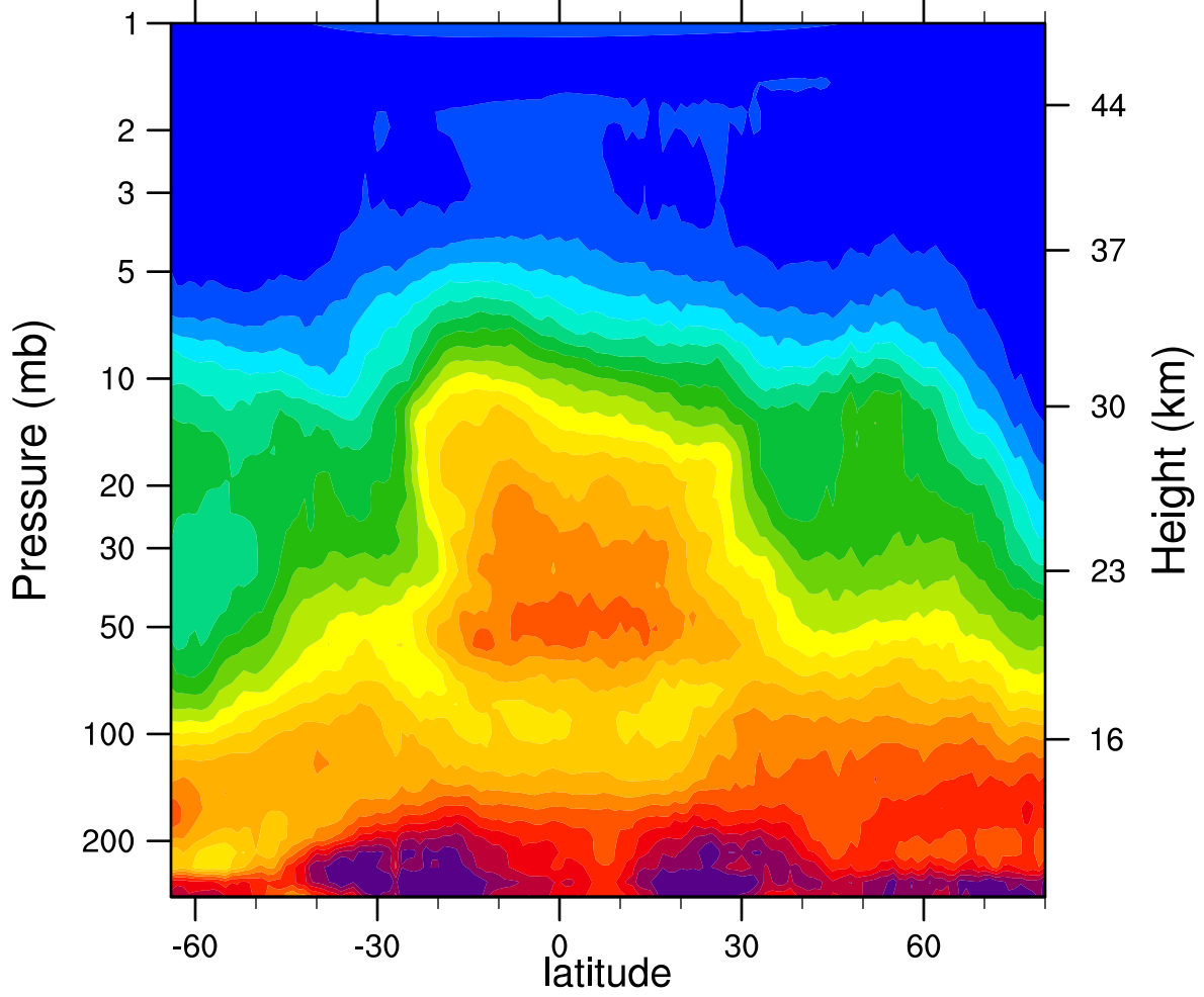
HIRDLSv6 2005d320 N2O_Combined (ppbv)
