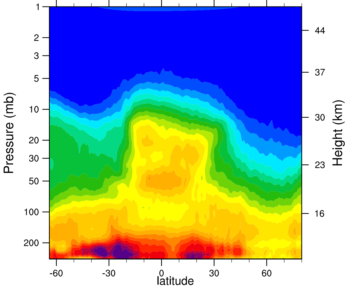
HIRDLSv6 2007d332 N2O_Combined (ppbv)
