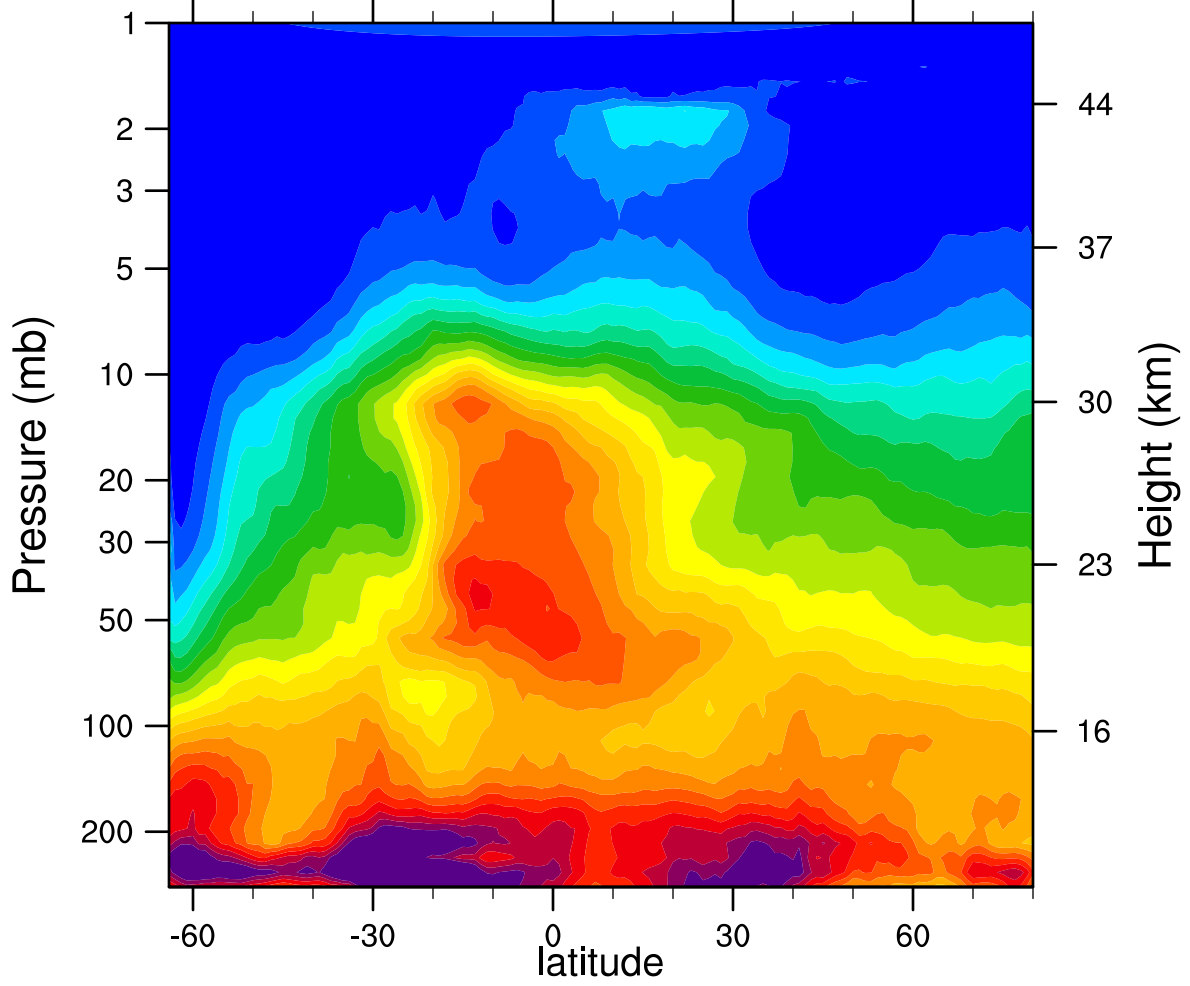
HIRDLSv6 2005d194 N2O_Combined (ppbv)
