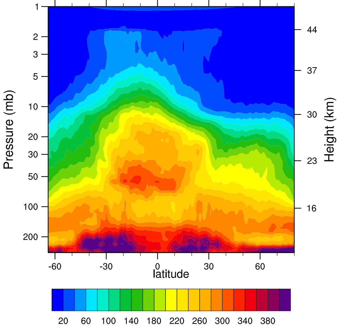
HIRDLSv6 2006d101 N2O_Combined (ppbv)
