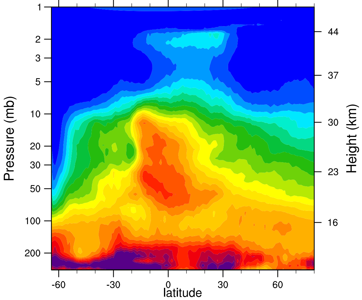
HIRDLSv6 2005d223 N2O_Combined (ppbv)
