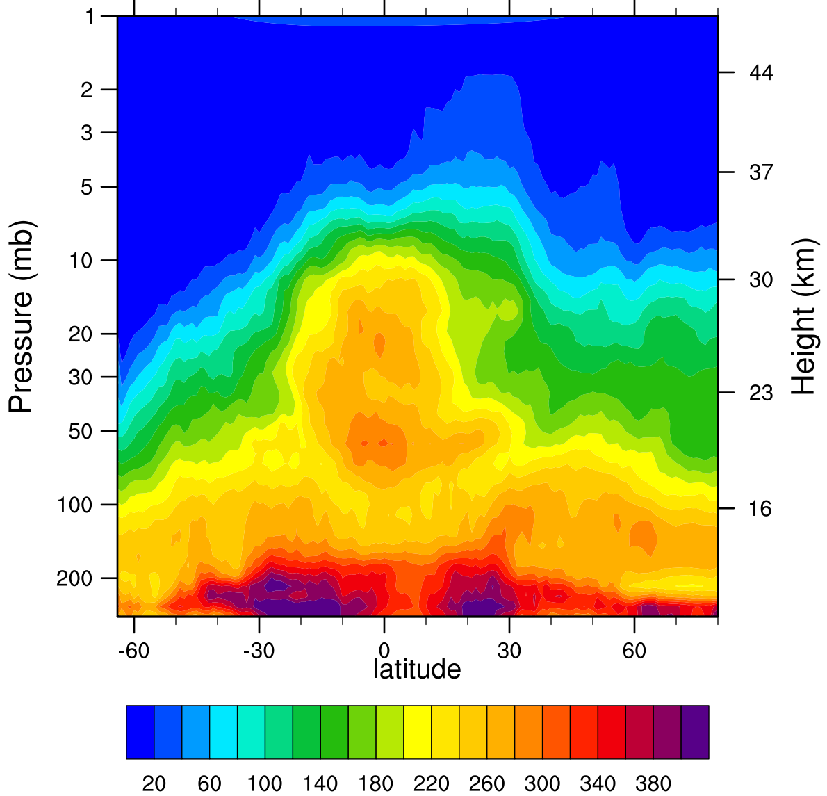
HIRDLSv6 2007d137 N2O_Combined (ppbv)
