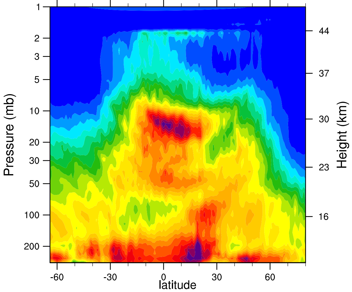
HIRDLSv6 2005d026 N2O_Combined (ppbv)
