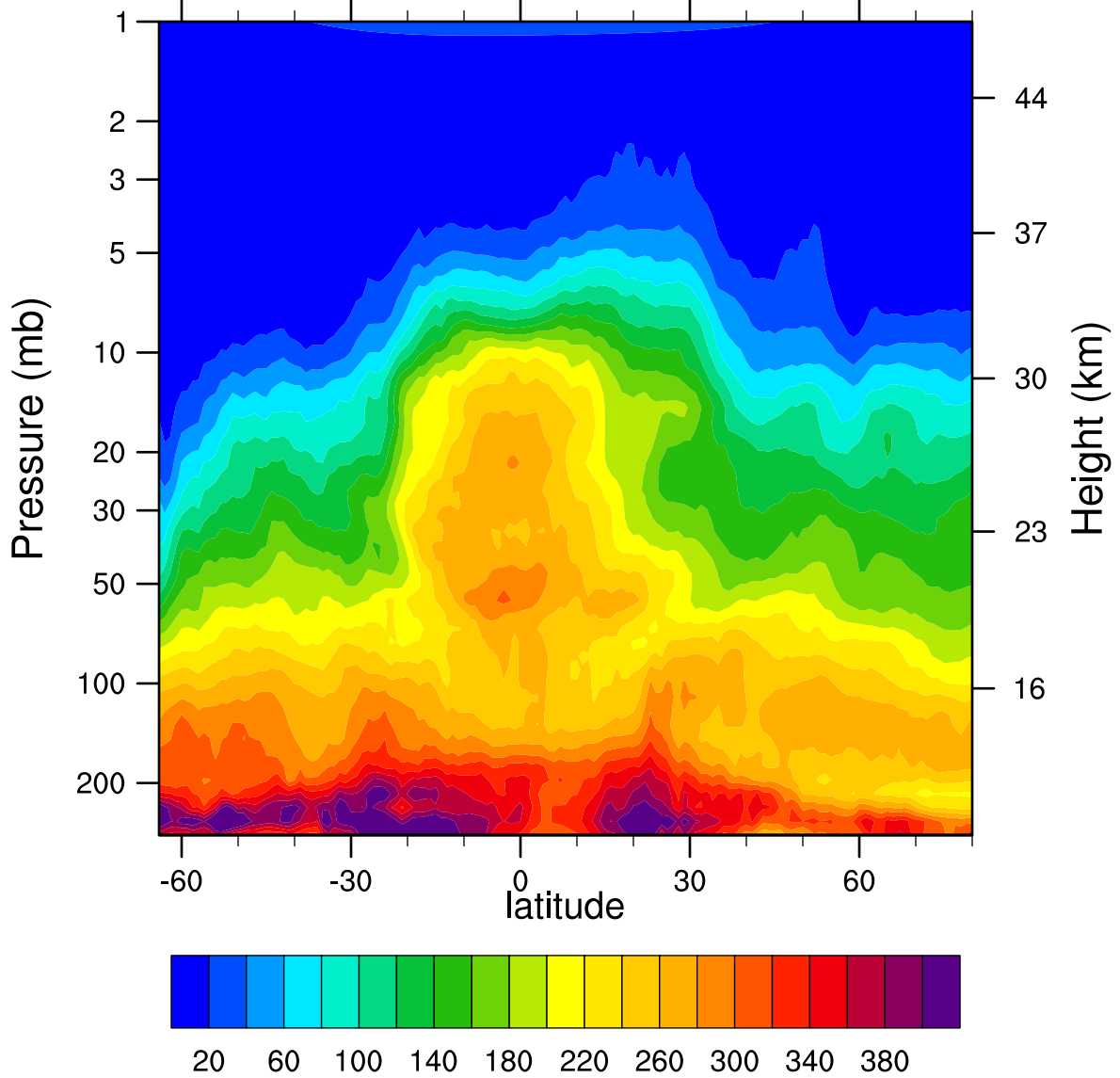
HIRDLSv6 2007d149 N2O_Combined (ppbv)
