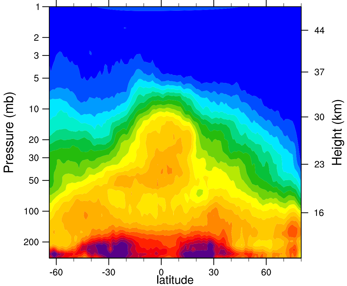
HIRDLSv6 2006d361 N2O_Combined (ppbv)
