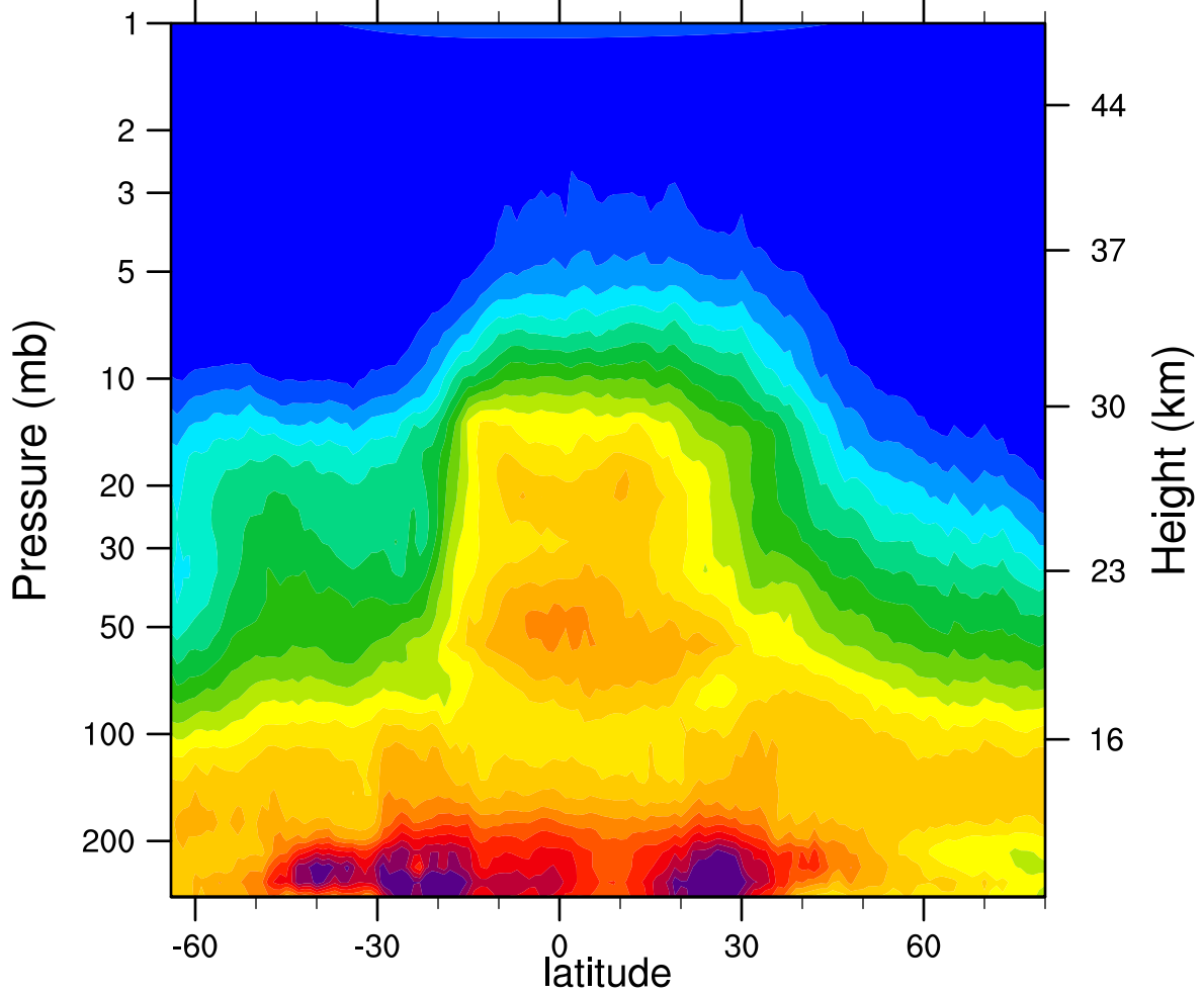
HIRDLSv6 2007d290 N2O_Combined (ppbv)
