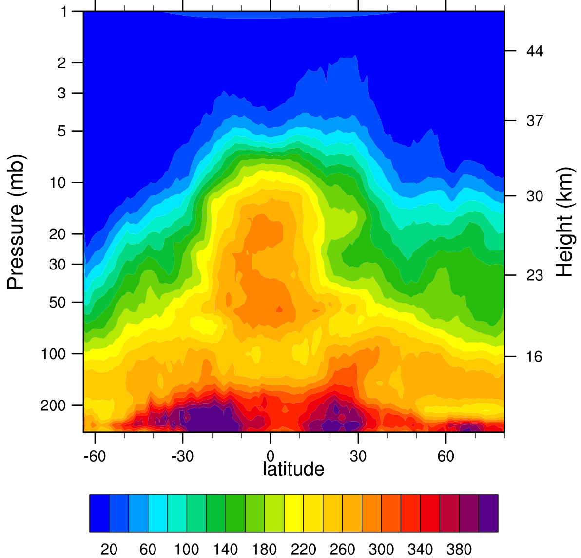
HIRDLSv6 2007d127 N2O_Combined (ppbv)
