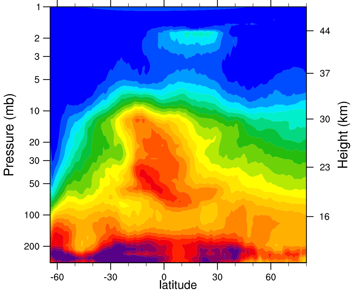
HIRDLSv6 2005d203 N2O_Combined (ppbv)
