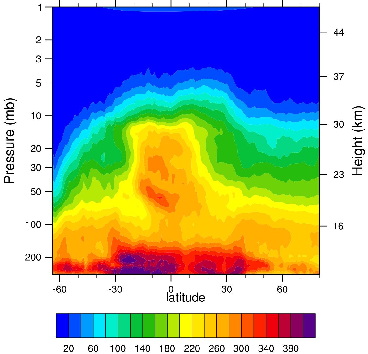
HIRDLSv6 2007d180 N2O_Combined (ppbv)
