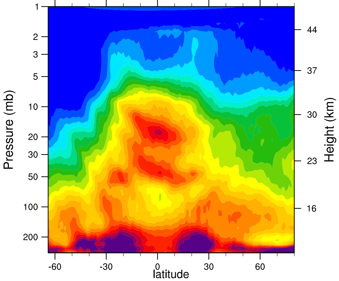
HIRDLSv6 2005d100 N2O_Combined (ppbv)
