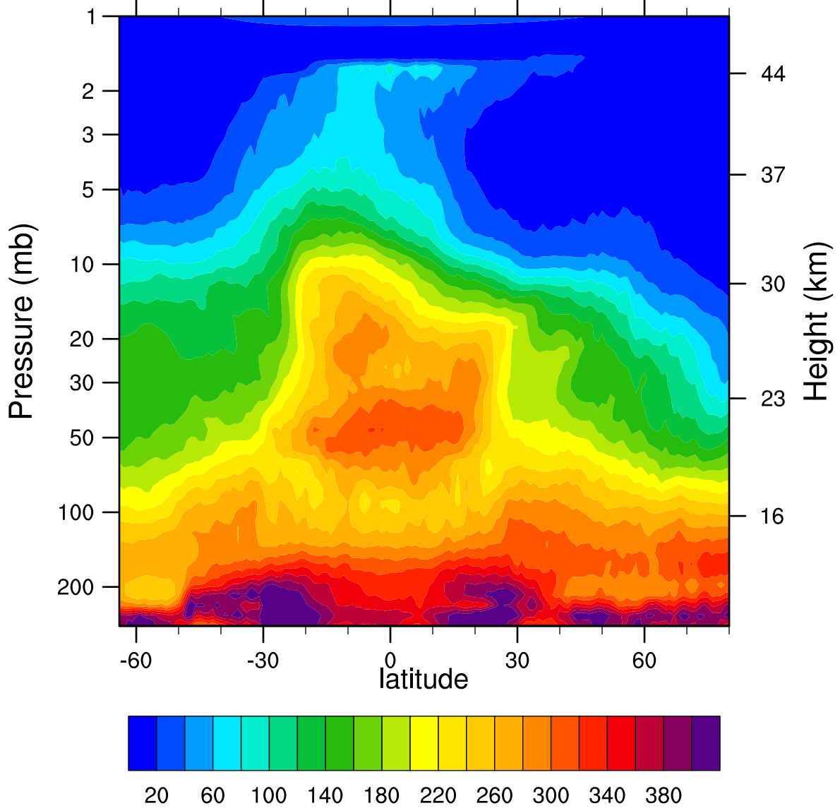
HIRDLSv6 2006d003 N2O_Combined (ppbv)
