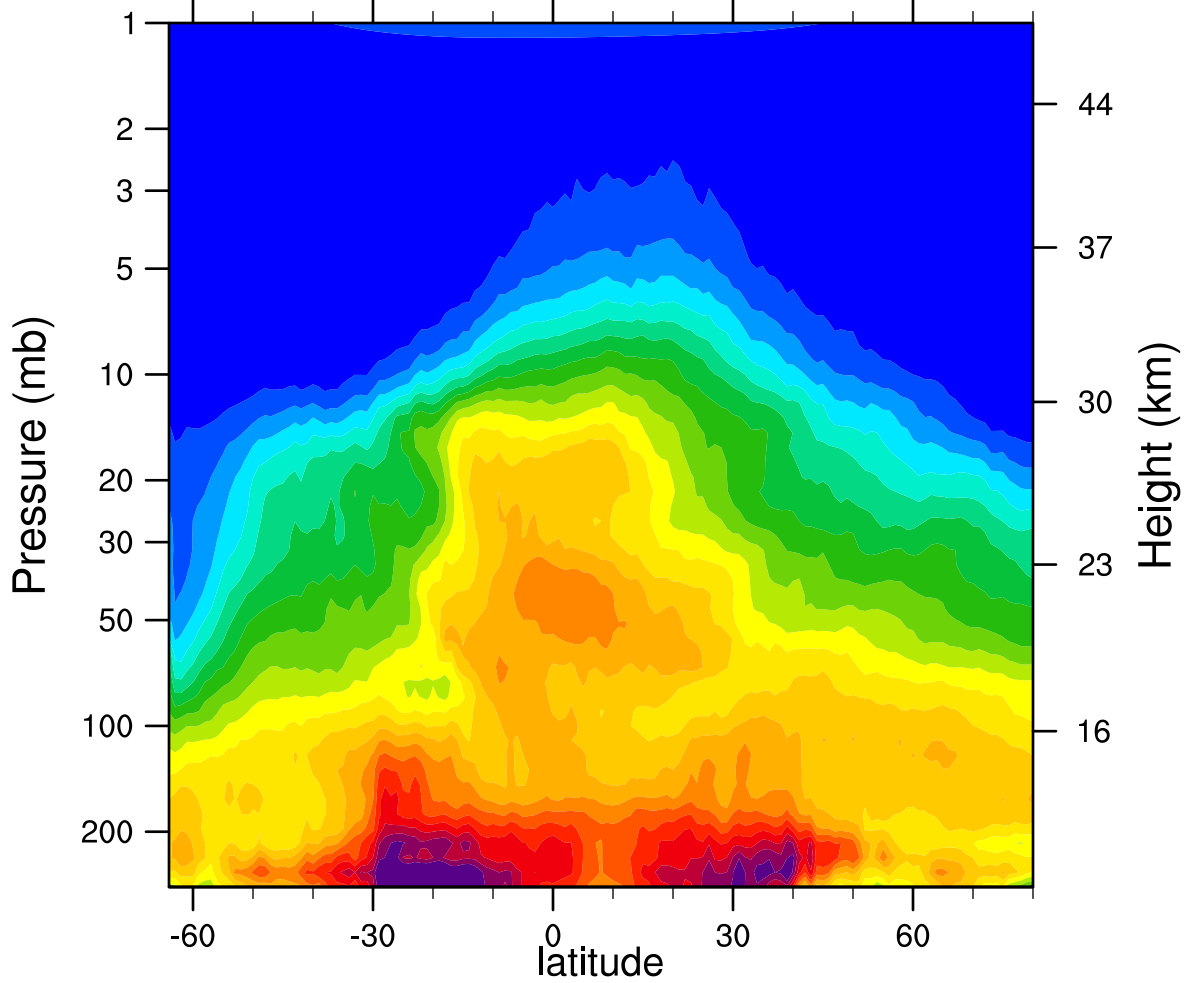
HIRDLSv6 2007d241 N2O_Combined (ppbv)
