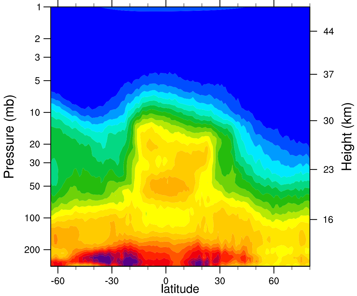
HIRDLSv6 2007d334 N2O_Combined (ppbv)
