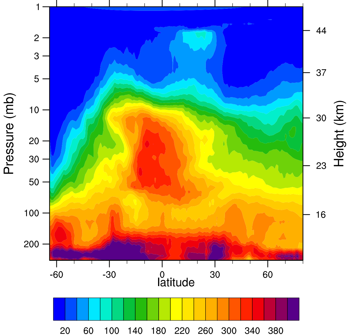
HIRDLSv6 2005d176 N2O_Combined (ppbv)
