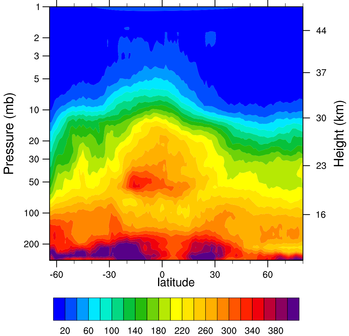
HIRDLSv6 2006d143 N2O_Combined (ppbv)
