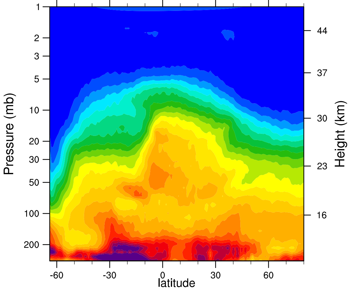
HIRDLSv6 2006d248 N2O_Combined (ppbv)
