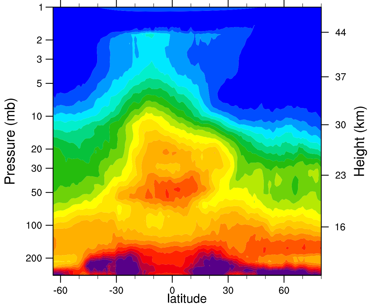
HIRDLSv6 2006d047 N2O_Combined (ppbv)
