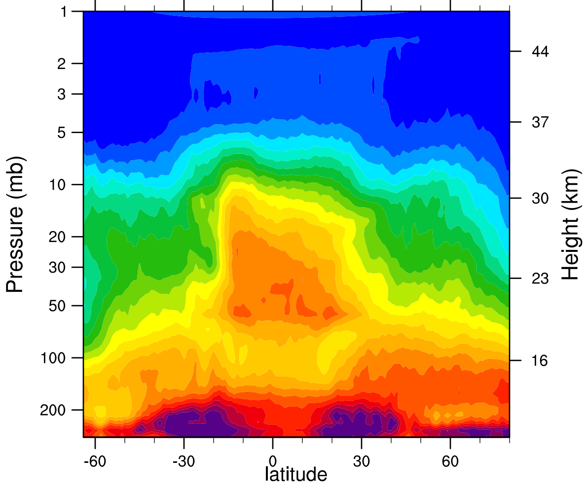
HIRDLSv6 2005d307 N2O_Combined (ppbv)
