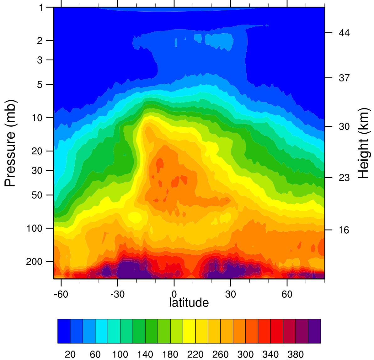
HIRDLSv6 2005d281 N2O_Combined (ppbv)
