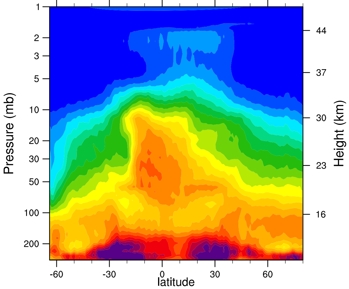
HIRDLSv6 2005d265 N2O_Combined (ppbv)
