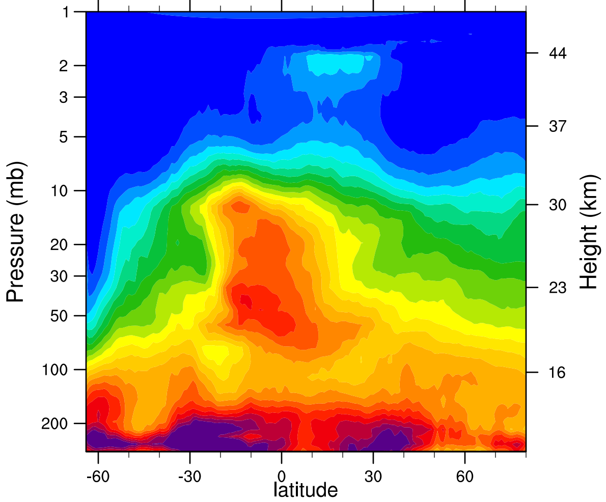
HIRDLSv6 2005d195 N2O_Combined (ppbv)
