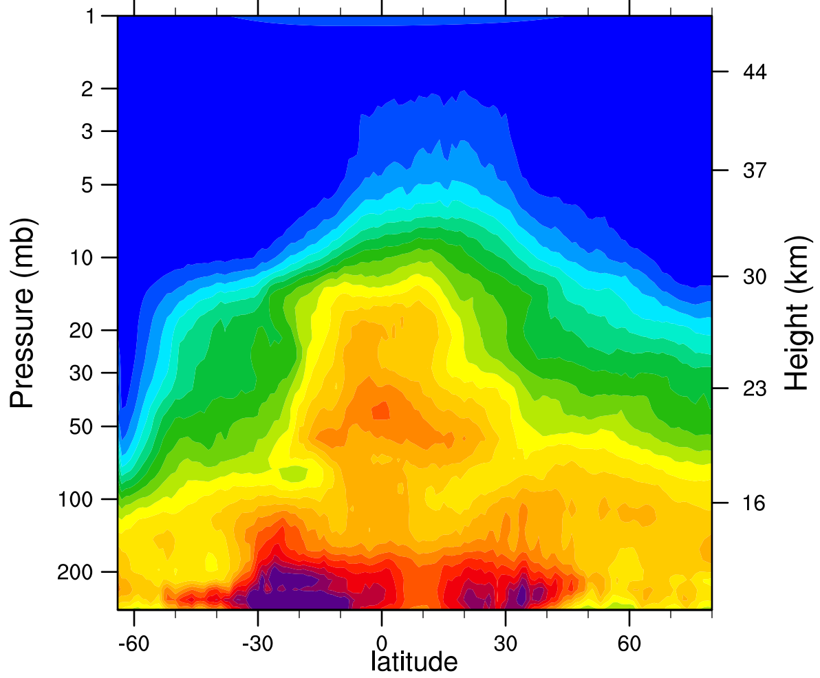
HIRDLSv6 2007d234 N2O_Combined (ppbv)
