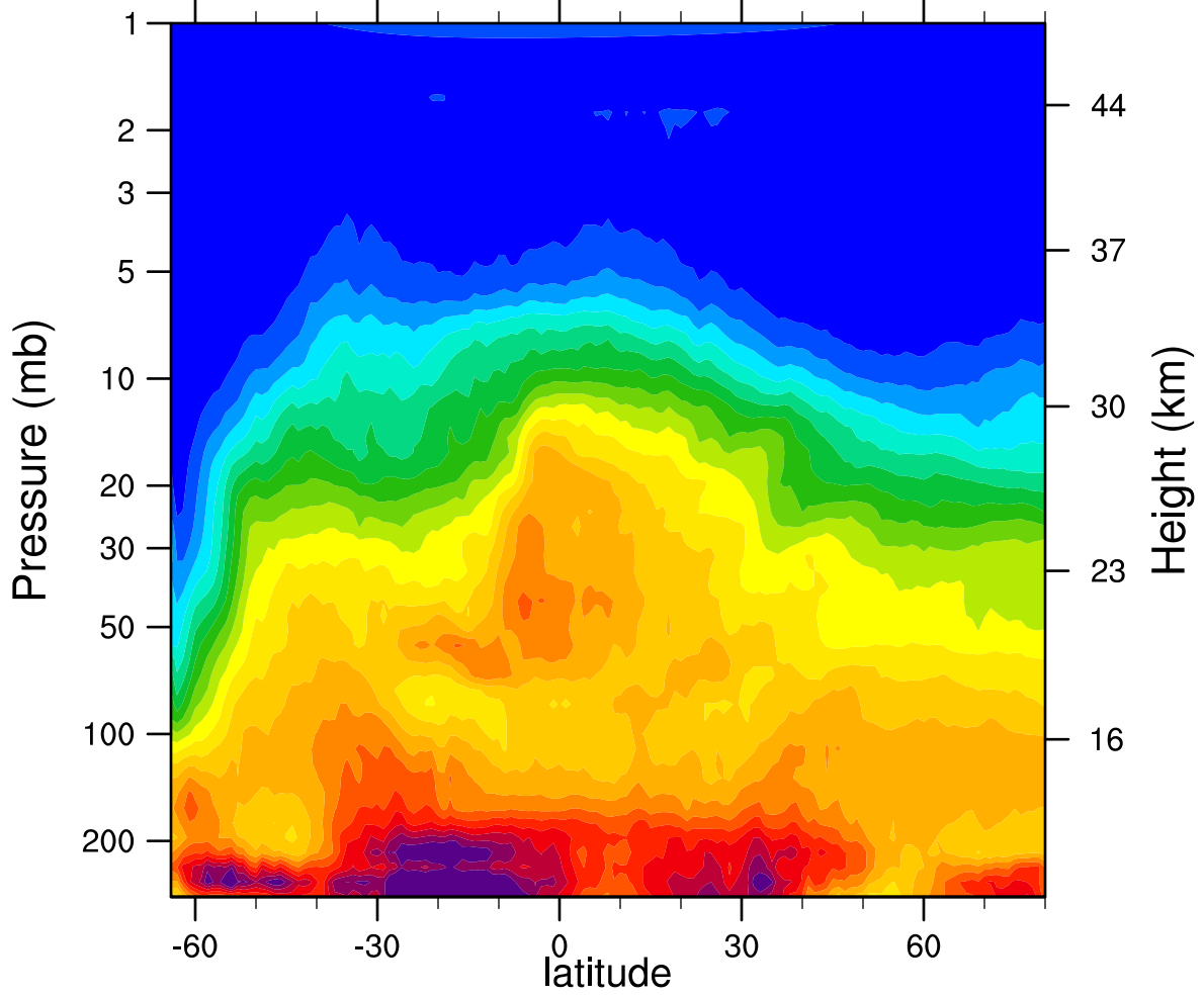
HIRDLSv6 2006d218 N2O_Combined (ppbv)
