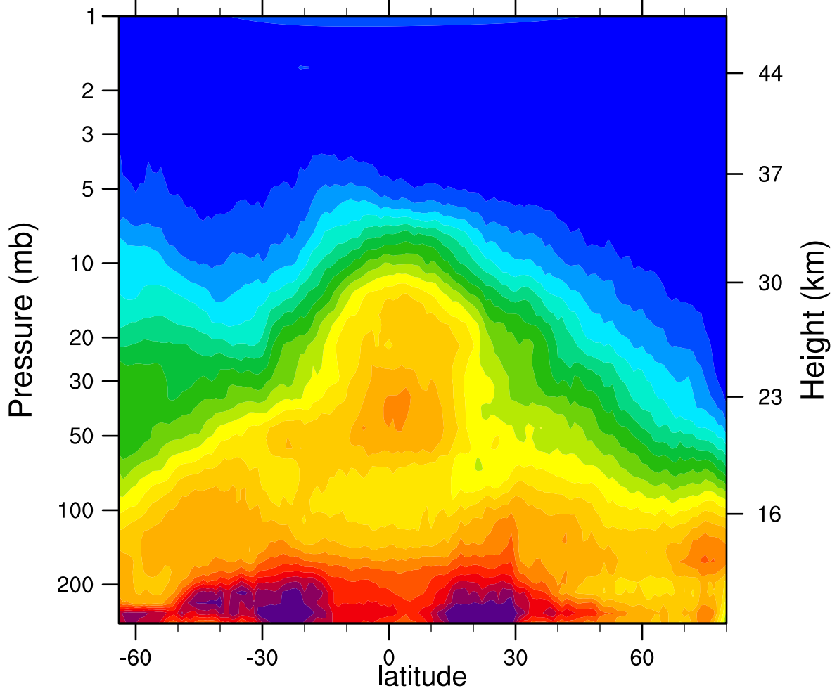
HIRDLSv6 2006d356 N2O_Combined (ppbv)
