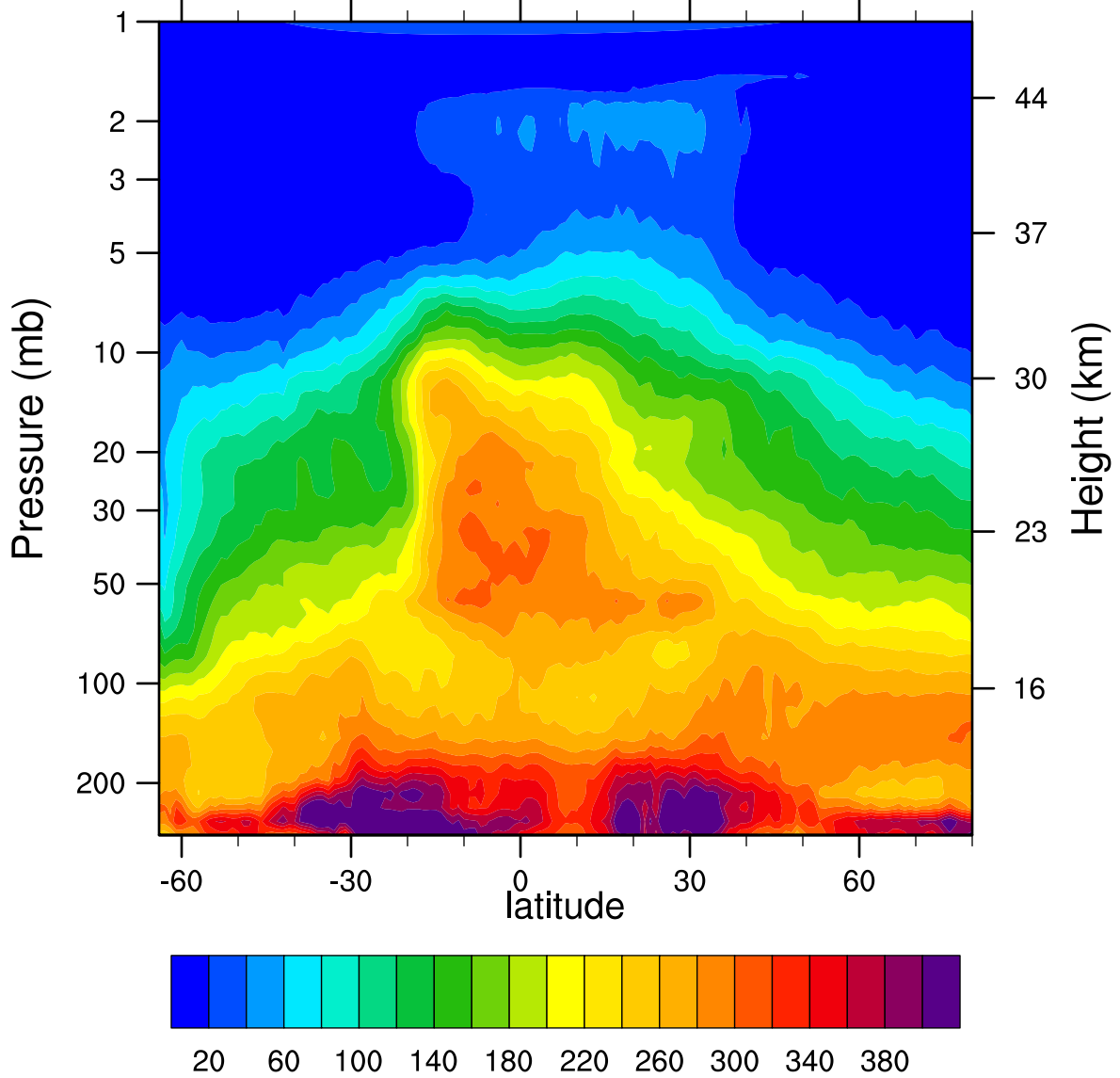
HIRDLSv6 2005d273 N2O_Combined (ppbv)
