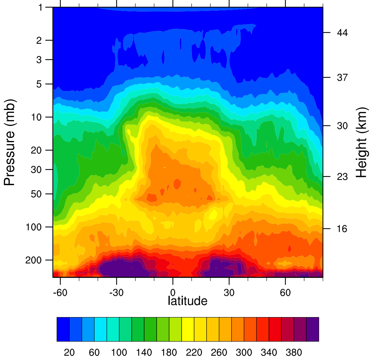
HIRDLSv6 2005d312 N2O_Combined (ppbv)
