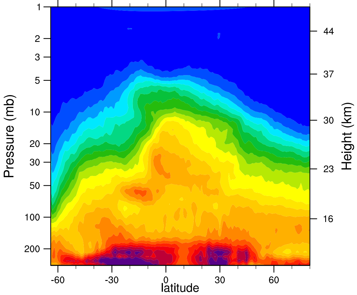
HIRDLSv6 2006d268 N2O_Combined (ppbv)
