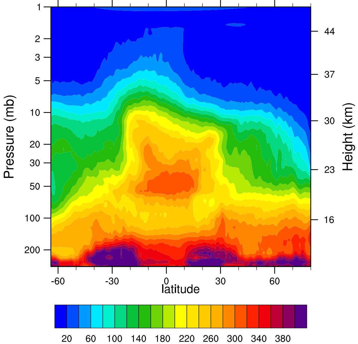
HIRDLSv6 2005d342 N2O_Combined (ppbv)
