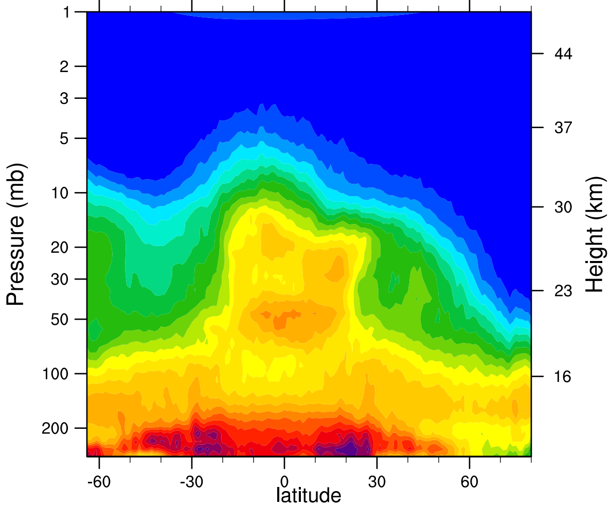
HIRDLSv6 2007d362 N2O_Combined (ppbv)
