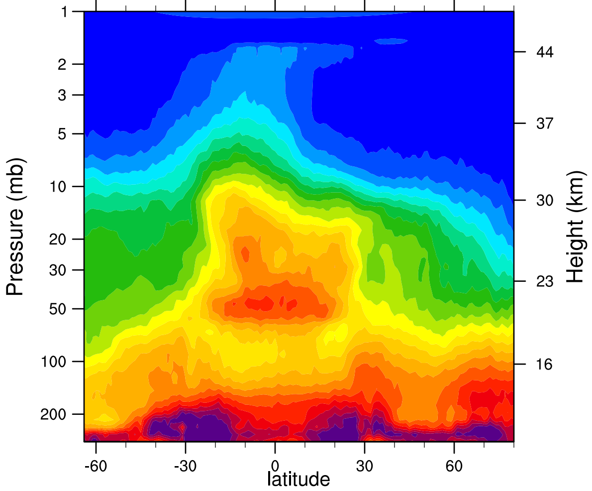
HIRDLSv6 2005d355 N2O_Combined (ppbv)
