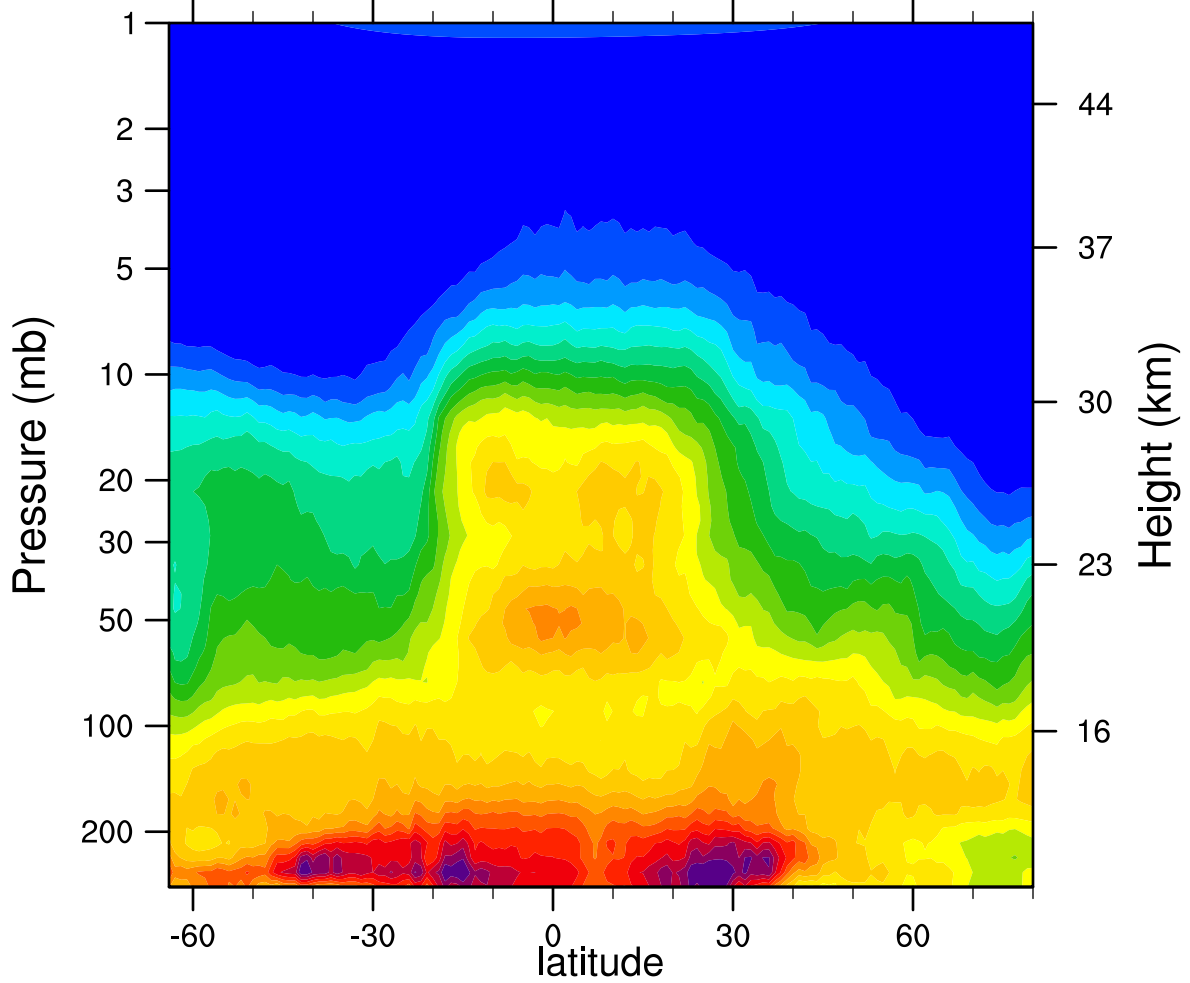
HIRDLSv6 2007d305 N2O_Combined (ppbv)
