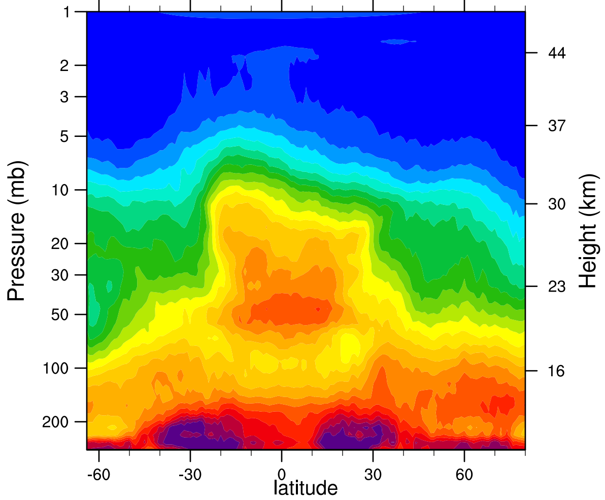
HIRDLSv6 2005d331 N2O_Combined (ppbv)
