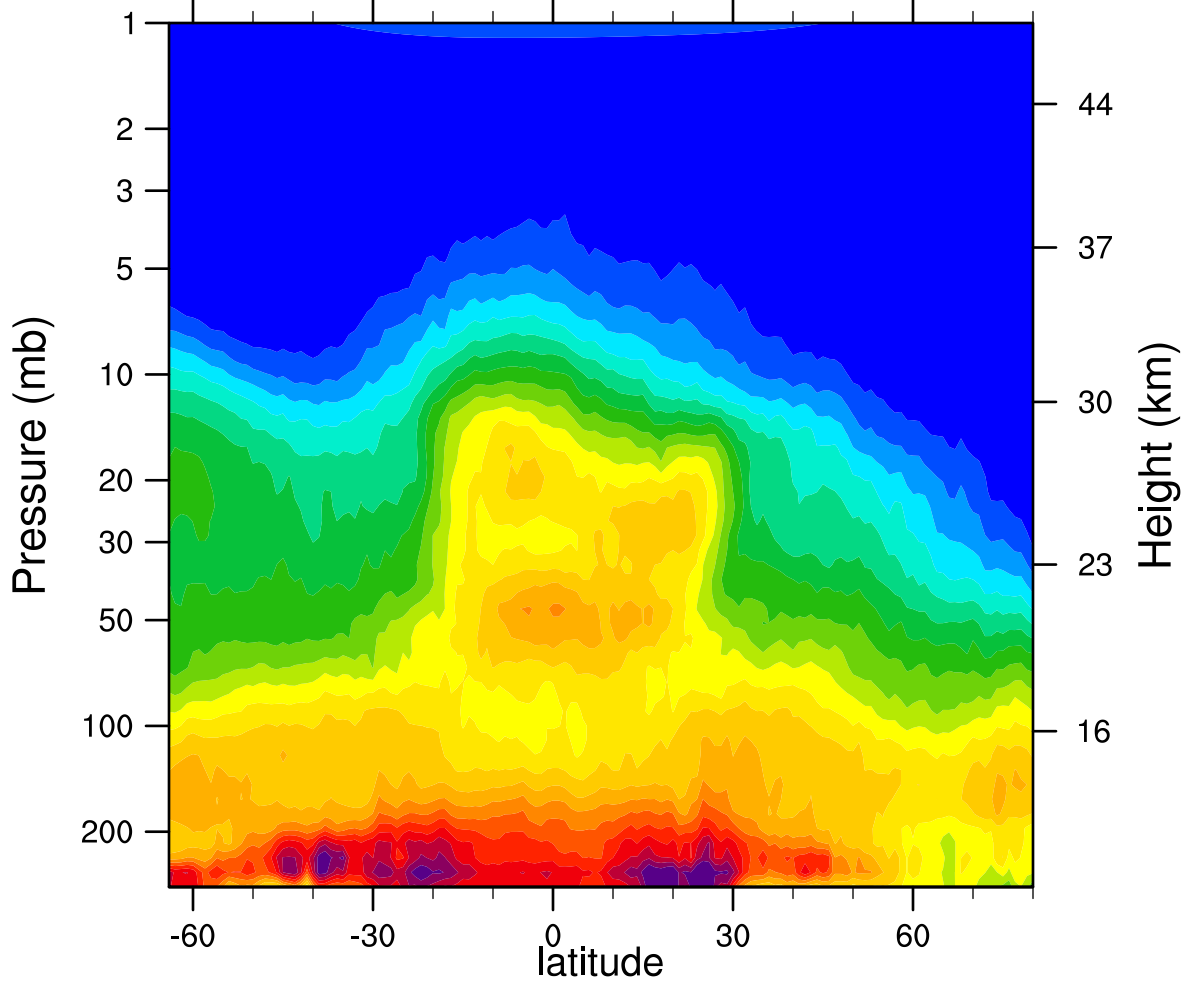
HIRDLSv6 2007d345 N2O_Combined (ppbv)
