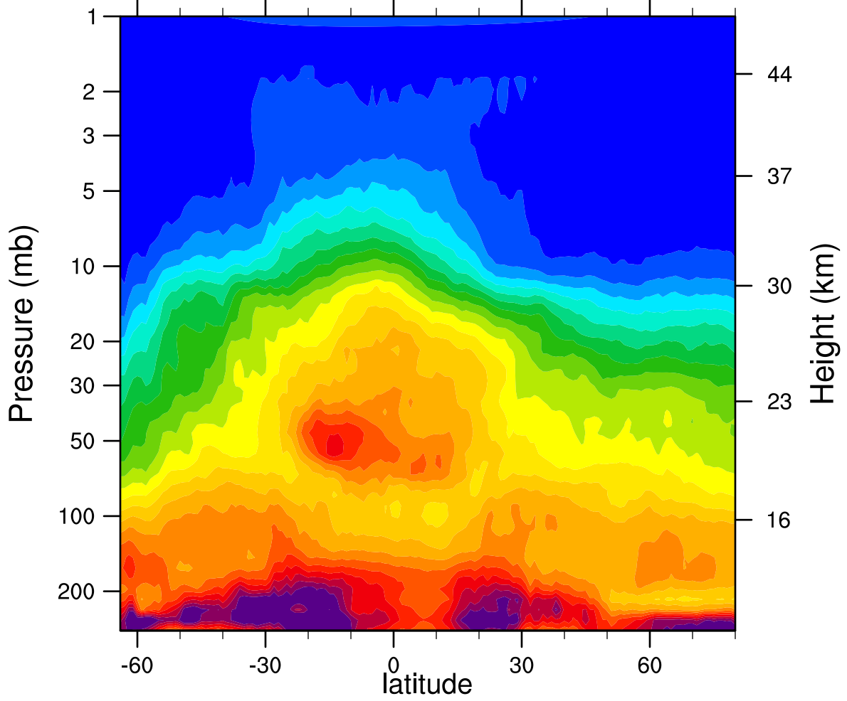
HIRDLSv6 2006d133 N2O_Combined (ppbv)
