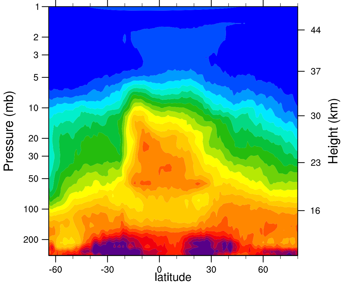
HIRDLSv6 2005d295 N2O_Combined (ppbv)
