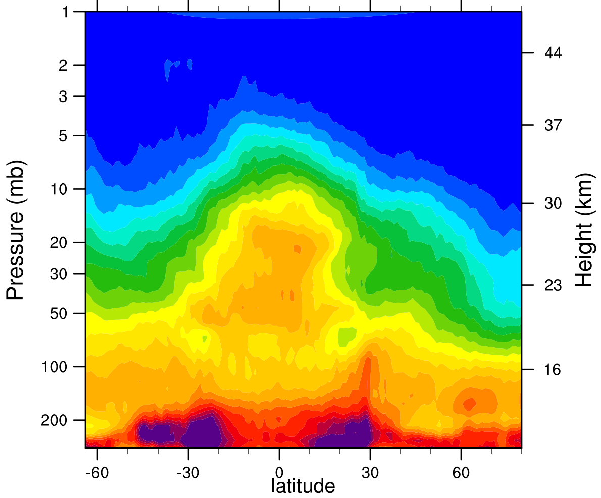
HIRDLSv6 2007d051 N2O_Combined (ppbv)
