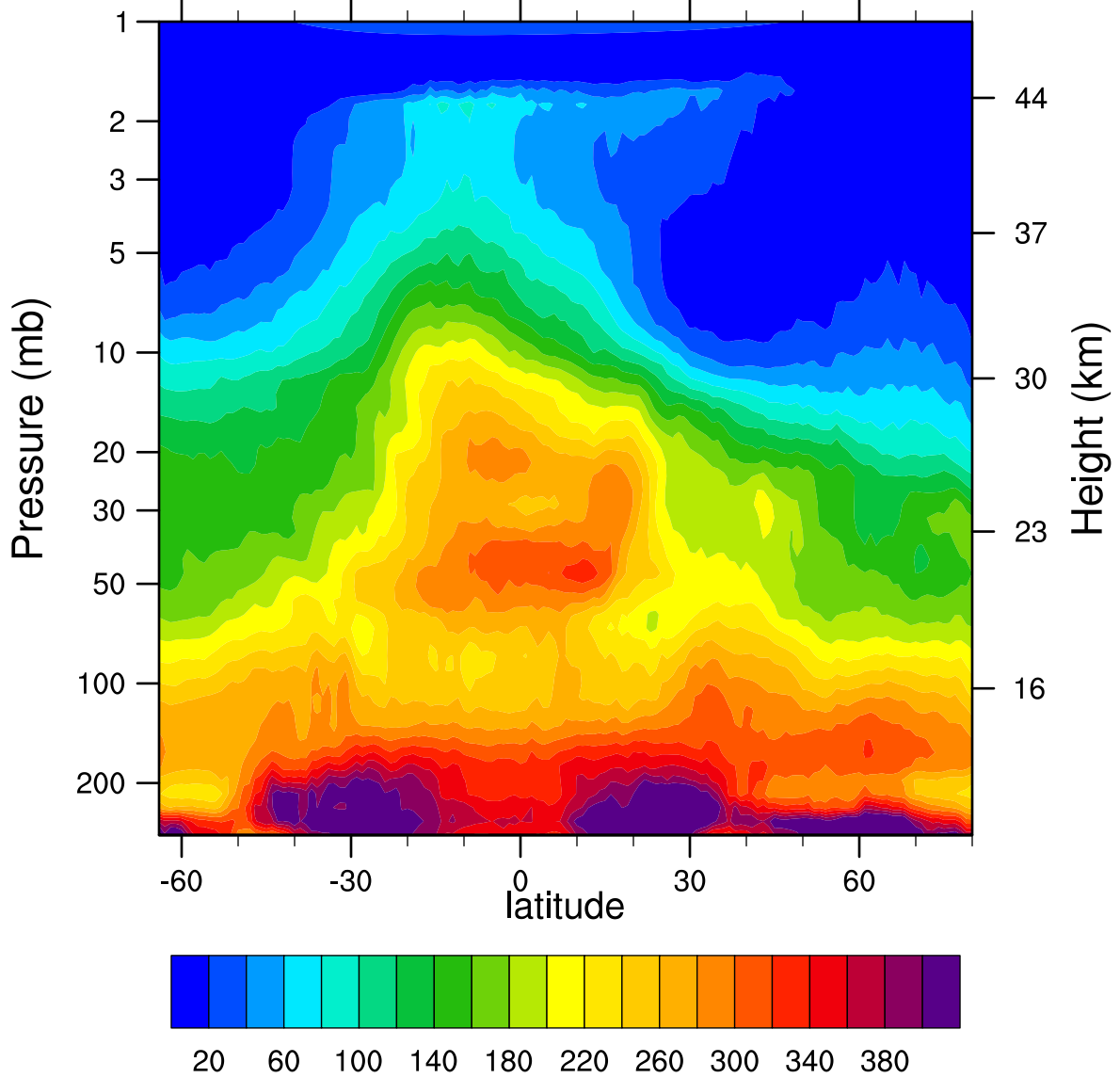
HIRDLSv6 2006d034 N2O_Combined (ppbv)
