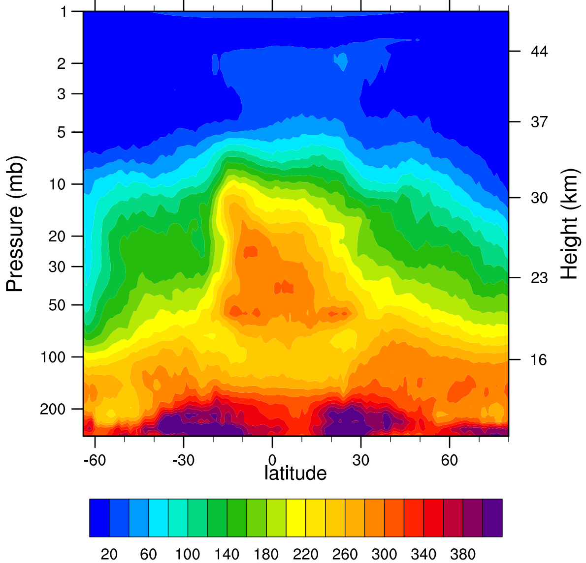
HIRDLSv6 2005d292 N2O_Combined (ppbv)
