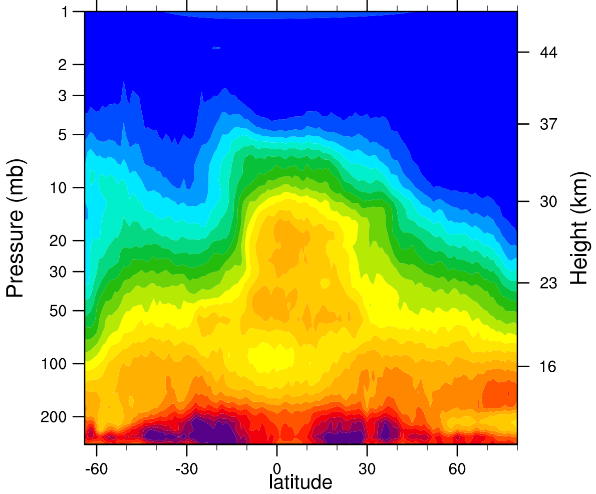
HIRDLSv6 2006d309 N2O_Combined (ppbv)
