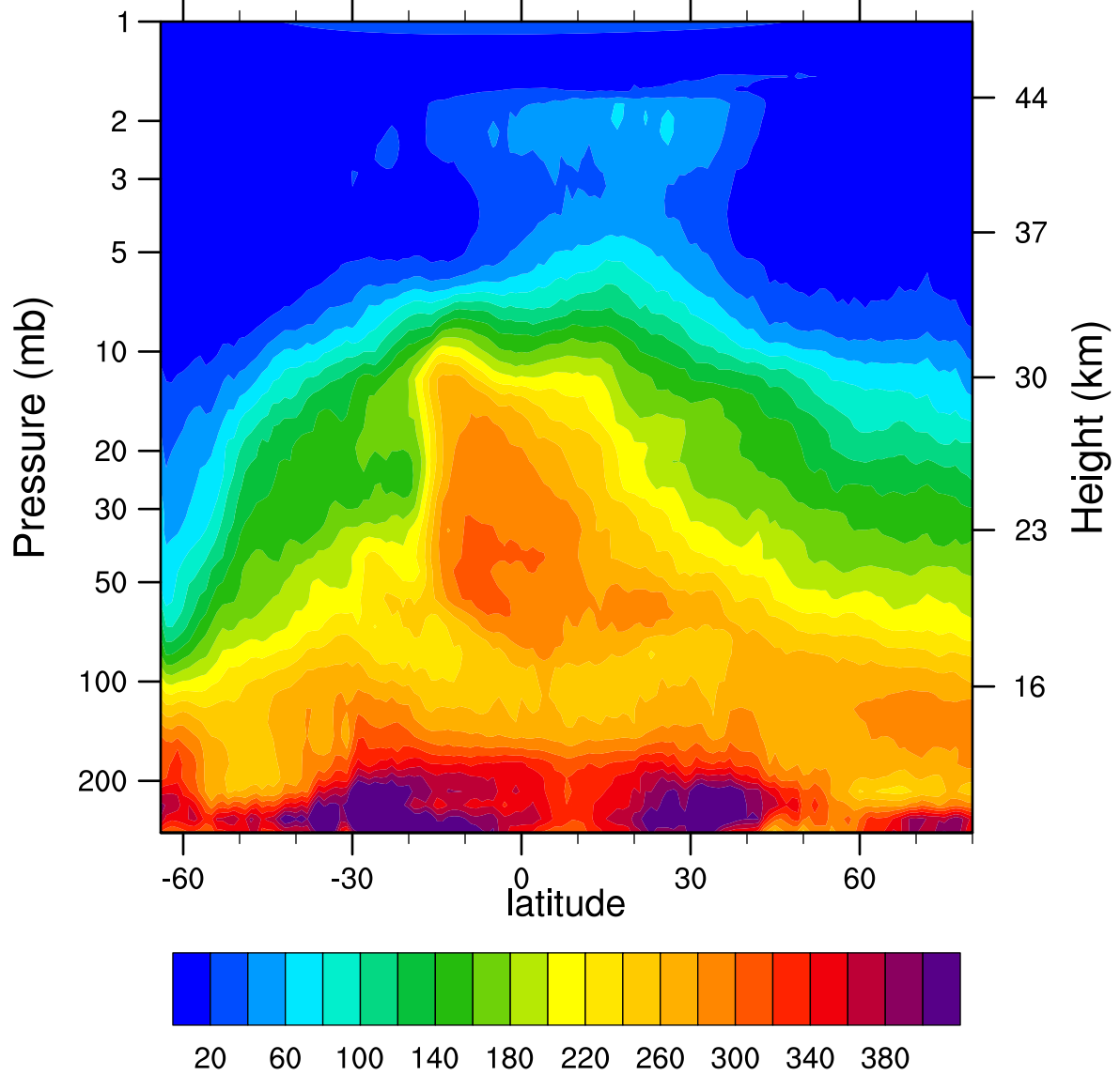
HIRDLSv6 2005d255 N2O_Combined (ppbv)
