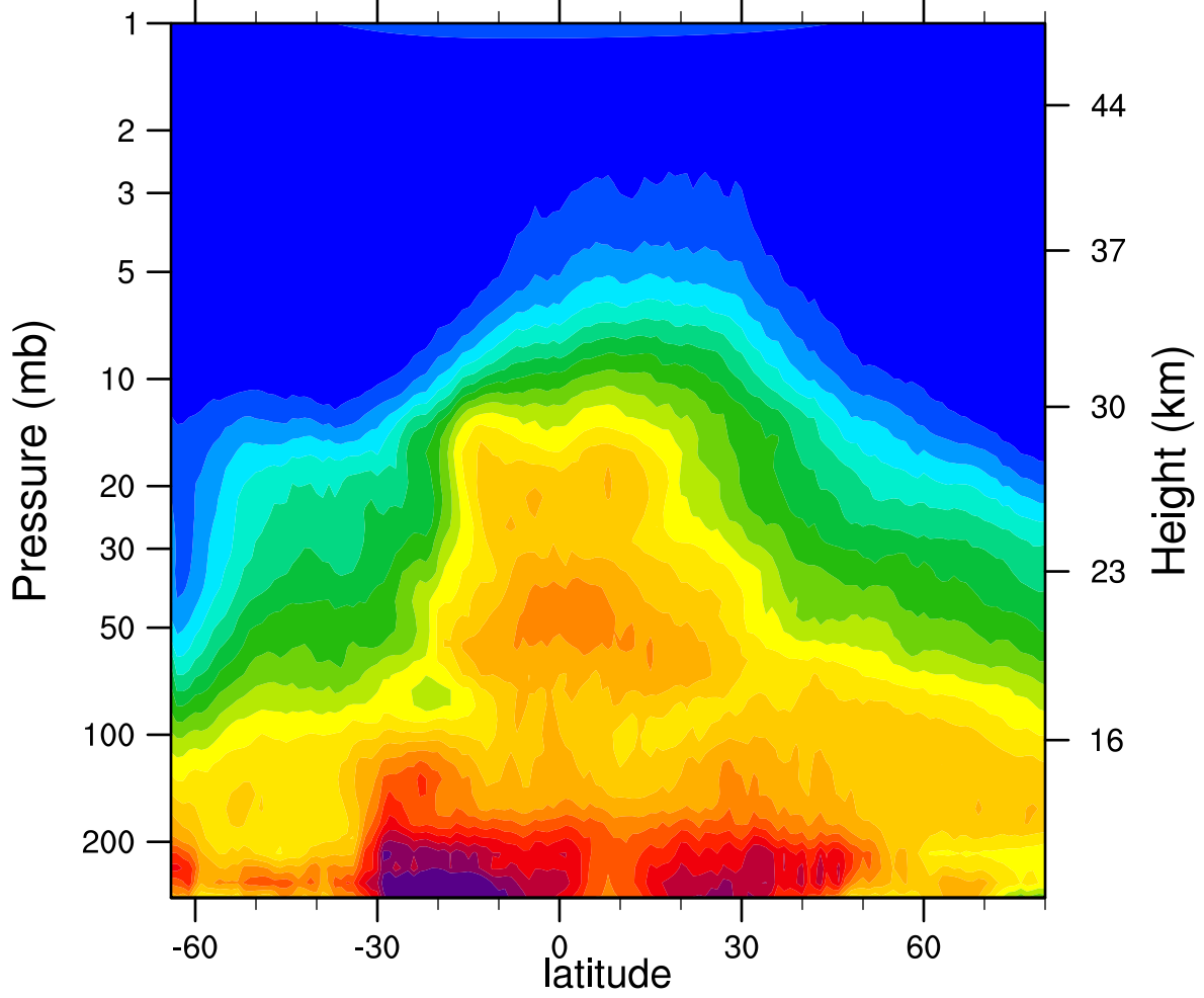
HIRDLSv6 2007d251 N2O_Combined (ppbv)
