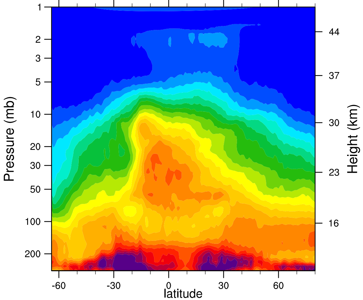
HIRDLSv6 2005d280 N2O_Combined (ppbv)
