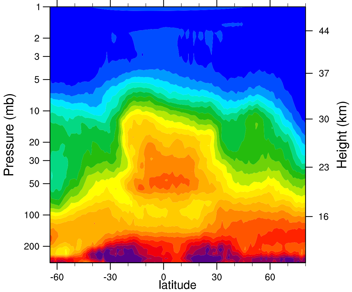
HIRDLSv6 2005d321 N2O_Combined (ppbv)
