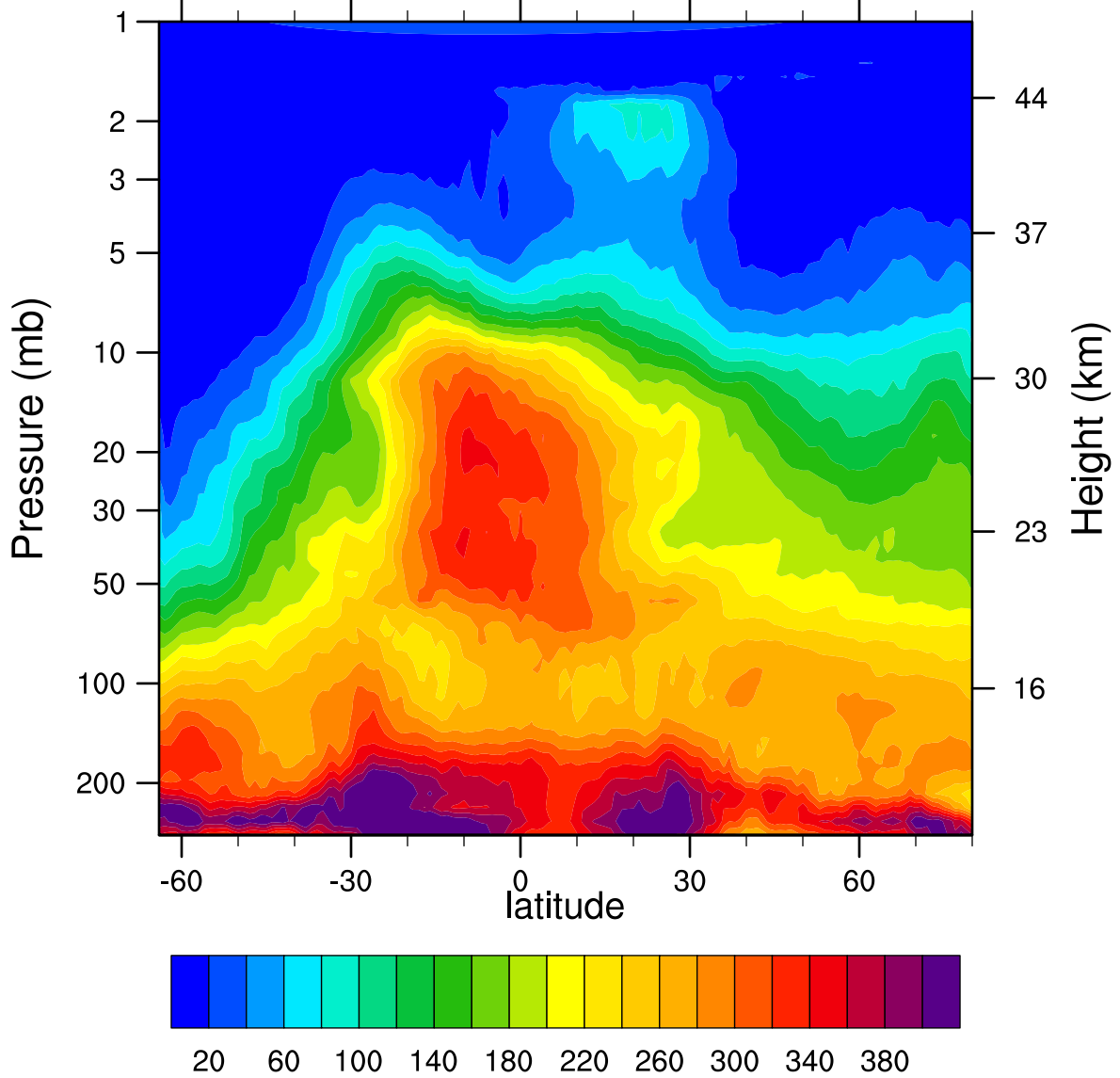
HIRDLSv6 2005d161 N2O_Combined (ppbv)
