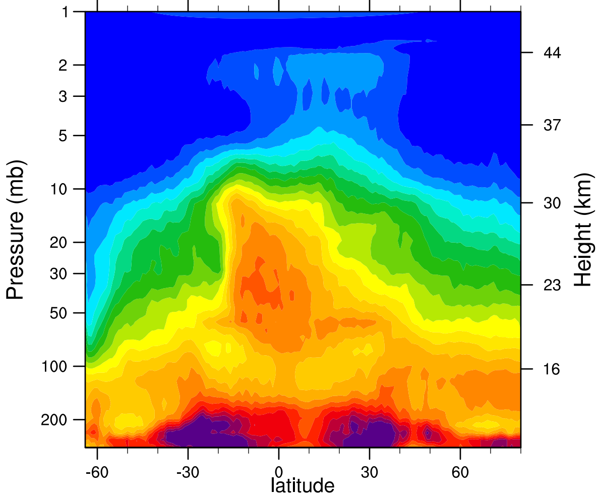
HIRDLSv6 2005d264 N2O_Combined (ppbv)
