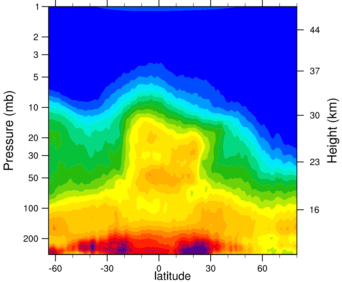
HIRDLSv6 2007d348 N2O_Combined (ppbv)
