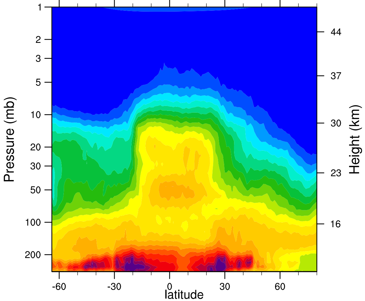
HIRDLSv6 2007d309 N2O_Combined (ppbv)
