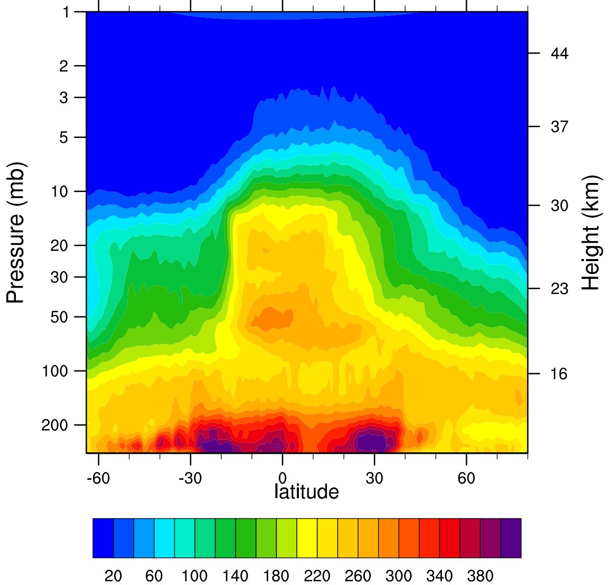
HIRDLSv6 2007d278 N2O_Combined (ppbv)
