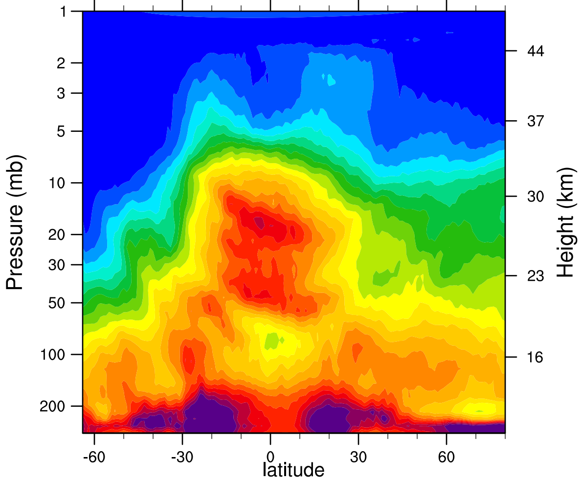
HIRDLSv6 2005d113 N2O_Combined (ppbv)
