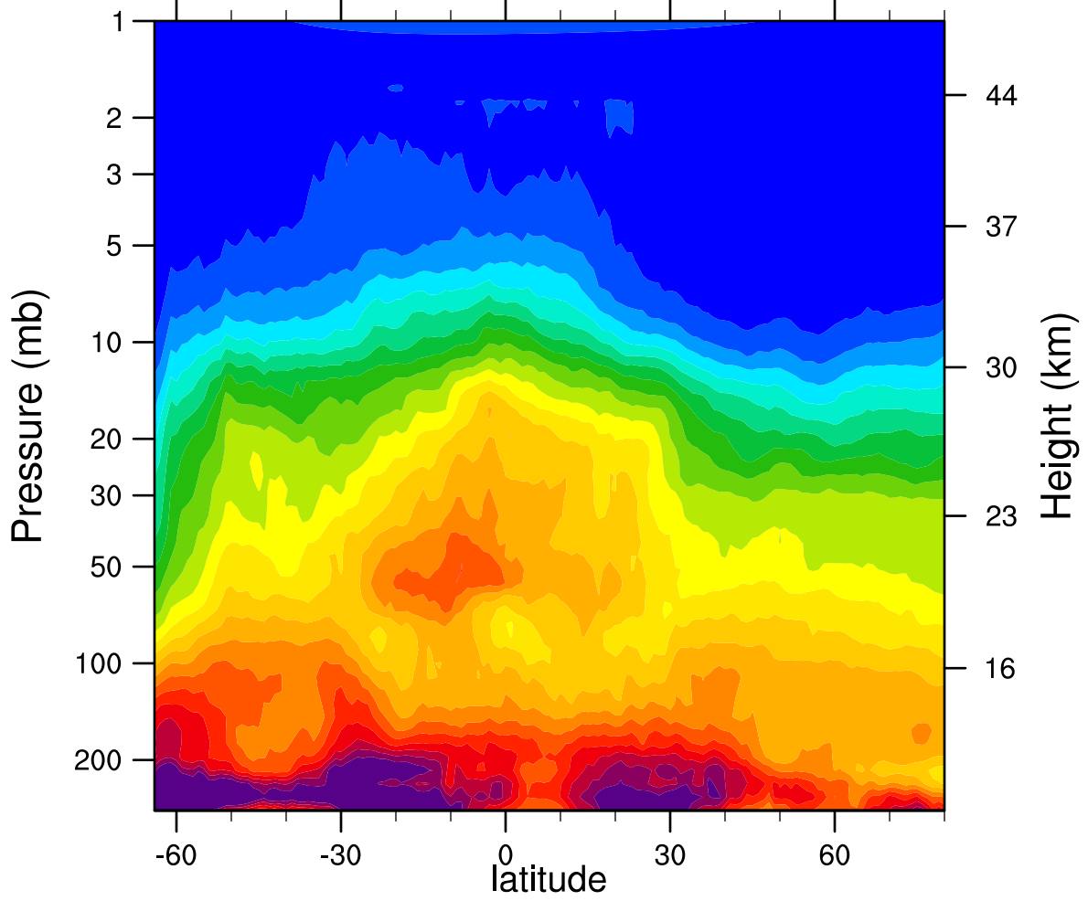
HIRDLSv6 2006d163 N2O_Combined (ppbv)
