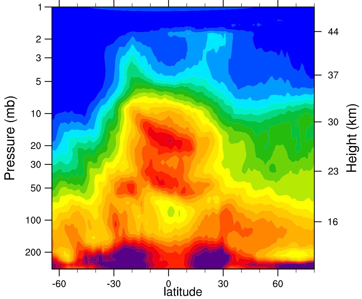
HIRDLSv6 2005d106 N2O_Combined (ppbv)
