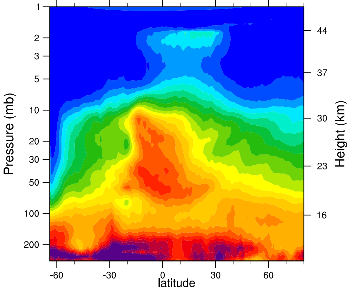
HIRDLSv6 2005d219 N2O_Combined (ppbv)
