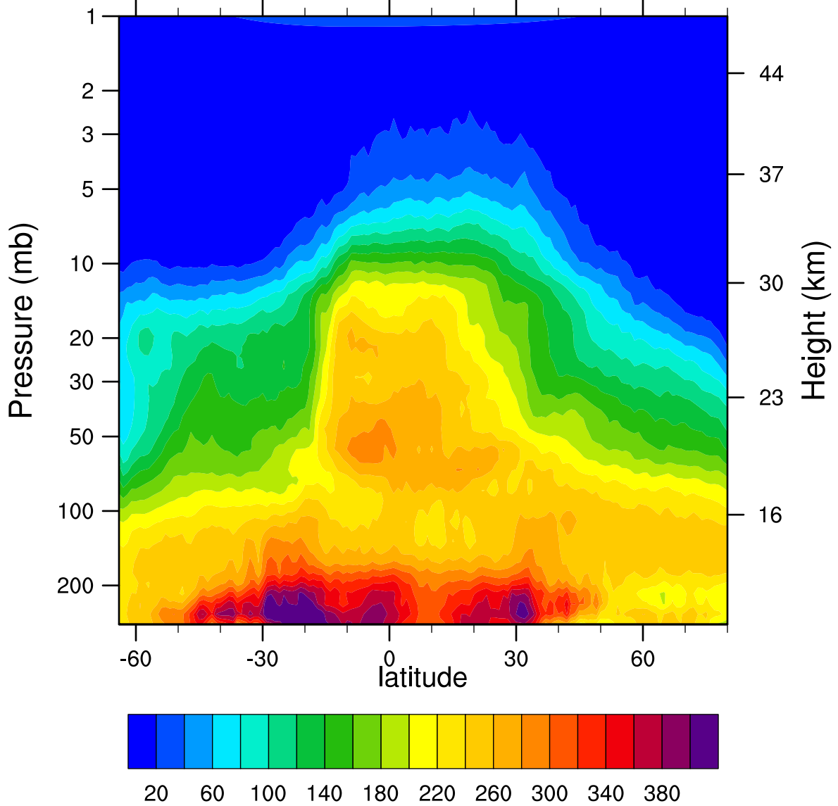
HIRDLSv6 2007d273 N2O_Combined (ppbv)
