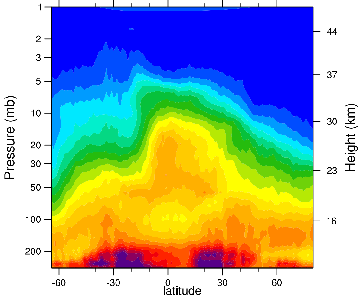
HIRDLSv6 2006d298 N2O_Combined (ppbv)
