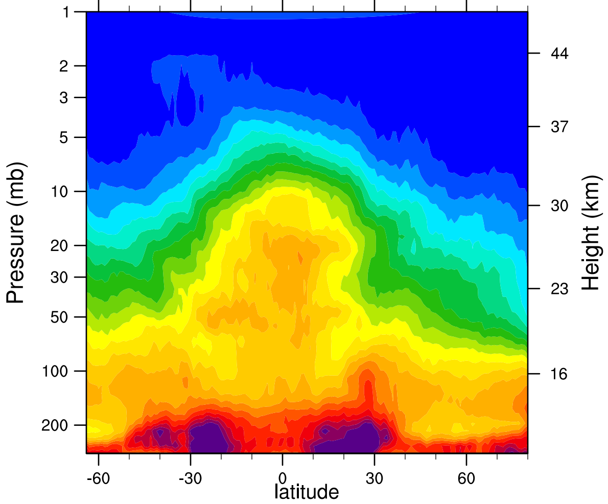
HIRDLSv6 2007d060 N2O_Combined (ppbv)
