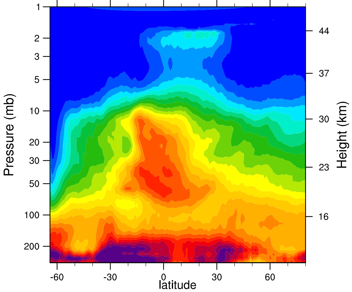
HIRDLSv6 2005d217 N2O_Combined (ppbv)
