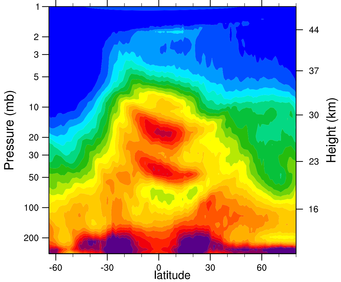
HIRDLSv6 2005d077 N2O_Combined (ppbv)
