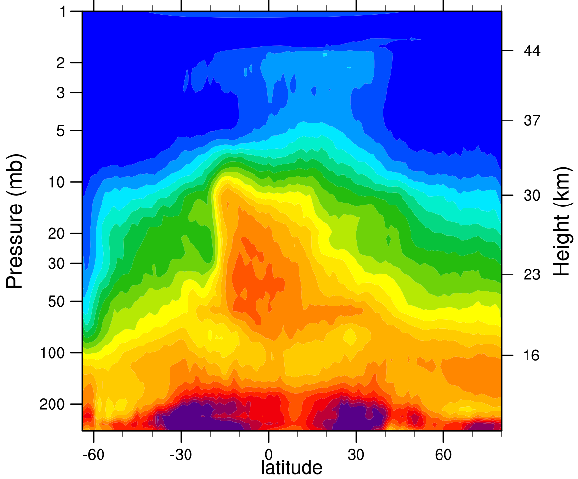
HIRDLSv6 2005d261 N2O_Combined (ppbv)
