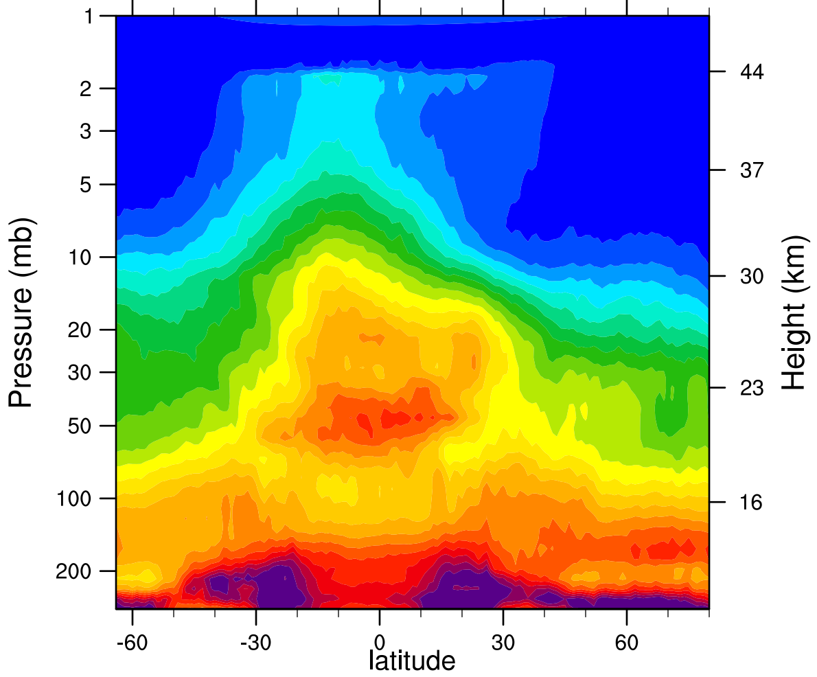
HIRDLSv6 2006d051 N2O_Combined (ppbv)
