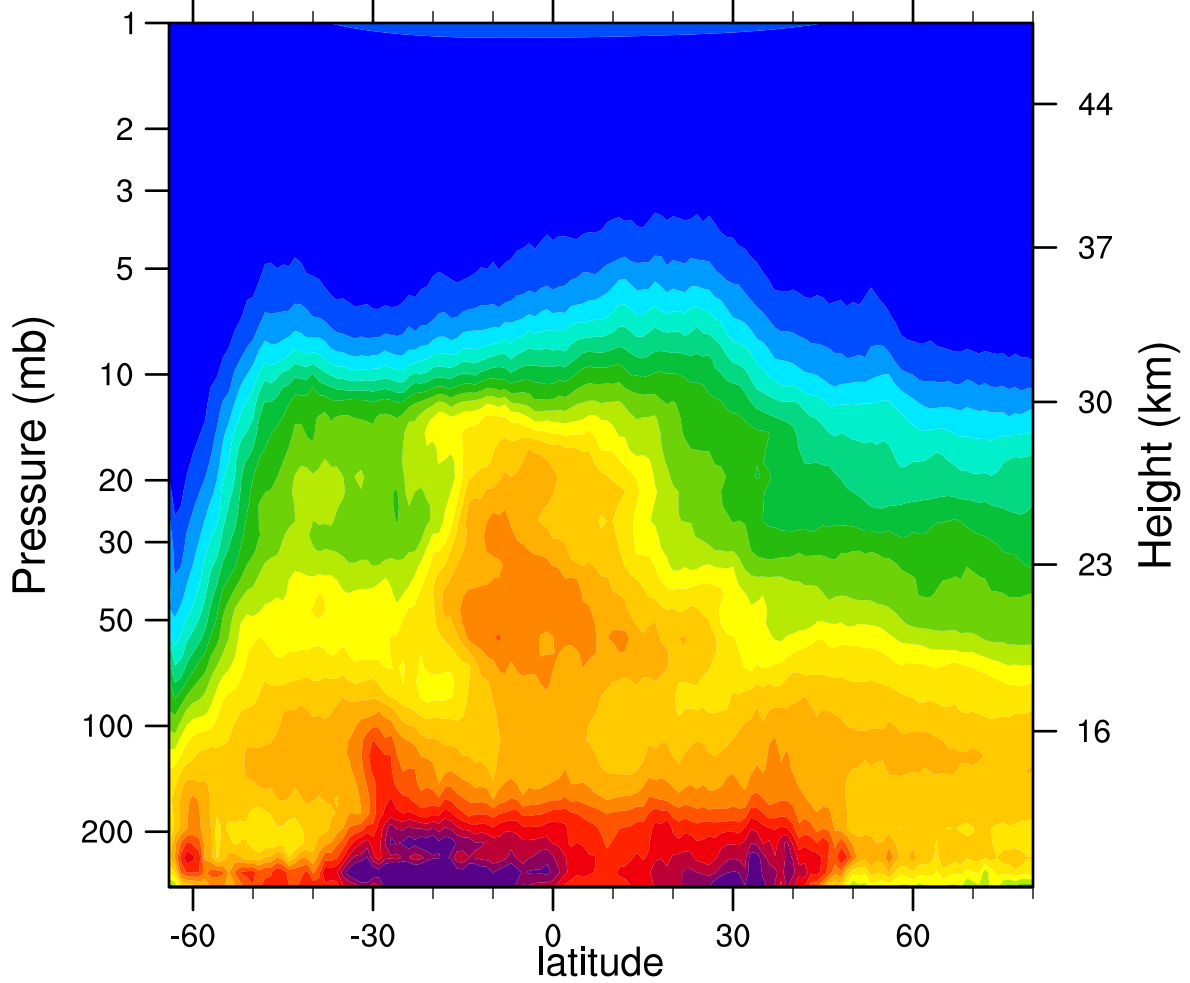
HIRDLSv6 2007d203 N2O_Combined (ppbv)
