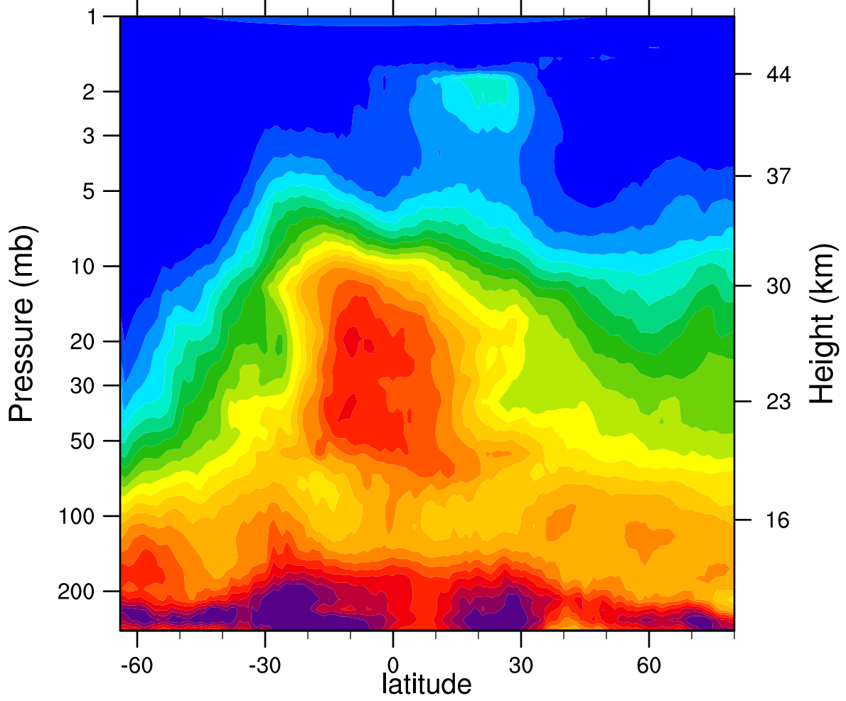
HIRDLSv6 2005d163 N2O_Combined (ppbv)
