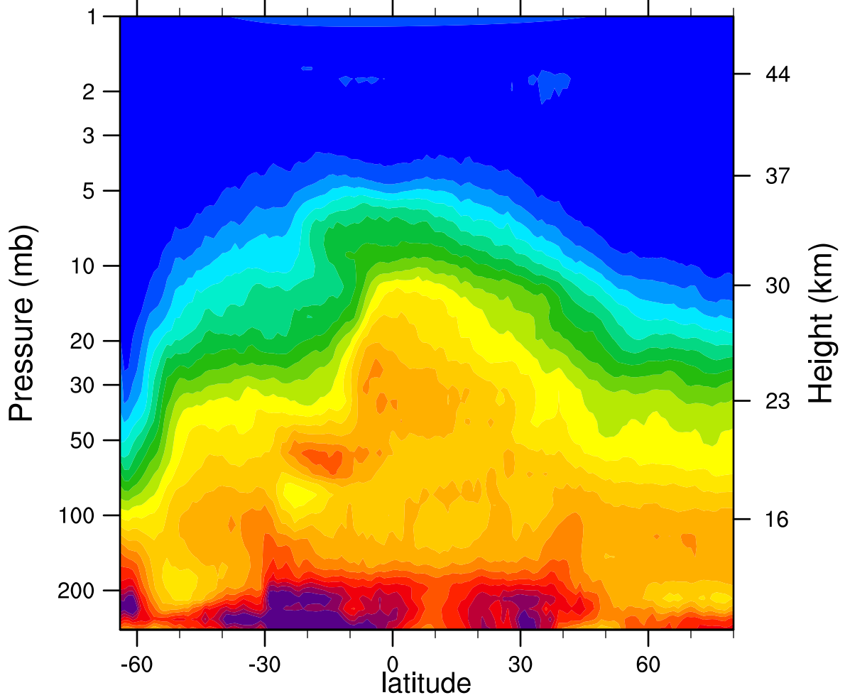
HIRDLSv6 2006d258 N2O_Combined (ppbv)
