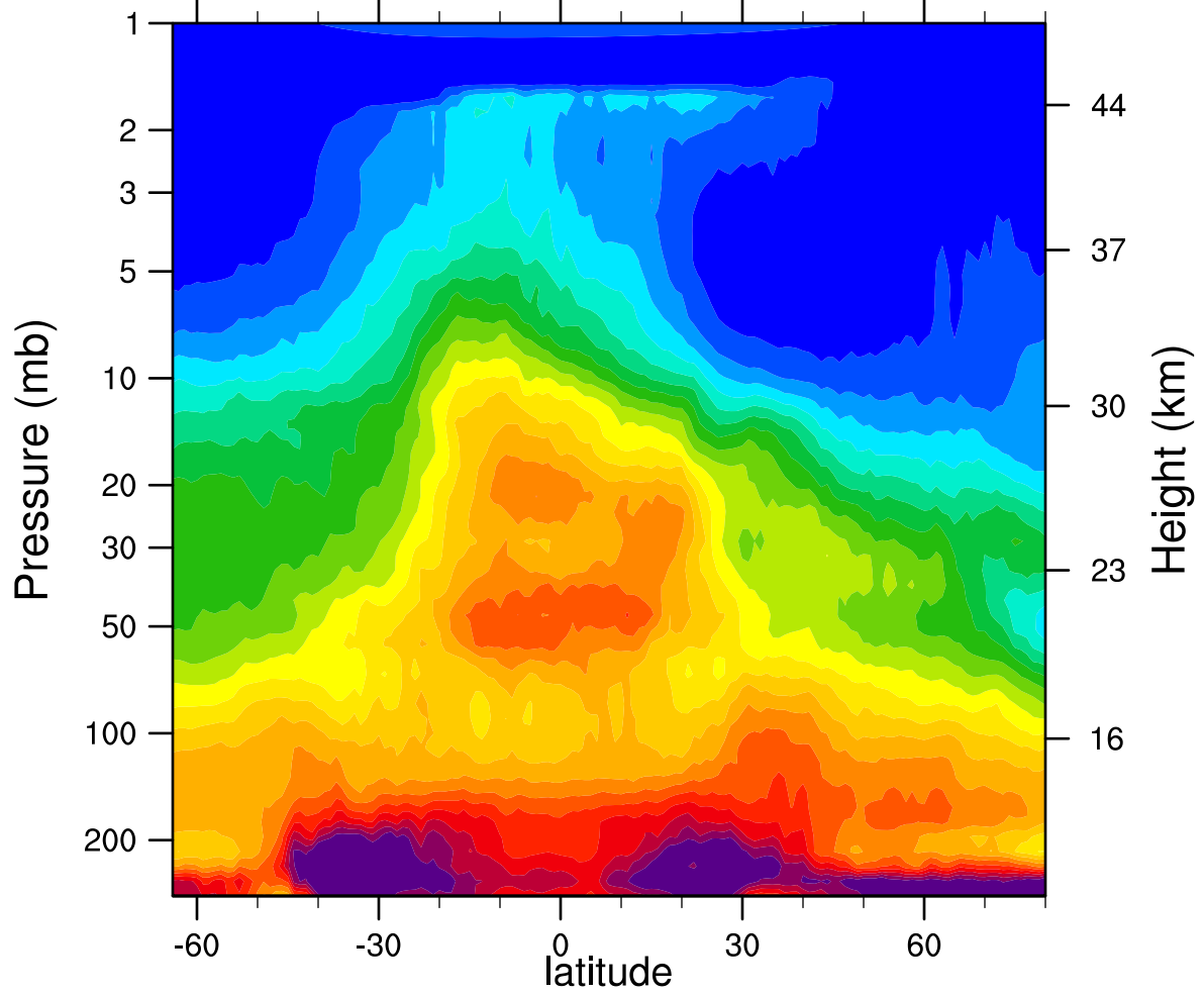
HIRDLSv6 2006d025 N2O_Combined (ppbv)
