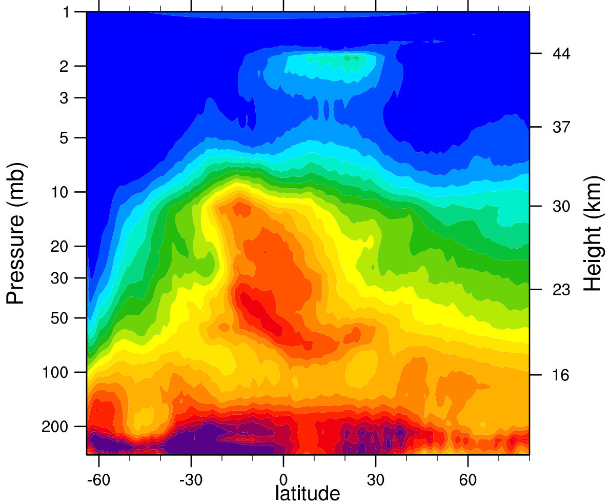
HIRDLSv6 2005d205 N2O_Combined (ppbv)
