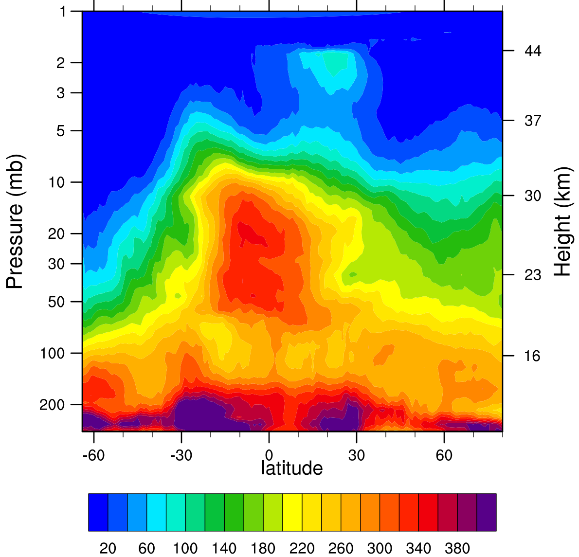
HIRDLSv6 2005d158 N2O_Combined (ppbv)
