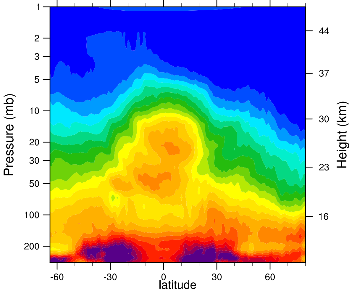
HIRDLSv6 2007d029 N2O_Combined (ppbv)
