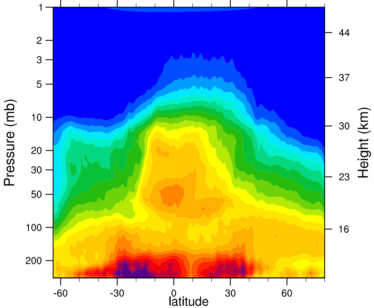
HIRDLSv6 2007d267 N2O_Combined (ppbv)
