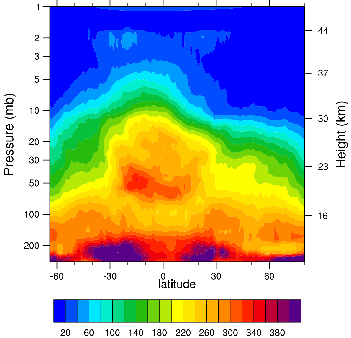
HIRDLSv6 2006d111 N2O_Combined (ppbv)
