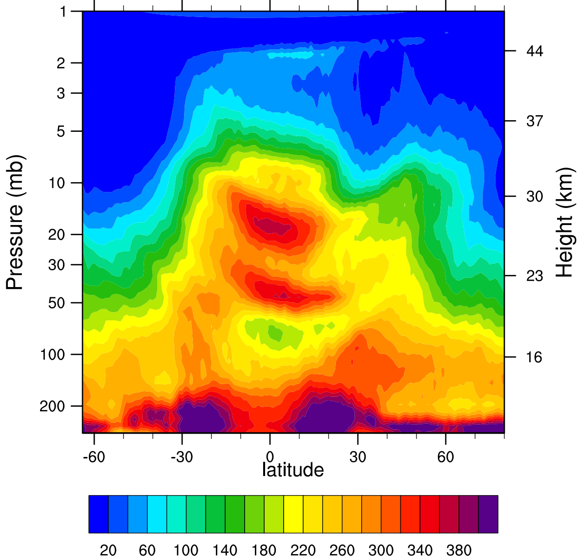
HIRDLSv6 2005d068 N2O_Combined (ppbv)
