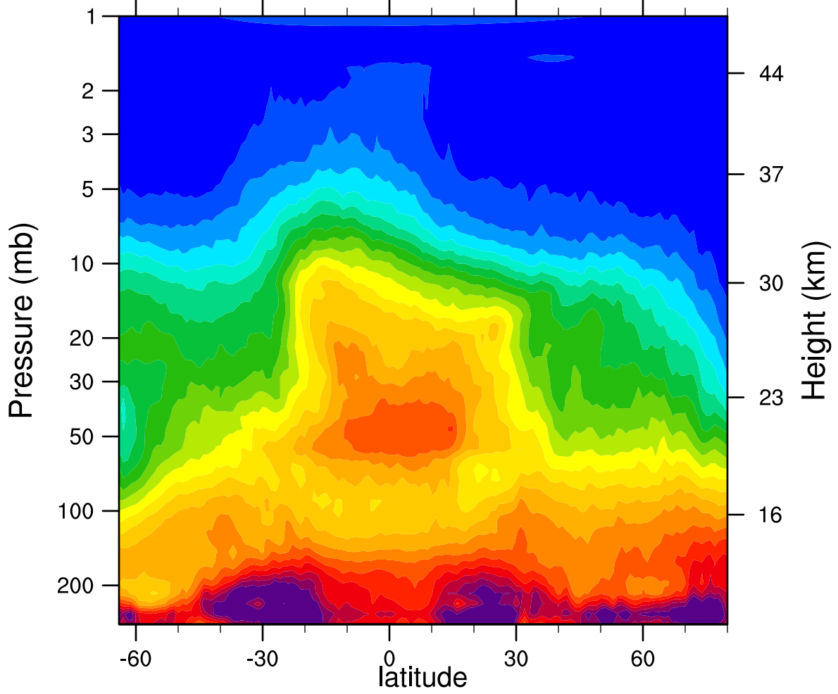
HIRDLSv6 2005d340 N2O_Combined (ppbv)
