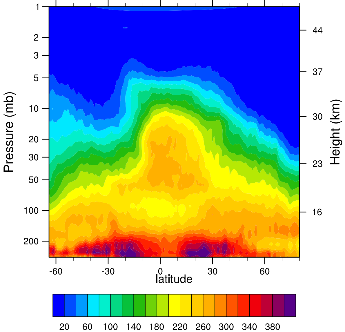
HIRDLSv6 2006d313 N2O_Combined (ppbv)
