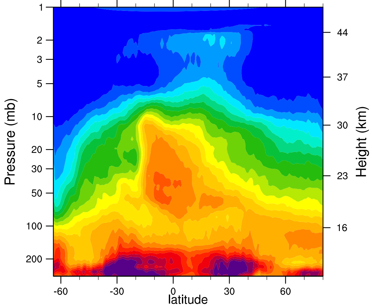
HIRDLSv6 2005d256 N2O_Combined (ppbv)
