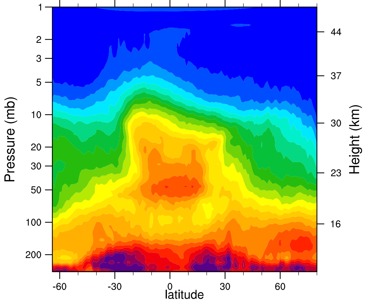
HIRDLSv6 2005d334 N2O_Combined (ppbv)
