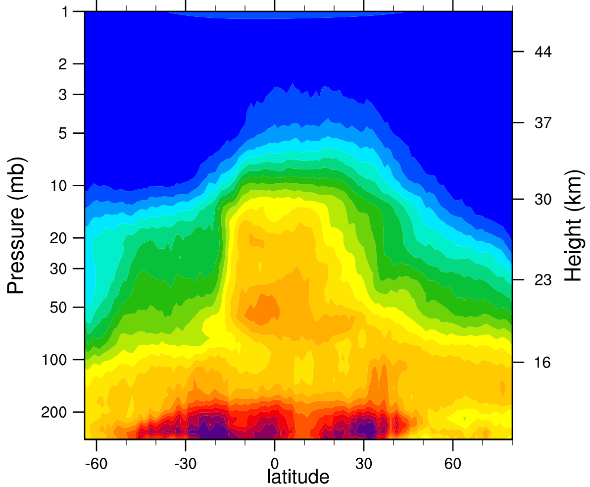
HIRDLSv6 2007d275 N2O_Combined (ppbv)
