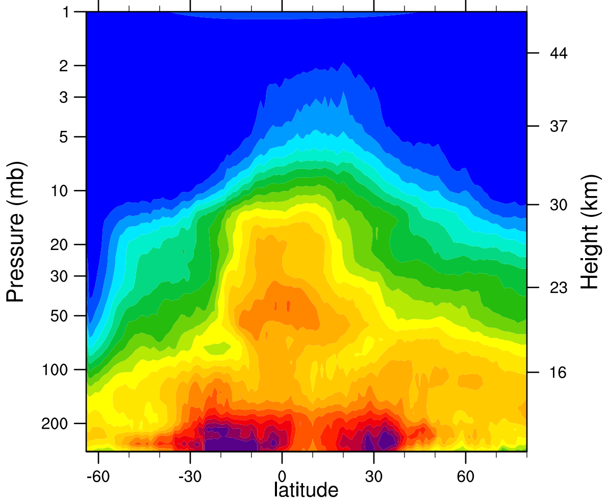
HIRDLSv6 2007d228 N2O_Combined (ppbv)
