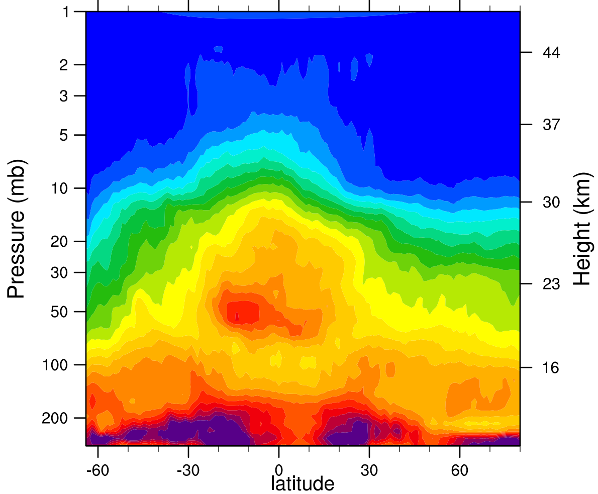
HIRDLSv6 2006d135 N2O_Combined (ppbv)
