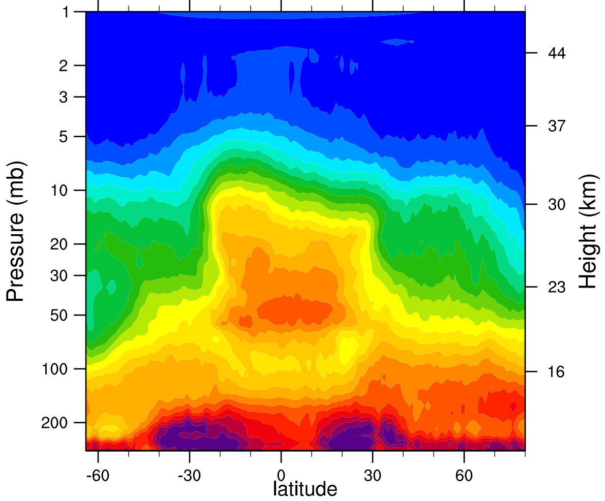
HIRDLSv6 2005d328 N2O_Combined (ppbv)
