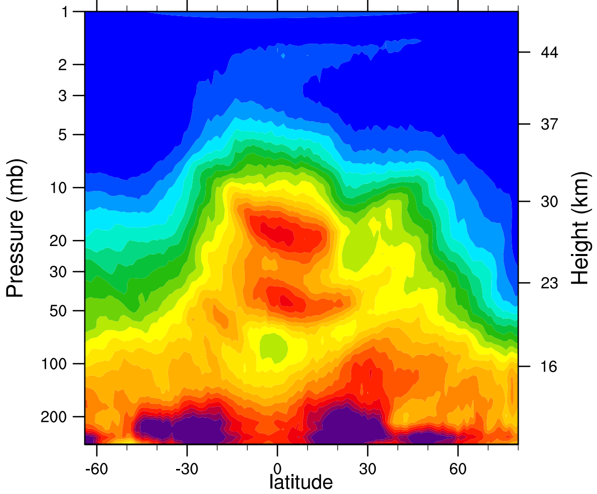
HIRDLSv6 2005d036 N2O_Combined (ppbv)
