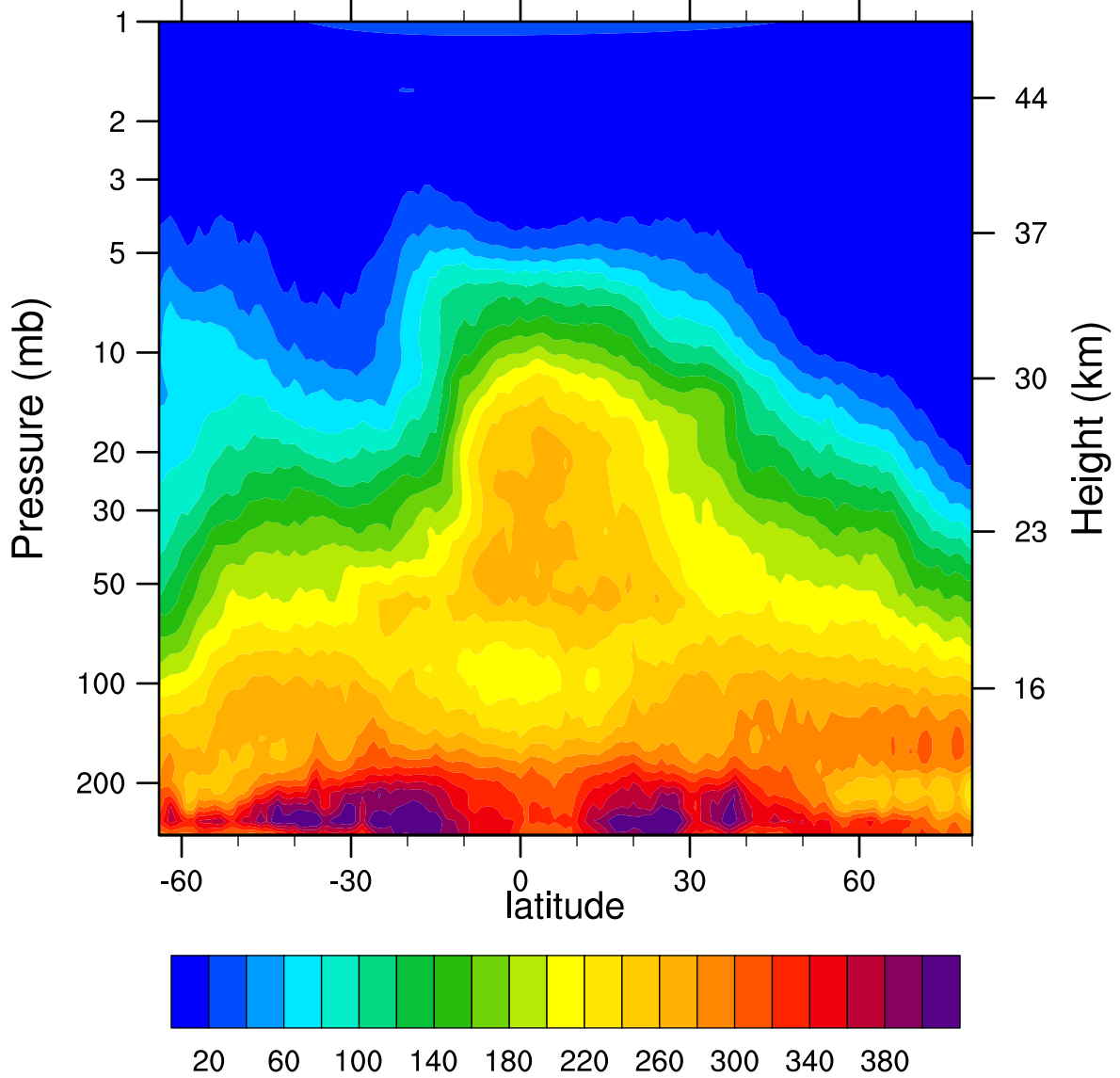
HIRDLSv6 2006d311 N2O_Combined (ppbv)
