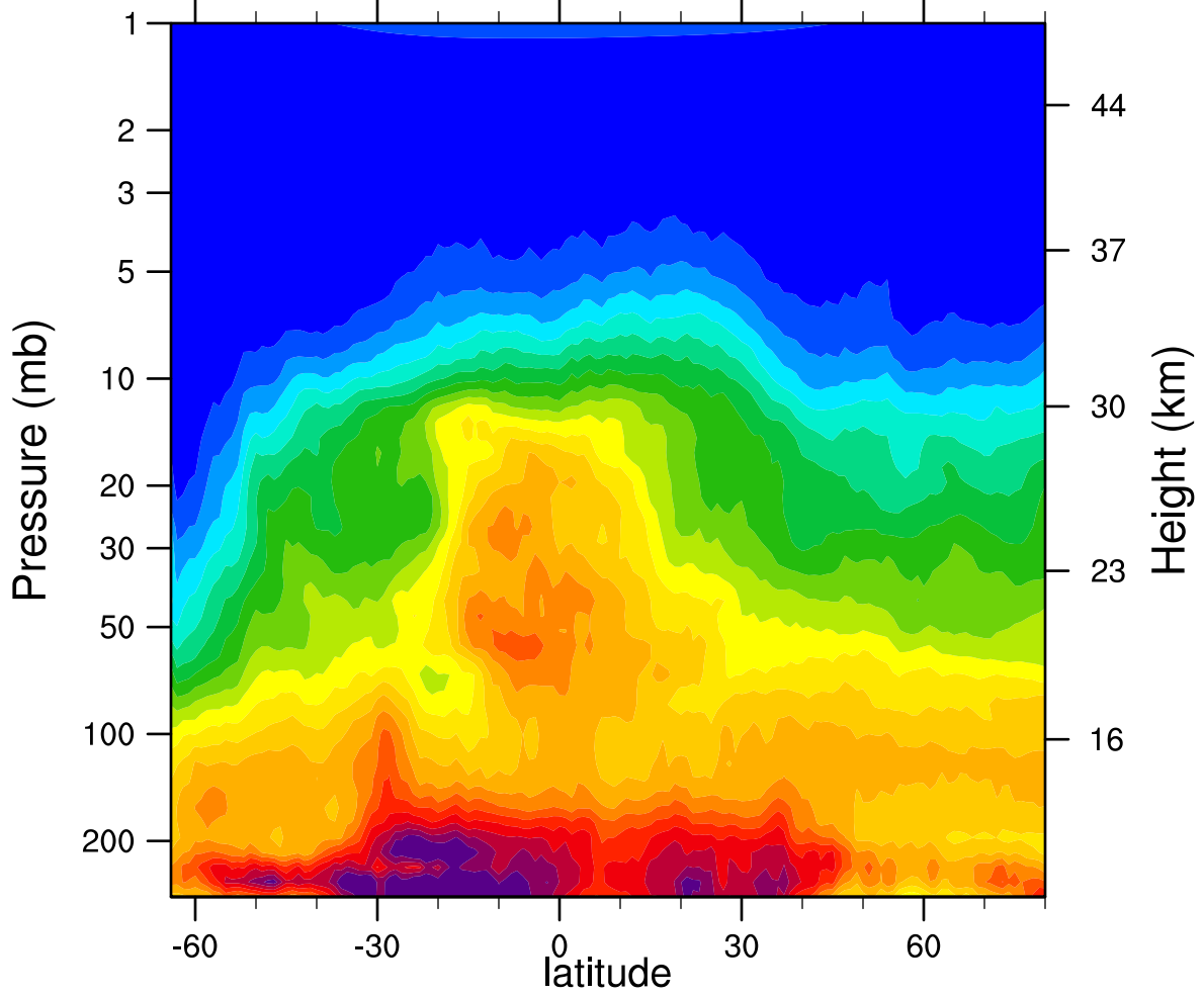
HIRDLSv6 2007d189 N2O_Combined (ppbv)
