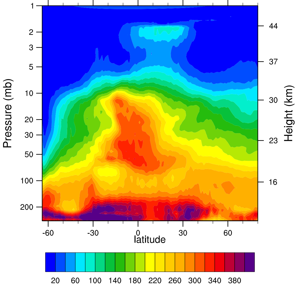
HIRDLSv6 2005d213 N2O_Combined (ppbv)
