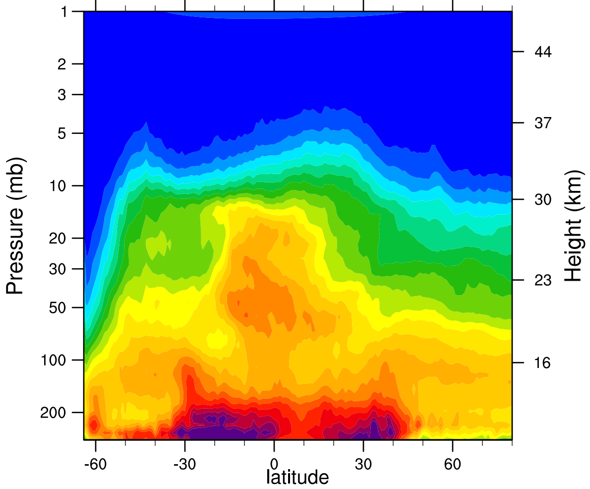
HIRDLSv6 2007d204 N2O_Combined (ppbv)
