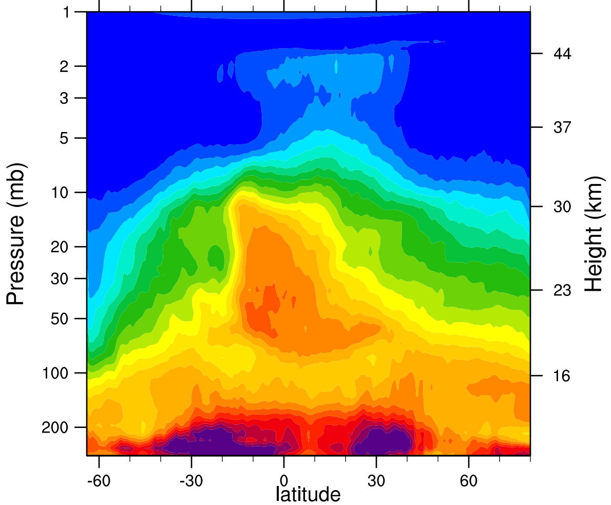
HIRDLSv6 2005d248 N2O_Combined (ppbv)
