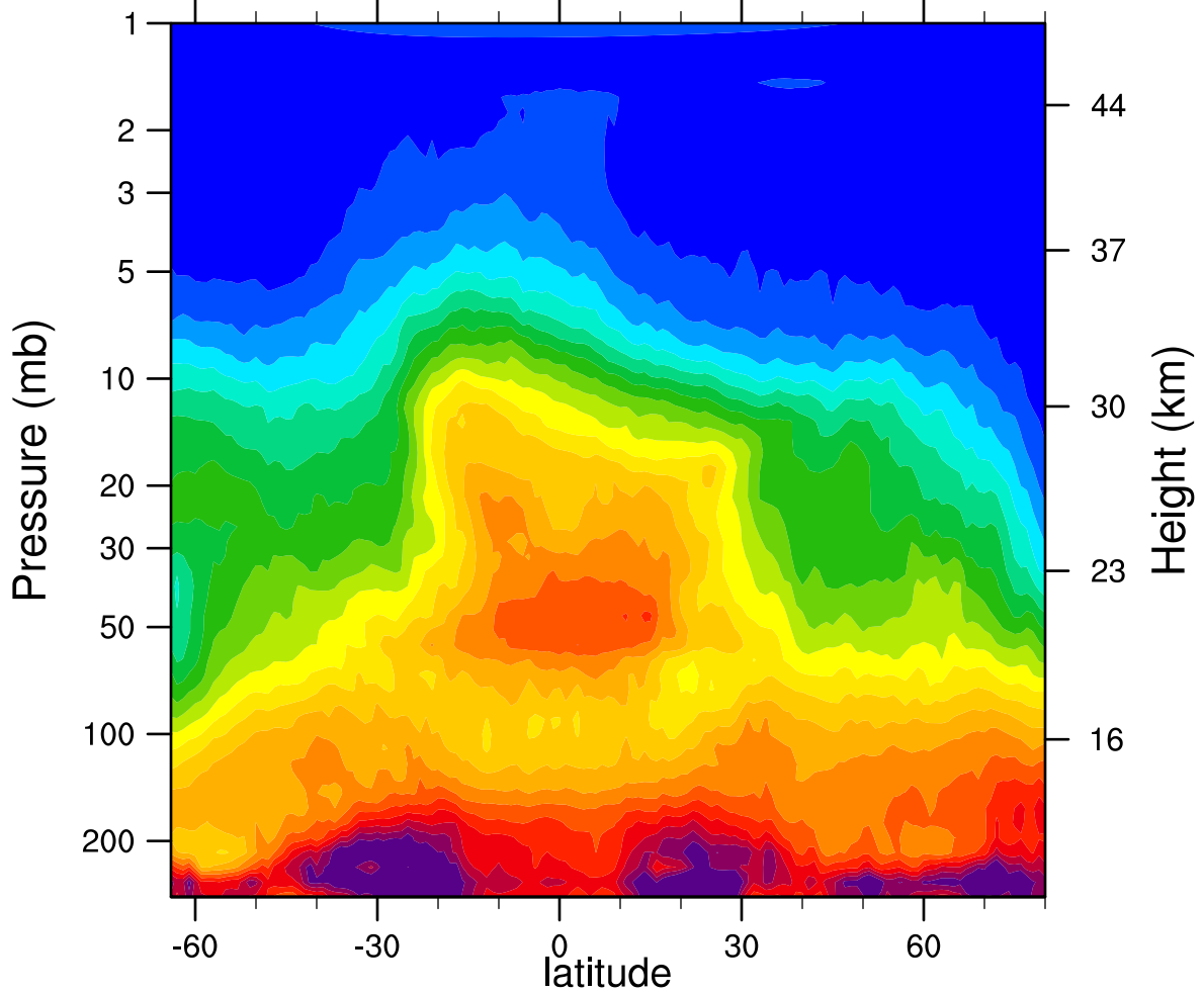
HIRDLSv6 2005d339 N2O_Combined (ppbv)
