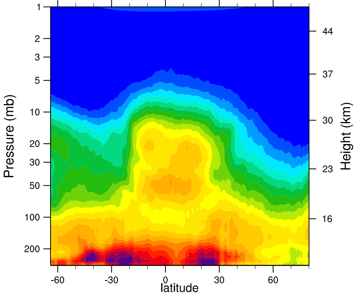
HIRDLSv6 2007d323 N2O_Combined (ppbv)
