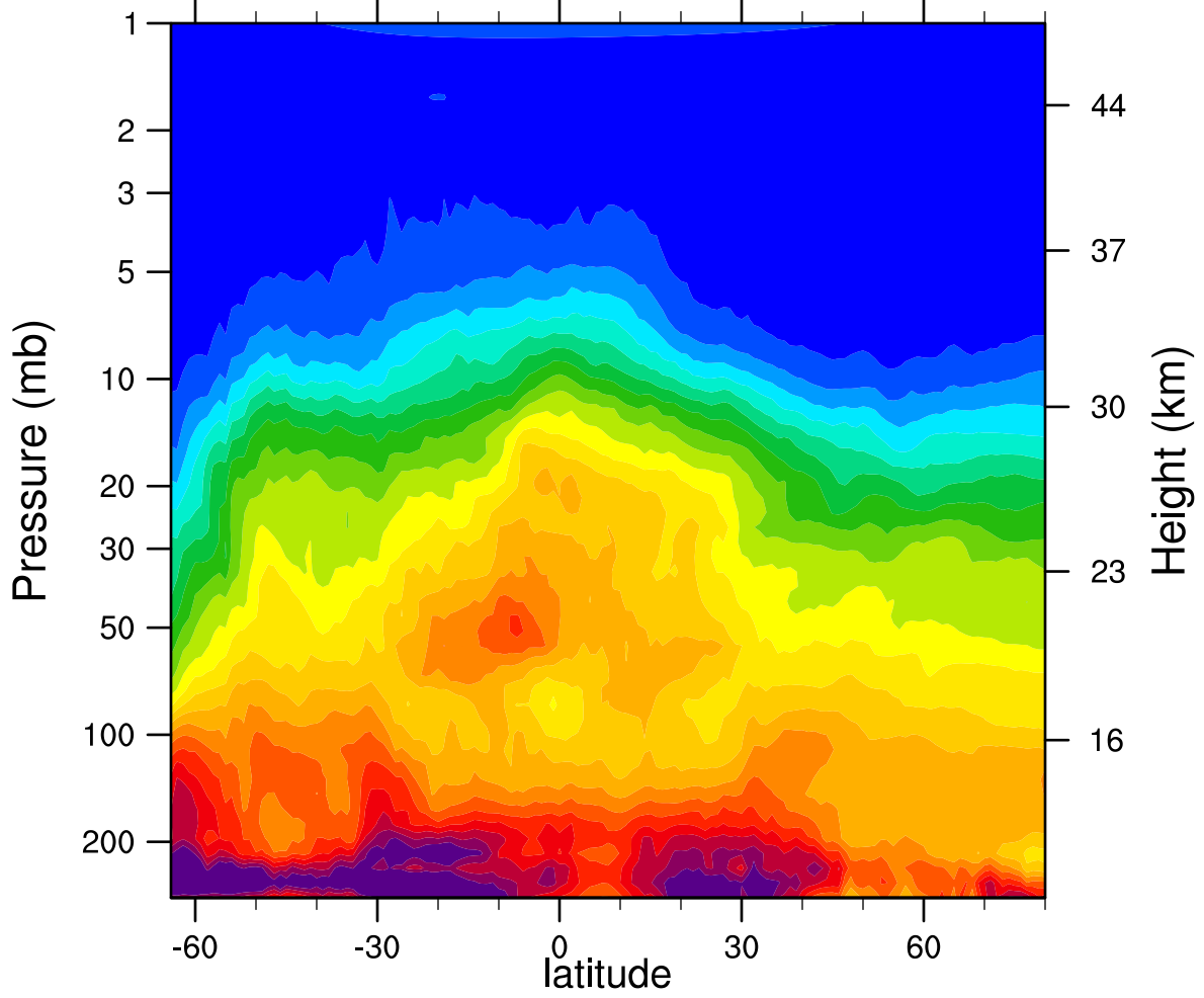
HIRDLSv6 2006d169 N2O_Combined (ppbv)
