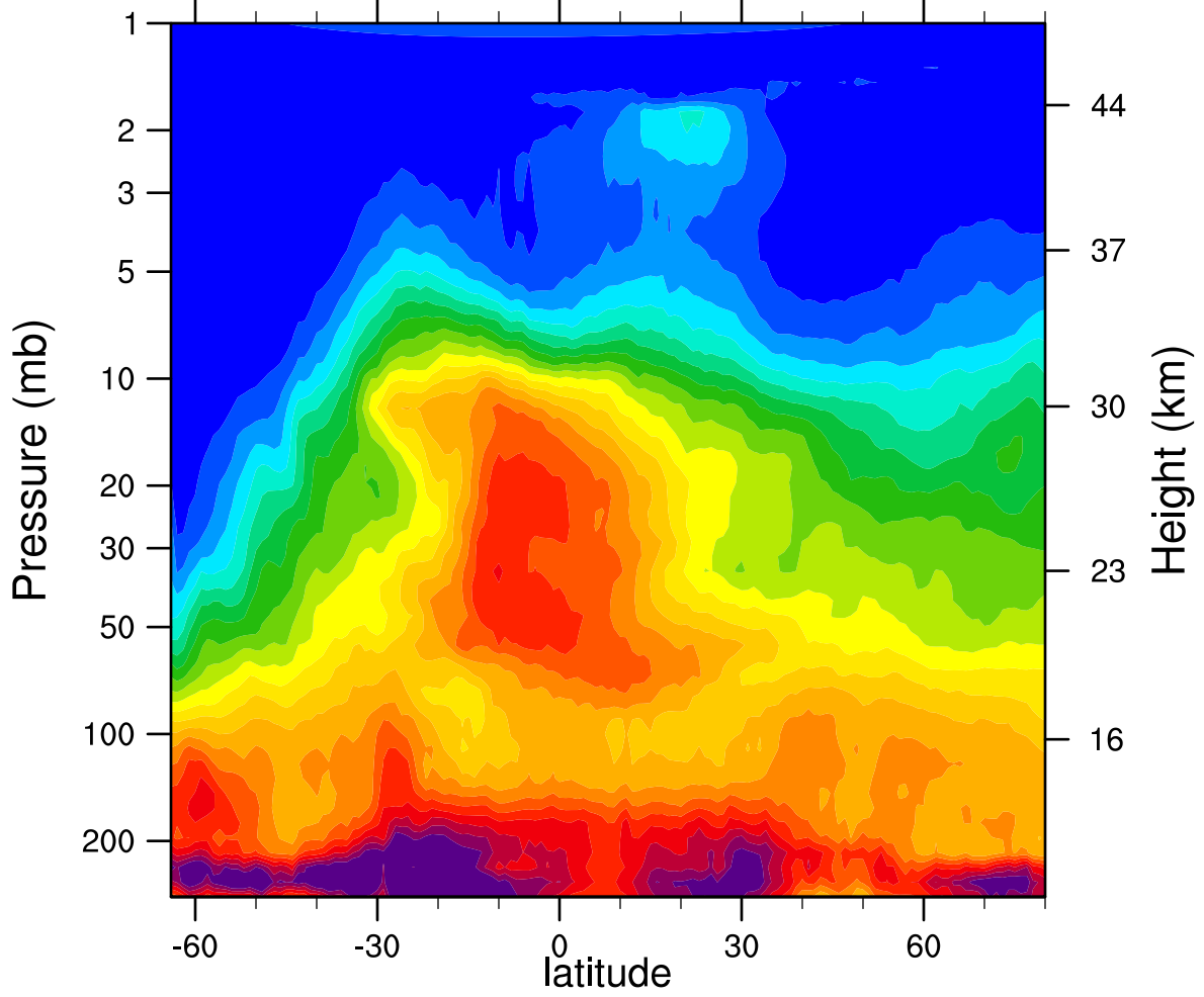
HIRDLSv6 2005d173 N2O_Combined (ppbv)
