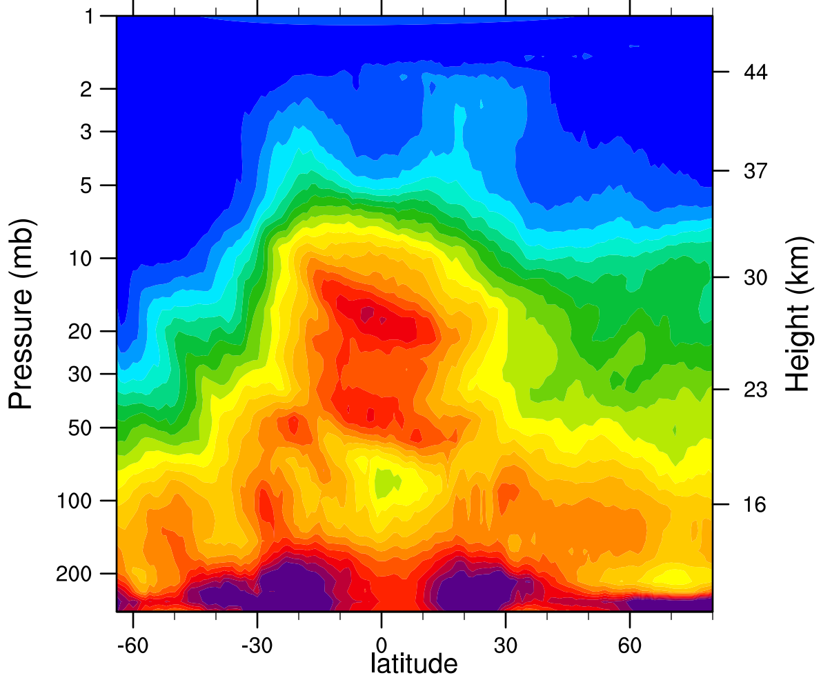
HIRDLSv6 2005d110 N2O_Combined (ppbv)
