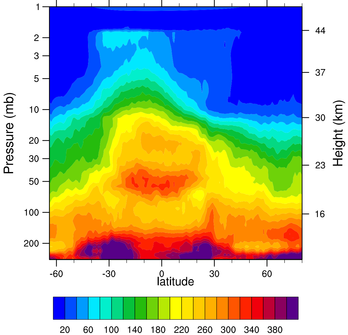
HIRDLSv6 2006d082 N2O_Combined (ppbv)
