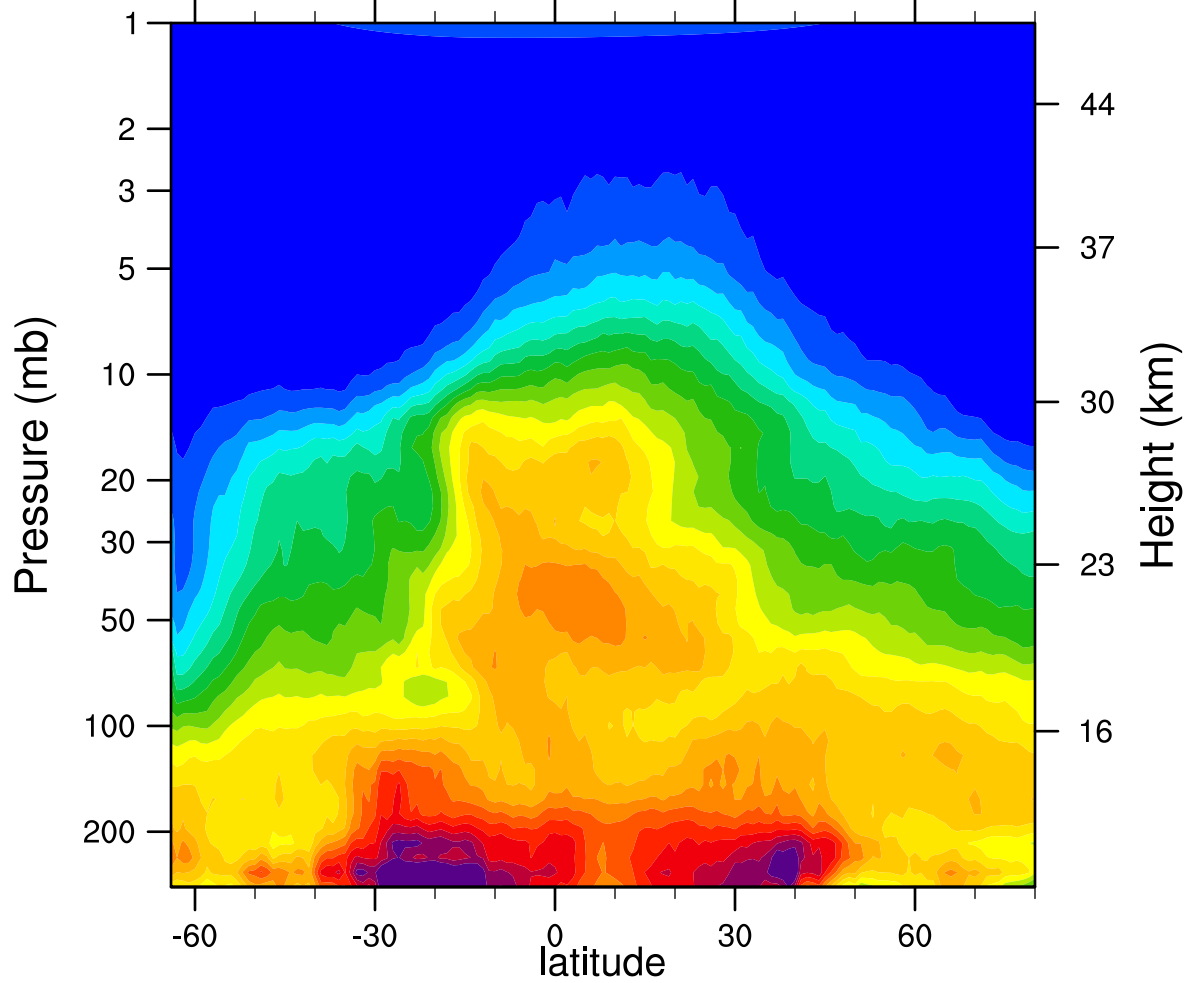
HIRDLSv6 2007d244 N2O_Combined (ppbv)
