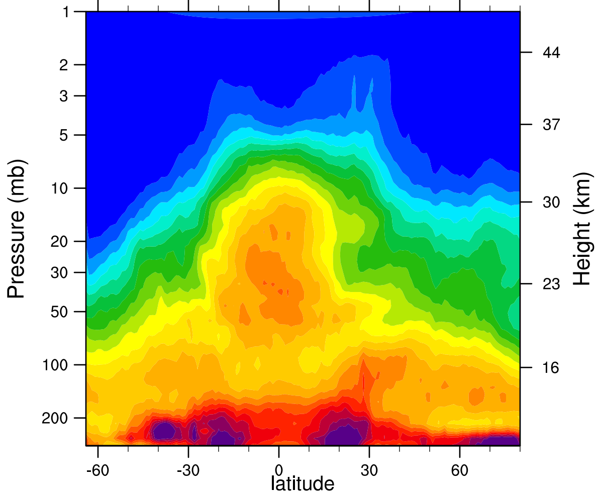
HIRDLSv6 2007d112 N2O_Combined (ppbv)
