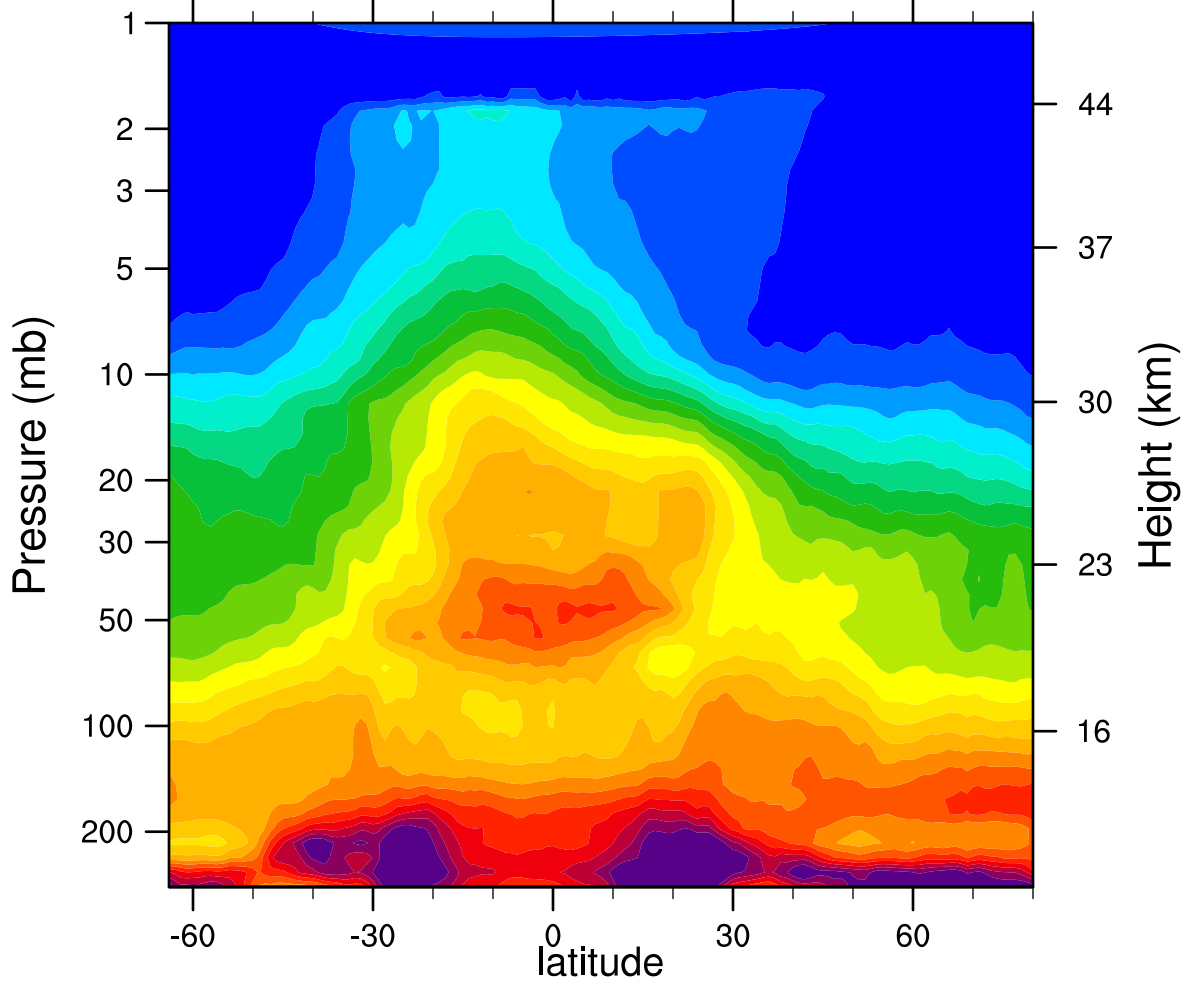
HIRDLSv6 2006d053 N2O_Combined (ppbv)
