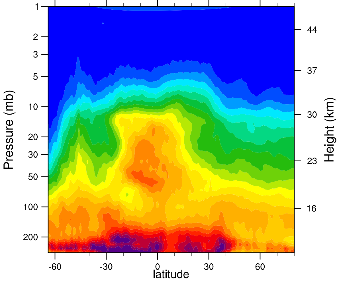
HIRDLSv6 2007d173 N2O_Combined (ppbv)
