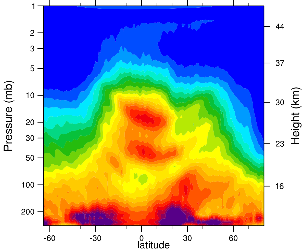
HIRDLSv6 2005d031 N2O_Combined (ppbv)
