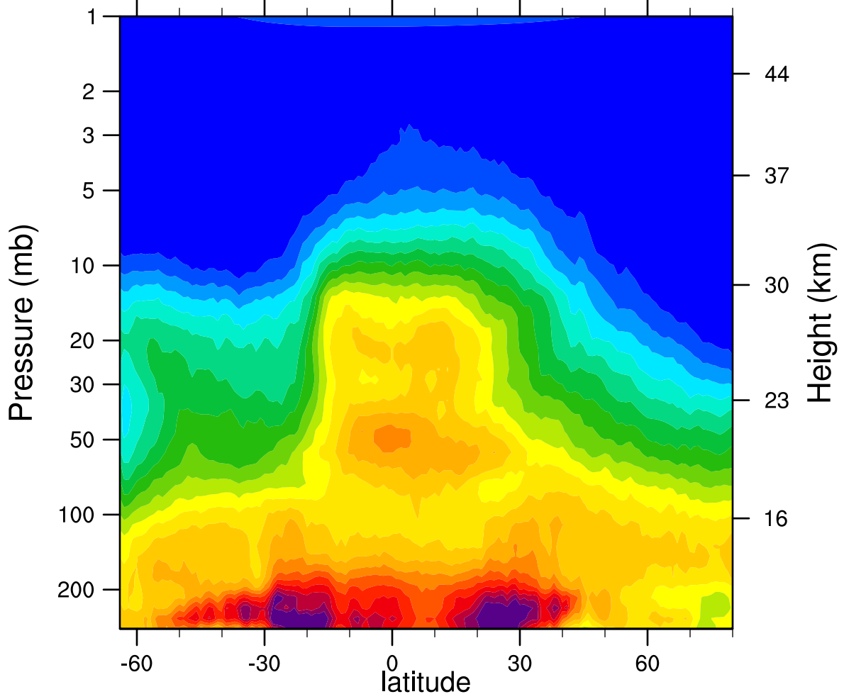
HIRDLSv6 2007d295 N2O_Combined (ppbv)
