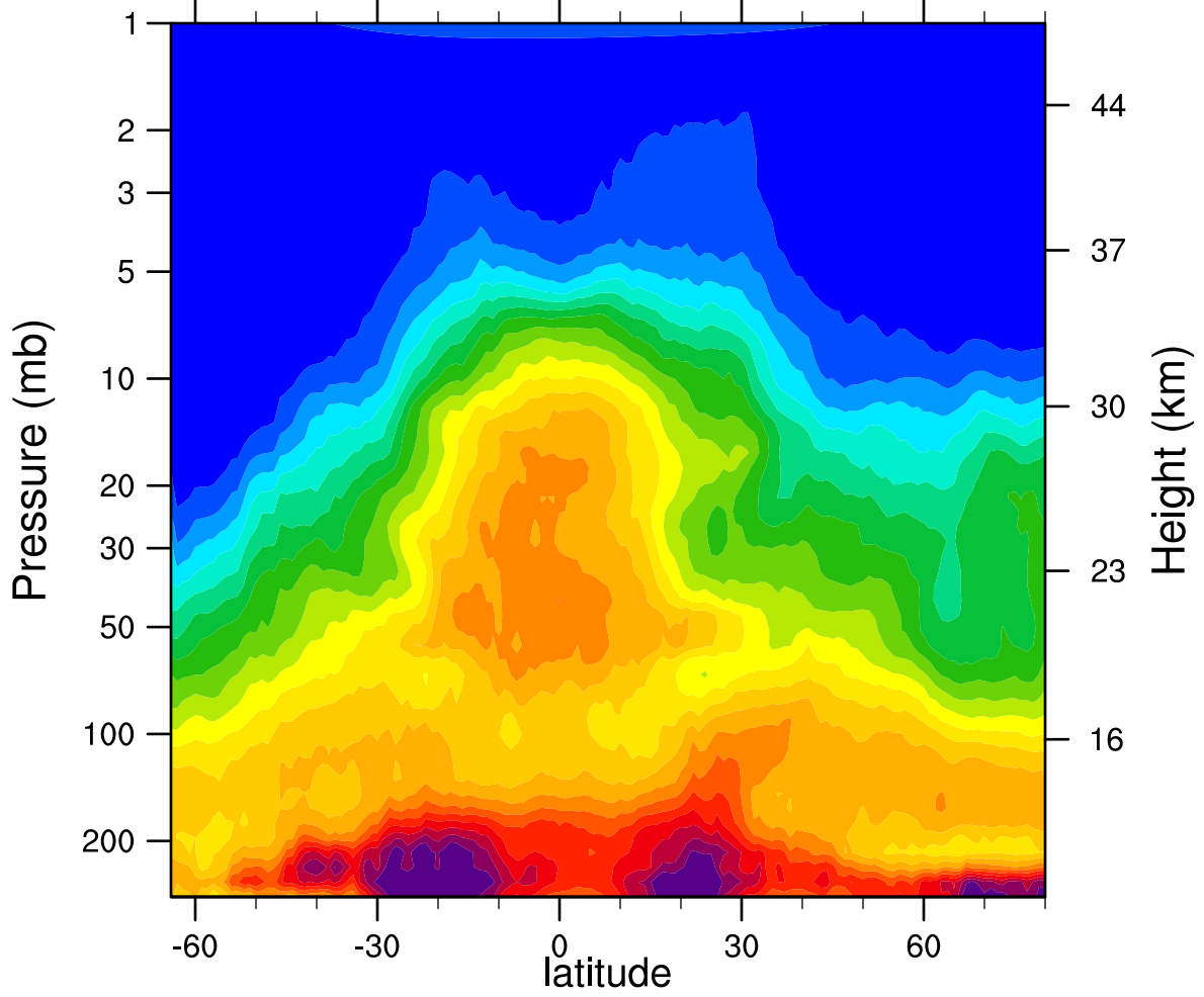
HIRDLSv6 2007d120 N2O_Combined (ppbv)
