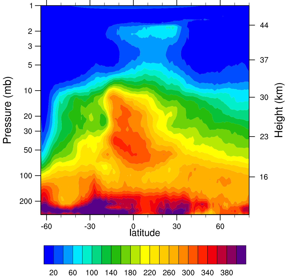
HIRDLSv6 2005d224 N2O_Combined (ppbv)
