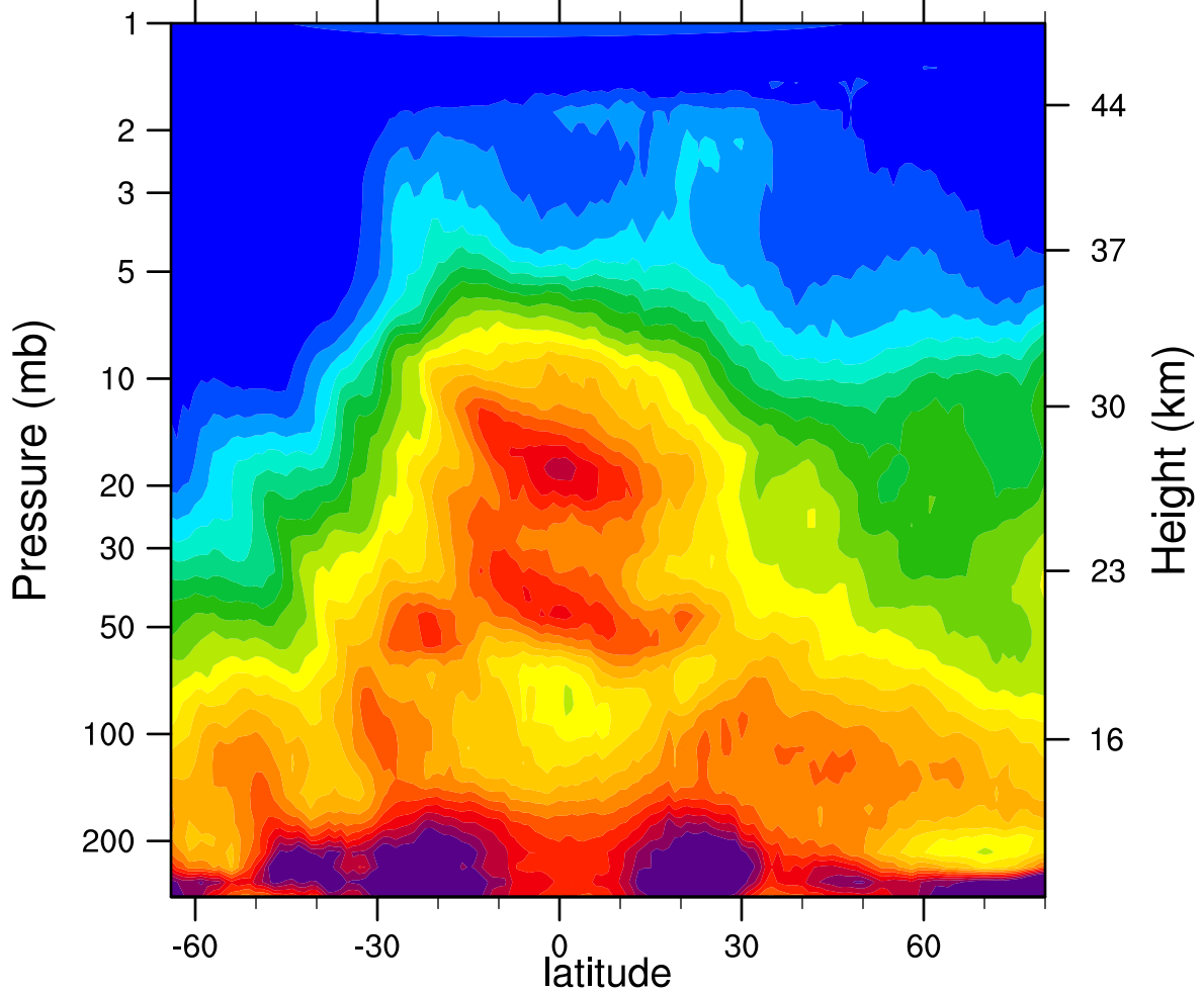
HIRDLSv6 2005d101 N2O_Combined (ppbv)
