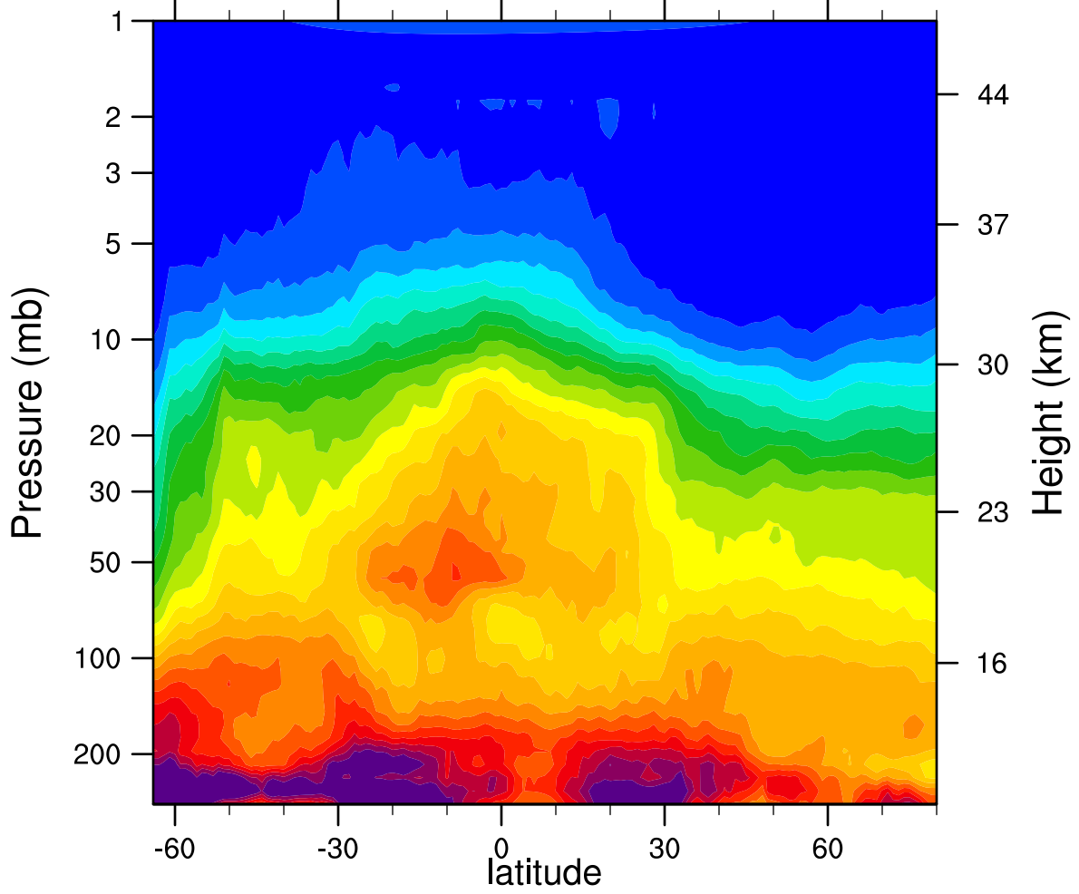
HIRDLSv6 2006d162 N2O_Combined (ppbv)
