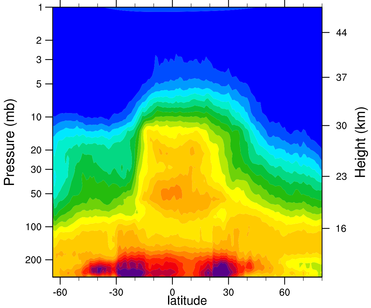
HIRDLSv6 2007d289 N2O_Combined (ppbv)
