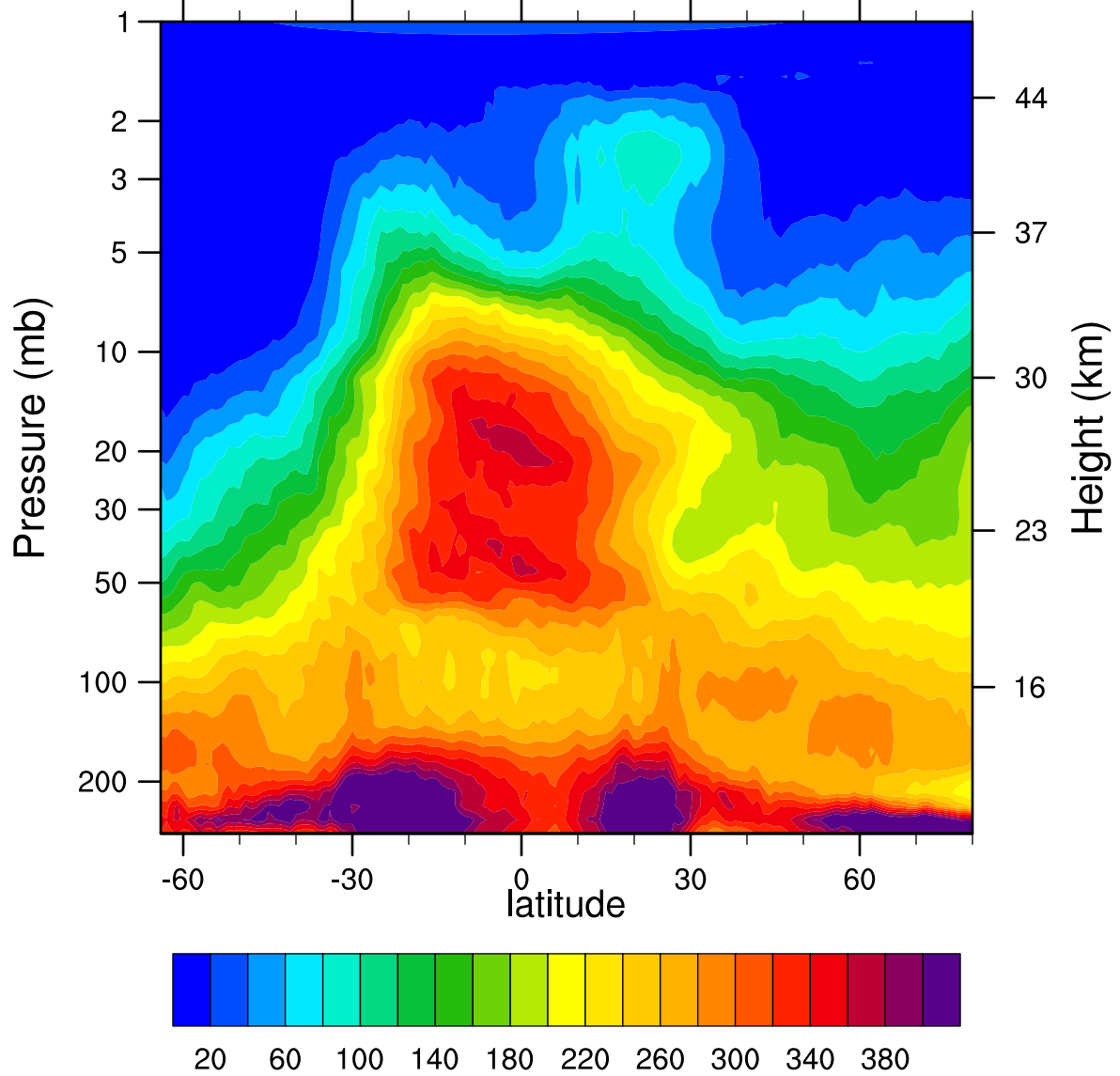
HIRDLSv6 2005d123 N2O_Combined (ppbv)
