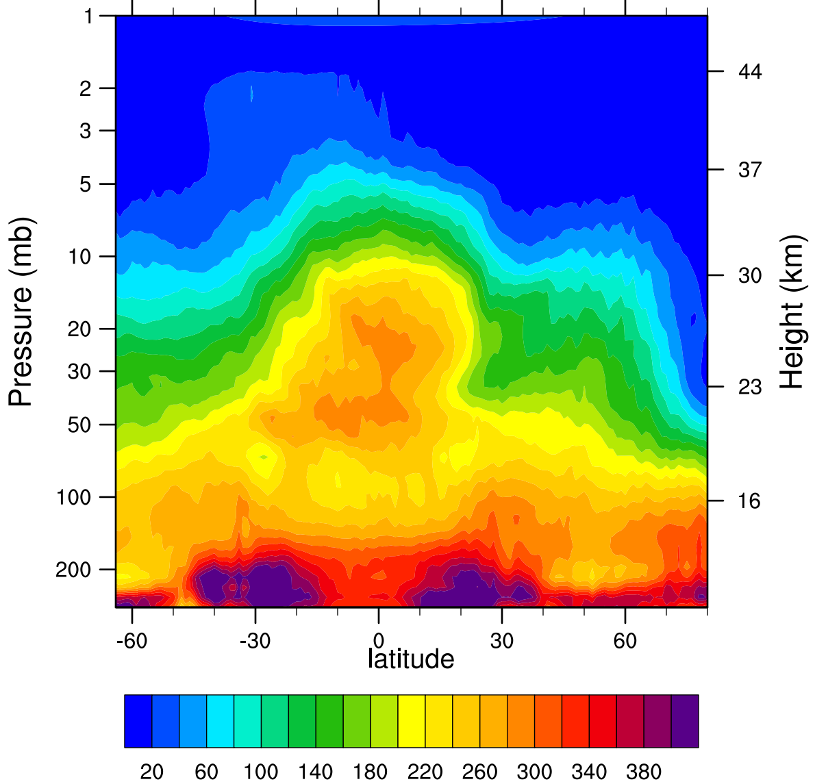
HIRDLSv6 2007d034 N2O_Combined (ppbv)
