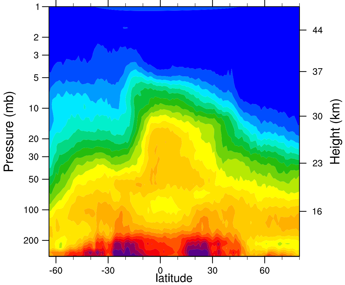
HIRDLSv6 2006d300 N2O_Combined (ppbv)
