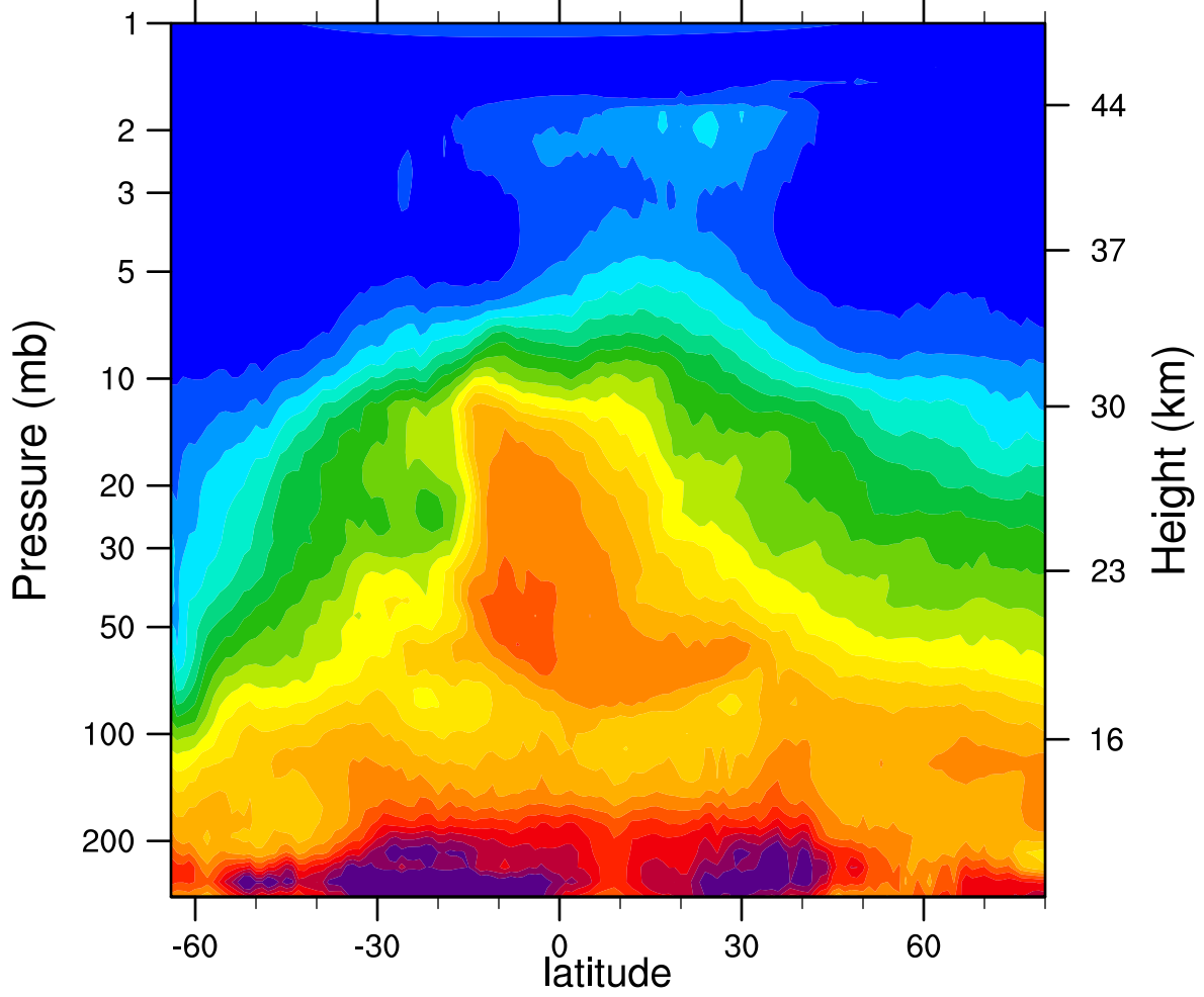
HIRDLSv6 2005d244 N2O_Combined (ppbv)
