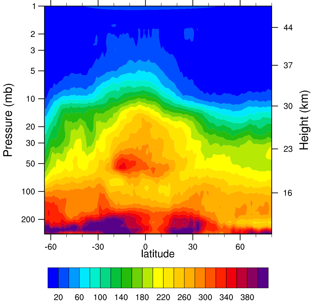
HIRDLSv6 2006d144 N2O_Combined (ppbv)
