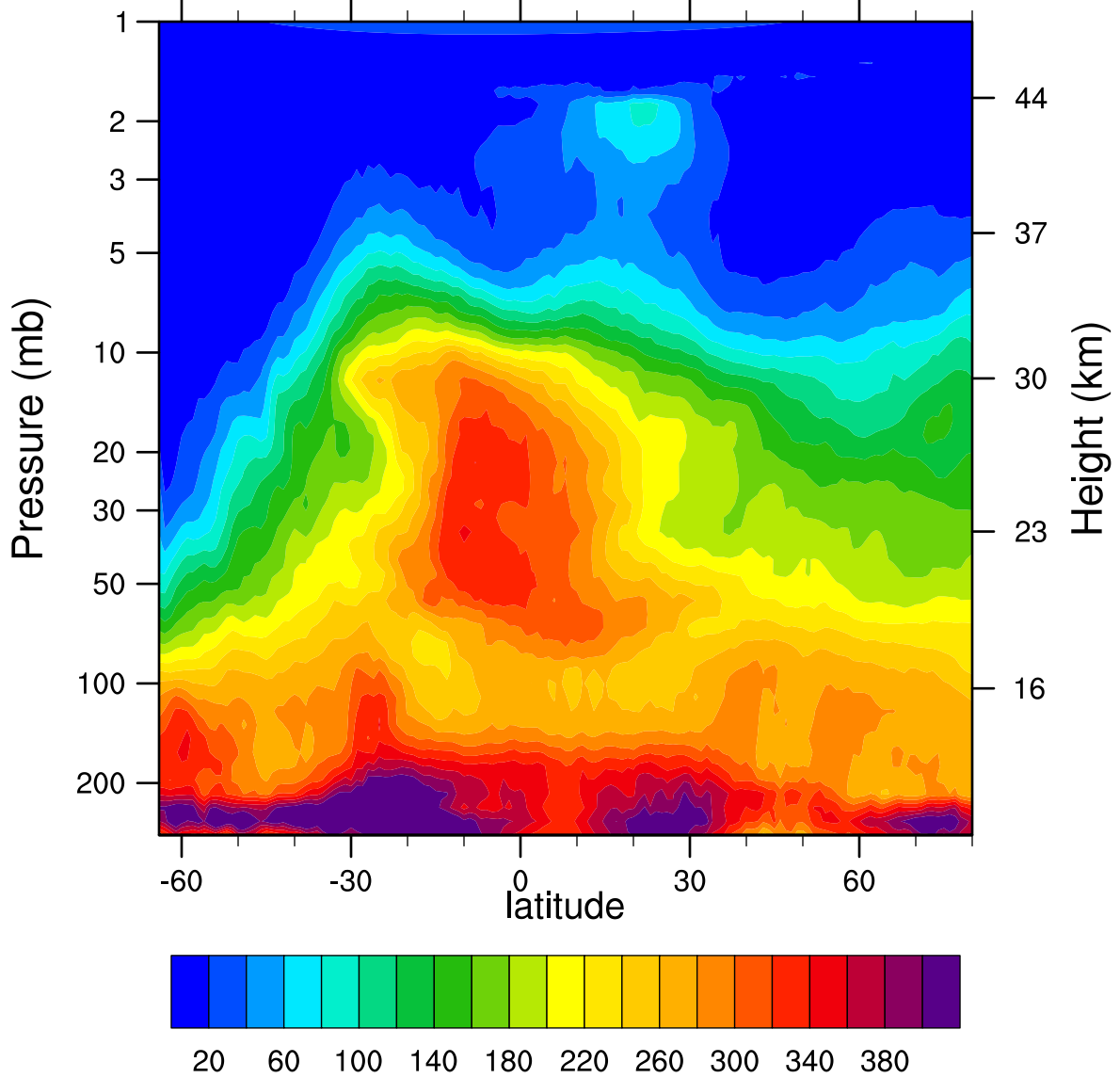
HIRDLSv6 2005d172 N2O_Combined (ppbv)
