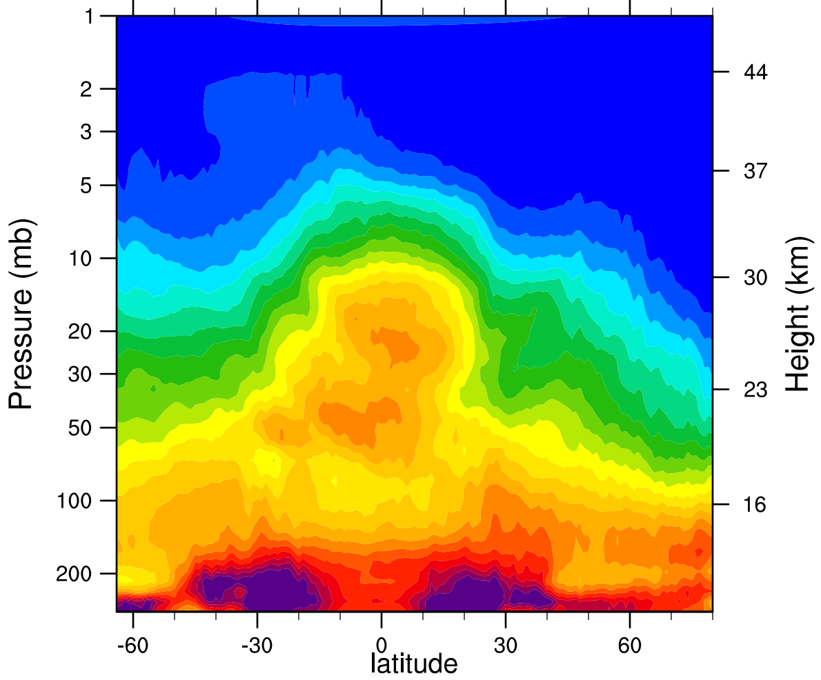
HIRDLSv6 2007d030 N2O_Combined (ppbv)
