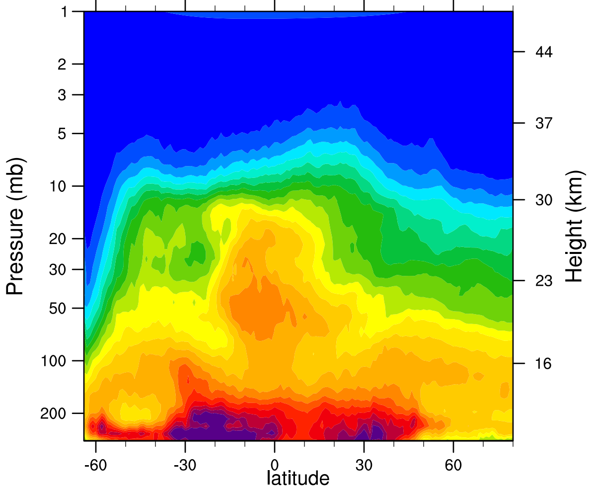
HIRDLSv6 2007d201 N2O_Combined (ppbv)
