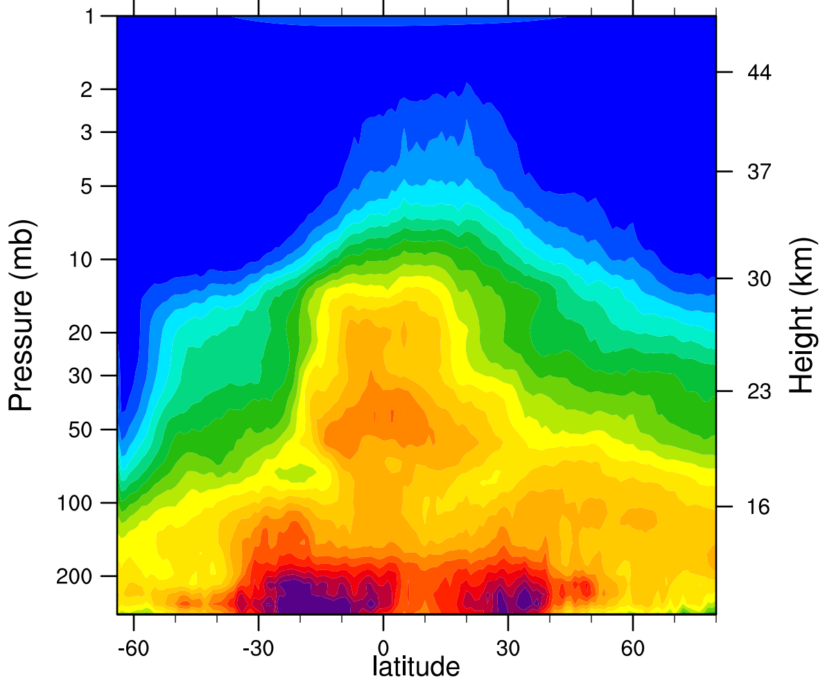
HIRDLSv6 2007d227 N2O_Combined (ppbv)
