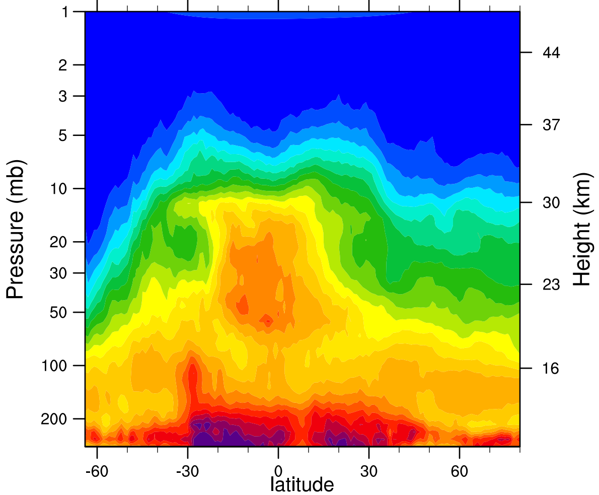
HIRDLSv6 2007d166 N2O_Combined (ppbv)
