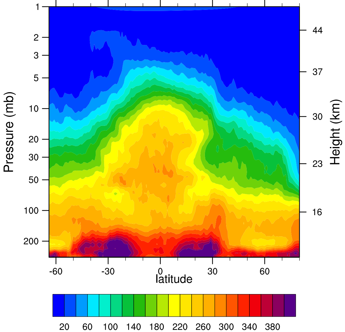
HIRDLSv6 2007d068 N2O_Combined (ppbv)
