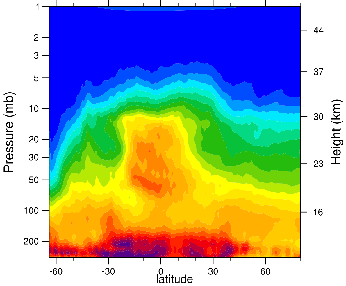
HIRDLSv6 2007d177 N2O_Combined (ppbv)
