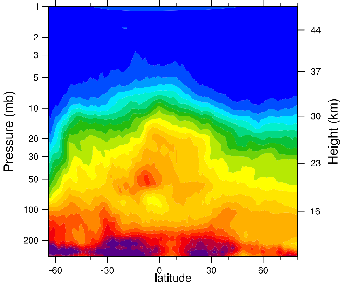
HIRDLSv6 2006d173 N2O_Combined (ppbv)
