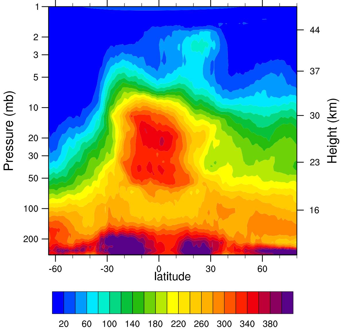
HIRDLSv6 2005d139 N2O_Combined (ppbv)
