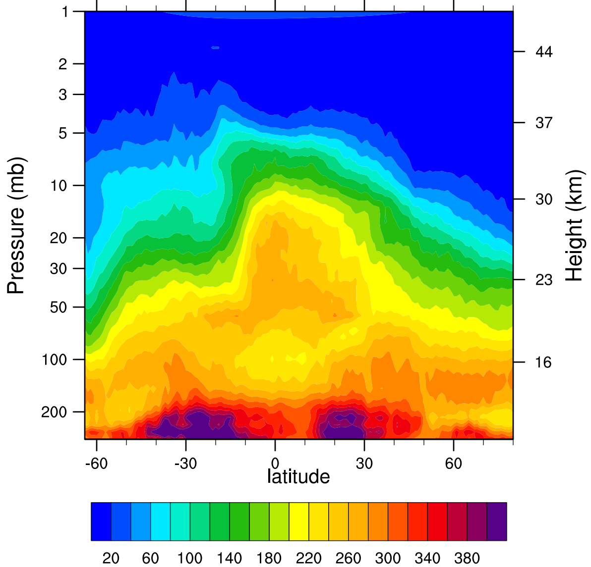
HIRDLSv6 2006d297 N2O_Combined (ppbv)
