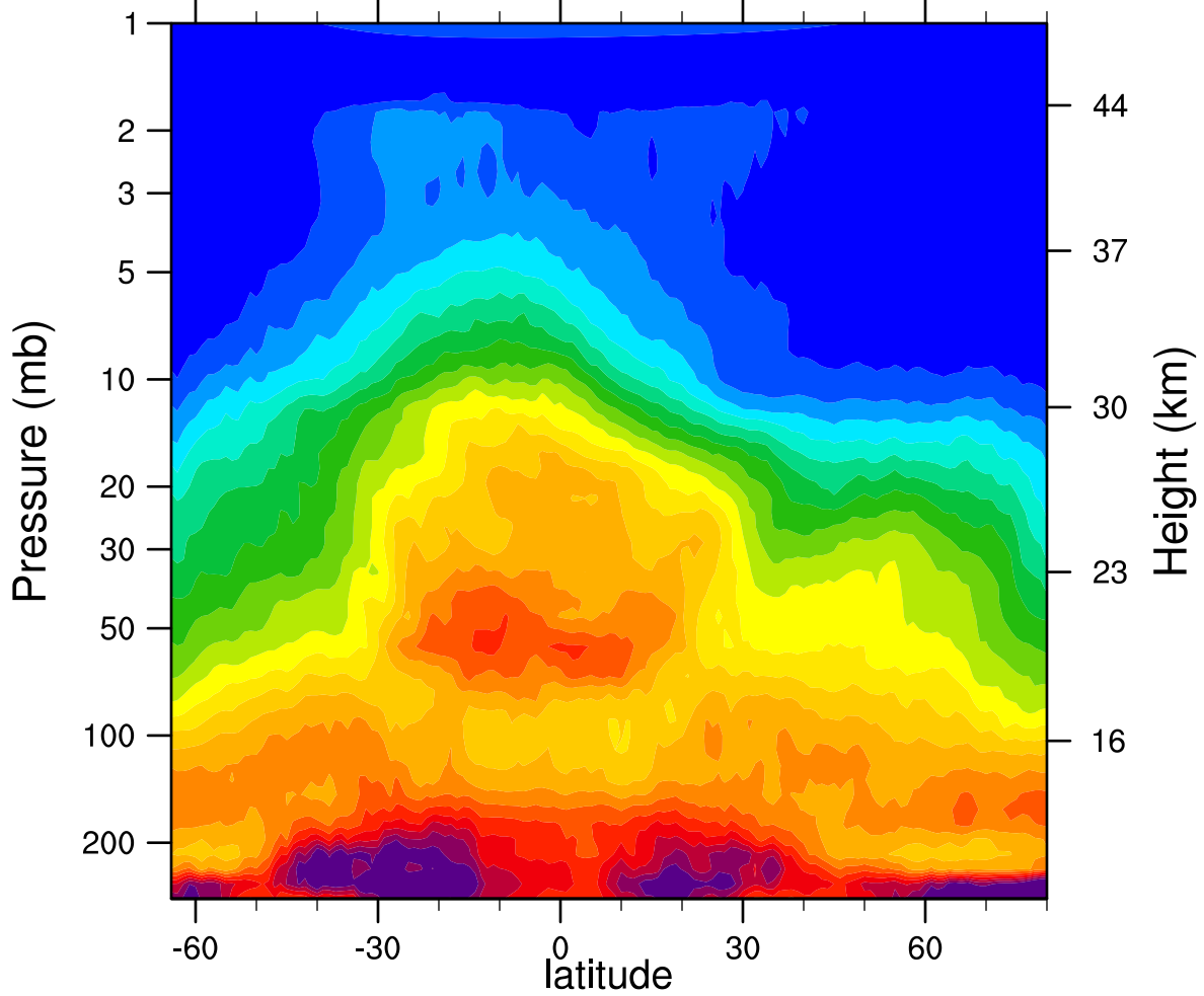
HIRDLSv6 2006d103 N2O_Combined (ppbv)
