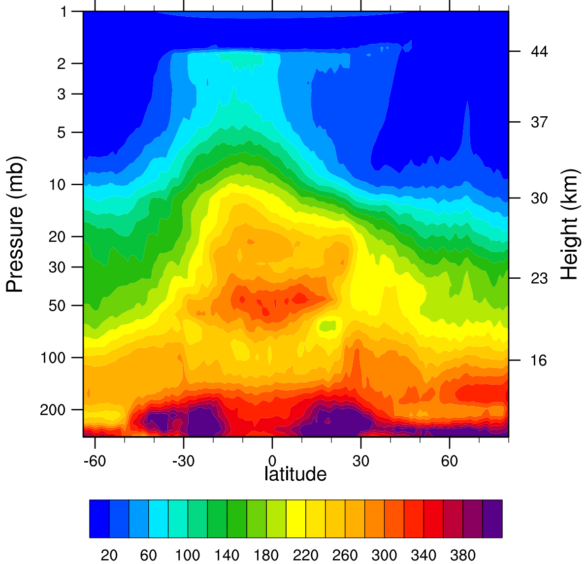
HIRDLSv6 2006d057 N2O_Combined (ppbv)
