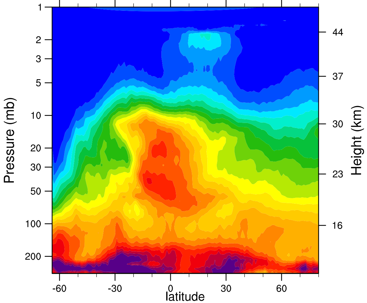
HIRDLSv6 2005d184 N2O_Combined (ppbv)
