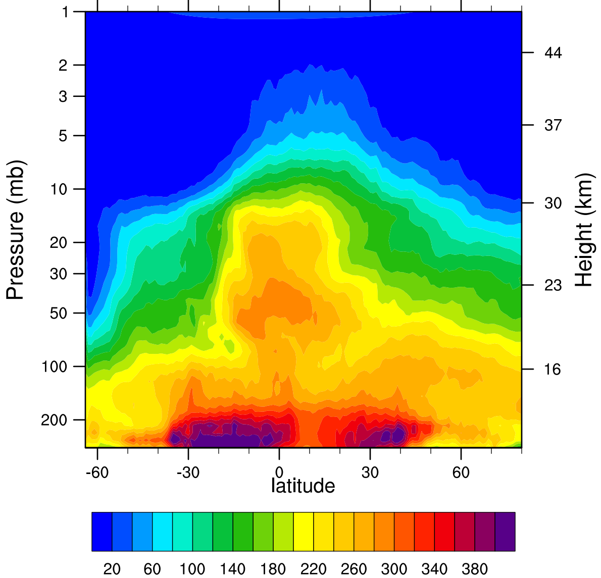
HIRDLSv6 2007d223 N2O_Combined (ppbv)
