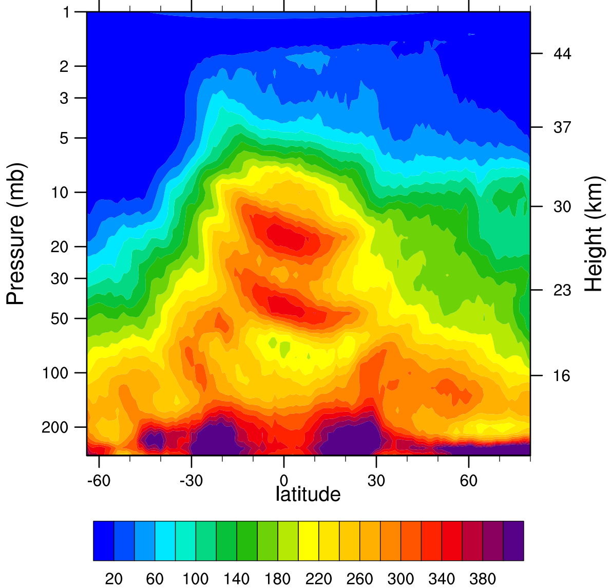
HIRDLSv6 2005d087 N2O_Combined (ppbv)
