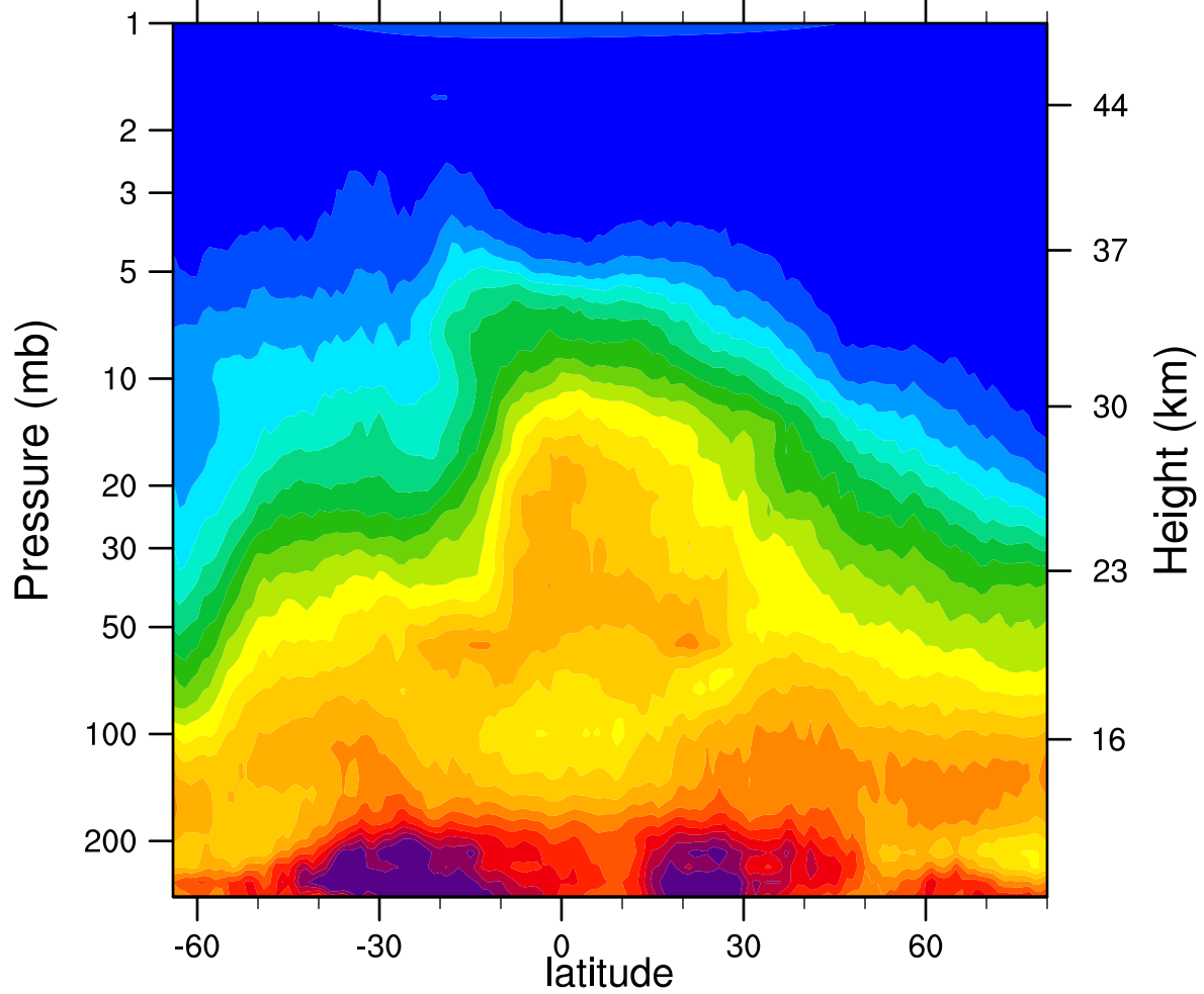
HIRDLSv6 2006d296 N2O_Combined (ppbv)
