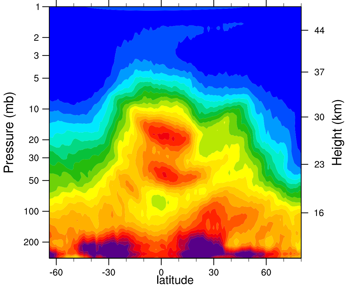
HIRDLSv6 2005d034 N2O_Combined (ppbv)
