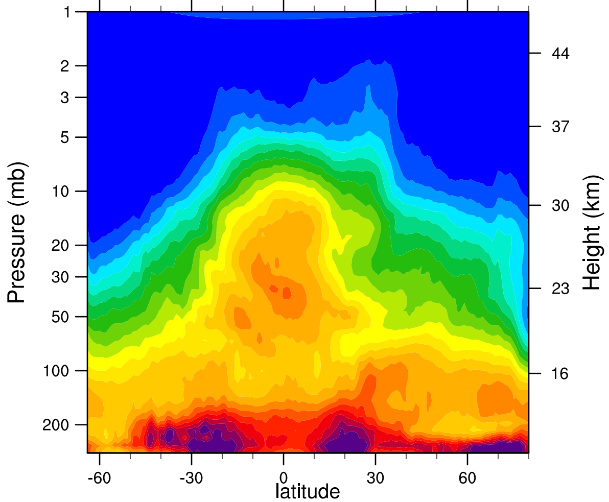
HIRDLSv6 2007d105 N2O_Combined (ppbv)
