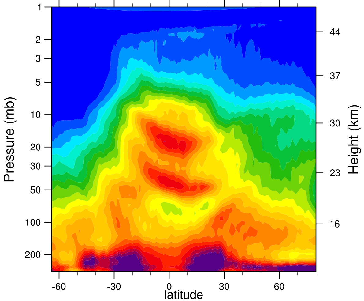
HIRDLSv6 2005d081 N2O_Combined (ppbv)
