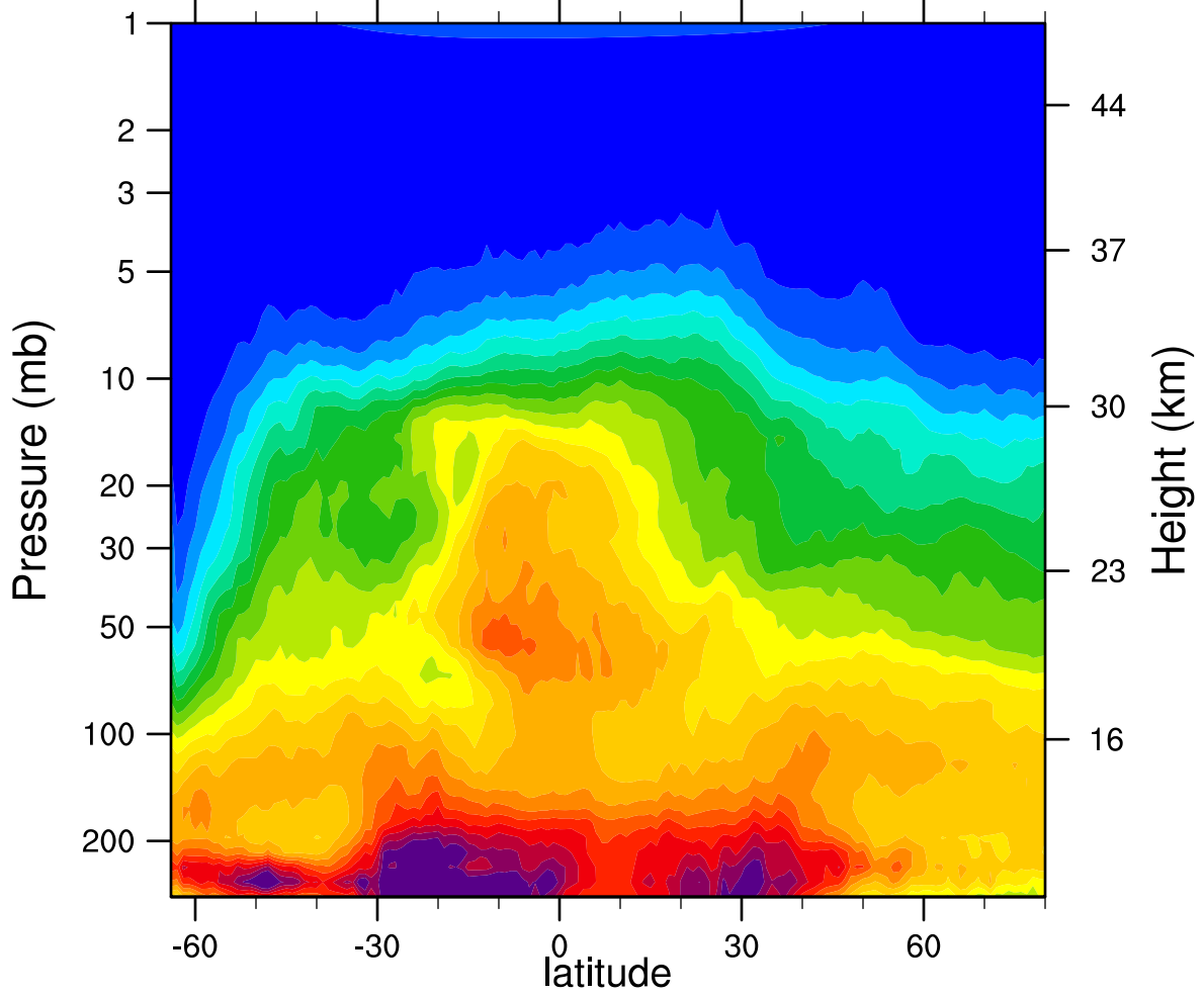
HIRDLSv6 2007d196 N2O_Combined (ppbv)
