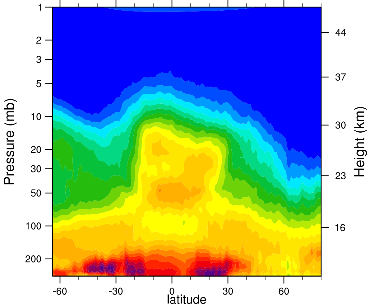
HIRDLSv6 2007d338 N2O_Combined (ppbv)
