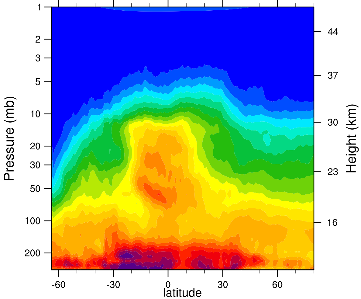
HIRDLSv6 2007d179 N2O_Combined (ppbv)
