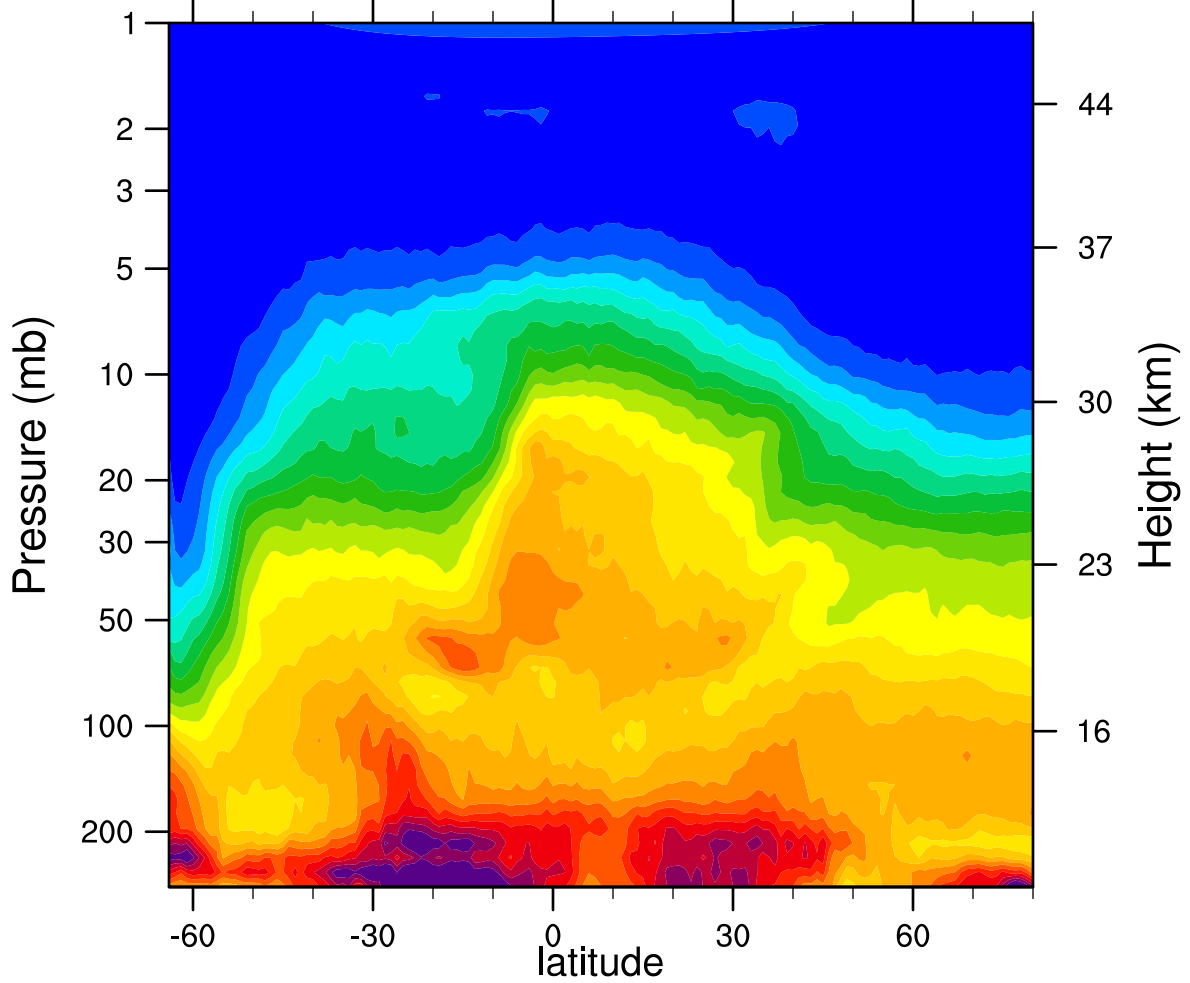
HIRDLSv6 2006d244 N2O_Combined (ppbv)
