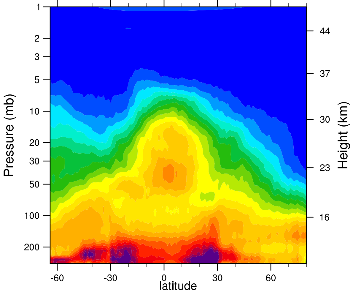
HIRDLSv6 2006d353 N2O_Combined (ppbv)
