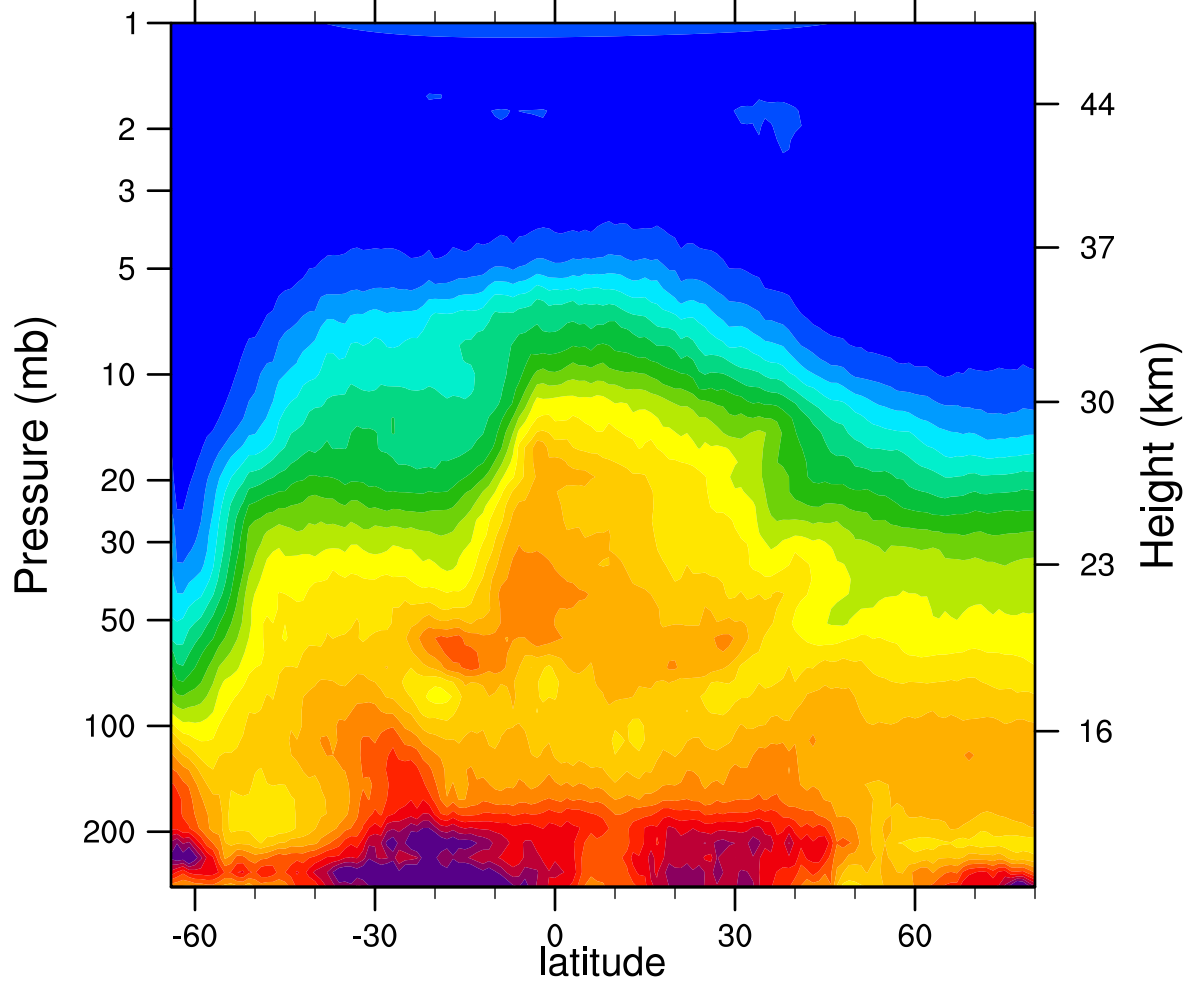
HIRDLSv6 2006d243 N2O_Combined (ppbv)
