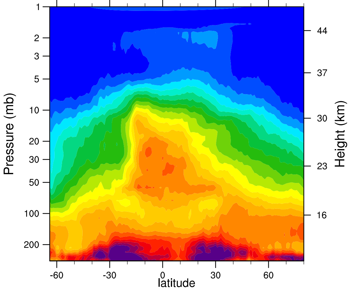
HIRDLSv6 2005d283 N2O_Combined (ppbv)
