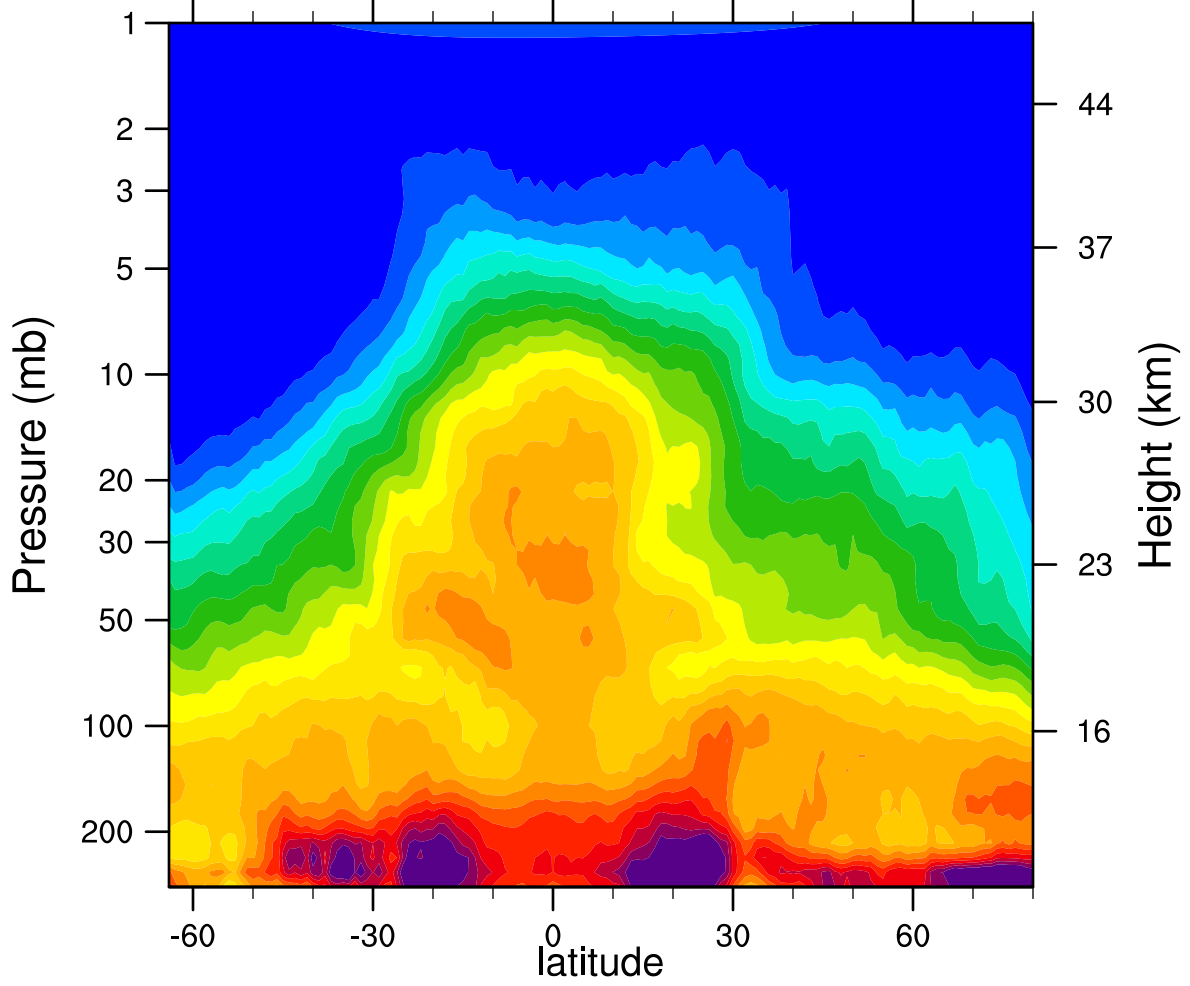
HIRDLSv6 2007d094 N2O_Combined (ppbv)
