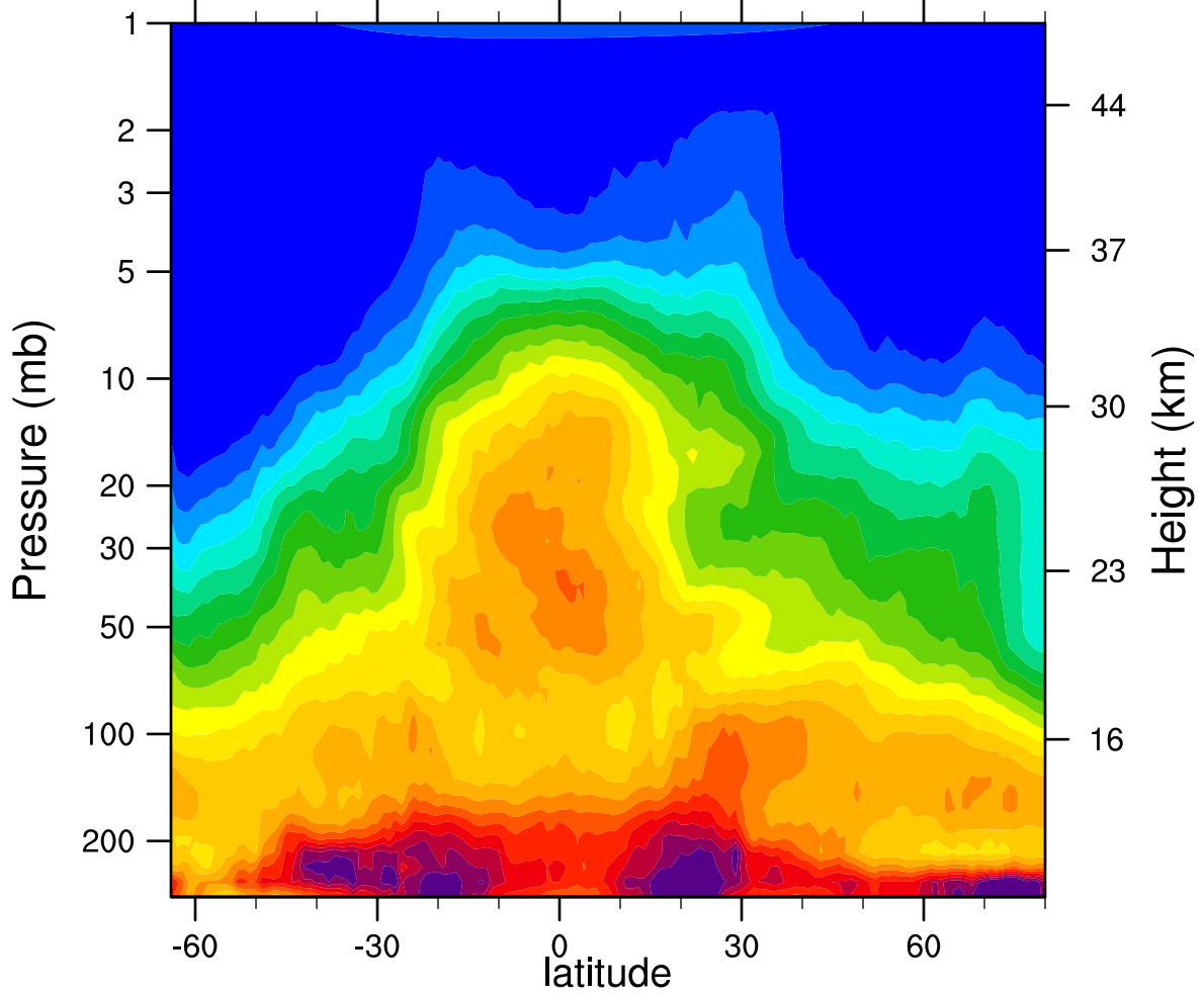
HIRDLSv6 2007d110 N2O_Combined (ppbv)
