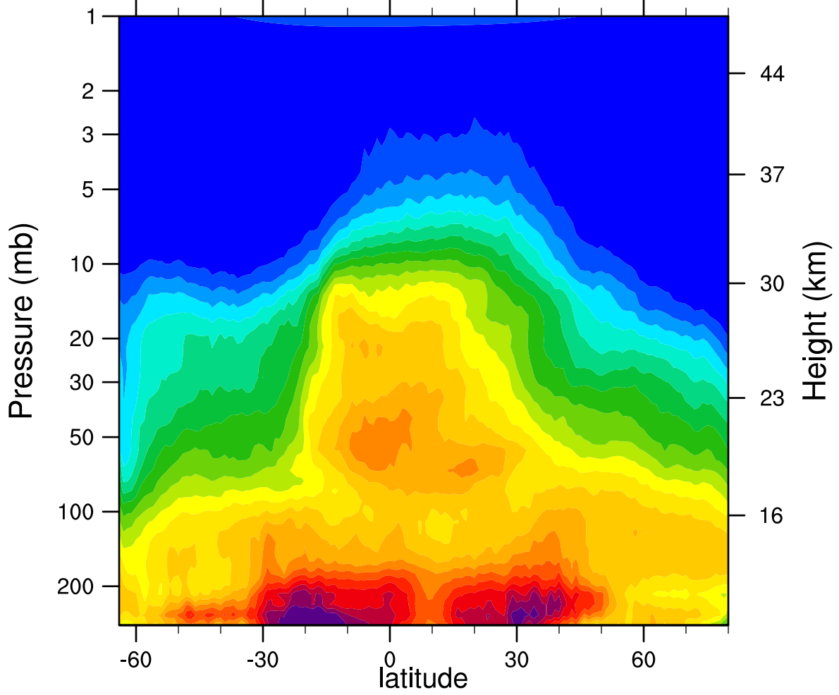
HIRDLSv6 2007d261 N2O_Combined (ppbv)
