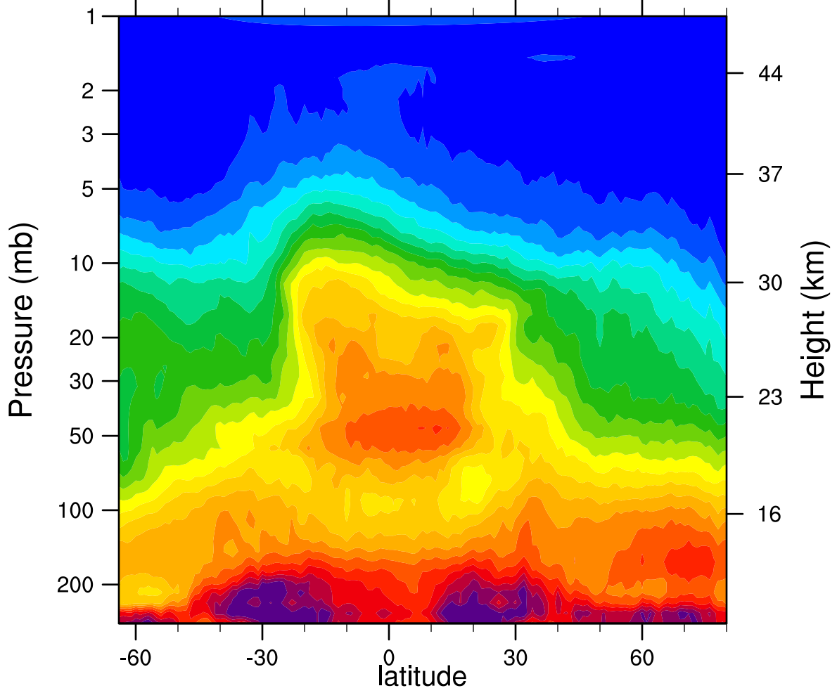
HIRDLSv6 2005d333 N2O_Combined (ppbv)
