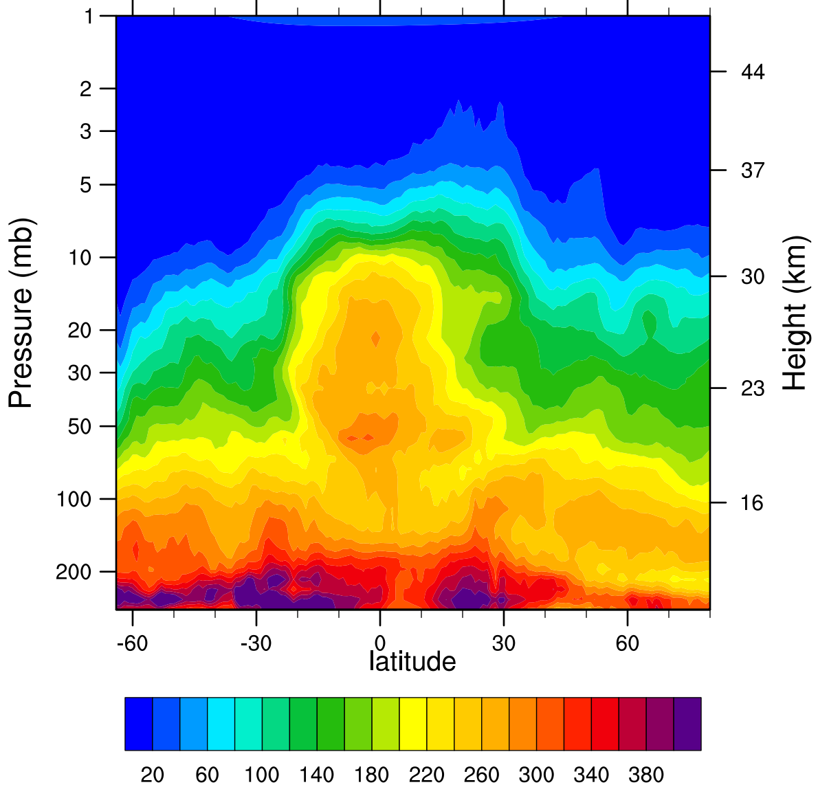
HIRDLSv6 2007d150 N2O_Combined (ppbv)
