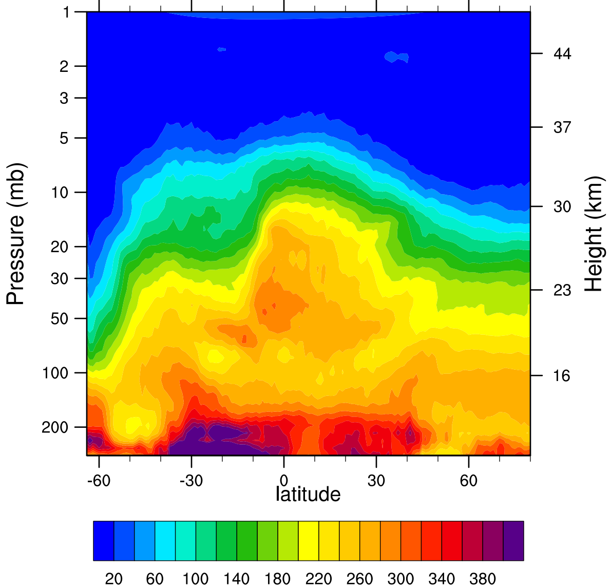
HIRDLSv6 2006d235 N2O_Combined (ppbv)
