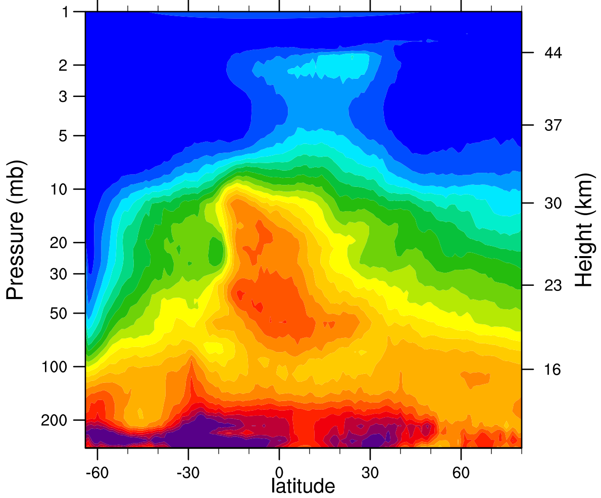
HIRDLSv6 2005d227 N2O_Combined (ppbv)
