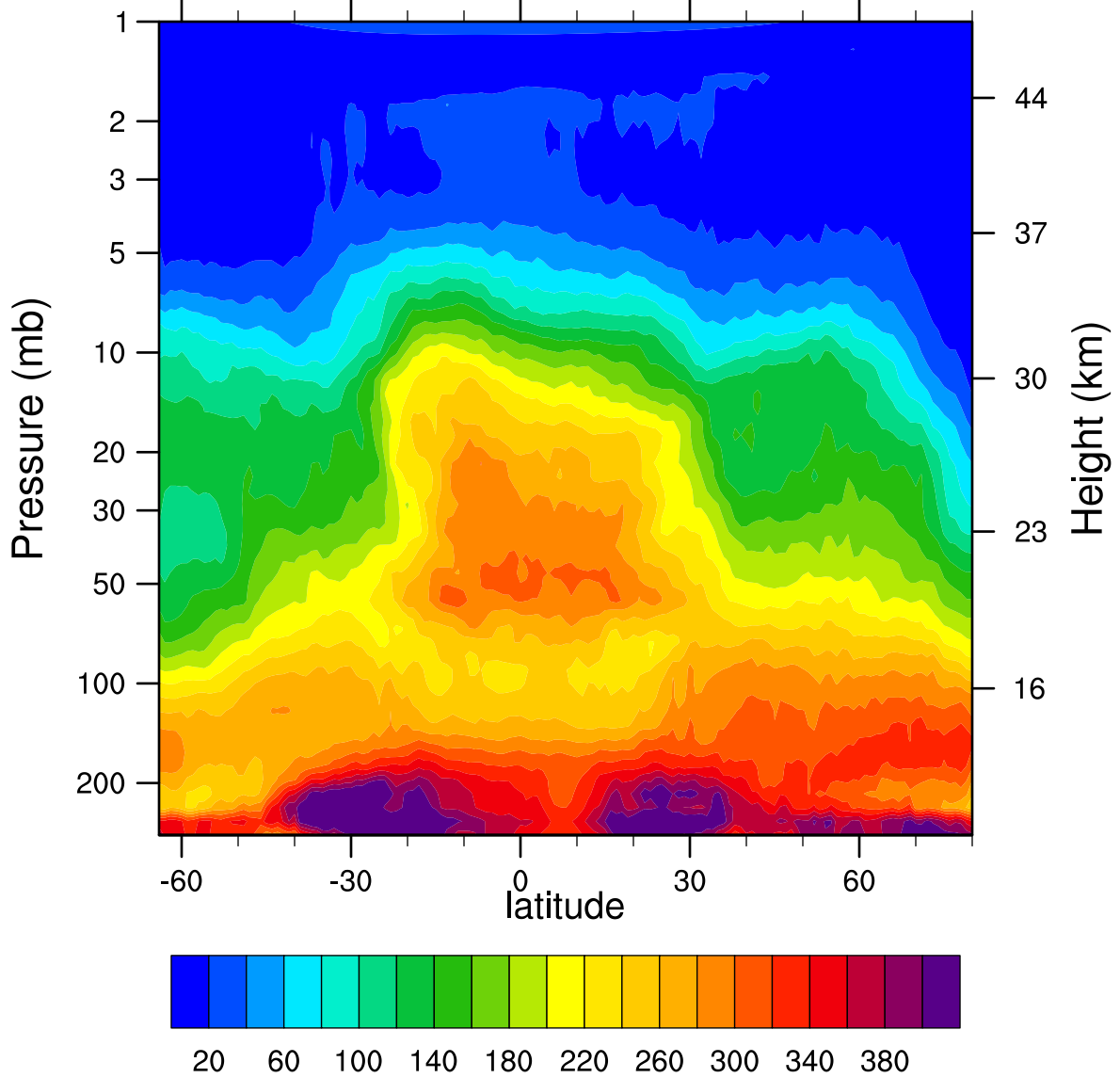
HIRDLSv6 2005d317 N2O_Combined (ppbv)
