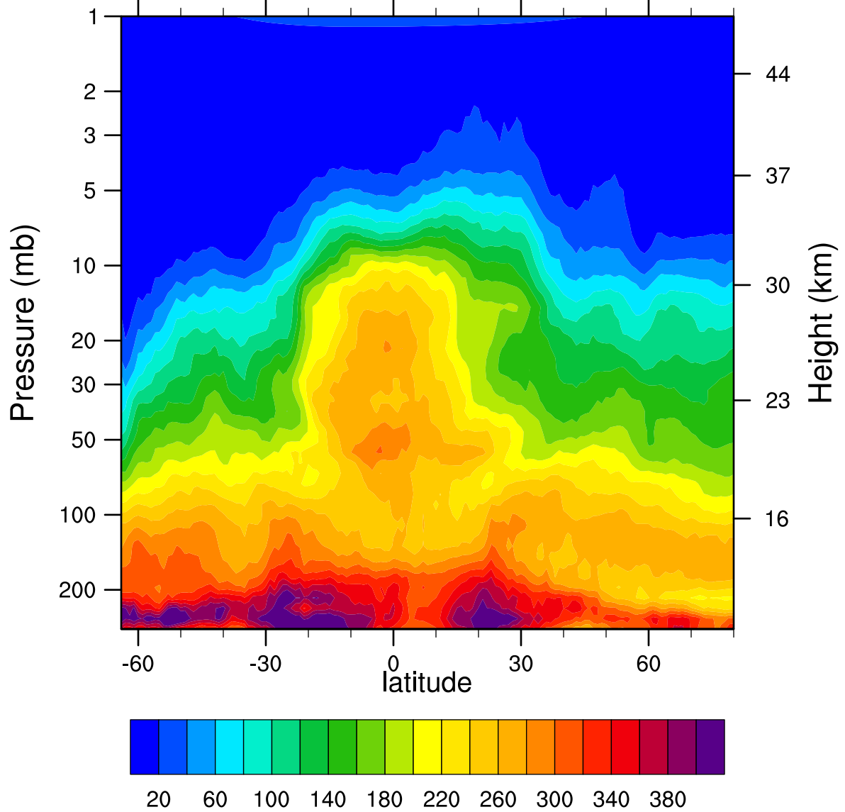
HIRDLSv6 2007d148 N2O_Combined (ppbv)
