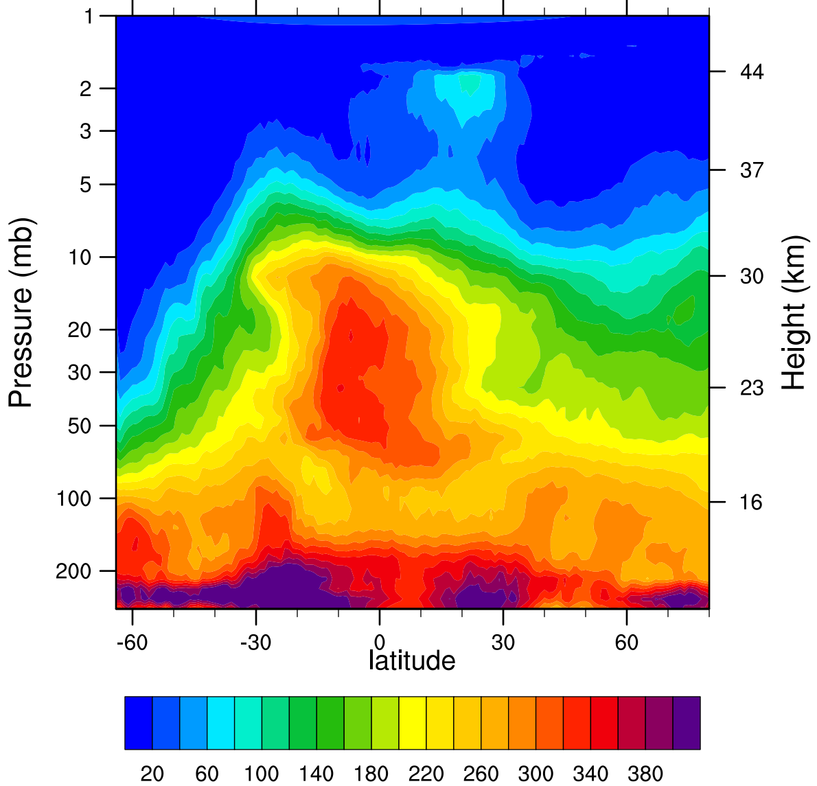
HIRDLSv6 2005d171 N2O_Combined (ppbv)
