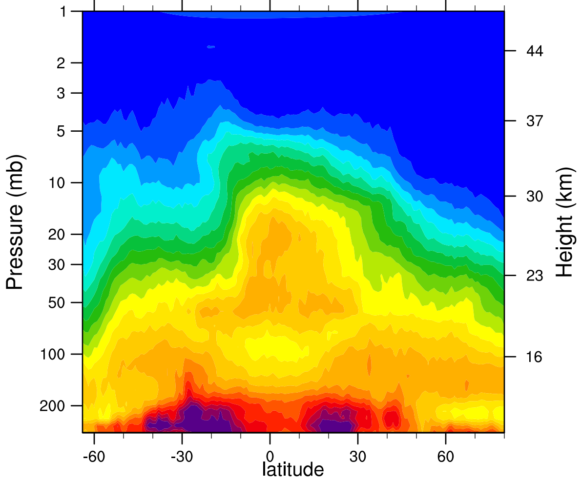
HIRDLSv6 2006d304 N2O_Combined (ppbv)
