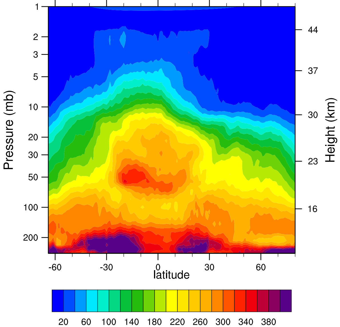
HIRDLSv6 2006d114 N2O_Combined (ppbv)
