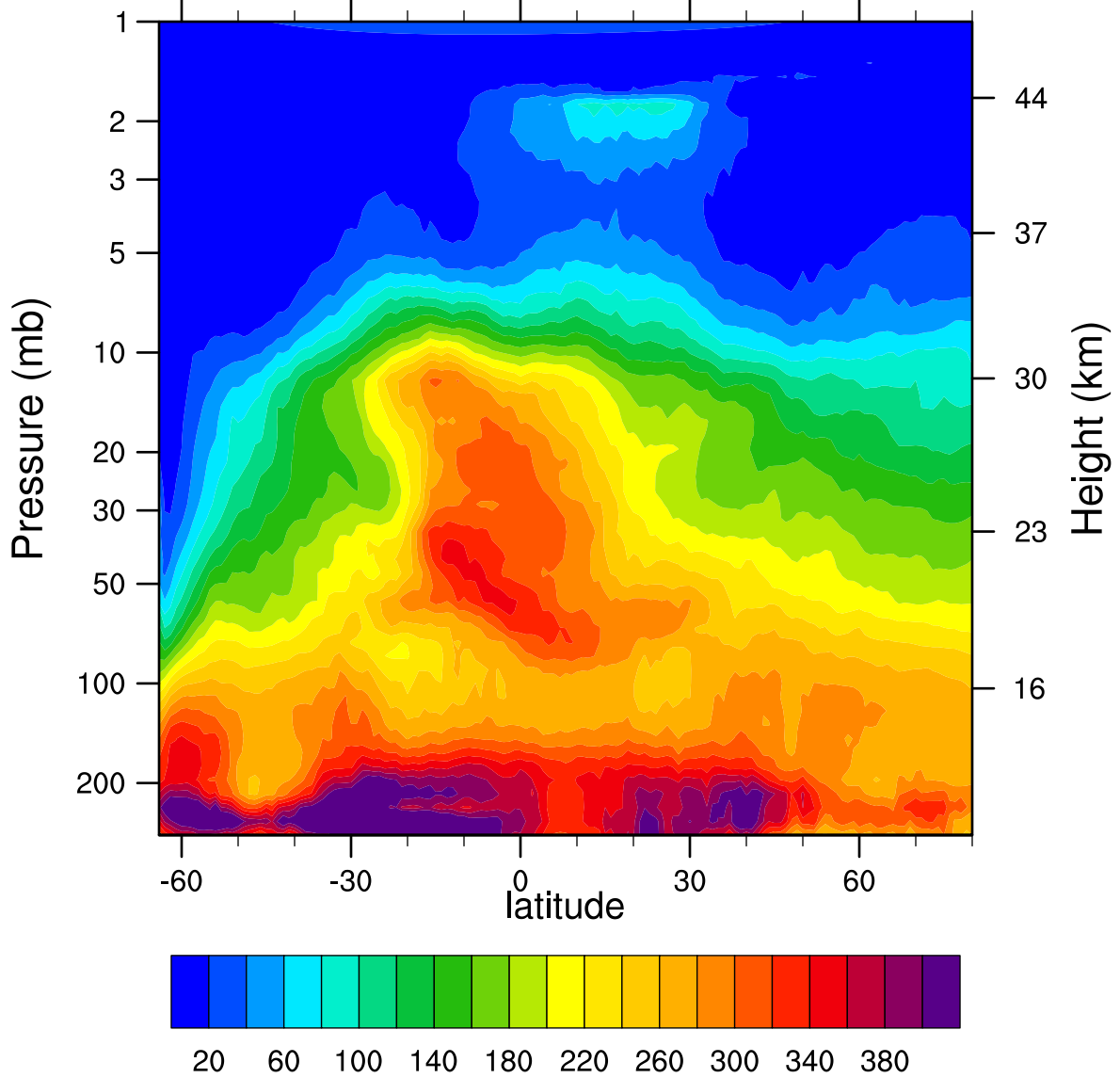
HIRDLSv6 2005d202 N2O_Combined (ppbv)
