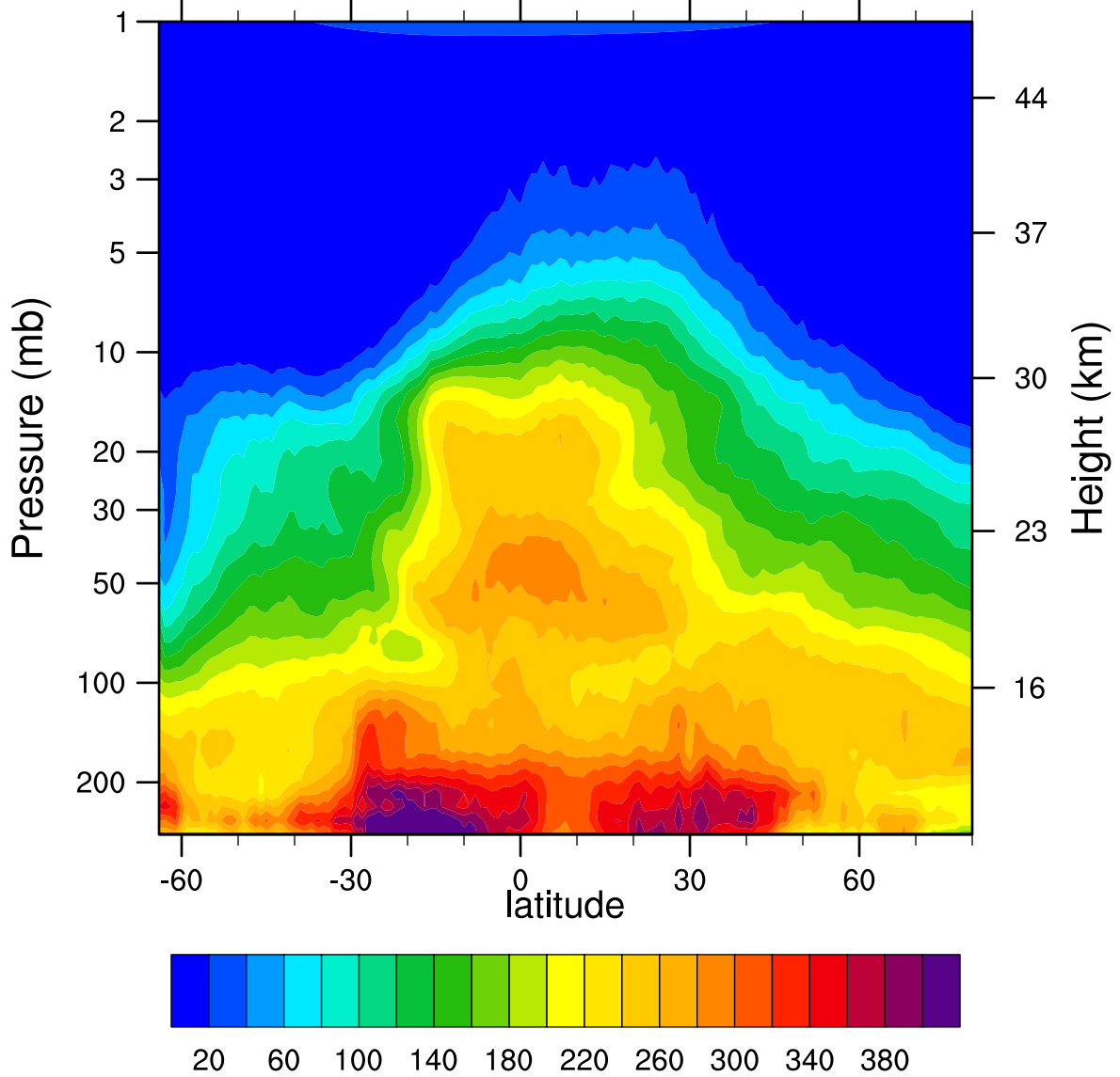
HIRDLSv6 2007d249 N2O_Combined (ppbv)
