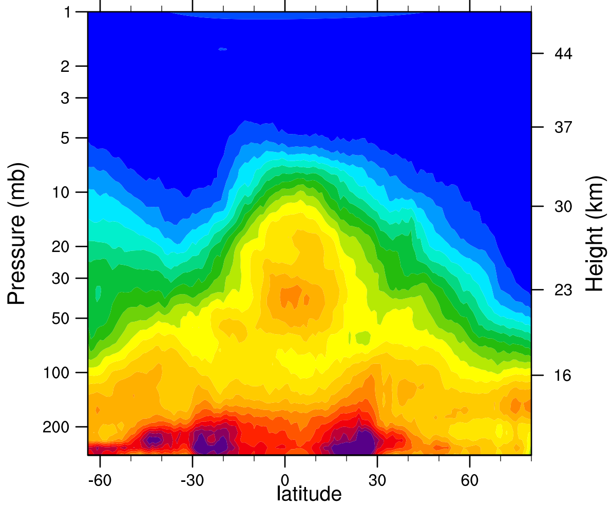
HIRDLSv6 2006d351 N2O_Combined (ppbv)
