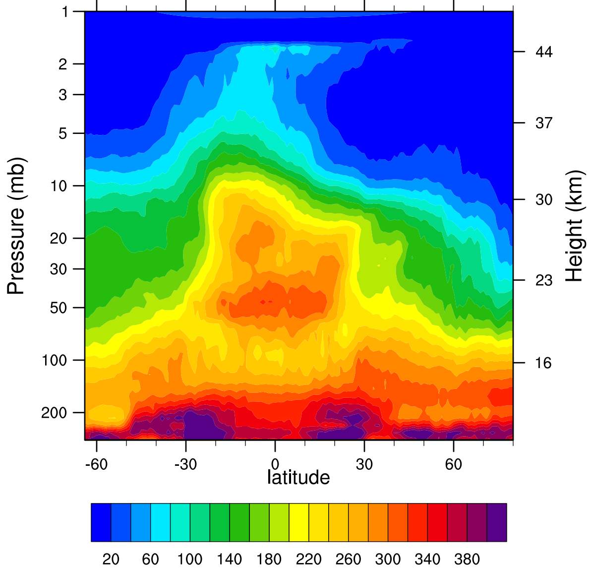
HIRDLSv6 2006d002 N2O_Combined (ppbv)
