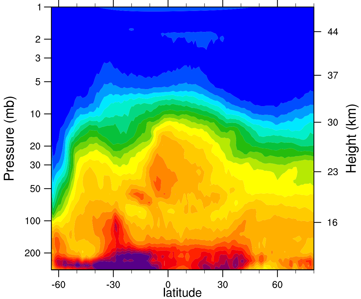
HIRDLSv6 2006d208 N2O_Combined (ppbv)
