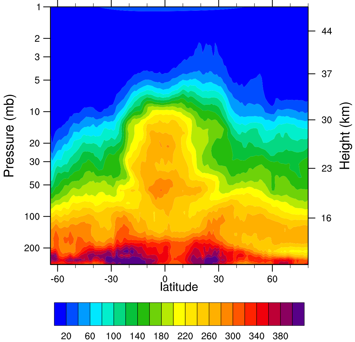
HIRDLSv6 2007d145 N2O_Combined (ppbv)
