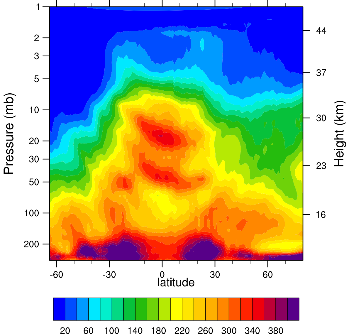
HIRDLSv6 2005d098 N2O_Combined (ppbv)
