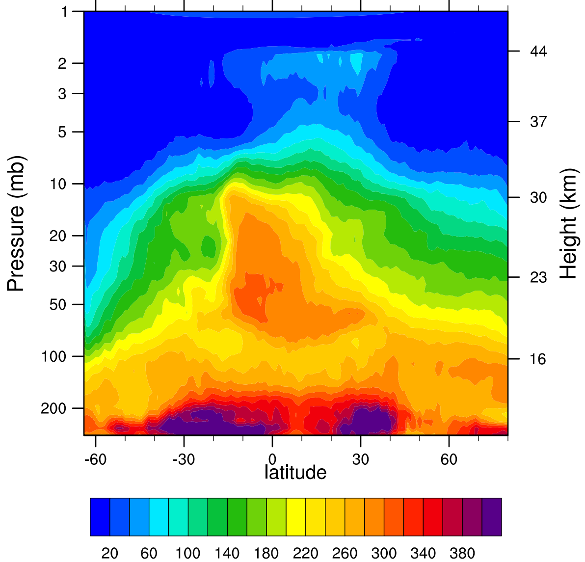
HIRDLSv6 2005d247 N2O_Combined (ppbv)
