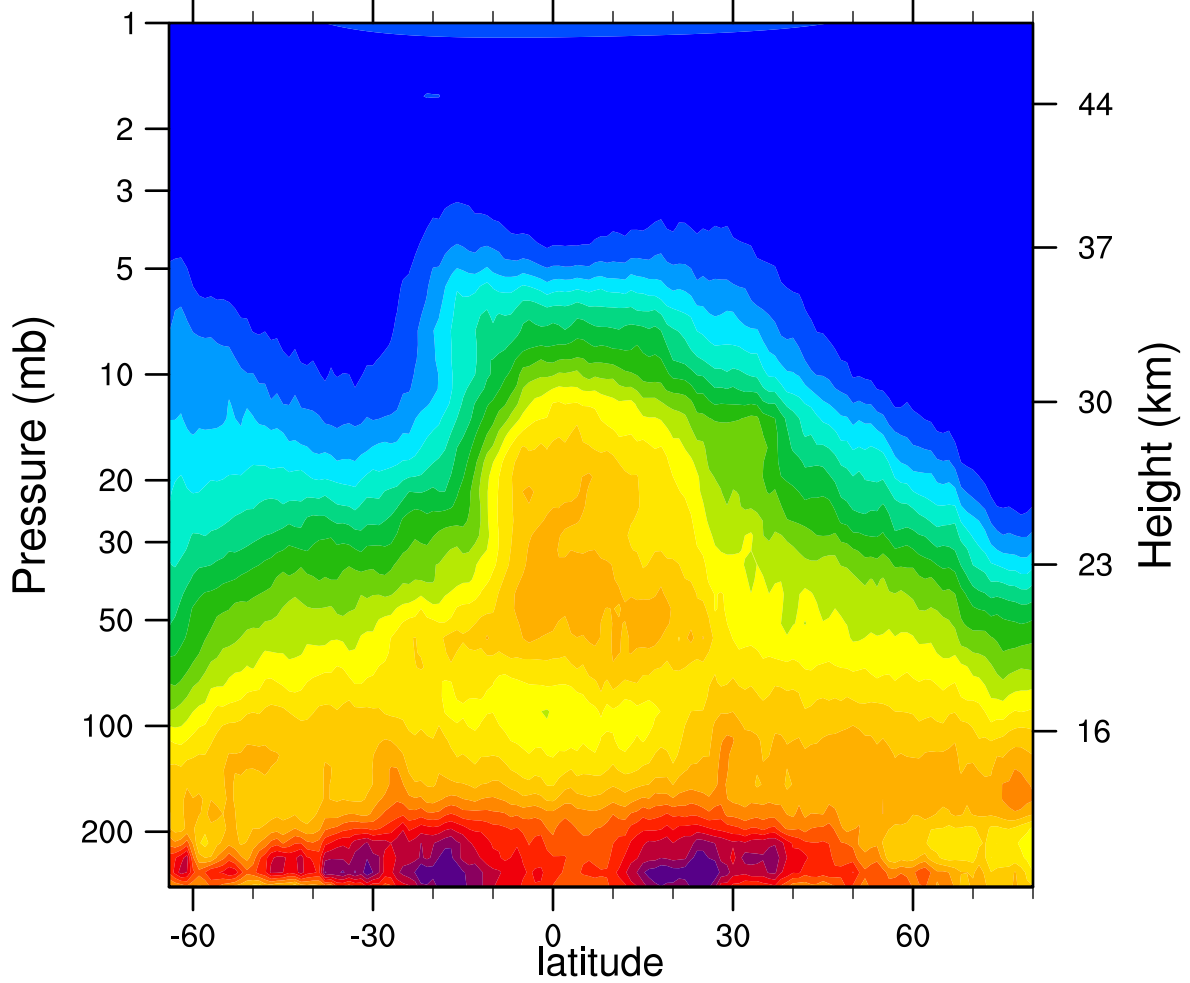
HIRDLSv6 2006d314 N2O_Combined (ppbv)
