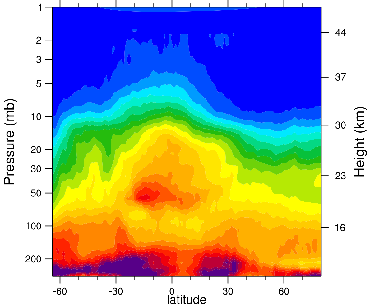
HIRDLSv6 2006d145 N2O_Combined (ppbv)
