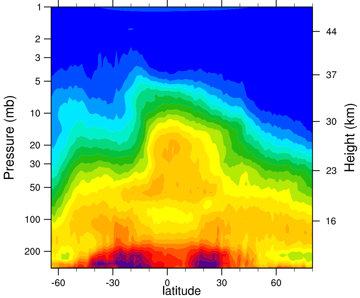
HIRDLSv6 2006d303 N2O_Combined (ppbv)
