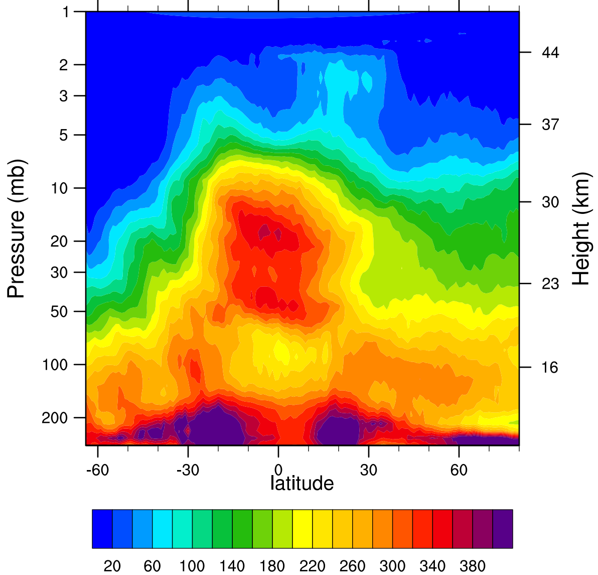
HIRDLSv6 2005d117 N2O_Combined (ppbv)
