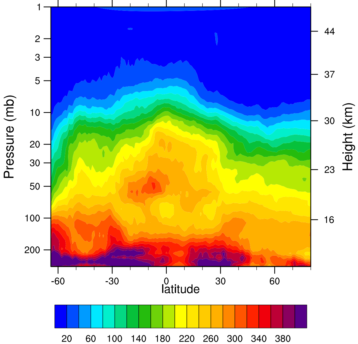
HIRDLSv6 2006d168 N2O_Combined (ppbv)
