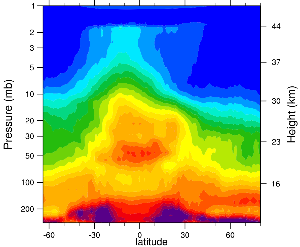
HIRDLSv6 2006d052 N2O_Combined (ppbv)
