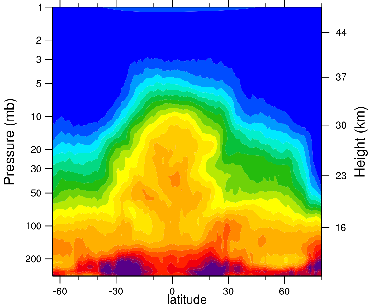
HIRDLSv6 2007d082 N2O_Combined (ppbv)
