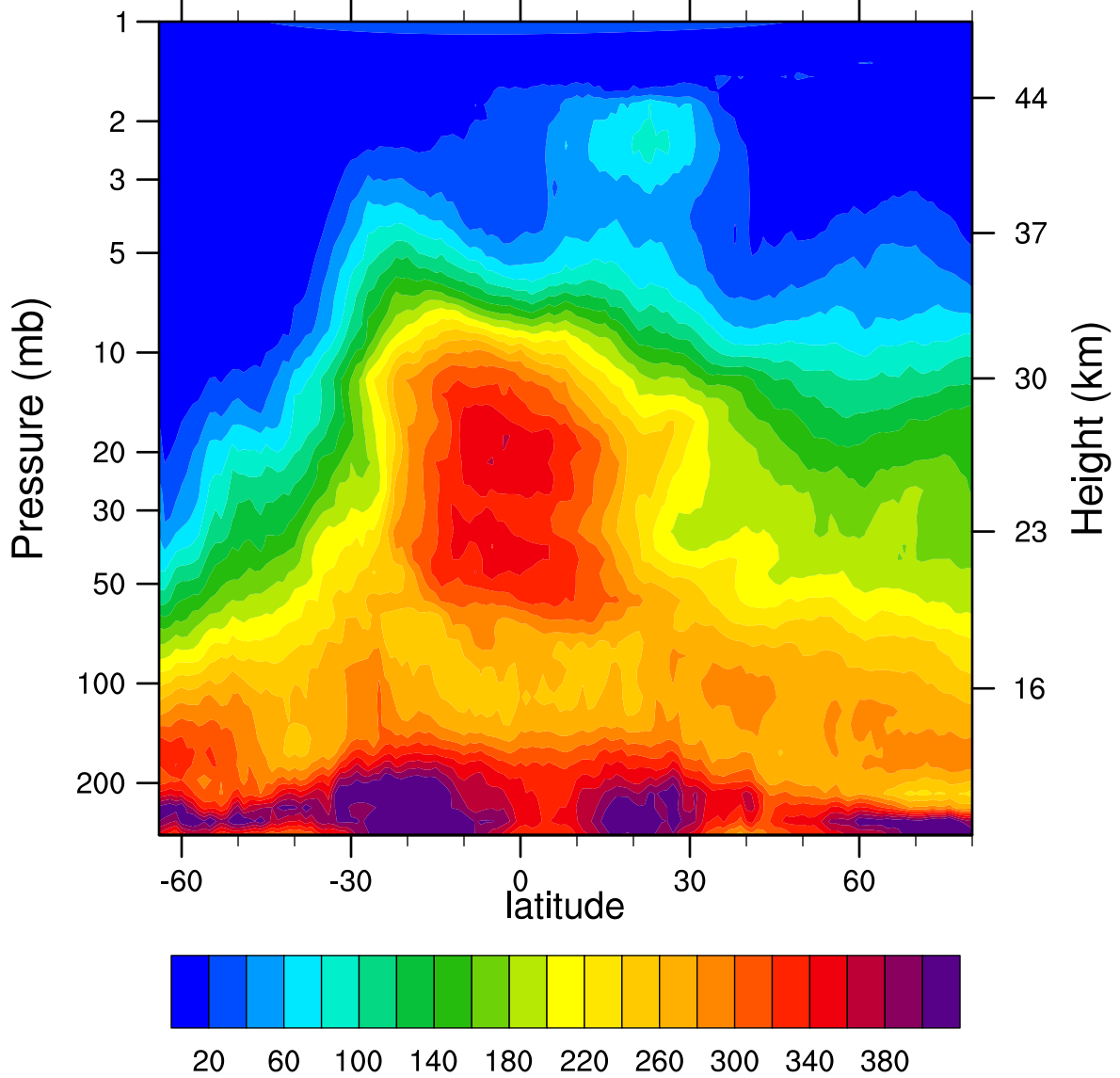
HIRDLSv6 2005d146 N2O_Combined (ppbv)
