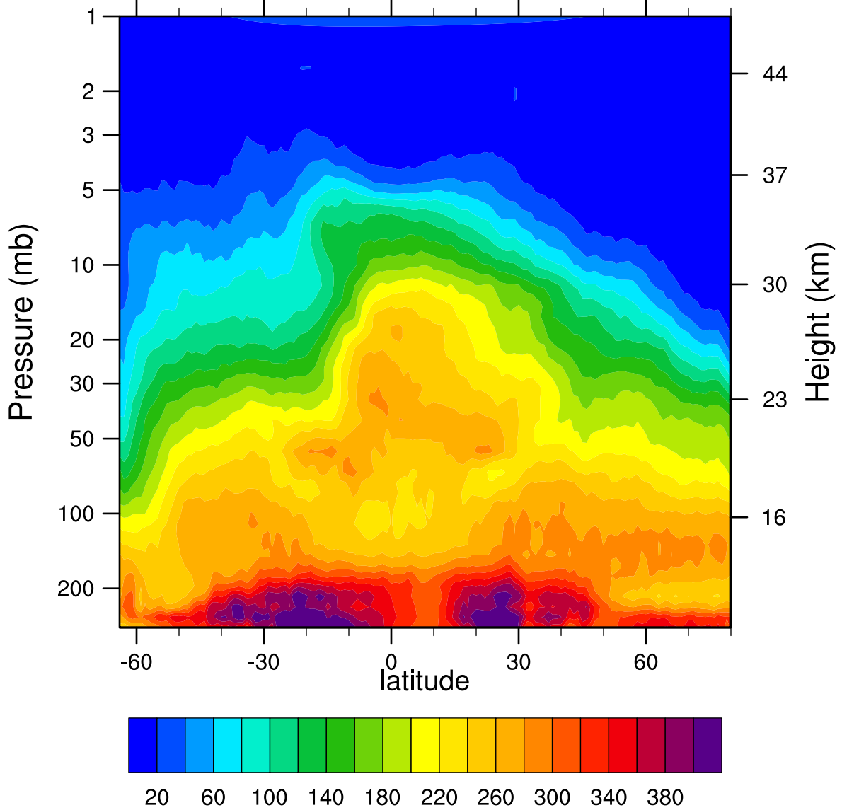
HIRDLSv6 2006d286 N2O_Combined (ppbv)
