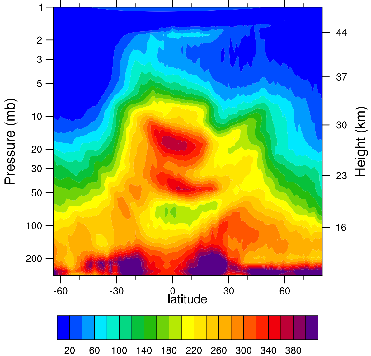
HIRDLSv6 2005d061 N2O_Combined (ppbv)
