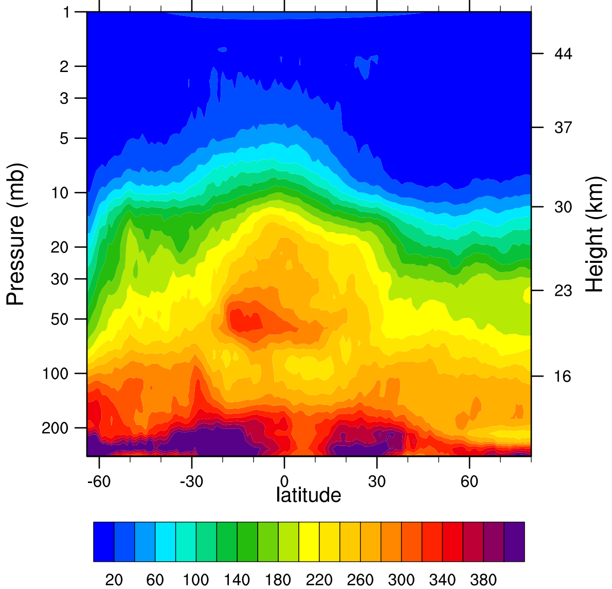
HIRDLSv6 2006d149 N2O_Combined (ppbv)
