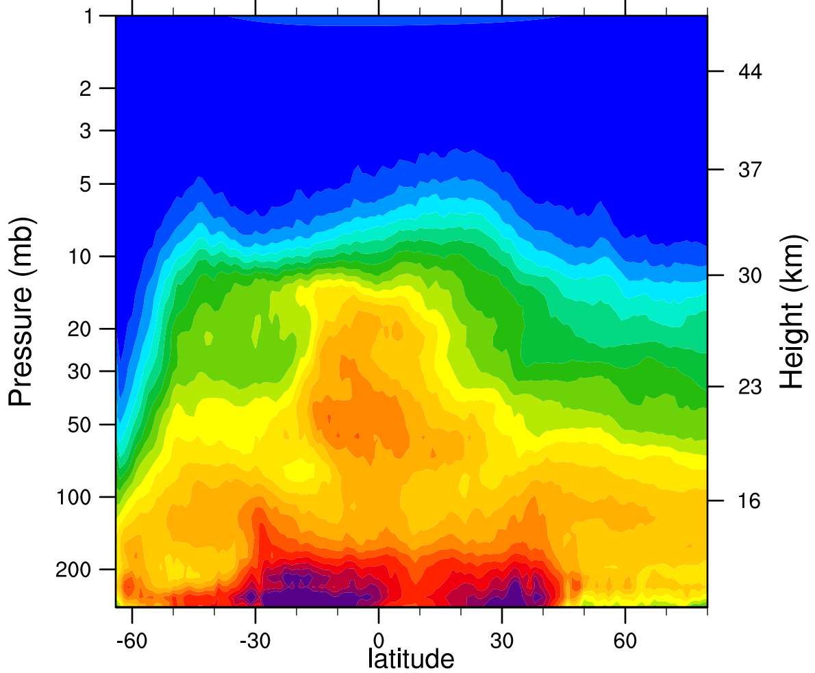
HIRDLSv6 2007d205 N2O_Combined (ppbv)
