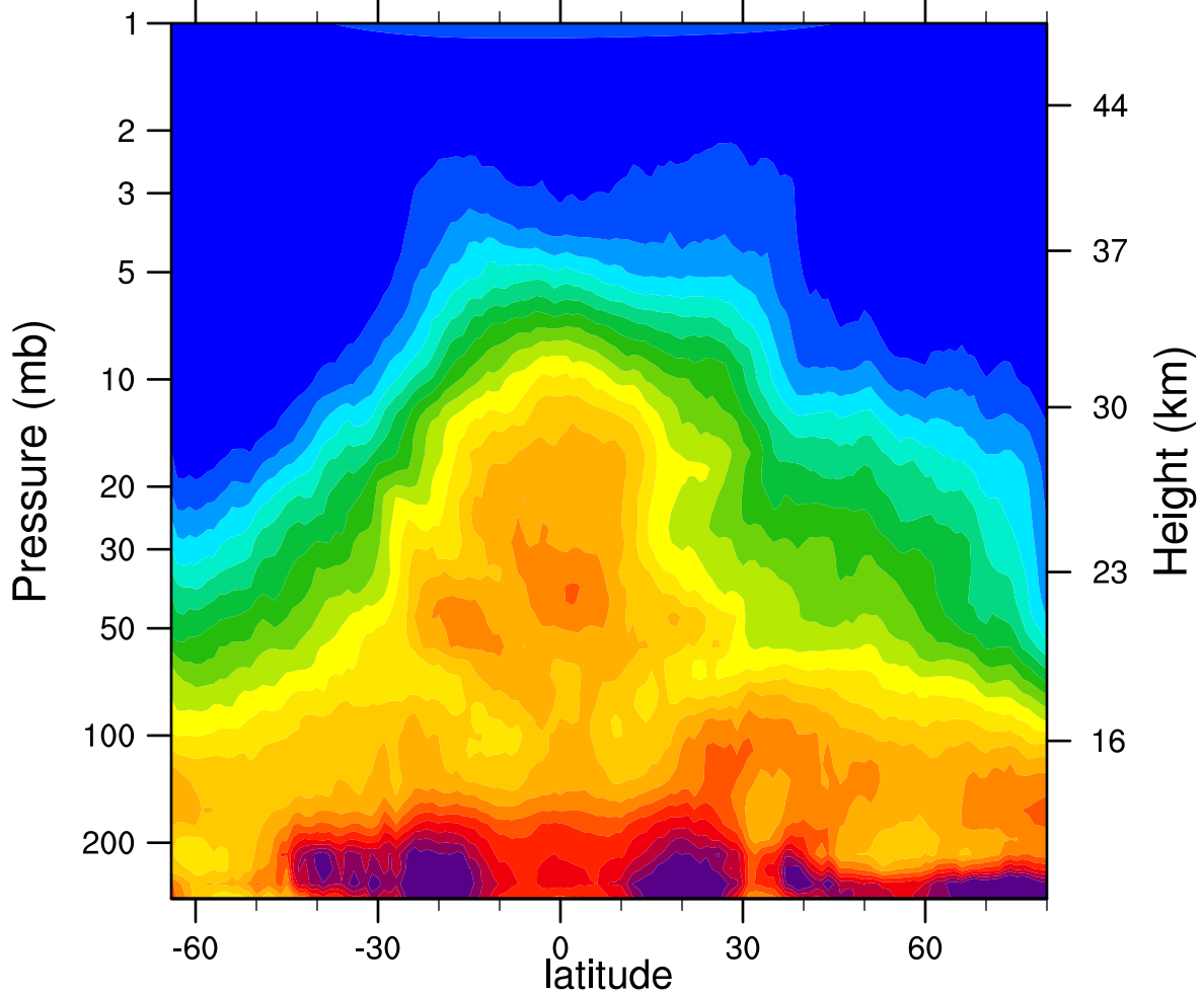
HIRDLSv6 2007d098 N2O_Combined (ppbv)
