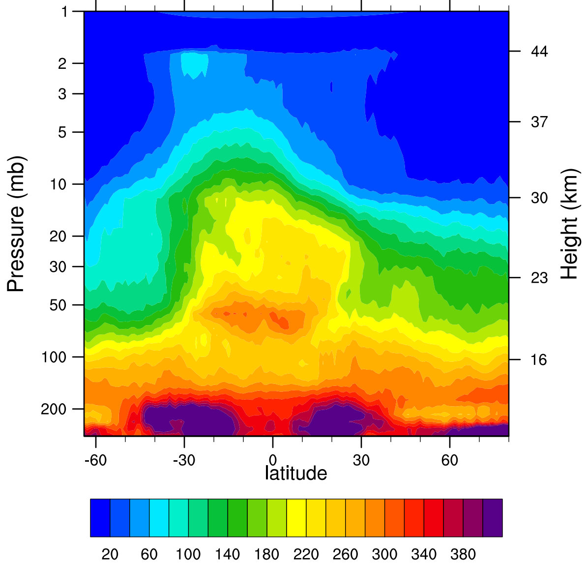
HIRDLSv6 2006d094 N2O_Combined (ppbv)
