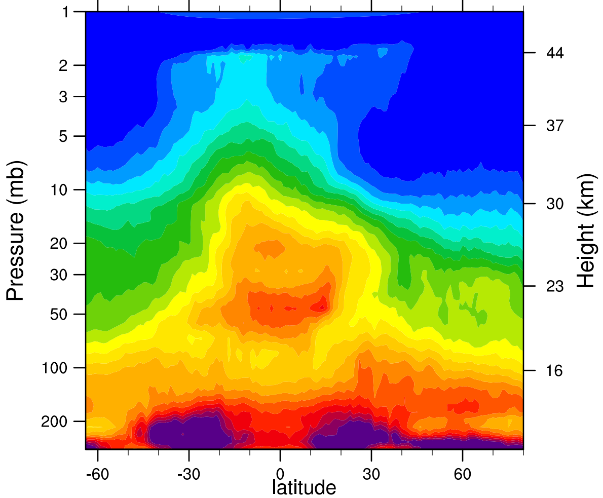
HIRDLSv6 2006d041 N2O_Combined (ppbv)
