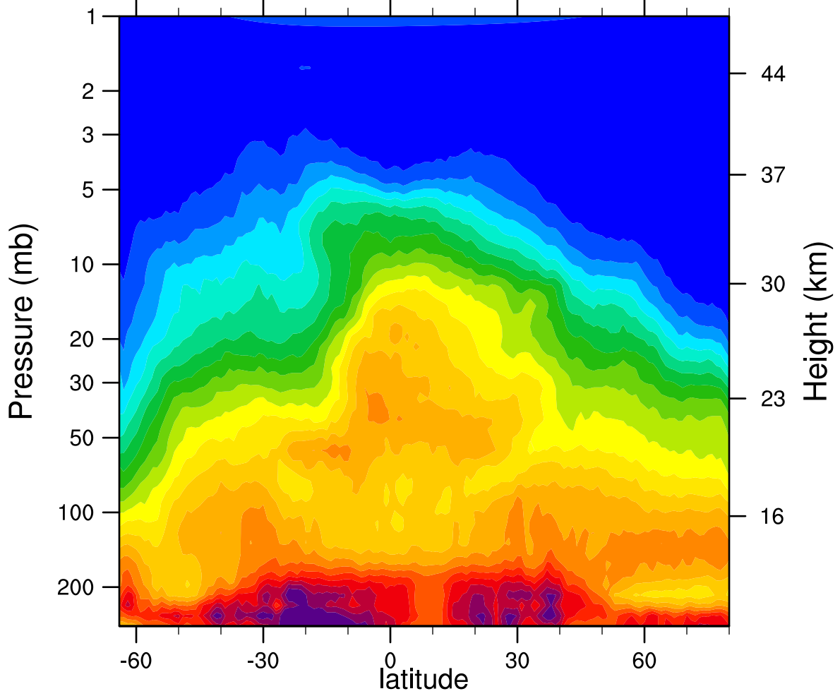
HIRDLSv6 2006d282 N2O_Combined (ppbv)
