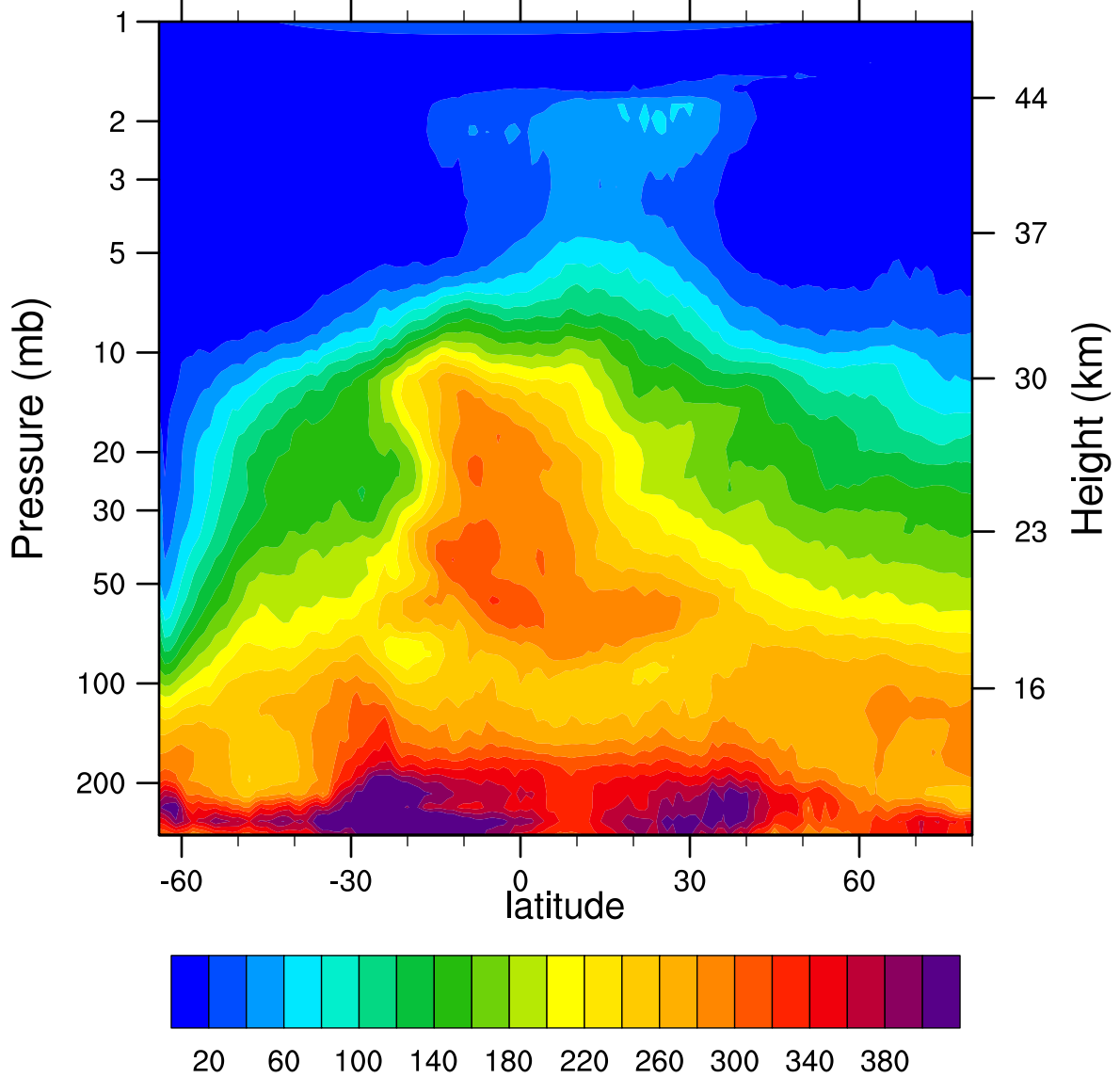
HIRDLSv6 2005d236 N2O_Combined (ppbv)
