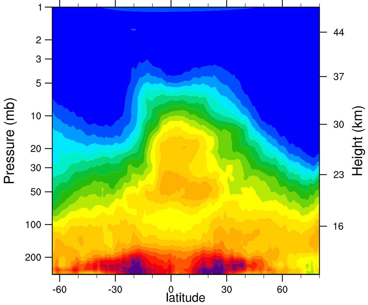
HIRDLSv6 2006d320 N2O_Combined (ppbv)
