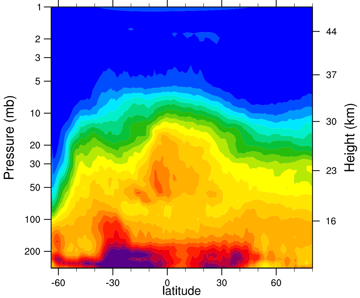
HIRDLSv6 2006d202 N2O_Combined (ppbv)
