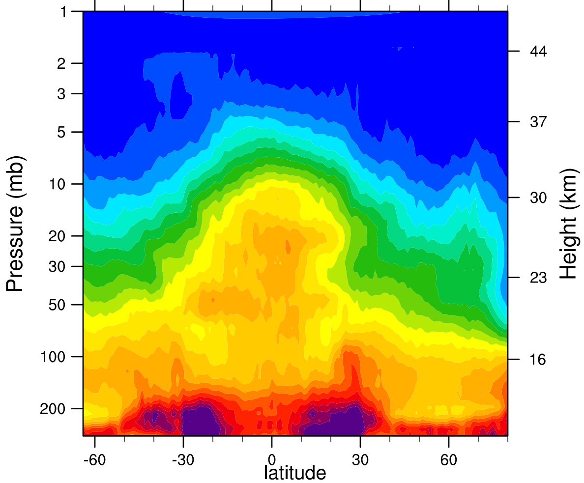
HIRDLSv6 2007d061 N2O_Combined (ppbv)
