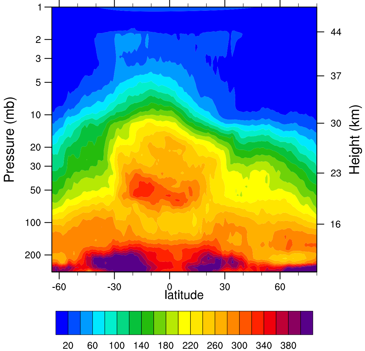
HIRDLSv6 2006d109 N2O_Combined (ppbv)
