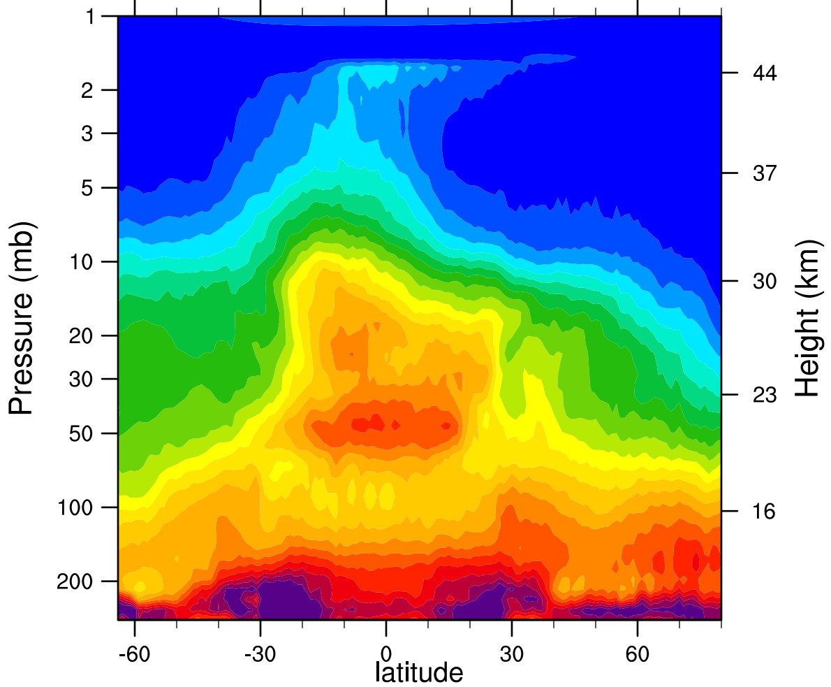
HIRDLSv6 2005d359 N2O_Combined (ppbv)
