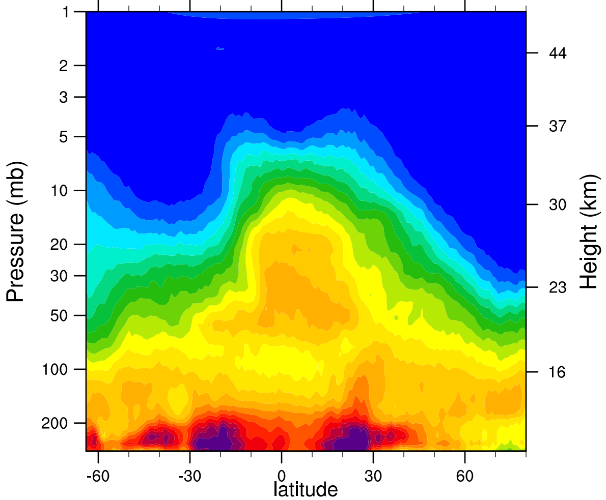
HIRDLSv6 2006d325 N2O_Combined (ppbv)
