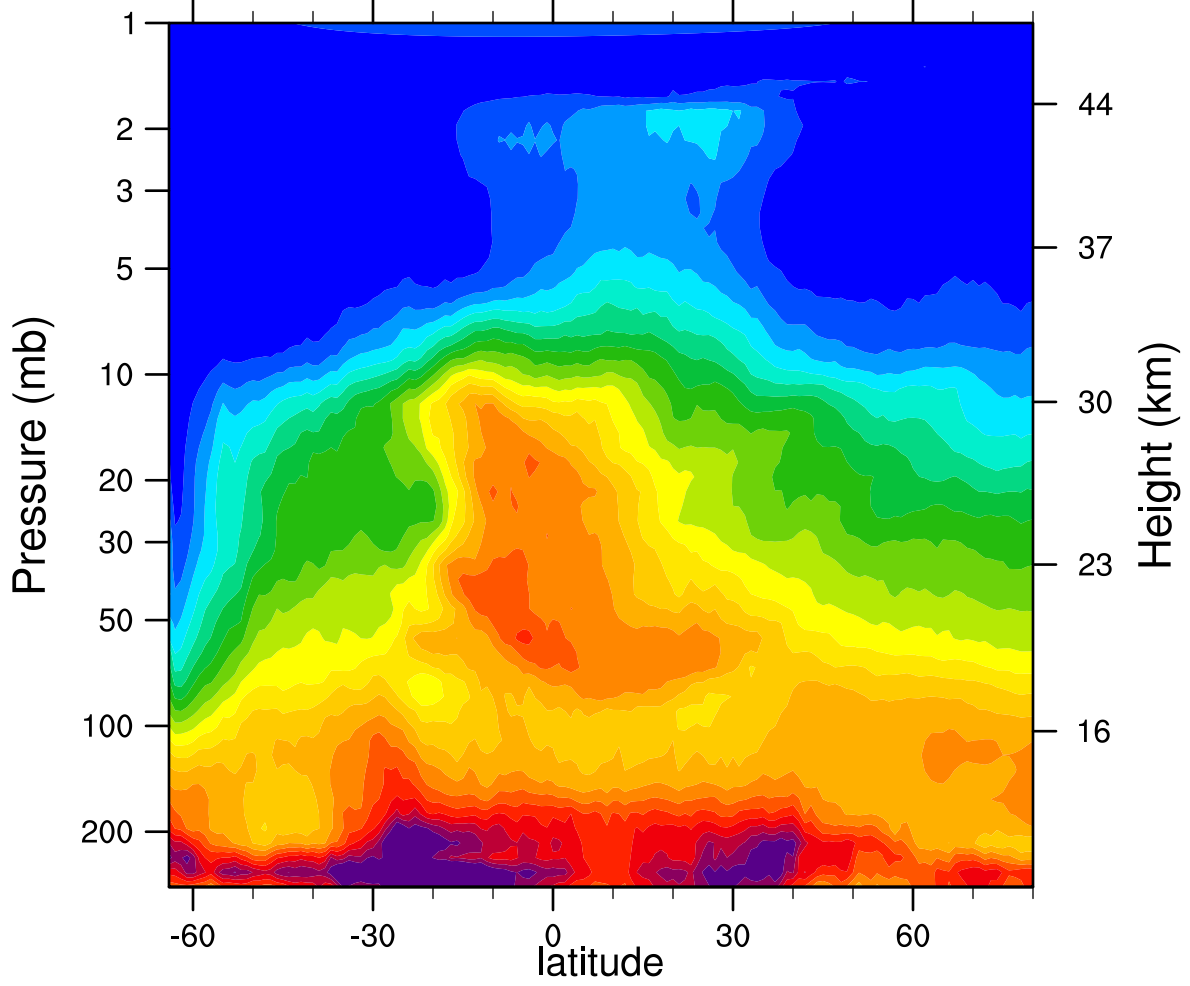
HIRDLSv6 2005d234 N2O_Combined (ppbv)
