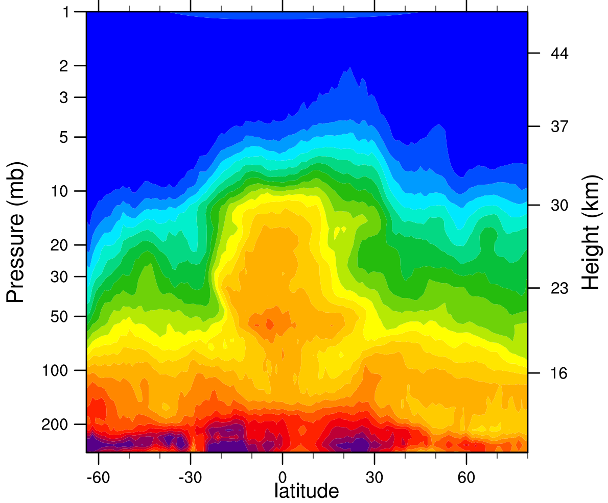
HIRDLSv6 2007d156 N2O_Combined (ppbv)
