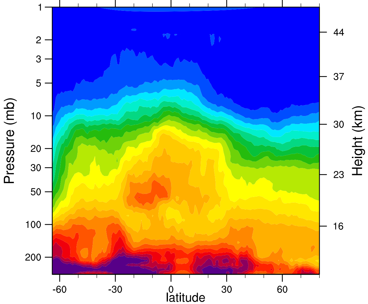
HIRDLSv6 2006d165 N2O_Combined (ppbv)
