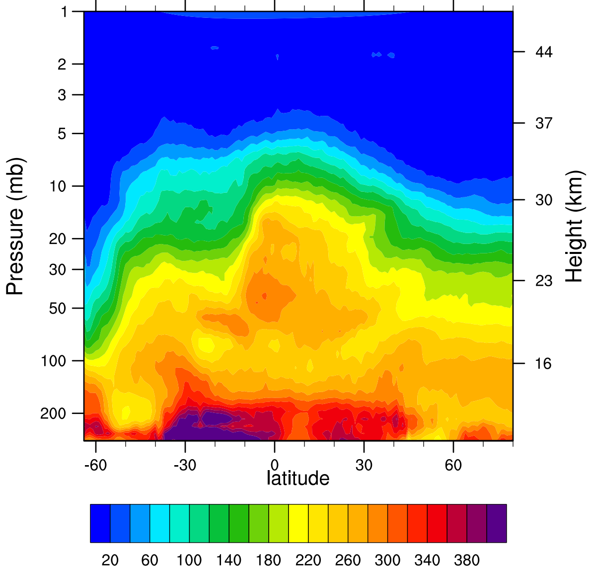
HIRDLSv6 2006d234 N2O_Combined (ppbv)
