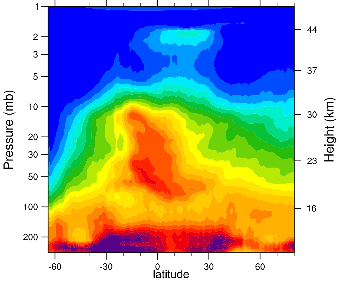
HIRDLSv6 2005d209 N2O_Combined (ppbv)
