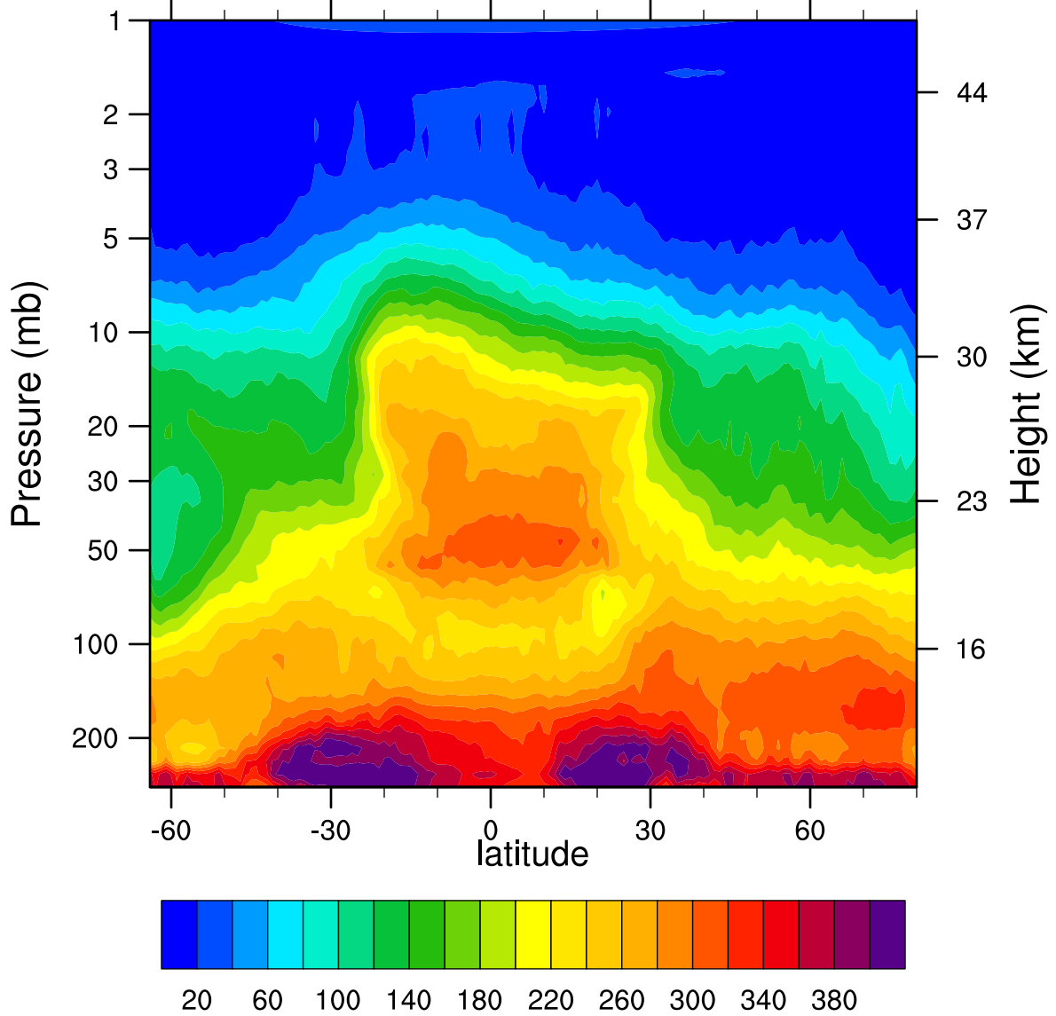
HIRDLSv6 2005d329 N2O_Combined (ppbv)
