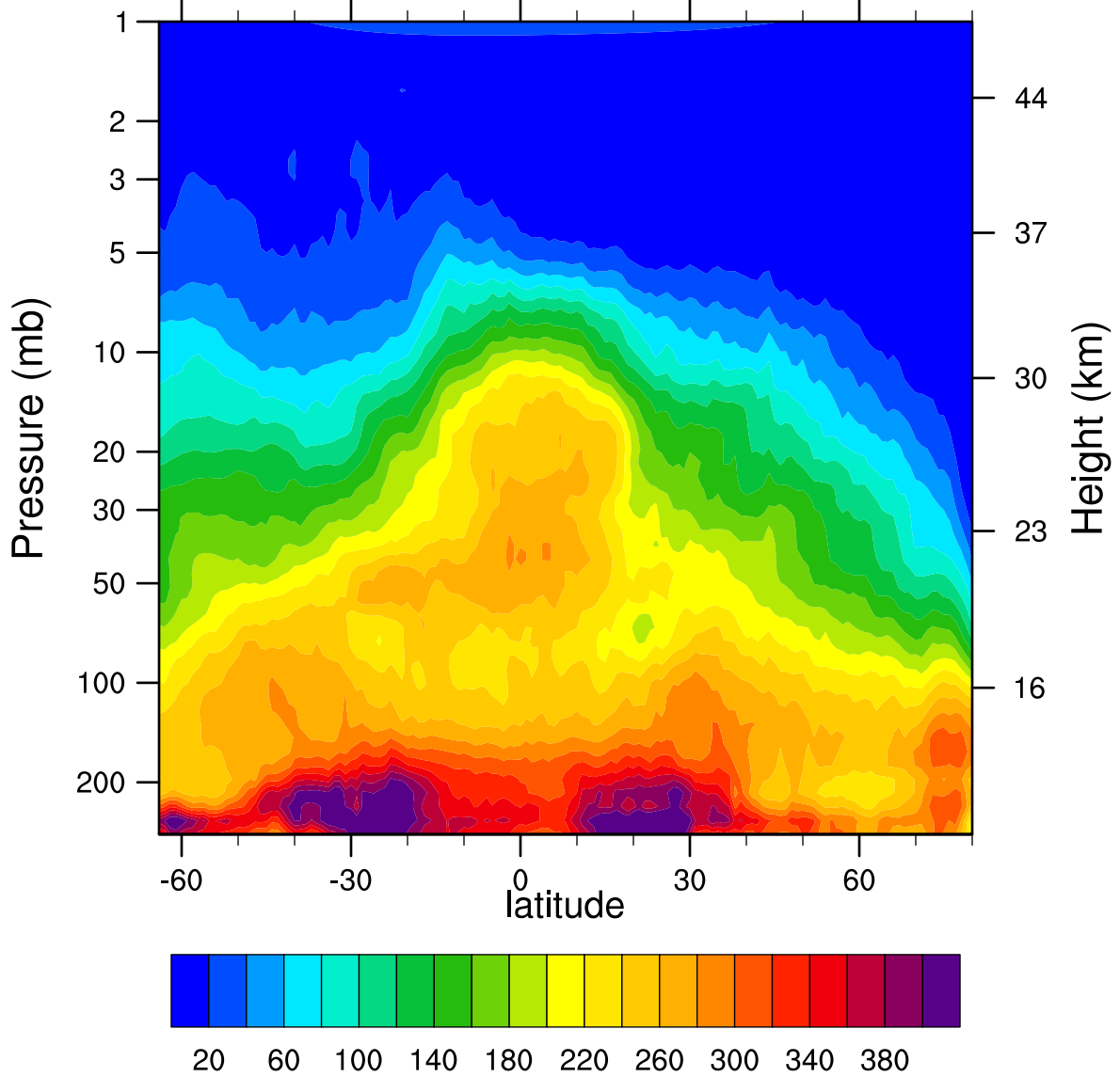
HIRDLSv6 2006d362 N2O_Combined (ppbv)
