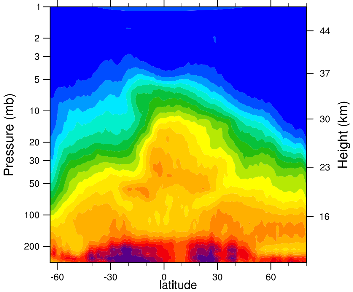
HIRDLSv6 2006d284 N2O_Combined (ppbv)
