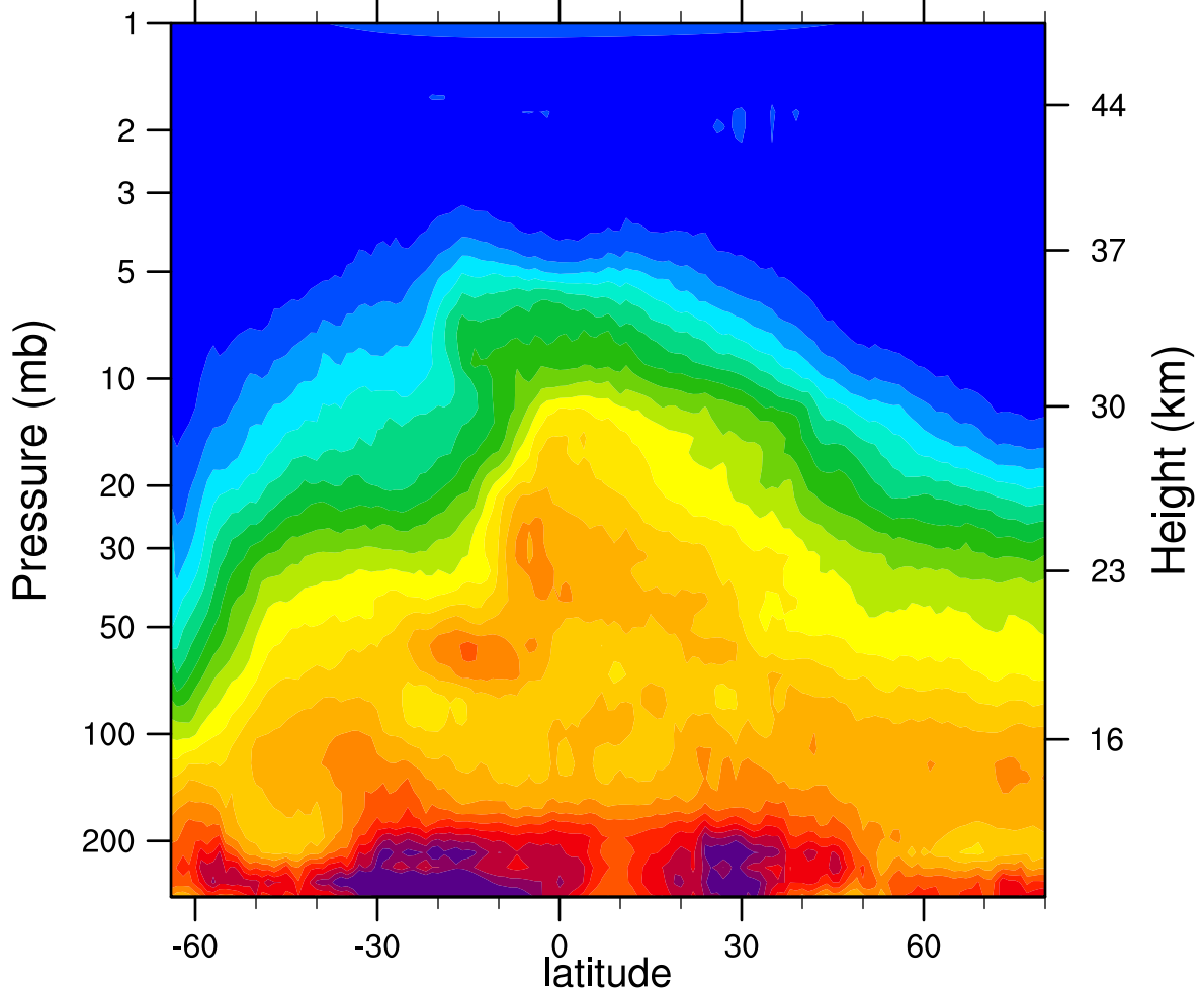
HIRDLSv6 2006d266 N2O_Combined (ppbv)
