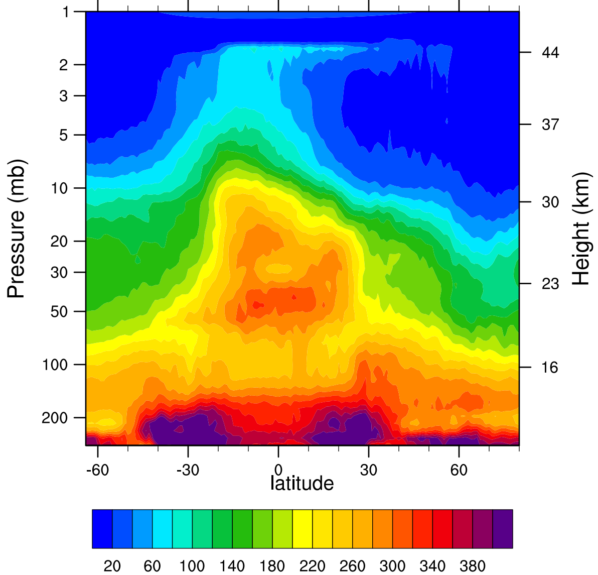
HIRDLSv6 2006d017 N2O_Combined (ppbv)
