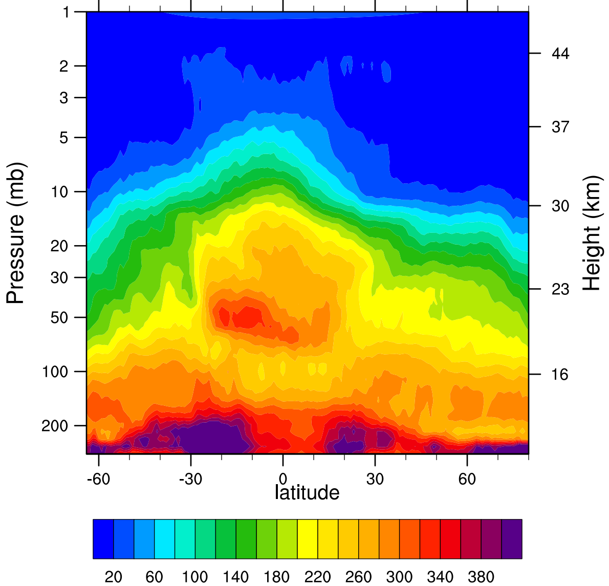
HIRDLSv6 2006d121 N2O_Combined (ppbv)
