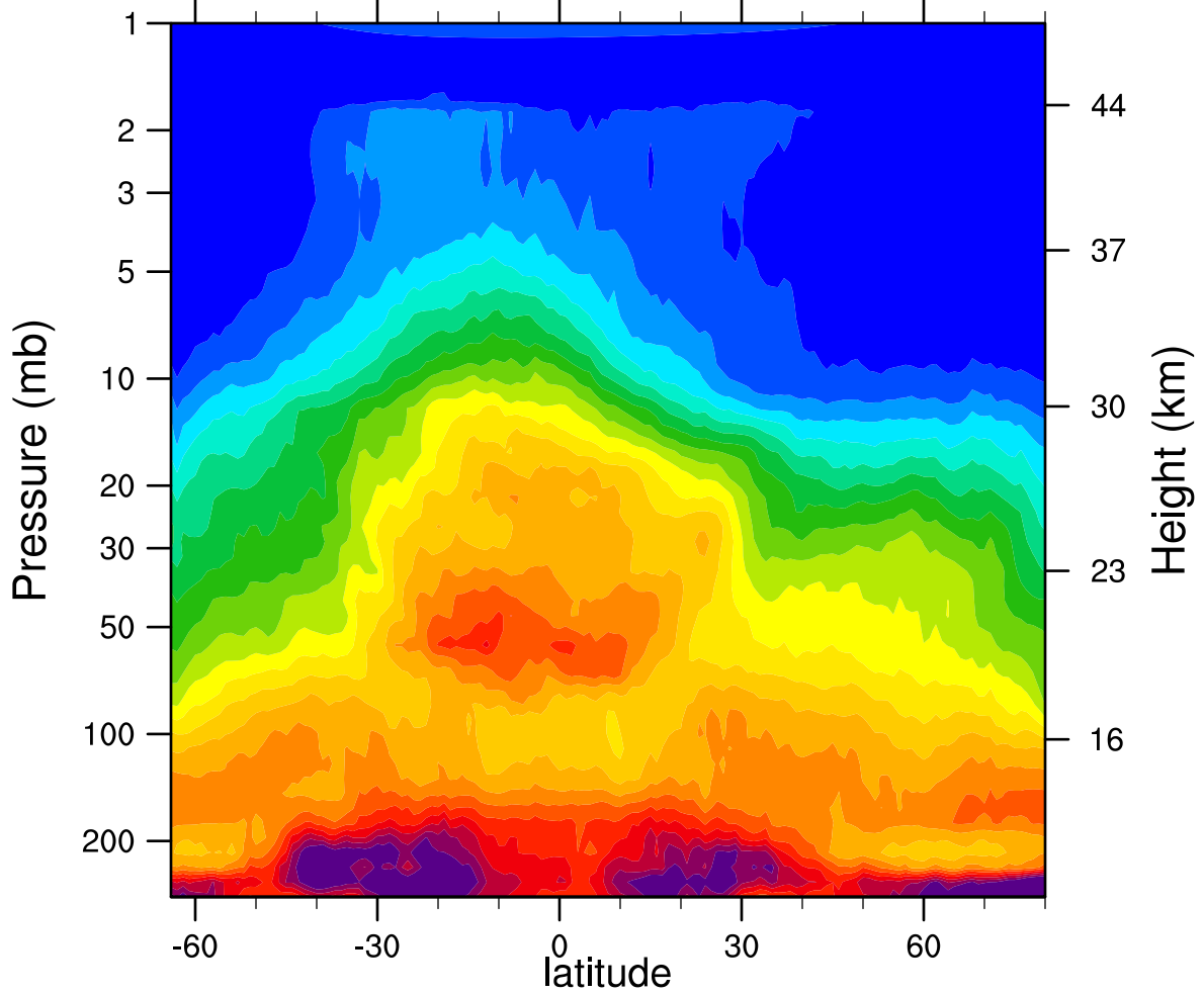
HIRDLSv6 2006d100 N2O_Combined (ppbv)
