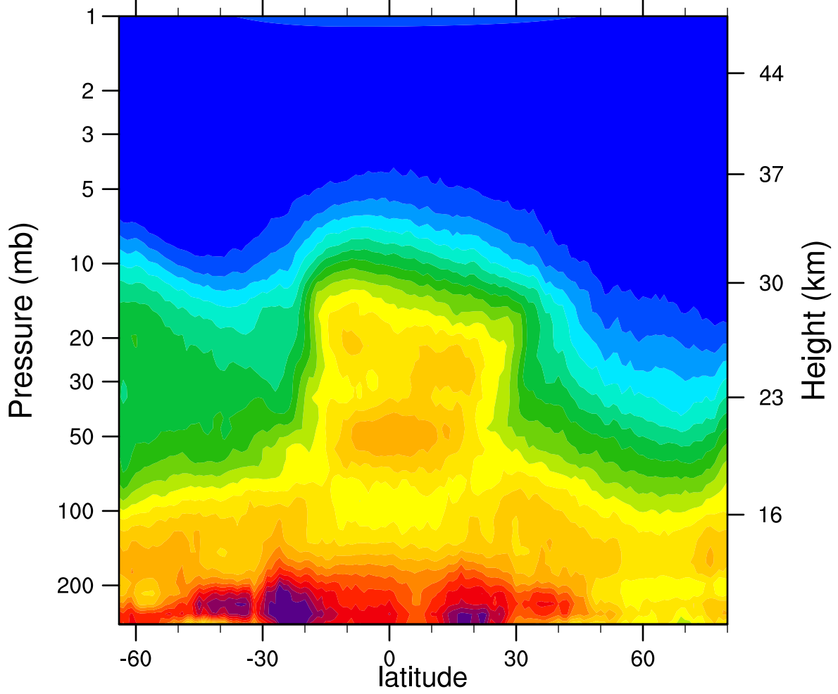
HIRDLSv6 2007d330 N2O_Combined (ppbv)
