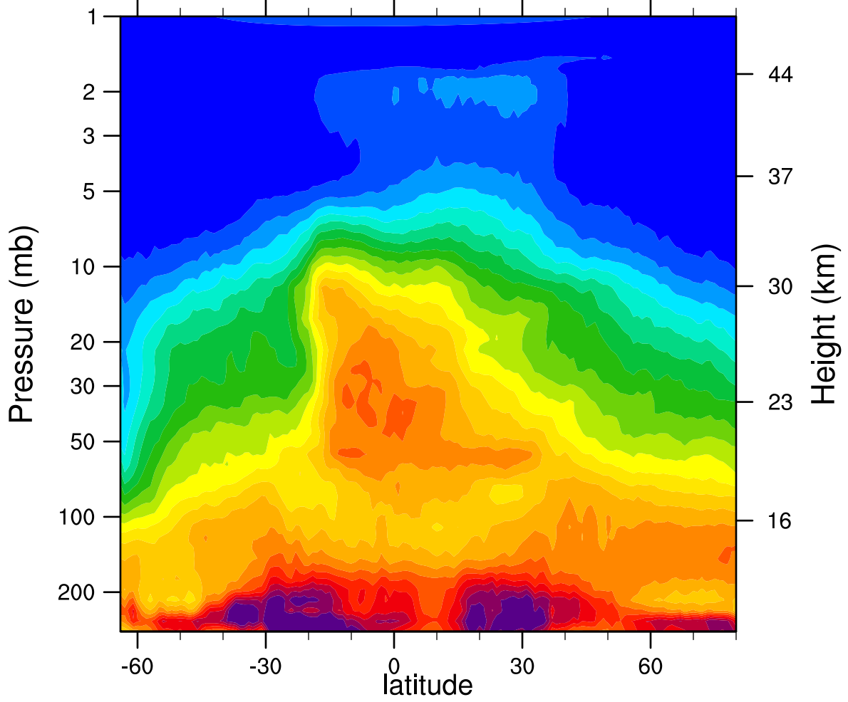
HIRDLSv6 2005d275 N2O_Combined (ppbv)
