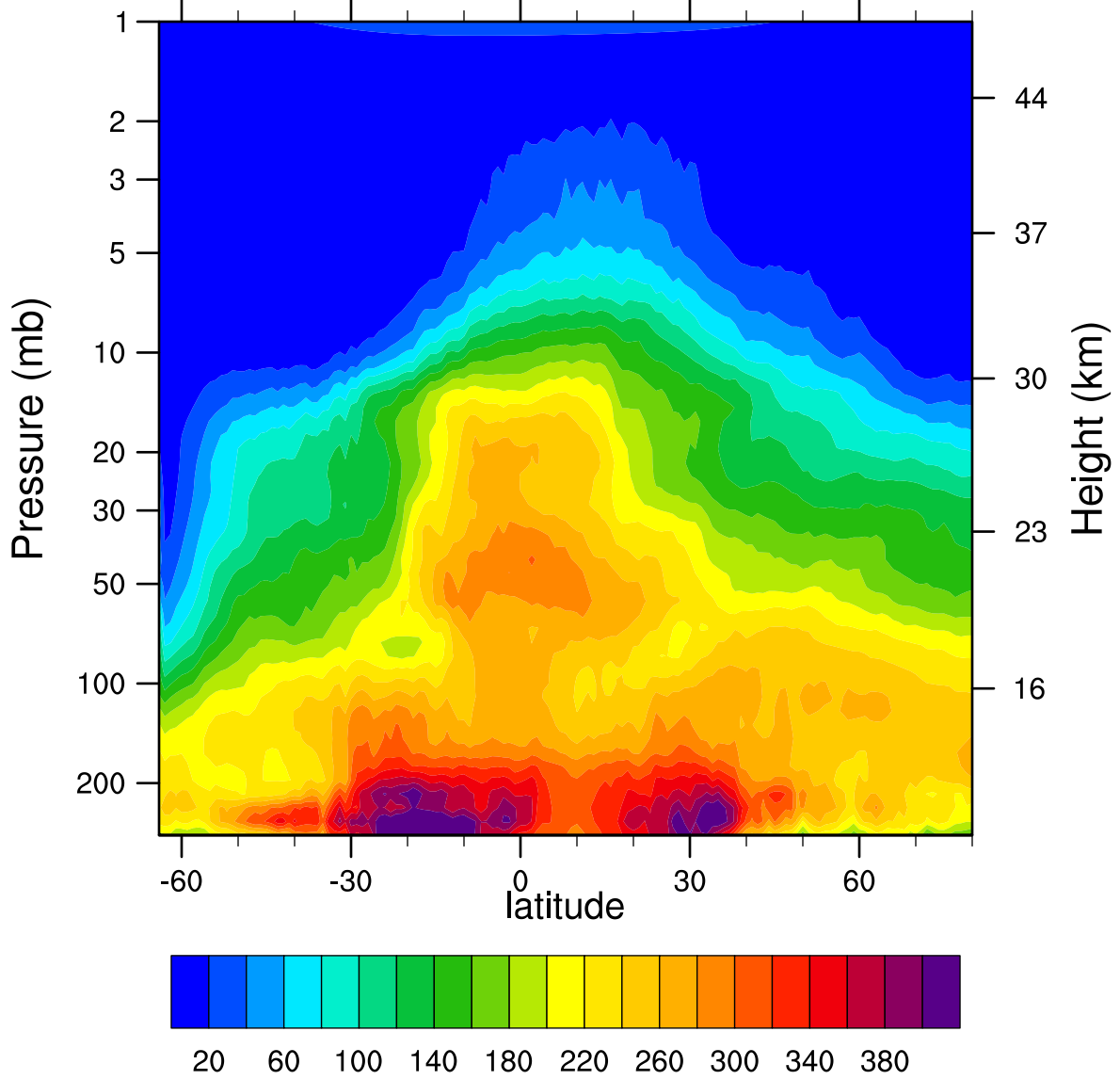
HIRDLSv6 2007d229 N2O_Combined (ppbv)
