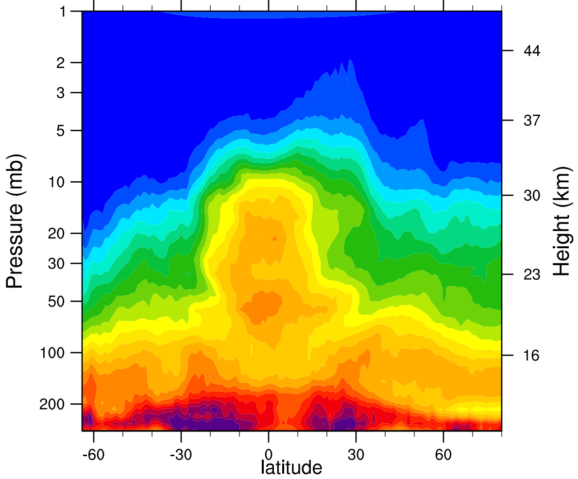
HIRDLSv6 2007d144 N2O_Combined (ppbv)
