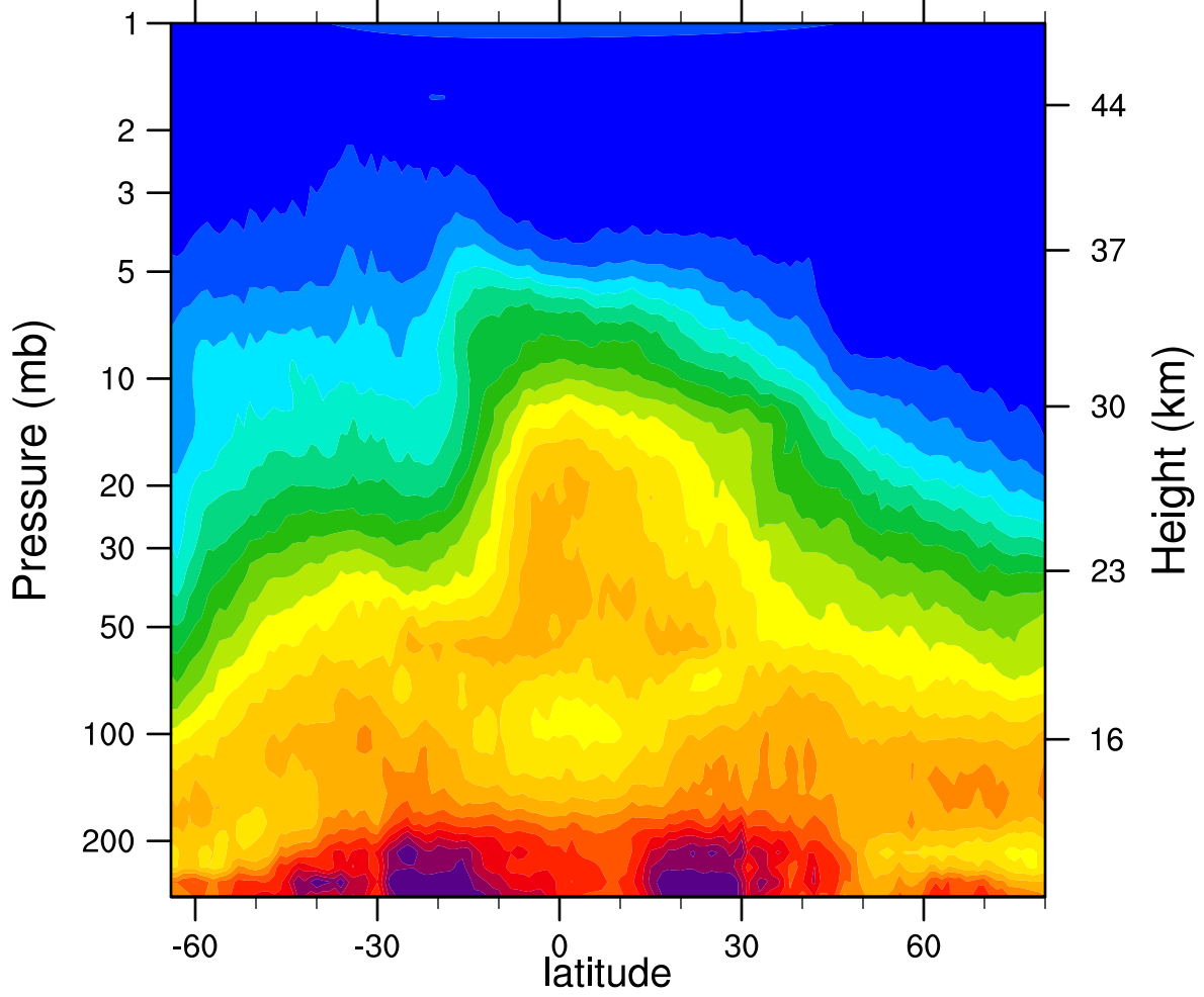
HIRDLSv6 2006d299 N2O_Combined (ppbv)
