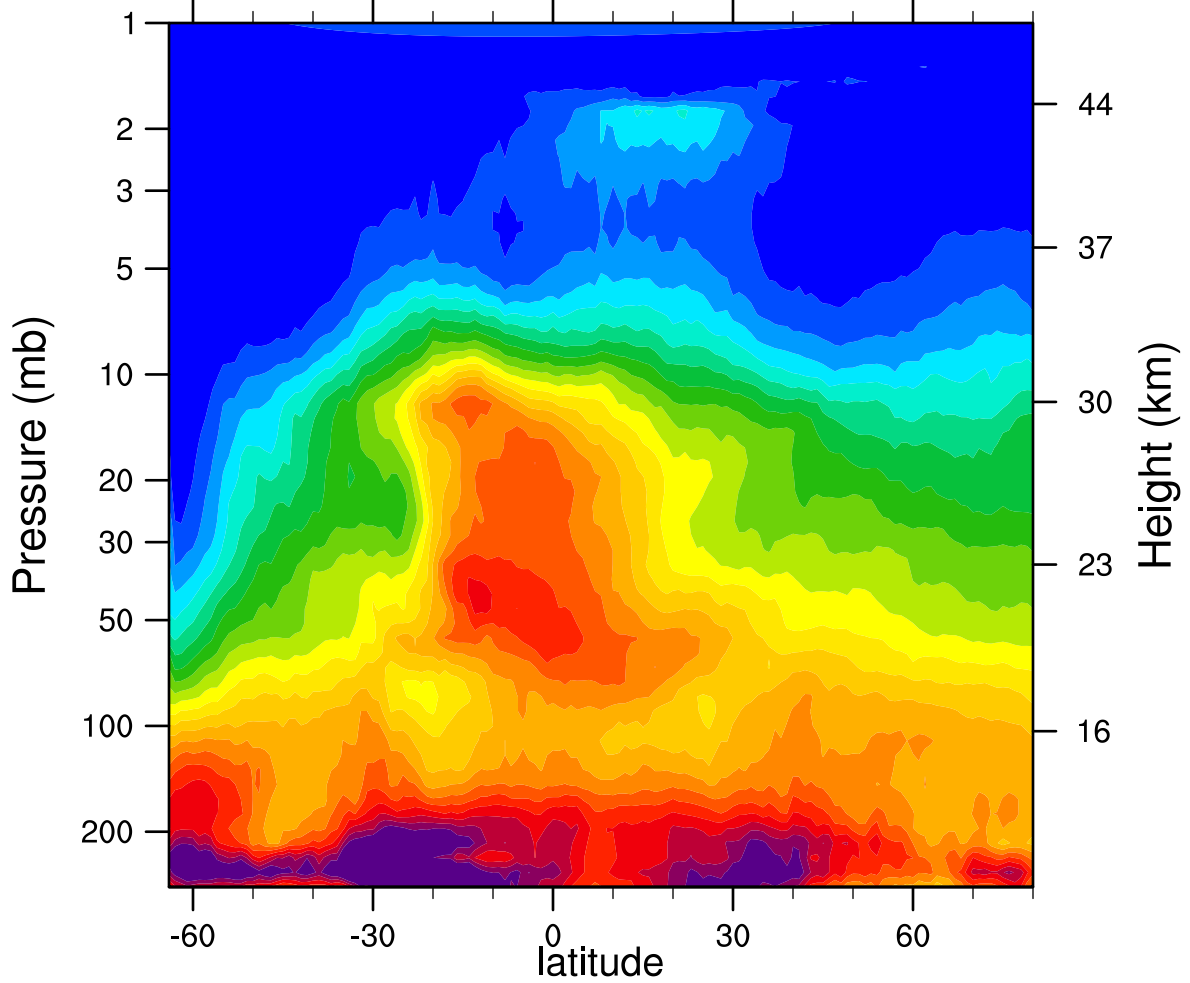
HIRDLSv6 2005d193 N2O_Combined (ppbv)
