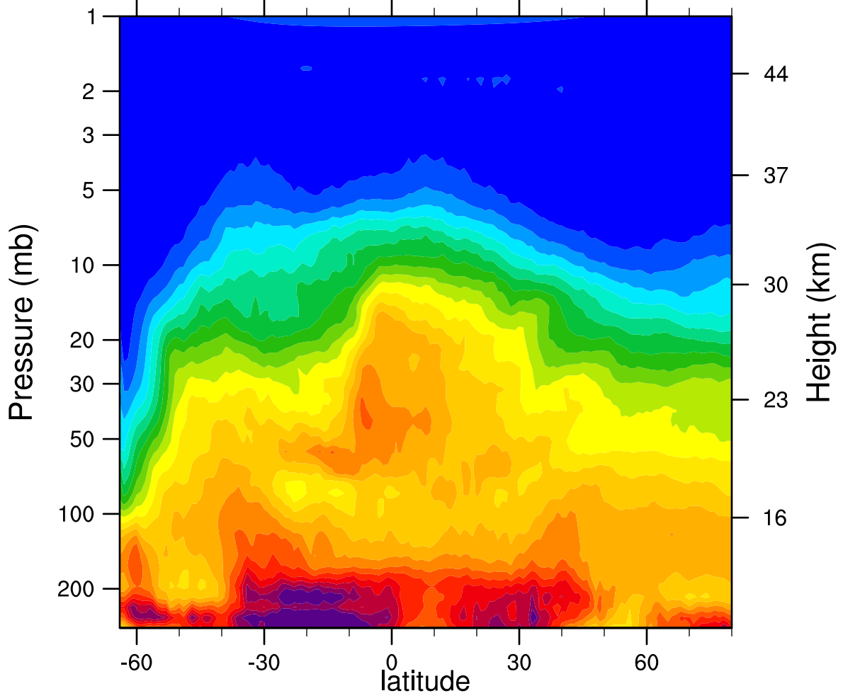
HIRDLSv6 2006d220 N2O_Combined (ppbv)
