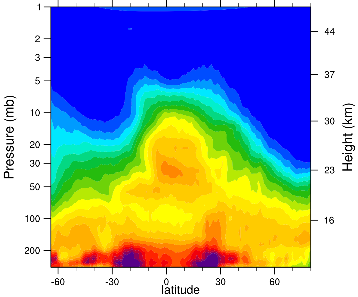
HIRDLSv6 2006d328 N2O_Combined (ppbv)
