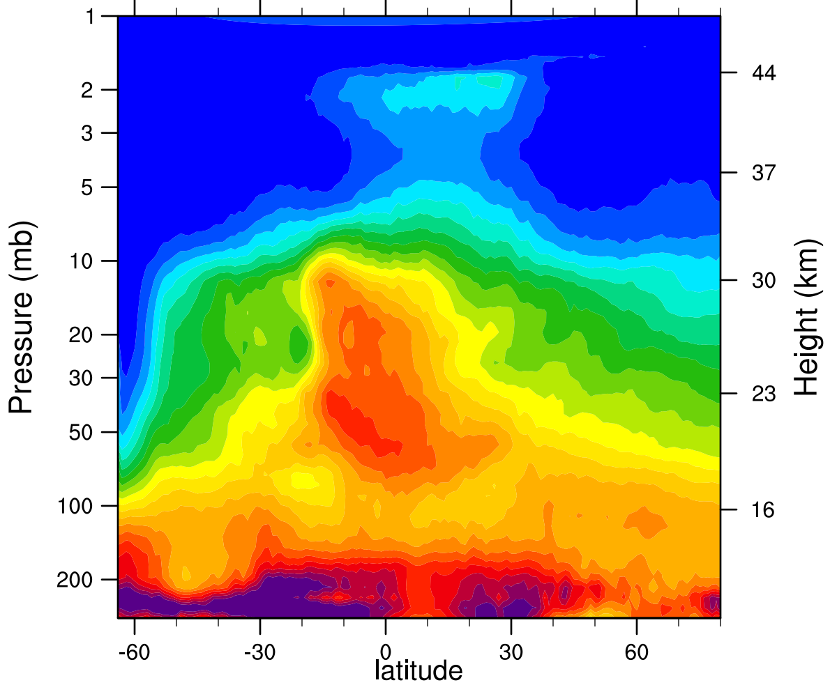
HIRDLSv6 2005d222 N2O_Combined (ppbv)
