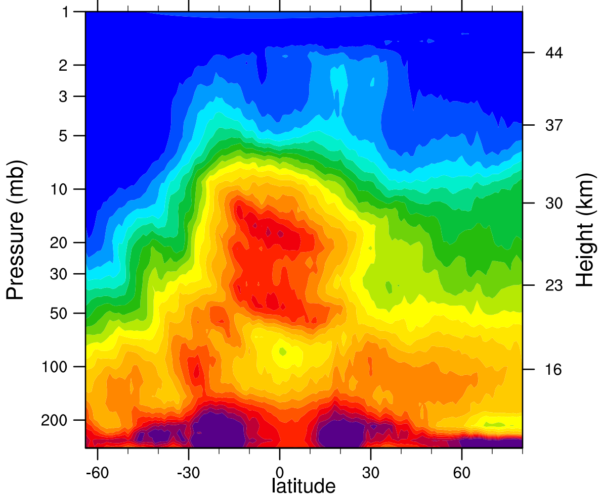
HIRDLSv6 2005d115 N2O_Combined (ppbv)
