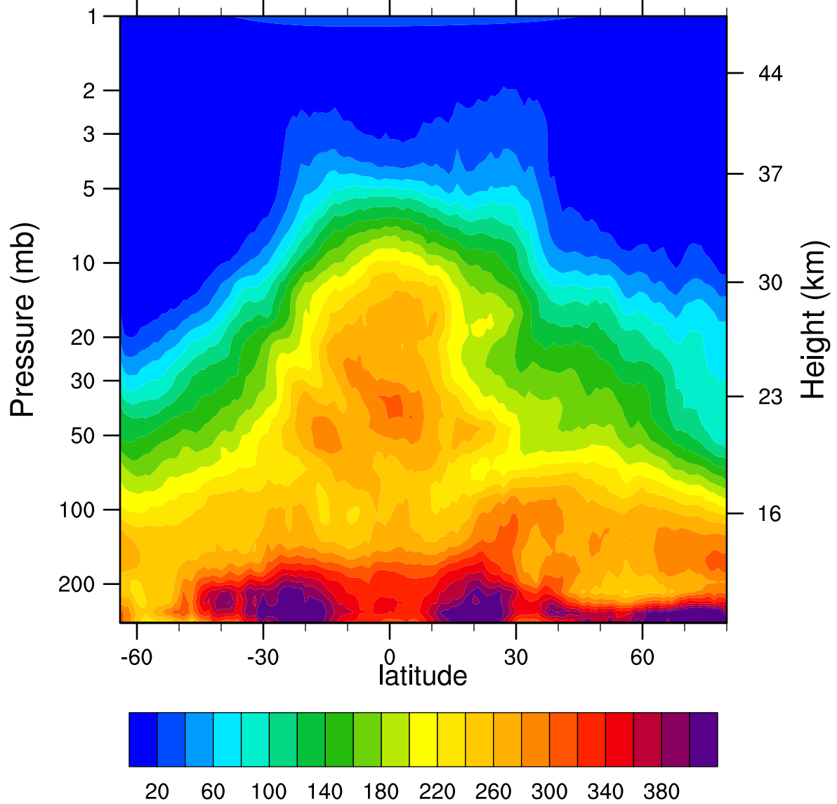
HIRDLSv6 2007d102 N2O_Combined (ppbv)
