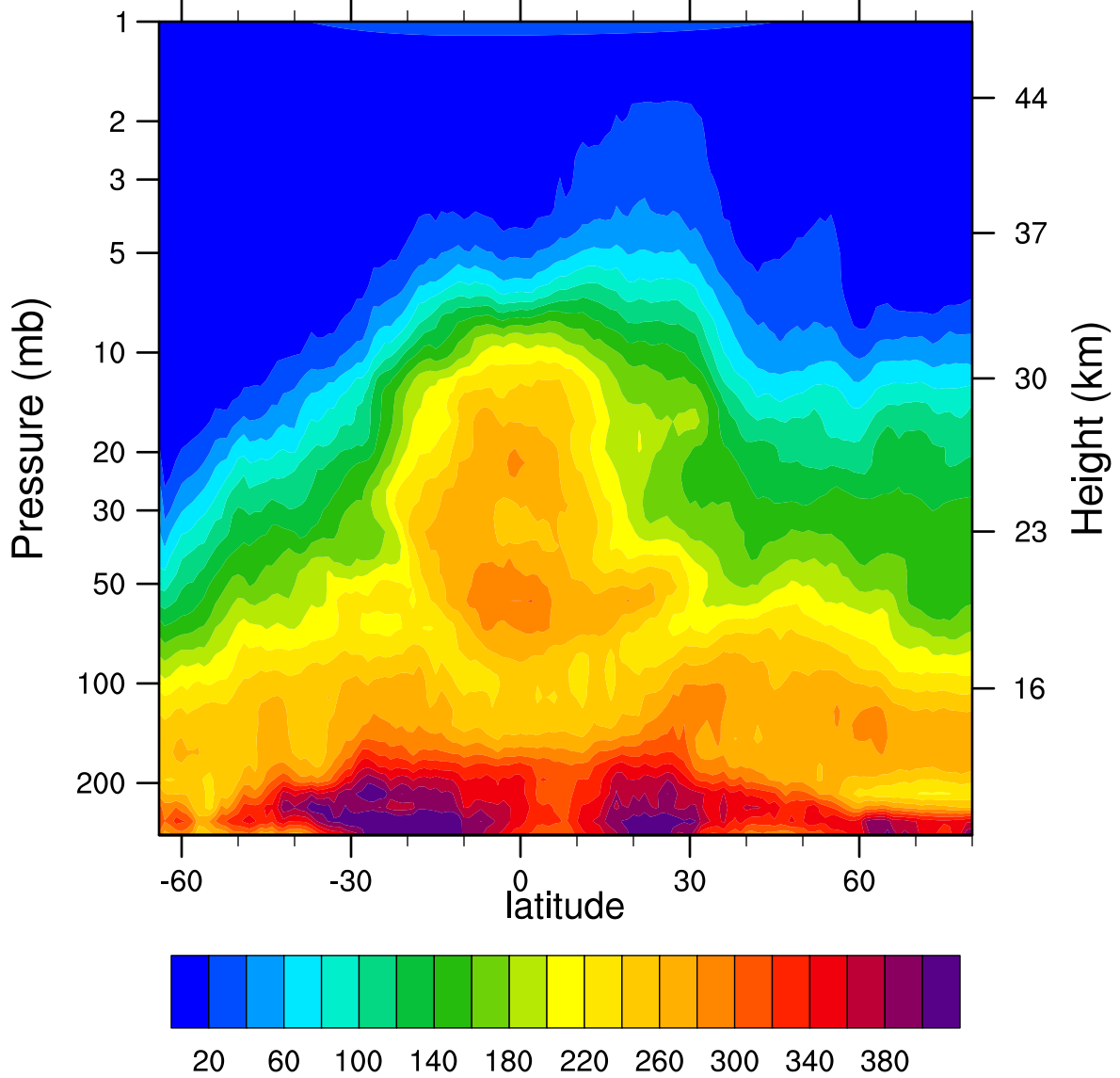
HIRDLSv6 2007d138 N2O_Combined (ppbv)
