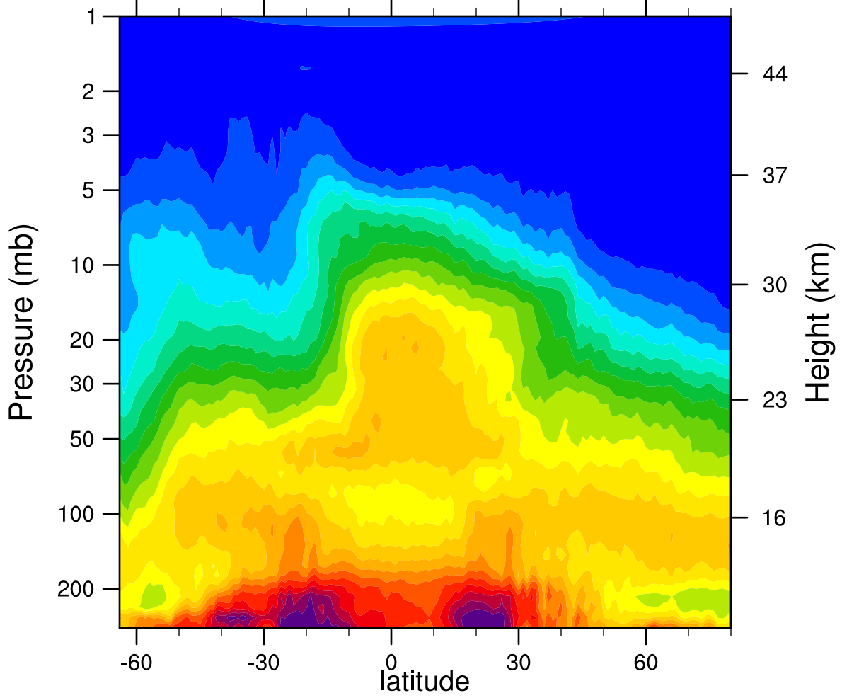
HIRDLSv6 2006d302 N2O_Combined (ppbv)
