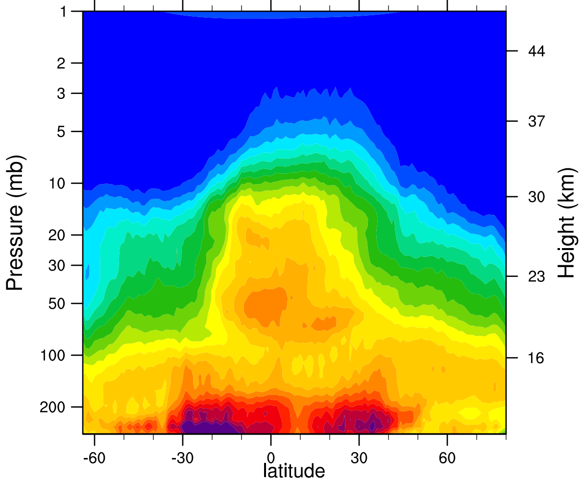
HIRDLSv6 2007d264 N2O_Combined (ppbv)
