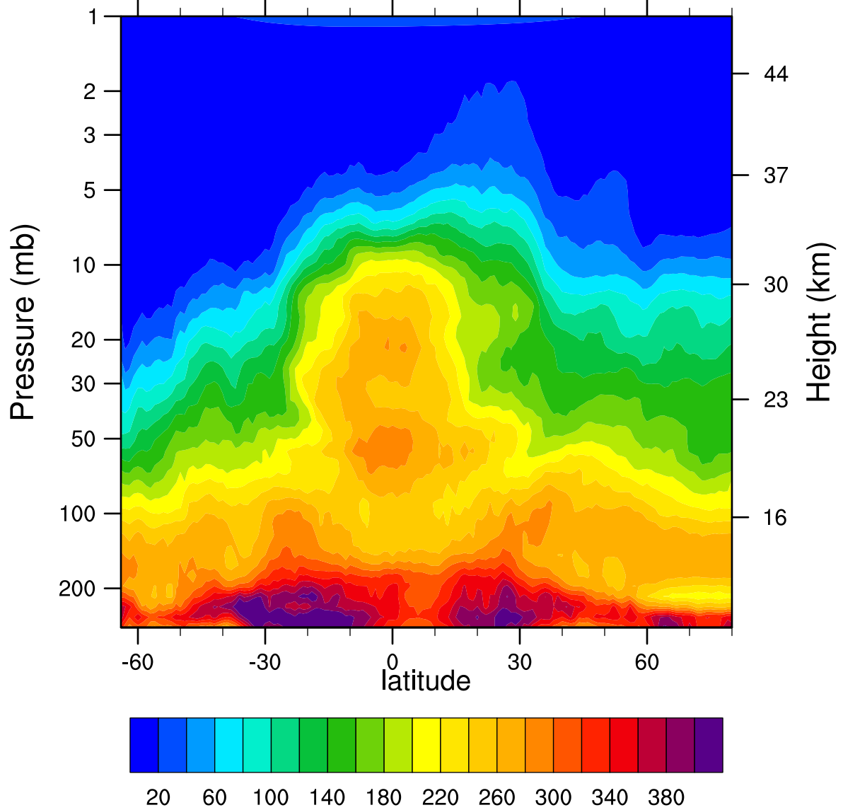
HIRDLSv6 2007d142 N2O_Combined (ppbv)
