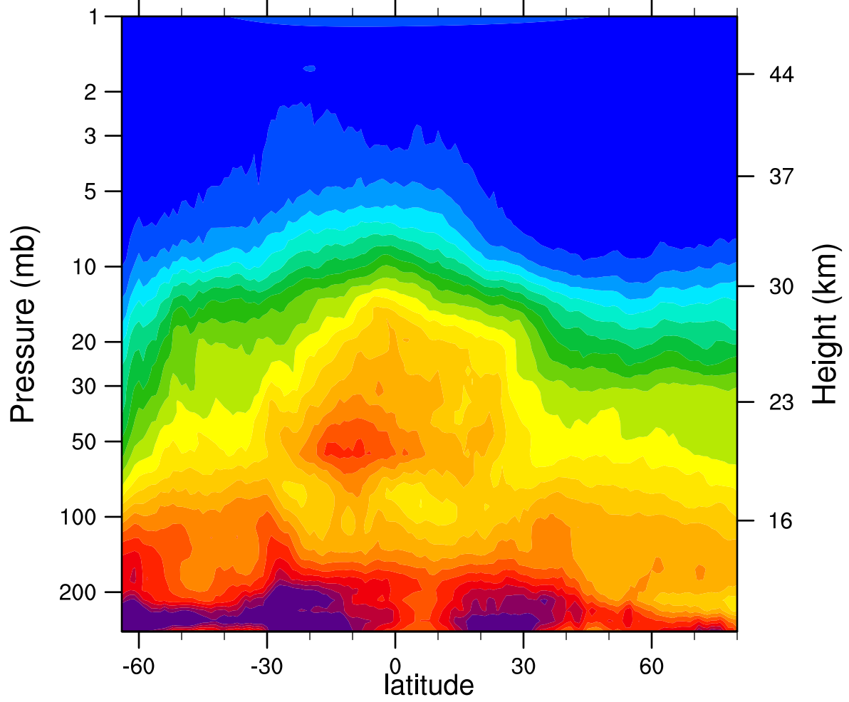
HIRDLSv6 2006d157 N2O_Combined (ppbv)
