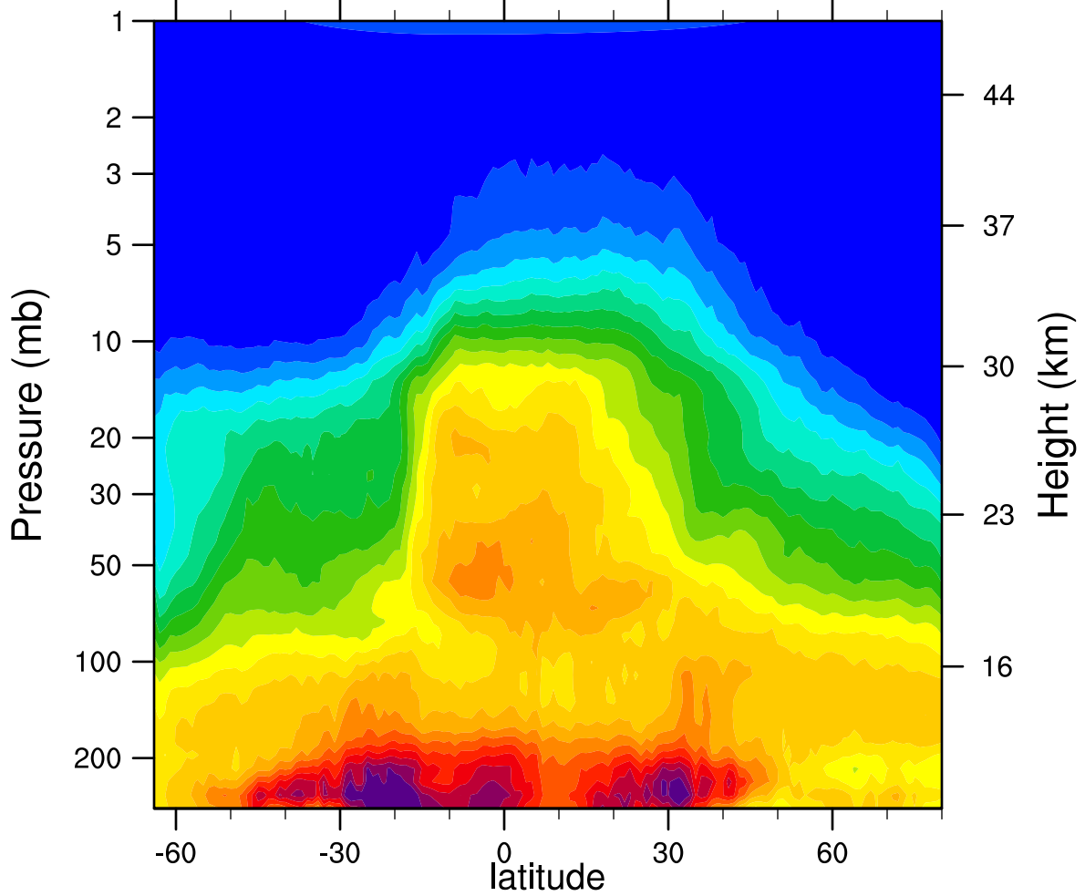
HIRDLSv6 2007d274 N2O_Combined (ppbv)
