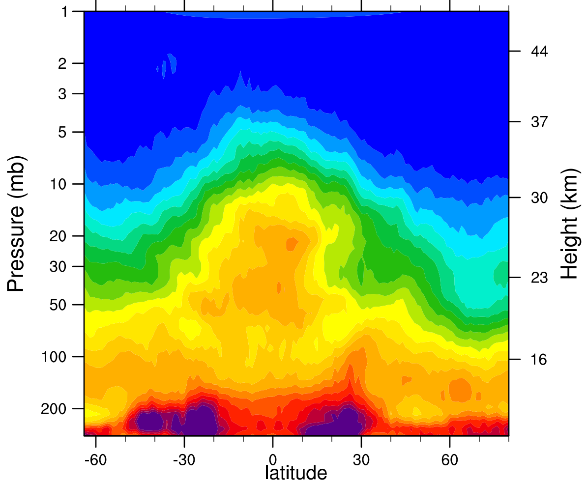
HIRDLSv6 2007d054 N2O_Combined (ppbv)
