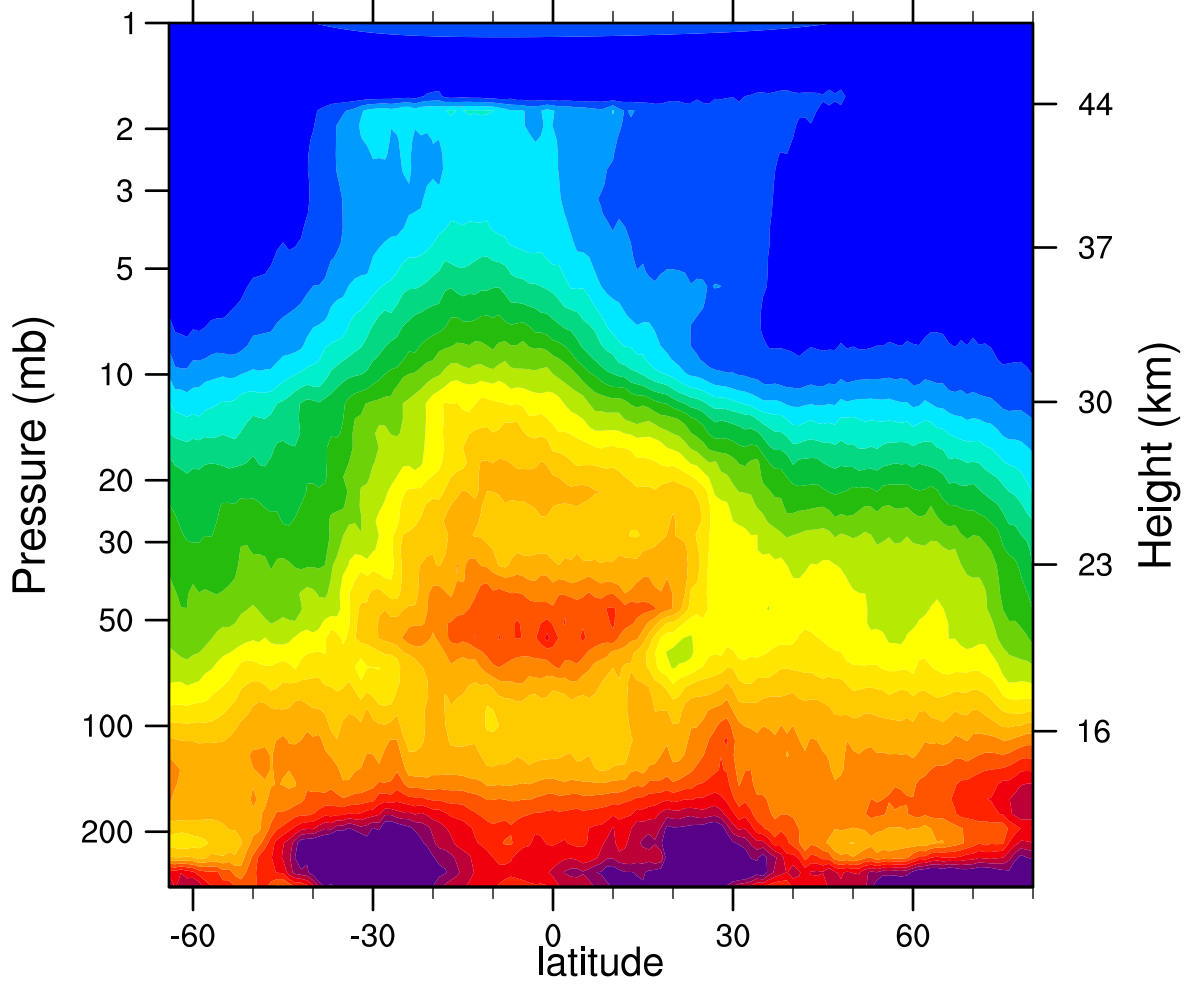
HIRDLSv6 2006d069 N2O_Combined (ppbv)
