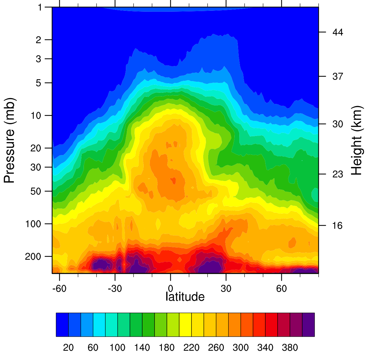
HIRDLSv6 2007d114 N2O_Combined (ppbv)
