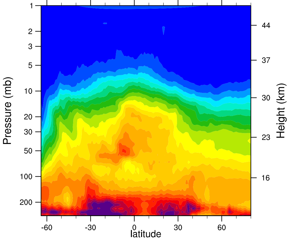
HIRDLSv6 2006d176 N2O_Combined (ppbv)
