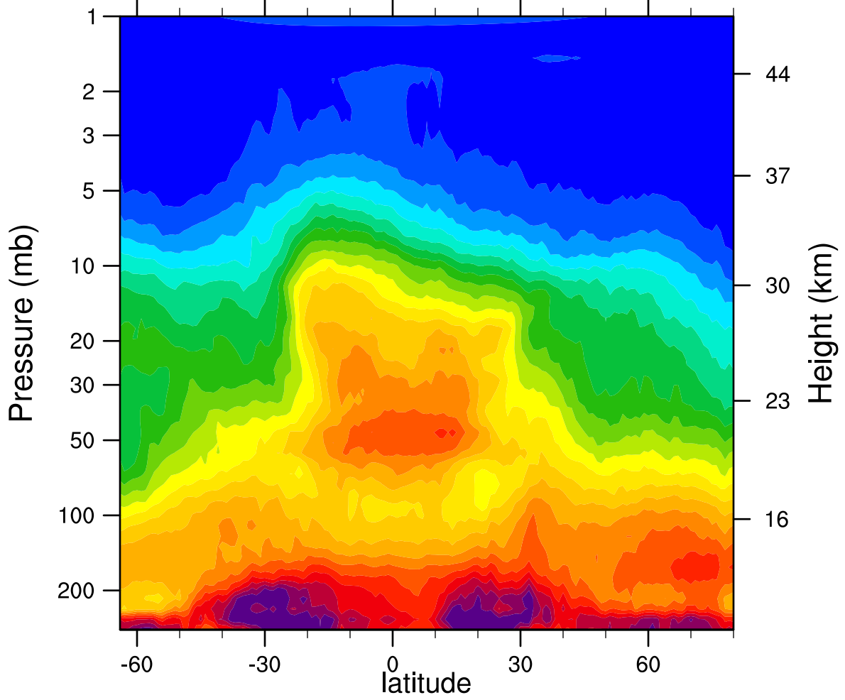
HIRDLSv6 2005d332 N2O_Combined (ppbv)
