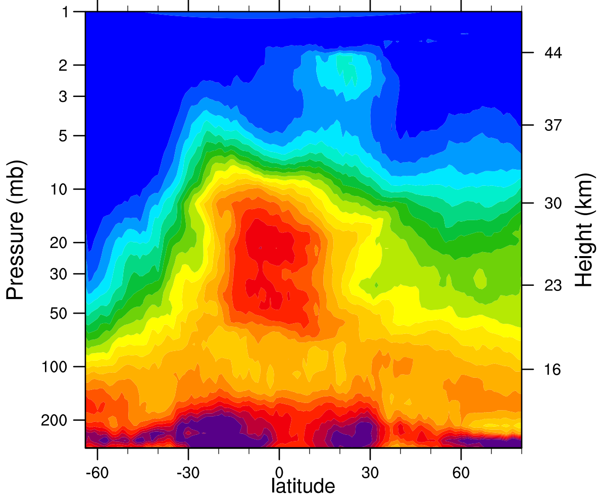
HIRDLSv6 2005d150 N2O_Combined (ppbv)
