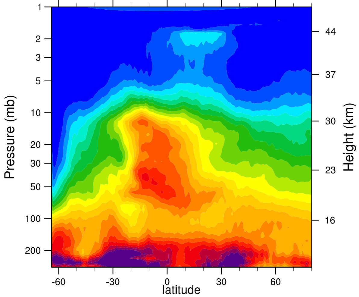
HIRDLSv6 2005d197 N2O_Combined (ppbv)
