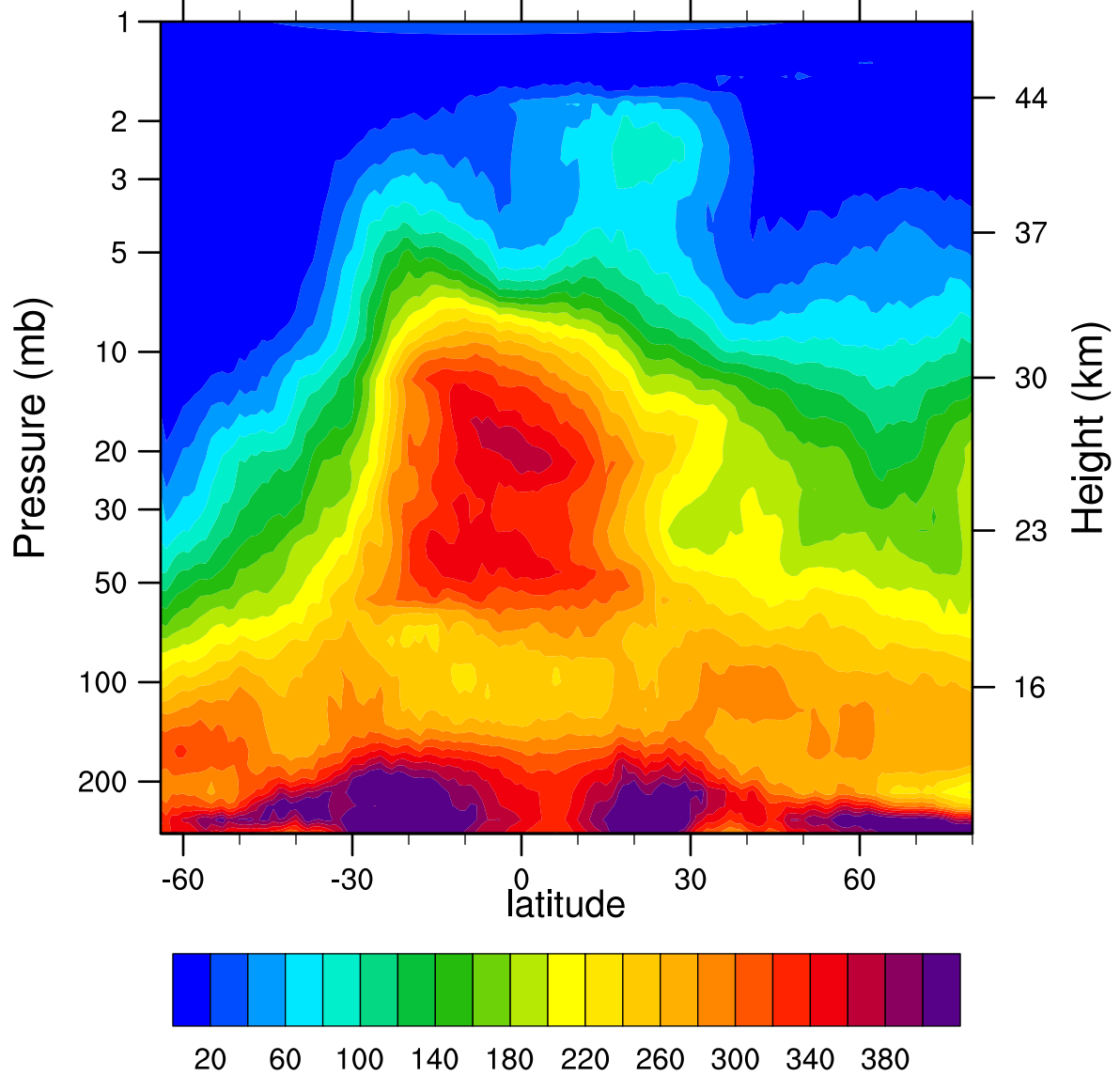
HIRDLSv6 2005d130 N2O_Combined (ppbv)
