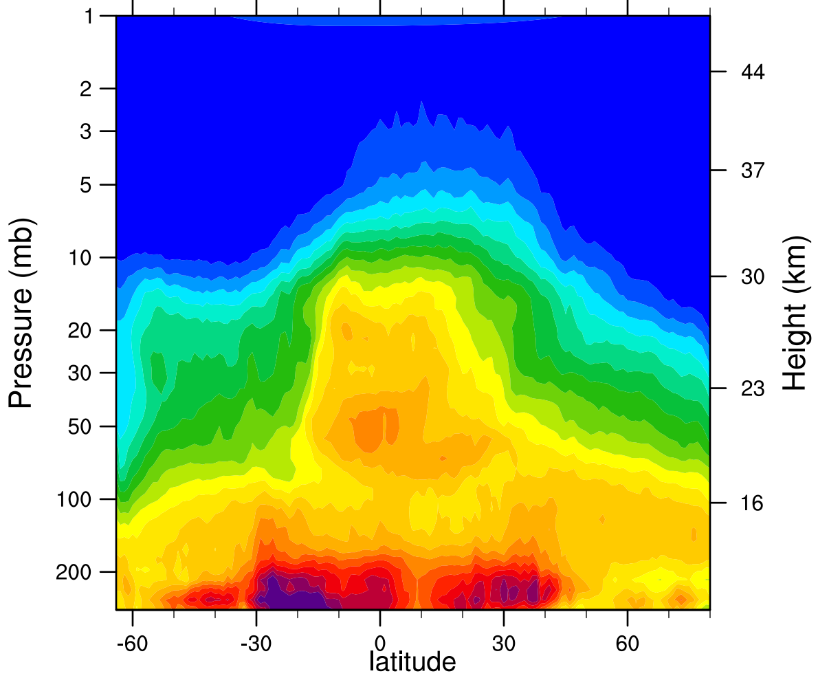
HIRDLSv6 2007d268 N2O_Combined (ppbv)
