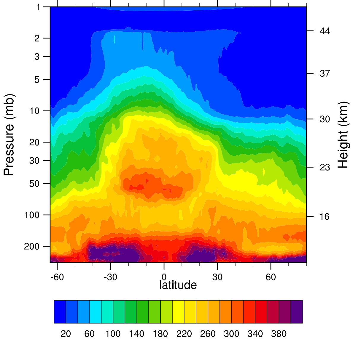
HIRDLSv6 2006d098 N2O_Combined (ppbv)
