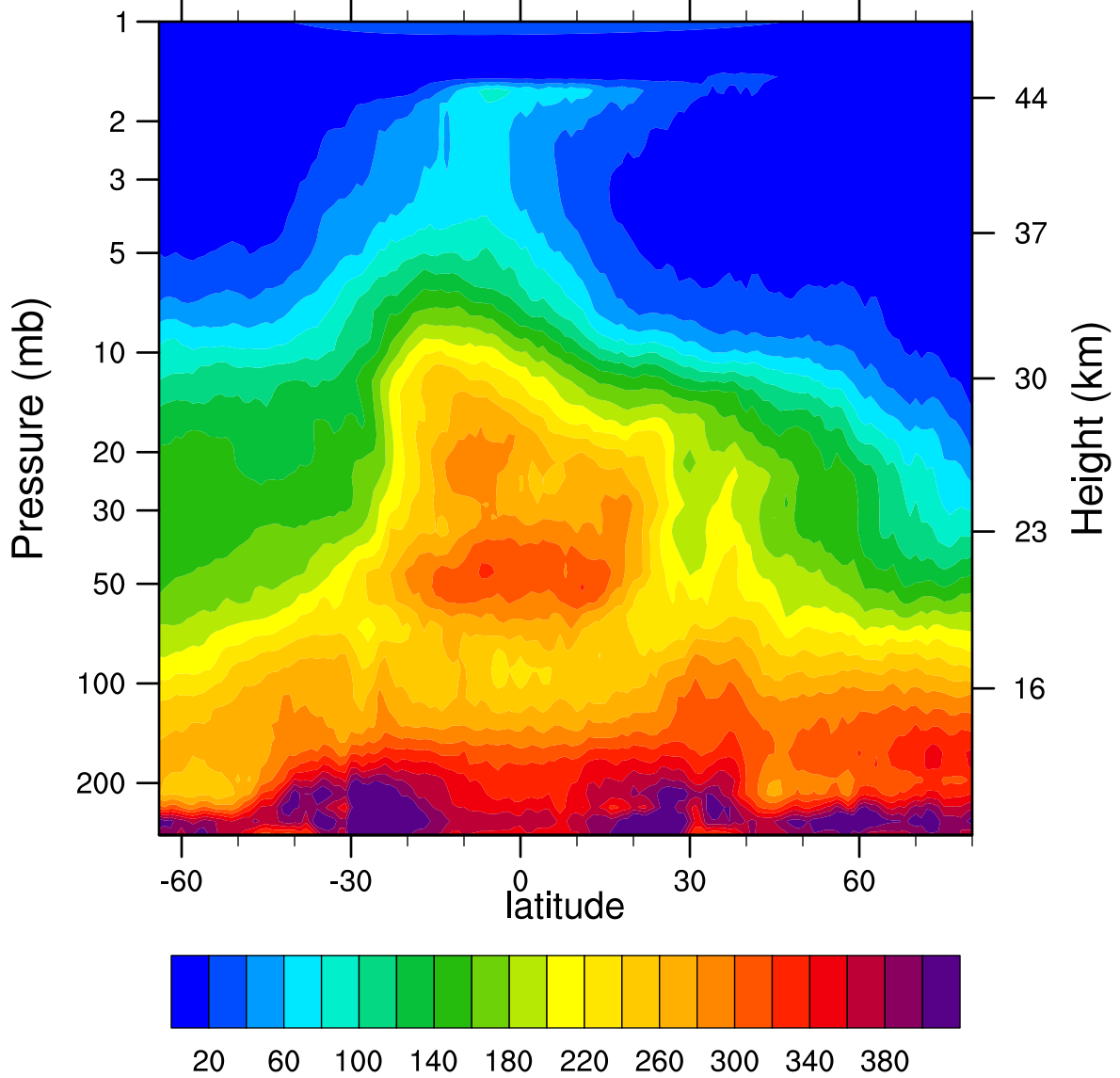
HIRDLSv6 2005d362 N2O_Combined (ppbv)
