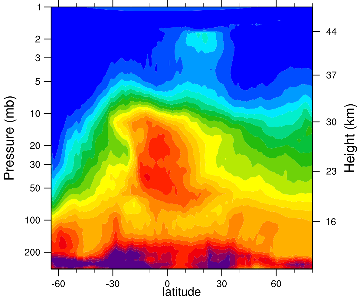
HIRDLSv6 2005d180 N2O_Combined (ppbv)
