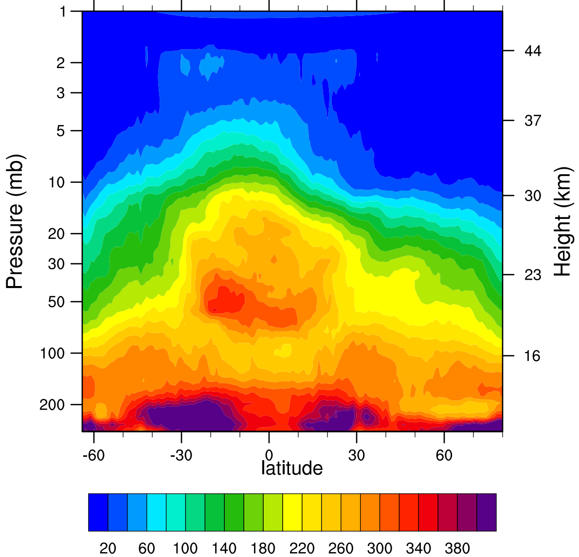
HIRDLSv6 2006d112 N2O_Combined (ppbv)
