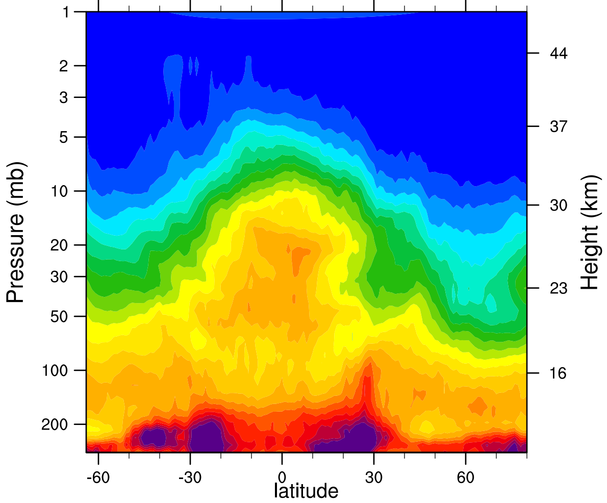
HIRDLSv6 2007d056 N2O_Combined (ppbv)
