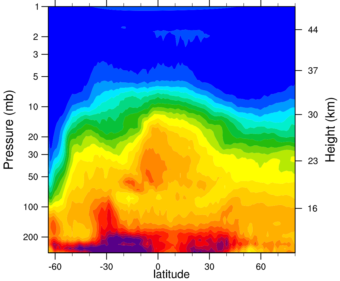
HIRDLSv6 2006d205 N2O_Combined (ppbv)
