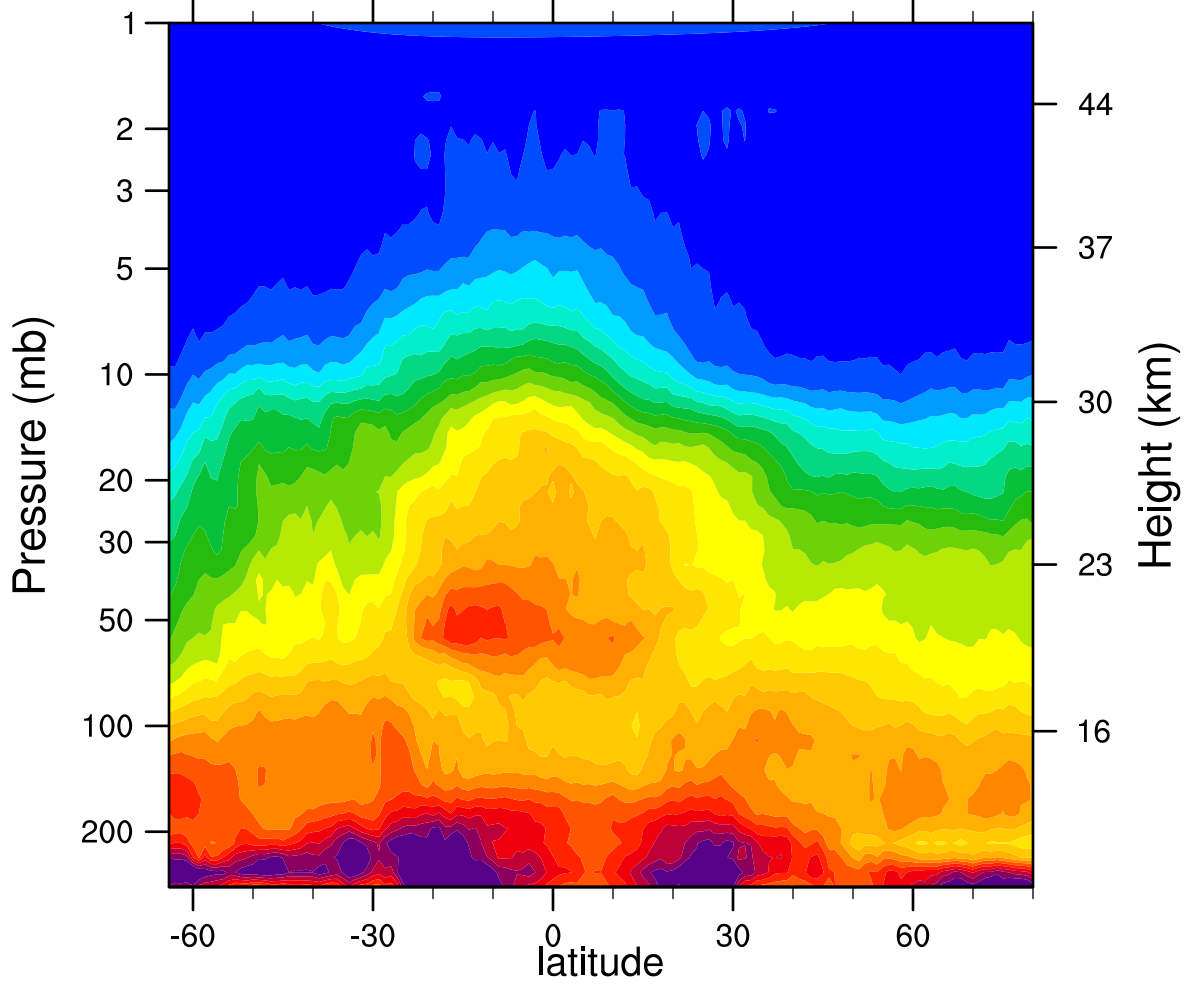
HIRDLSv6 2006d140 N2O_Combined (ppbv)
