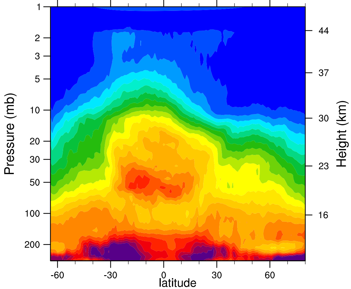
HIRDLSv6 2006d108 N2O_Combined (ppbv)
