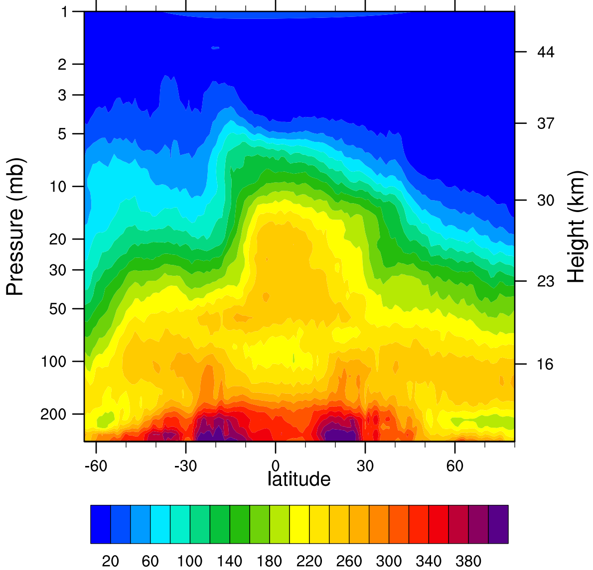
HIRDLSv6 2006d301 N2O_Combined (ppbv)
