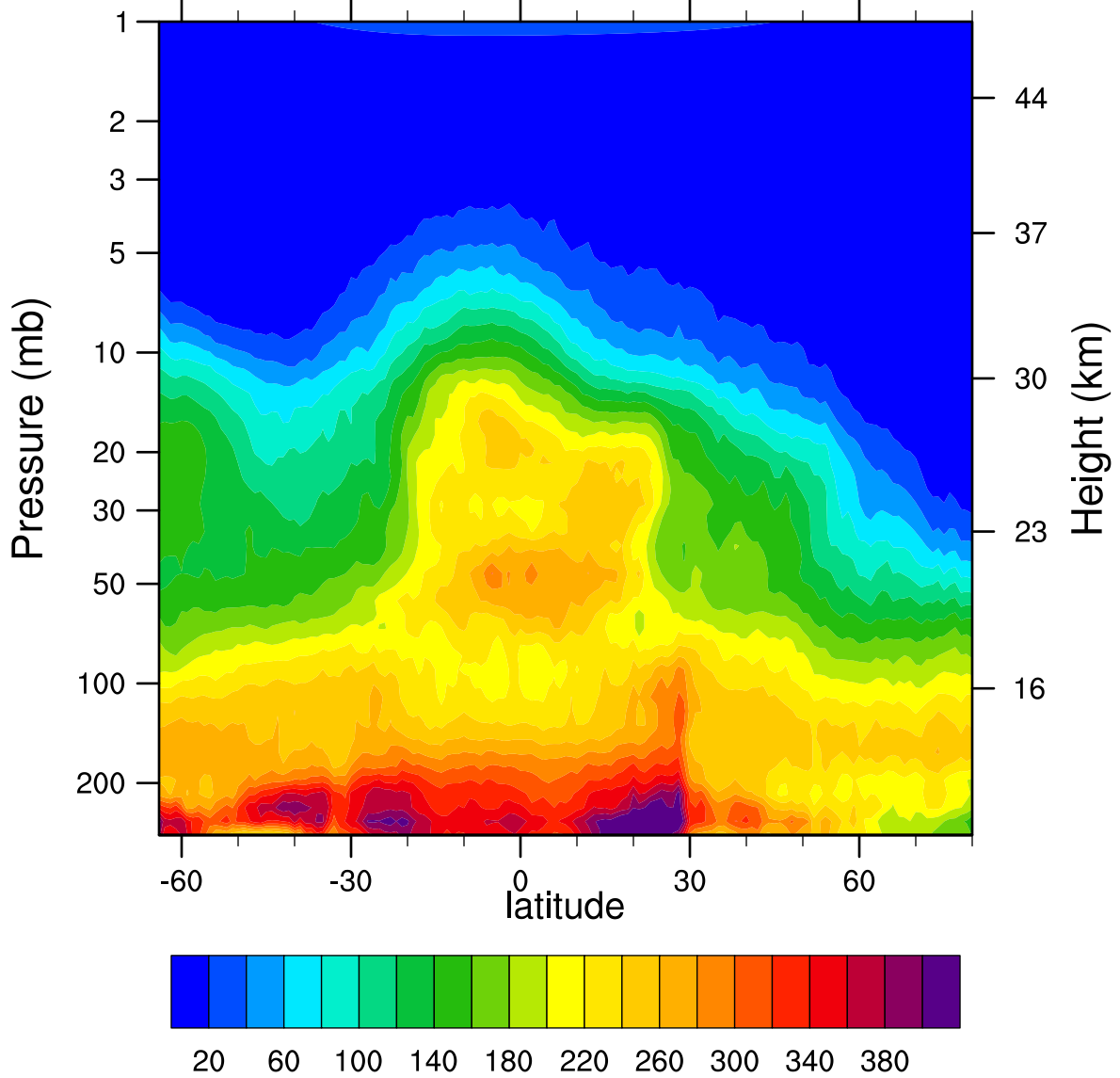
HIRDLSv6 2007d357 N2O_Combined (ppbv)
