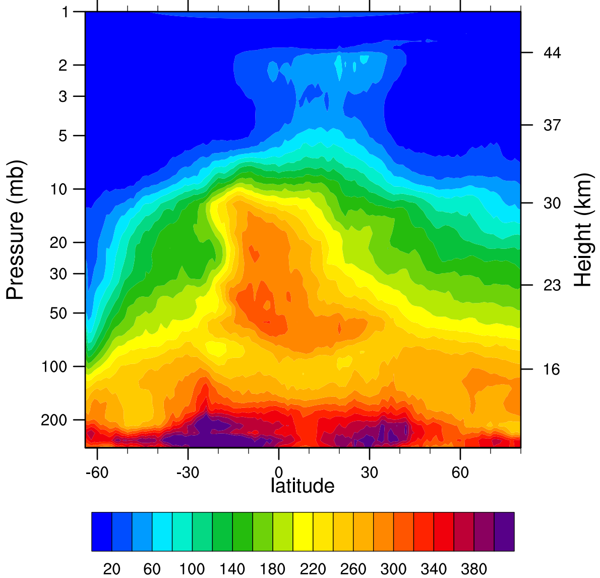
HIRDLSv6 2005d238 N2O_Combined (ppbv)
