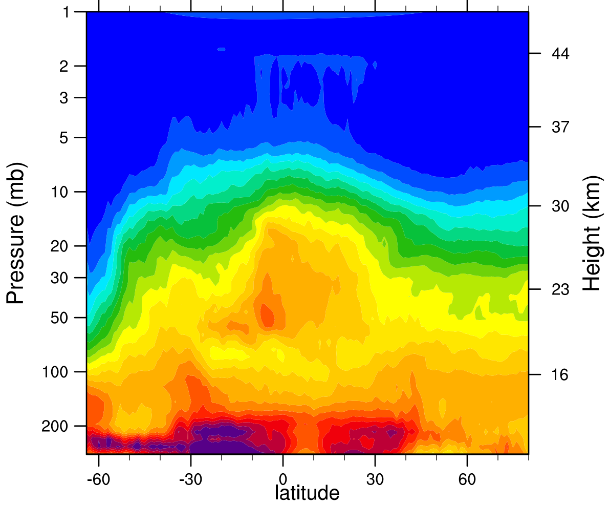
HIRDLSv6 2006d192 N2O_Combined (ppbv)
