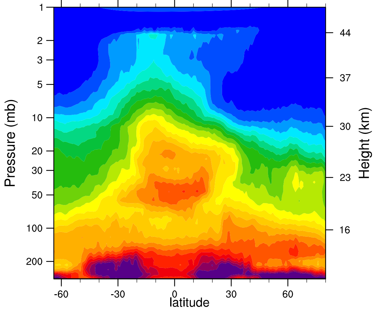
HIRDLSv6 2006d043 N2O_Combined (ppbv)
