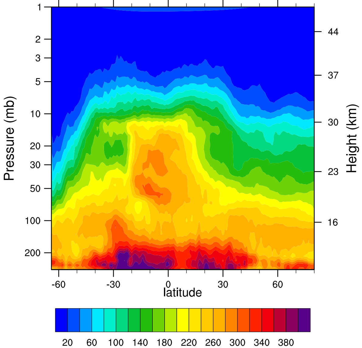
HIRDLSv6 2007d169 N2O_Combined (ppbv)
