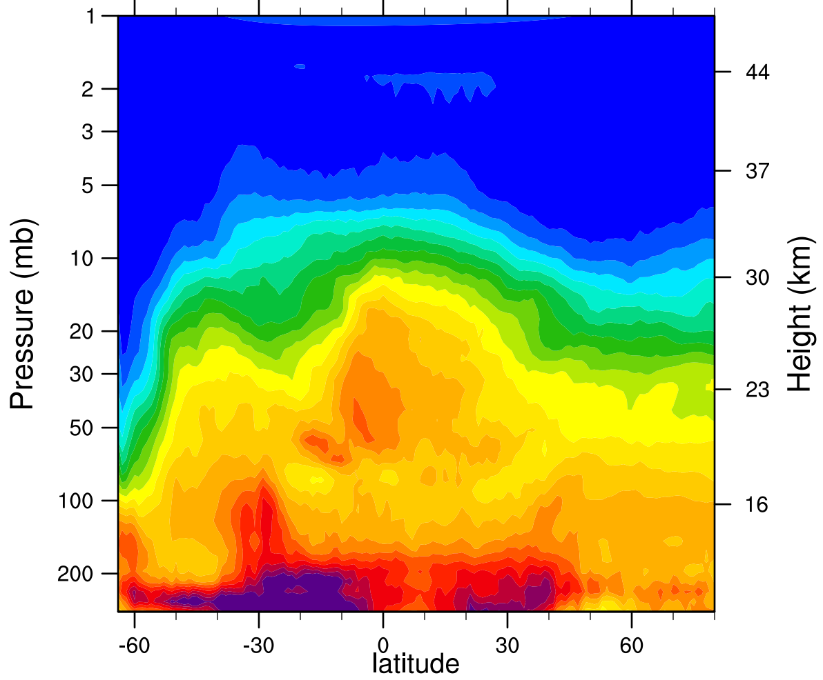
HIRDLSv6 2006d206 N2O_Combined (ppbv)
