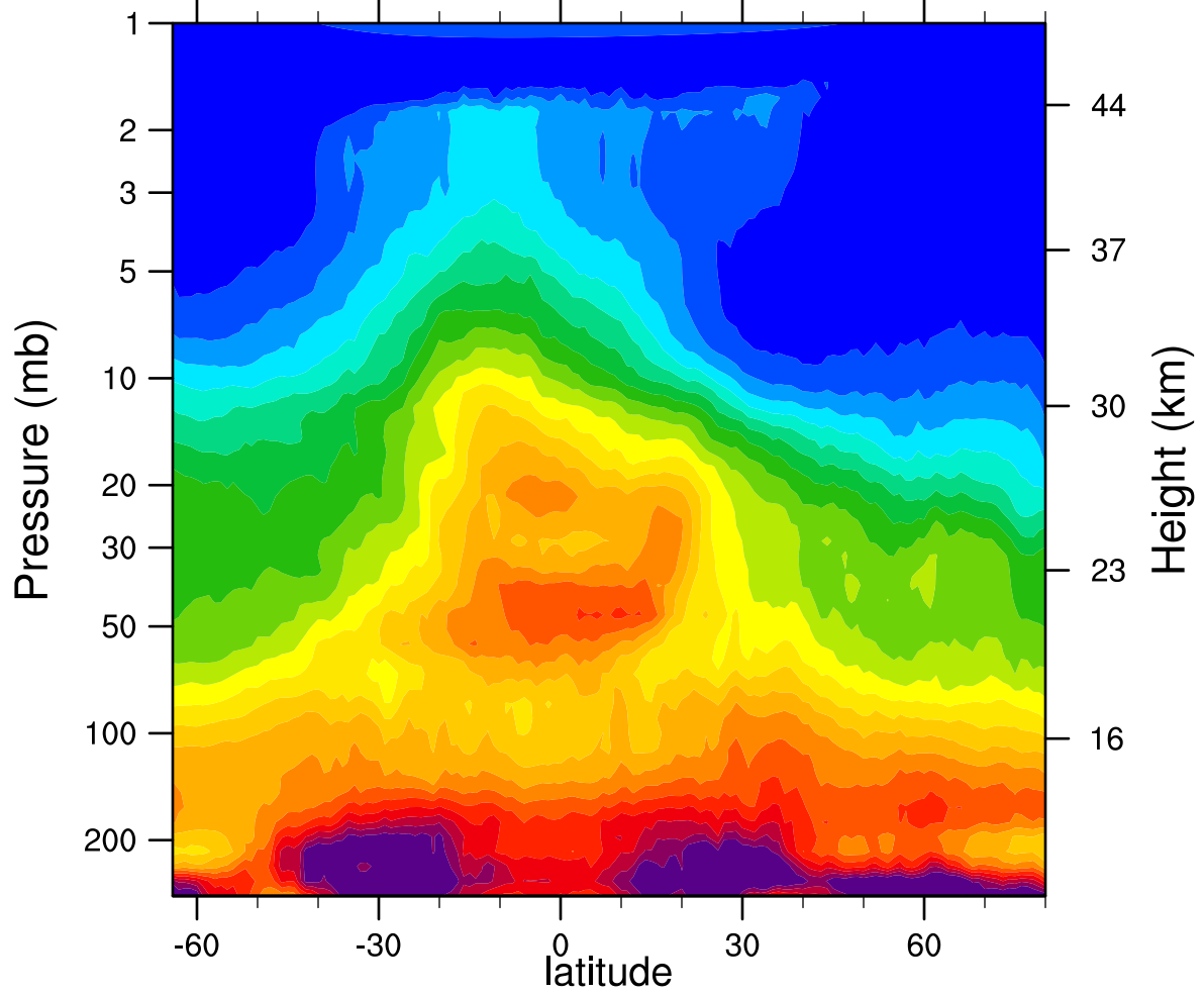
HIRDLSv6 2006d038 N2O_Combined (ppbv)
