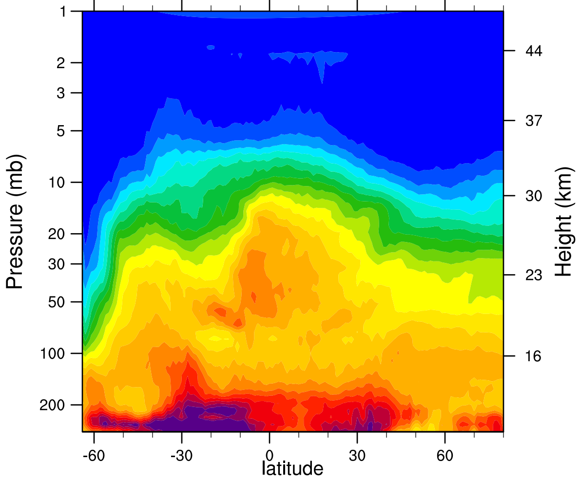
HIRDLSv6 2006d213 N2O_Combined (ppbv)
