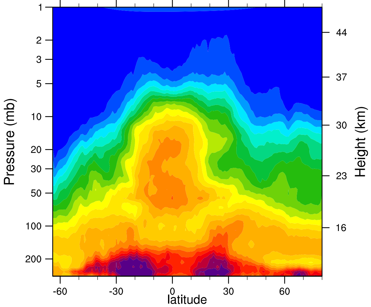
HIRDLSv6 2007d126 N2O_Combined (ppbv)
