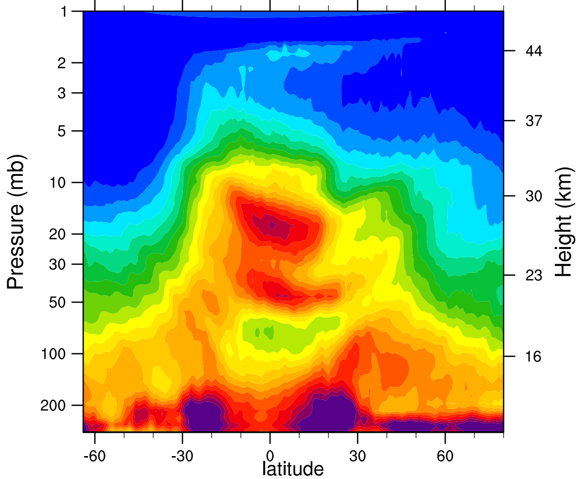
HIRDLSv6 2005d058 N2O_Combined (ppbv)
