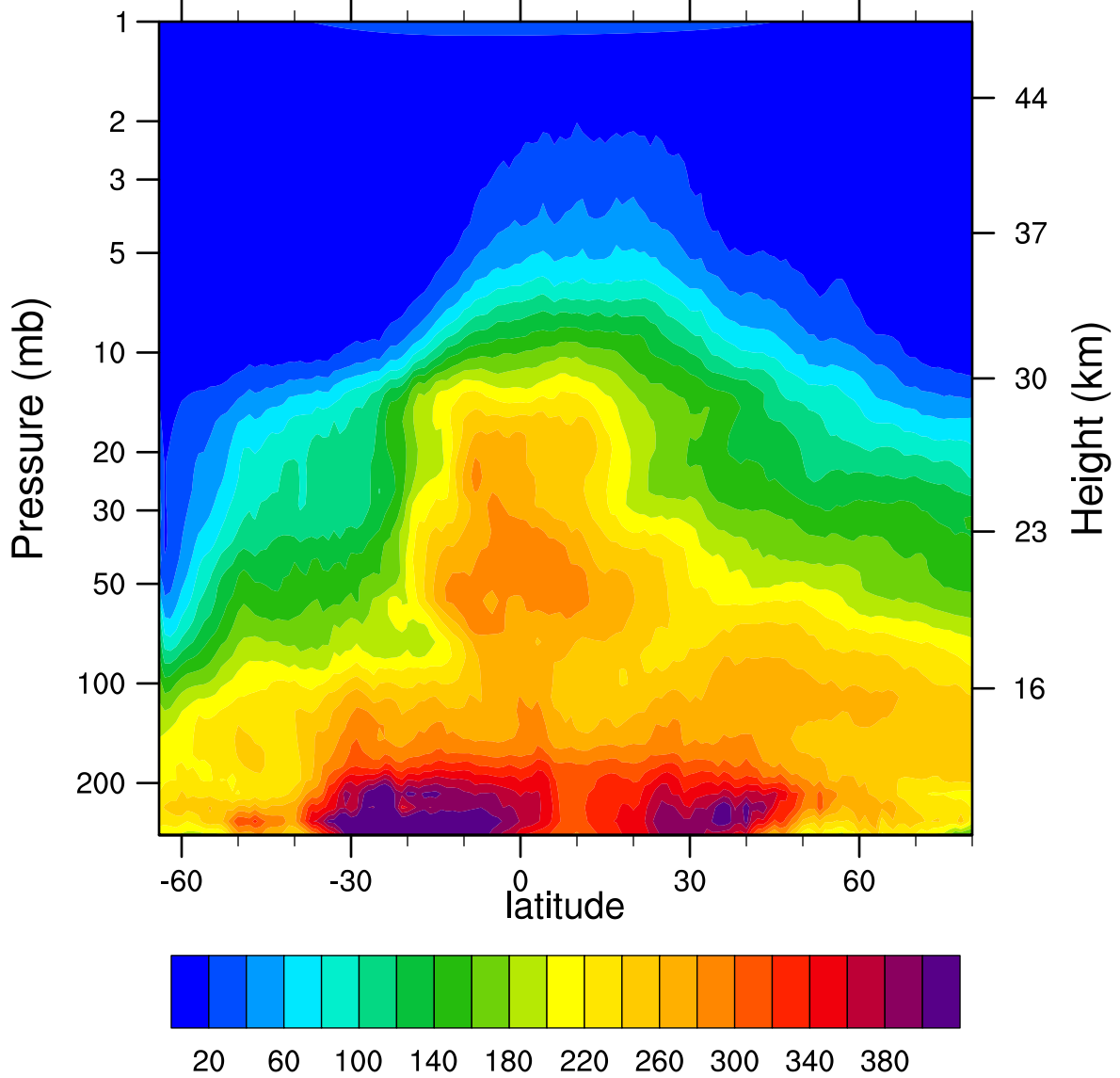
HIRDLSv6 2007d220 N2O_Combined (ppbv)
