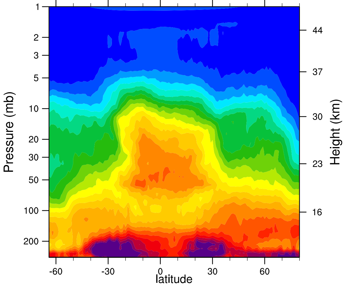
HIRDLSv6 2005d315 N2O_Combined (ppbv)
