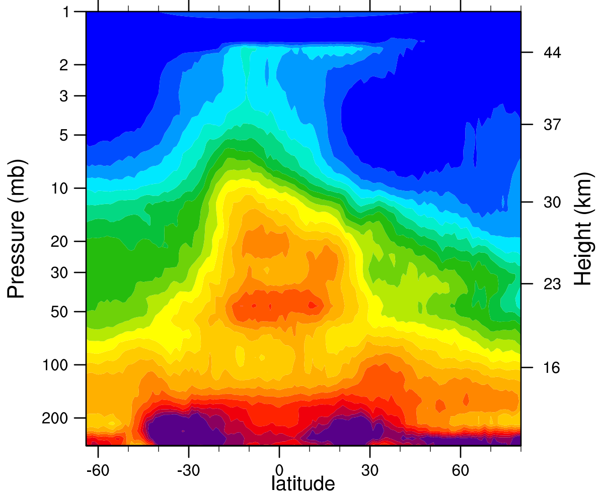
HIRDLSv6 2006d023 N2O_Combined (ppbv)
