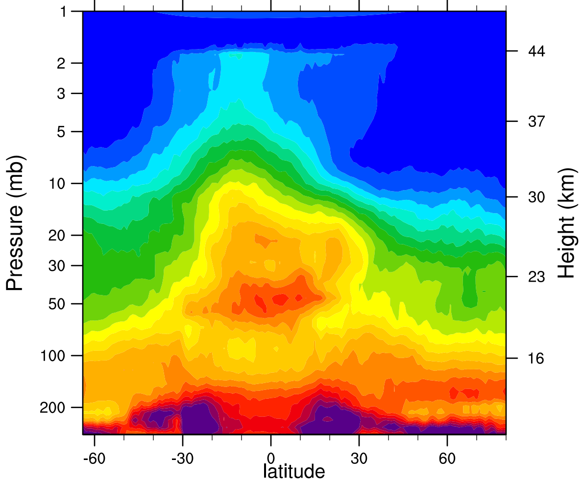
HIRDLSv6 2006d049 N2O_Combined (ppbv)
