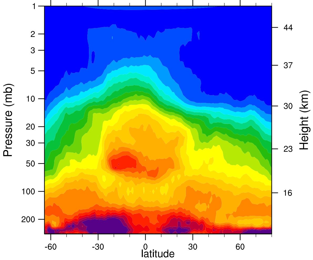
HIRDLSv6 2006d116 N2O_Combined (ppbv)
