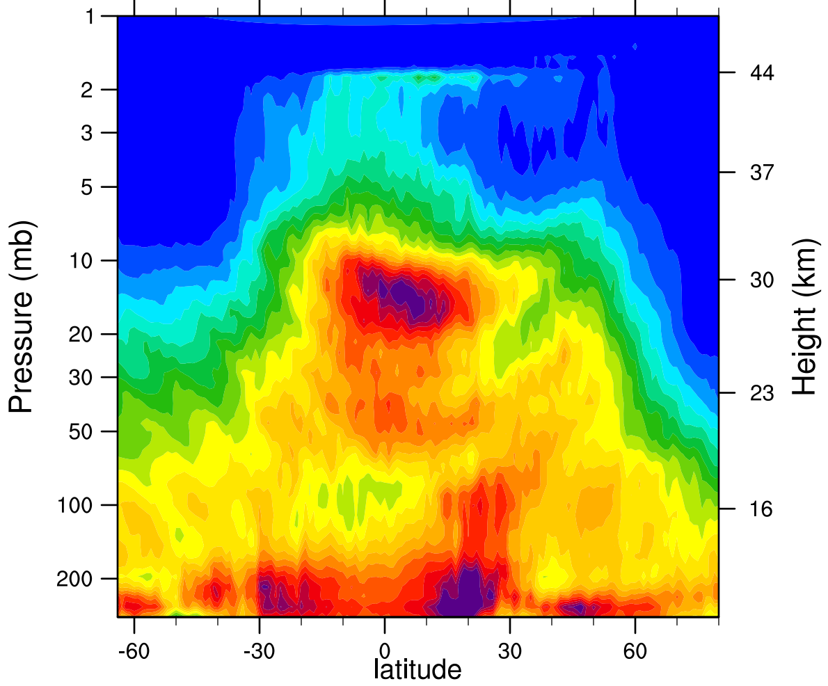
HIRDLSv6 2005d027 N2O_Combined (ppbv)
