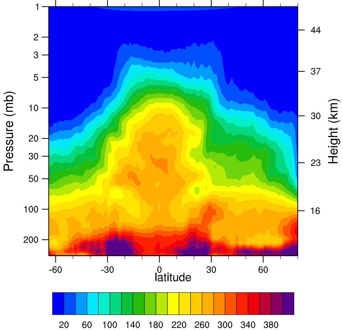
HIRDLSv6 2007d087 N2O_Combined (ppbv)
