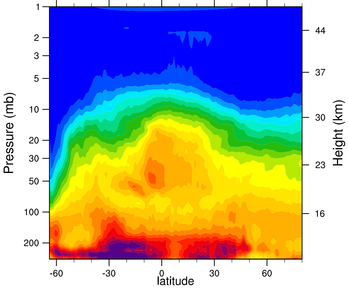
HIRDLSv6 2006d199 N2O_Combined (ppbv)
