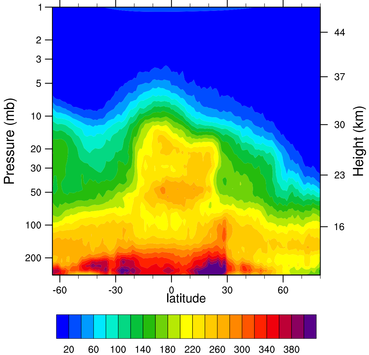
HIRDLSv6 2007d358 N2O_Combined (ppbv)
