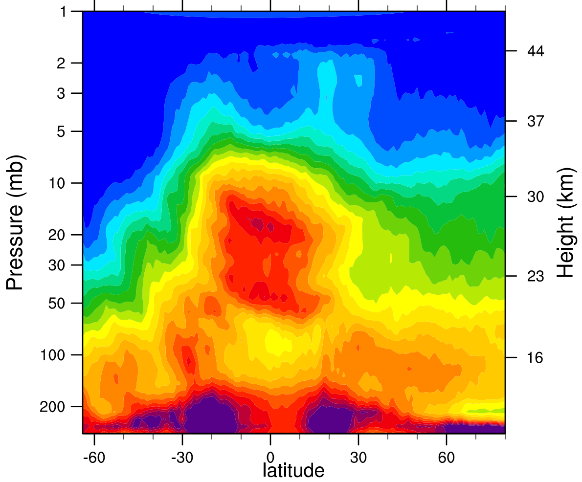
HIRDLSv6 2005d116 N2O_Combined (ppbv)
