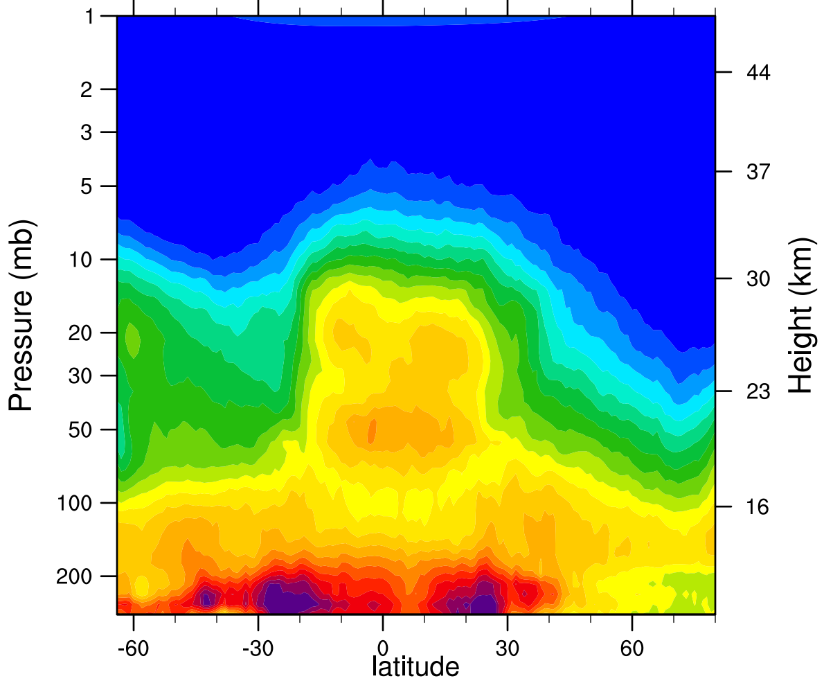
HIRDLSv6 2007d320 N2O_Combined (ppbv)
