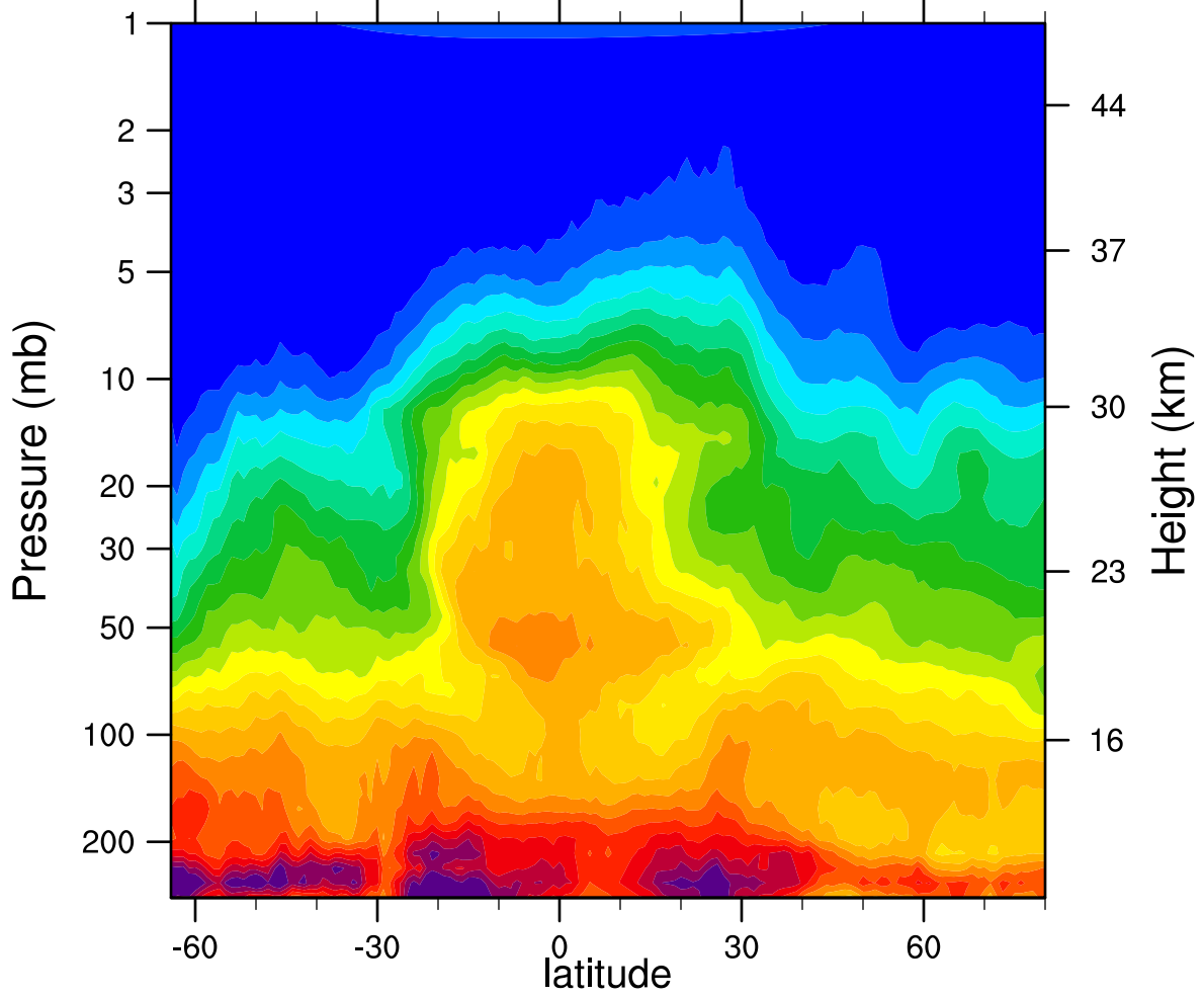
HIRDLSv6 2007d159 N2O_Combined (ppbv)
