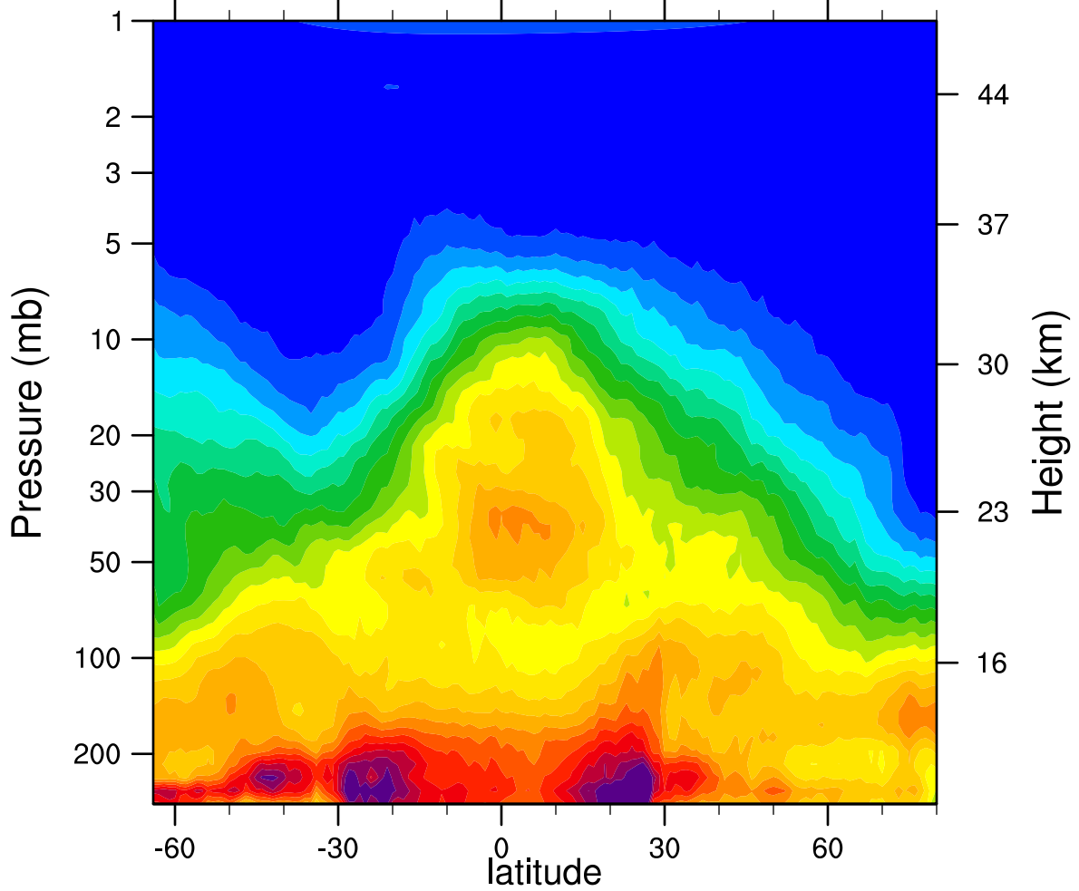
HIRDLSv6 2006d349 N2O_Combined (ppbv)
