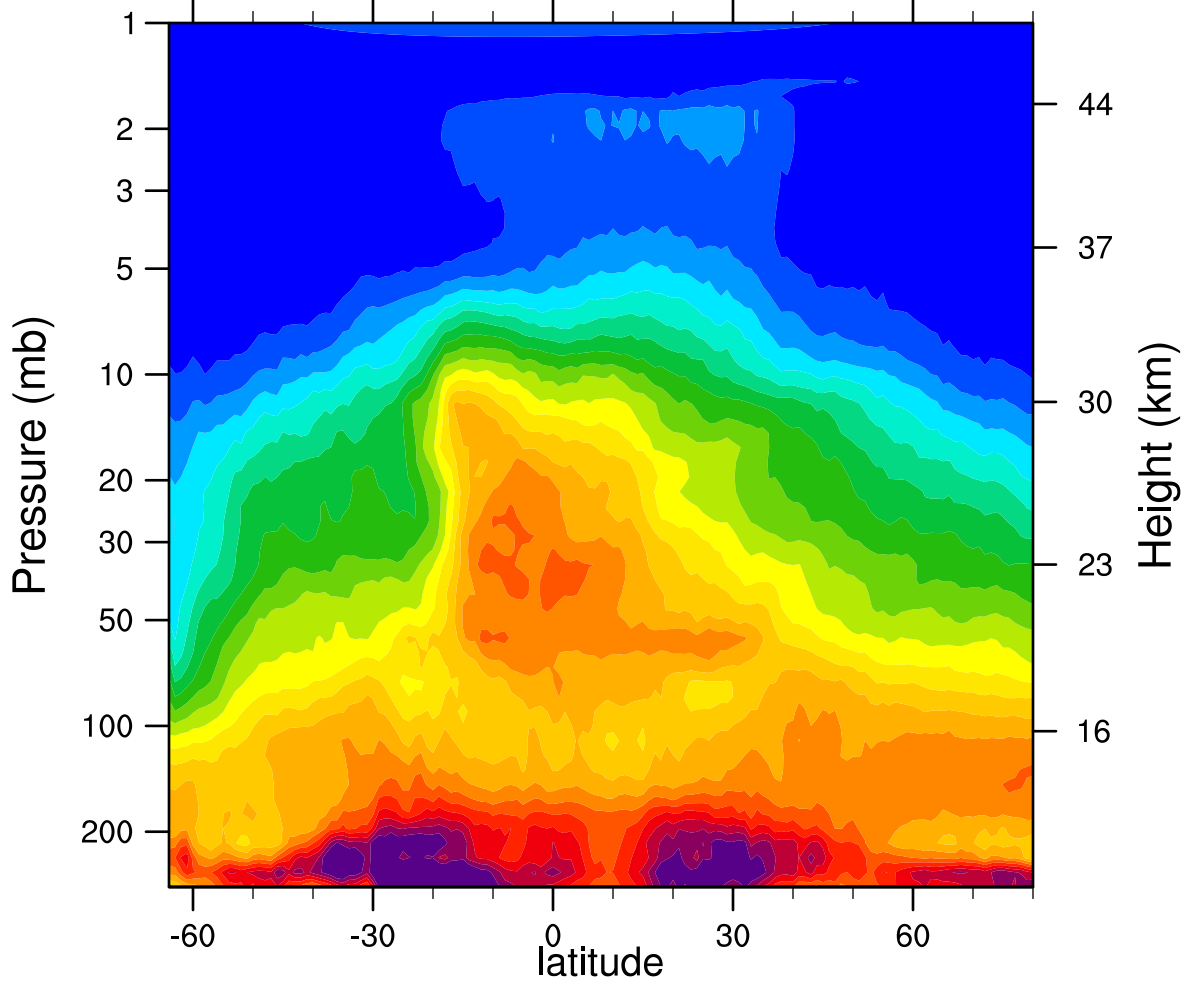
HIRDLSv6 2005d276 N2O_Combined (ppbv)
