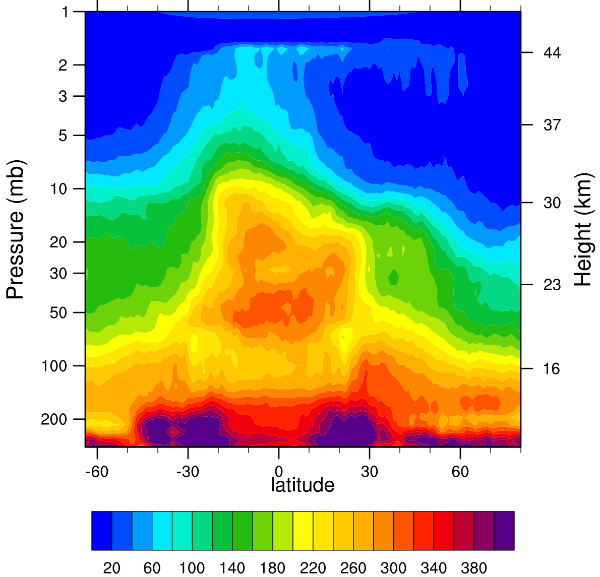
HIRDLSv6 2006d013 N2O_Combined (ppbv)
