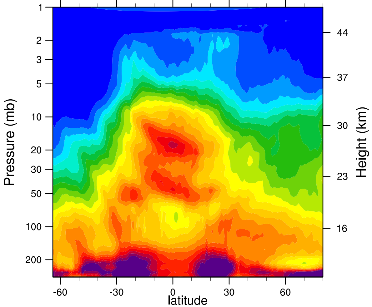
HIRDLSv6 2005d102 N2O_Combined (ppbv)
