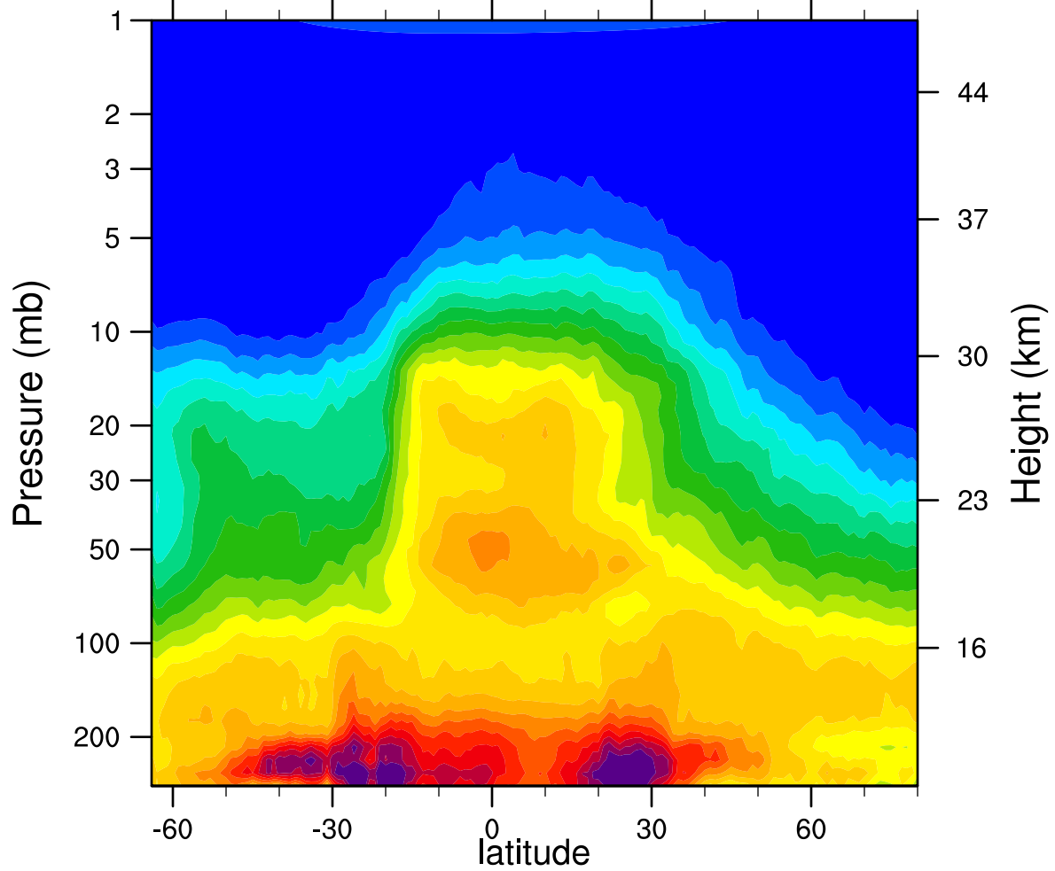
HIRDLSv6 2007d292 N2O_Combined (ppbv)
