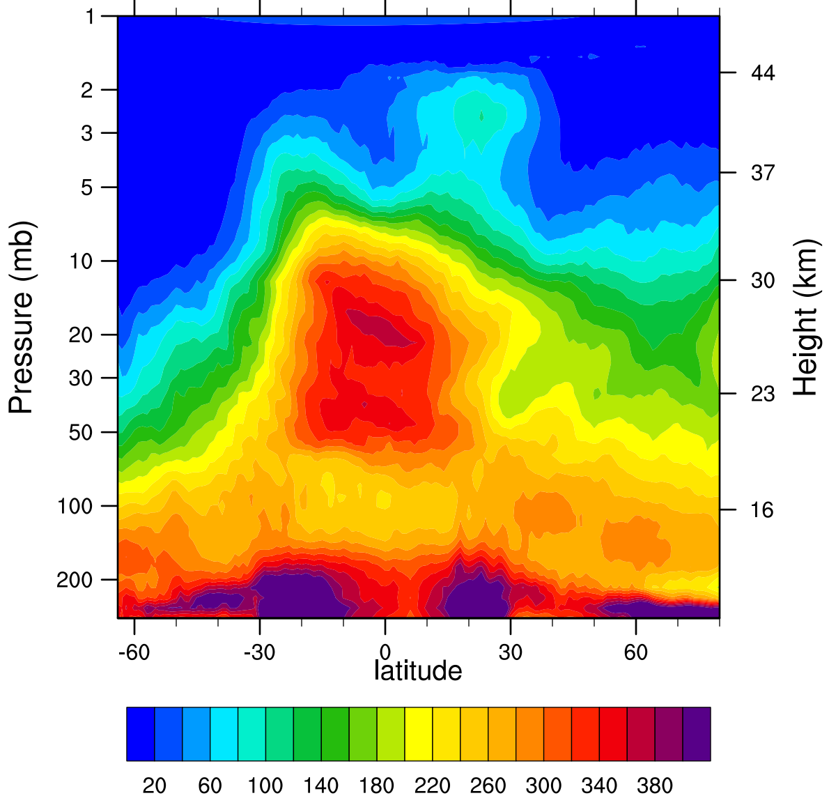
HIRDLSv6 2005d125 N2O_Combined (ppbv)
