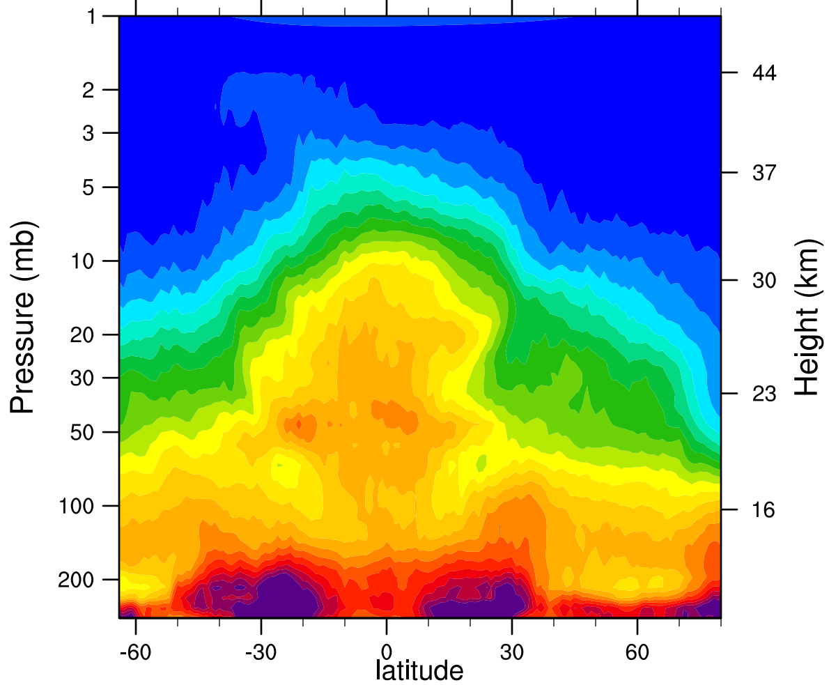
HIRDLSv6 2007d070 N2O_Combined (ppbv)
