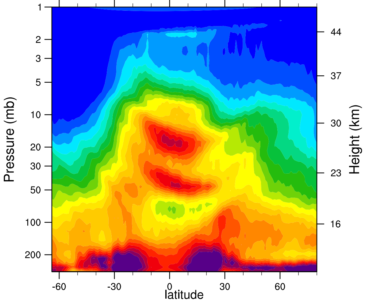
HIRDLSv6 2005d071 N2O_Combined (ppbv)
