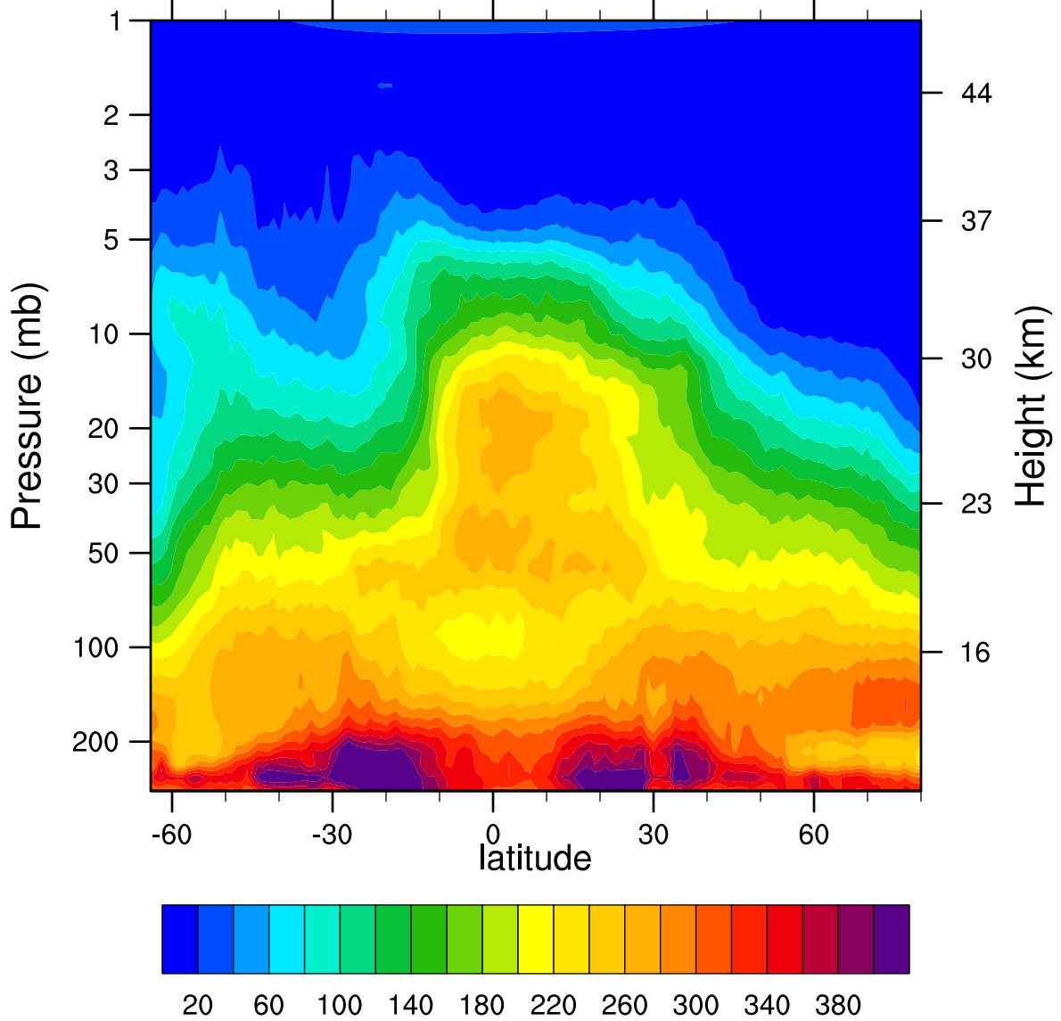
HIRDLSv6 2006d308 N2O_Combined (ppbv)
