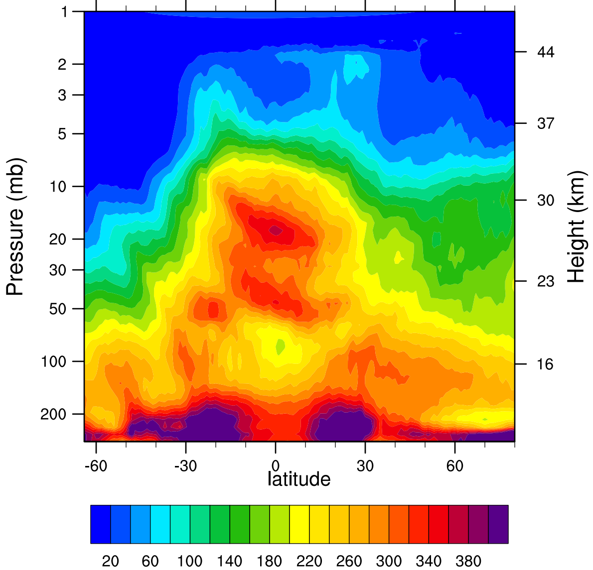
HIRDLSv6 2005d103 N2O_Combined (ppbv)
