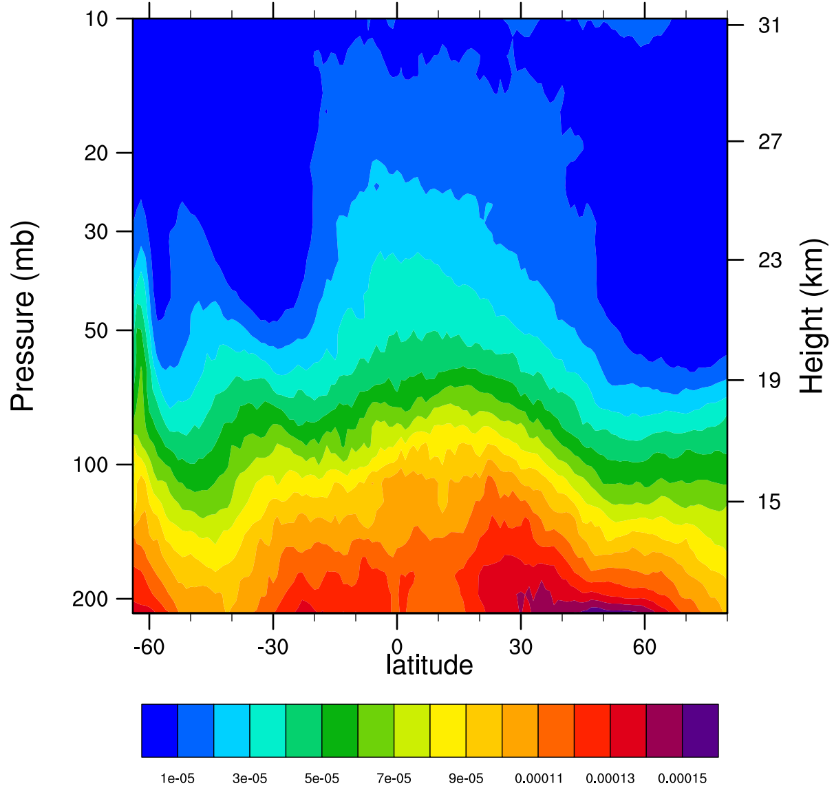
2007d235 12.1MicronExtinction_Combined (km -1 )
