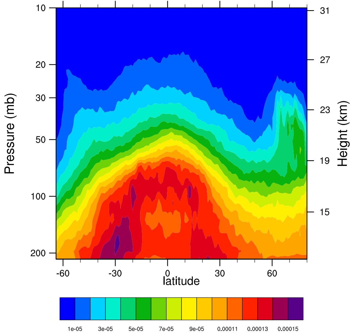
2006d359 12.1MicronExtinction_Combined (km -1 )
