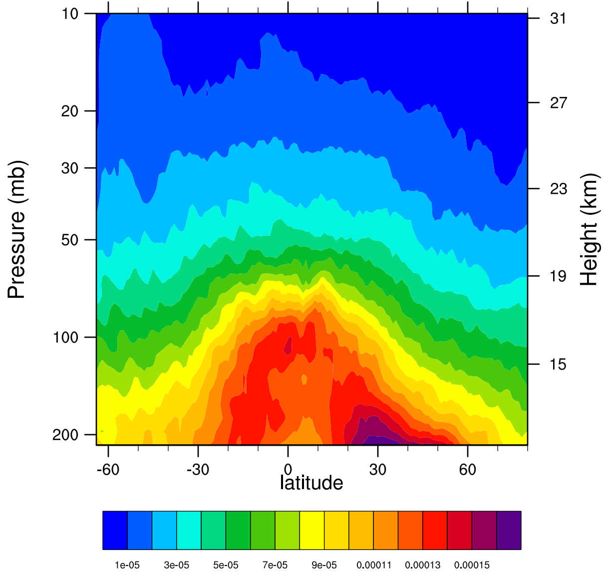
2006d149 12.1MicronExtinction_Combined ( \text{km}^{-1} )
