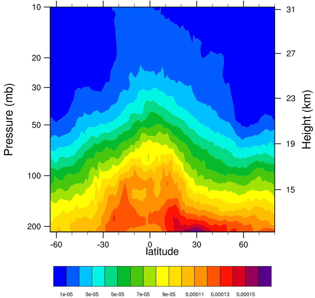
2007d101 12.1MicronExtinction_Combined (km -1 )
