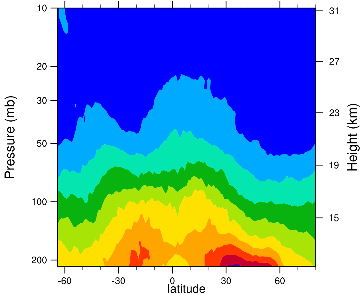
2007d144 12.1MicronExtinction_Combined (km -1 )
