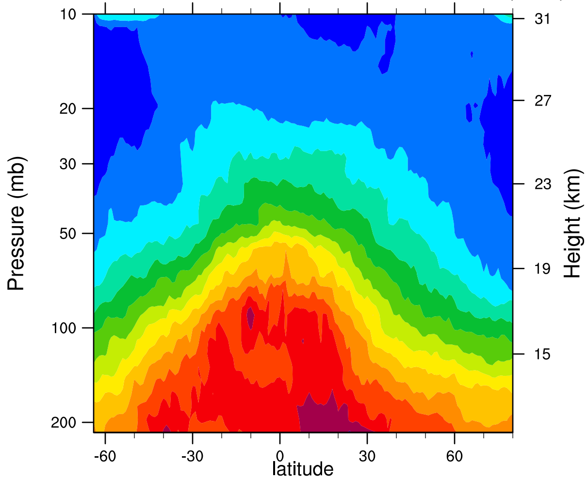
2006d024 12.1MicronExtinction_Combined ( \text{km}^{-1} )
