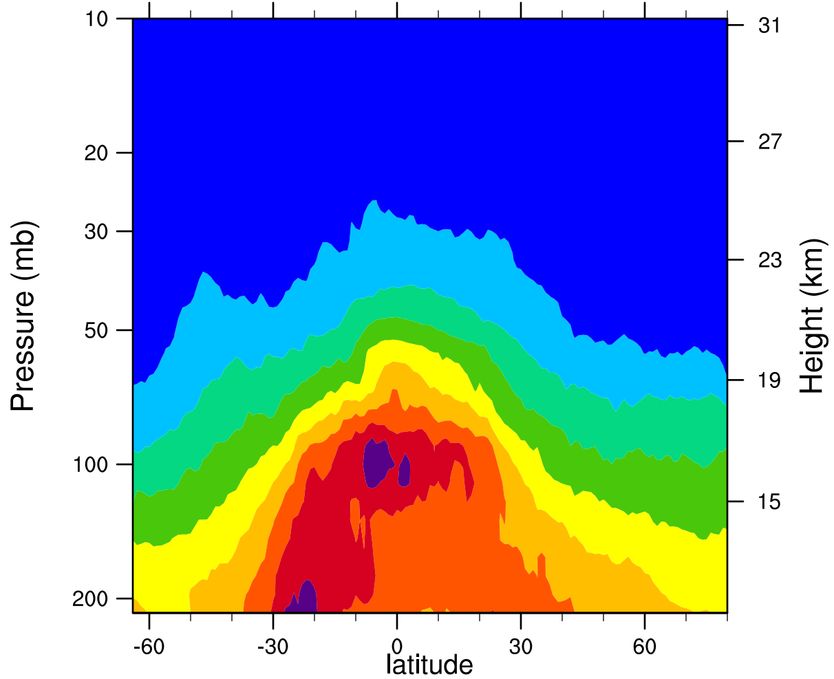
2006d312 12.1MicronExtinction_Combined (km -1 )
