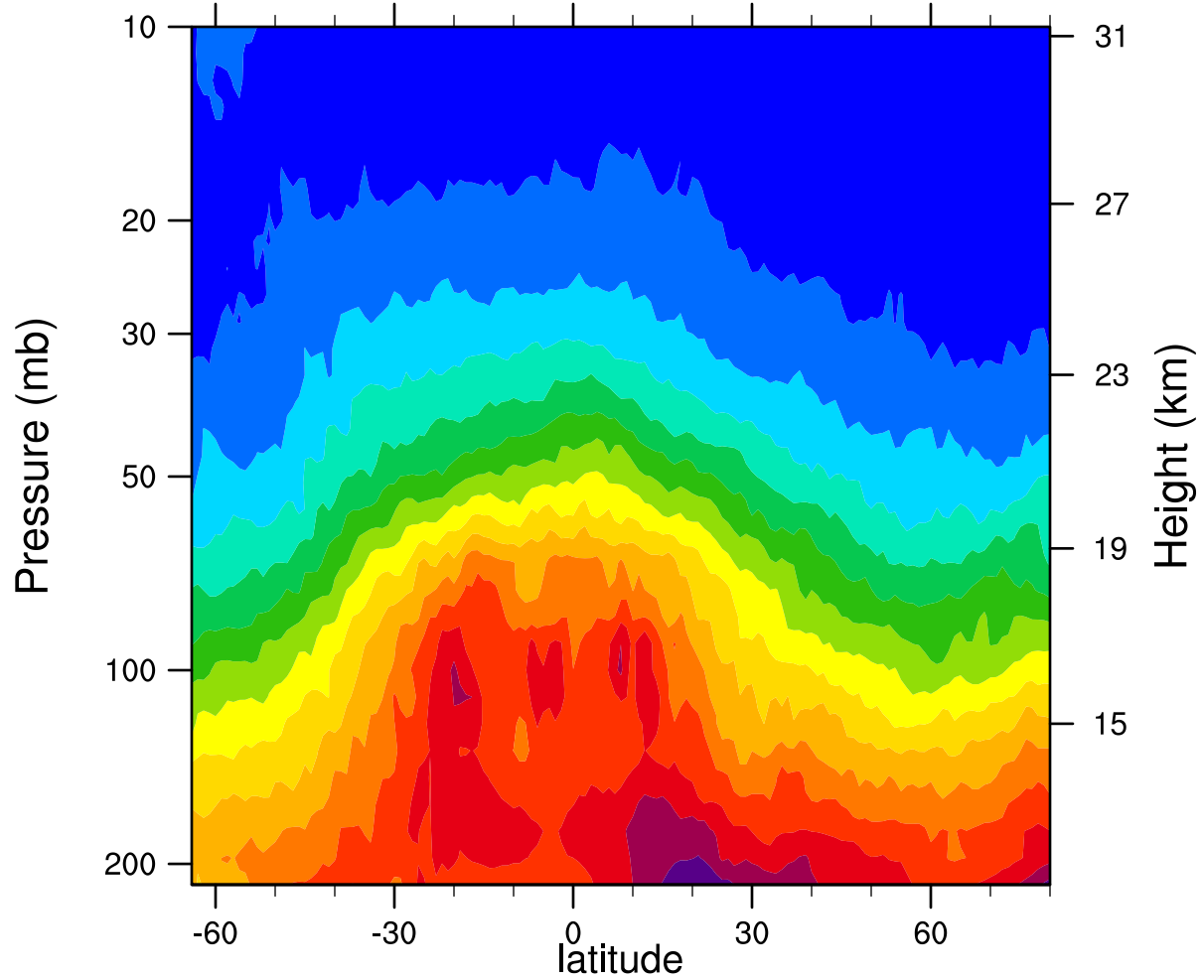
2007d073 12.1MicronExtinction_Combined ( \text{km}^{-1} )
