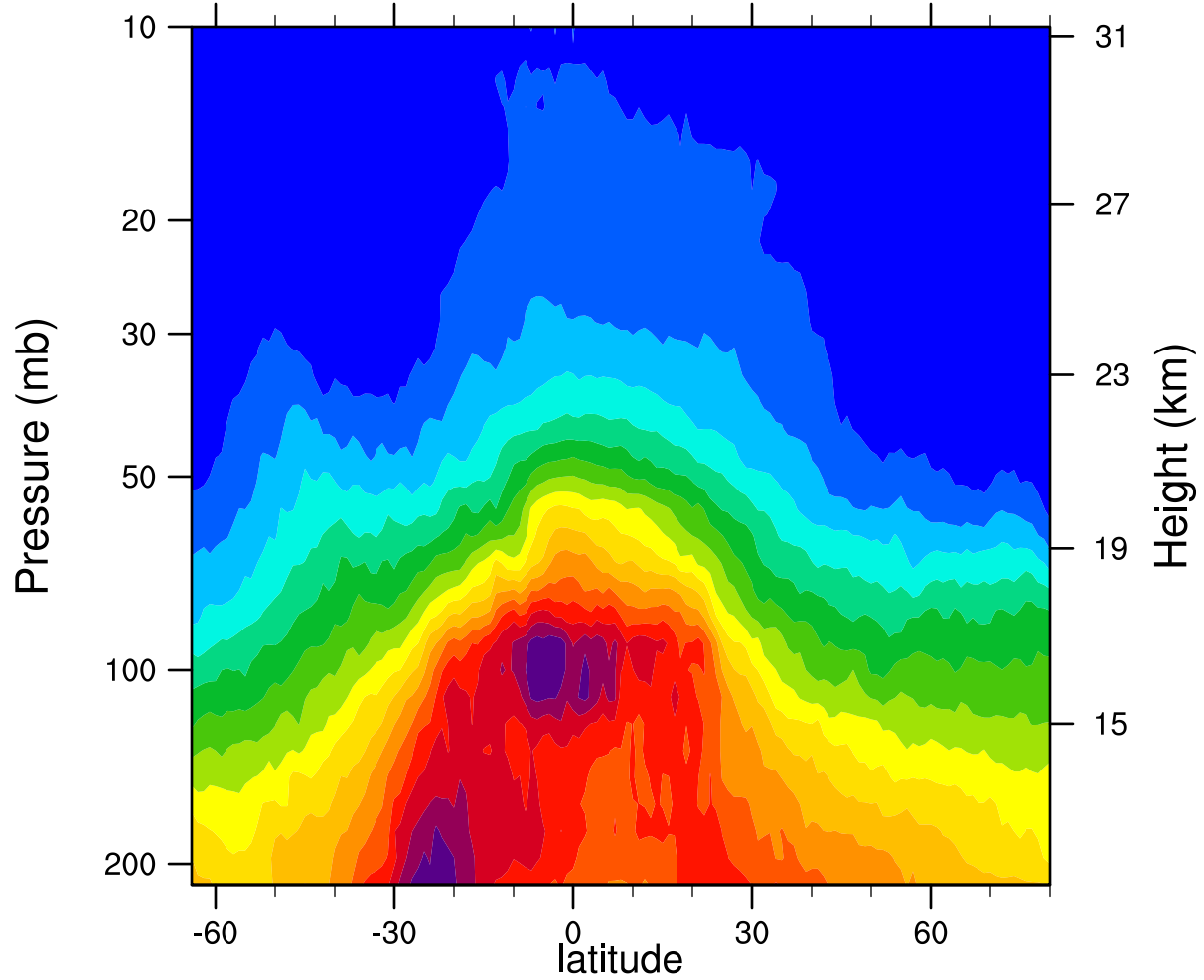
2006d313 12.1MicronExtinction_Combined (km -1 )
