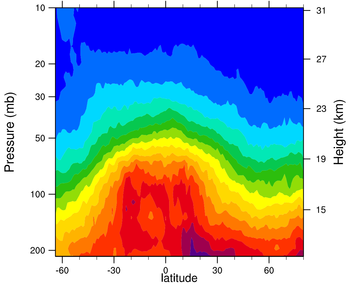
2007d069 12.1MicronExtinction_Combined (km -1 )
