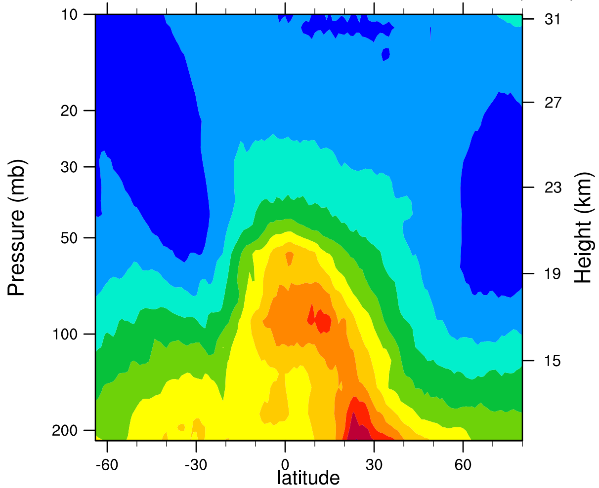
2005d124 12.1MicronExtinction_Combined (km -1 )
