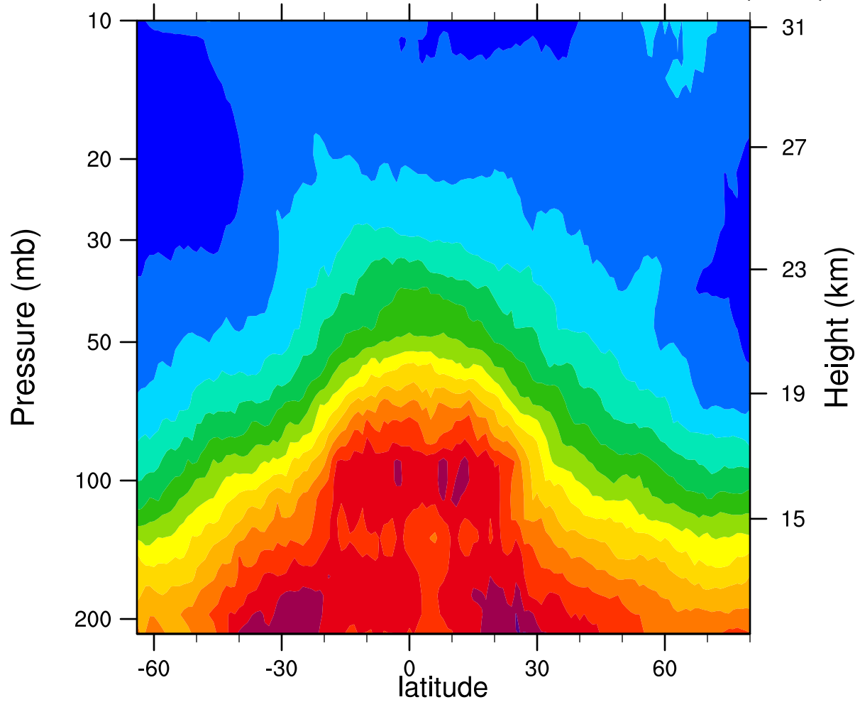
2005d325 12.1MicronExtinction_Combined (km -1 )
