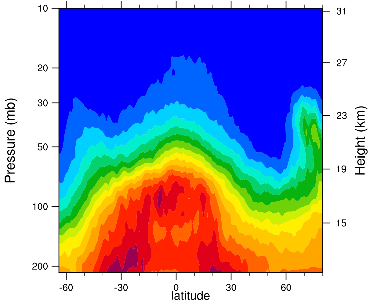
2006d353 12.1MicronExtinction_Combined ( \text{km}^{-1} )
