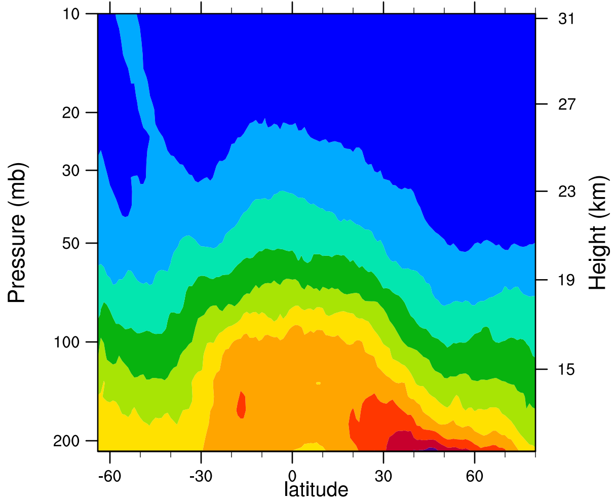
2007d174 12.1MicronExtinction_Combined (km -1 )
