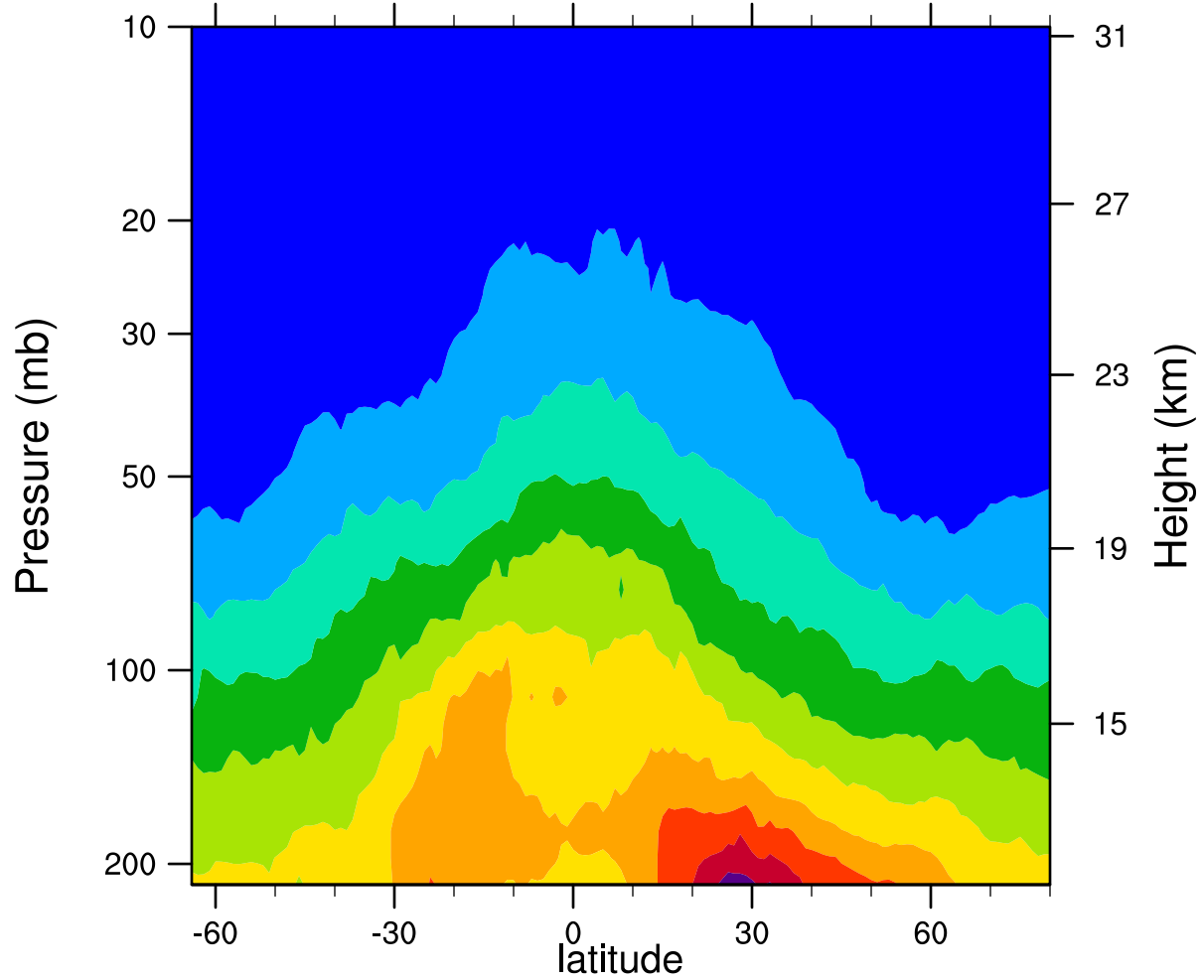
2007d117 12.1MicronExtinction_Combined (km -1 )
