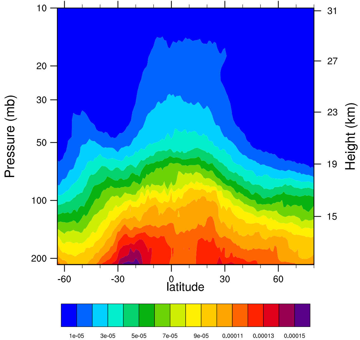
2007d304 12.1MicronExtinction_Combined (km -1 )
