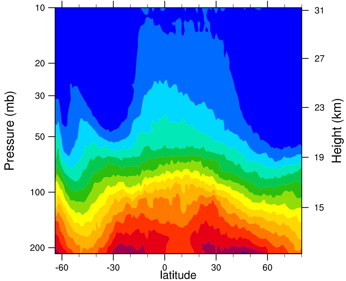
2007d254 12.1MicronExtinction_Combined (km -1 )
