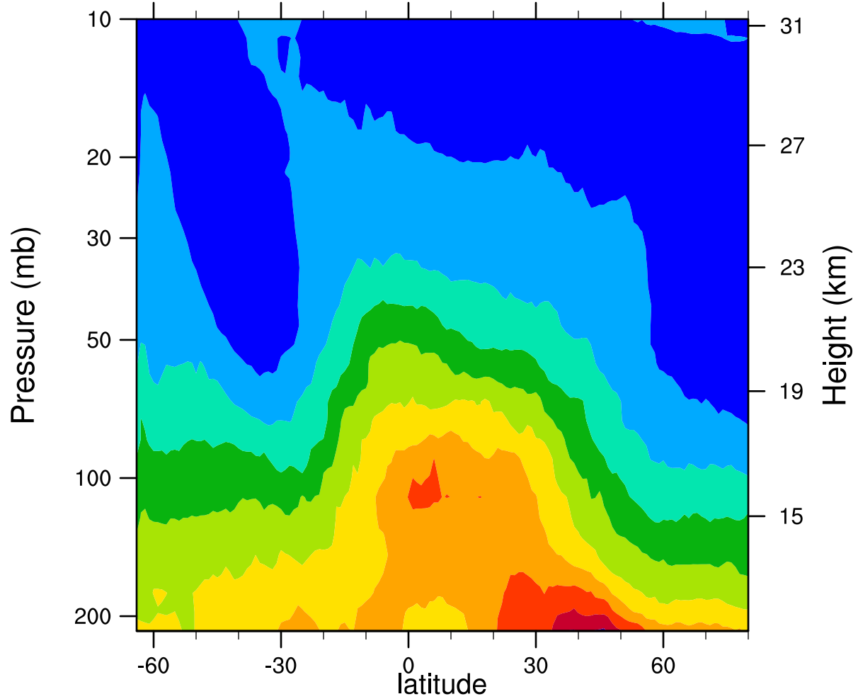
2005d182 12.1MicronExtinction_Combined (km -1 )
