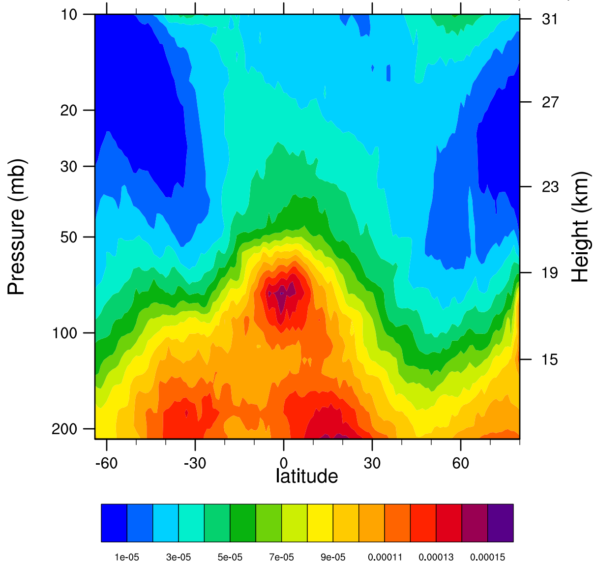
2005d046 12.1MicronExtinction_Combined (km -1 )
