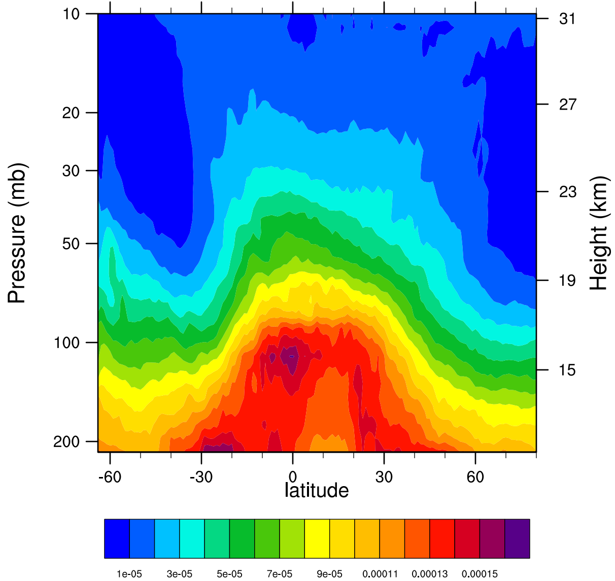
2005d252 12.1MicronExtinction_Combined (km -1 )
