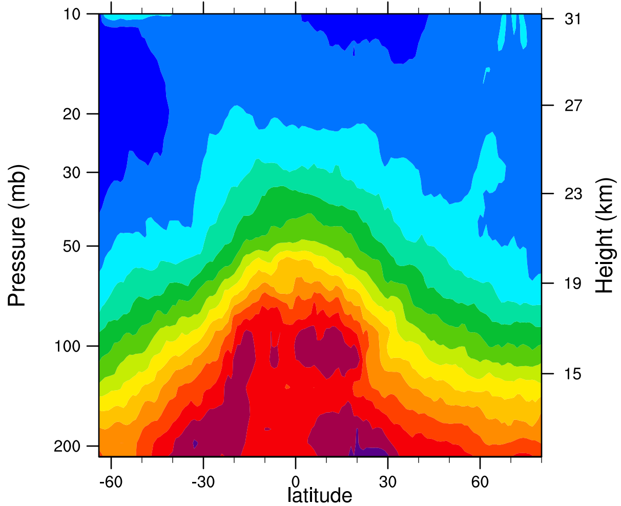
2005d349 12.1MicronExtinction_Combined ( \text{km}^{-1} )
