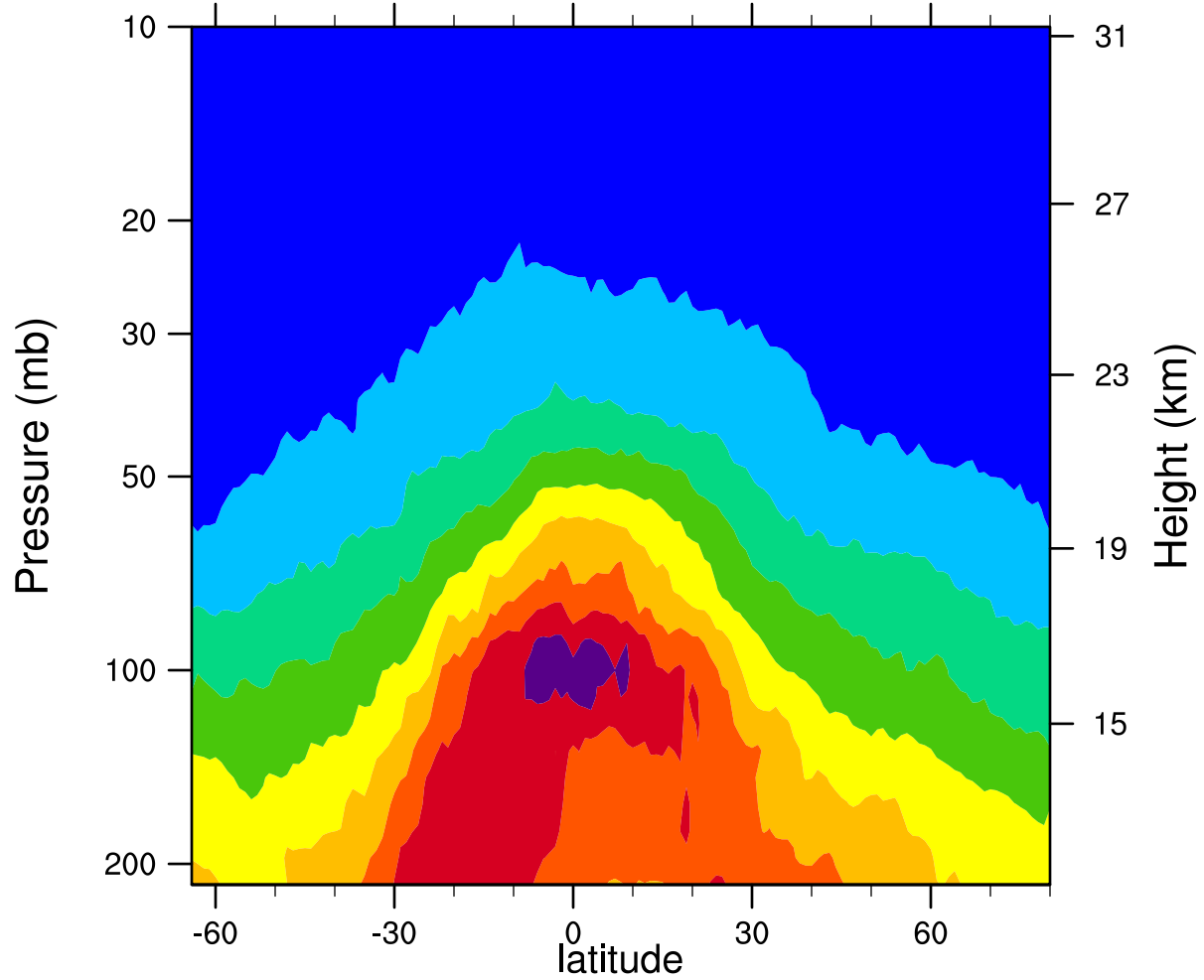
2006d305 12.1MicronExtinction_Combined (km -1 )
