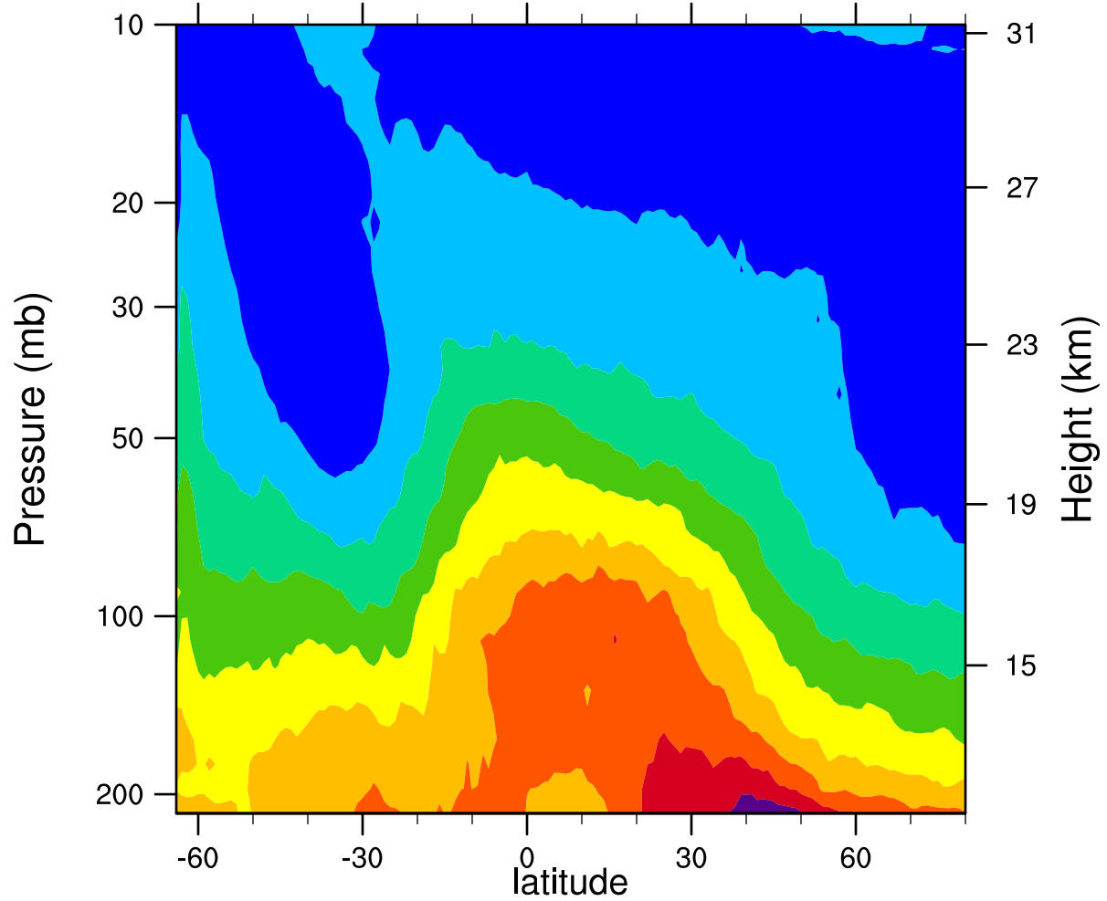
2005d191 12.1MicronExtinction_Combined (km -1 )
