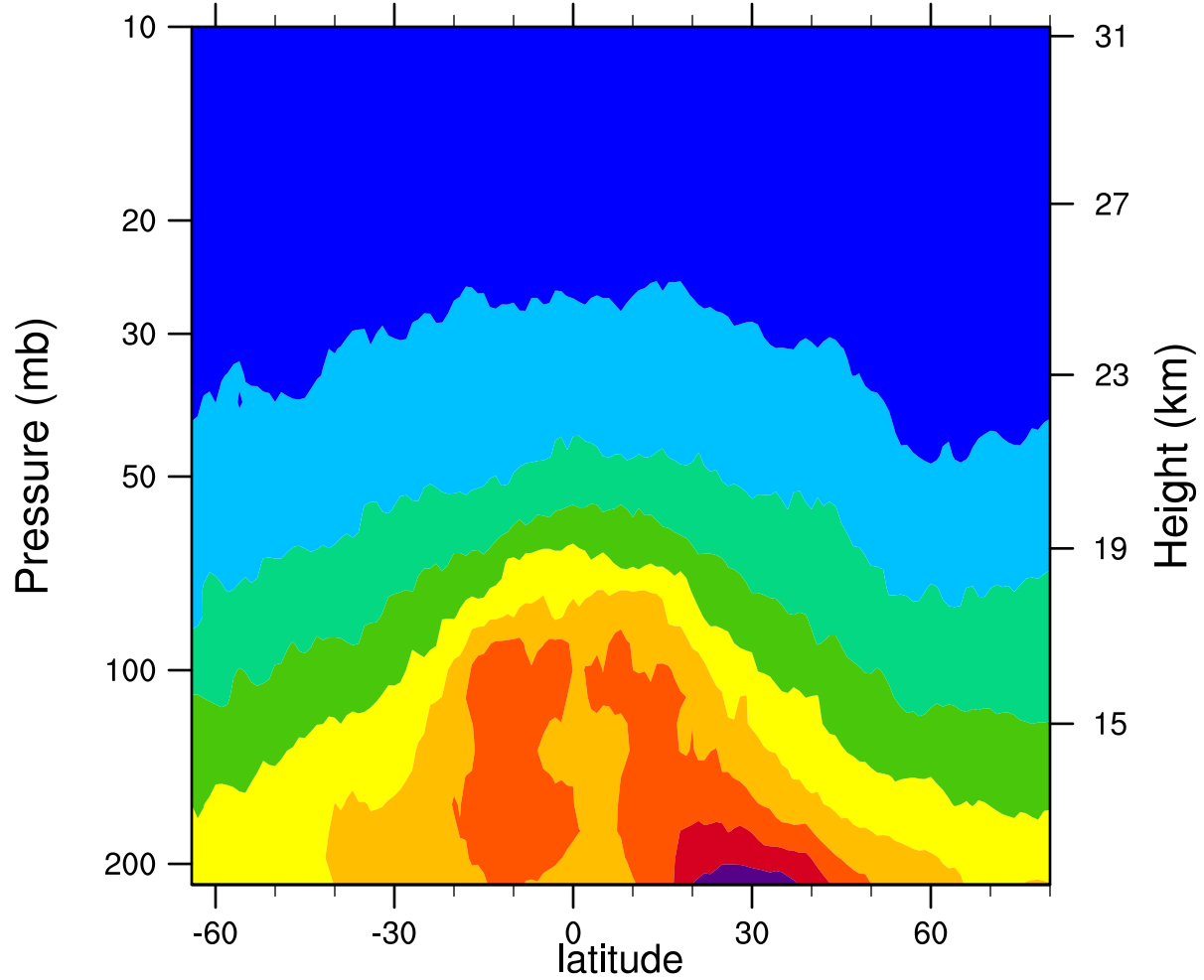
2006d121 12.1MicronExtinction_Combined (km -1 )
