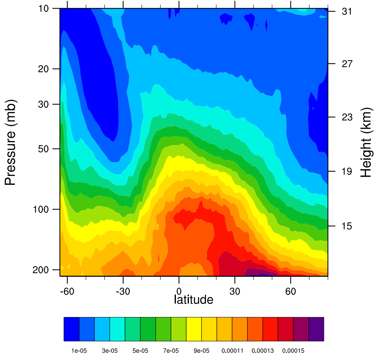
2005d195 12.1MicronExtinction_Combined (km -1 )
