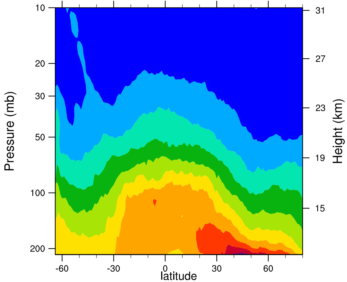
2007d179 12.1MicronExtinction_Combined (km -1 )
