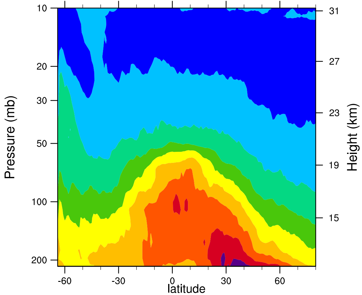
2006d195 12.1MicronExtinction_Combined (km -1 )
