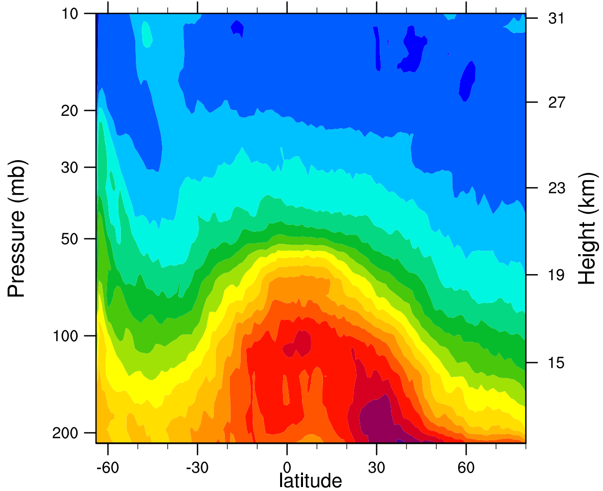
2006d210 12.1MicronExtinction_Combined (km -1 )
