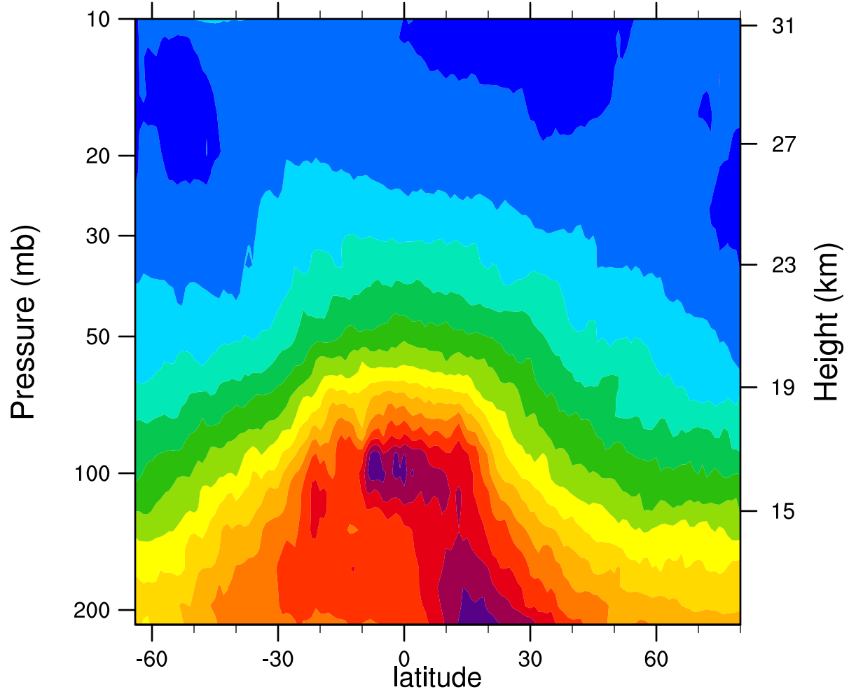
2006d073 12.1MicronExtinction_Combined (km -1 )
