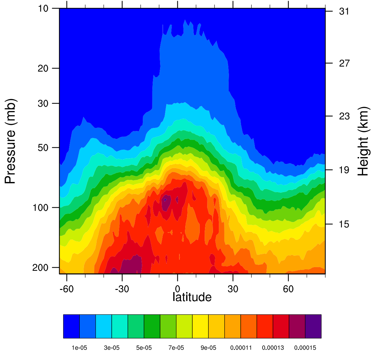
2006d336 12.1MicronExtinction_Combined ( \text{km}^{-1} )
