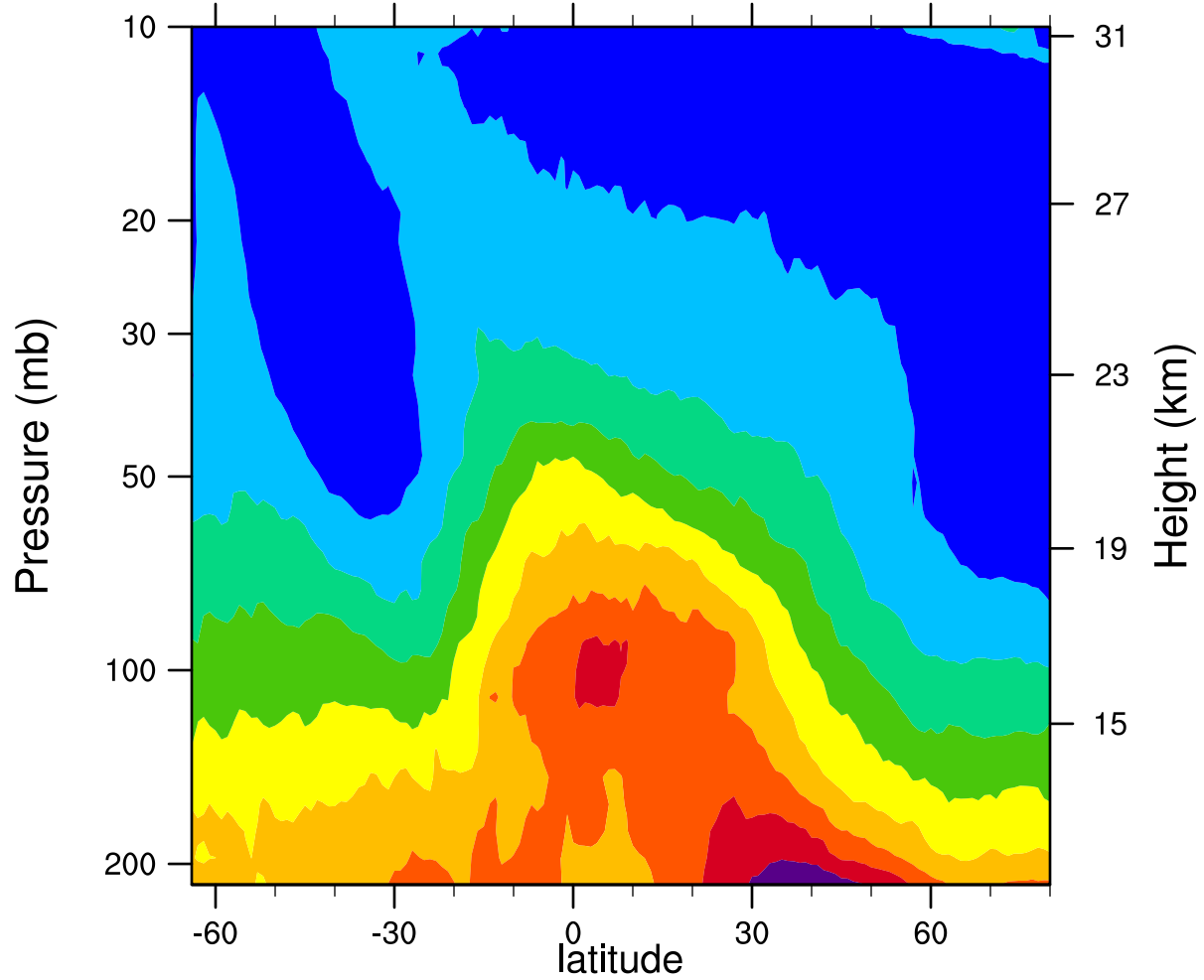
2005d172 12.1MicronExtinction_Combined ( \text{km}^{-1} )
