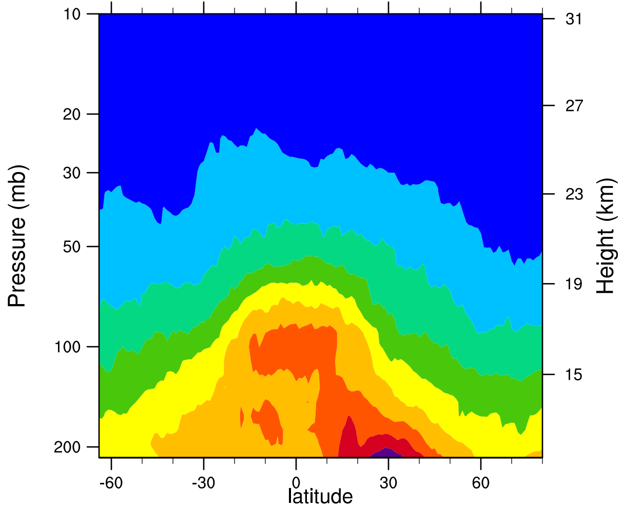
2006d104 12.1MicronExtinction_Combined (km -1 )
