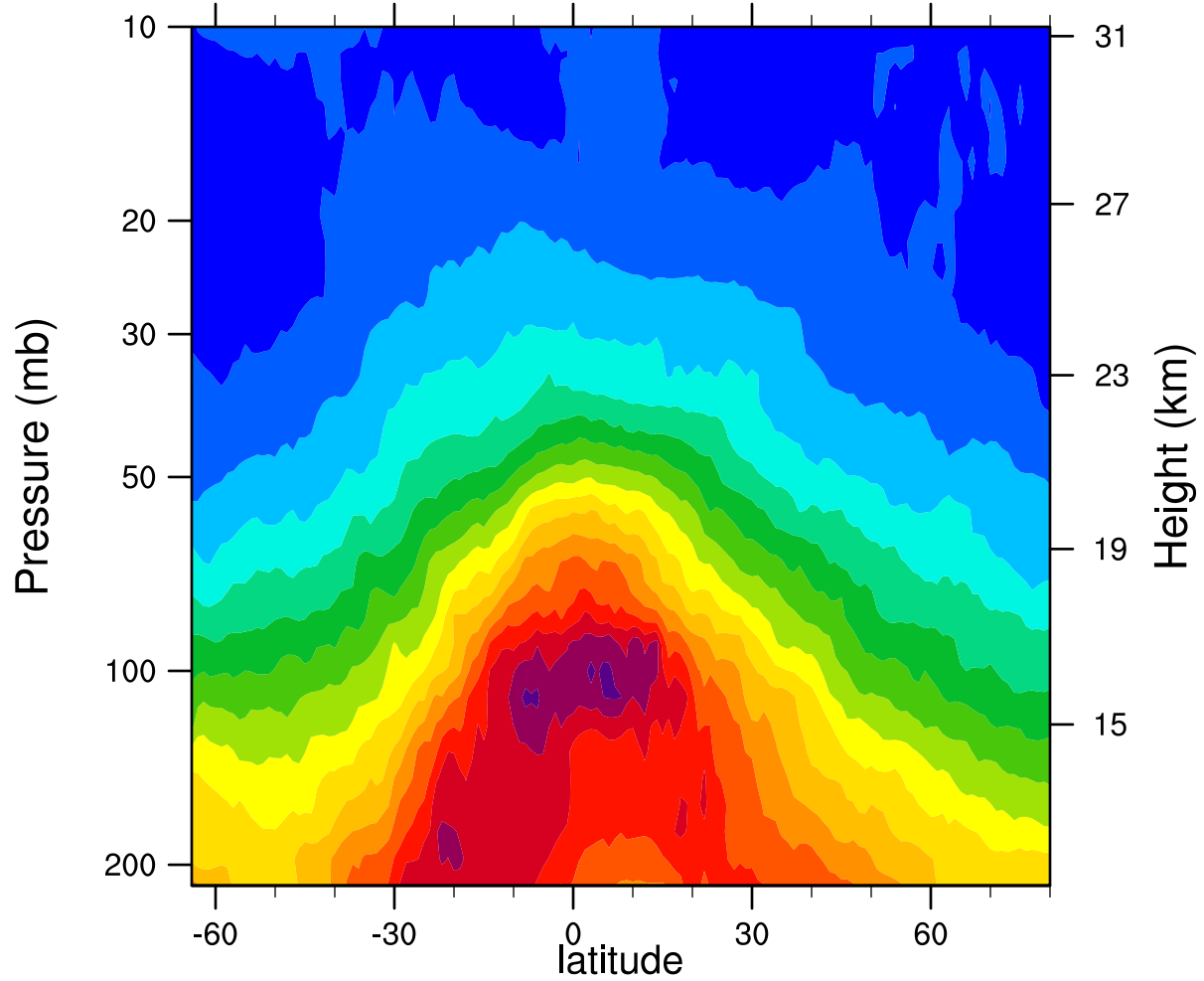
2006d295 12.1MicronExtinction_Combined (km -1 )
