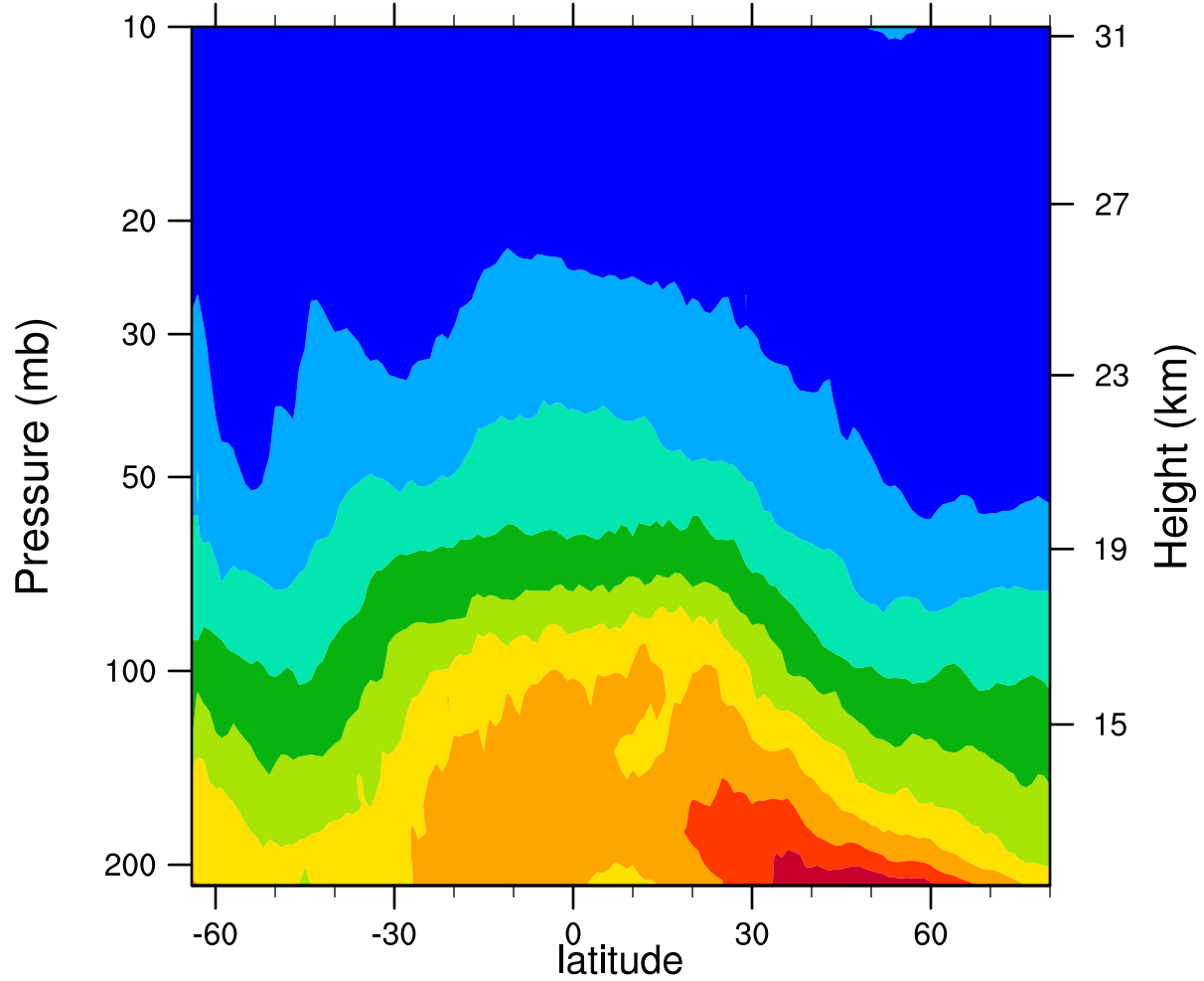
2007d198 12.1MicronExtinction_Combined (km -1 )
