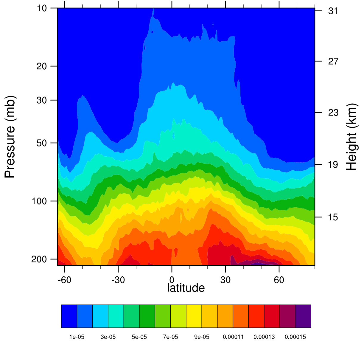
2007d241 12.1MicronExtinction_Combined (km -1 )
