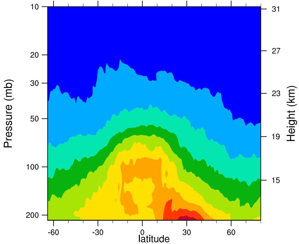
2006d108 12.1MicronExtinction_Combined (km -1 )
