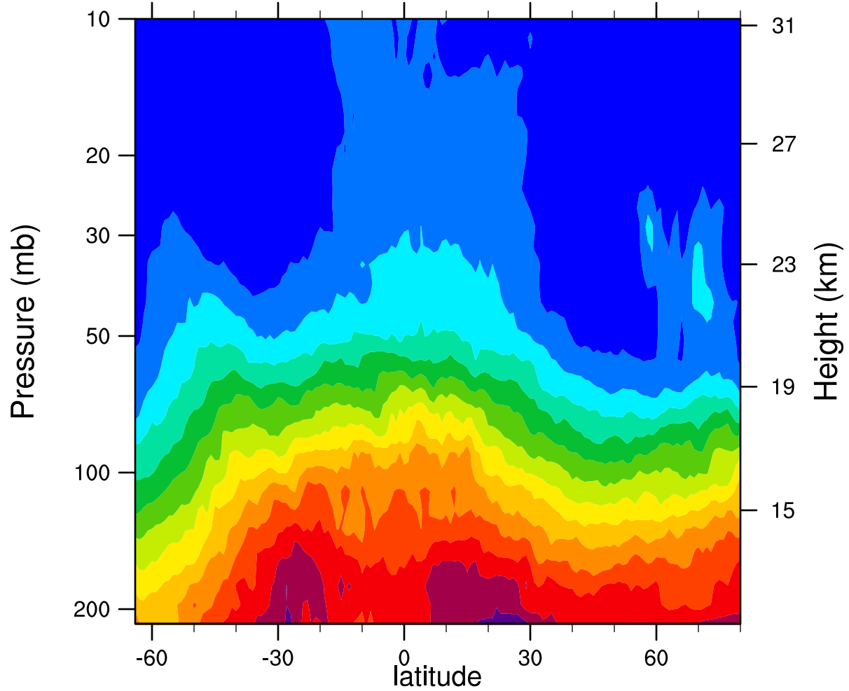
2007d355 12.1MicronExtinction_Combined (km -1 )
