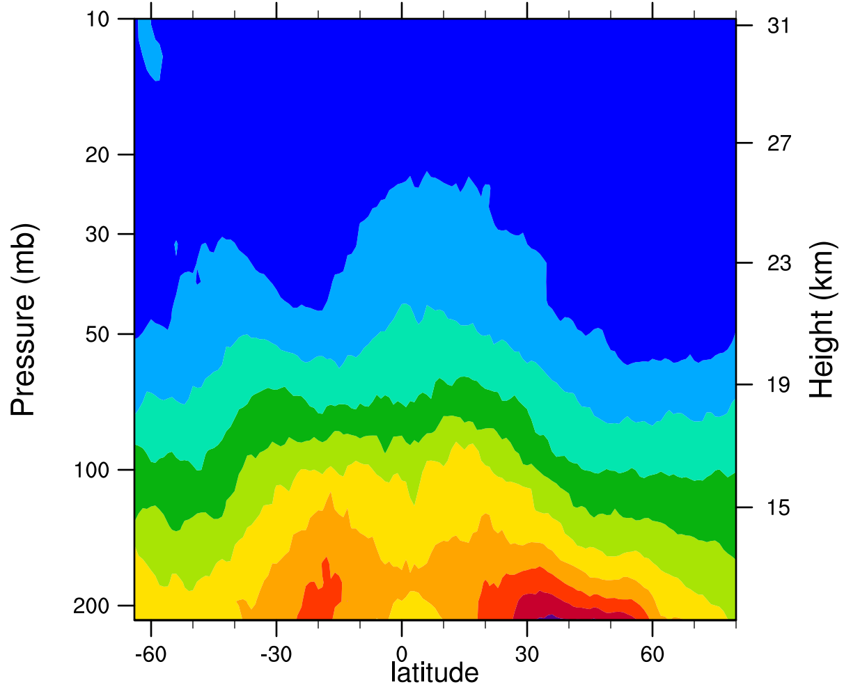
2007d145 12.1MicronExtinction_Combined (km -1 )
