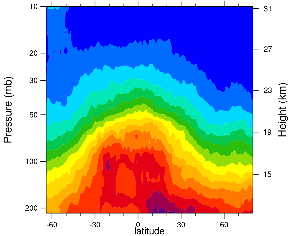
2007d063 12.1MicronExtinction_Combined (km -1 )
