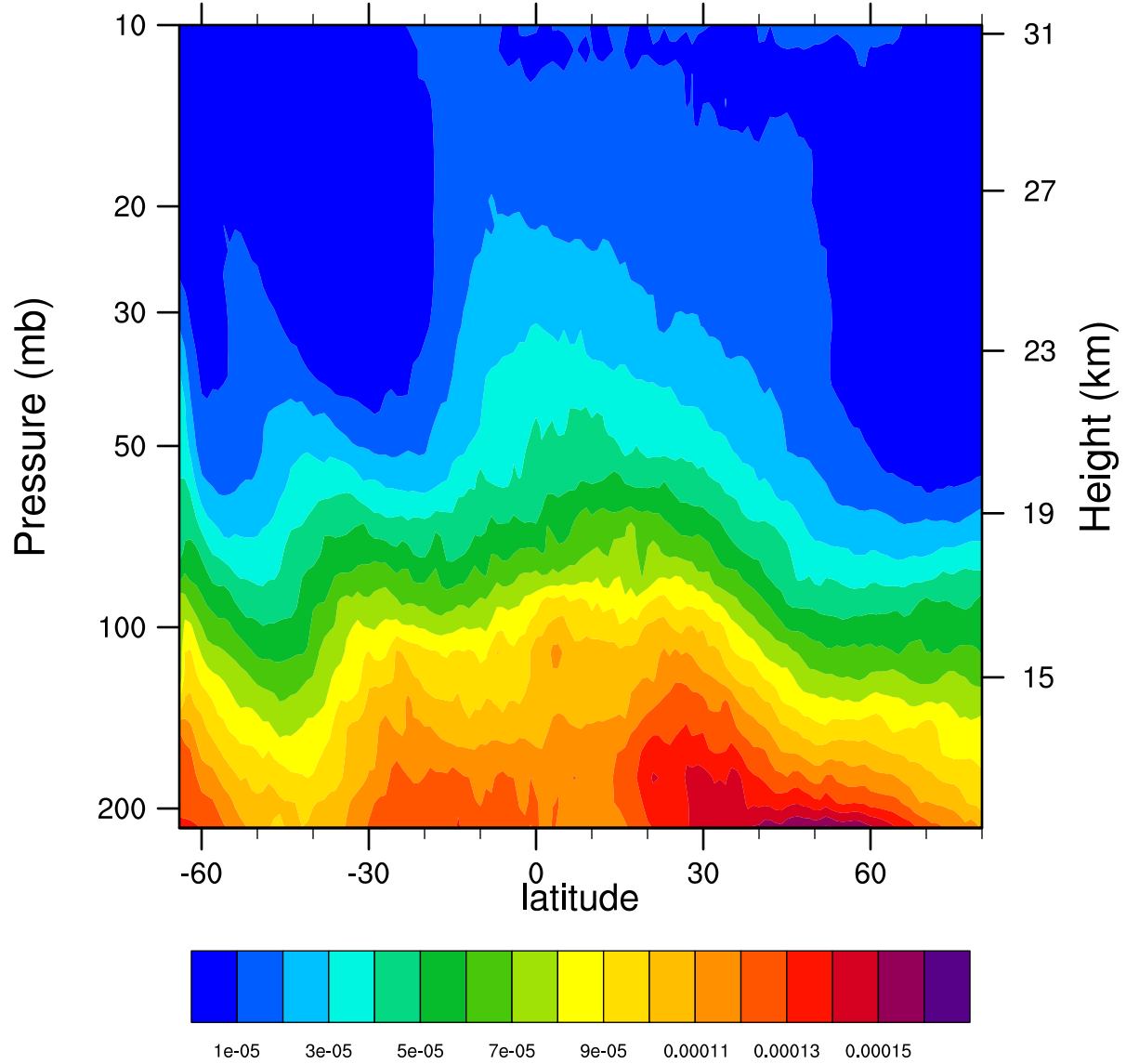
2007d224 12.1MicronExtinction_Combined (km -1 )
