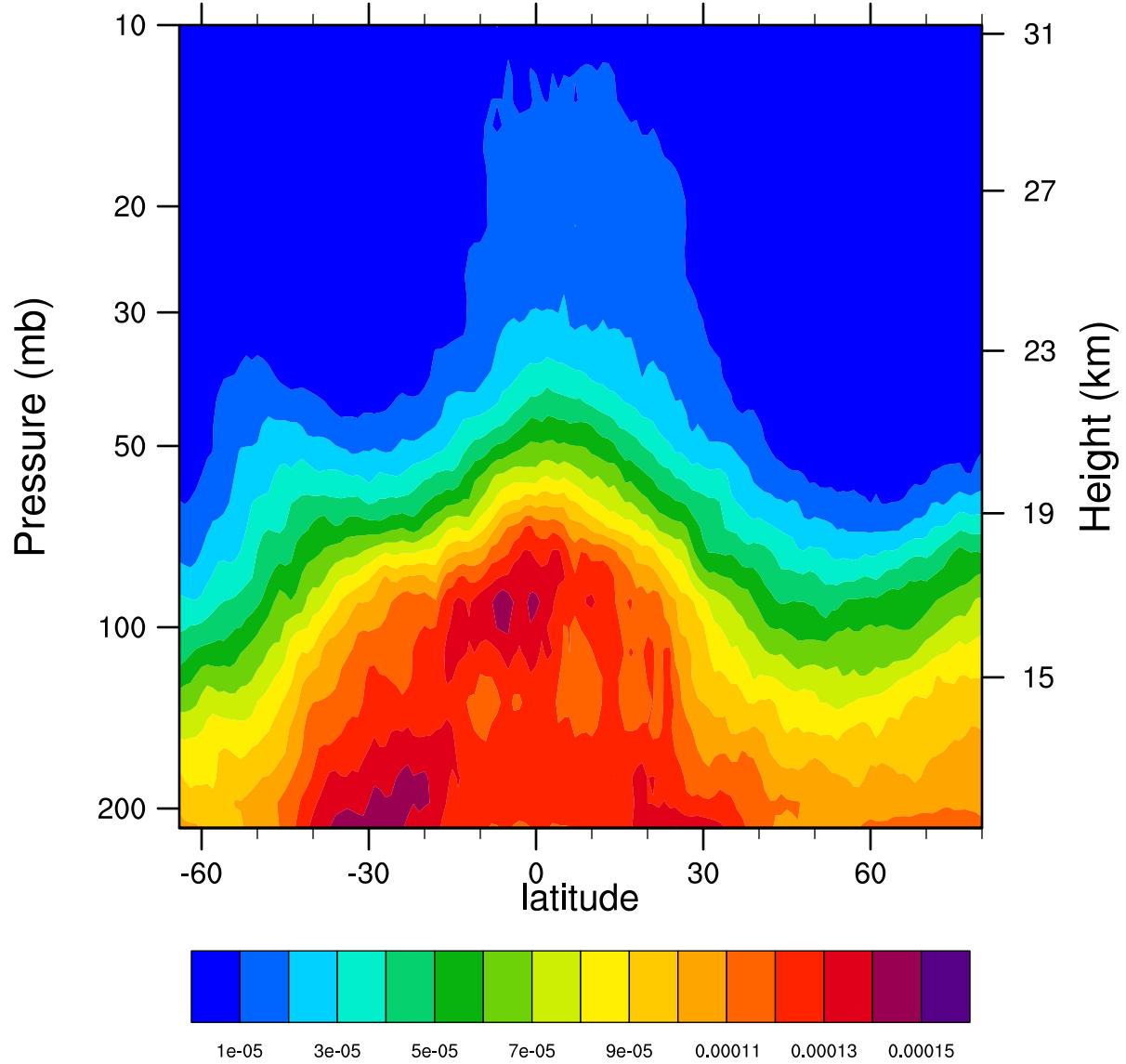
2006d339 12.1MicronExtinction_Combined (km -1 )
