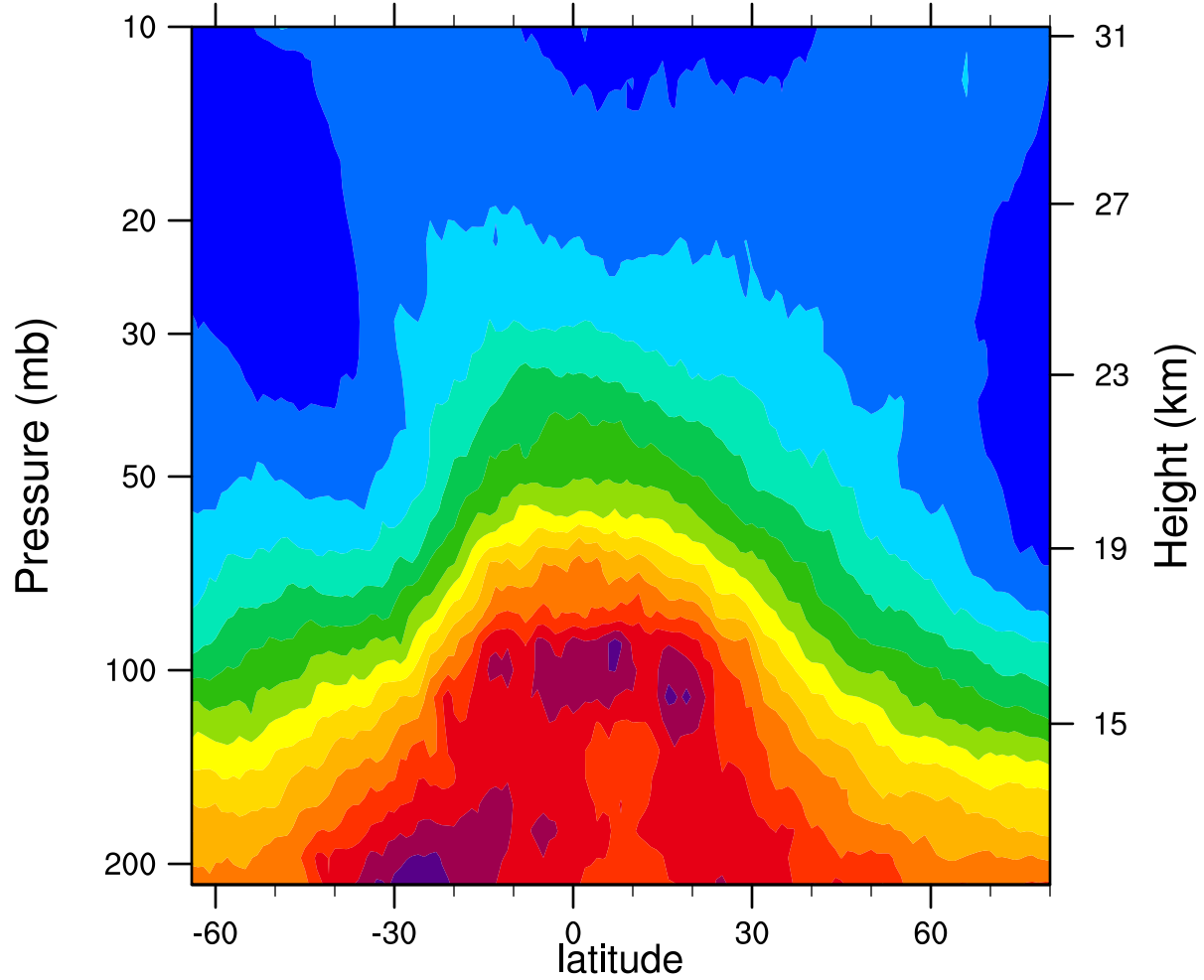
2005d301 12.1MicronExtinction_Combined (km -1 )
