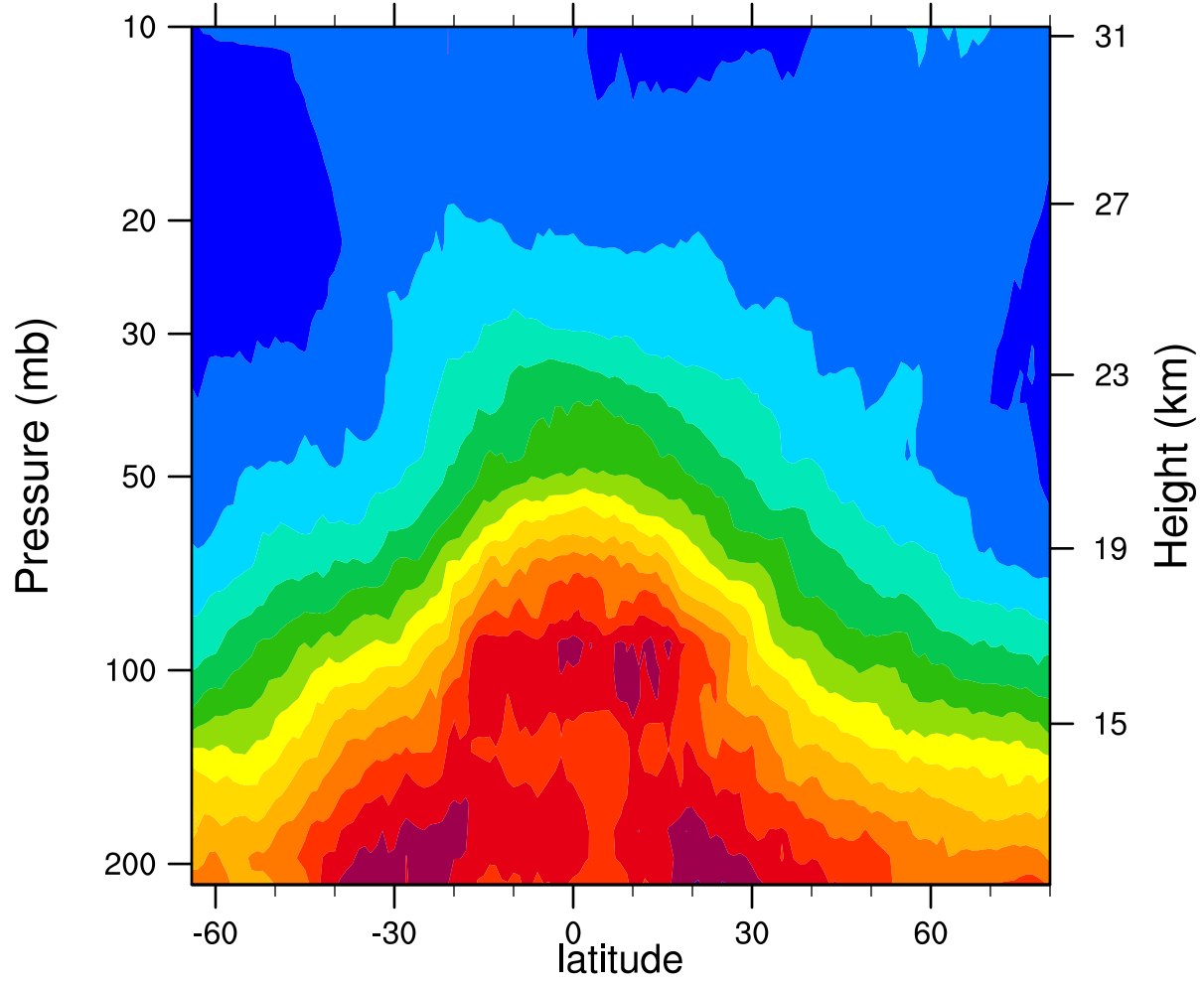
2005d329 12.1MicronExtinction_Combined (km -1 )
