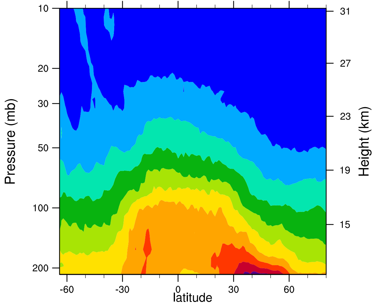
2007d166 12.1MicronExtinction_Combined (km -1 )
