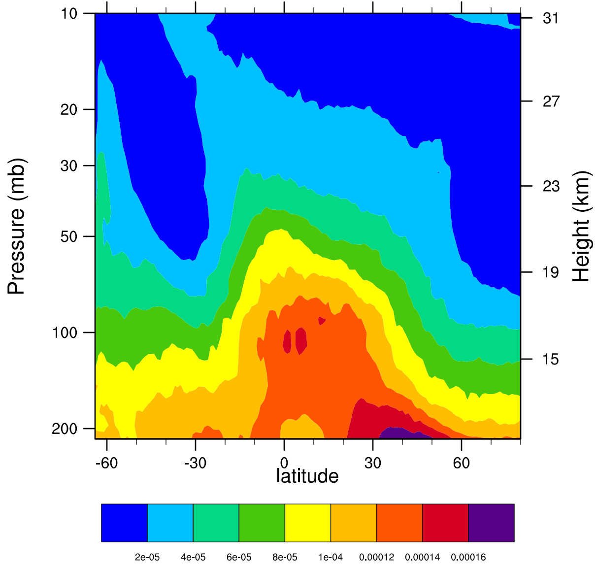
2005d178 12.1MicronExtinction_Combined (km -1 )
