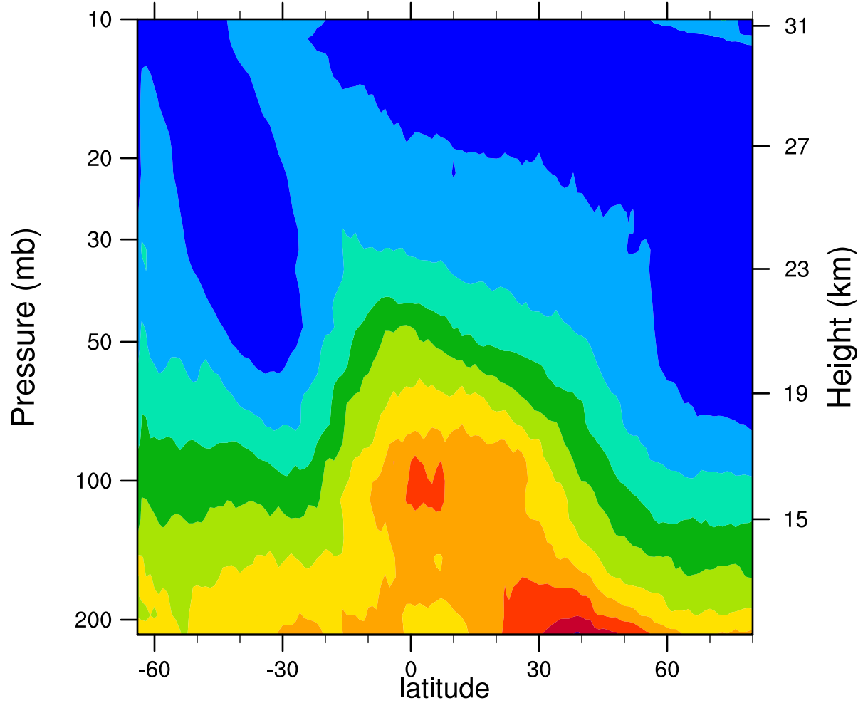
2005d175 12.1MicronExtinction_Combined (km -1 )
