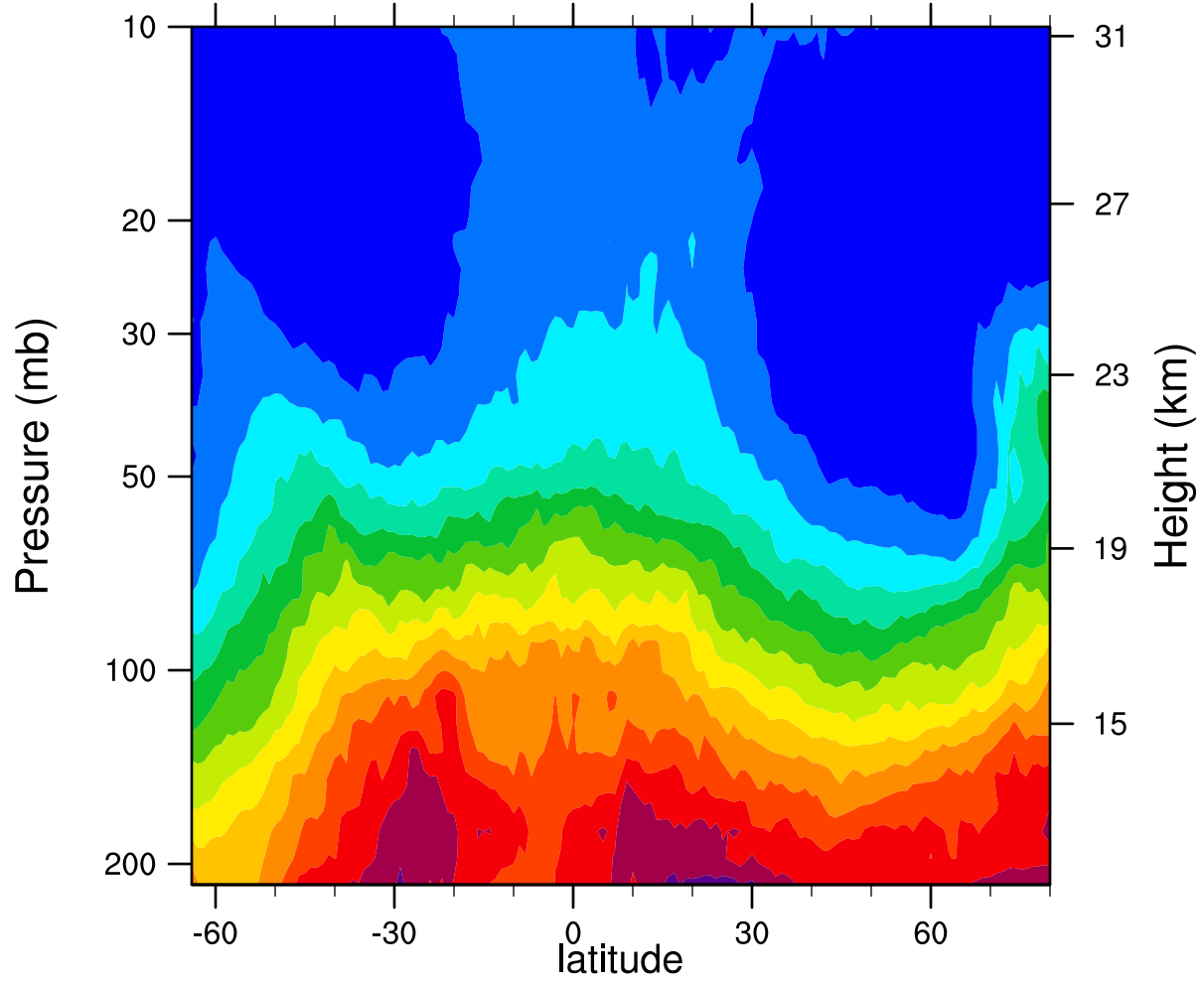
2007d361 12.1MicronExtinction_Combined ( \text{km}^{-1} )
