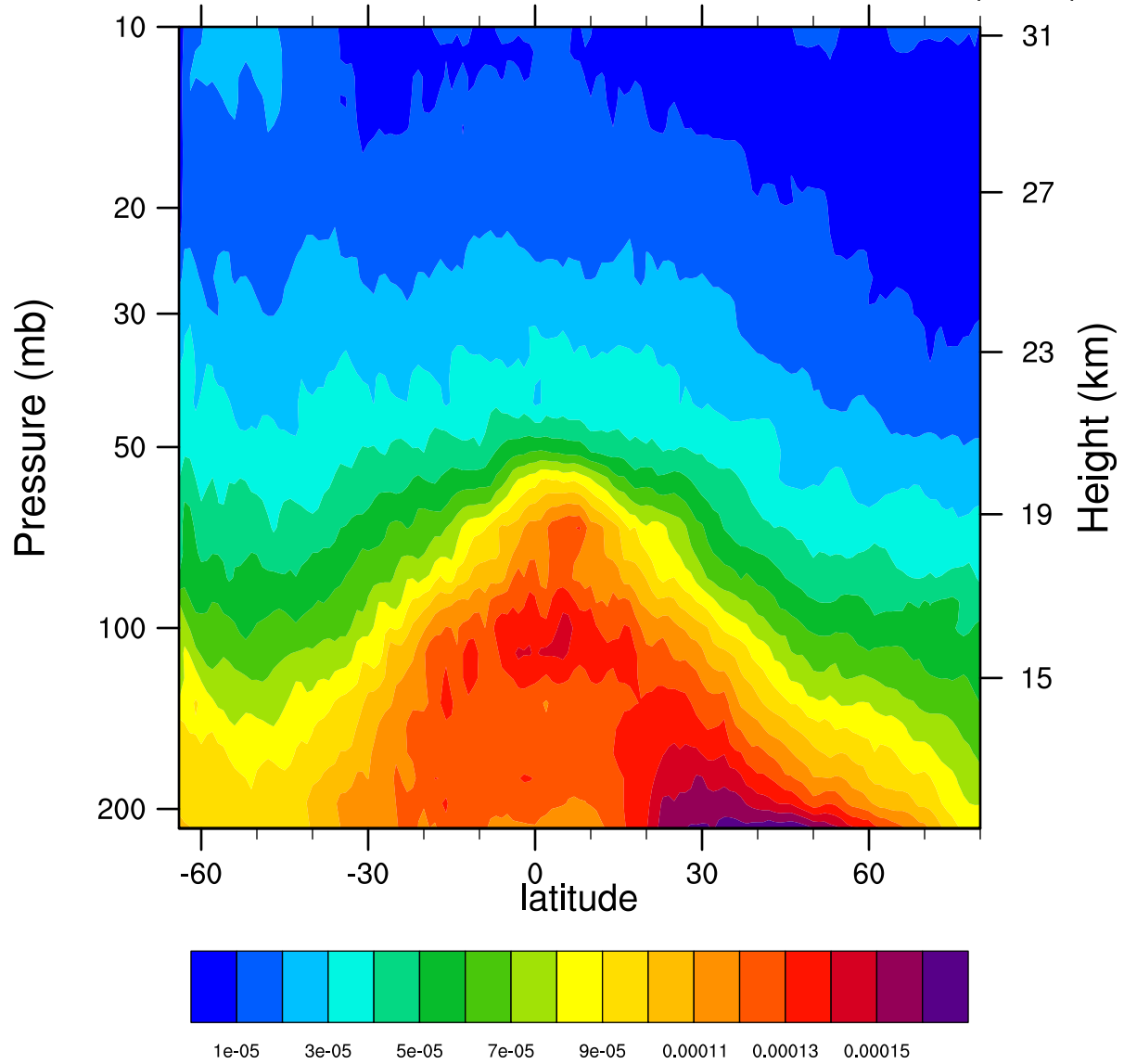
2006d174 12.1MicronExtinction_Combined (km -1 )
