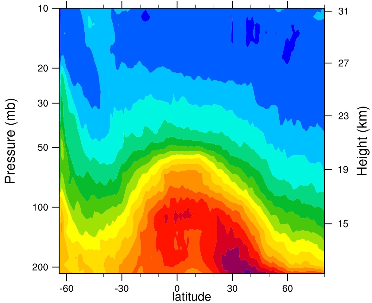
2006d212 12.1MicronExtinction_Combined (km -1 )
