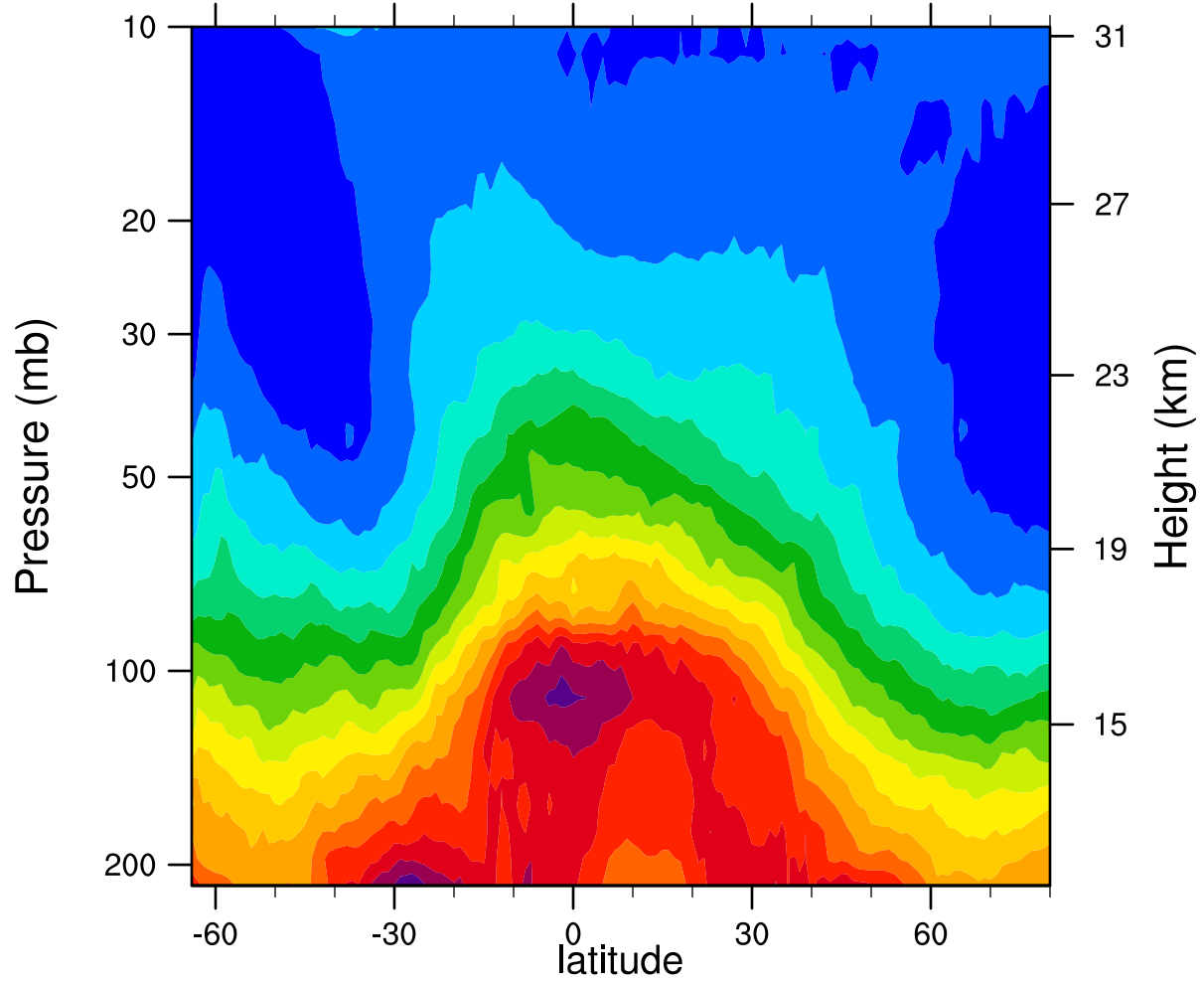
2005d259 12.1MicronExtinction_Combined (km -1 )
