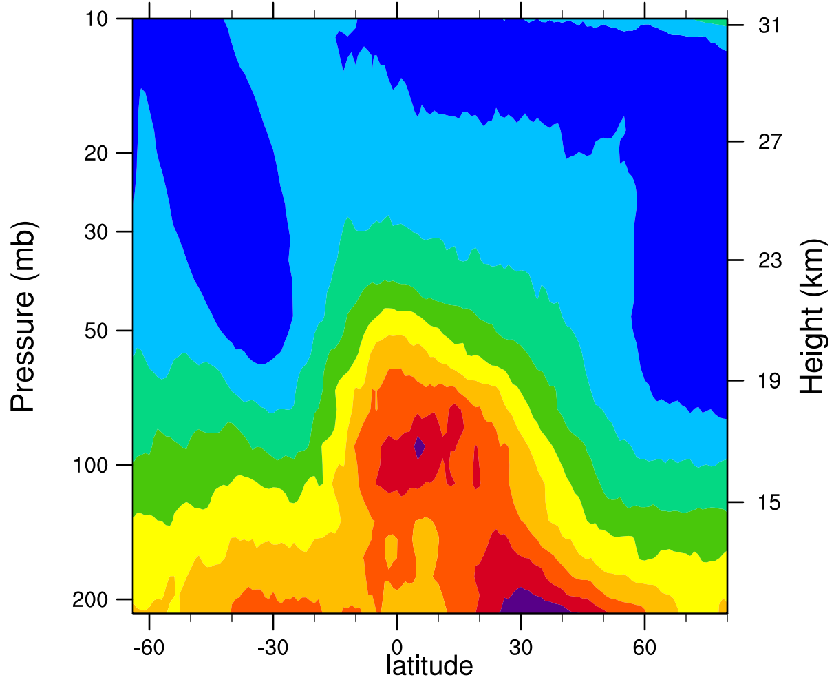
2005d154 12.1MicronExtinction_Combined (km -1 )
