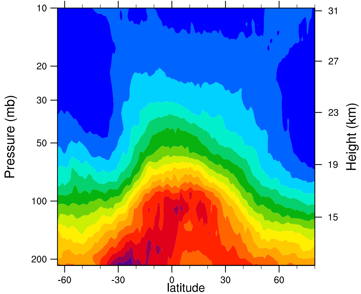
2005d284 12.1MicronExtinction_Combined (km -1 )
