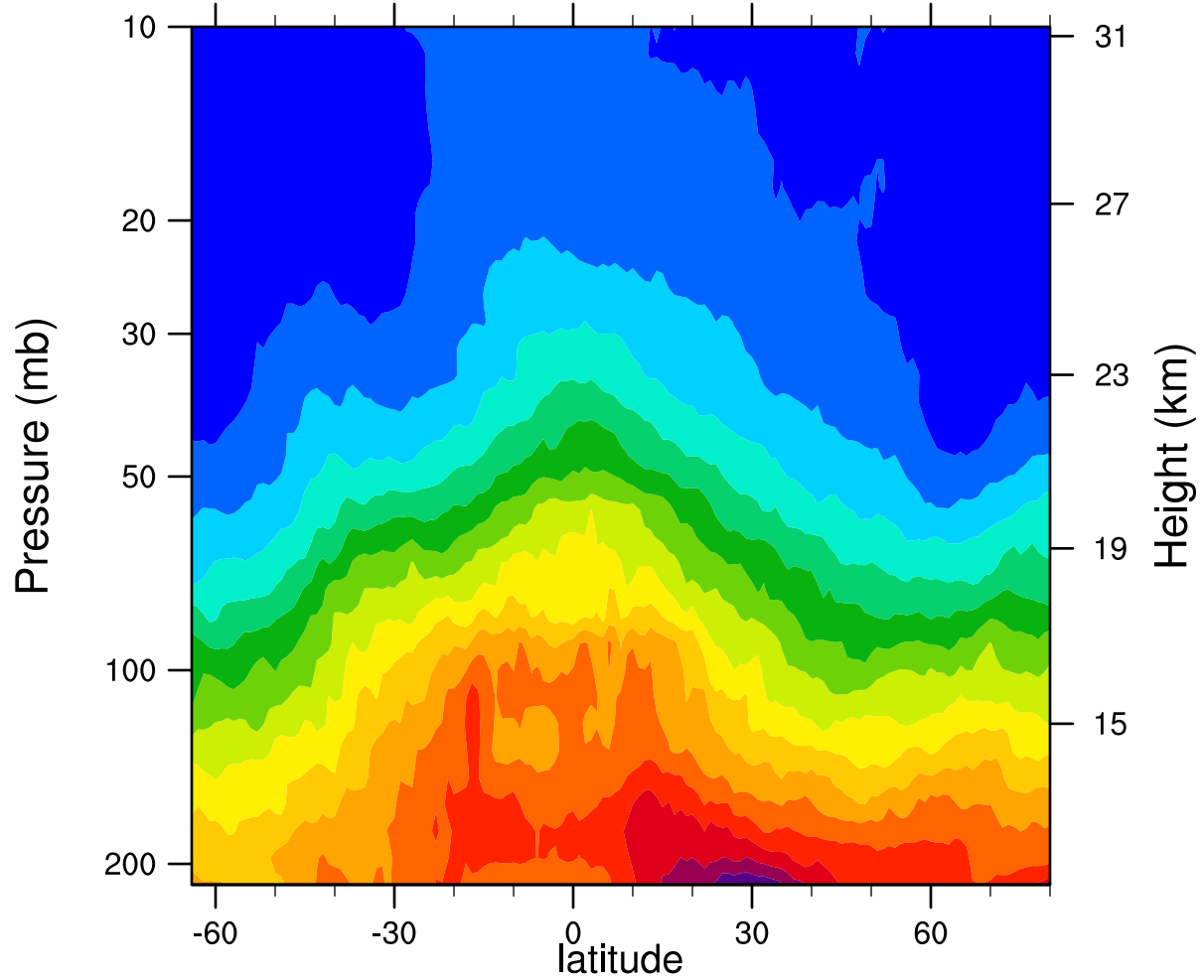
2007d093 12.1MicronExtinction_Combined (km -1 )
