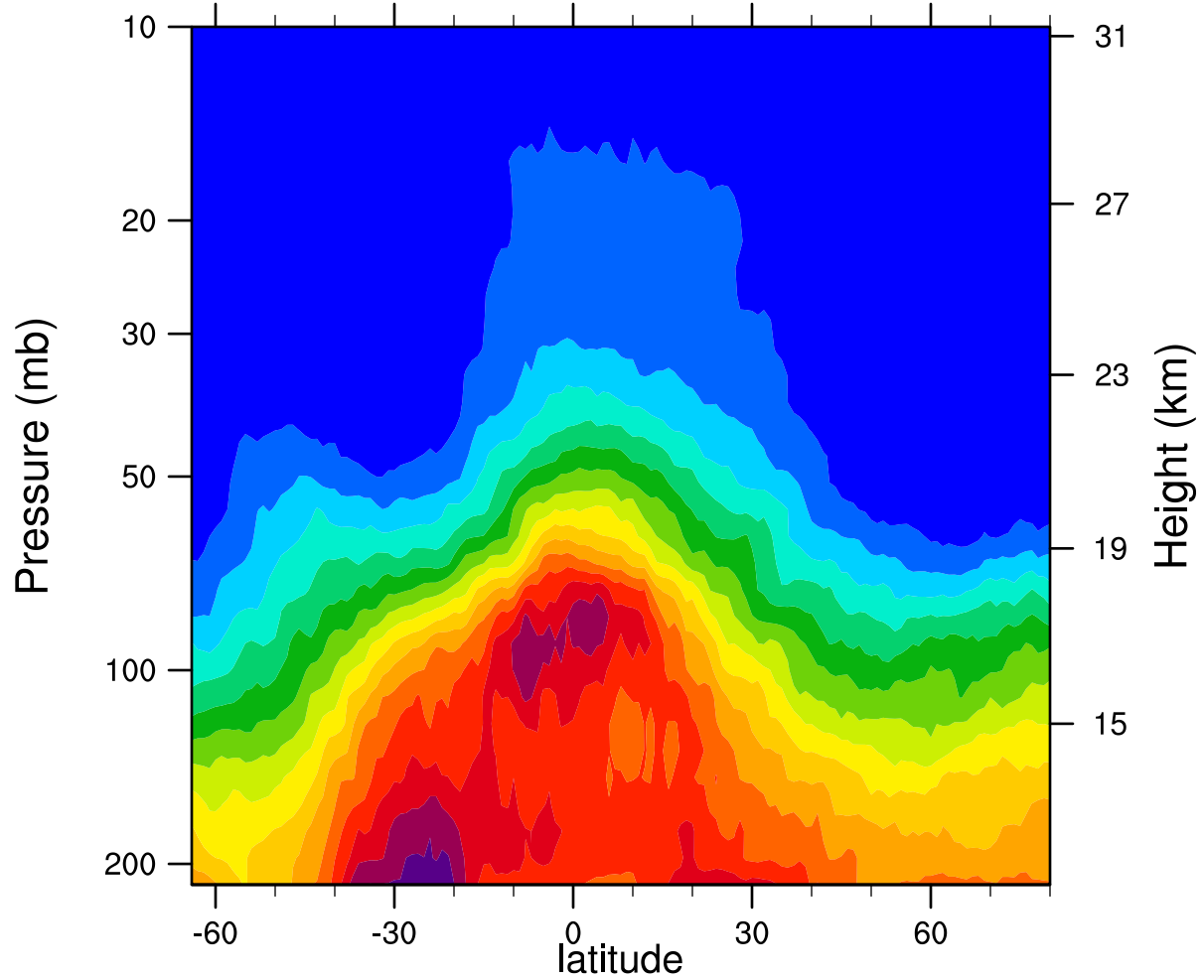
2006d328 12.1MicronExtinction_Combined (km -1 )
