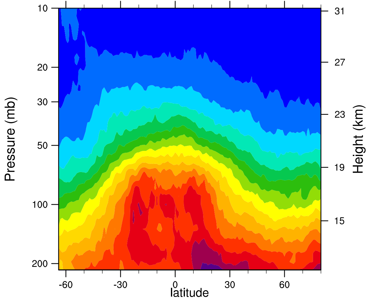
2007d070 12.1MicronExtinction_Combined (km -1 )
