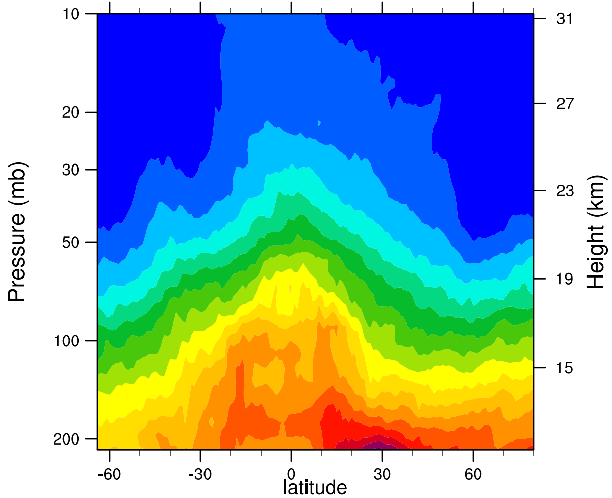
2007d096 12.1MicronExtinction_Combined ( \text{km}^{-1} )
