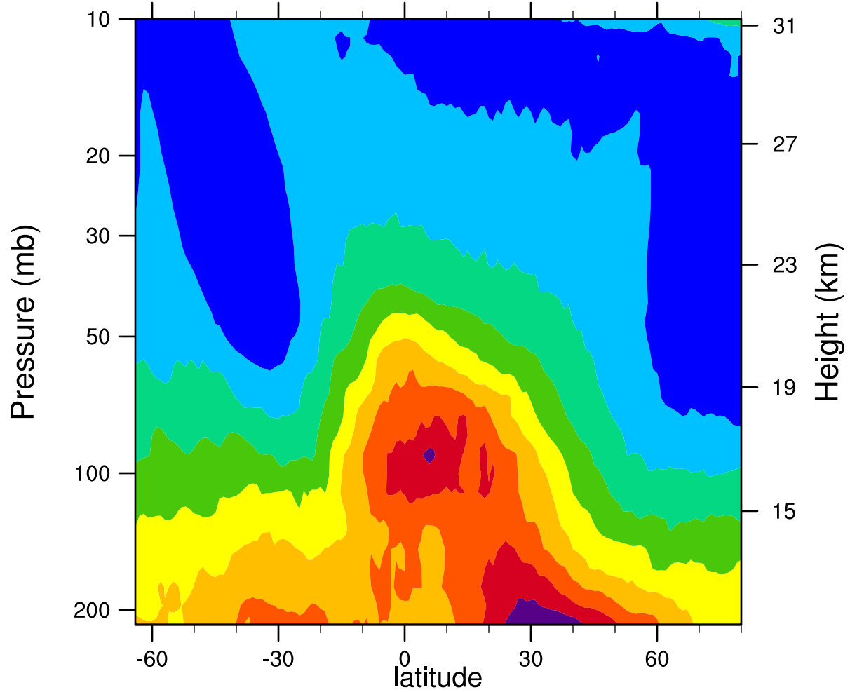
2005d152 12.1MicronExtinction_Combined (km -1 )
