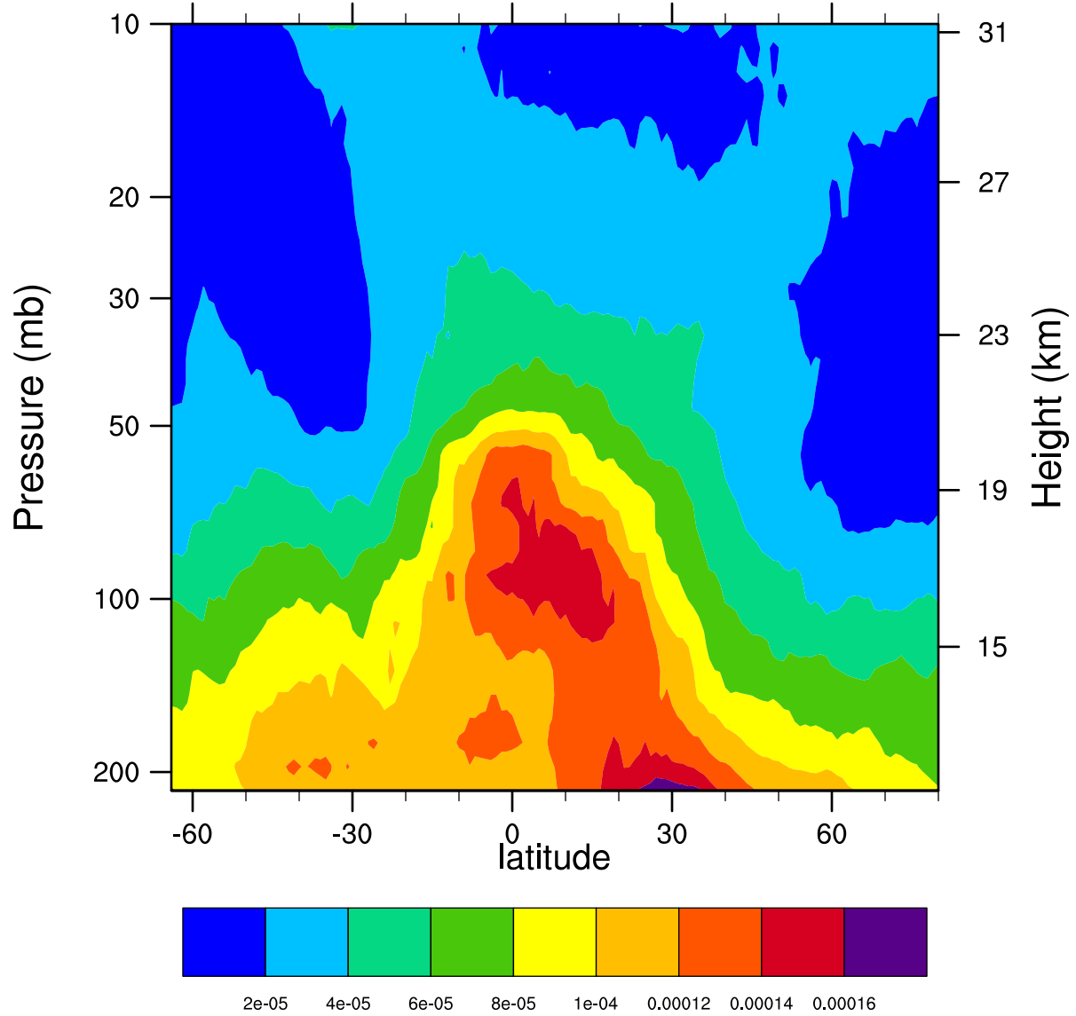
2005d111 12.1MicronExtinction_Combined (km -1 )
