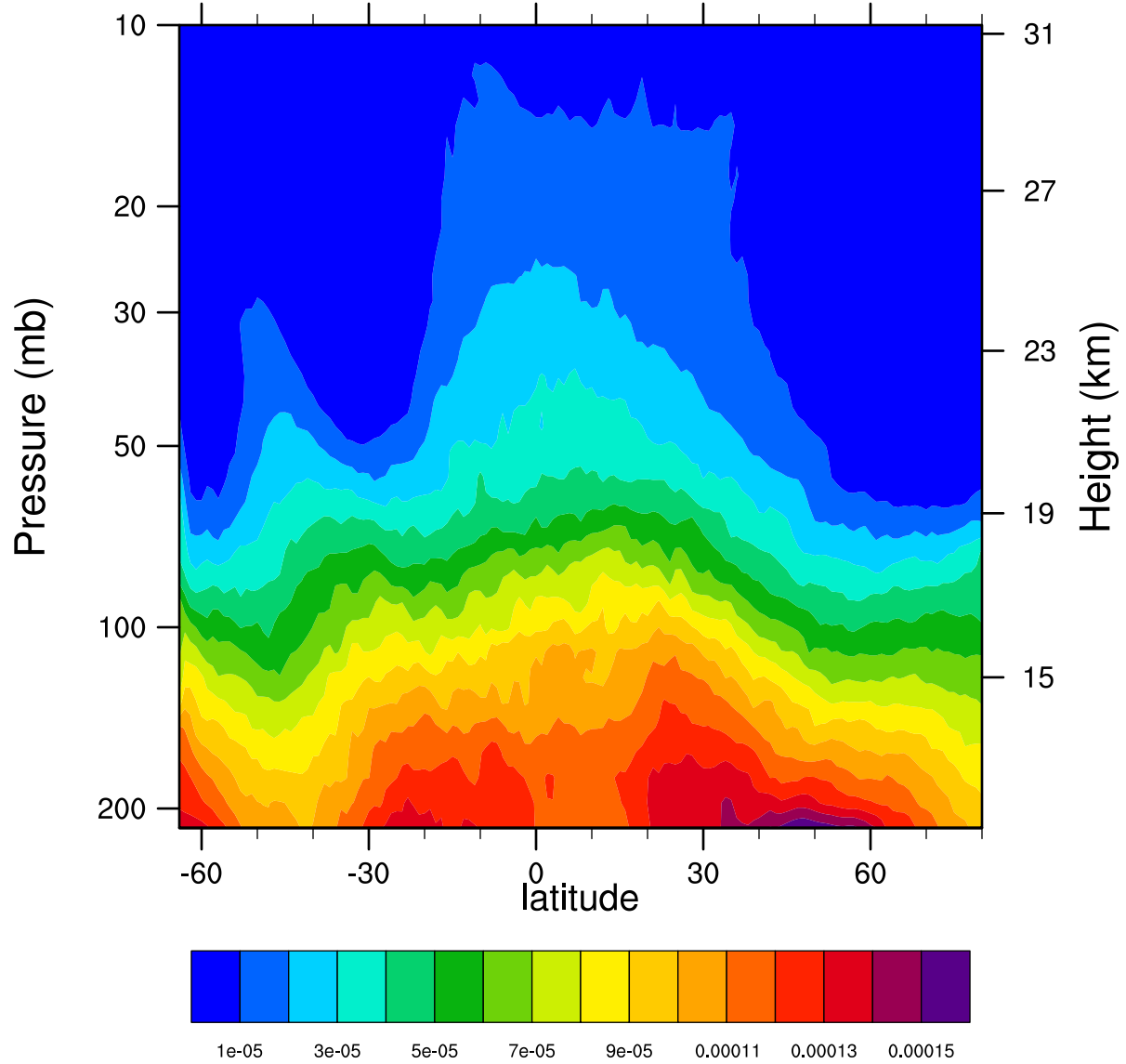
2007d240 12.1MicronExtinction_Combined (km -1 )
