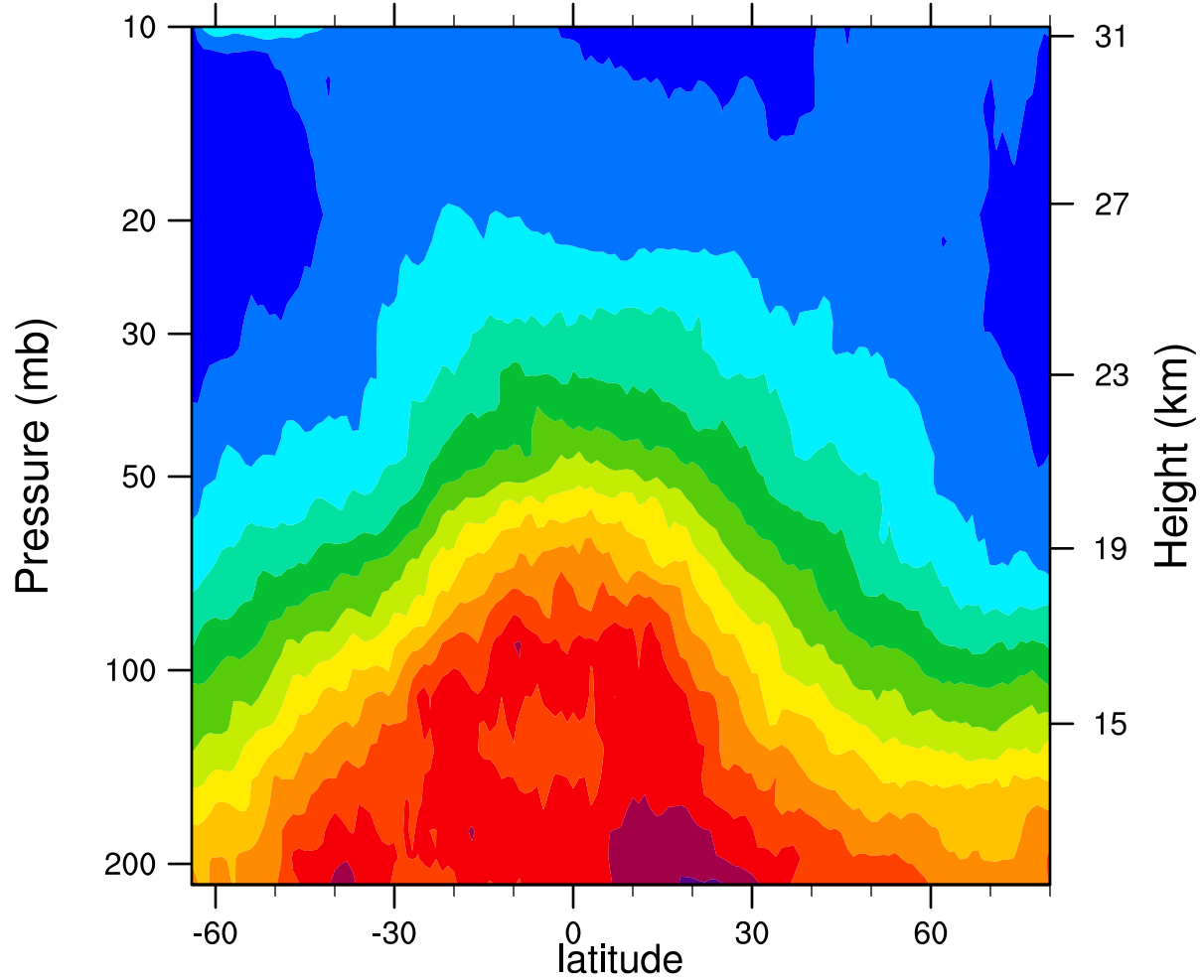
2006d021 12.1MicronExtinction_Combined (km -1 )
