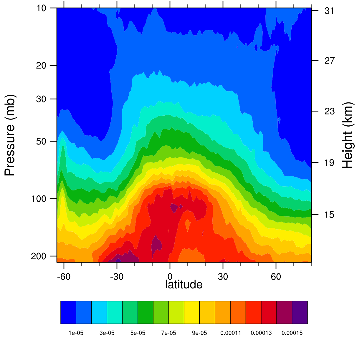
2005d278 12.1MicronExtinction_Combined ( \text{km}^{-1} )
