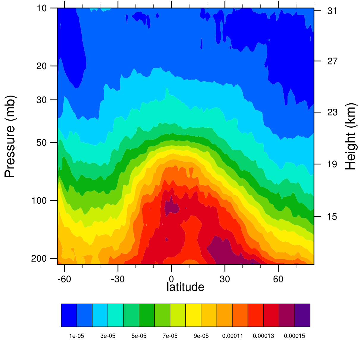
2006d234 12.1MicronExtinction_Combined (km -1 )
