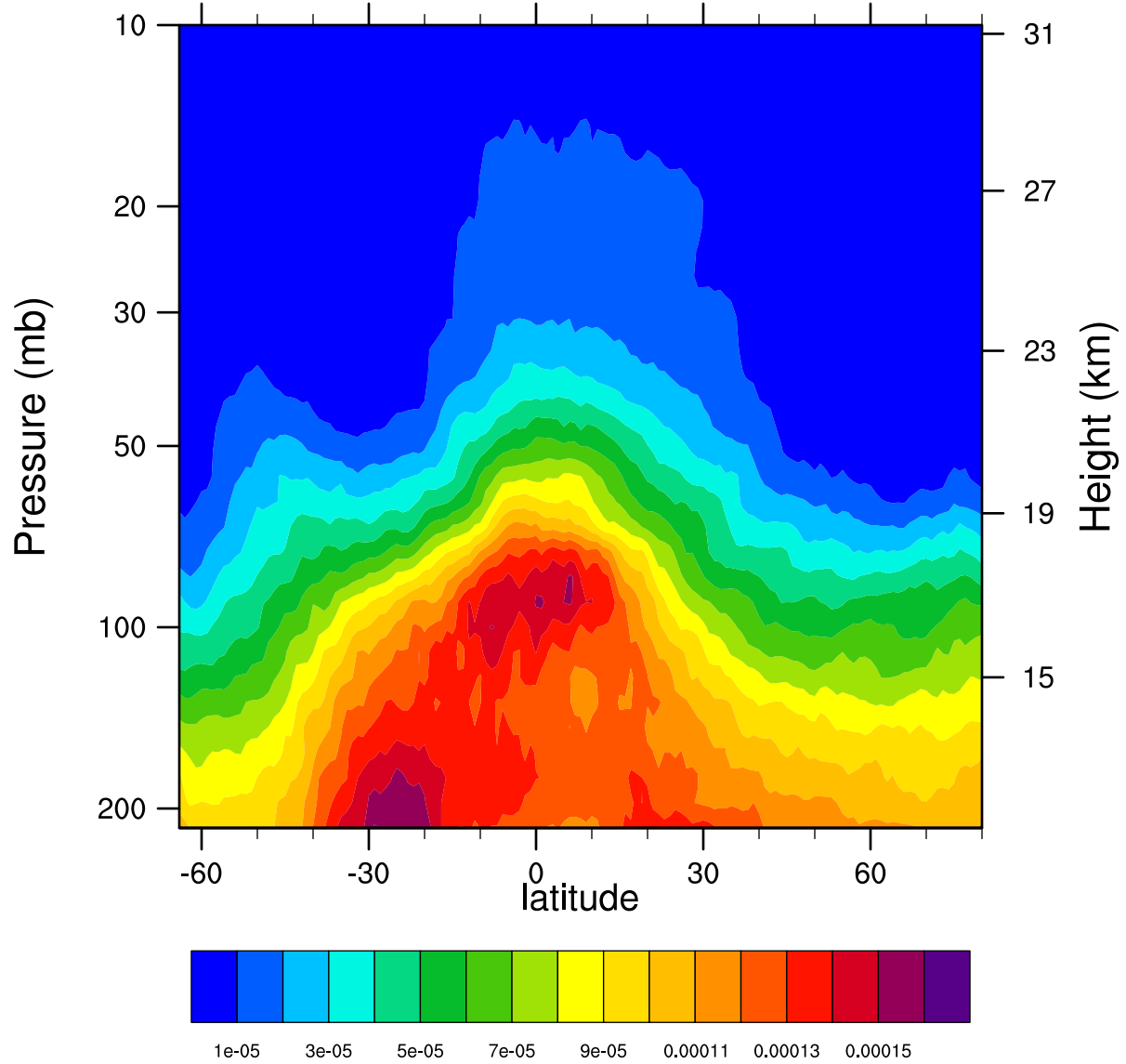
2006d324 12.1MicronExtinction_Combined ( \text{km}^{-1} )
