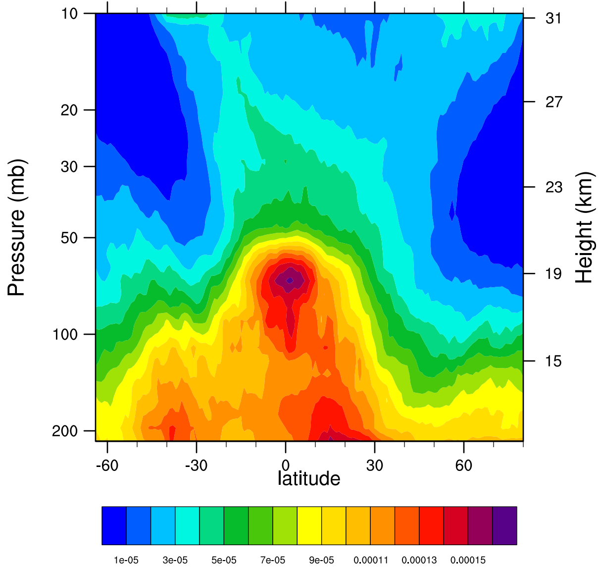
2005d068 12.1MicronExtinction_Combined ( \text{km}^{-1} )
