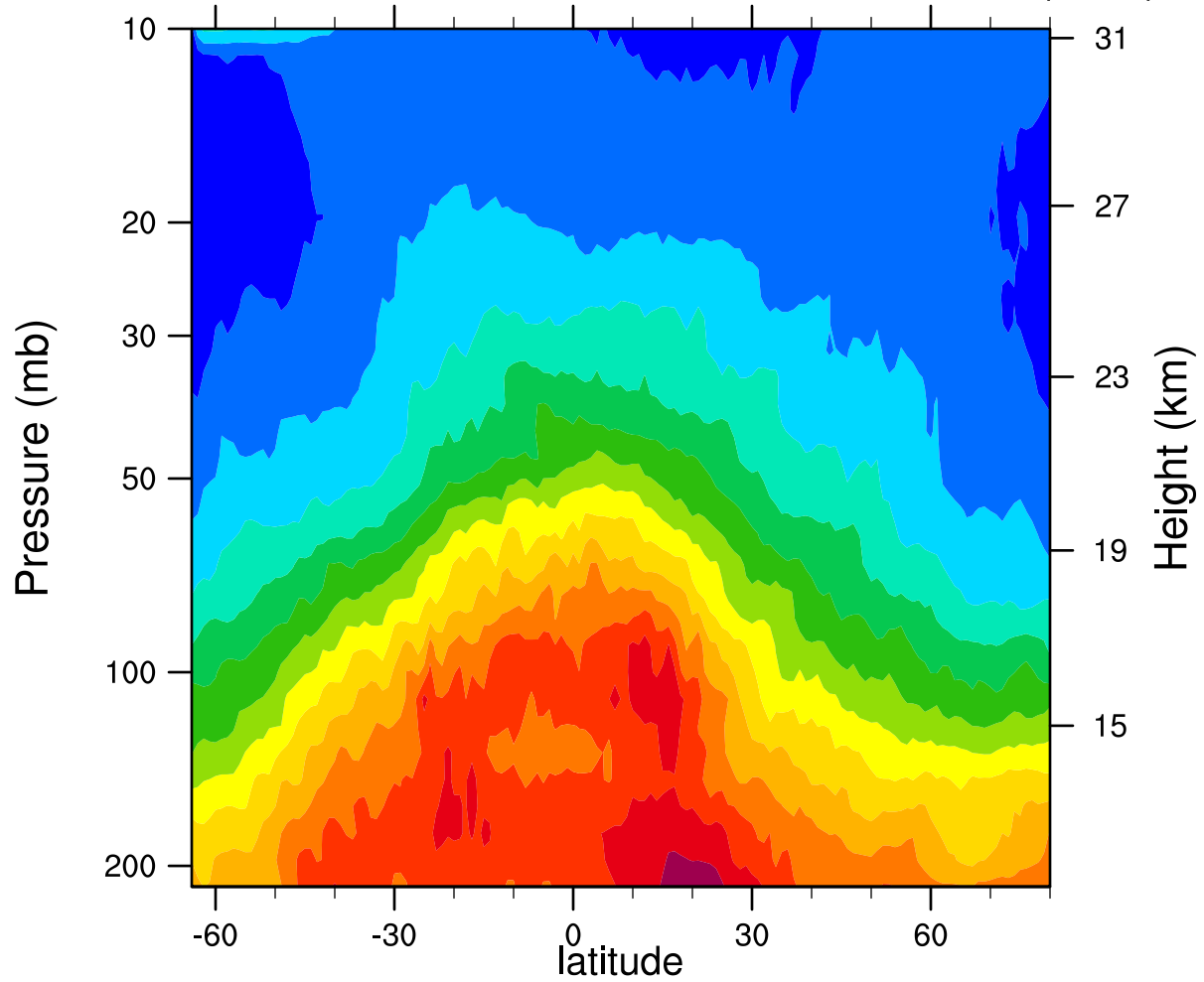
2006d016 12.1MicronExtinction_Combined (km -1 )
