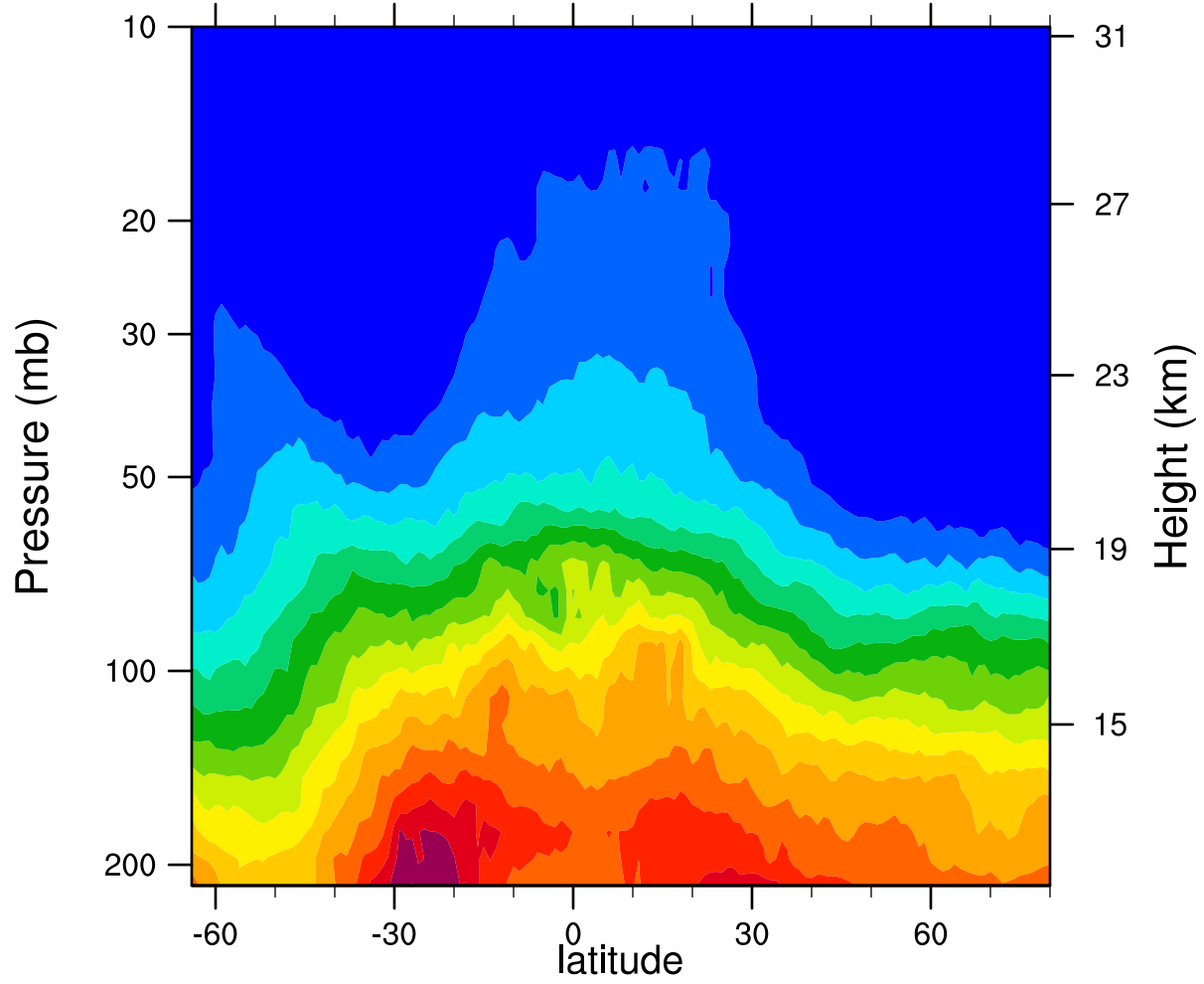
2007d317 12.1MicronExtinction_Combined (km -1 )
