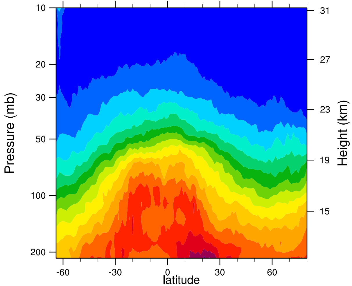
2007d051 12.1MicronExtinction_Combined ( \text{km}^{-1} )
