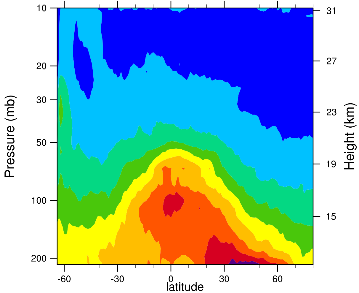
2006d181 12.1MicronExtinction_Combined (km -1 )
