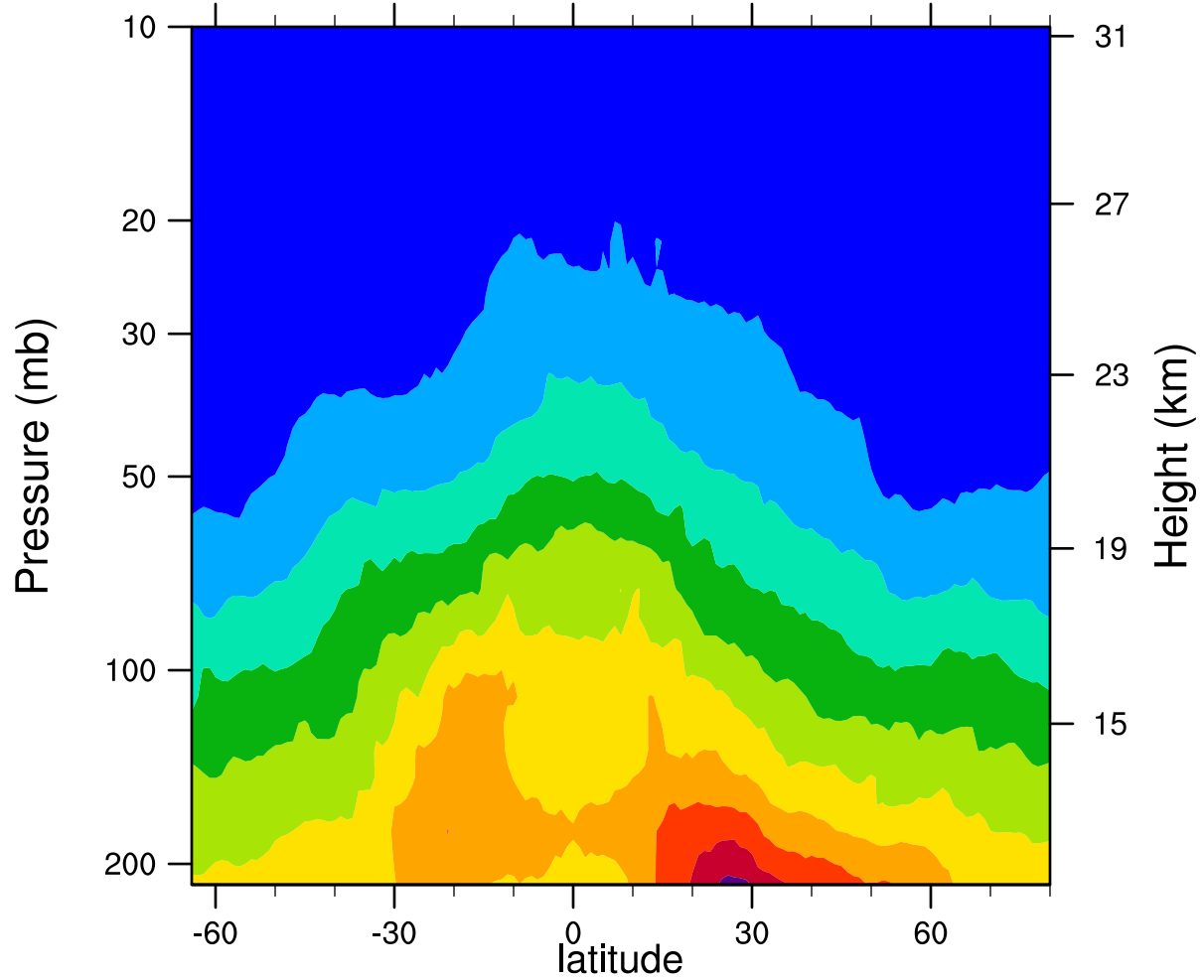
2007d113 12.1MicronExtinction_Combined (km -1 )
