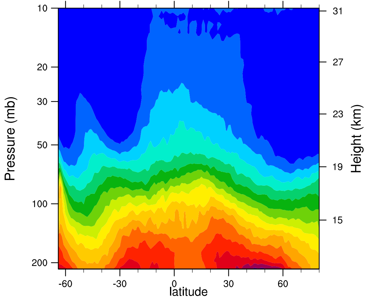
2007d247 12.1MicronExtinction_Combined (km -1 )
