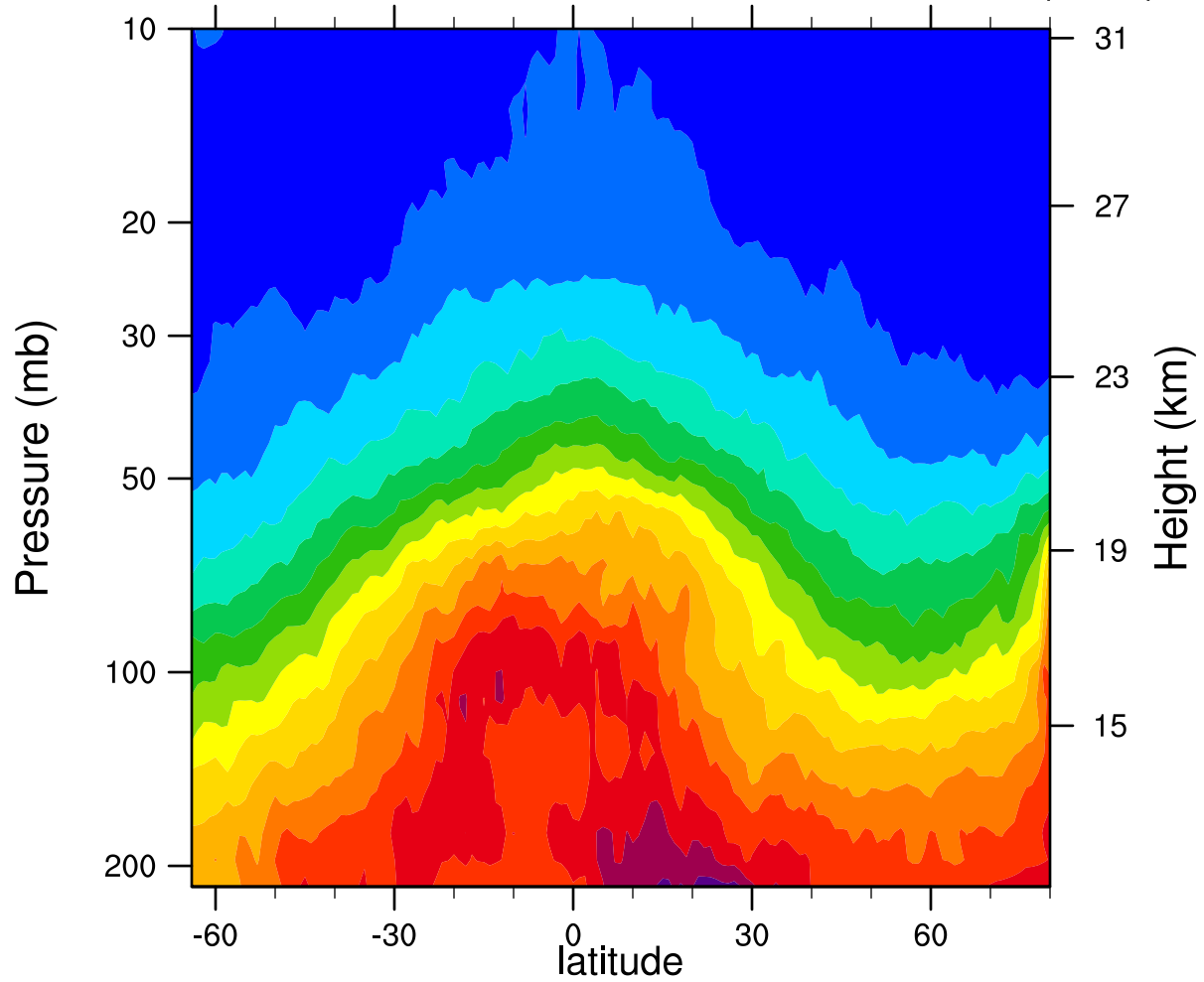
2007d046 12.1MicronExtinction_Combined (km -1 )
