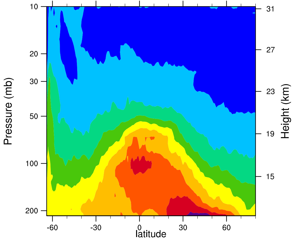
2006d183 12.1MicronExtinction_Combined (km -1 )
