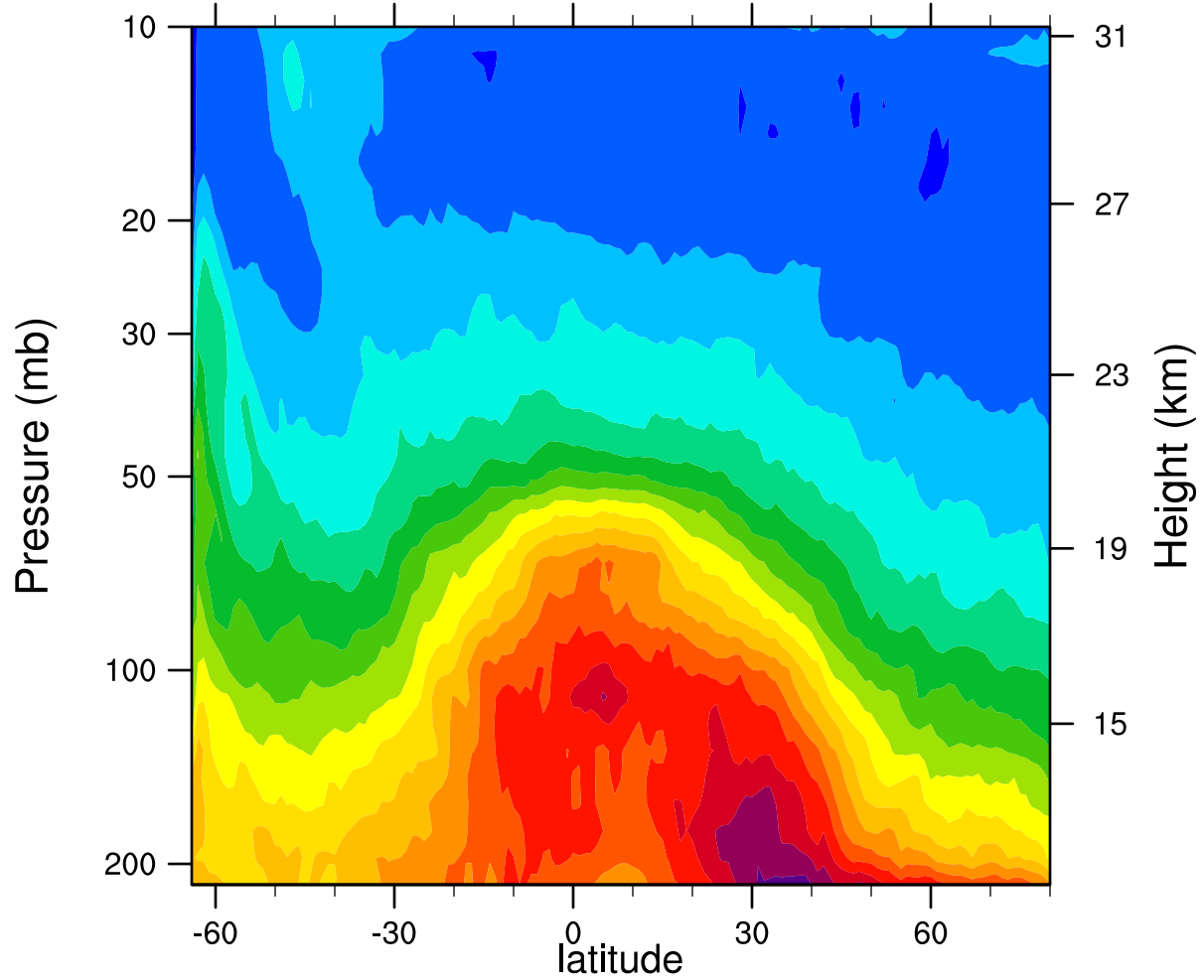
2006d206 12.1MicronExtinction_Combined (km -1 )
