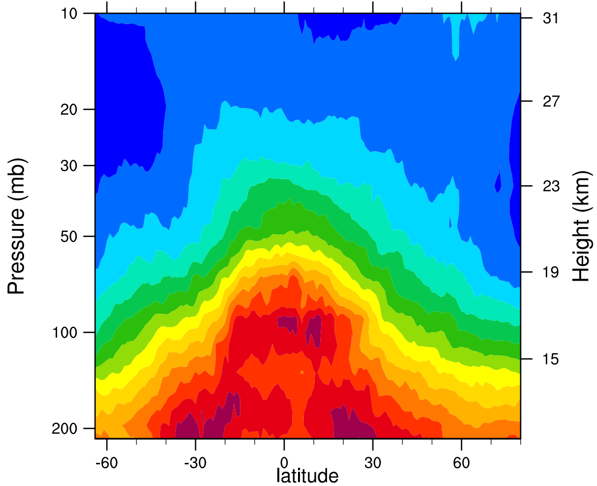
2005d332 12.1MicronExtinction_Combined (km -1 )
