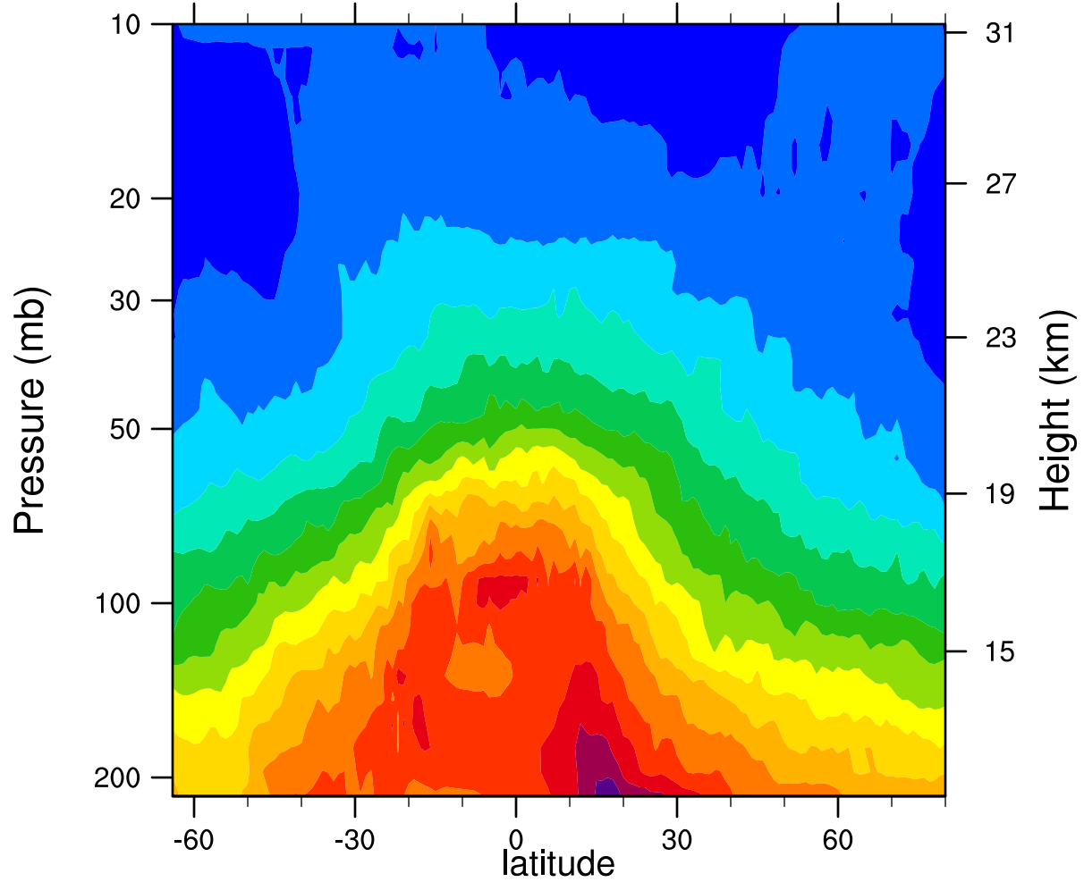
2006d052 12.1MicronExtinction_Combined (km -1 )
