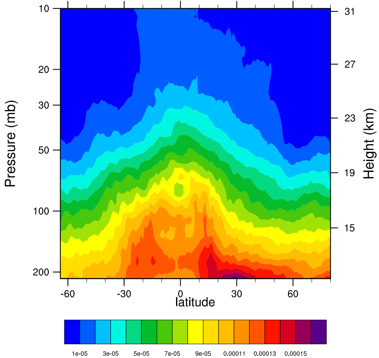
2007d103 12.1MicronExtinction_Combined ( \text{km}^{-1} )
