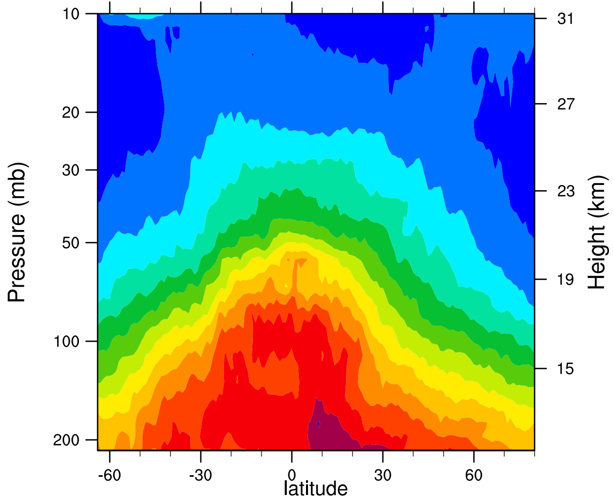
2006d031 12.1MicronExtinction_Combined (km -1 )
