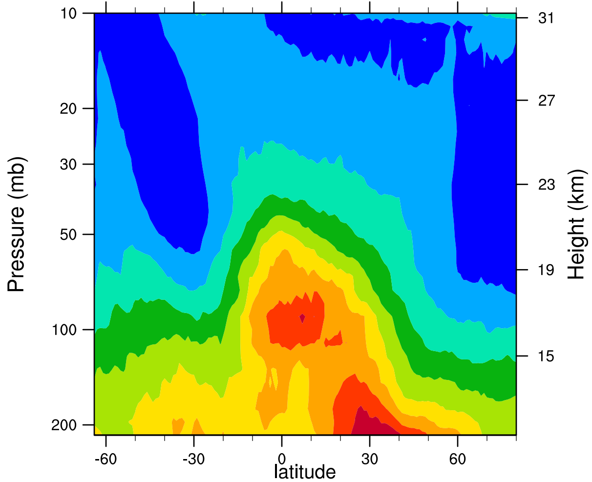
2005d146 12.1MicronExtinction_Combined (km -1 )
