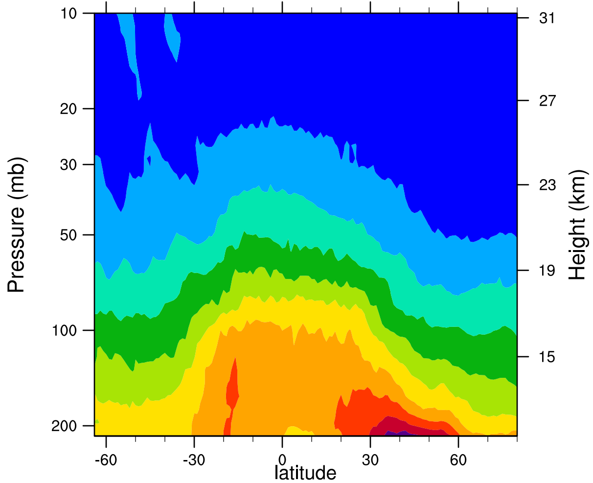
2007d165 12.1MicronExtinction_Combined (km -1 )
