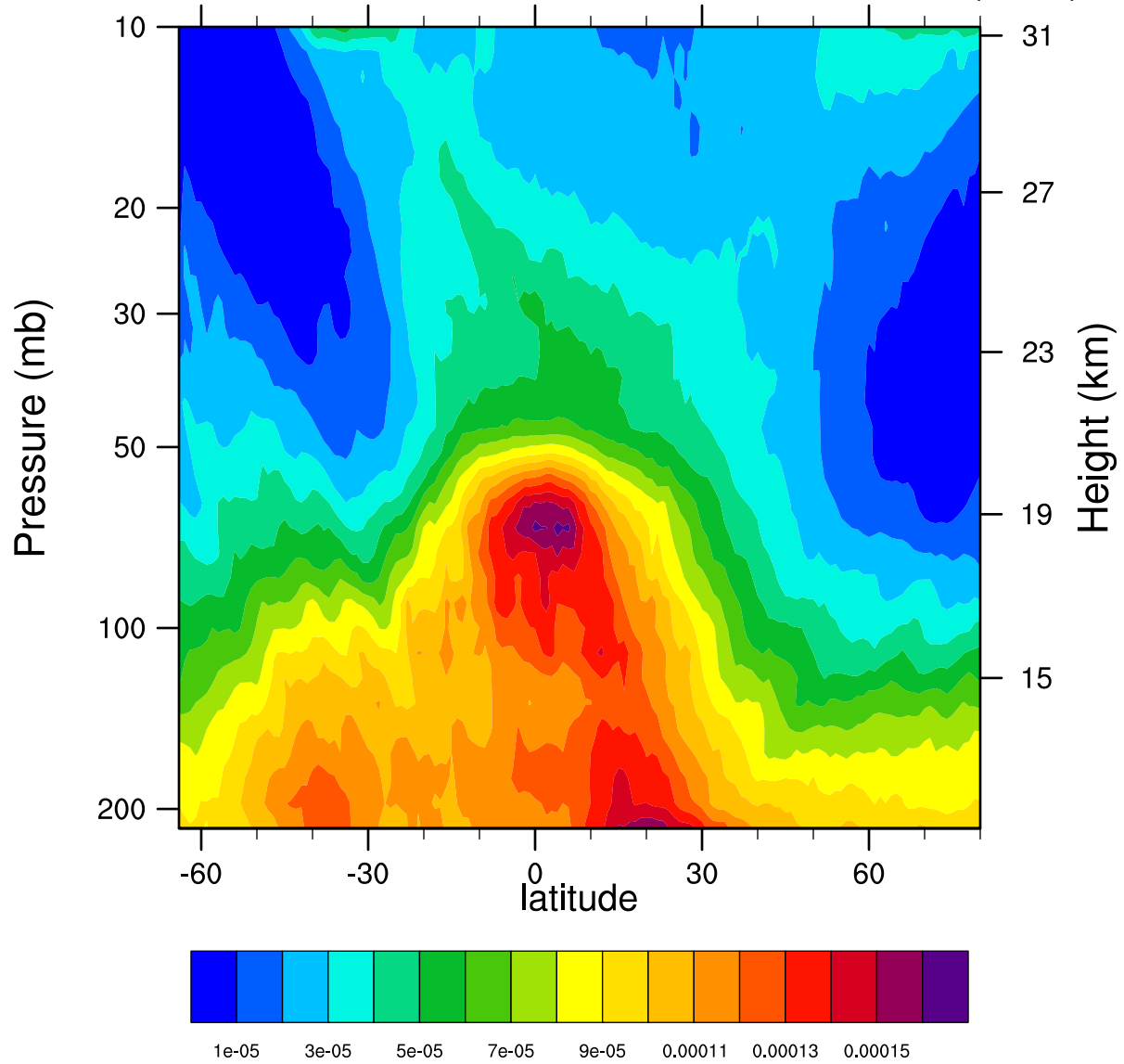
2005d075 12.1MicronExtinction_Combined (km -1 )
