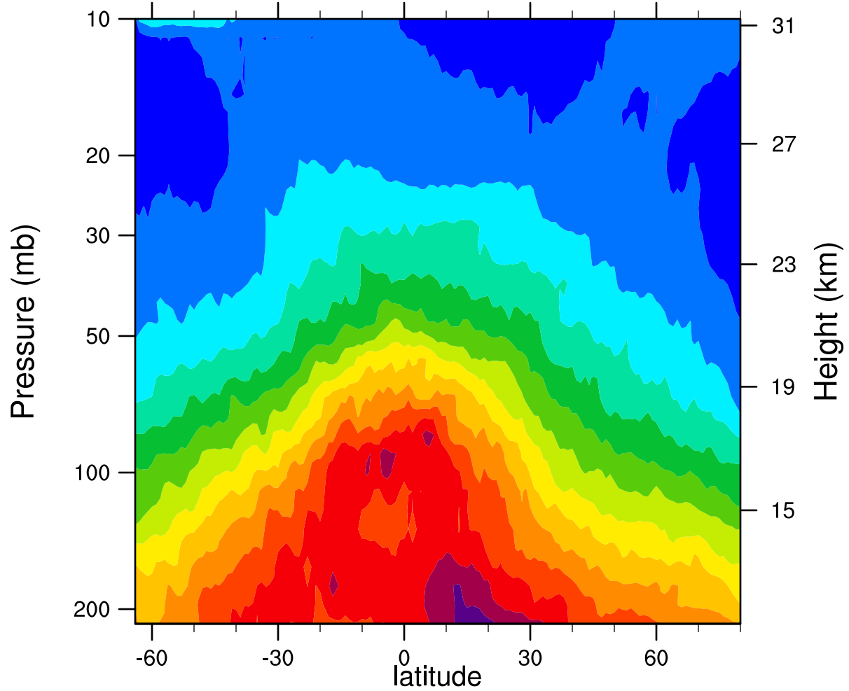
2006d042 12.1MicronExtinction_Combined (km -1 )
