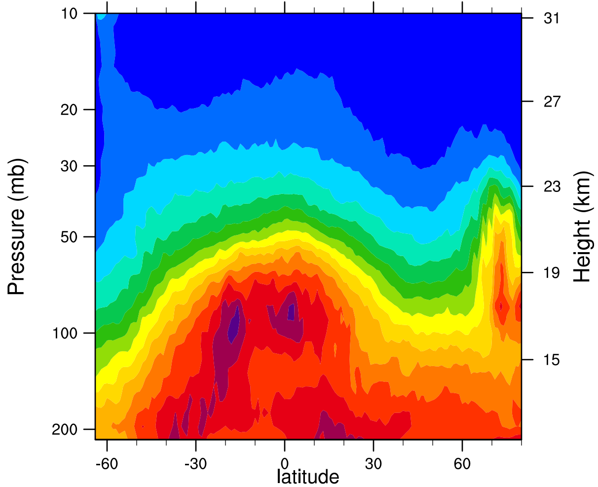
2007d028 12.1MicronExtinction_Combined ( \text{km}^{-1} )
