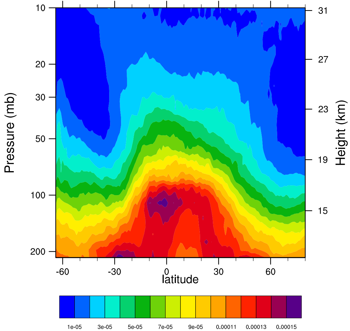
2005d256 12.1MicronExtinction_Combined (km -1 )
