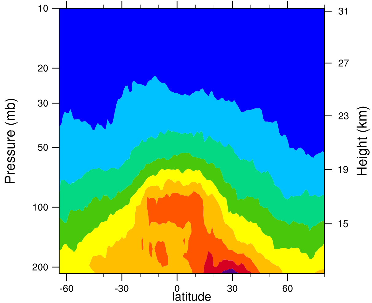
2006d102 12.1MicronExtinction_Combined (km -1 )
