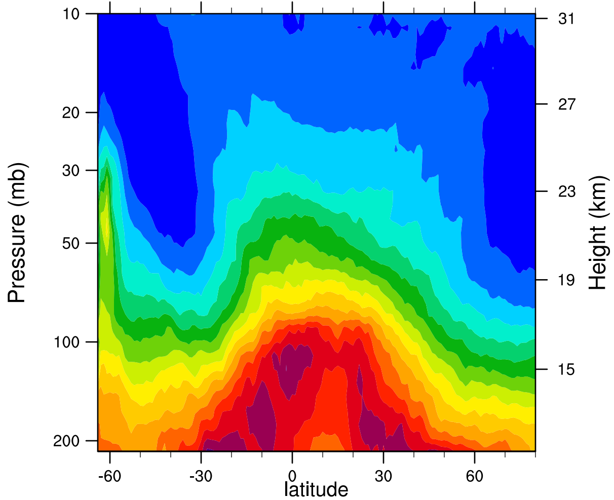
2005d243 12.1MicronExtinction_Combined (km -1 )
