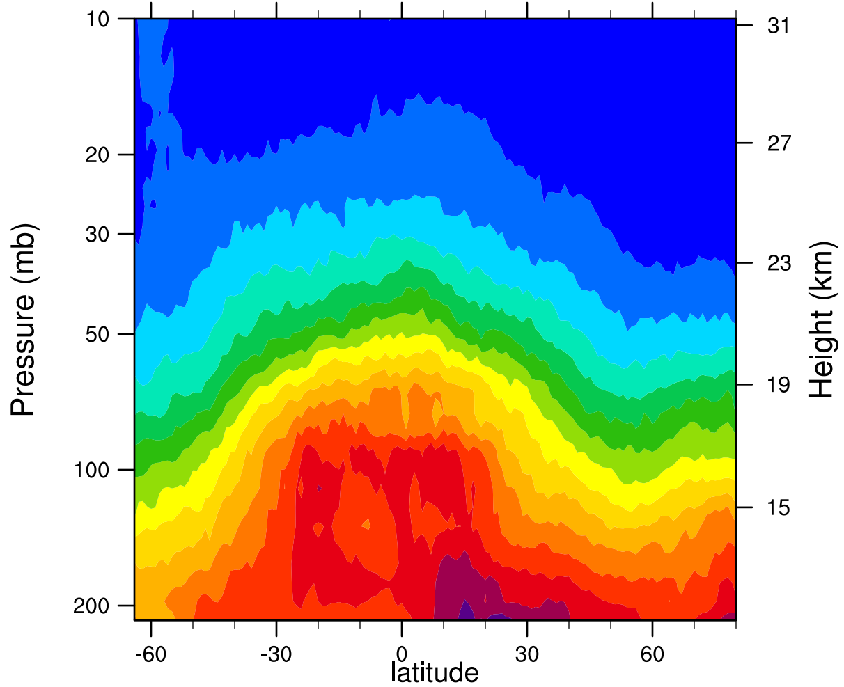
2007d066 12.1MicronExtinction_Combined (km -1 )
