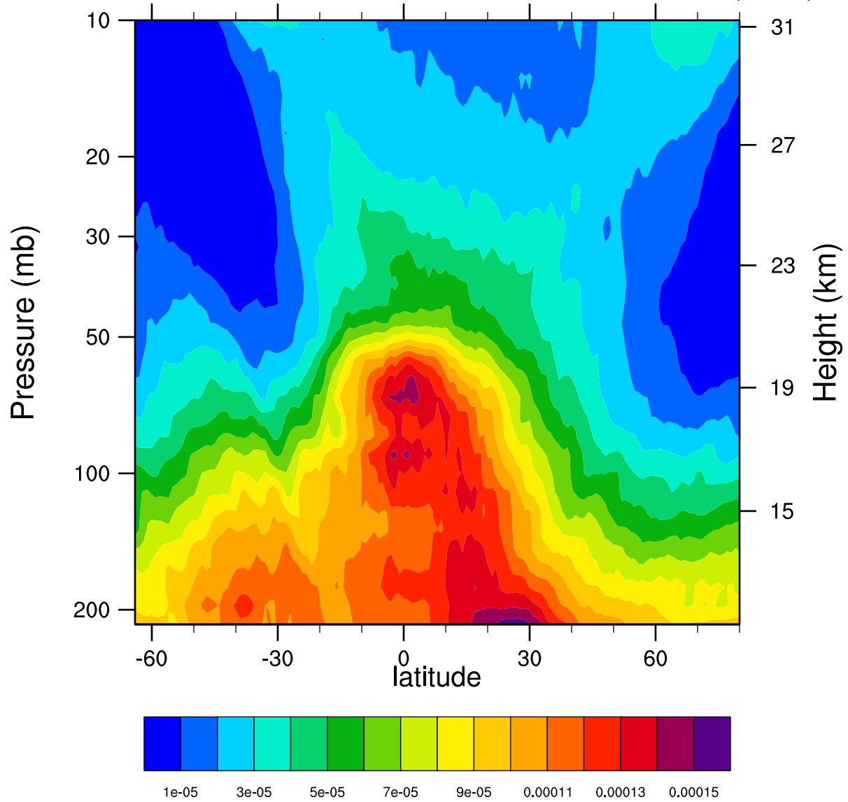
2005d090 12.1MicronExtinction_Combined (km -1 )
