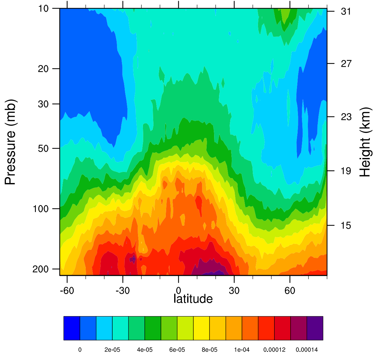
2005d029 12.1MicronExtinction_Combined (km -1 )
