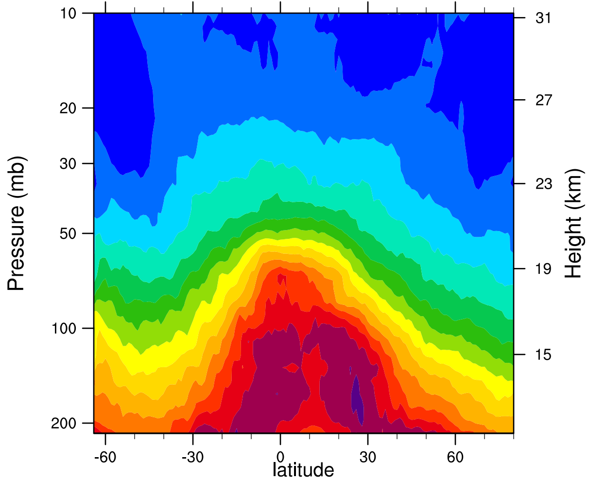
2006d256 12.1MicronExtinction_Combined (km -1 )
