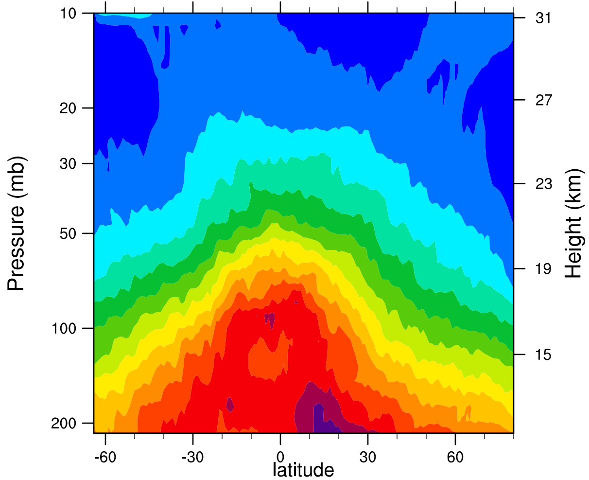
2006d043 12.1MicronExtinction_Combined (km -1 )
