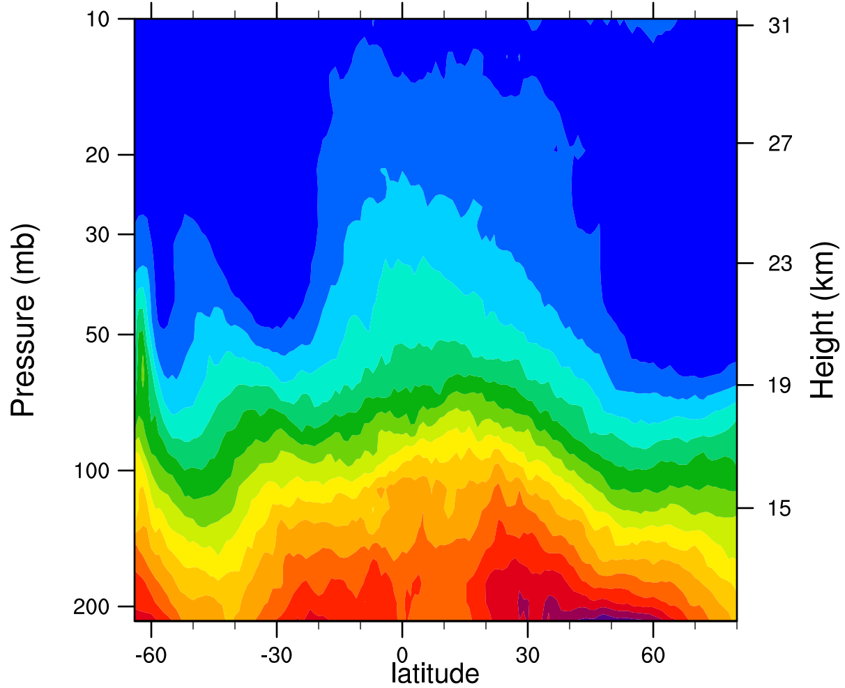
2007d236 12.1MicronExtinction_Combined (km -1 )
