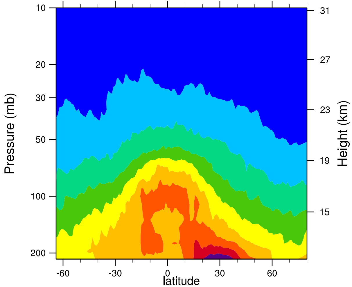
2006d111 12.1MicronExtinction_Combined (km -1 )
