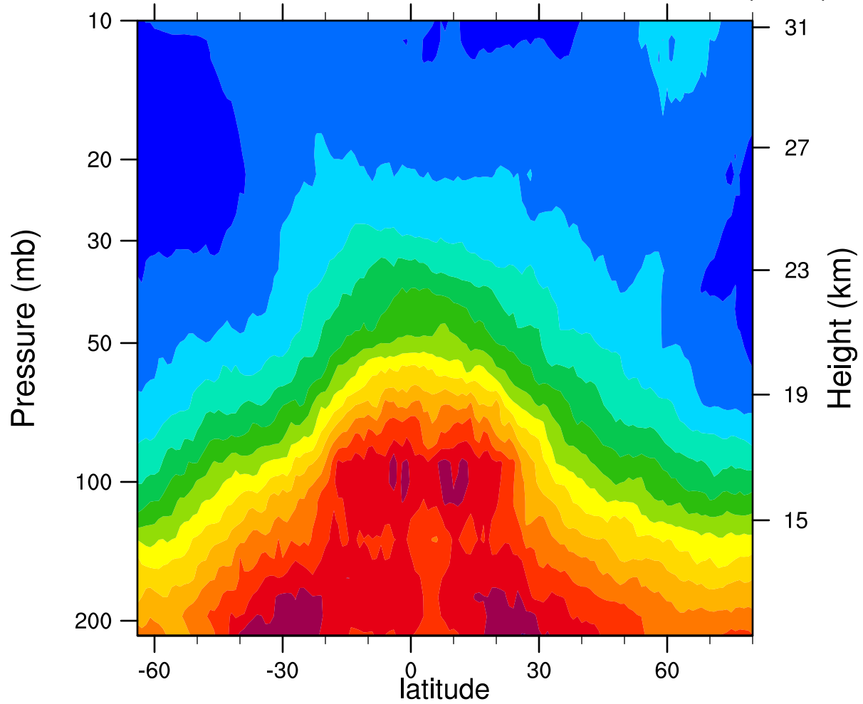
2005d324 12.1MicronExtinction_Combined (km -1 )
