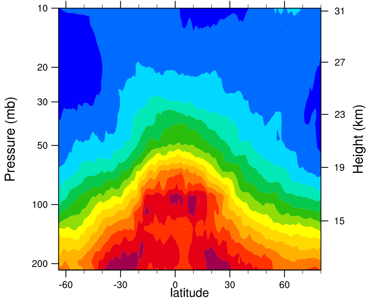
2005d330 12.1MicronExtinction_Combined ( \text{km}^{-1} )
