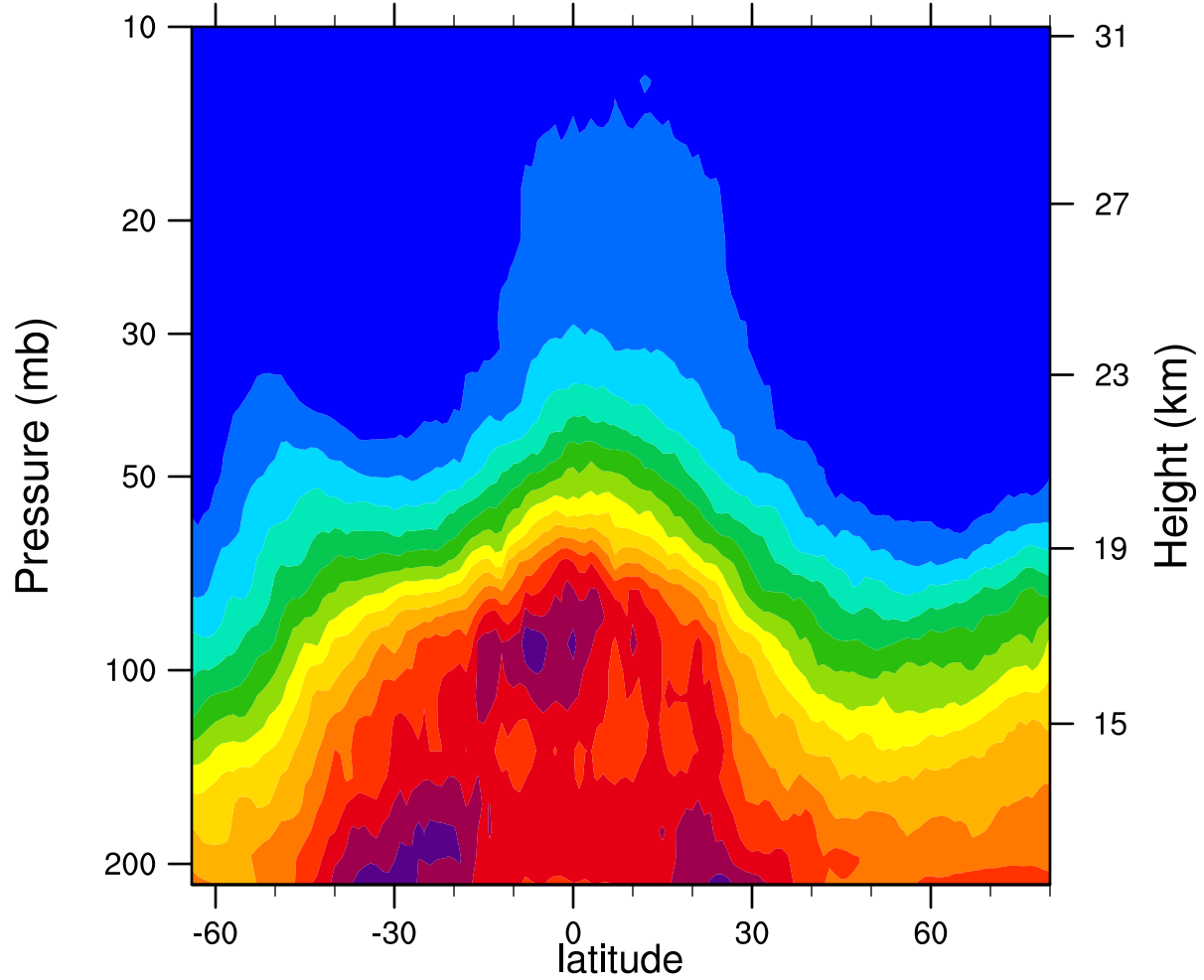
2006d341 12.1MicronExtinction_Combined (km -1 )
