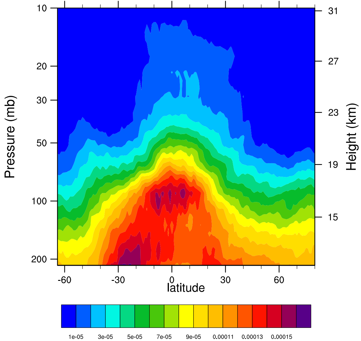
2006d320 12.1MicronExtinction_Combined (km -1 )
