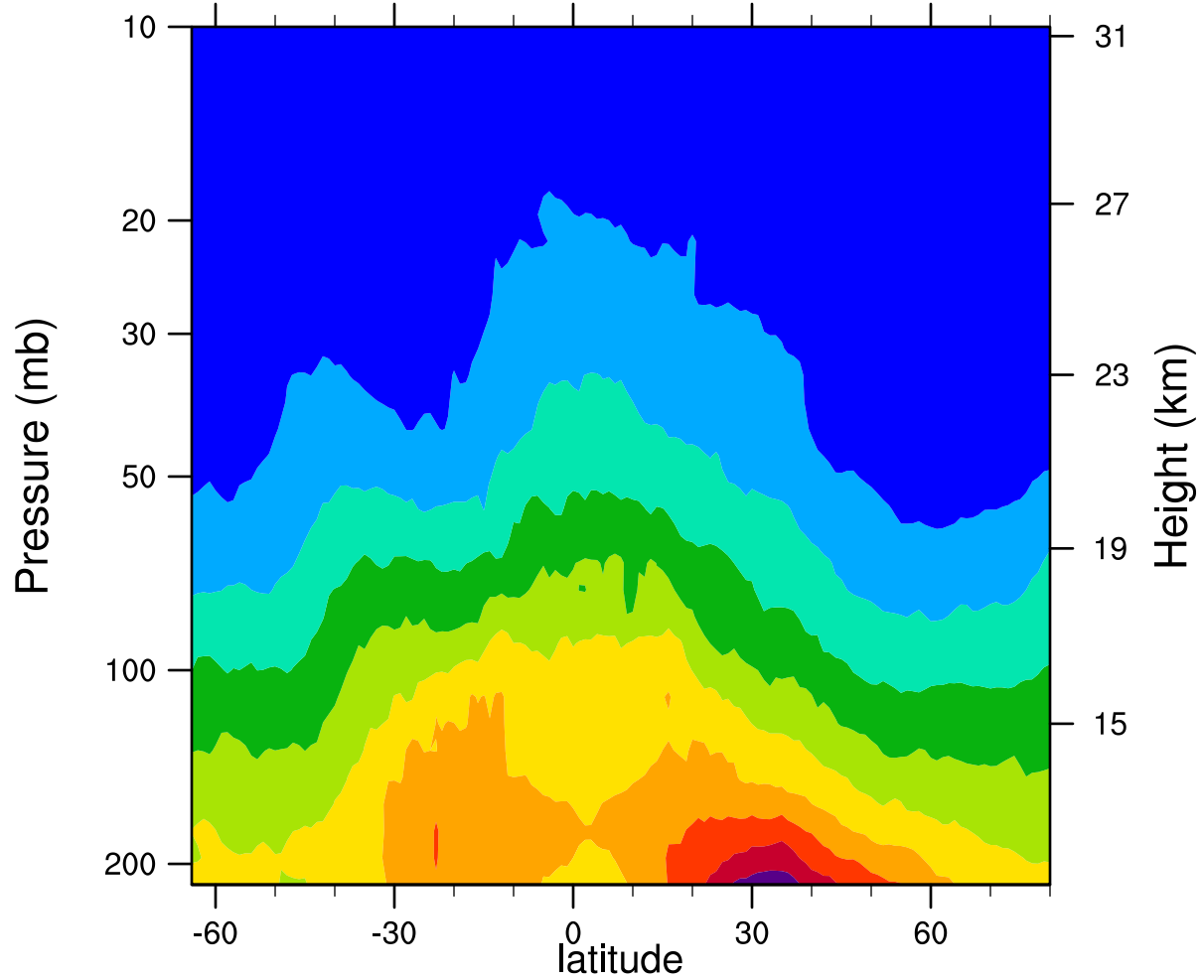
2007d129 12.1MicronExtinction_Combined (km -1 )
