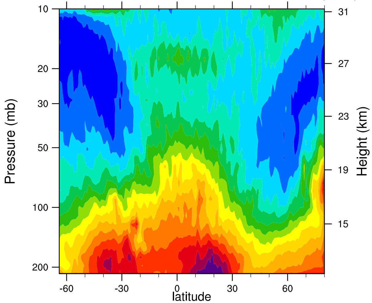
2005d026 12.1MicronExtinction_Combined (km -1 )
