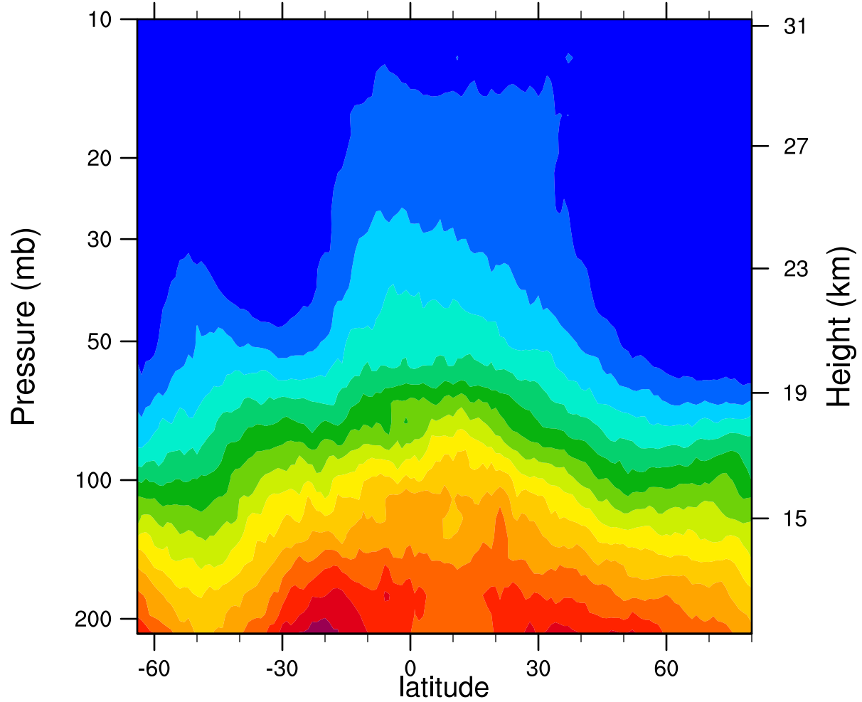
2007d270 12.1MicronExtinction_Combined (km -1 )
