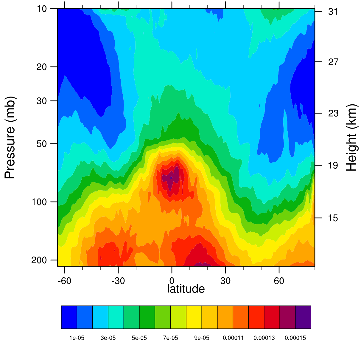
2005d047 12.1MicronExtinction_Combined (km -1 )
