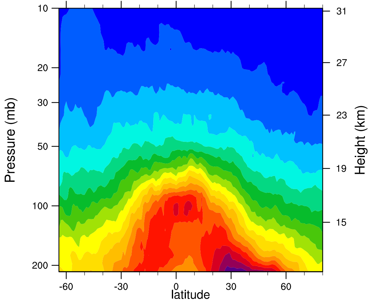
2006d155 12.1MicronExtinction_Combined ( \text{km}^{-1} )
