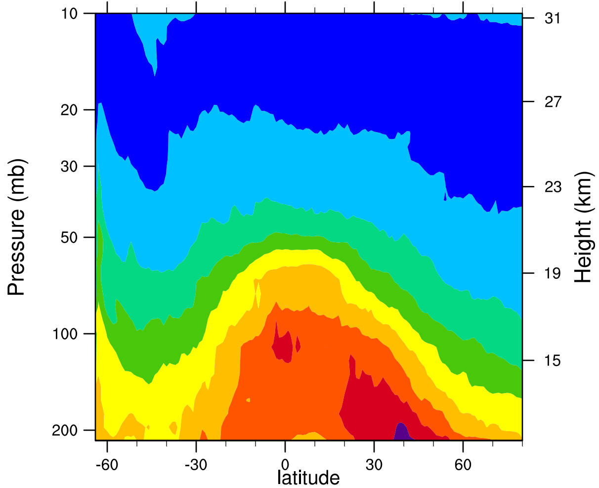
2006d220 12.1MicronExtinction_Combined (km -1 )
