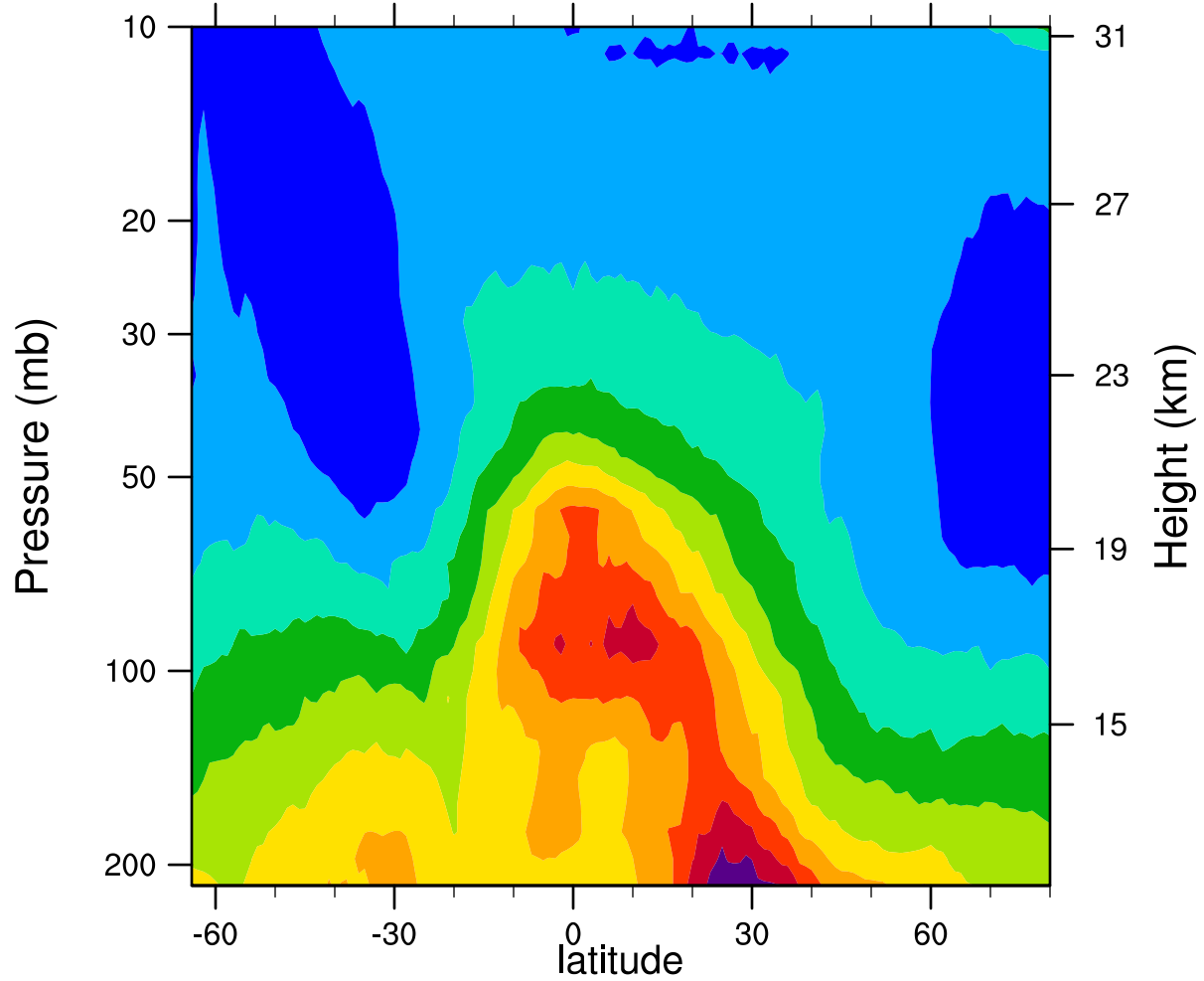
2005d130 12.1MicronExtinction_Combined (km -1 )
