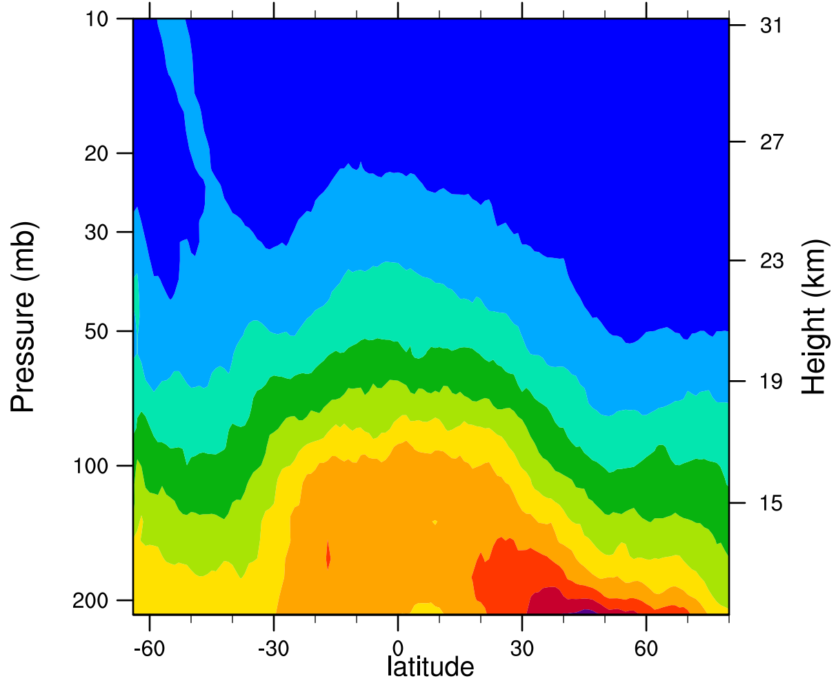
2007d175 12.1MicronExtinction_Combined ( \text{km}^{-1} )
