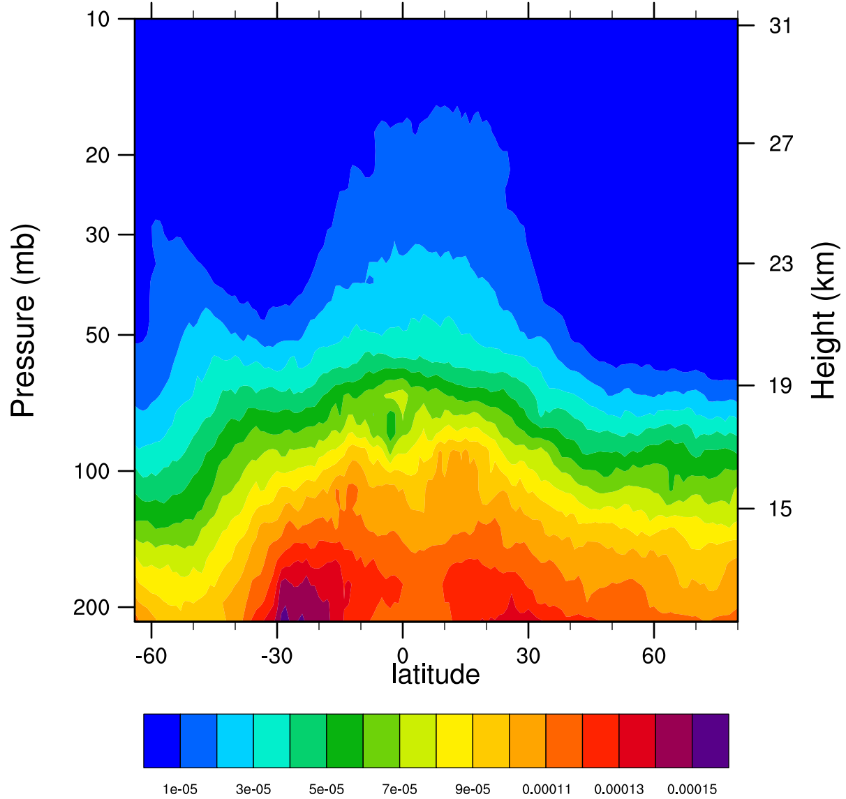
2007d315 12.1MicronExtinction_Combined (km -1 )
