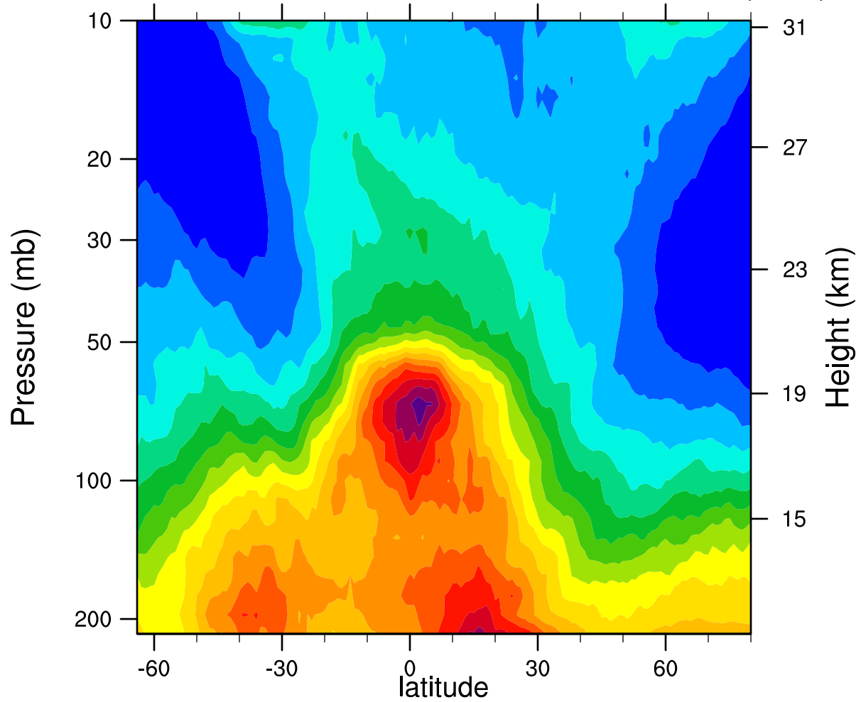
2005d061 12.1MicronExtinction_Combined (km -1 )
