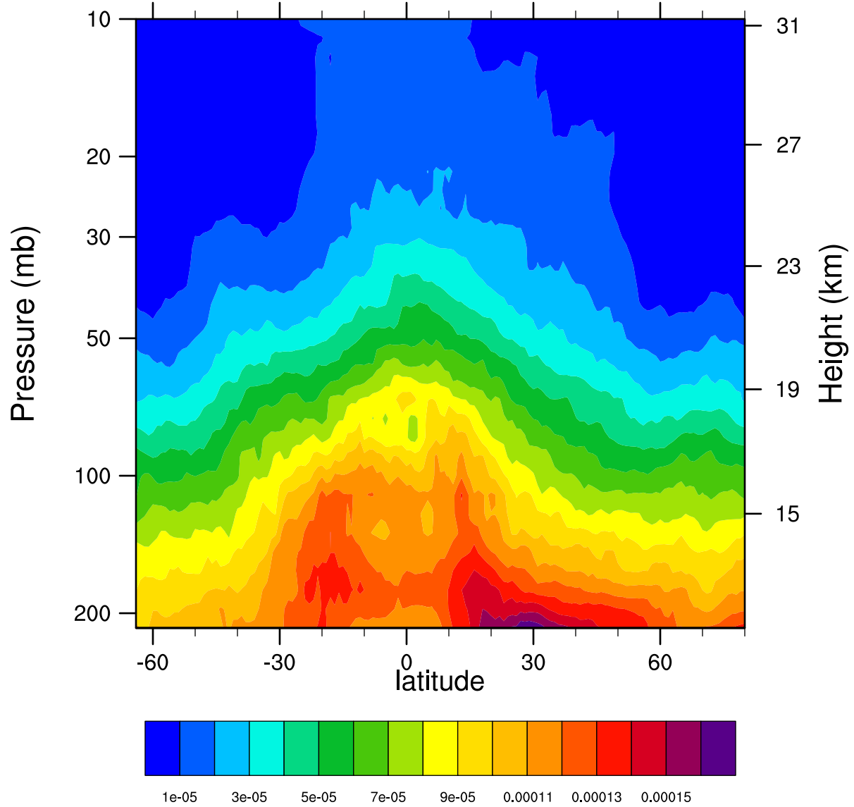
2007d106 12.1MicronExtinction_Combined ( \text{km}^{-1} )
