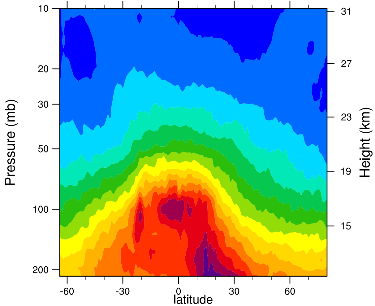
2006d076 12.1MicronExtinction_Combined (km -1 )
