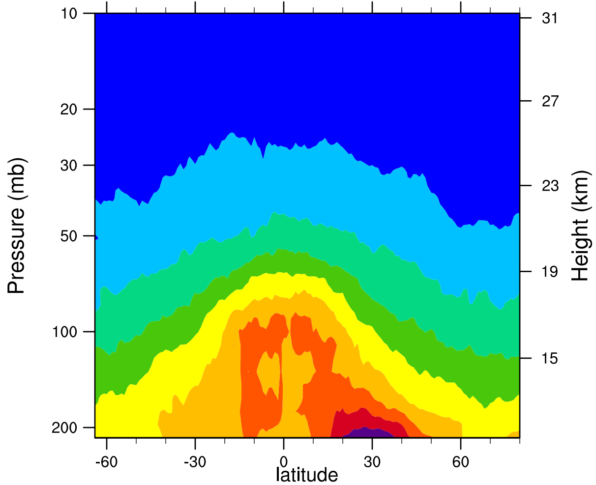
2006d116 12.1MicronExtinction_Combined (km -1 )
