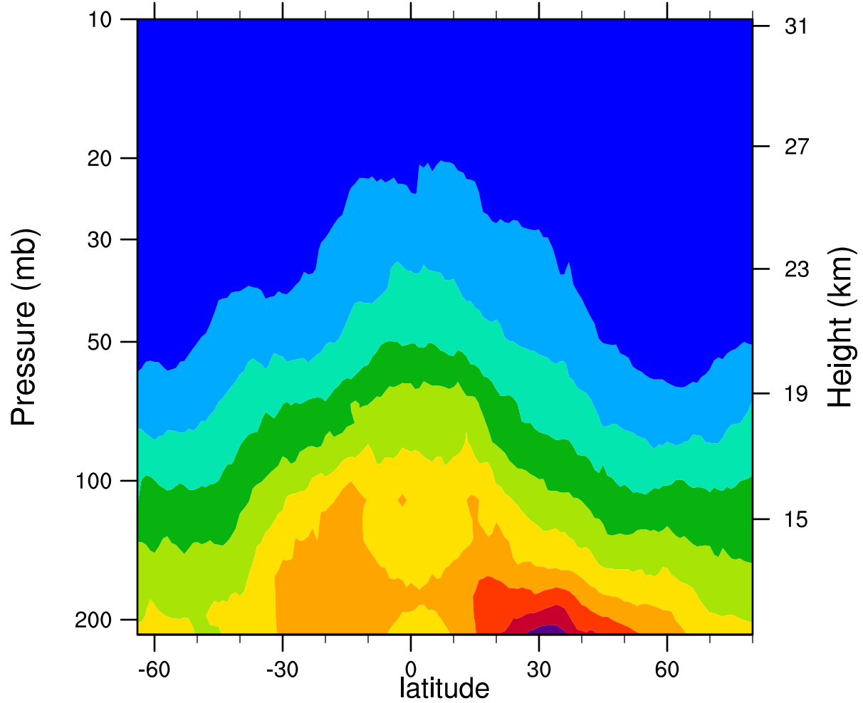
2007d122 12.1MicronExtinction_Combined (km -1 )
