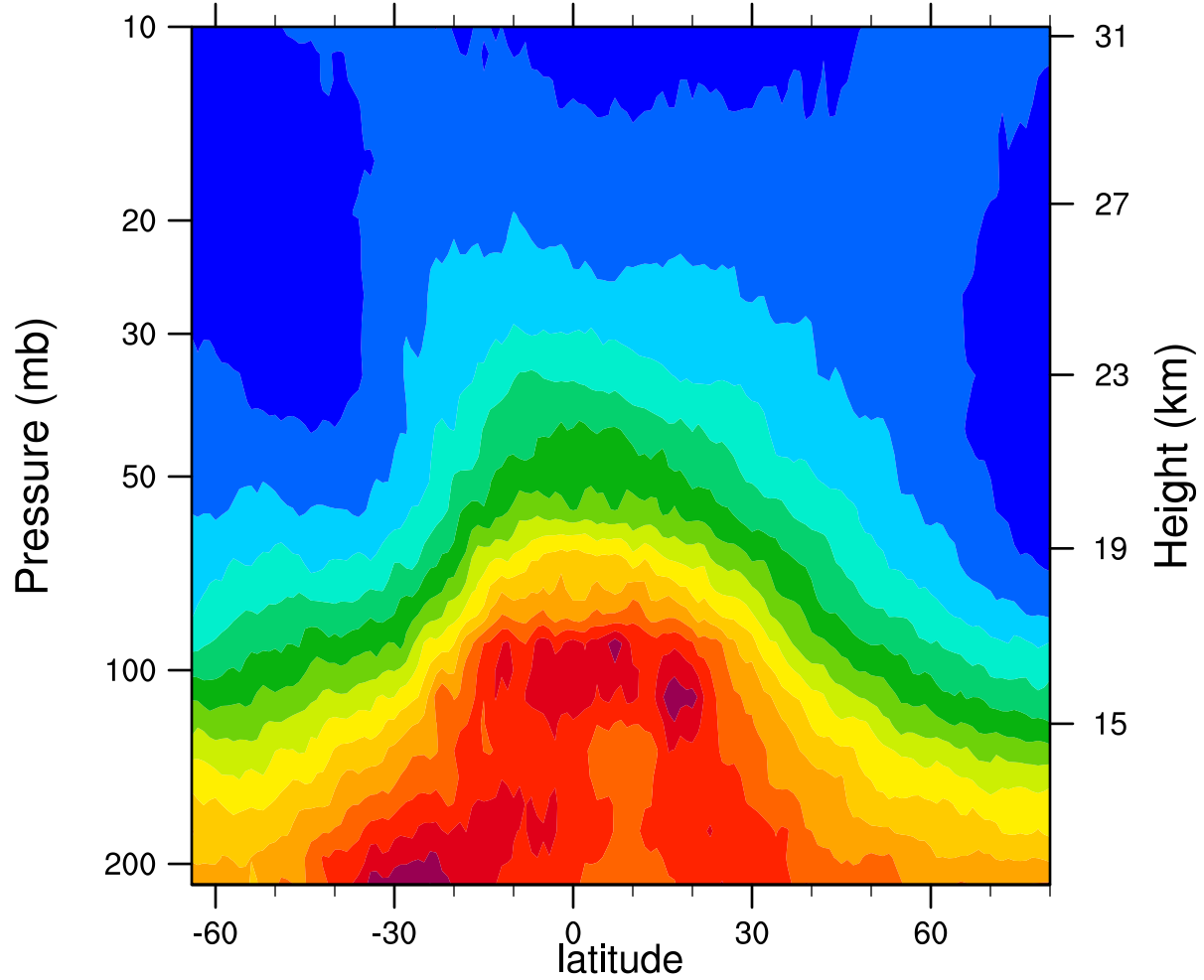
2005d299 12.1MicronExtinction_Combined (km -1 )
