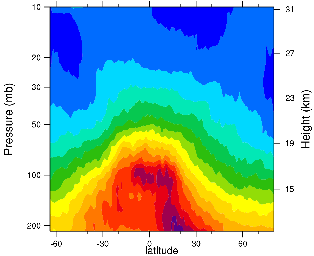
2006d068 12.1MicronExtinction_Combined (km -1 )
