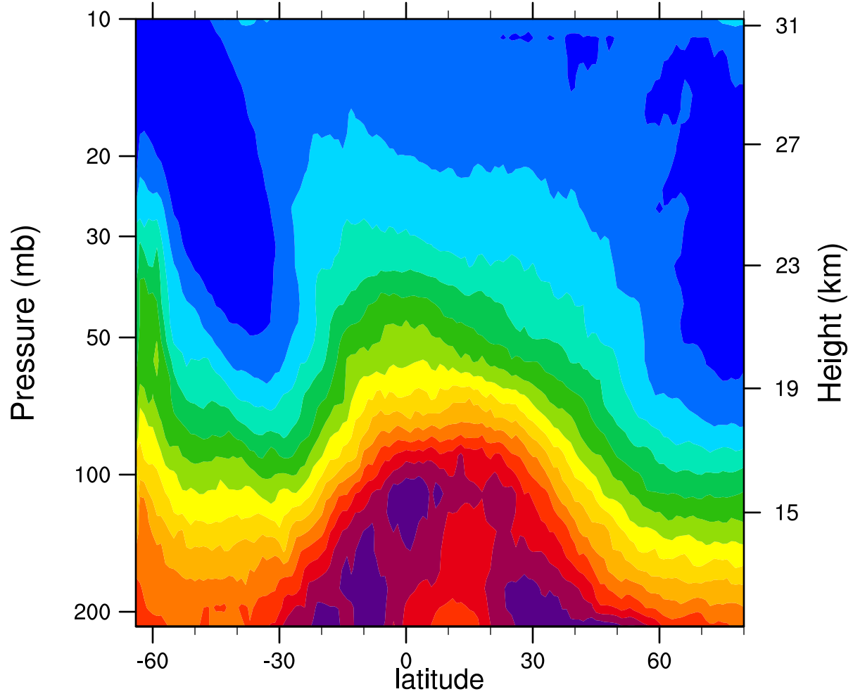
2005d235 12.1MicronExtinction_Combined (km -1 )
