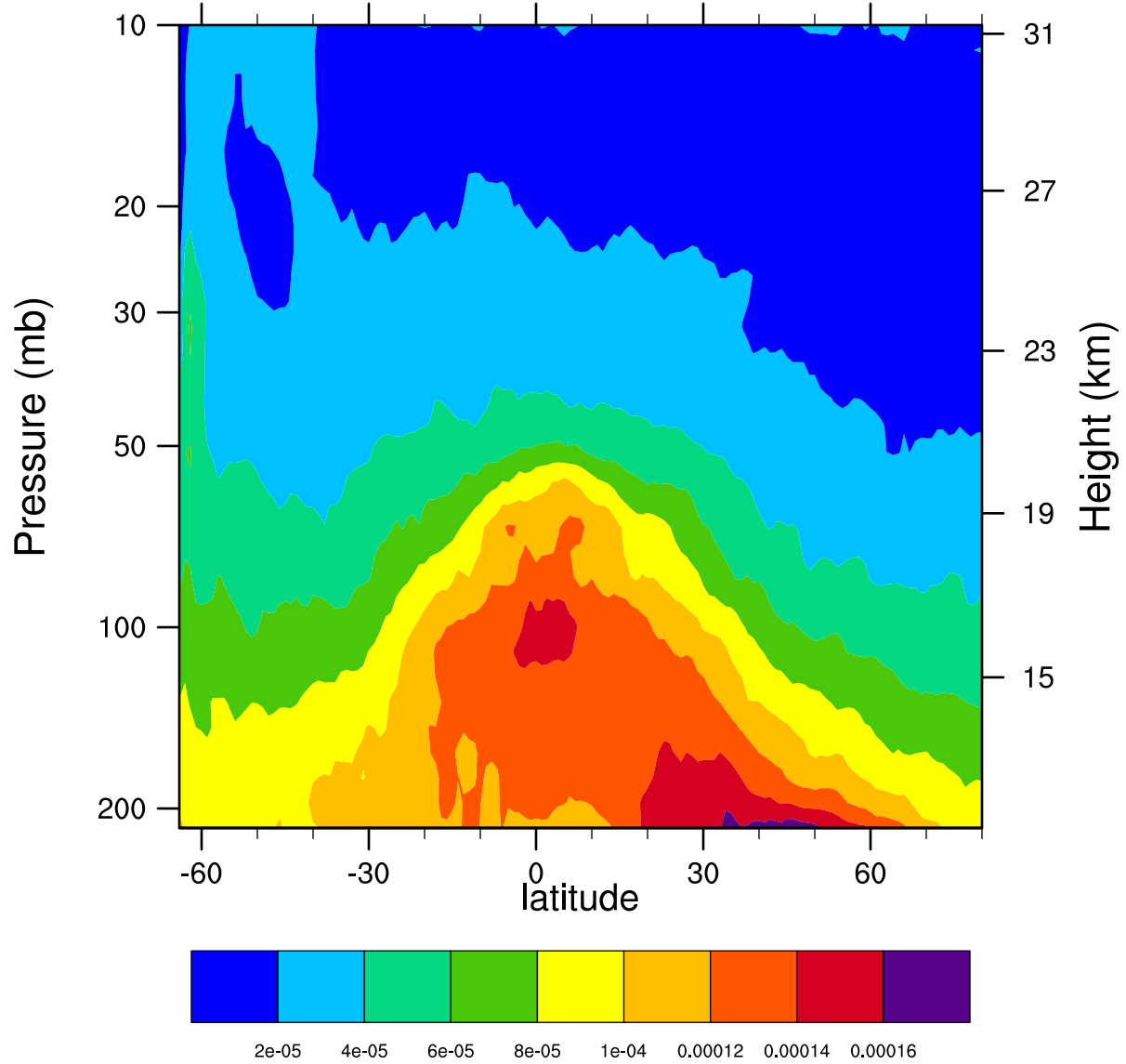
2006d178 12.1MicronExtinction_Combined (km -1 )
