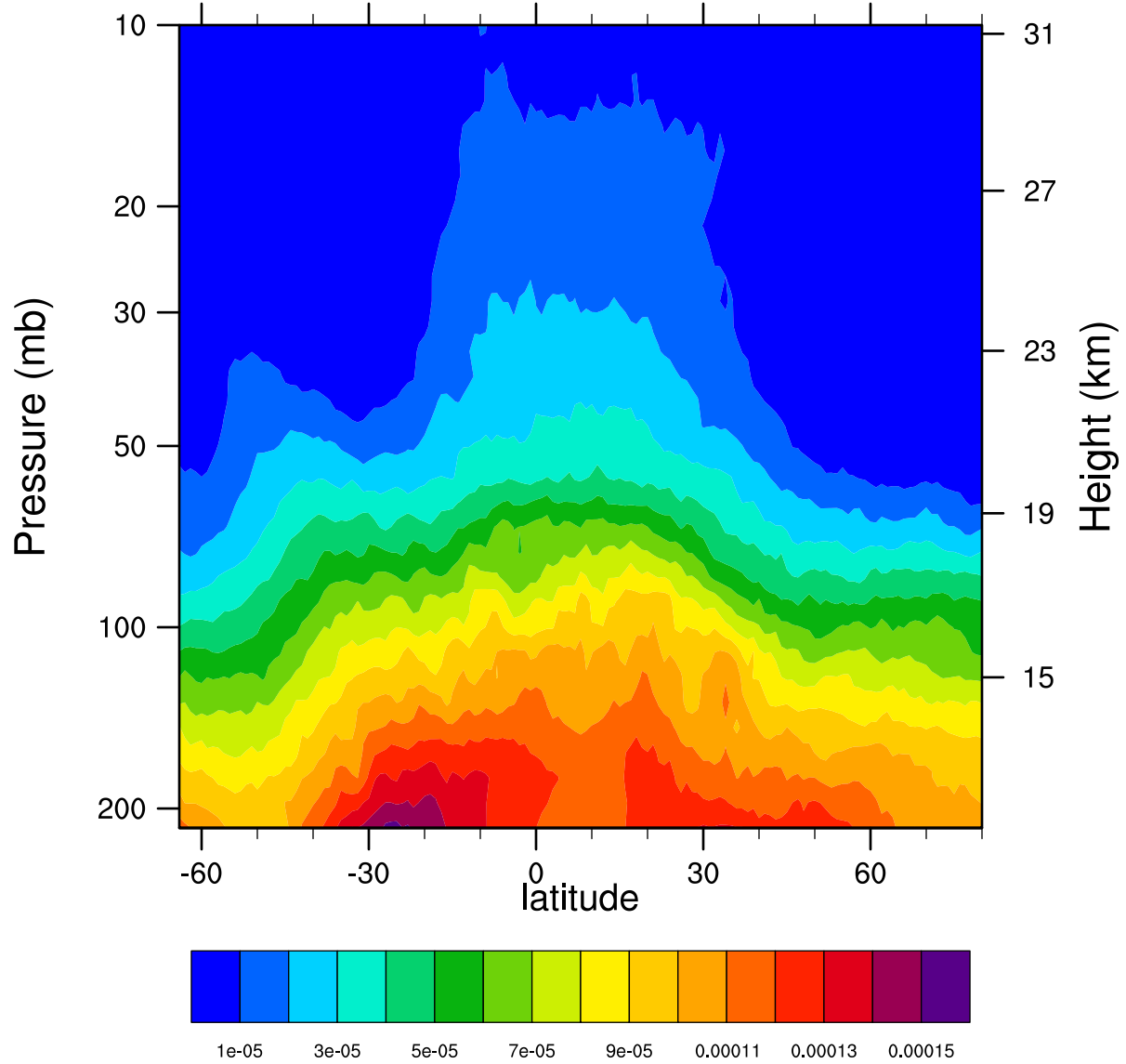
2007d291 12.1MicronExtinction_Combined (km -1 )
