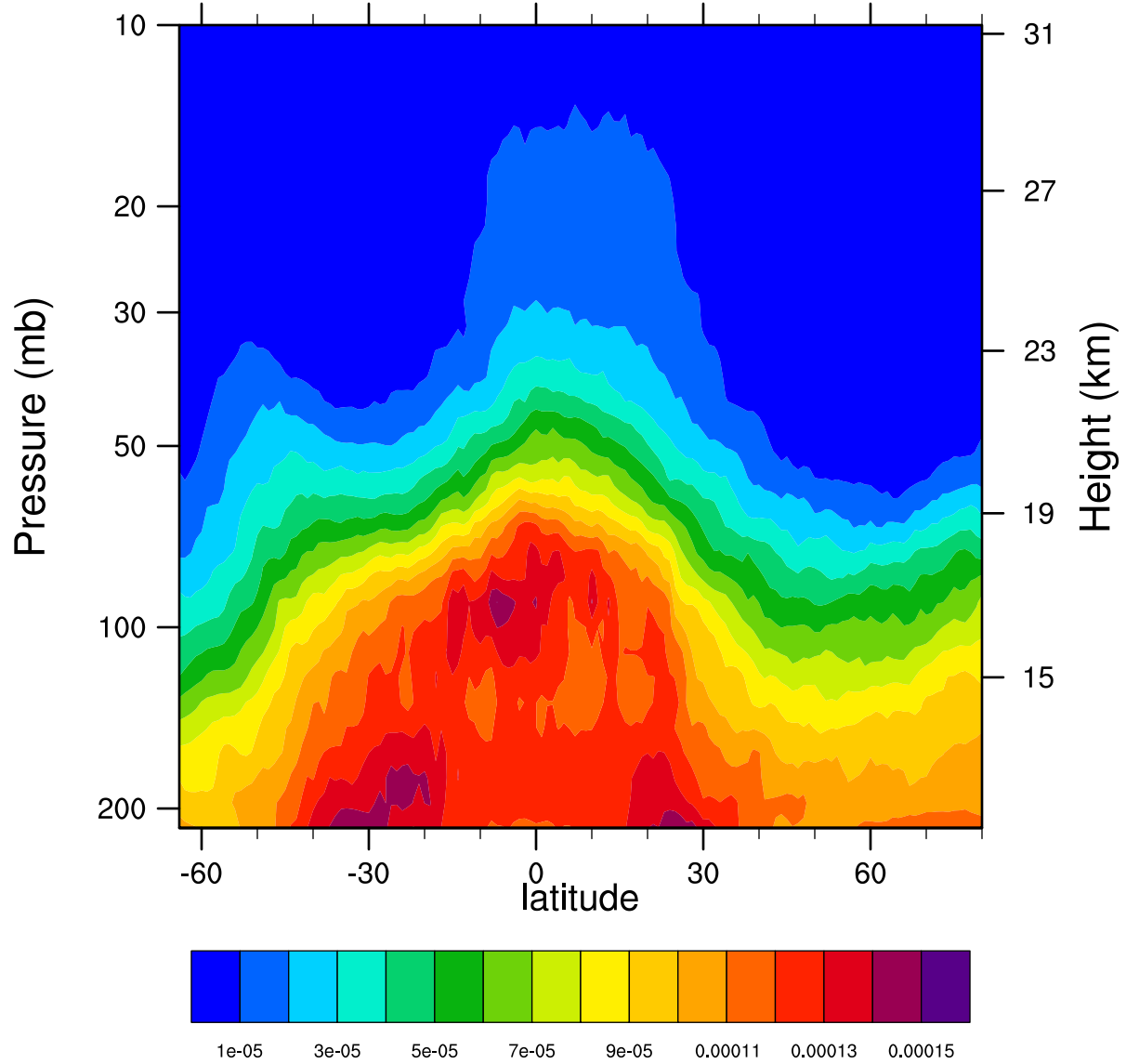
2006d342 12.1MicronExtinction_Combined (km -1 )
