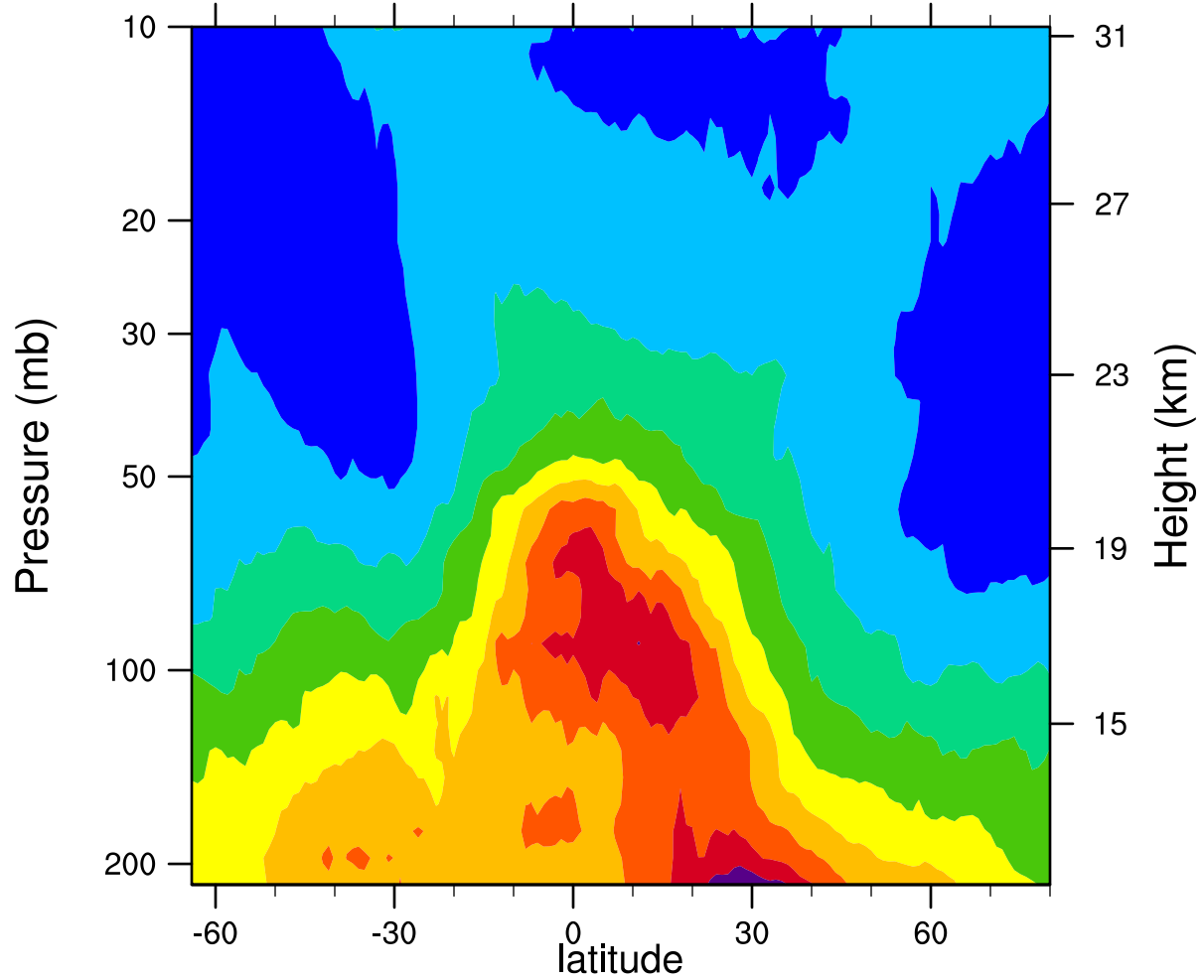
2005d113 12.1MicronExtinction_Combined (km -1 )
