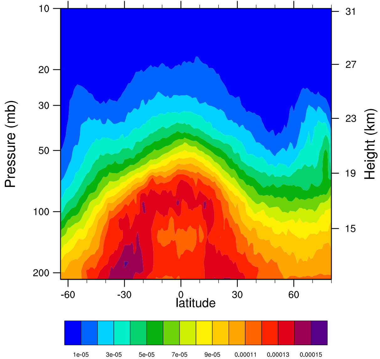
2006d358 12.1MicronExtinction_Combined (km -1 )
