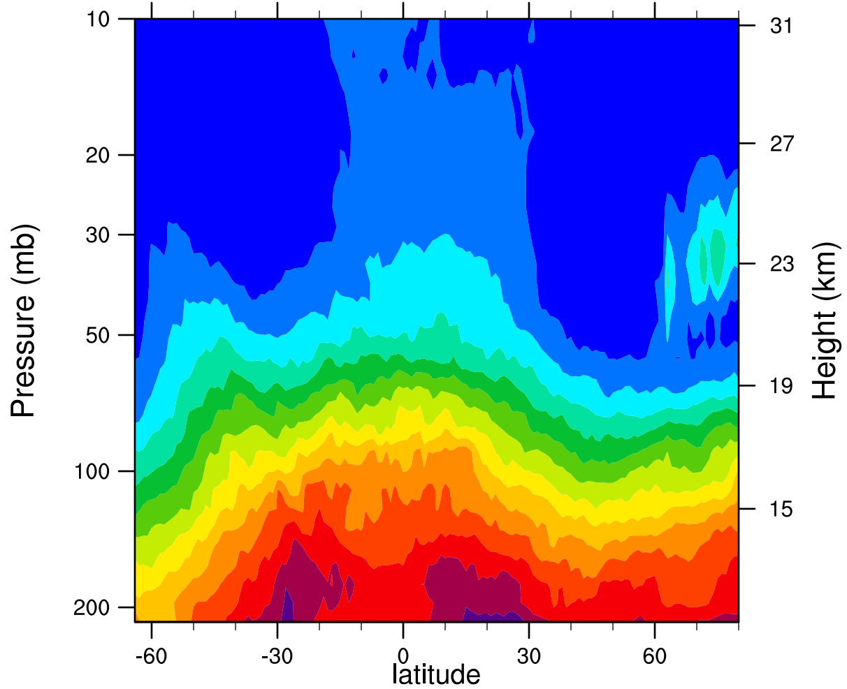
2007d351 12.1MicronExtinction_Combined ( \text{km}^{-1} )
