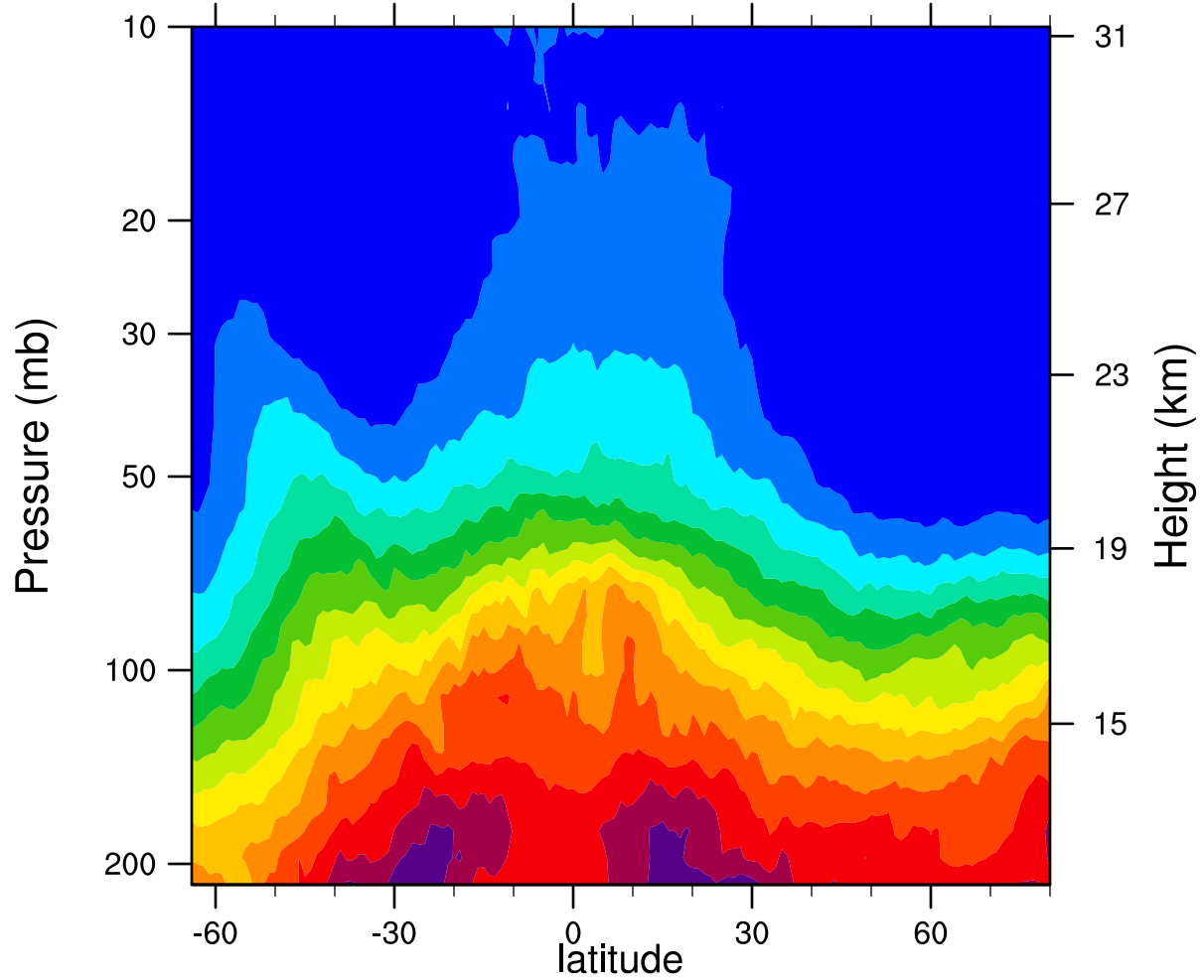
2007d335 12.1MicronExtinction_Combined (km -1 )
