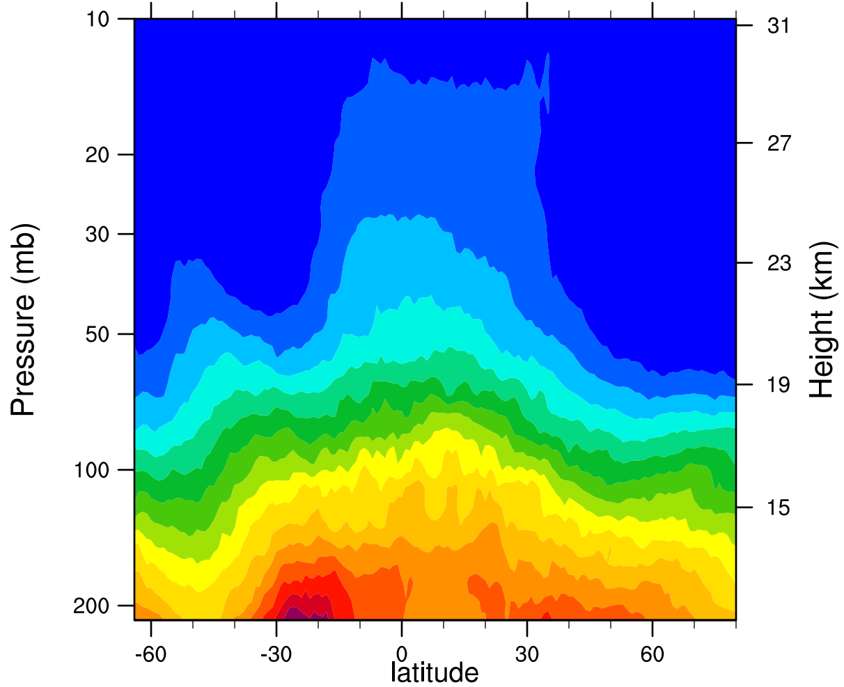
2007d278 12.1MicronExtinction_Combined (km -1 )
