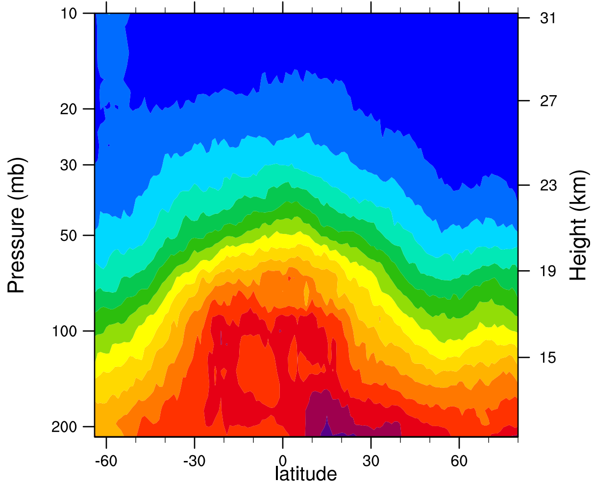
2007d065 12.1MicronExtinction_Combined (km -1 )
