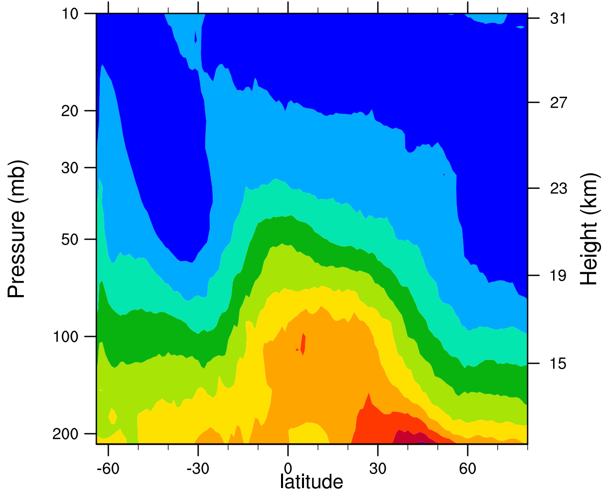
2005d185 12.1MicronExtinction_Combined (km -1 )
