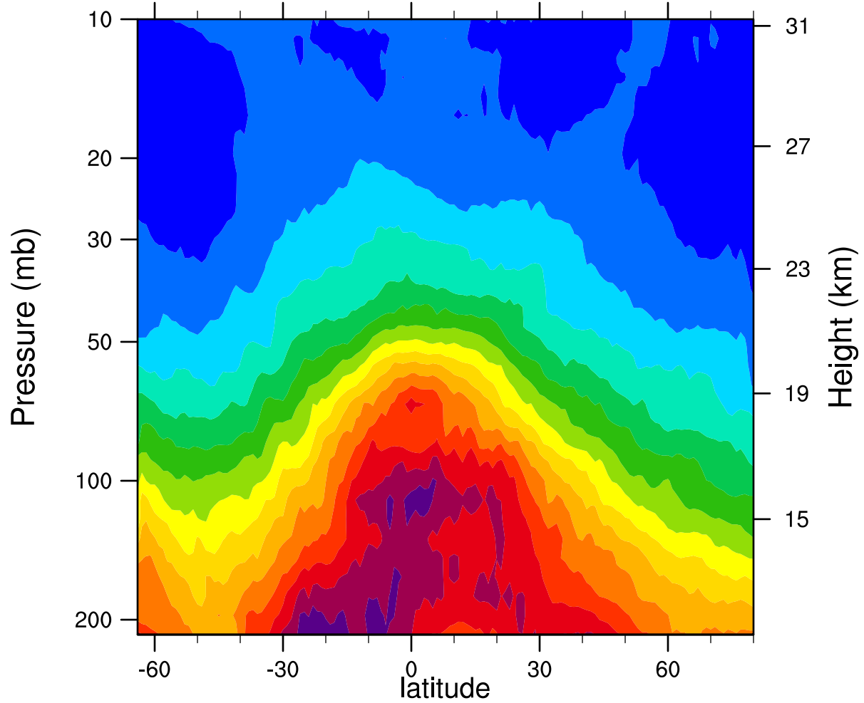
2006d281 12.1MicronExtinction_Combined (km -1 )
