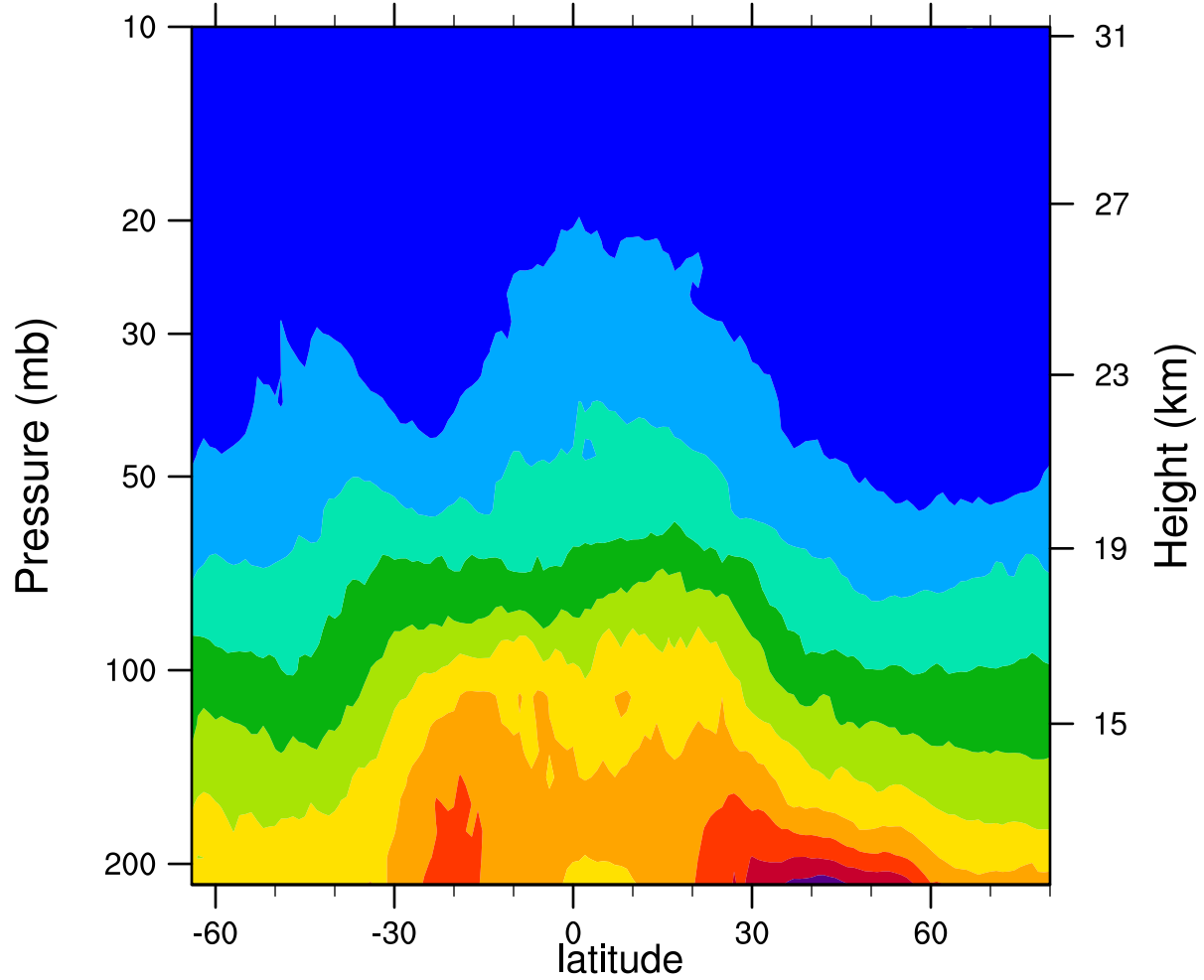
2007d159 12.1MicronExtinction_Combined (km -1 )
