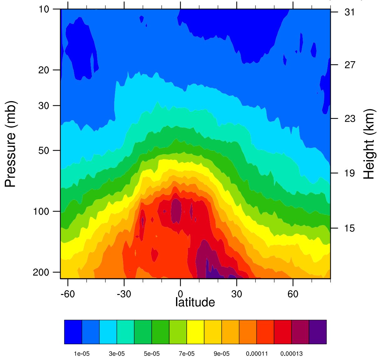
2006d079 12.1MicronExtinction_Combined ( \text{km}^{-1} )
