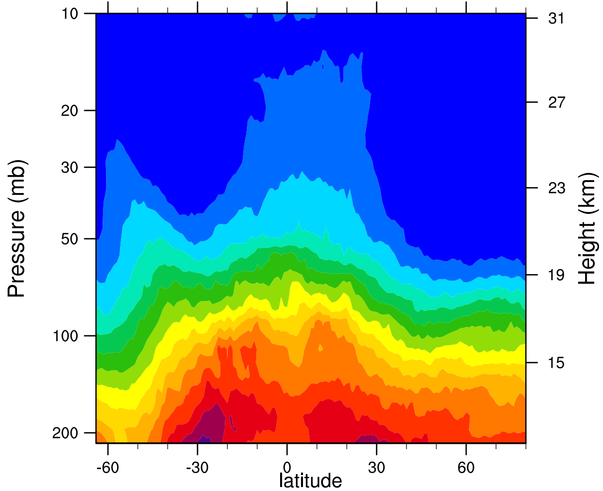
2007d323 12.1MicronExtinction_Combined (km -1 )
