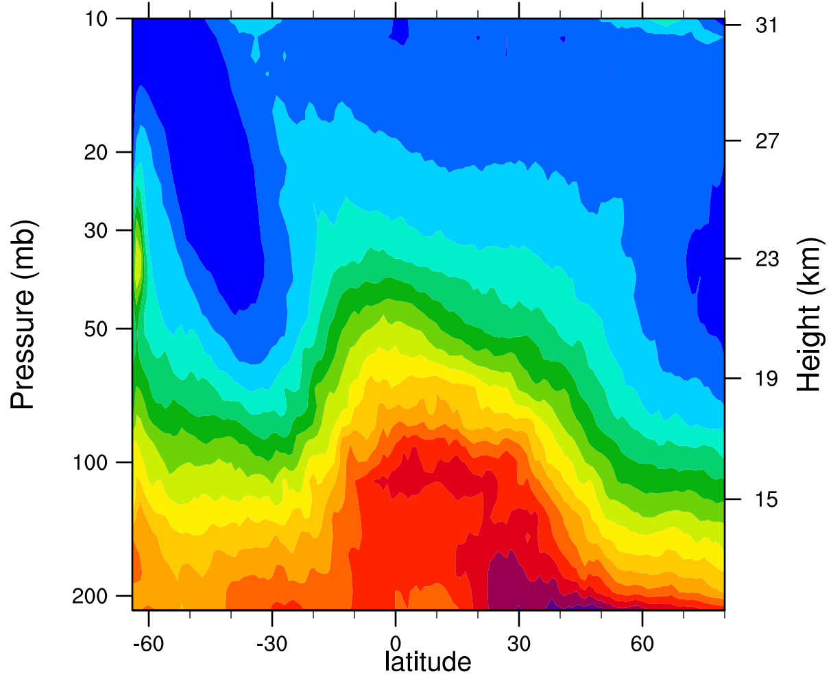
2005d202 12.1MicronExtinction_Combined (km -1 )
