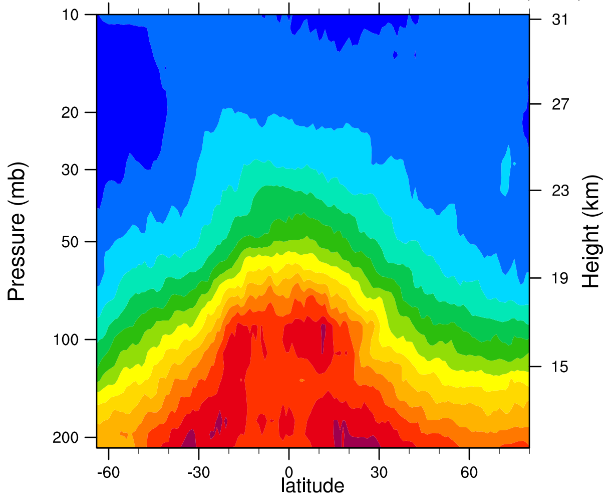
2005d342 12.1MicronExtinction_Combined (km -1 )
