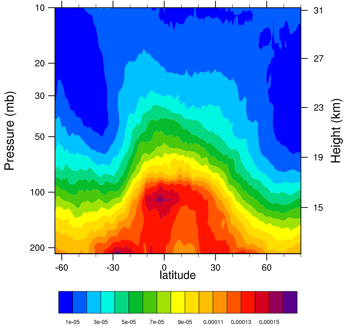
2005d257 12.1MicronExtinction_Combined (km -1 )
