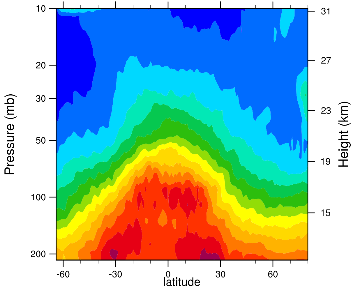
2005d358 12.1MicronExtinction_Combined (km -1 )
