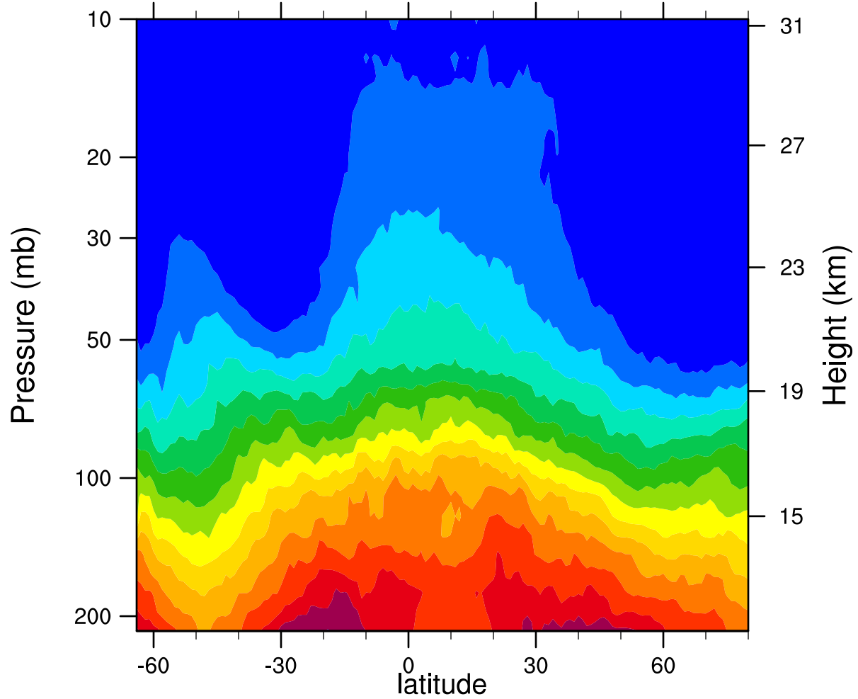
2007d264 12.1MicronExtinction_Combined (km -1 )
