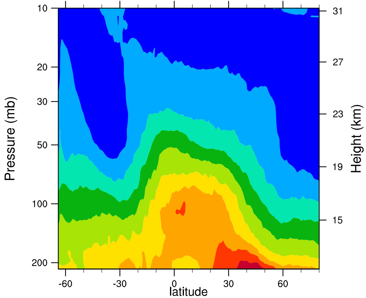
2005d184 12.1MicronExtinction_Combined ( \text{km}^{-1} )
