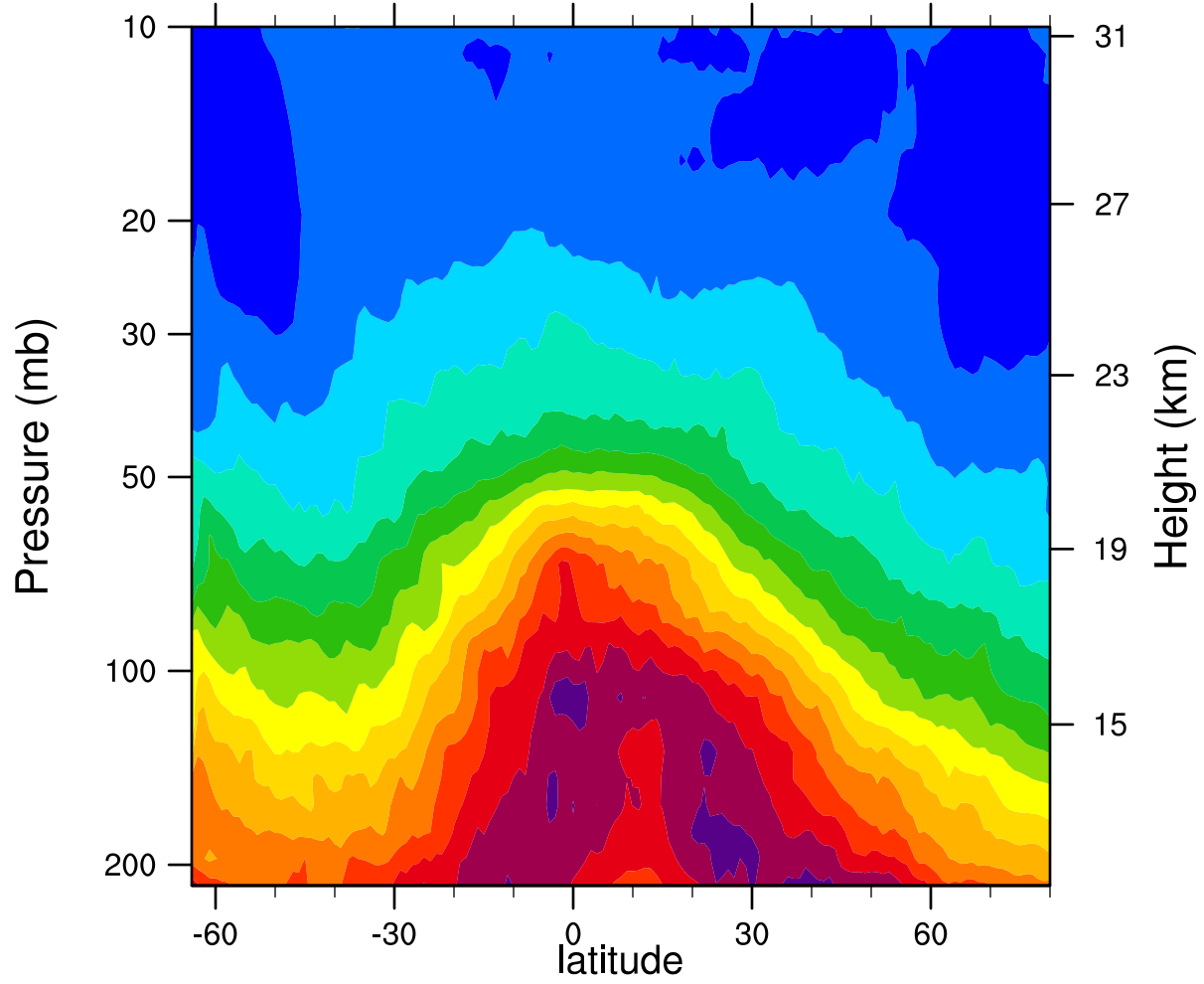
2006d246 12.1MicronExtinction_Combined (km -1 )
