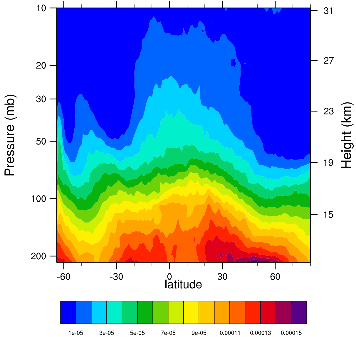
2007d237 12.1MicronExtinction_Combined (km -1 )
