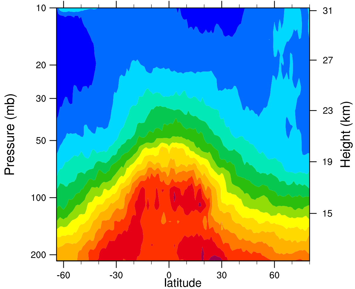
2005d352 12.1MicronExtinction_Combined ( \text{km}^{-1} )
