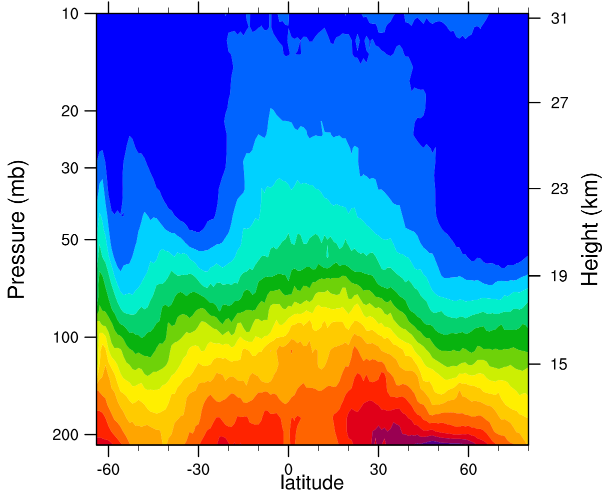
2007d234 12.1MicronExtinction_Combined (km -1 )
