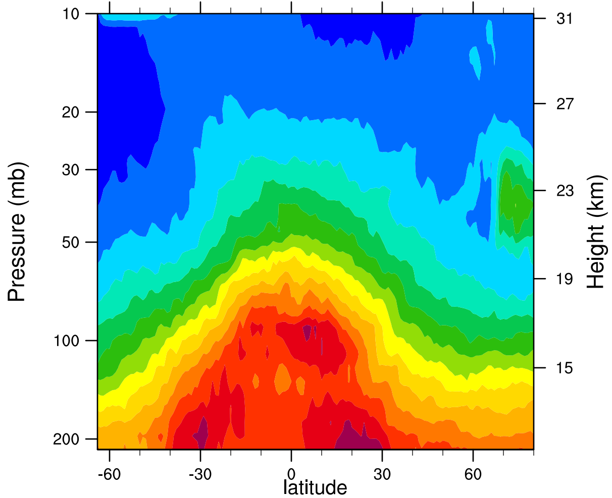
2005d362 12.1MicronExtinction_Combined (km -1 )
