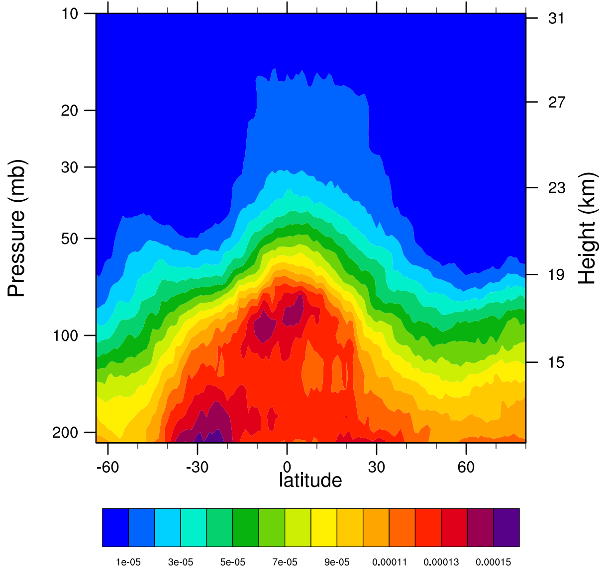
2006d330 12.1MicronExtinction_Combined (km -1 )
