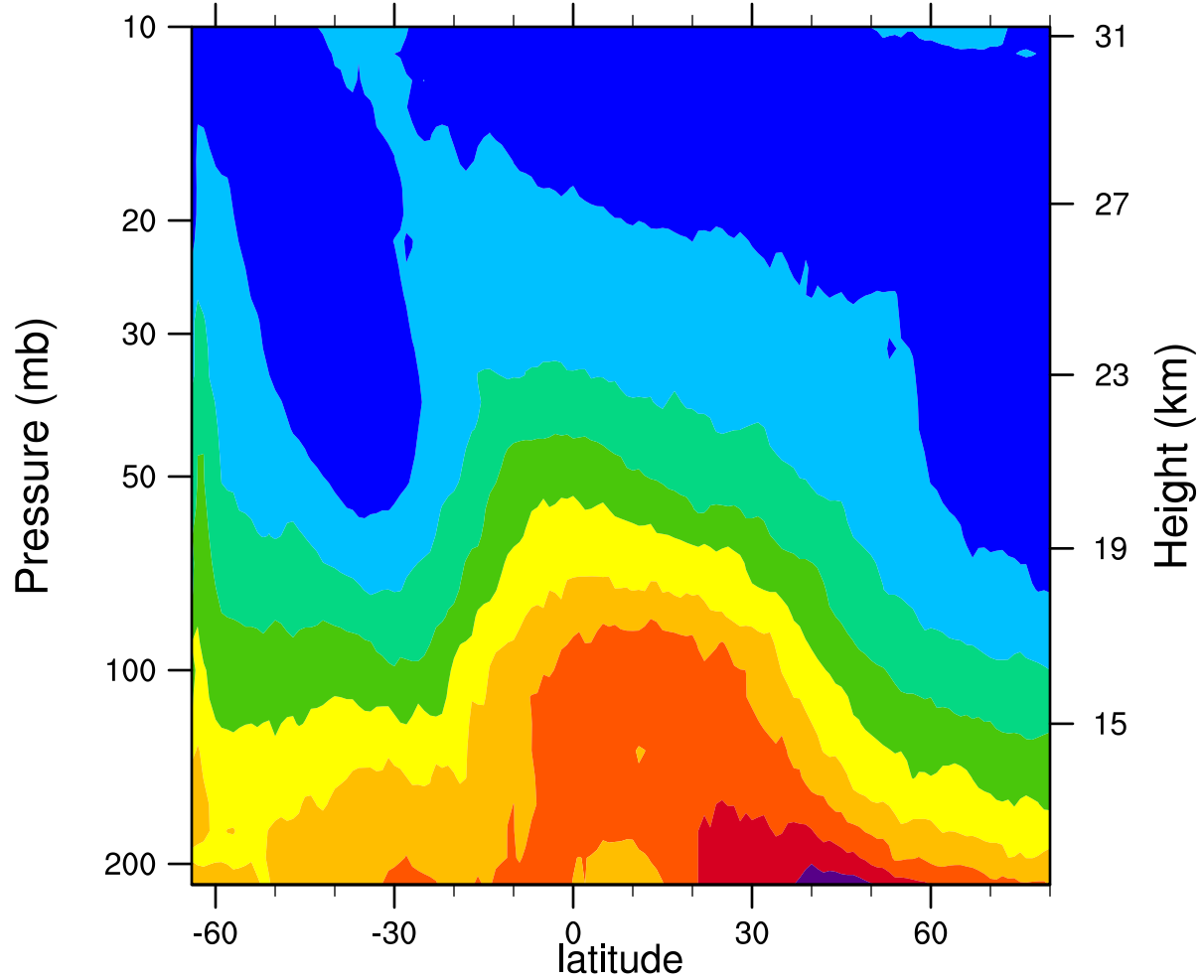
2005d192 12.1MicronExtinction_Combined (km -1 )
