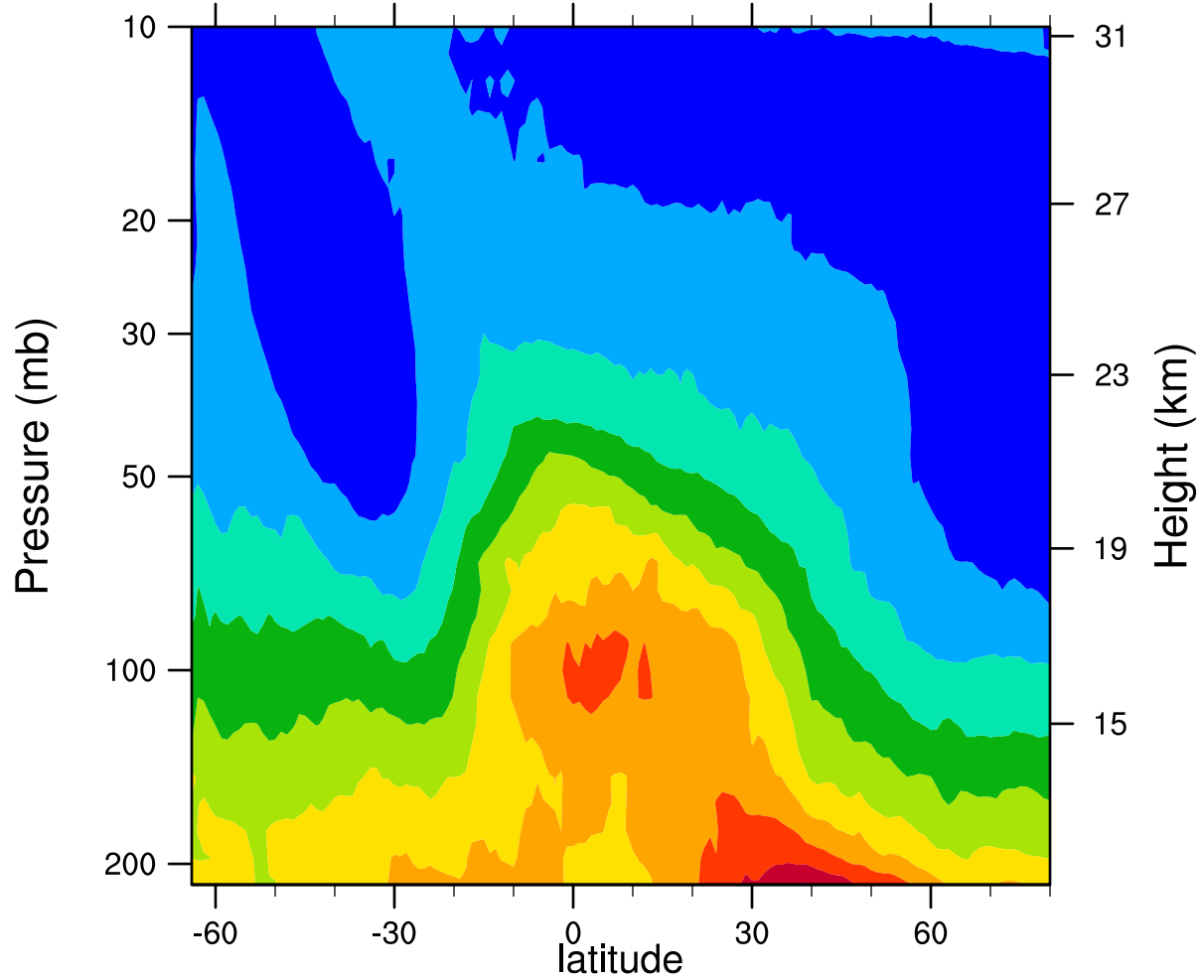
2005d168 12.1MicronExtinction_Combined (km -1 )
