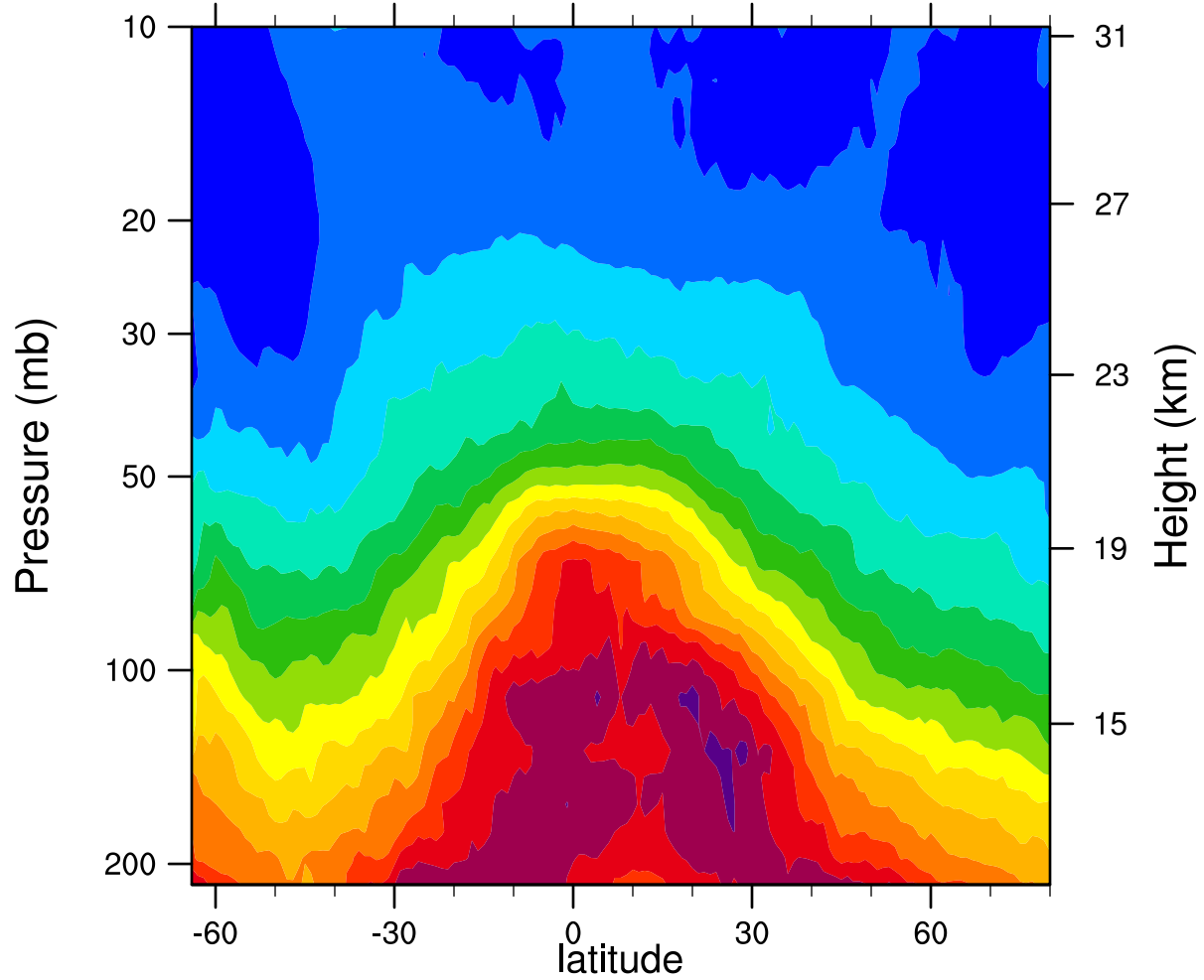
2006d259 12.1MicronExtinction_Combined (km -1 )
