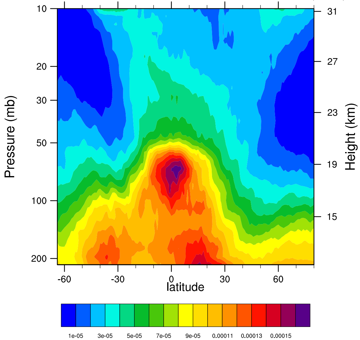
2005d060 12.1MicronExtinction_Combined ( \text{km}^{-1} )
