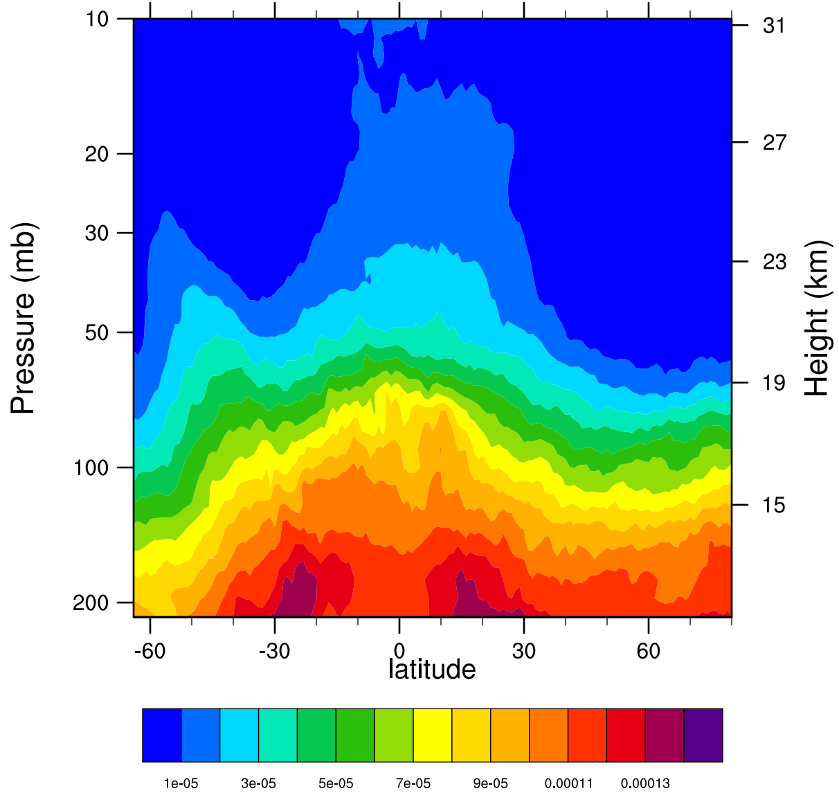
2007d338 12.1MicronExtinction_Combined ( \text{km}^{-1} )
