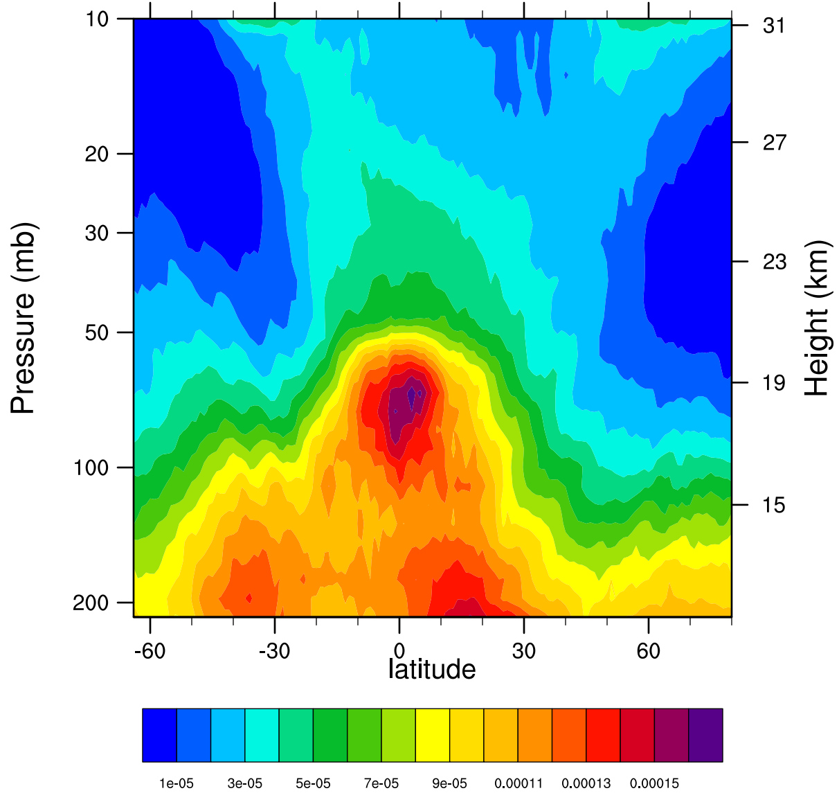
2005d057 12.1MicronExtinction_Combined ( \text{km}^{-1} )
