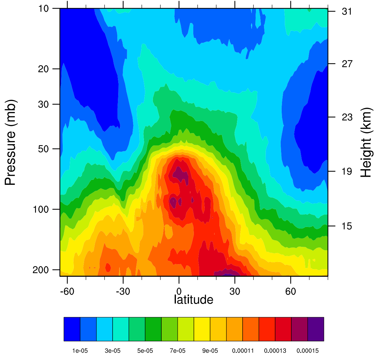
2005d096 12.1MicronExtinction_Combined (km -1 )
