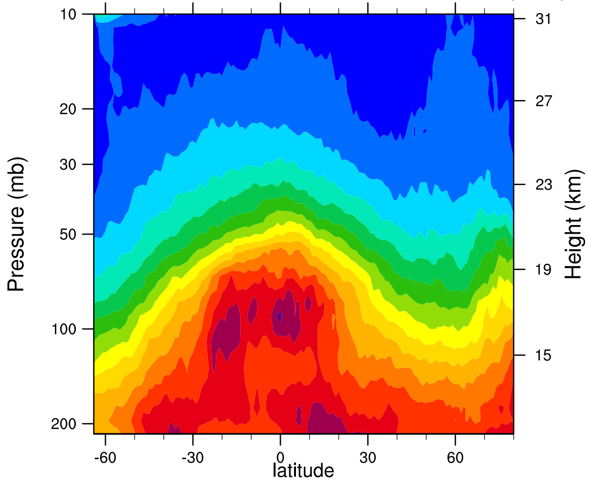
2007d033 12.1MicronExtinction_Combined ( \text{km}^{-1} )
