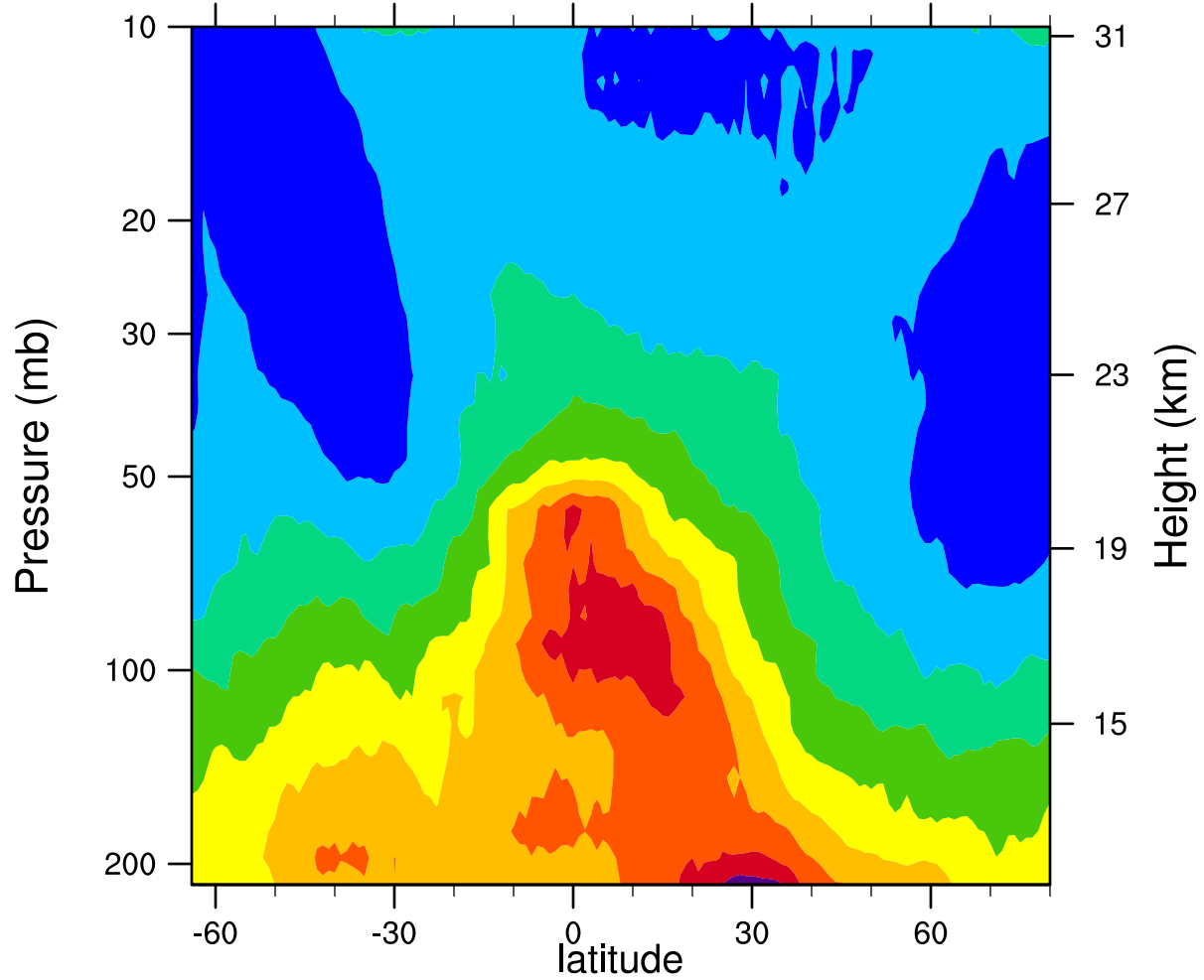
2005d108 12.1MicronExtinction_Combined (km -1 )
