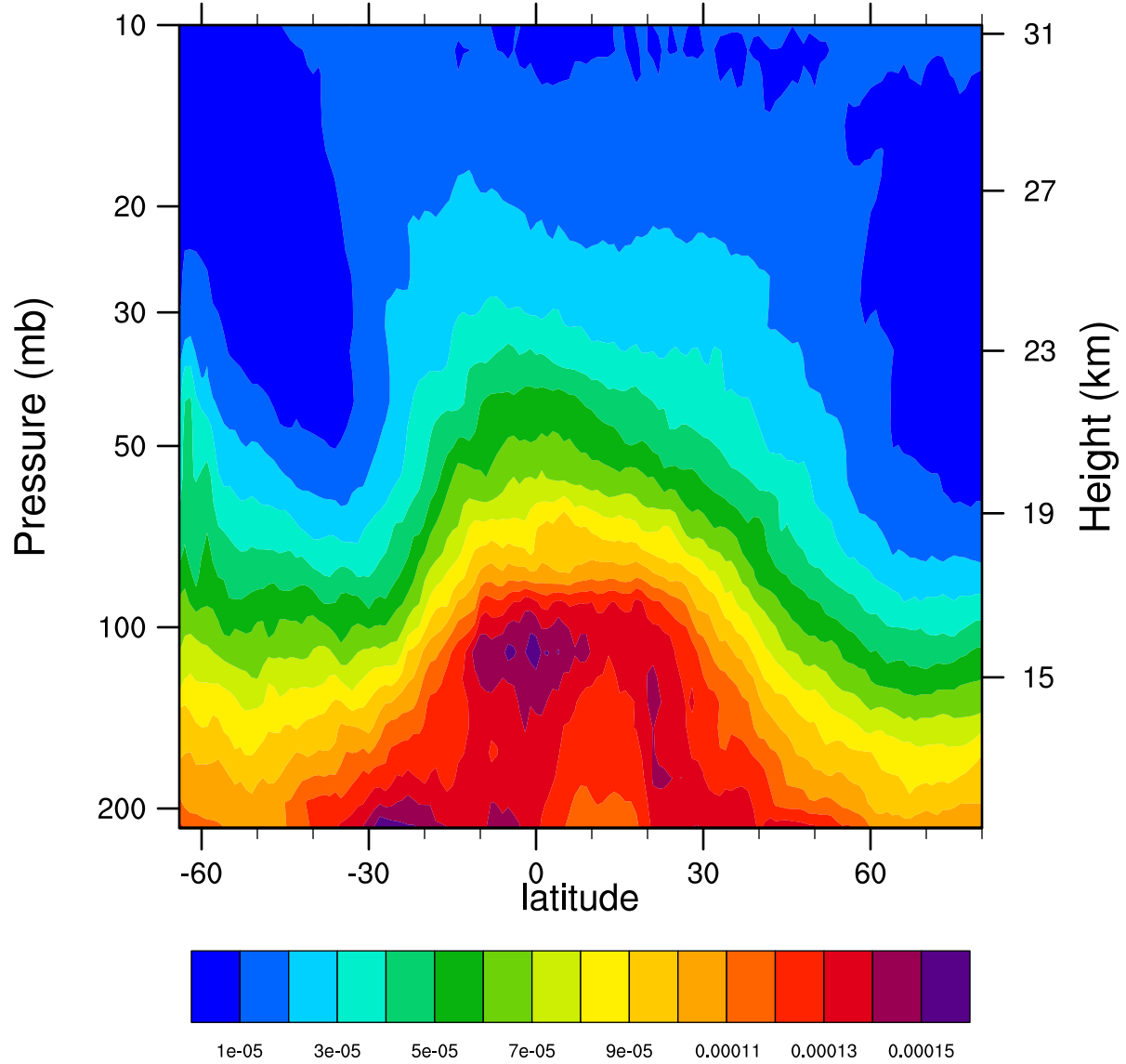
2005d255 12.1MicronExtinction_Combined ( \text{km}^{-1} )
