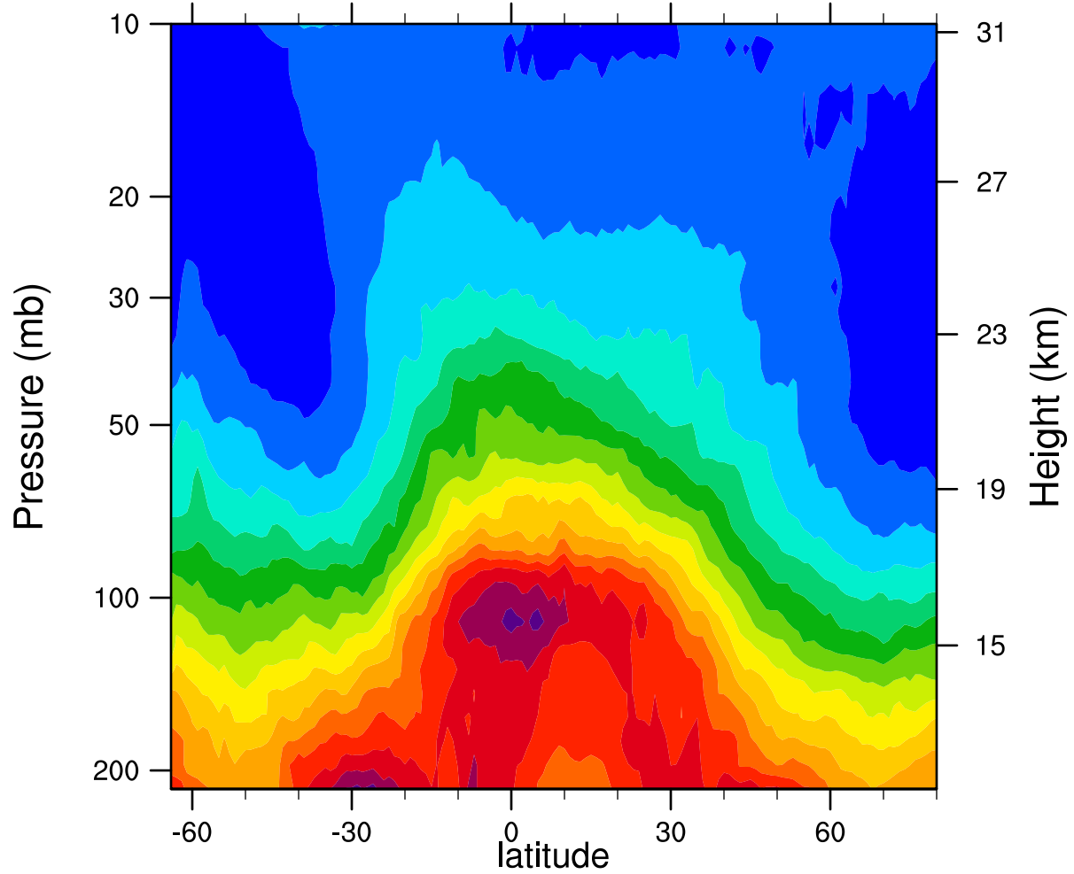
2005d261 12.1MicronExtinction_Combined (km -1 )
