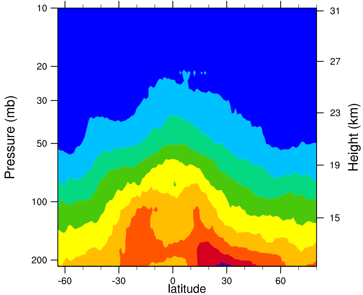
2007d108 12.1MicronExtinction_Combined (km -1 )
