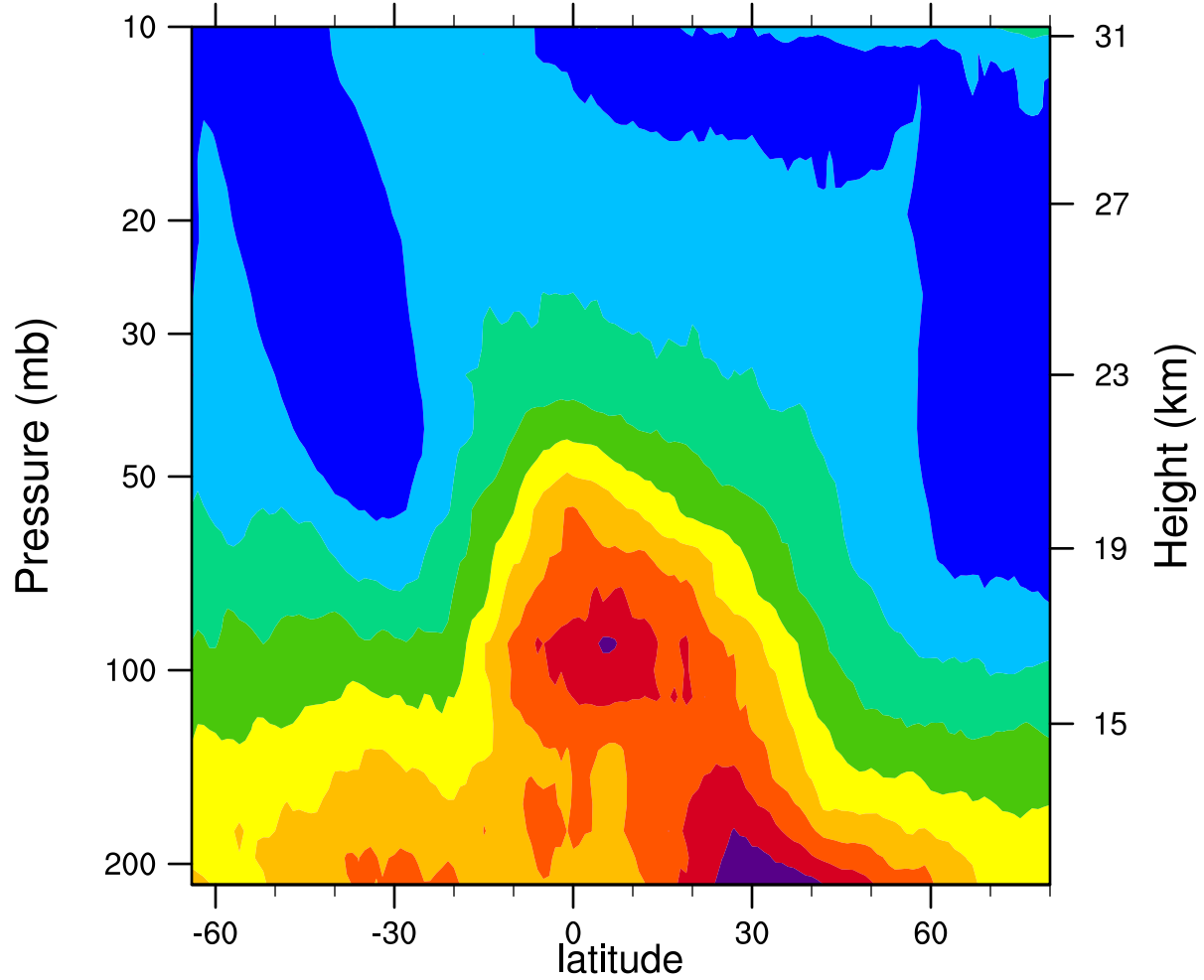
2005d149 12.1MicronExtinction_Combined (km -1 )
