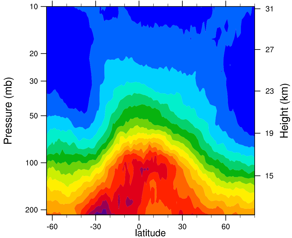
2005d282 12.1MicronExtinction_Combined (km -1 )
