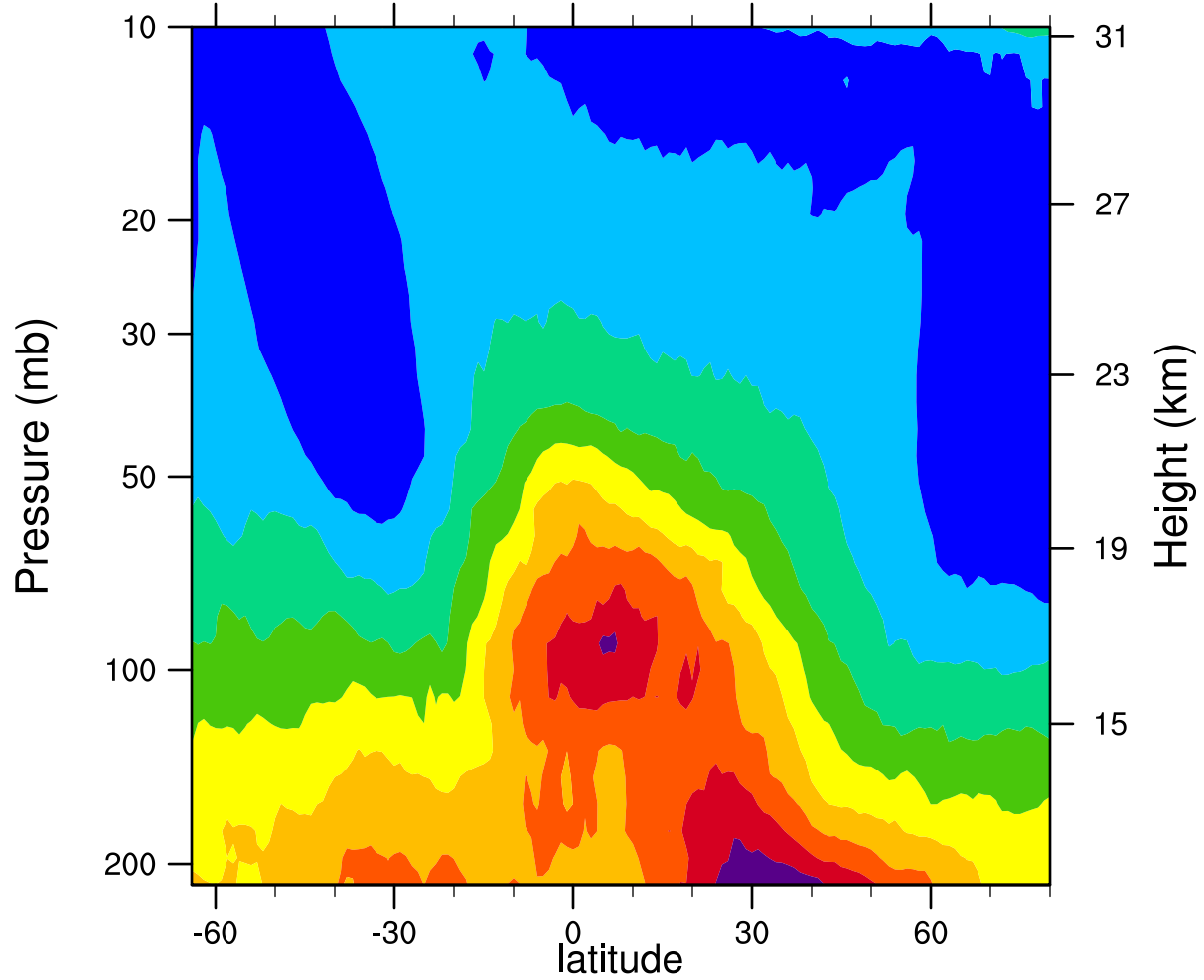
2005d151 12.1MicronExtinction_Combined (km -1 )
