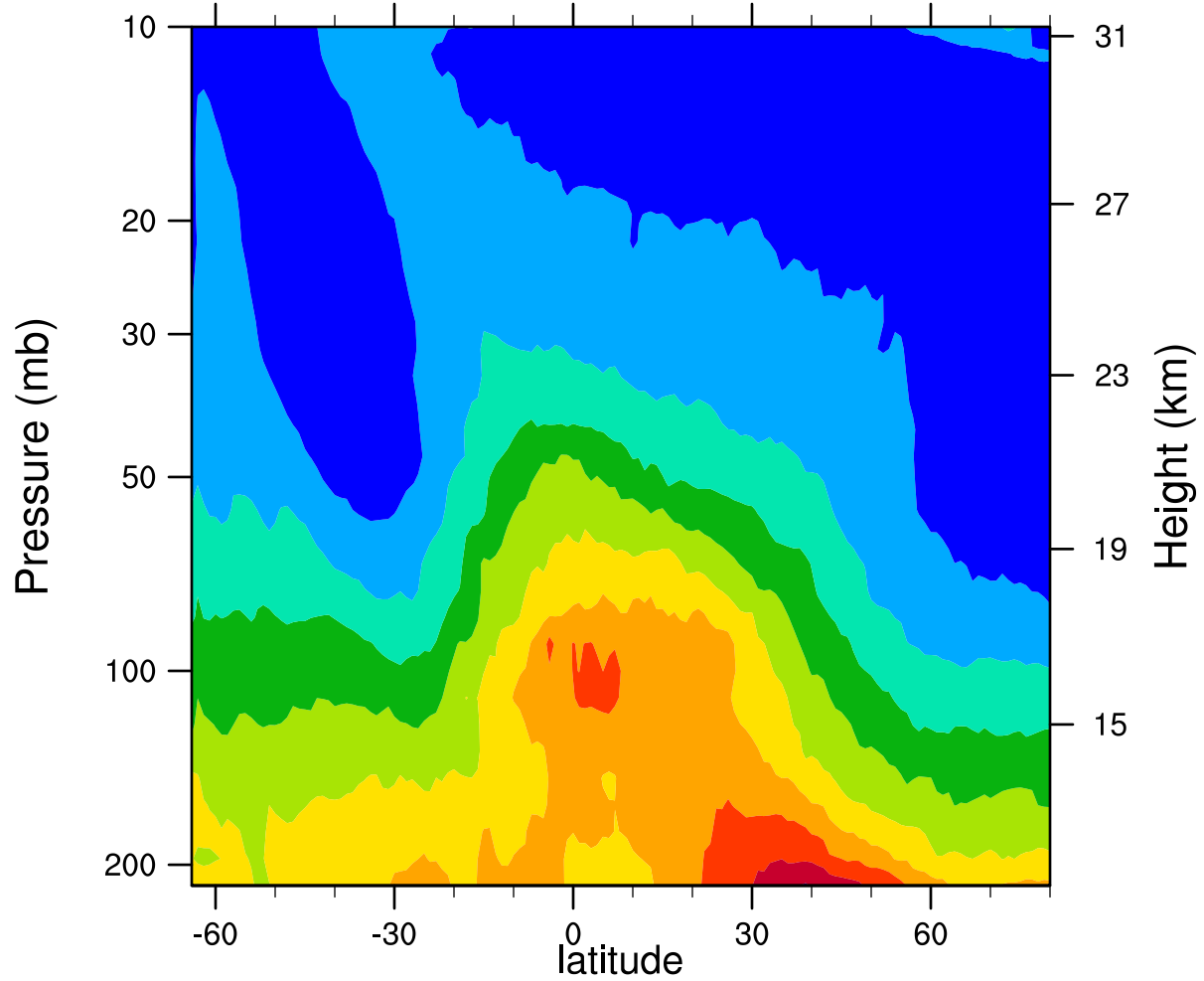
2005d174 12.1MicronExtinction_Combined (km -1 )
