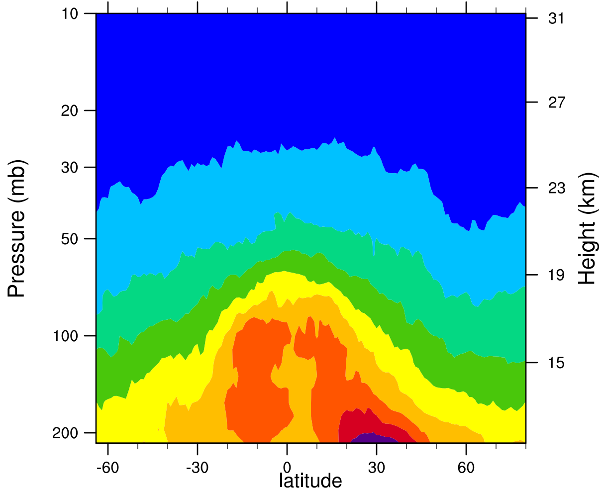
2006d123 12.1MicronExtinction_Combined (km -1 )
