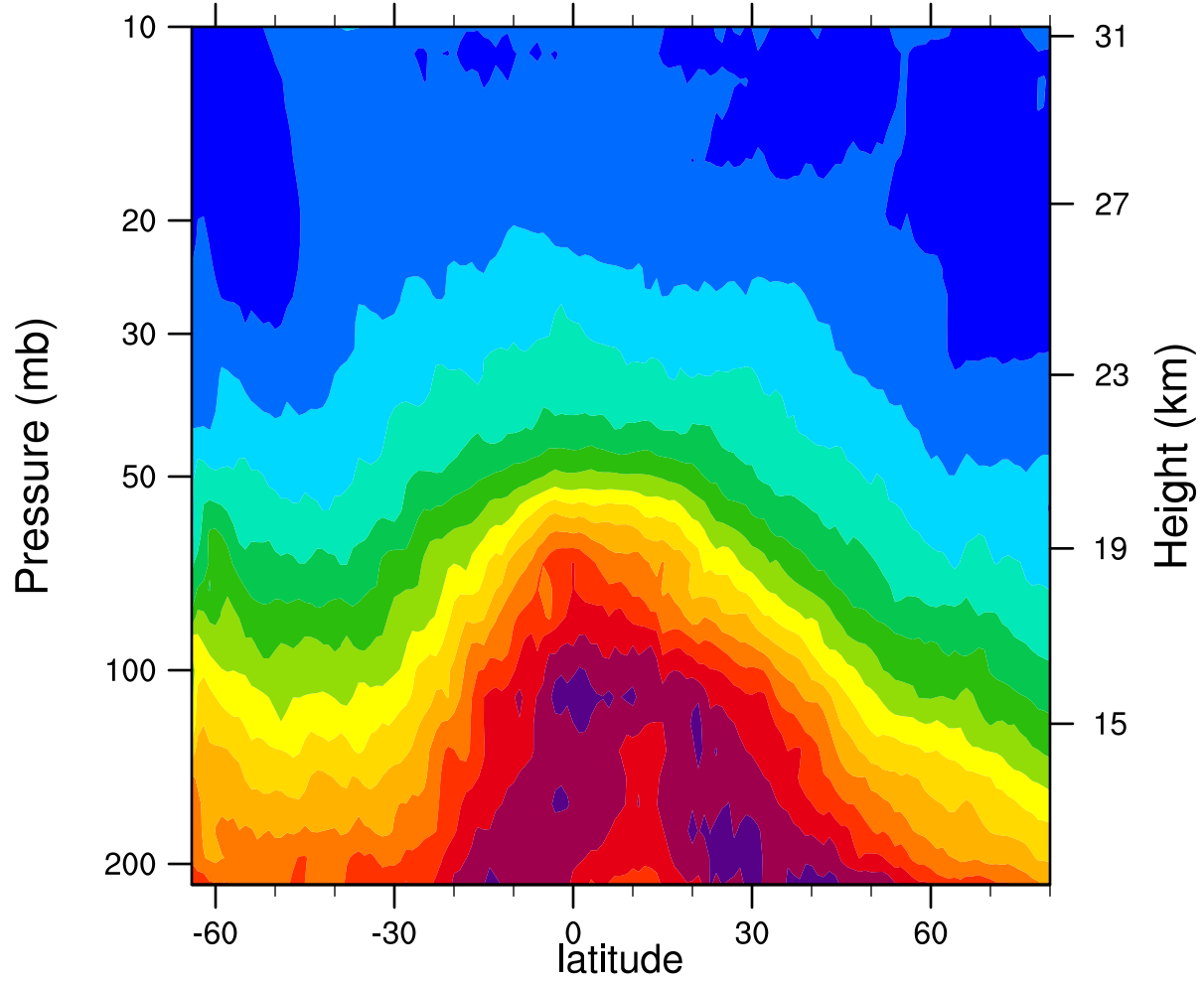
2006d243 12.1MicronExtinction_Combined (km -1 )
