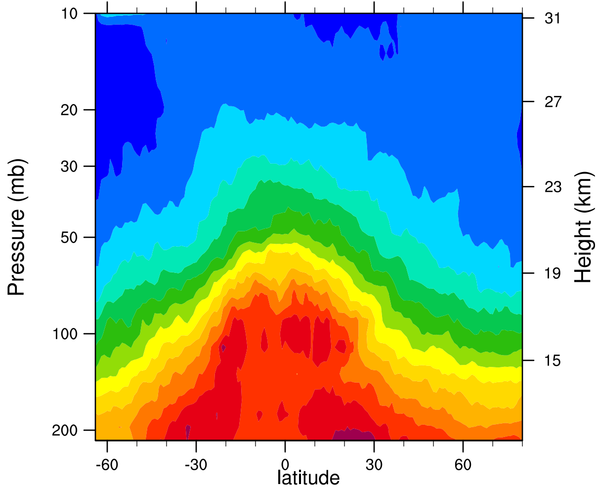
2005d345 12.1MicronExtinction_Combined (km -1 )
