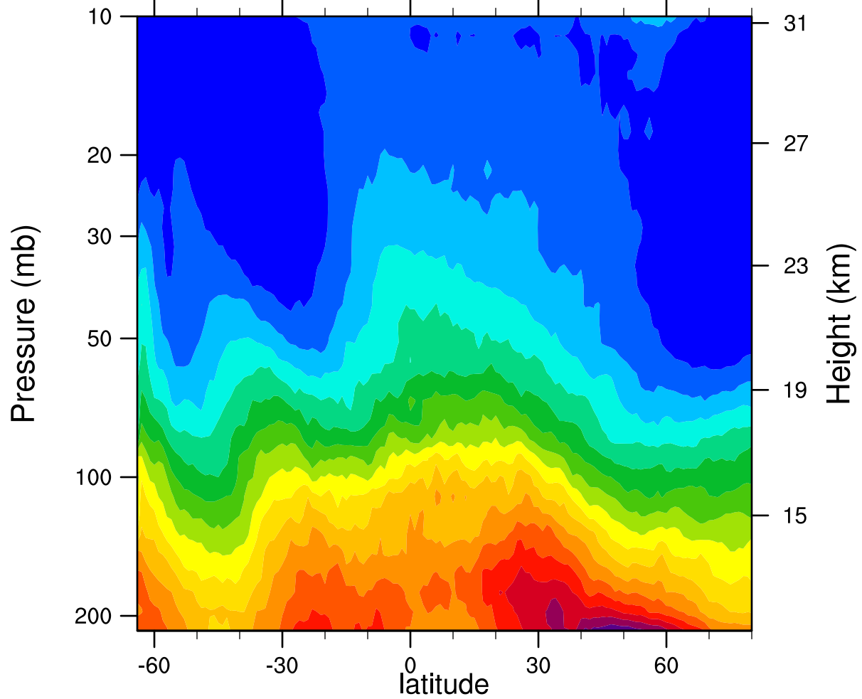
2007d215 12.1MicronExtinction_Combined (km -1 )
