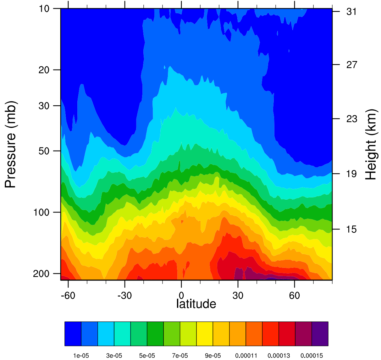
2007d233 12.1MicronExtinction_Combined (km -1 )
