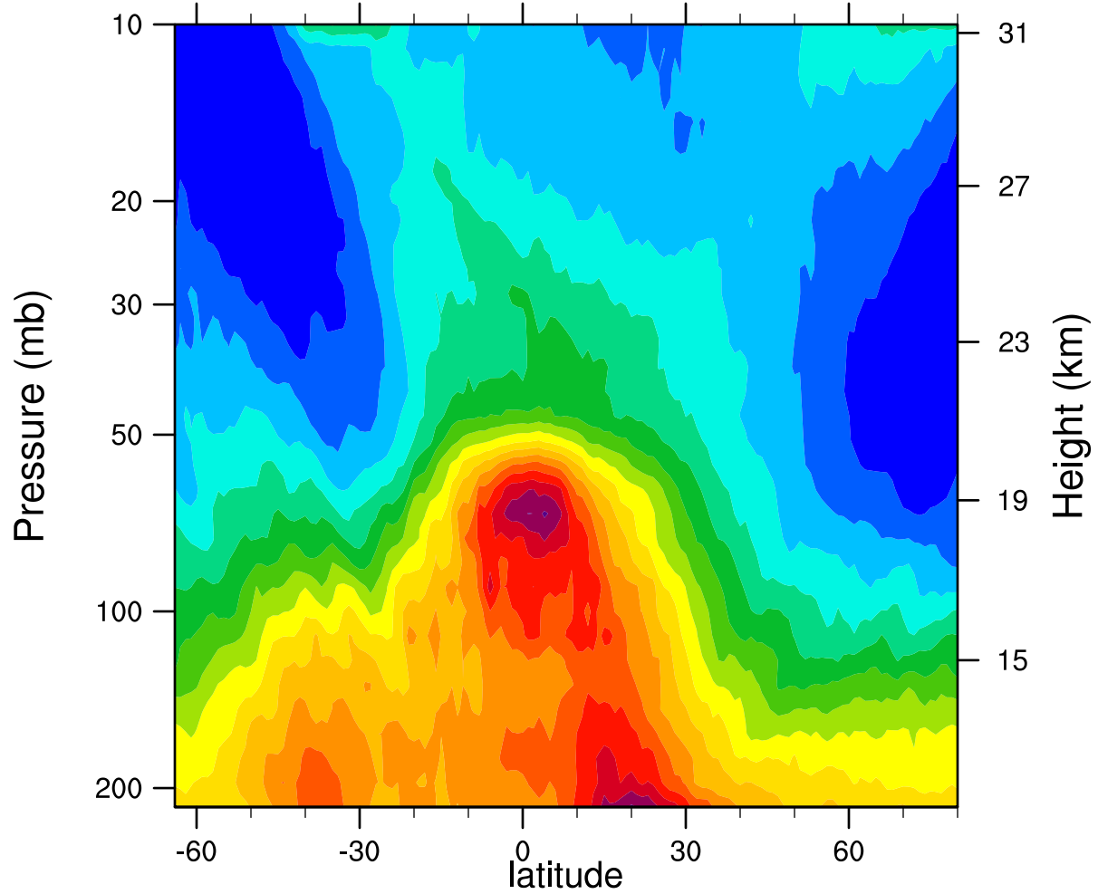
2005d076 12.1MicronExtinction_Combined (km -1 )
