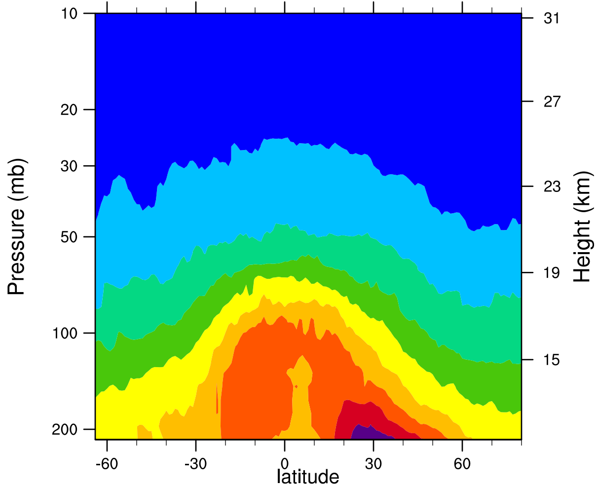
2006d138 12.1MicronExtinction_Combined (km -1 )
