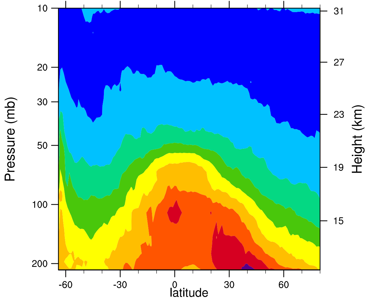
2006d223 12.1MicronExtinction_Combined ( \text{km}^{-1} )
