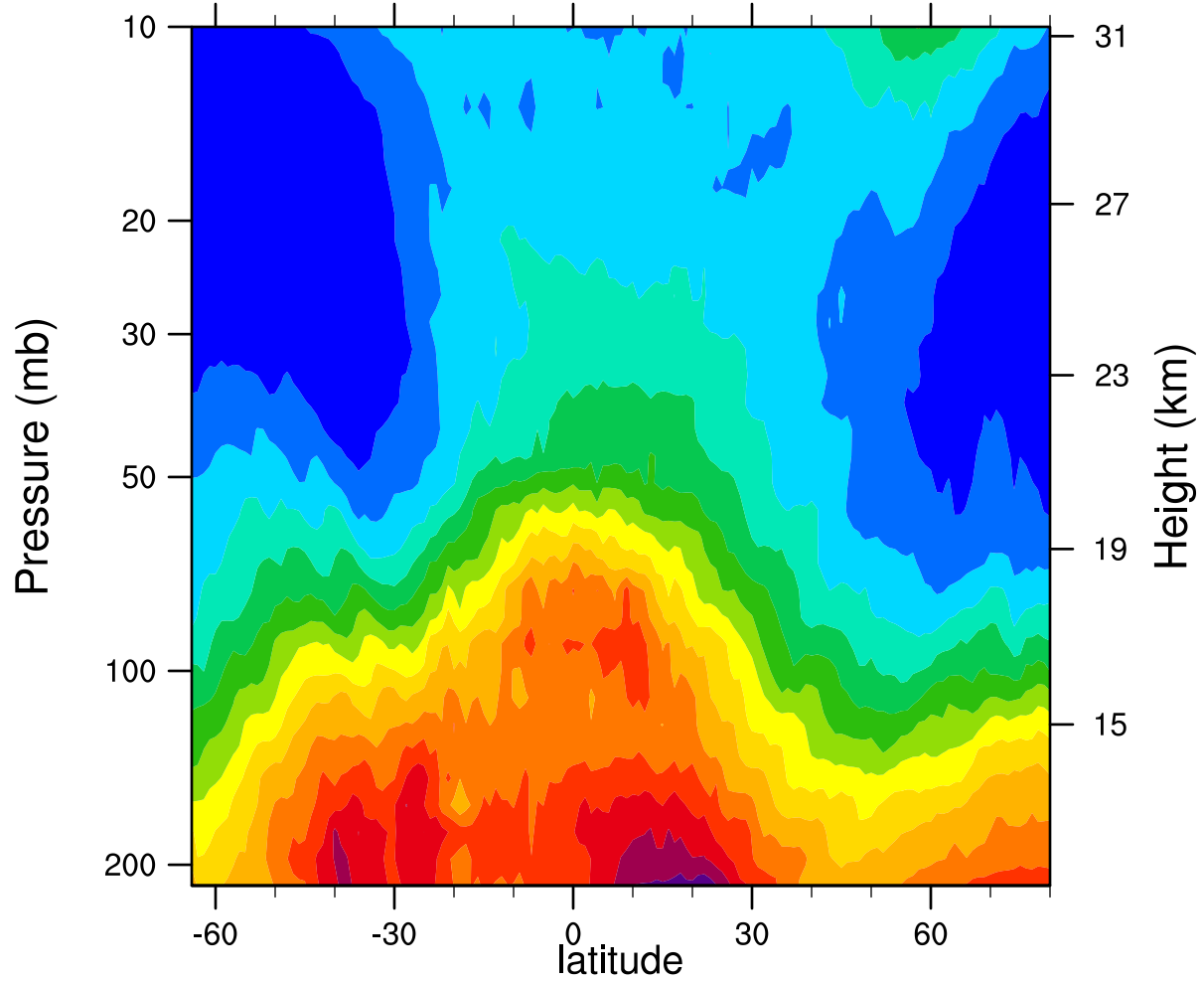
2005d034 12.1MicronExtinction_Combined (km -1 )
