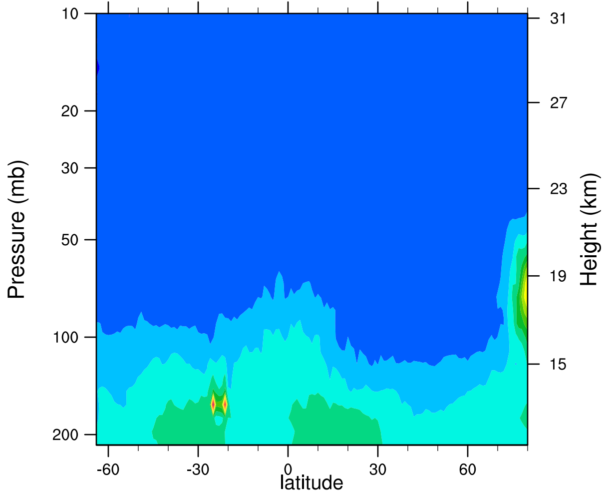
2005d023 12.1MicronExtinction_Combined (km -1 )
