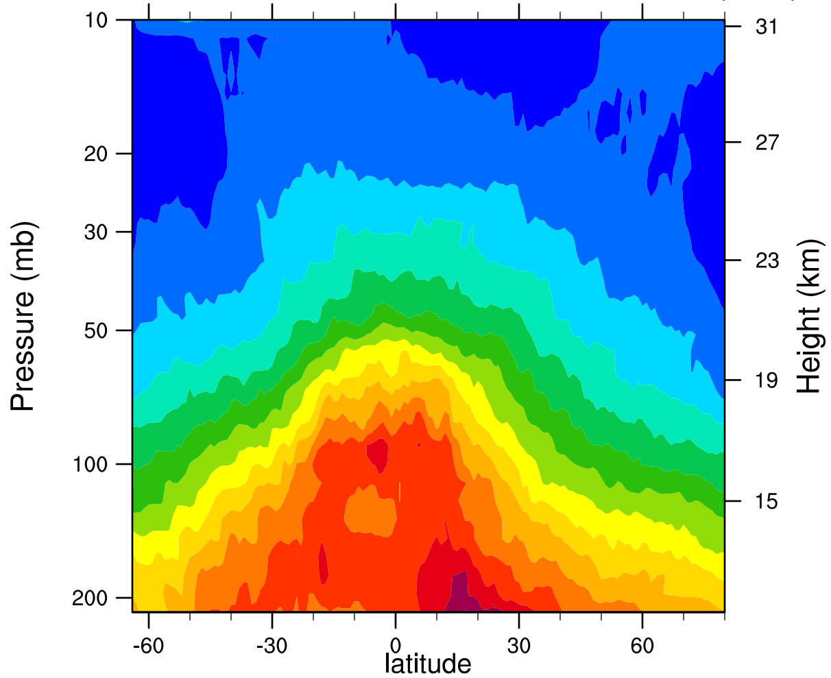
2006d046 12.1MicronExtinction_Combined (km -1 )
