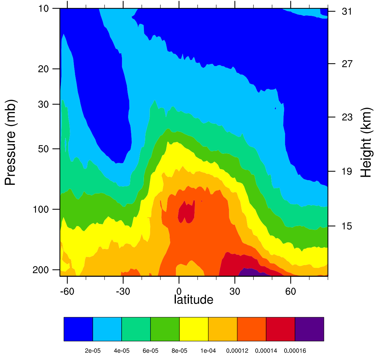
2005d177 12.1MicronExtinction_Combined (km -1 )
