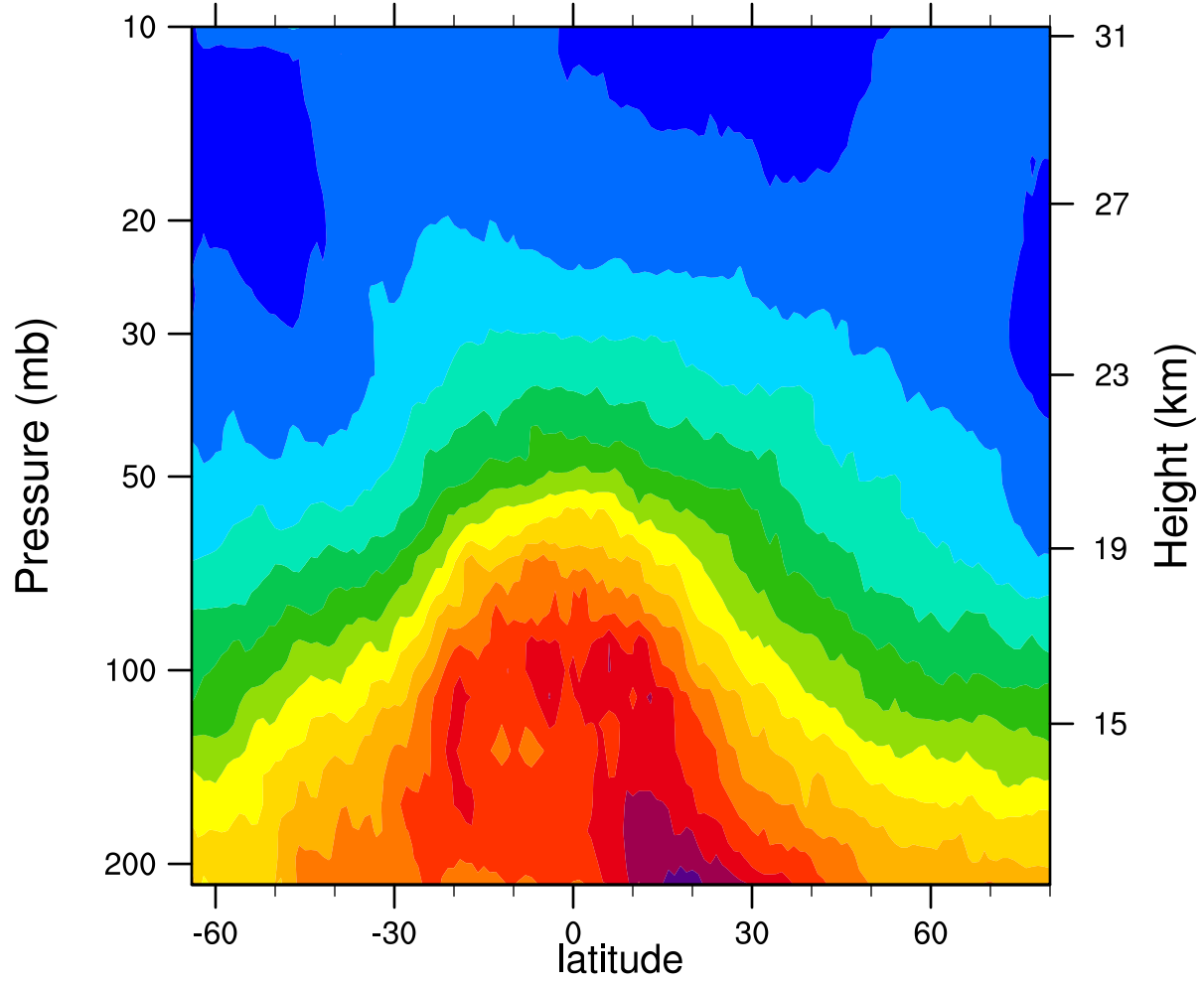
2006d063 12.1MicronExtinction_Combined (km -1 )
