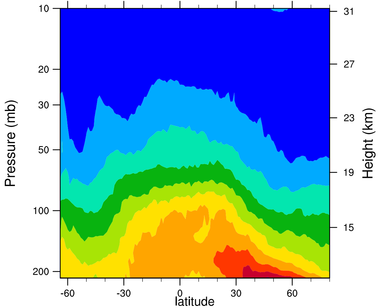
2007d197 12.1MicronExtinction_Combined (km -1 )
