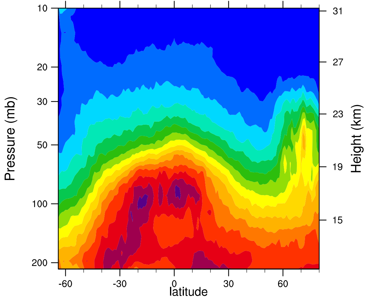
2007d023 12.1MicronExtinction_Combined (km -1 )
