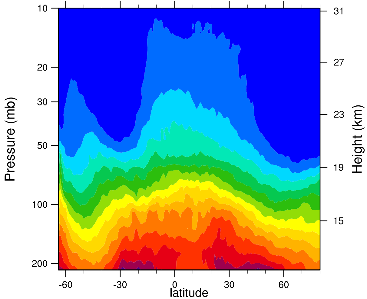
2007d257 12.1MicronExtinction_Combined (km -1 )
