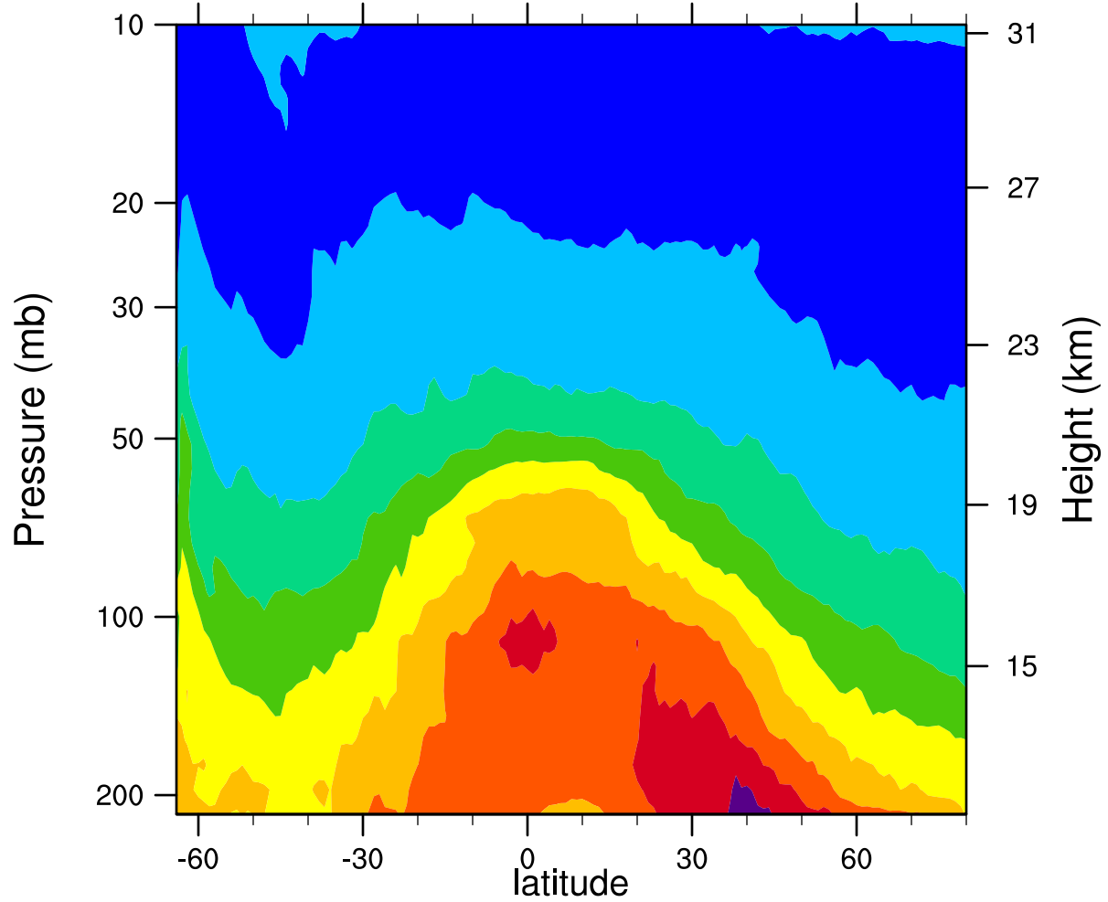
2006d221 12.1MicronExtinction_Combined (km -1 )
