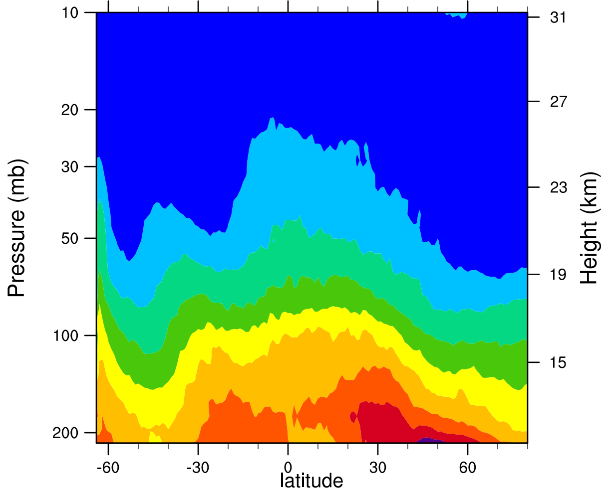
2007d213 12.1MicronExtinction_Combined (km -1 )
