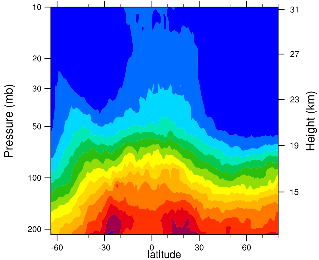
2007d344 12.1MicronExtinction_Combined (km -1 )
