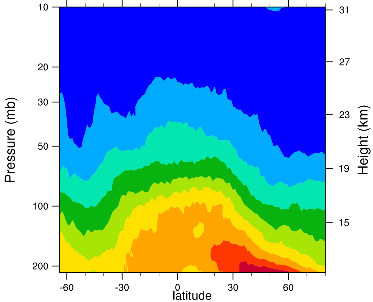
2007d196 12.1MicronExtinction_Combined (km -1 )
