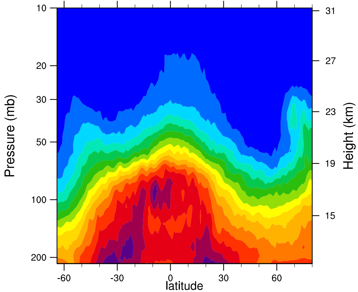
2006d352 12.1MicronExtinction_Combined (km -1 )
