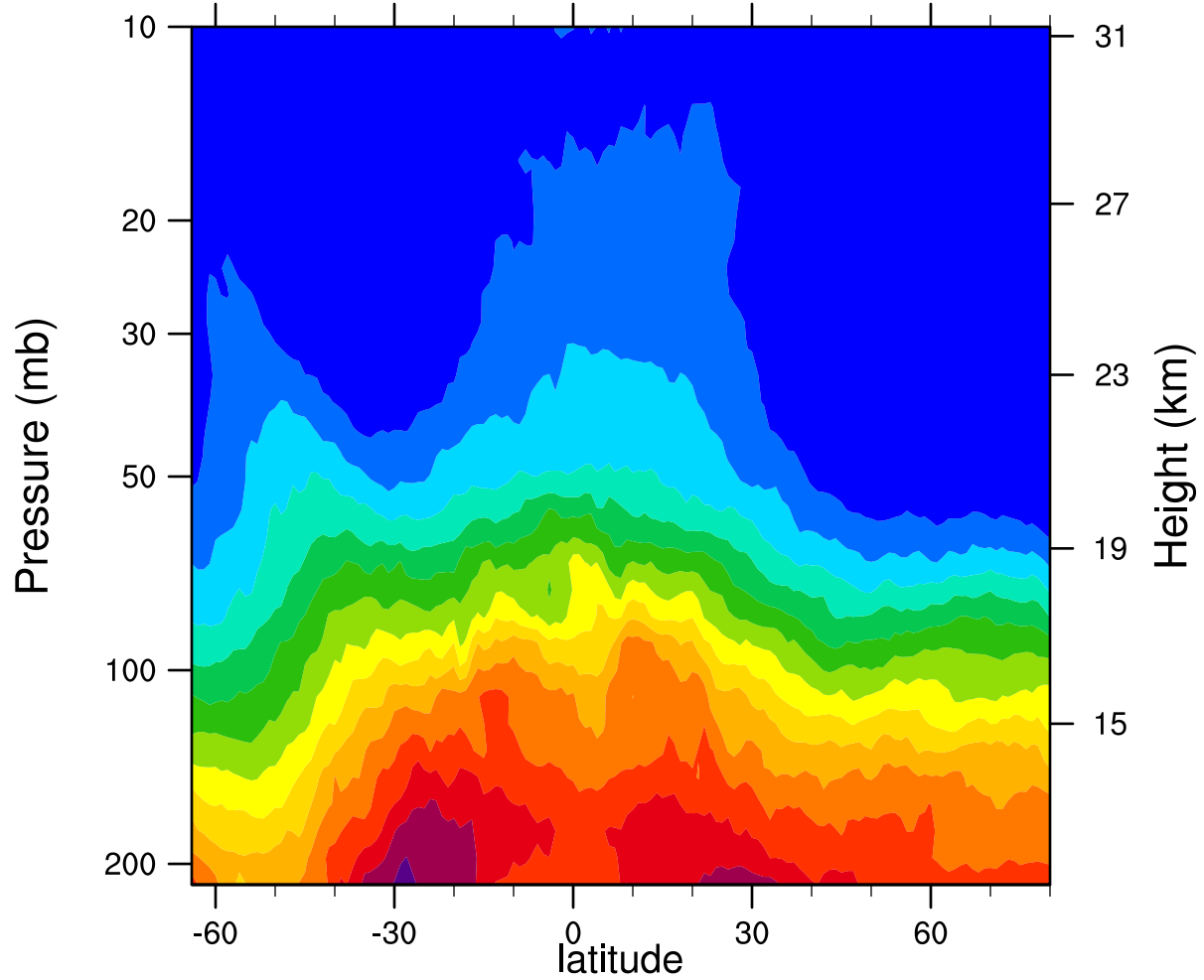
2007d321 12.1MicronExtinction_Combined (km -1 )
