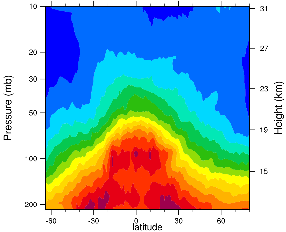
2005d335 12.1MicronExtinction_Combined ( \text{km}^{-1} )
