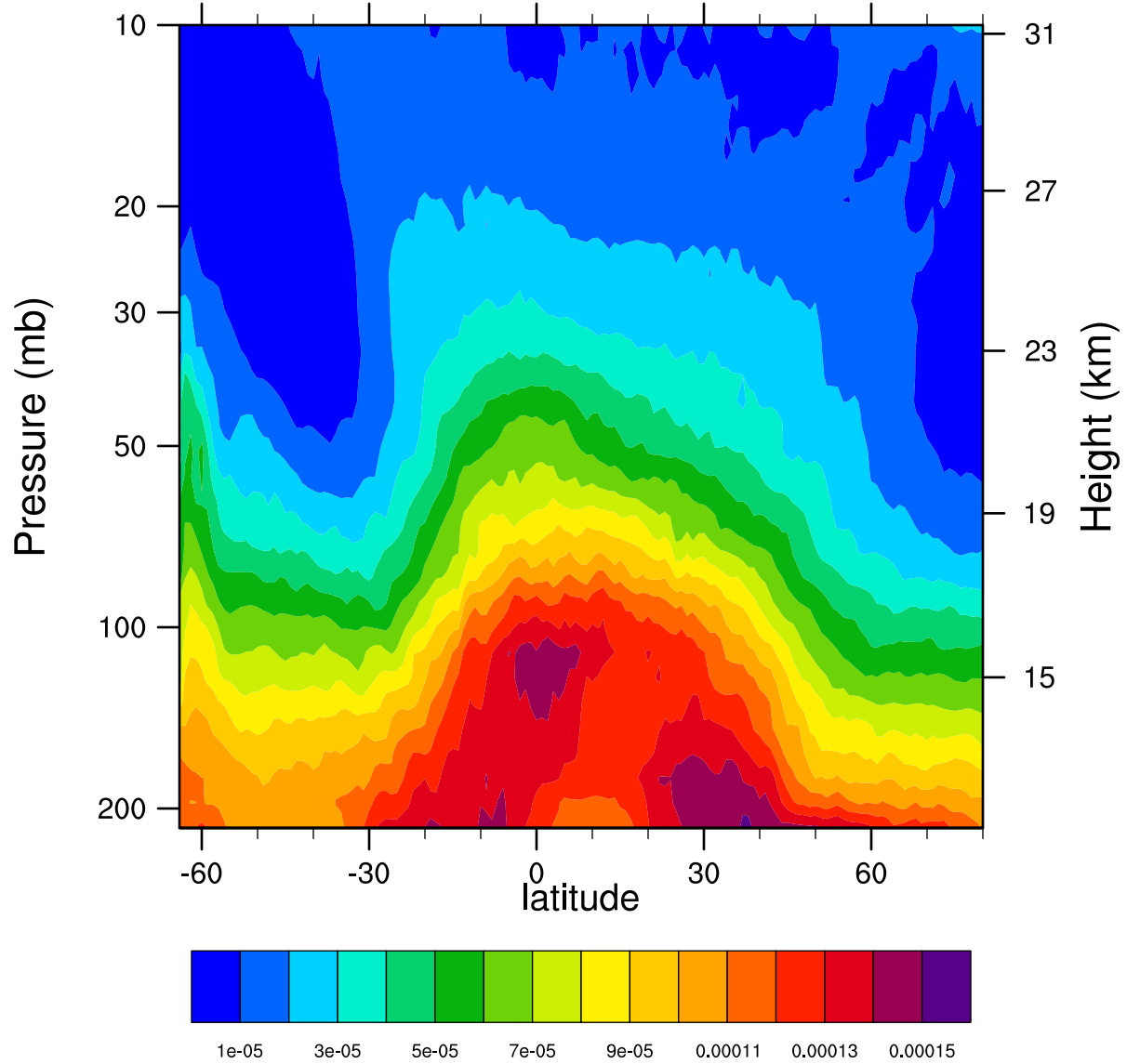
2005d227 12.1MicronExtinction_Combined (km -1 )
