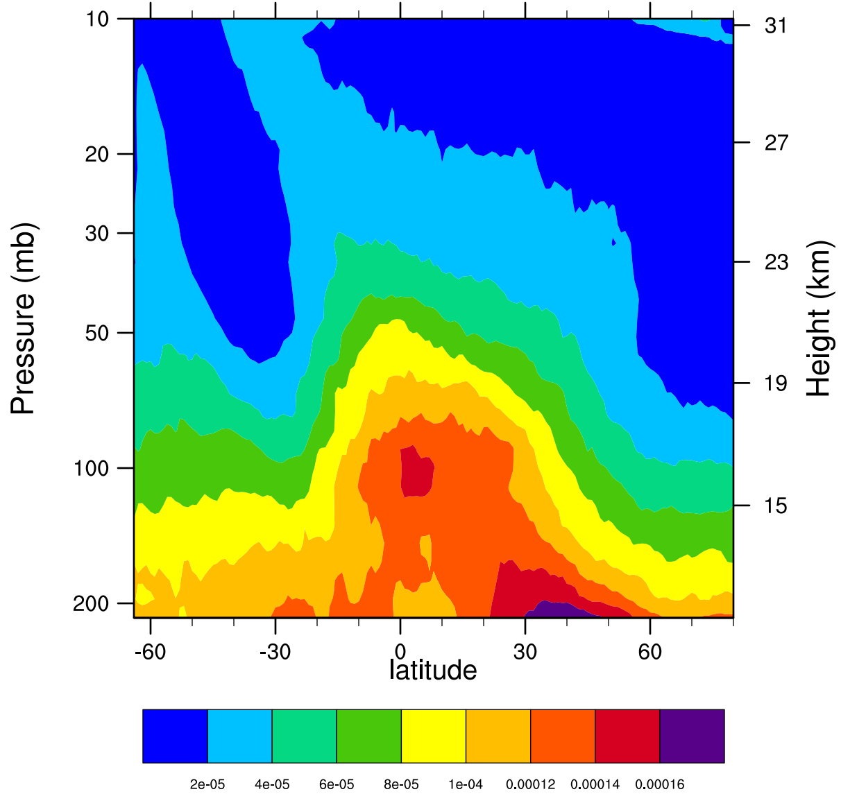
2005d173 12.1MicronExtinction_Combined ( \text{km}^{-1} )
