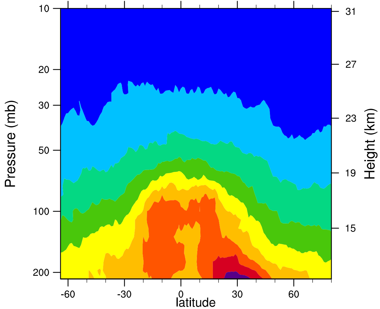
2006d126 12.1MicronExtinction_Combined (km -1 )
