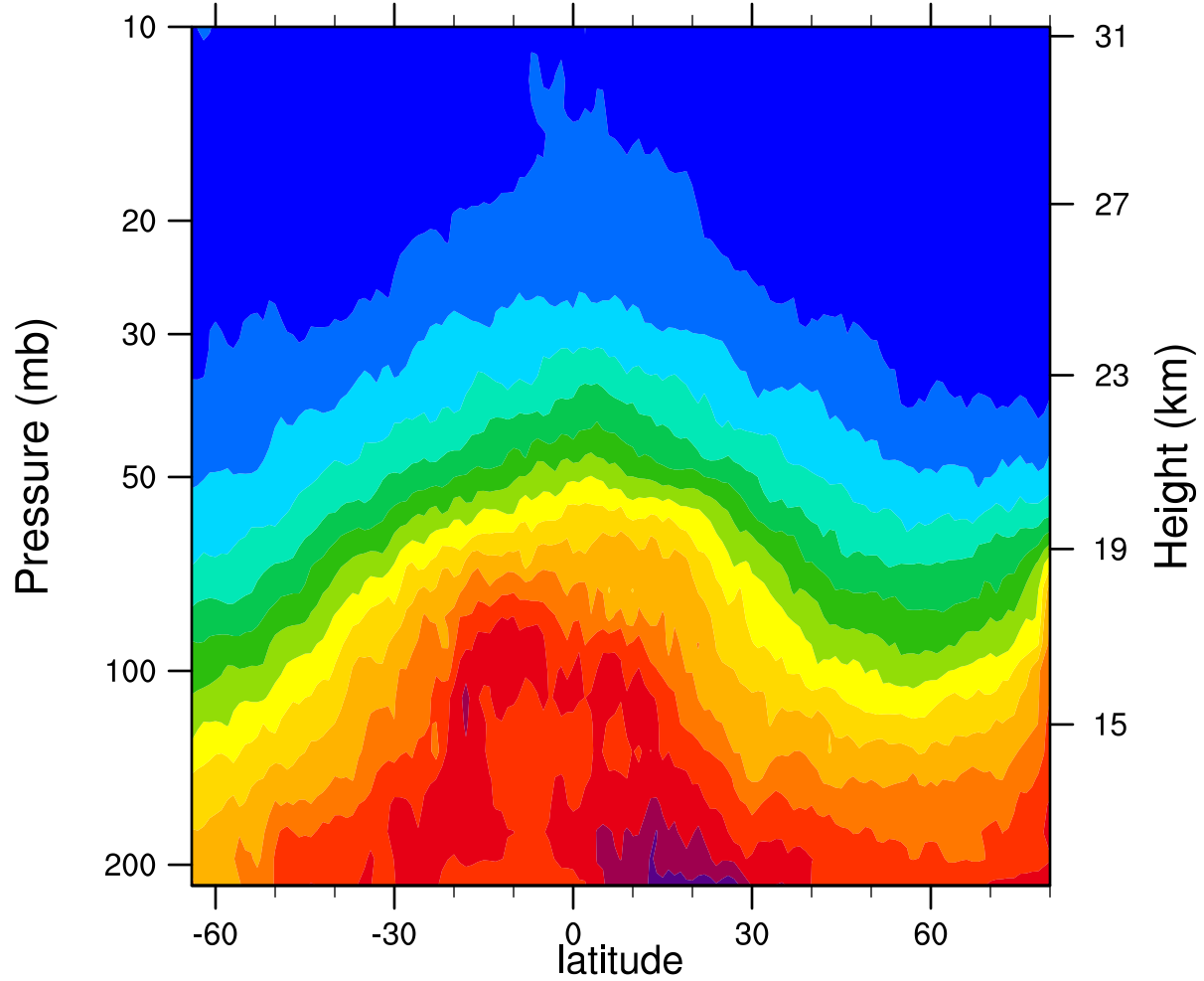
2007d048 12.1MicronExtinction_Combined (km -1 )
