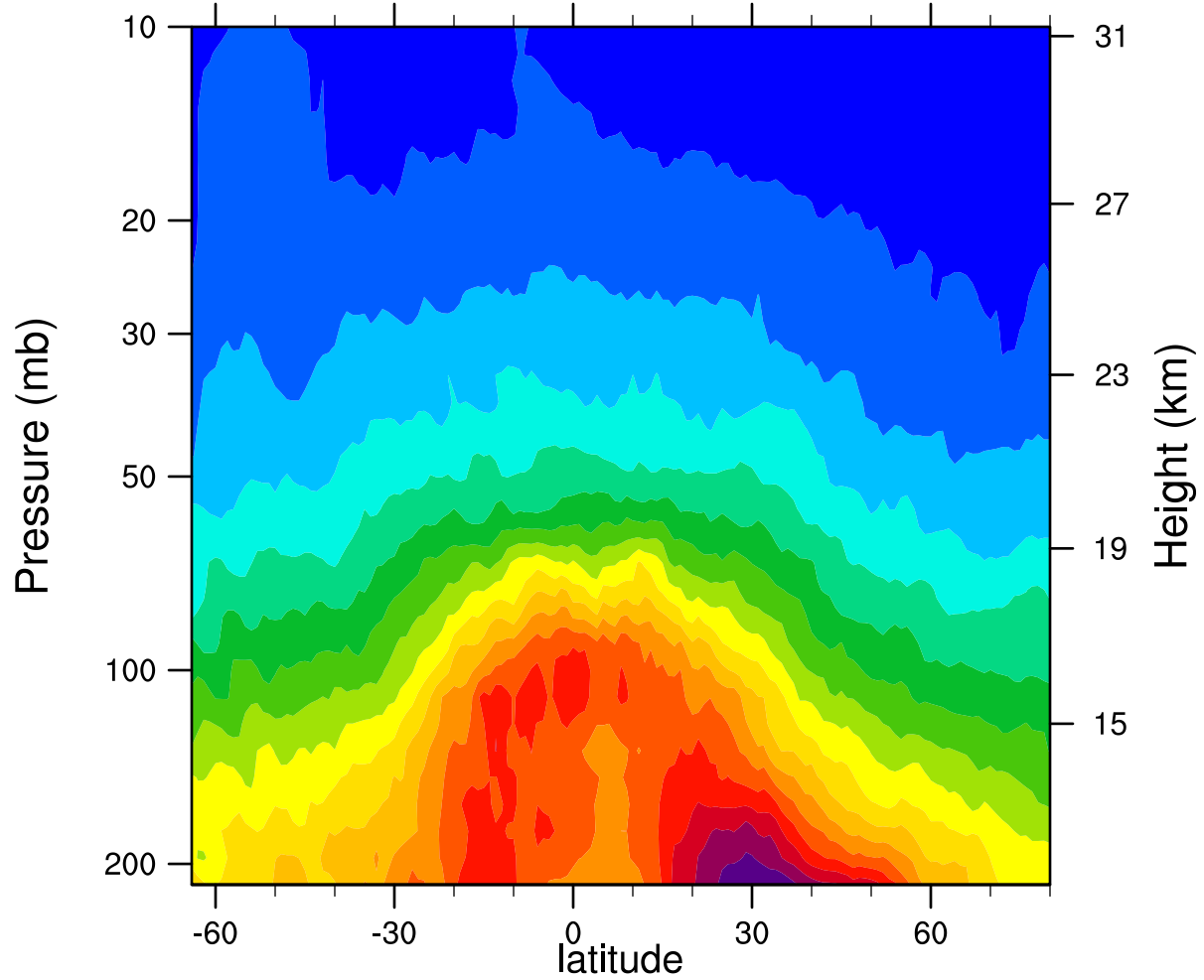
2006d143 12.1MicronExtinction_Combined (km -1 )
