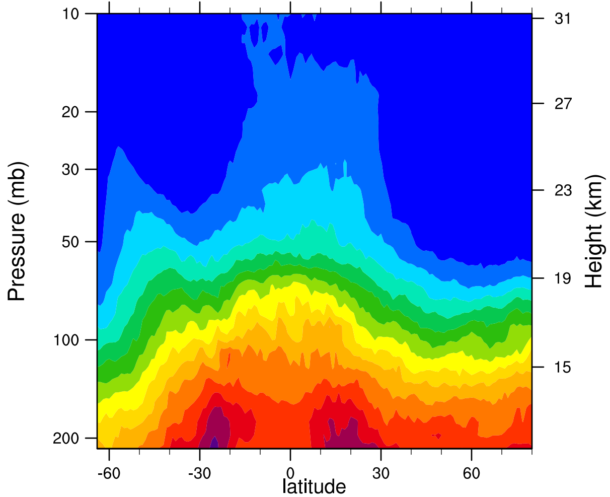
2007d342 12.1MicronExtinction_Combined (km -1 )
