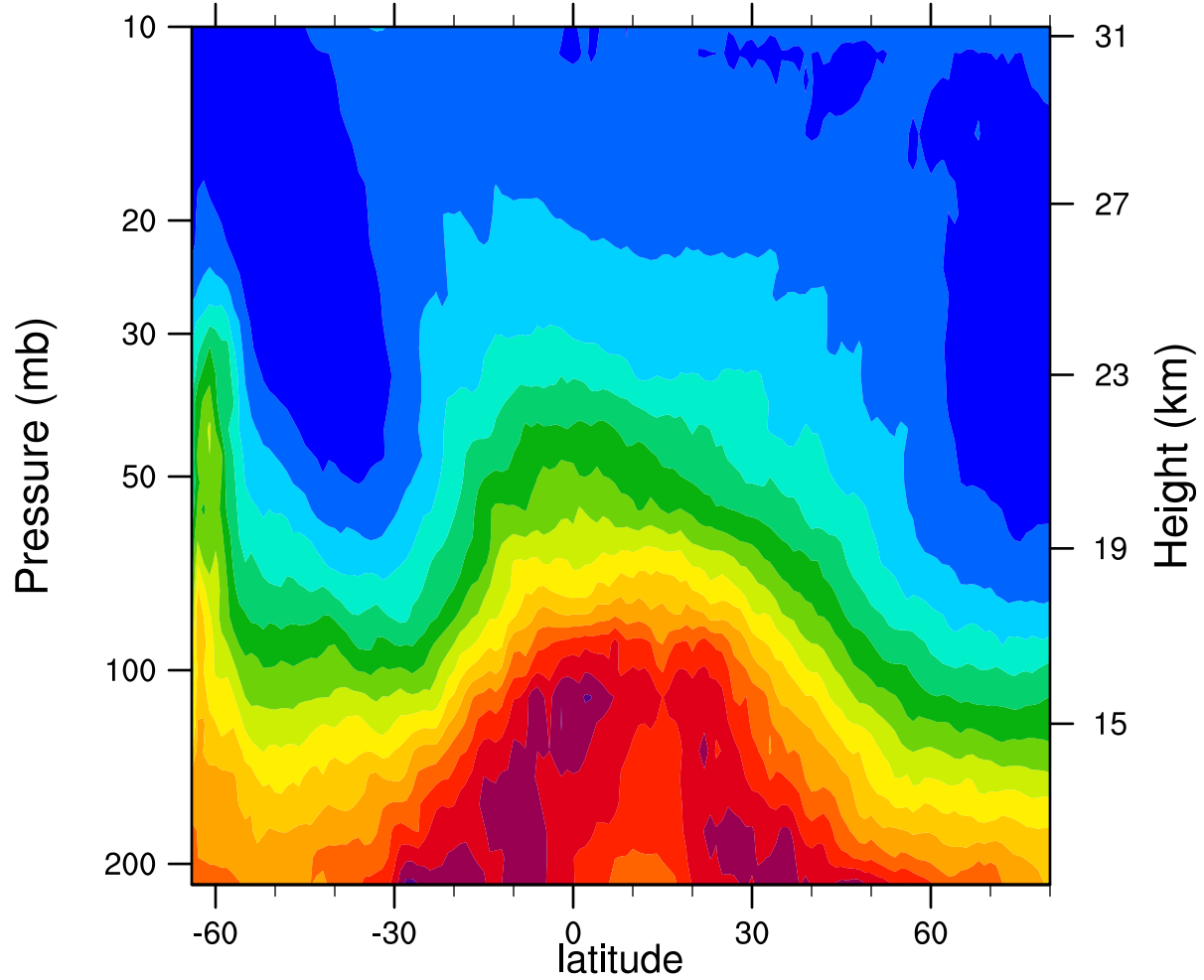
2005d242 12.1MicronExtinction_Combined (km -1 )
