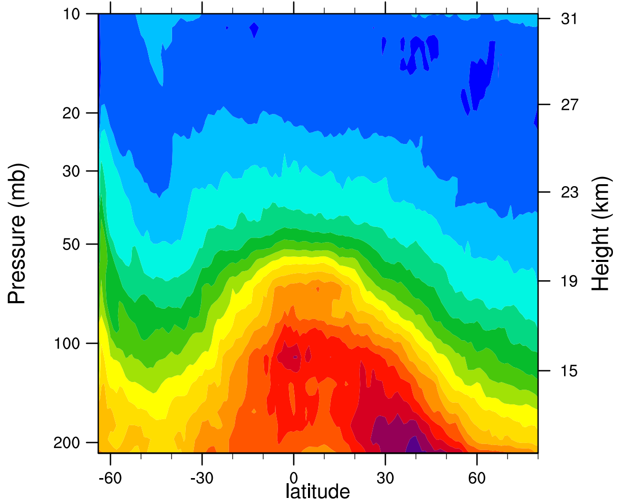
2006d219 12.1MicronExtinction_Combined (km -1 )
