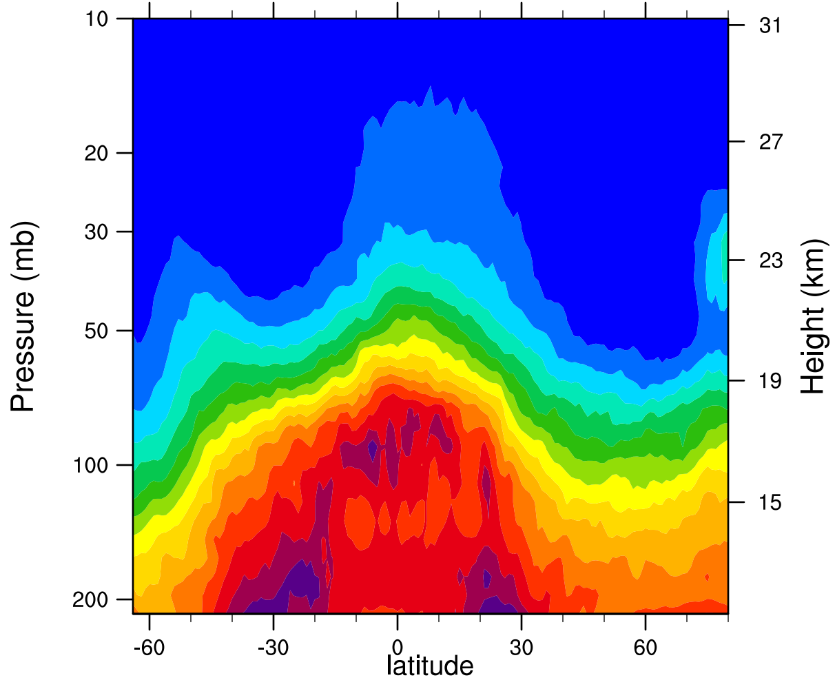
2006d345 12.1MicronExtinction_Combined (km -1 )
