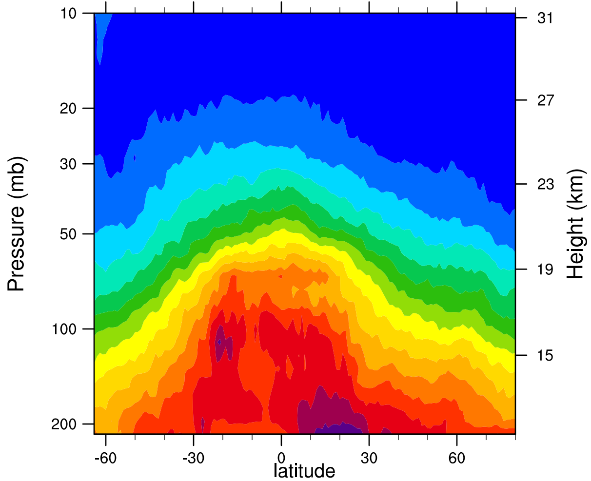
2007d056 12.1MicronExtinction_Combined ( \text{km}^{-1} )
