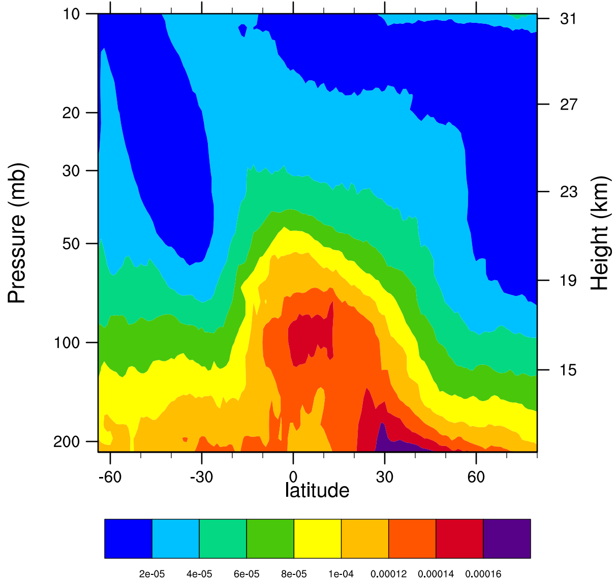
2005d163 12.1MicronExtinction_Combined (km -1 )
