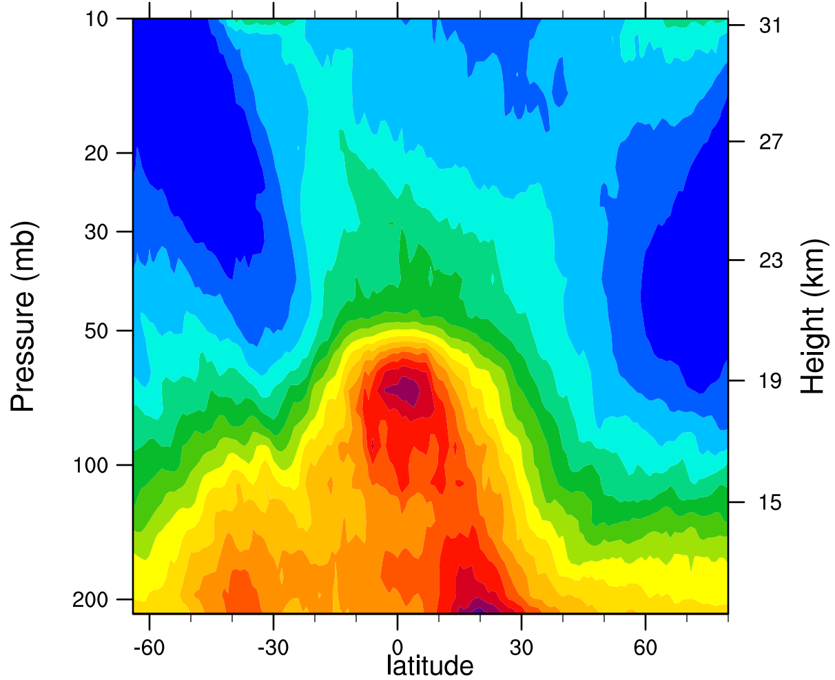
2005d077 12.1MicronExtinction_Combined (km -1 )
