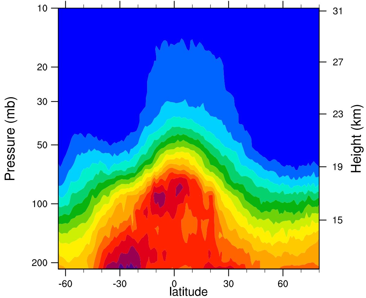
2006d332 12.1MicronExtinction_Combined (km -1 )
