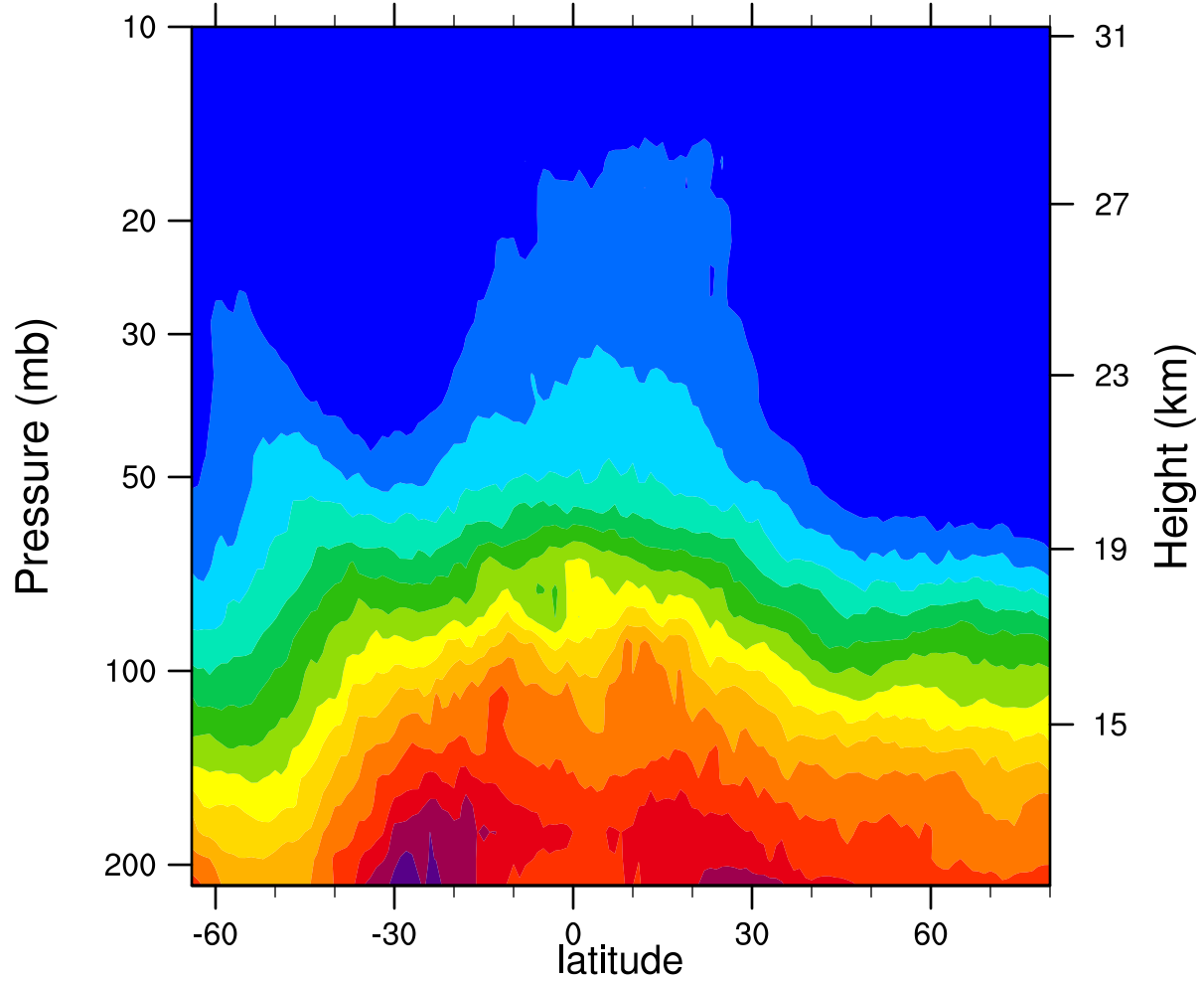
2007d318 12.1MicronExtinction_Combined (km -1 )
