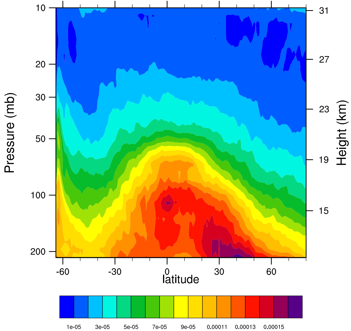
2006d224 12.1MicronExtinction_Combined (km -1 )
