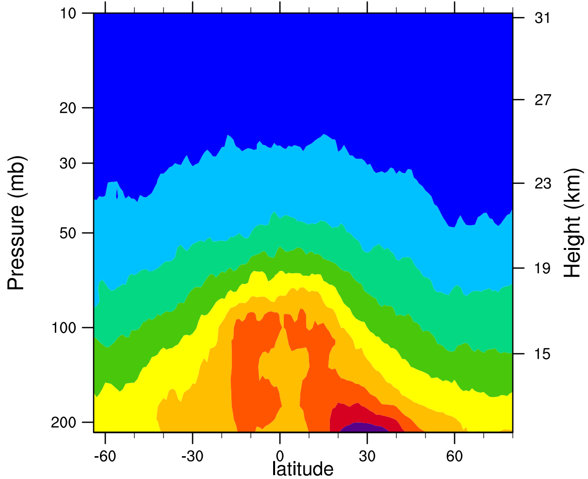
2006d119 12.1MicronExtinction_Combined (km -1 )
