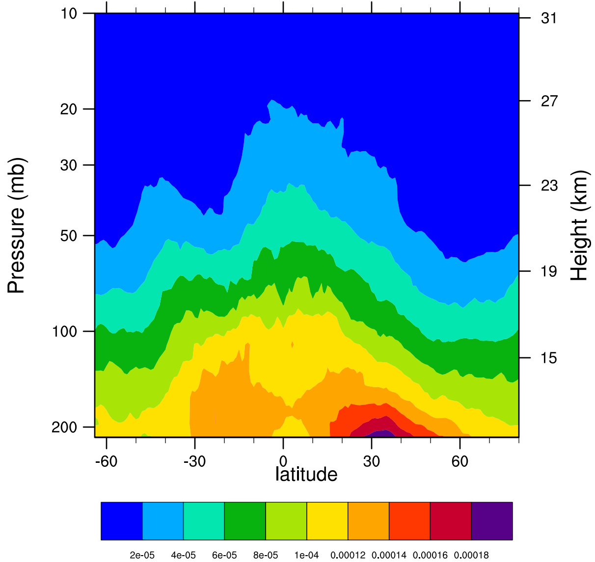
2007d130 12.1MicronExtinction_Combined (km -1 )
