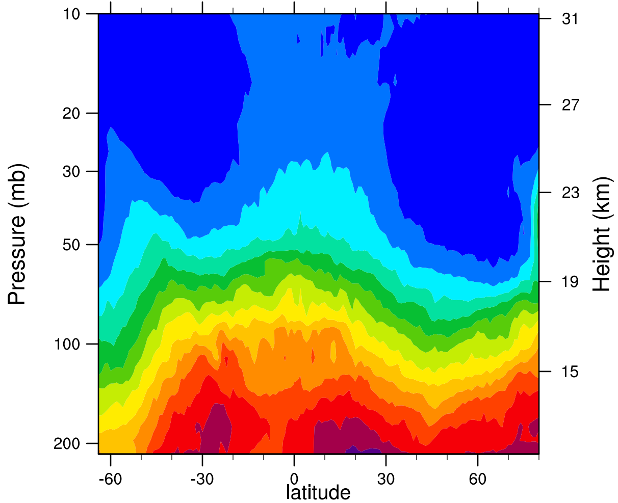
2007d365 12.1MicronExtinction_Combined (km -1 )
