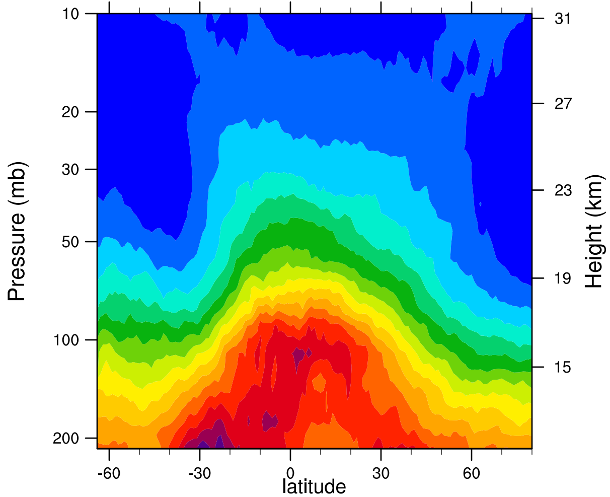
2005d281 12.1MicronExtinction_Combined (km -1 )
