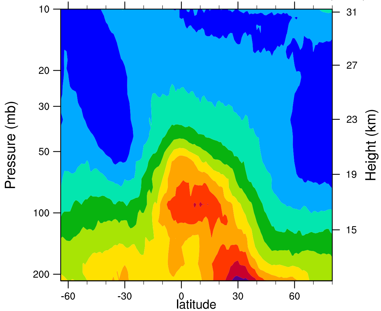
2005d139 12.1MicronExtinction_Combined (km -1 )
