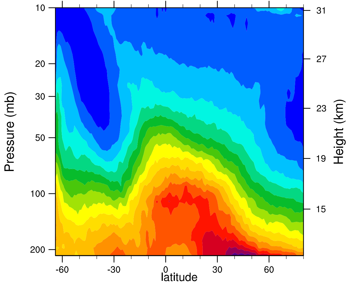
2005d196 12.1MicronExtinction_Combined (km -1 )
