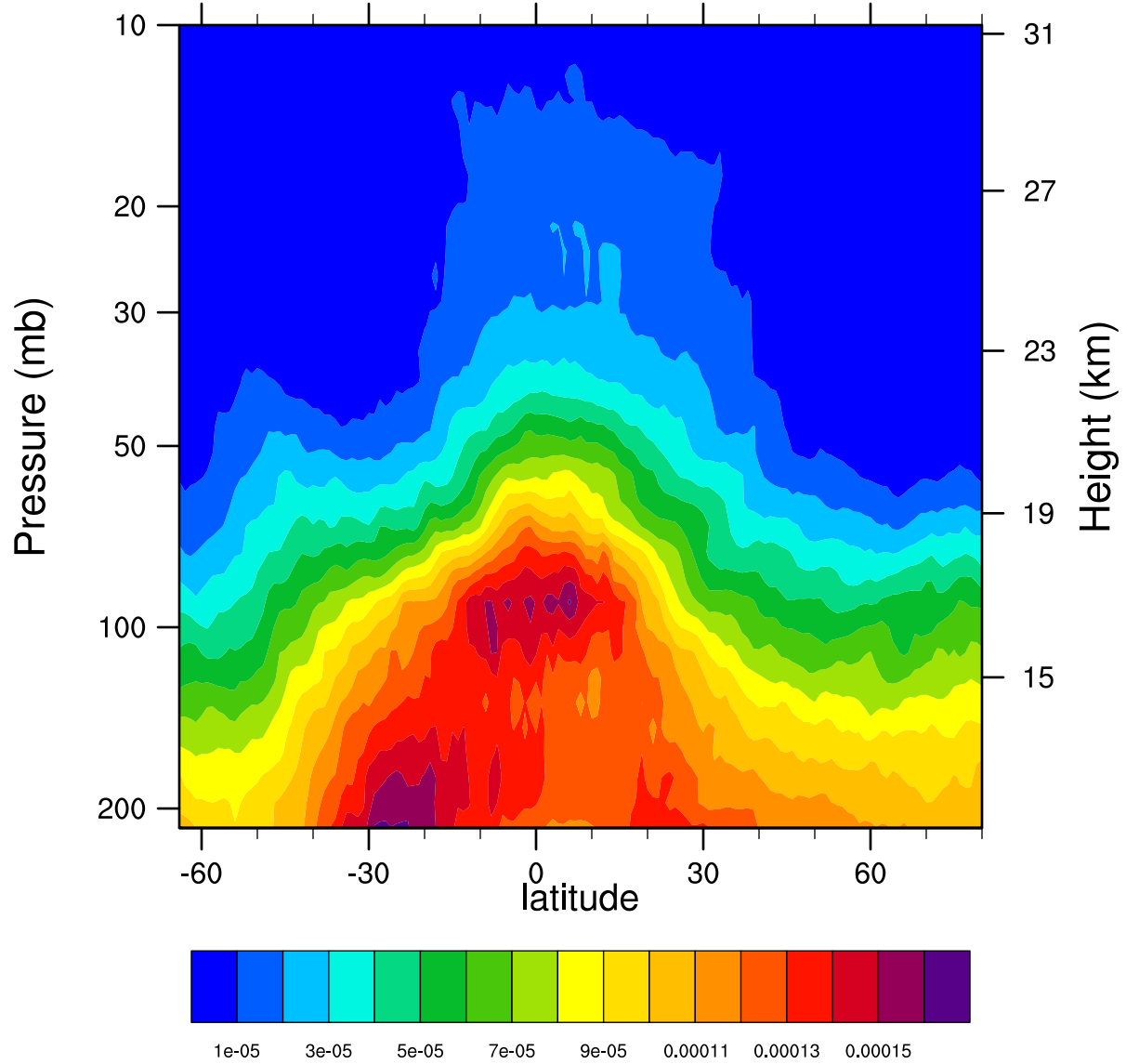
2006d321 12.1MicronExtinction_Combined (km -1 )
