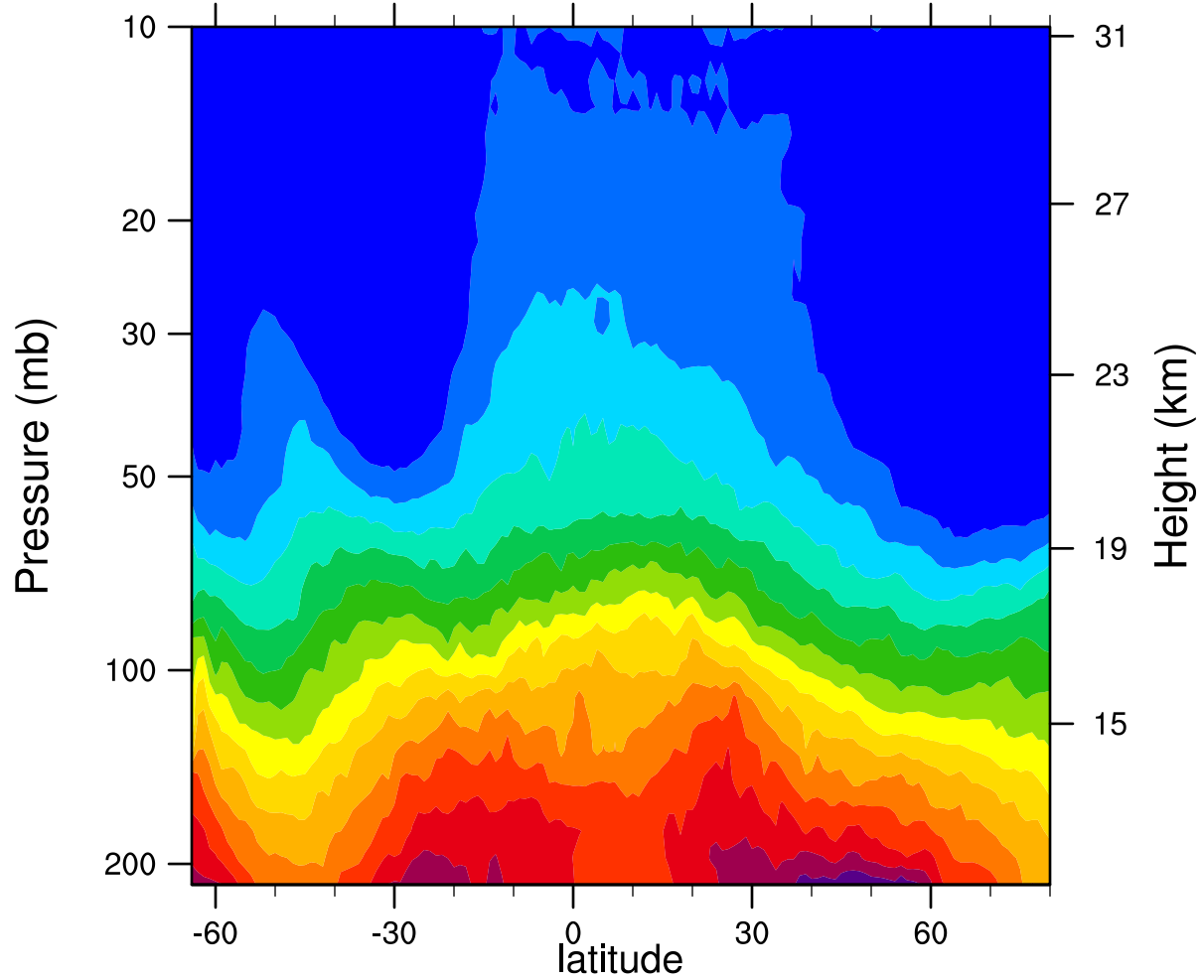
2007d250 12.1MicronExtinction_Combined (km -1 )
