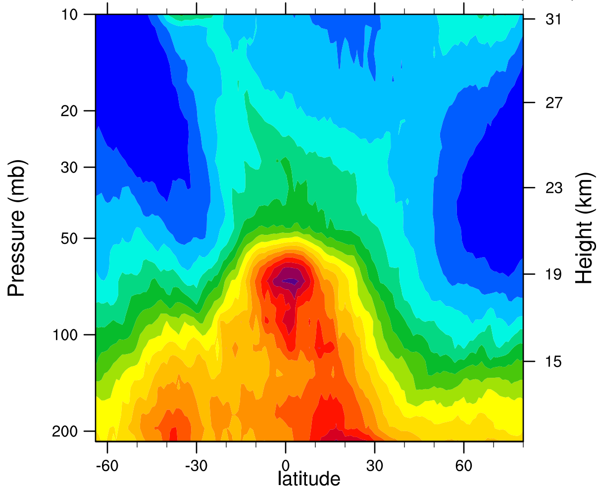
2005d071 12.1MicronExtinction_Combined (km -1 )
