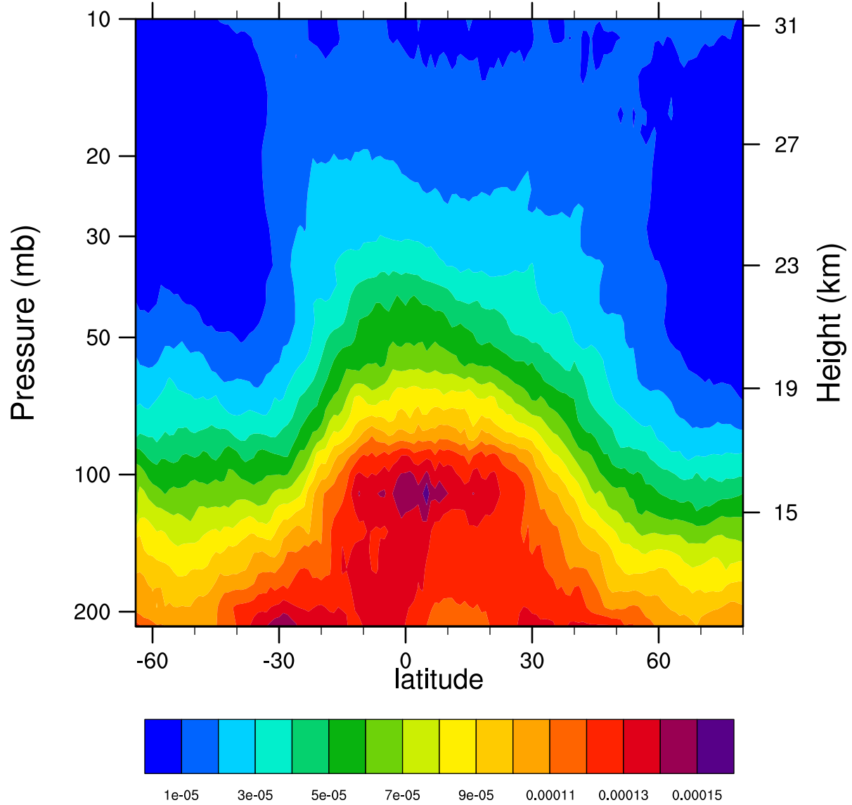
2005d266 12.1MicronExtinction_Combined (km -1 )
