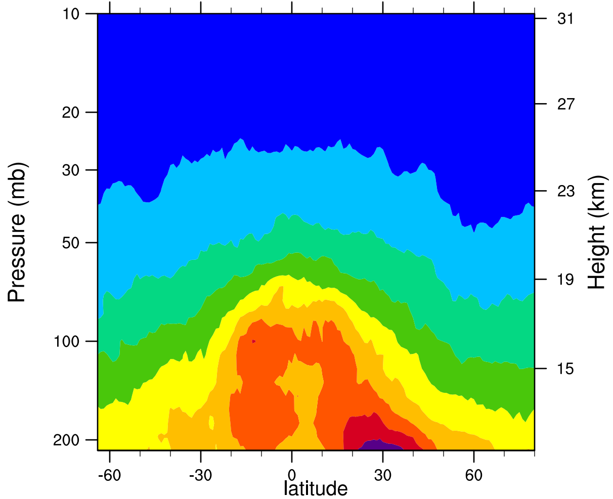
2006d124 12.1MicronExtinction_Combined (km -1 )
