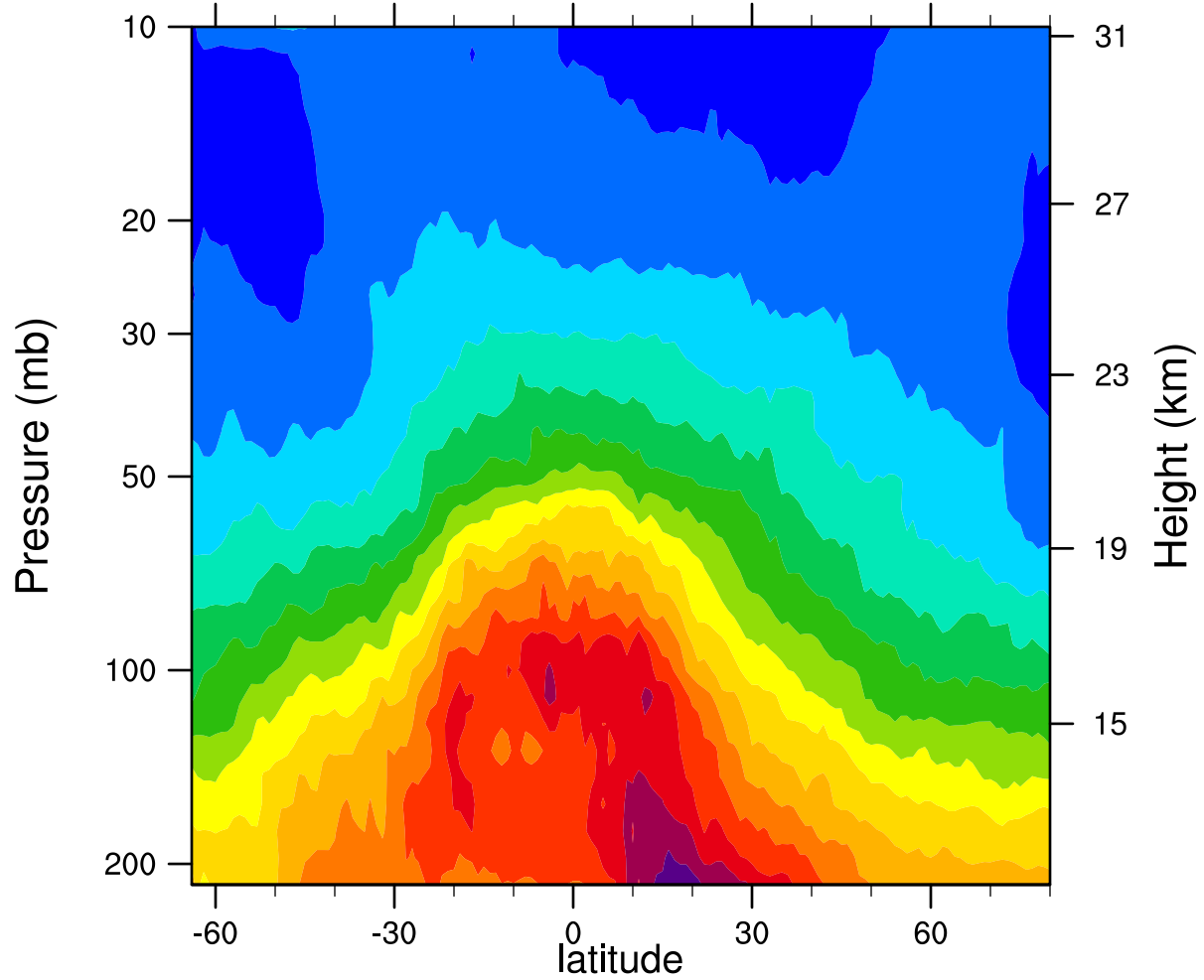
2006d064 12.1MicronExtinction_Combined (km -1 )
