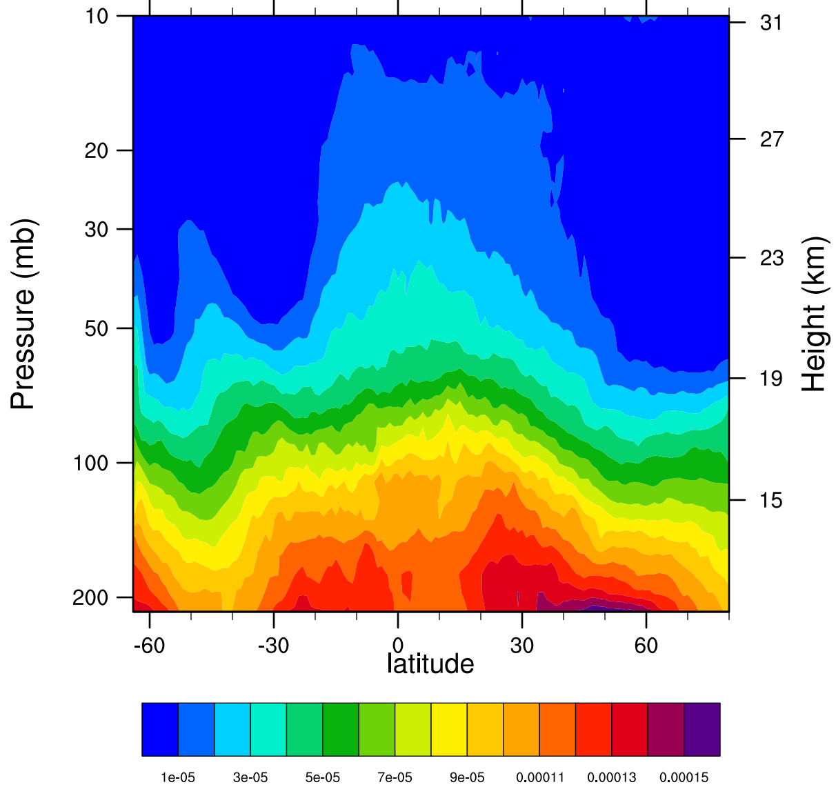
2007d238 12.1MicronExtinction_Combined (km -1 )
