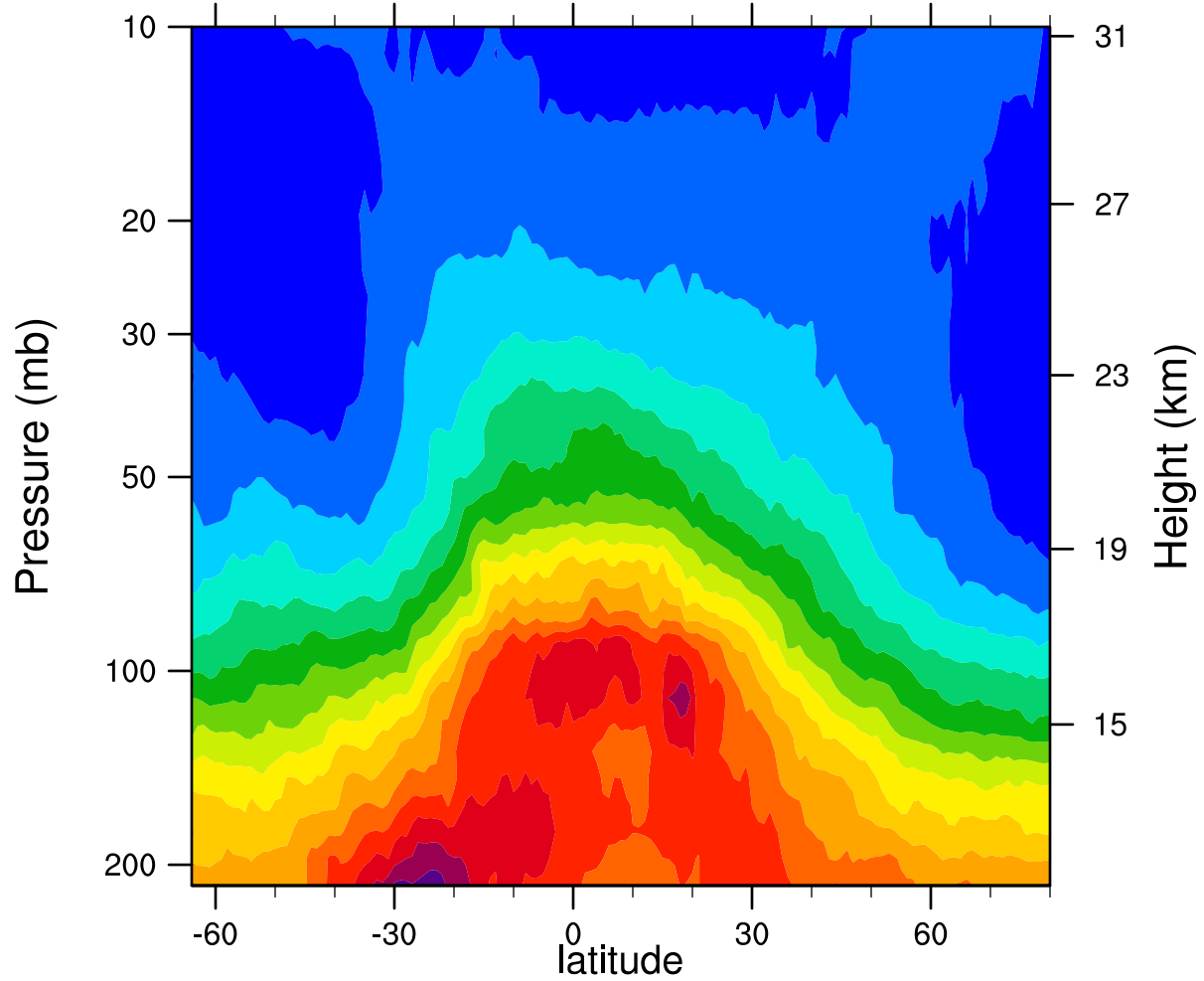
2005d295 12.1MicronExtinction_Combined (km -1 )
