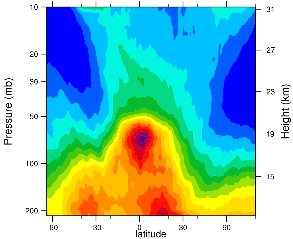
2005d062 12.1MicronExtinction_Combined (km -1 )
