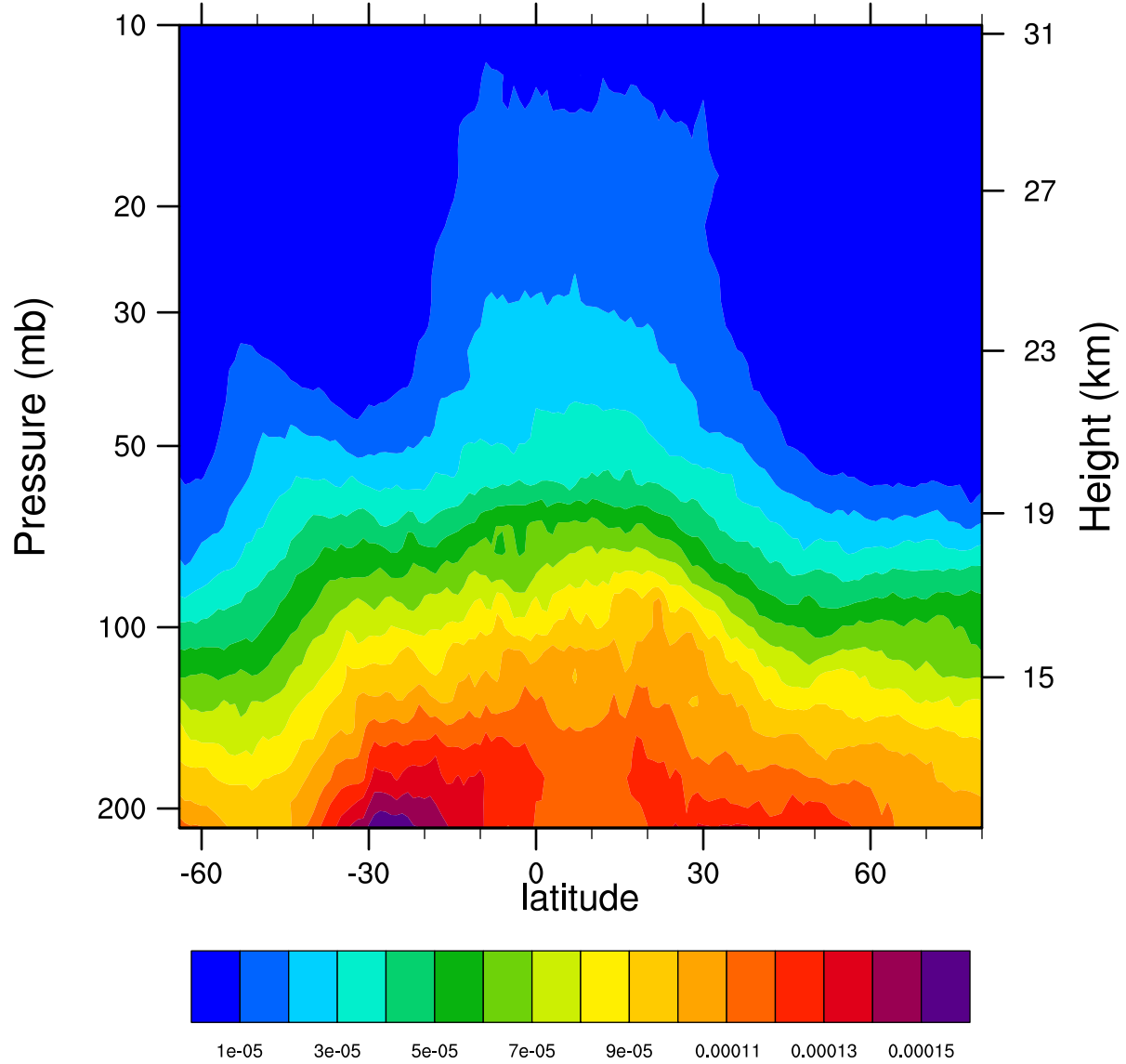
2007d289 12.1MicronExtinction_Combined (km -1 )
