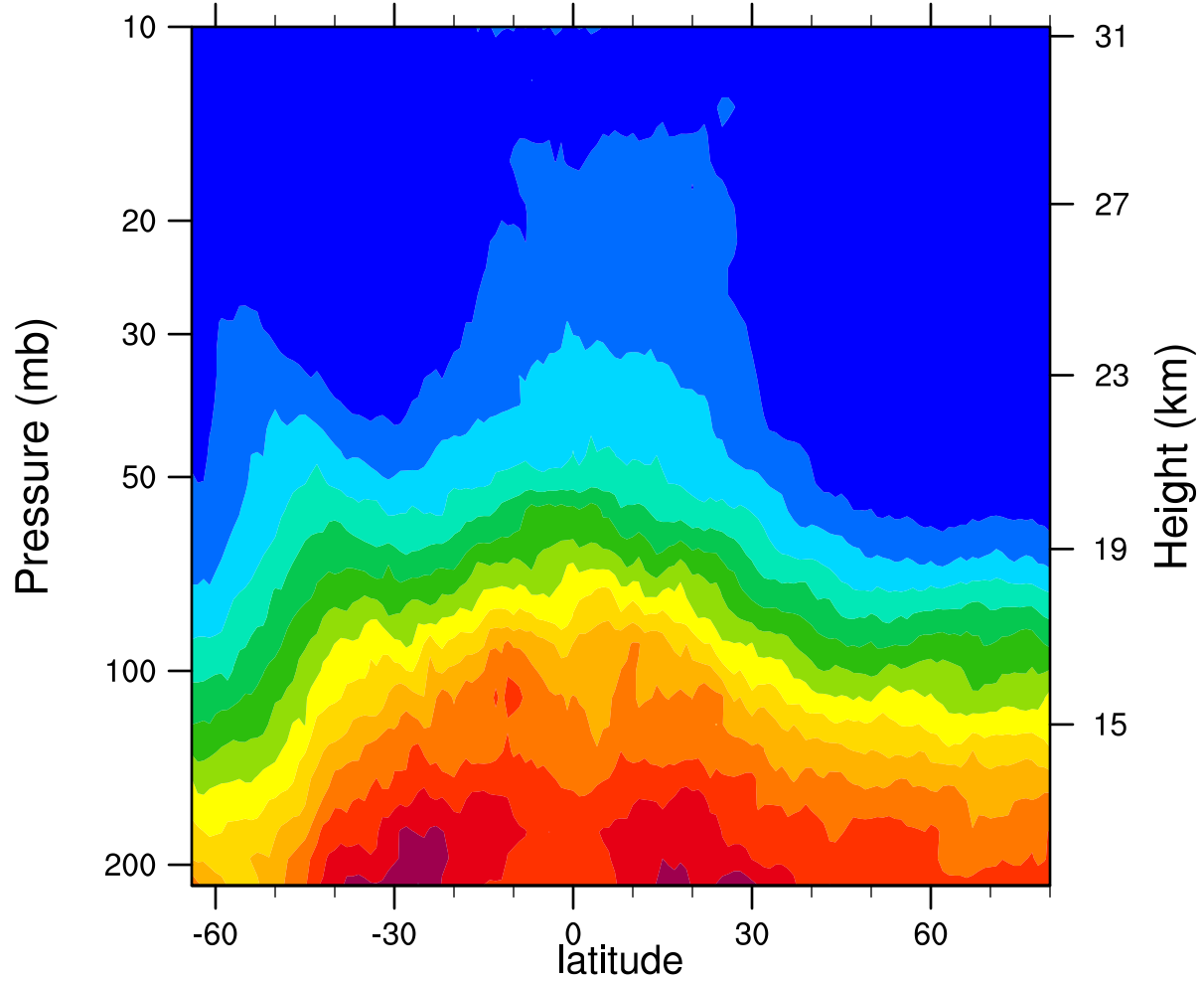
2007d329 12.1MicronExtinction_Combined (km -1 )
