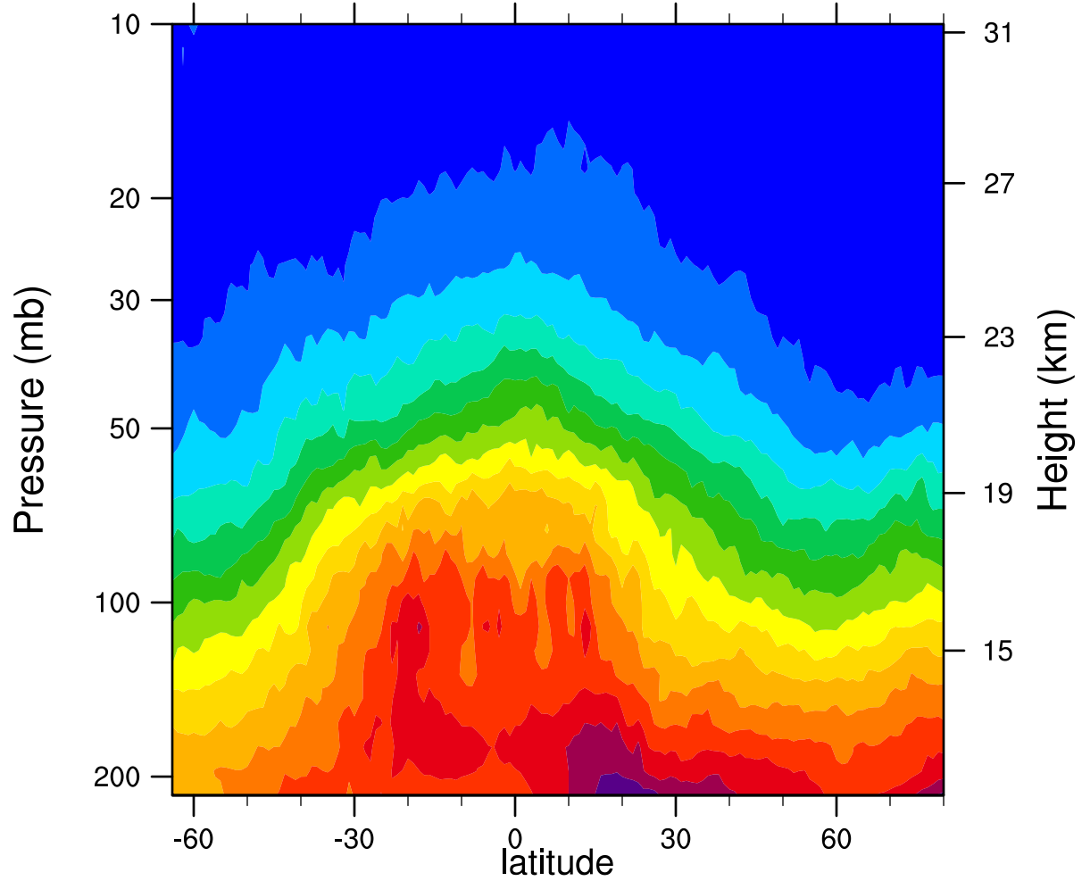
2007d075 12.1MicronExtinction_Combined (km -1 )
