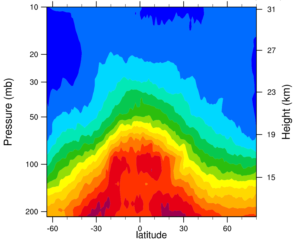
2005d340 12.1MicronExtinction_Combined ( \text{km}^{-1} )
