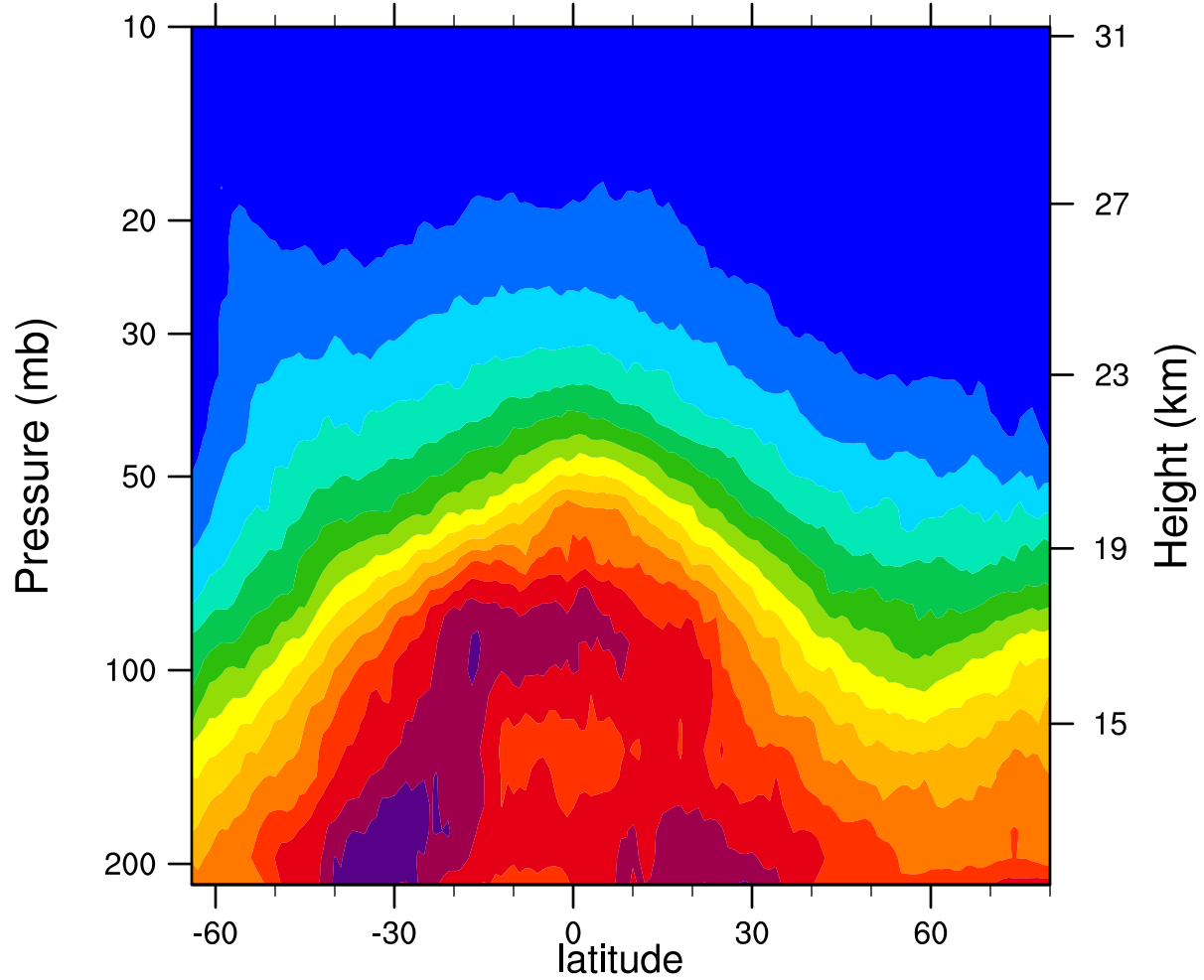
2007d001 12.1MicronExtinction_Combined ( \text{km}^{-1} )
