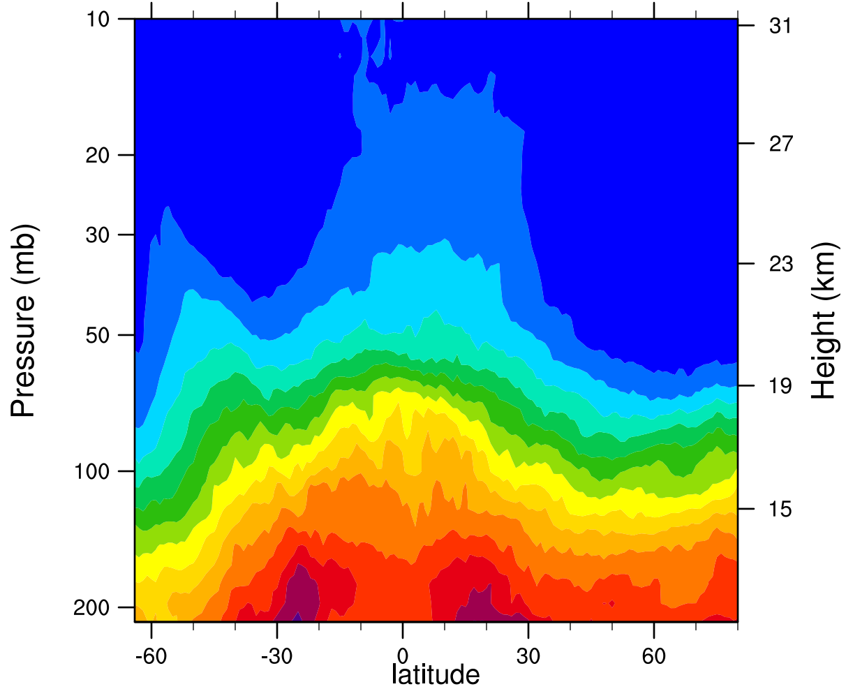
2007d340 12.1MicronExtinction_Combined (km -1 )
