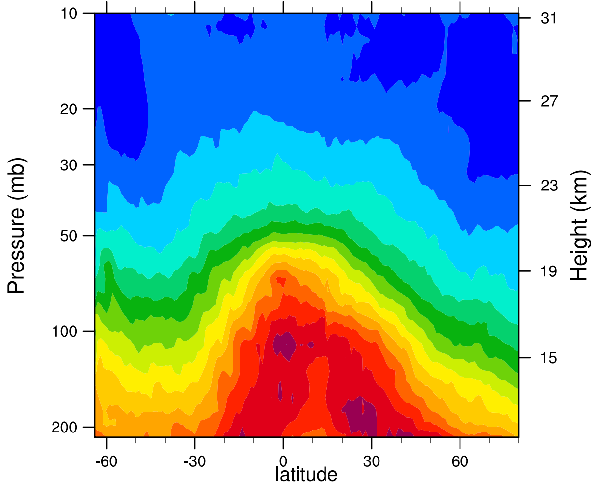
2006d242 12.1MicronExtinction_Combined (km -1 )
