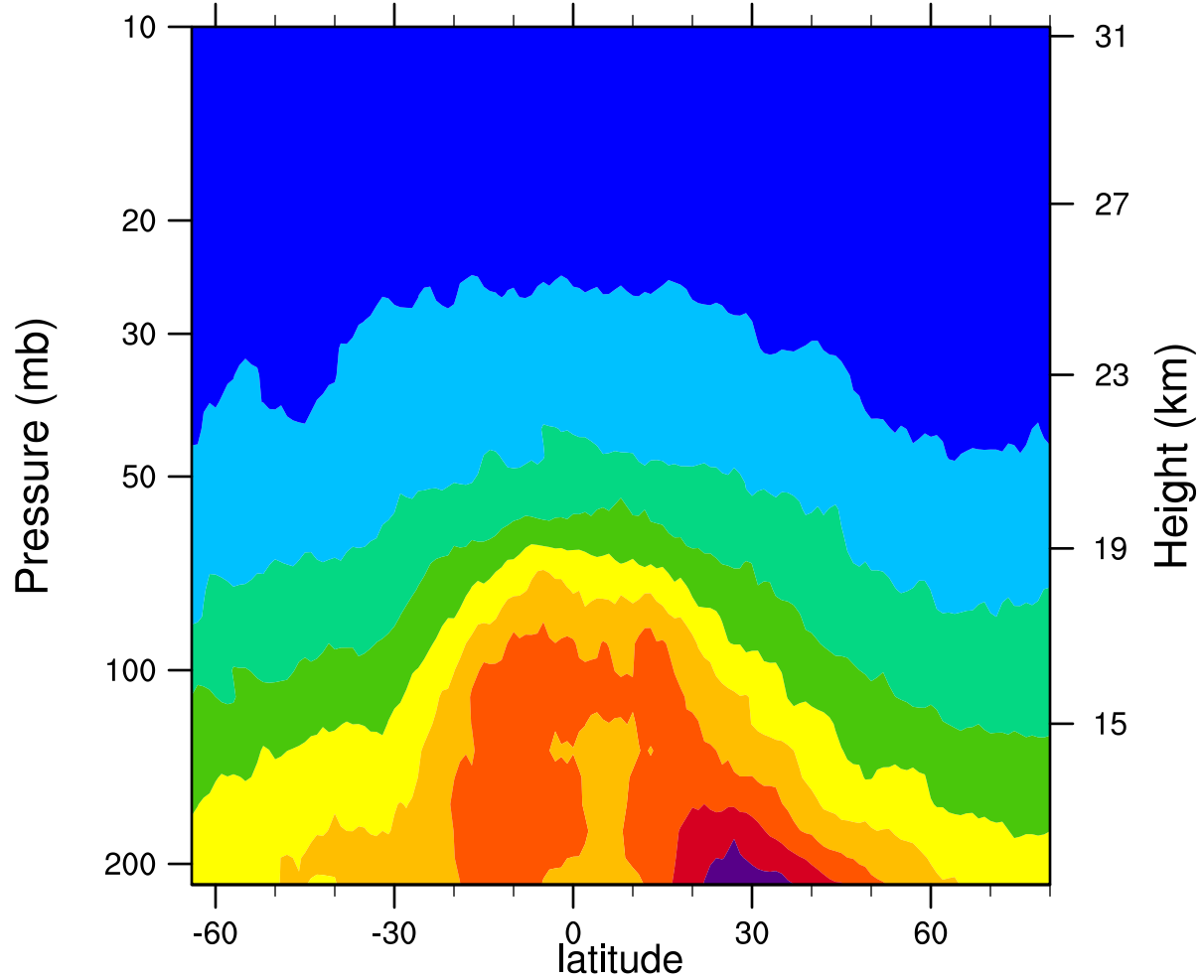
2006d132 12.1MicronExtinction_Combined (km -1 )
