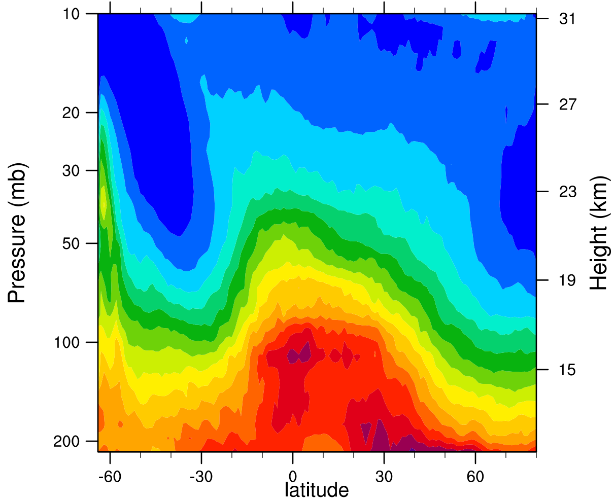
2005d211 12.1MicronExtinction_Combined (km -1 )
