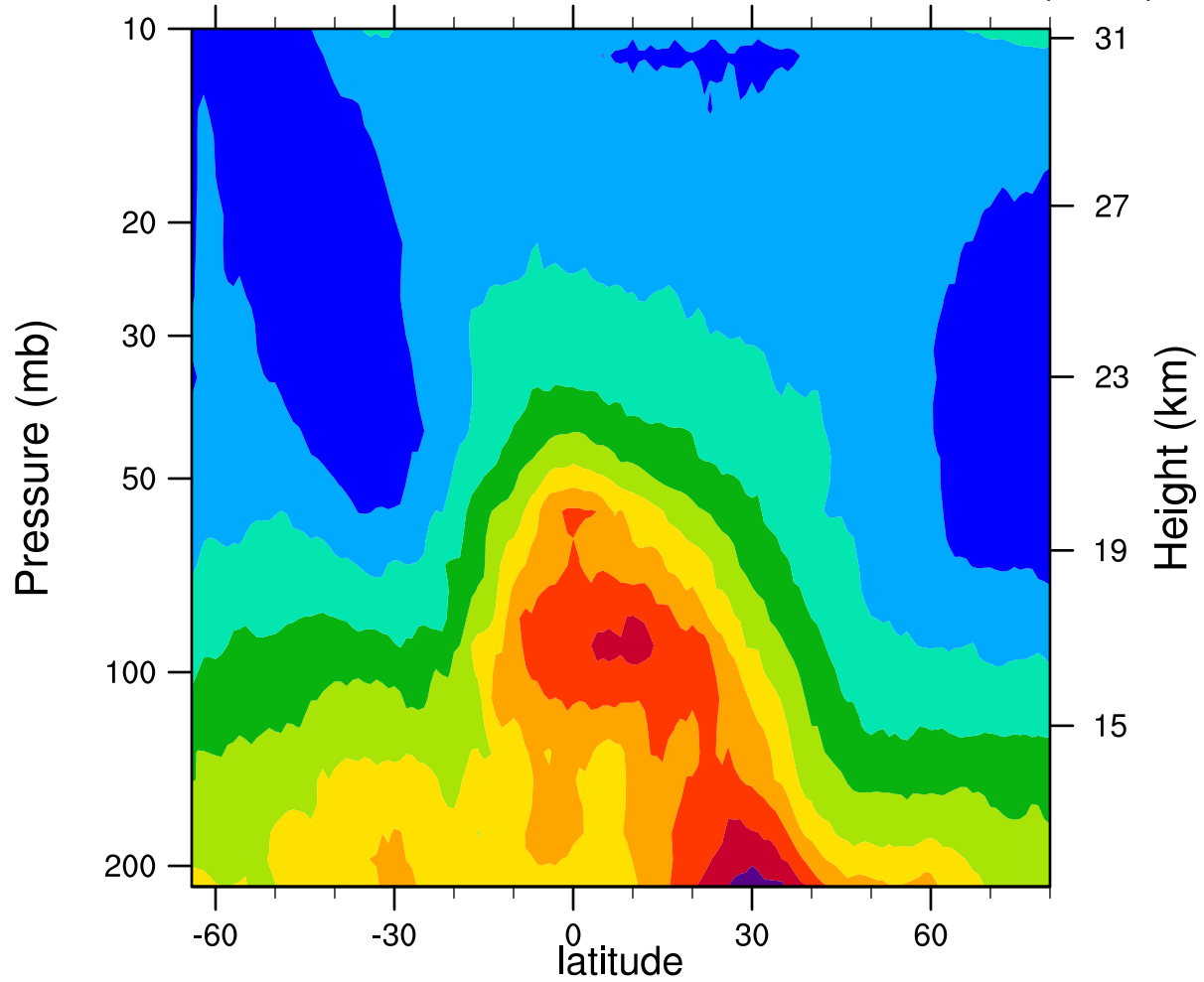
2005d134 12.1MicronExtinction_Combined (km -1 )
