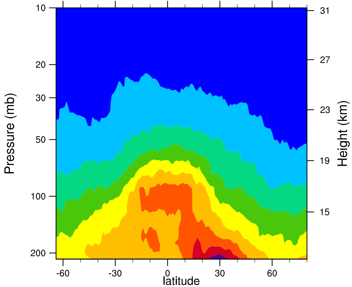
2006d103 12.1MicronExtinction_Combined (km -1 )
