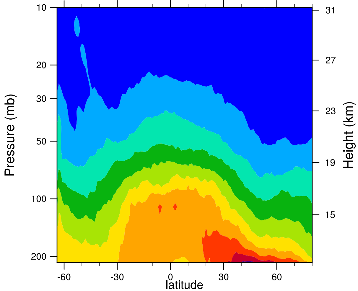
2007d180 12.1MicronExtinction_Combined (km -1 )
