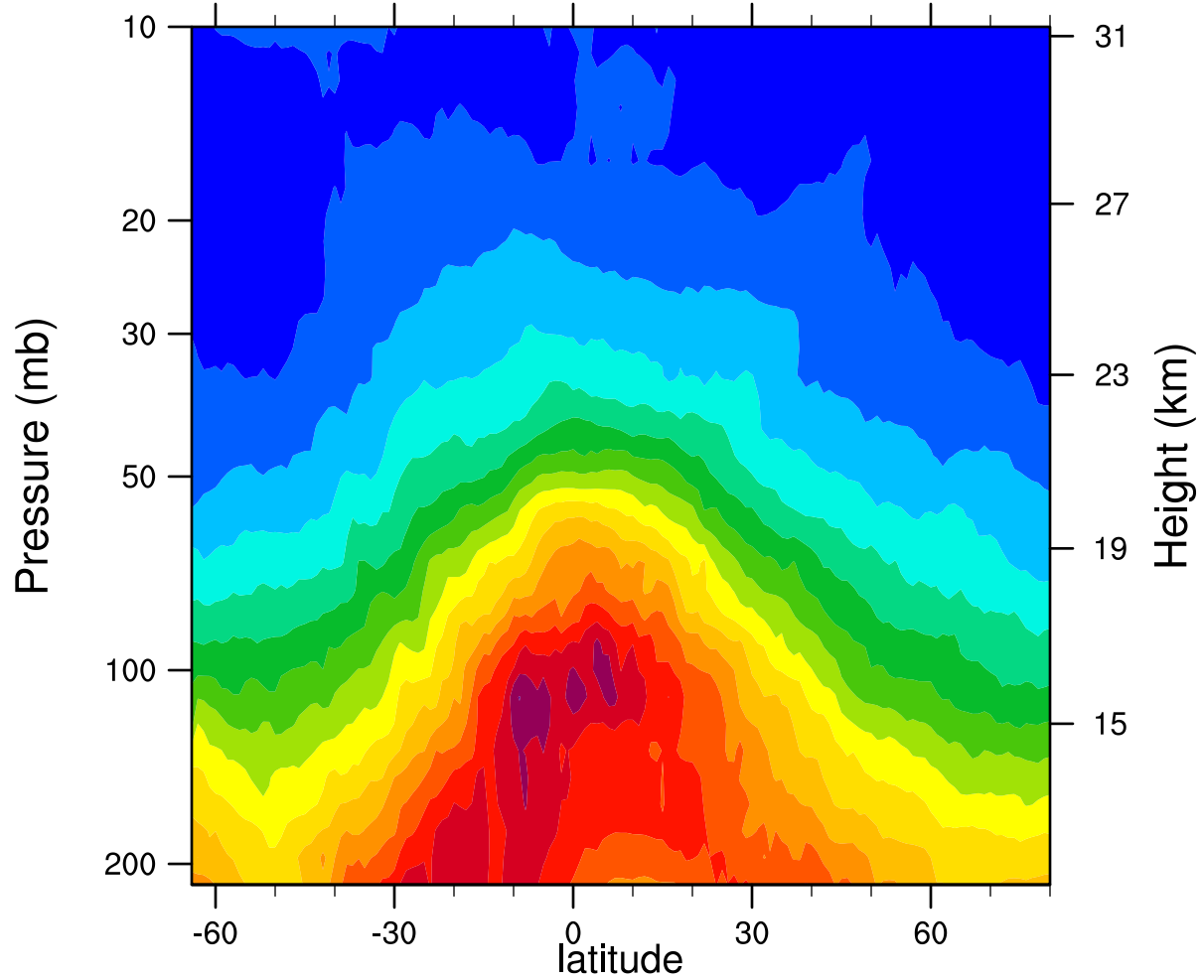
2006d290 12.1MicronExtinction_Combined (km -1 )
