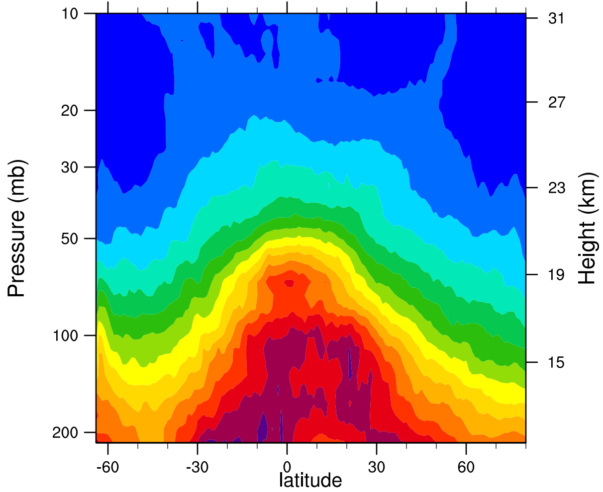
2006d274 12.1MicronExtinction_Combined (km -1 )
