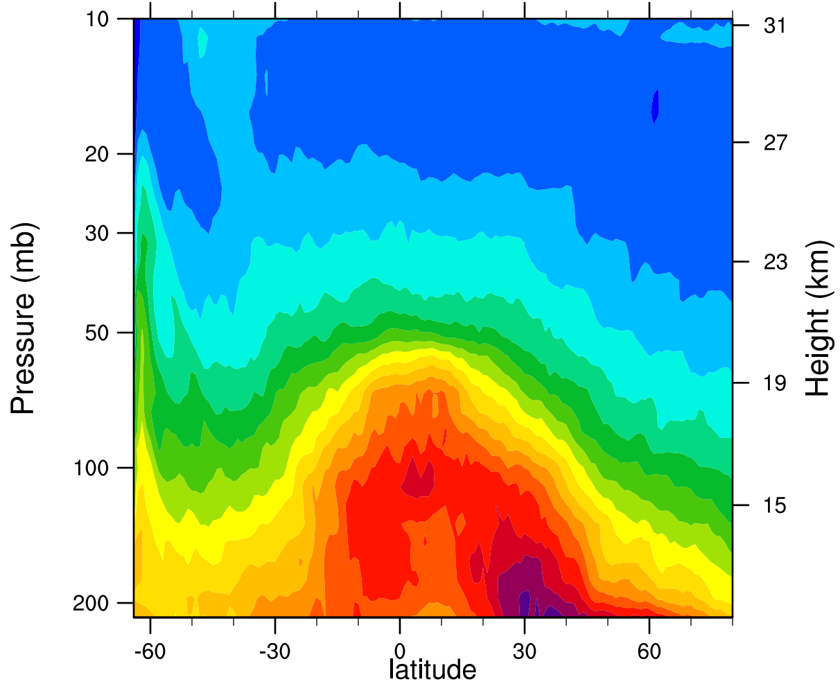
2006d202 12.1MicronExtinction_Combined (km -1 )
