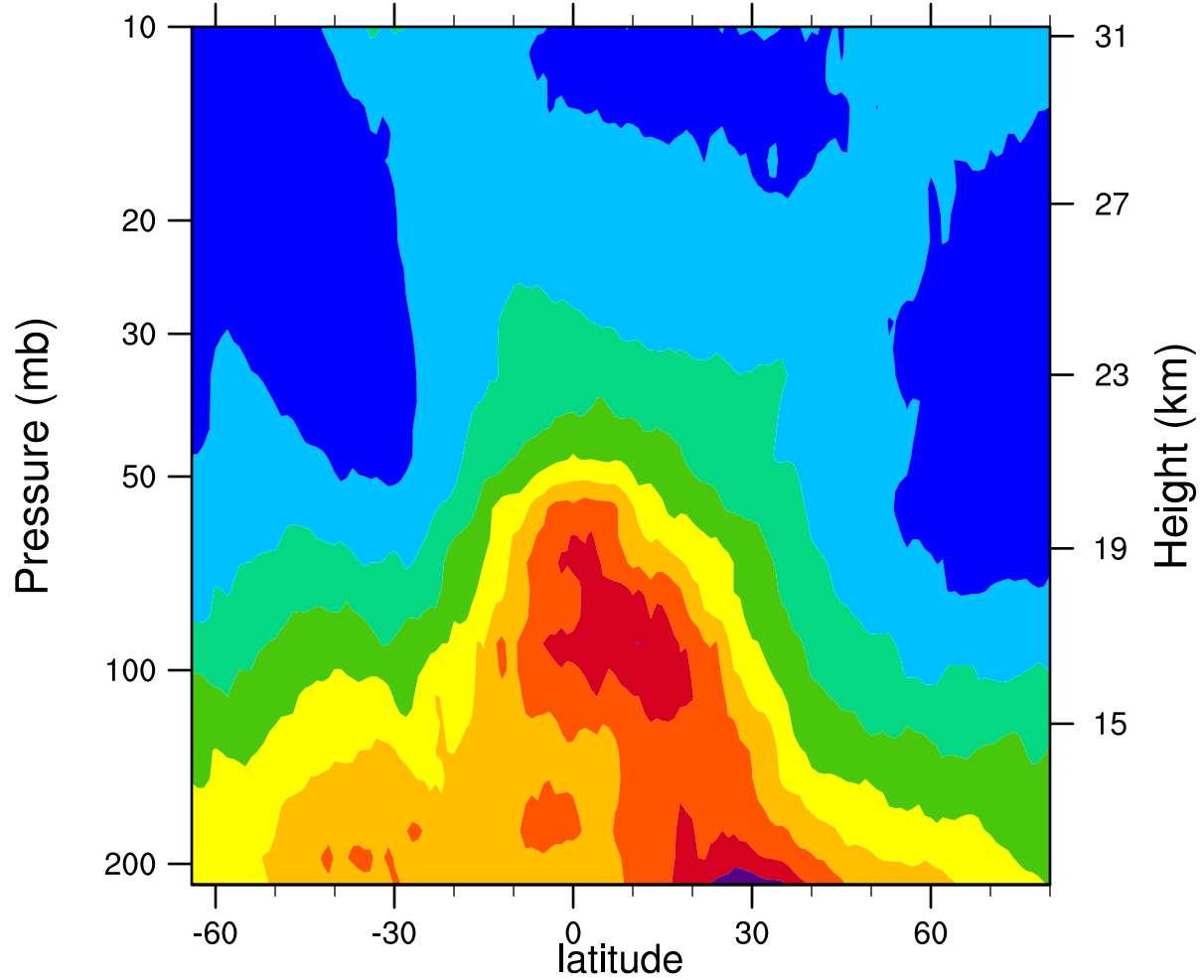
2005d112 12.1MicronExtinction_Combined (km -1 )
