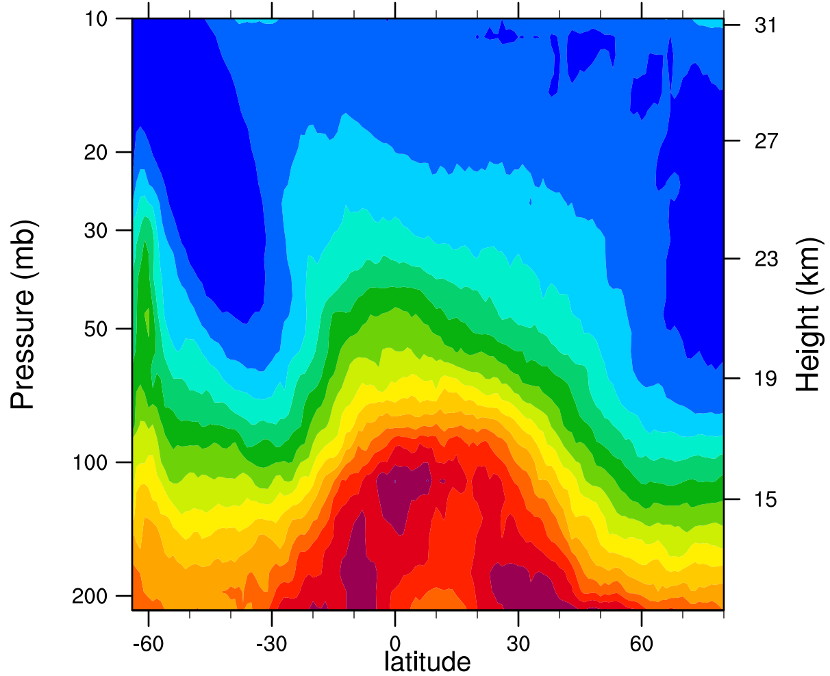
2005d232 12.1MicronExtinction_Combined (km -1 )
