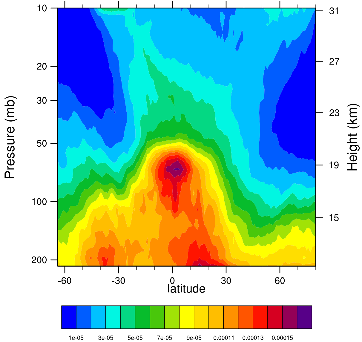
2005d067 12.1MicronExtinction_Combined (km -1 )
