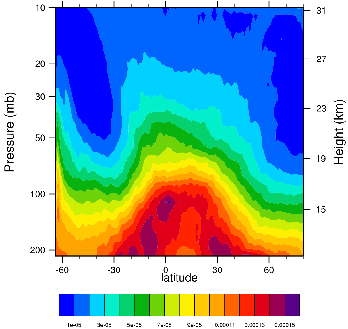
2005d238 12.1MicronExtinction_Combined (km -1 )
