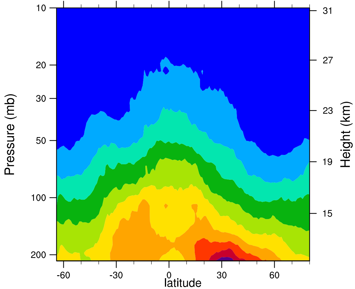
2007d124 12.1MicronExtinction_Combined (km -1 )
