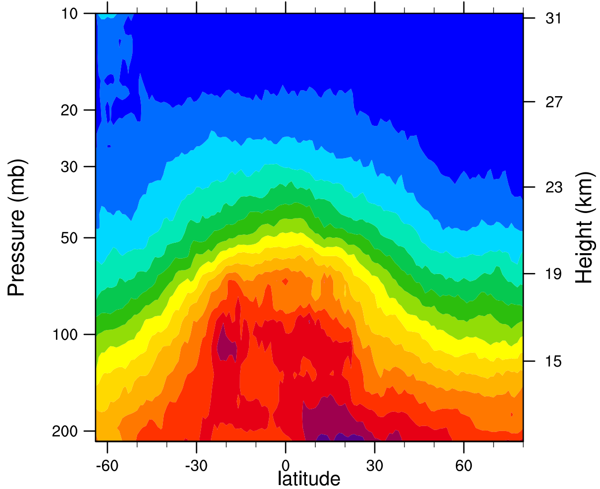
2007d060 12.1MicronExtinction_Combined (km -1 )
