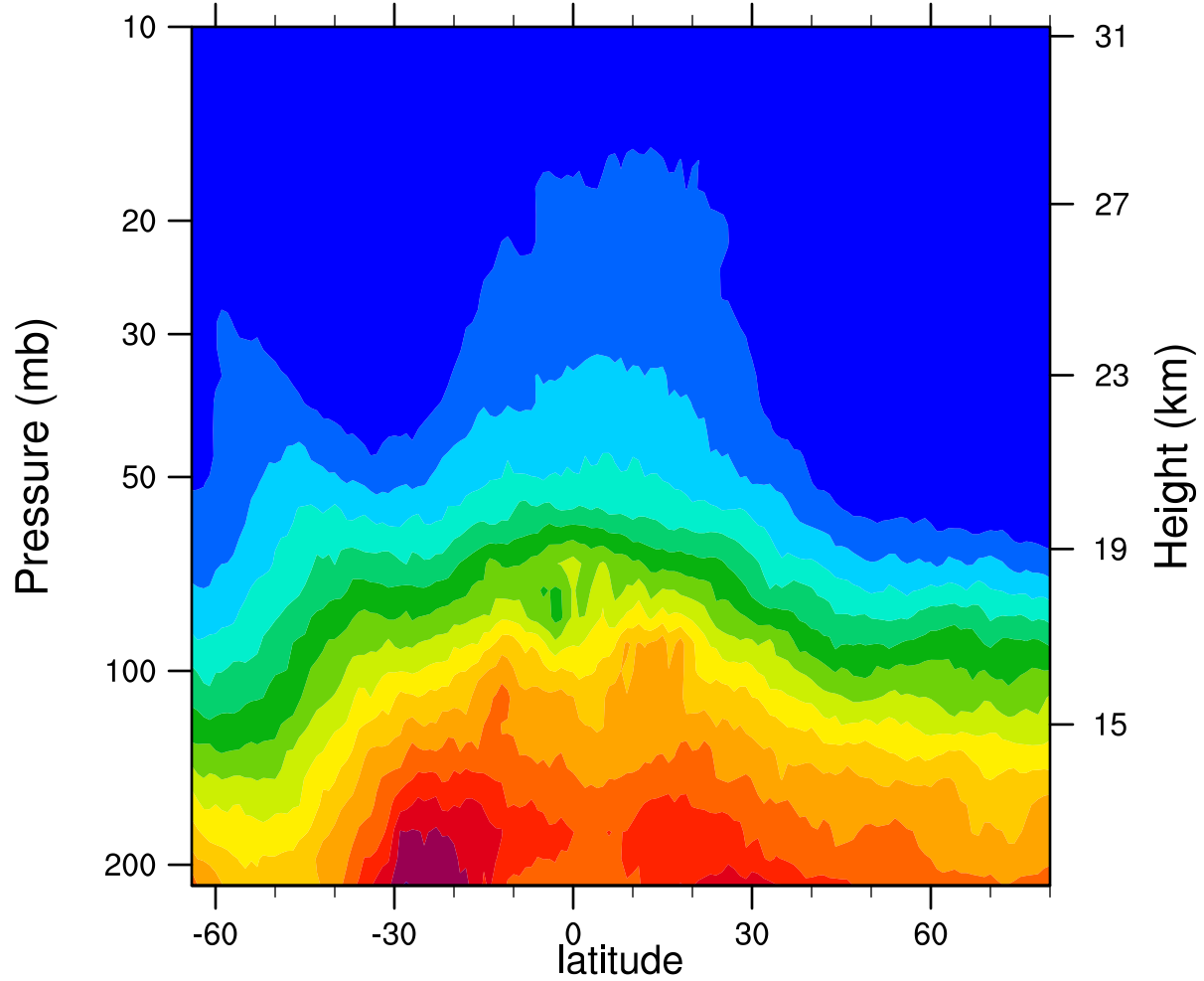
2007d316 12.1MicronExtinction_Combined (km -1 )
