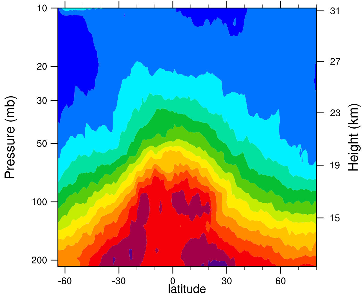
2005d347 12.1MicronExtinction_Combined ( \text{km}^{-1} )
