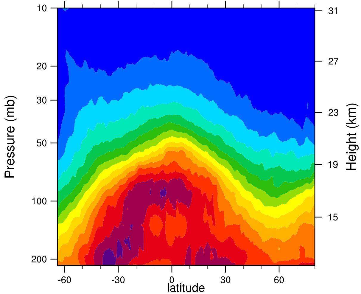
2007d004 12.1MicronExtinction_Combined ( \text{km}^{-1} )
