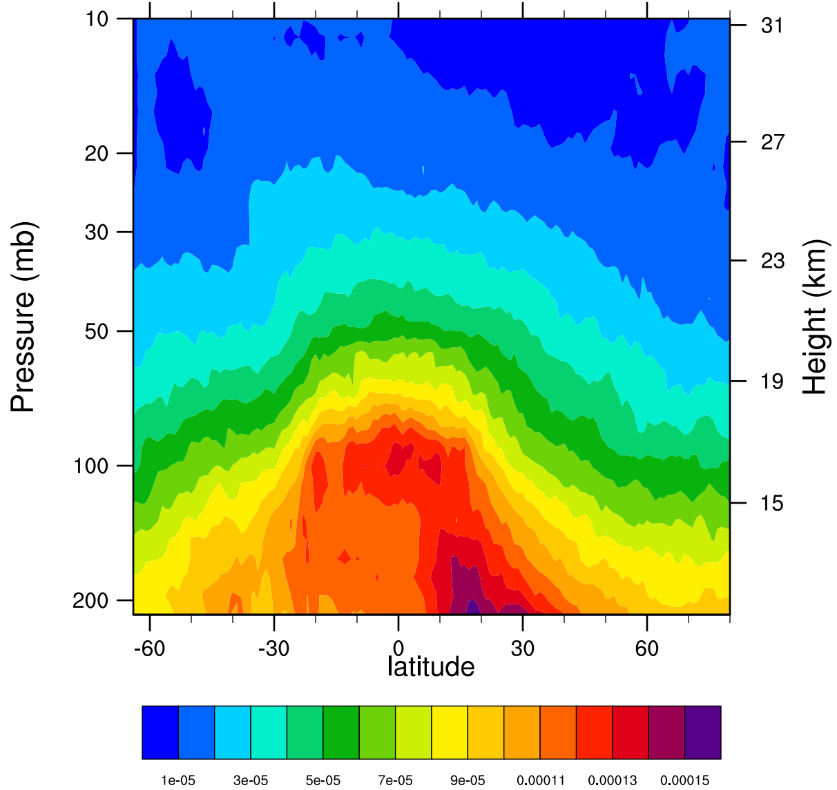
2006d087 12.1MicronExtinction_Combined ( \text{km}^{-1} )
