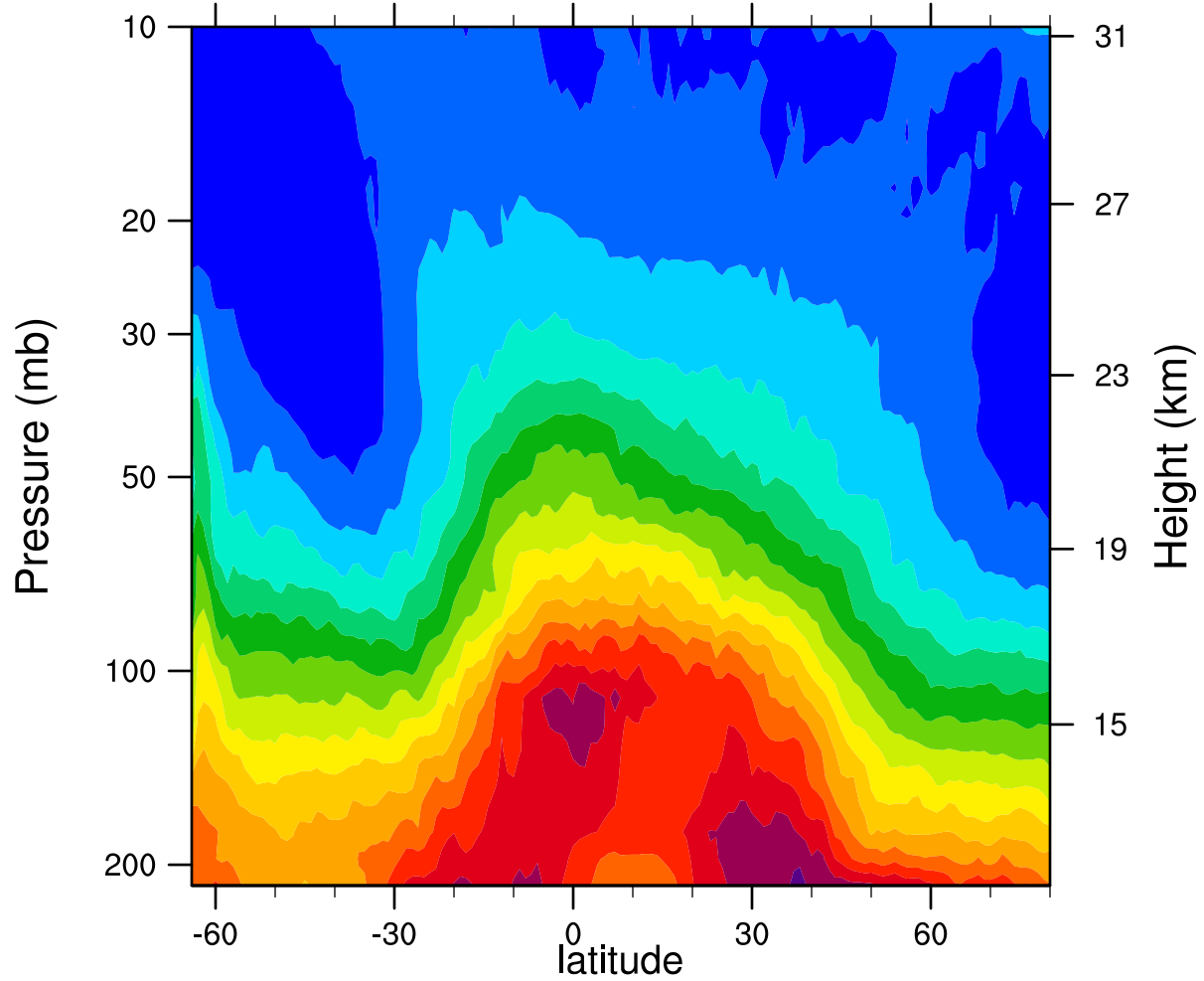
2005d226 12.1MicronExtinction_Combined (km -1 )
