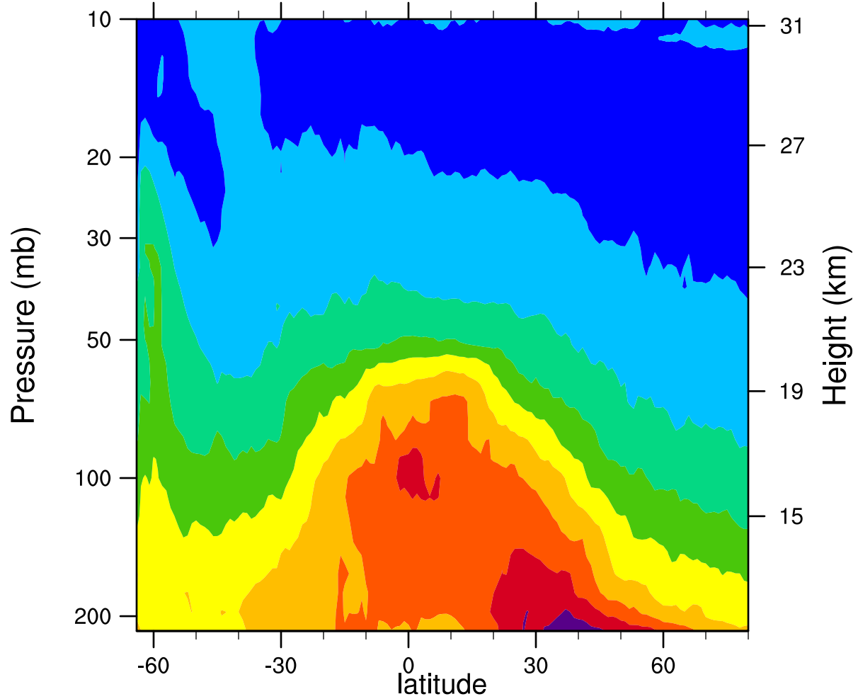
2006d191 12.1MicronExtinction_Combined (km -1 )
