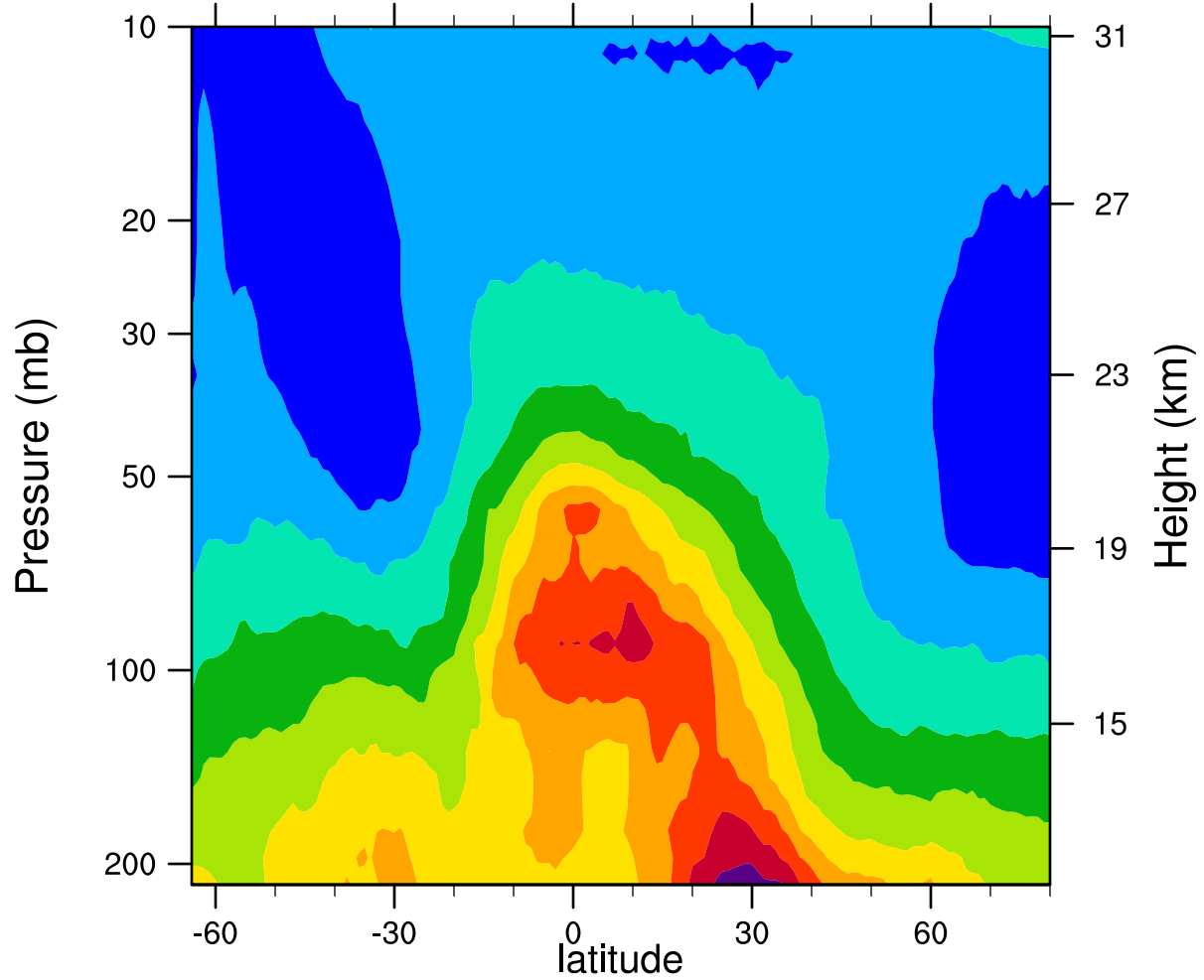
2005d132 12.1MicronExtinction_Combined (km -1 )
