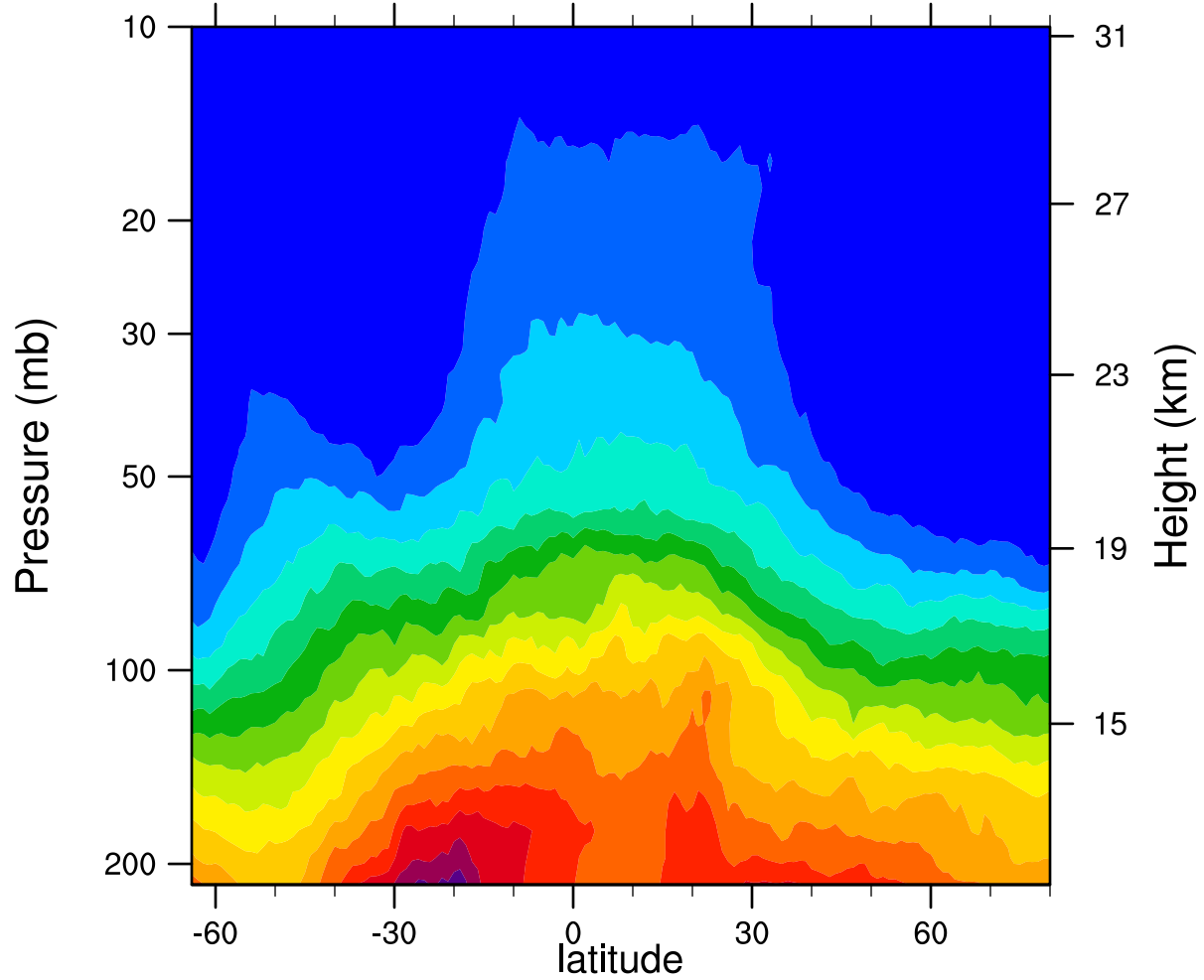
2007d296 12.1MicronExtinction_Combined (km -1 )
