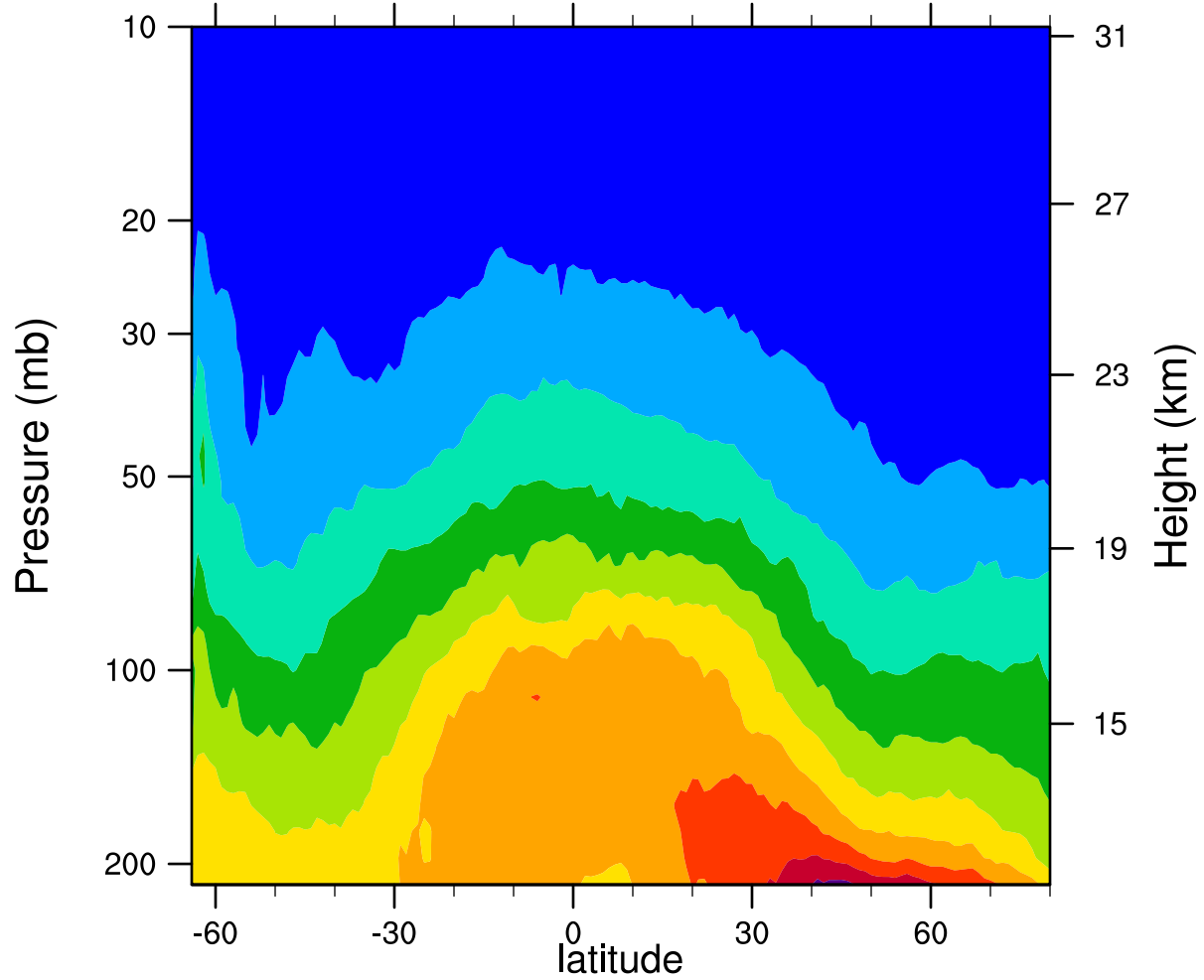
2007d183 12.1MicronExtinction_Combined ( \text{km}^{-1} )
