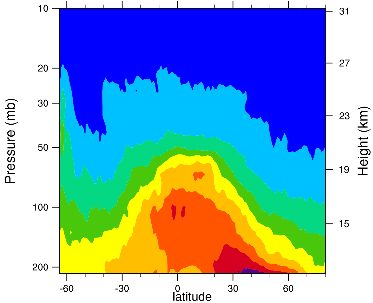
2006d186 12.1MicronExtinction_Combined (km -1 )
