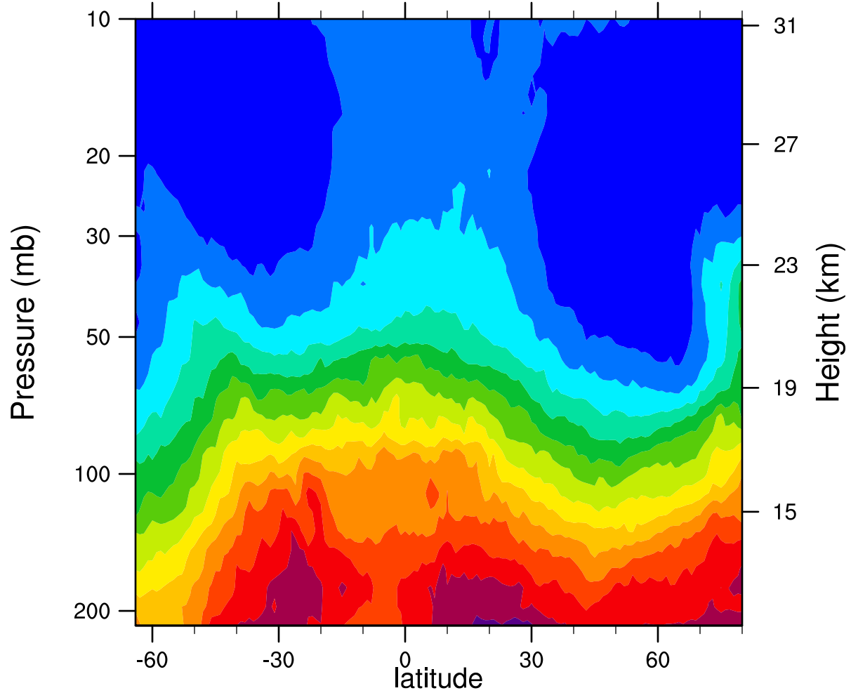
2007d363 12.1MicronExtinction_Combined (km -1 )
