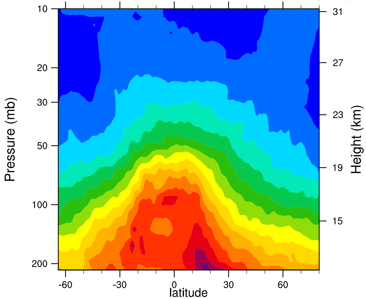
2006d053 12.1MicronExtinction_Combined (km -1 )
