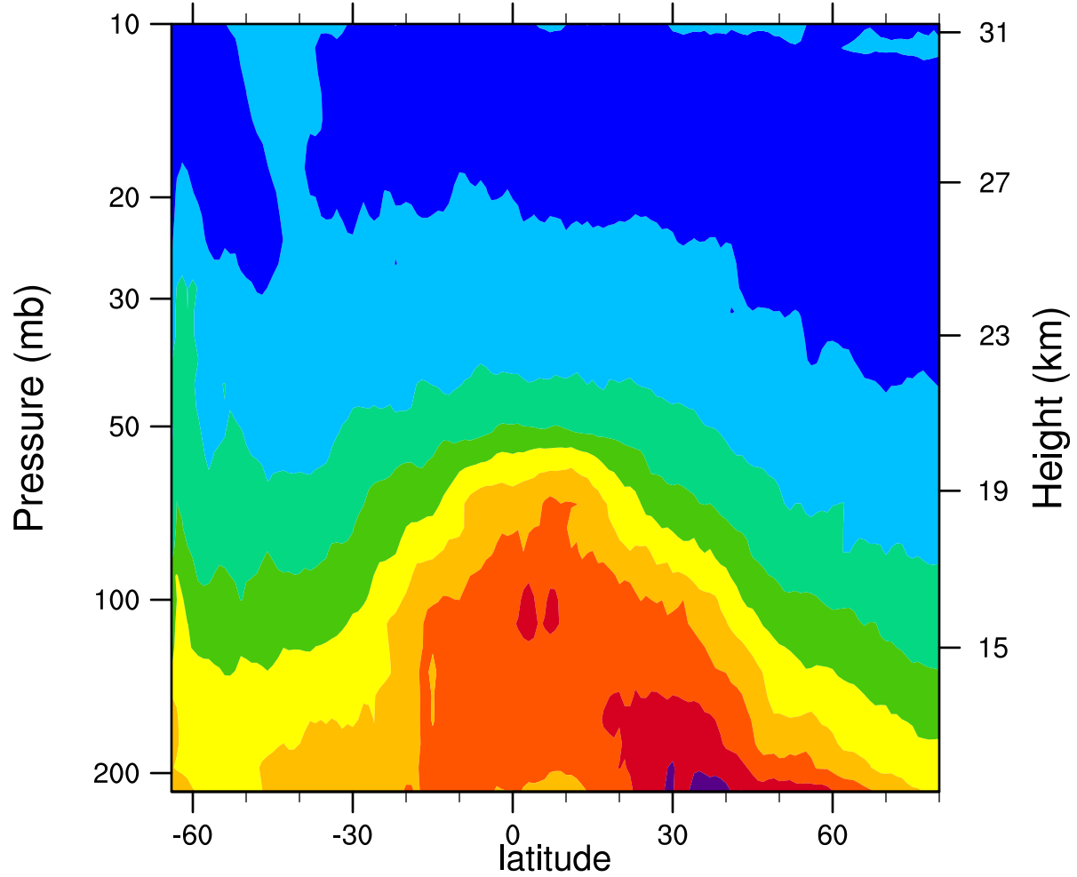
2006d198 12.1MicronExtinction_Combined (km -1 )
