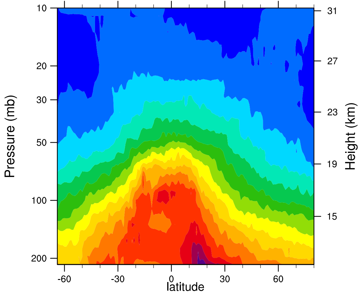
2006d051 12.1MicronExtinction_Combined (km -1 )
