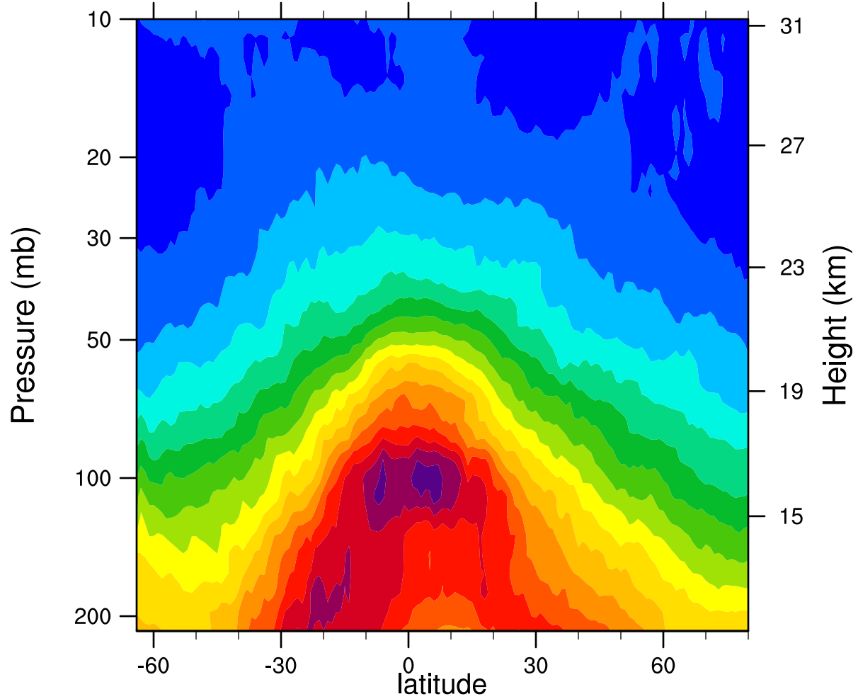
2006d298 12.1MicronExtinction_Combined (km -1 )
