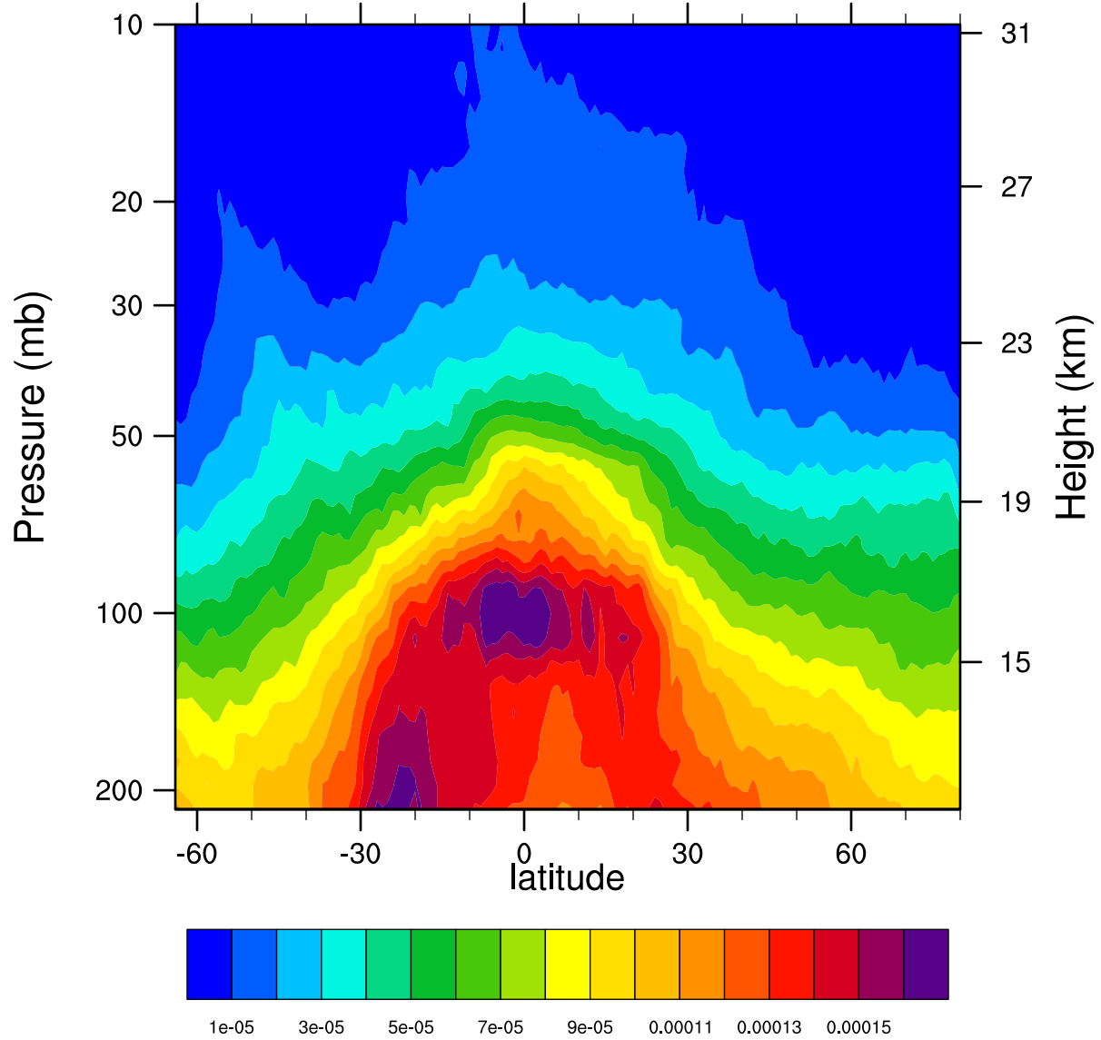
2006d310 12.1MicronExtinction_Combined (km -1 )
