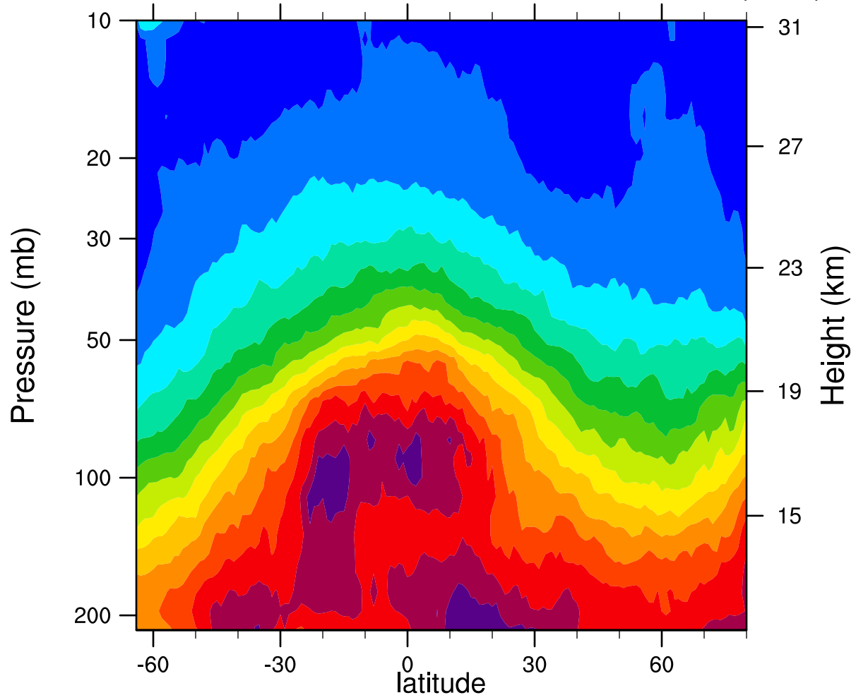
2007d035 12.1MicronExtinction_Combined ( \text{km}^{-1} )
