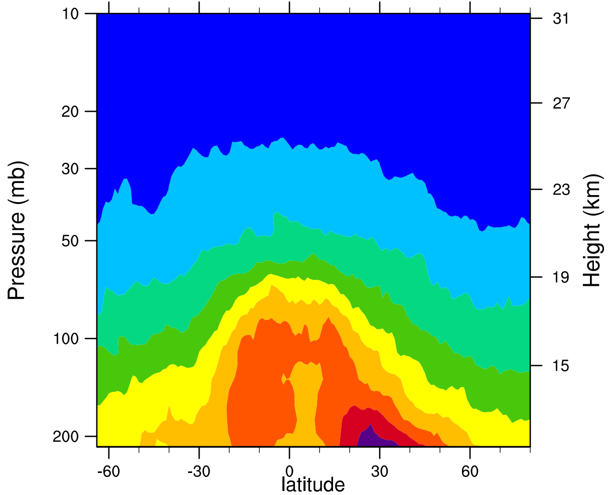
2006d133 12.1MicronExtinction_Combined (km -1 )
