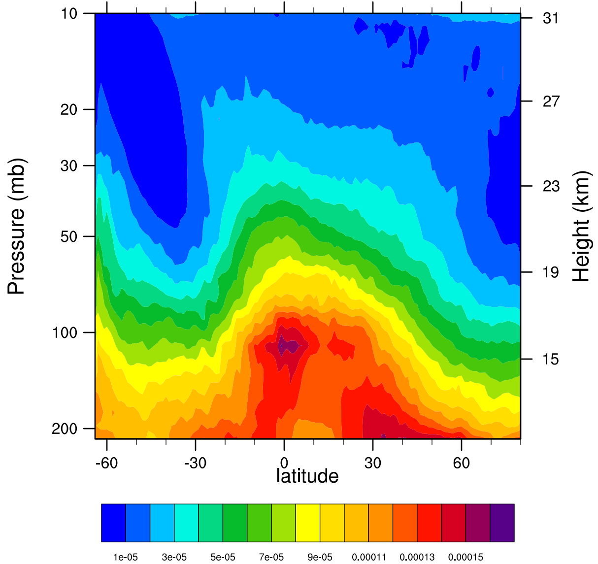
2005d217 12.1MicronExtinction_Combined (km -1 )
