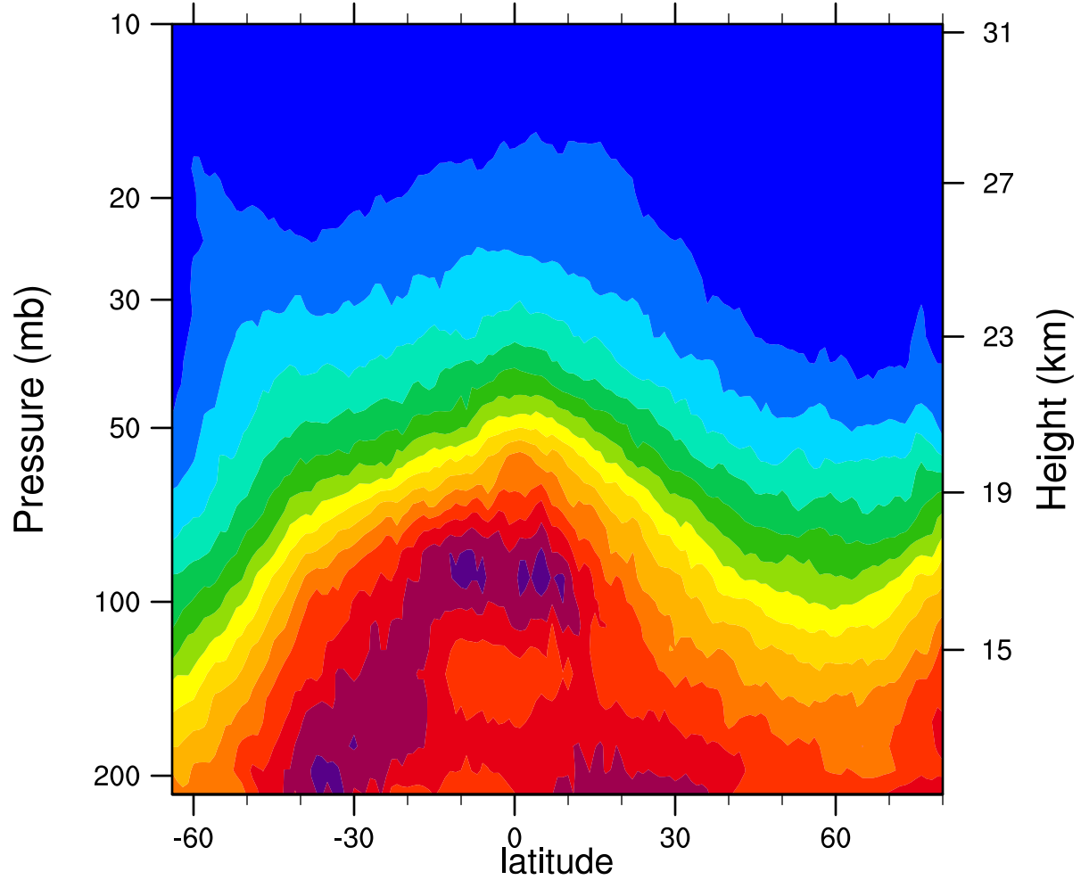
2007d010 12.1MicronExtinction_Combined (km -1 )
