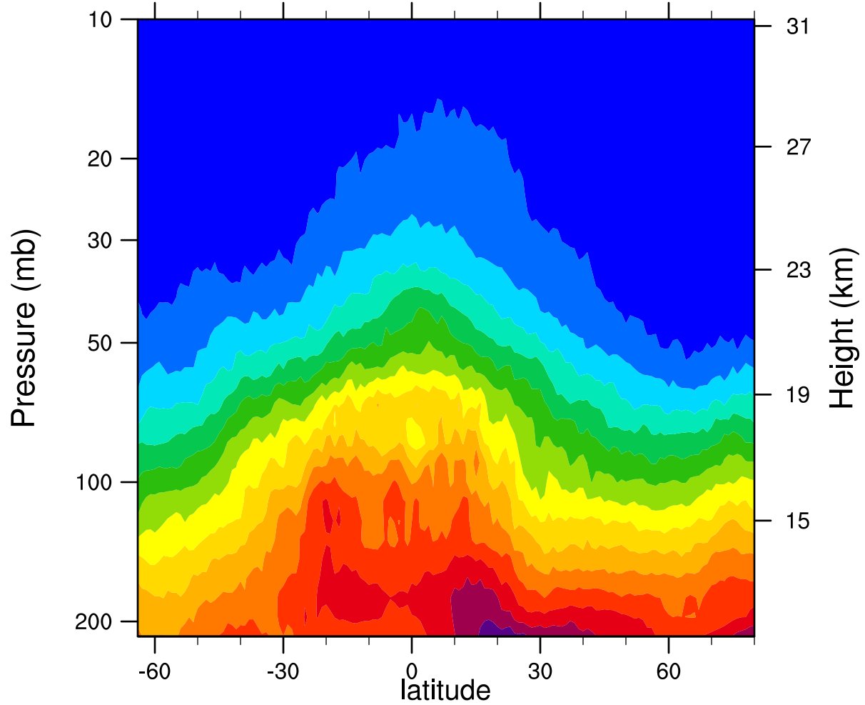
2007d077 12.1MicronExtinction_Combined ( \text{km}^{-1} )
