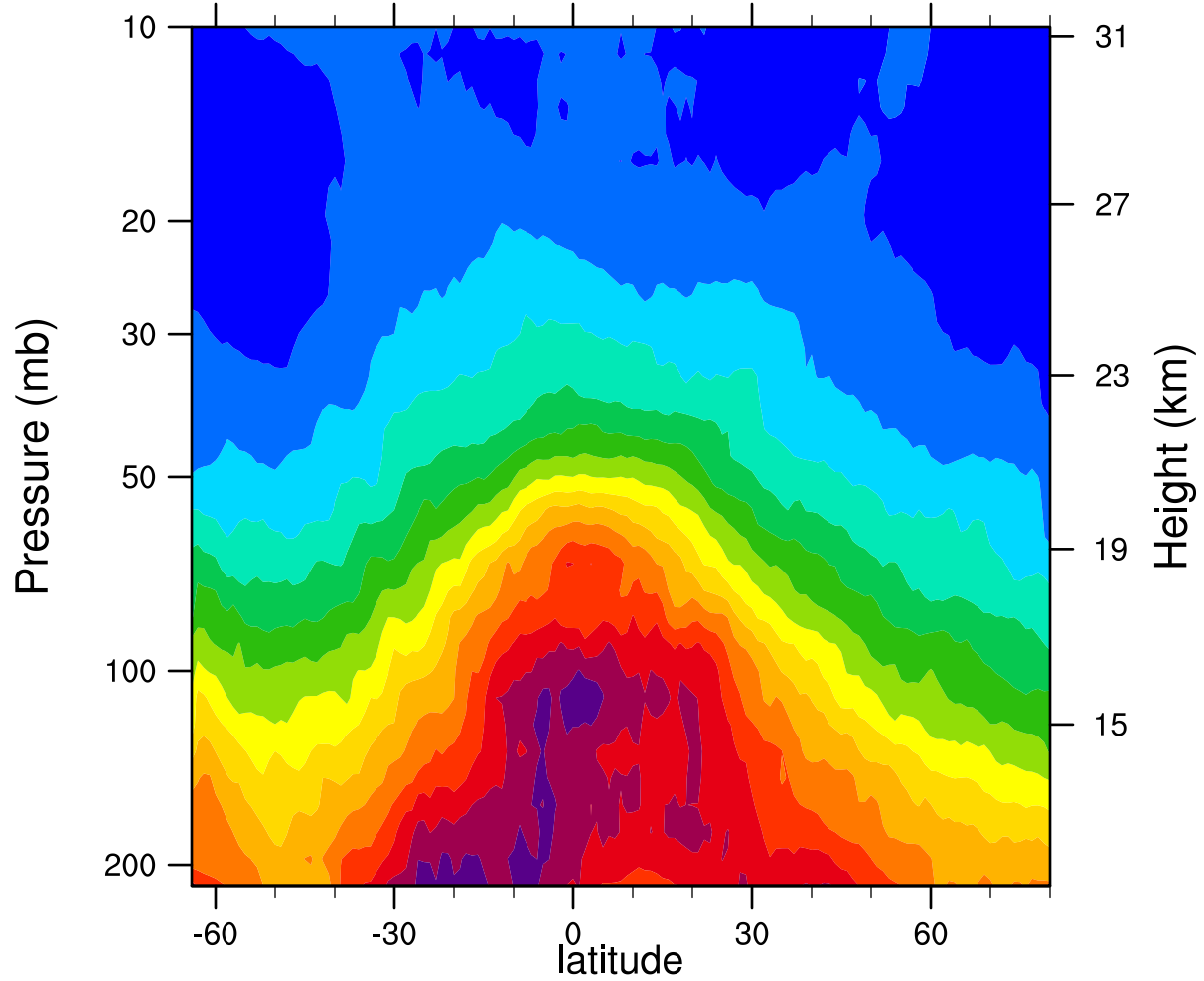
2006d282 12.1MicronExtinction_Combined ( \text{km}^{-1} )
