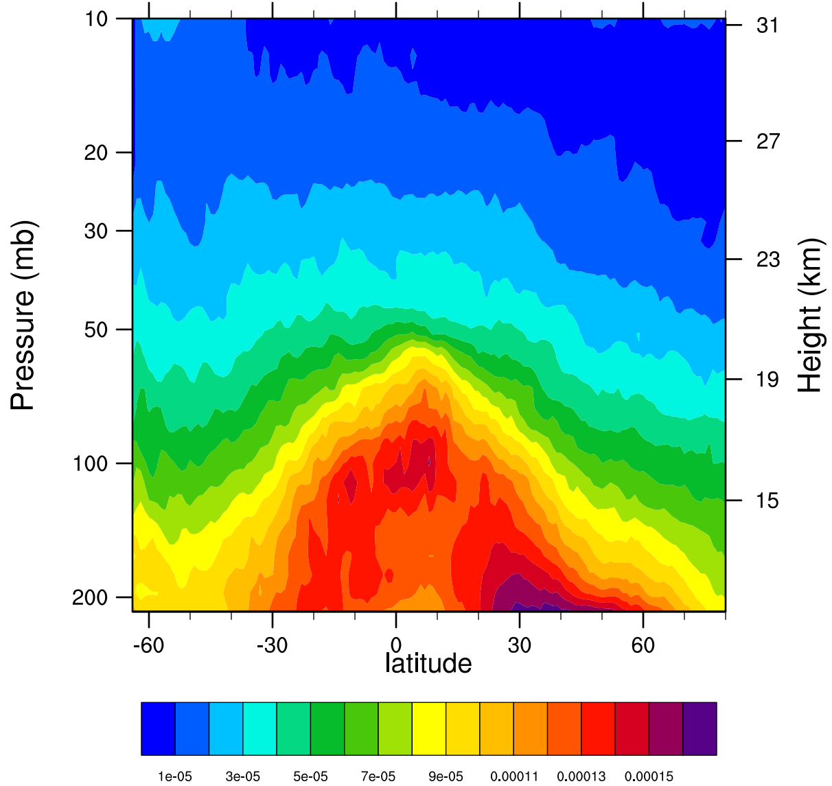
2006d165 12.1MicronExtinction_Combined ( \text{km}^{-1} )
