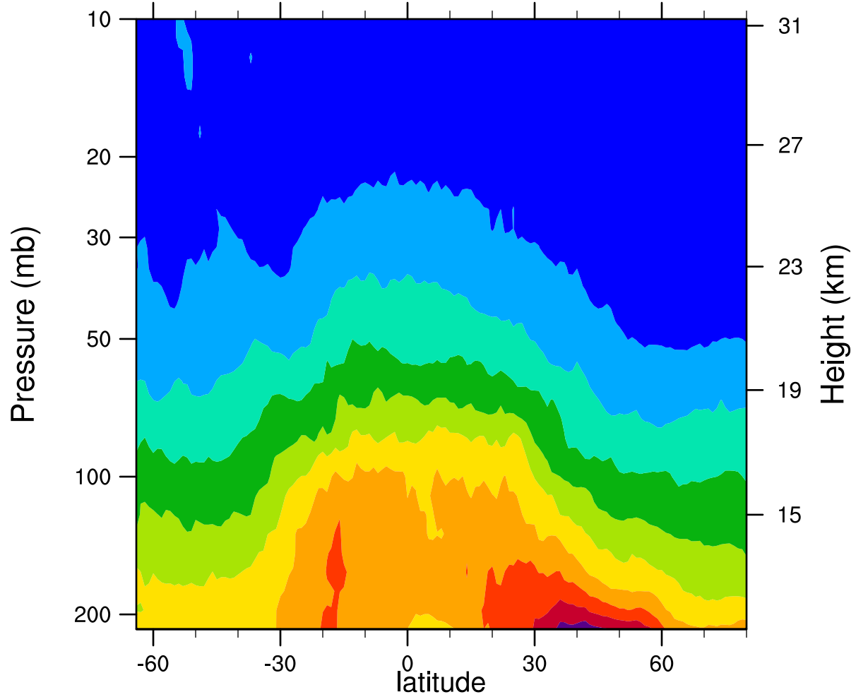
2007d164 12.1MicronExtinction_Combined (km -1 )
