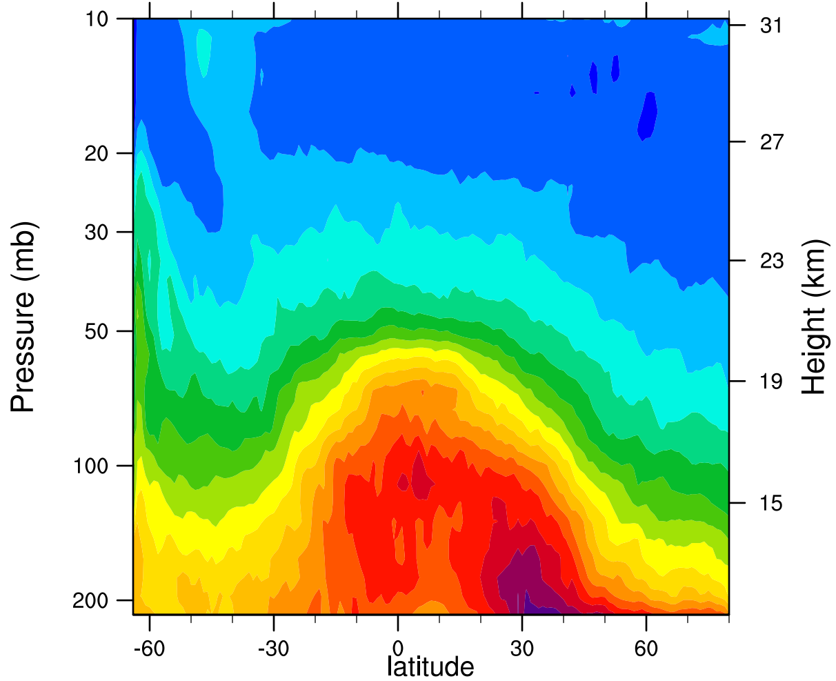
2006d207 12.1MicronExtinction_Combined (km -1 )
