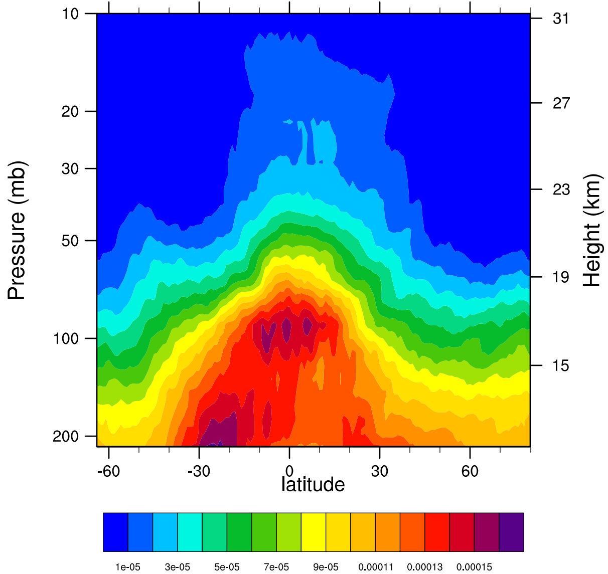
2006d319 12.1MicronExtinction_Combined (km -1 )
