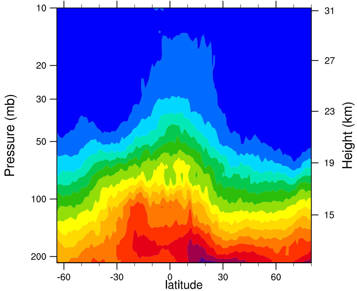
2007d080 12.1MicronExtinction_Combined (km -1 )
