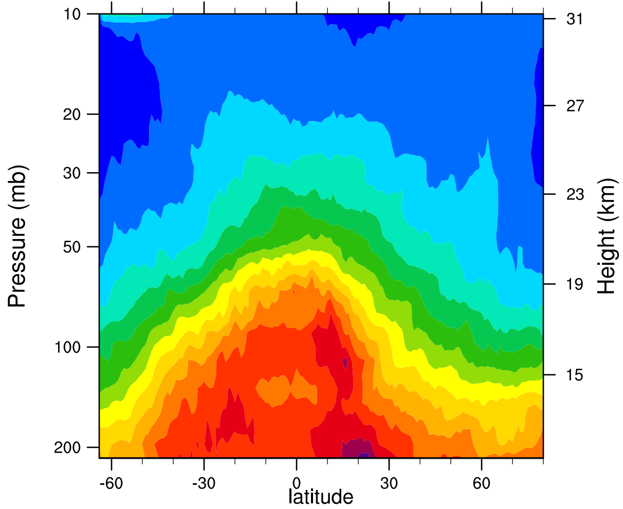
2006d012 12.1MicronExtinction_Combined (km -1 )
