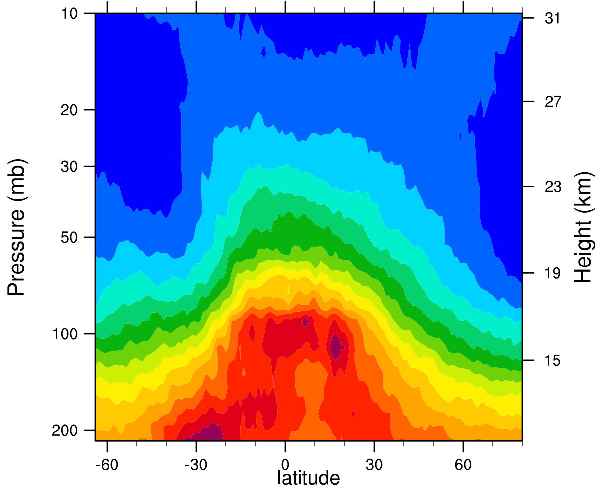
2005d298 12.1MicronExtinction_Combined (km -1 )
