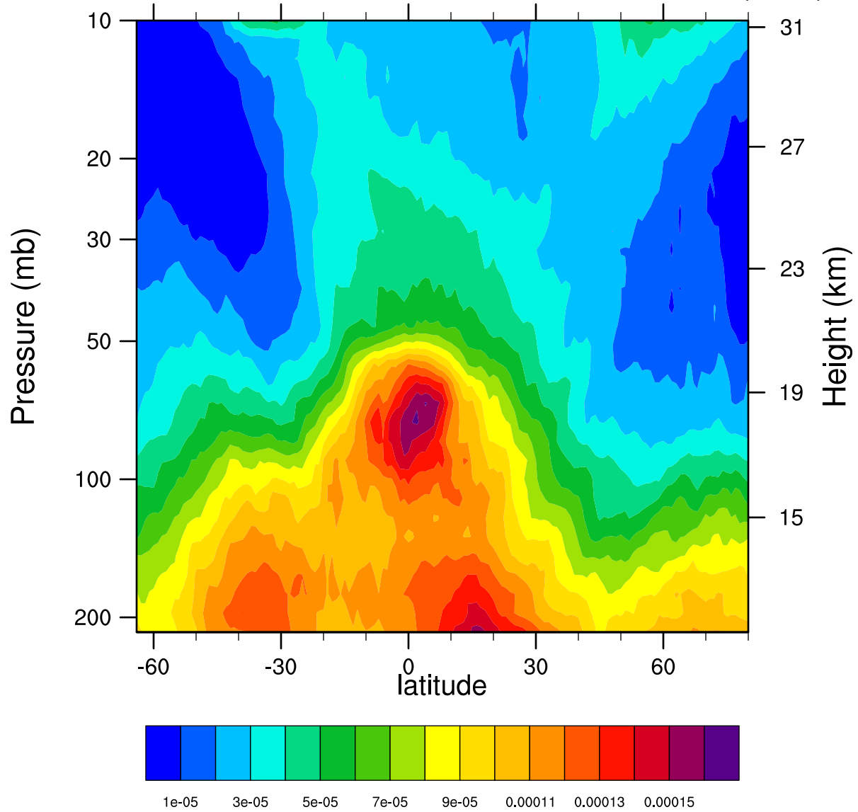
2005d054 12.1MicronExtinction_Combined (km -1 )
