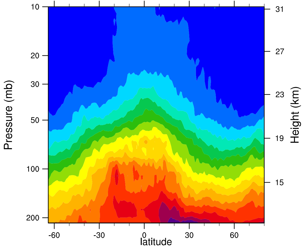
2007d085 12.1MicronExtinction_Combined ( \text{km}^{-1} )
