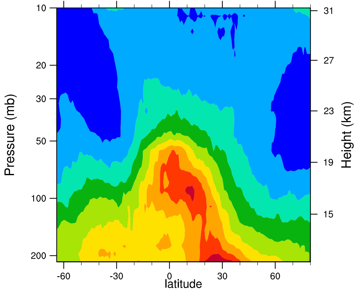
2005d117 12.1MicronExtinction_Combined (km -1 )
