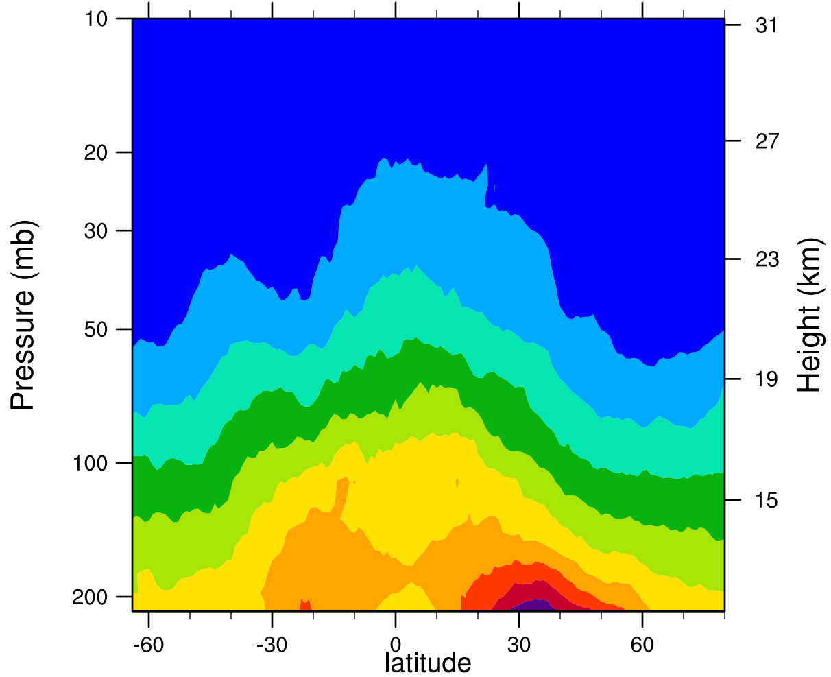
2007d134 12.1MicronExtinction_Combined (km -1 )
