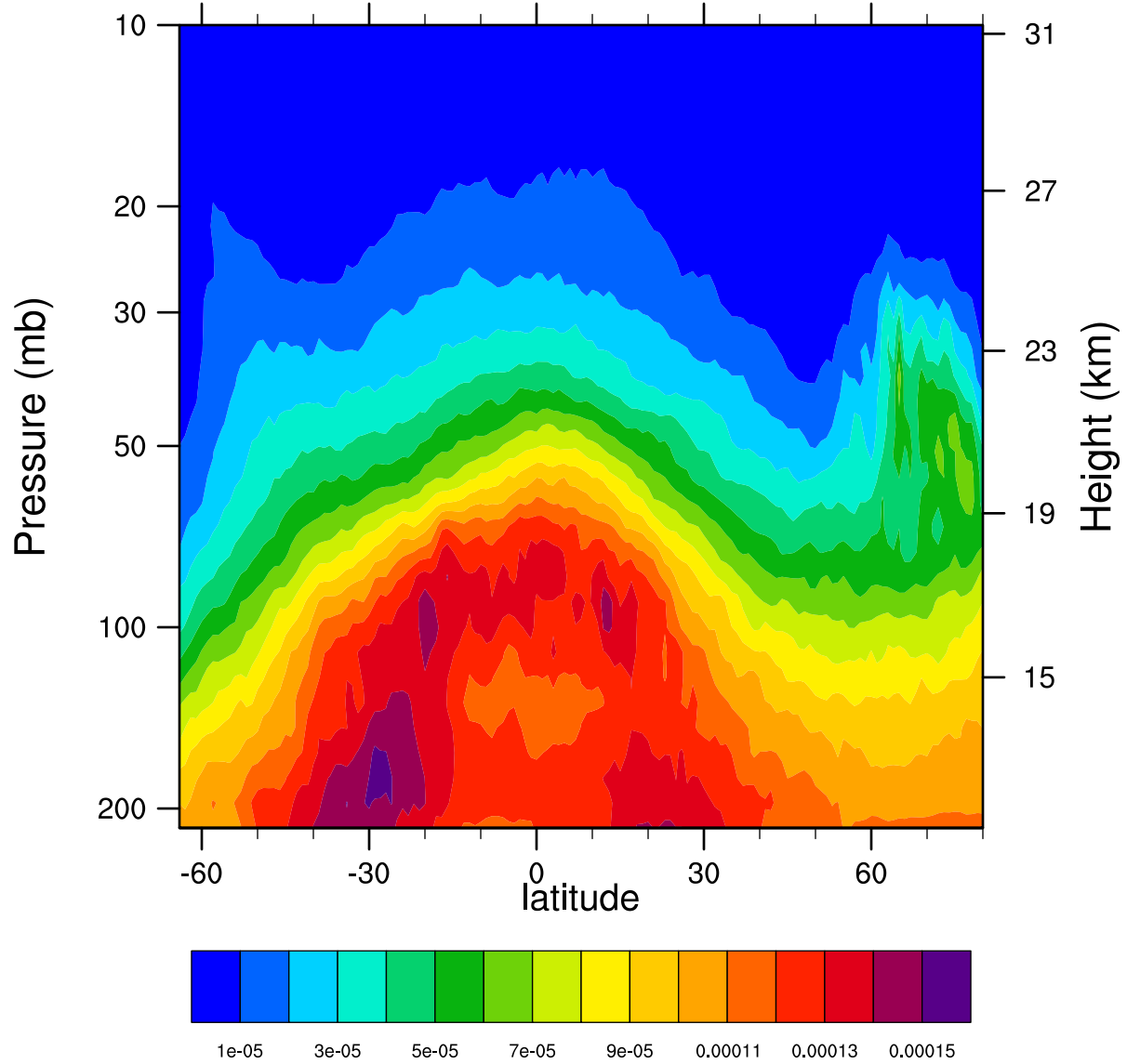
2006d360 12.1MicronExtinction_Combined (km -1 )
