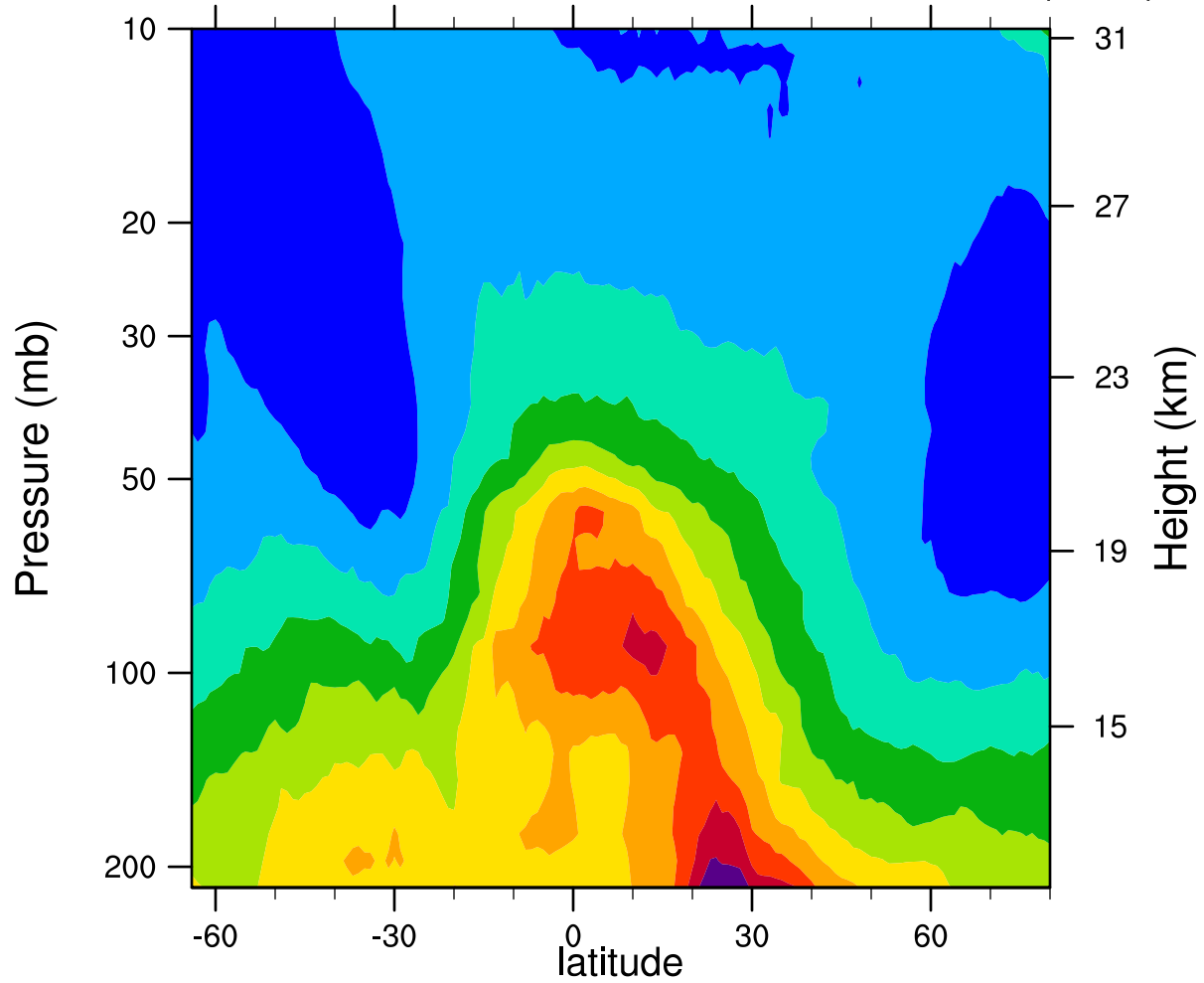
2005d122 12.1MicronExtinction_Combined (km -1 )
