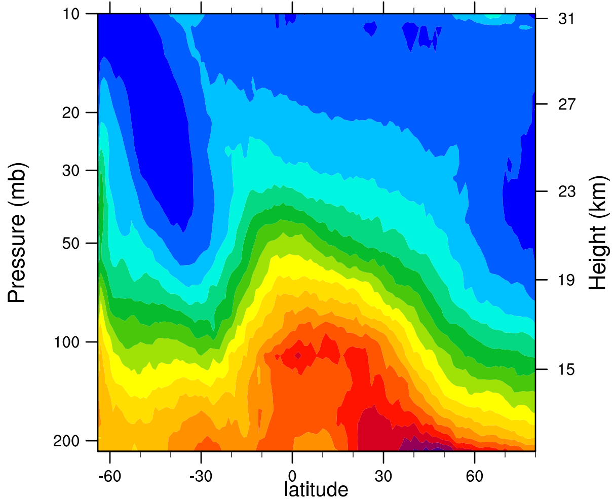
2005d197 12.1MicronExtinction_Combined (km -1 )
