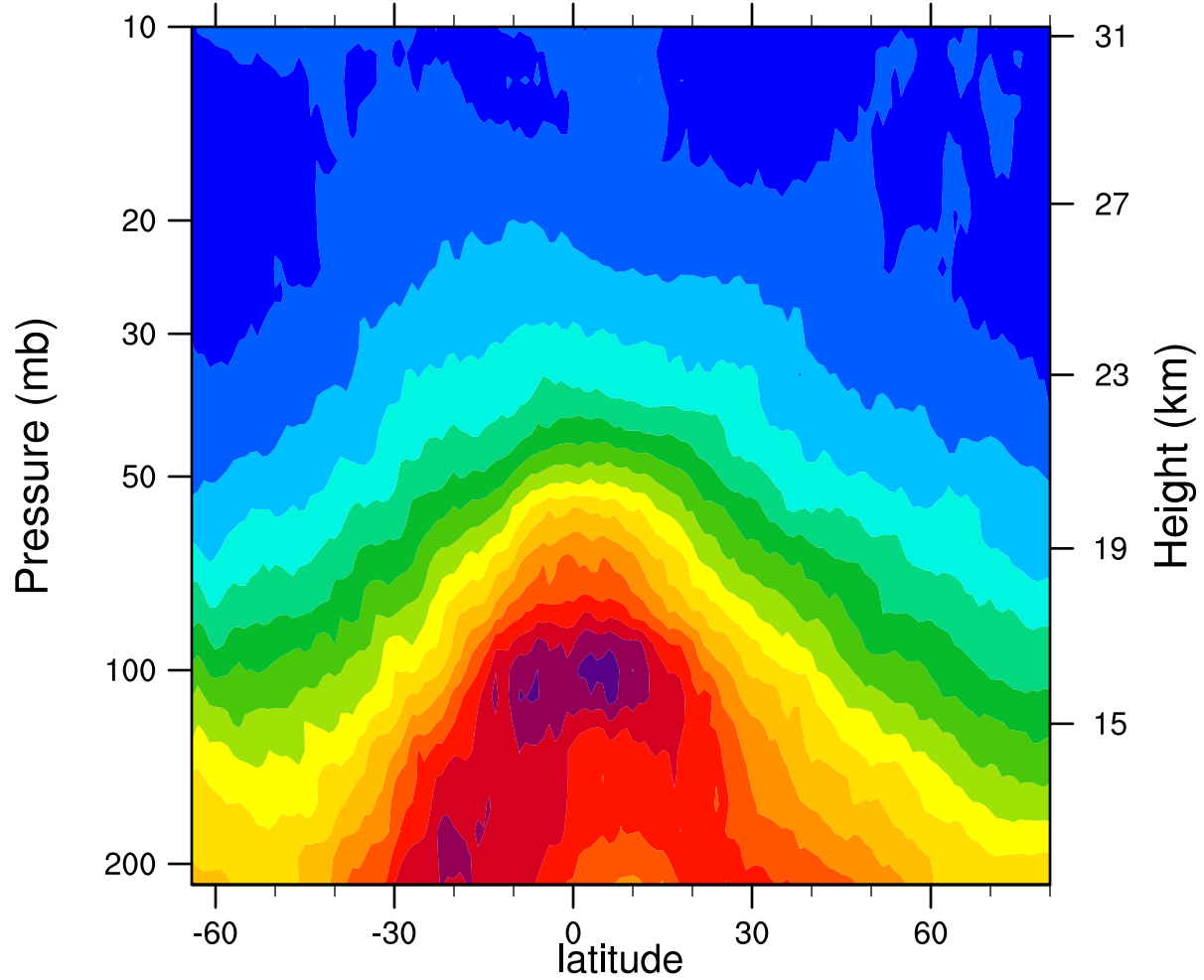
2006d297 12.1MicronExtinction_Combined (km -1 )
