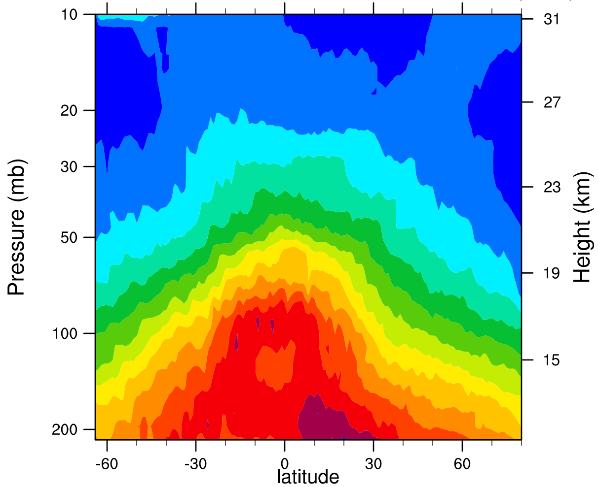
2006d038 12.1MicronExtinction_Combined (km -1 )
