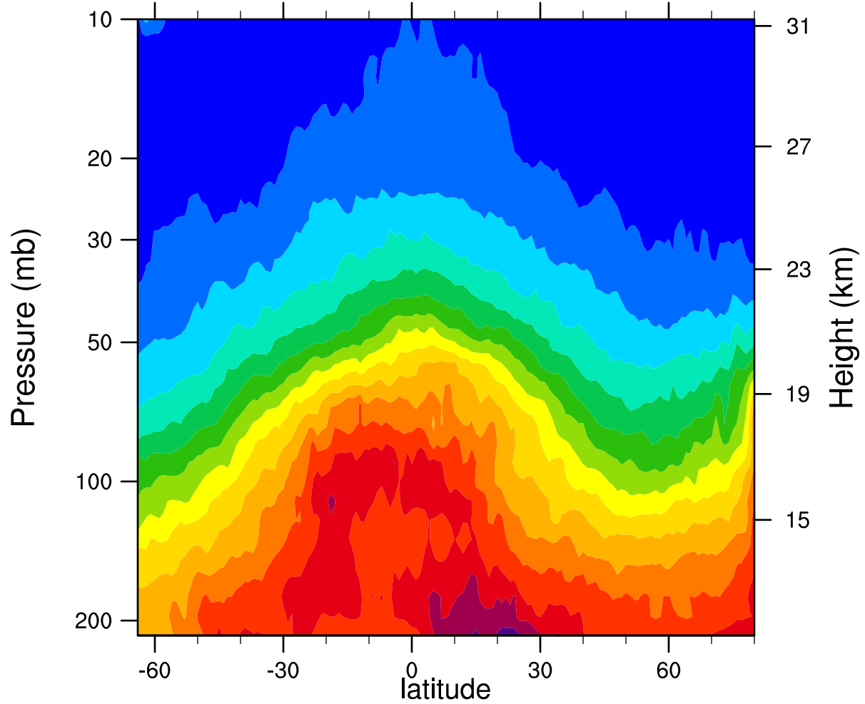
2007d045 12.1MicronExtinction_Combined ( \text{km}^{-1} )
