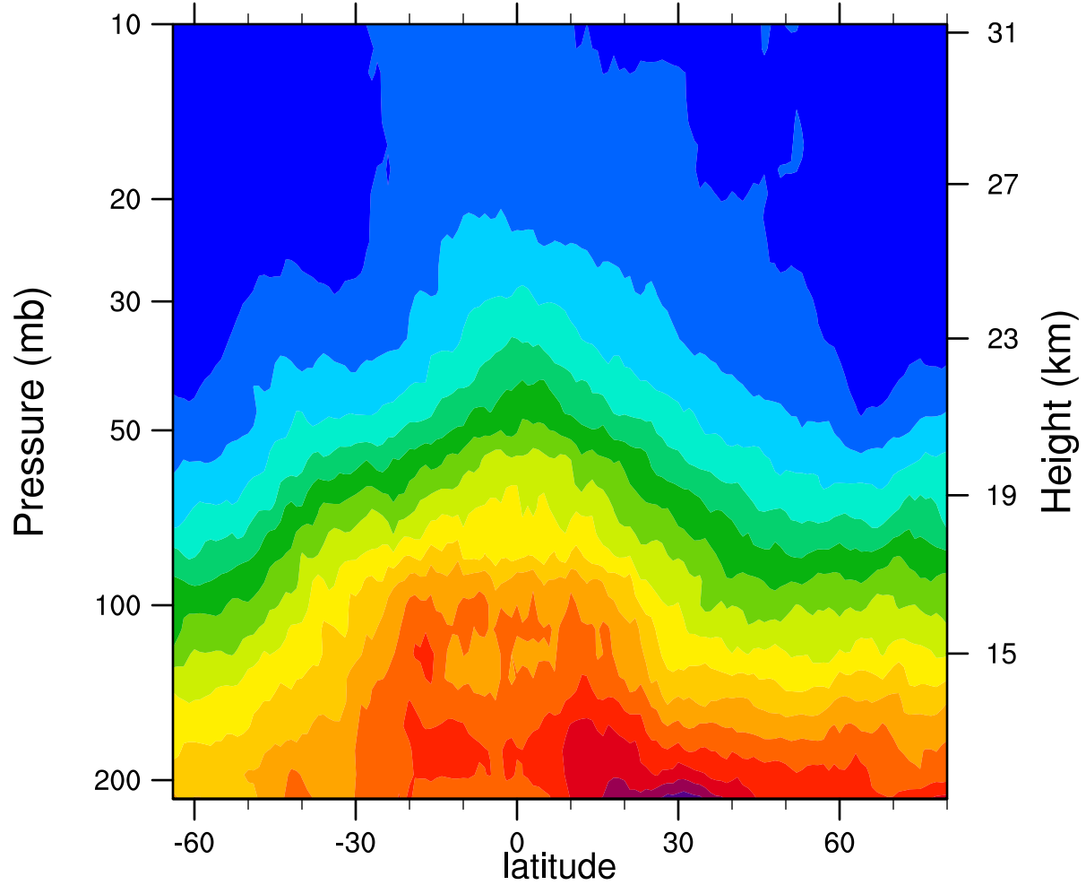
2007d090 12.1MicronExtinction_Combined (km -1 )
