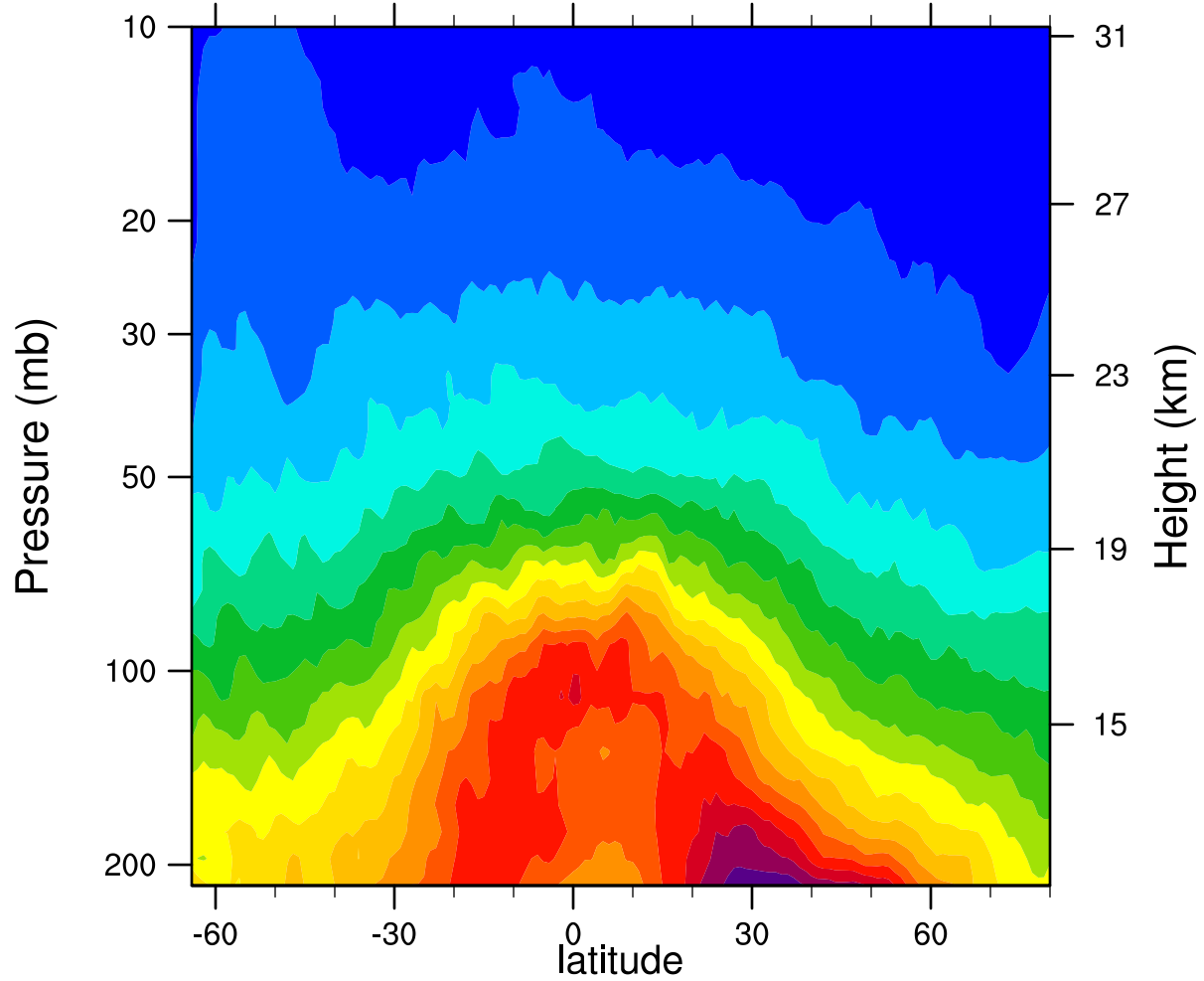
2006d150 12.1MicronExtinction_Combined ( \text{km}^{-1} )
