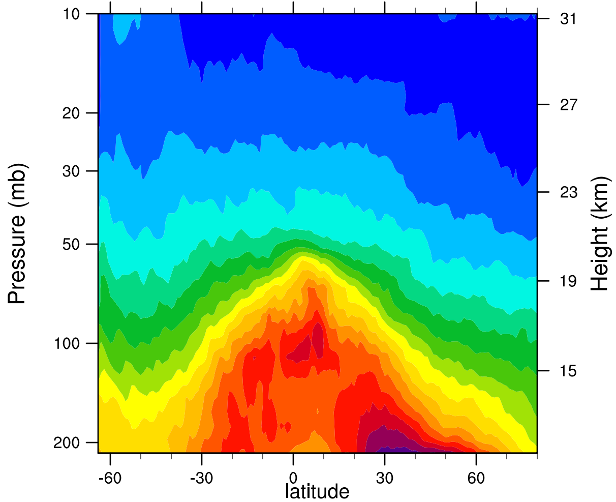
2006d167 12.1MicronExtinction_Combined ( \text{km}^{-1} )
