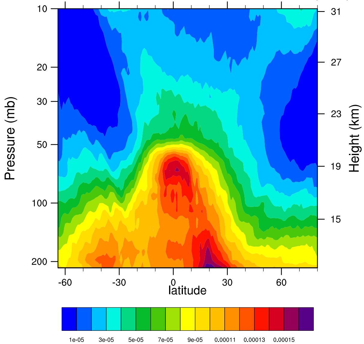
2005d081 12.1MicronExtinction_Combined (km -1 )
