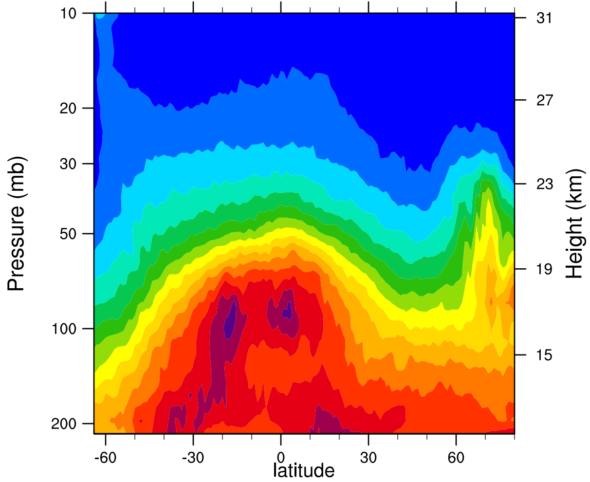
2007d027 12.1MicronExtinction_Combined (km -1 )
