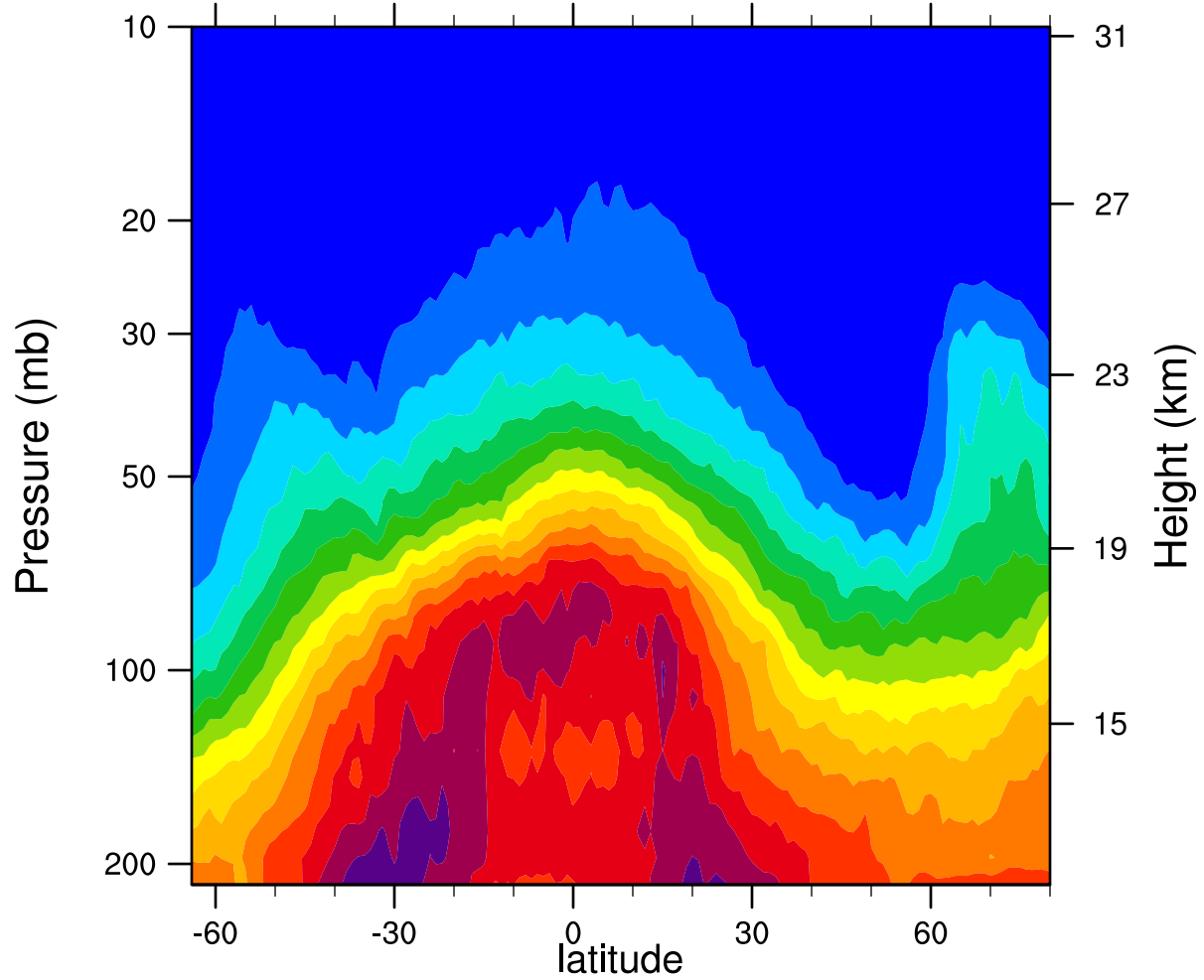
2006d355 12.1MicronExtinction_Combined (km -1 )
