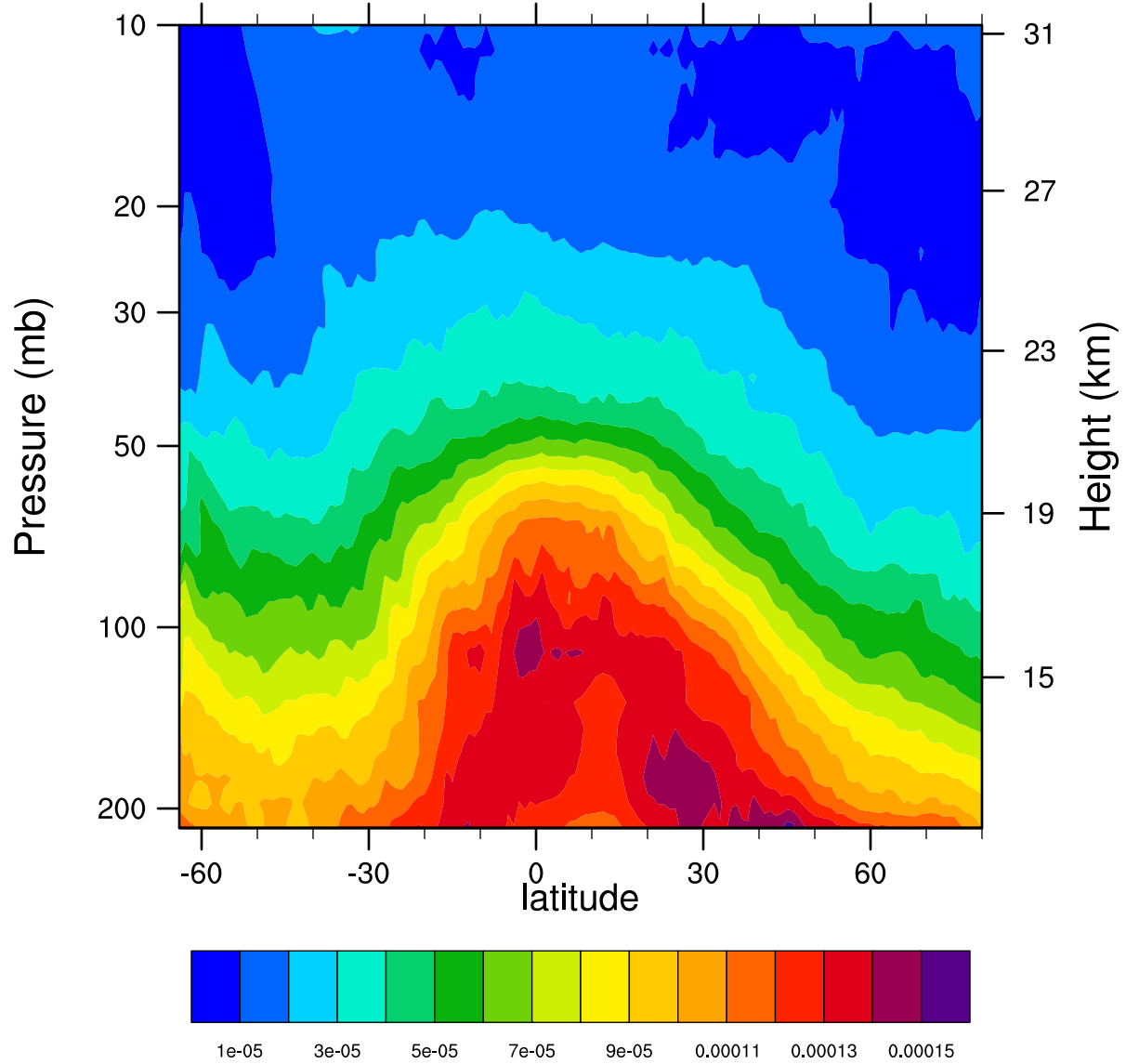
2006d236 12.1MicronExtinction_Combined (km -1 )
