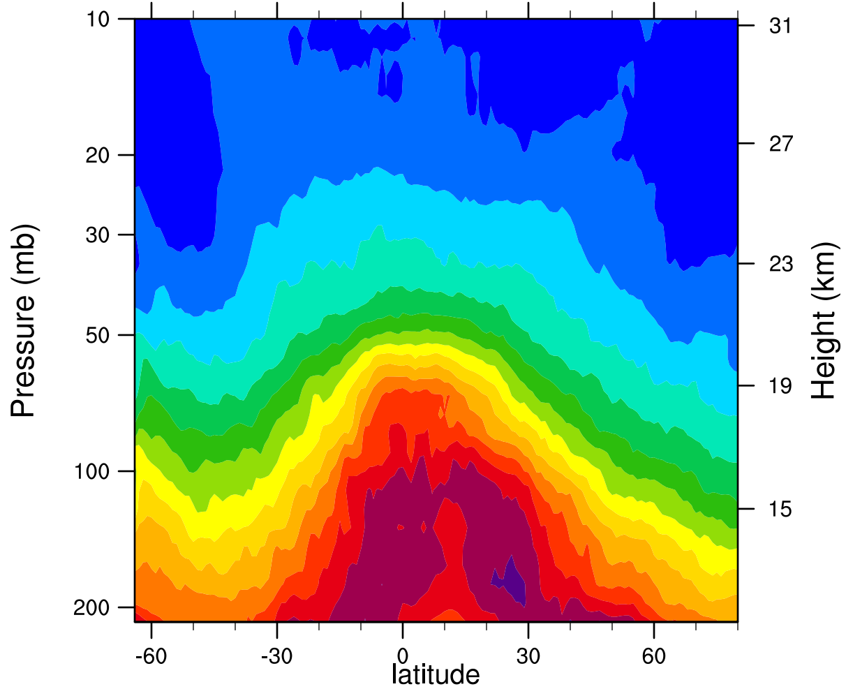
2006d253 12.1MicronExtinction_Combined (km -1 )
