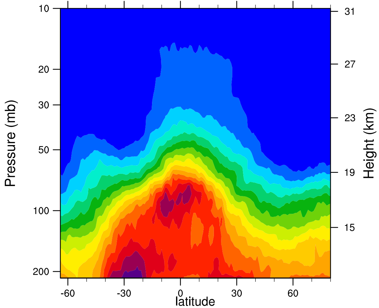
2006d329 12.1MicronExtinction_Combined (km -1 )
