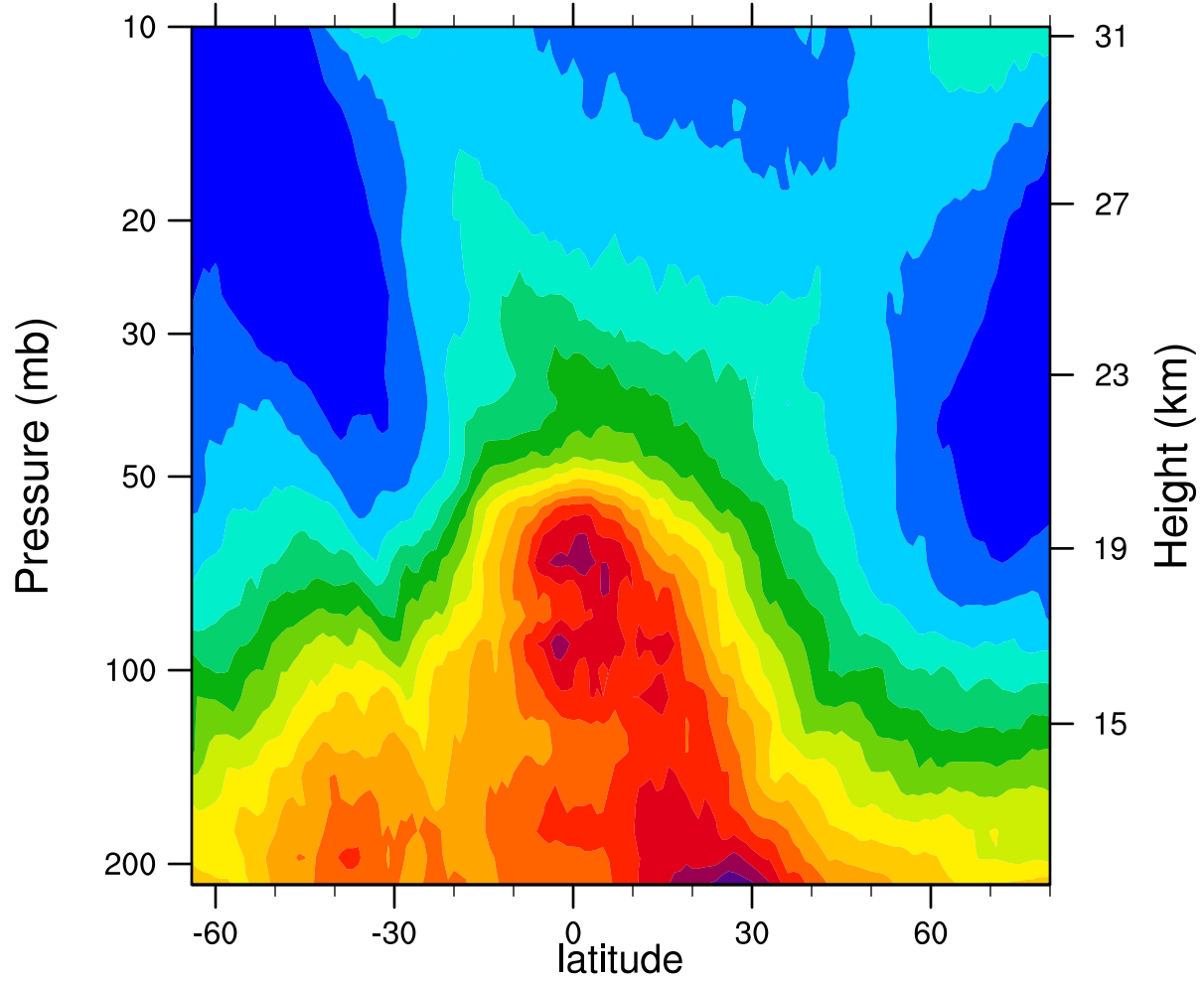
2005d093 12.1MicronExtinction_Combined (km -1 )
