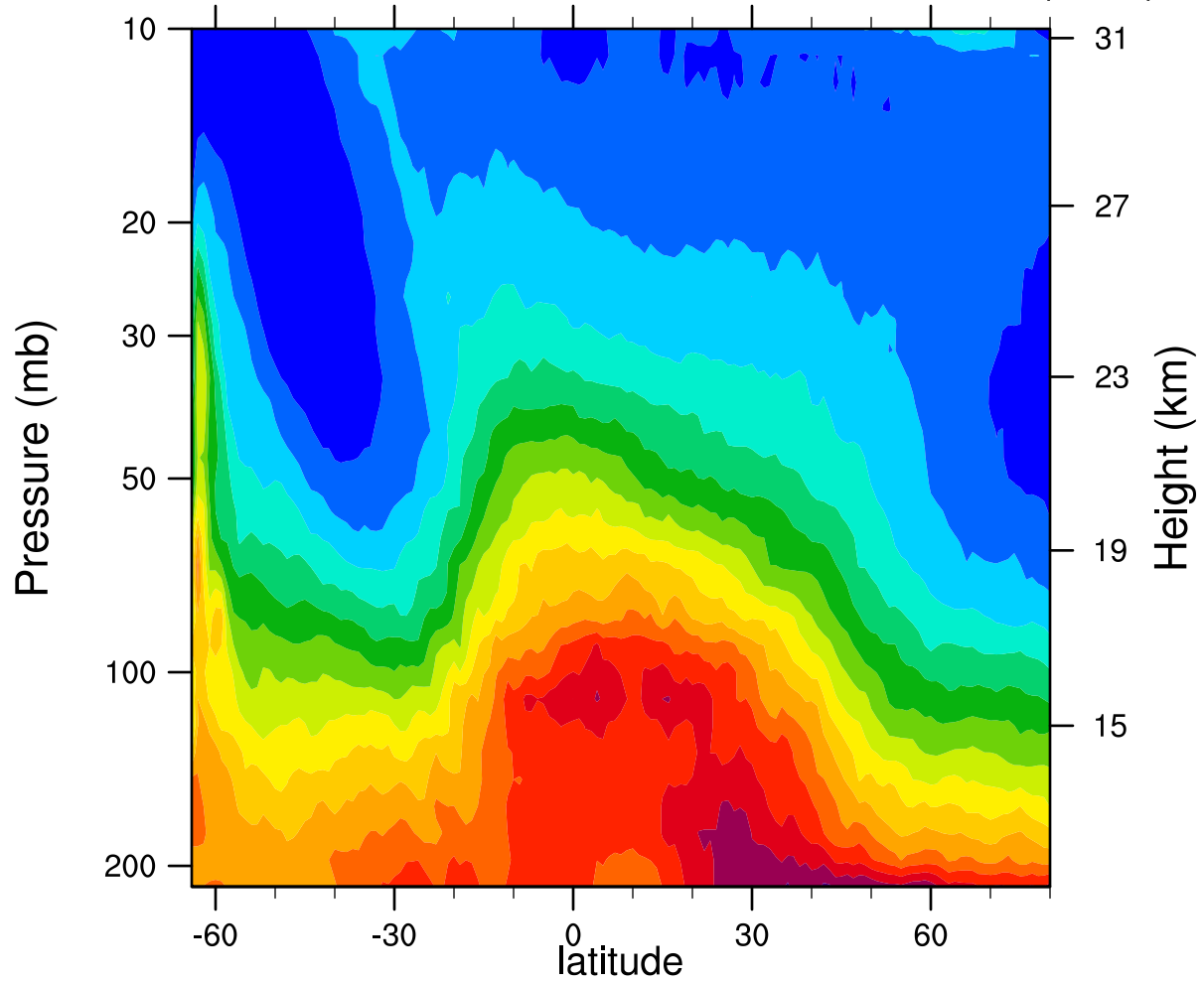
2005d206 12.1MicronExtinction_Combined (km -1 )
