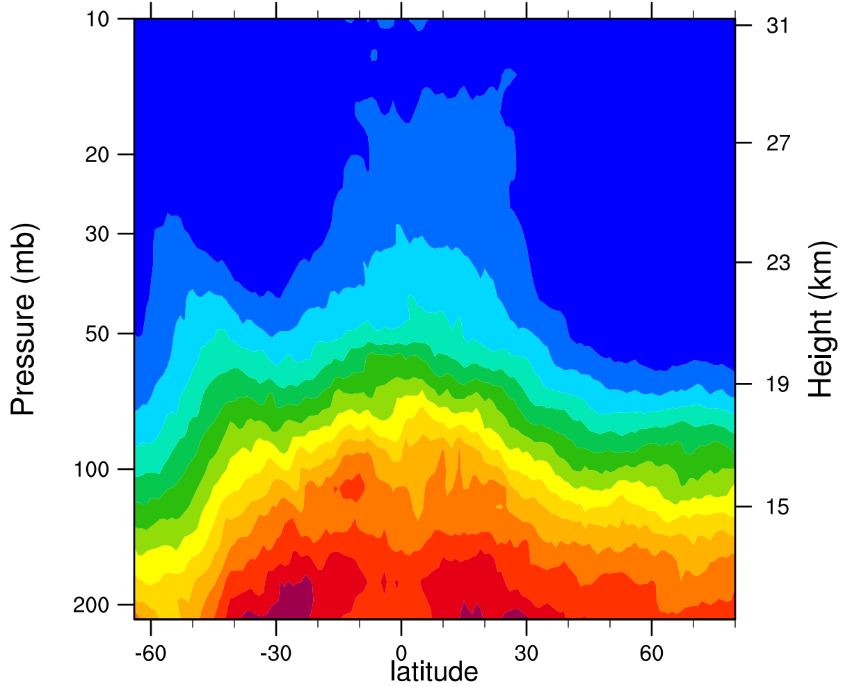
2007d328 12.1MicronExtinction_Combined (km -1 )
