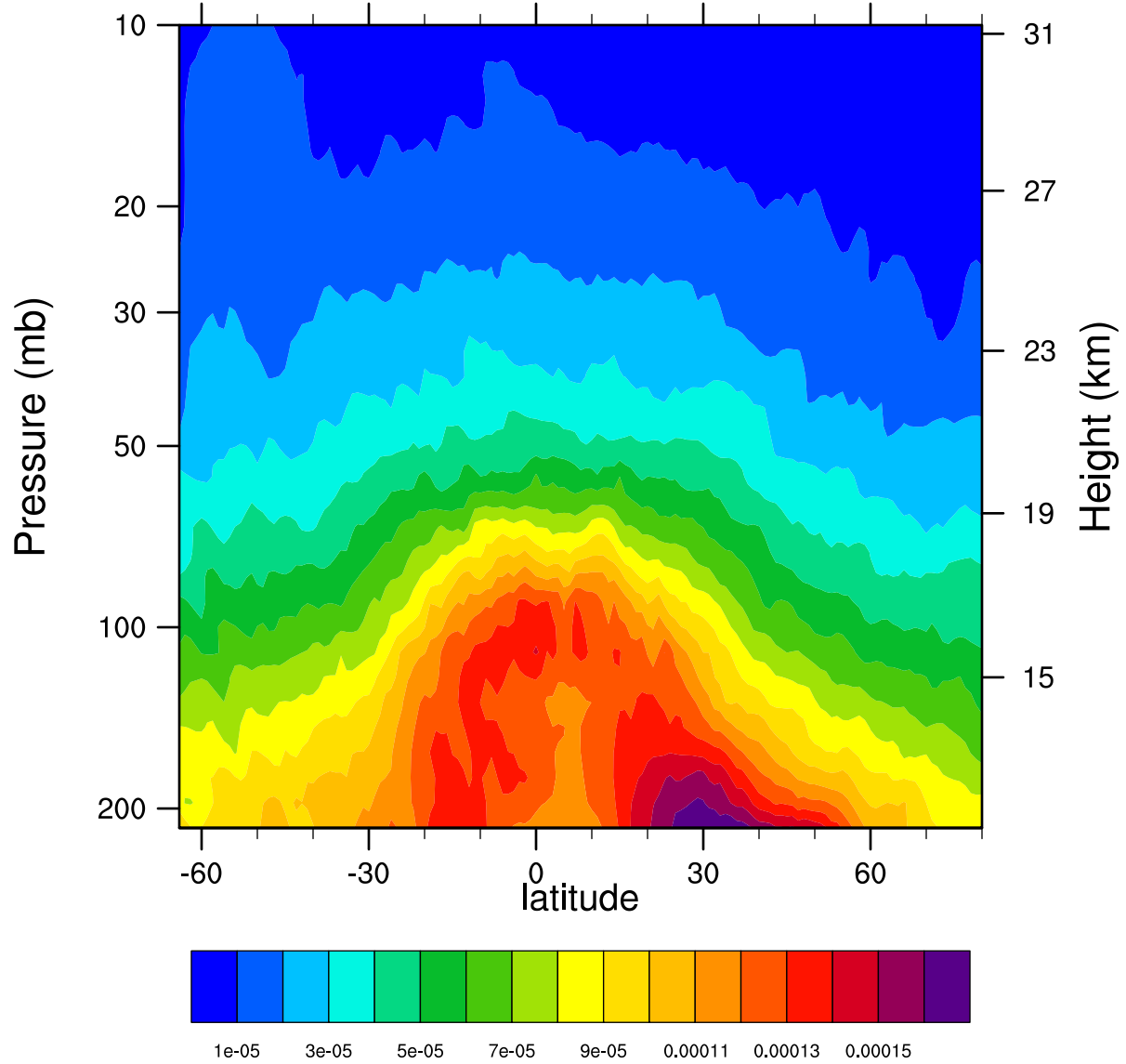
2006d145 12.1MicronExtinction_Combined ( \text{km}^{-1} )
