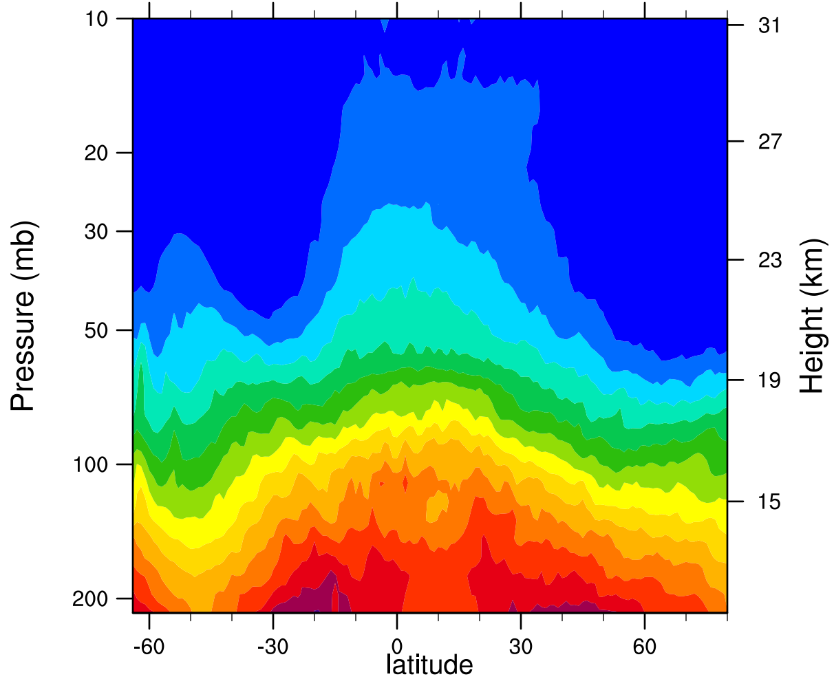
2007d266 12.1MicronExtinction_Combined (km -1 )
