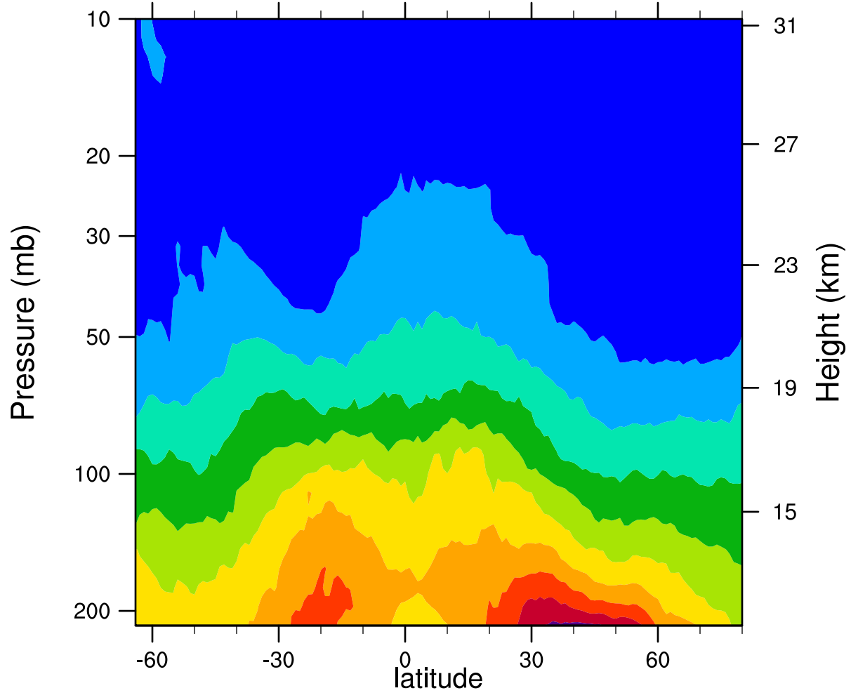
2007d147 12.1MicronExtinction_Combined (km -1 )
