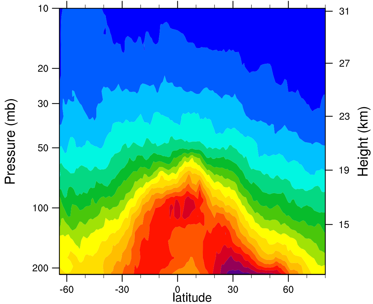
2006d158 12.1MicronExtinction_Combined ( \text{km}^{-1} )
