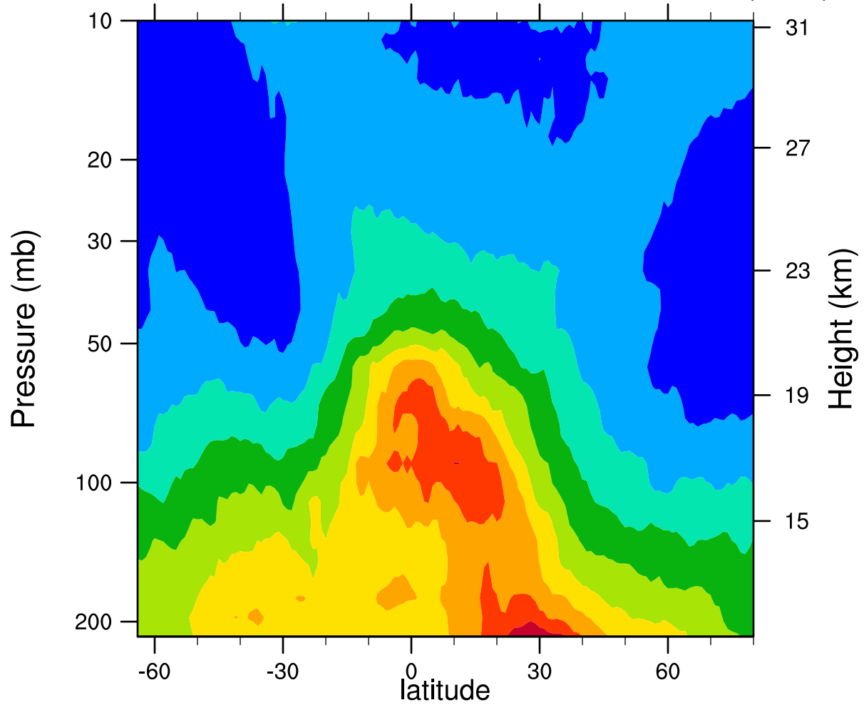
2005d114 12.1MicronExtinction_Combined (km -1 )
