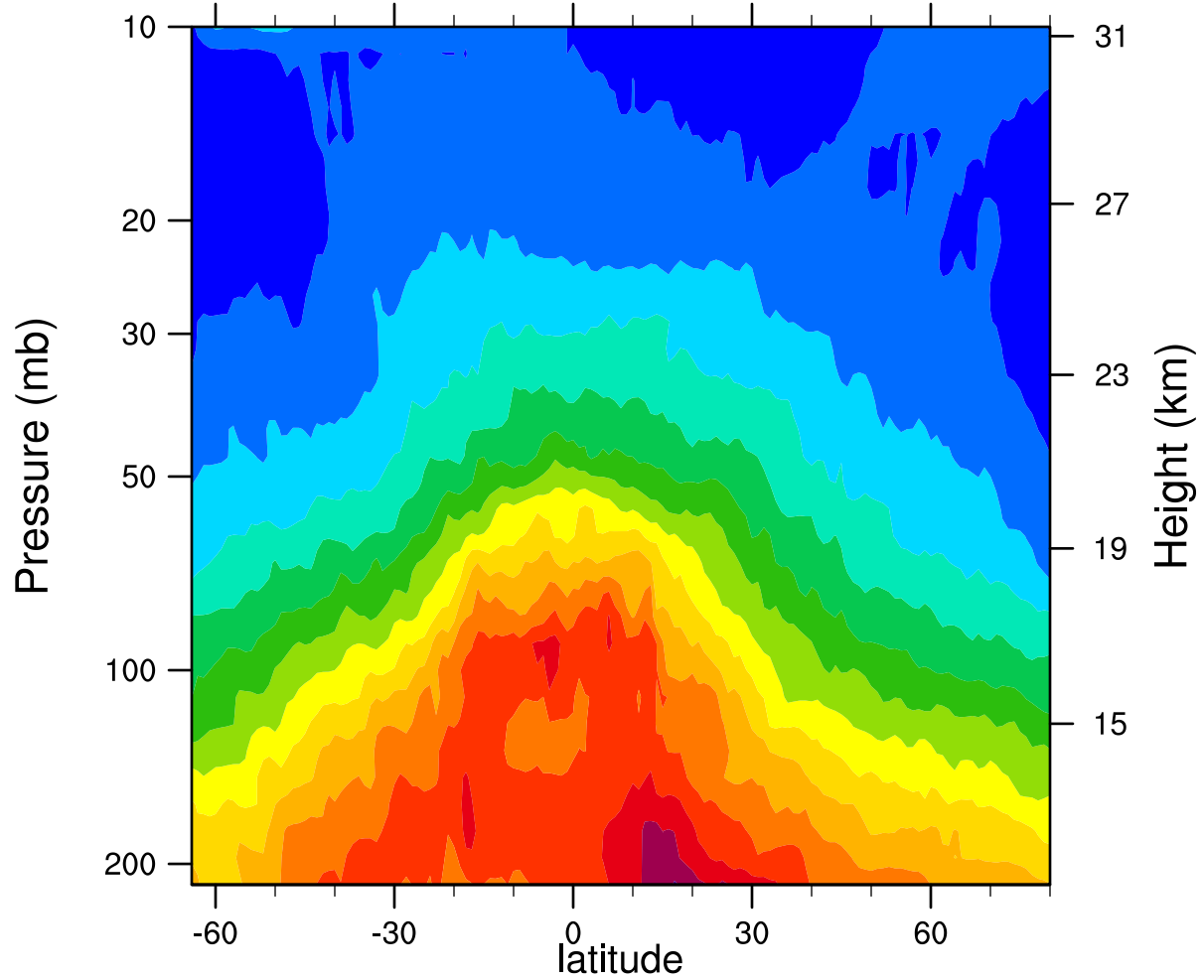
2006d045 12.1MicronExtinction_Combined (km -1 )
