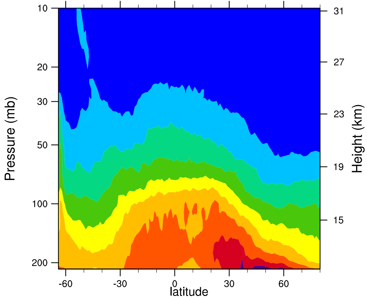
2007d204 12.1MicronExtinction_Combined (km -1 )
