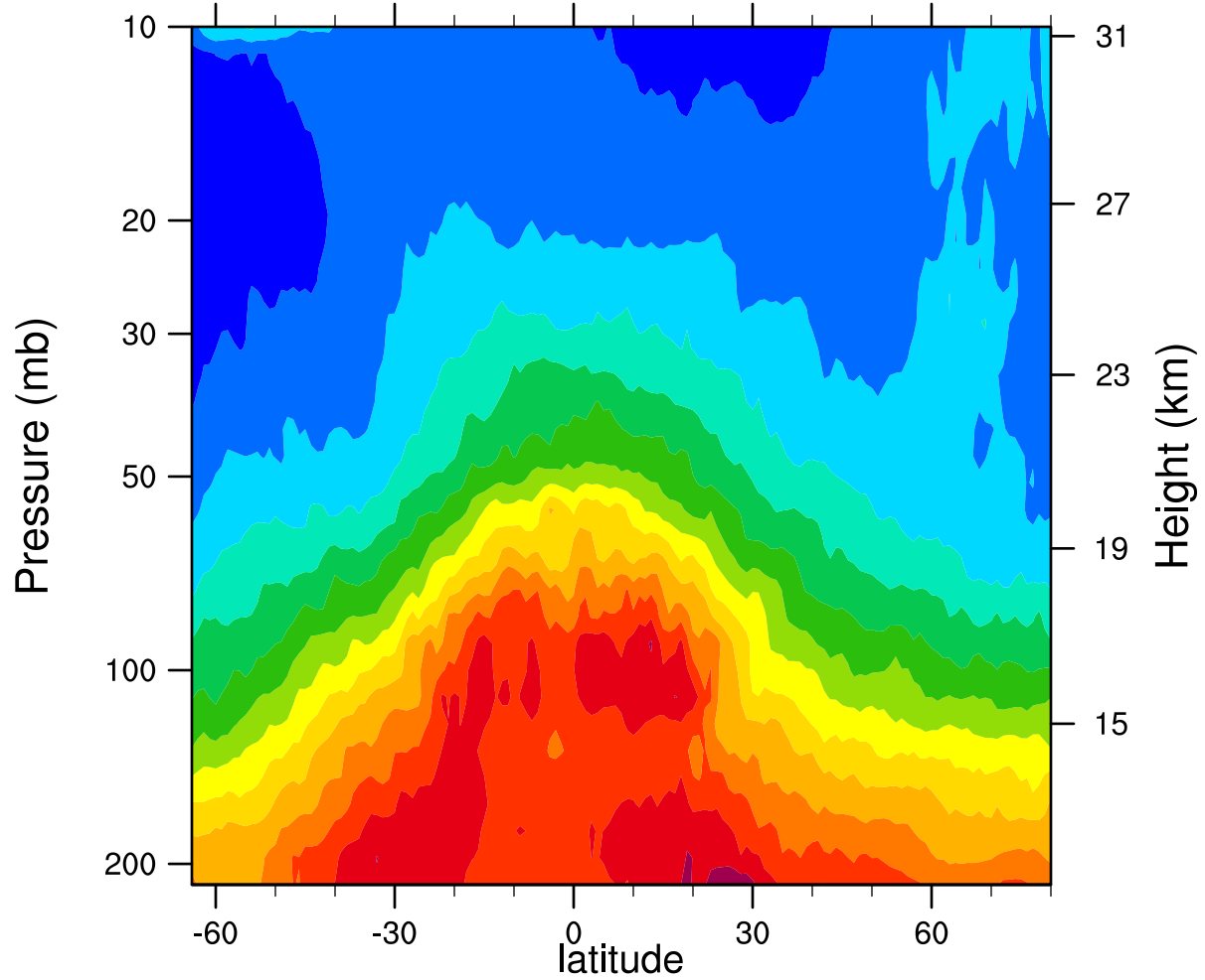
2005d351 12.1MicronExtinction_Combined (km -1 )
