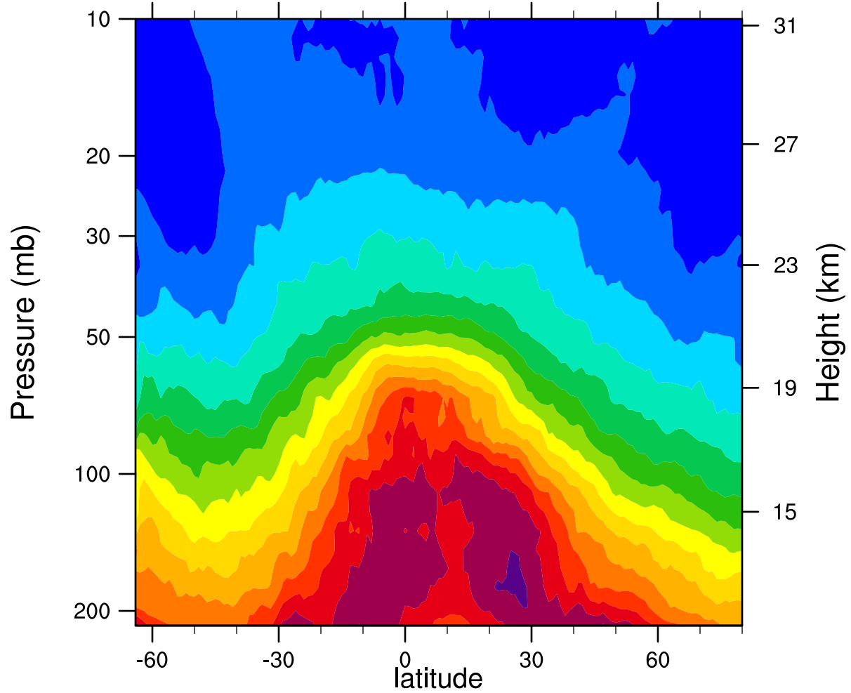
2006d255 12.1MicronExtinction_Combined ( \text{km}^{-1} )
