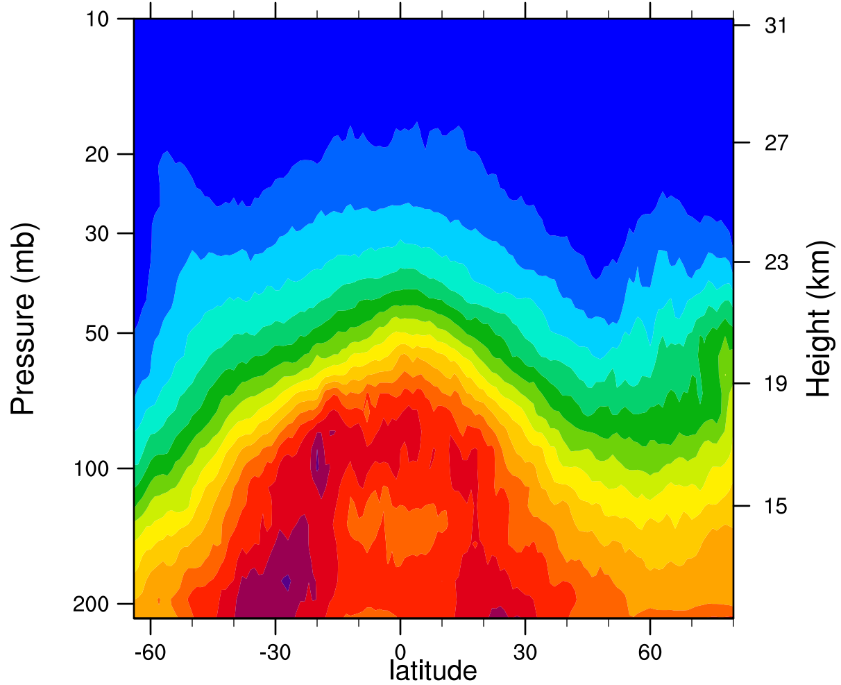
2006d362 12.1MicronExtinction_Combined (km -1 )
