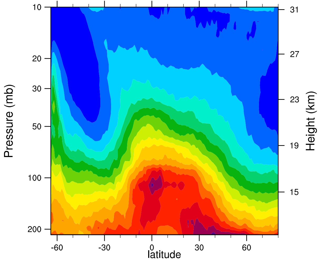
2005d212 12.1MicronExtinction_Combined (km -1 )
