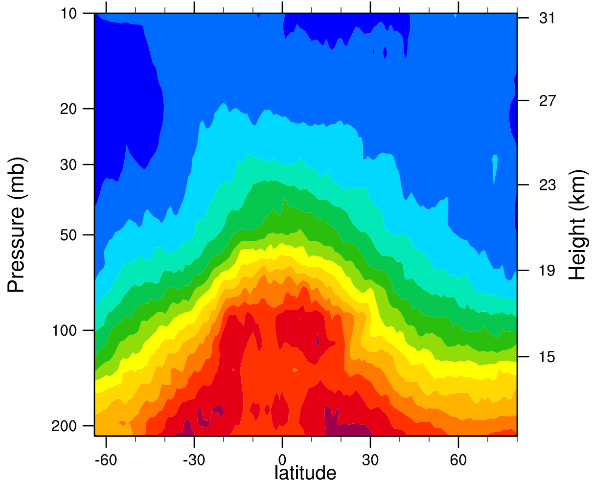
2005d341 12.1MicronExtinction_Combined (km -1 )
