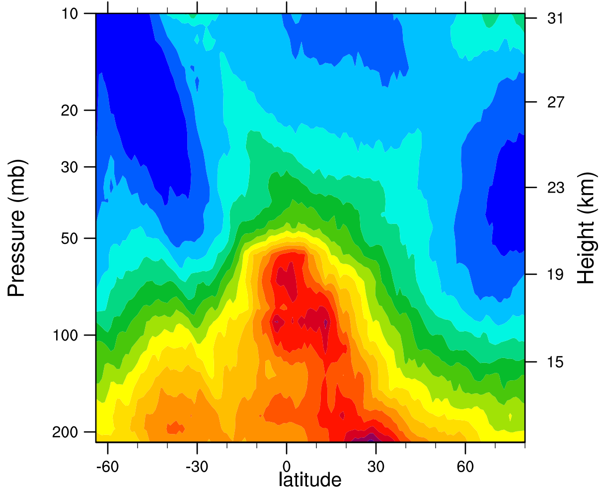
2005d101 12.1MicronExtinction_Combined (km -1 )
