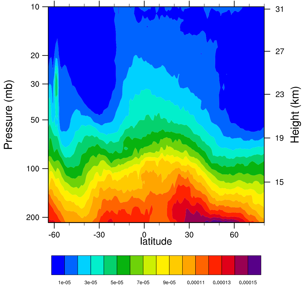
2007d229 12.1MicronExtinction_Combined (km -1 )
