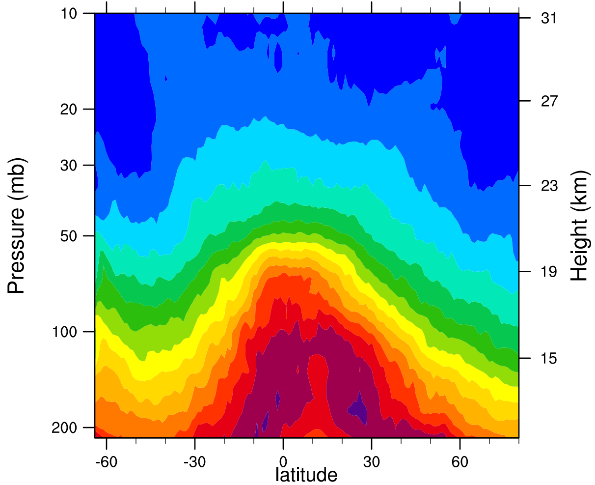
2006d252 12.1MicronExtinction_Combined (km -1 )
