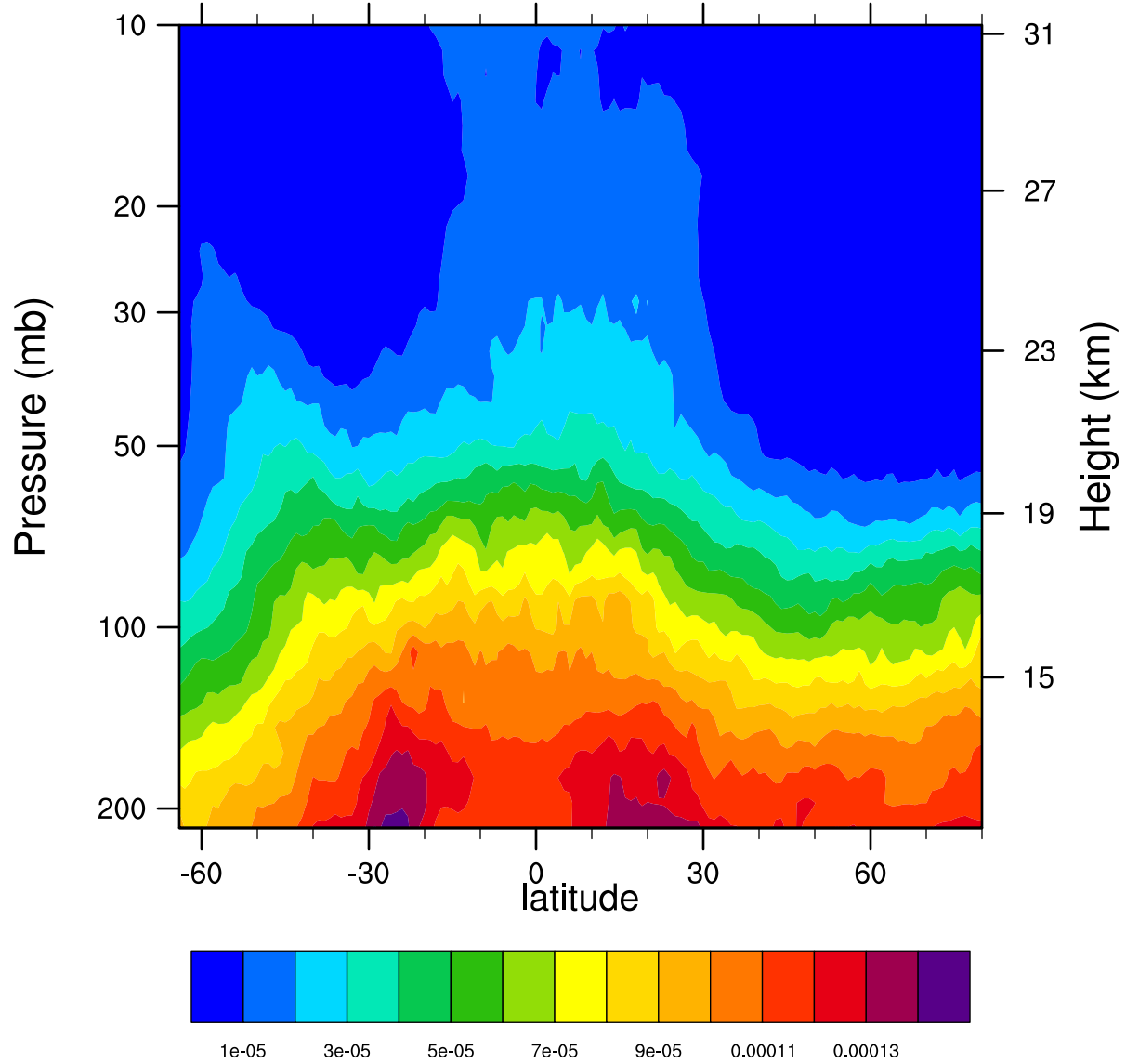
2007d345 12.1MicronExtinction_Combined ( \text{km}^{-1} )
