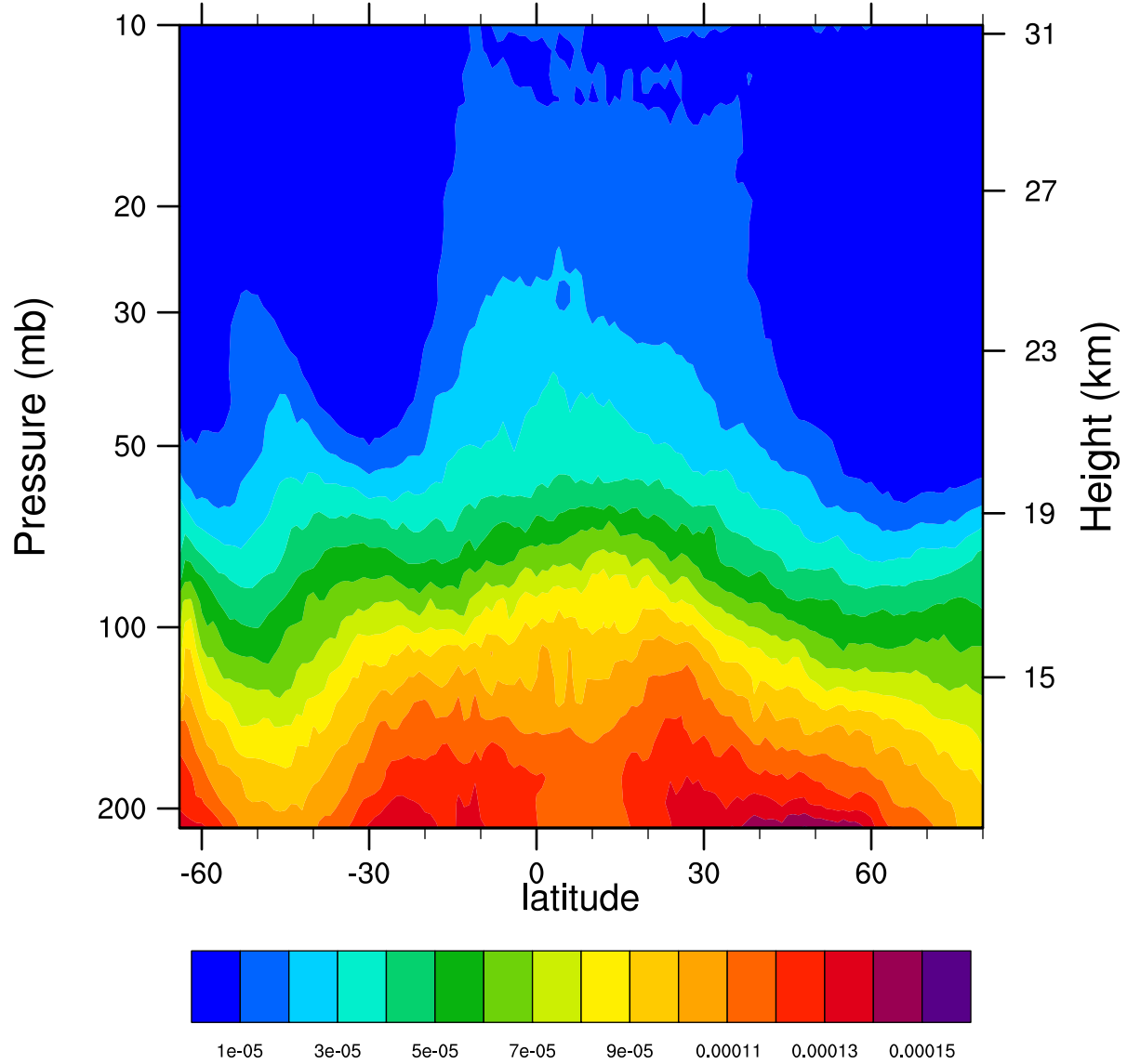
2007d249 12.1MicronExtinction_Combined (km -1 )
