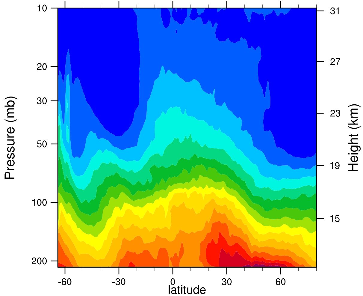
2007d228 12.1MicronExtinction_Combined (km -1 )
