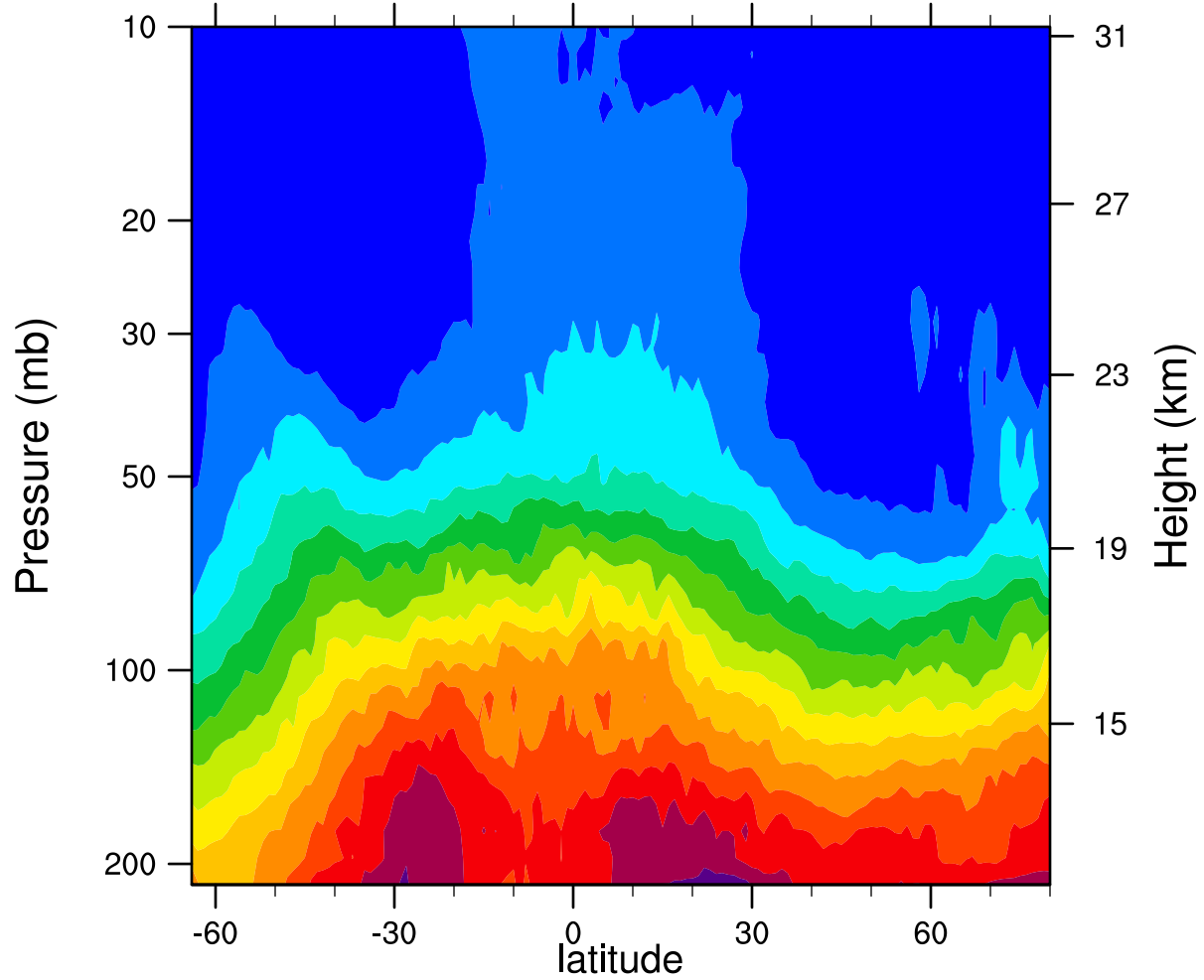
2007d356 12.1MicronExtinction_Combined (km -1 )
