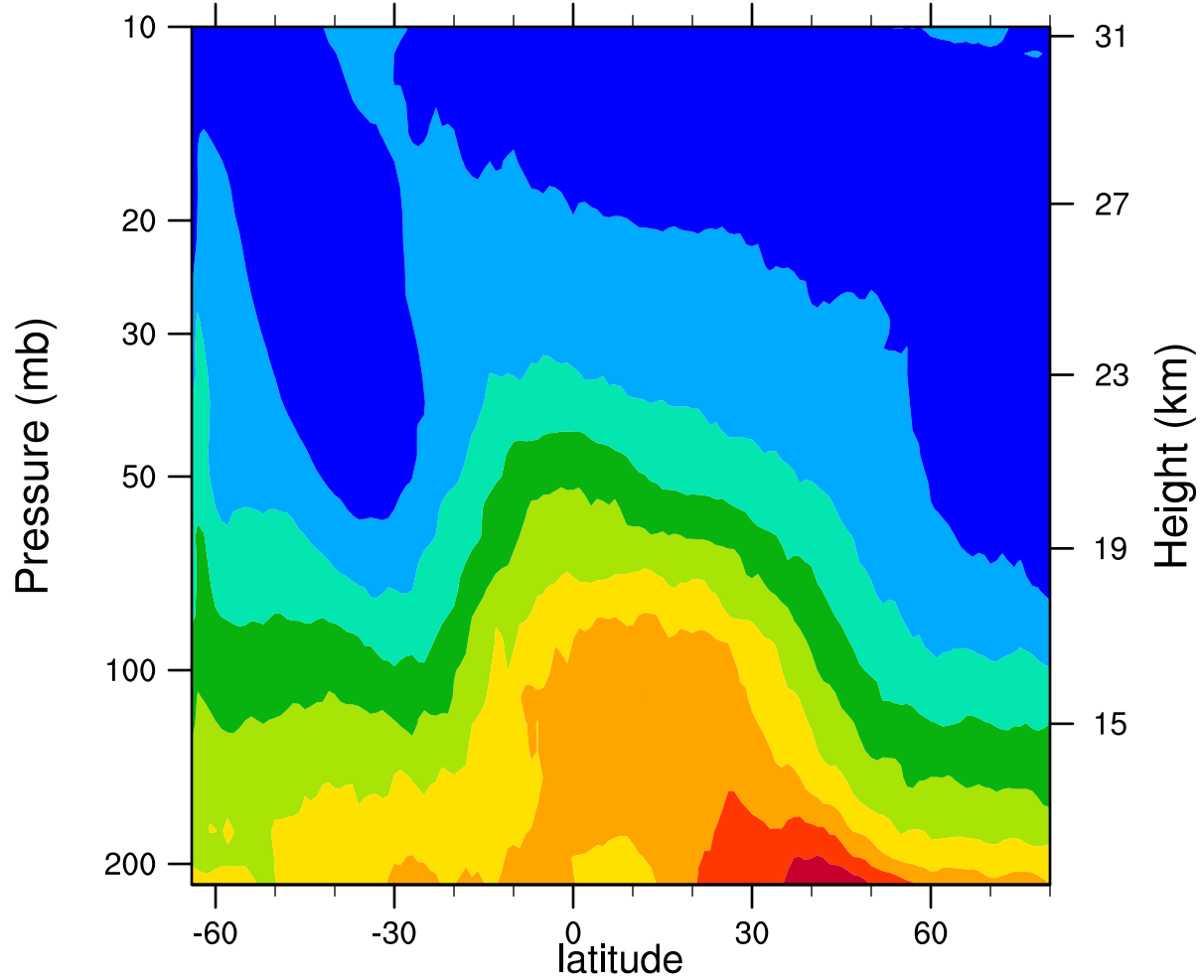
2005d187 12.1MicronExtinction_Combined (km -1 )
