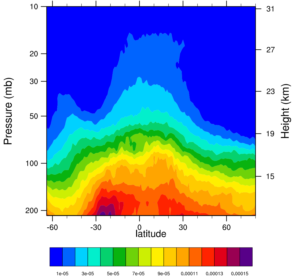
2007d307 12.1MicronExtinction_Combined ( \text{km}^{-1} )
