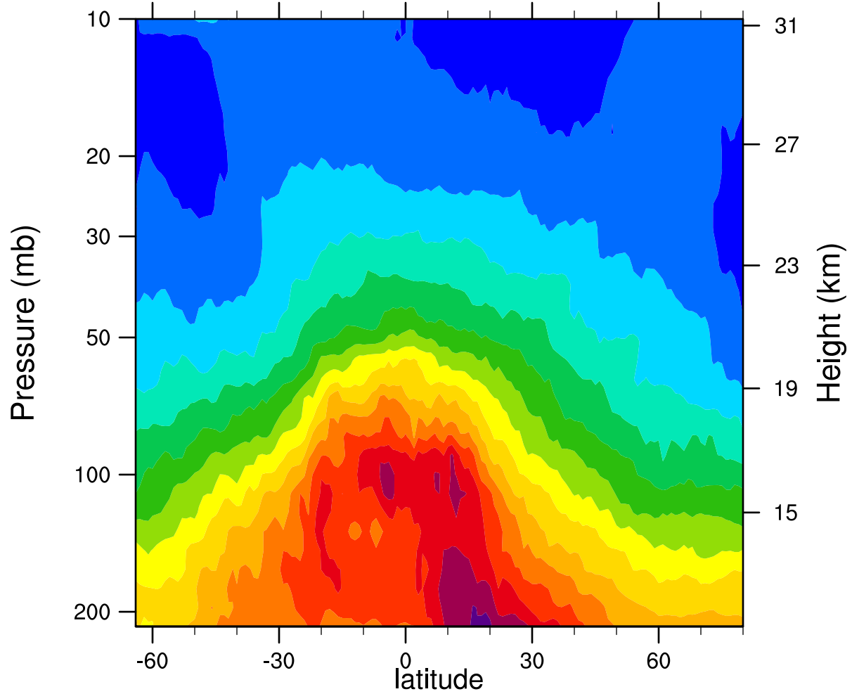
2006d066 12.1MicronExtinction_Combined (km -1 )
