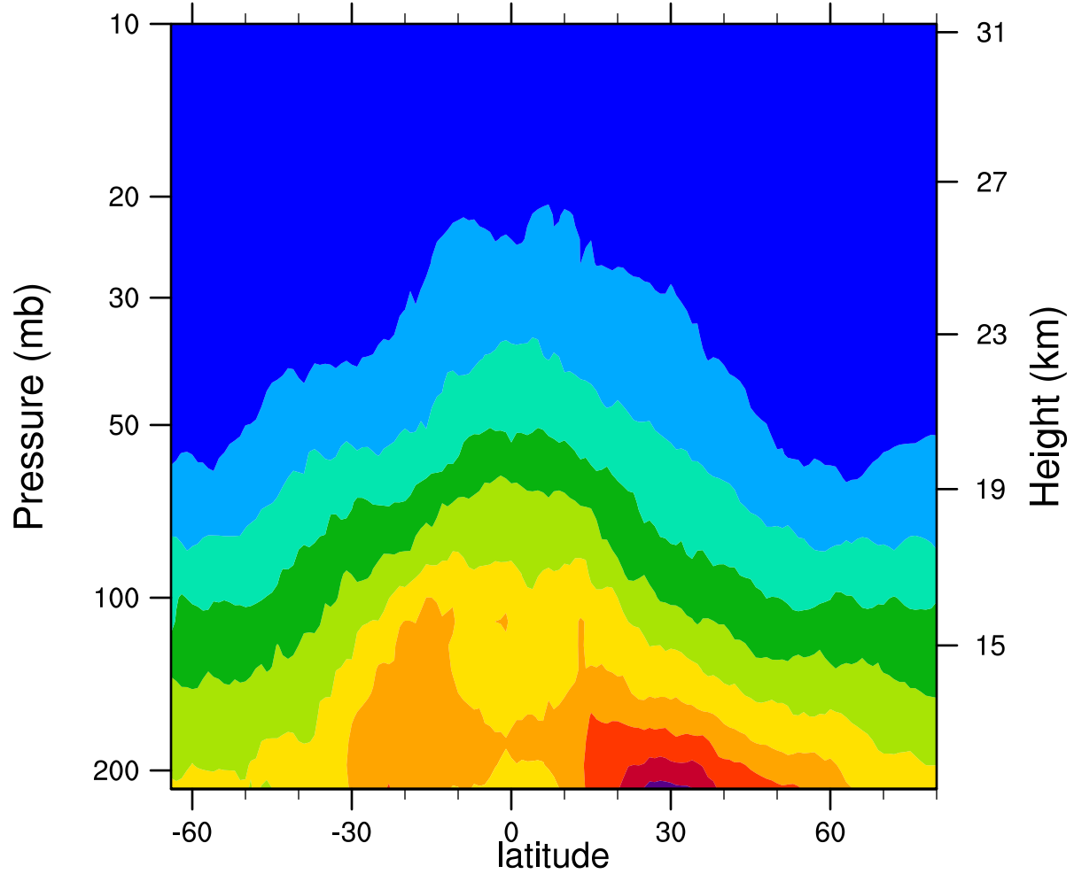
2007d118 12.1MicronExtinction_Combined (km -1 )
