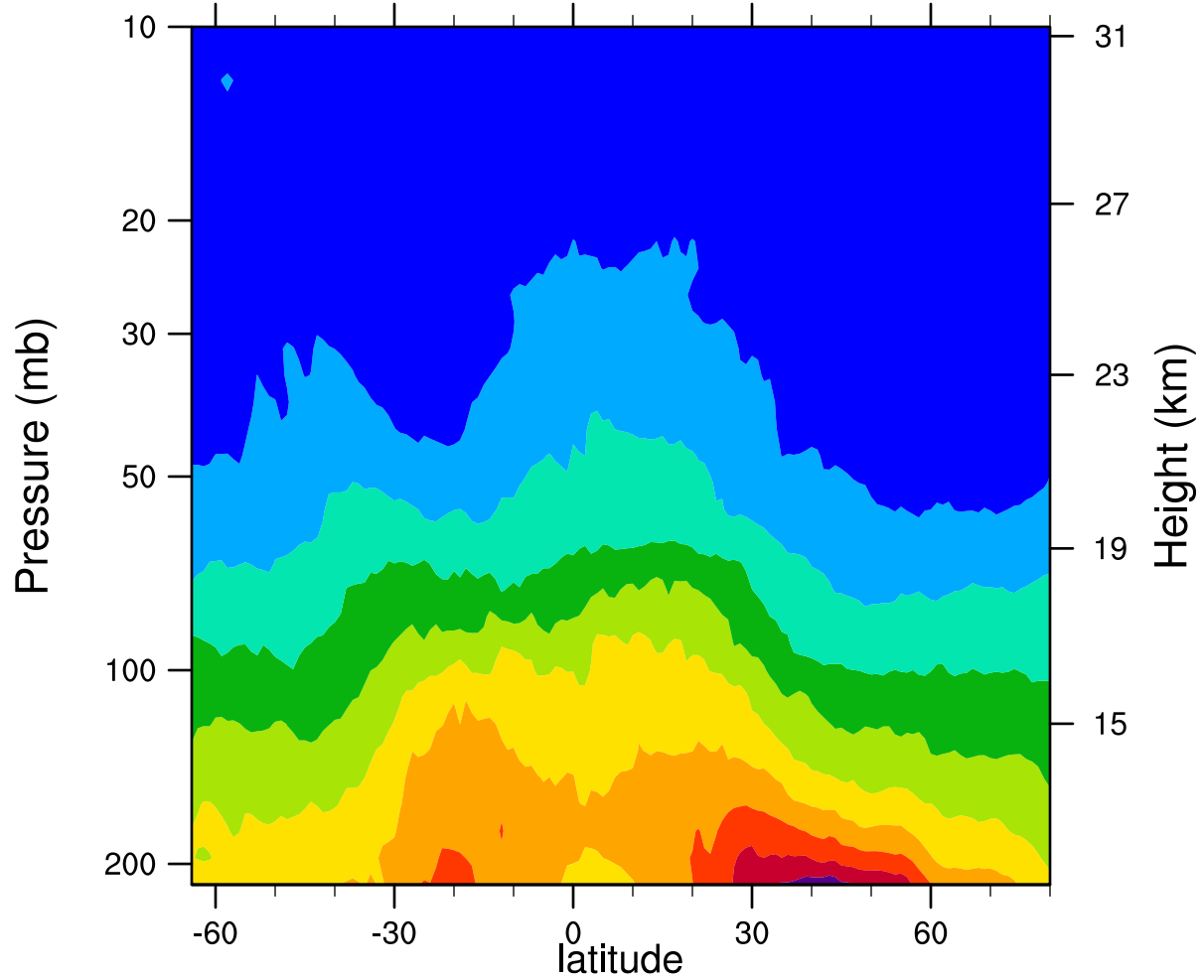
2007d153 12.1MicronExtinction_Combined (km -1 )
