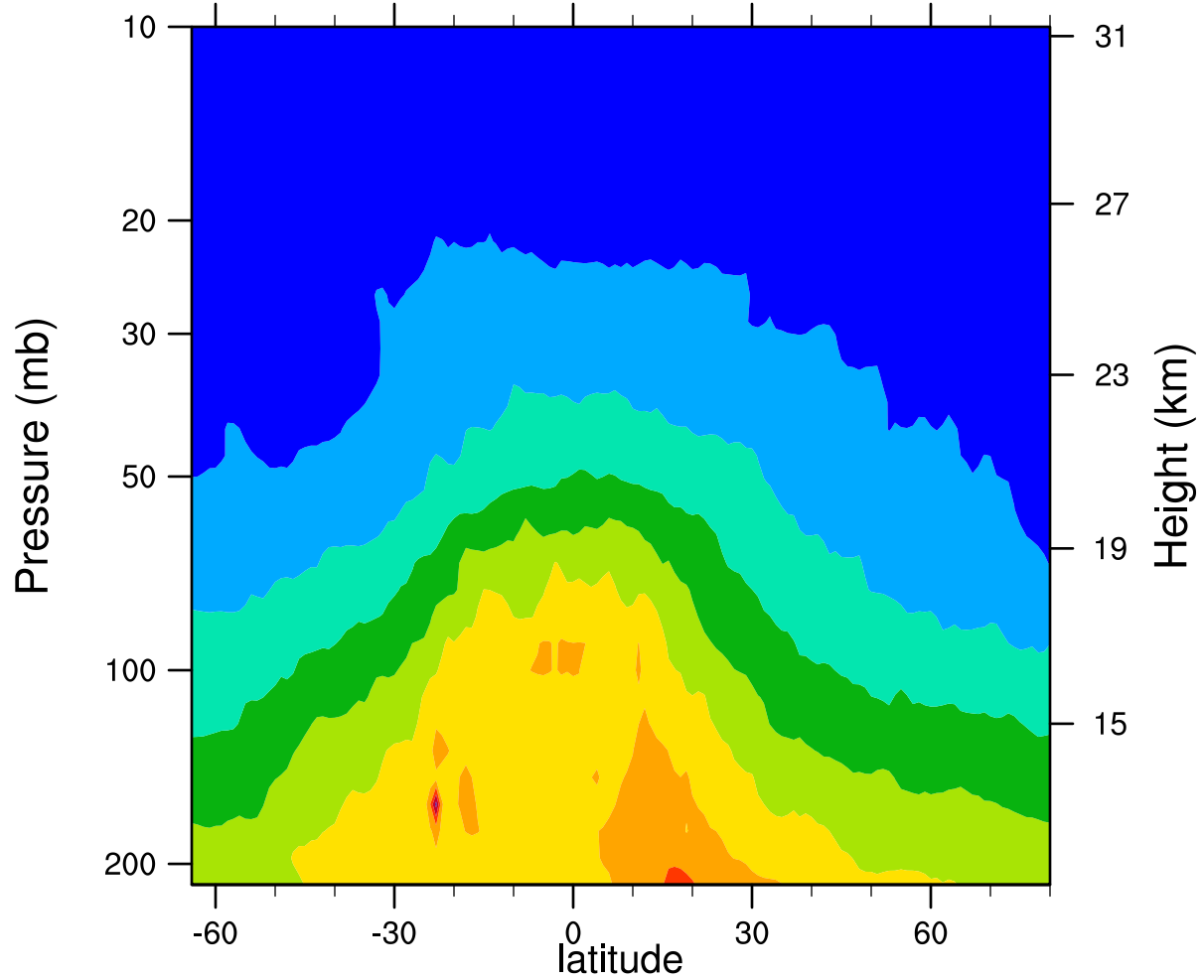
2006d054 12.1MicronExtinction_Combined (km -1 )
