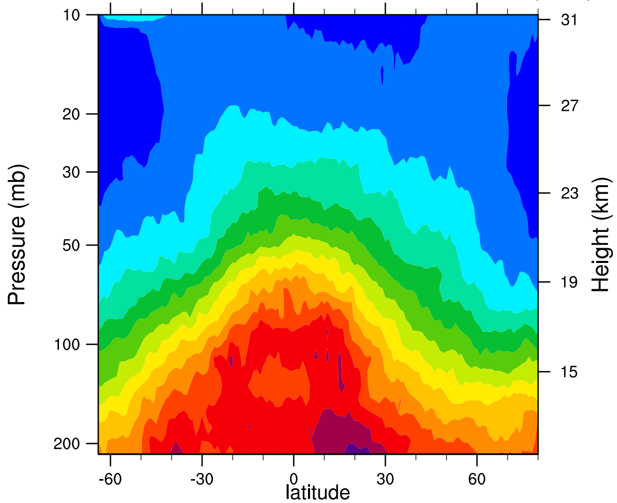
2006d019 12.1MicronExtinction_Combined ( \text{km}^{-1} )
