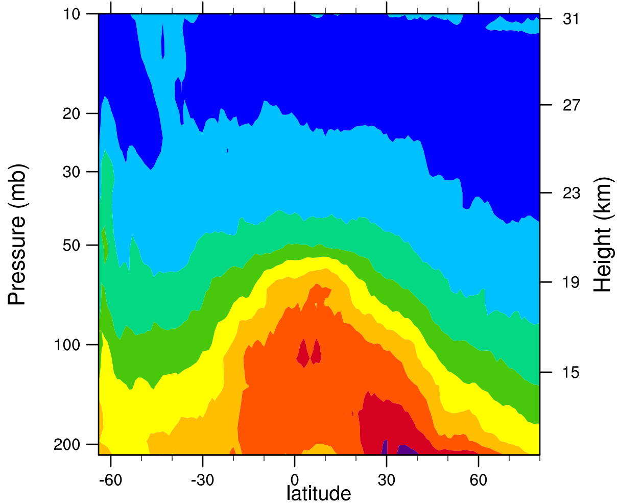
2006d199 12.1MicronExtinction_Combined (km -1 )
