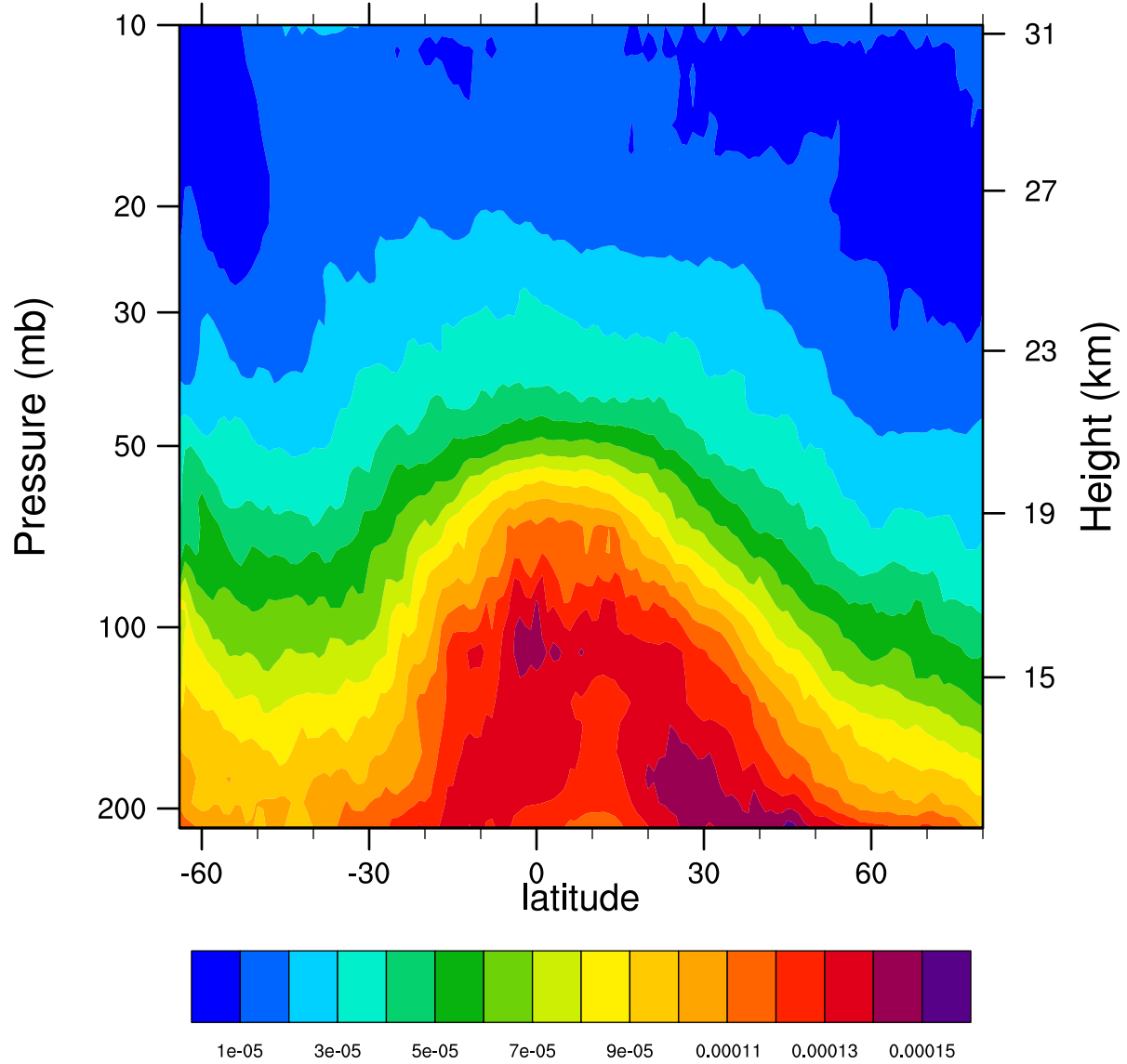
2006d235 12.1MicronExtinction_Combined ( \text{km}^{-1} )
