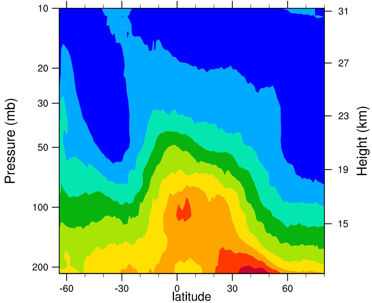
2005d180 12.1MicronExtinction_Combined (km -1 )
