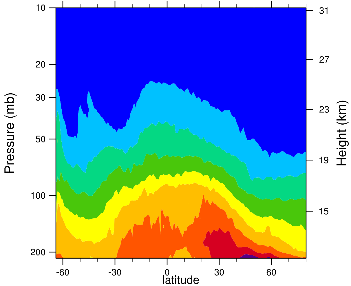
2007d207 12.1MicronExtinction_Combined (km -1 )
