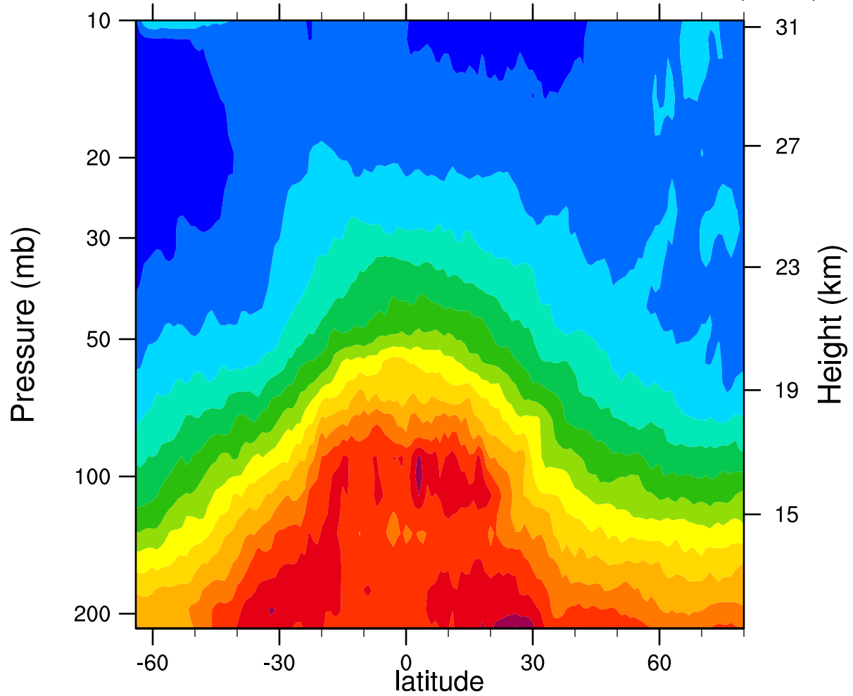
2005d354 12.1MicronExtinction_Combined (km -1 )
