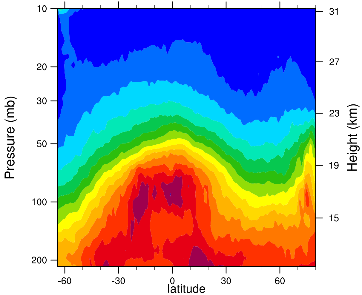
2007d031 12.1MicronExtinction_Combined ( \text{km}^{-1} )
