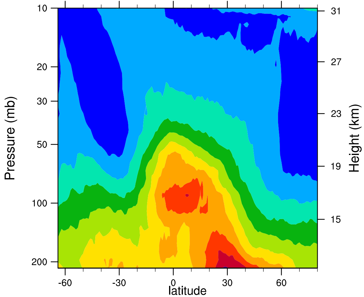
2005d144 12.1MicronExtinction_Combined (km -1 )
