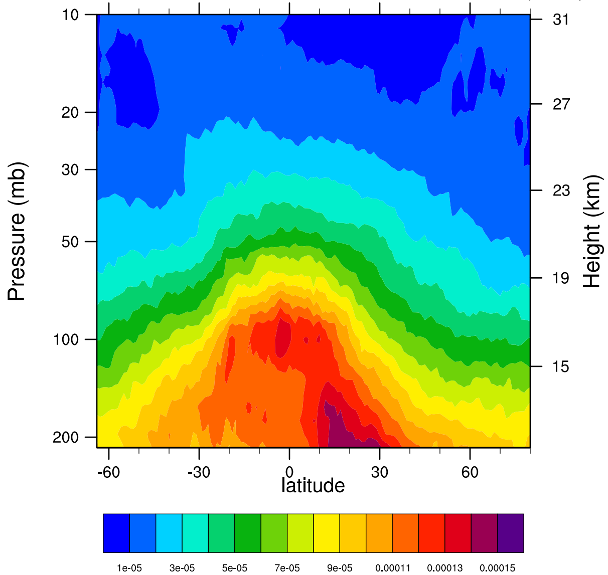
2006d082 12.1MicronExtinction_Combined ( \text{km}^{-1} )
