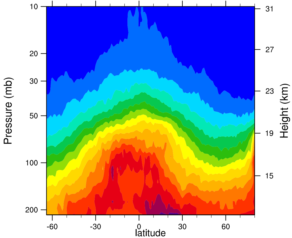
2007d047 12.1MicronExtinction_Combined (km -1 )
