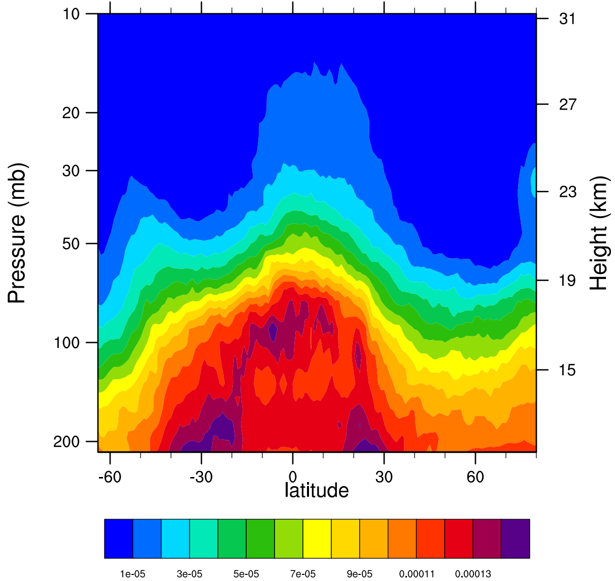
2006d344 12.1MicronExtinction_Combined ( \text{km}^{-1} )
