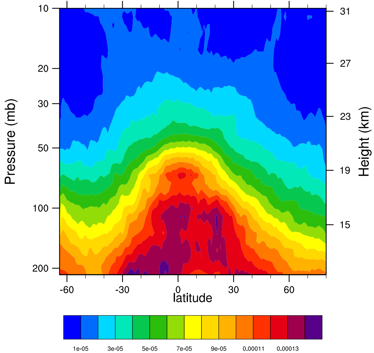
2006d276 12.1MicronExtinction_Combined ( \text{km}^{-1} )
