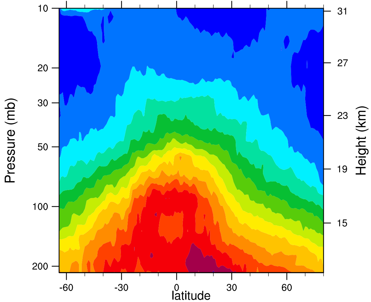
2006d036 12.1MicronExtinction_Combined ( \text{km}^{-1} )
