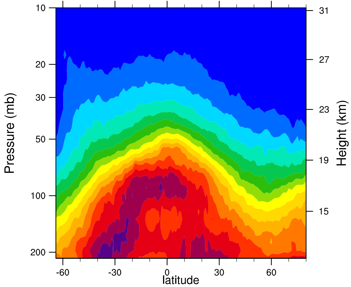
2007d003 12.1MicronExtinction_Combined ( \text{km}^{-1} )
