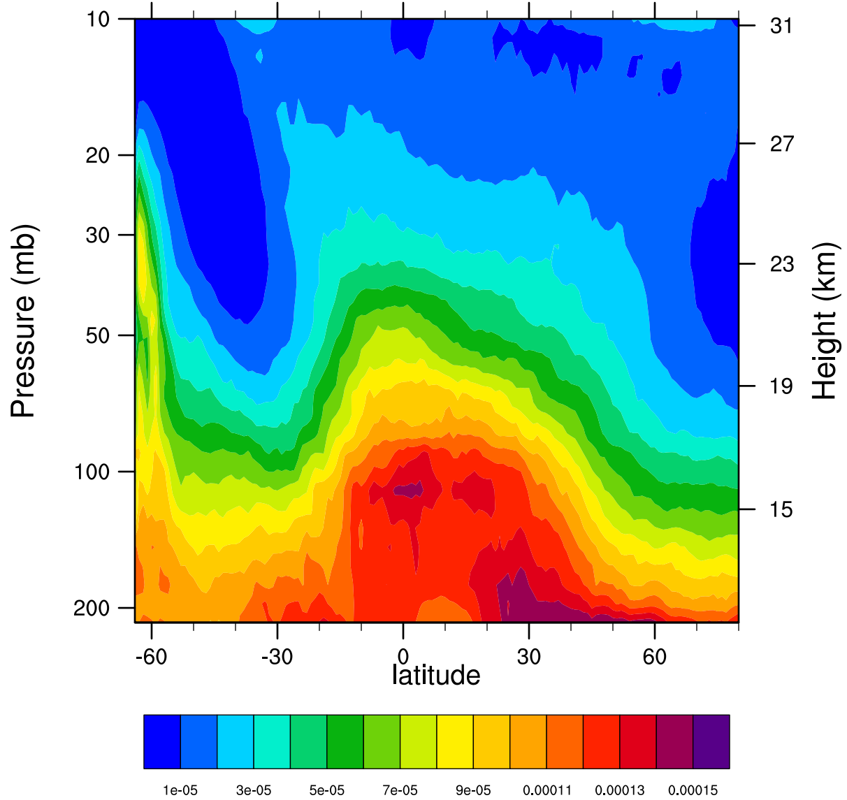
2005d209 12.1MicronExtinction_Combined (km -1 )
