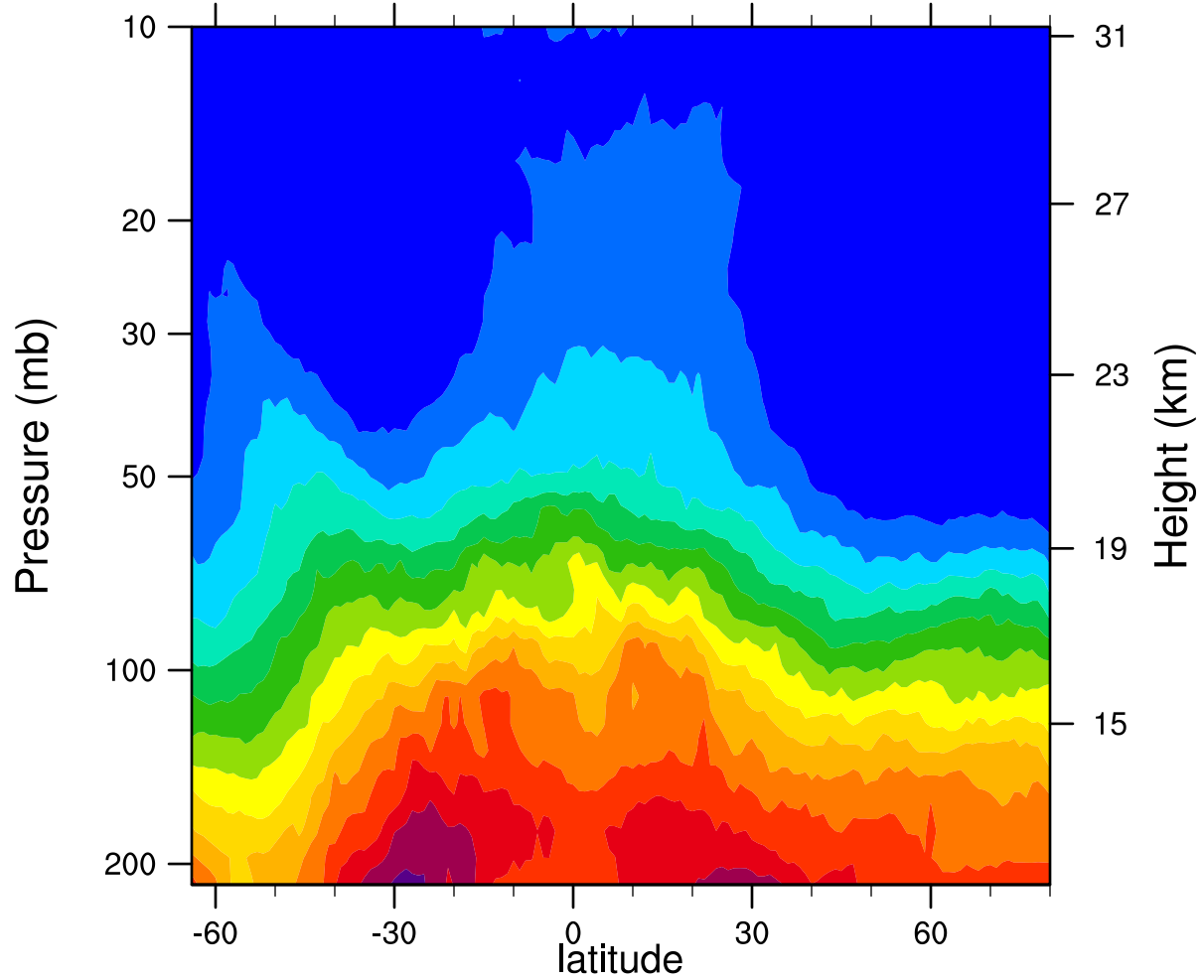
2007d322 12.1MicronExtinction_Combined (km -1 )
