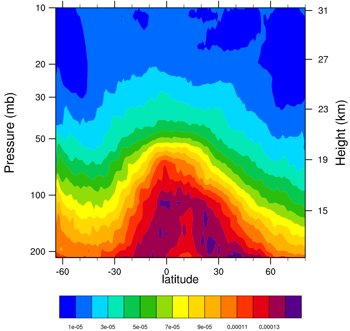
2006d247 12.1MicronExtinction_Combined ( \text{km}^{-1} )
