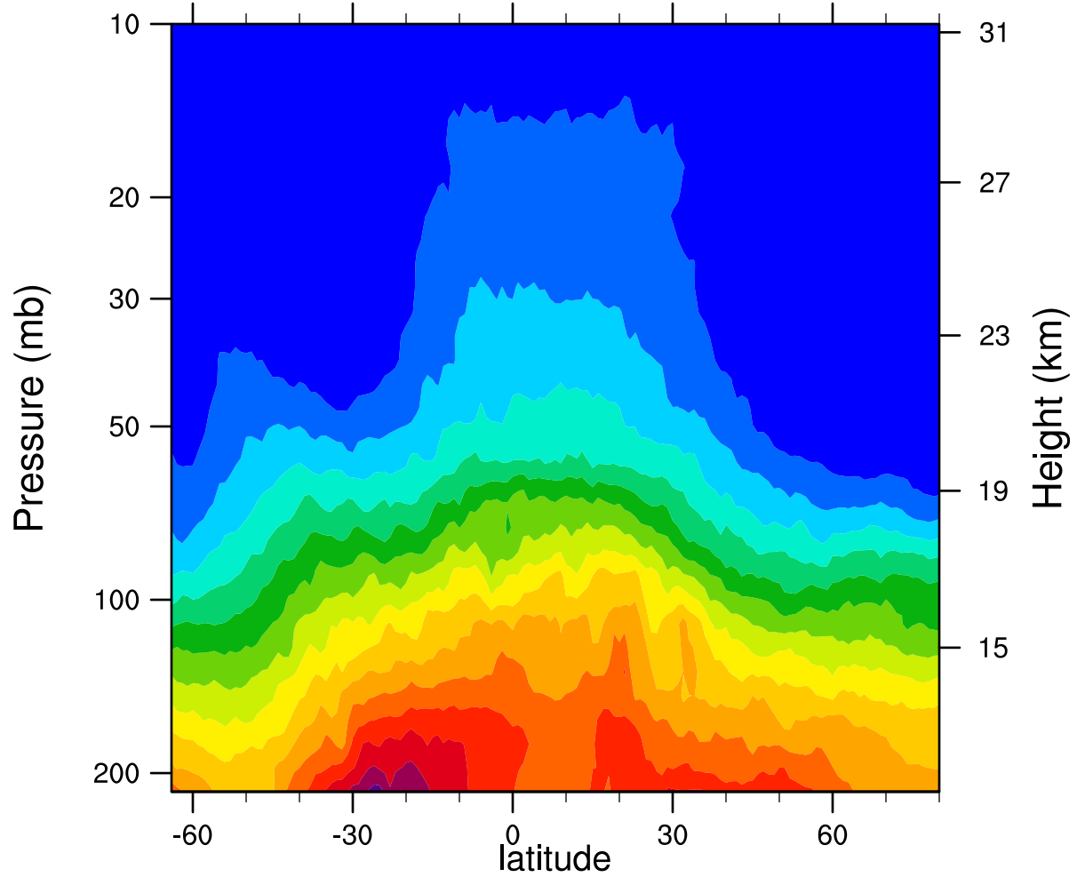
2007d293 12.1MicronExtinction_Combined (km -1 )
