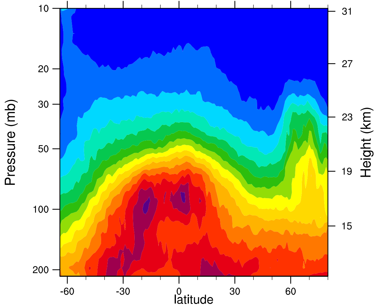
2007d026 12.1MicronExtinction_Combined ( \text{km}^{-1} )
