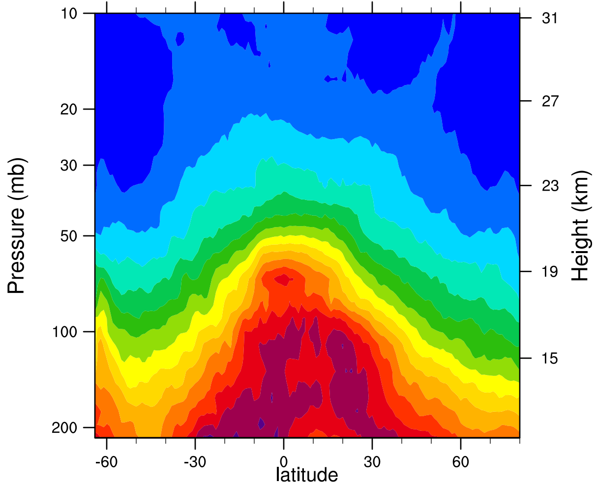
2006d271 12.1MicronExtinction_Combined (km -1 )
