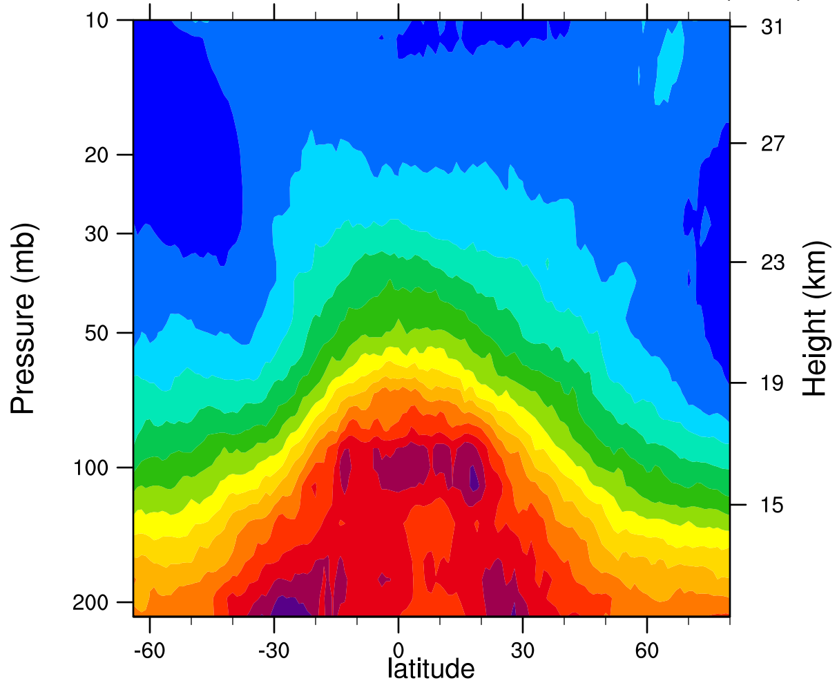
2005d307 12.1MicronExtinction_Combined (km -1 )
