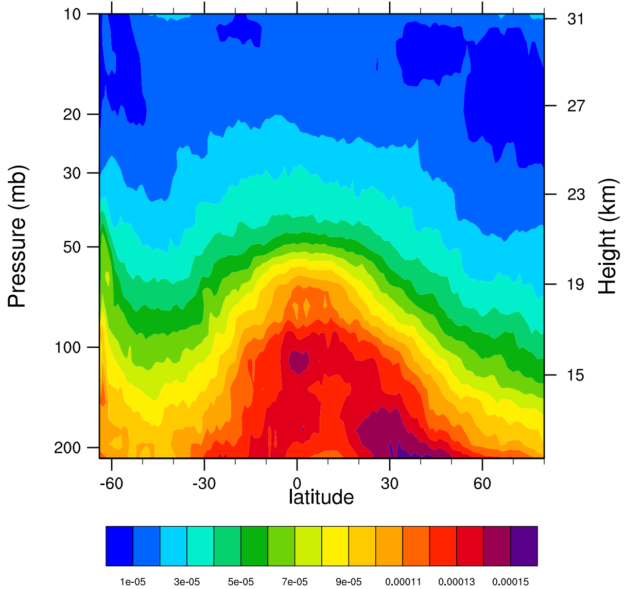
2006d231 12.1MicronExtinction_Combined (km -1 )
