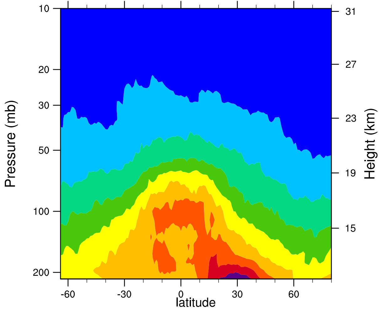
2006d109 12.1MicronExtinction_Combined (km -1 )
