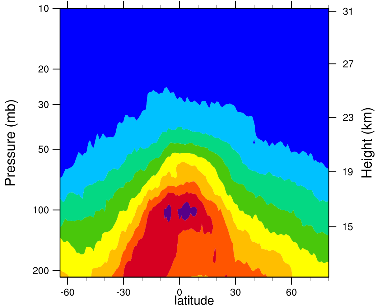
2006d303 12.1MicronExtinction_Combined (km -1 )
