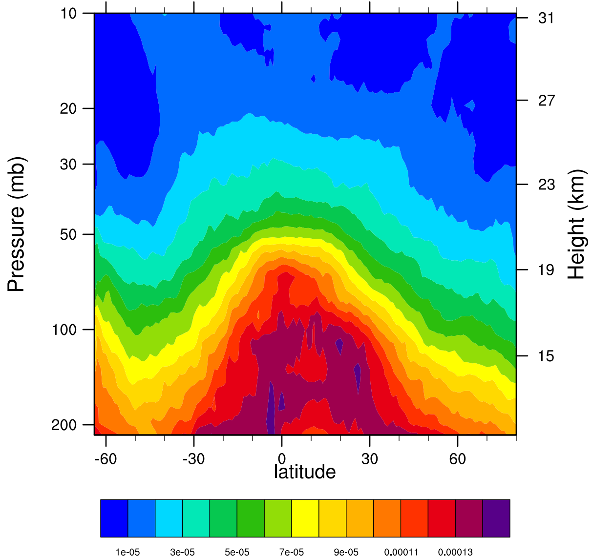
2006d262 12.1MicronExtinction_Combined (km -1 )
