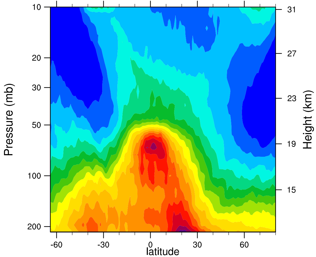
2005d079 12.1MicronExtinction_Combined (km -1 )
