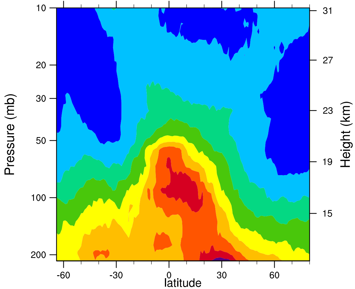
2005d110 12.1MicronExtinction_Combined (km -1 )
