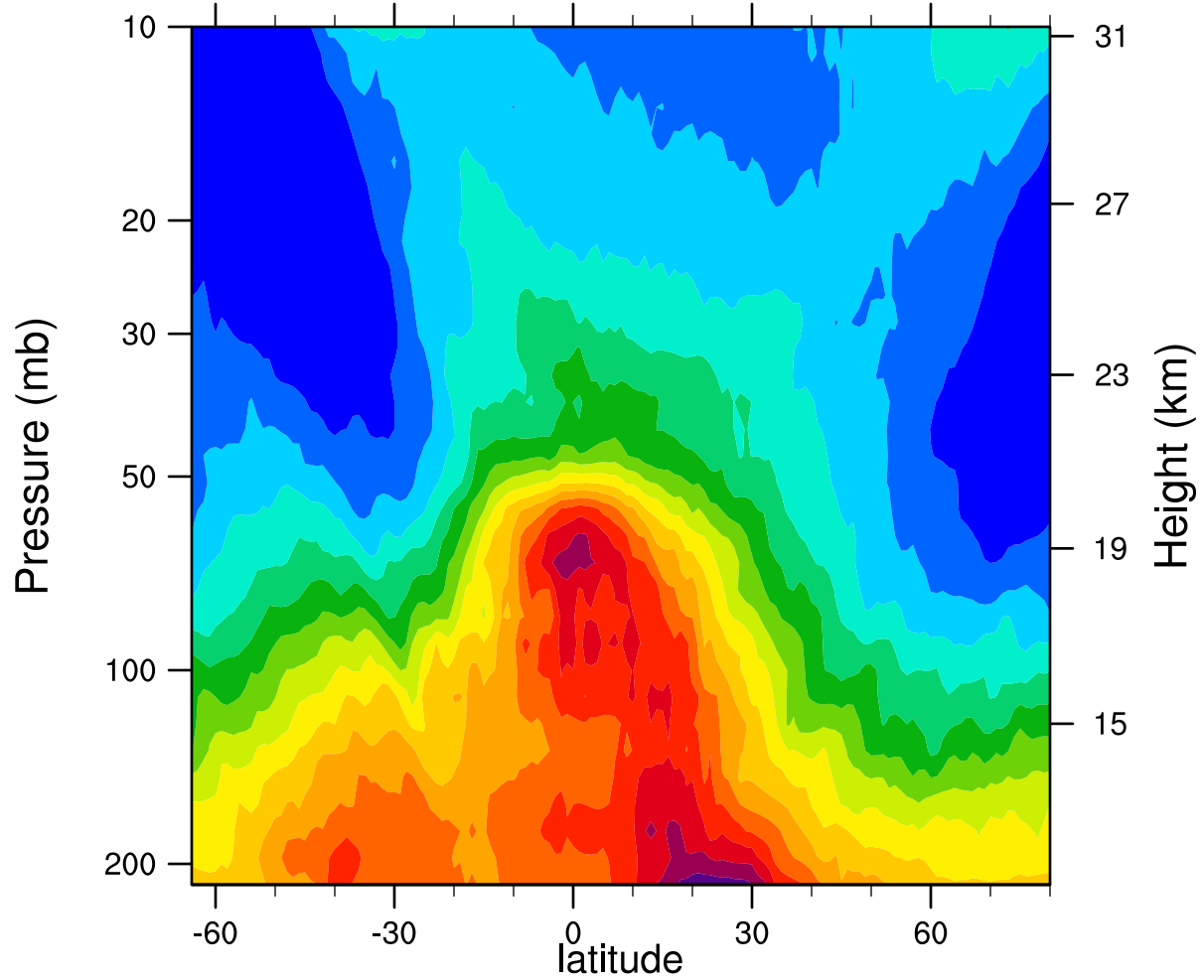
2005d087 12.1MicronExtinction_Combined (km -1 )
