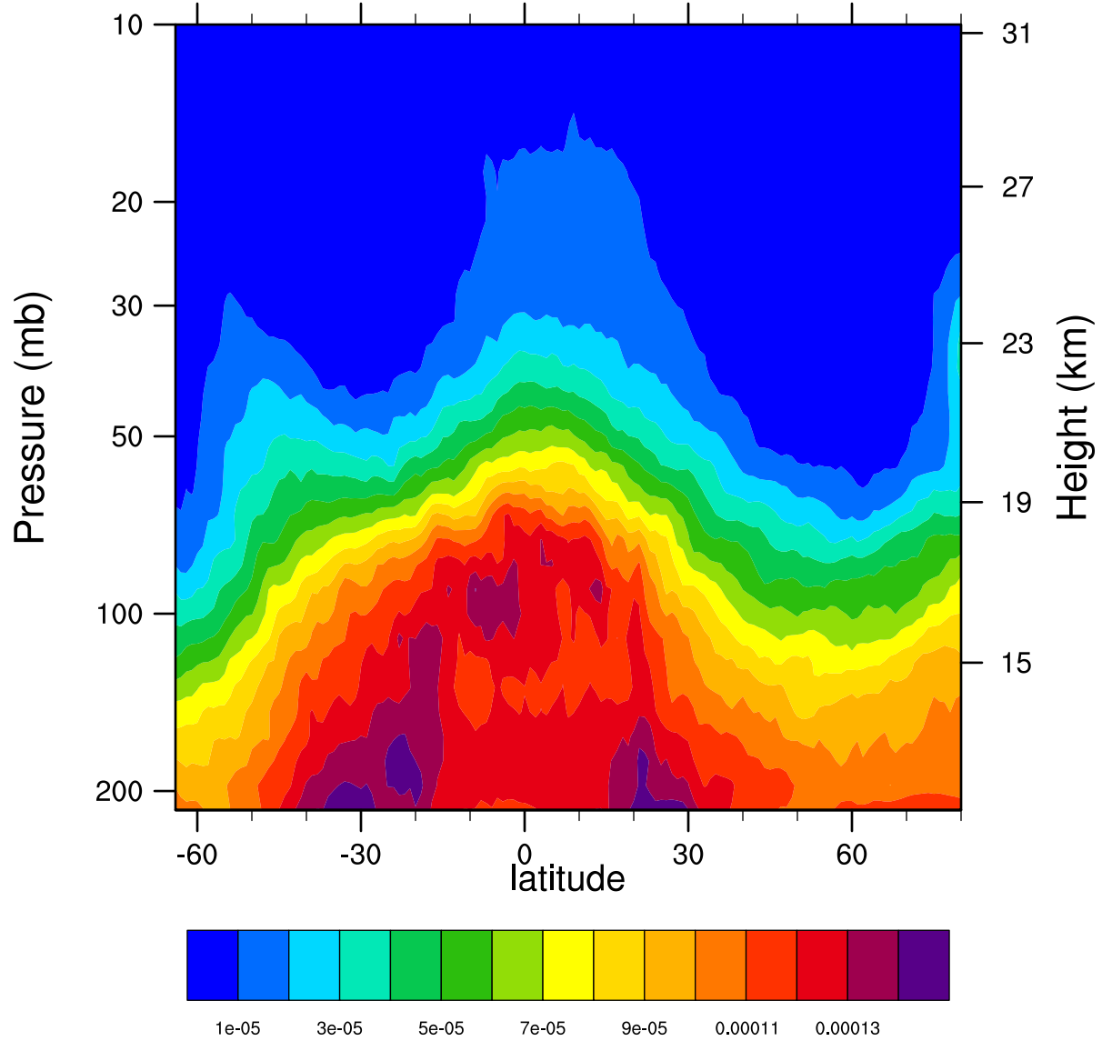
2006d349 12.1MicronExtinction_Combined ( \text{km}^{-1} )
