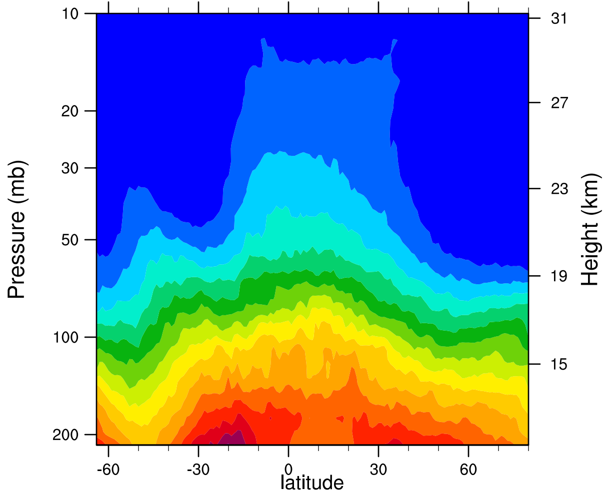
2007d274 12.1MicronExtinction_Combined (km -1 )
