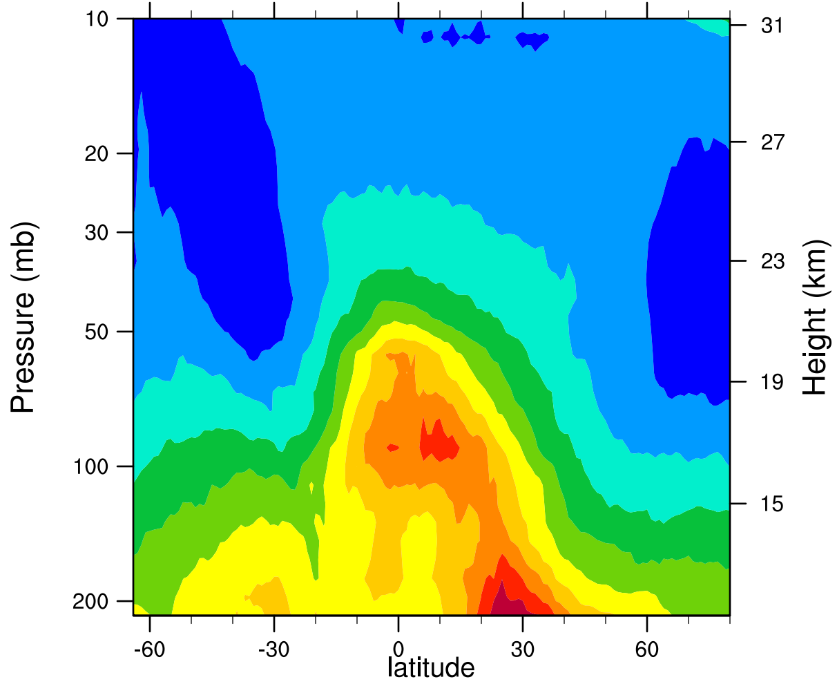
2005d129 12.1MicronExtinction_Combined ( \text{km}^{-1} )
