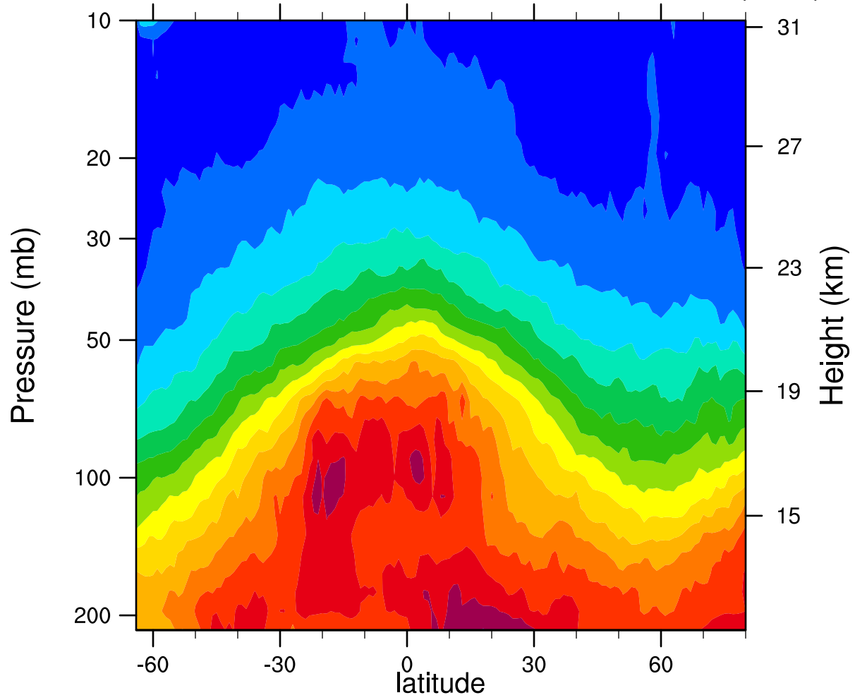
2007d038 12.1MicronExtinction_Combined ( \text{km}^{-1} )
