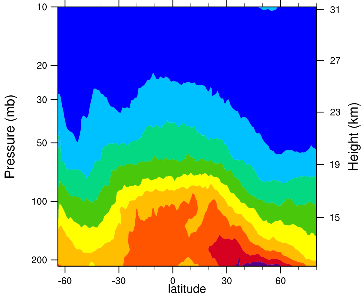
2007d200 12.1MicronExtinction_Combined (km -1 )
