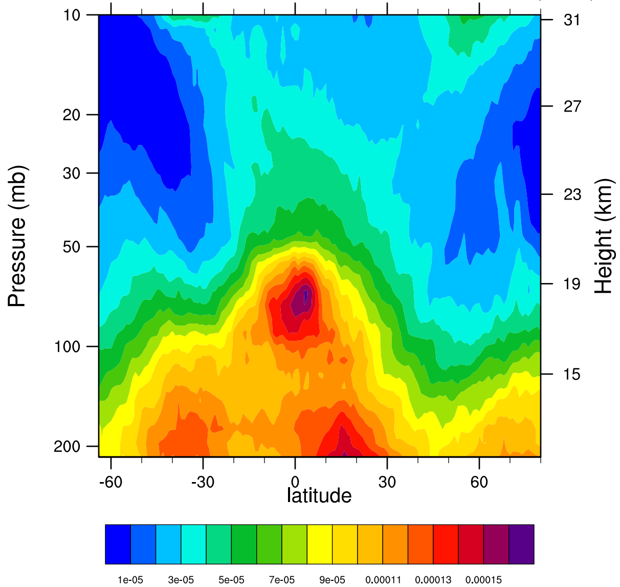
2005d051 12.1MicronExtinction_Combined (km -1 )
