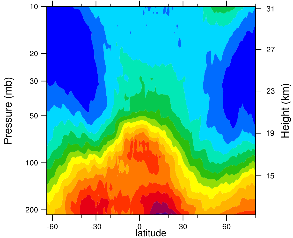
2005d037 12.1MicronExtinction_Combined (km -1 )
