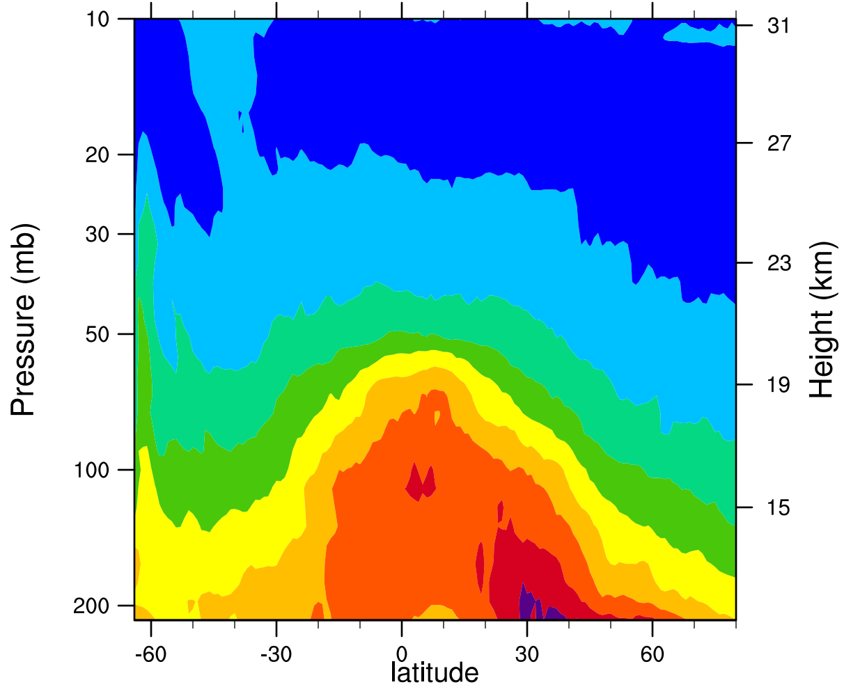
2006d201 12.1MicronExtinction_Combined ( \text{km}^{-1} )
