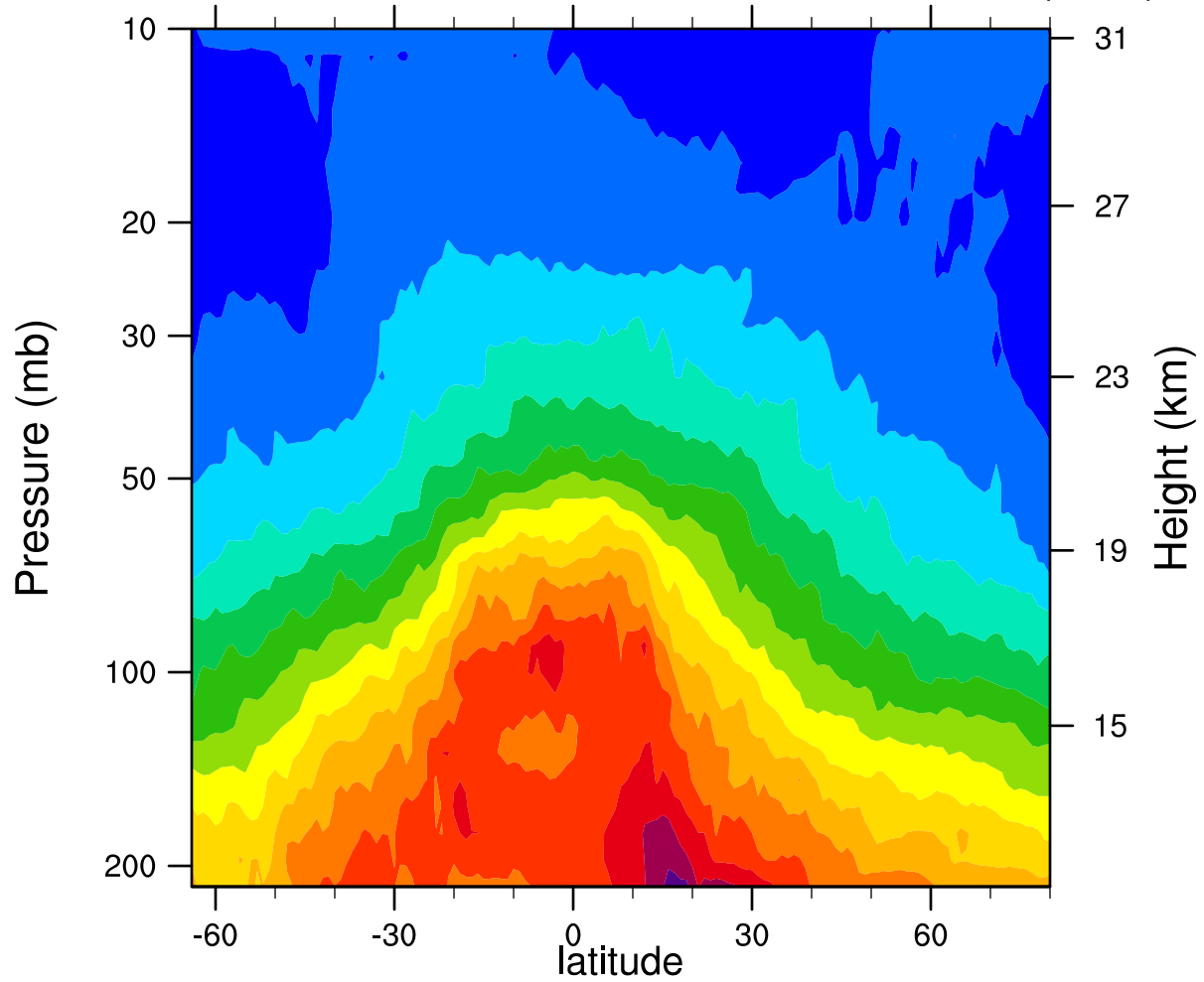
2006d049 12.1MicronExtinction_Combined (km -1 )
