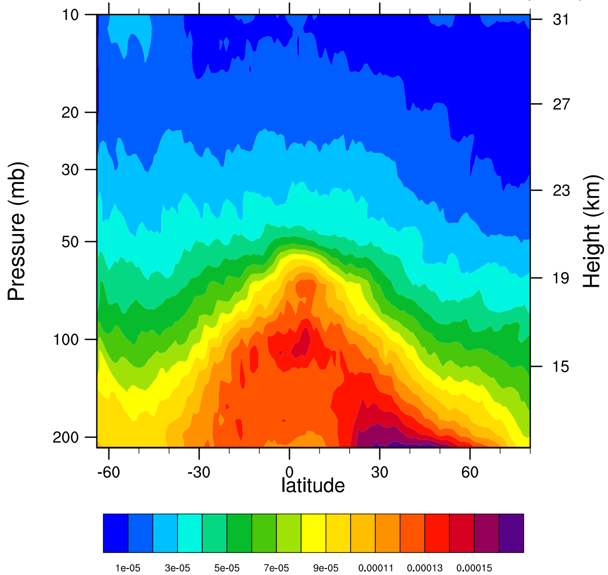
2006d173 12.1MicronExtinction_Combined ( \text{km}^{-1} )
