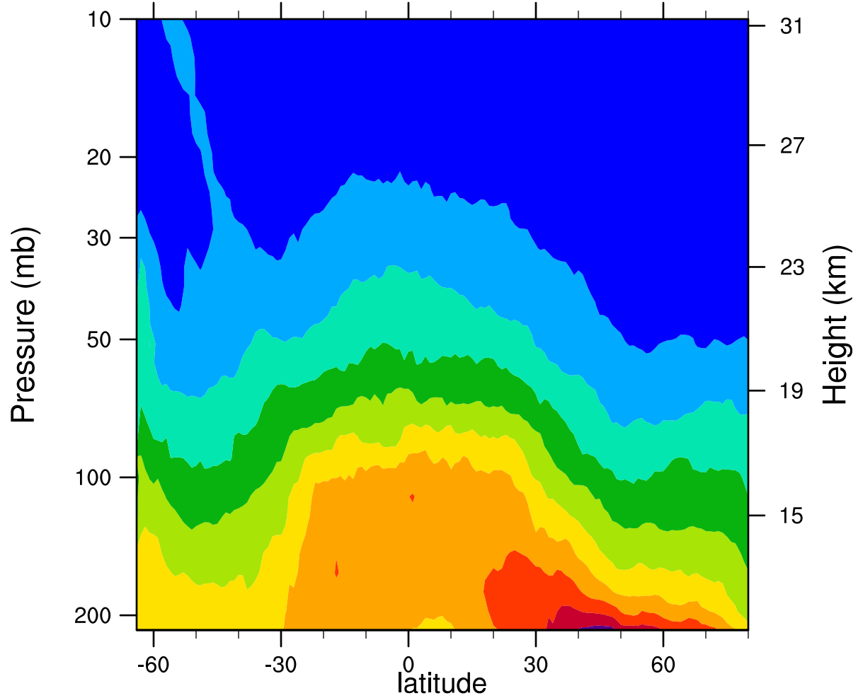
2007d178 12.1MicronExtinction_Combined (km -1 )
