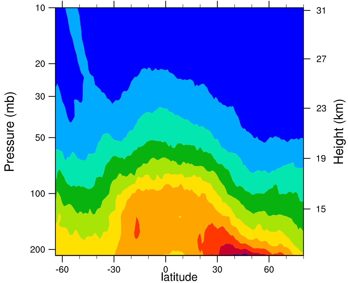
2007d173 12.1MicronExtinction_Combined ( \text{km}^{-1} )
