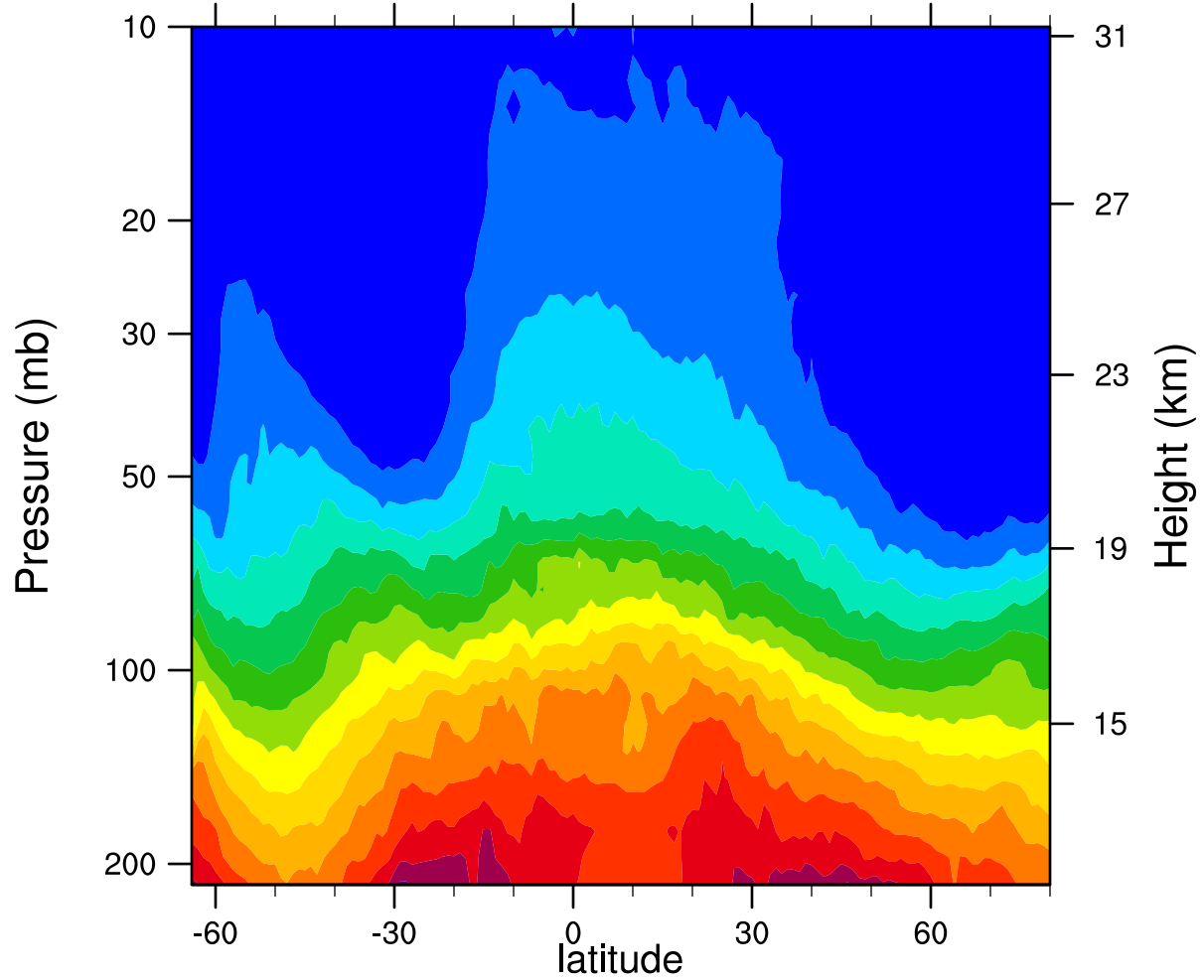
2007d261 12.1MicronExtinction_Combined (km -1 )
