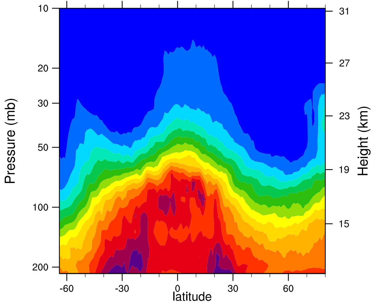
2006d348 12.1MicronExtinction_Combined (km -1 )
