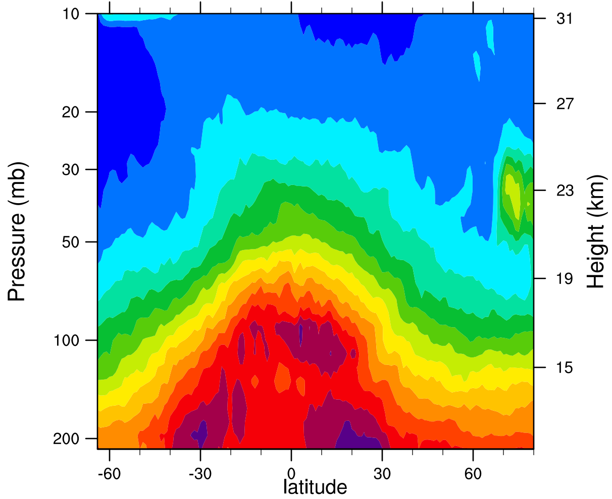
2005d361 12.1MicronExtinction_Combined (km -1 )
