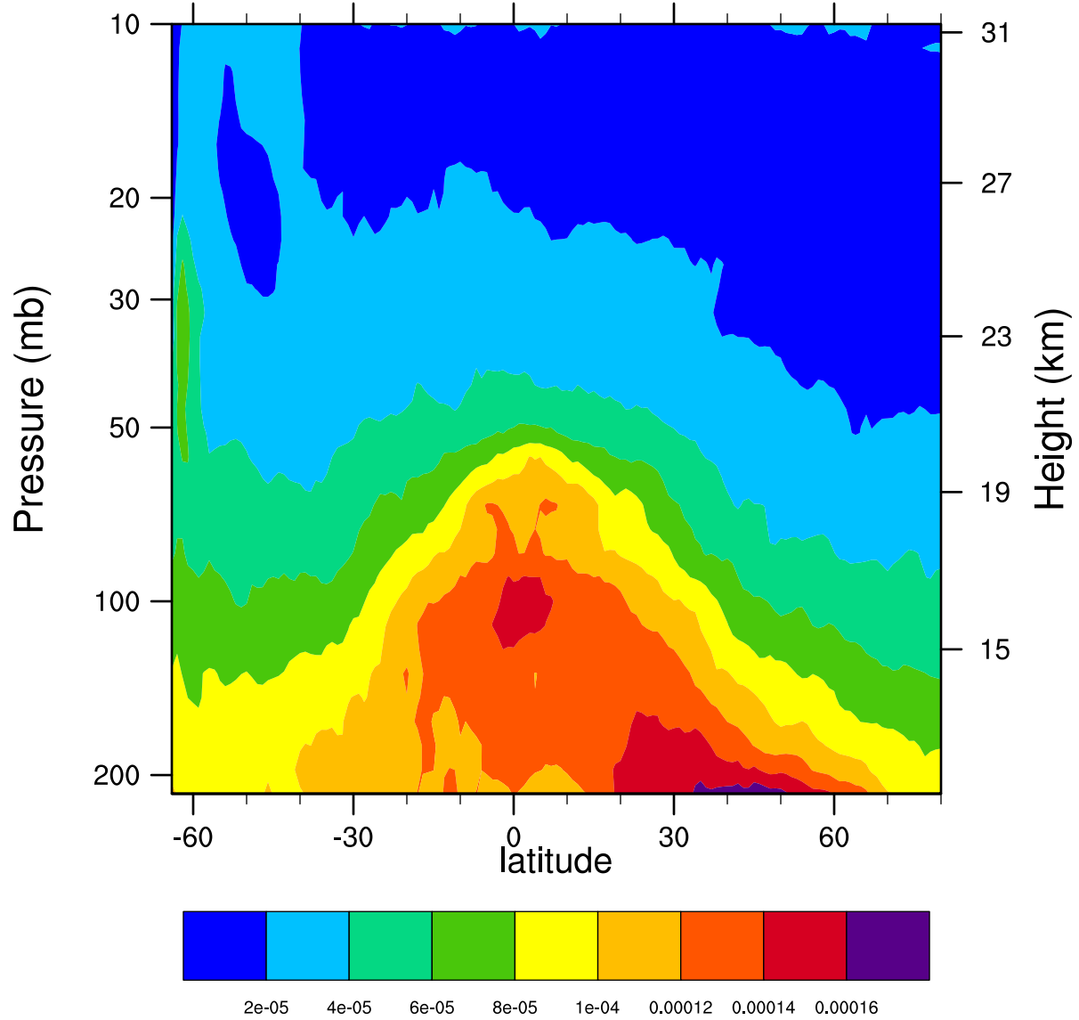
2006d179 12.1MicronExtinction_Combined (km -1 )
