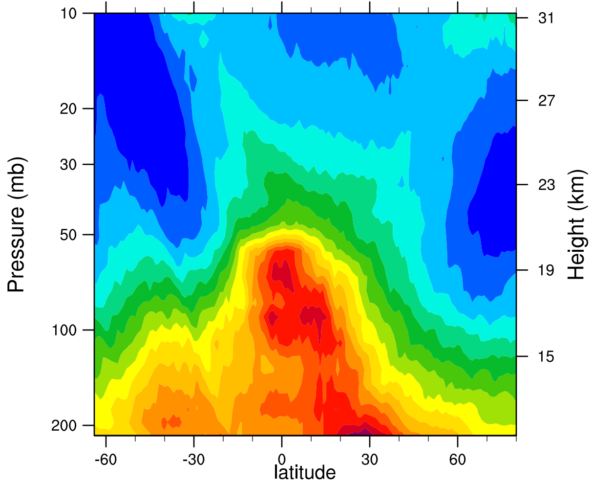
2005d100 12.1MicronExtinction_Combined (km -1 )
