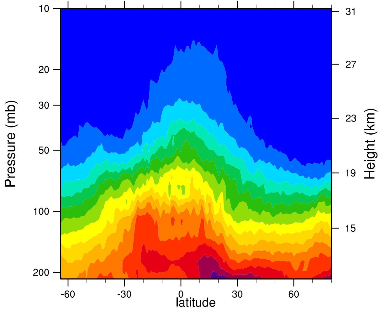
2007d078 12.1MicronExtinction_Combined (km -1 )
