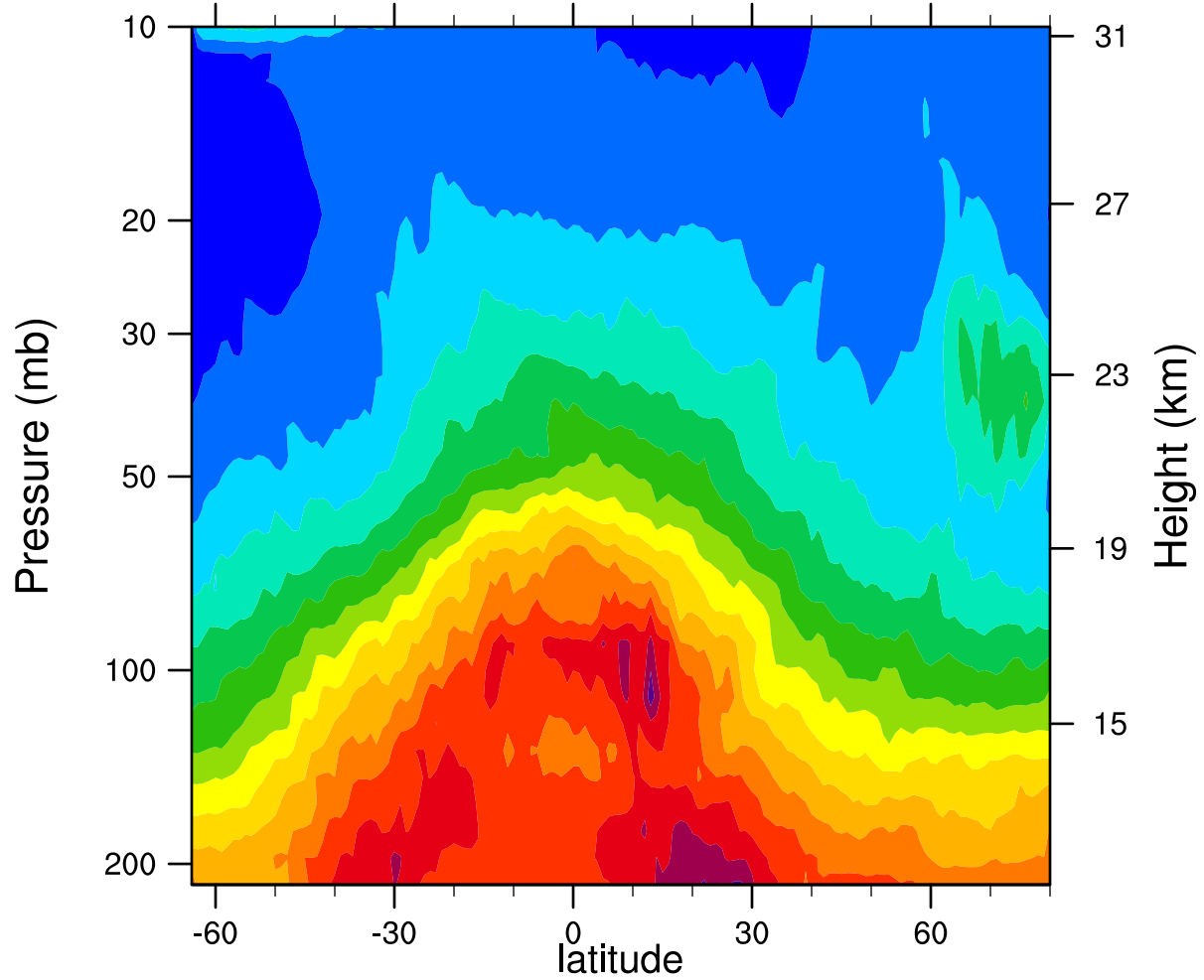
2006d002 12.1MicronExtinction_Combined (km -1 )
