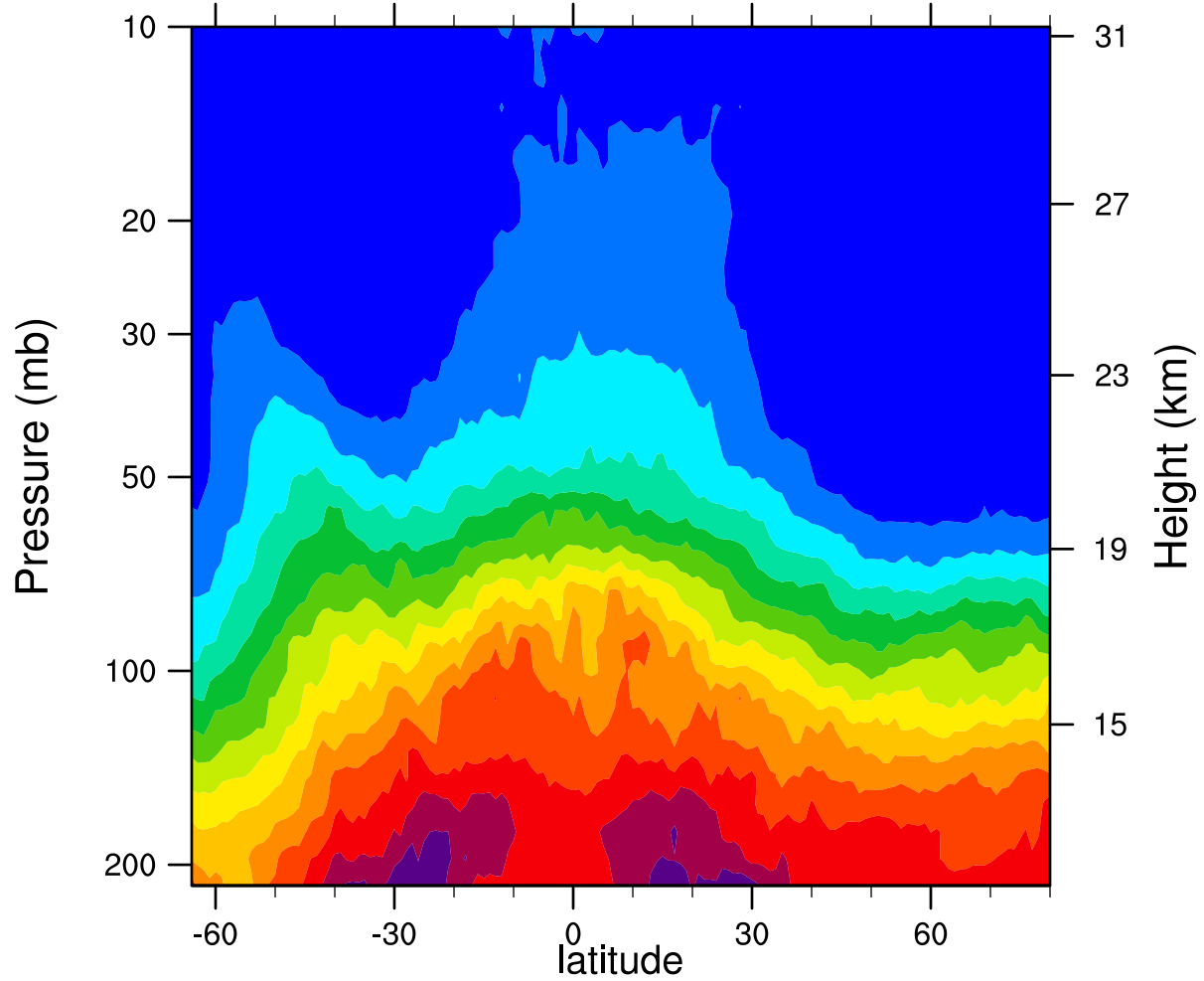
2007d333 12.1MicronExtinction_Combined ( \text{km}^{-1} )
