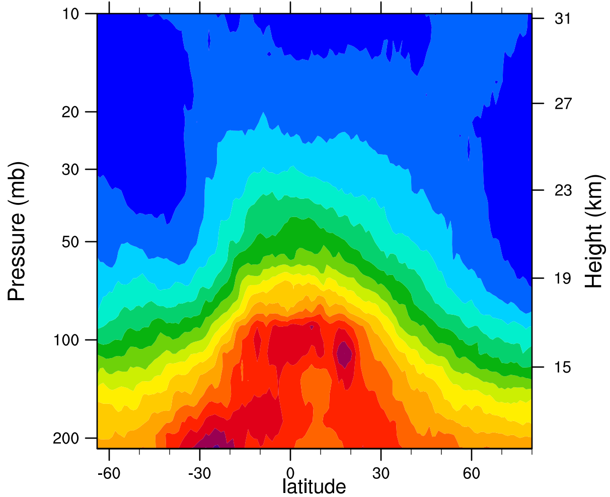
2005d297 12.1MicronExtinction_Combined (km -1 )
