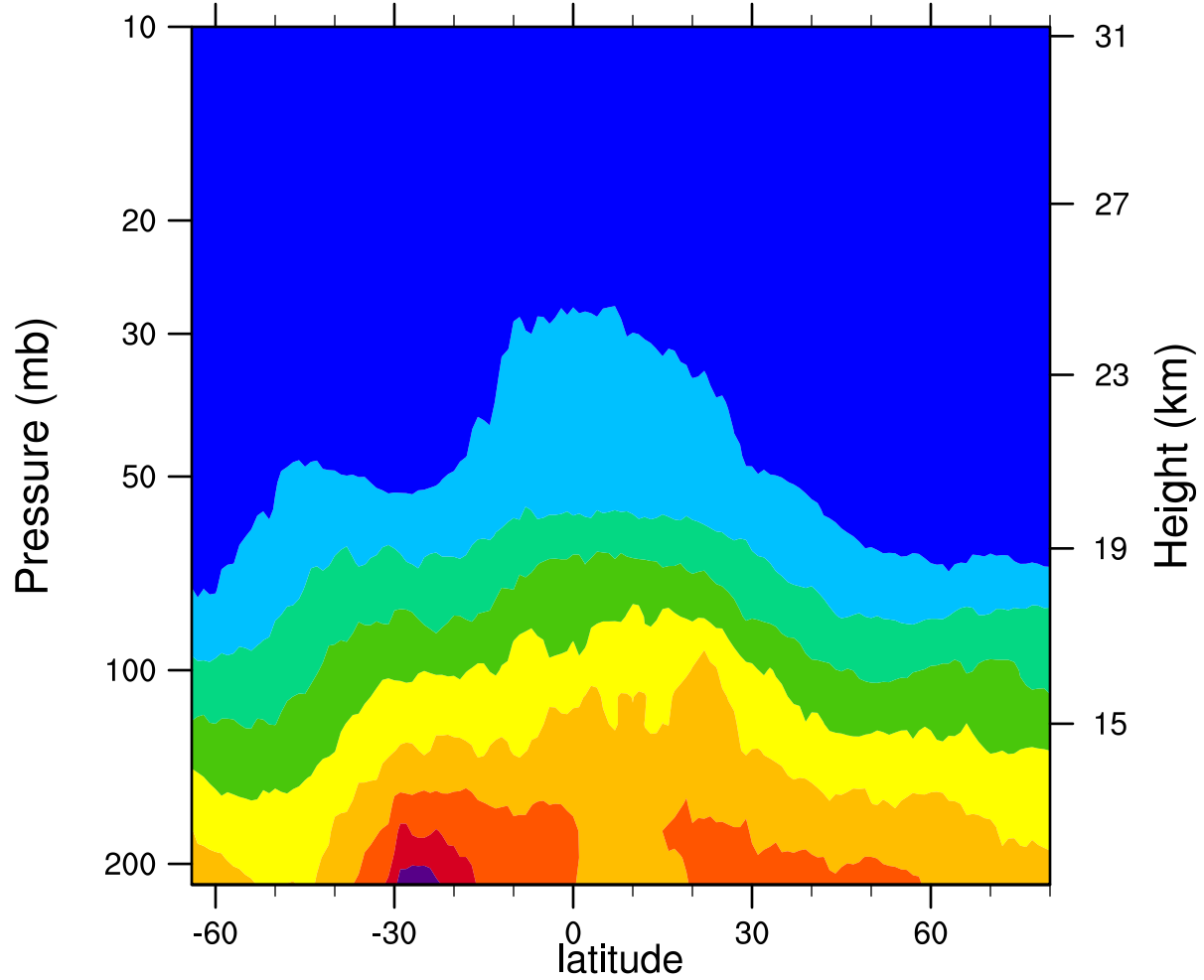
2007d284 12.1MicronExtinction_Combined (km -1 )
