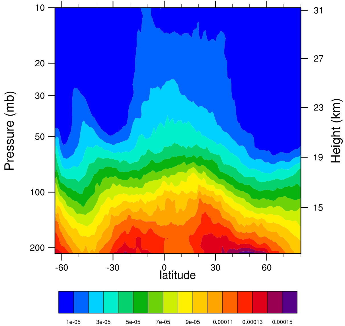
2007d244 12.1MicronExtinction_Combined ( \text{km}^{-1} )
