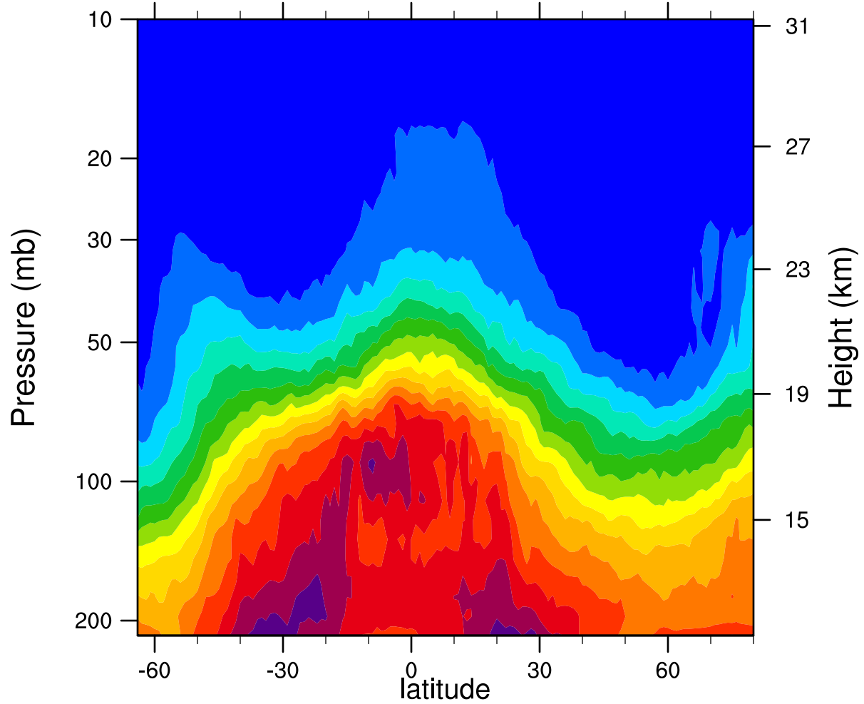
2006d351 12.1MicronExtinction_Combined ( \text{km}^{-1} )
