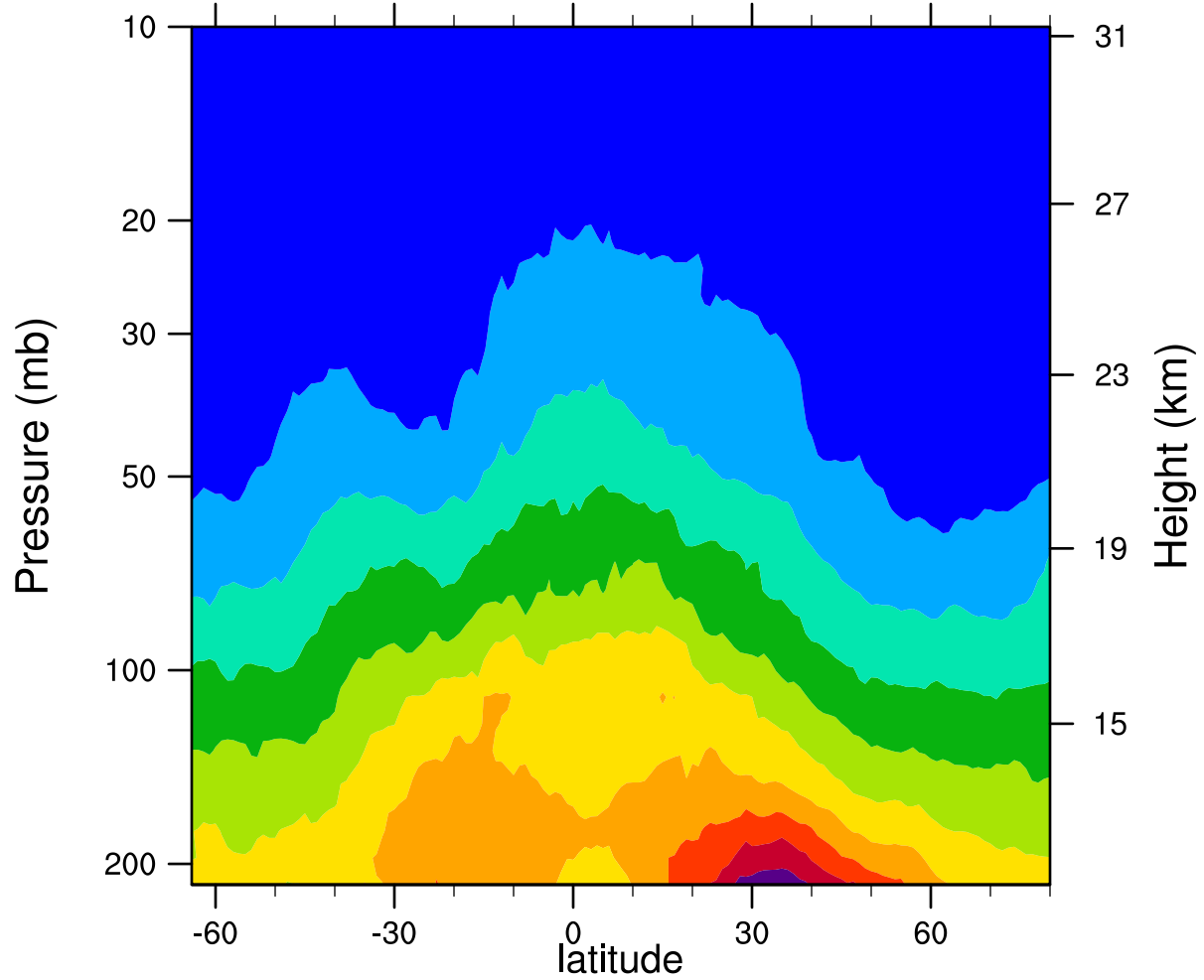
2007d133 12.1MicronExtinction_Combined (km -1 )
