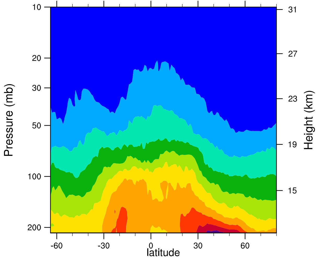
2007d162 12.1MicronExtinction_Combined (km -1 )
