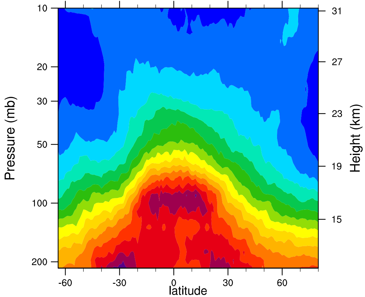
2005d315 12.1MicronExtinction_Combined (km -1 )
