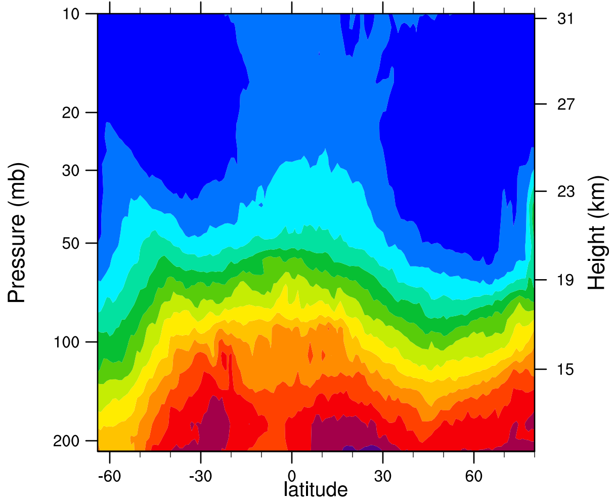
2007d364 12.1MicronExtinction_Combined (km -1 )
