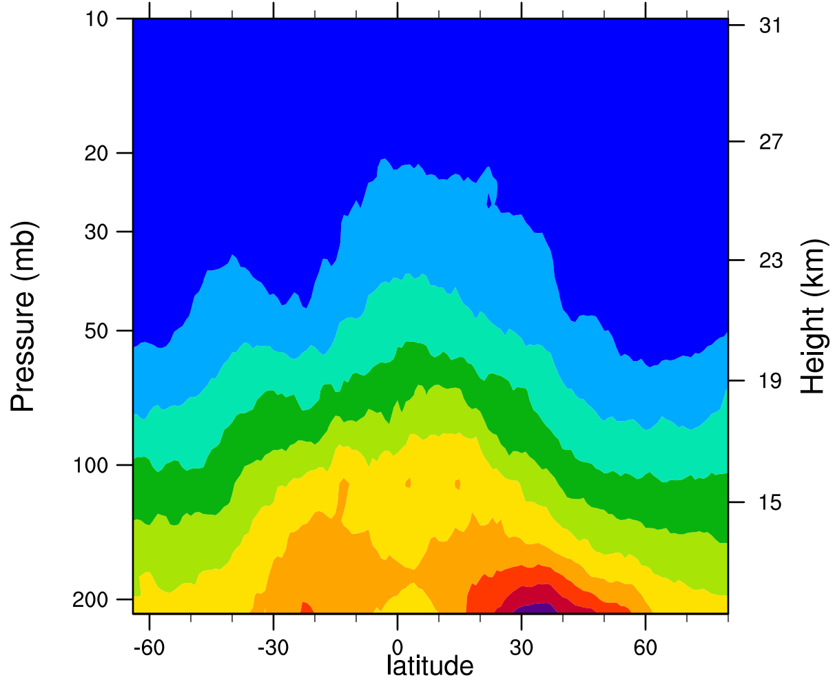
2007d135 12.1MicronExtinction_Combined (km -1 )
