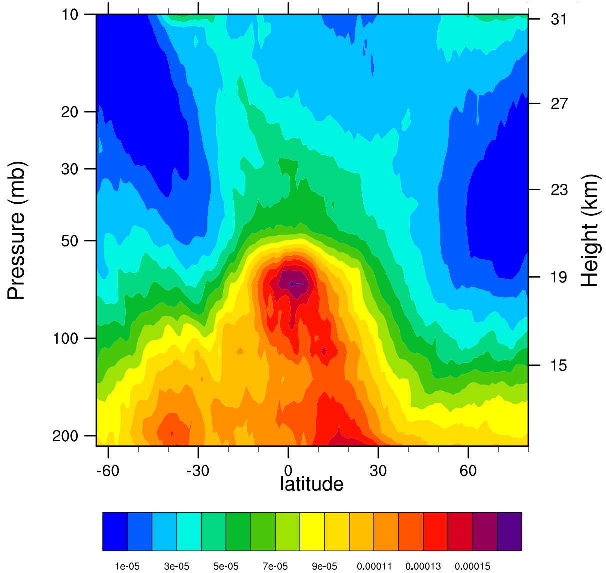
2005d073 12.1MicronExtinction_Combined (km -1 )
