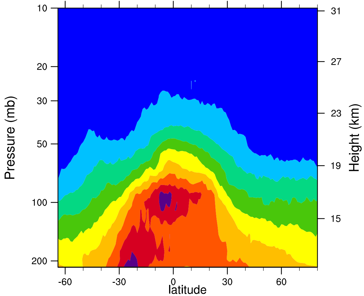
2006d314 12.1MicronExtinction_Combined (km -1 )
