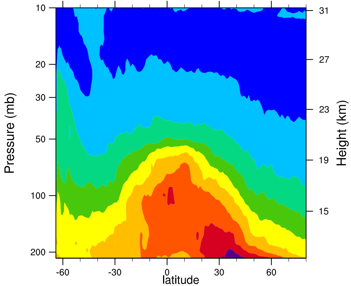
2006d193 12.1MicronExtinction_Combined (km -1 )
