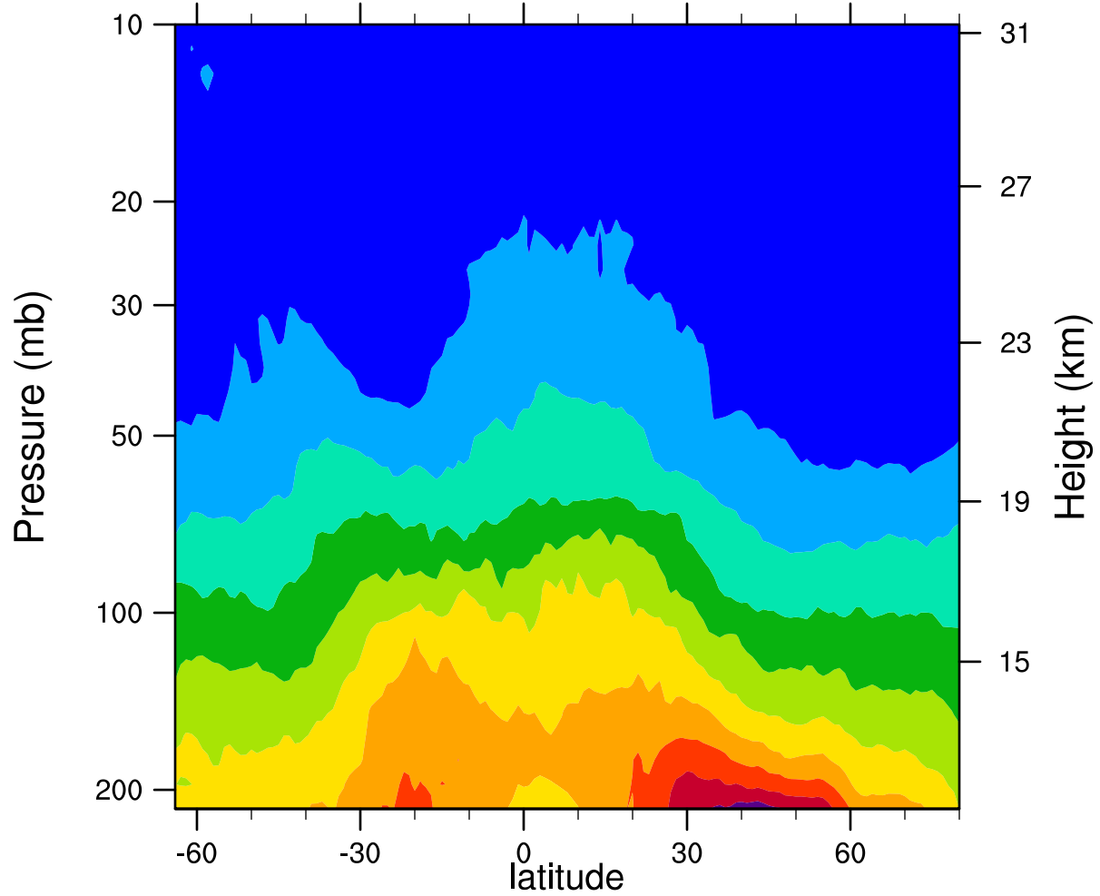
2007d152 12.1MicronExtinction_Combined (km -1 )
