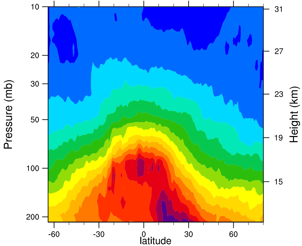
2006d080 12.1MicronExtinction_Combined ( \text{km}^{-1} )
