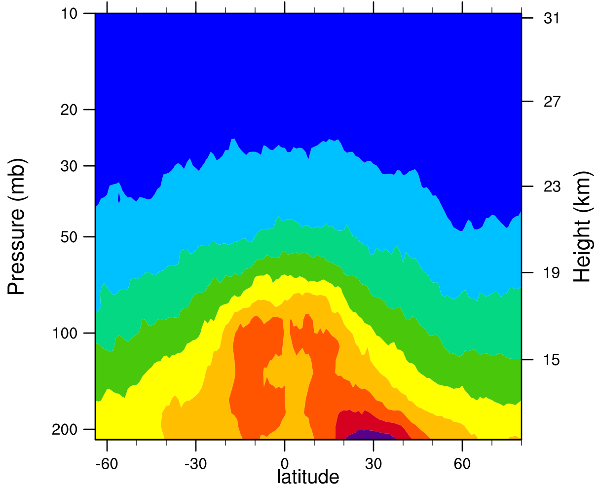
2006d120 12.1MicronExtinction_Combined (km -1 )
