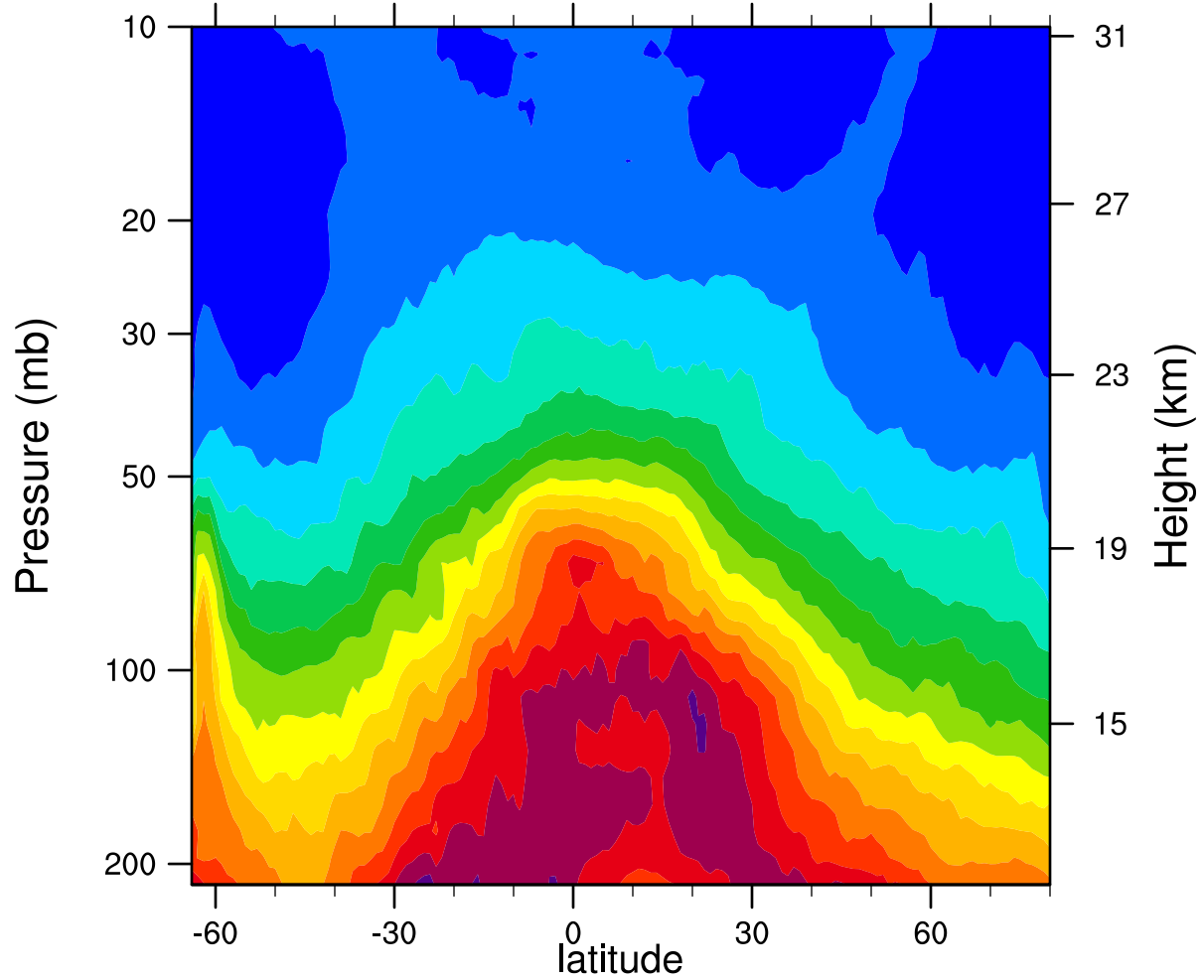
2006d268 12.1MicronExtinction_Combined (km -1 )
