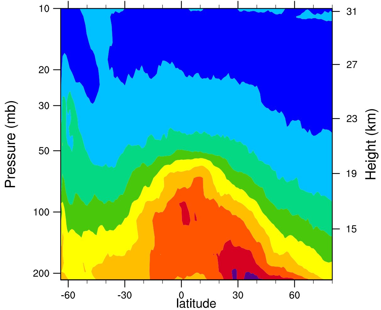
2006d196 12.1MicronExtinction_Combined (km -1 )
