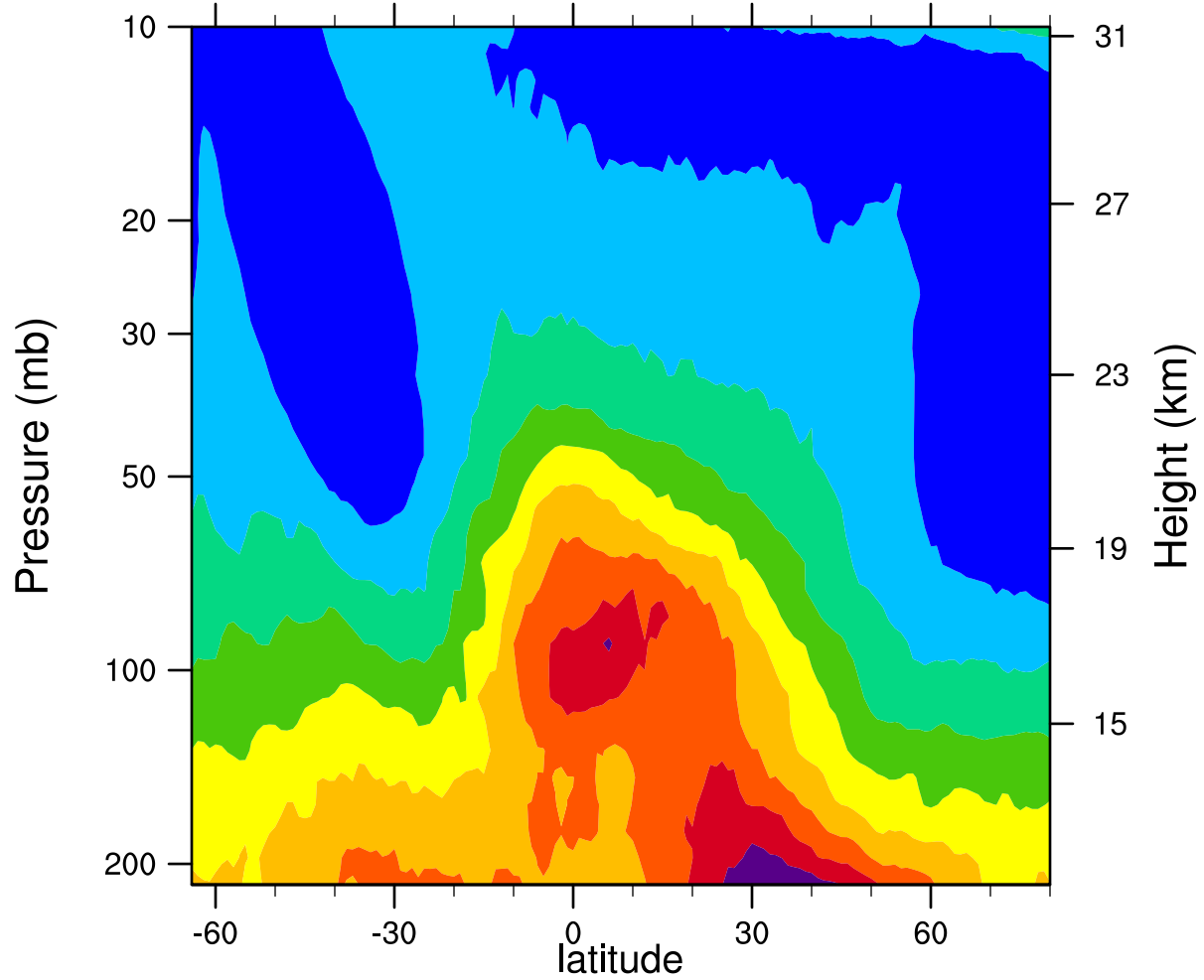
2005d155 12.1MicronExtinction_Combined (km -1 )
