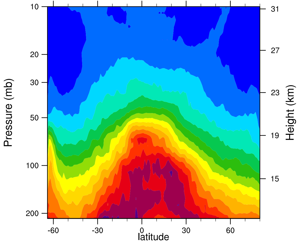
2006d269 12.1MicronExtinction_Combined (km -1 )
