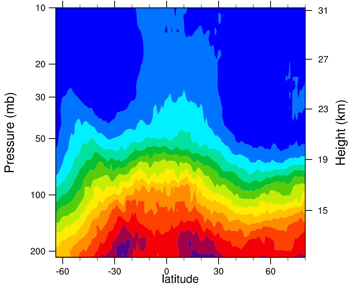
2007d349 12.1MicronExtinction_Combined (km -1 )
