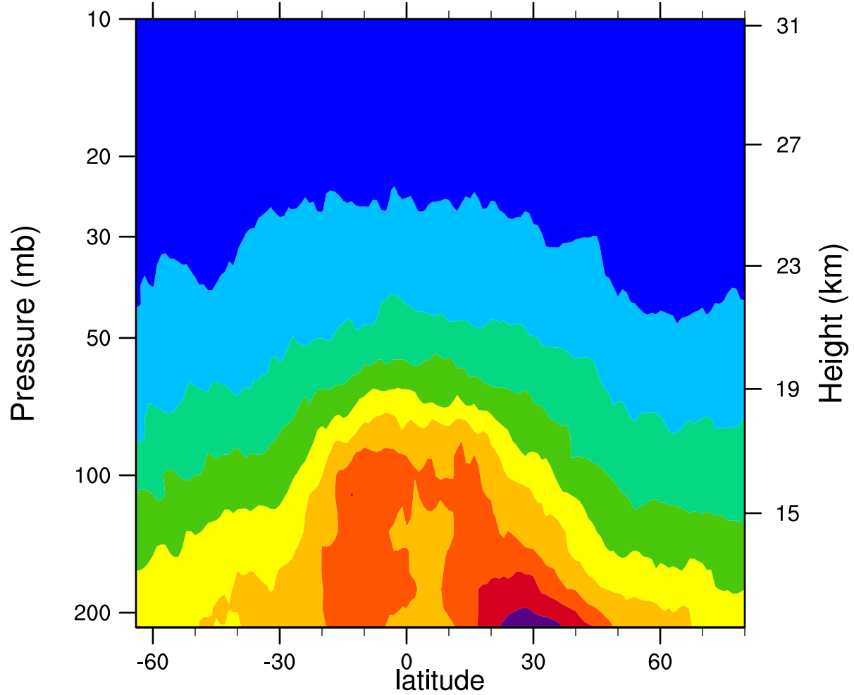
2006d128 12.1MicronExtinction_Combined (km -1 )
