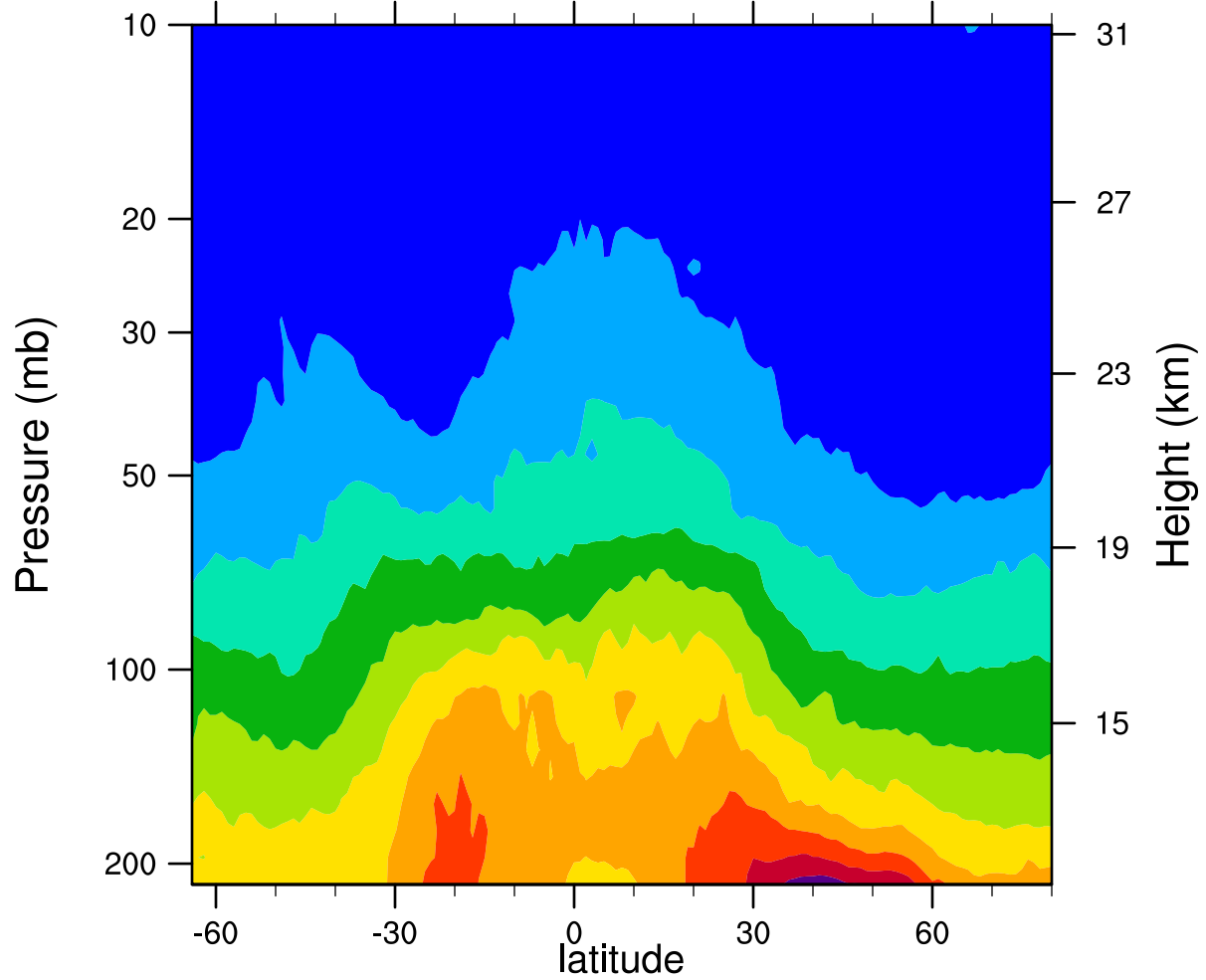
2007d160 12.1MicronExtinction_Combined (km -1 )
