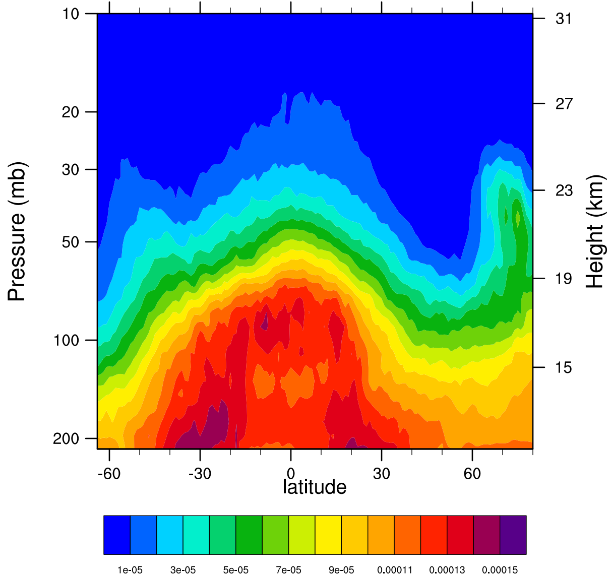
2006d354 12.1MicronExtinction_Combined (km -1 )
