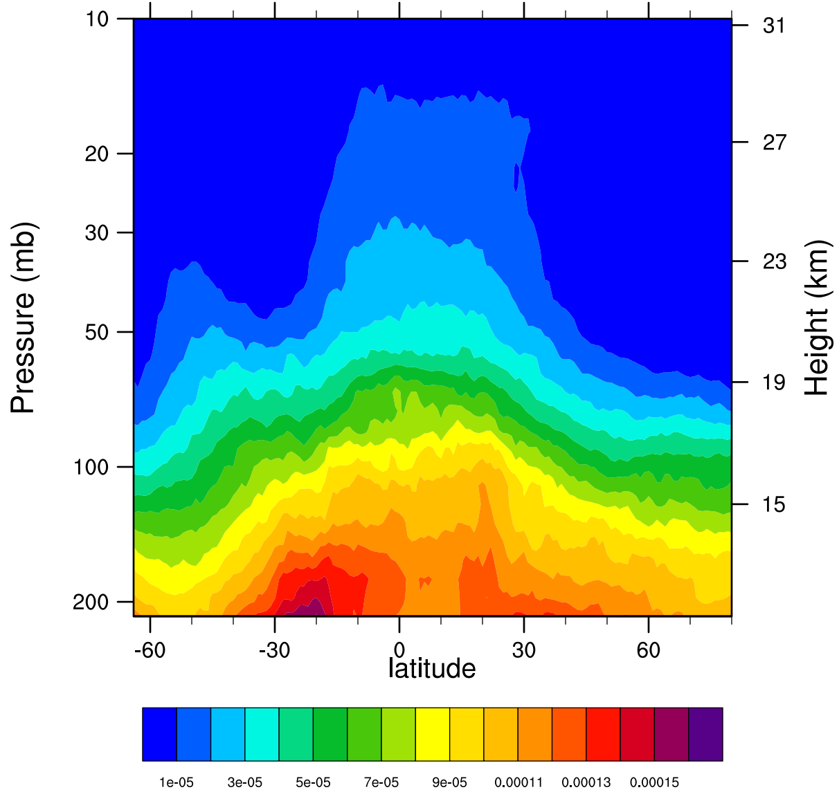
2007d300 12.1MicronExtinction_Combined (km -1 )
