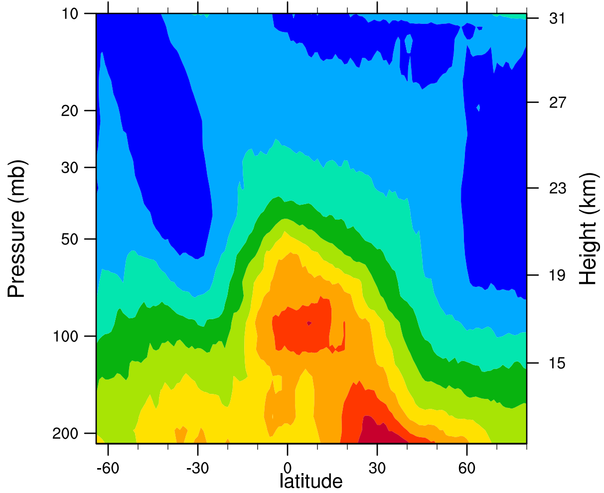
2005d145 12.1MicronExtinction_Combined (km -1 )
