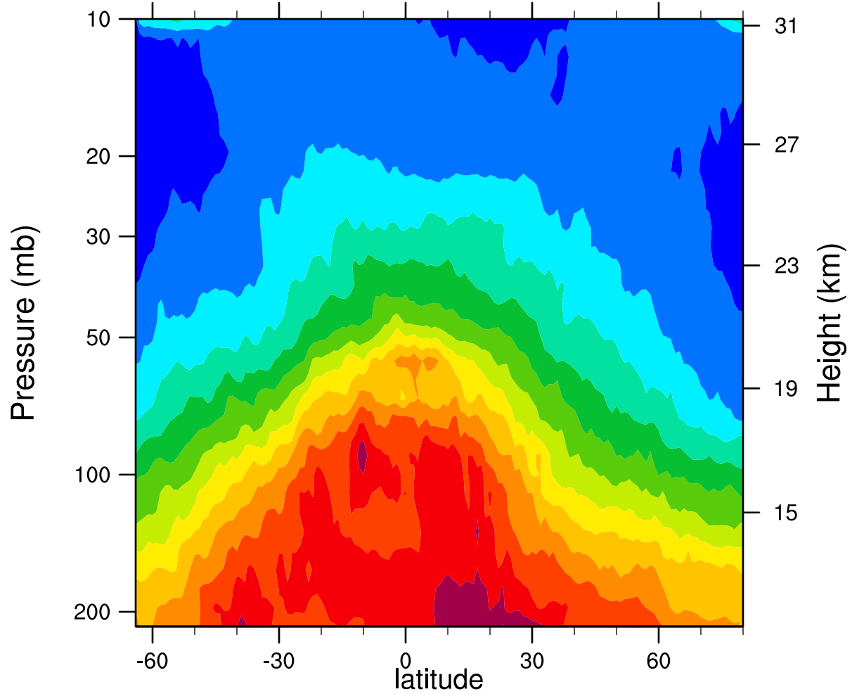
2006d025 12.1MicronExtinction_Combined (km -1 )
