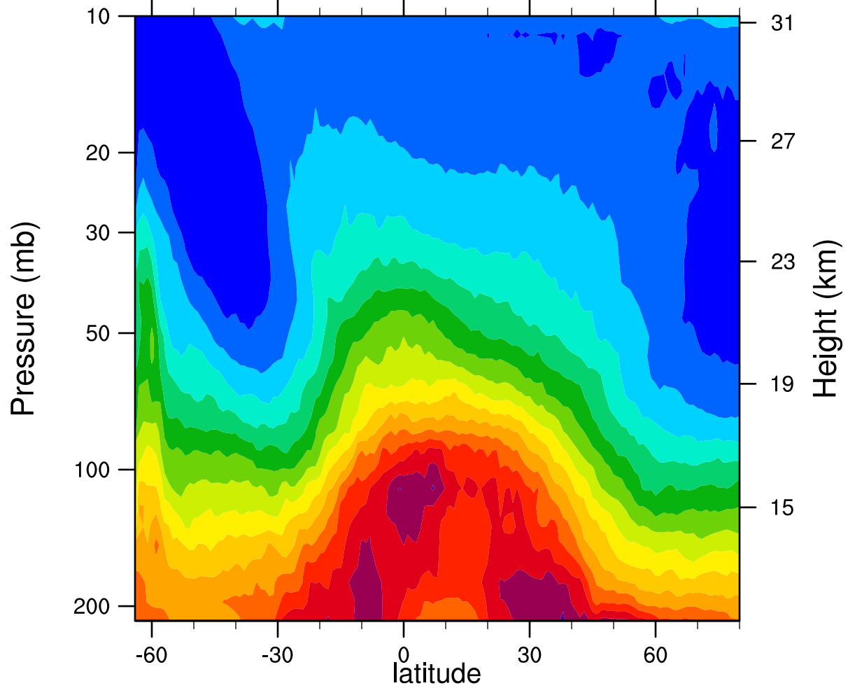
2005d230 12.1MicronExtinction_Combined (km -1 )
