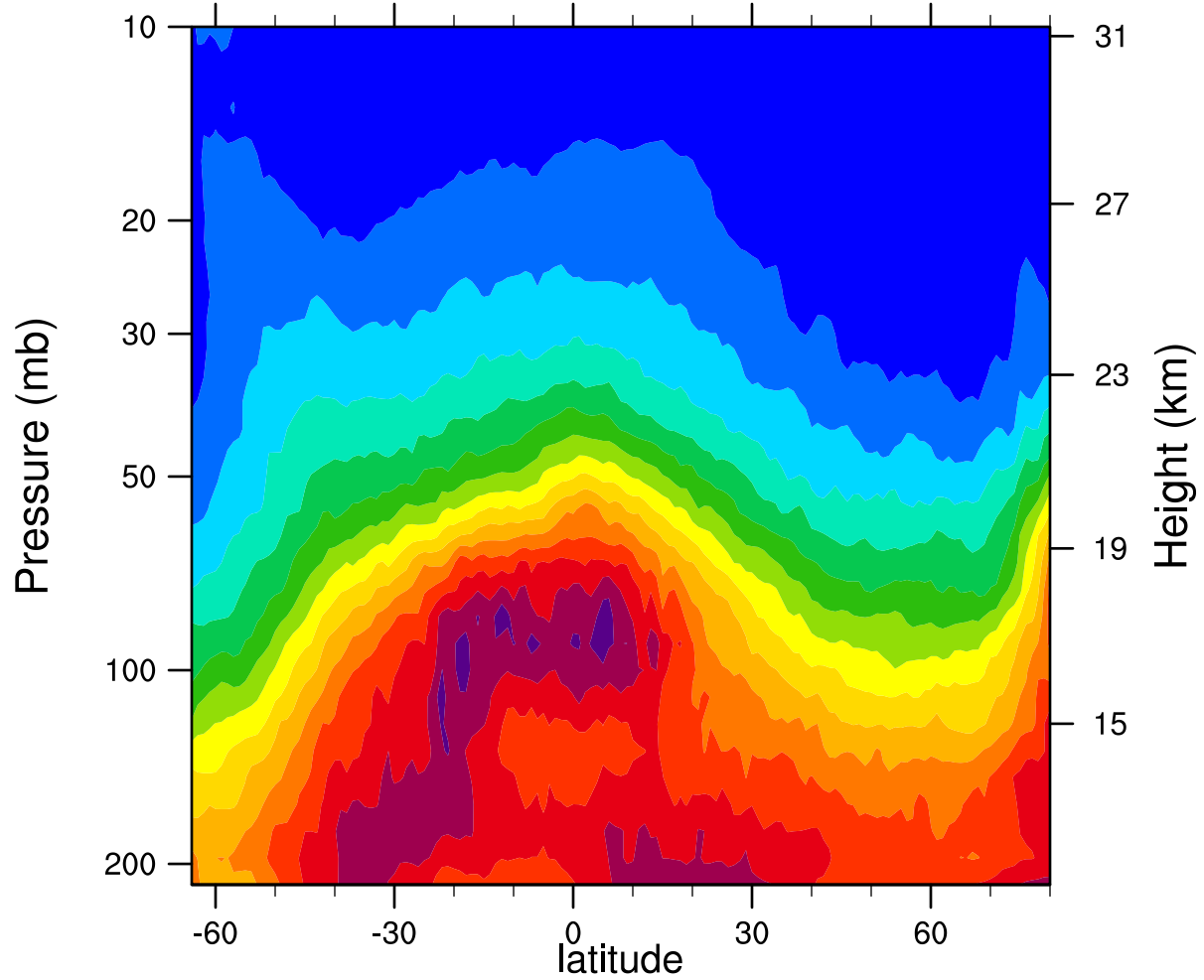
2007d016 12.1MicronExtinction_Combined ( \text{km}^{-1} )
