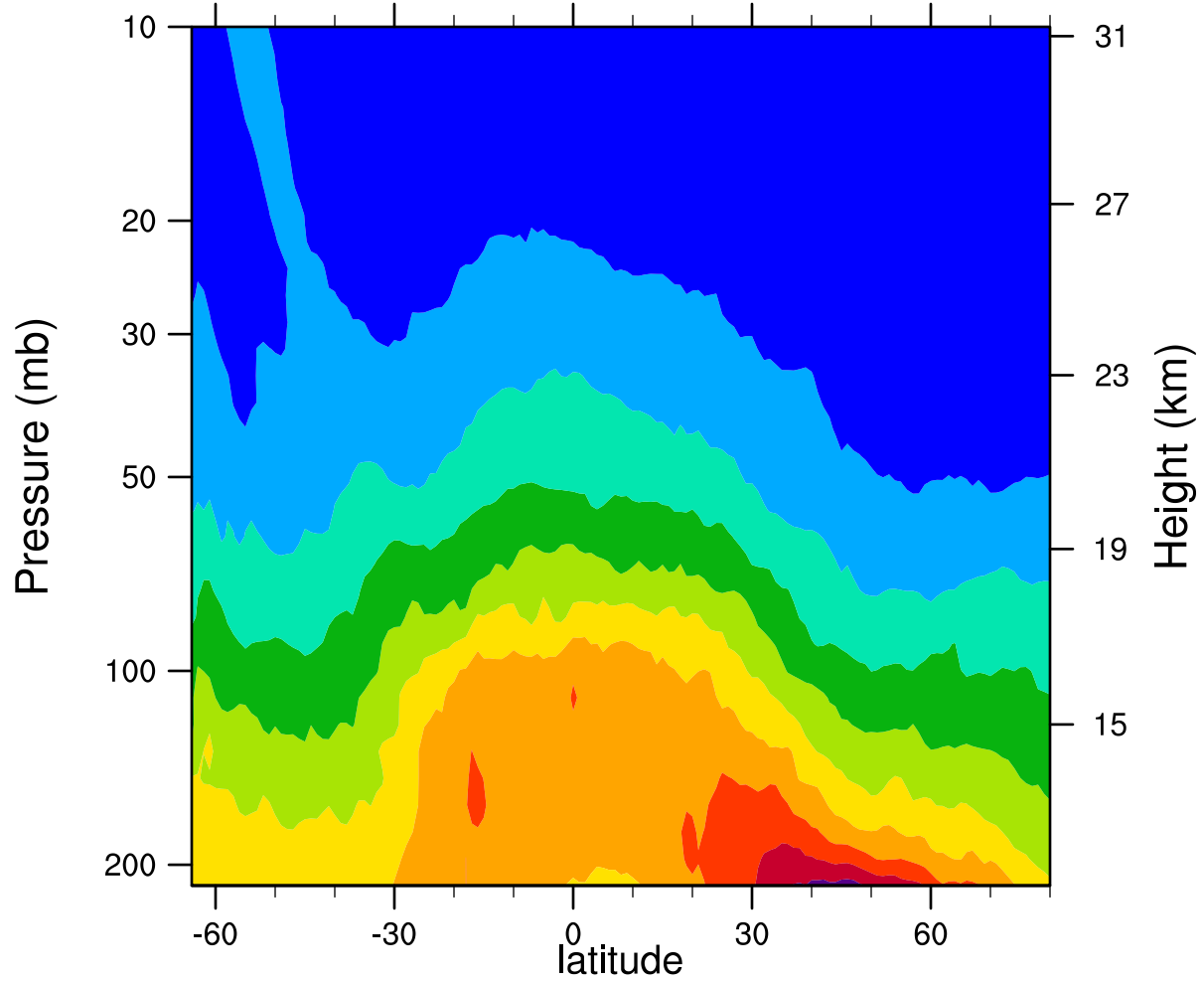
2007d172 12.1MicronExtinction_Combined (km -1 )
