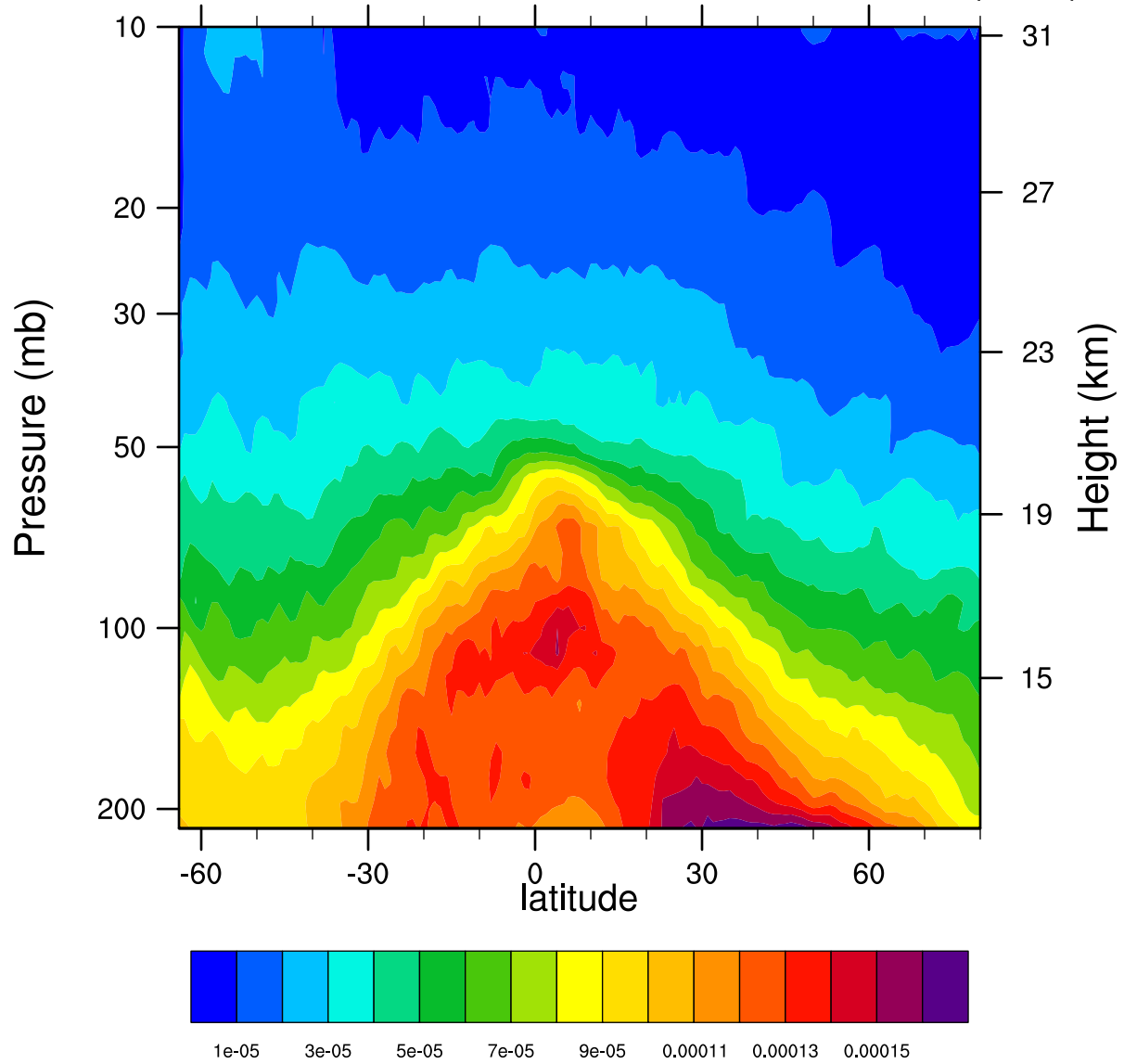
2006d170 12.1MicronExtinction_Combined (km -1 )
