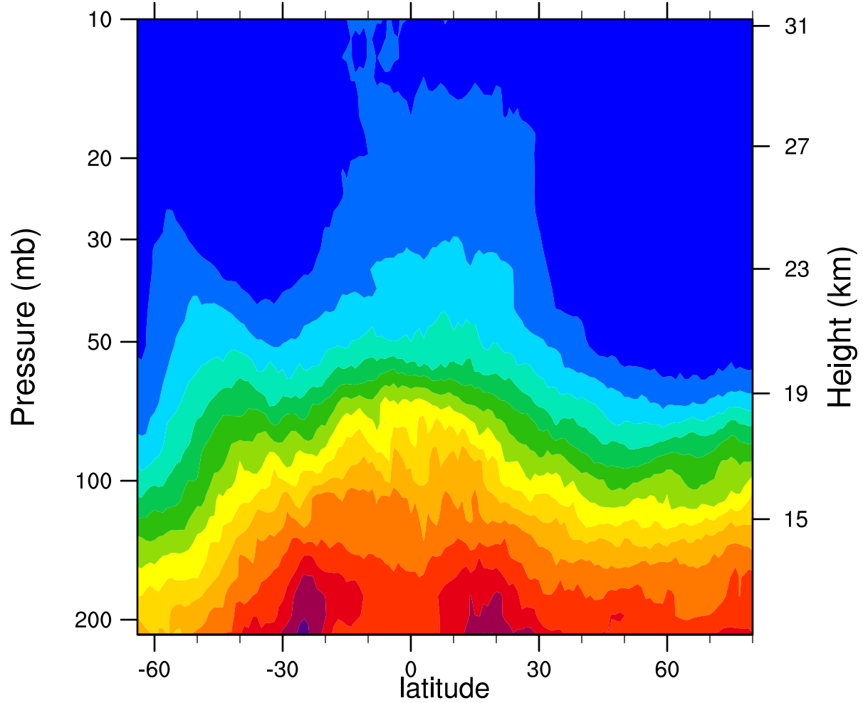
2007d341 12.1MicronExtinction_Combined (km -1 )
