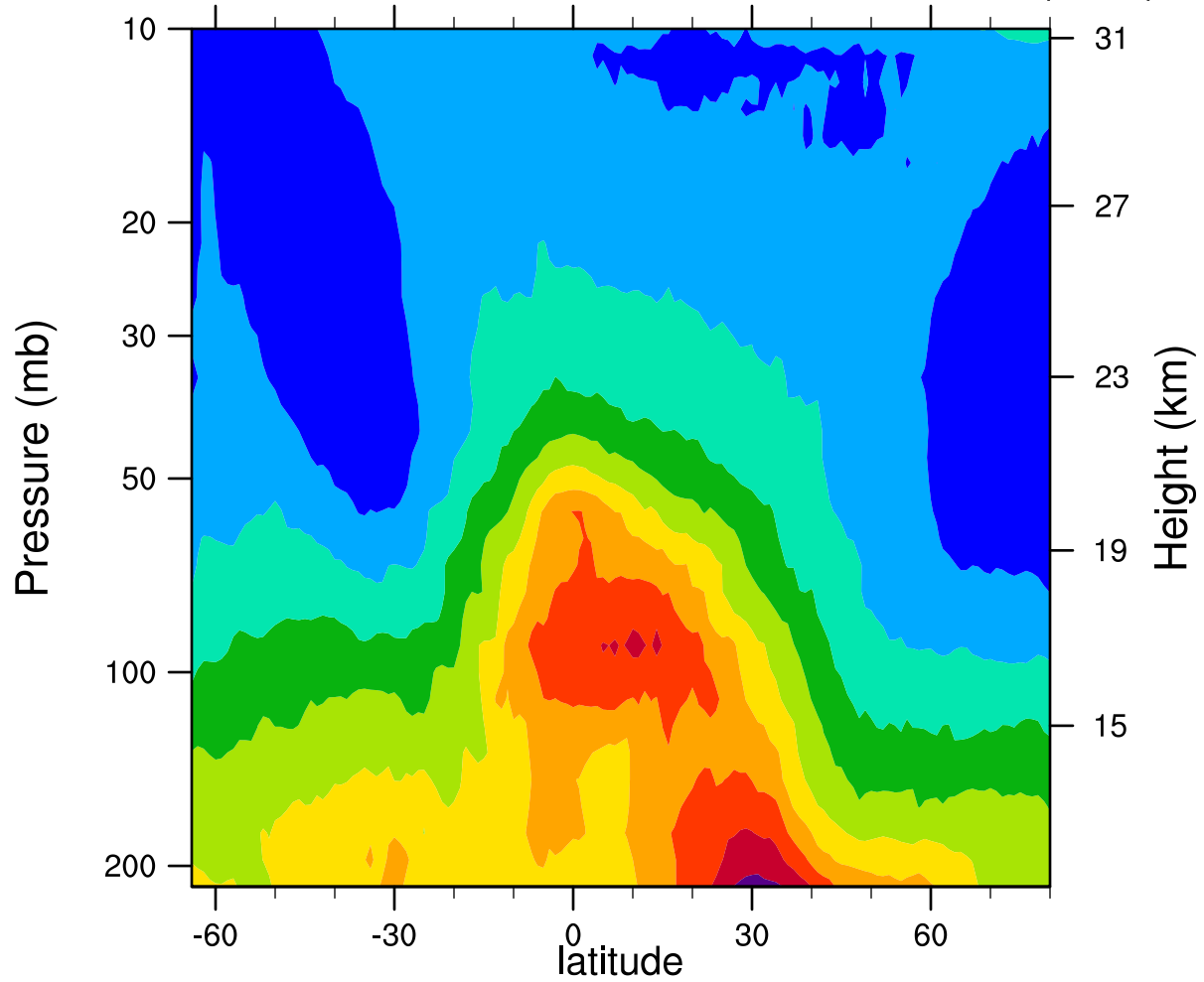
2005d138 12.1MicronExtinction_Combined (km -1 )
