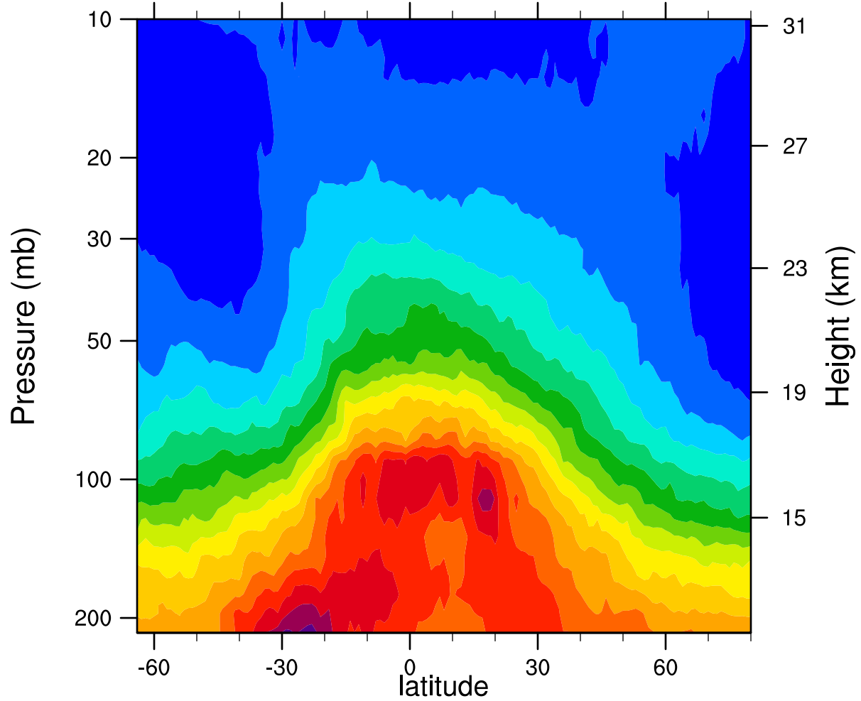
2005d296 12.1MicronExtinction_Combined ( \text{km}^{-1} )
