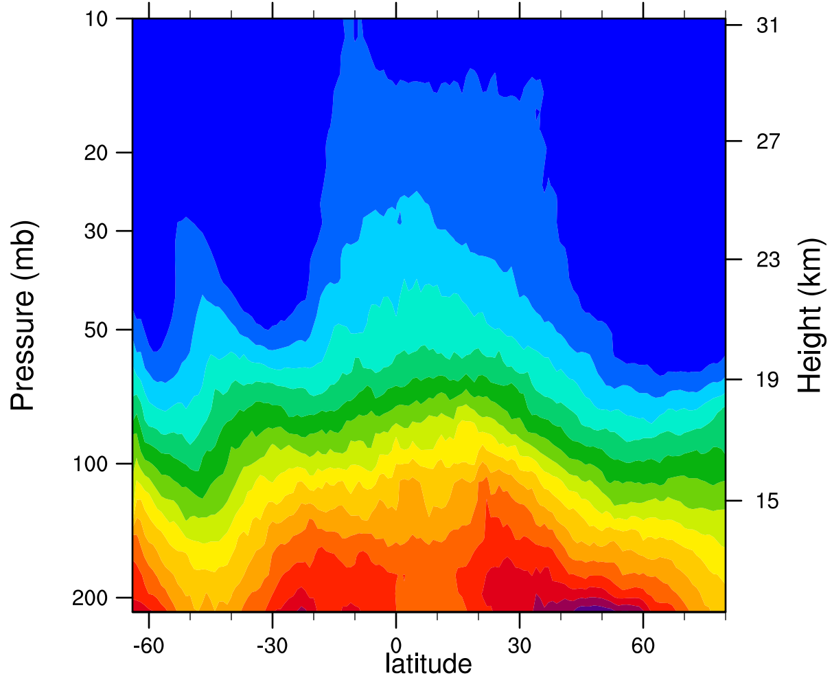
2007d243 12.1MicronExtinction_Combined (km -1 )
