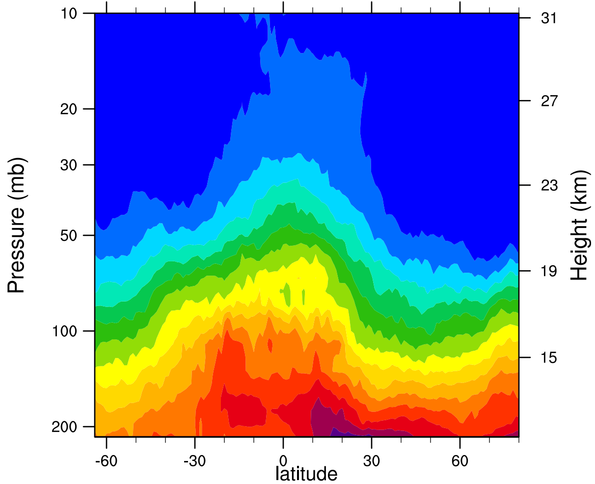
2007d082 12.1MicronExtinction_Combined ( \text{km}^{-1} )
