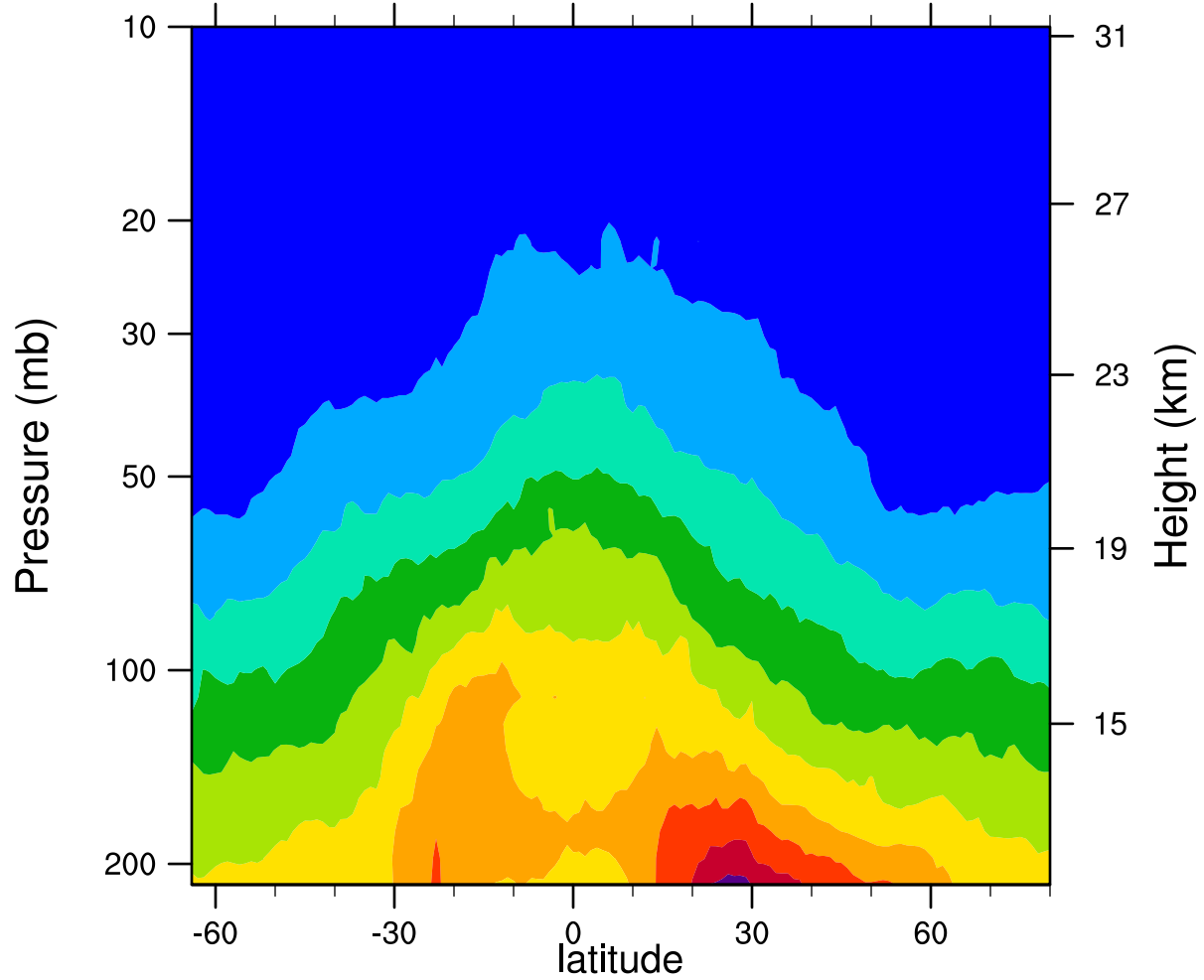
2007d115 12.1MicronExtinction_Combined ( \text{km}^{-1} )
