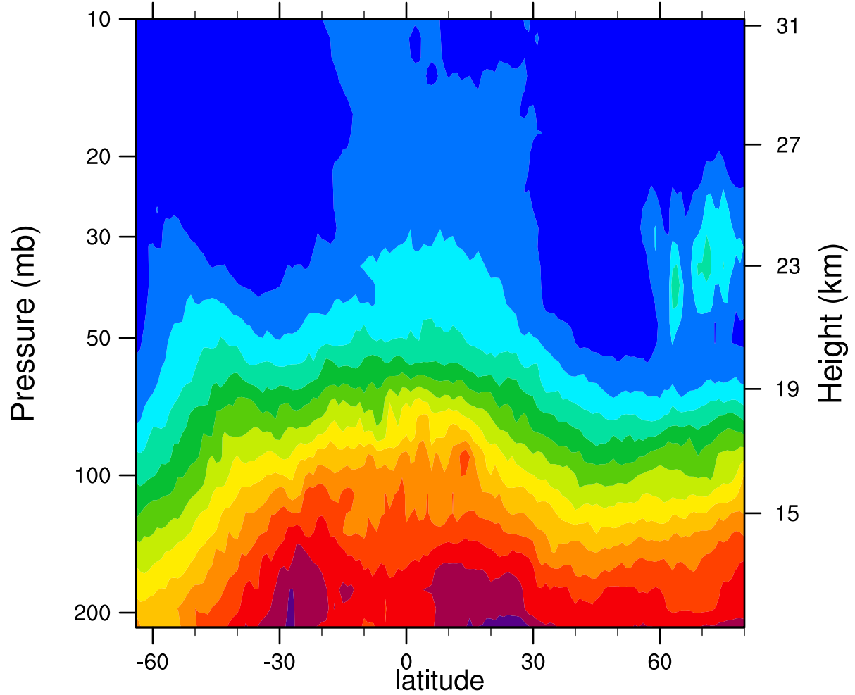
2007d353 12.1MicronExtinction_Combined (km -1 )
