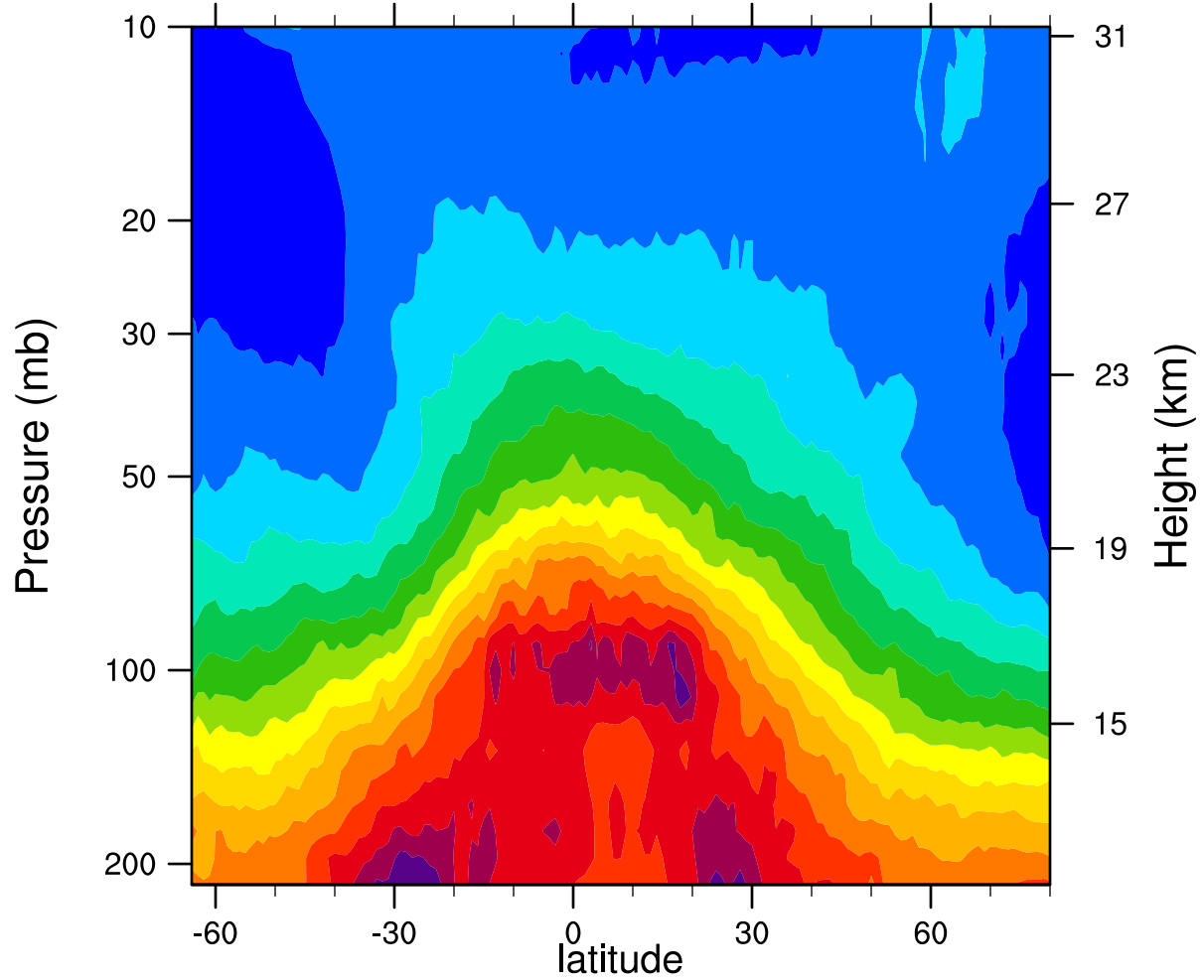
2005d308 12.1MicronExtinction_Combined (km -1 )
