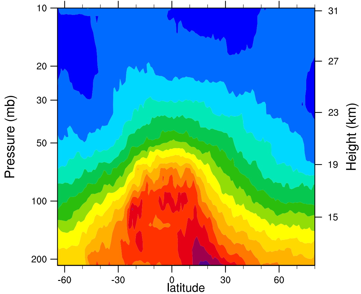
2006d059 12.1MicronExtinction_Combined (km -1 )
