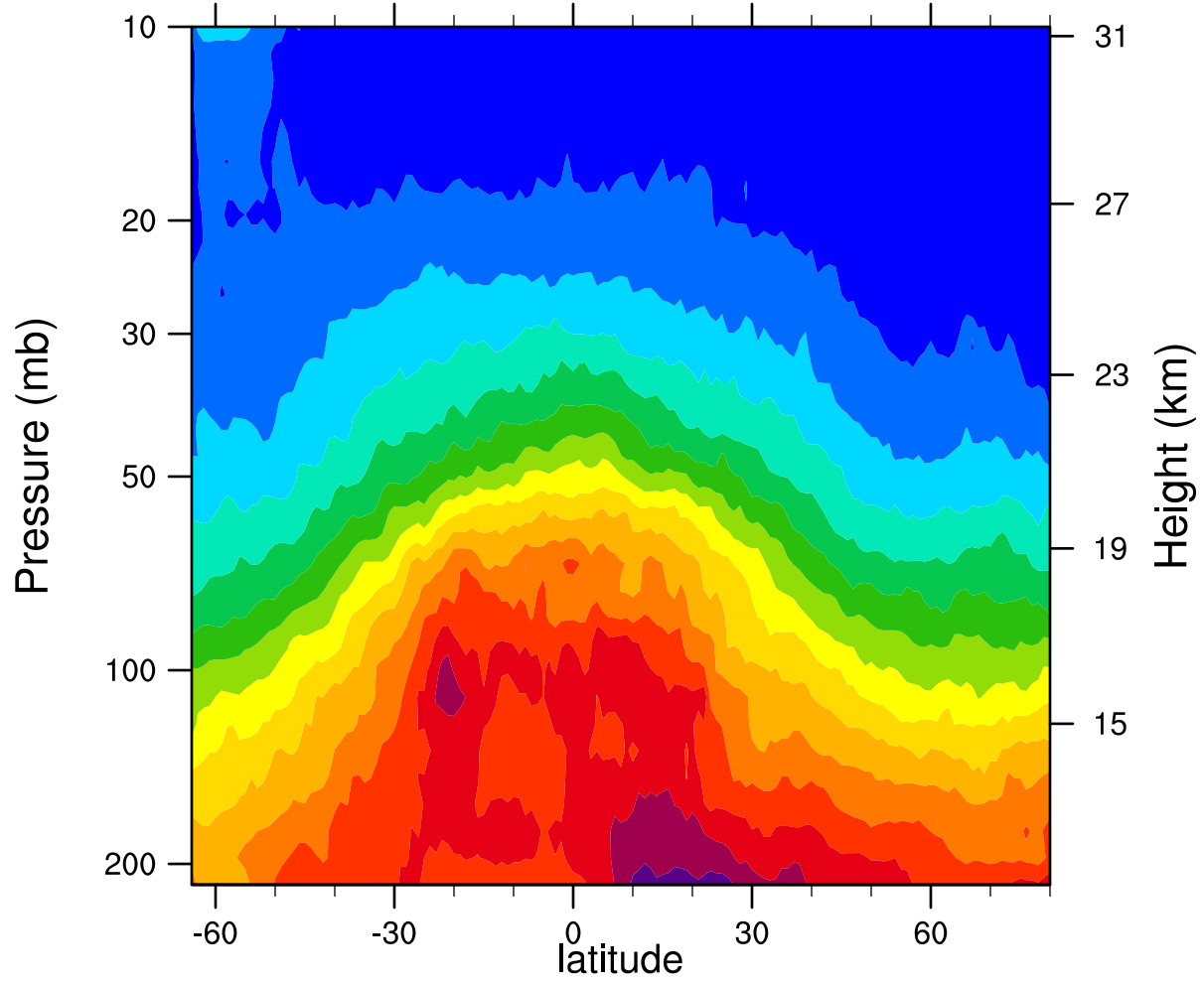
2007d061 12.1MicronExtinction_Combined (km -1 )
