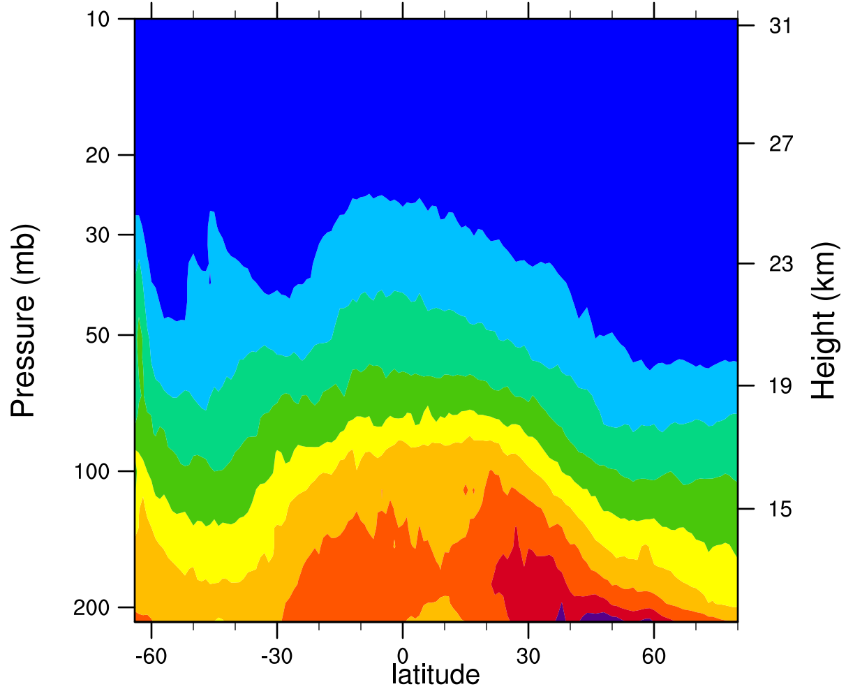
2007d206 12.1MicronExtinction_Combined (km -1 )
