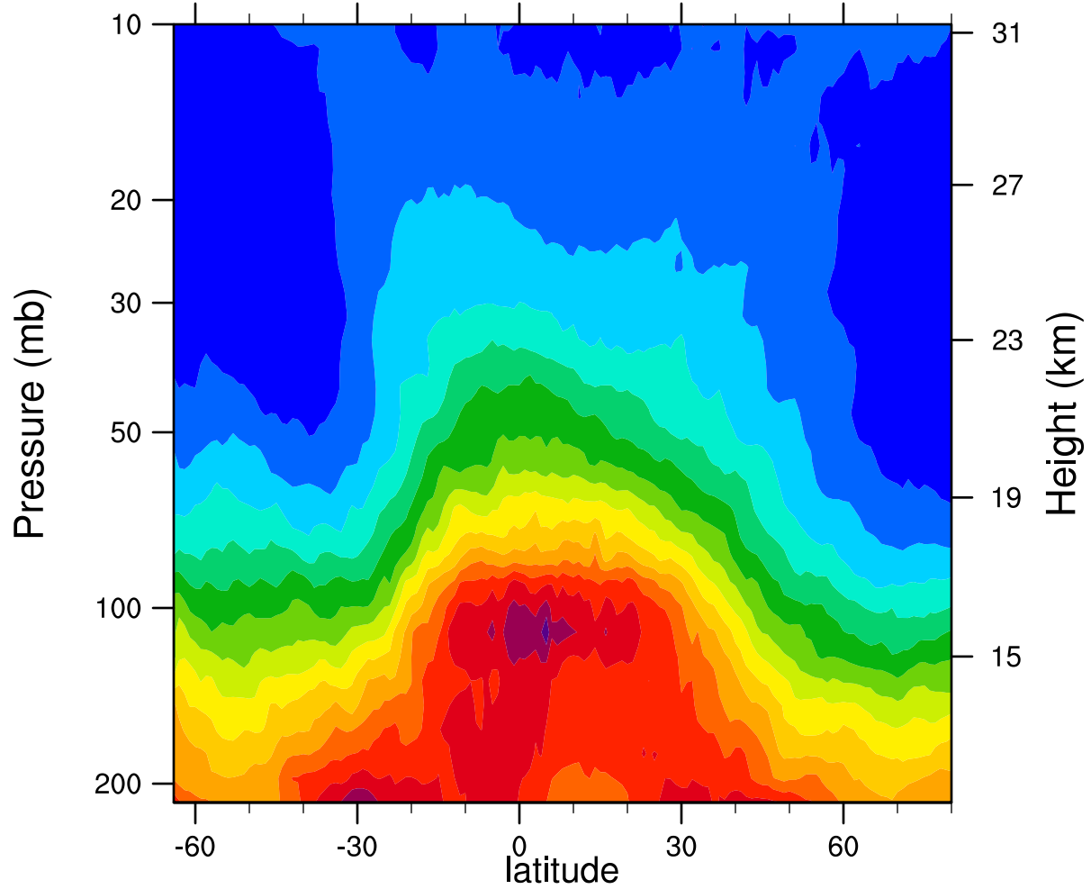
2005d265 12.1MicronExtinction_Combined (km -1 )
