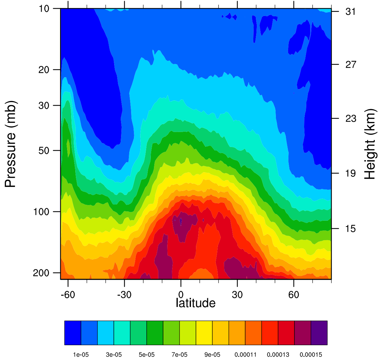
2005d233 12.1MicronExtinction_Combined (km -1 )
