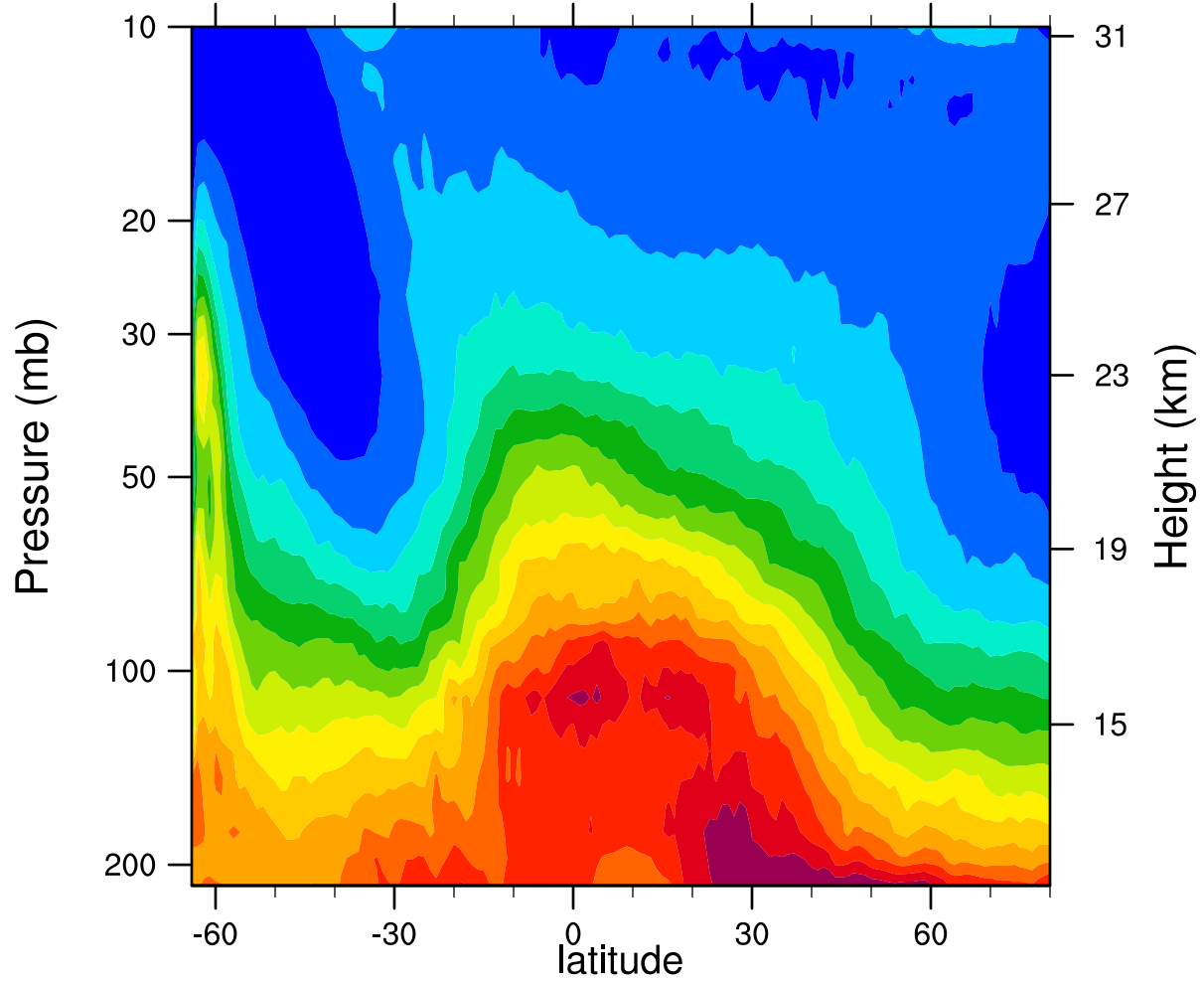
2005d208 12.1MicronExtinction_Combined (km -1 )
