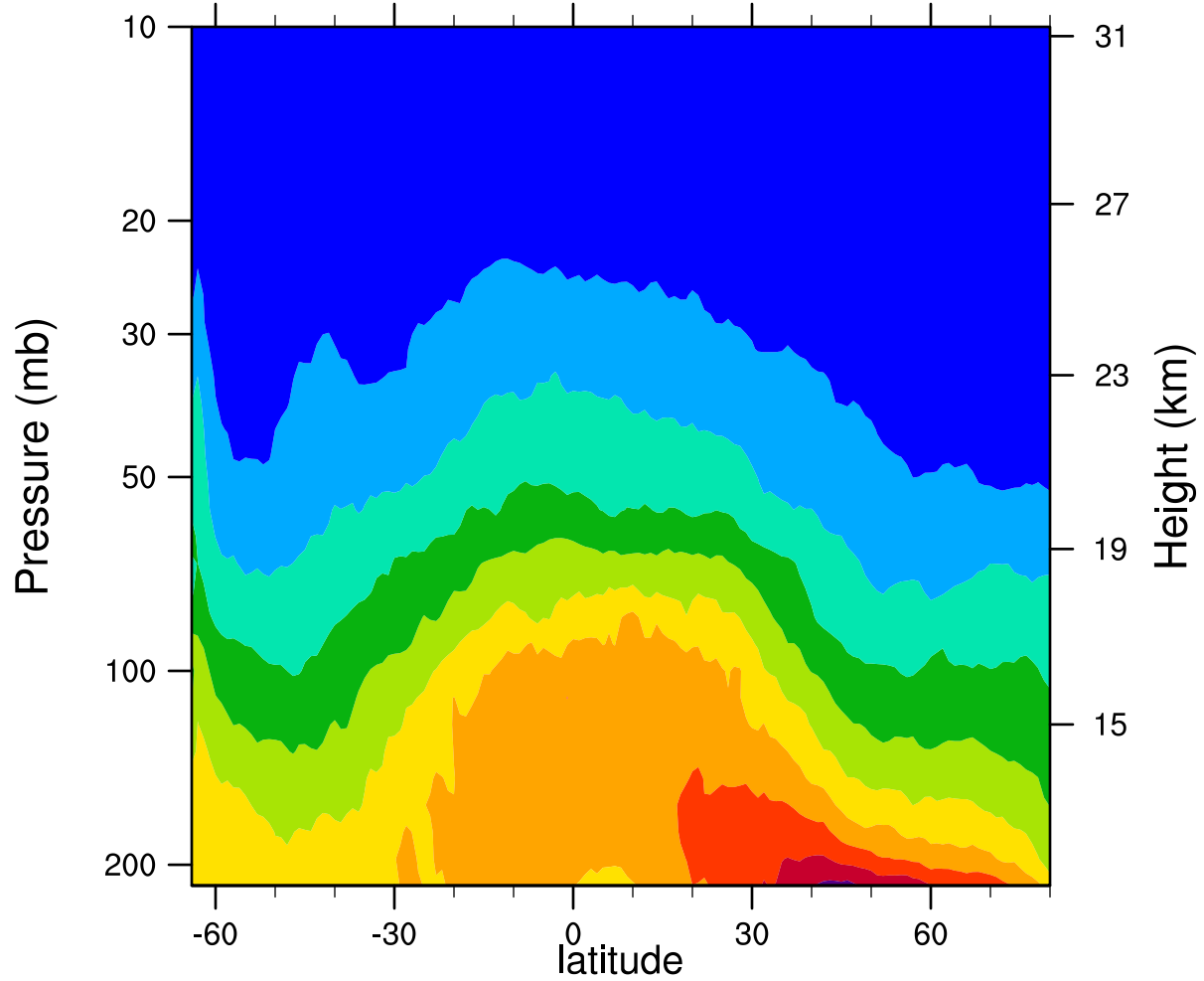
2007d186 12.1MicronExtinction_Combined (km -1 )
