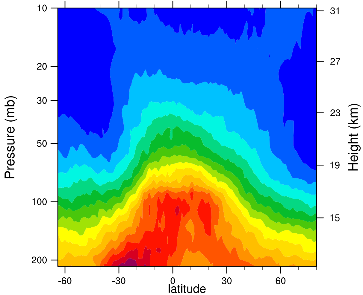
2005d286 12.1MicronExtinction_Combined (km -1 )
