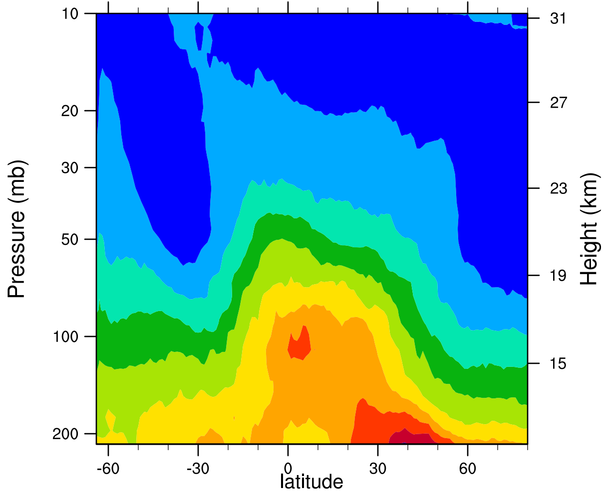
2005d181 12.1MicronExtinction_Combined (km -1 )
