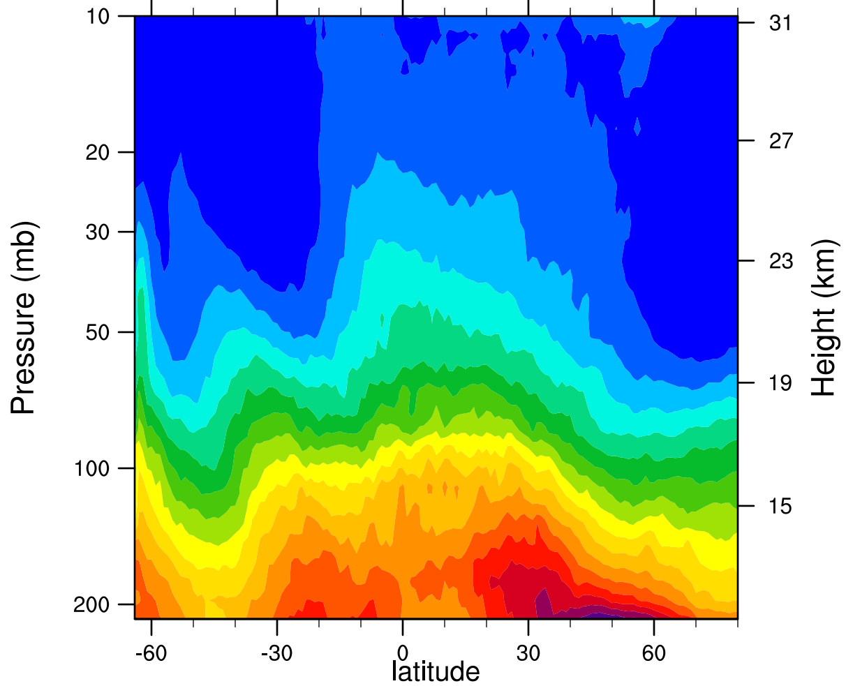
2007d214 12.1MicronExtinction_Combined (km -1 )
