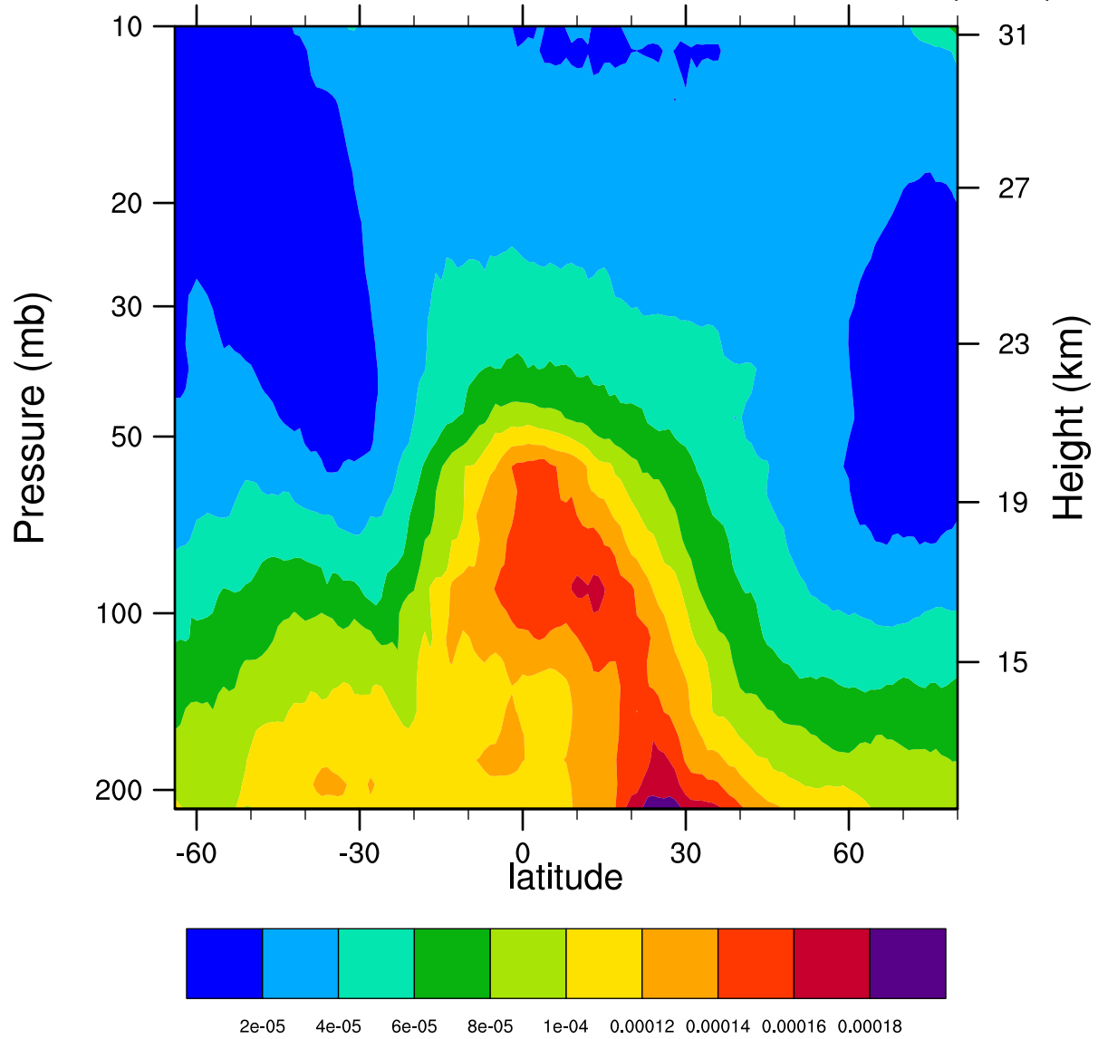
2005d120 12.1MicronExtinction_Combined ( \text{km}^{-1} )
