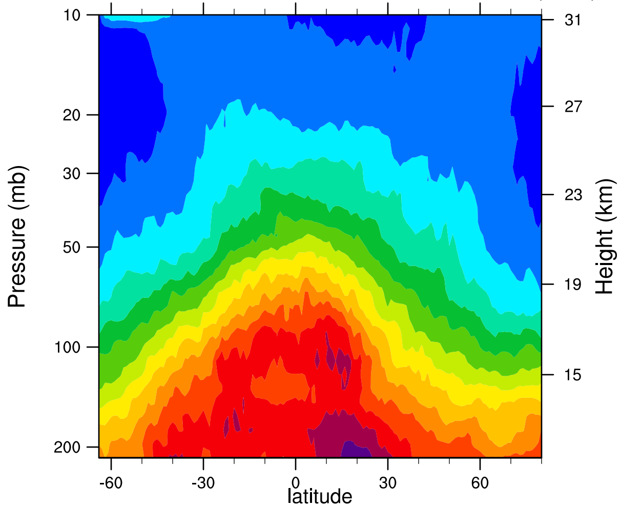
2006d017 12.1MicronExtinction_Combined (km -1 )
