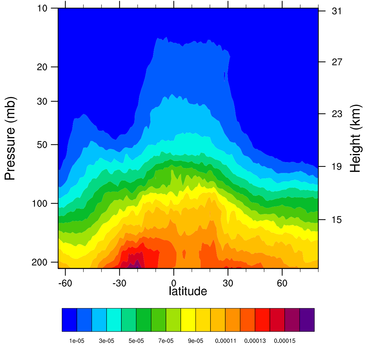
2007d299 12.1MicronExtinction_Combined (km -1 )
