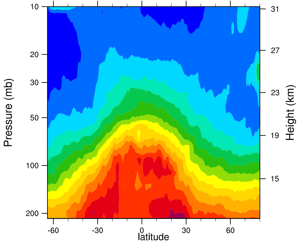
2005d356 12.1MicronExtinction_Combined (km -1 )
