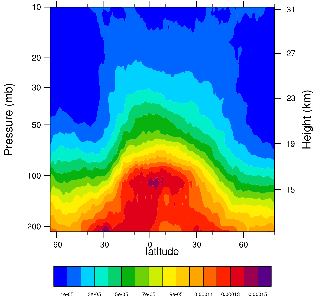
2005d271 12.1MicronExtinction_Combined (km -1 )
