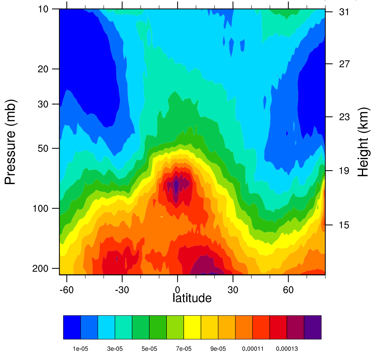
2005d045 12.1MicronExtinction_Combined ( \text{km}^{-1} )
