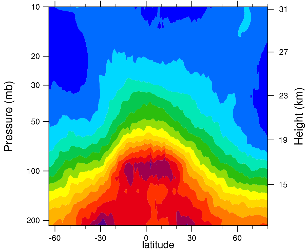
2005d314 12.1MicronExtinction_Combined ( \text{km}^{-1} )
