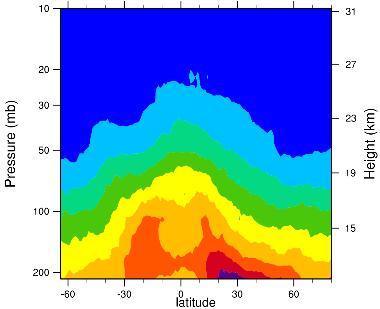
2007d110 12.1MicronExtinction_Combined ( \text{km}^{-1} )
