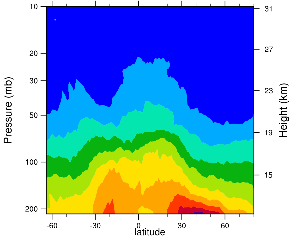
2007d155 12.1MicronExtinction_Combined ( \text{km}^{-1} )
