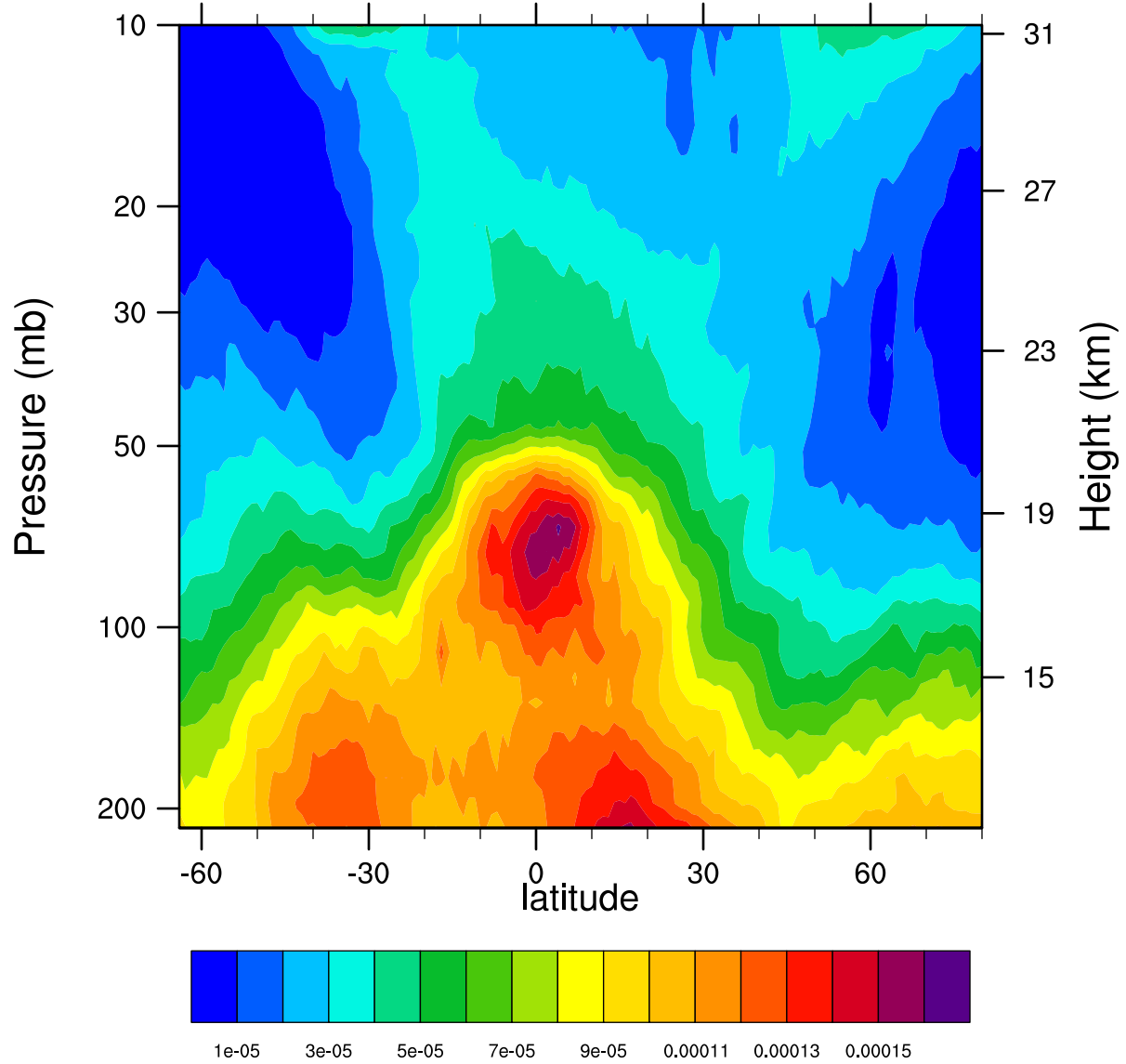
2005d055 12.1MicronExtinction_Combined (km -1 )
