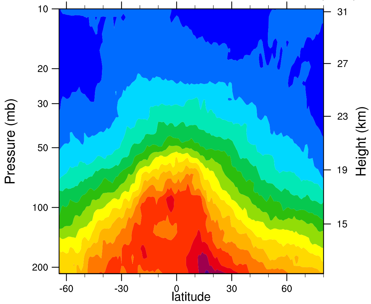
2006d048 12.1MicronExtinction_Combined ( \text{km}^{-1} )
