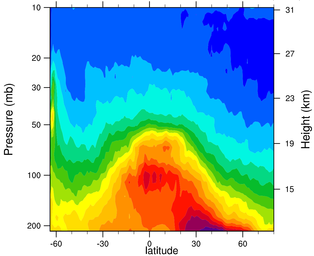
2006d185 12.1MicronExtinction_Combined (km -1 )
