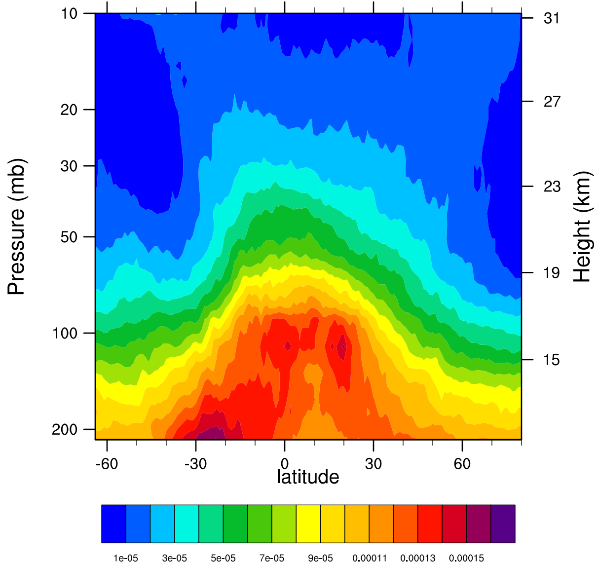
2005d289 12.1MicronExtinction_Combined (km -1 )
