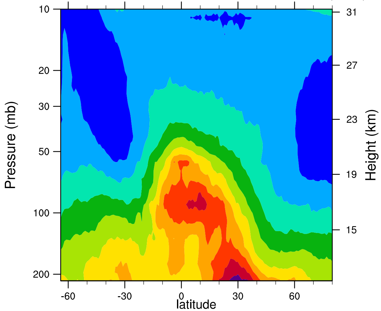
2005d133 12.1MicronExtinction_Combined (km -1 )
