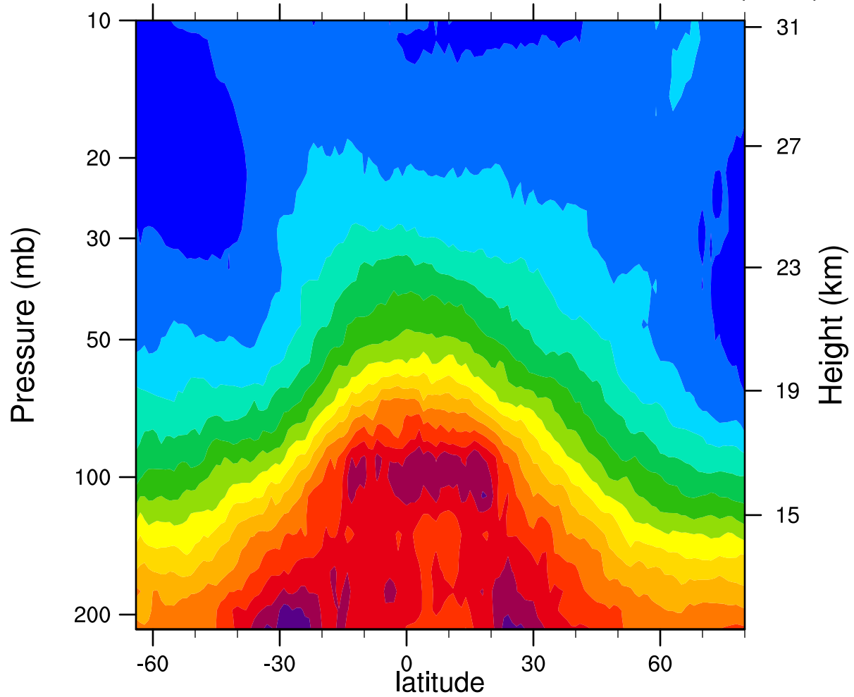
2005d309 12.1MicronExtinction_Combined (km -1 )
