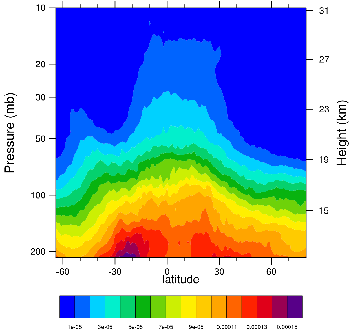
2007d303 12.1MicronExtinction_Combined (km -1 )
