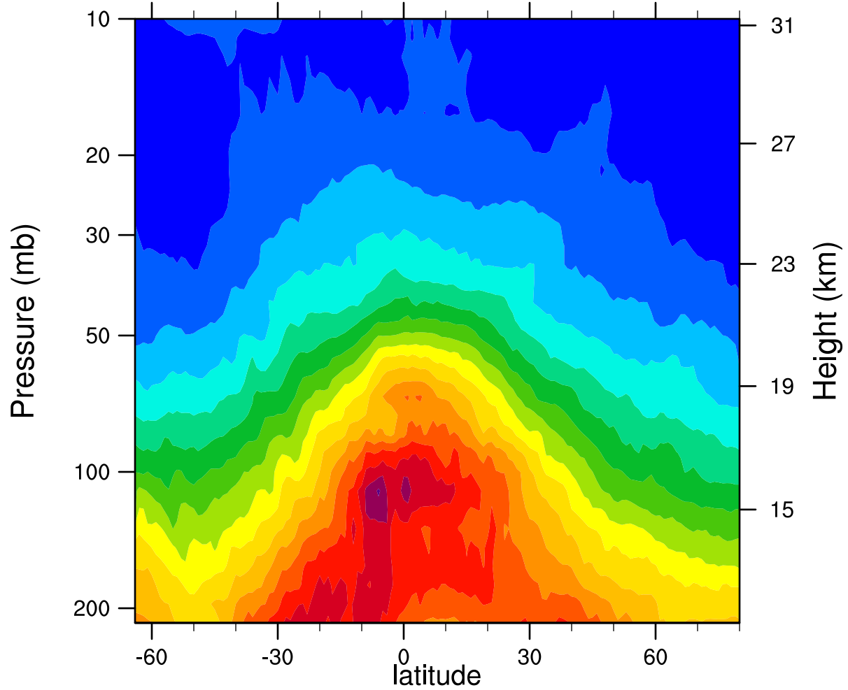
2006d287 12.1MicronExtinction_Combined (km -1 )
