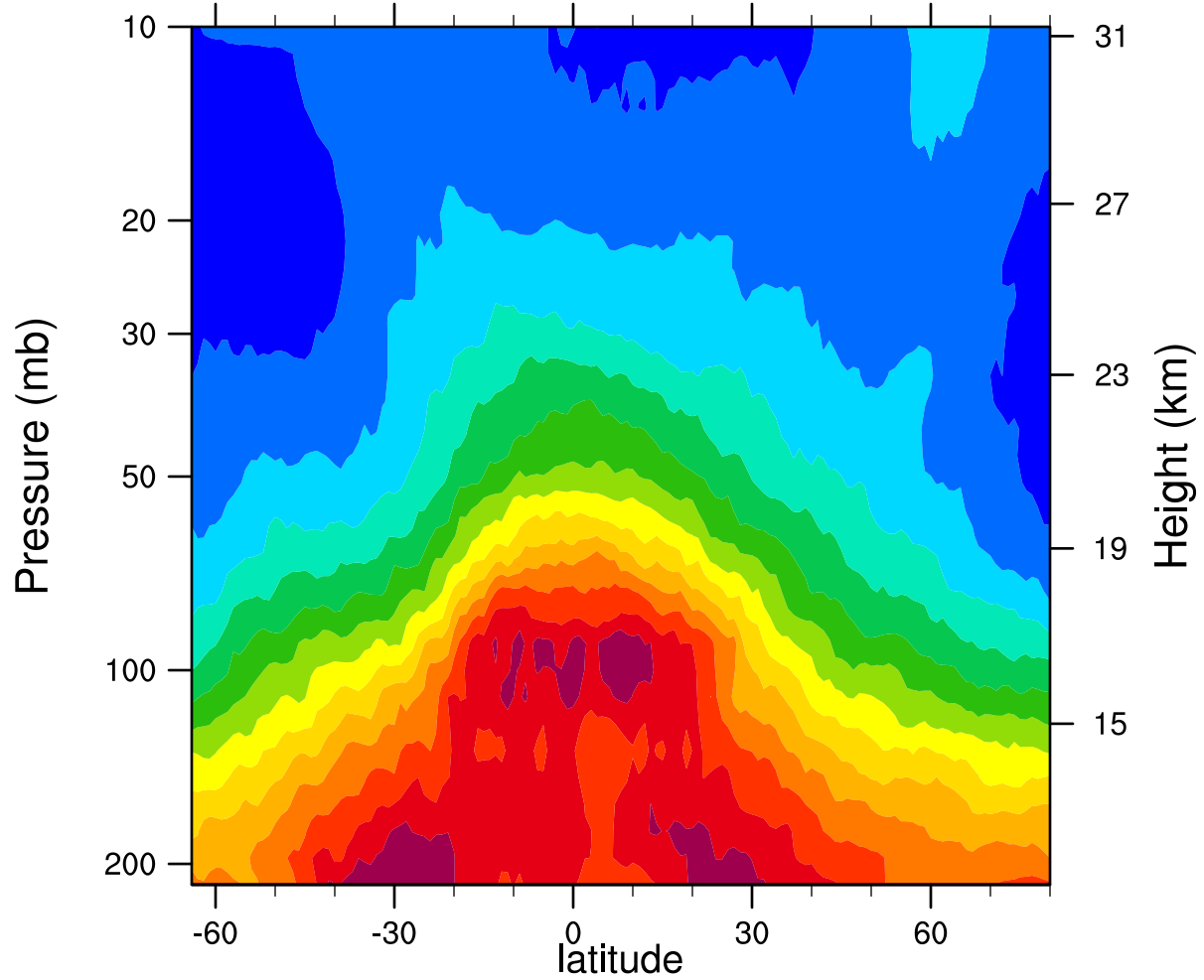
2005d319 12.1MicronExtinction_Combined (km -1 )
