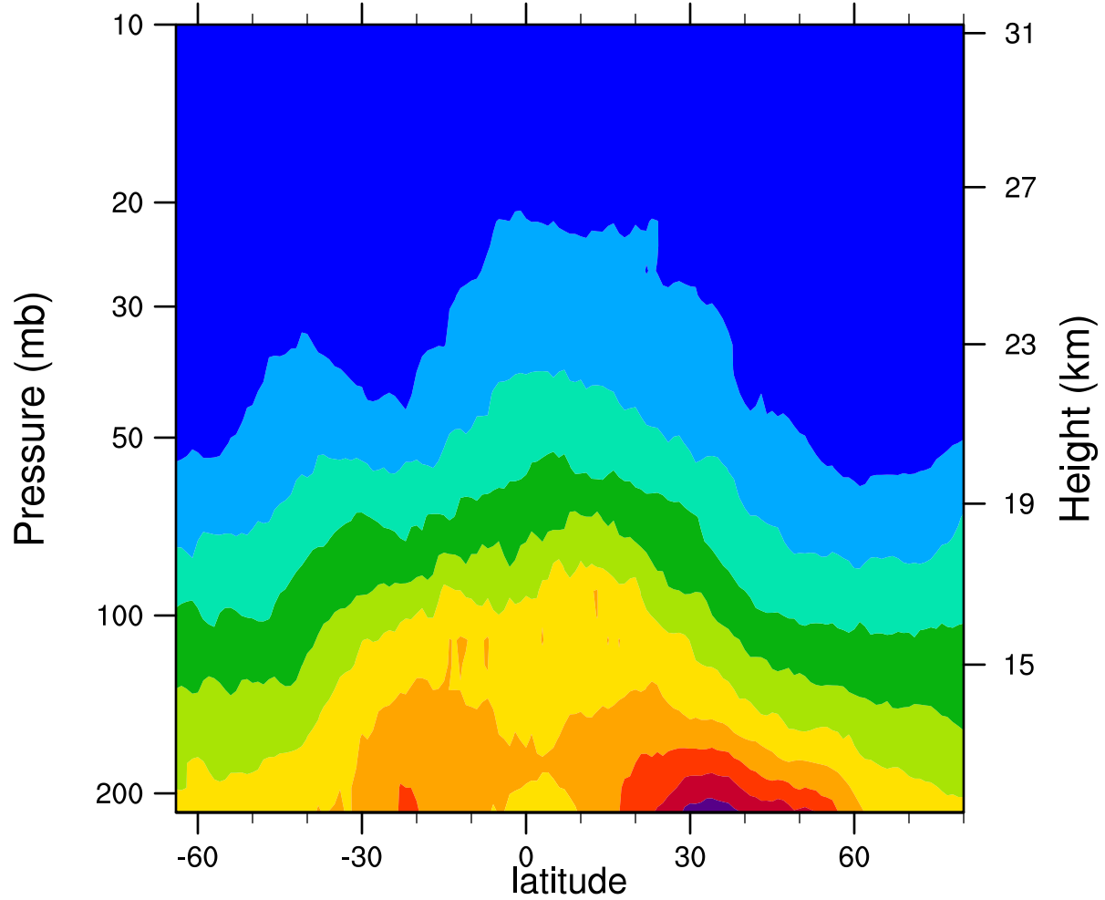
2007d137 12.1MicronExtinction_Combined ( \text{km}^{-1} )
