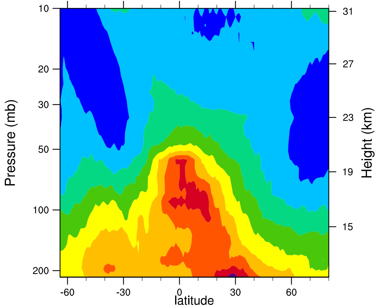
2005d104 12.1MicronExtinction_Combined ( \text{km}^{-1} )
