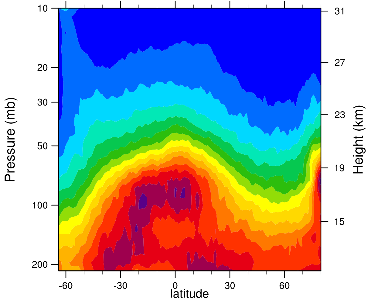
2007d019 12.1MicronExtinction_Combined ( \text{km}^{-1} )
