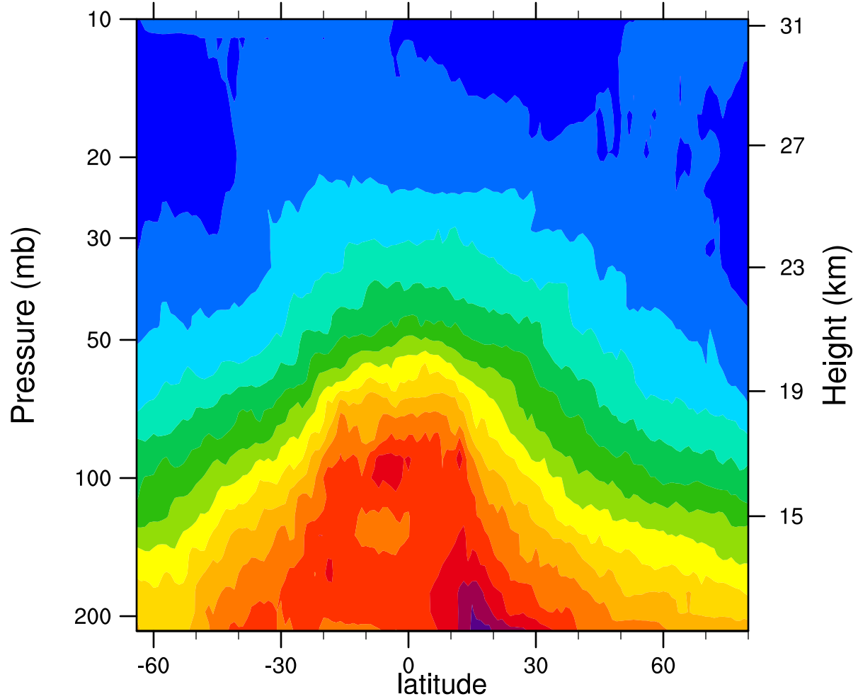
2006d050 12.1MicronExtinction_Combined (km -1 )
