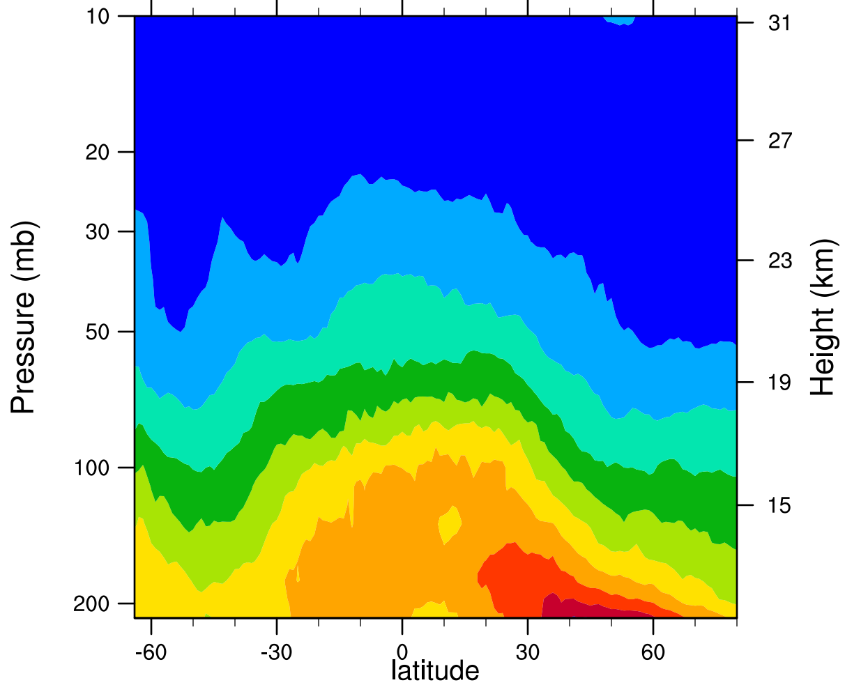
2007d195 12.1MicronExtinction_Combined (km -1 )
