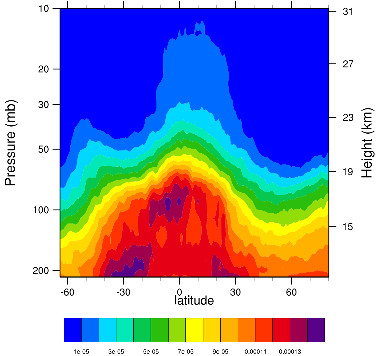
2006d340 12.1MicronExtinction_Combined ( \text{km}^{-1} )
