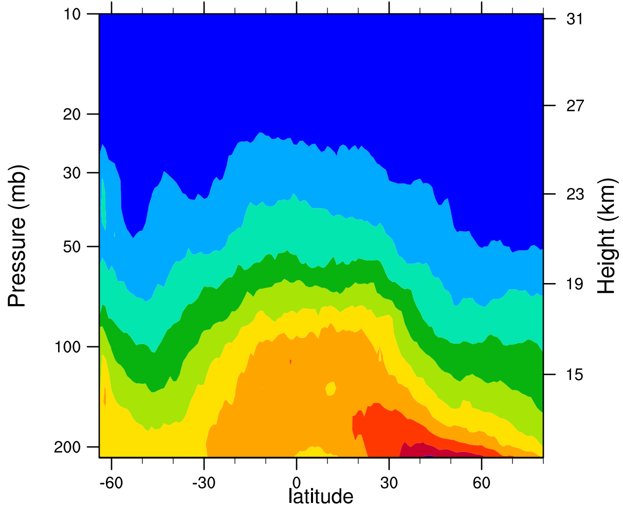
2007d191 12.1MicronExtinction_Combined (km -1 )
