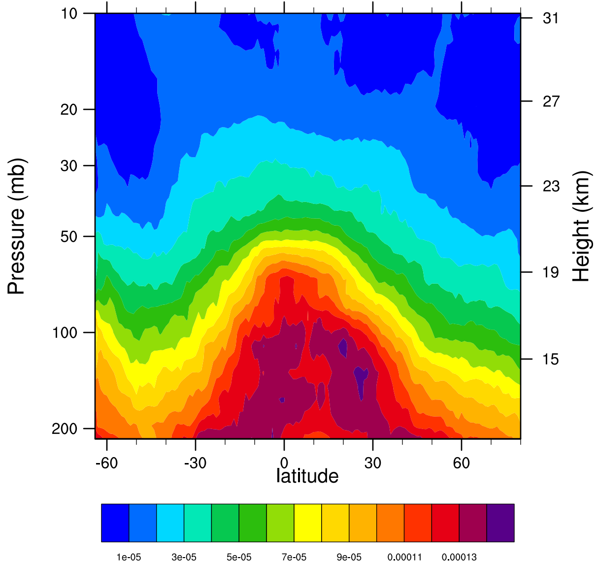
2006d260 12.1MicronExtinction_Combined ( \text{km}^{-1} )
