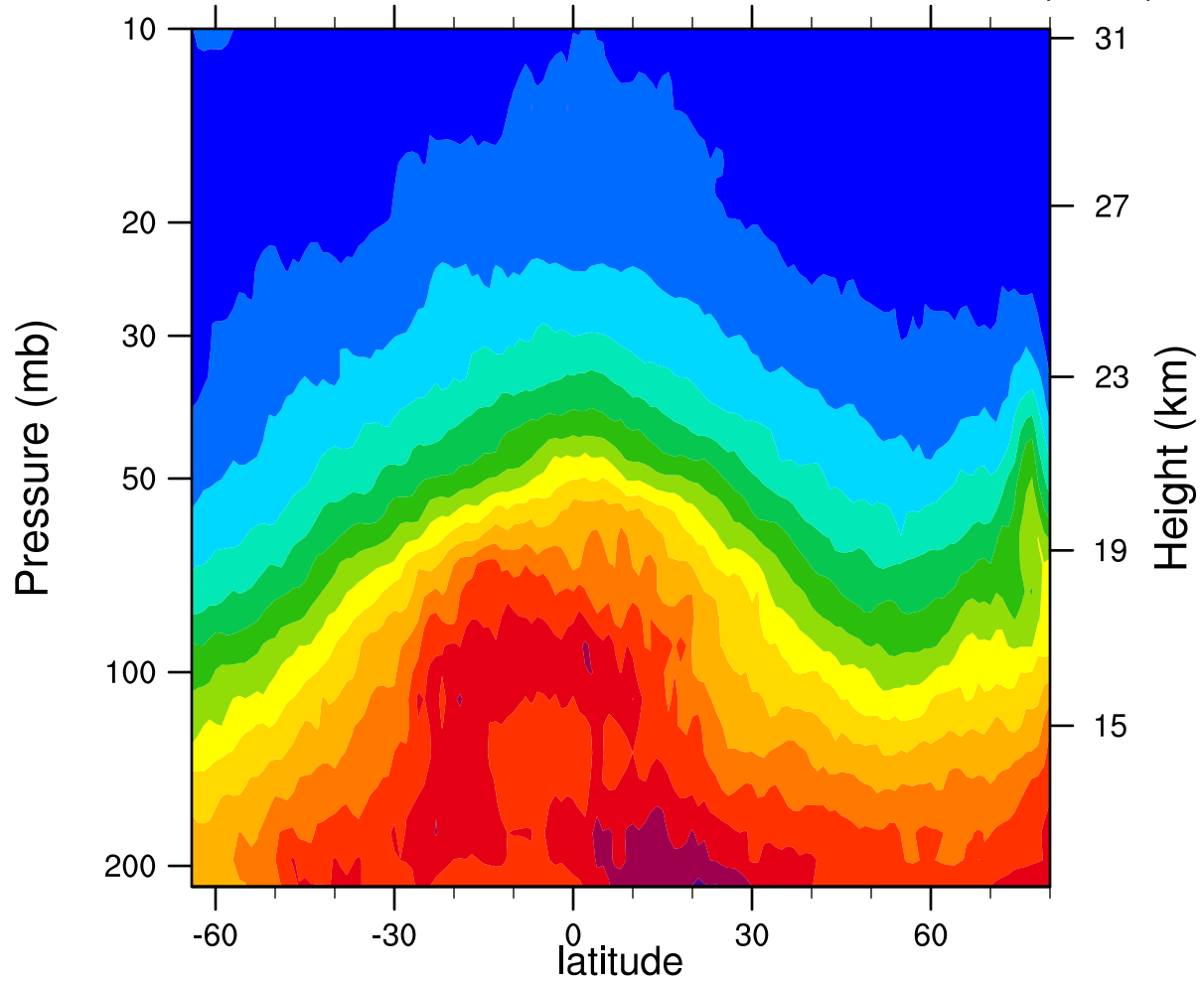
2007d043 12.1MicronExtinction_Combined ( \text{km}^{-1} )
