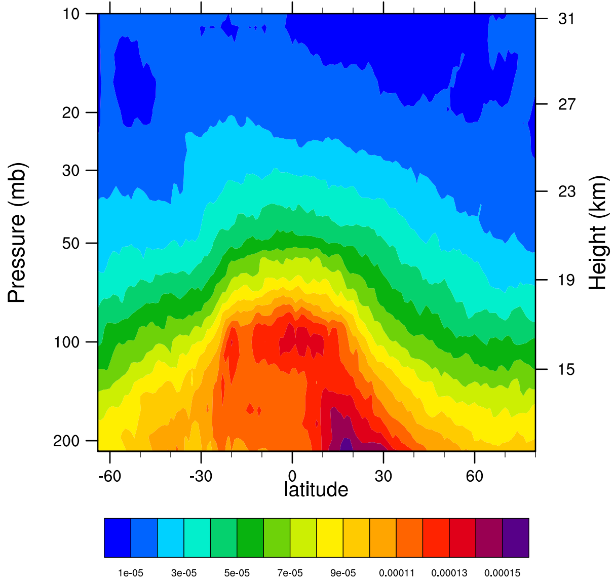
2006d086 12.1MicronExtinction_Combined (km -1 )
