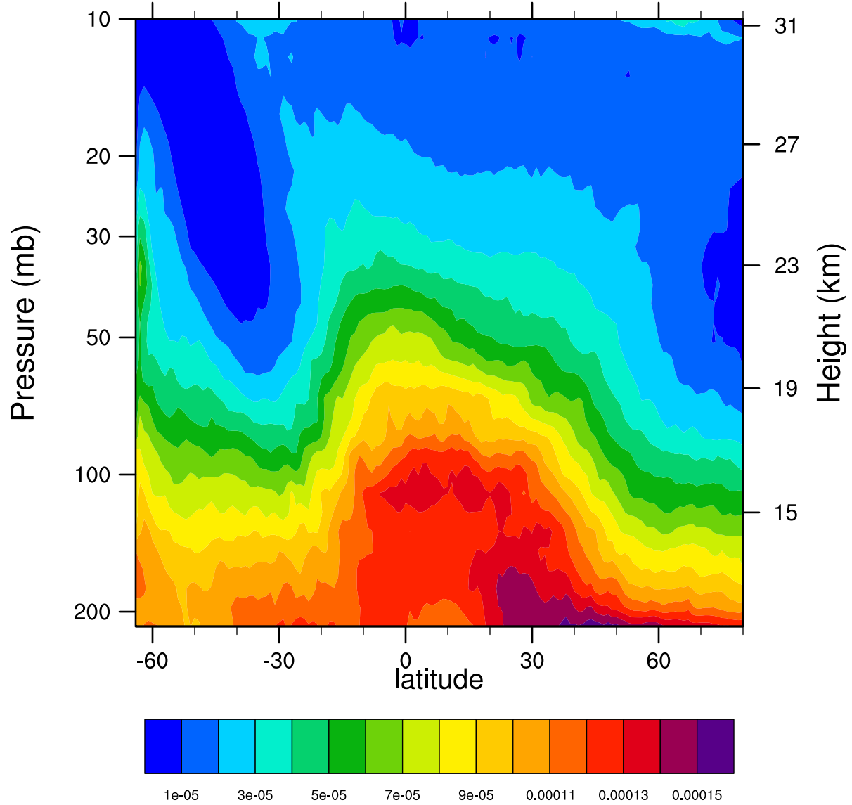
2005d203 12.1MicronExtinction_Combined (km -1 )
