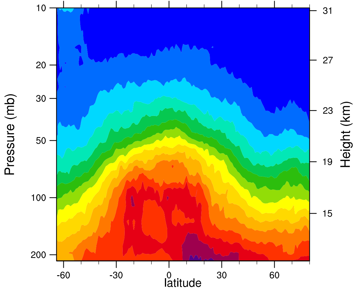
2007d064 12.1MicronExtinction_Combined ( \text{km}^{-1} )
