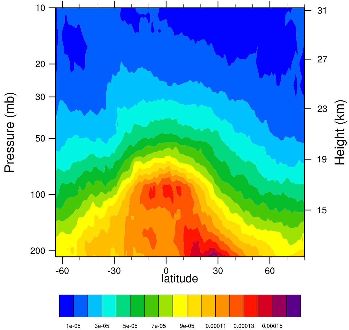
2006d095 12.1MicronExtinction_Combined ( \text{km}^{-1} )
