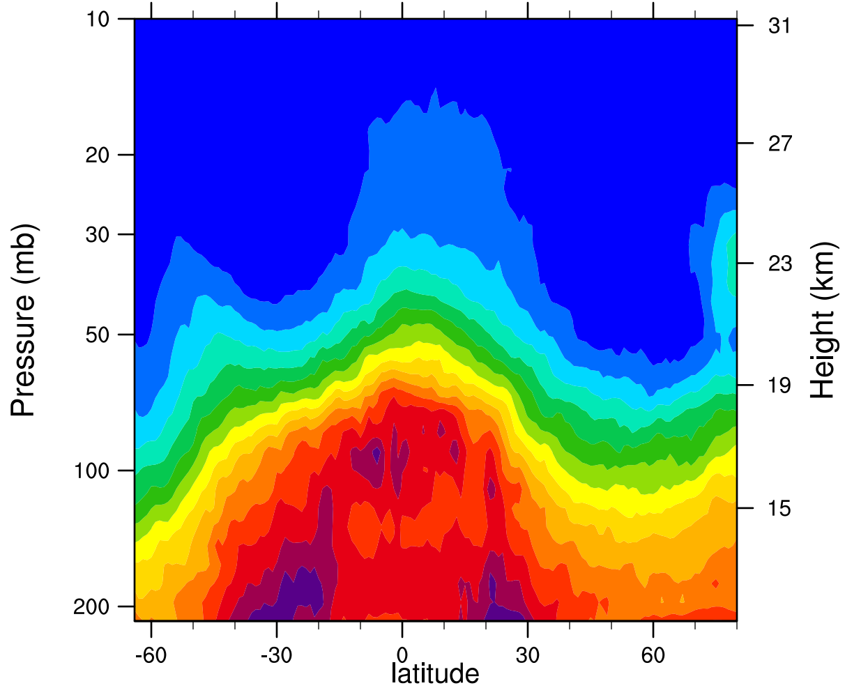
2006d346 12.1MicronExtinction_Combined (km -1 )
