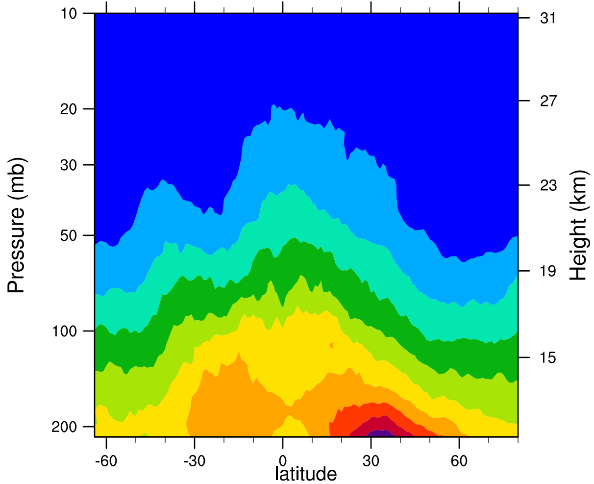
2007d131 12.1MicronExtinction_Combined (km -1 )
