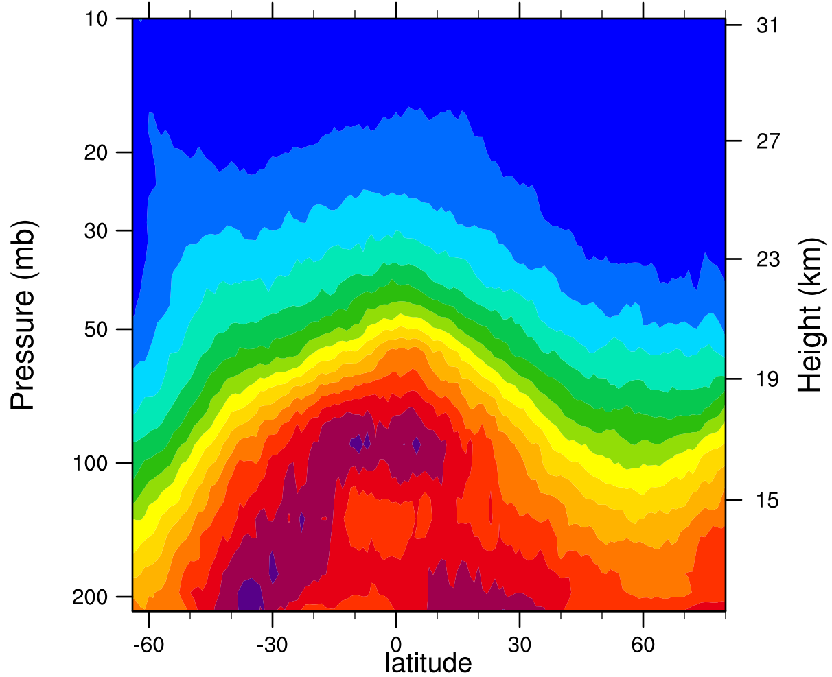
2007d008 12.1MicronExtinction_Combined ( \text{km}^{-1} )
