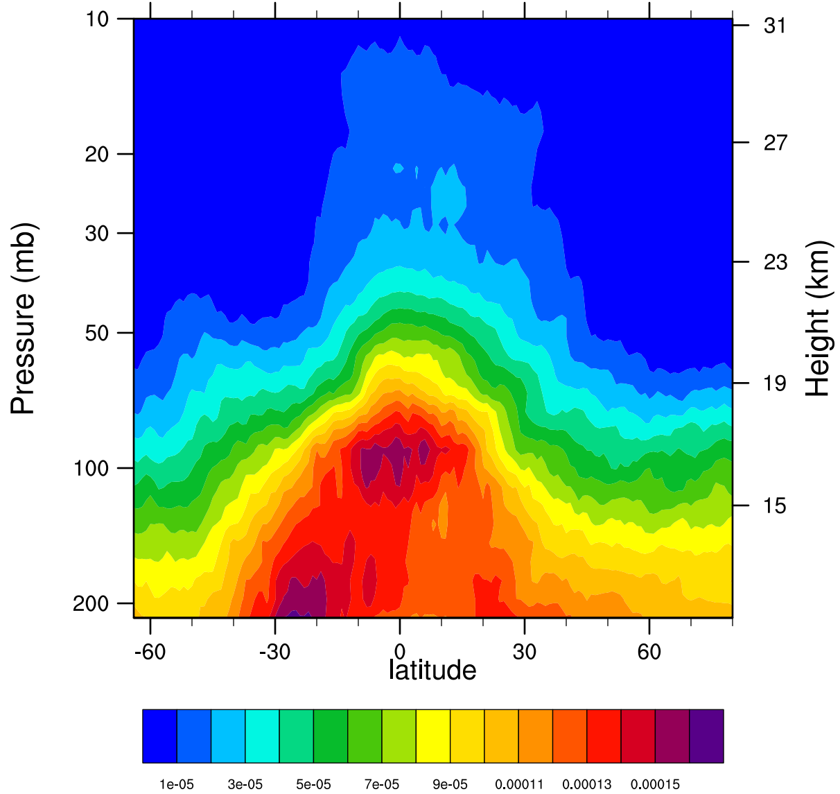
2006d318 12.1MicronExtinction_Combined (km -1 )
