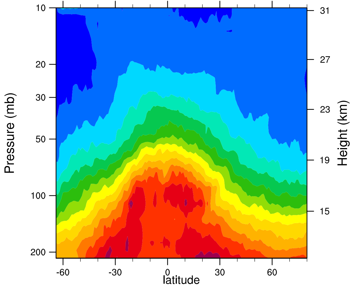
2005d344 12.1MicronExtinction_Combined (km -1 )
