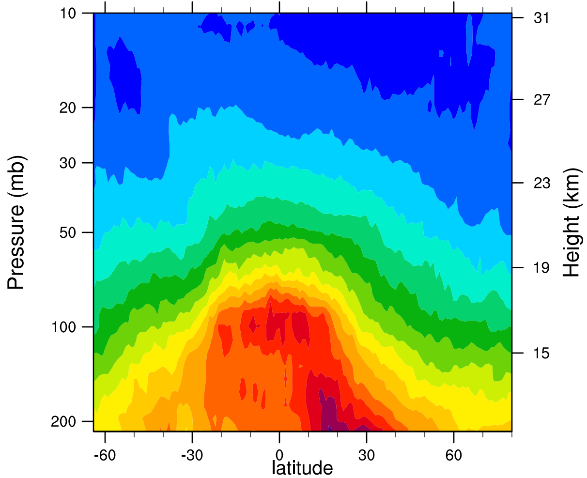
2006d089 12.1MicronExtinction_Combined (km -1 )
