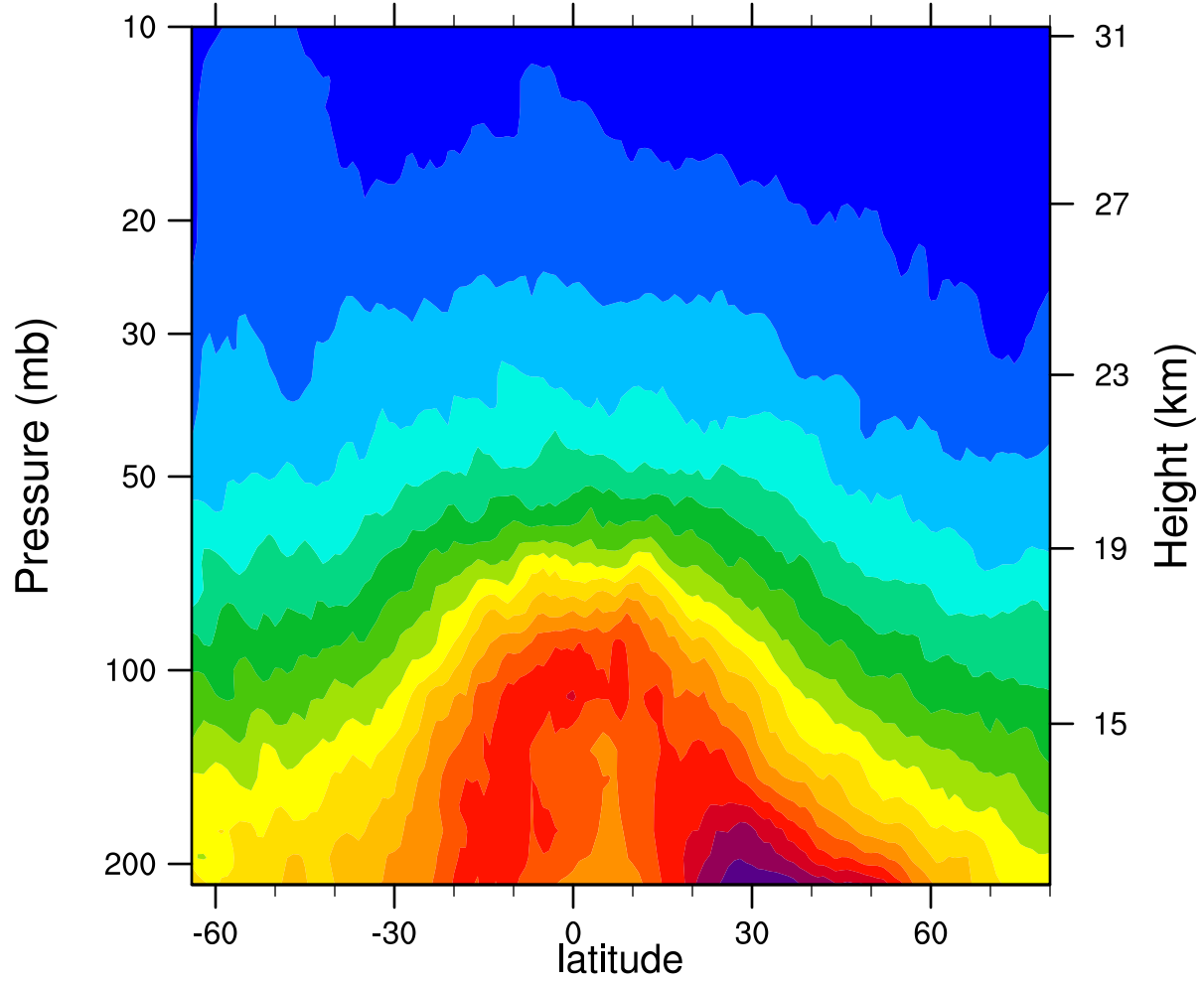
2006d148 12.1MicronExtinction_Combined (km -1 )
