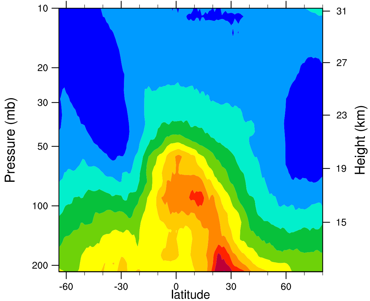
2005d125 12.1MicronExtinction_Combined ( \text{km}^{-1} )
