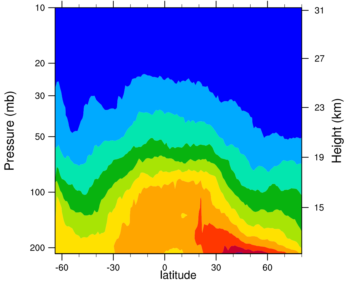
2007d189 12.1MicronExtinction_Combined (km -1 )
