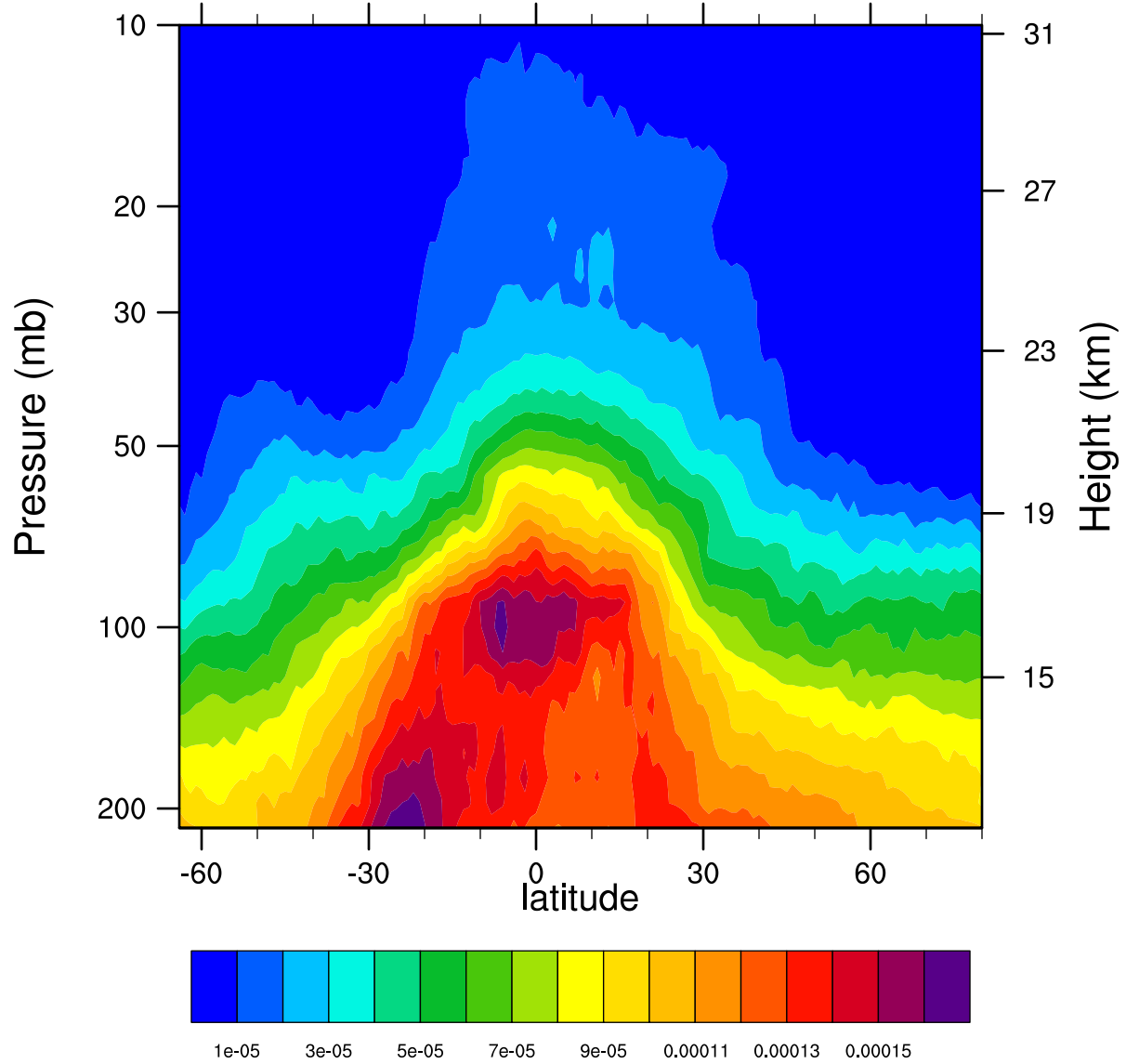
2006d315 12.1MicronExtinction_Combined (km -1 )
