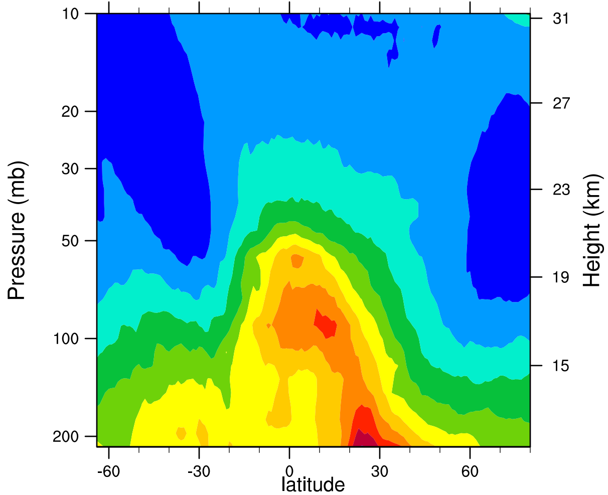
2005d123 12.1MicronExtinction_Combined ( \text{km}^{-1} )
