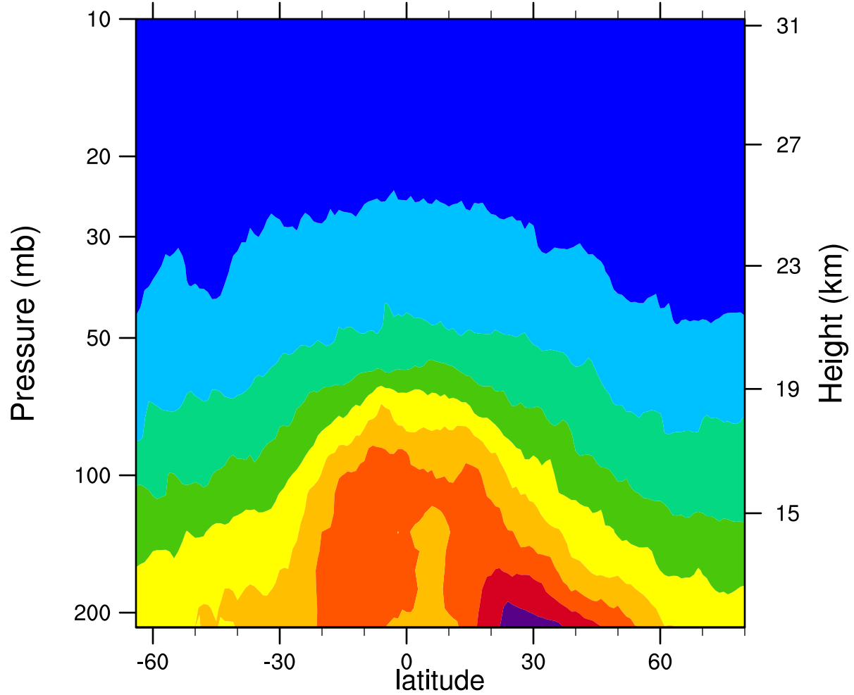
2006d135 12.1MicronExtinction_Combined (km -1 )
