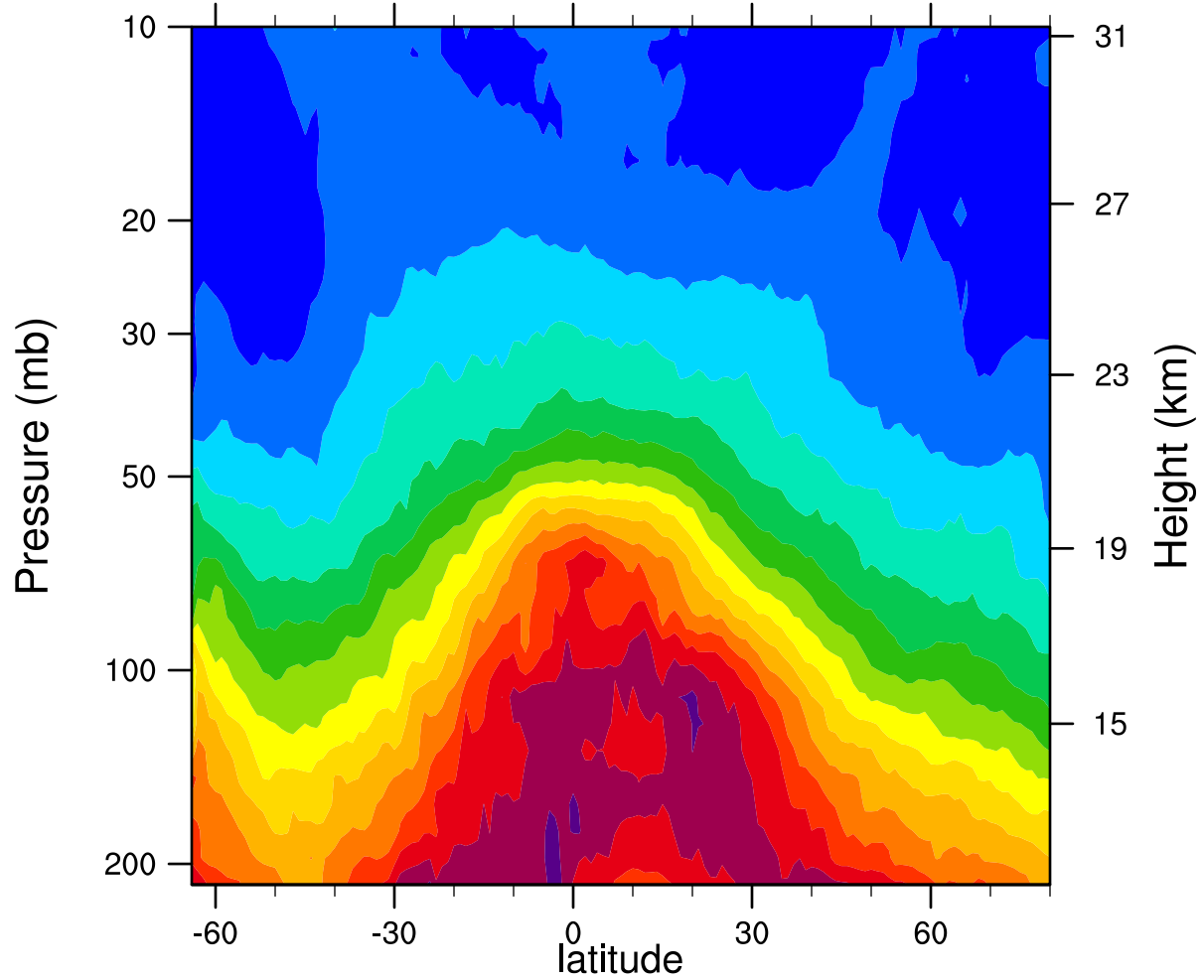
2006d263 12.1MicronExtinction_Combined ( \text{km}^{-1} )
