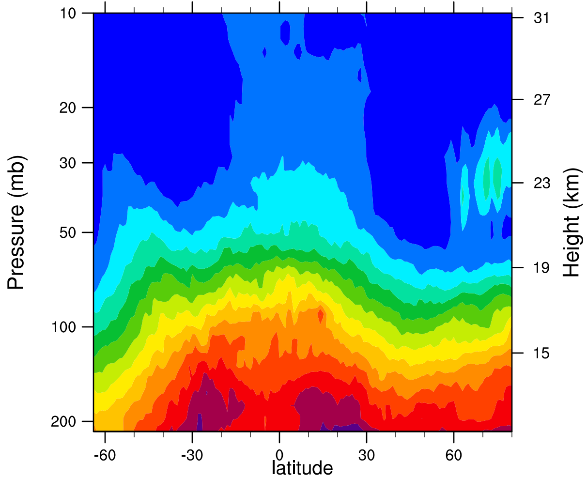
2007d352 12.1MicronExtinction_Combined ( \text{km}^{-1} )
