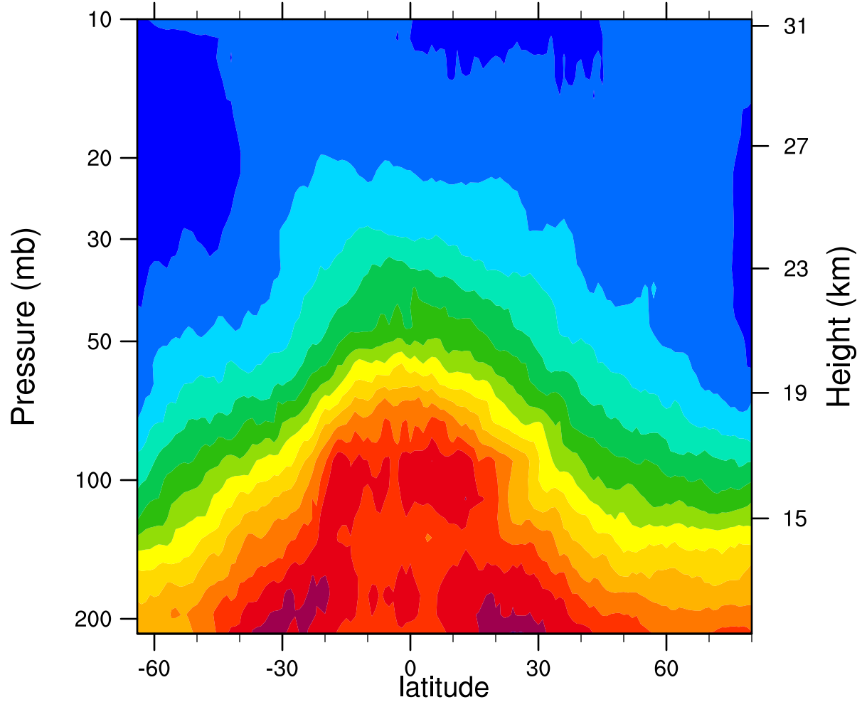
2005d339 12.1MicronExtinction_Combined (km -1 )
