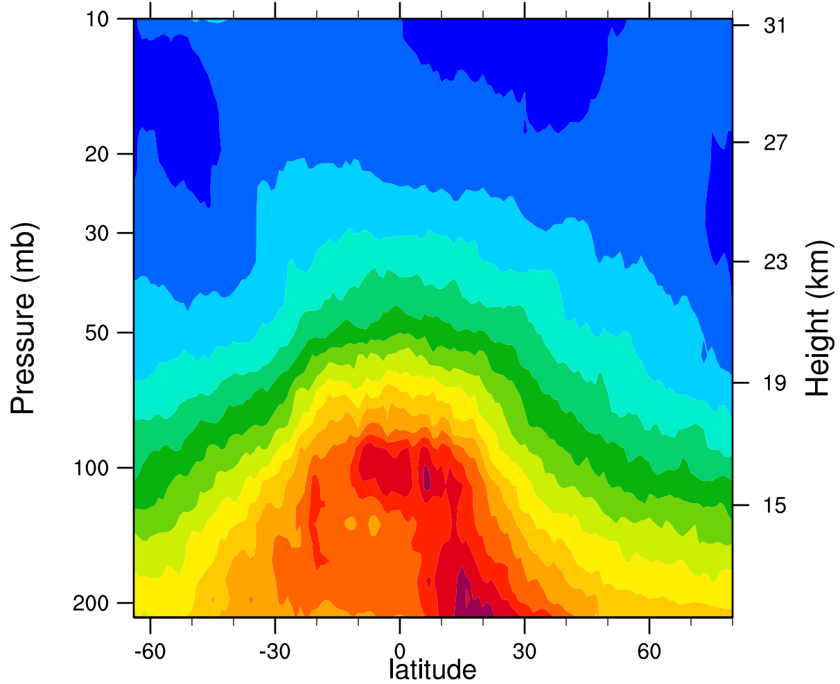
2006d069 12.1MicronExtinction_Combined (km -1 )
