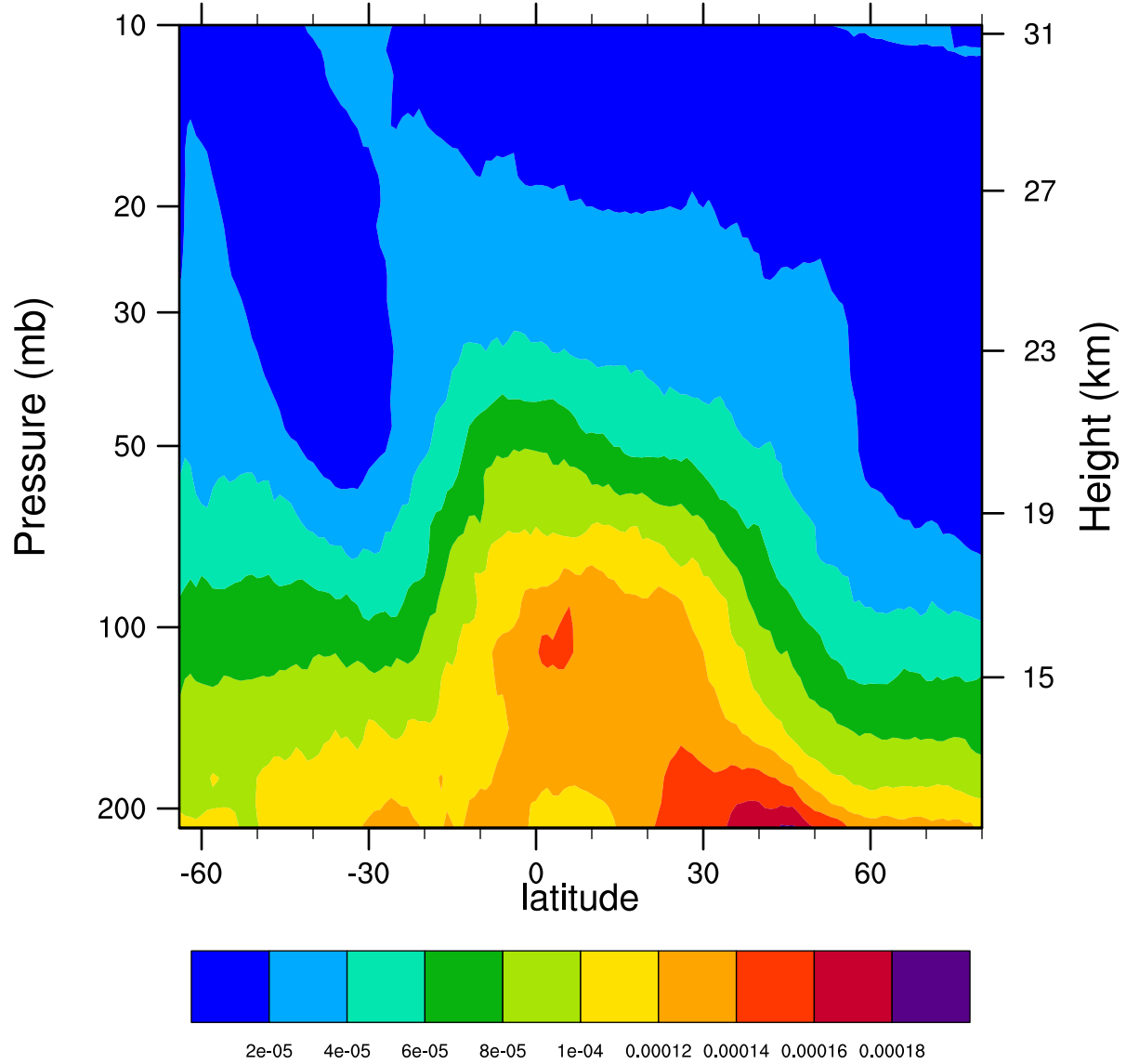
2005d183 12.1MicronExtinction_Combined ( \text{km}^{-1} )
