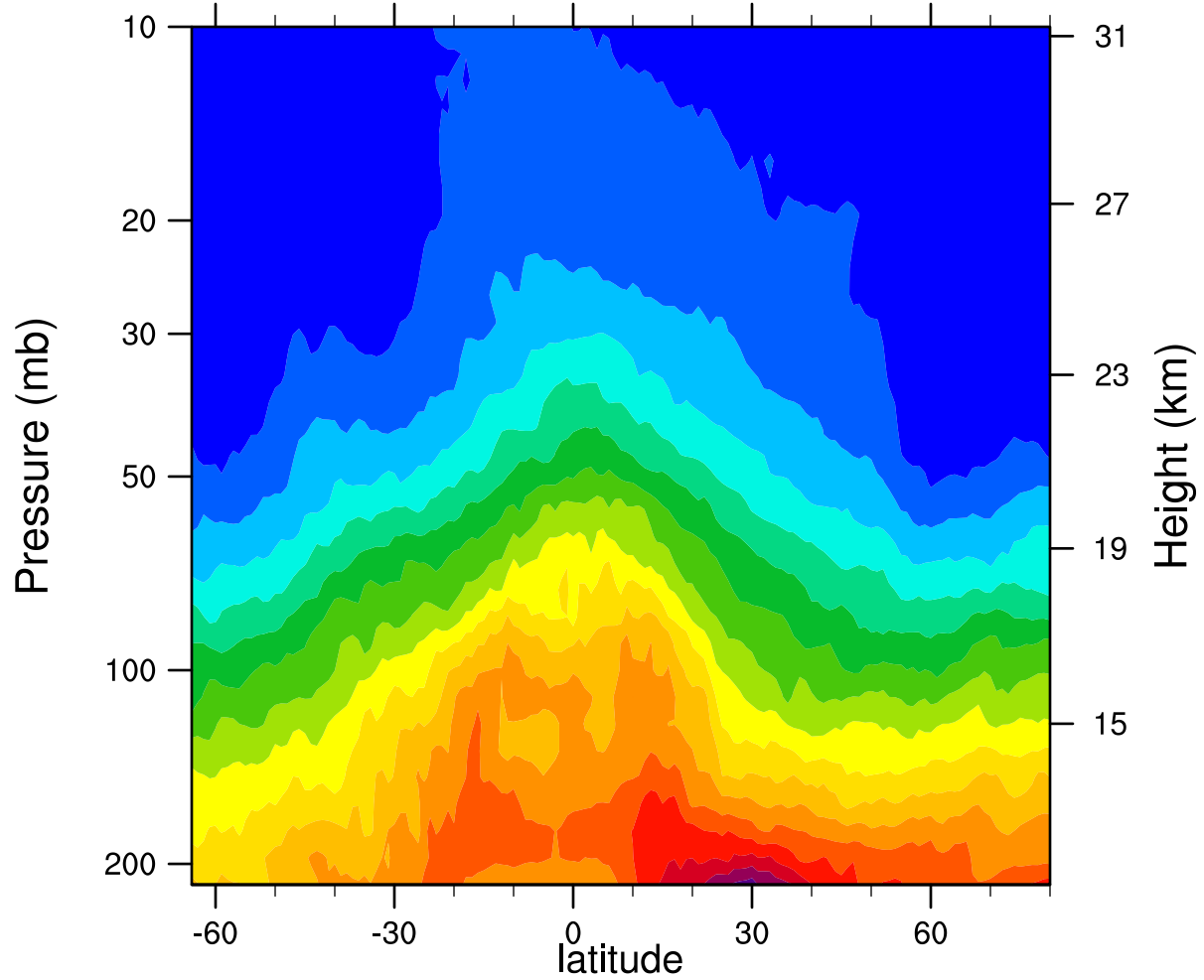
2007d098 12.1MicronExtinction_Combined (km -1 )
