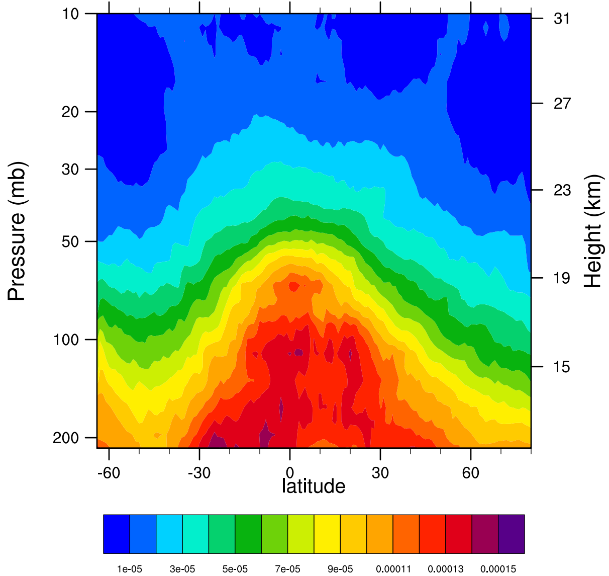
2006d278 12.1MicronExtinction_Combined (km -1 )
