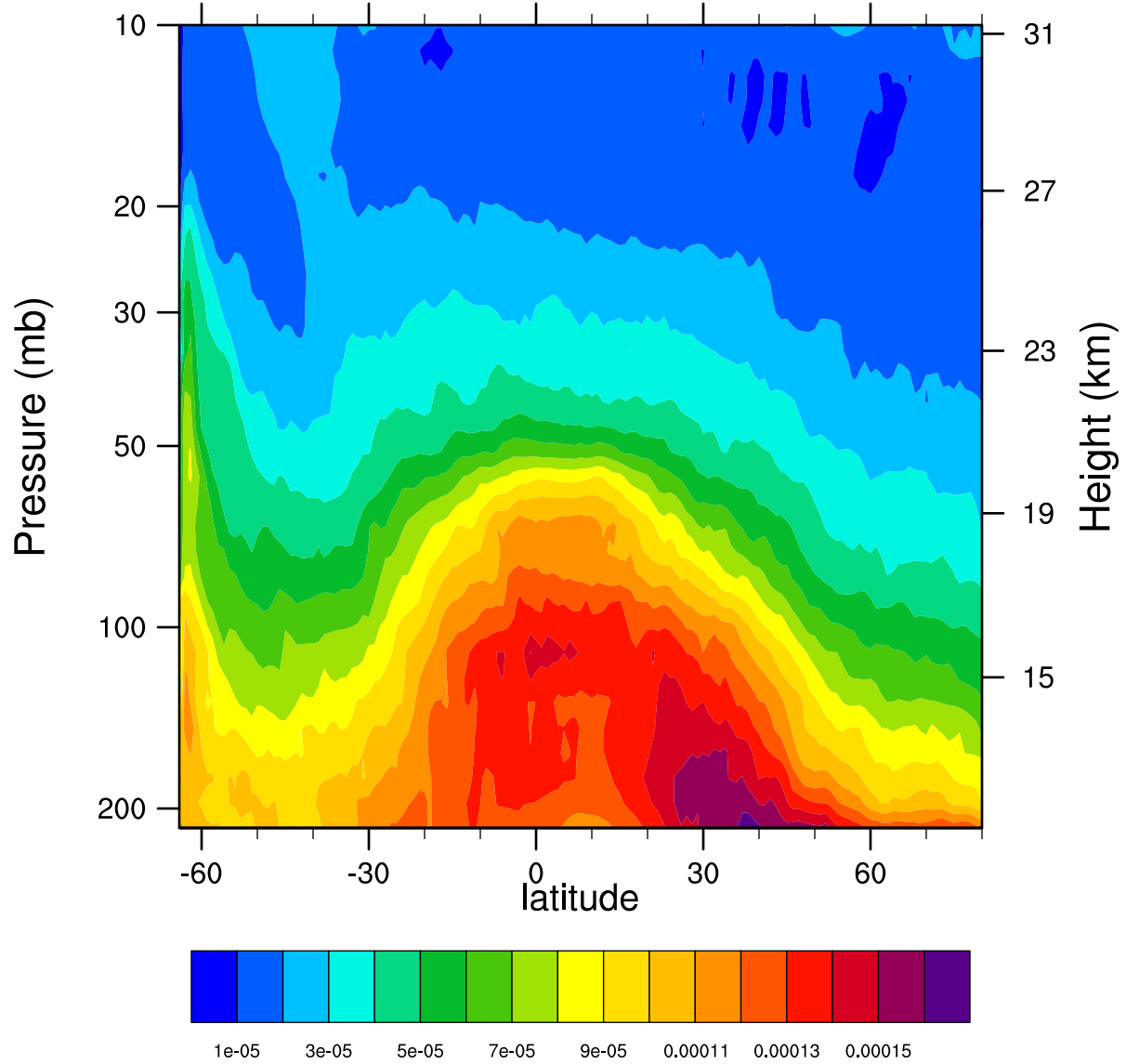
2006d213 12.1MicronExtinction_Combined ( \text{km}^{-1} )
