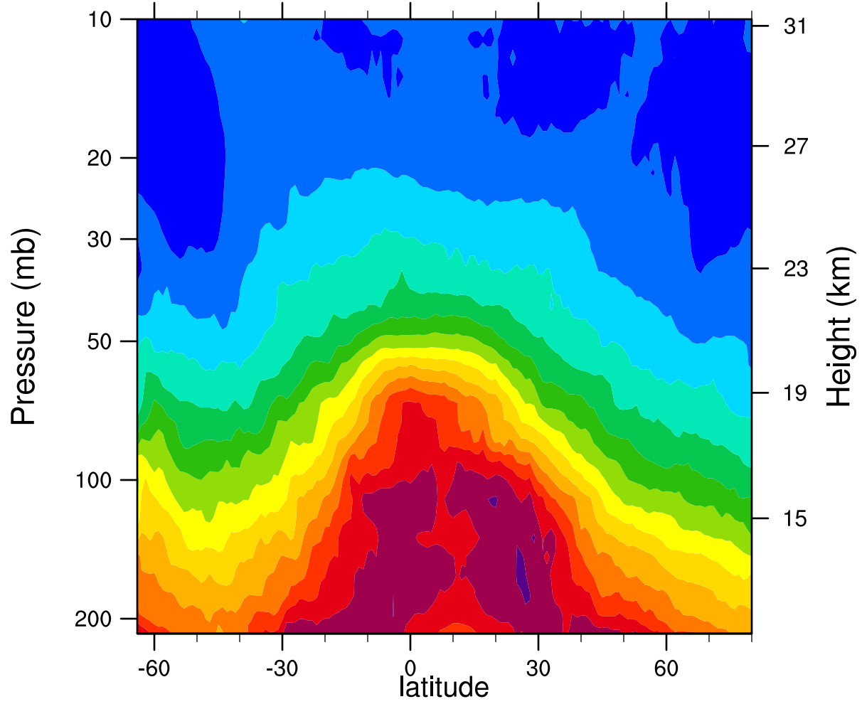
2006d258 12.1MicronExtinction_Combined ( \text{km}^{-1} )
