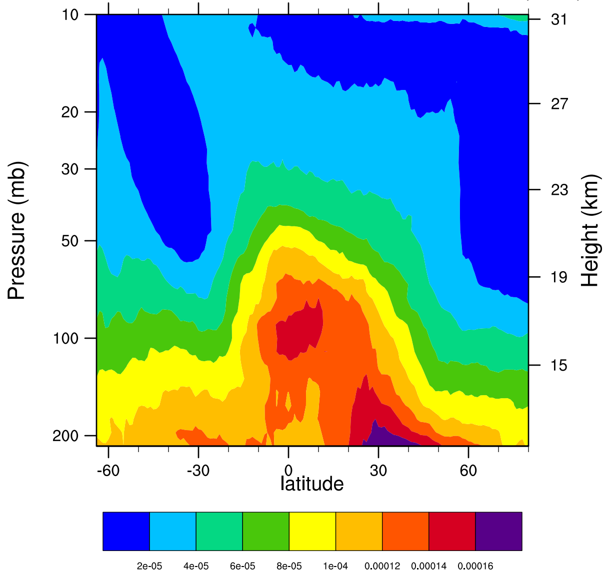
2005d158 12.1MicronExtinction_Combined (km -1 )
