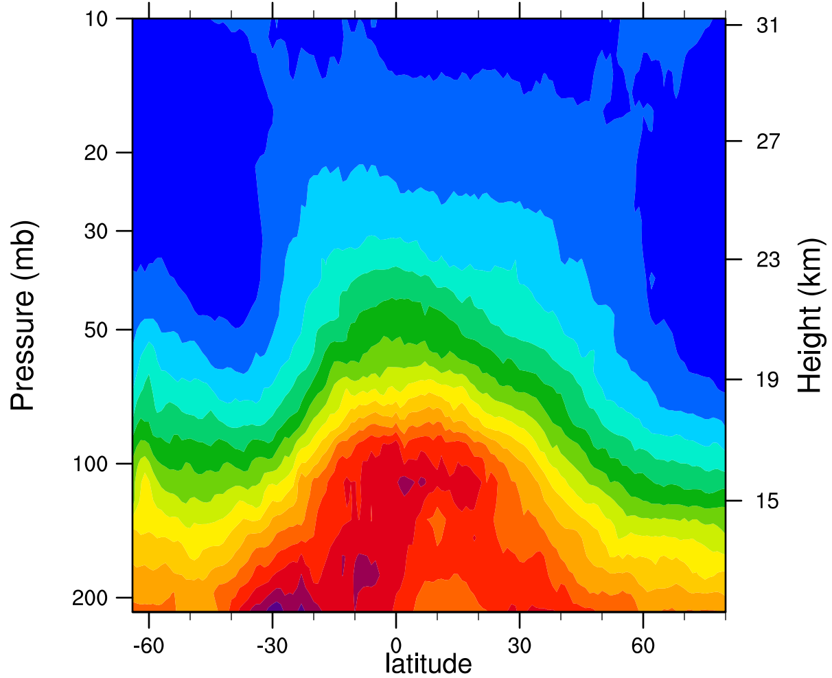
2005d279 12.1MicronExtinction_Combined (km -1 )
