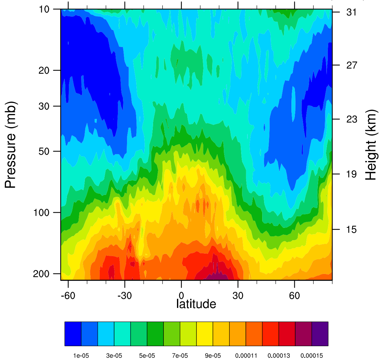
2005d027 12.1MicronExtinction_Combined (km -1 )
