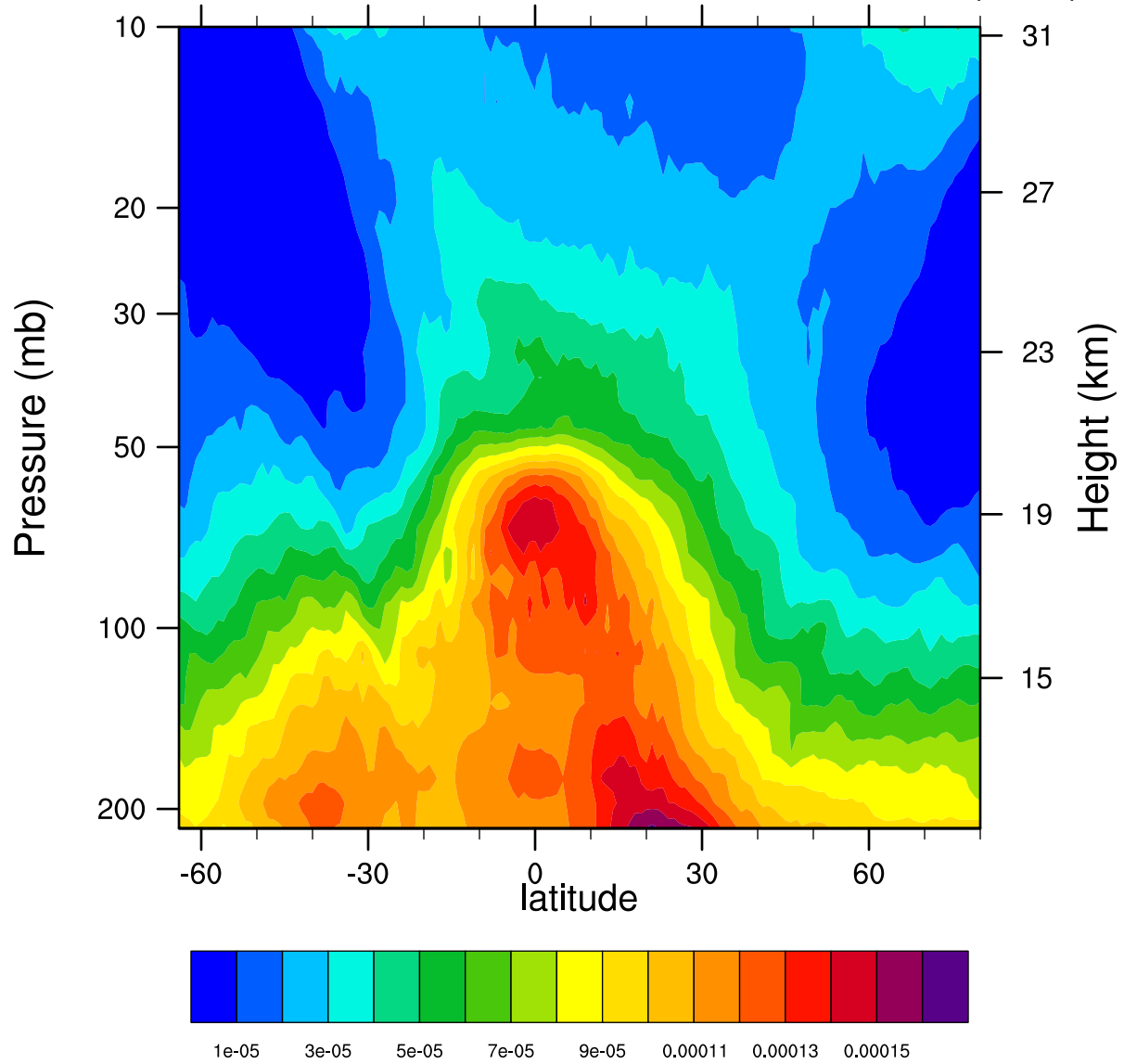
2005d084 12.1MicronExtinction_Combined ( \text{km}^{-1} )
