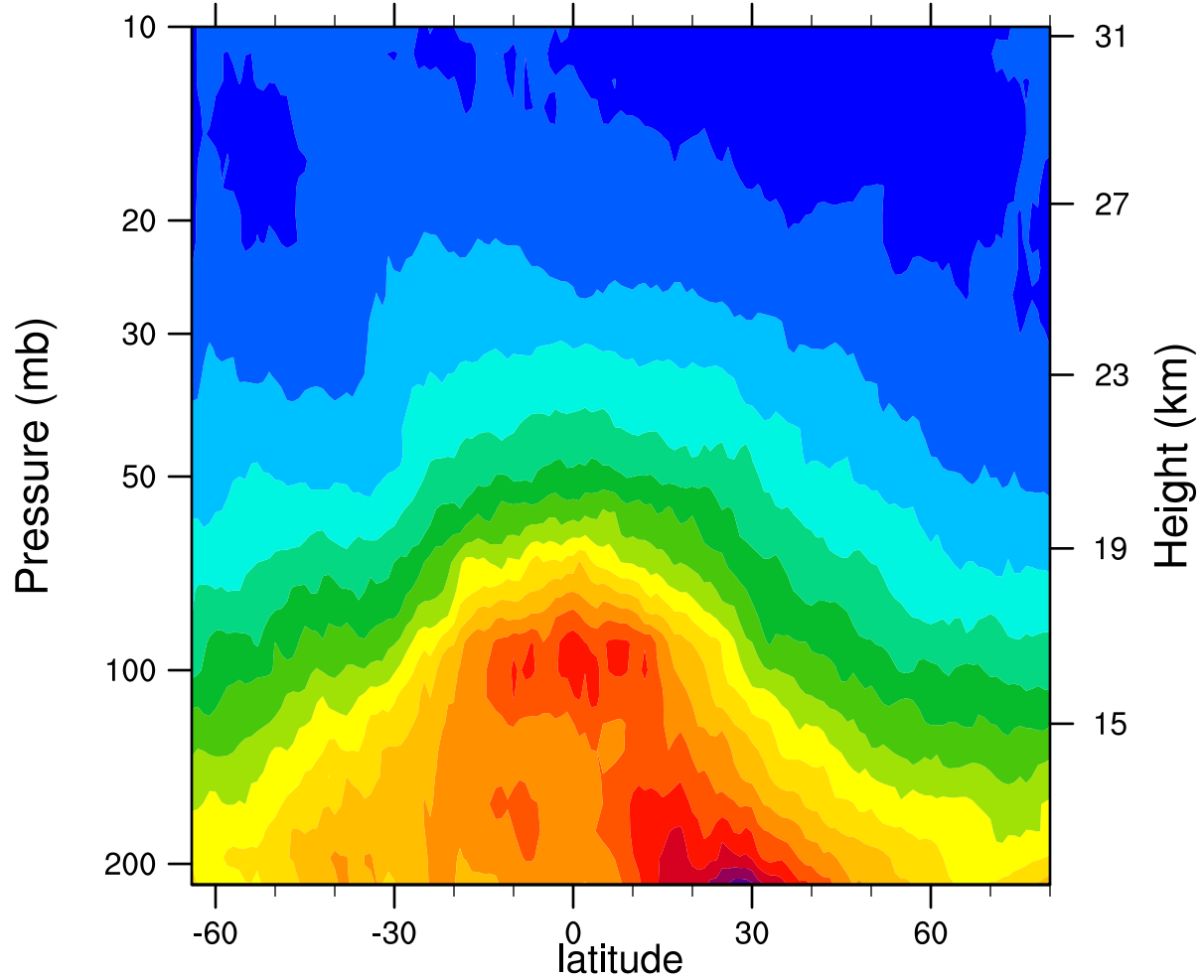
2006d096 12.1MicronExtinction_Combined (km -1 )
