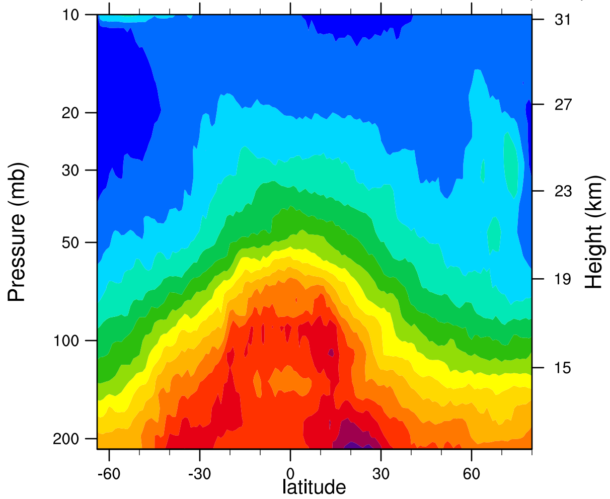
2006d005 12.1MicronExtinction_Combined (km -1 )
