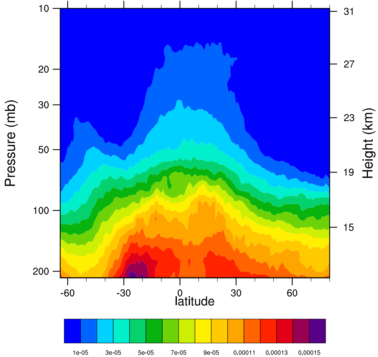
2007d308 12.1MicronExtinction_Combined (km -1 )
