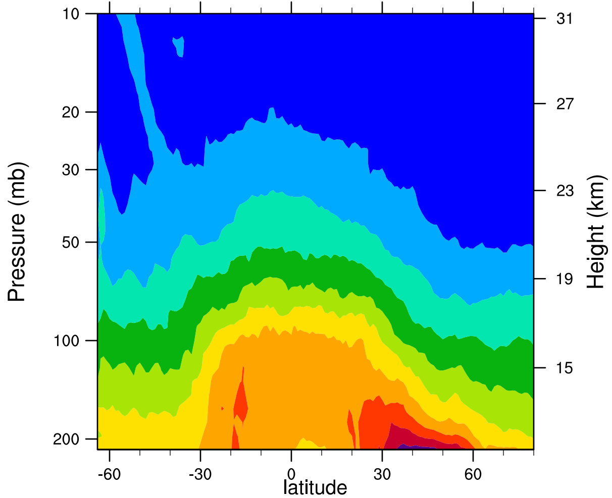
2007d168 12.1MicronExtinction_Combined (km -1 )
