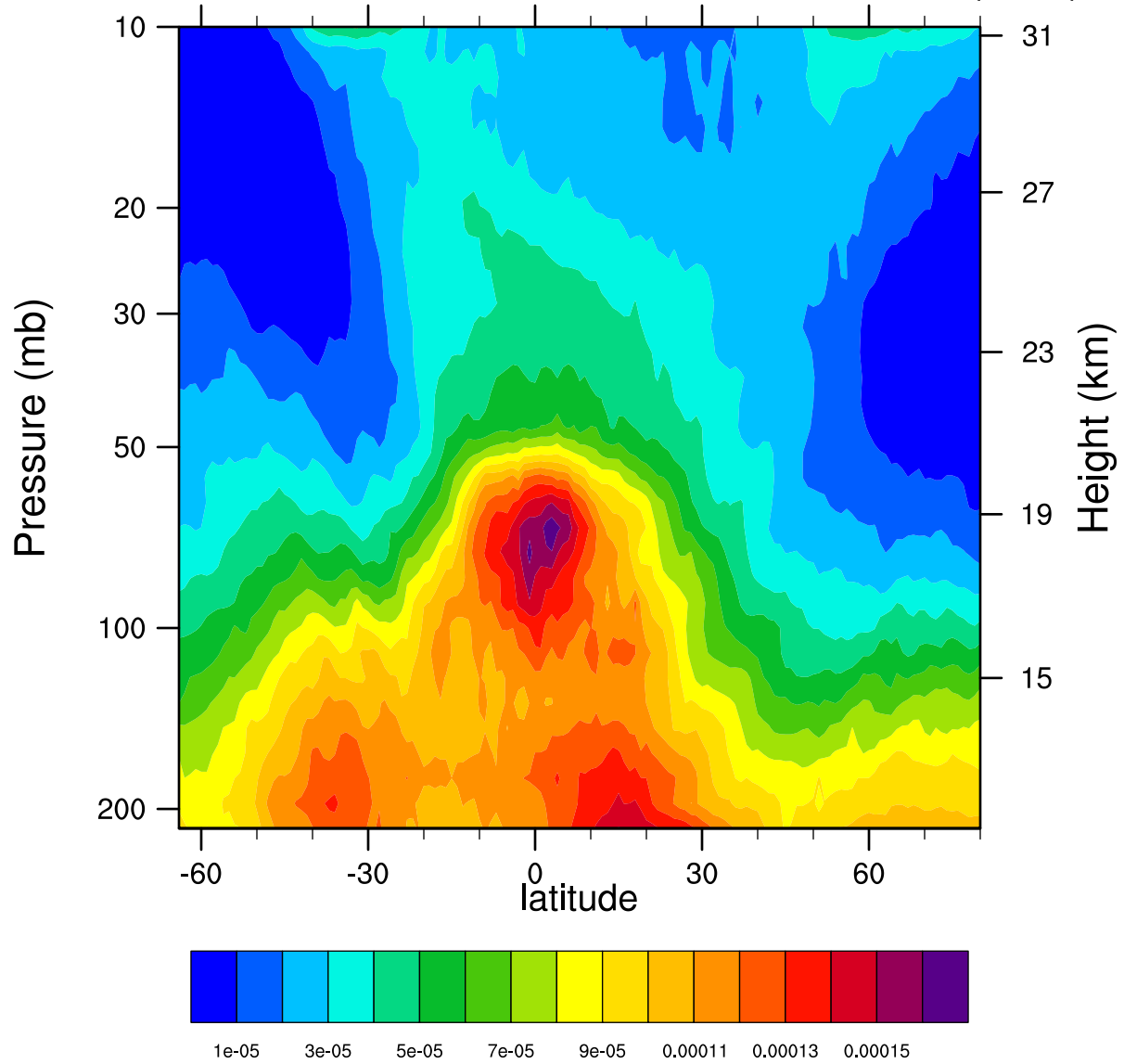
2005d058 12.1MicronExtinction_Combined (km -1 )
