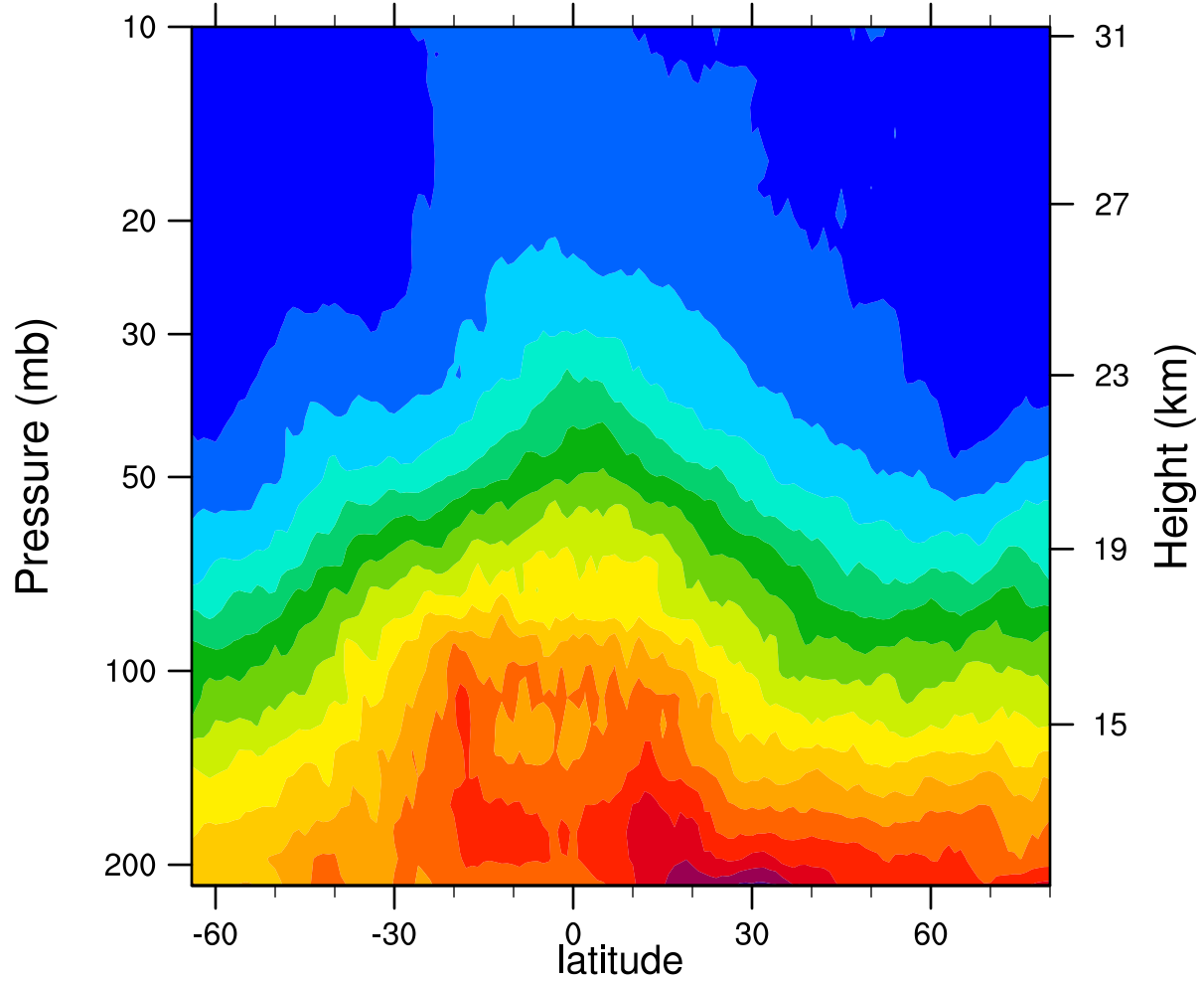
2007d088 12.1MicronExtinction_Combined (km -1 )
