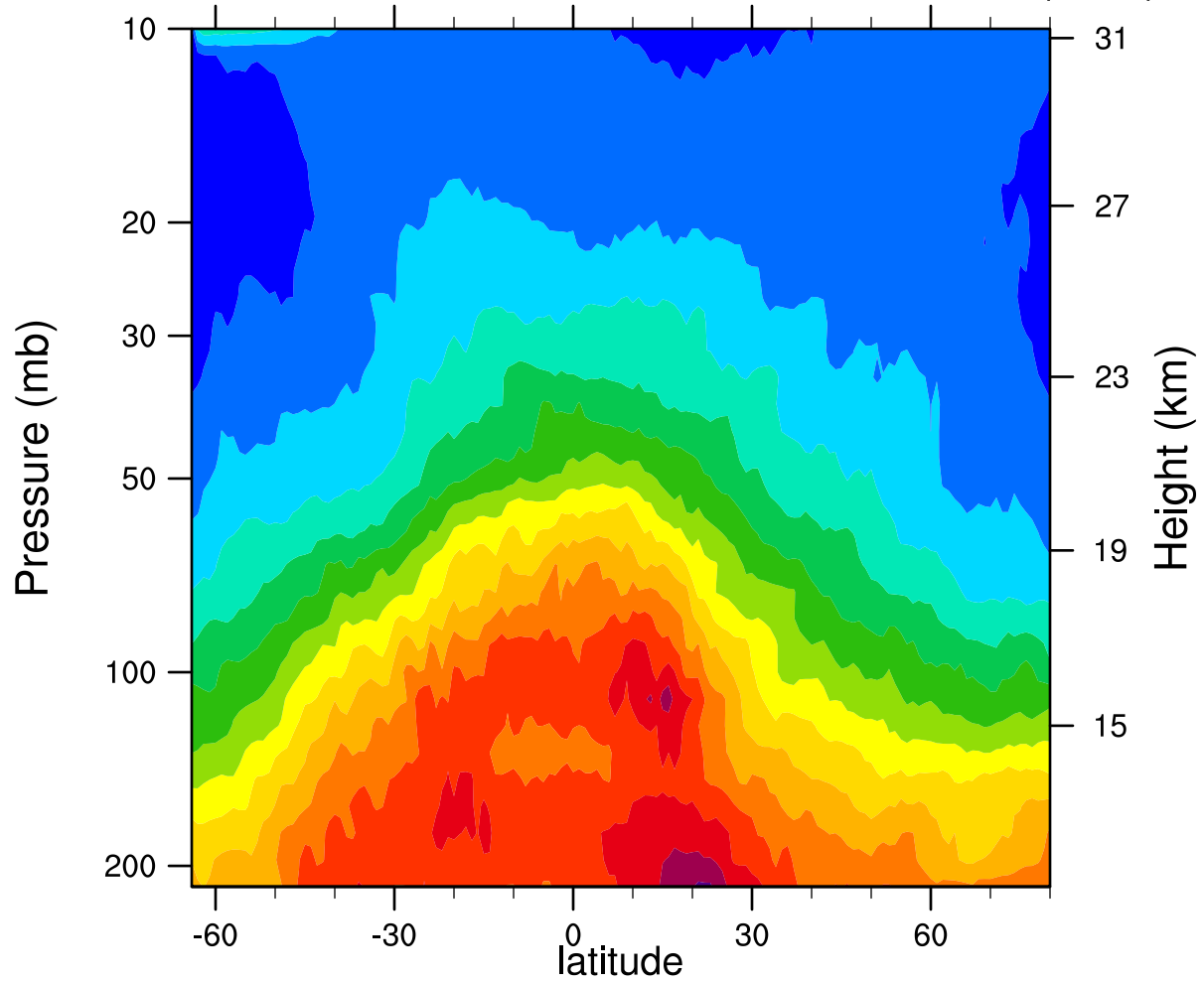
2006d015 12.1MicronExtinction_Combined (km -1 )
