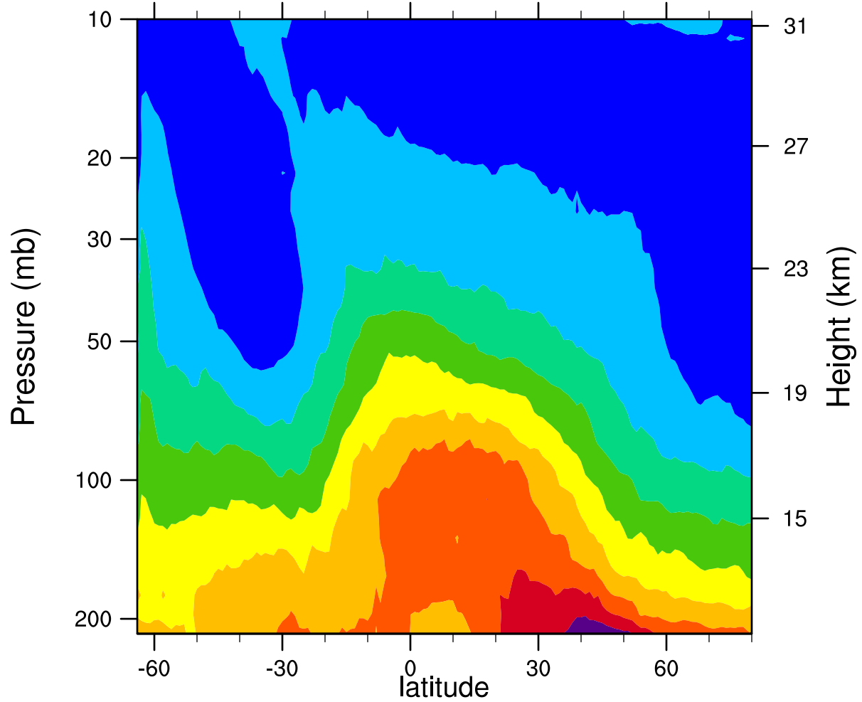
2005d190 12.1MicronExtinction_Combined (km -1 )
