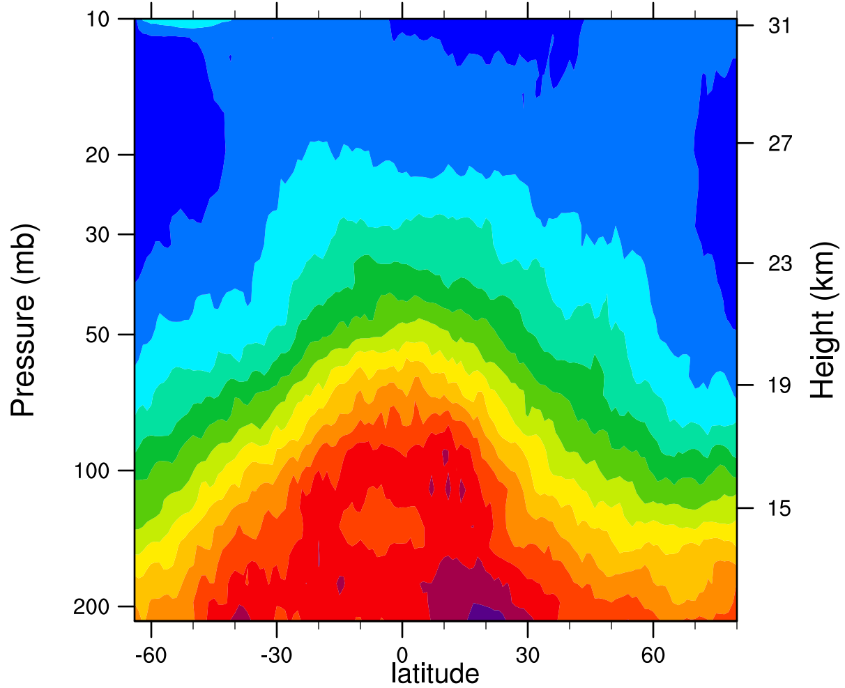
2006d018 12.1MicronExtinction_Combined ( \text{km}^{-1} )
