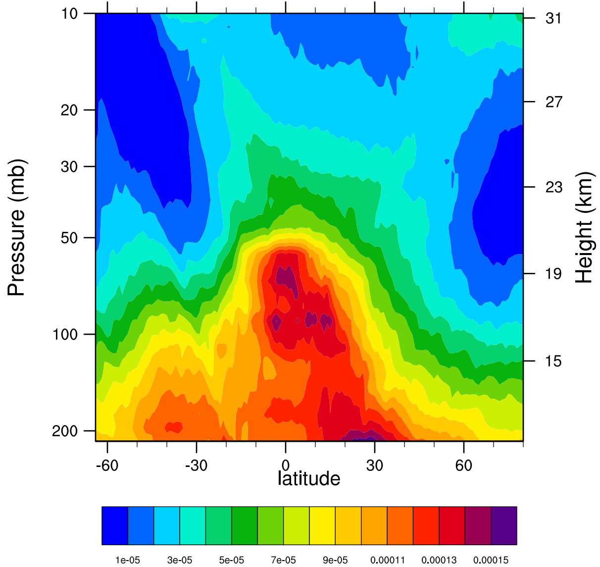
2005d099 12.1MicronExtinction_Combined (km -1 )
