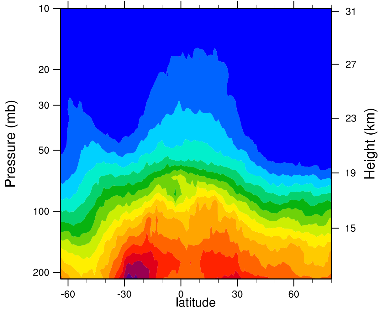
2007d313 12.1MicronExtinction_Combined (km -1 )
