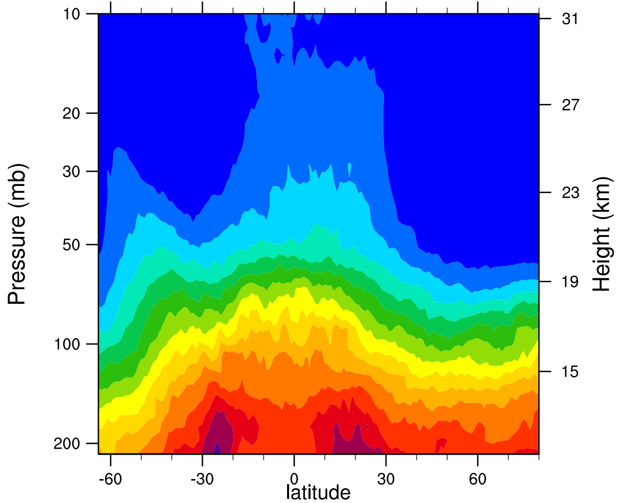
2007d343 12.1MicronExtinction_Combined (km -1 )
