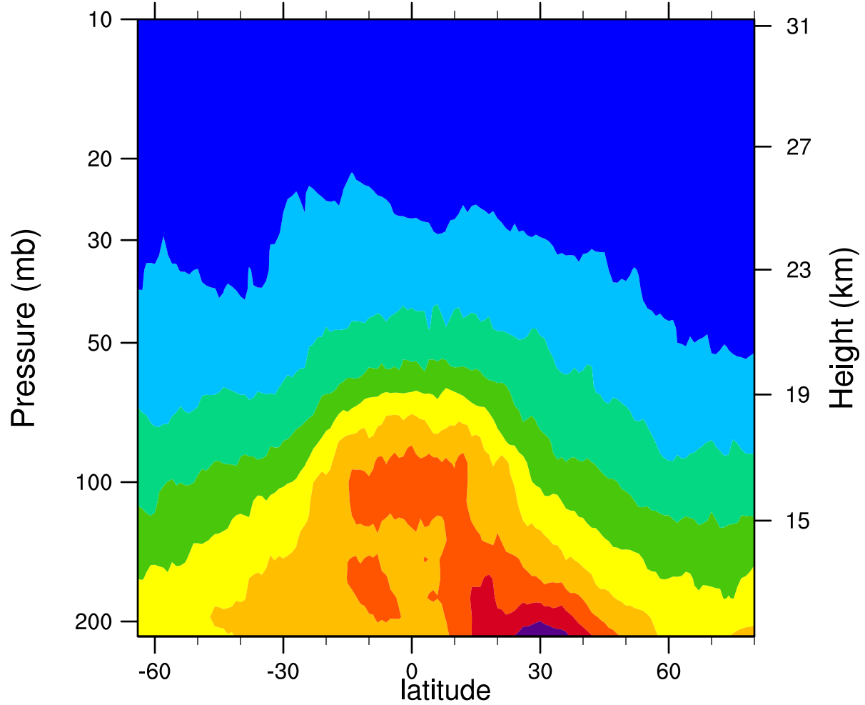
2006d106 12.1MicronExtinction_Combined (km -1 )
