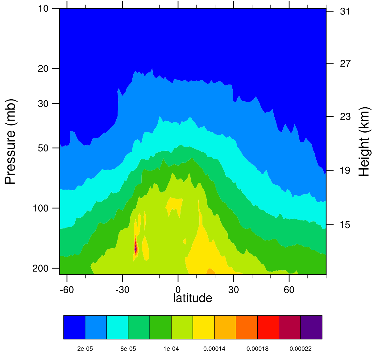
2006d055 12.1MicronExtinction_Combined ( \text{km}^{-1} )
