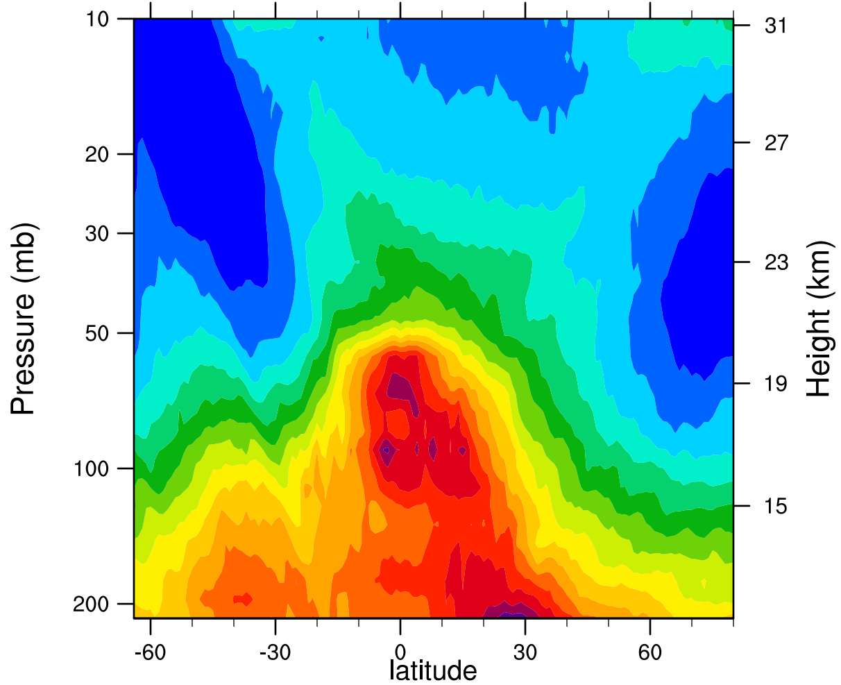
2005d098 12.1MicronExtinction_Combined ( \text{km}^{-1} )
