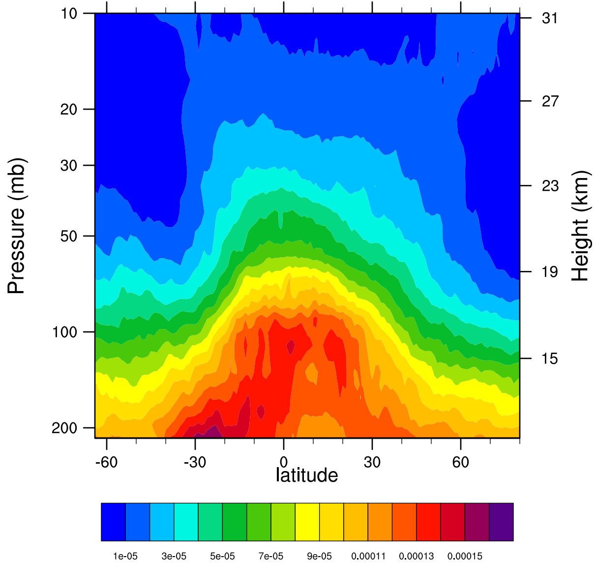
2005d285 12.1MicronExtinction_Combined (km -1 )
