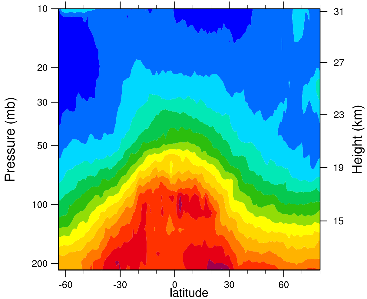
2005d355 12.1MicronExtinction_Combined (km -1 )
