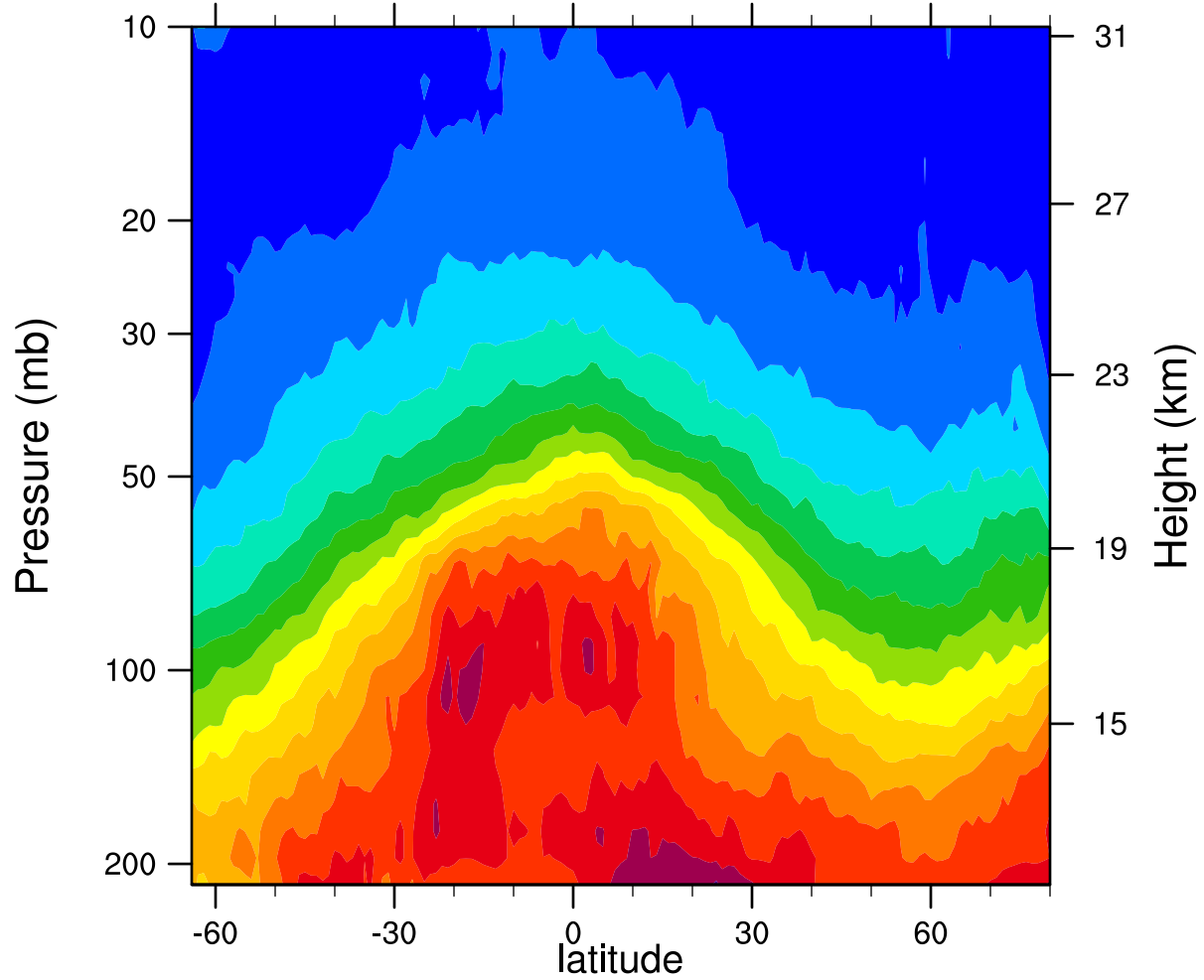
2007d039 12.1MicronExtinction_Combined (km -1 )
