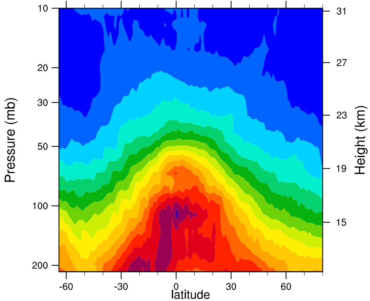
2006d285 12.1MicronExtinction_Combined (km -1 )
