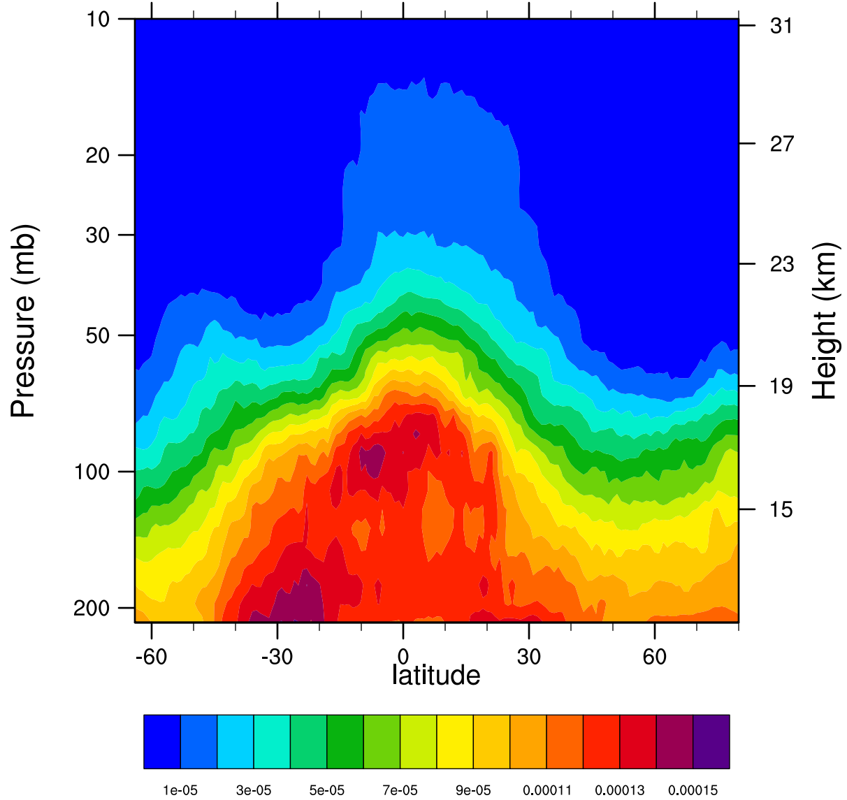
2006d334 12.1MicronExtinction_Combined (km -1 )
