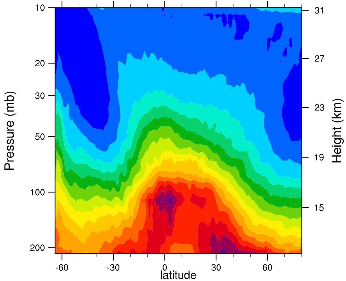
2005d219 12.1MicronExtinction_Combined (km -1 )
