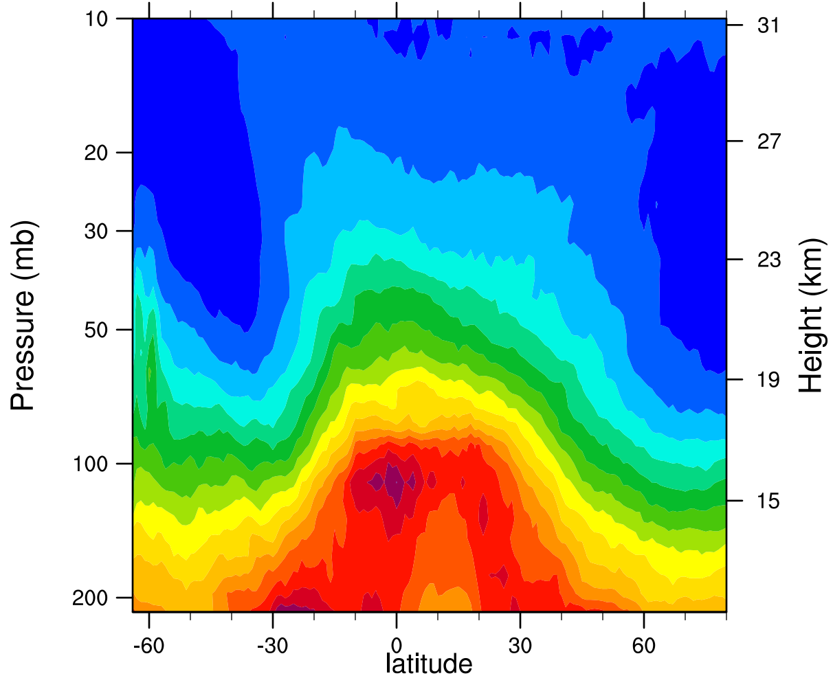
2005d254 12.1MicronExtinction_Combined (km -1 )
