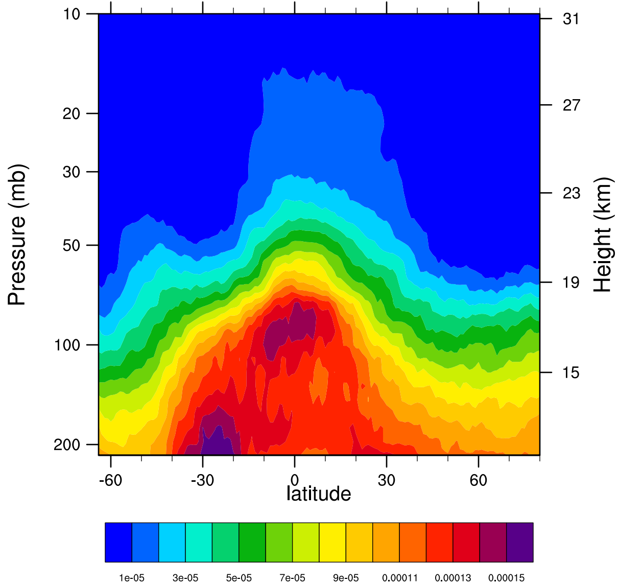
2006d326 12.1MicronExtinction_Combined (km -1 )
