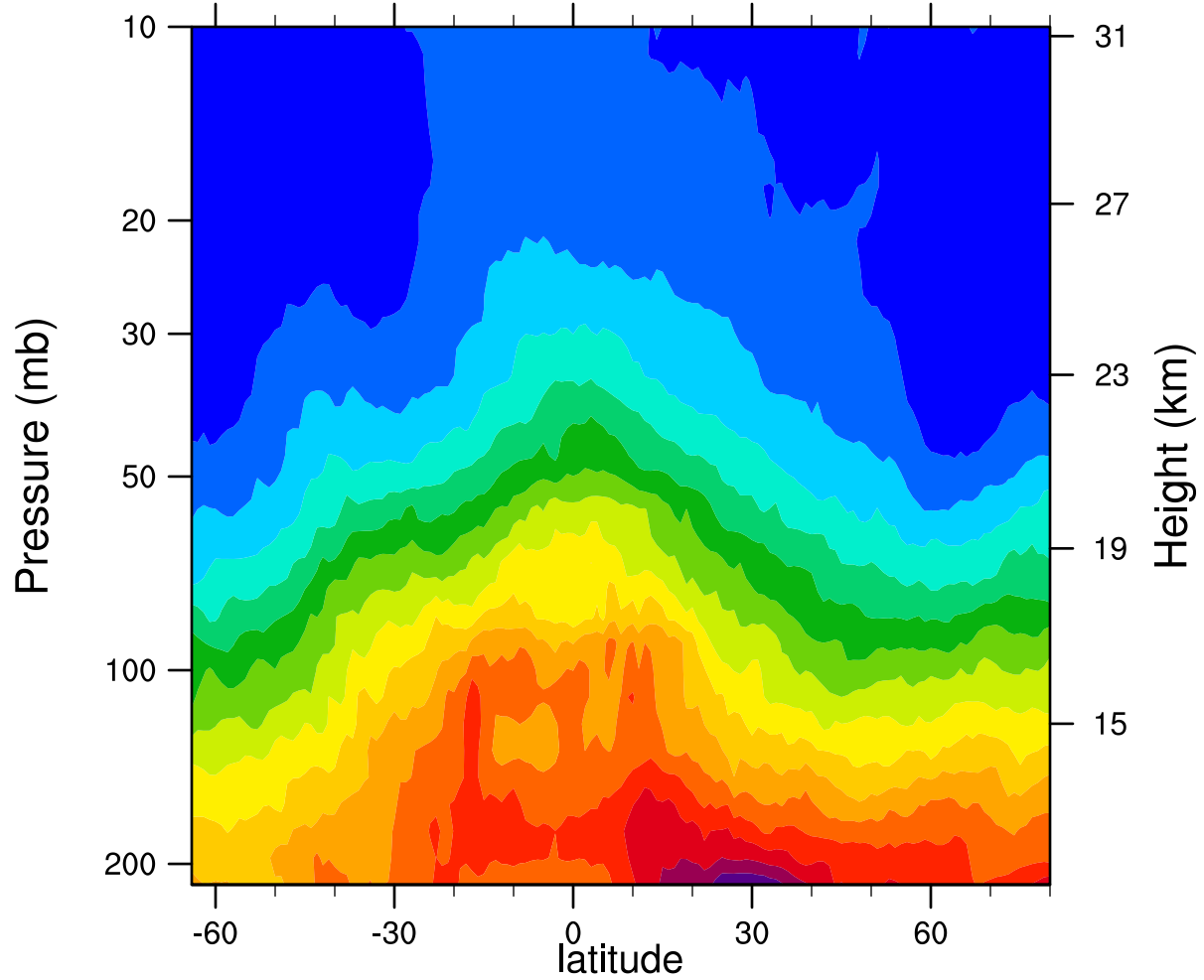
2007d094 12.1MicronExtinction_Combined (km -1 )
