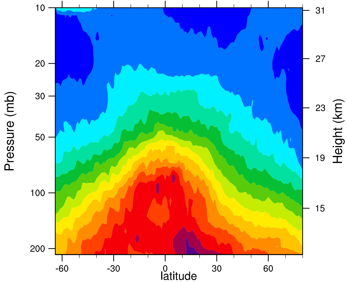
2006d041 12.1MicronExtinction_Combined (km -1 )
