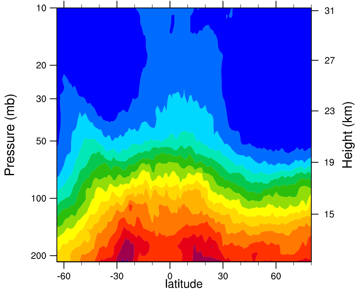
2007d346 12.1MicronExtinction_Combined (km -1 )
