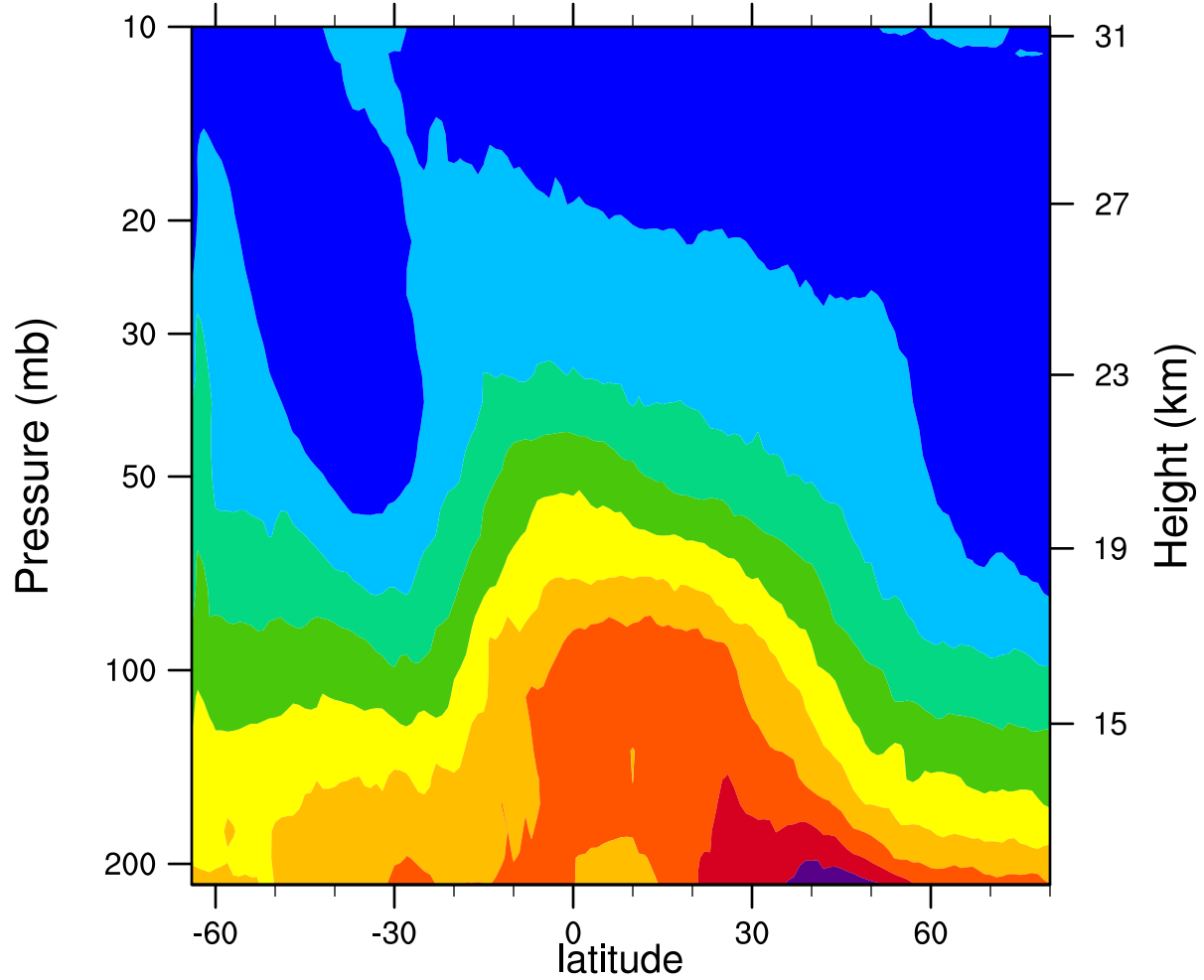
2005d189 12.1MicronExtinction_Combined (km -1 )
