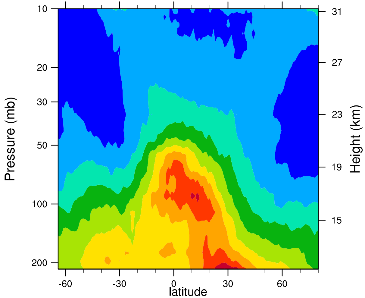
2005d115 12.1MicronExtinction_Combined (km -1 )
