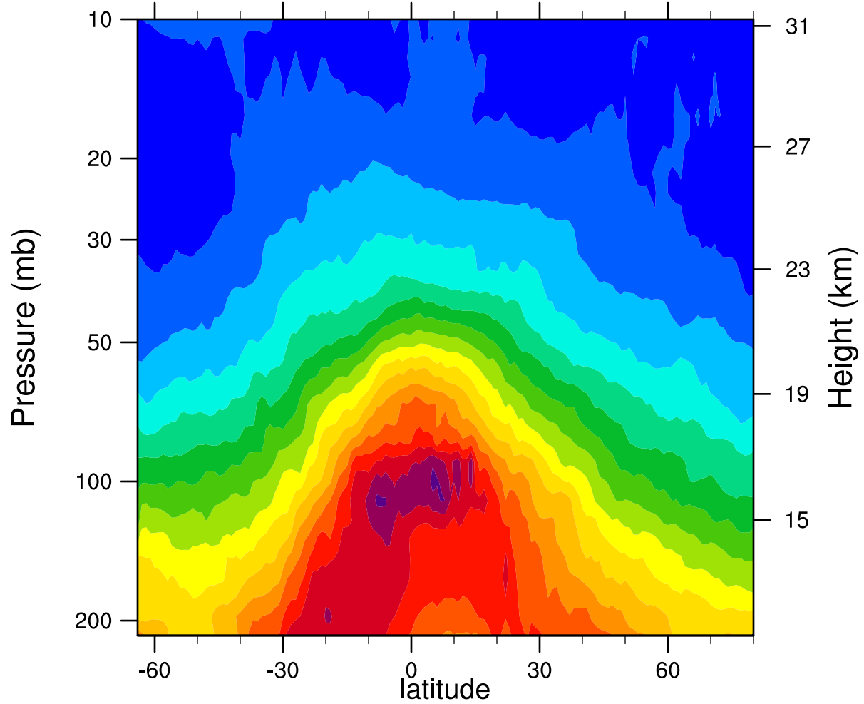
2006d294 12.1MicronExtinction_Combined (km -1 )
