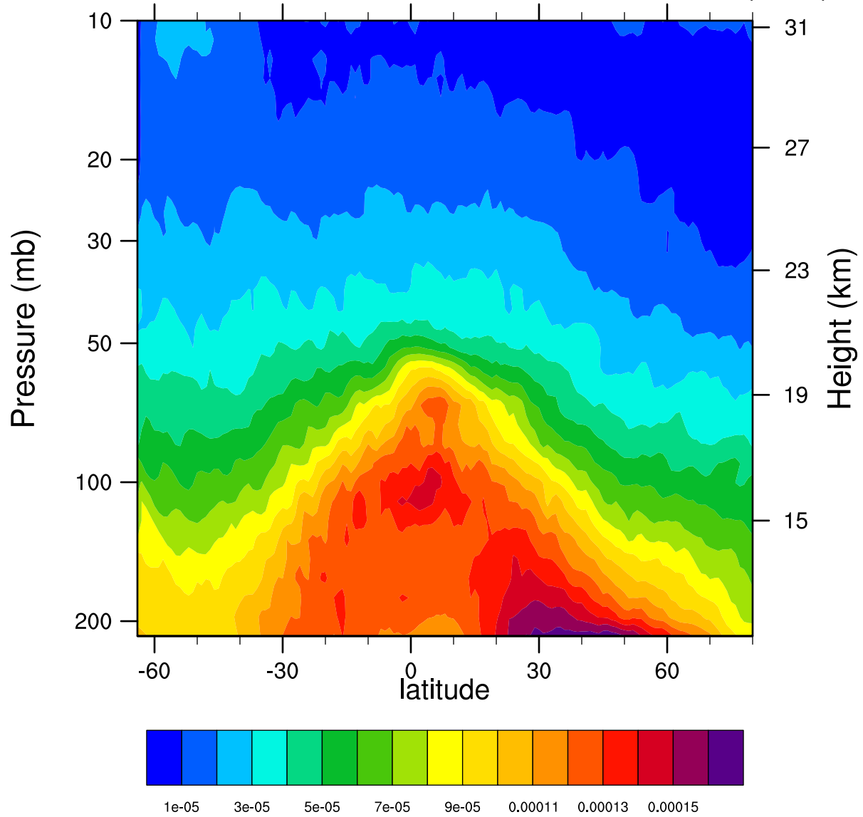
2006d172 12.1MicronExtinction_Combined ( \text{km}^{-1} )
