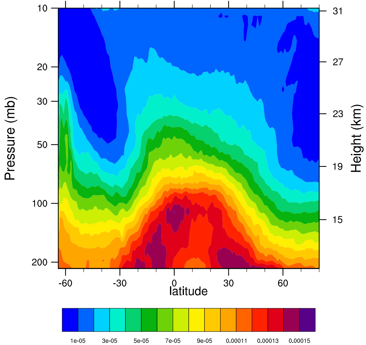
2005d234 12.1MicronExtinction_Combined ( \text{km}^{-1} )
