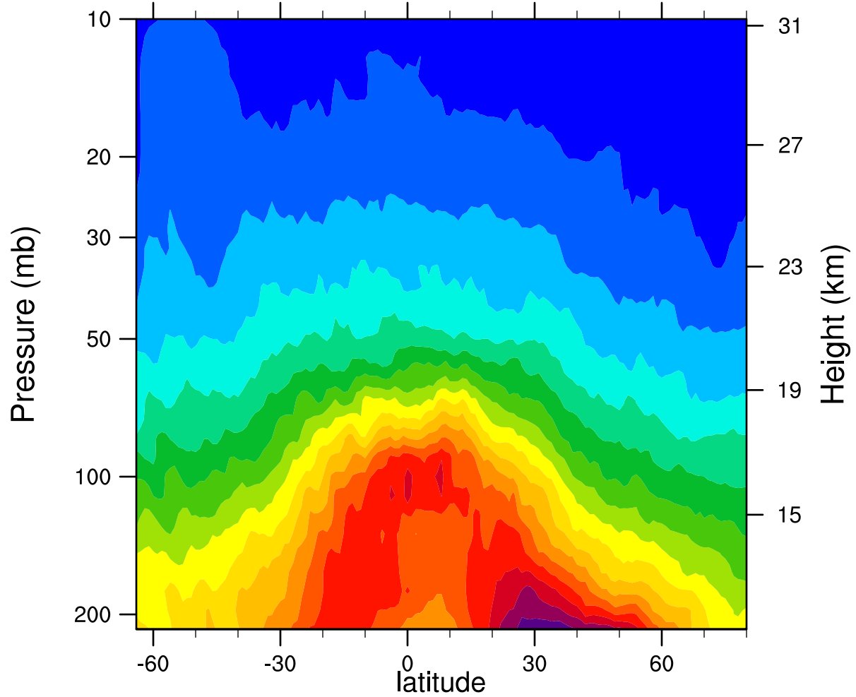
2006d153 12.1MicronExtinction_Combined (km -1 )
