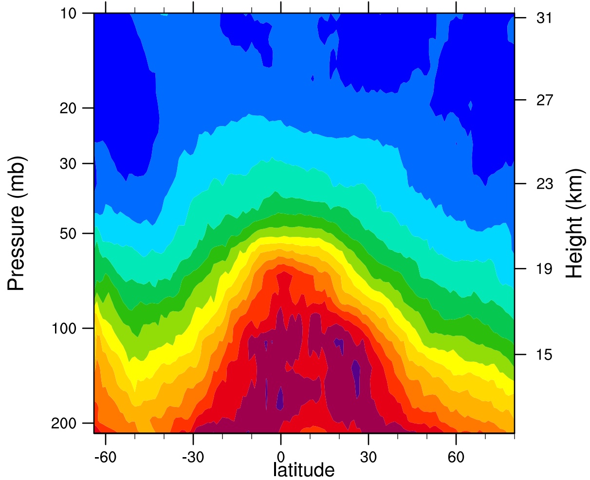
2006d261 12.1MicronExtinction_Combined (km -1 )
