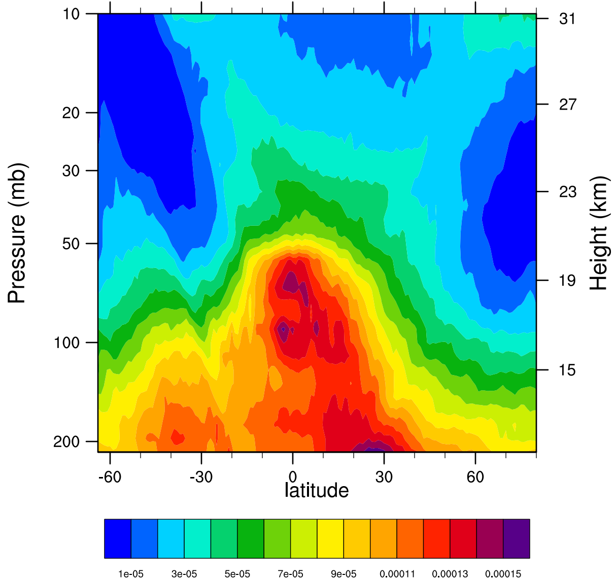
2005d097 12.1MicronExtinction_Combined (km -1 )
