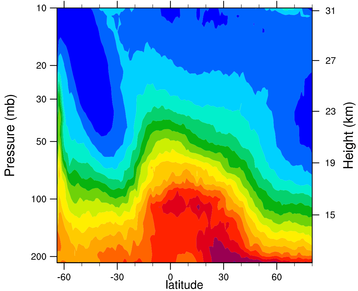
2005d205 12.1MicronExtinction_Combined ( \text{km}^{-1} )
