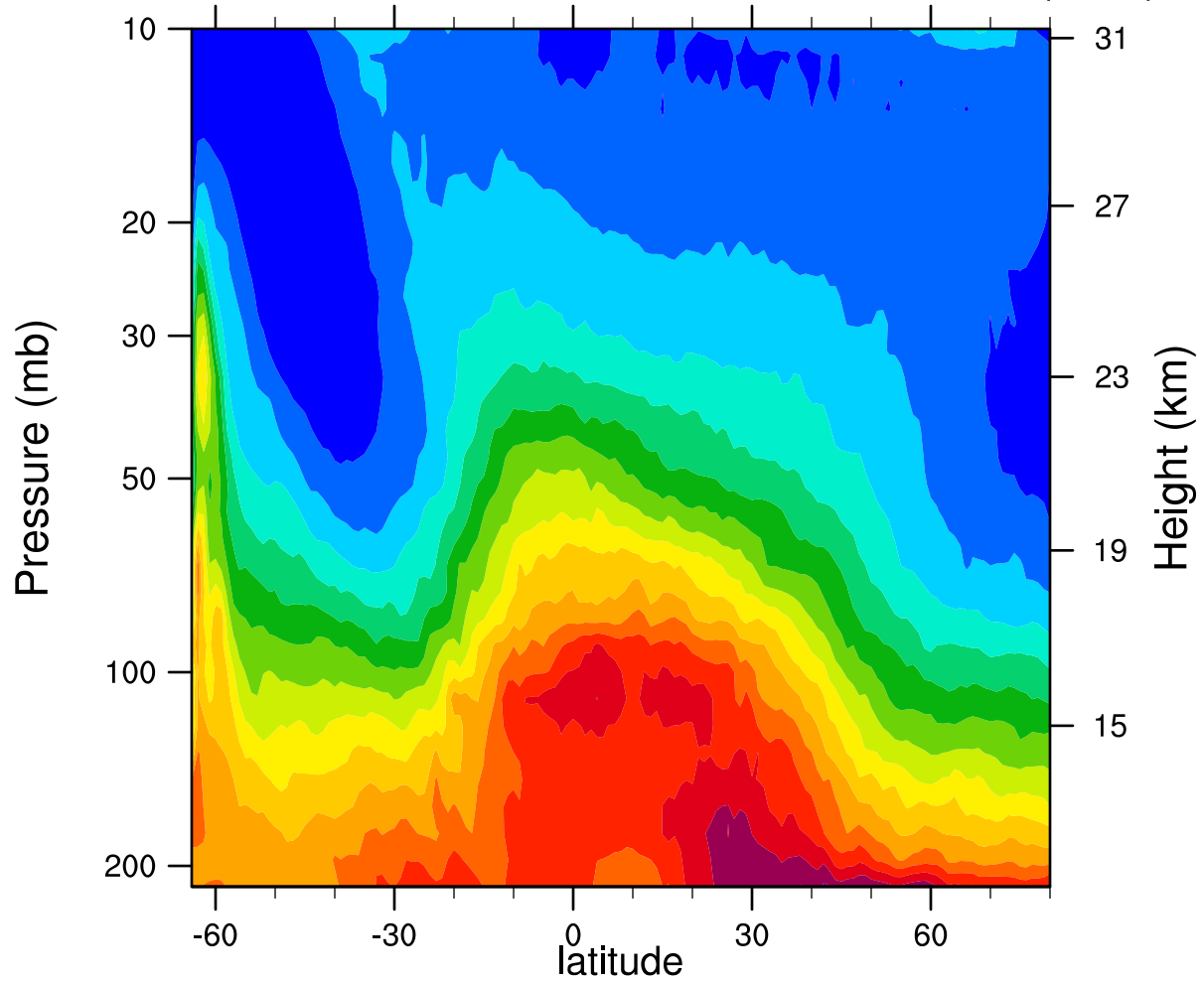
2005d207 12.1MicronExtinction_Combined (km -1 )
