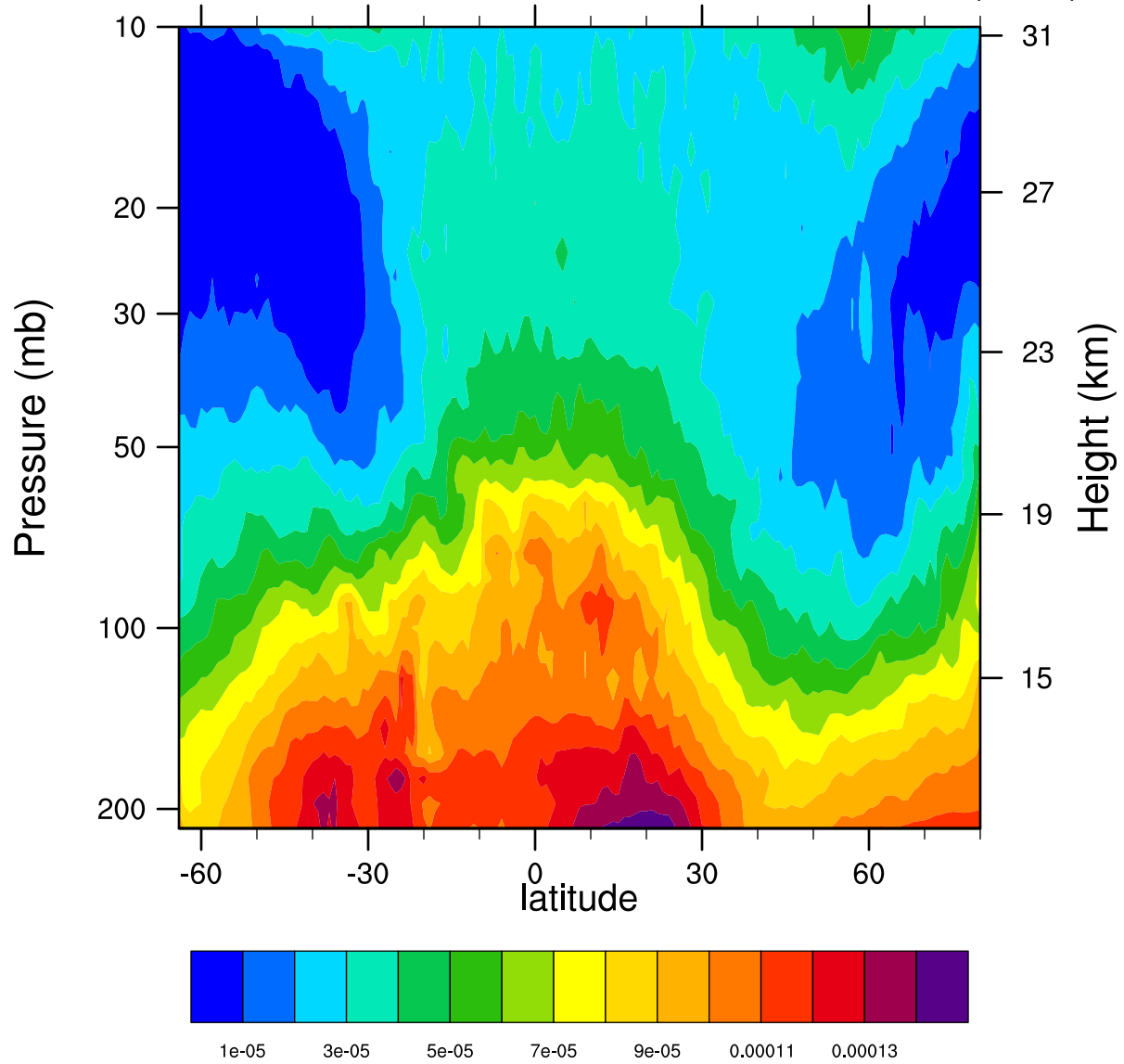
2005d028 12.1MicronExtinction_Combined (km -1 )
