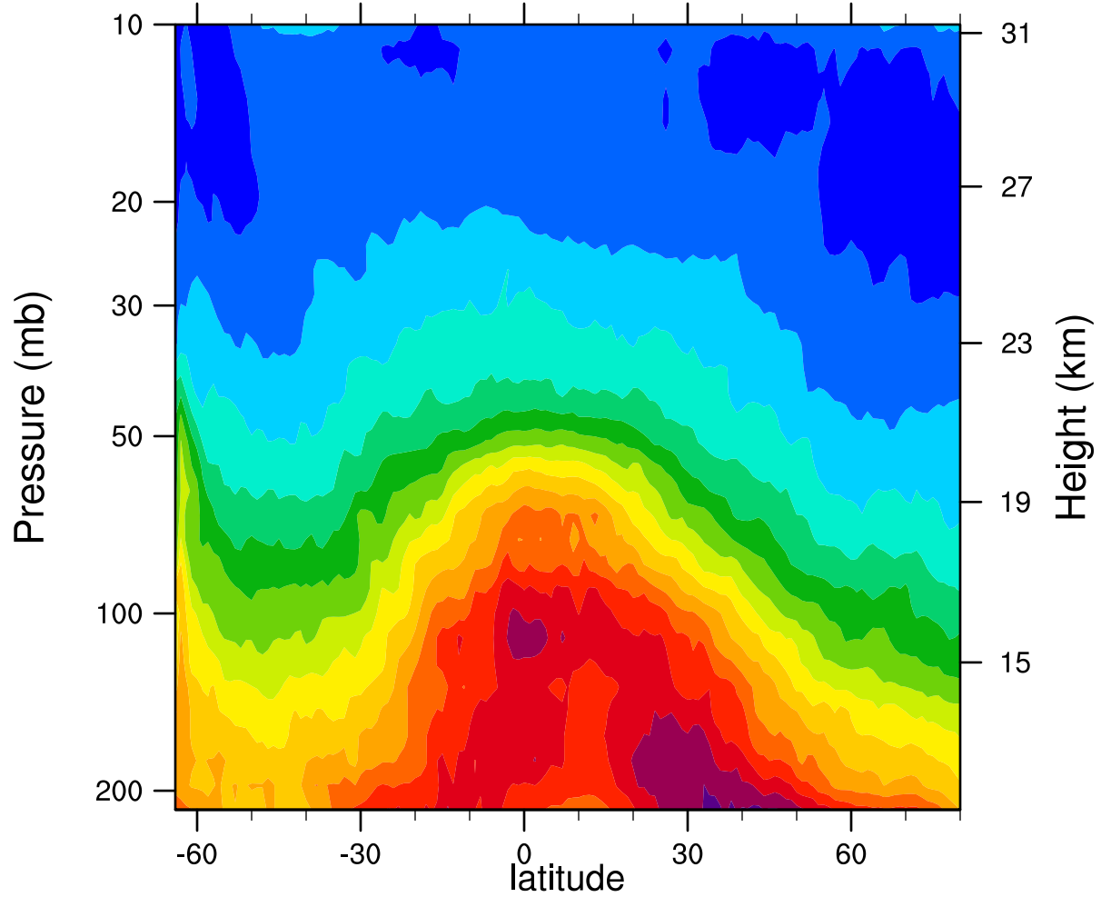
2006d232 12.1MicronExtinction_Combined (km -1 )
