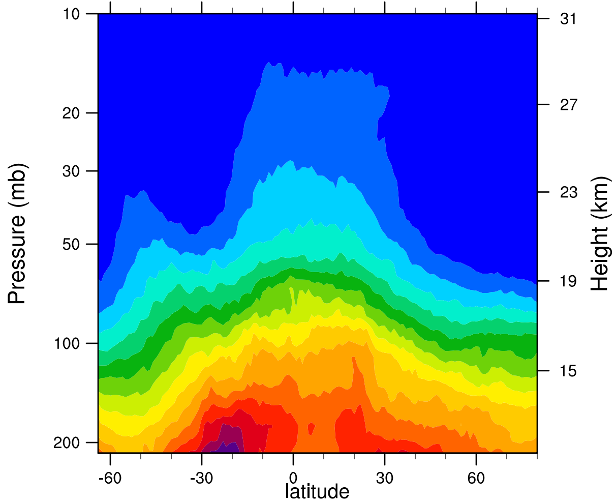
2007d301 12.1MicronExtinction_Combined (km -1 )
