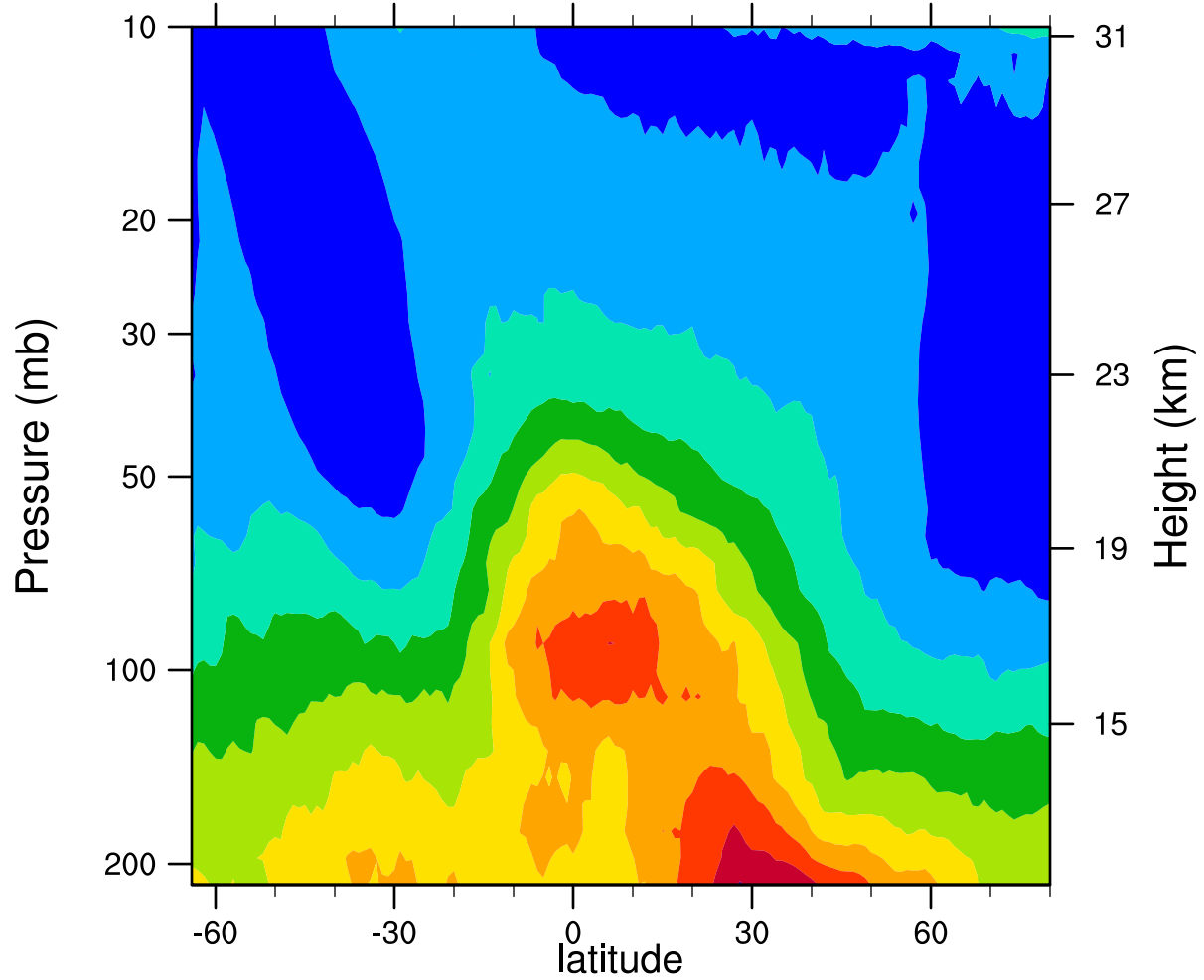
2005d147 12.1MicronExtinction_Combined (km -1 )
