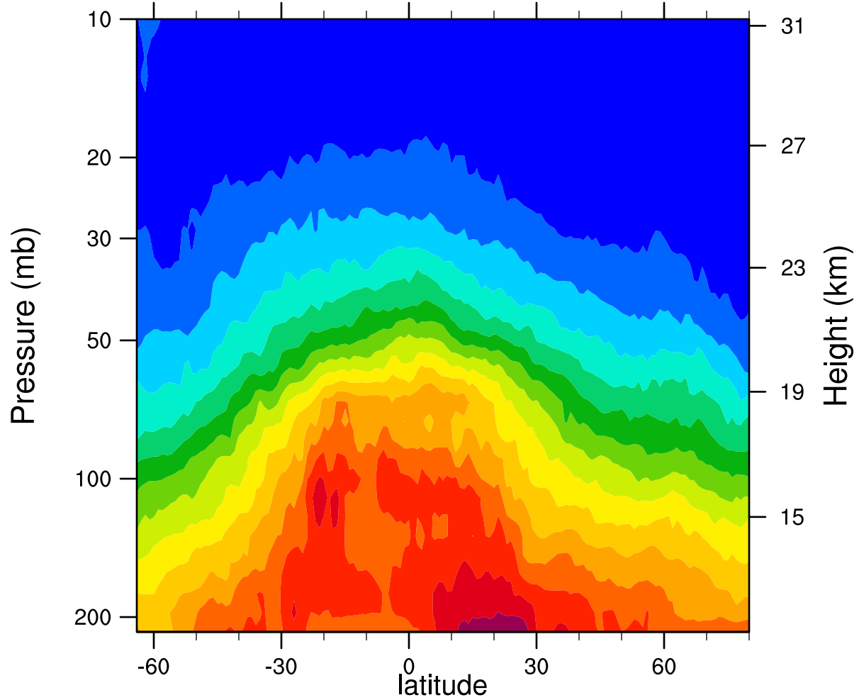
2007d055 12.1MicronExtinction_Combined (km -1 )
