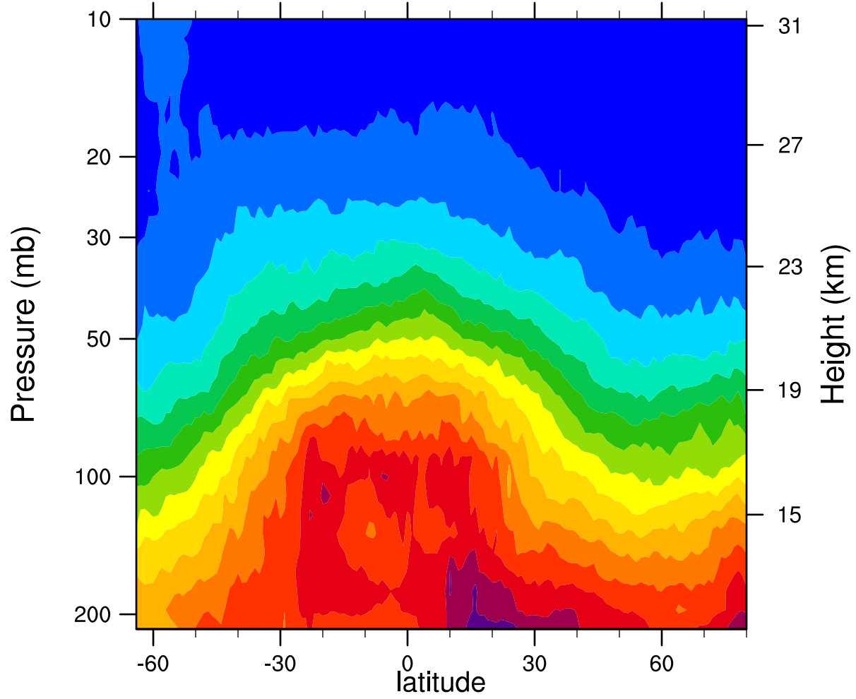
2007d068 12.1MicronExtinction_Combined (km -1 )
