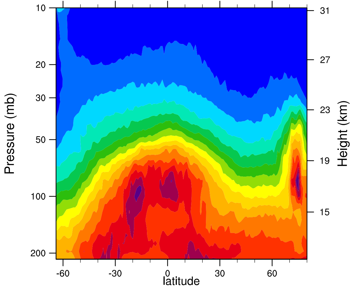
2007d029 12.1MicronExtinction_Combined ( \text{km}^{-1} )
