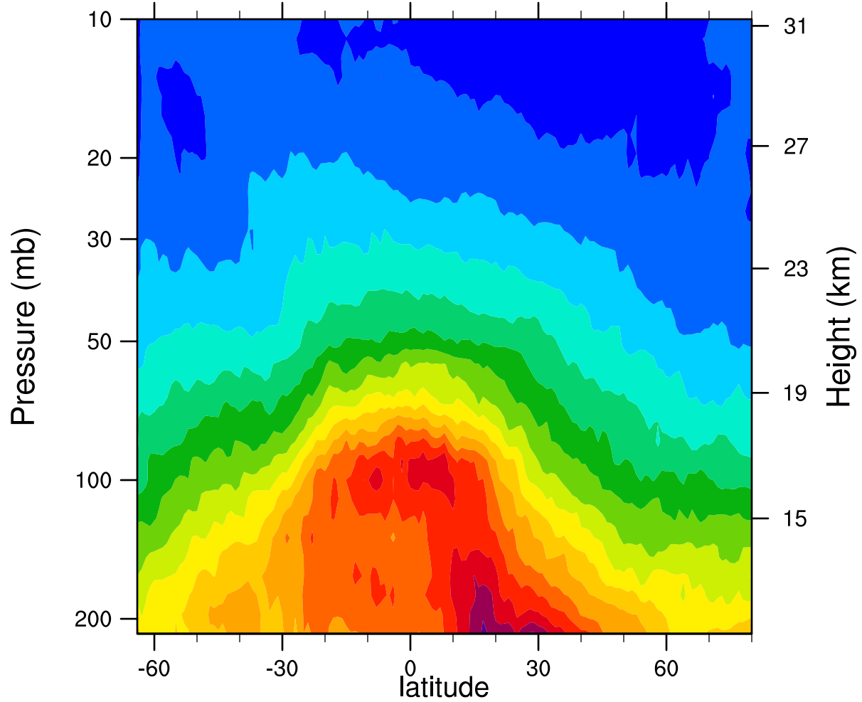
2006d091 12.1MicronExtinction_Combined (km -1 )
