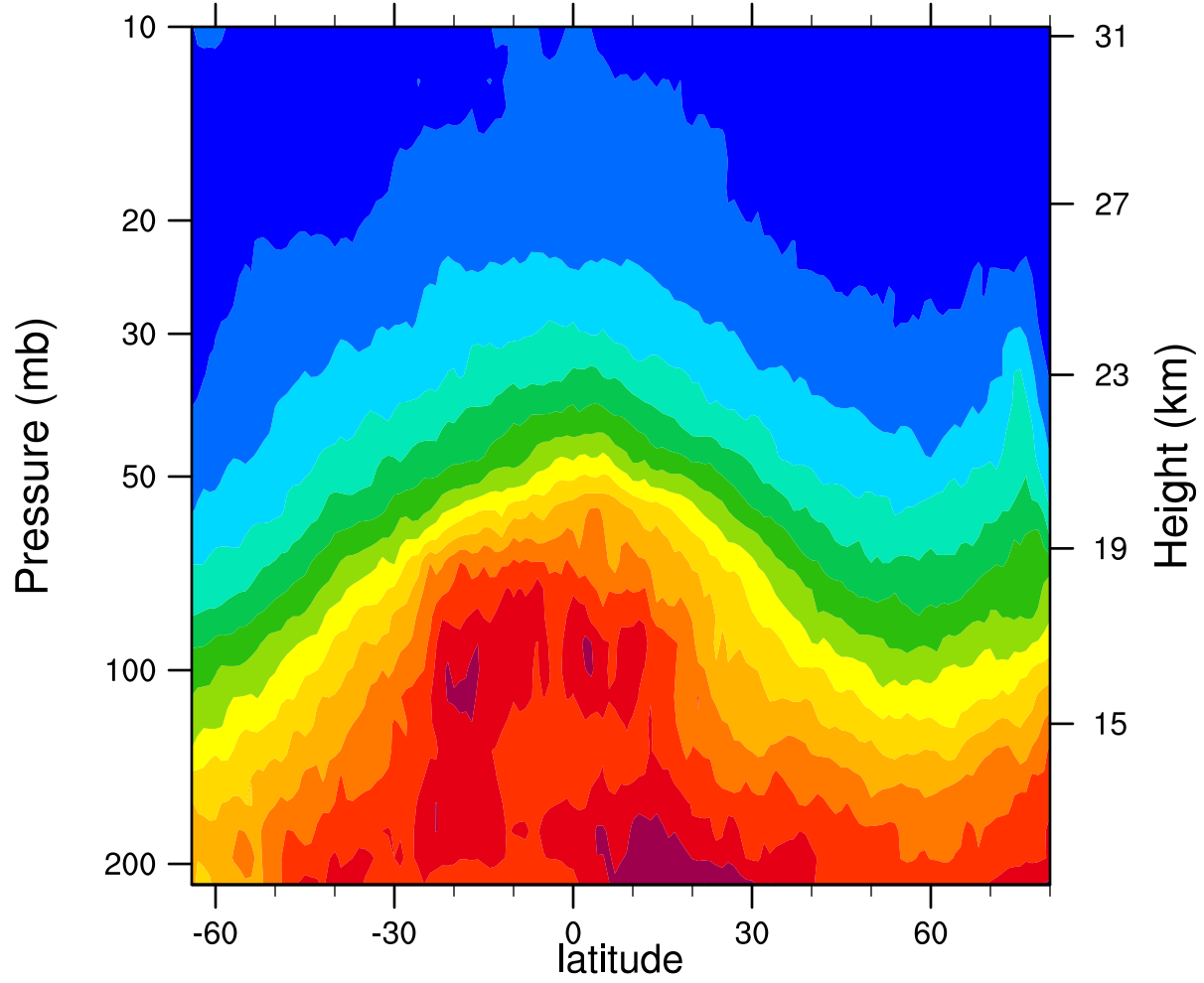
2007d040 12.1MicronExtinction_Combined (km -1 )
