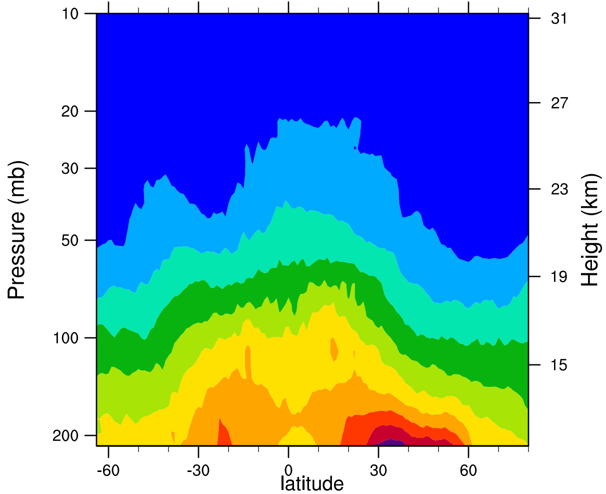
2007d140 12.1MicronExtinction_Combined (km -1 )
