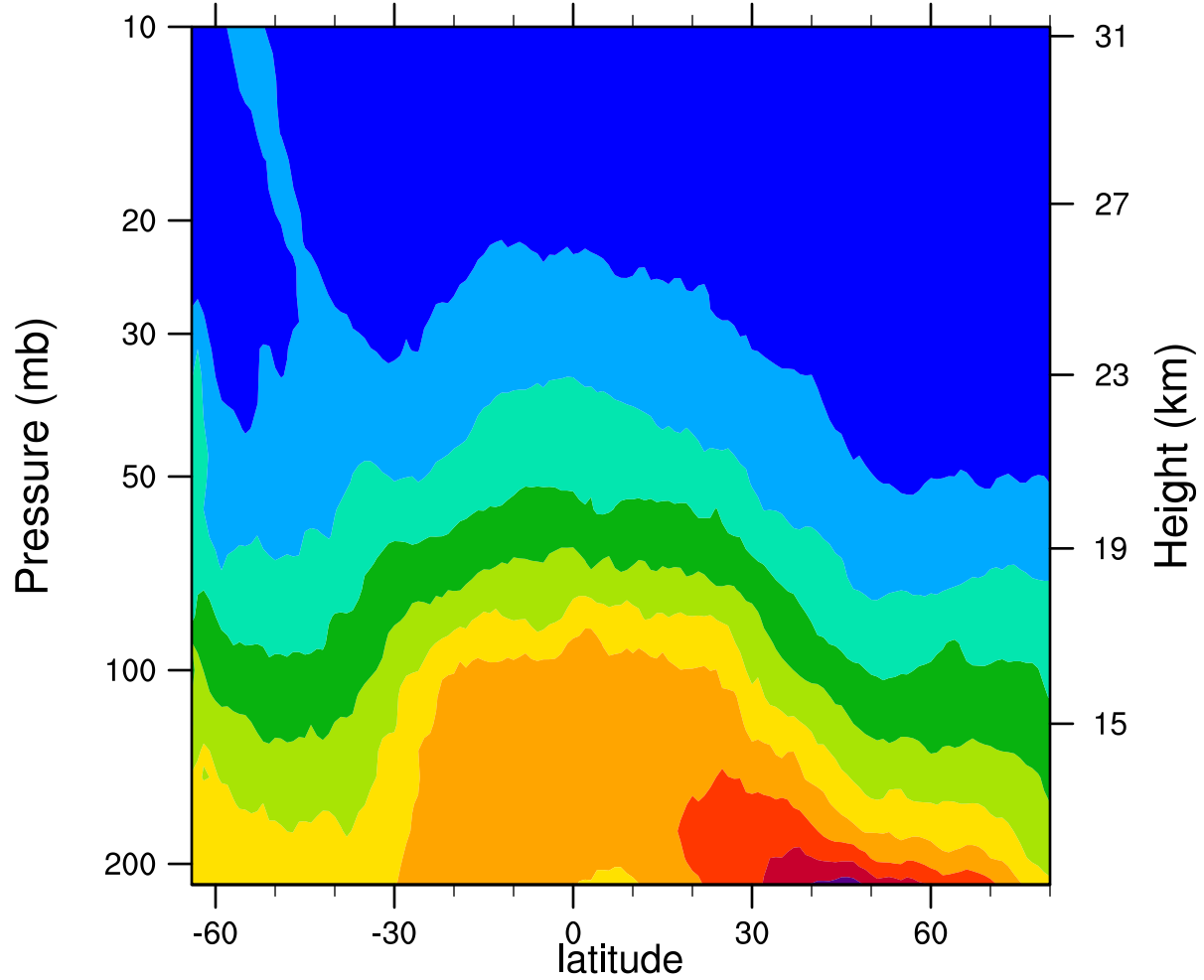
2007d176 12.1MicronExtinction_Combined (km -1 )
