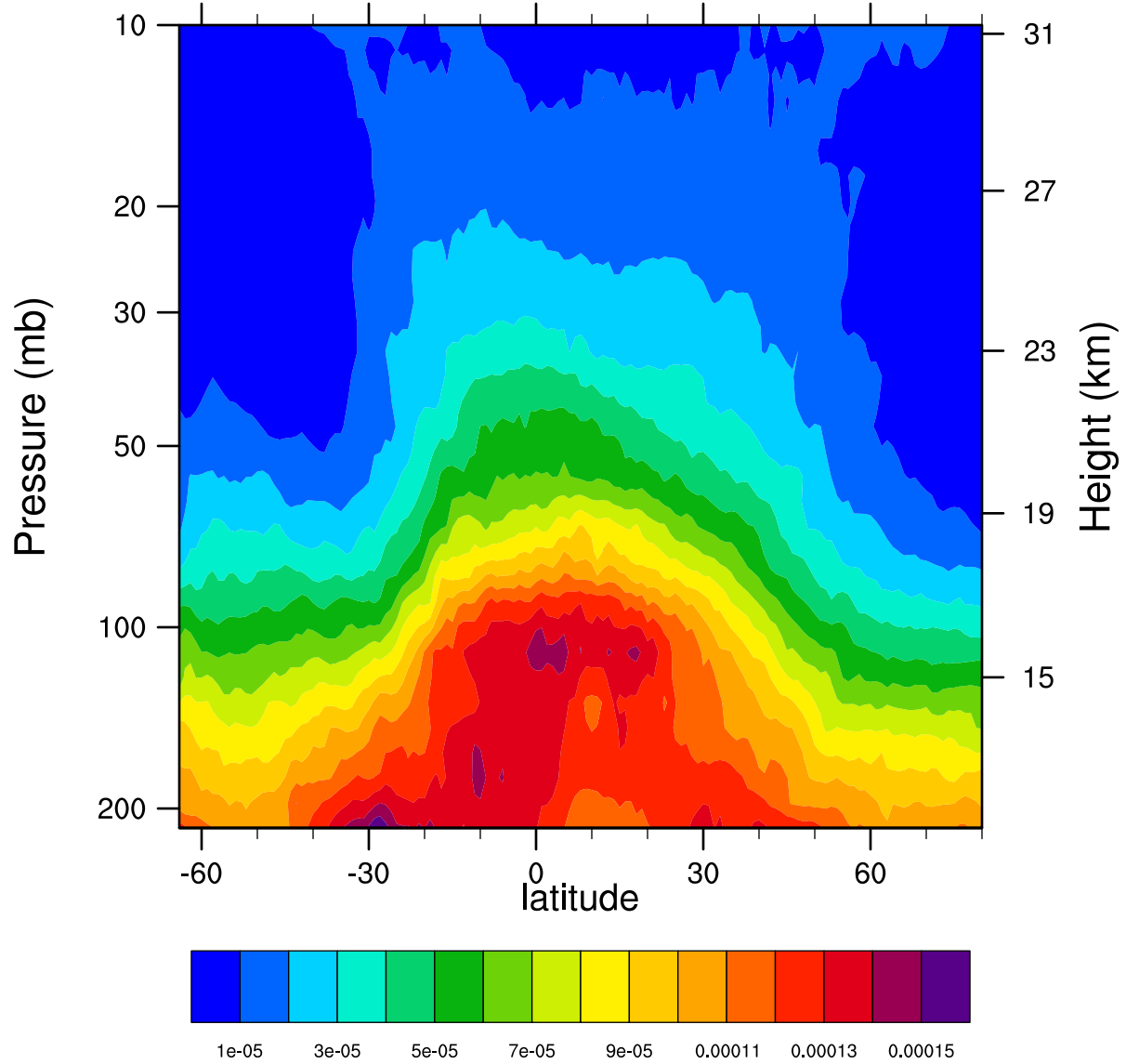
2005d272 12.1MicronExtinction_Combined (km -1 )
