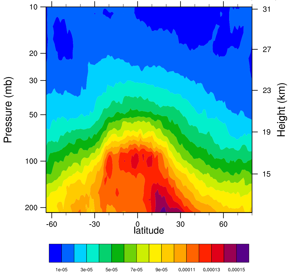
2006d085 12.1MicronExtinction_Combined (km -1 )
