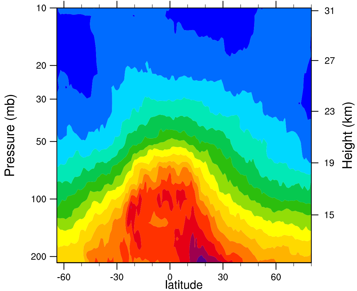
2006d058 12.1MicronExtinction_Combined (km -1 )
