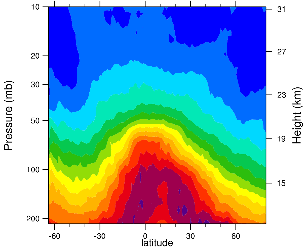
2006d250 12.1MicronExtinction_Combined ( \text{km}^{-1} )
