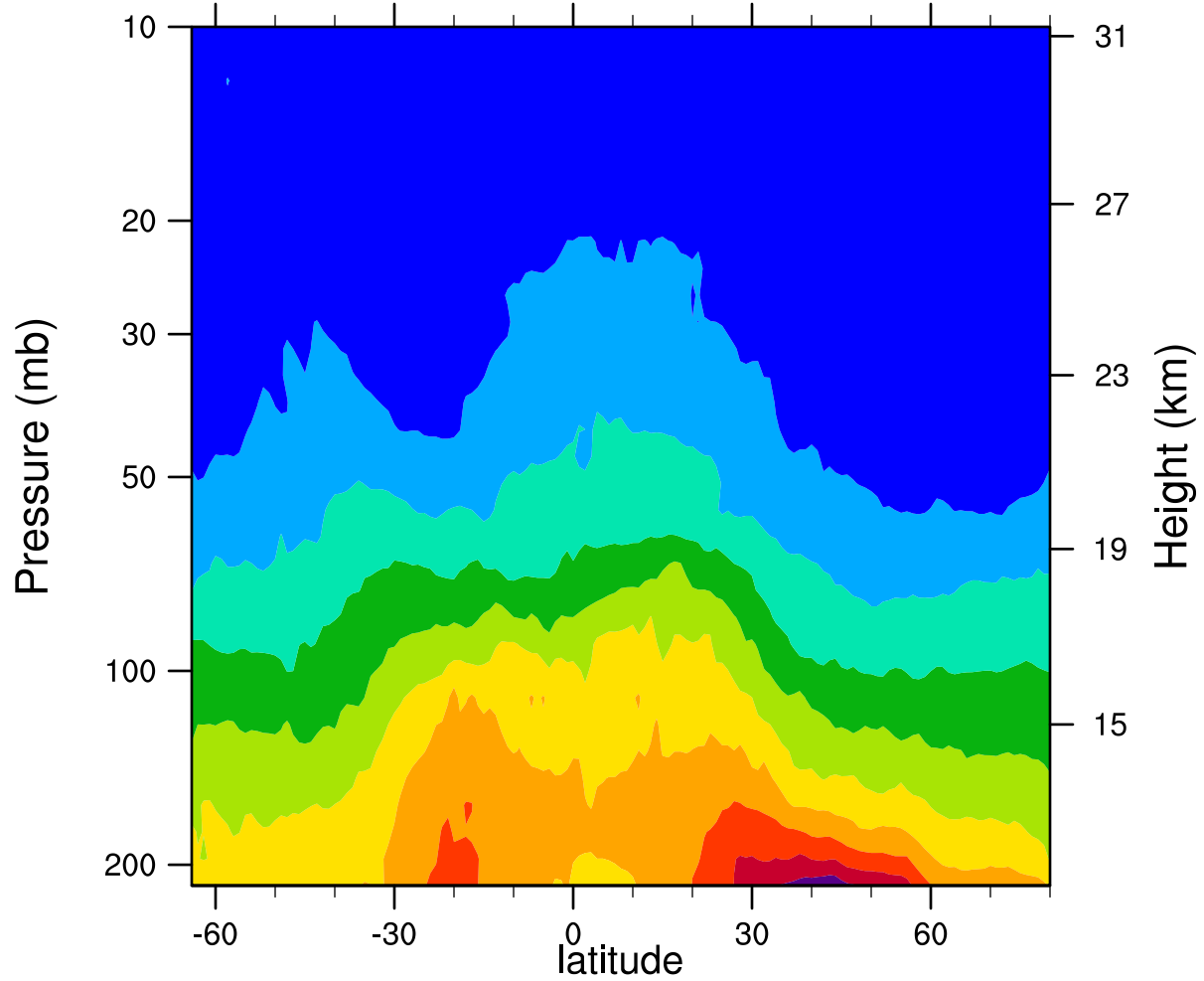
2007d156 12.1MicronExtinction_Combined (km -1 )
