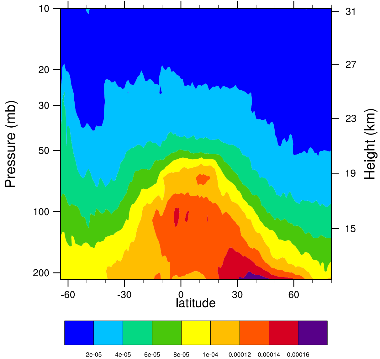
2006d187 12.1MicronExtinction_Combined (km -1 )
