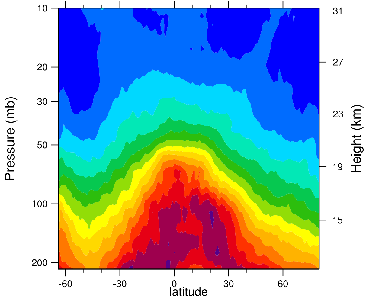
2006d266 12.1MicronExtinction_Combined (km -1 )
