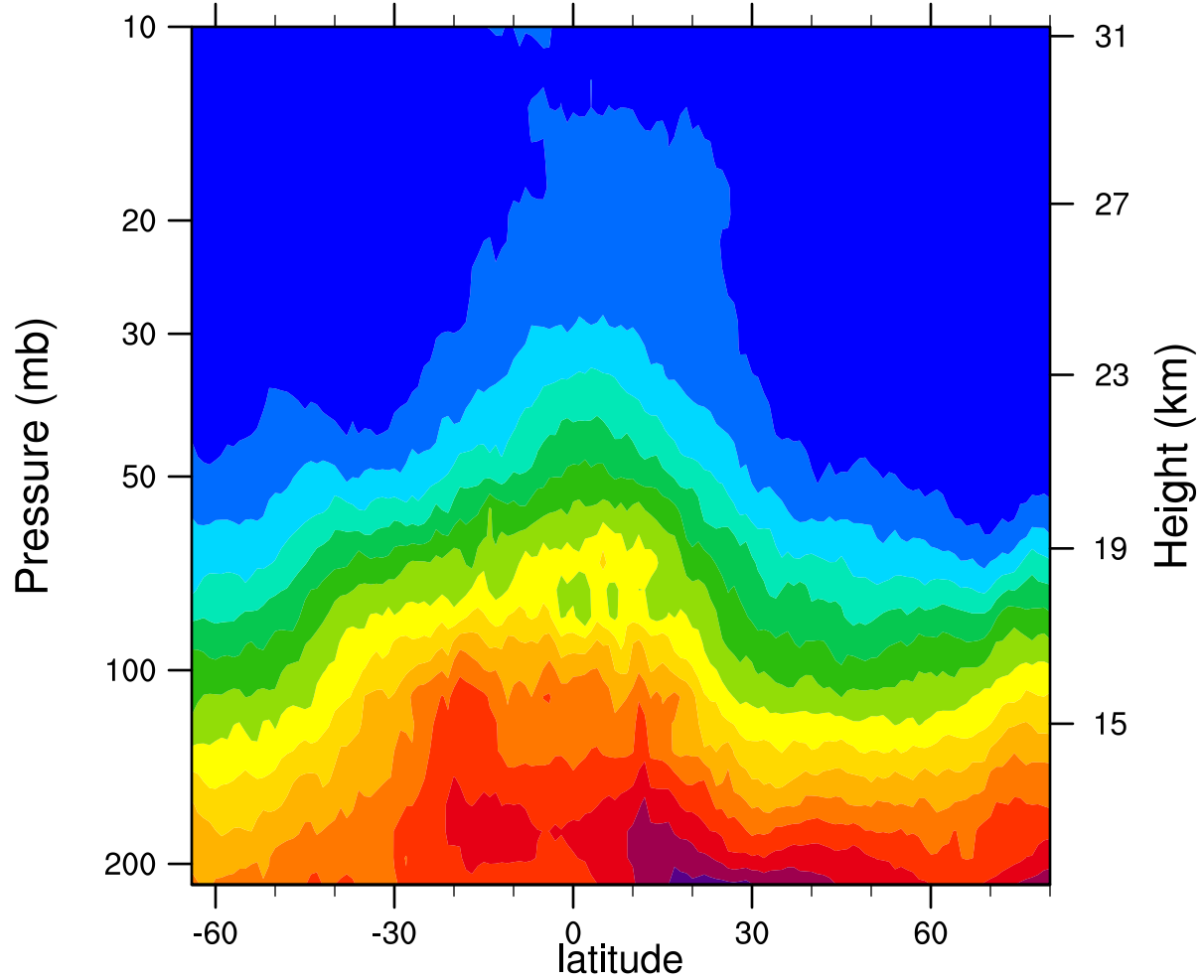
2007d081 12.1MicronExtinction_Combined (km -1 )
