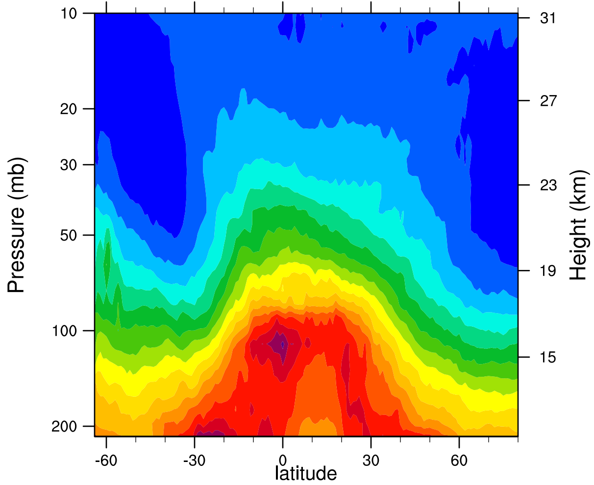
2005d253 12.1MicronExtinction_Combined (km -1 )
