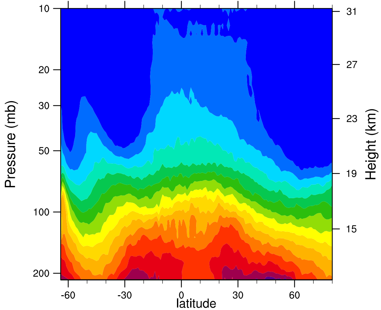
2007d252 12.1MicronExtinction_Combined ( \text{km}^{-1} )
