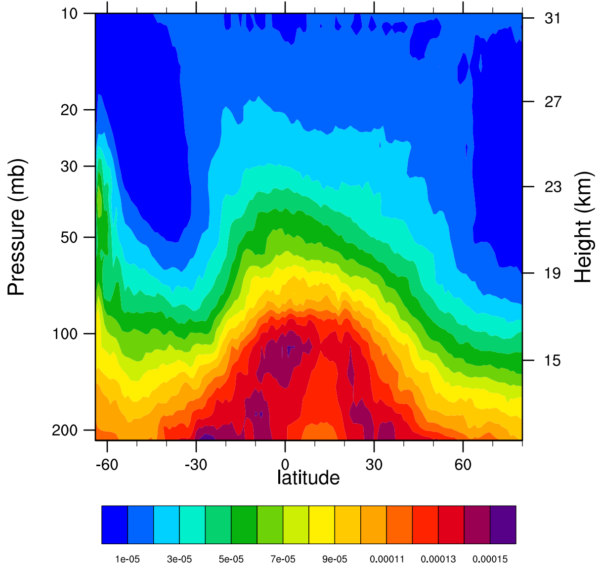
2005d248 12.1MicronExtinction_Combined ( \text{km}^{-1} )
