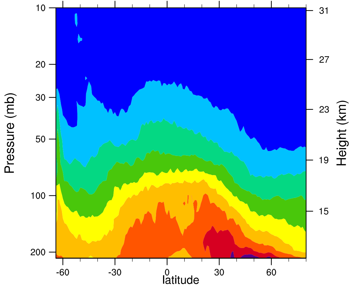
2007d205 12.1MicronExtinction_Combined (km -1 )
