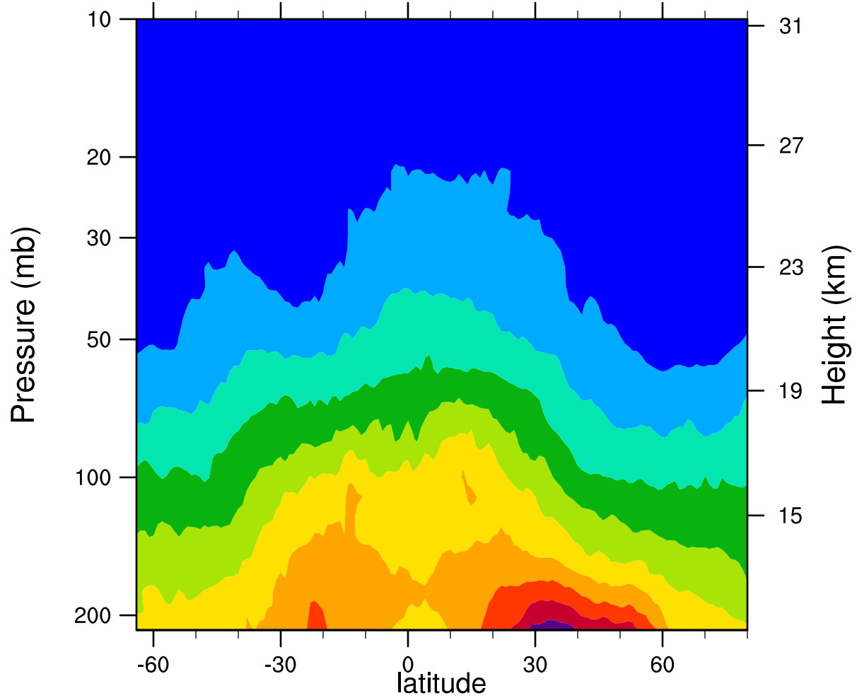
2007d139 12.1MicronExtinction_Combined ( \text{km}^{-1} )
