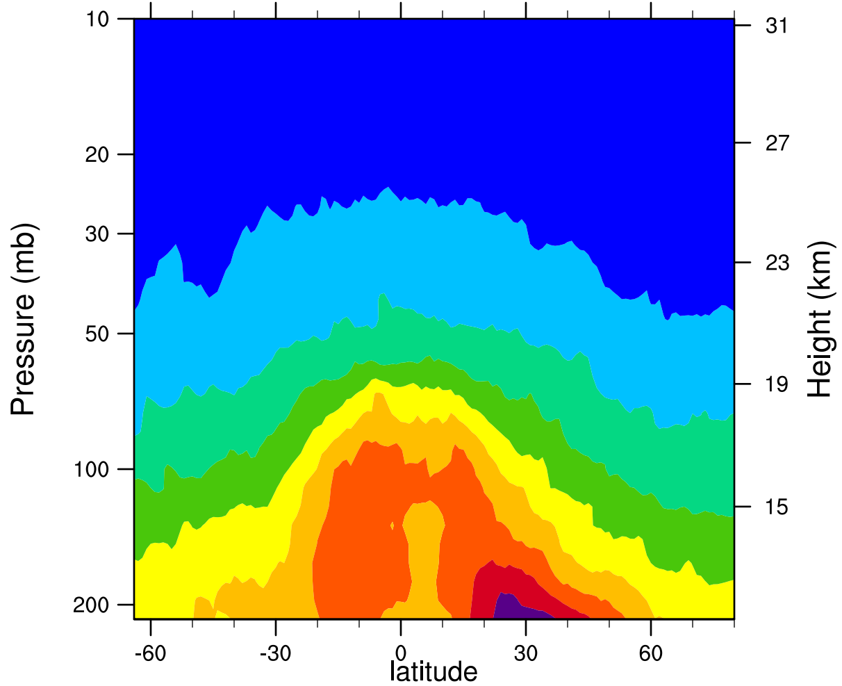
2006d134 12.1MicronExtinction_Combined (km -1 )
