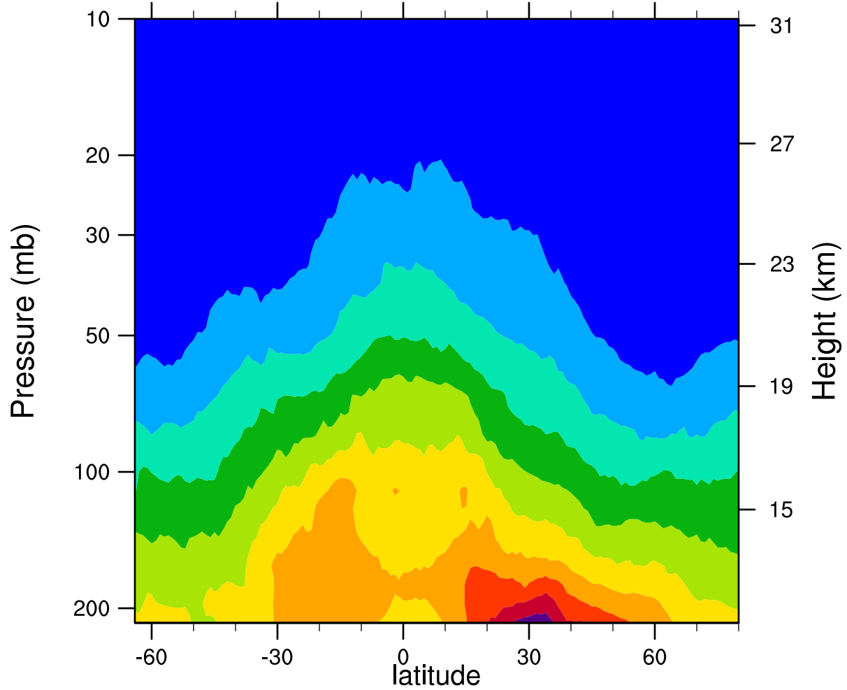
2007d121 12.1MicronExtinction_Combined (km -1 )
