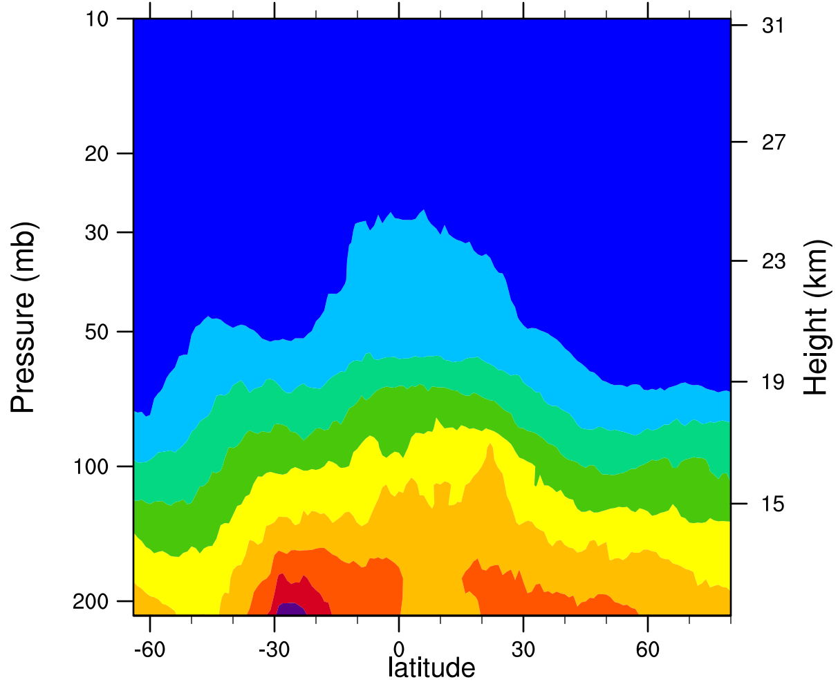
2007d285 12.1MicronExtinction_Combined (km -1 )
