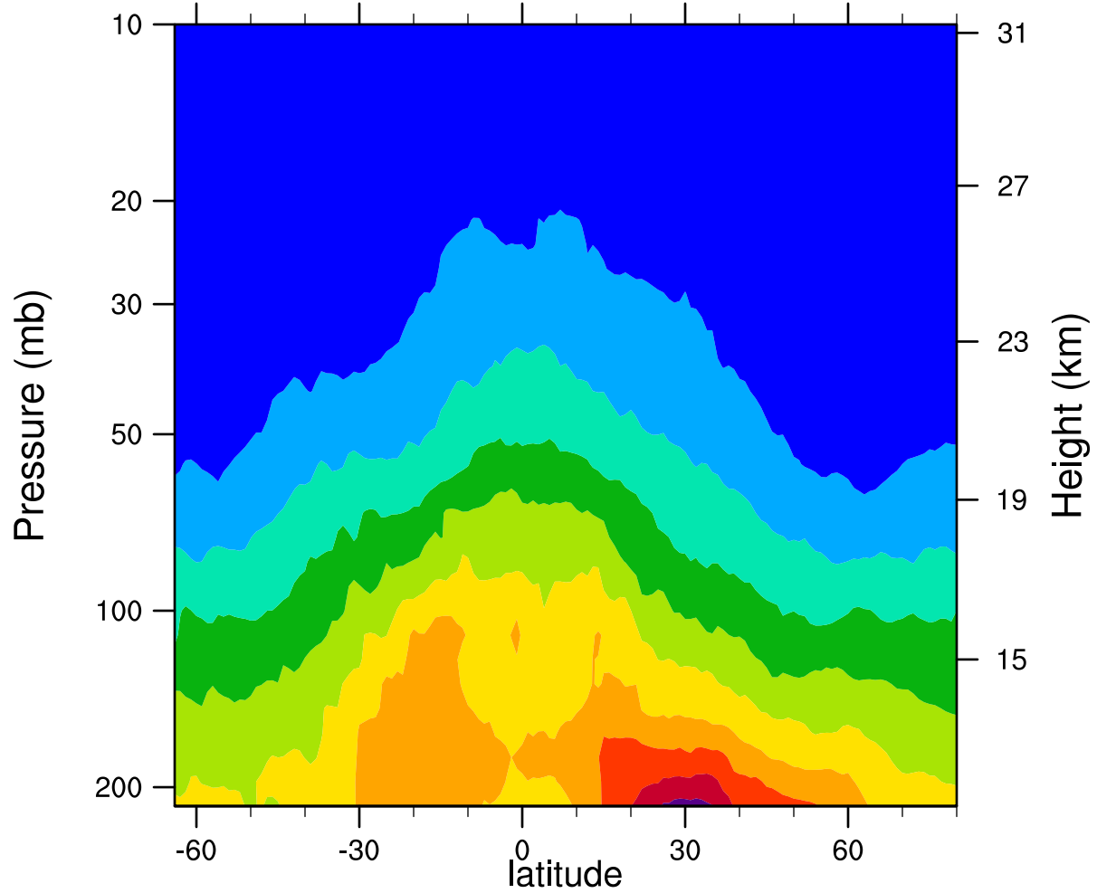
2007d119 12.1MicronExtinction_Combined (km -1 )
