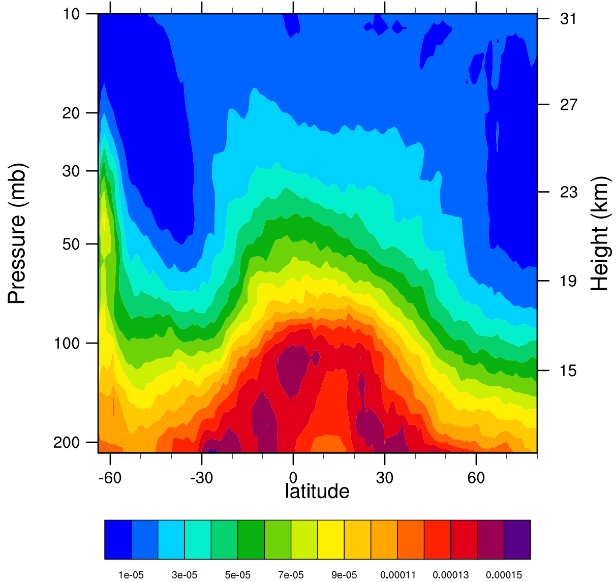
2005d245 12.1MicronExtinction_Combined (km -1 )
