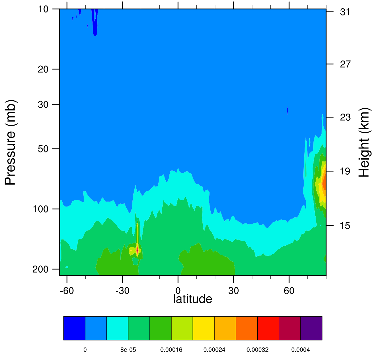
2005d024 12.1MicronExtinction_Combined (km -1 )
