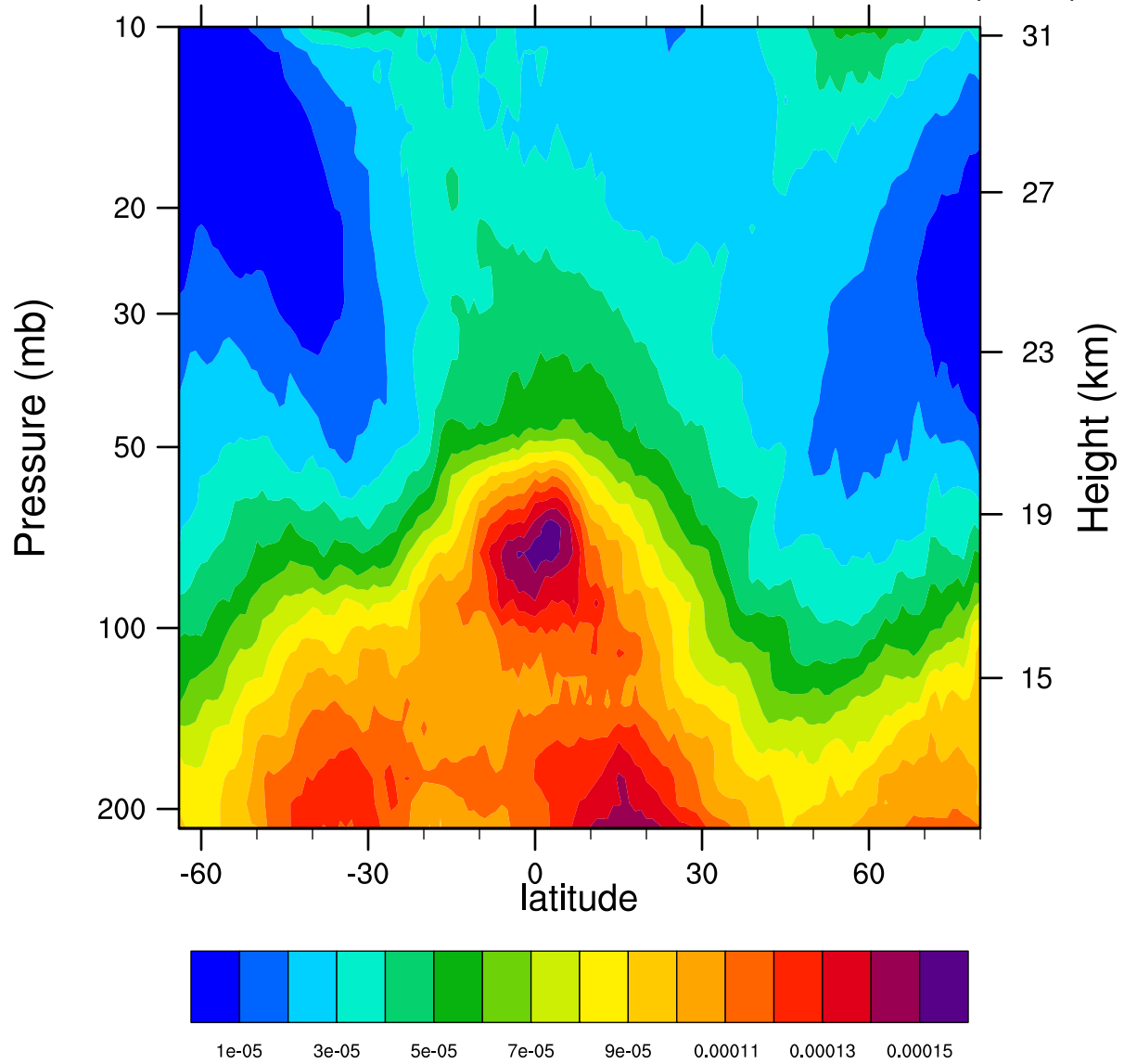
2005d049 12.1MicronExtinction_Combined (km -1 )
