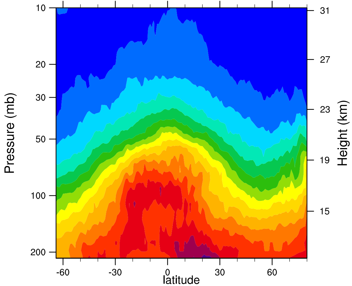
2007d044 12.1MicronExtinction_Combined (km -1 )
