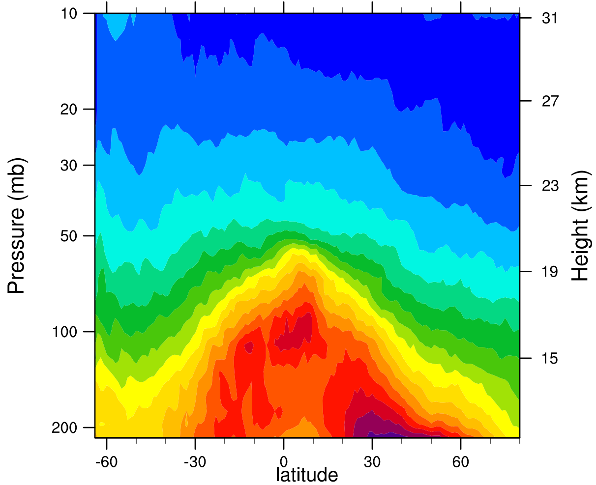
2006d166 12.1MicronExtinction_Combined ( \text{km}^{-1} )
