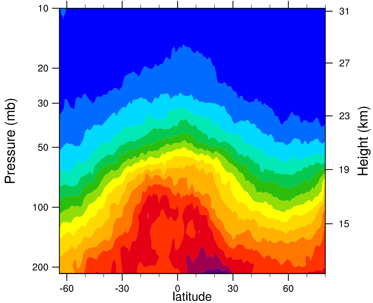
2007d049 12.1MicronExtinction_Combined (km -1 )
