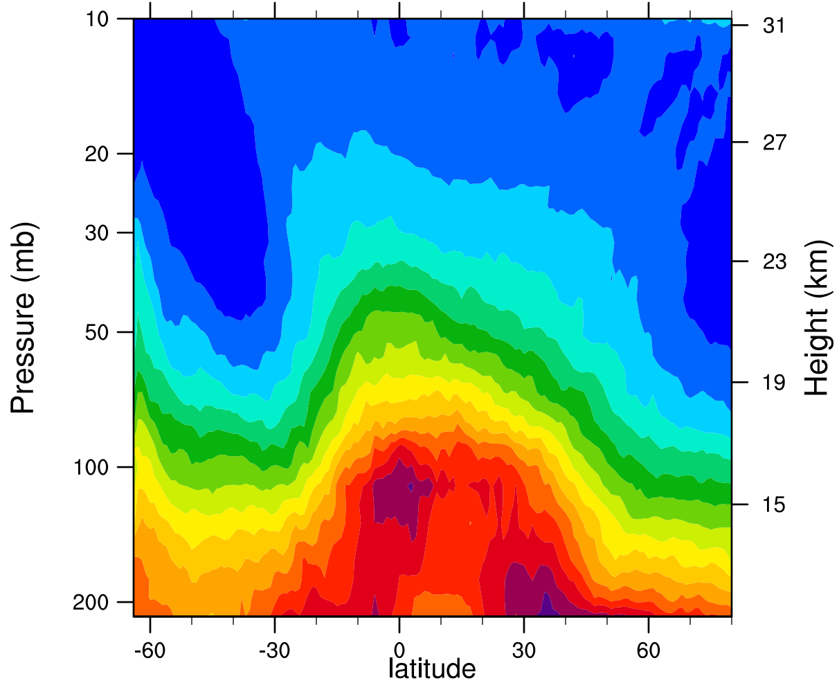
2005d223 12.1MicronExtinction_Combined (km -1 )
