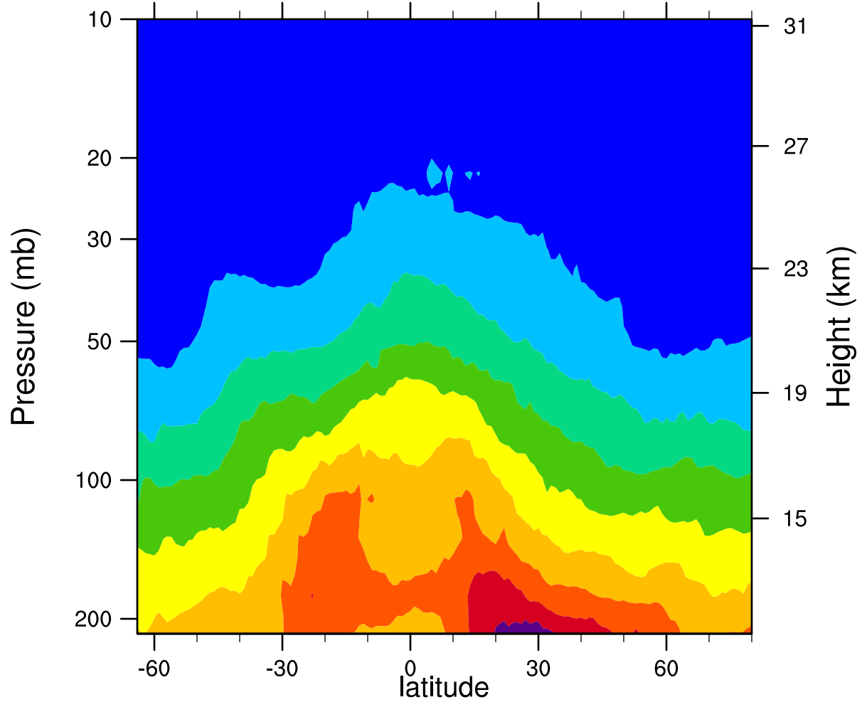
2007d109 12.1MicronExtinction_Combined (km -1 )
