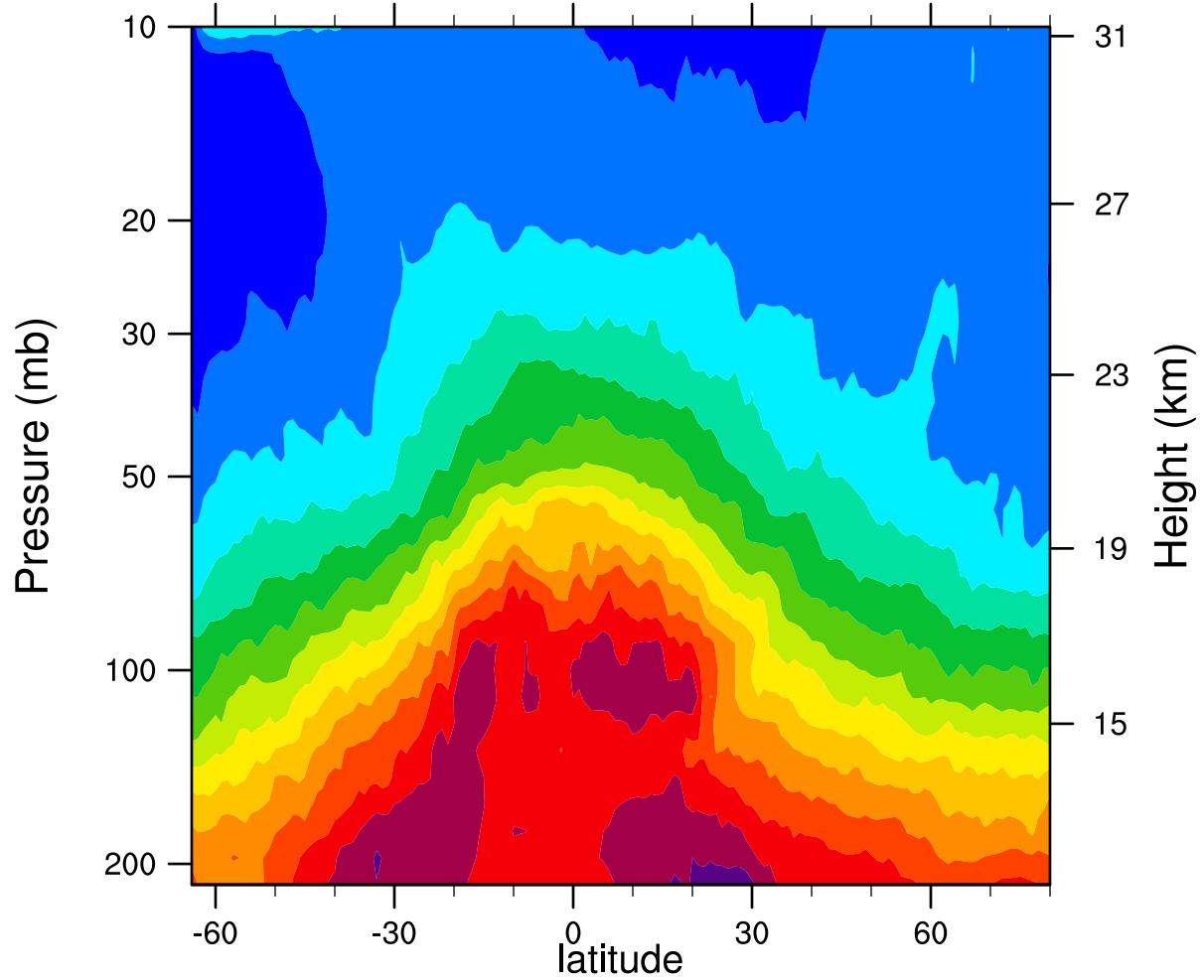
2005d348 12.1MicronExtinction_Combined (km -1 )
