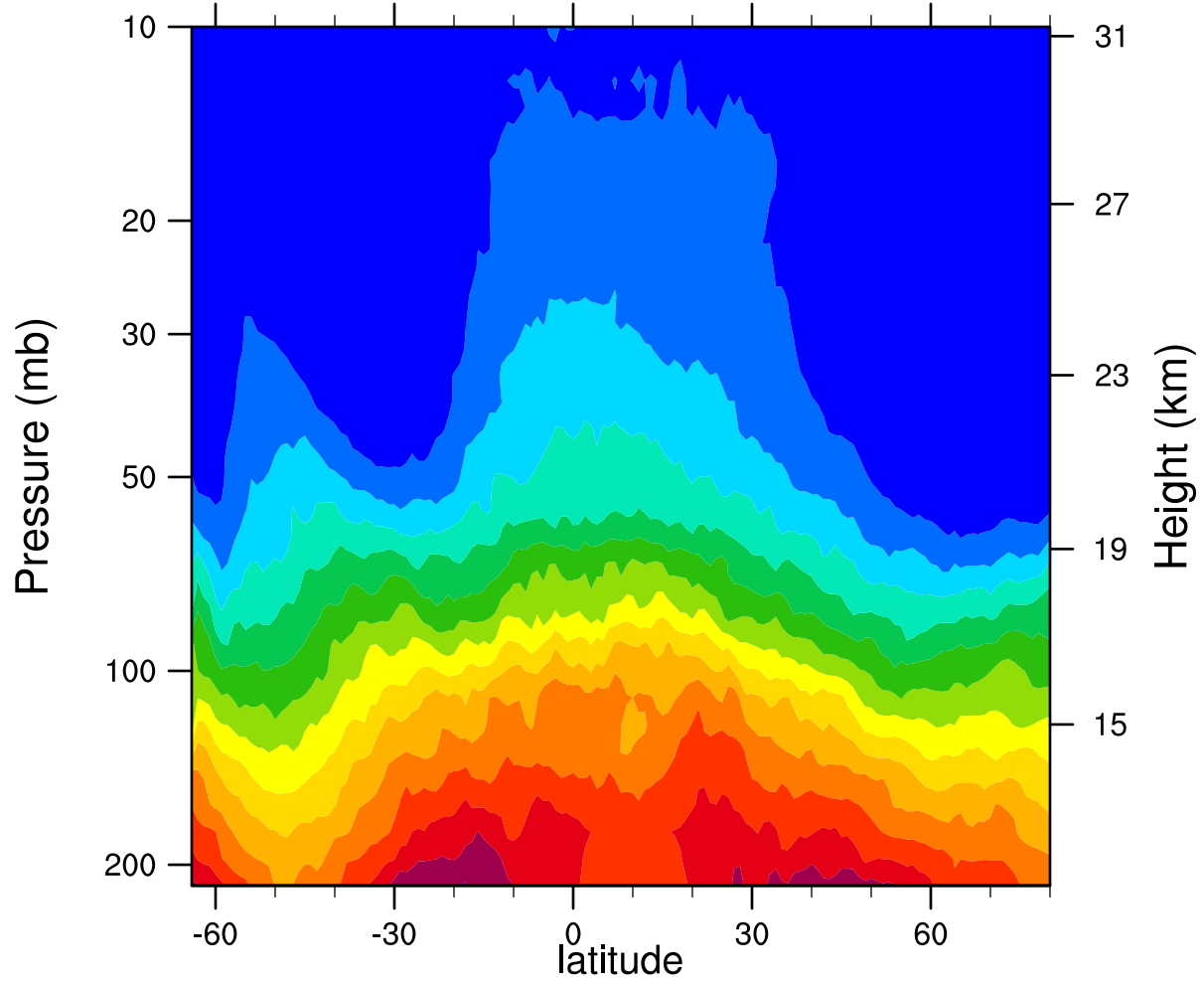
2007d263 12.1MicronExtinction_Combined (km -1 )
