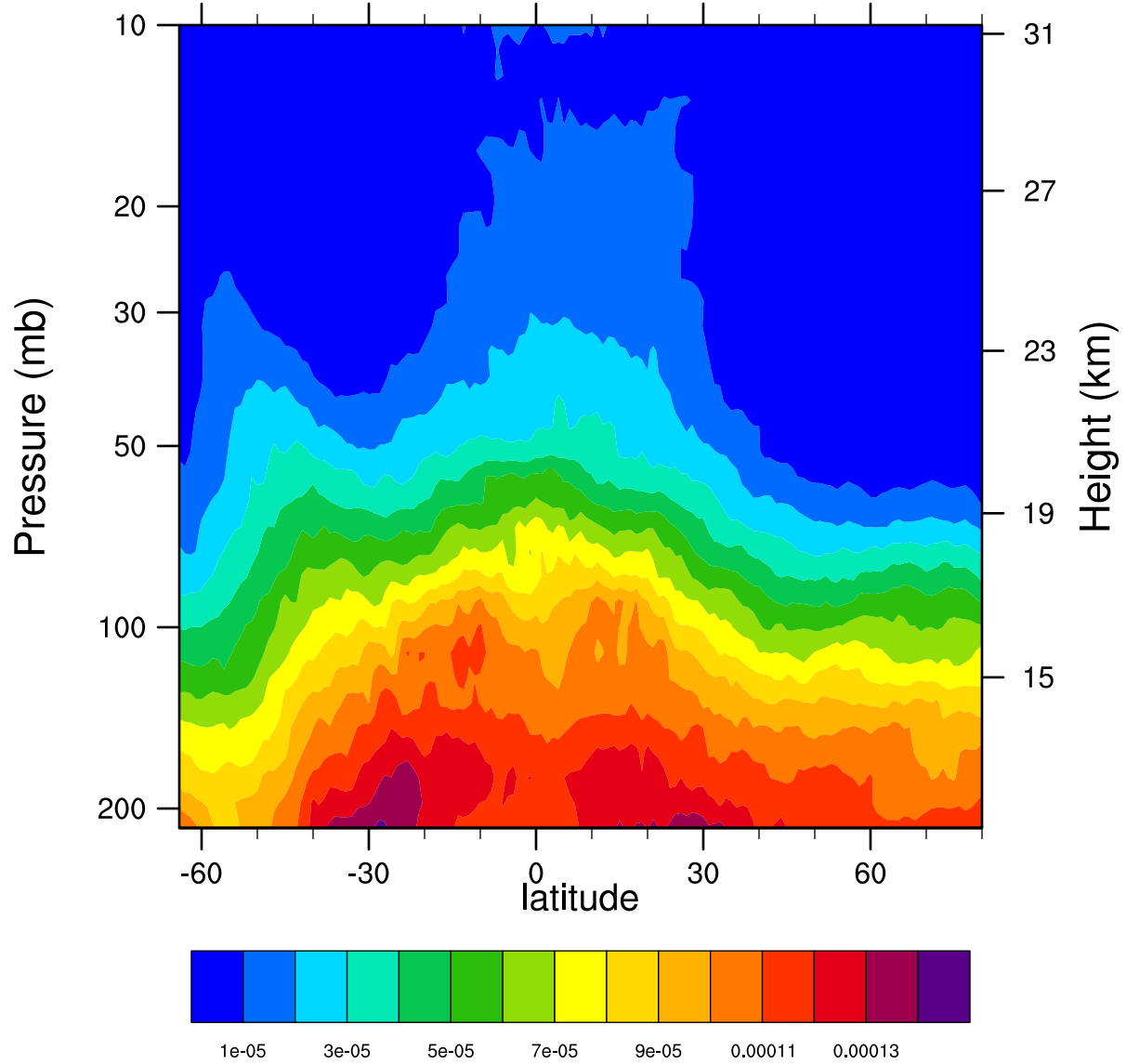
2007d325 12.1MicronExtinction_Combined (km -1 )
