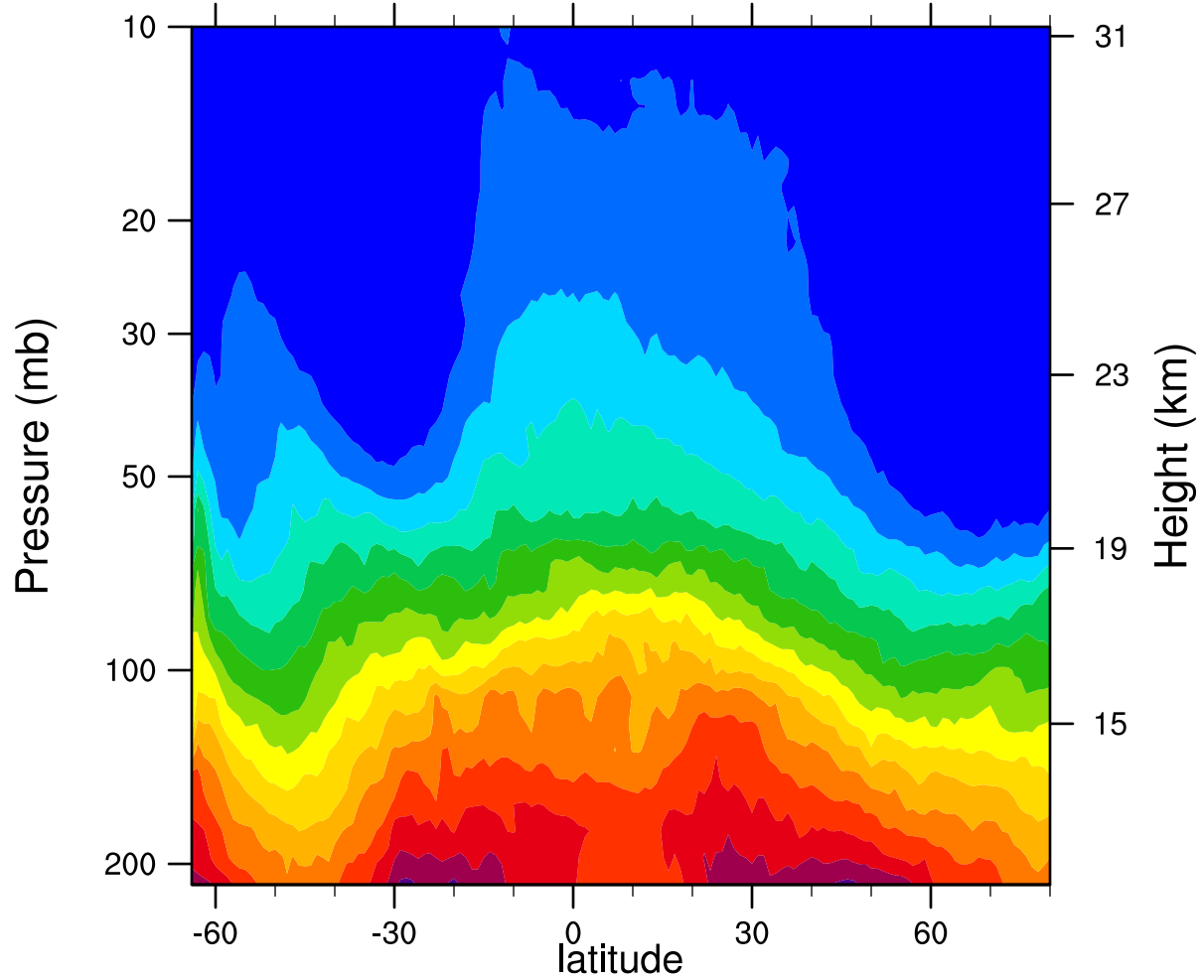
2007d256 12.1MicronExtinction_Combined (km -1 )
