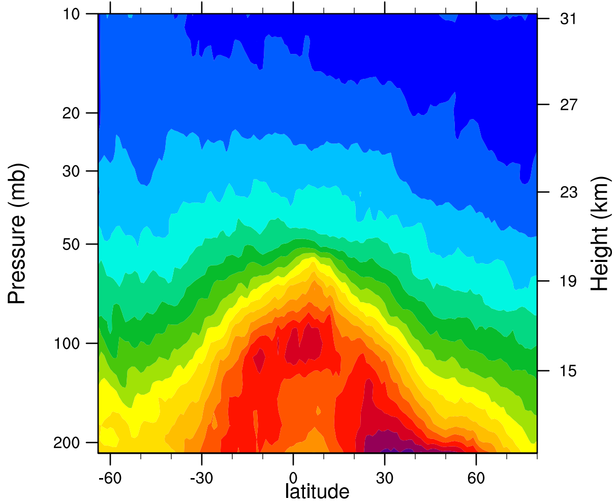
2006d163 12.1MicronExtinction_Combined (km -1 )
