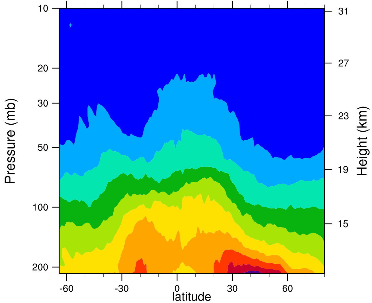
2007d154 12.1MicronExtinction_Combined ( \text{km}^{-1} )
