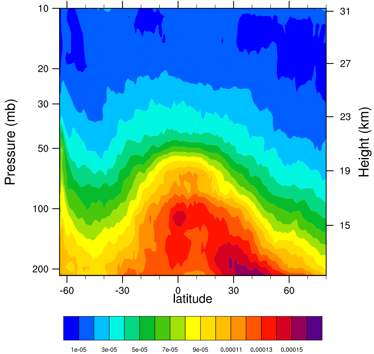
2006d227 12.1MicronExtinction_Combined (km -1 )
