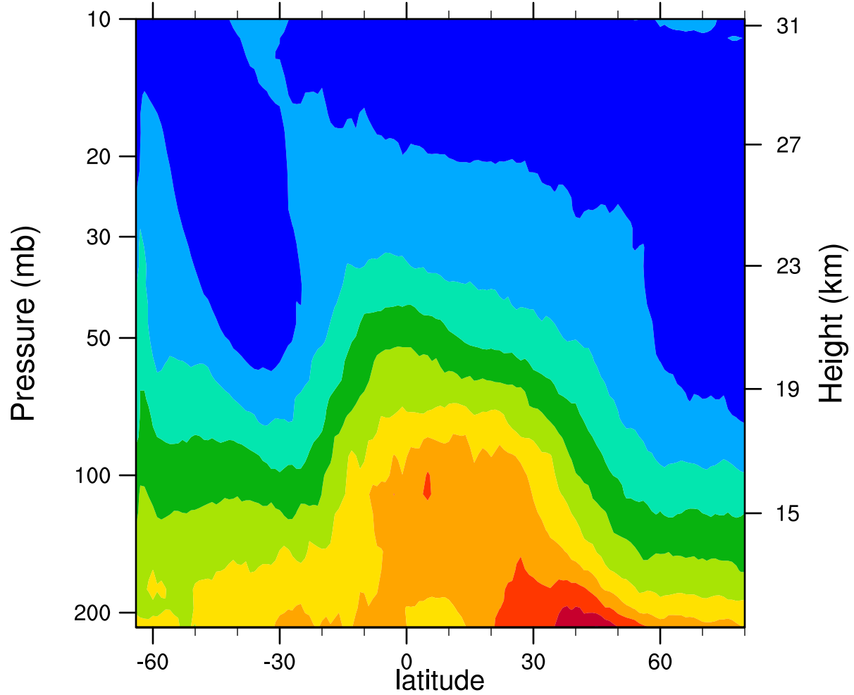
2005d186 12.1MicronExtinction_Combined ( \text{km}^{-1} )
