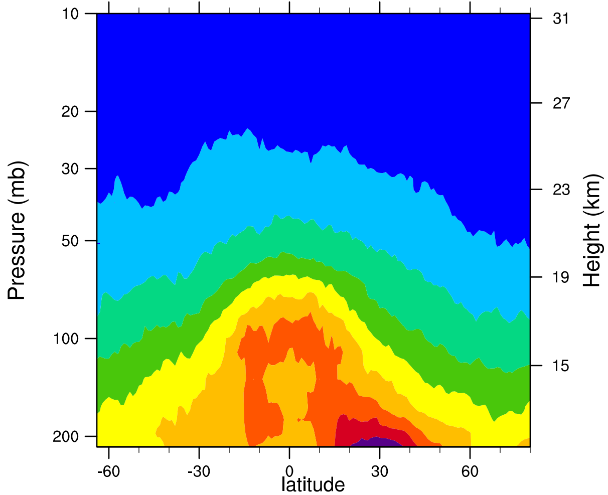
2006d114 12.1MicronExtinction_Combined (km -1 )
