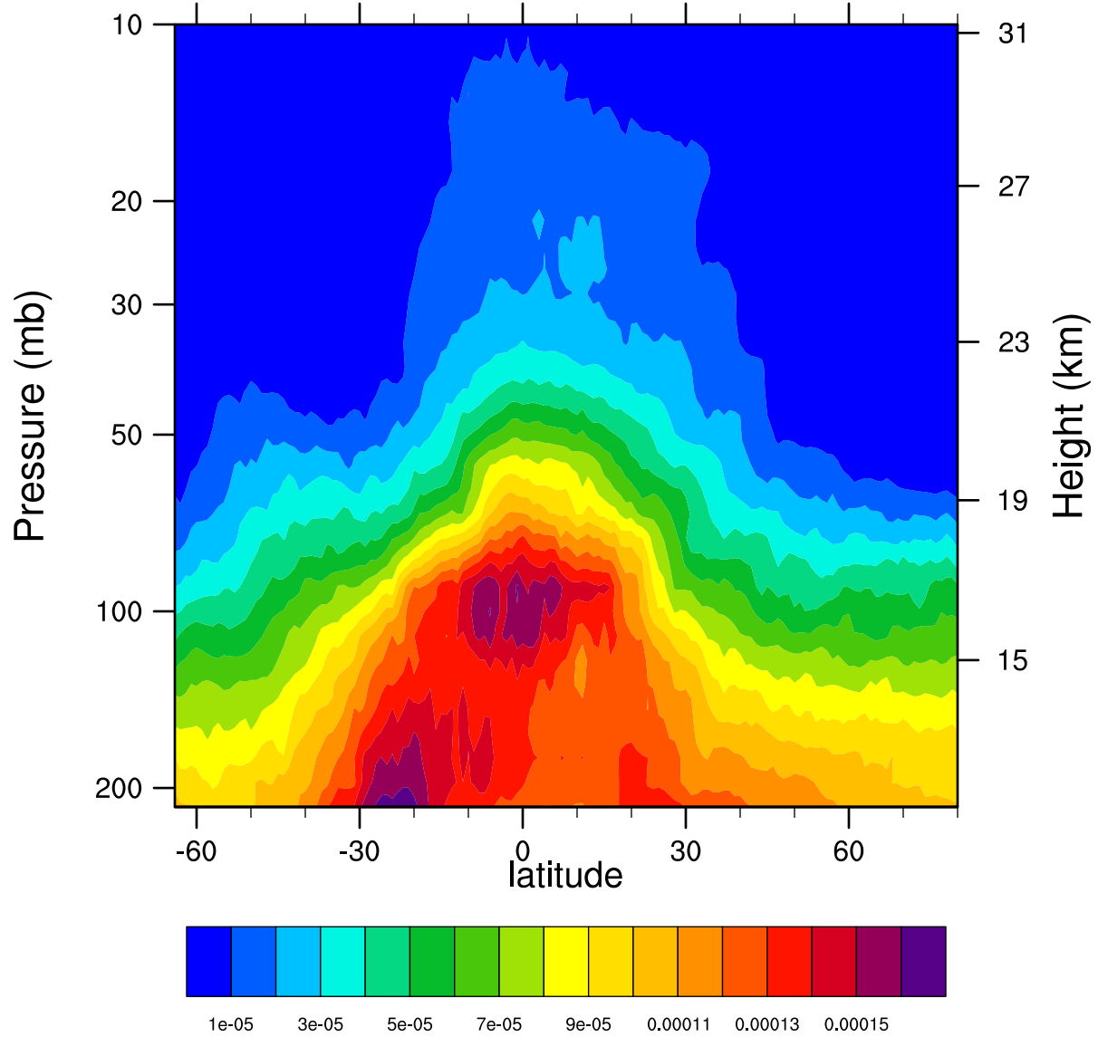
2006d316 12.1MicronExtinction_Combined ( \text{km}^{-1} )
