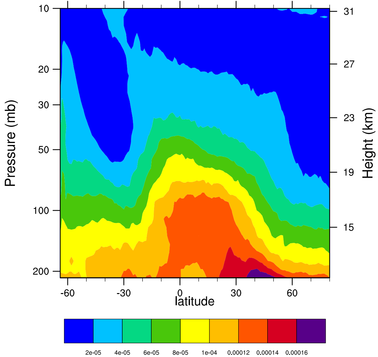
2005d188 12.1MicronExtinction_Combined (km -1 )
