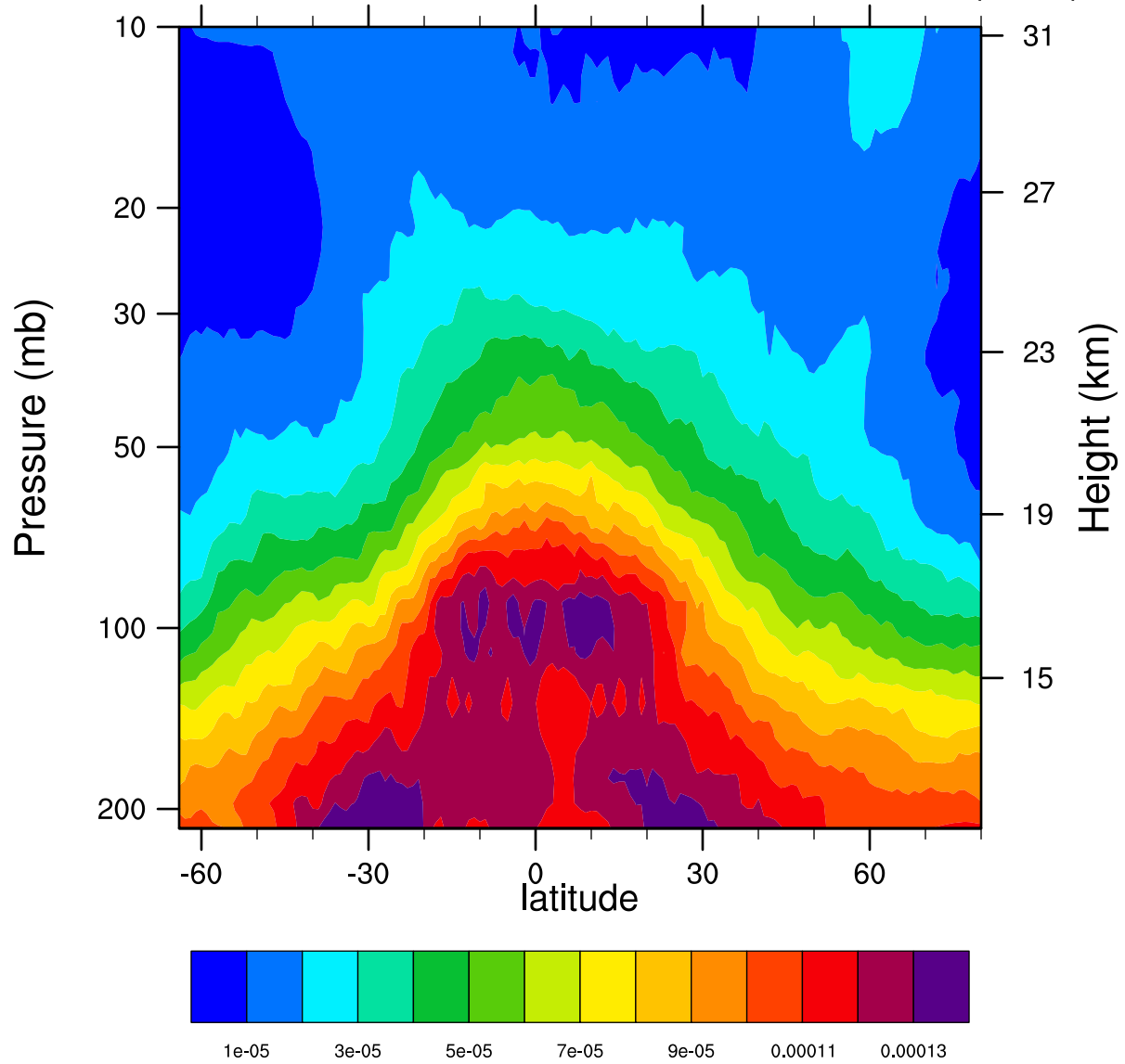
2005d320 12.1MicronExtinction_Combined ( \text{km}^{-1} )
