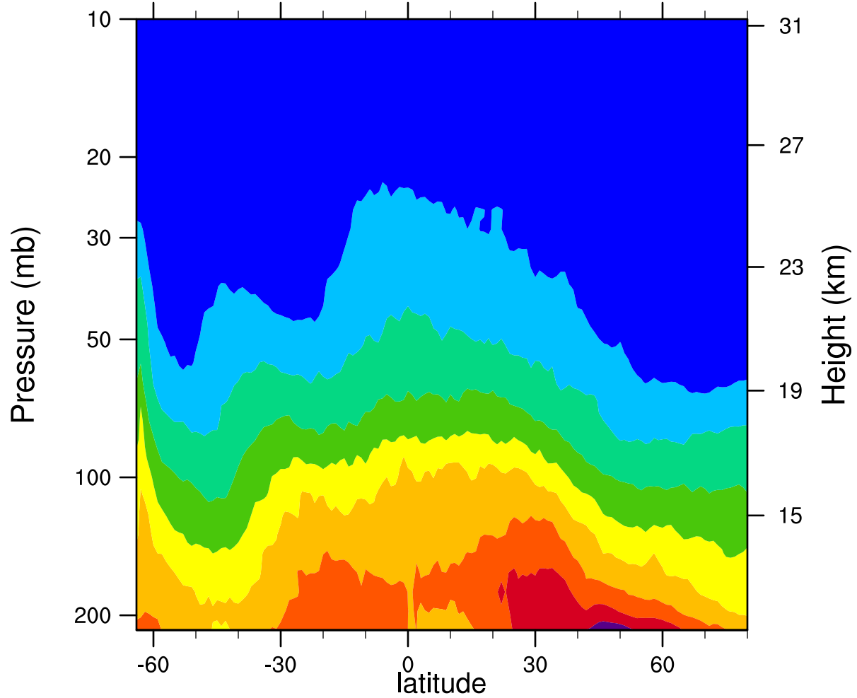
2007d212 12.1MicronExtinction_Combined (km -1 )
