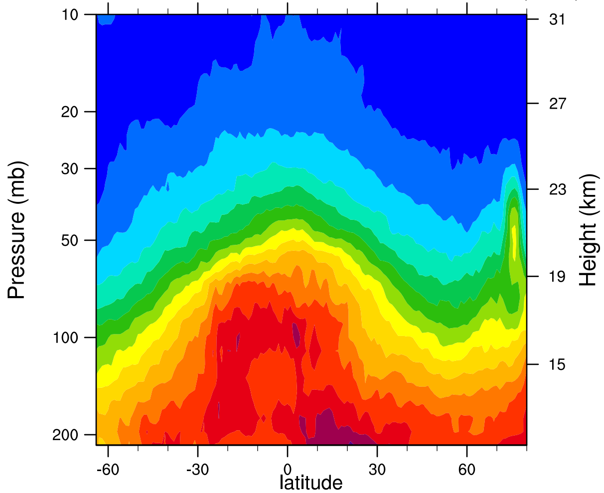
2007d042 12.1MicronExtinction_Combined (km -1 )
