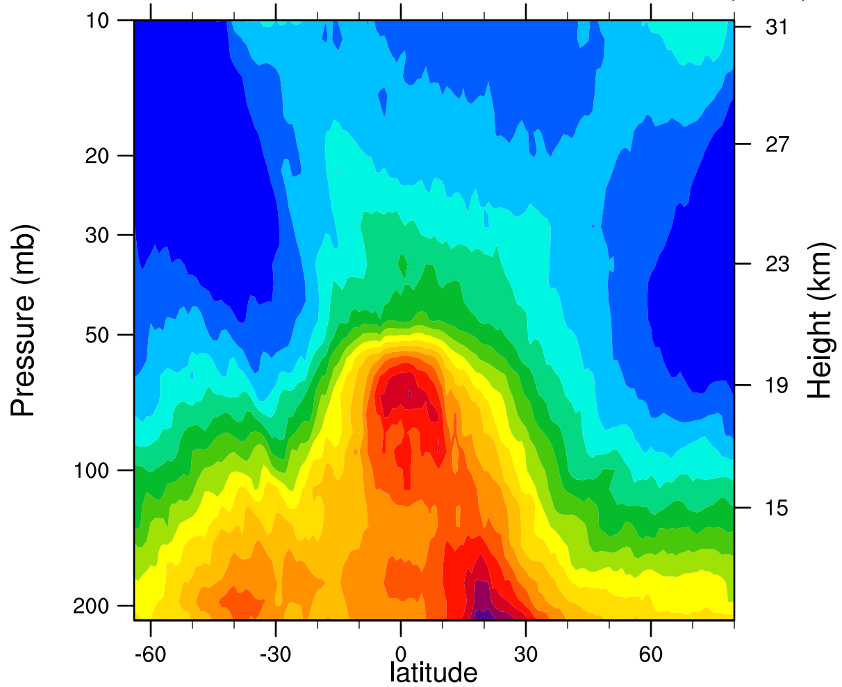
2005d082 12.1MicronExtinction_Combined ( \text{km}^{-1} )
