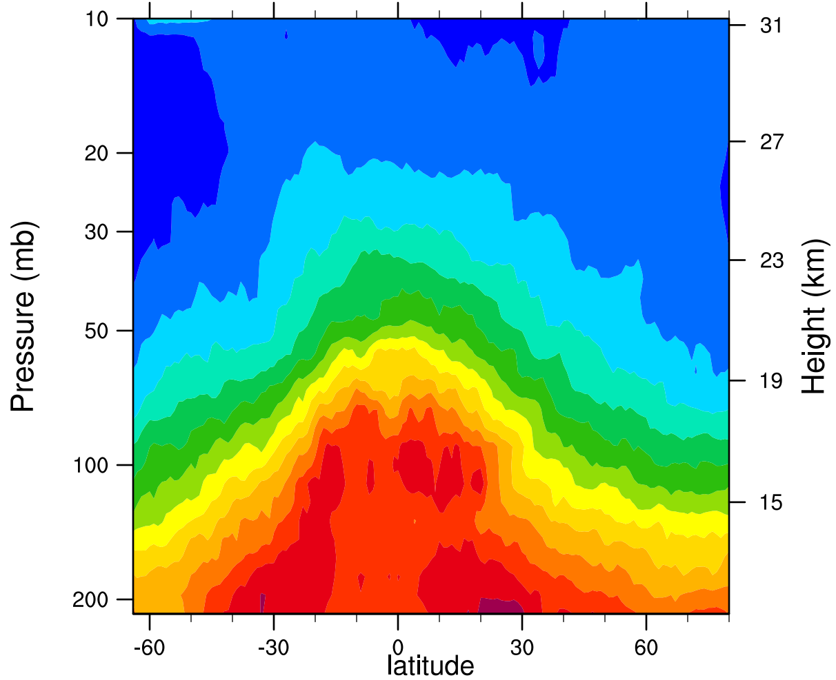
2005d346 12.1MicronExtinction_Combined (km -1 )
