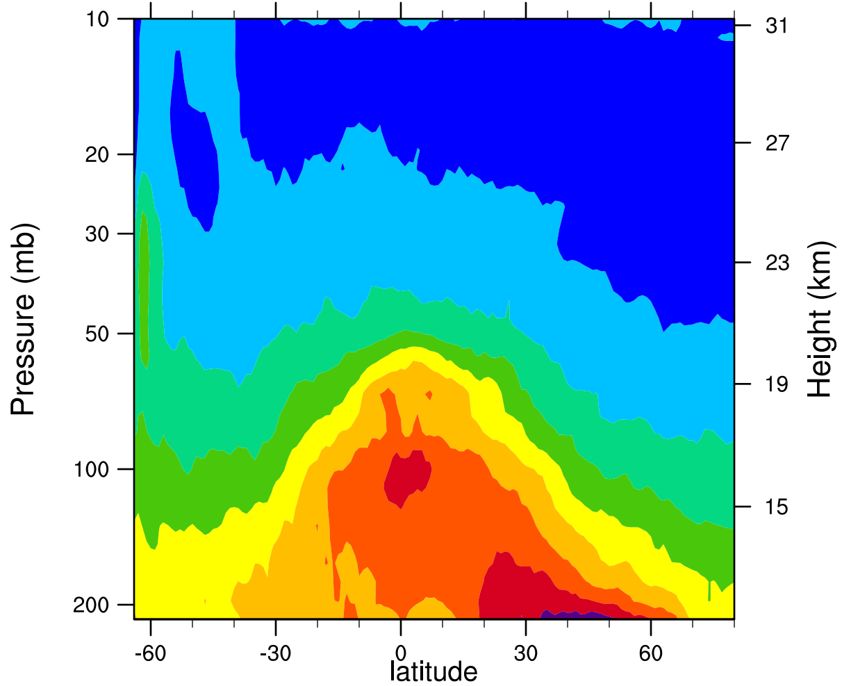
2006d180 12.1MicronExtinction_Combined (km -1 )
