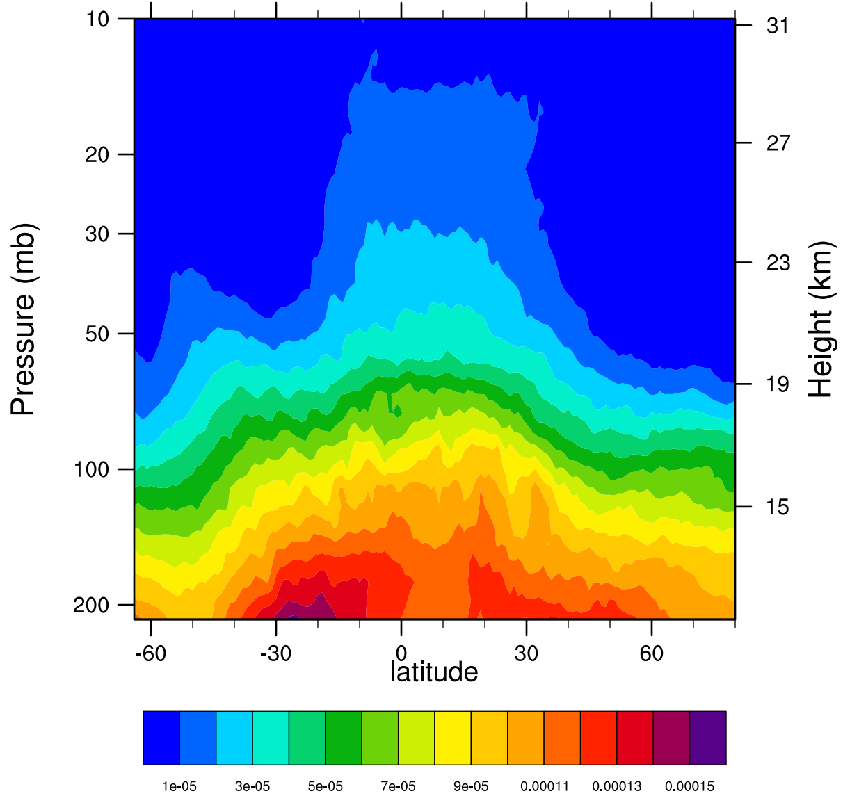
2007d292 12.1MicronExtinction_Combined ( \text{km}^{-1} )
