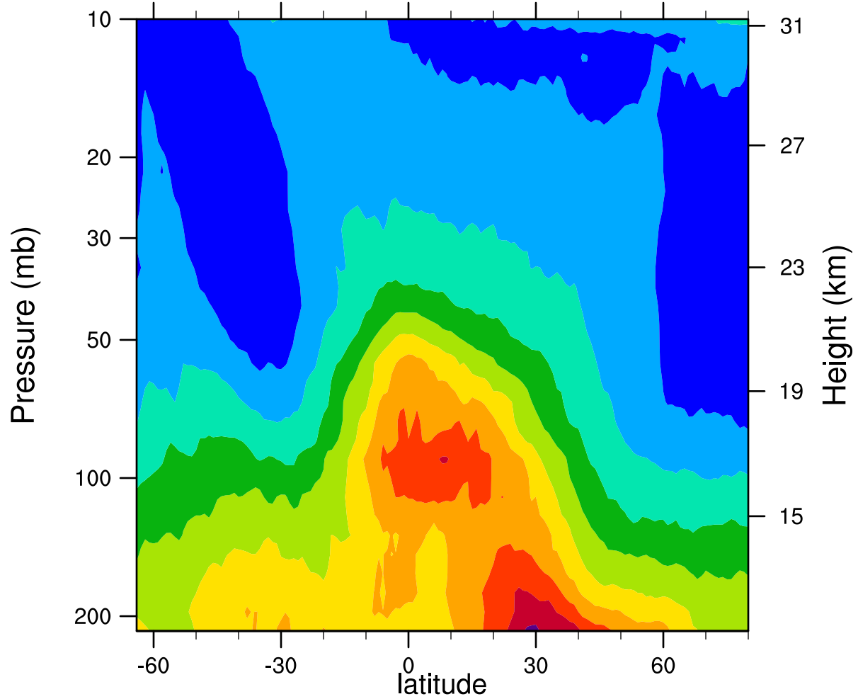
2005d143 12.1MicronExtinction_Combined (km -1 )
