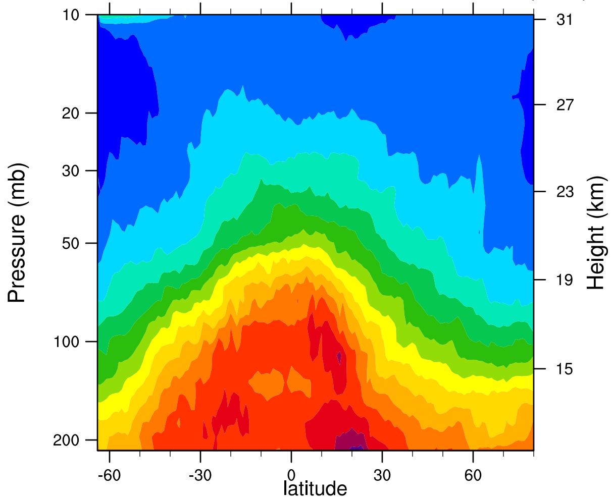
2006d013 12.1MicronExtinction_Combined ( \text{km}^{-1} )
