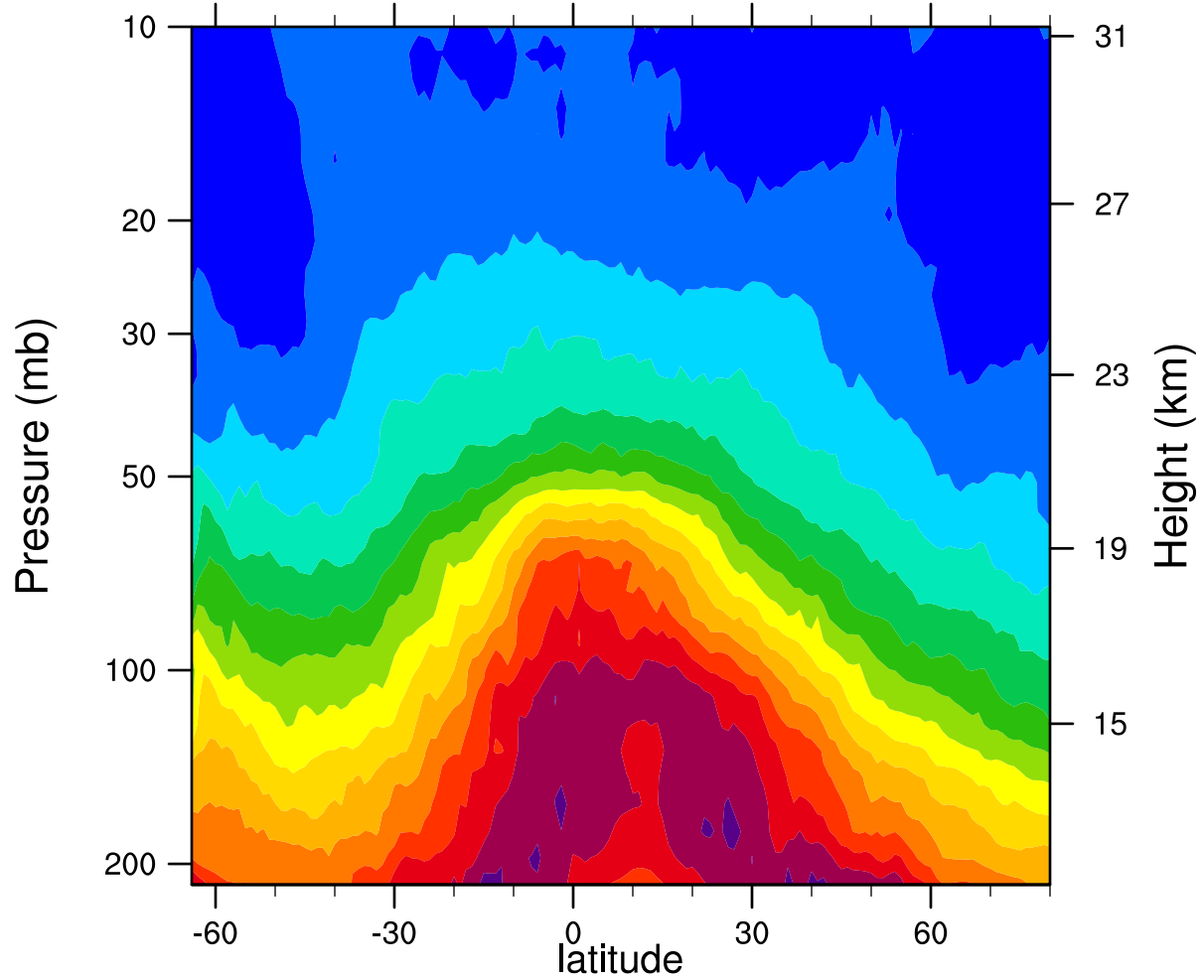
2006d251 12.1MicronExtinction_Combined ( \text{km}^{-1} )
