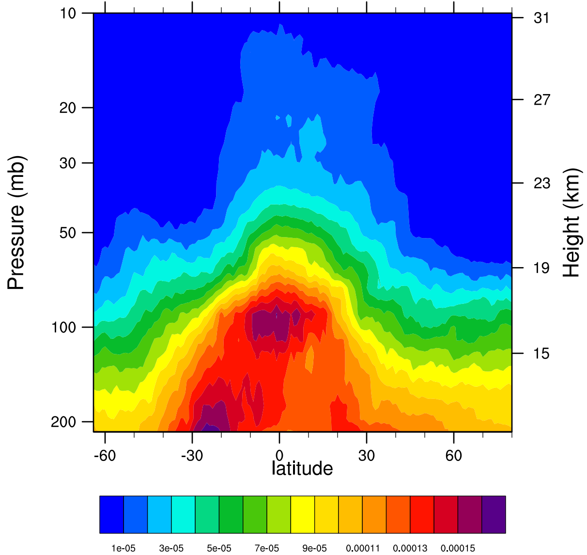
2006d317 12.1MicronExtinction_Combined (km -1 )
