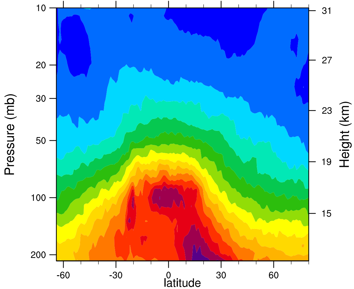
2006d075 12.1MicronExtinction_Combined ( \text{km}^{-1} )
