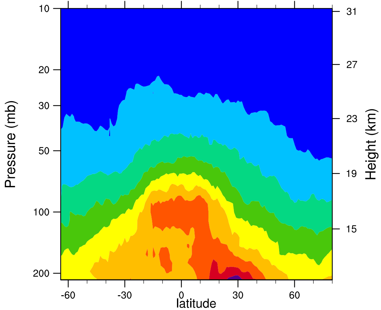
2006d101 12.1MicronExtinction_Combined (km -1 )
