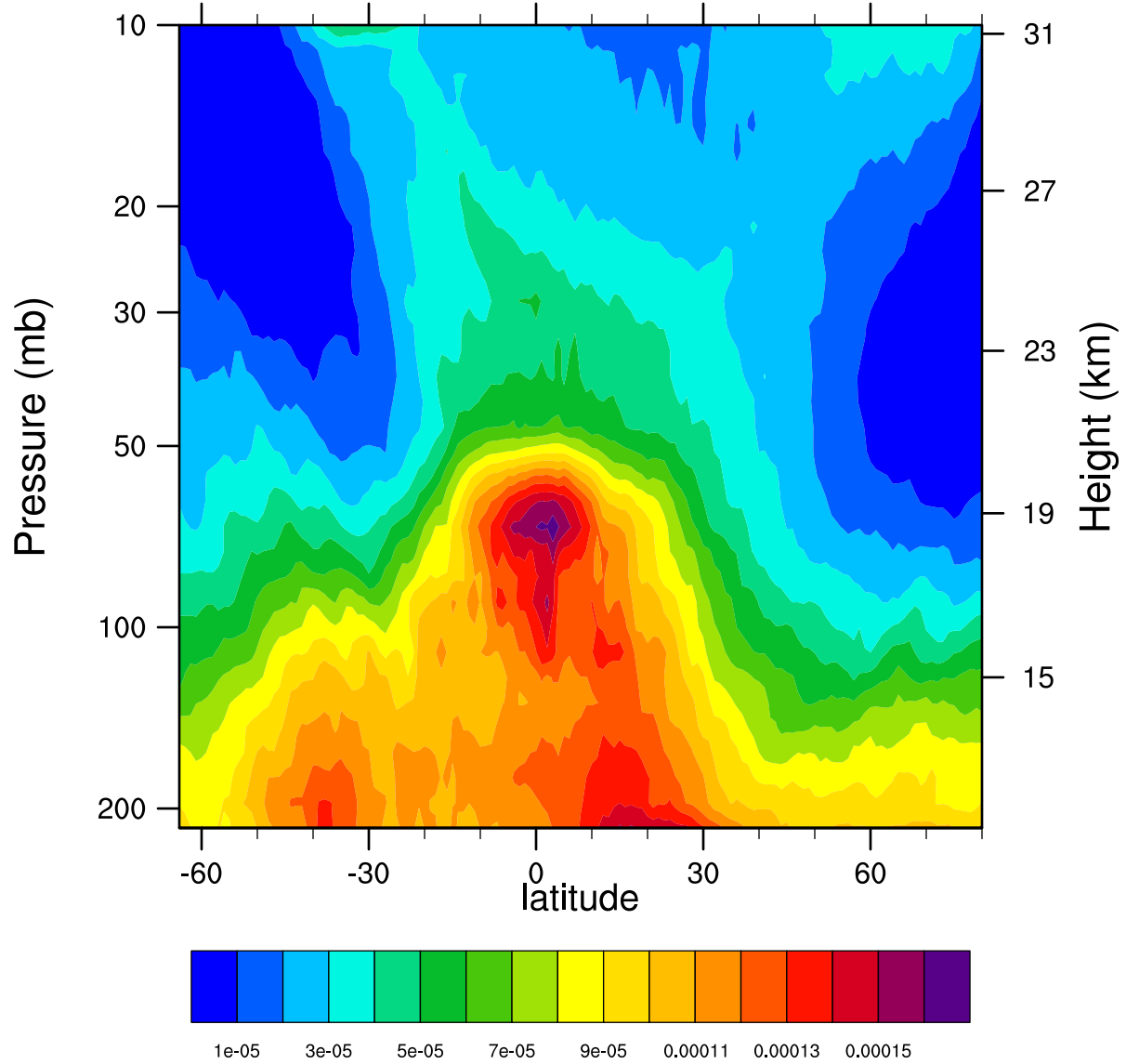
2005d070 12.1MicronExtinction_Combined (km -1 )
