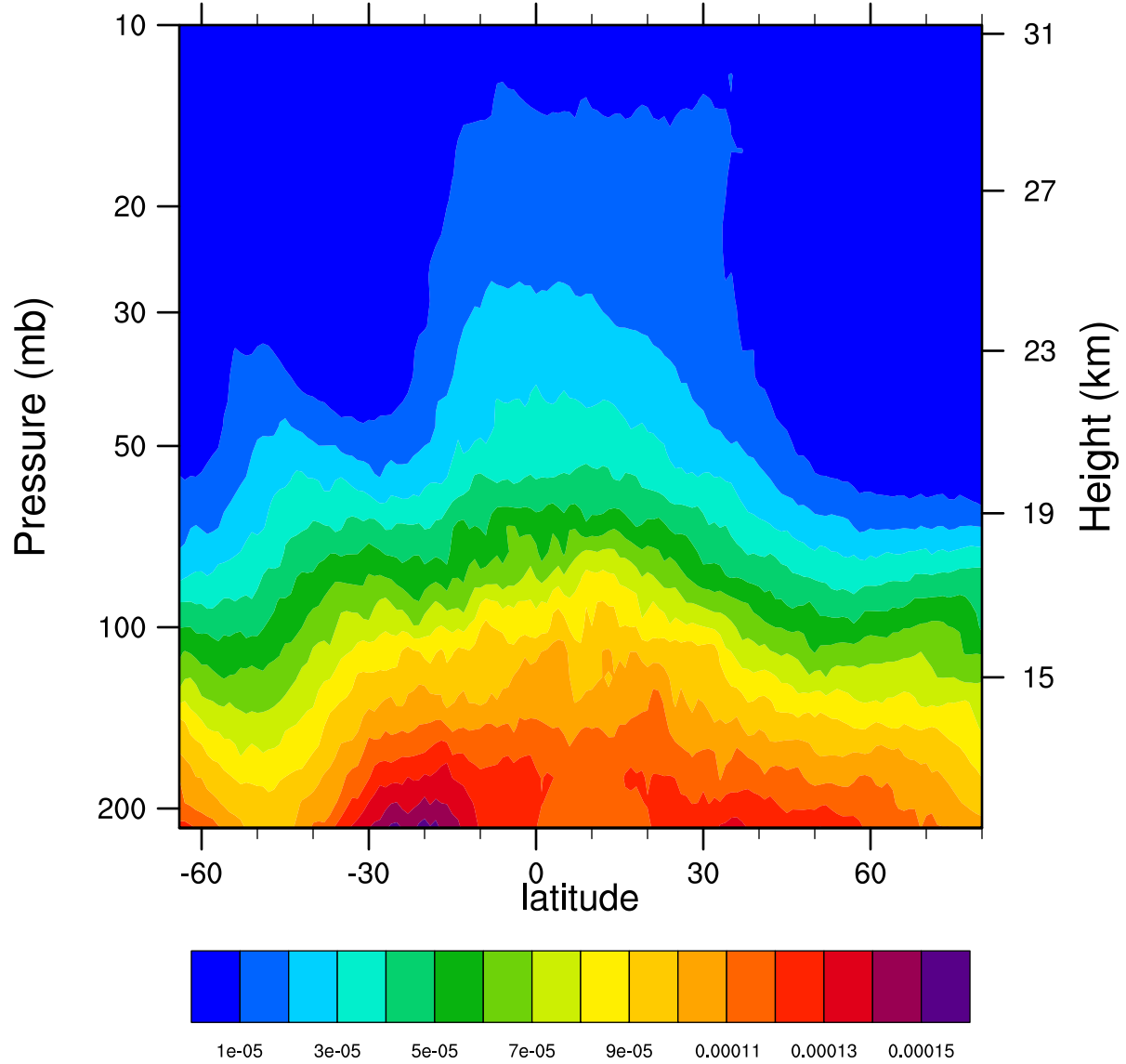
2007d276 12.1MicronExtinction_Combined (km -1 )
