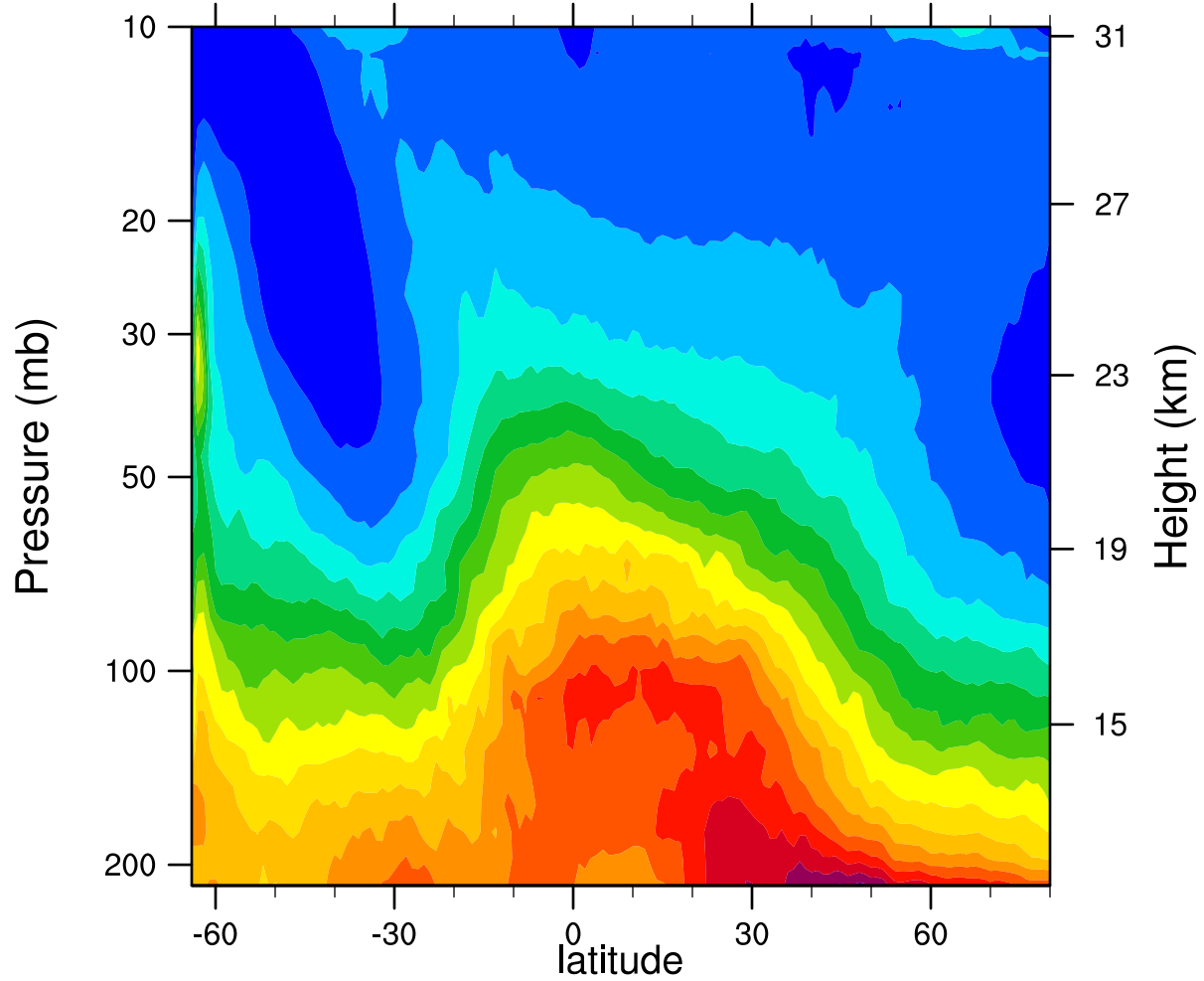
2005d200 12.1MicronExtinction_Combined (km -1 )
