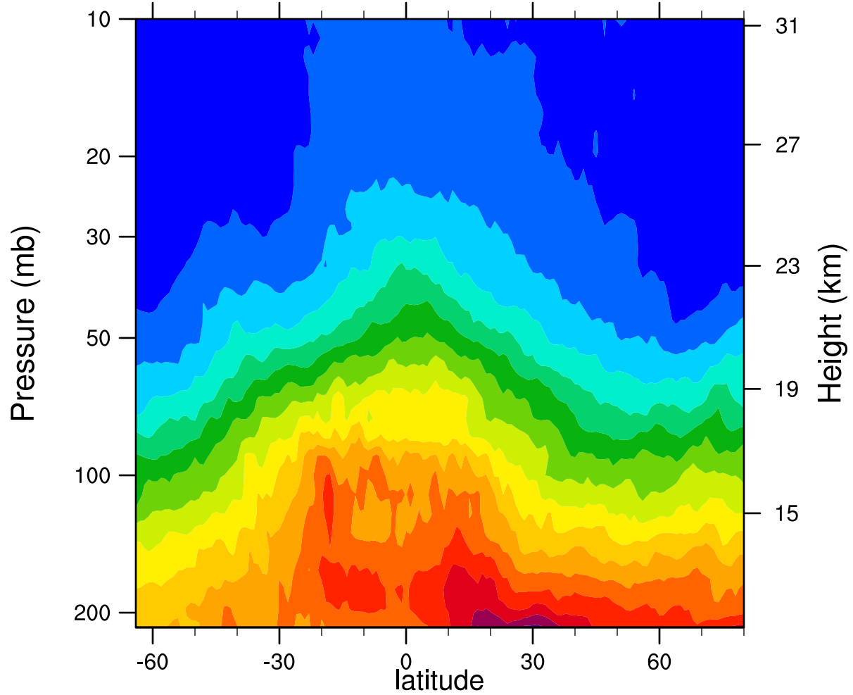
2007d087 12.1MicronExtinction_Combined ( \text{km}^{-1} )
