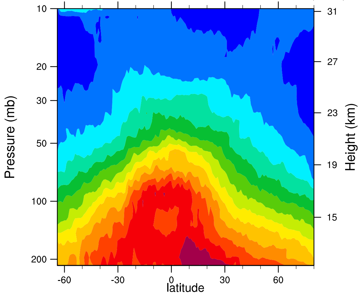
2006d037 12.1MicronExtinction_Combined (km -1 )
