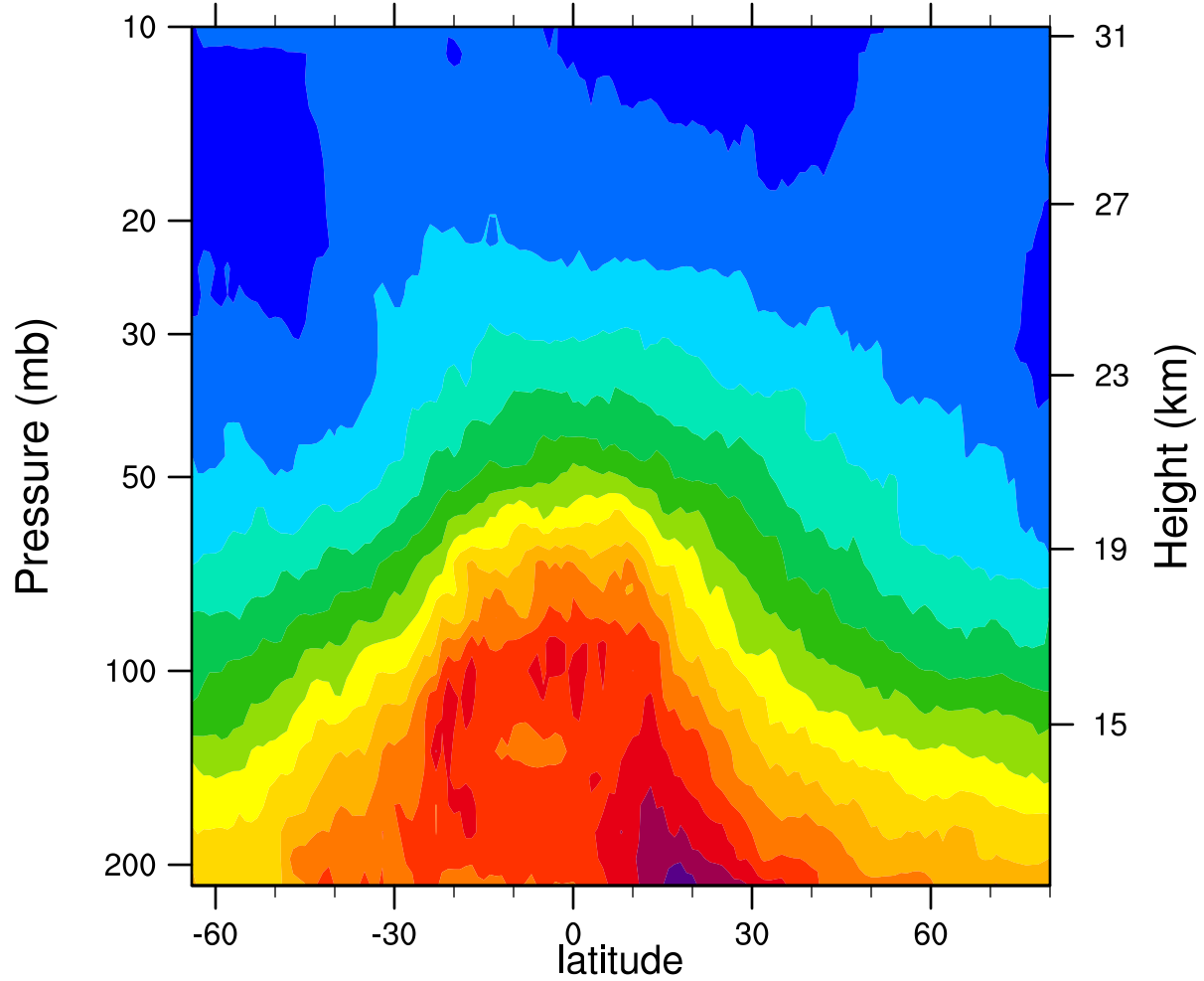
2006d057 12.1MicronExtinction_Combined (km -1 )
