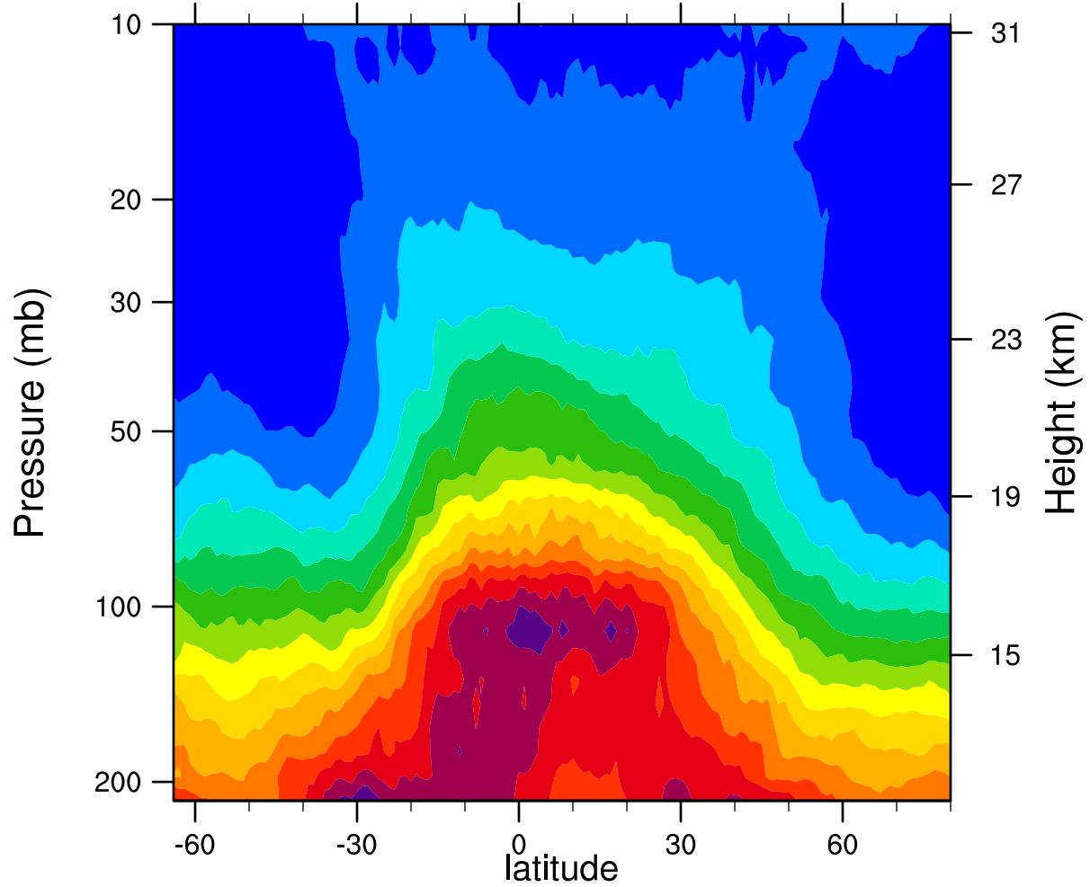
2005d269 12.1MicronExtinction_Combined (km -1 )
