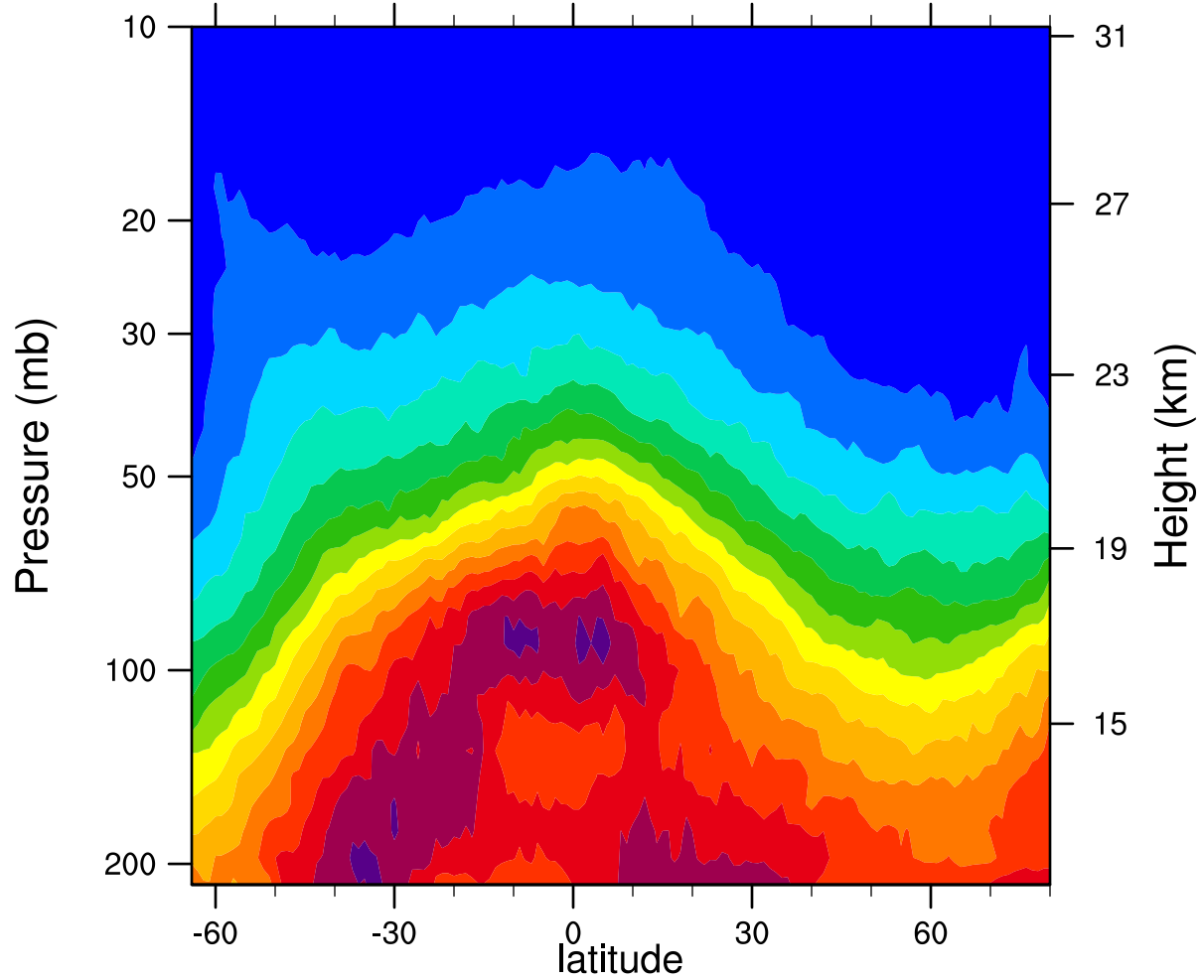
2007d009 12.1MicronExtinction_Combined (km -1 )
