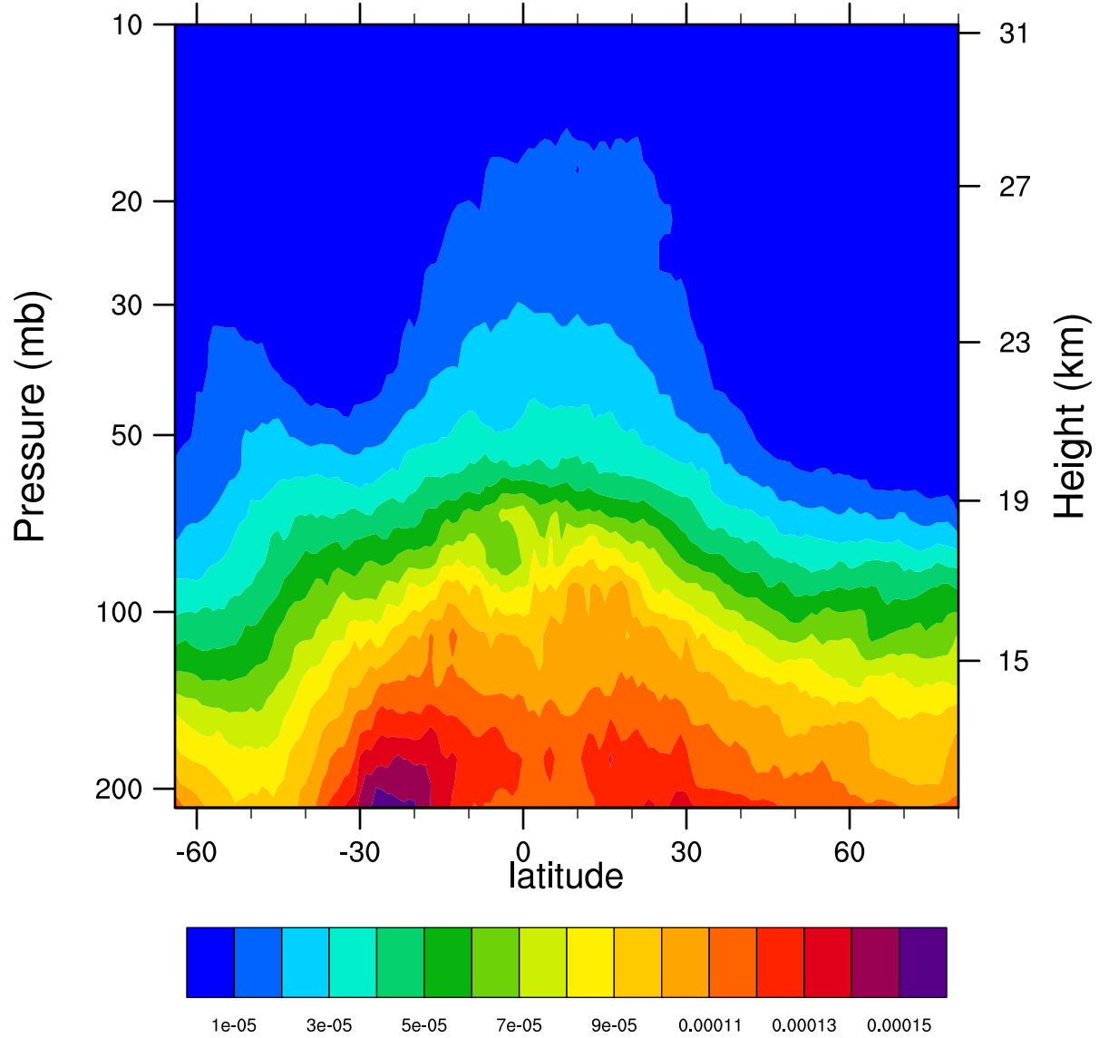
2007d311 12.1MicronExtinction_Combined (km -1 )
