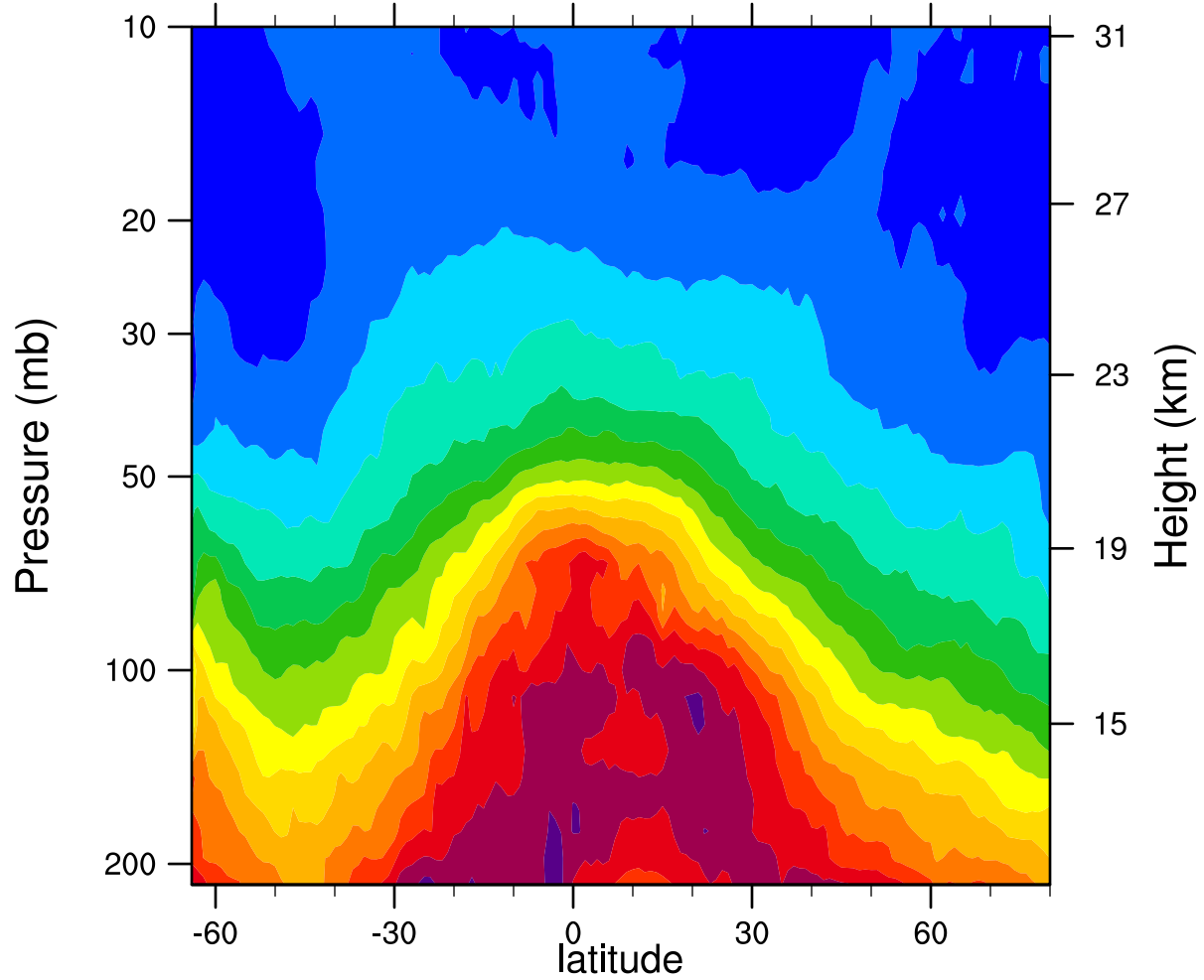
2006d264 12.1MicronExtinction_Combined (km -1 )
