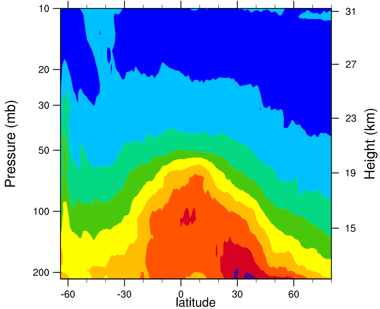
2006d200 12.1MicronExtinction_Combined (km -1 )
