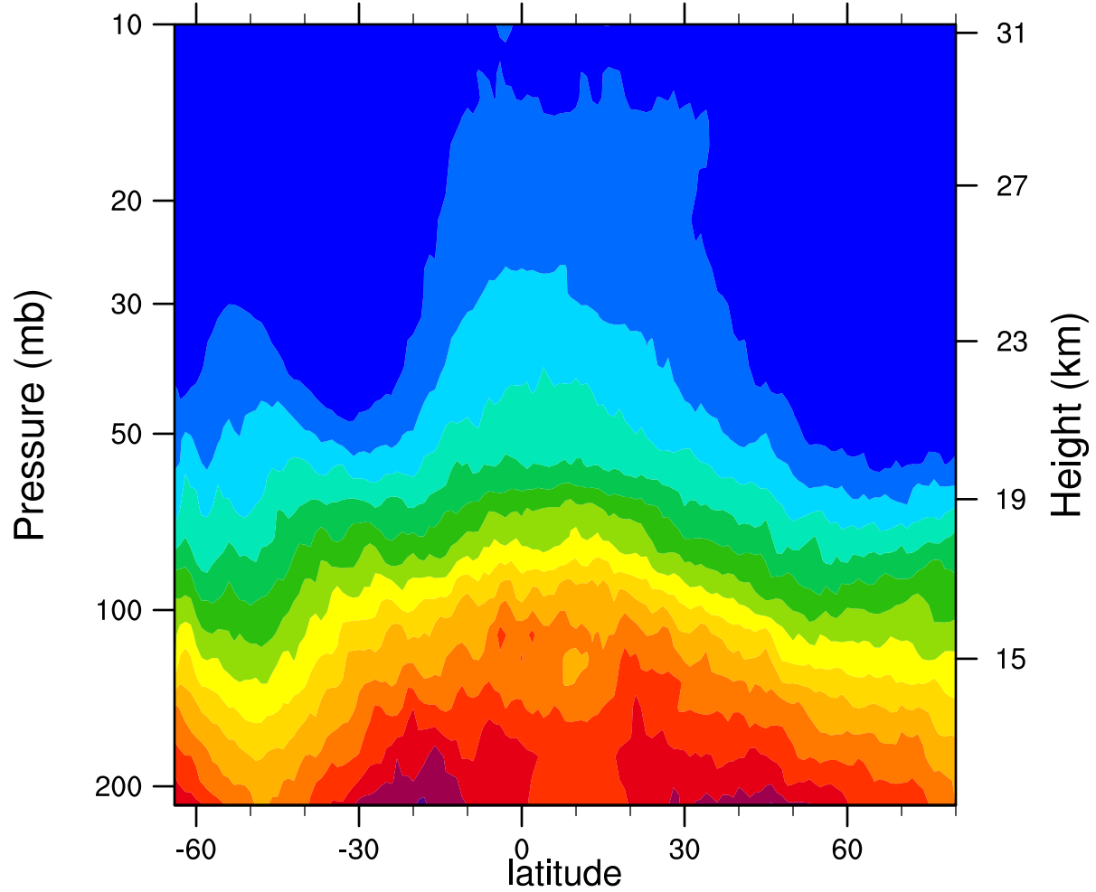
2007d265 12.1MicronExtinction_Combined (km -1 )
