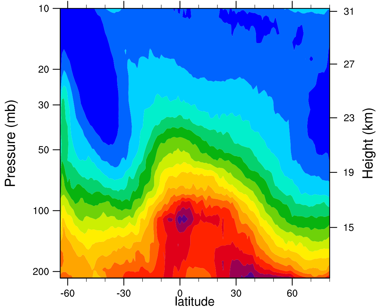
2005d214 12.1MicronExtinction_Combined (km -1 )
