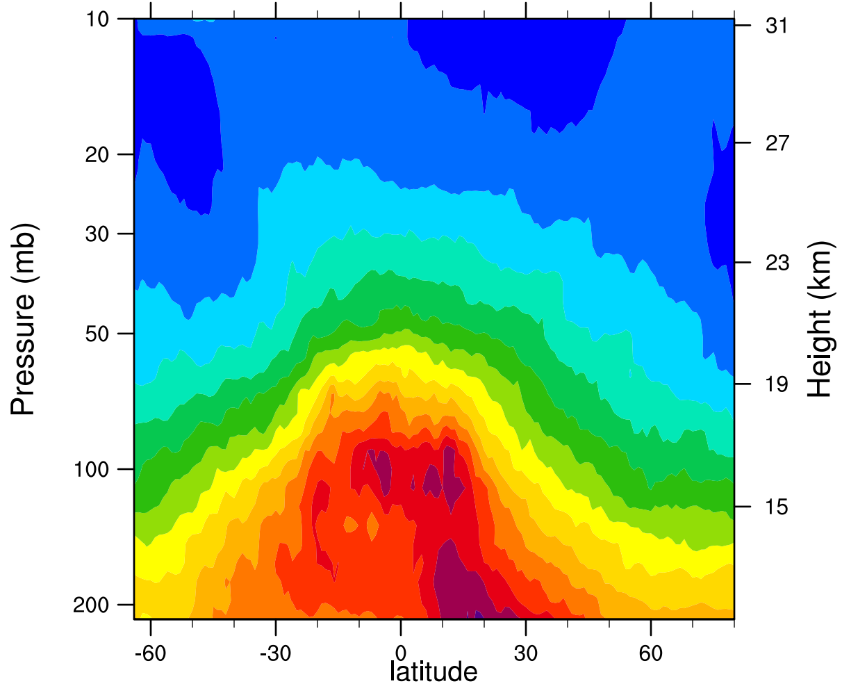
2006d067 12.1MicronExtinction_Combined (km -1 )
