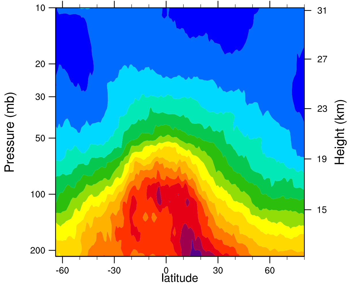
2006d065 12.1MicronExtinction_Combined (km -1 )
