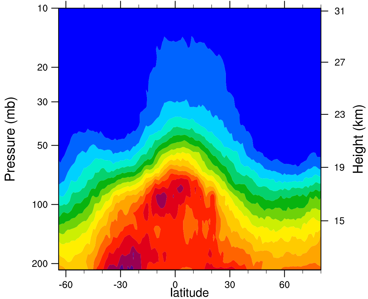
2006d333 12.1MicronExtinction_Combined ( \text{km}^{-1} )
