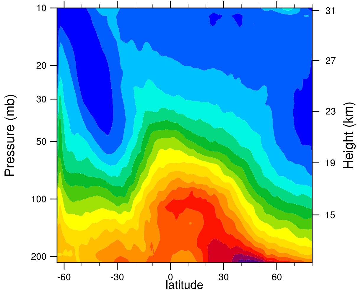
2005d194 12.1MicronExtinction_Combined (km -1 )
