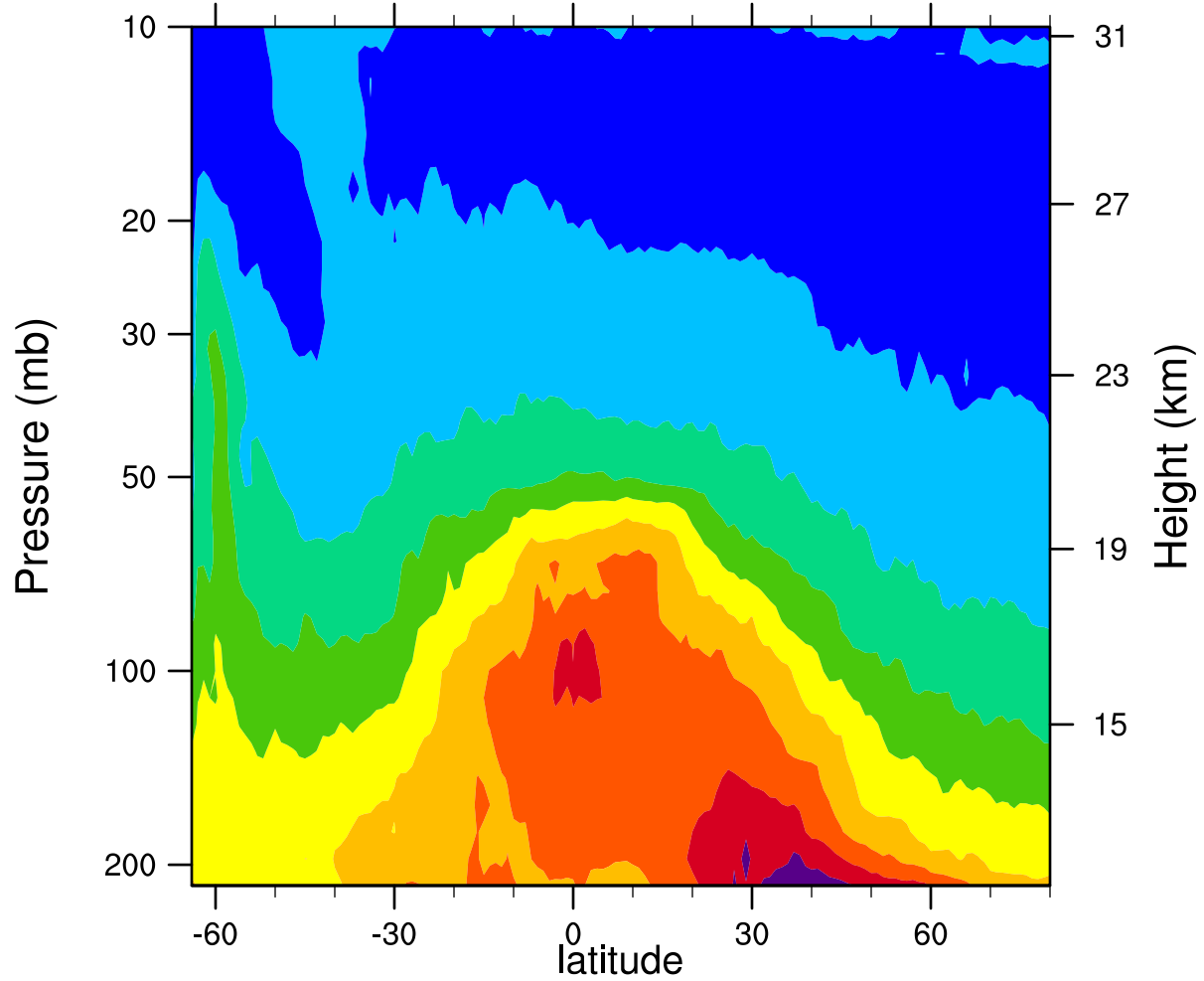
2006d190 12.1MicronExtinction_Combined (km -1 )
