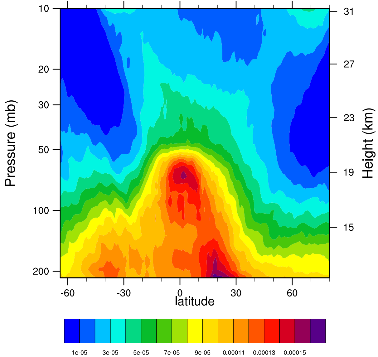
2005d080 12.1MicronExtinction_Combined ( \text{km}^{-1} )
