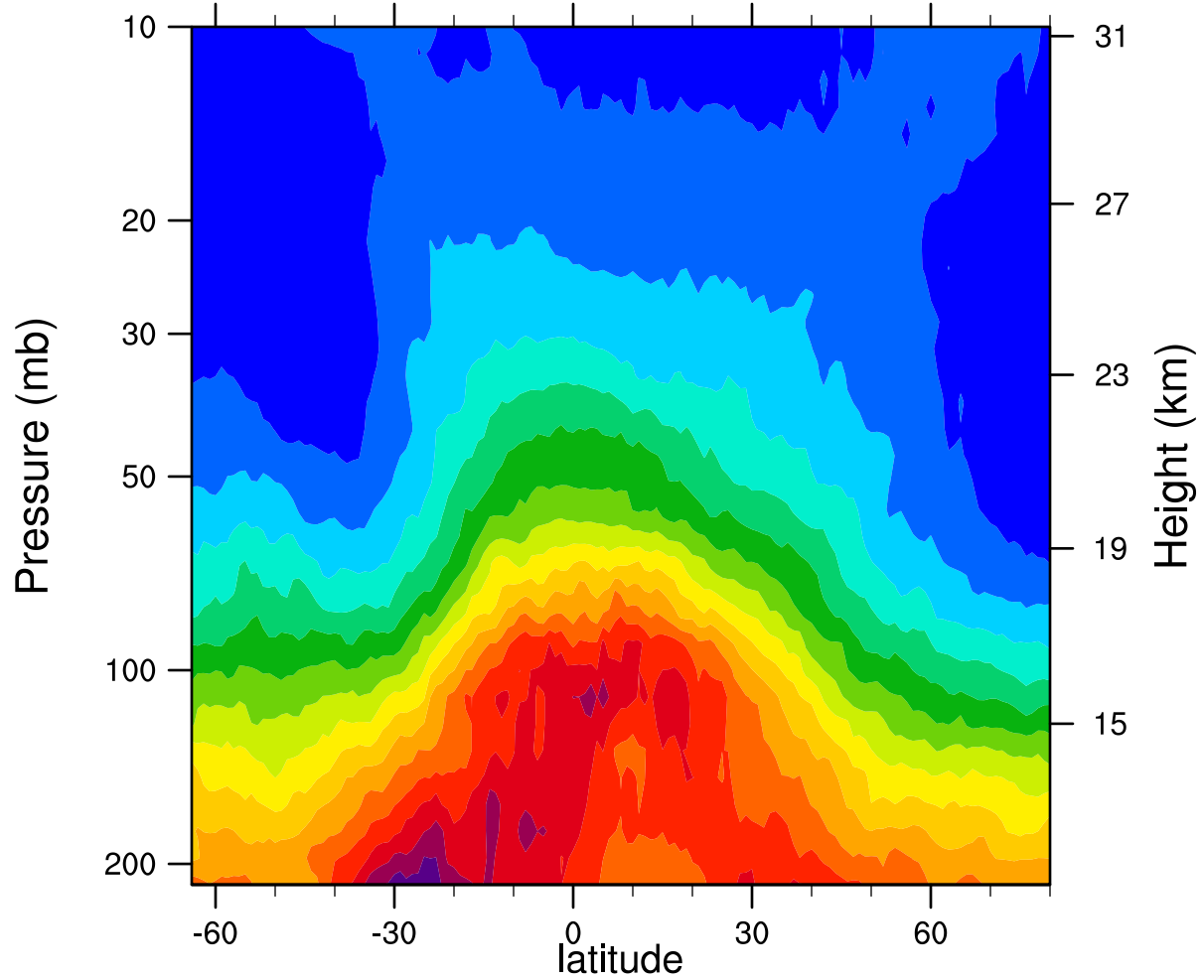
2005d283 12.1MicronExtinction_Combined (km -1 )
