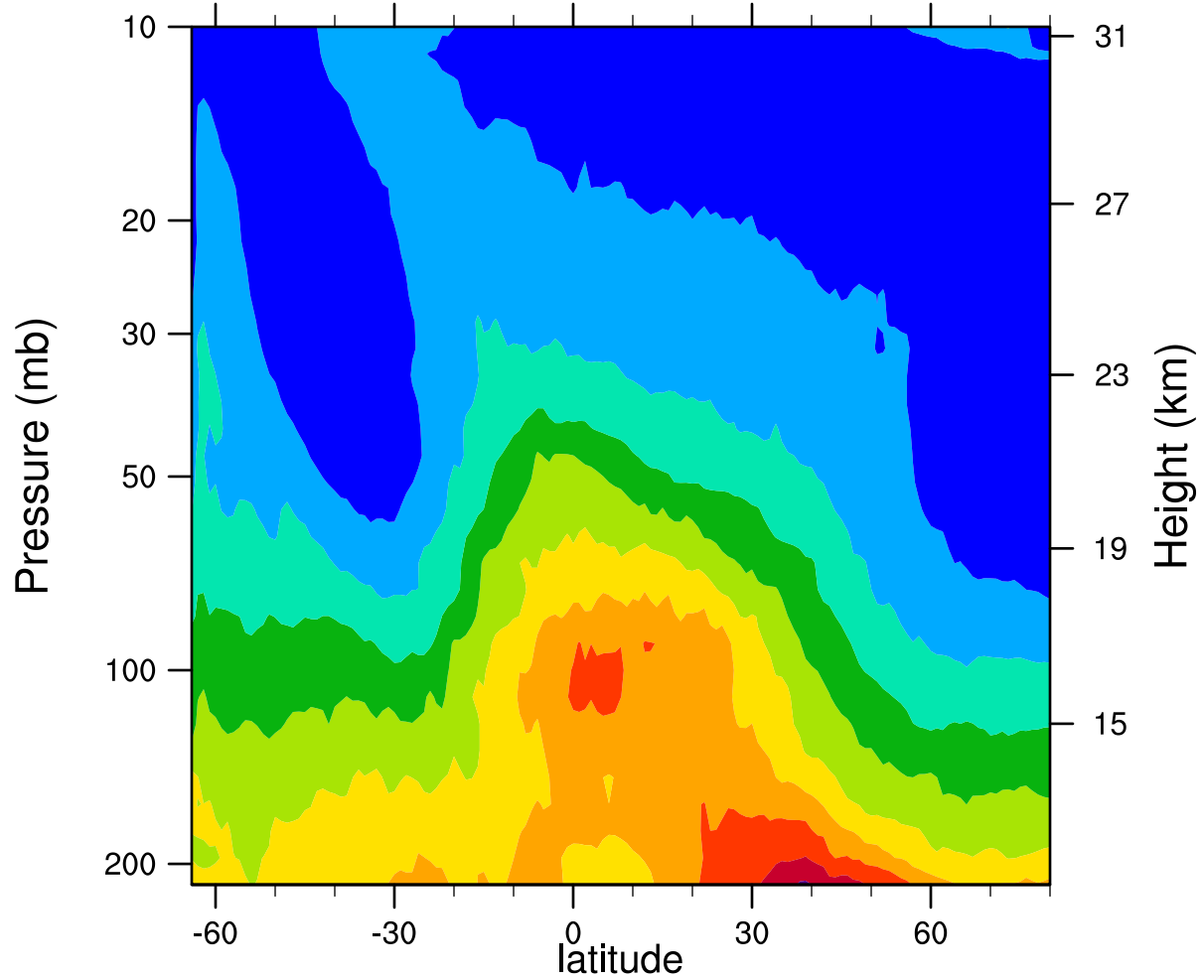
2005d176 12.1MicronExtinction_Combined ( \text{km}^{-1} )
