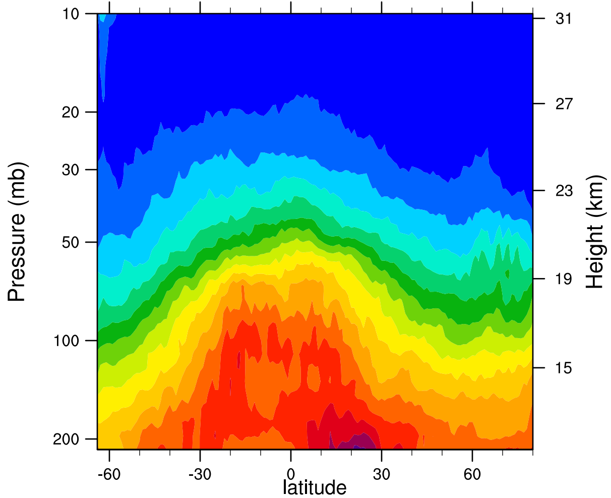
2007d052 12.1MicronExtinction_Combined (km -1 )
