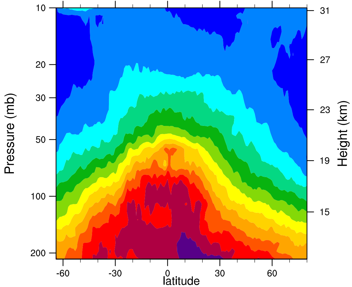
2006d030 12.1MicronExtinction_Combined (km -1 )
