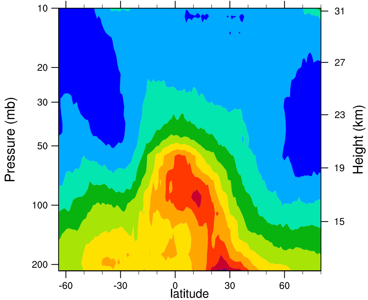
2005d118 12.1MicronExtinction_Combined (km -1 )
