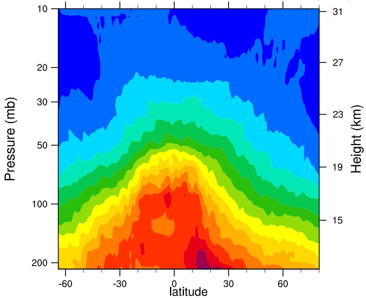
2006d047 12.1MicronExtinction_Combined (km -1 )
