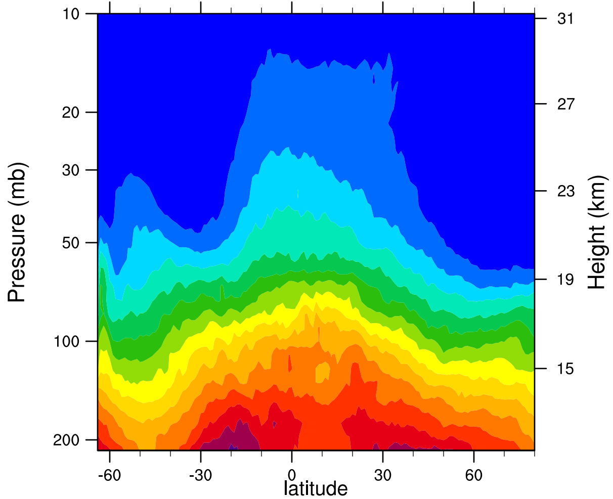
2007d268 12.1MicronExtinction_Combined (km -1 )
