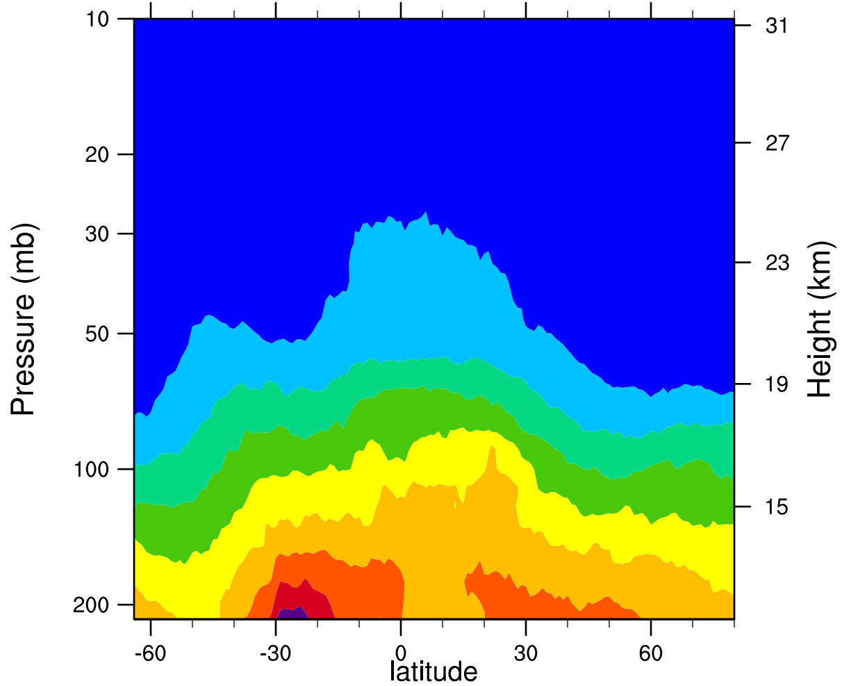
2007d286 12.1MicronExtinction_Combined (km -1 )
