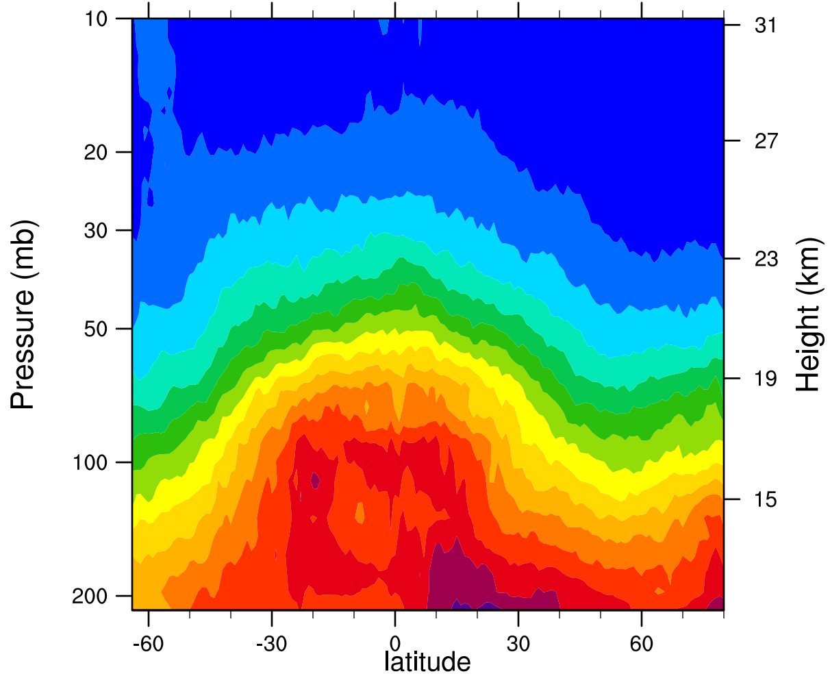
2007d067 12.1MicronExtinction_Combined (km -1 )
