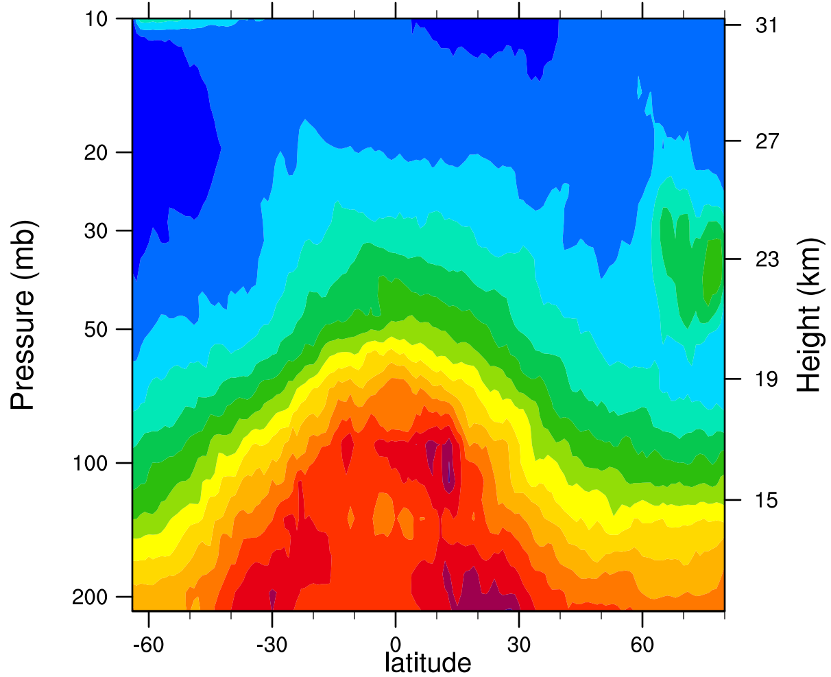
2006d001 12.1MicronExtinction_Combined (km -1 )
