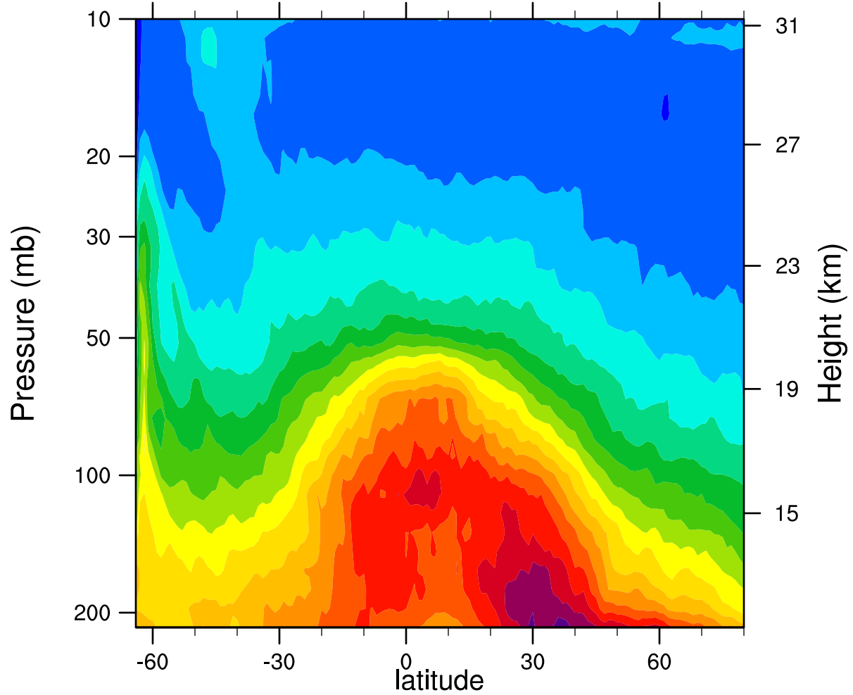
2006d203 12.1MicronExtinction_Combined ( \text{km}^{-1} )
