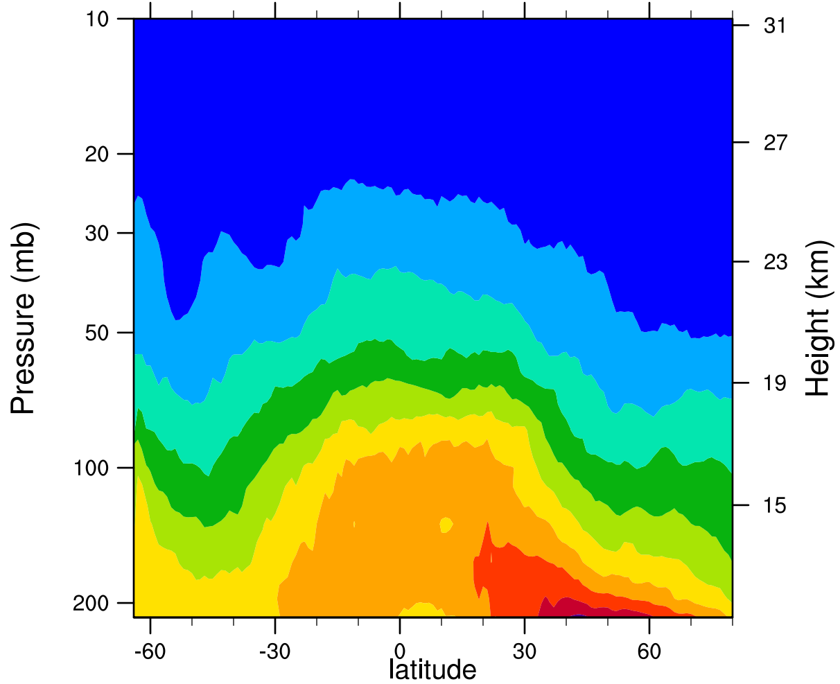
2007d190 12.1MicronExtinction_Combined (km -1 )
