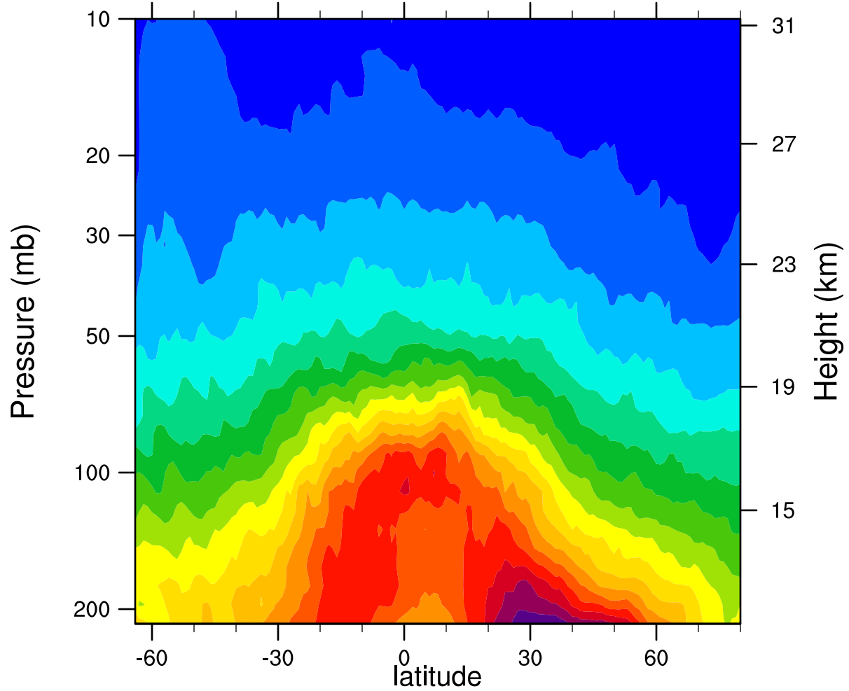
2006d151 12.1MicronExtinction_Combined ( \text{km}^{-1} )
