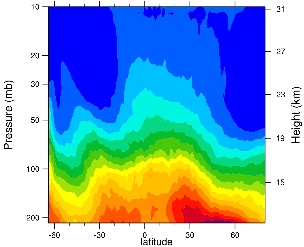
2007d221 12.1MicronExtinction_Combined (km -1 )
