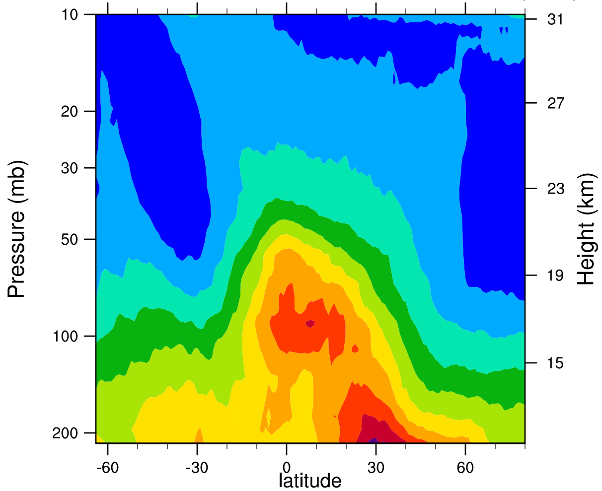
2005d142 12.1MicronExtinction_Combined (km -1 )
