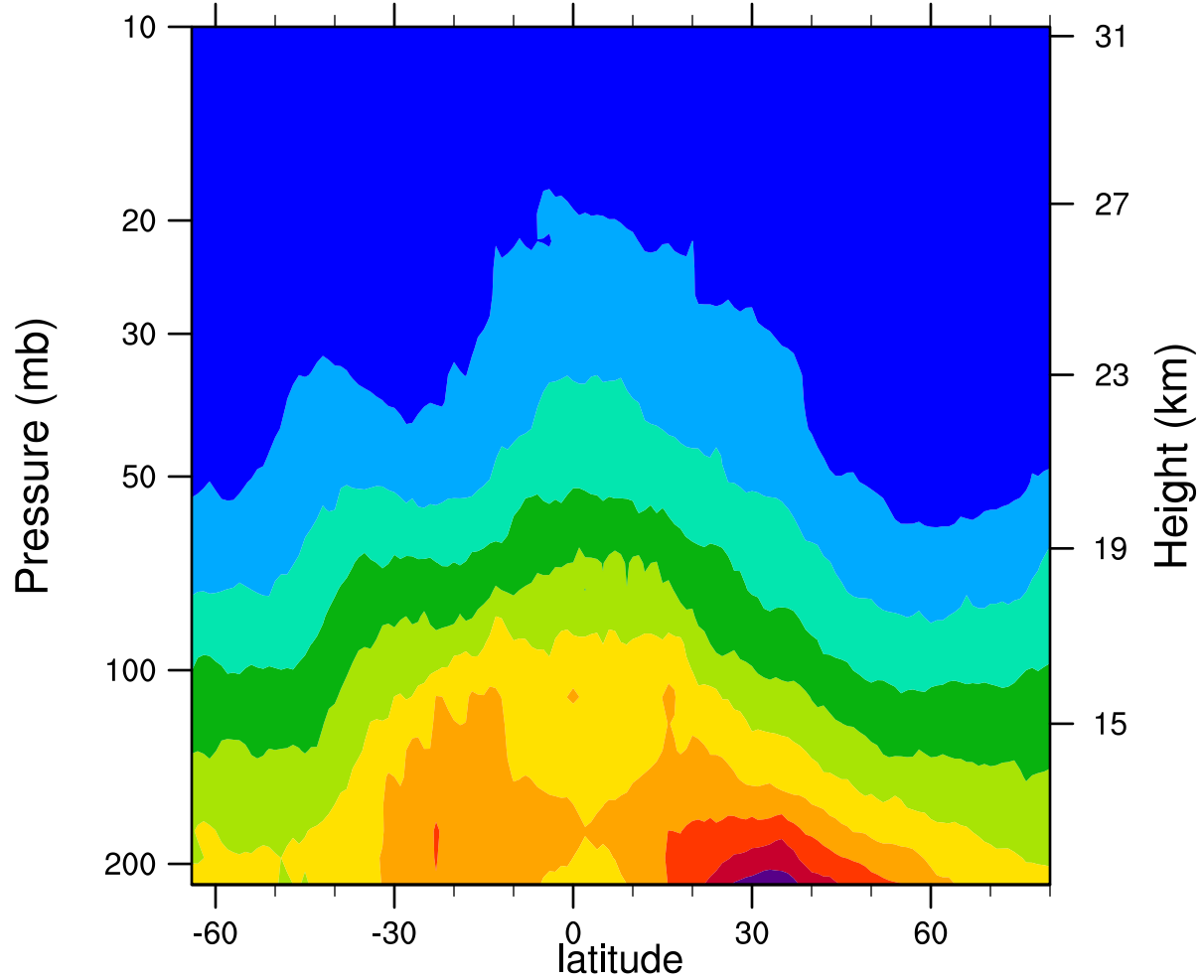
2007d128 12.1MicronExtinction_Combined (km -1 )
