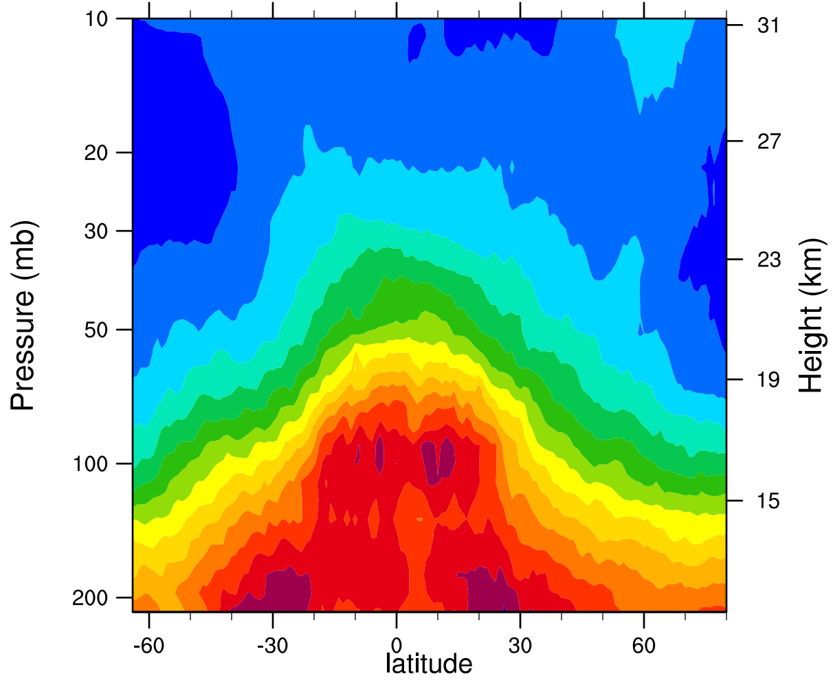
2005d323 12.1MicronExtinction_Combined (km -1 )
