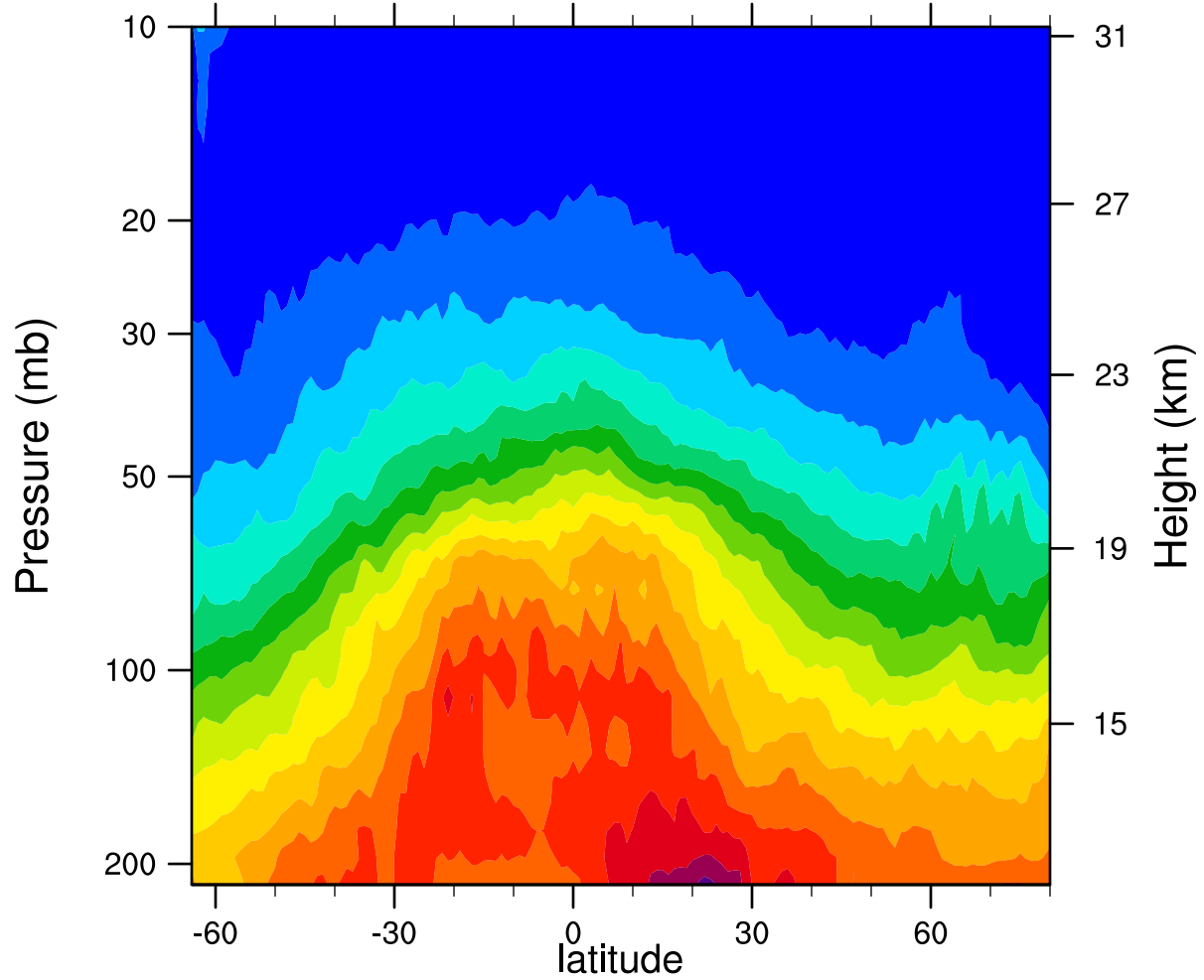
2007d053 12.1MicronExtinction_Combined (km -1 )
