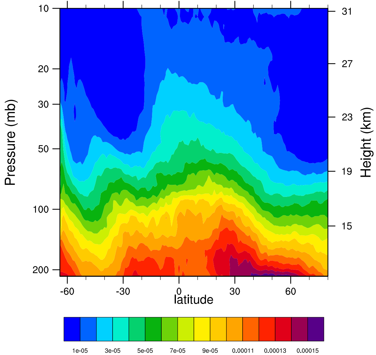
2007d227 12.1MicronExtinction_Combined (km -1 )
