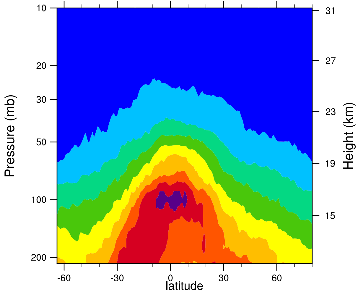
2006d304 12.1MicronExtinction_Combined ( \text{km}^{-1} )
