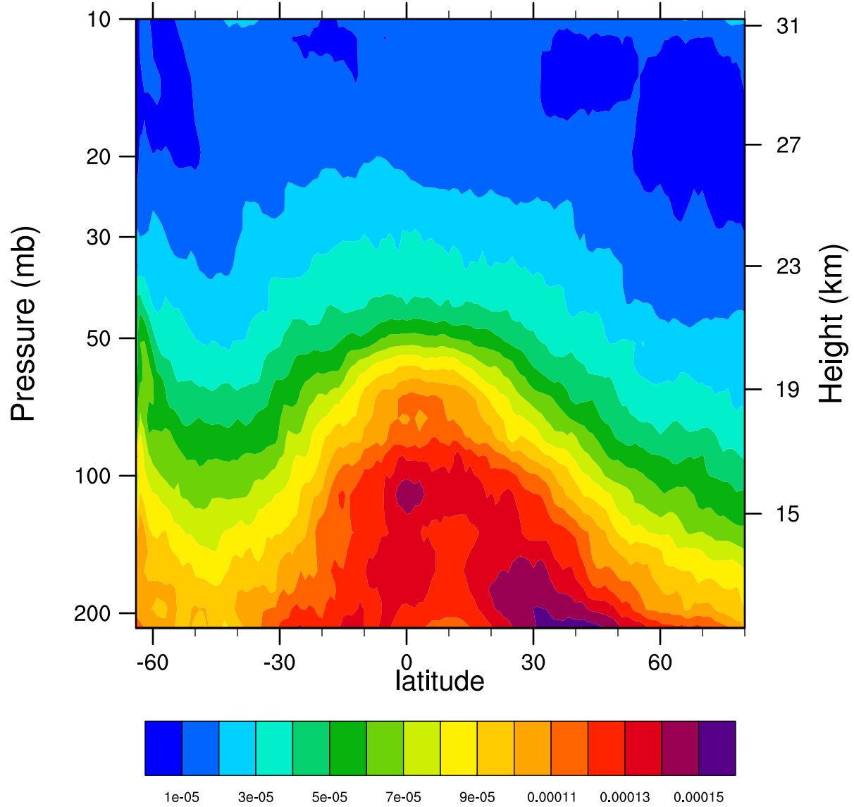
2006d230 12.1MicronExtinction_Combined (km -1 )
