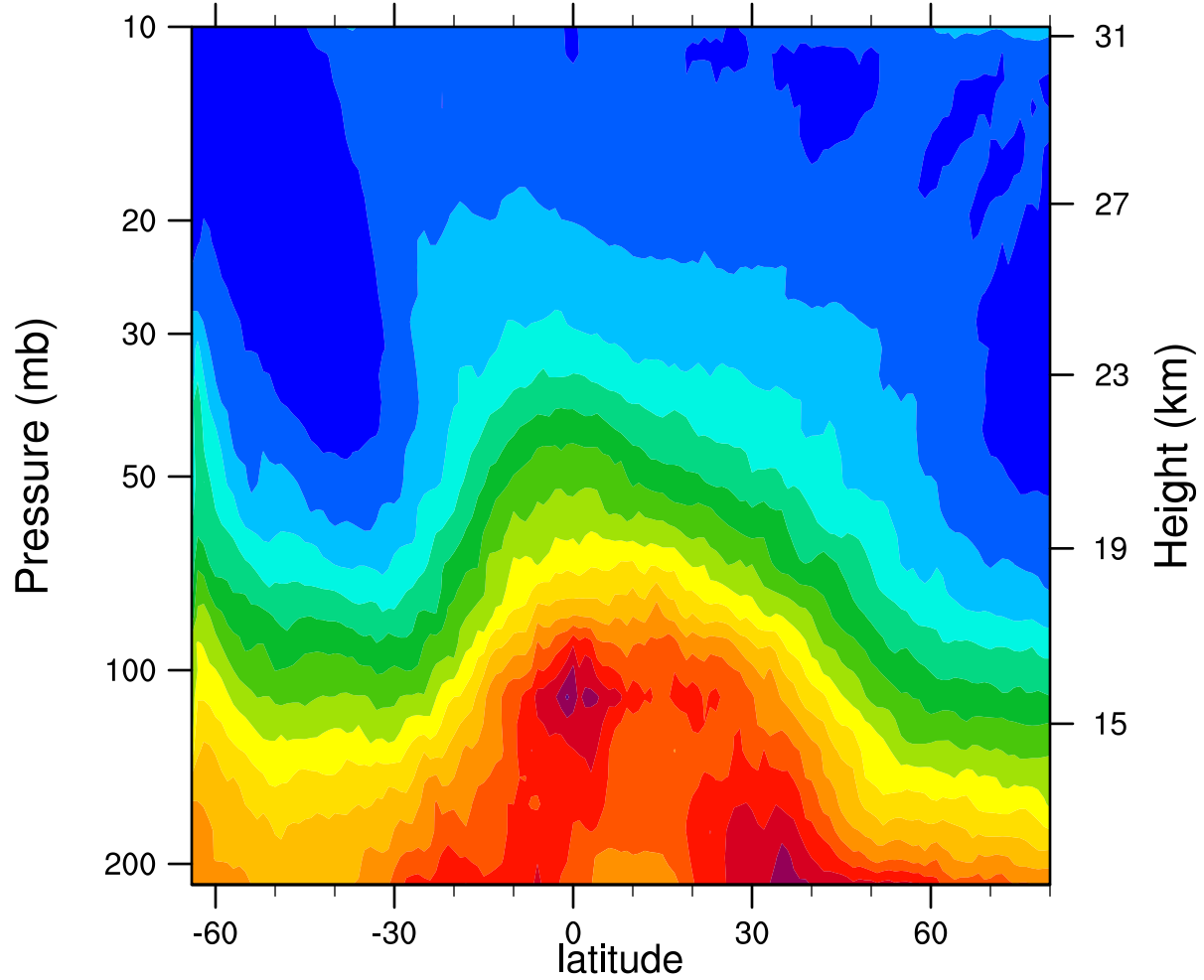
2005d222 12.1MicronExtinction_Combined (km -1 )
