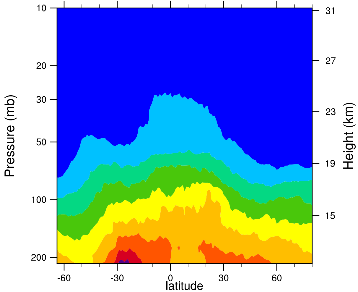
2007d287 12.1MicronExtinction_Combined (km -1 )
