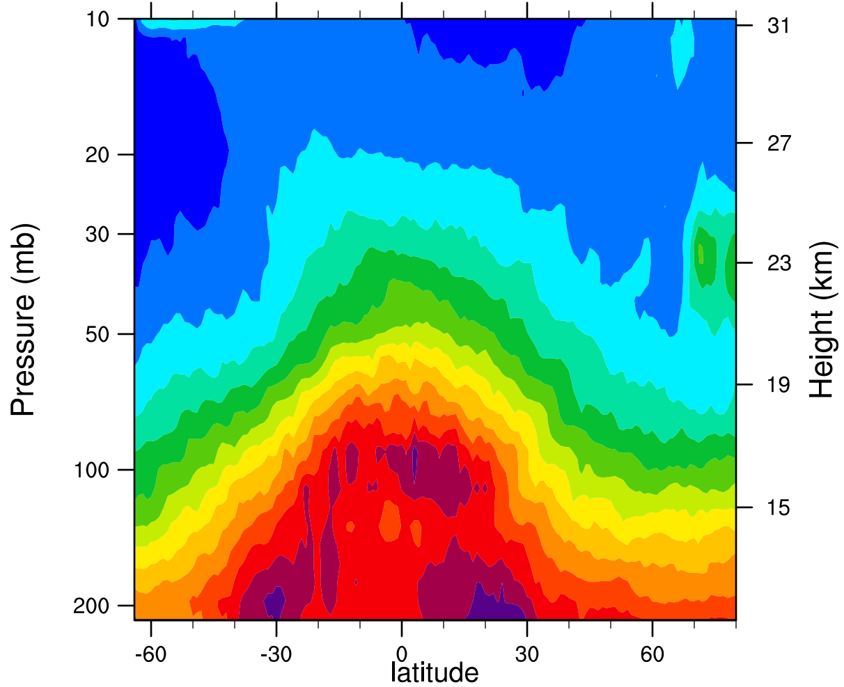
2005d360 12.1MicronExtinction_Combined (km -1 )
