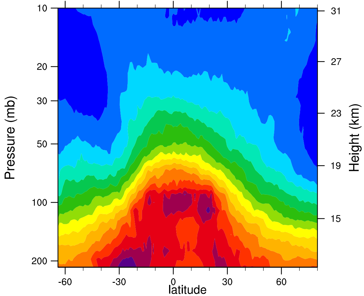
2005d303 12.1MicronExtinction_Combined (km -1 )
