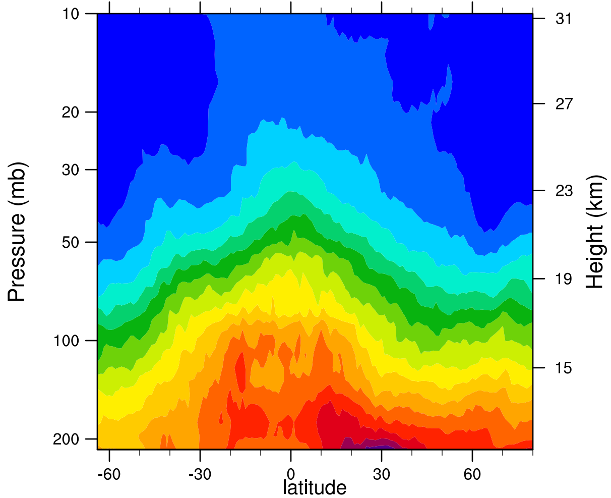
2007d091 12.1MicronExtinction_Combined (km -1 )
