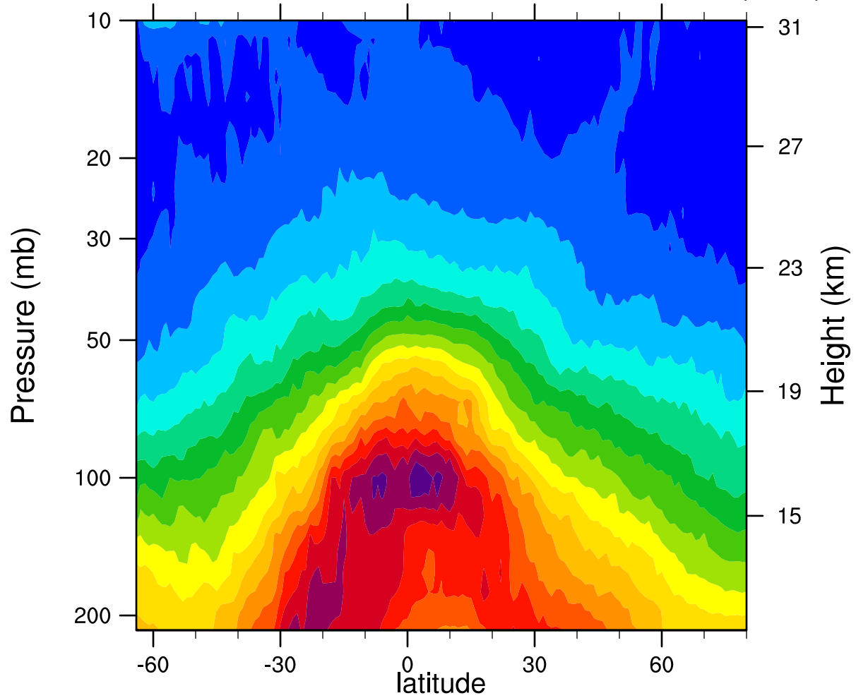
2006d300 12.1MicronExtinction_Combined (km -1 )
