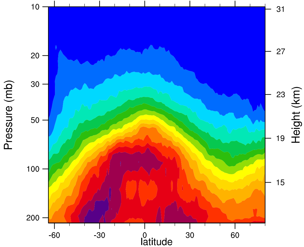
2007d002 12.1MicronExtinction_Combined (km -1 )
