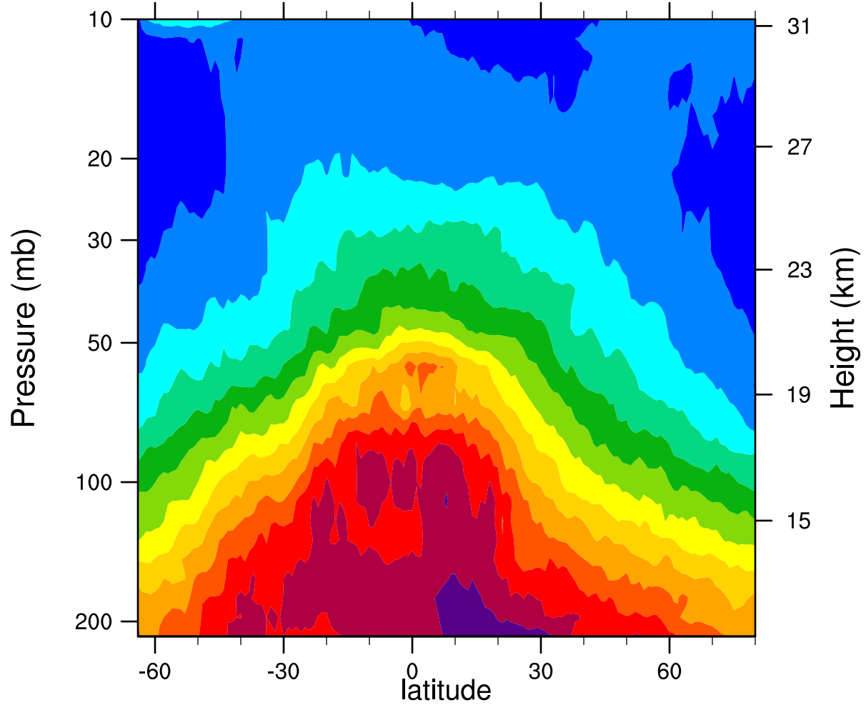
2006d029 12.1MicronExtinction_Combined (km -1 )
