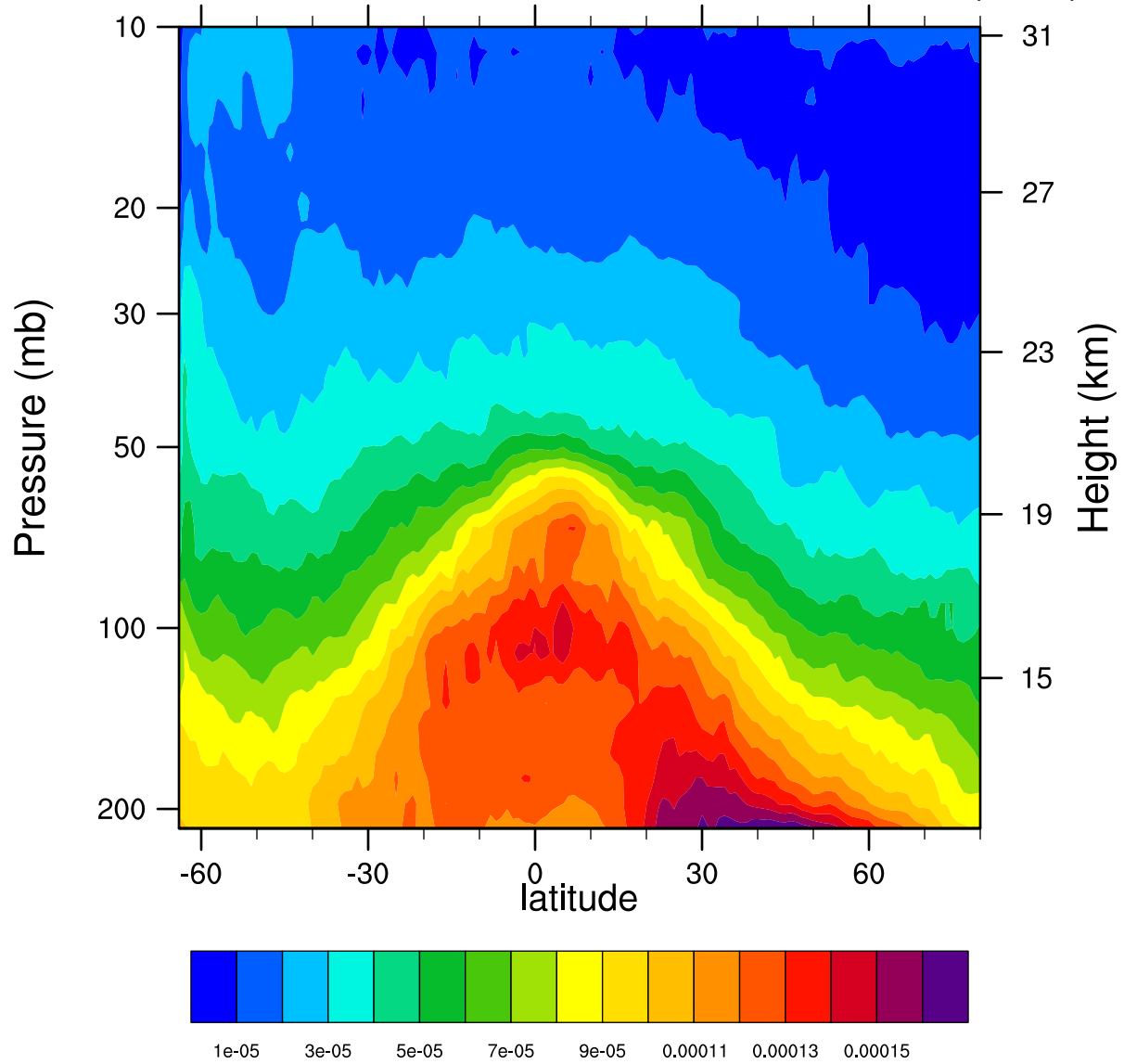
2006d175 12.1MicronExtinction_Combined (km -1 )
