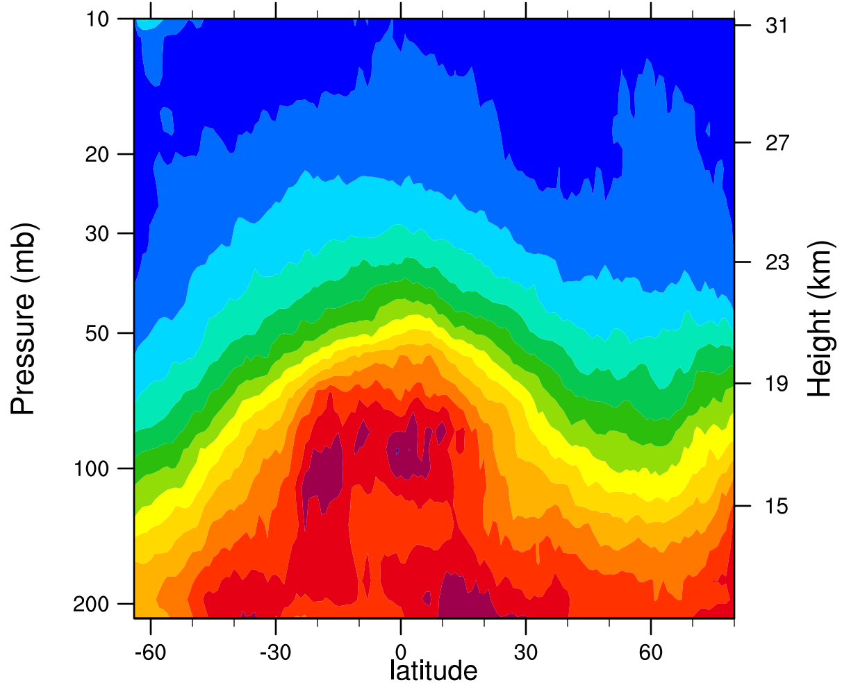
2007d034 12.1MicronExtinction_Combined (km -1 )
