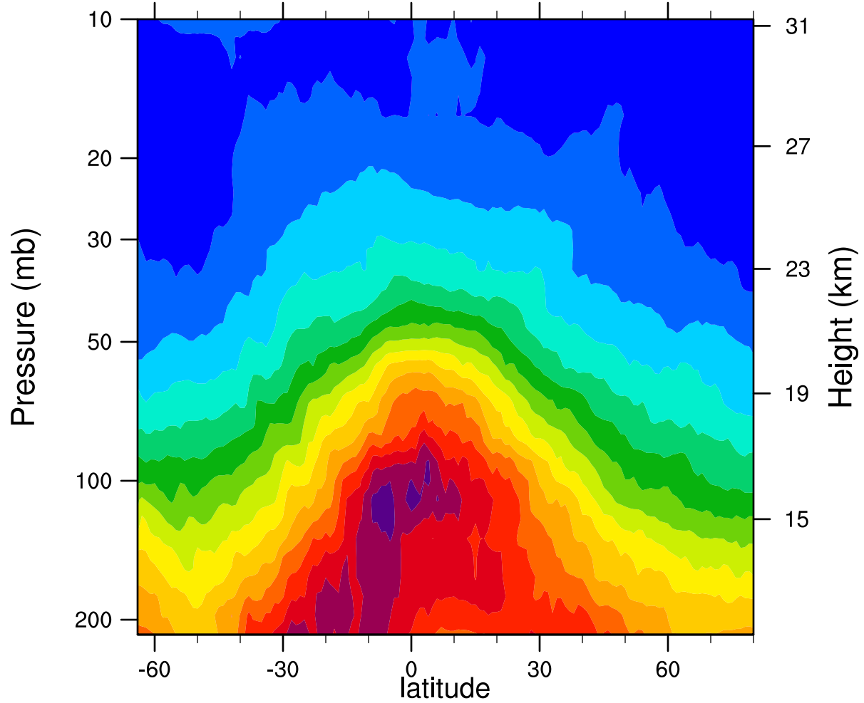
2006d289 12.1MicronExtinction_Combined (km -1 )
