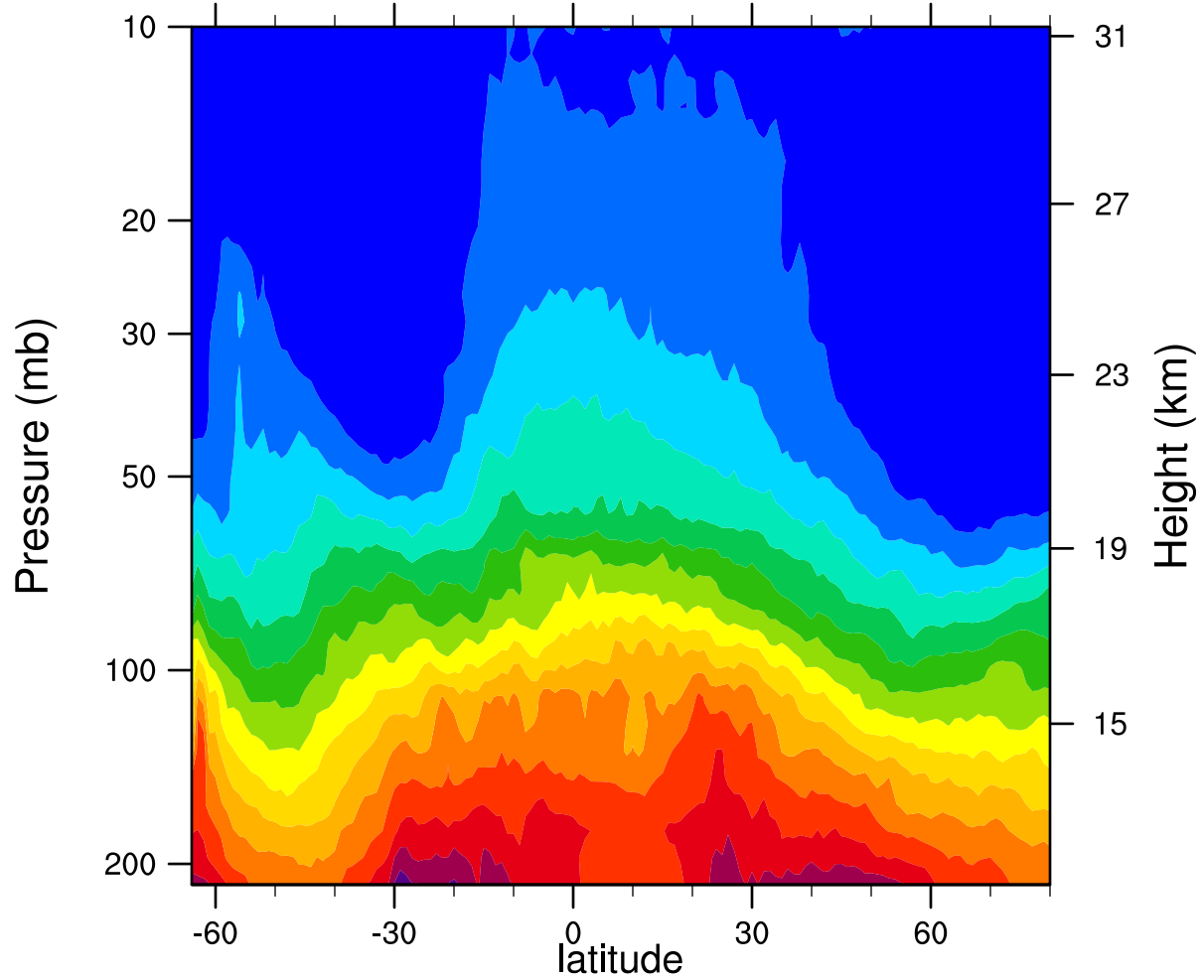
2007d259 12.1MicronExtinction_Combined ( \text{km}^{-1} )
