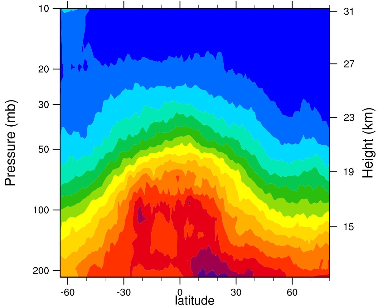
2007d062 12.1MicronExtinction_Combined (km -1 )
