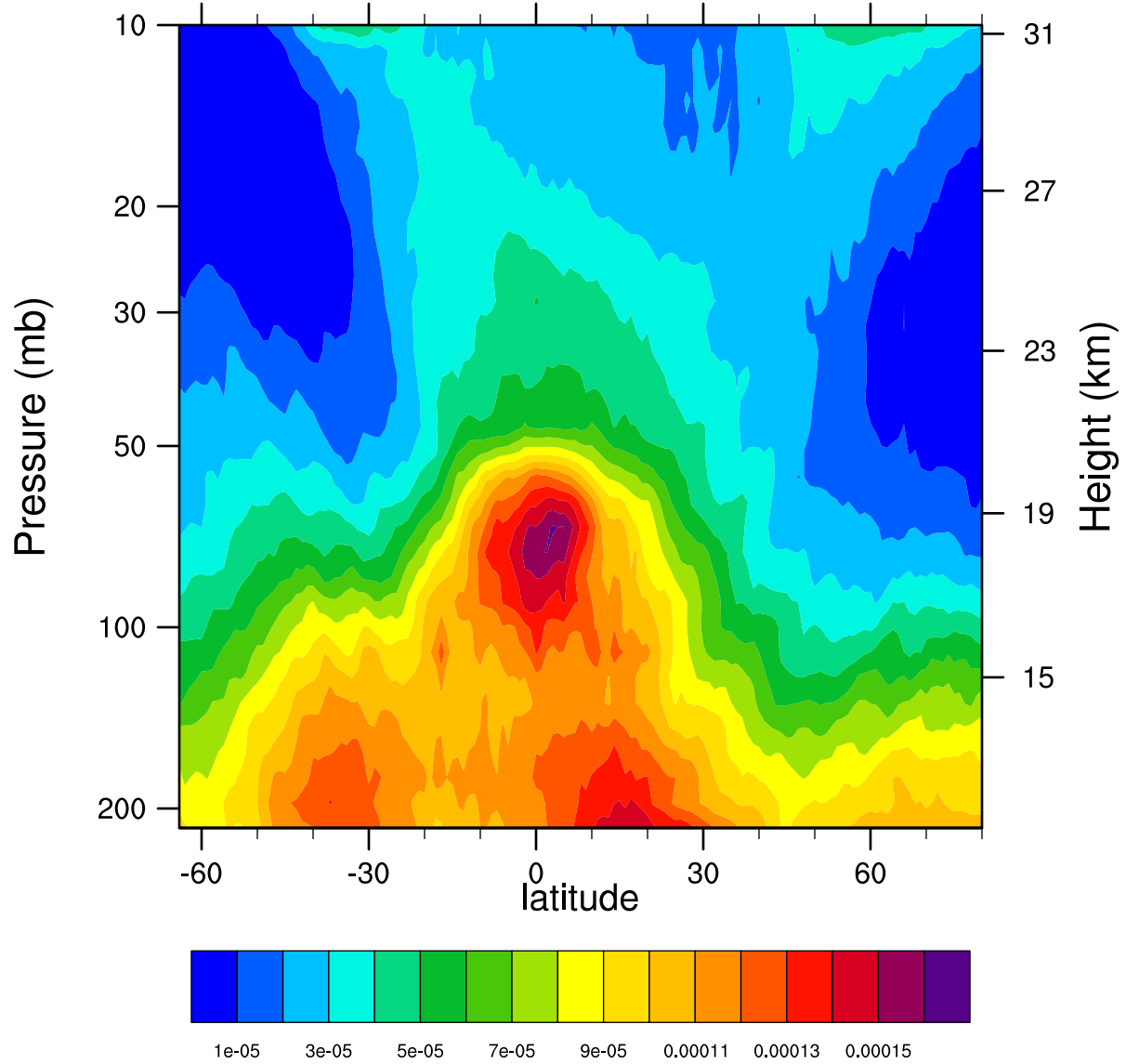
2005d056 12.1MicronExtinction_Combined (km -1 )
