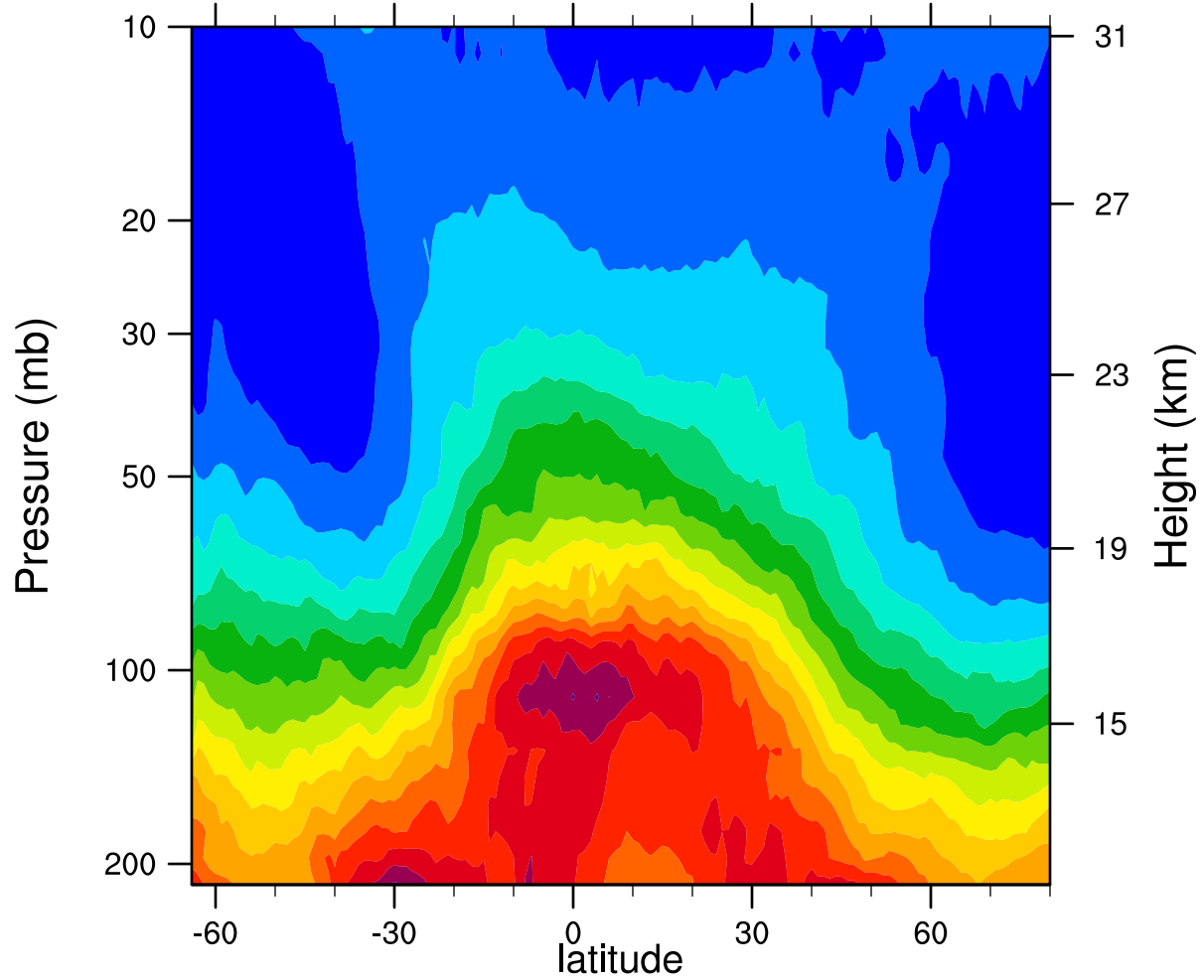
2005d263 12.1MicronExtinction_Combined (km -1 )
