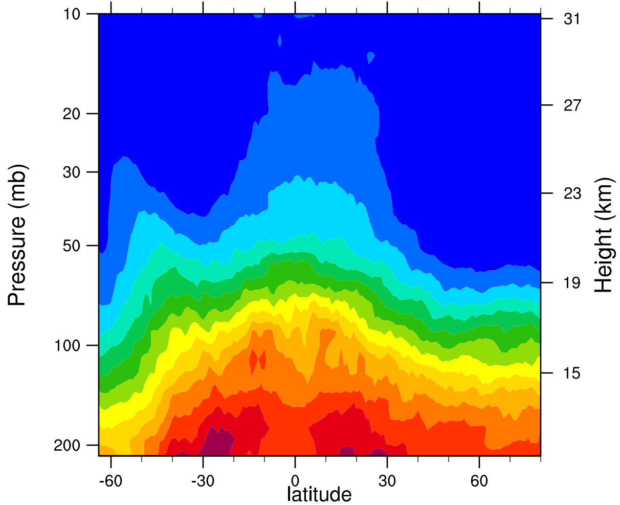
2007d331 12.1MicronExtinction_Combined (km -1 )
