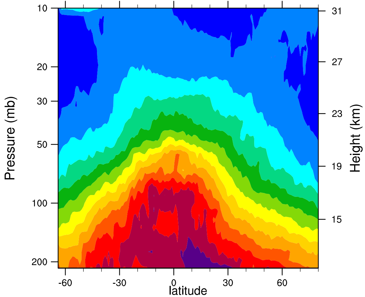
2006d033 12.1MicronExtinction_Combined (km -1 )
