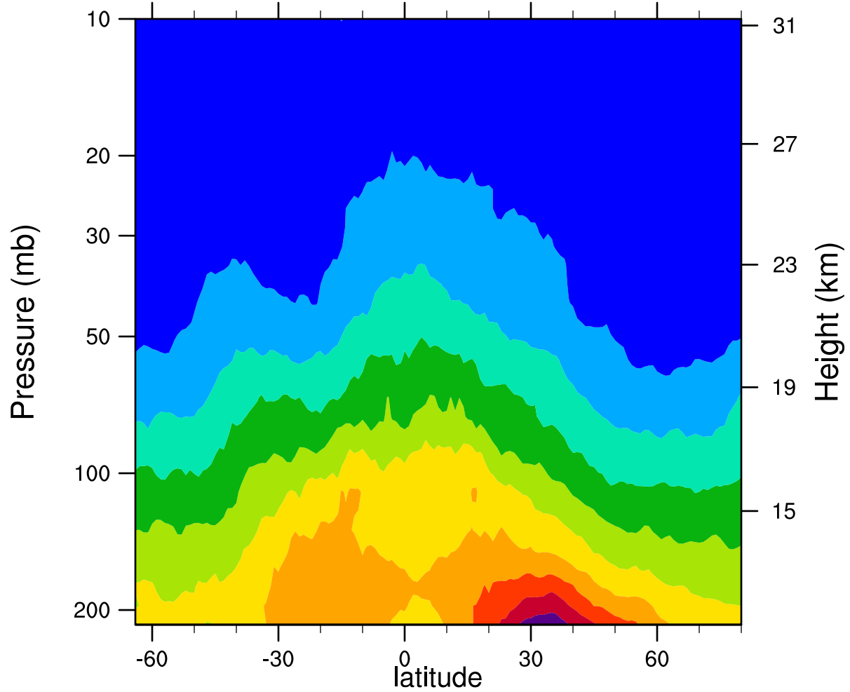
2007d132 12.1MicronExtinction_Combined (km -1 )
