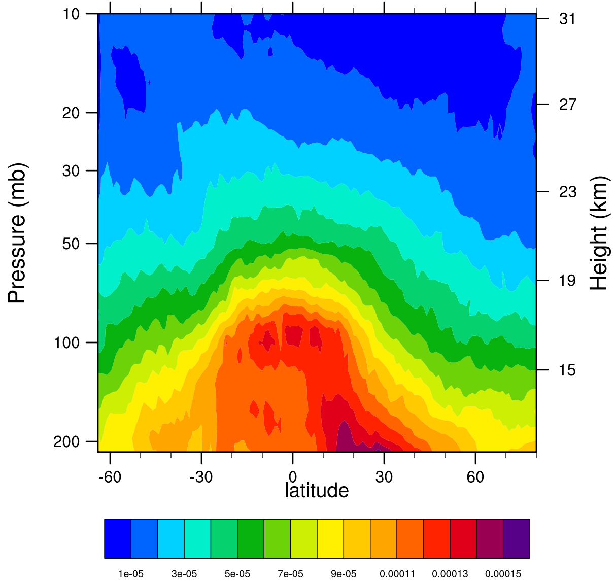
2006d092 12.1MicronExtinction_Combined (km -1 )
