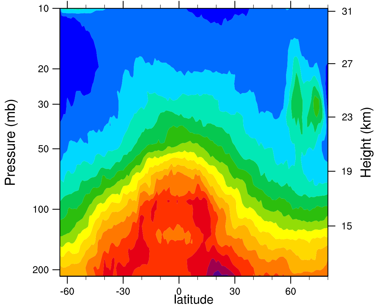
2006d007 12.1MicronExtinction_Combined ( \text{km}^{-1} )
