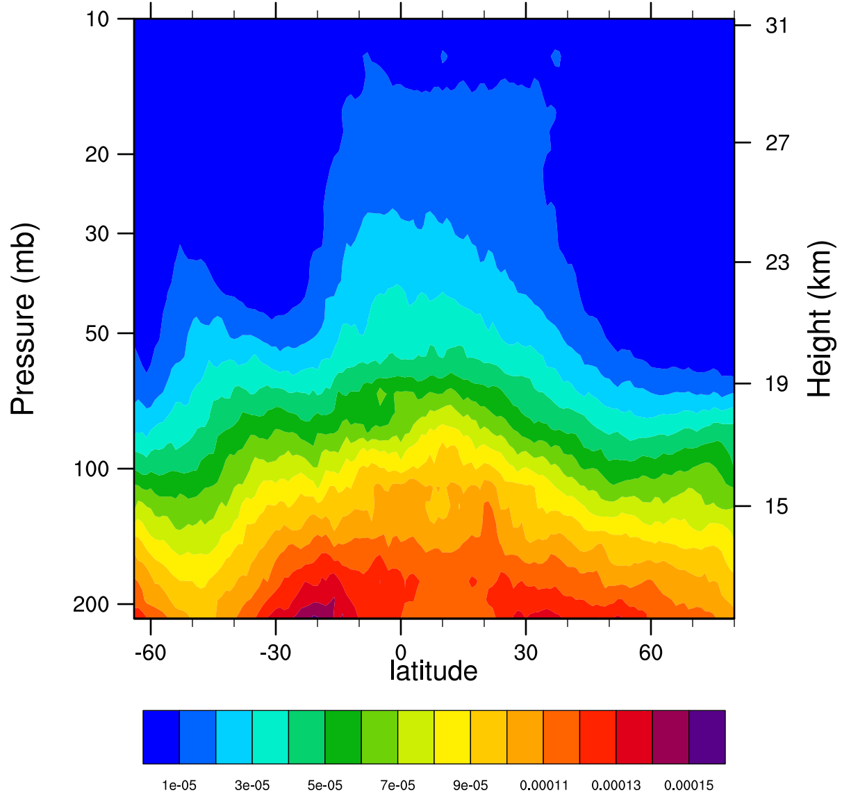
2007d272 12.1MicronExtinction_Combined (km -1 )
