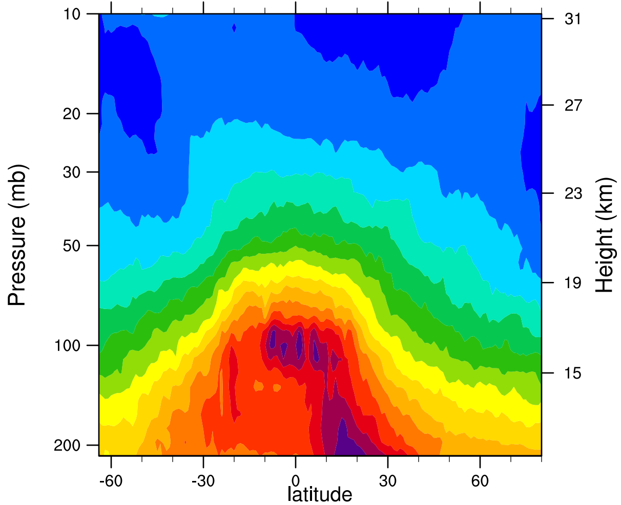
2006d070 12.1MicronExtinction_Combined (km -1 )
