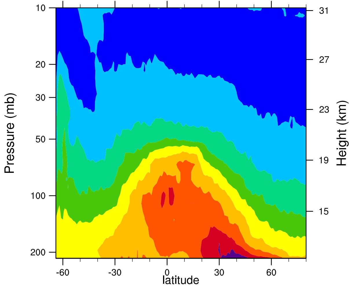
2006d189 12.1MicronExtinction_Combined (km -1 )
