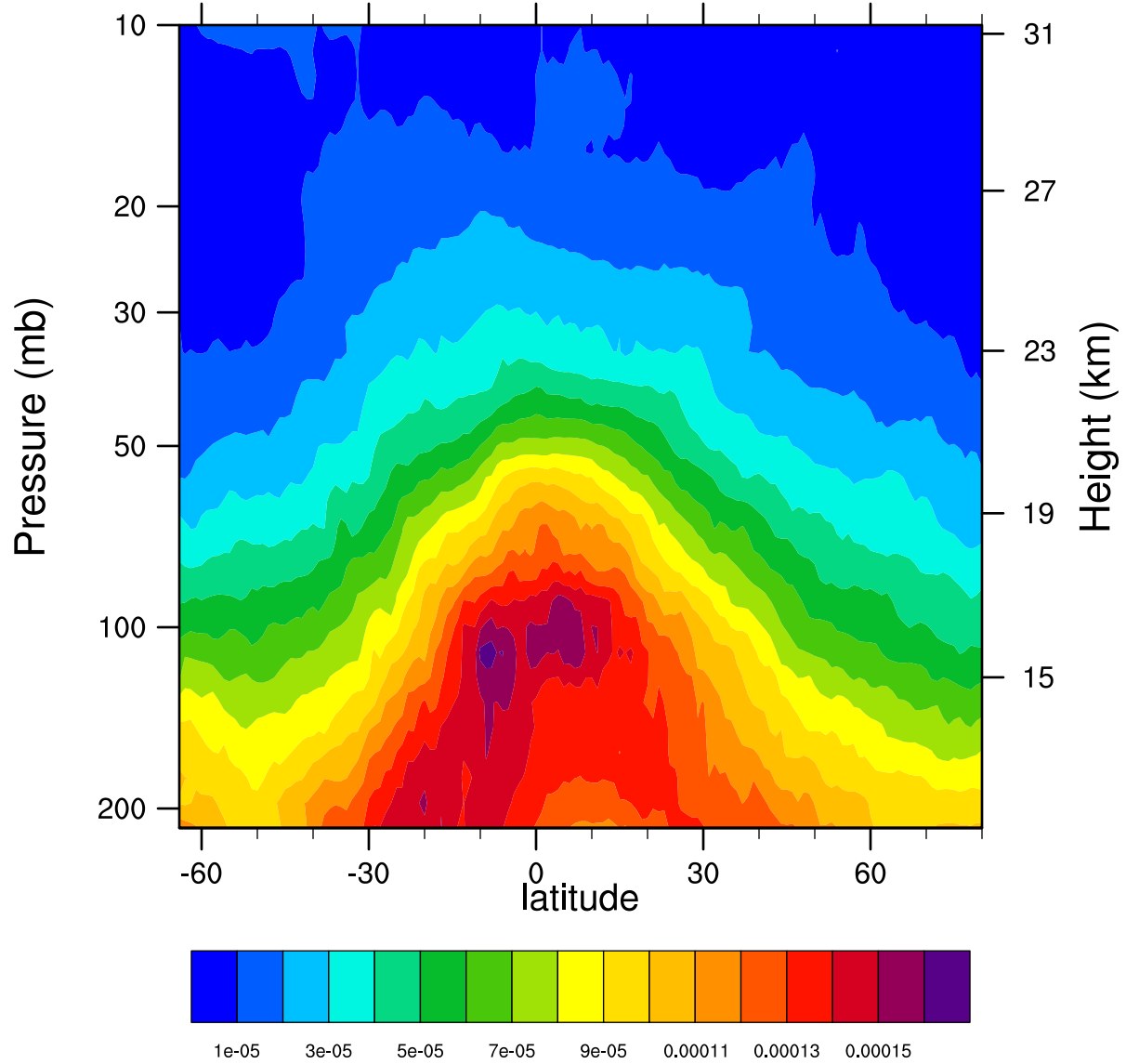
2006d292 12.1MicronExtinction_Combined ( \text{km}^{-1} )
