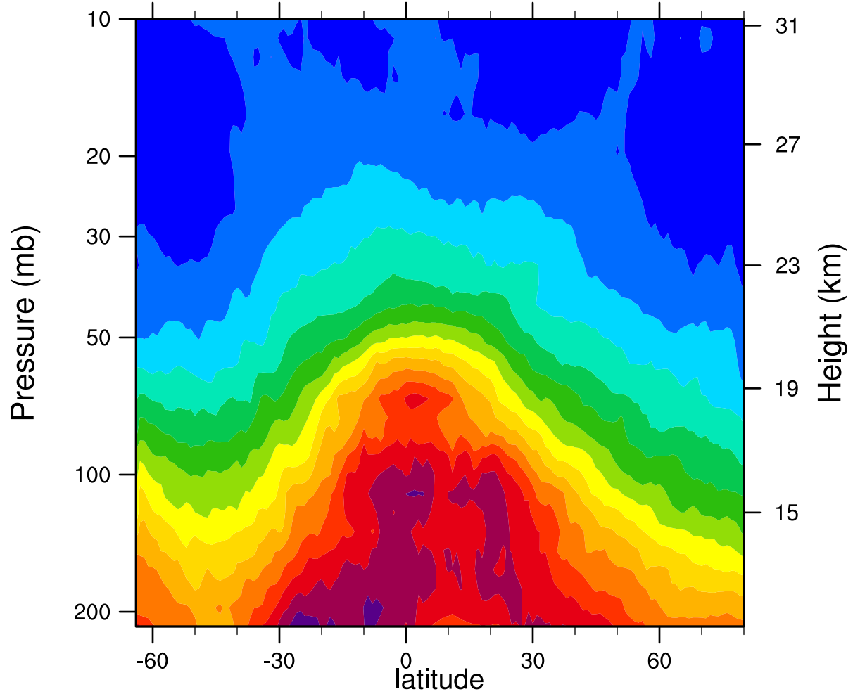
2006d277 12.1MicronExtinction_Combined (km -1 )
