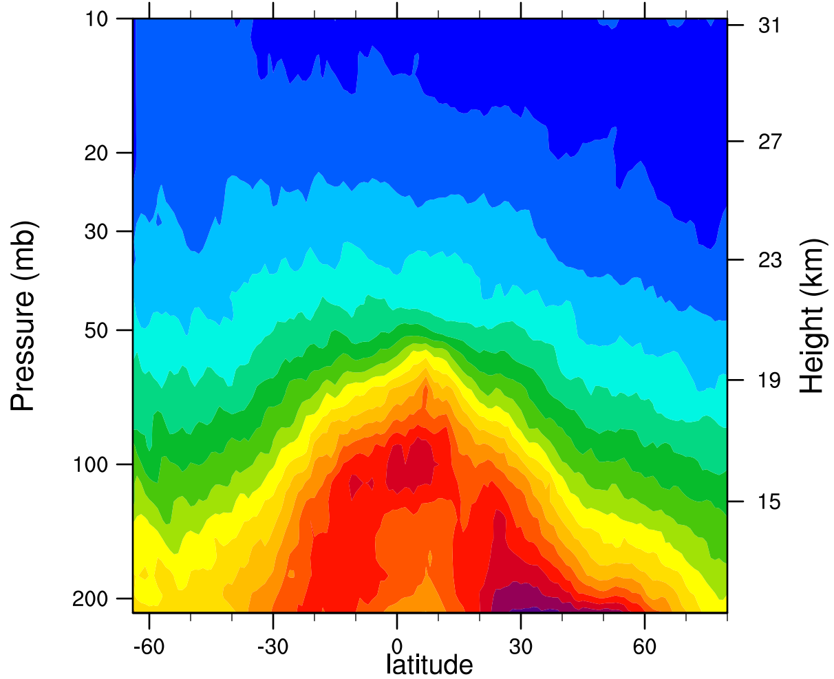
2006d162 12.1MicronExtinction_Combined ( \text{km}^{-1} )
