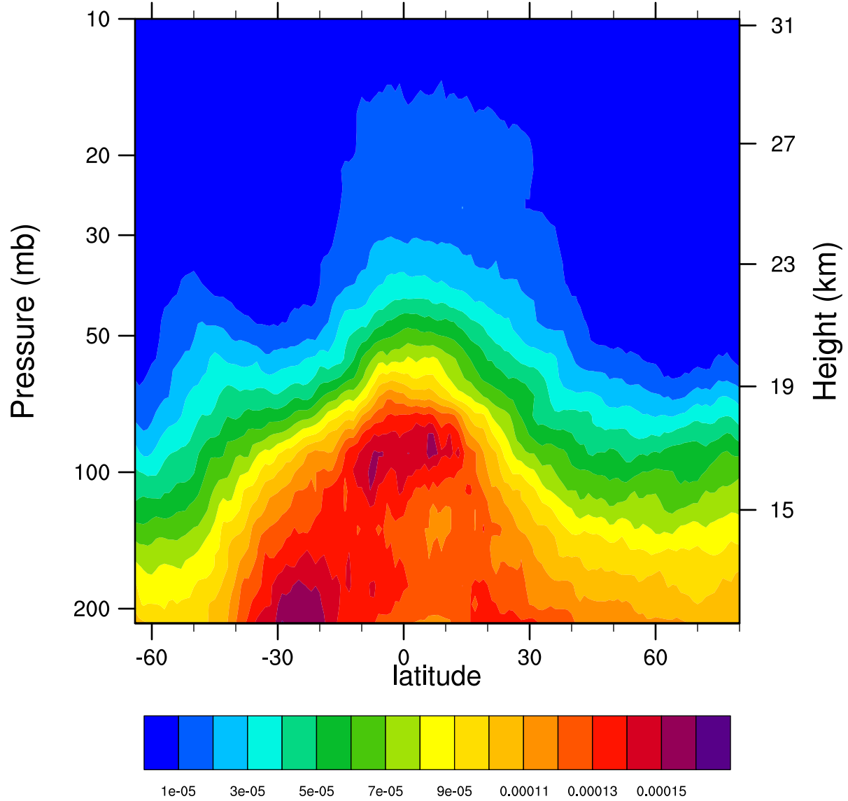
2006d323 12.1MicronExtinction_Combined ( \text{km}^{-1} )
