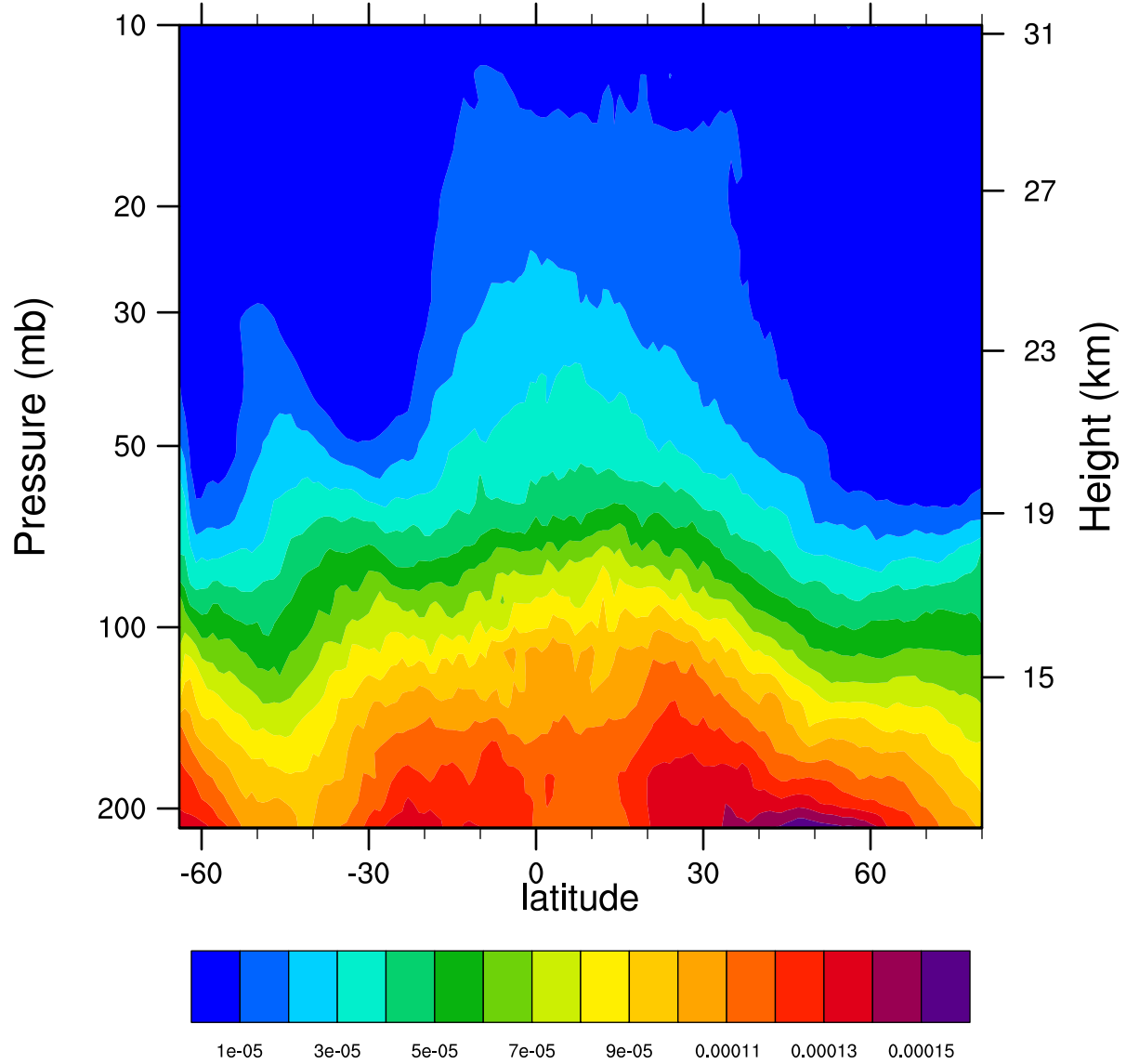
2007d239 12.1MicronExtinction_Combined (km -1 )
