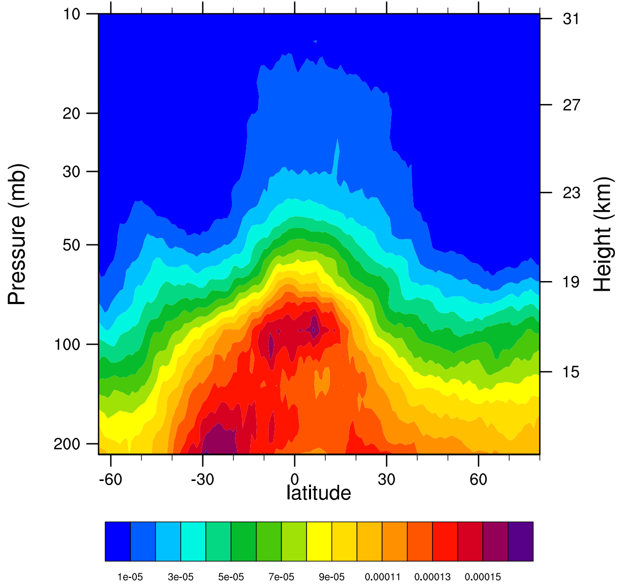
2006d322 12.1MicronExtinction_Combined (km -1 )
