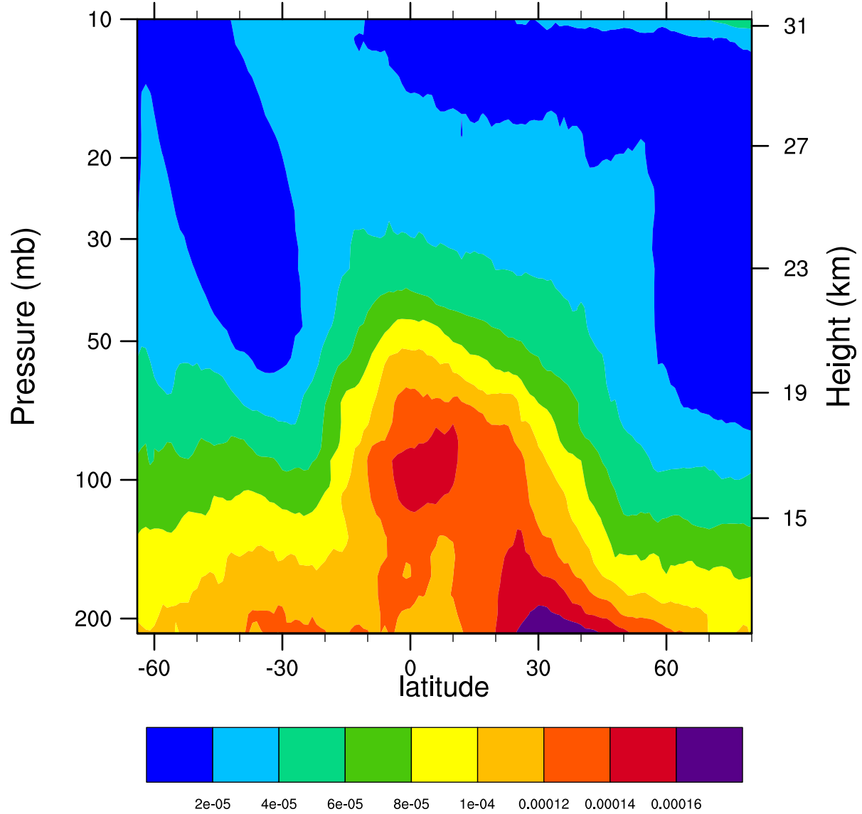
2005d157 12.1MicronExtinction_Combined (km -1 )
