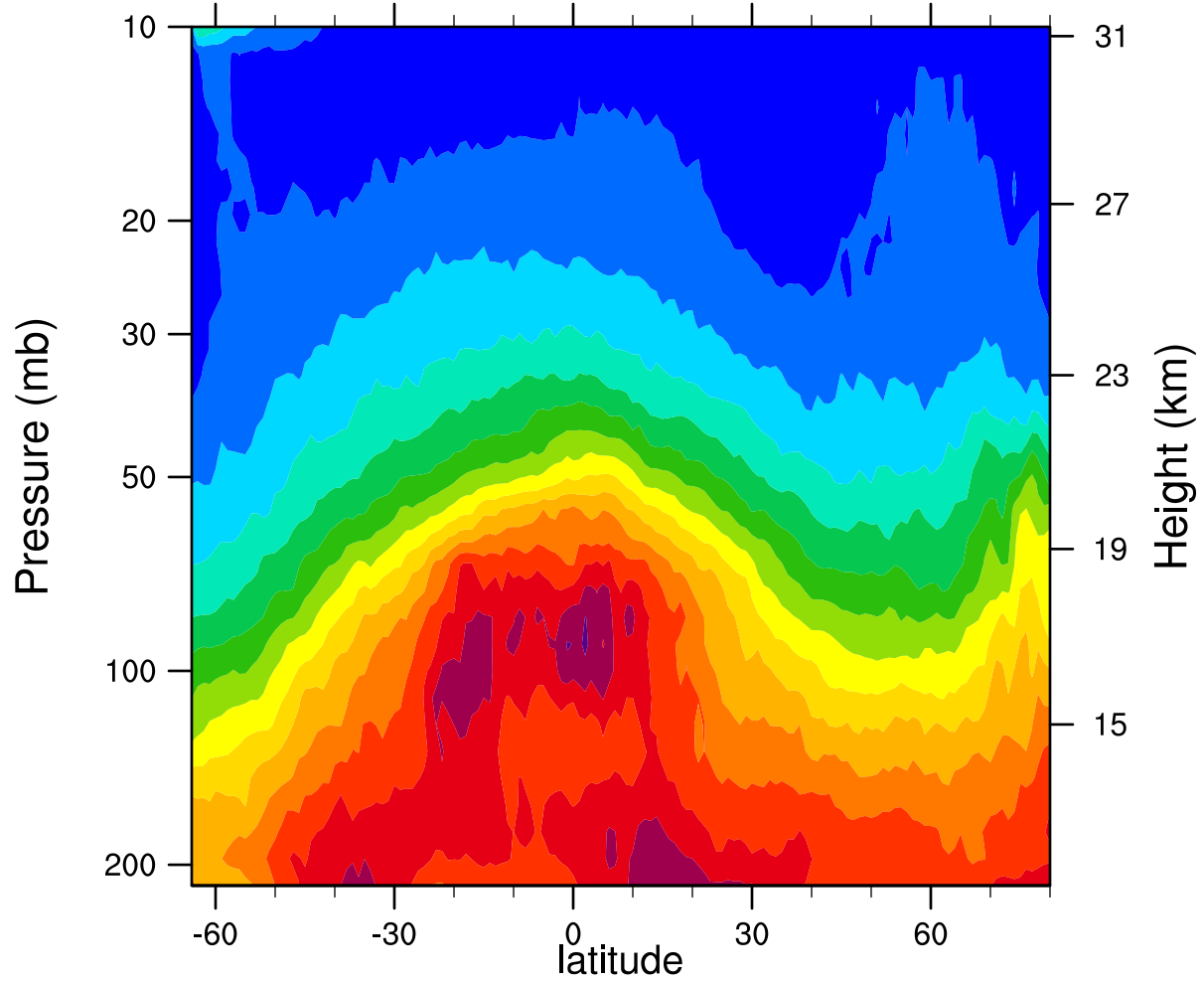
2007d032 12.1MicronExtinction_Combined (km -1 )
