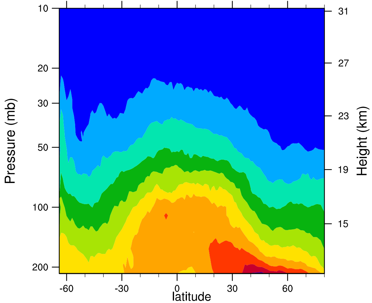
2007d184 12.1MicronExtinction_Combined (km -1 )
