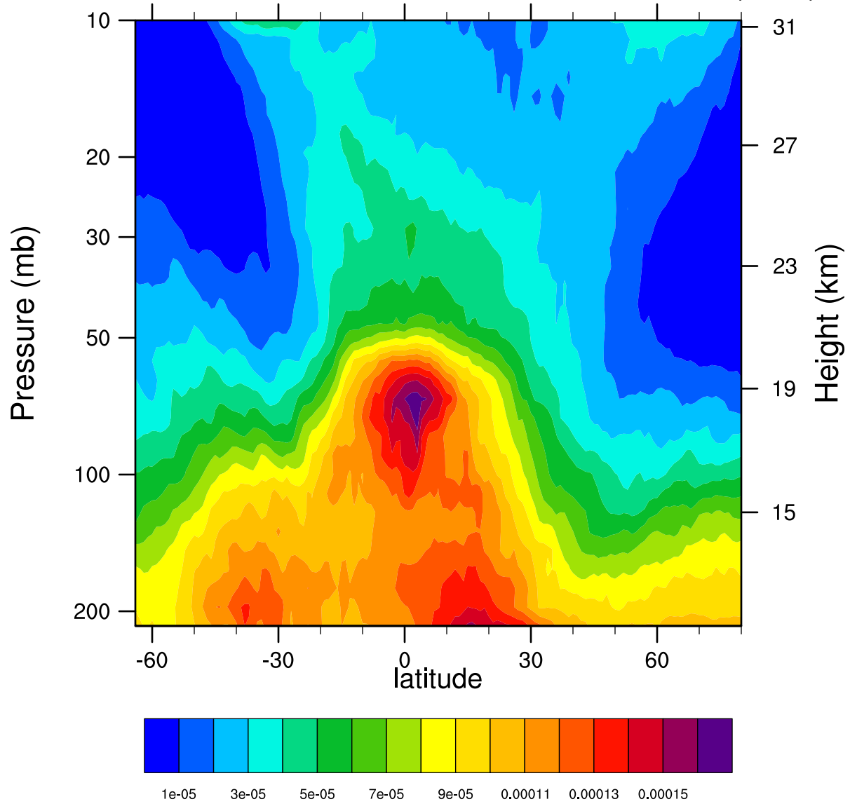
2005d064 12.1MicronExtinction_Combined (km -1 )
