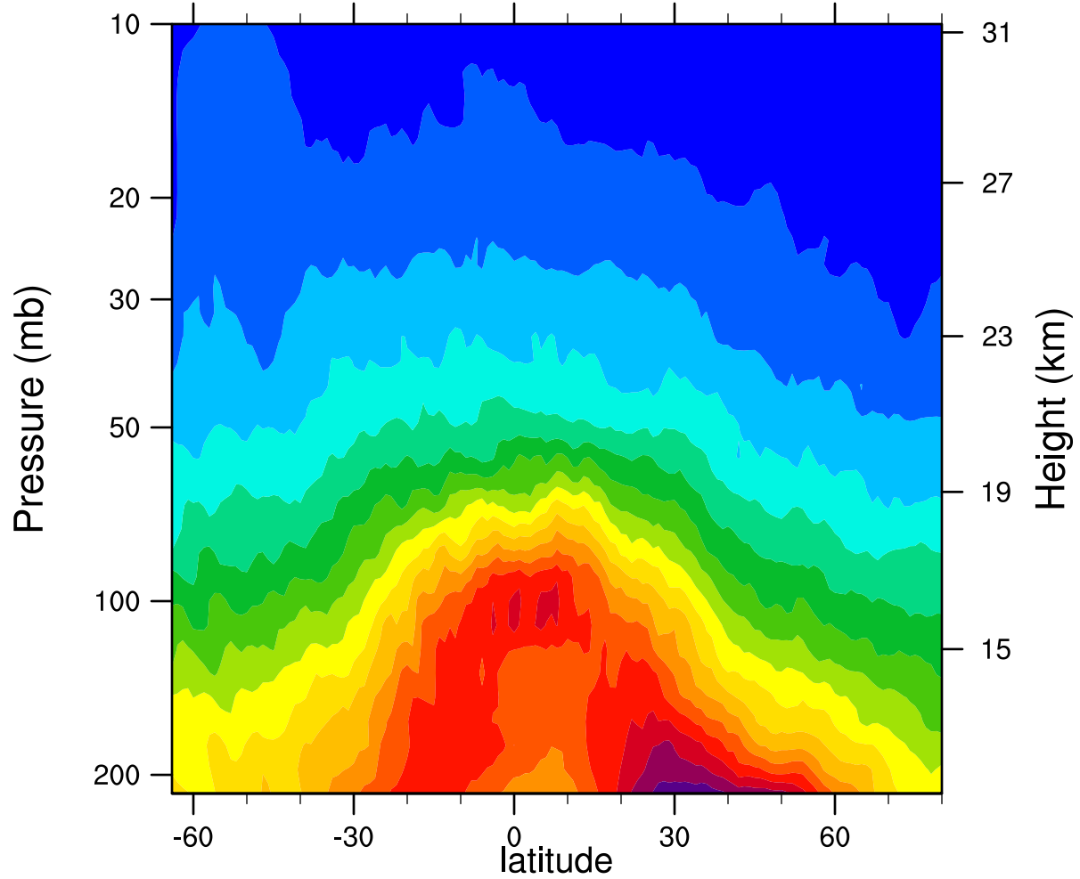
2006d154 12.1MicronExtinction_Combined (km -1 )
