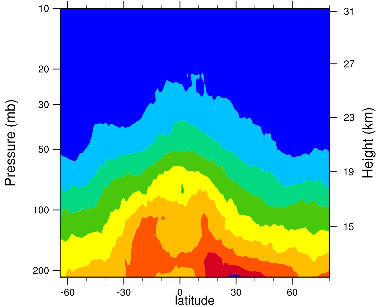
2007d107 12.1MicronExtinction_Combined (km -1 )
