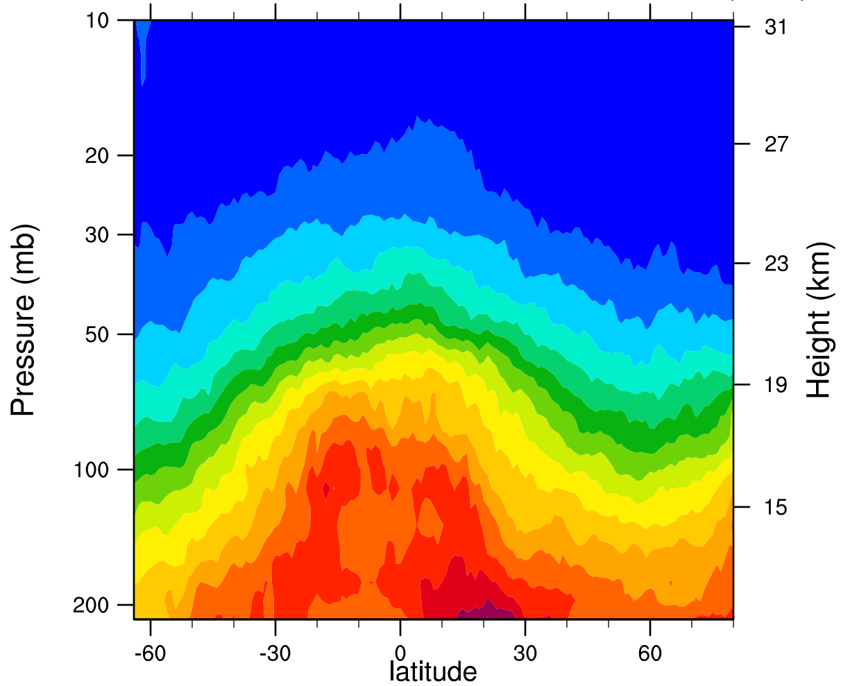
2007d050 12.1MicronExtinction_Combined (km -1 )
