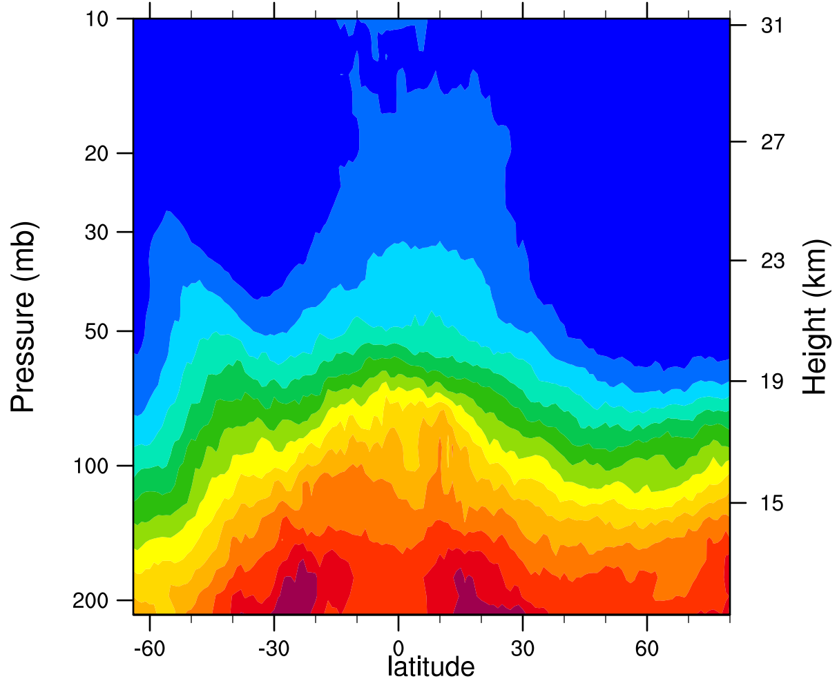
2007d337 12.1MicronExtinction_Combined (km -1 )
