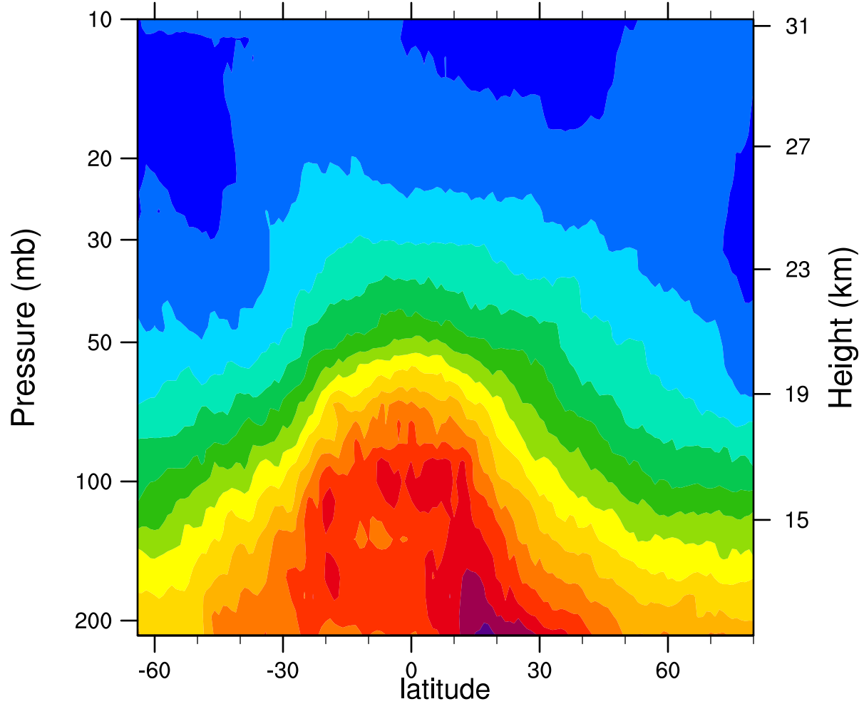
2006d061 12.1MicronExtinction_Combined (km -1 )
