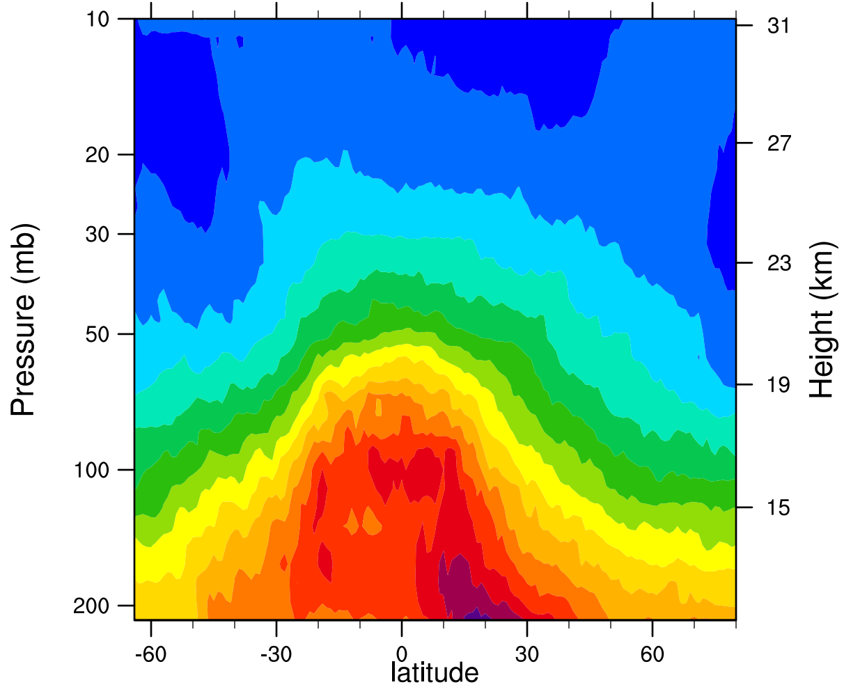
2006d062 12.1MicronExtinction_Combined (km -1 )
