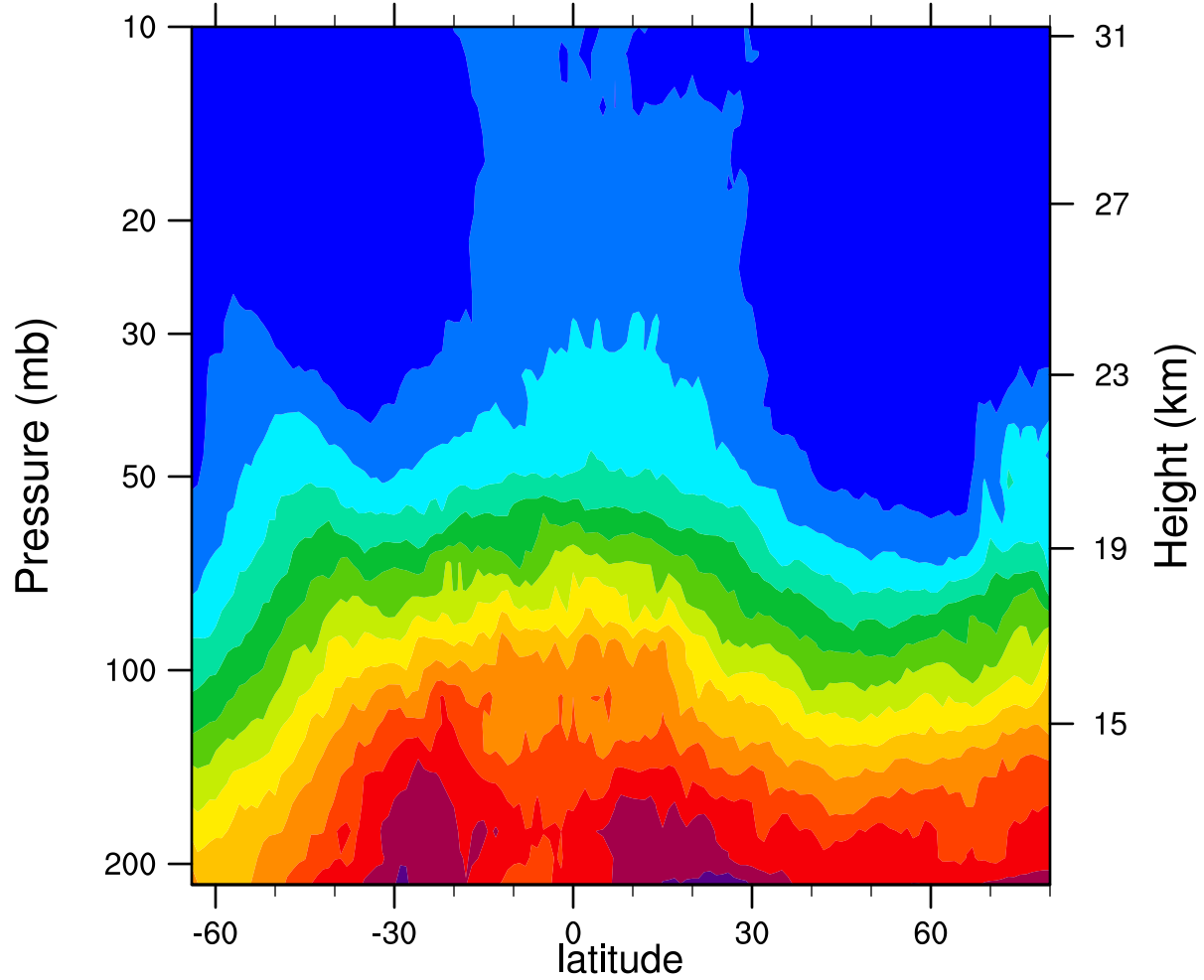
2007d357 12.1MicronExtinction_Combined ( \text{km}^{-1} )
