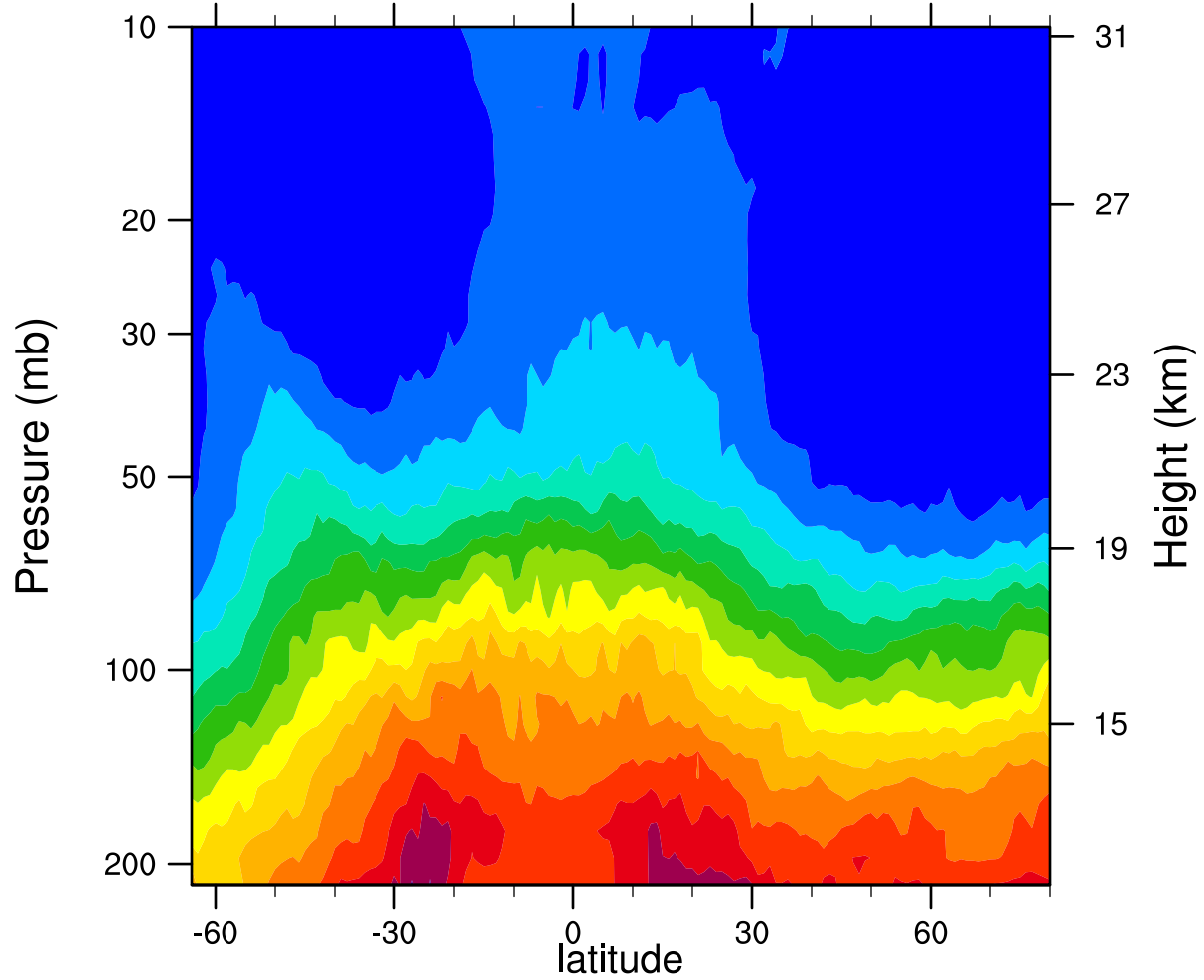
2007d347 12.1MicronExtinction_Combined (km -1 )
