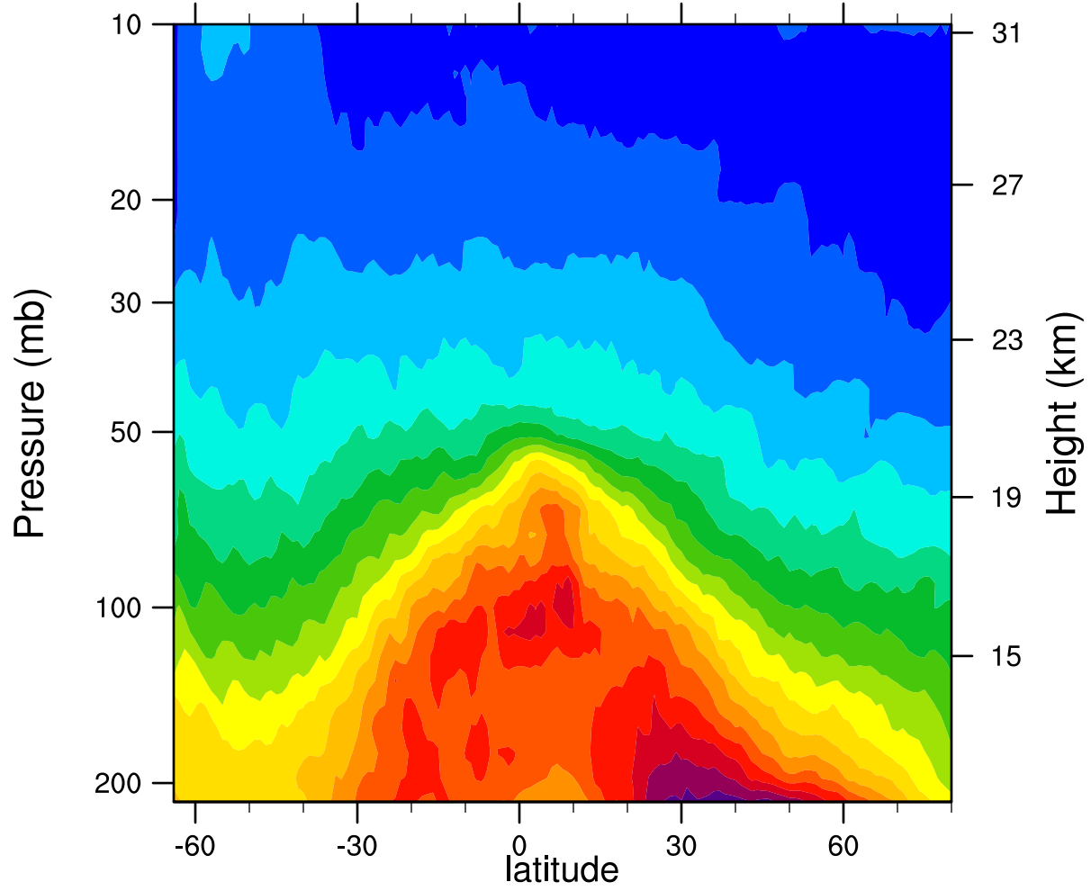
2006d168 12.1MicronExtinction_Combined (km -1 )
