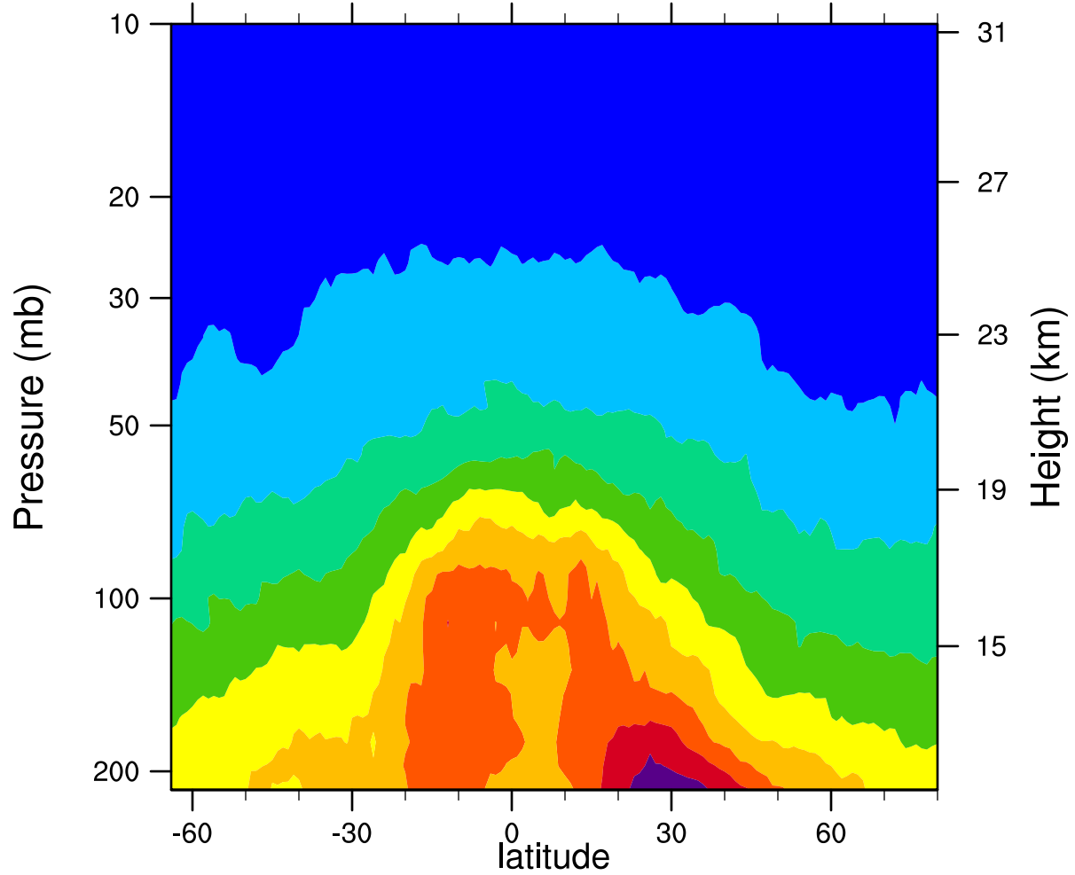
2006d130 12.1MicronExtinction_Combined ( \text{km}^{-1} )
