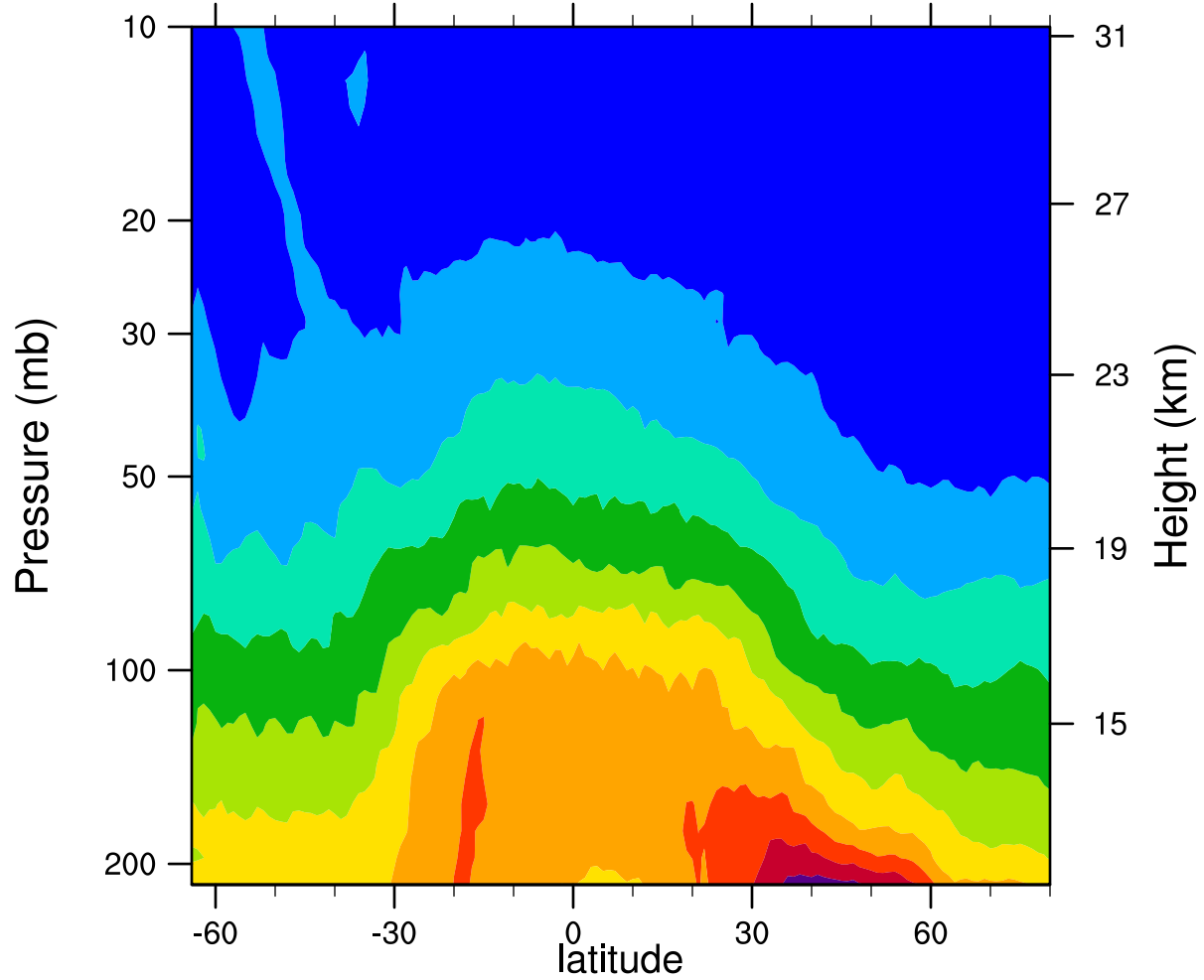
2007d167 12.1MicronExtinction_Combined (km -1 )
