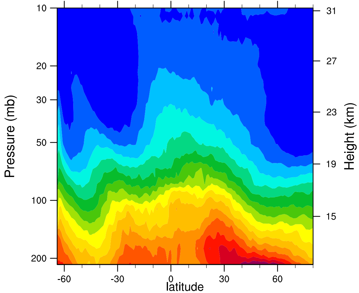
2007d225 12.1MicronExtinction_Combined (km -1 )
