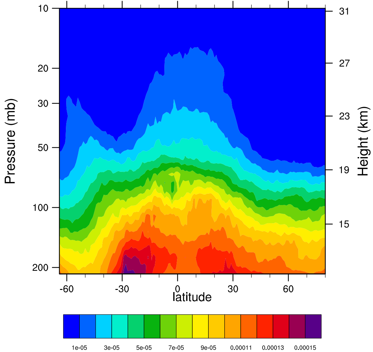
2007d314 12.1MicronExtinction_Combined (km -1 )
