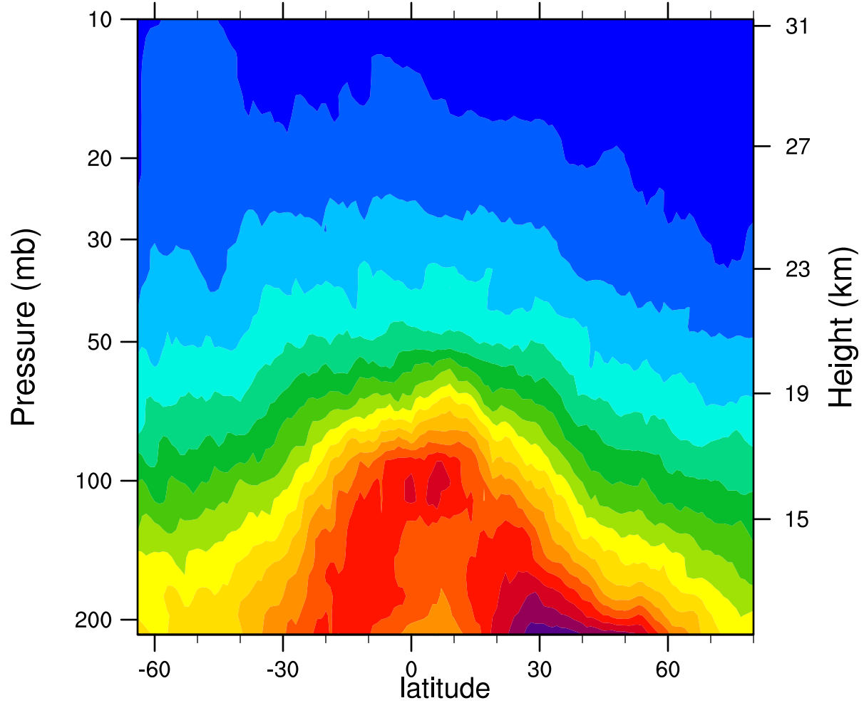
2006d156 12.1MicronExtinction_Combined (km -1 )
