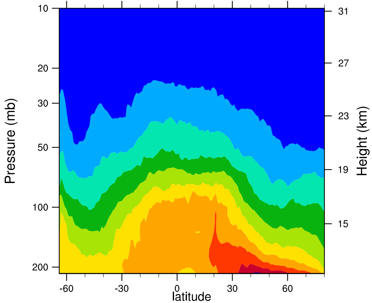
2007d188 12.1MicronExtinction_Combined (km -1 )
