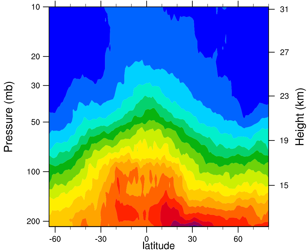
2007d089 12.1MicronExtinction_Combined (km -1 )
