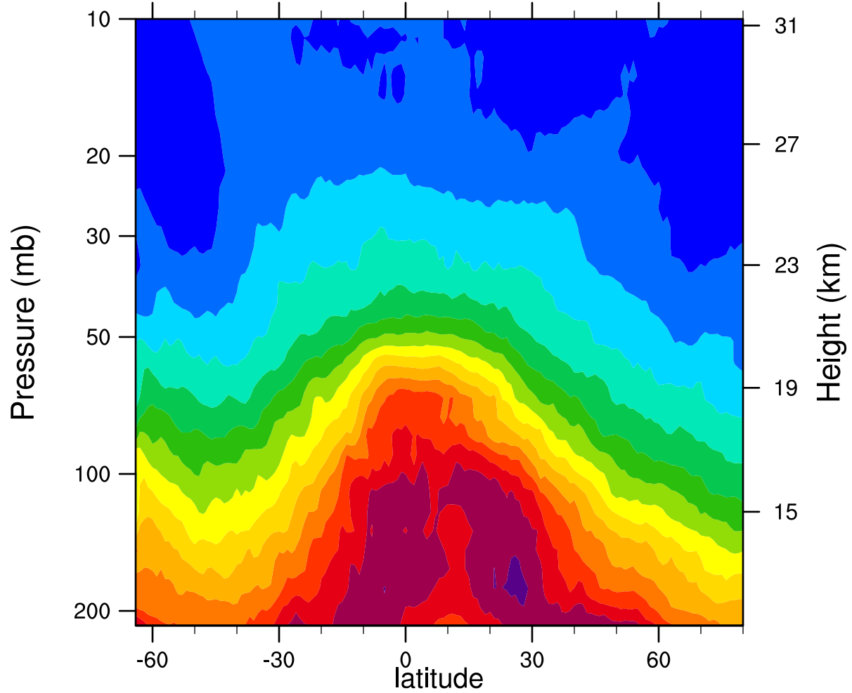
2006d254 12.1MicronExtinction_Combined (km -1 )
