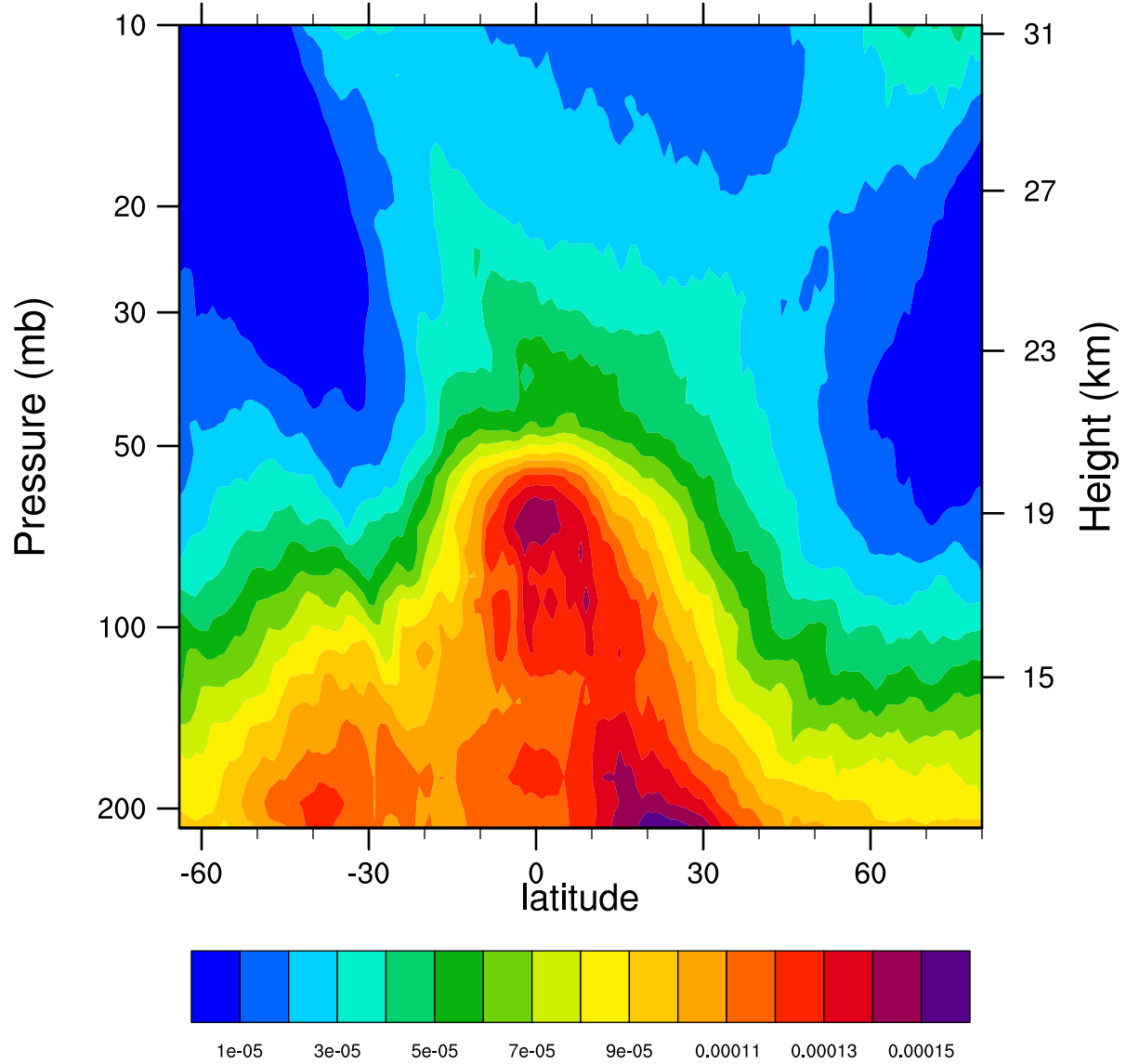
2005d085 12.1MicronExtinction_Combined (km -1 )
