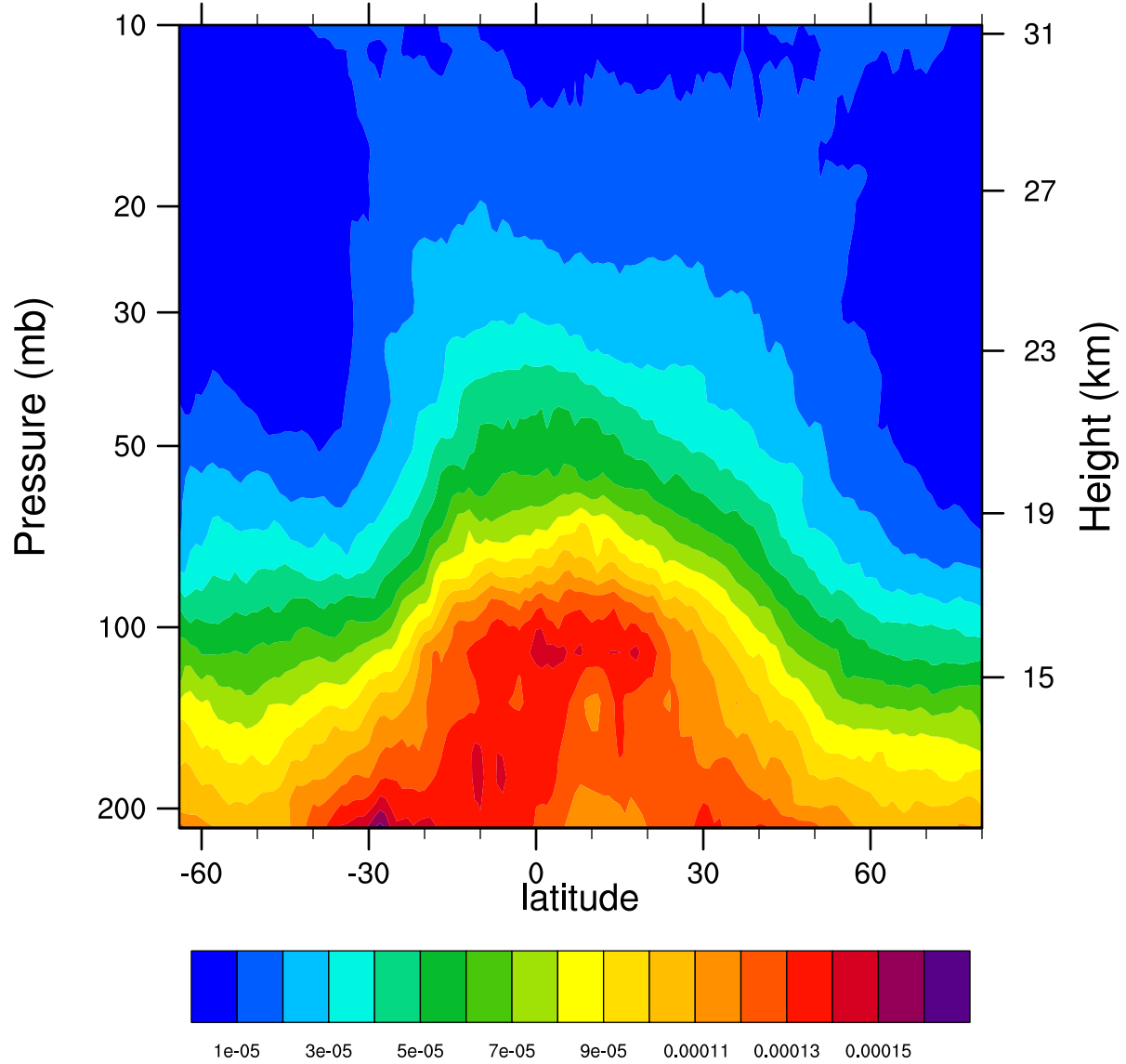
2005d273 12.1MicronExtinction_Combined ( \text{km}^{-1} )
