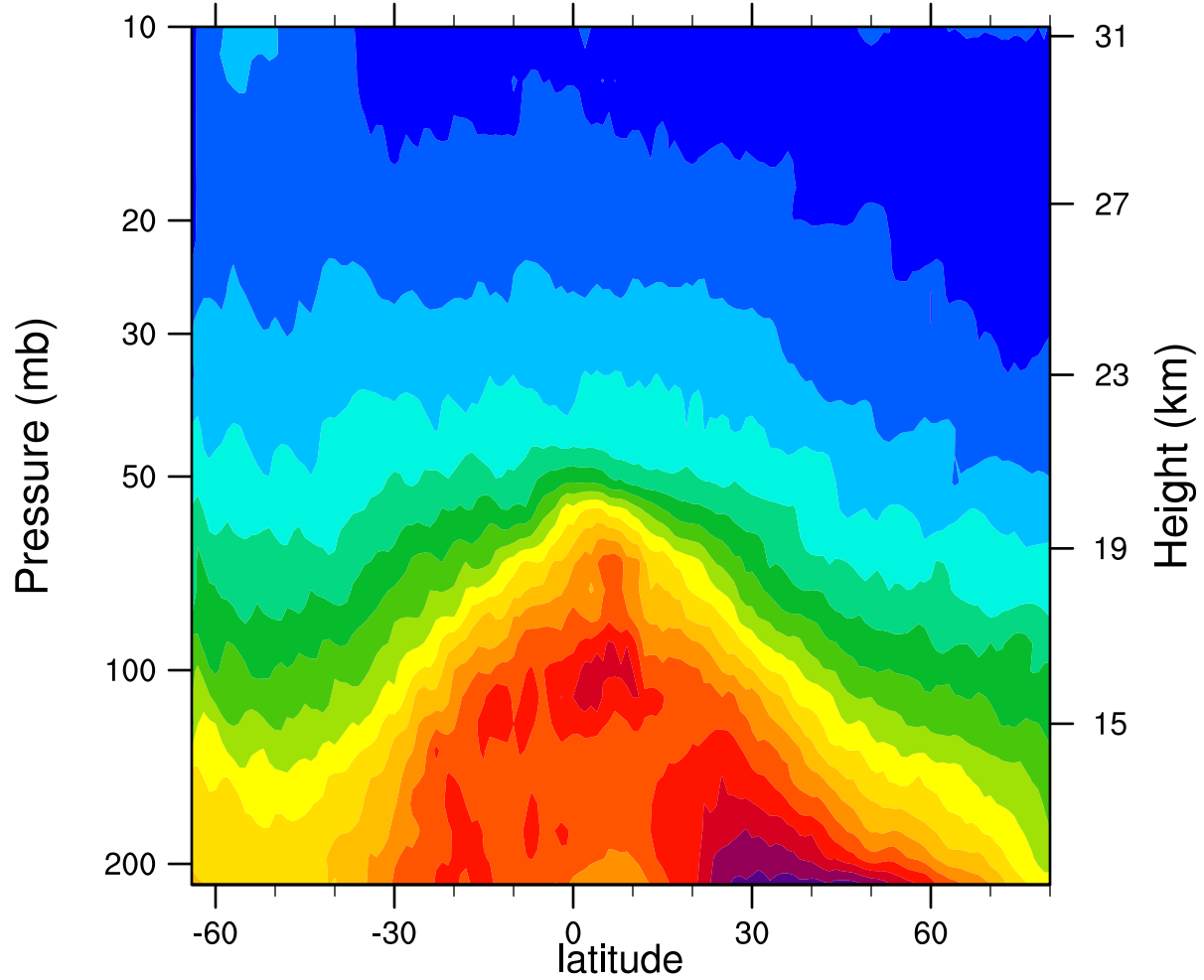
2006d169 12.1MicronExtinction_Combined (km -1 )
