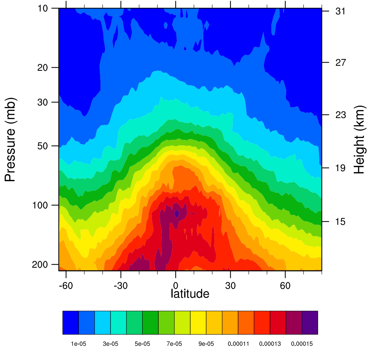
2006d284 12.1MicronExtinction_Combined (km -1 )
