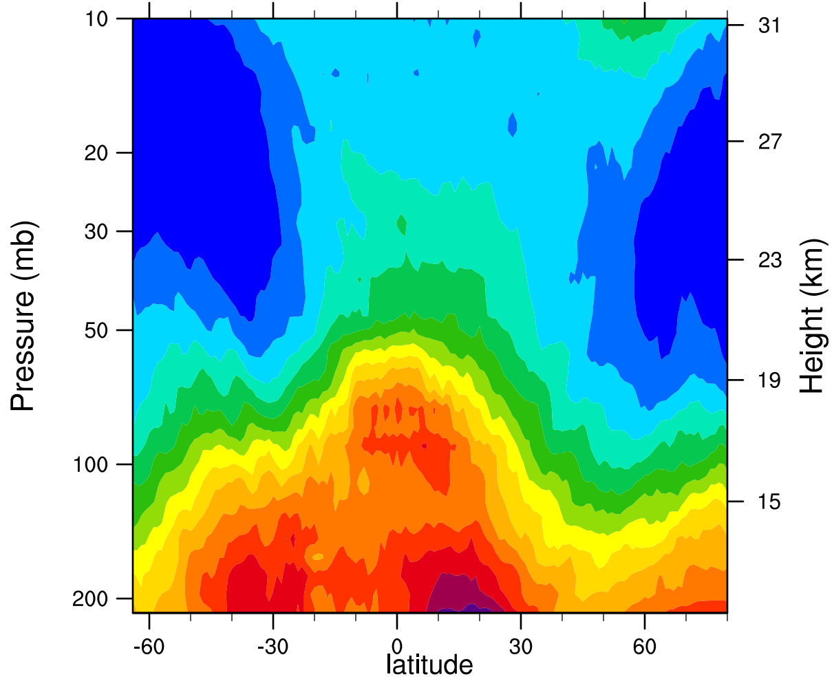
2005d036 12.1MicronExtinction_Combined (km -1 )
