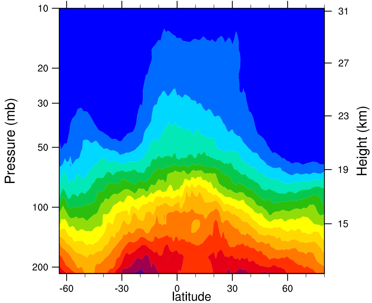
2007d269 12.1MicronExtinction_Combined (km -1 )
