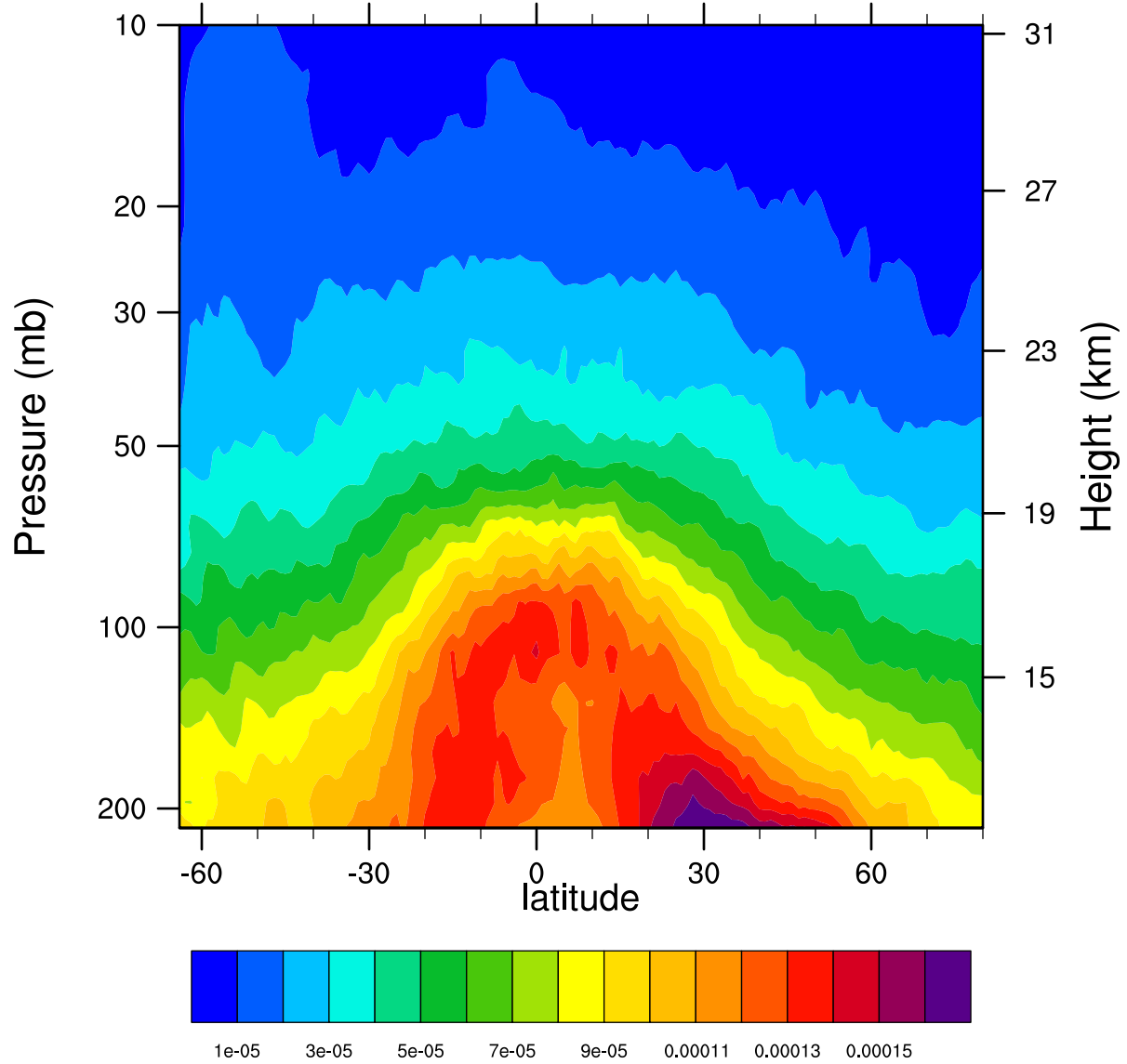
2006d147 12.1MicronExtinction_Combined (km -1 )
