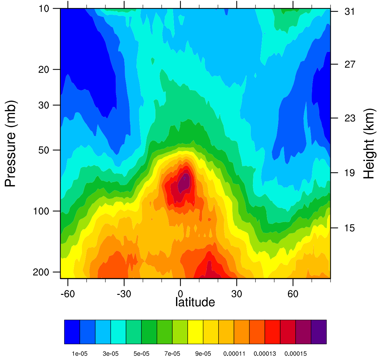
2005d050 12.1MicronExtinction_Combined (km -1 )
