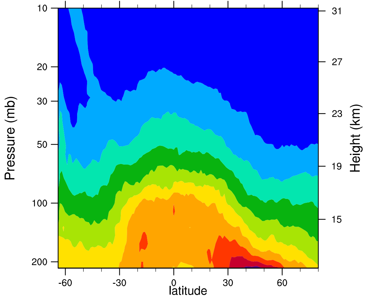
2007d171 12.1MicronExtinction_Combined (km -1 )
