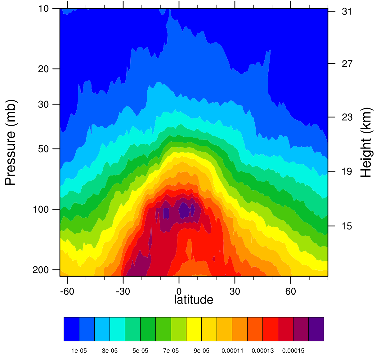
2006d301 12.1MicronExtinction_Combined ( \text{km}^{-1} )
