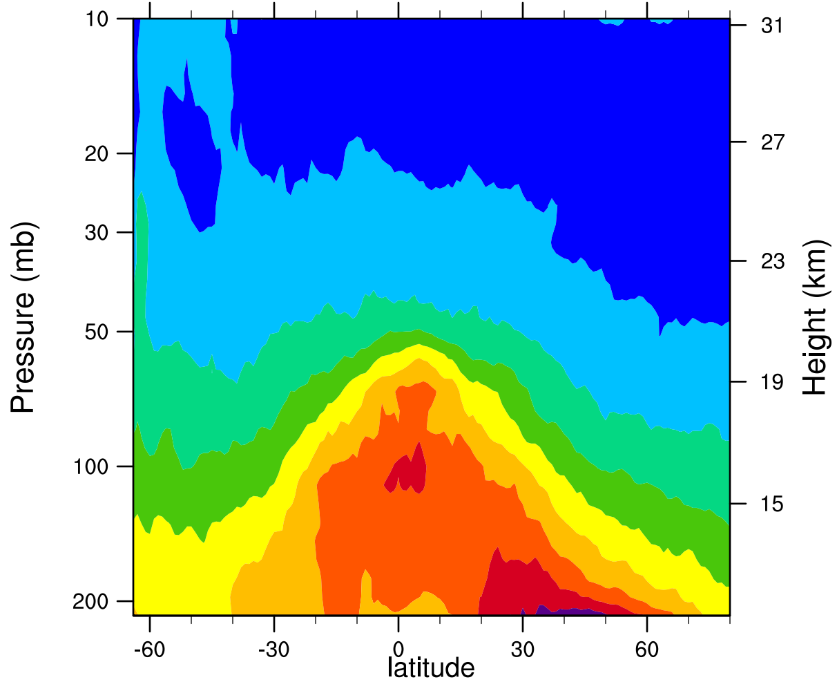
2006d176 12.1MicronExtinction_Combined (km -1 )
