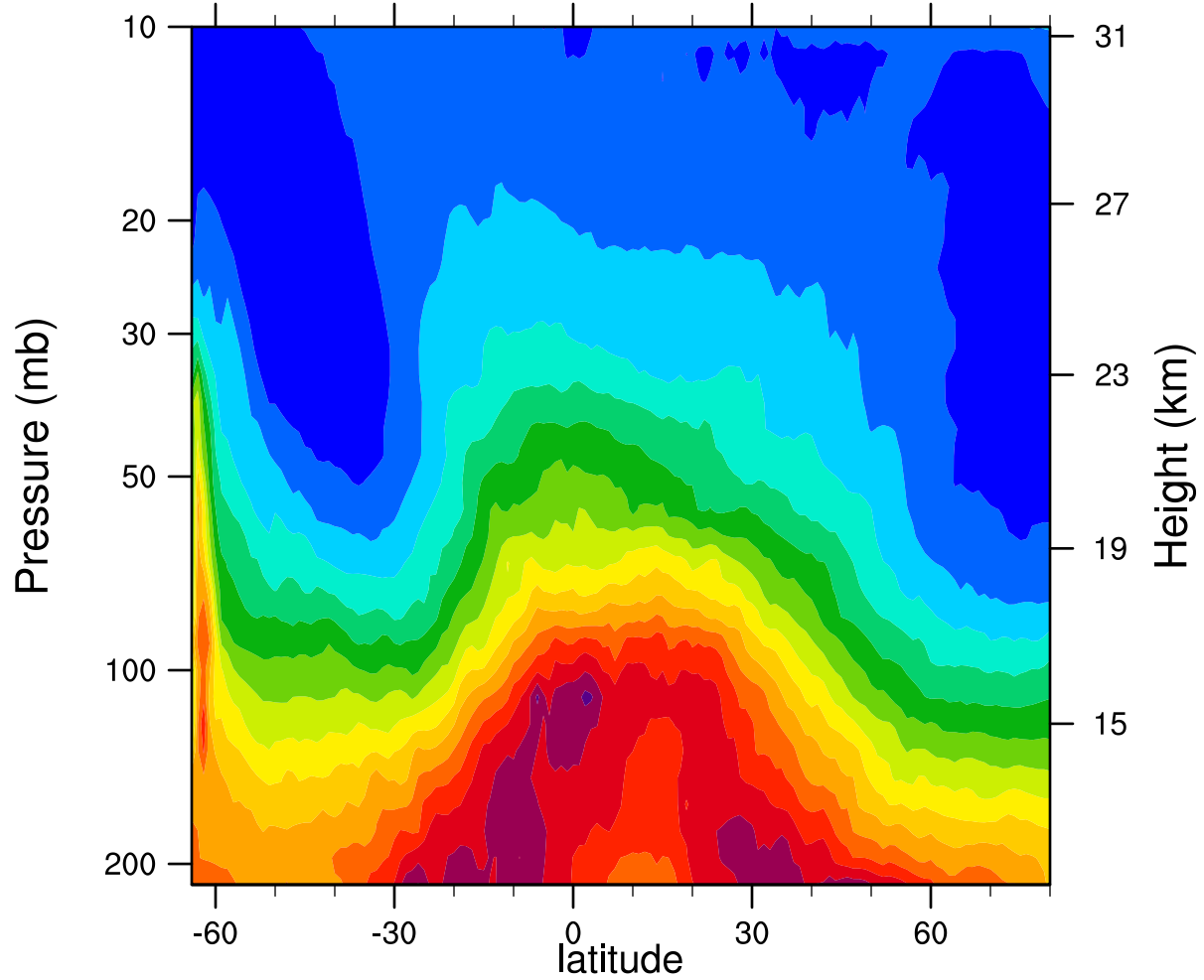
2005d239 12.1MicronExtinction_Combined (km -1 )
