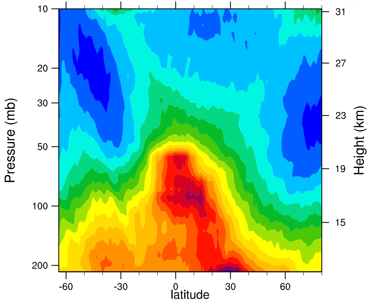
2005d106 12.1MicronExtinction_Combined ( \text{km}^{-1} )
