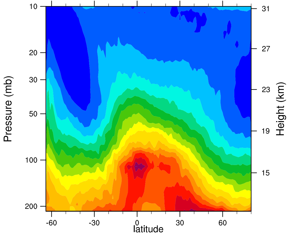
2005d216 12.1MicronExtinction_Combined (km -1 )
