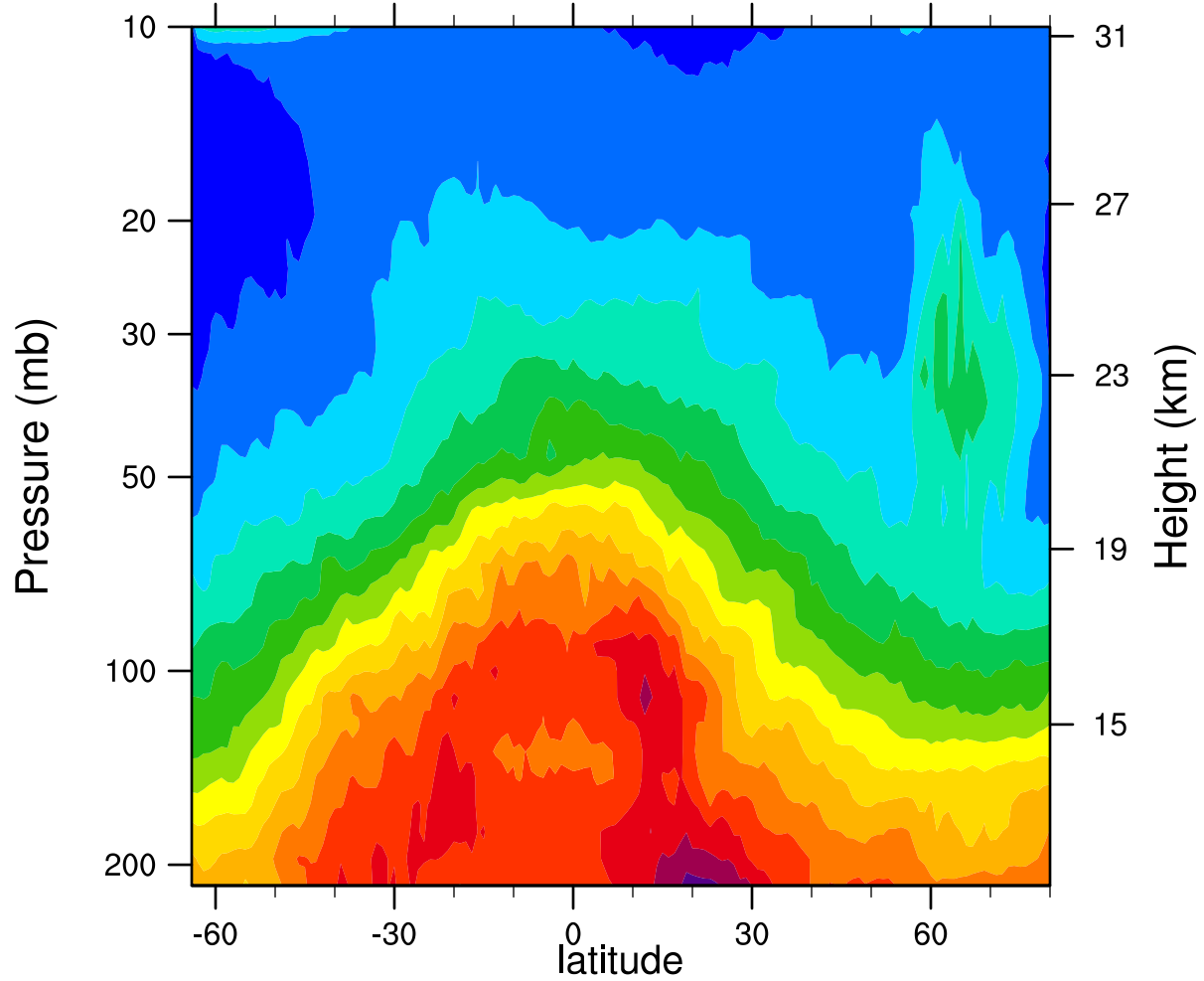
2006d009 12.1MicronExtinction_Combined (km -1 )
