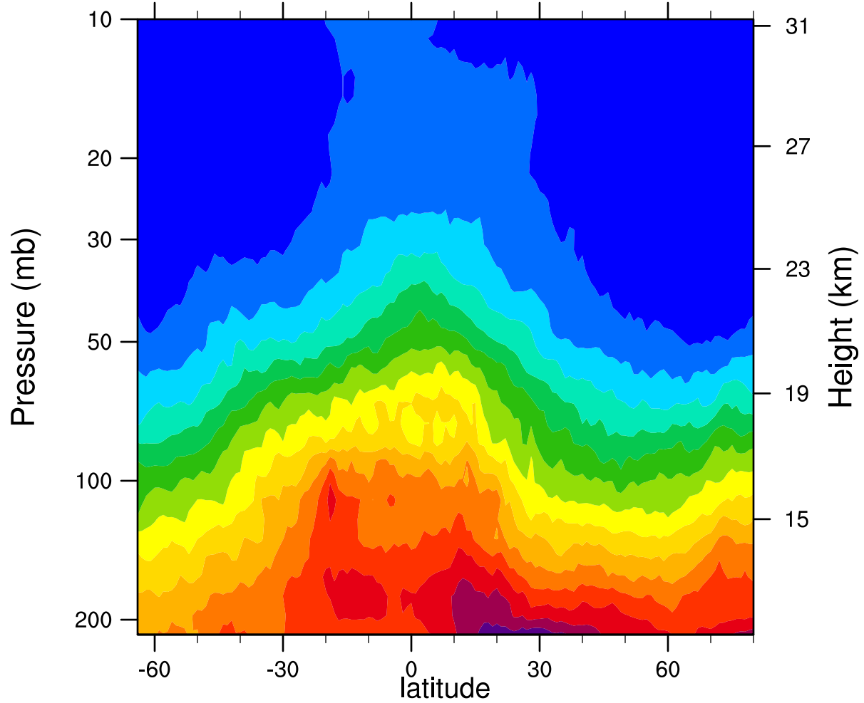
2007d084 12.1MicronExtinction_Combined ( \text{km}^{-1} )
