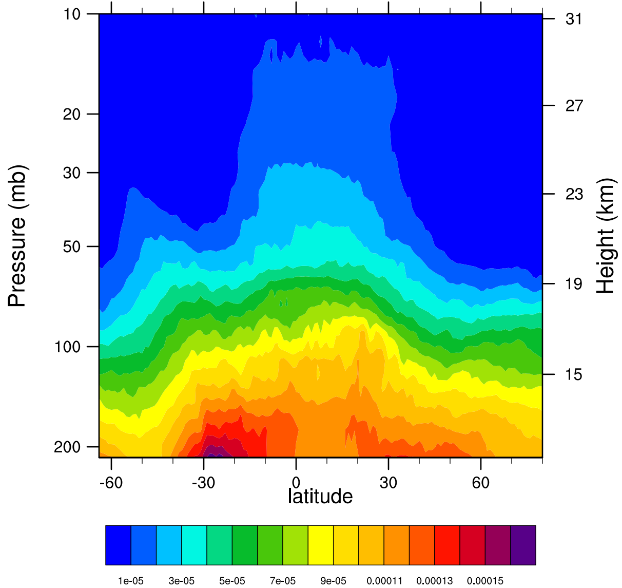
2007d288 12.1MicronExtinction_Combined (km -1 )
