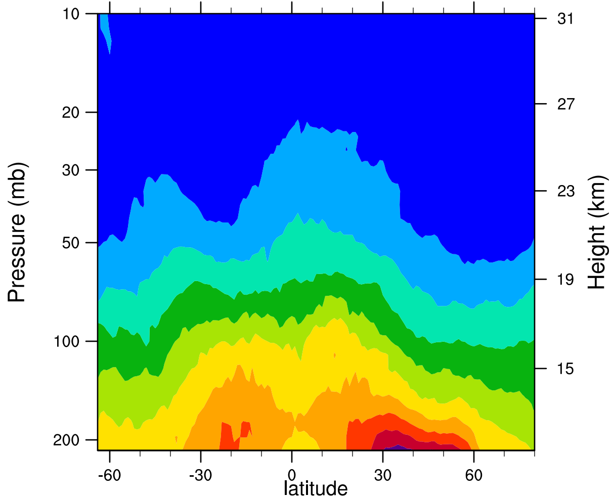
2007d143 12.1MicronExtinction_Combined (km -1 )
