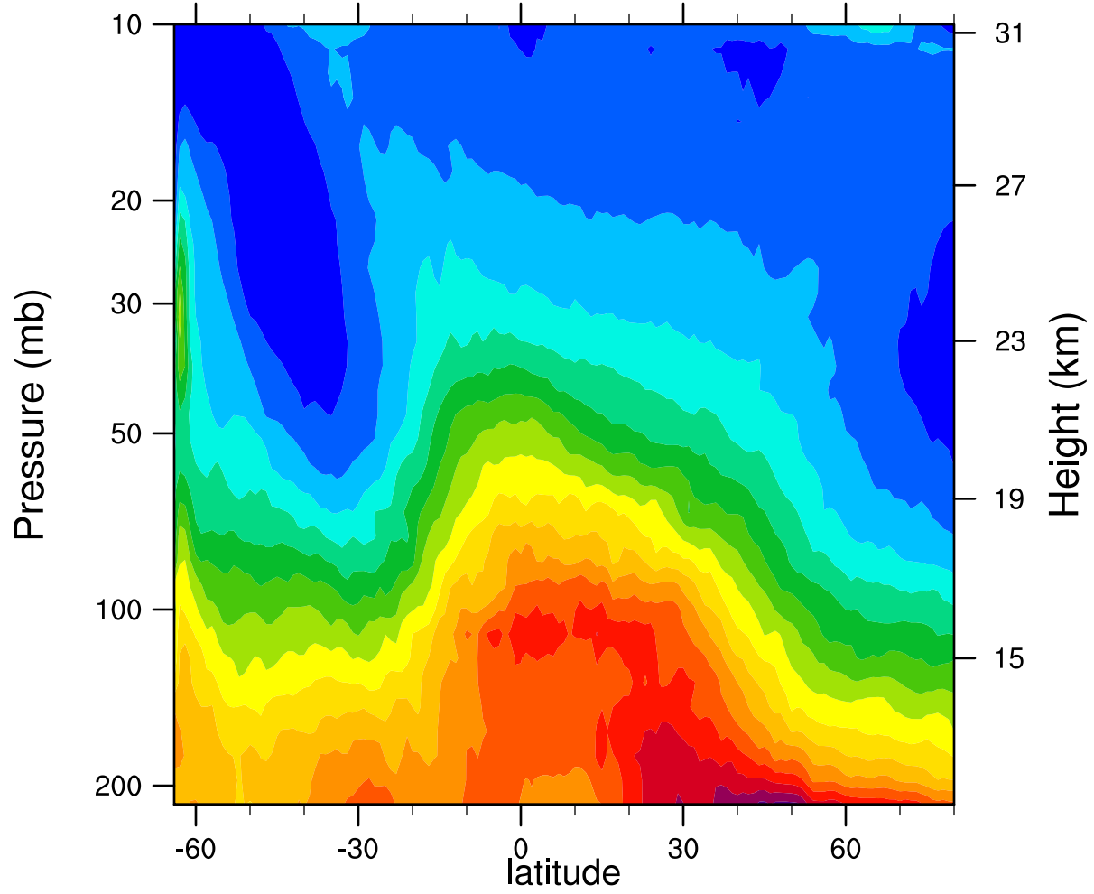
2005d199 12.1MicronExtinction_Combined (km -1 )
