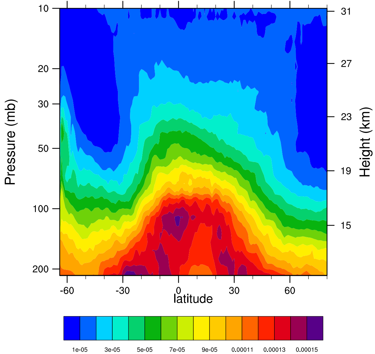
2005d249 12.1MicronExtinction_Combined (km -1 )
