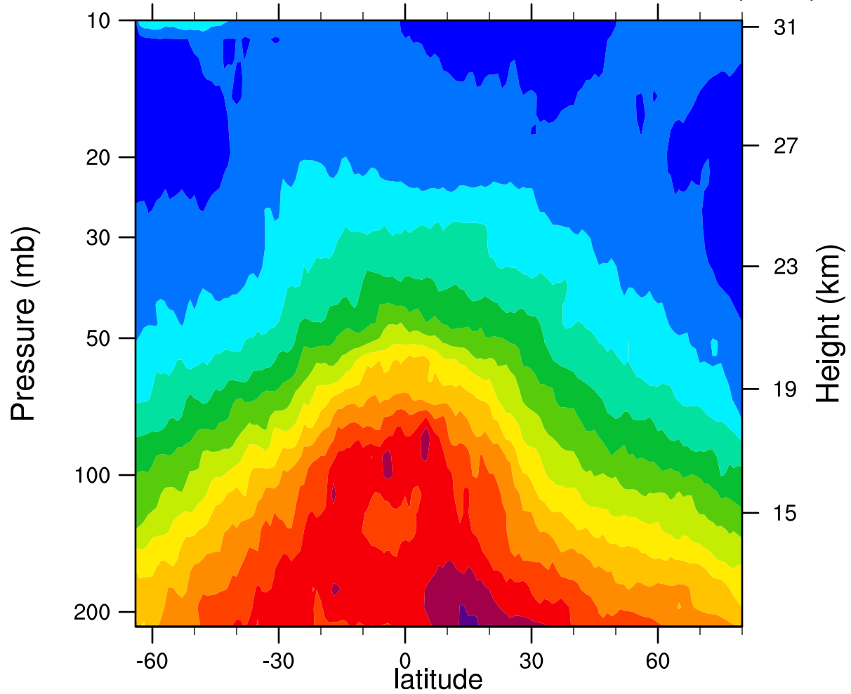
2006d040 12.1MicronExtinction_Combined (km -1 )
