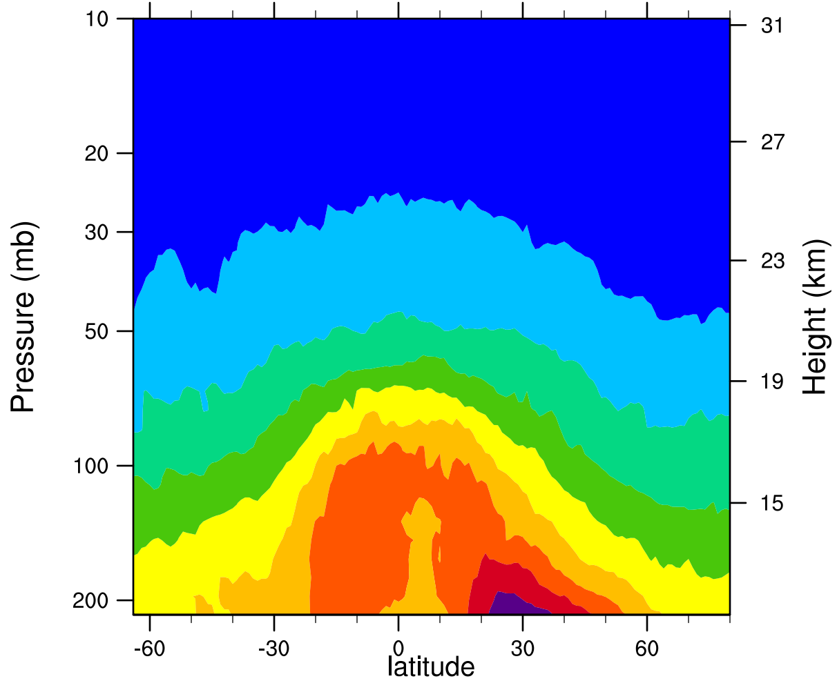
2006d137 12.1MicronExtinction_Combined (km -1 )
