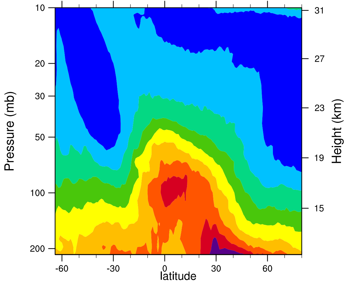
2005d162 12.1MicronExtinction_Combined (km -1 )
