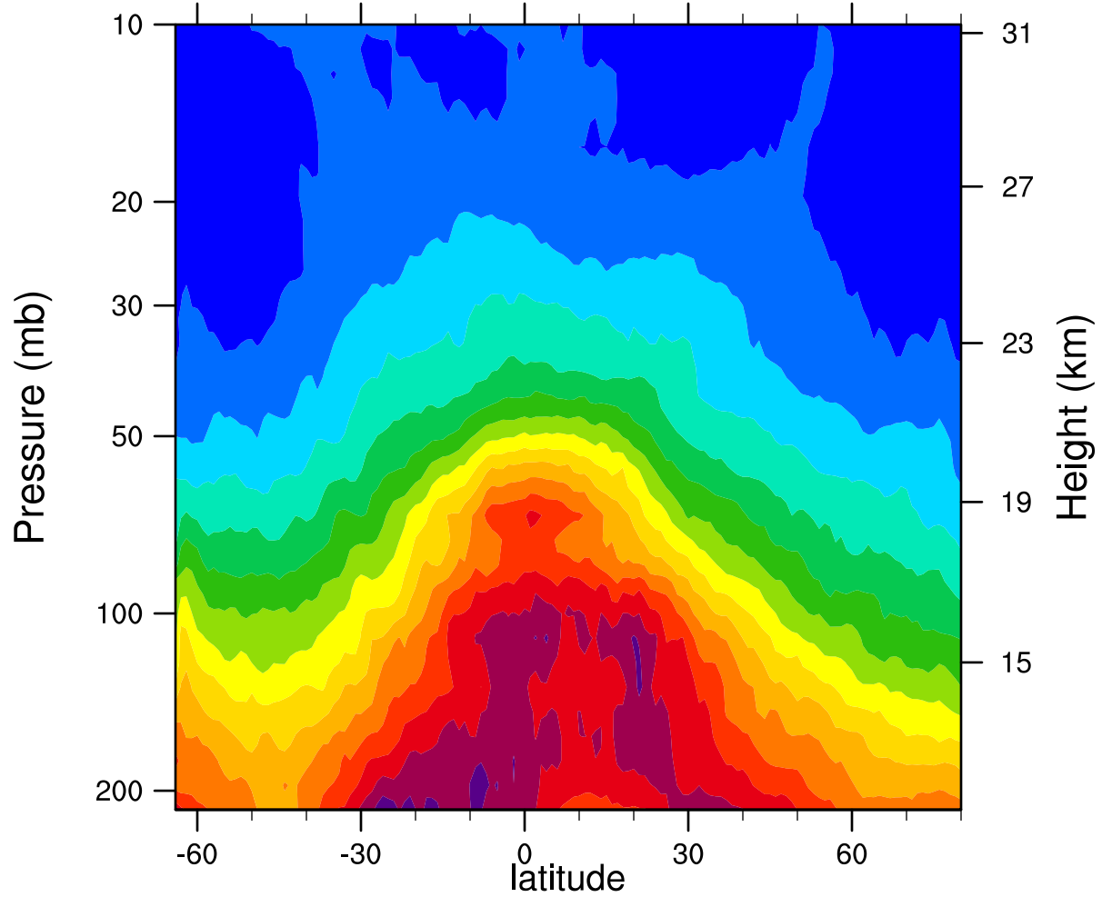
2006d275 12.1MicronExtinction_Combined (km -1 )
