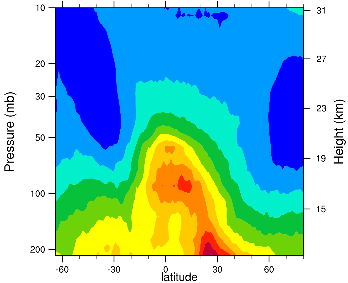
2005d127 12.1MicronExtinction_Combined (km -1 )
