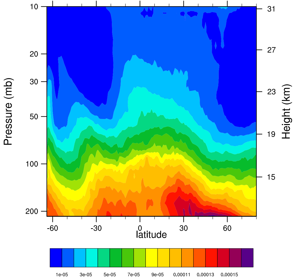
2007d219 12.1MicronExtinction_Combined ( \text{km}^{-1} )
