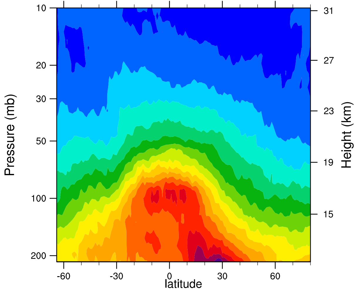
2006d094 12.1MicronExtinction_Combined (km -1 )
