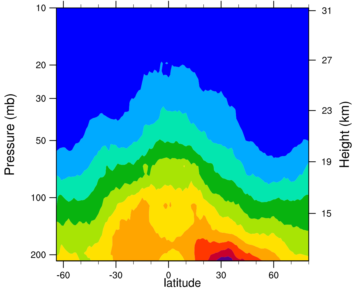
2007d123 12.1MicronExtinction_Combined (km -1 )
