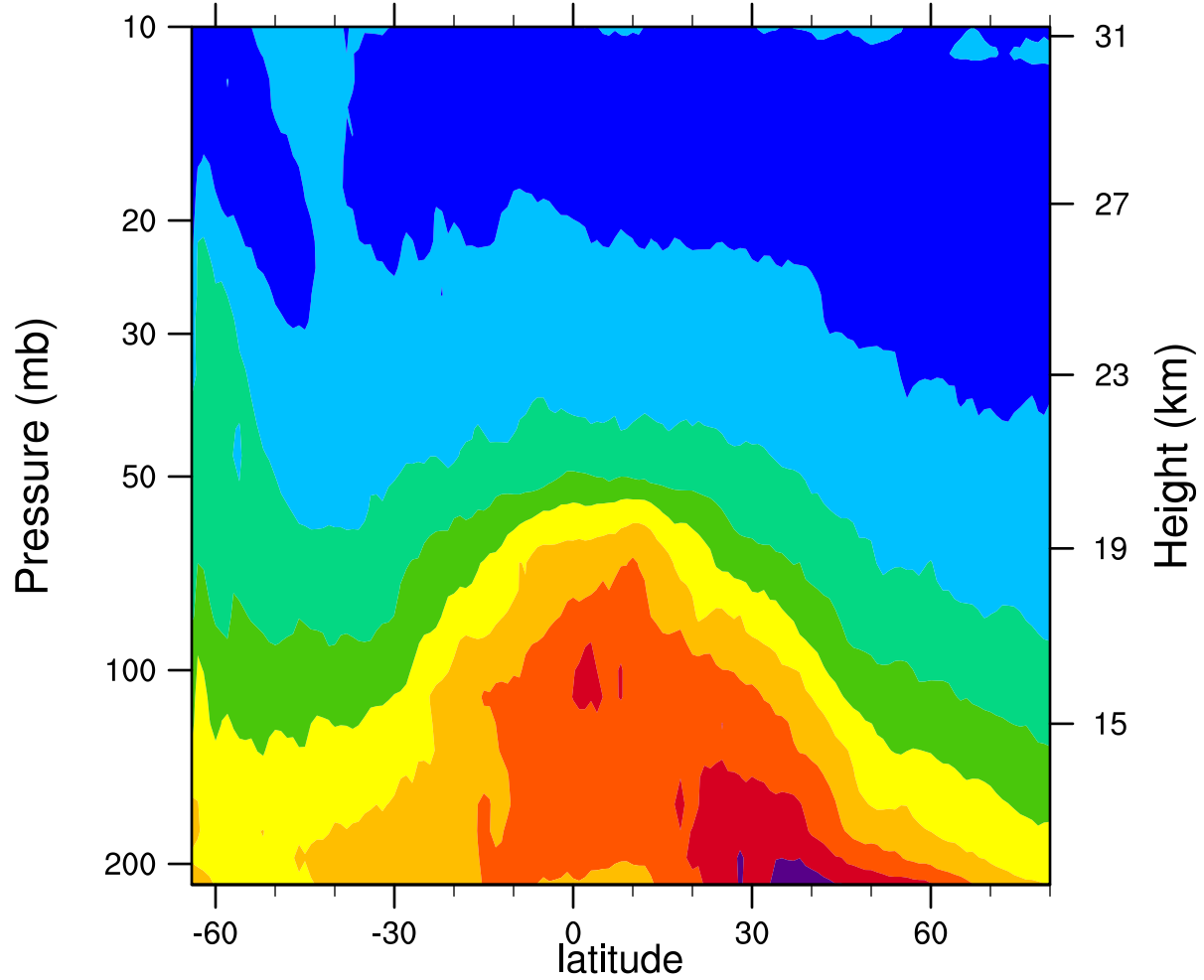
2006d194 12.1MicronExtinction_Combined (km -1 )
