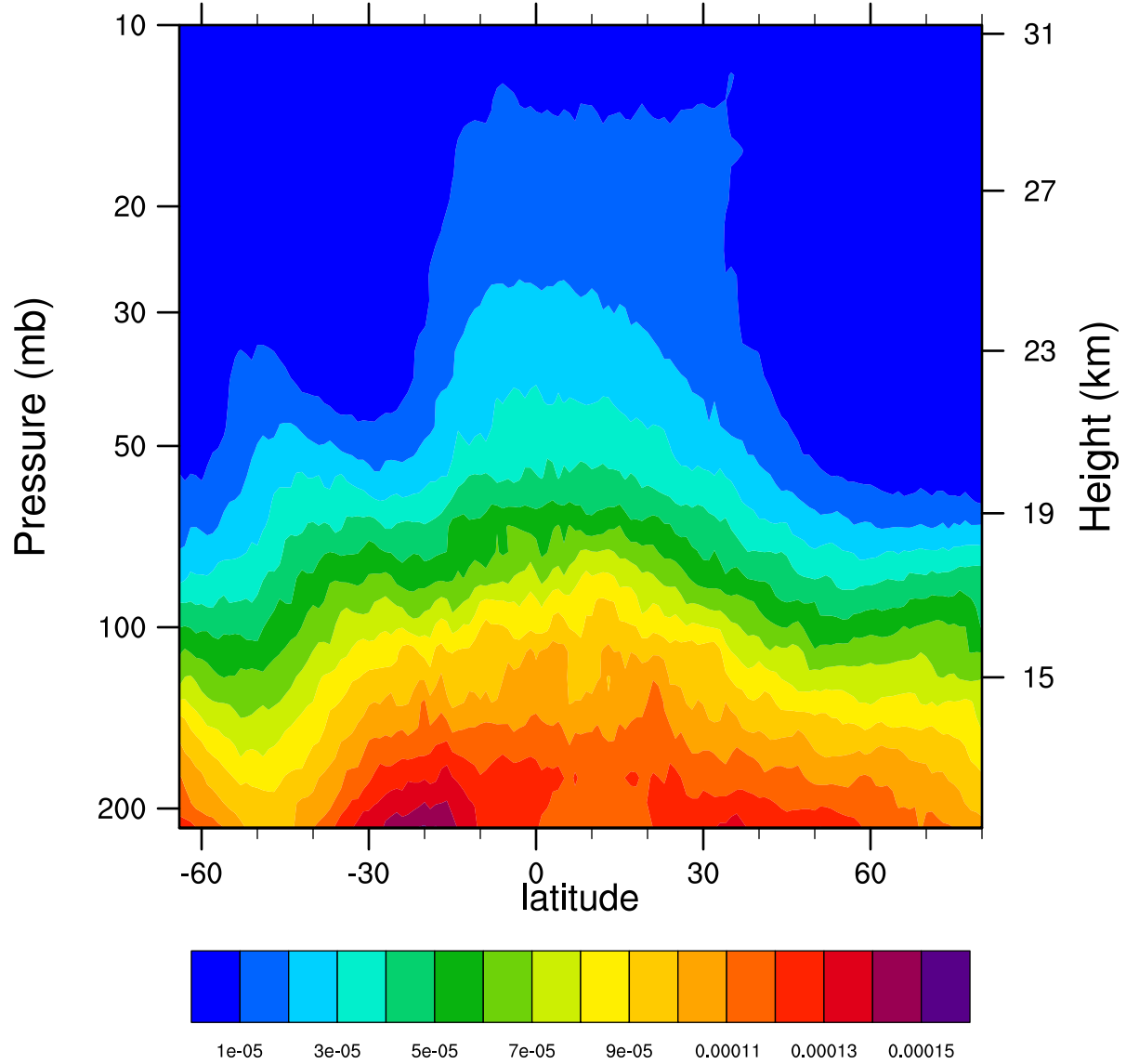
2007d275 12.1MicronExtinction_Combined (km -1 )
