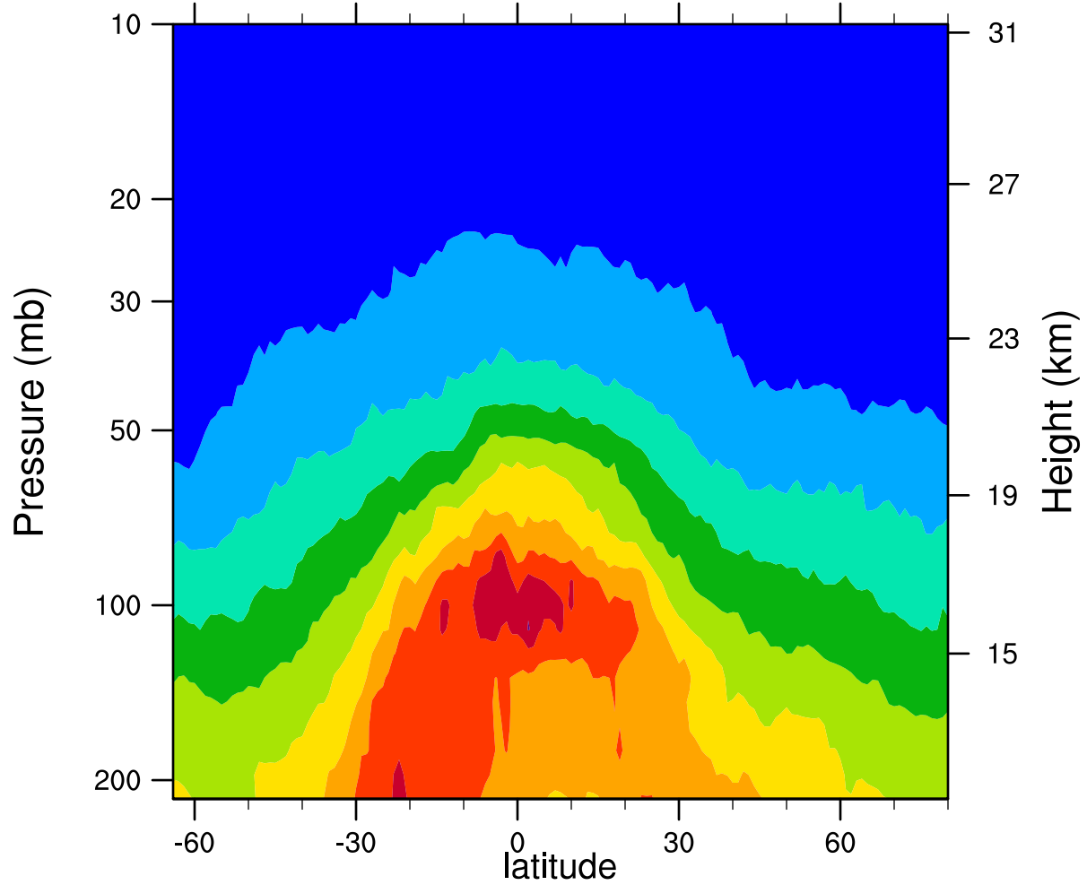
2006d307 12.1MicronExtinction_Combined (km -1 )
