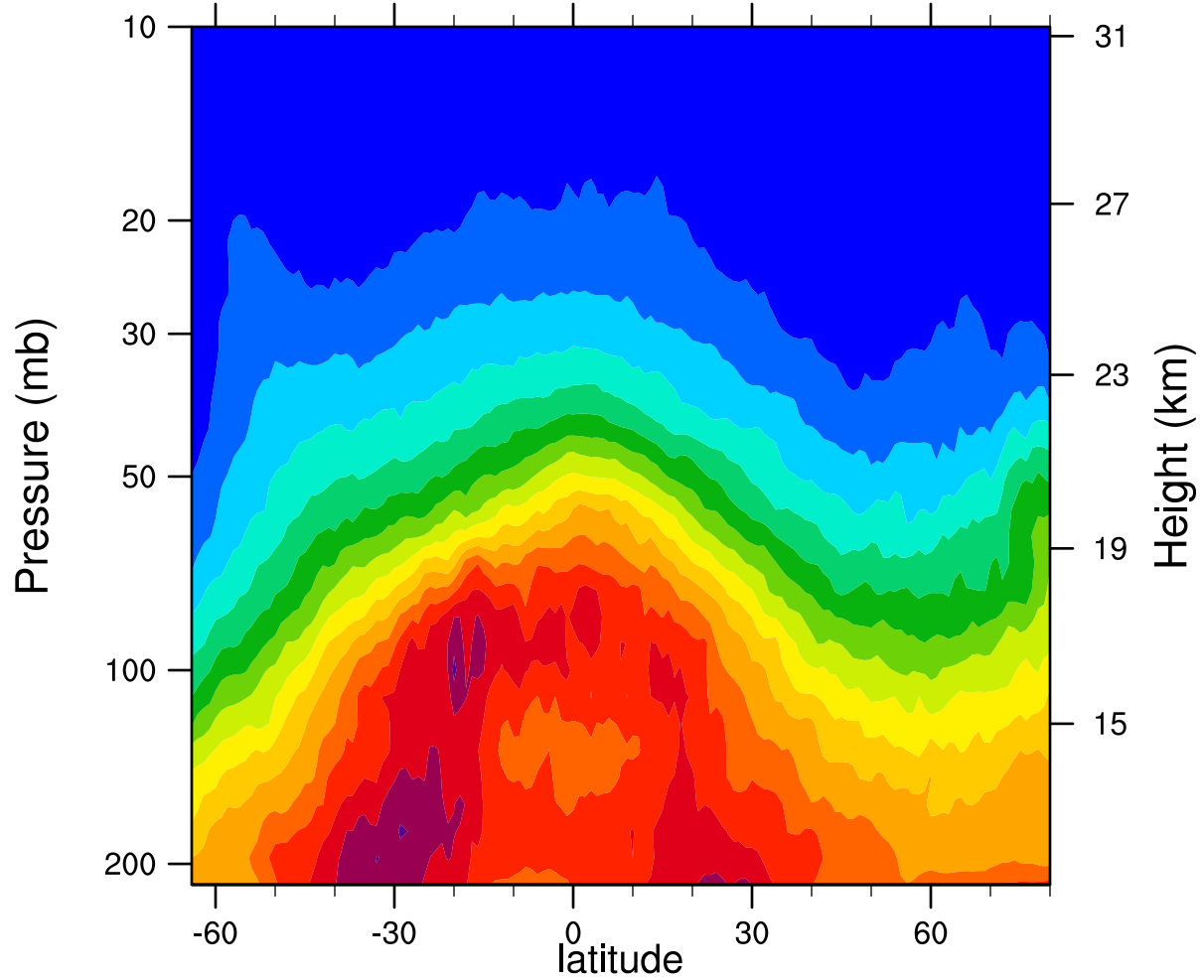
2006d363 12.1MicronExtinction_Combined (km -1 )
