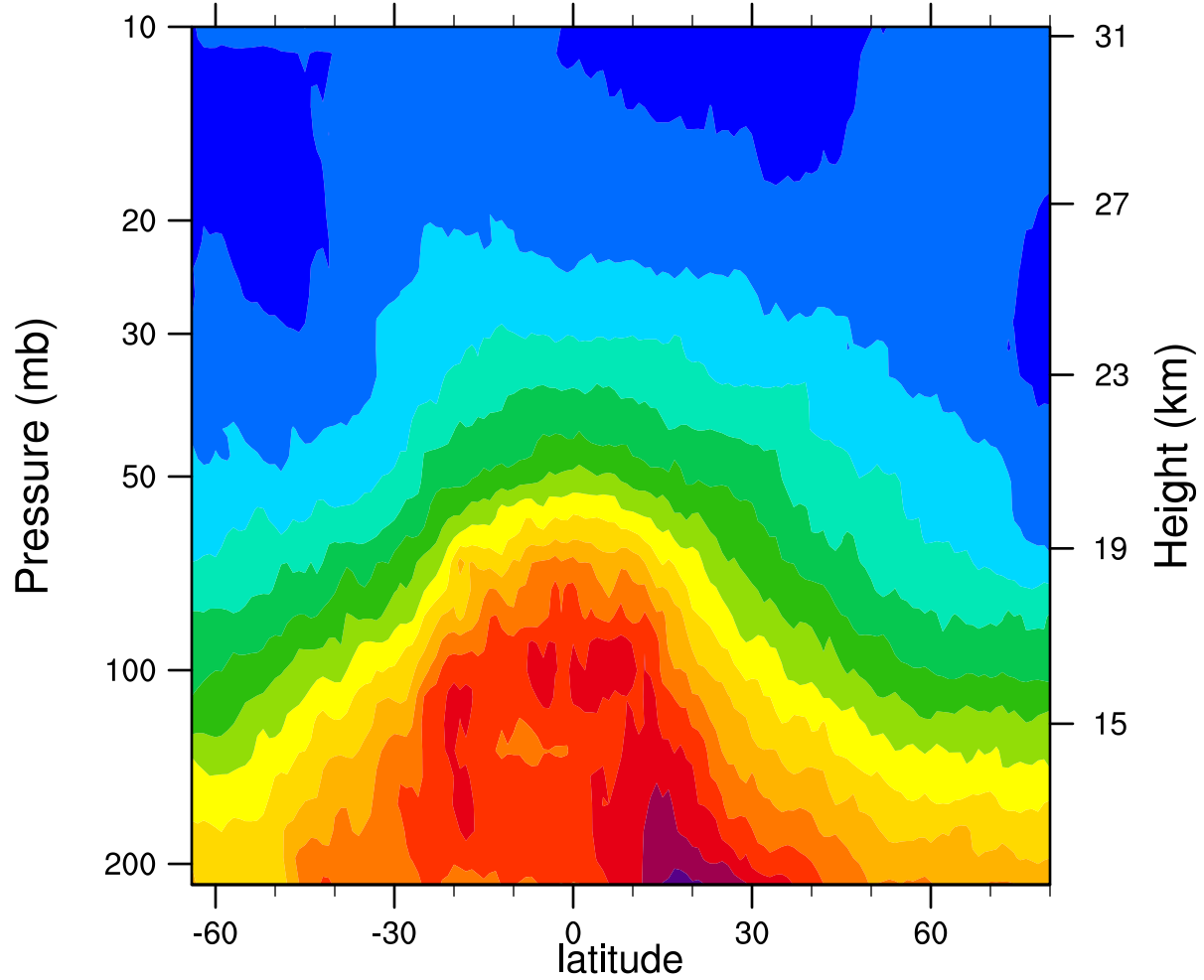
2006d060 12.1MicronExtinction_Combined (km -1 )
