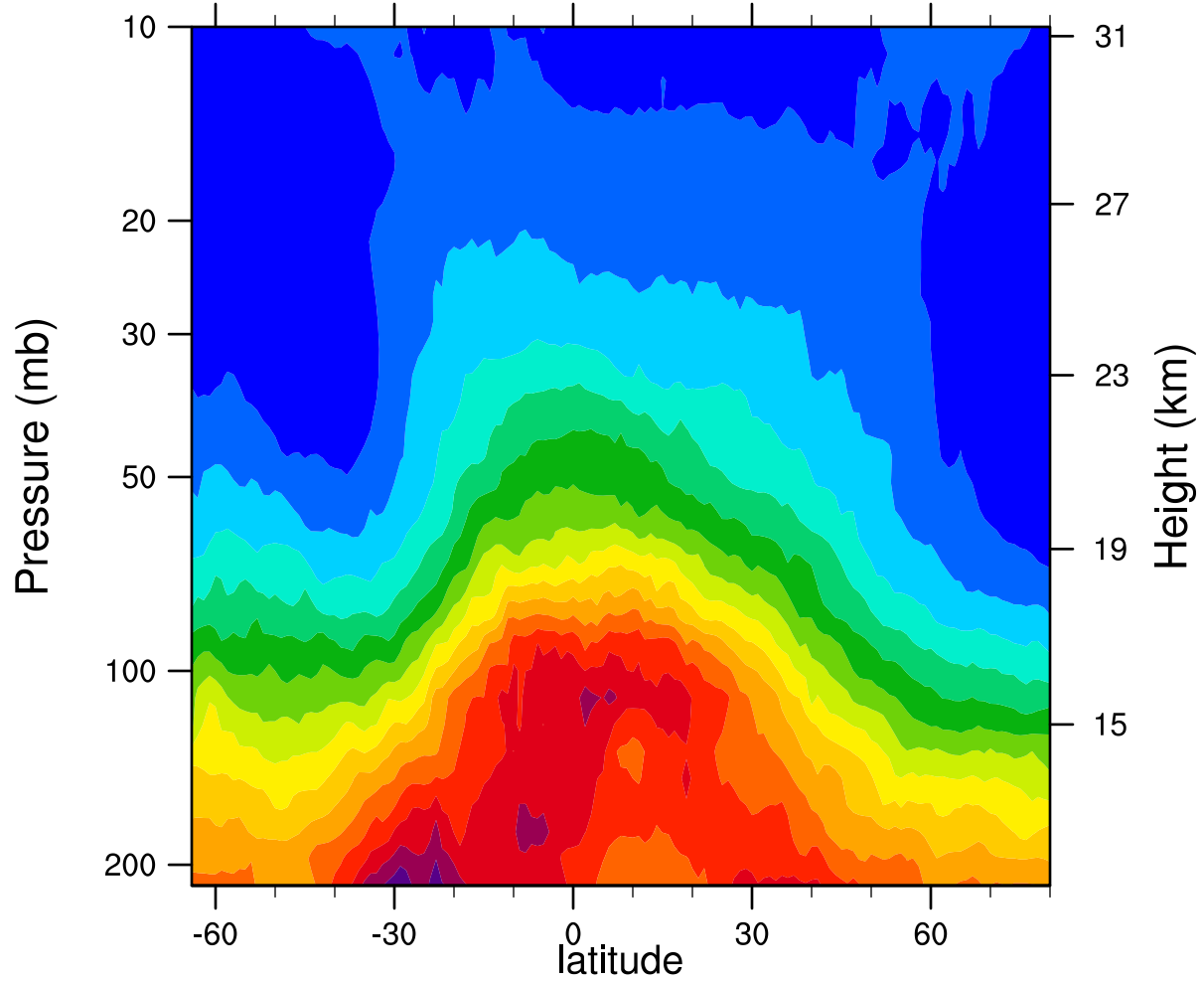
2005d280 12.1MicronExtinction_Combined (km -1 )
