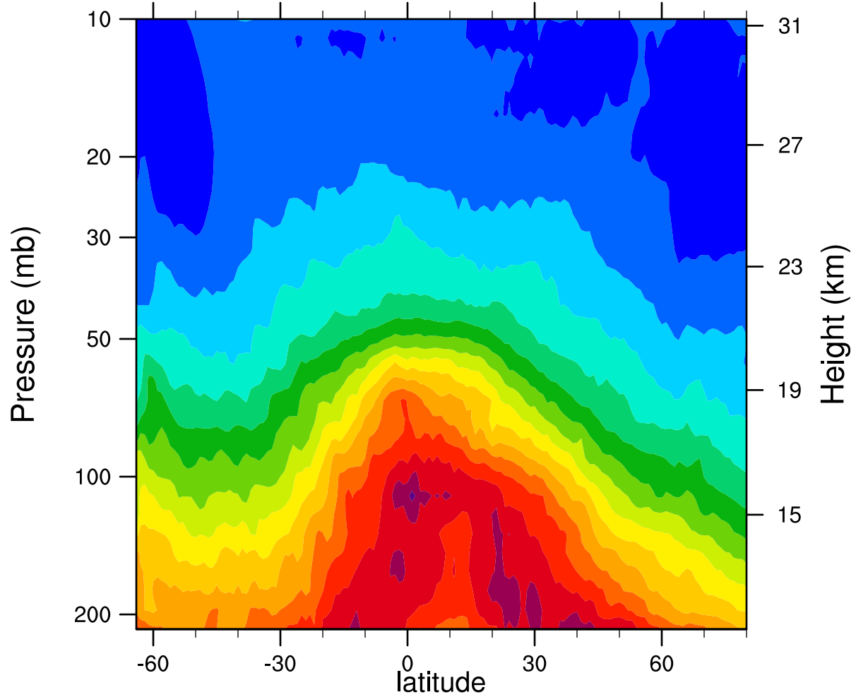
2006d244 12.1MicronExtinction_Combined (km -1 )
