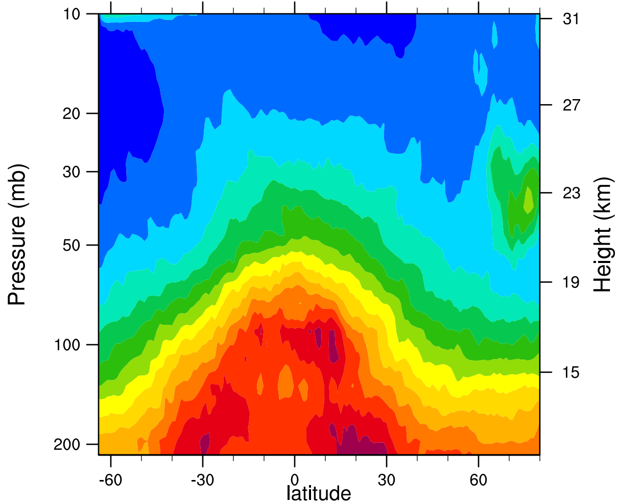
2005d365 12.1MicronExtinction_Combined (km -1 )
