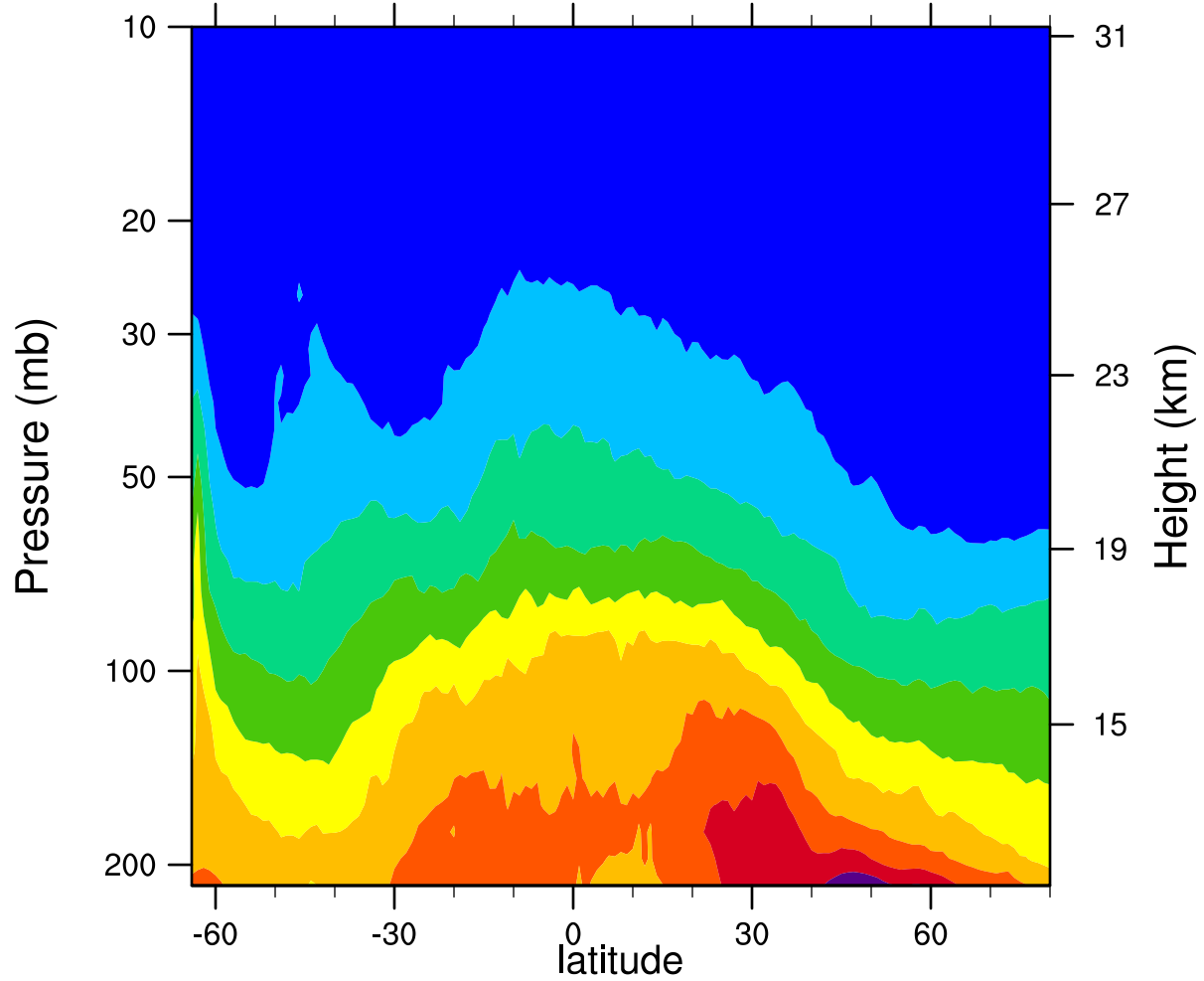
2007d210 12.1MicronExtinction_Combined (km -1 )
