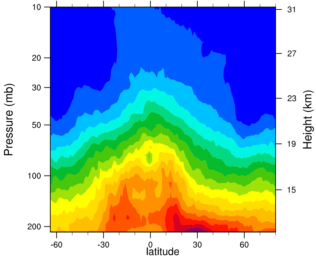
2007d102 12.1MicronExtinction_Combined (km -1 )
