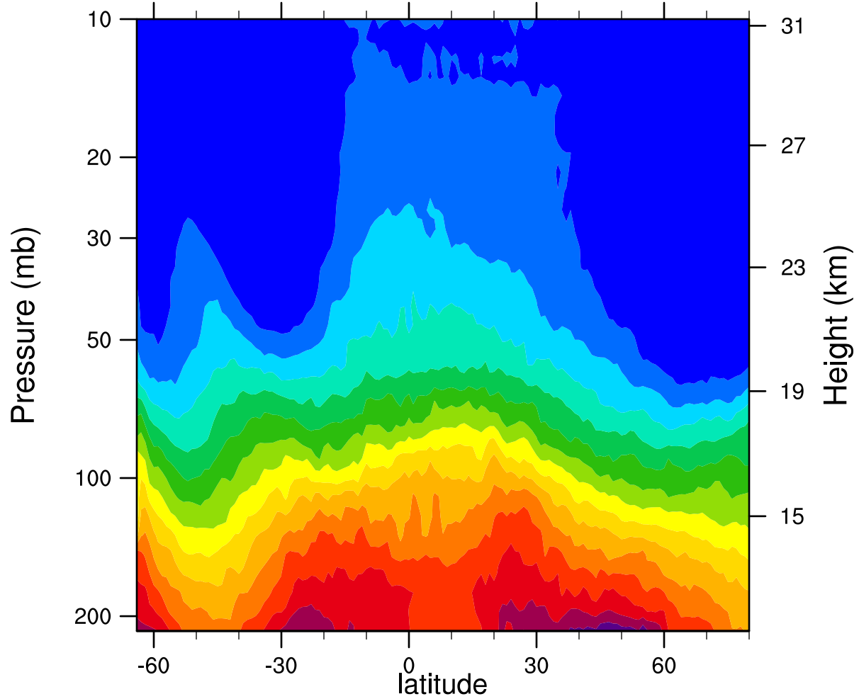
2007d251 12.1MicronExtinction_Combined (km -1 )
