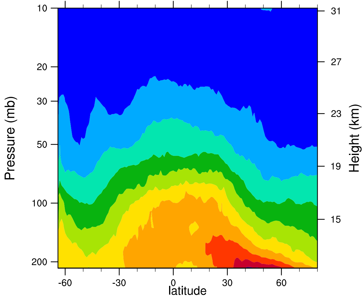
2007d194 12.1MicronExtinction_Combined (km -1 )
