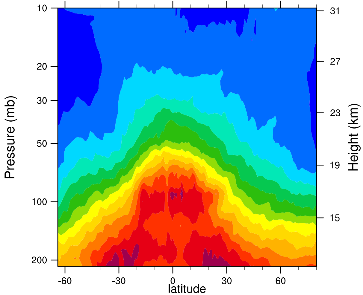
2005d336 12.1MicronExtinction_Combined (km -1 )
