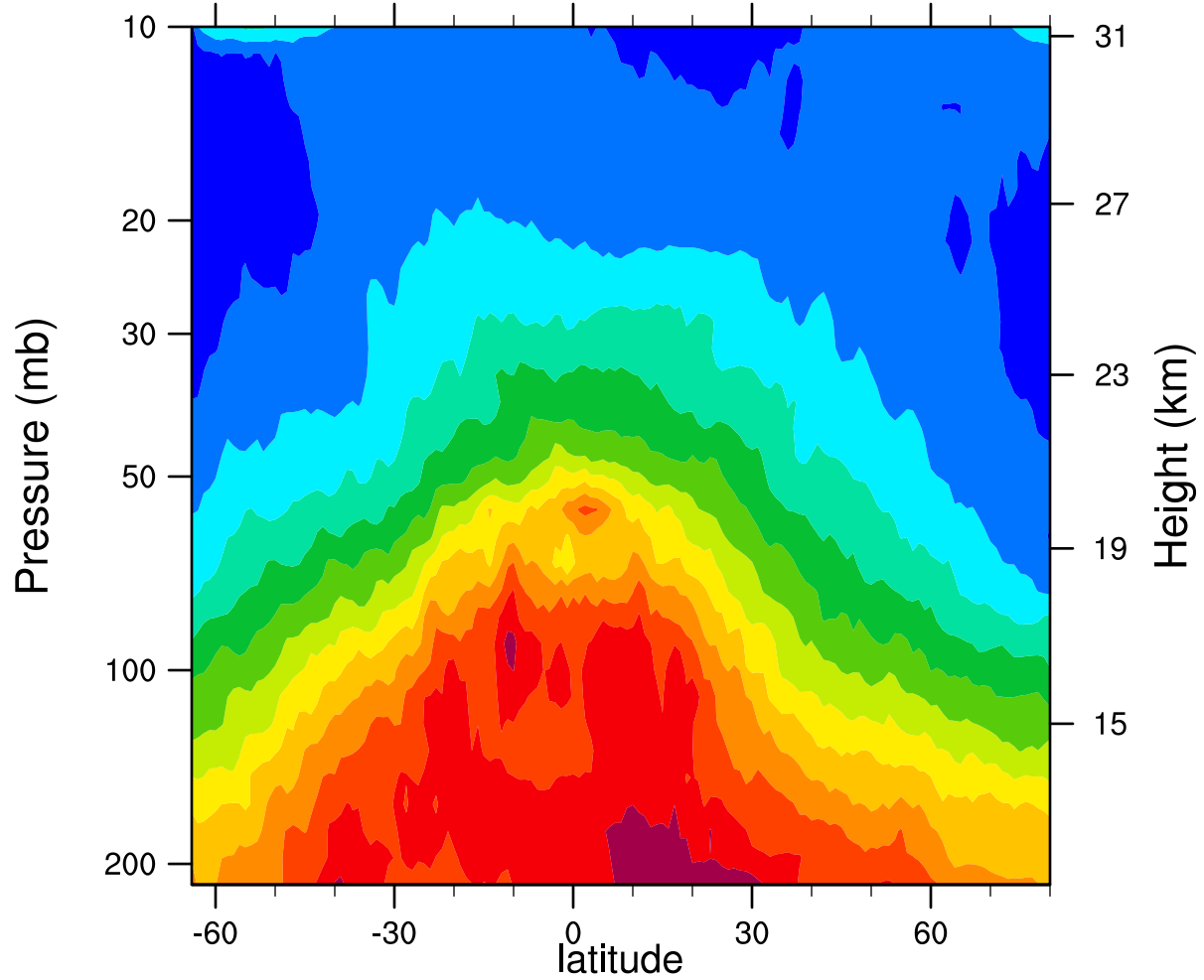
2006d026 12.1MicronExtinction_Combined ( \text{km}^{-1} )
