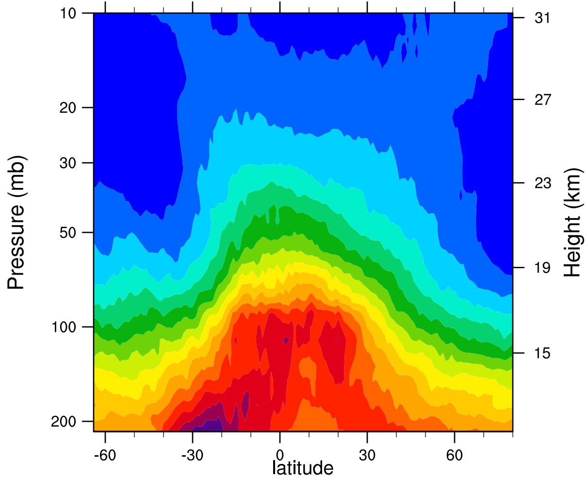
2005d287 12.1MicronExtinction_Combined (km -1 )
