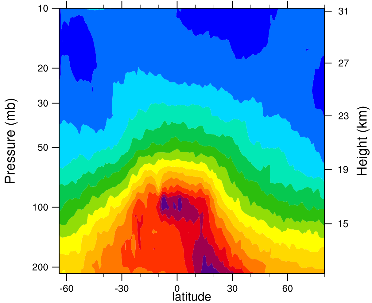
2006d072 12.1MicronExtinction_Combined (km -1 )
