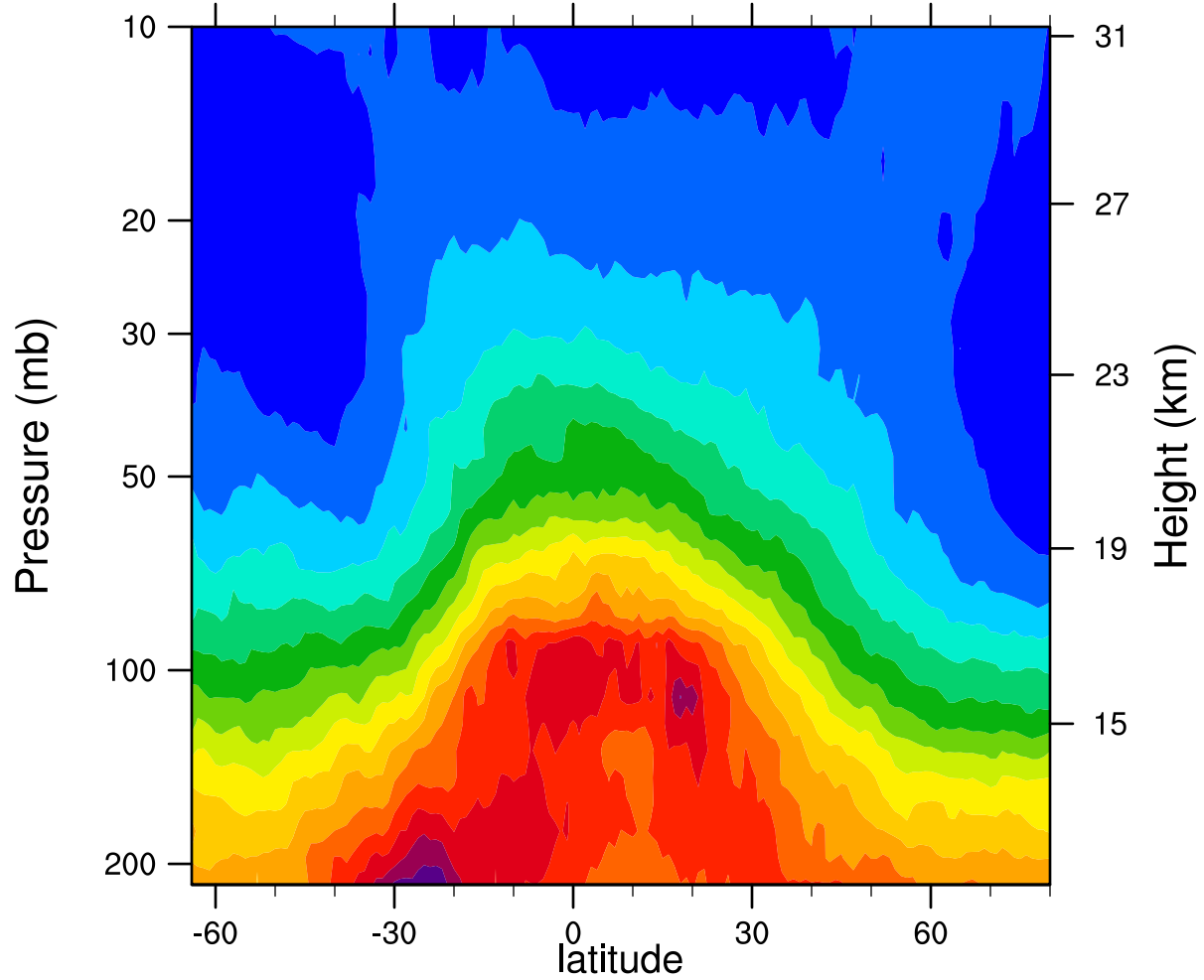
2005d293 12.1MicronExtinction_Combined (km -1 )
