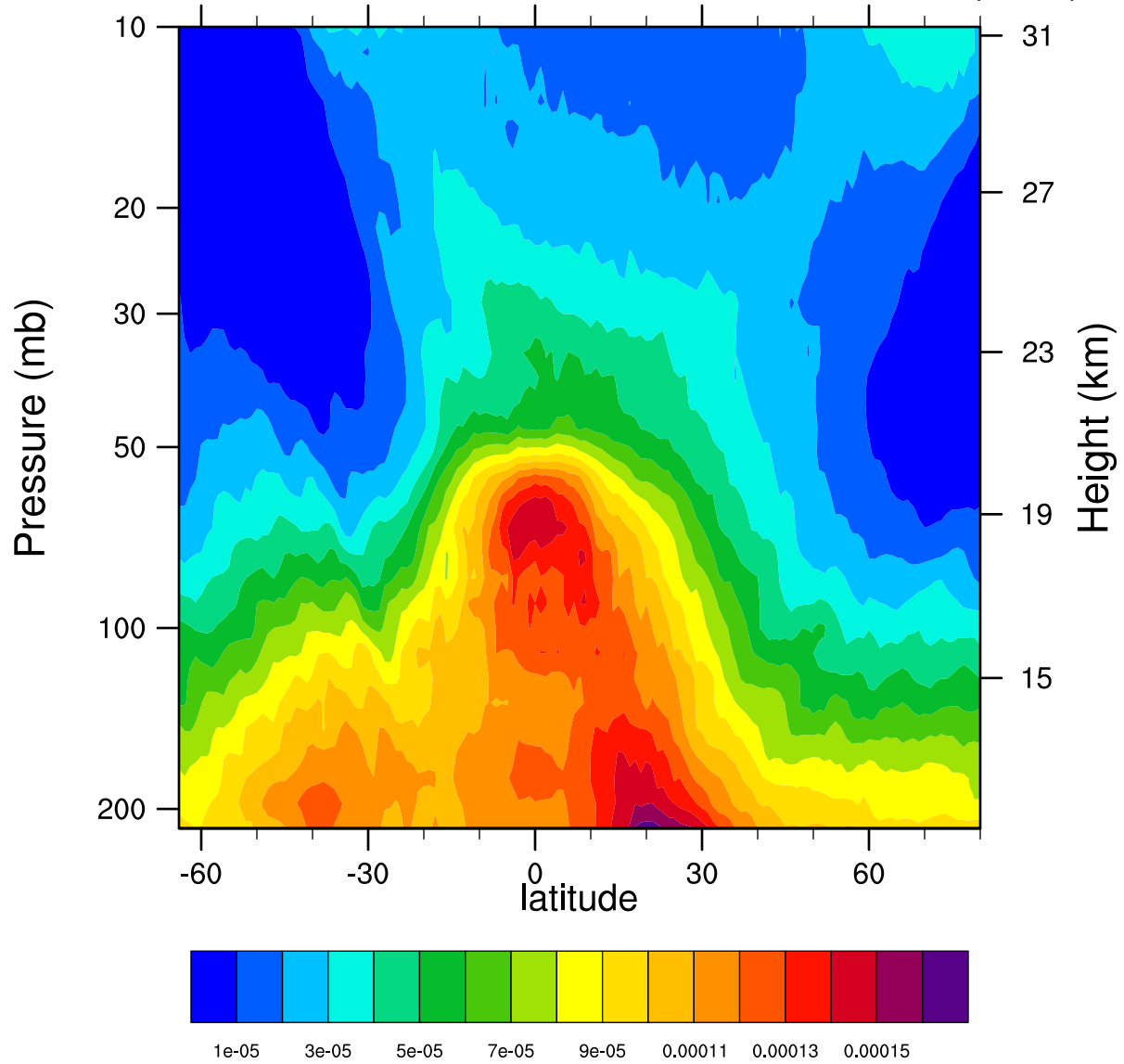
2005d083 12.1MicronExtinction_Combined ( \text{km}^{-1} )
