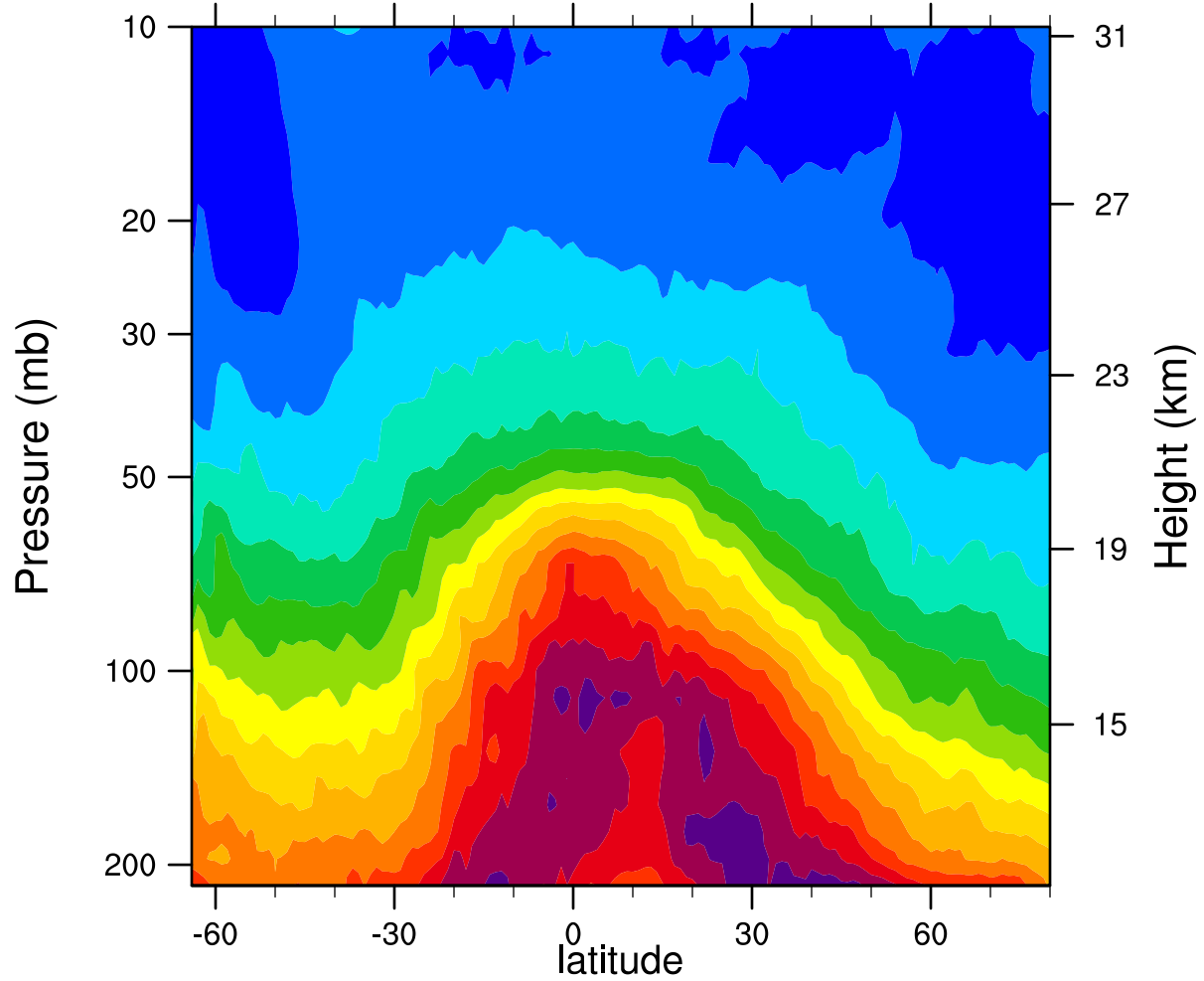
2006d240 12.1MicronExtinction_Combined (km -1 )
