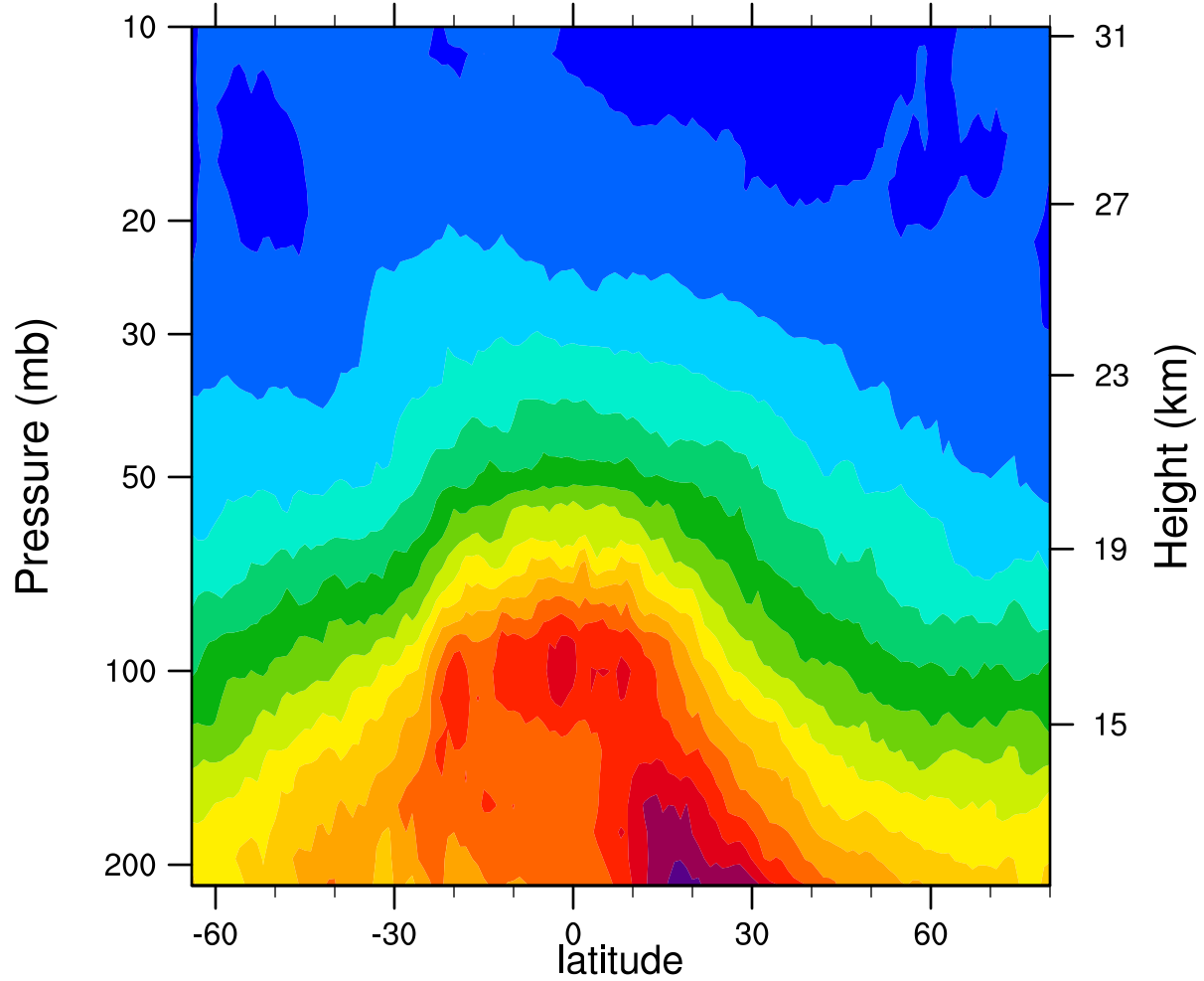
2006d084 12.1MicronExtinction_Combined (km -1 )
