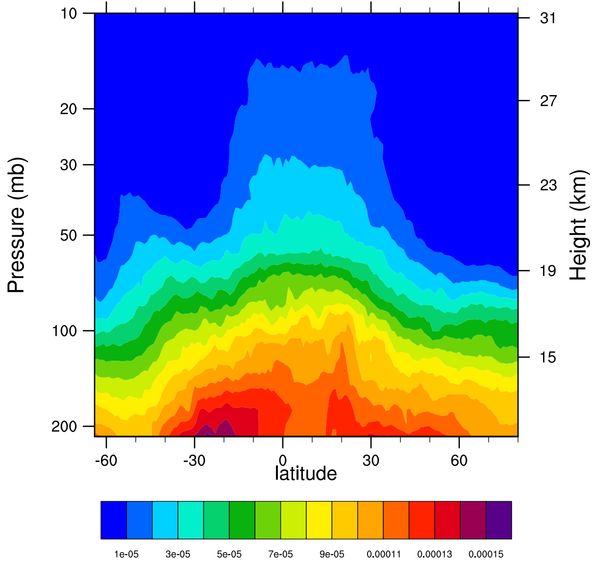
2007d294 12.1MicronExtinction_Combined (km -1 )
