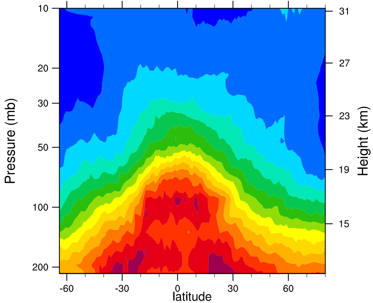
2005d334 12.1MicronExtinction_Combined (km -1 )
