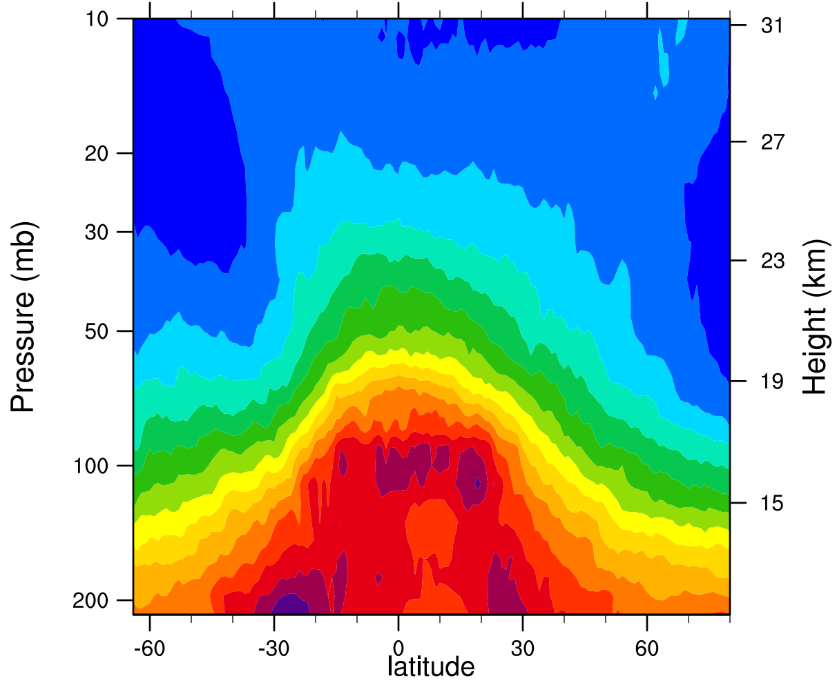
2005d304 12.1MicronExtinction_Combined (km -1 )
