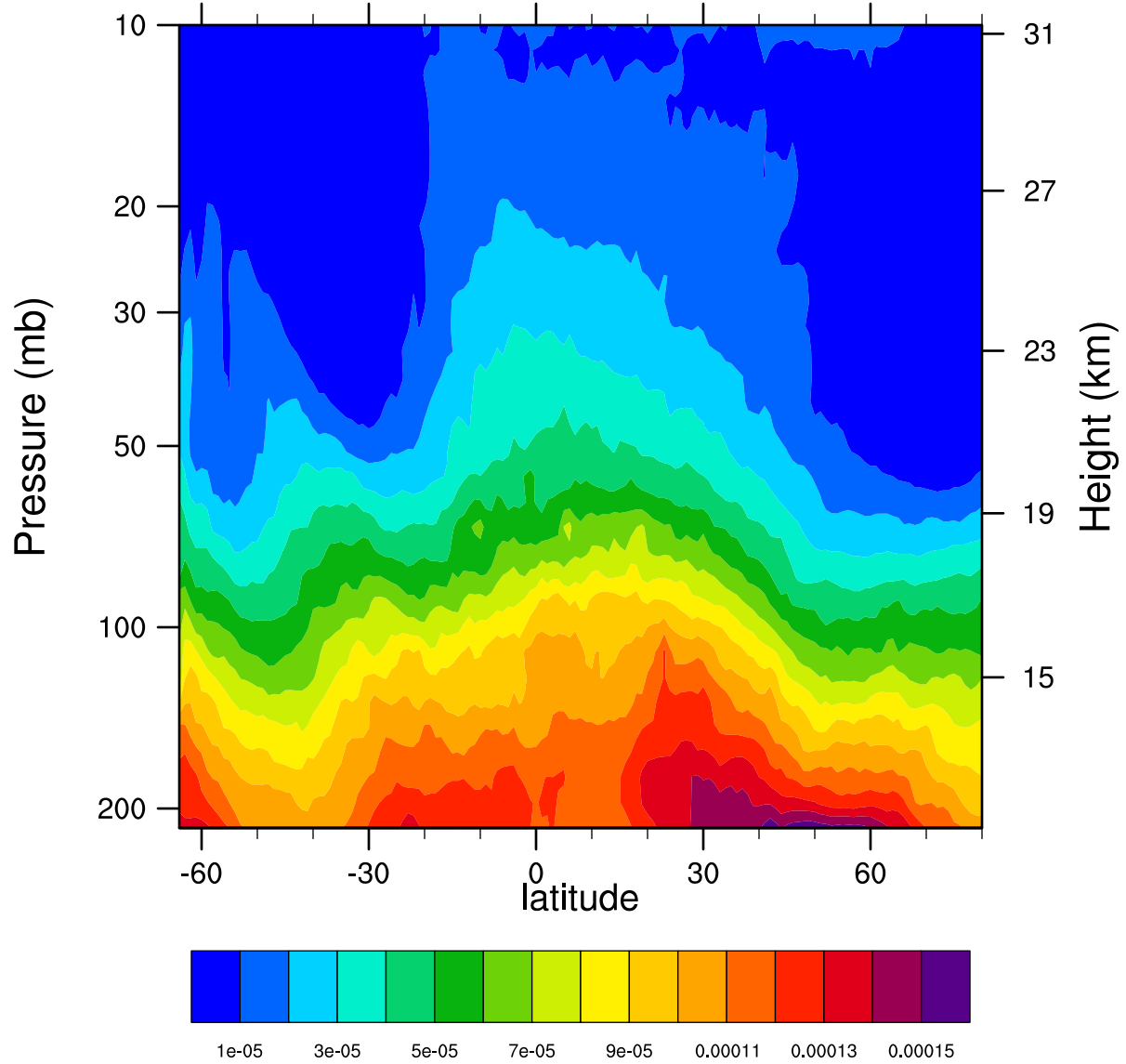
2007d231 12.1MicronExtinction_Combined (km -1 )
