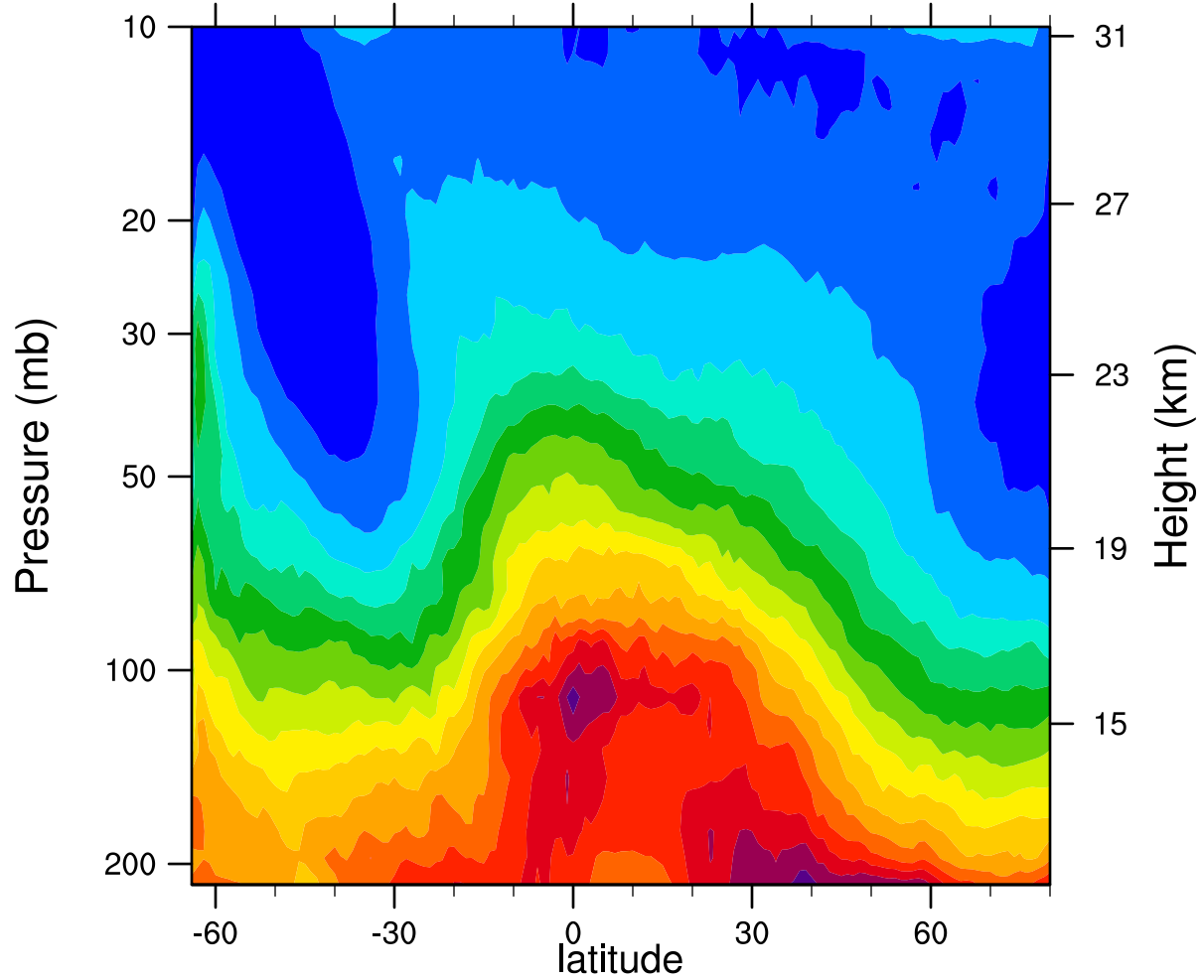
2005d213 12.1MicronExtinction_Combined (km -1 )
