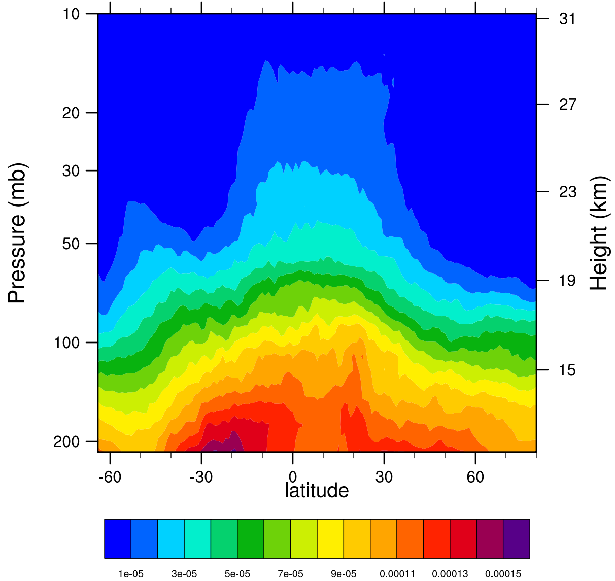
2007d295 12.1MicronExtinction_Combined (km -1 )
