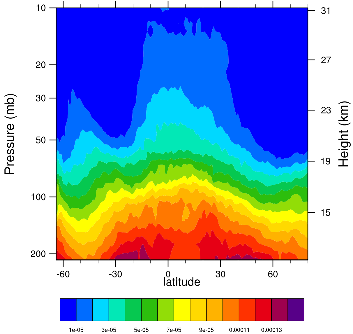
2007d262 12.1MicronExtinction_Combined (km -1 )
