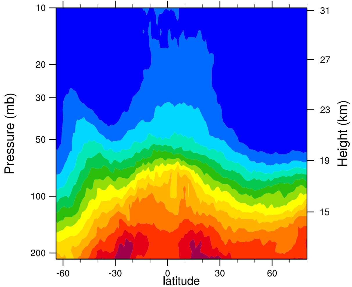
2007d336 12.1MicronExtinction_Combined (km -1 )
