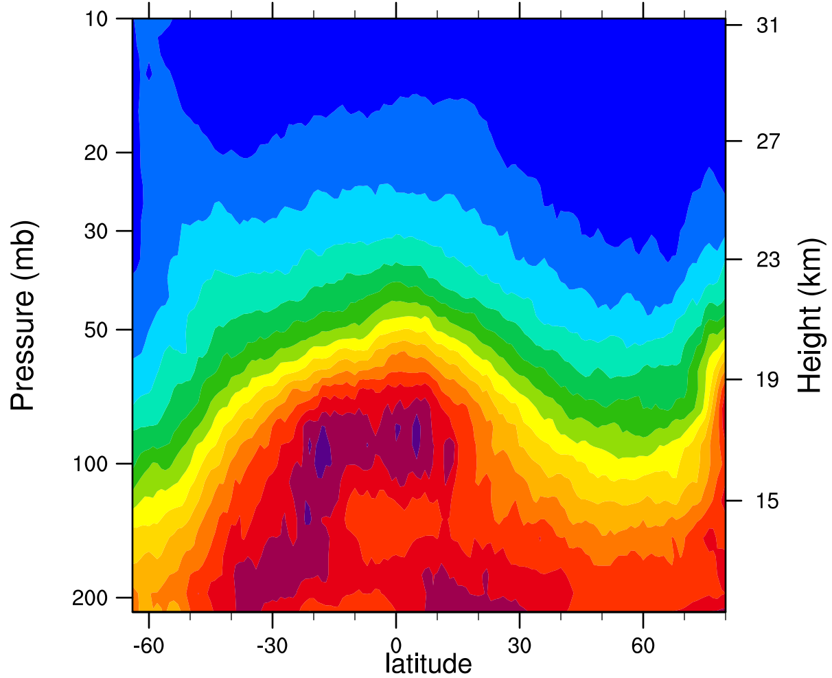
2007d018 12.1MicronExtinction_Combined ( \text{km}^{-1} )
