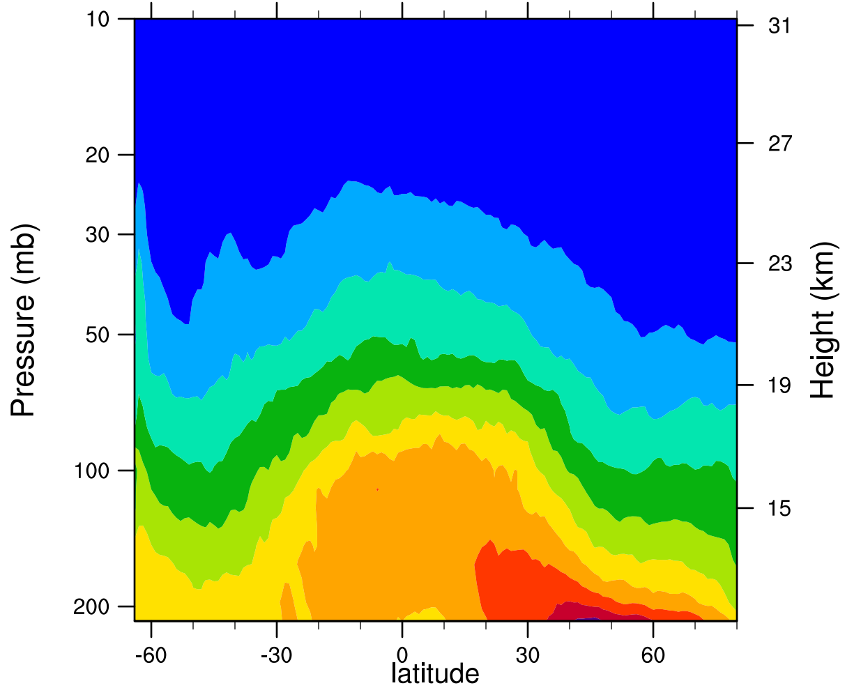
2007d185 12.1MicronExtinction_Combined ( \text{km}^{-1} )
