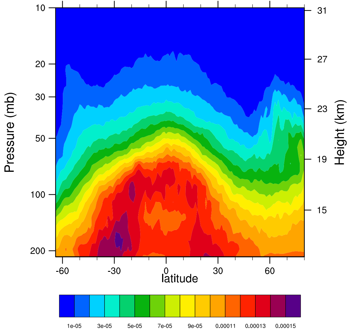
2006d361 12.1MicronExtinction_Combined (km -1 )
