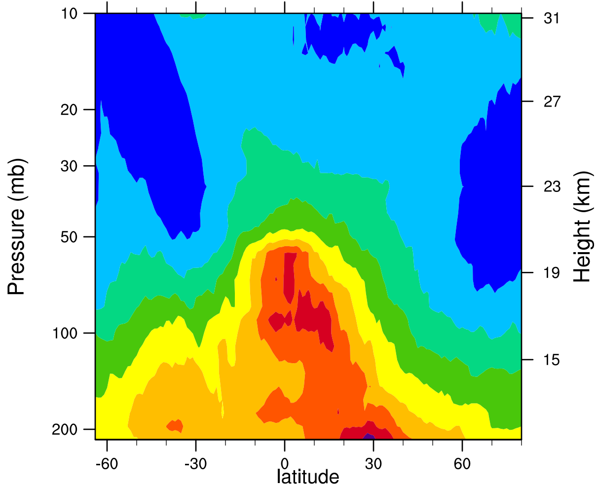
2005d103 12.1MicronExtinction_Combined ( \text{km}^{-1} )
