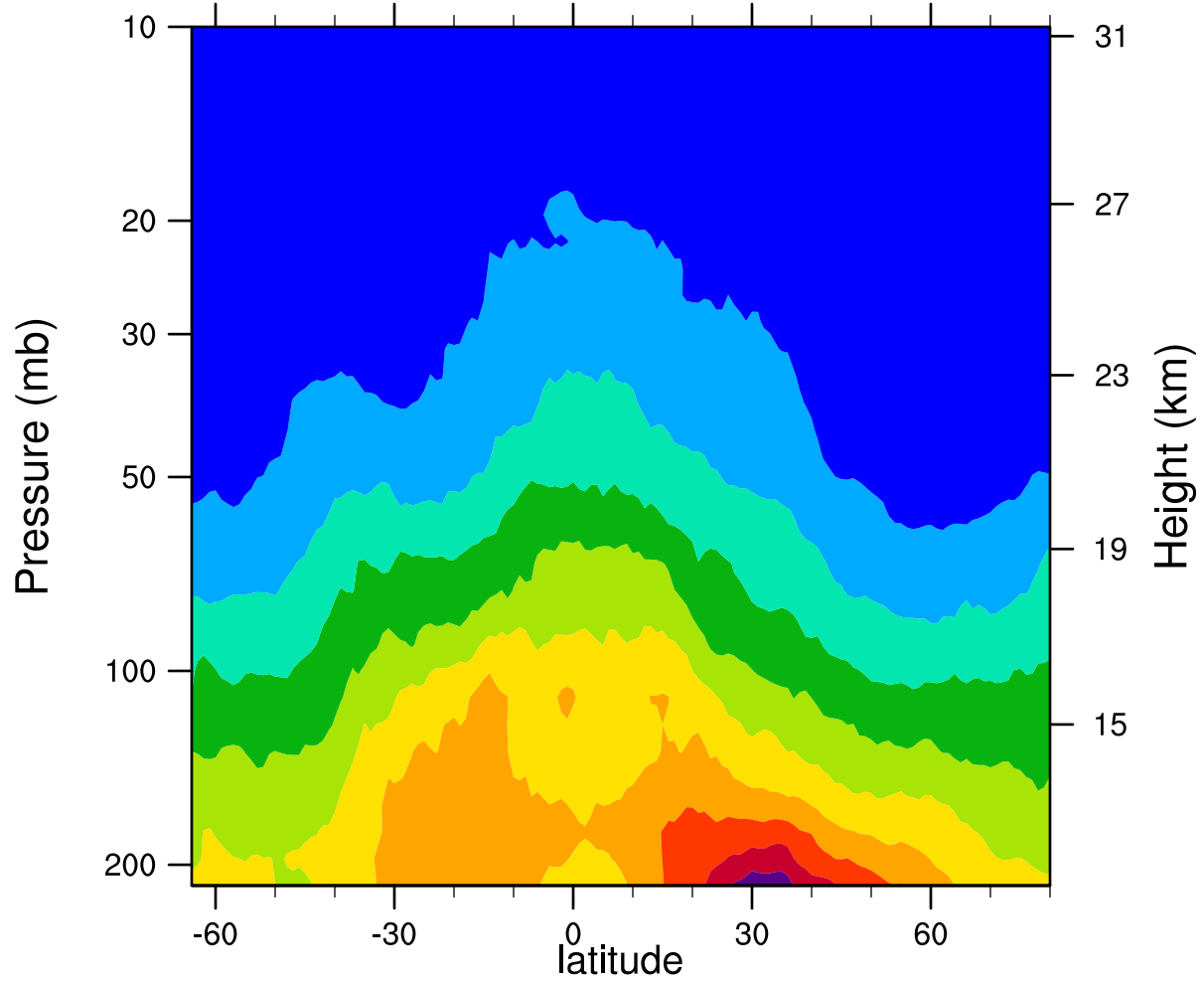
2007d125 12.1MicronExtinction_Combined (km -1 )
