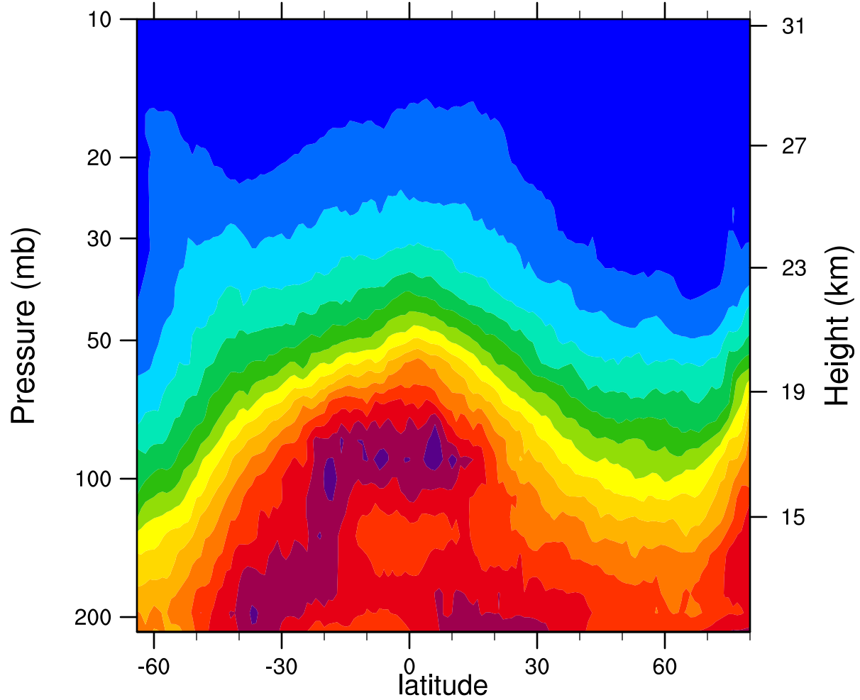
2007d014 12.1MicronExtinction_Combined (km -1 )
