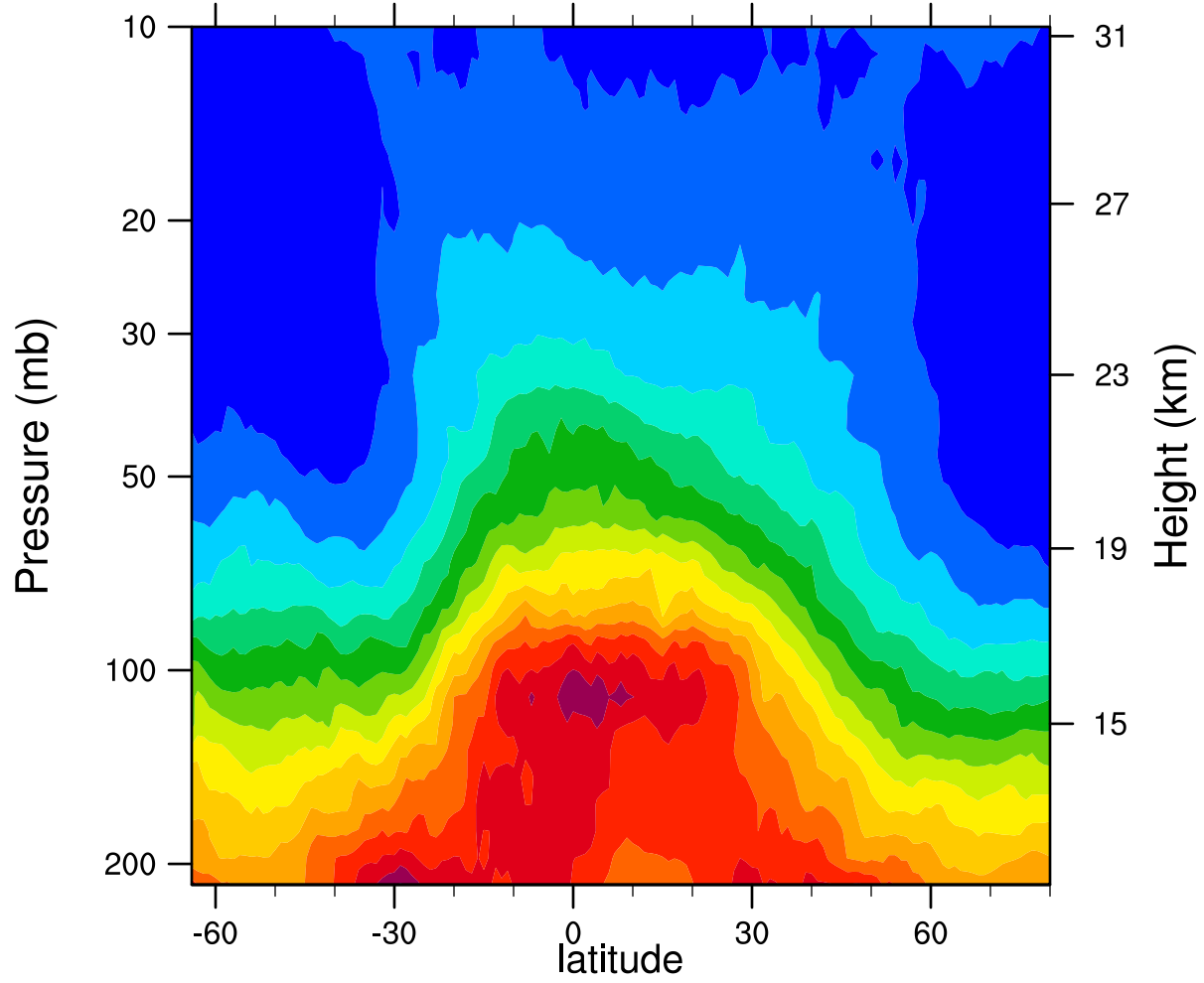
2005d267 12.1MicronExtinction_Combined (km -1 )
