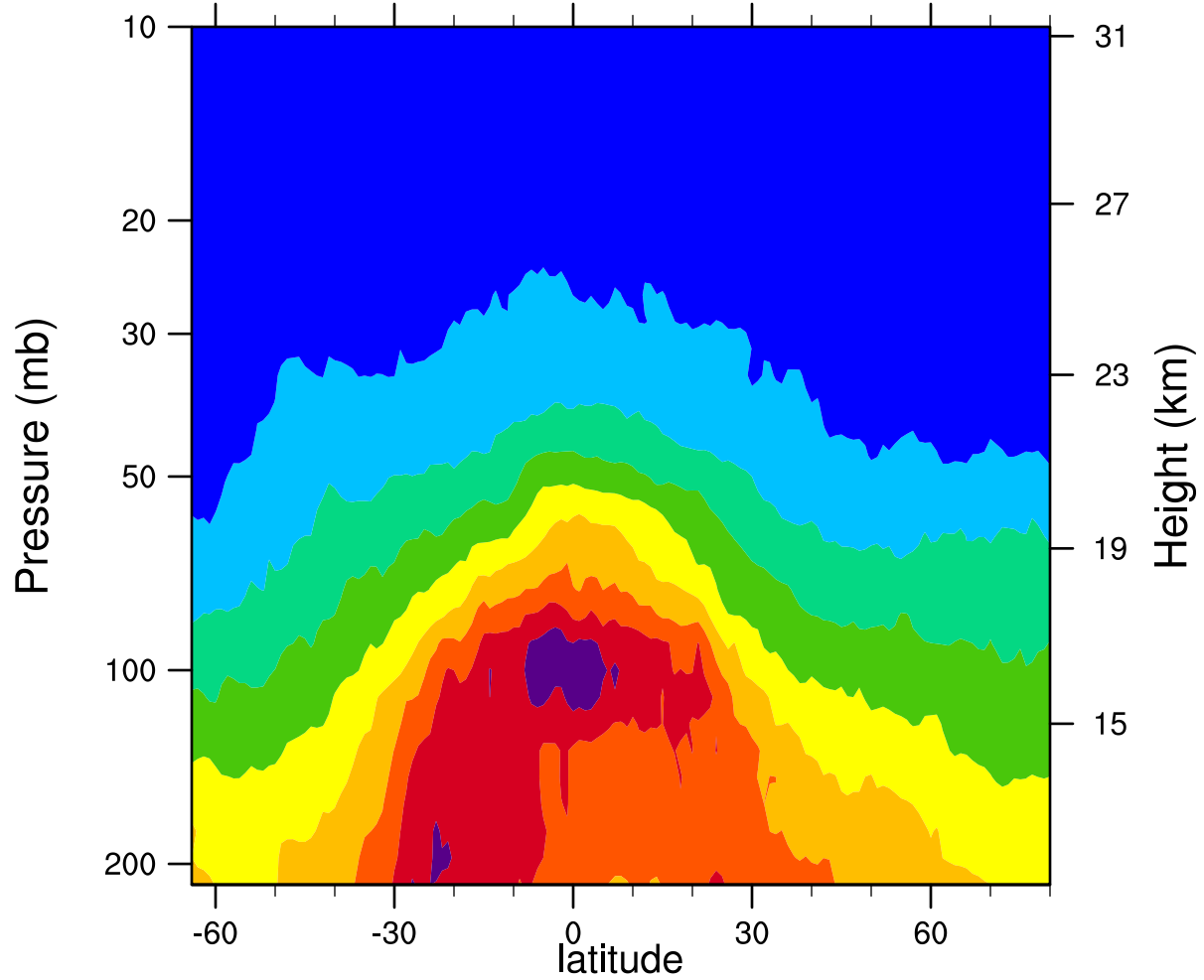
2006d309 12.1MicronExtinction_Combined (km -1 )
