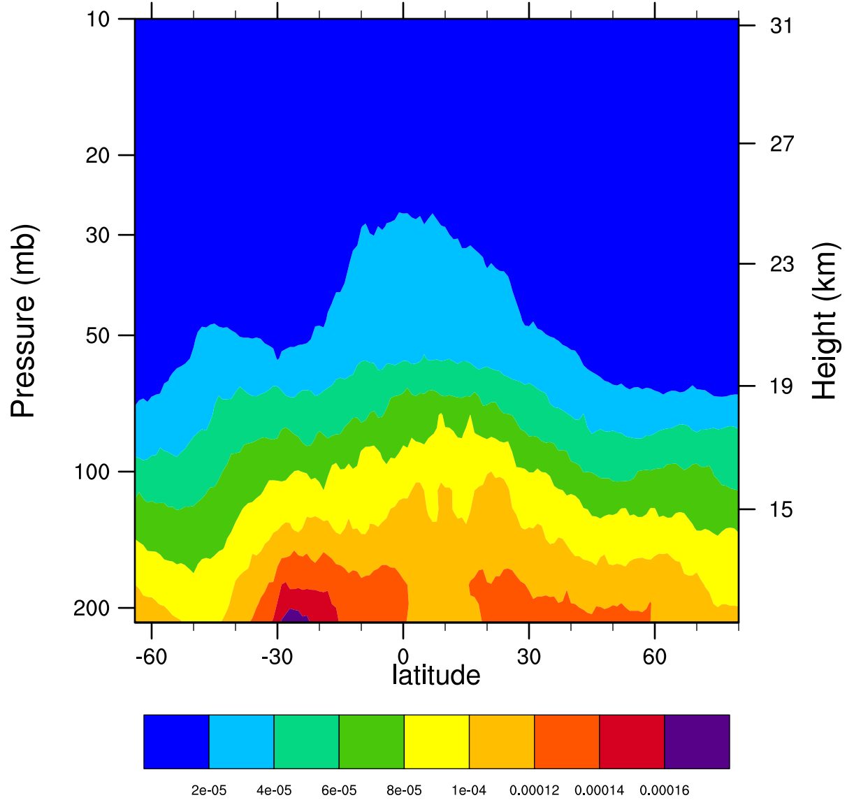
2007d282 12.1MicronExtinction_Combined (km -1 )
