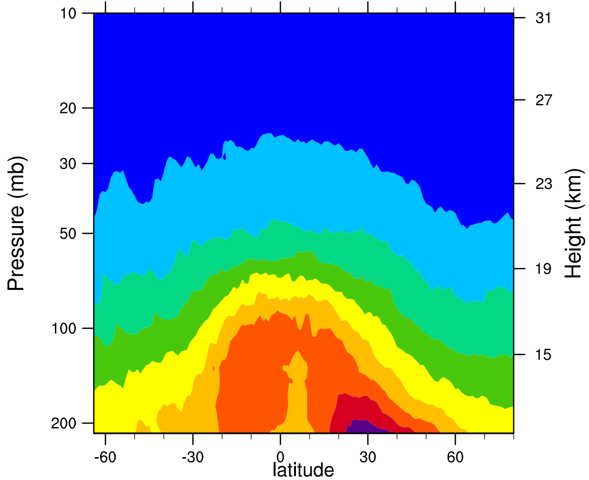
2006d139 12.1MicronExtinction_Combined (km -1 )
