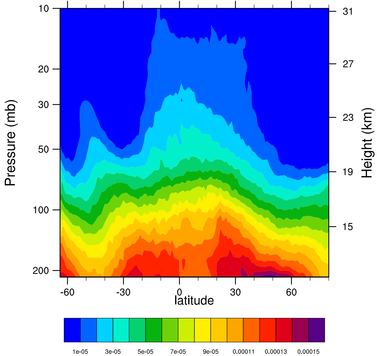
2007d242 12.1MicronExtinction_Combined (km -1 )
