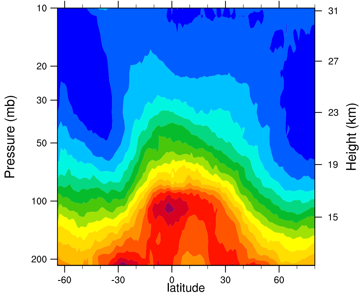
2005d258 12.1MicronExtinction_Combined (km -1 )
