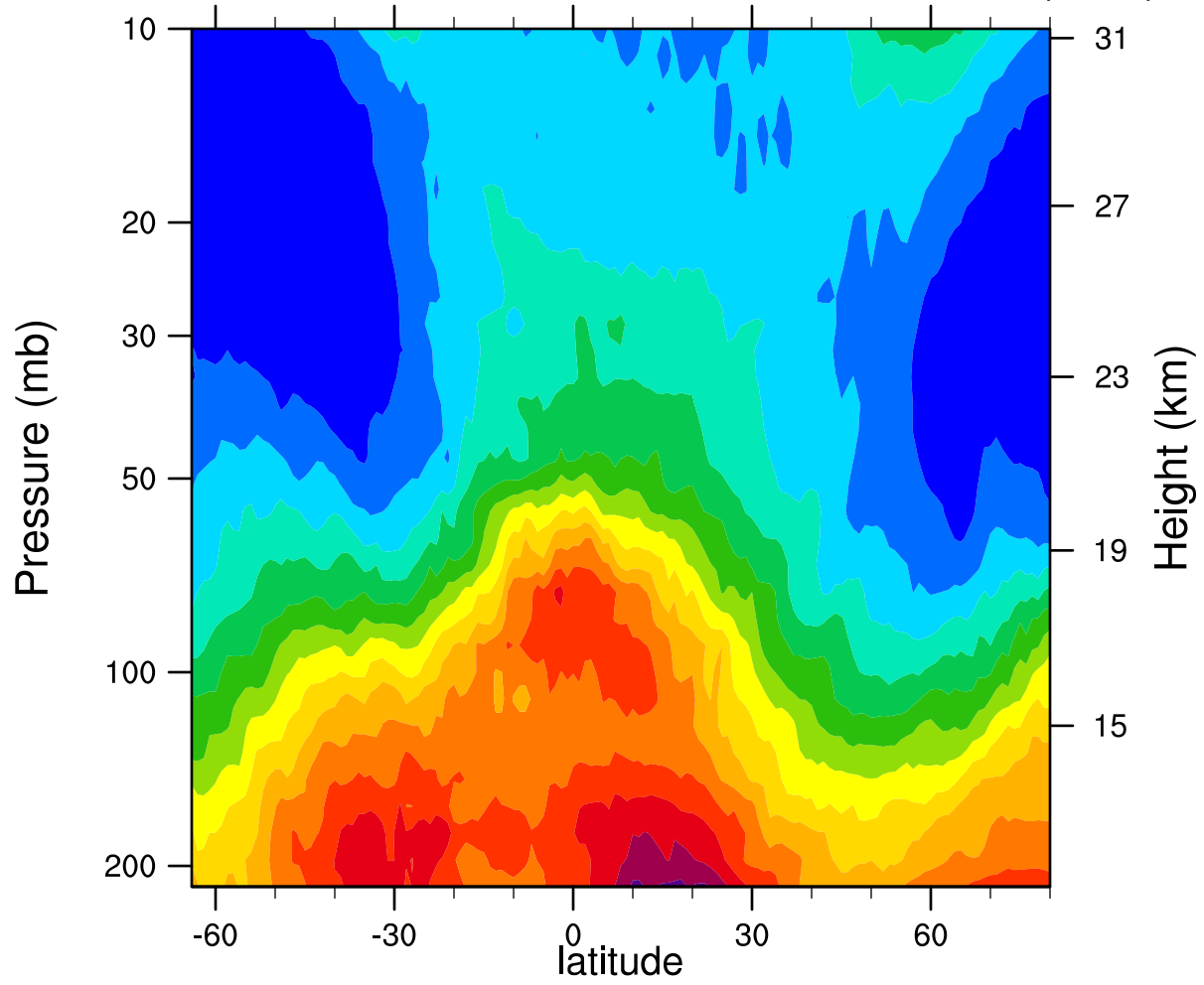
2005d039 12.1MicronExtinction_Combined (km -1 )
