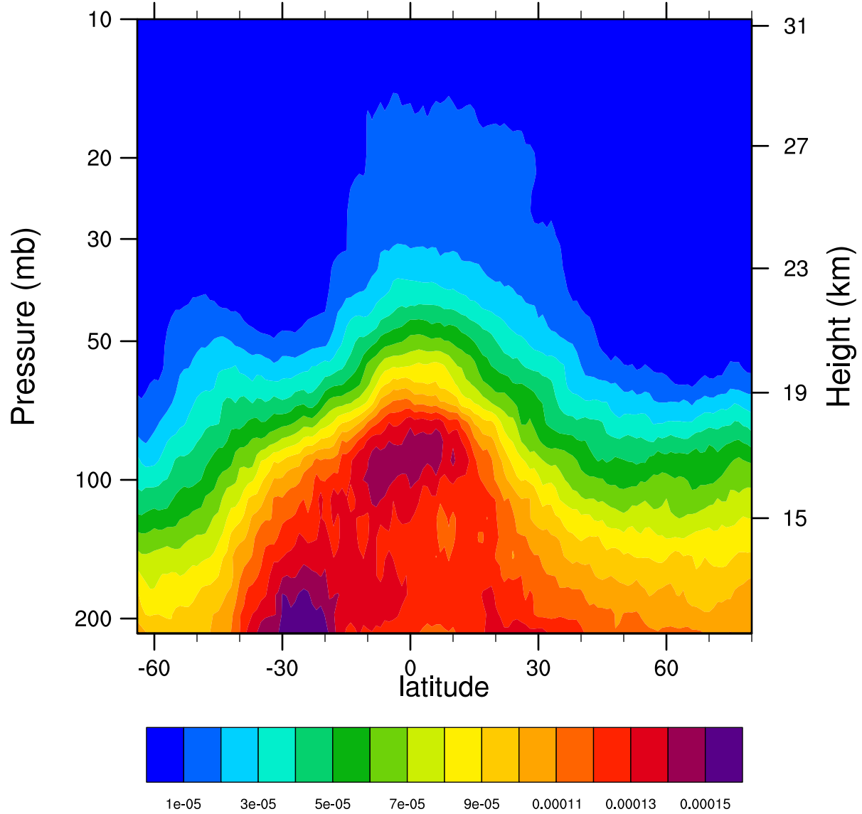
2006d325 12.1MicronExtinction_Combined (km -1 )
