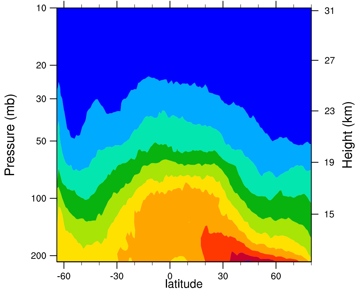
2007d187 12.1MicronExtinction_Combined (km -1 )
