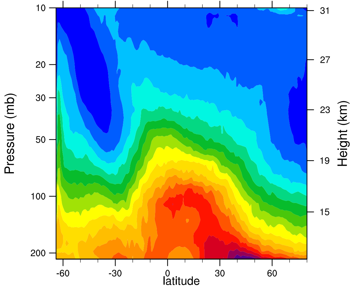
2005d193 12.1MicronExtinction_Combined (km -1 )
