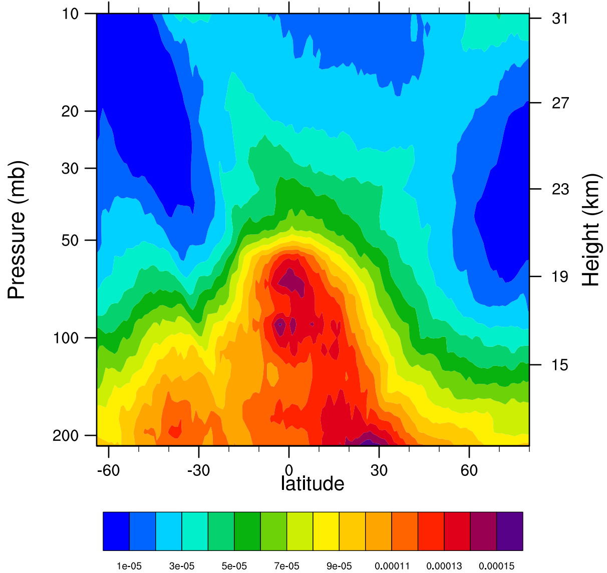
2005d095 12.1MicronExtinction_Combined (km -1 )
