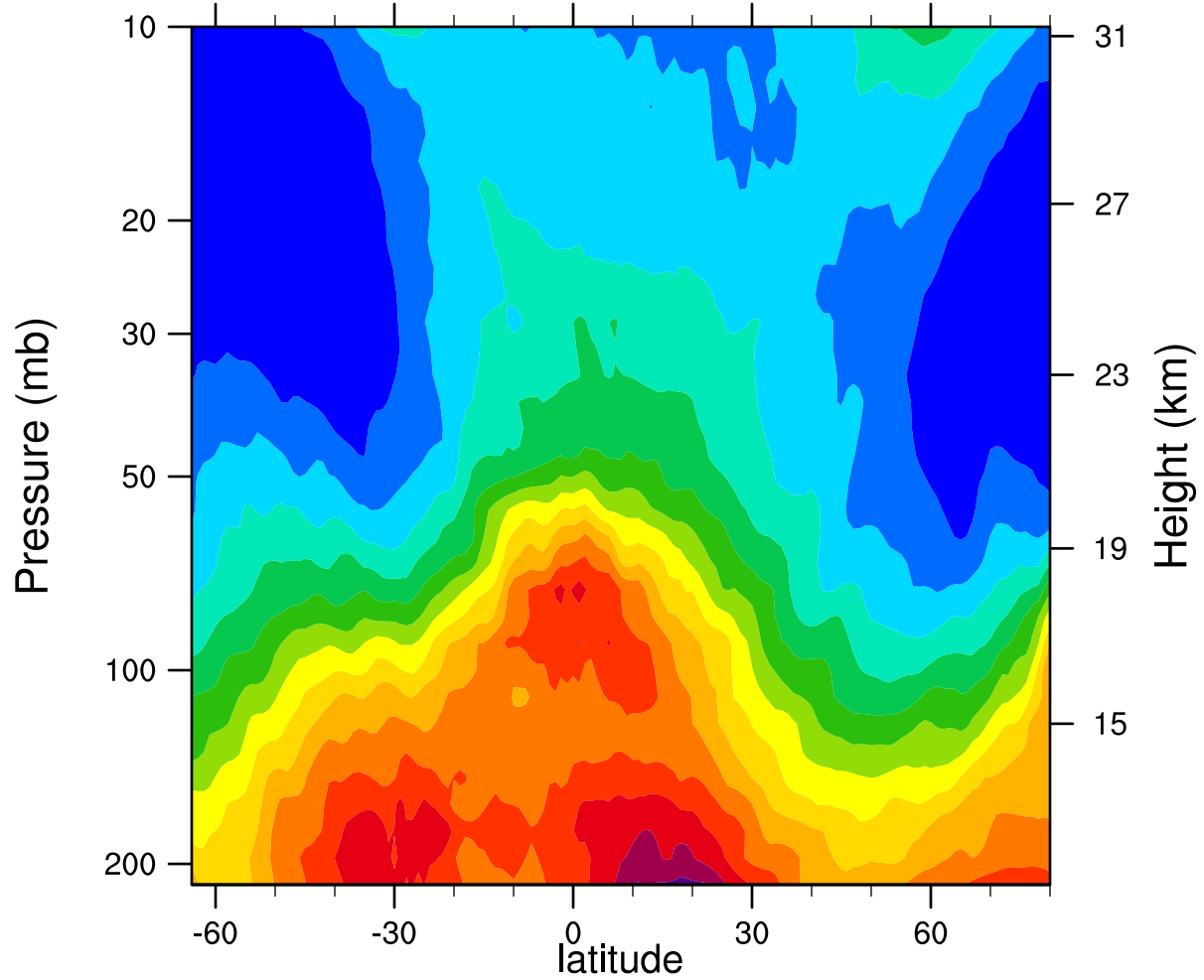
2005d040 12.1MicronExtinction_Combined (km -1 )
