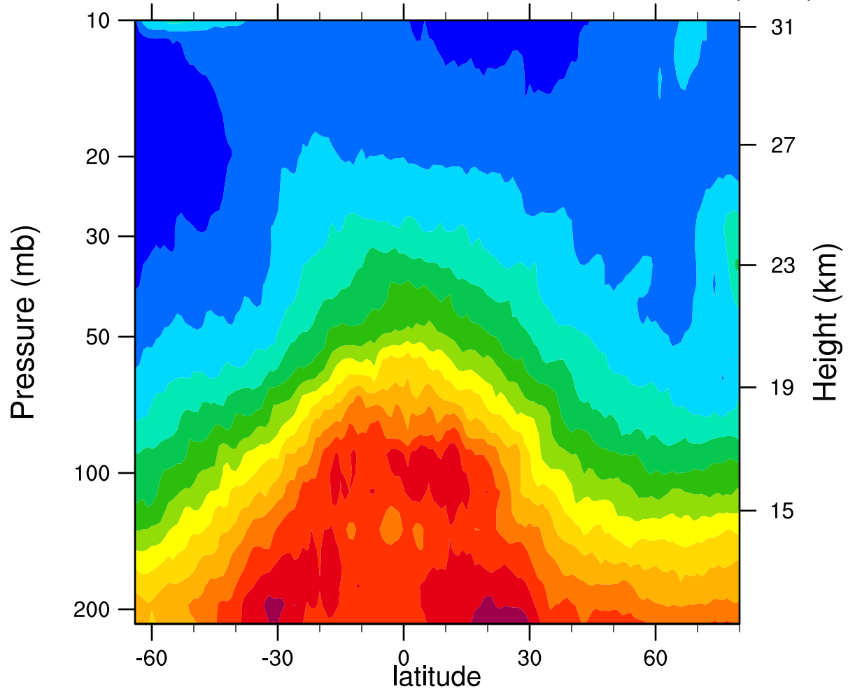
2005d359 12.1MicronExtinction_Combined (km -1 )
