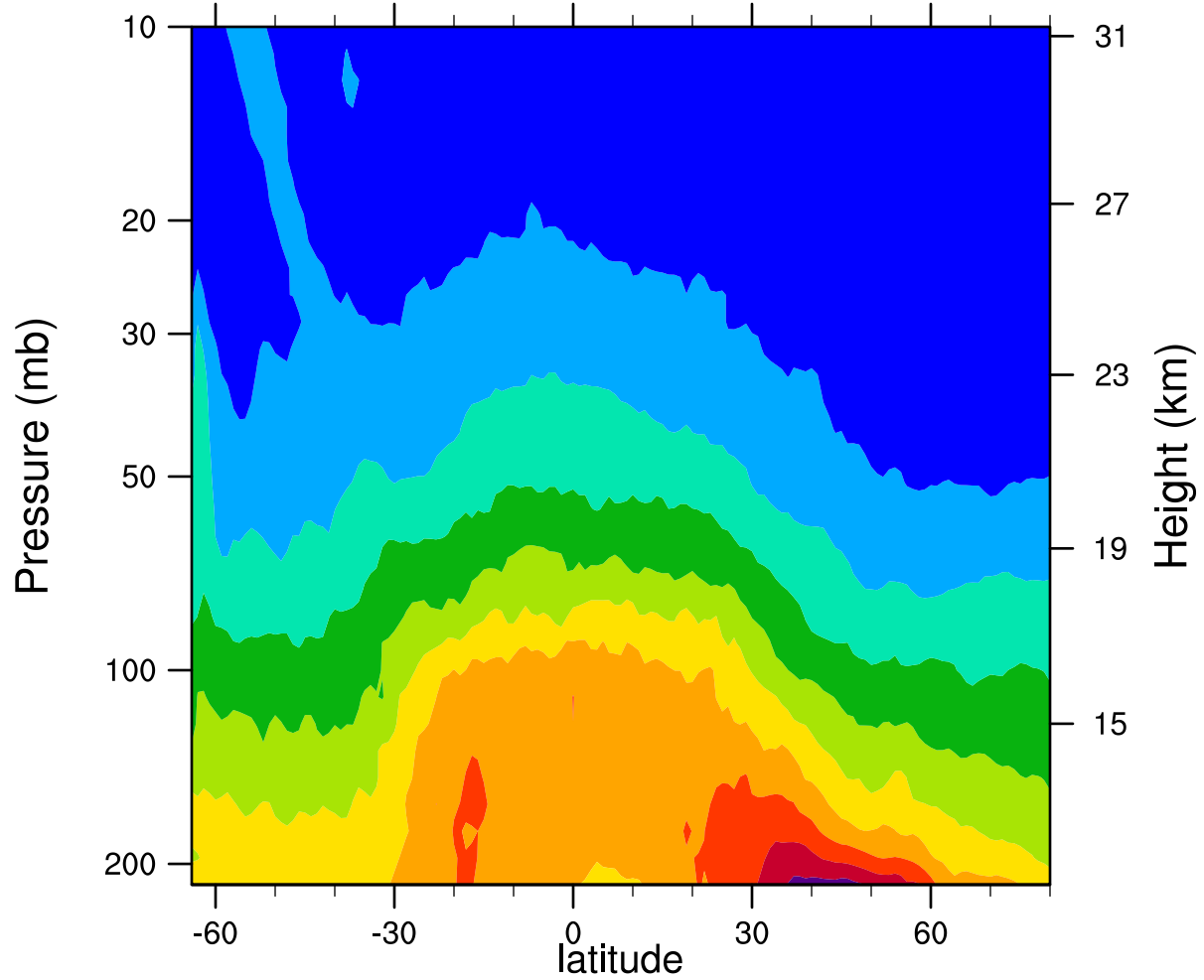
2007d169 12.1MicronExtinction_Combined (km -1 )
