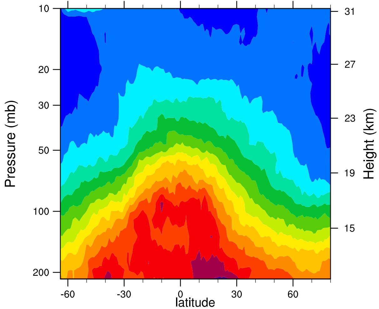
2006d022 12.1MicronExtinction_Combined ( \text{km}^{-1} )
