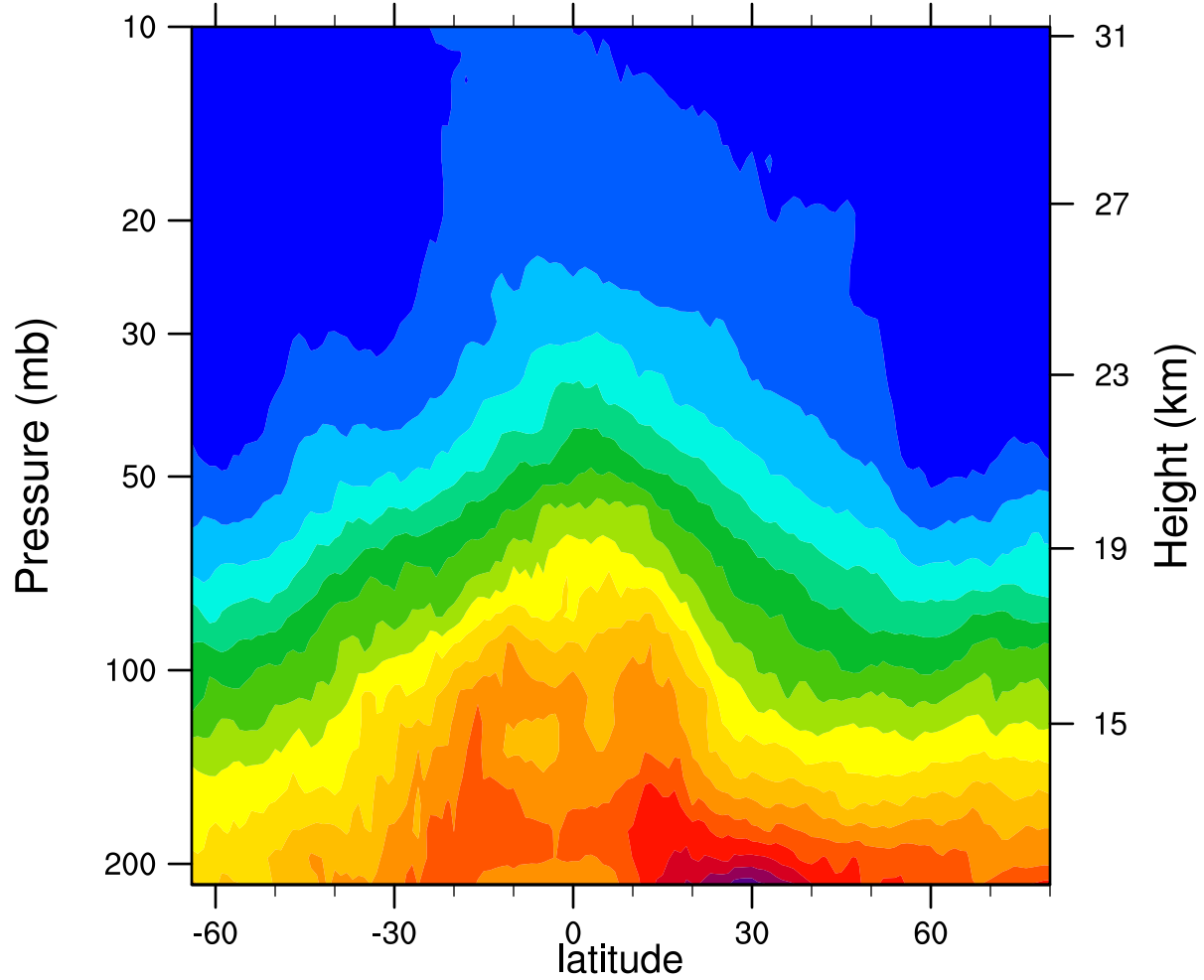
2007d099 12.1MicronExtinction_Combined (km -1 )
