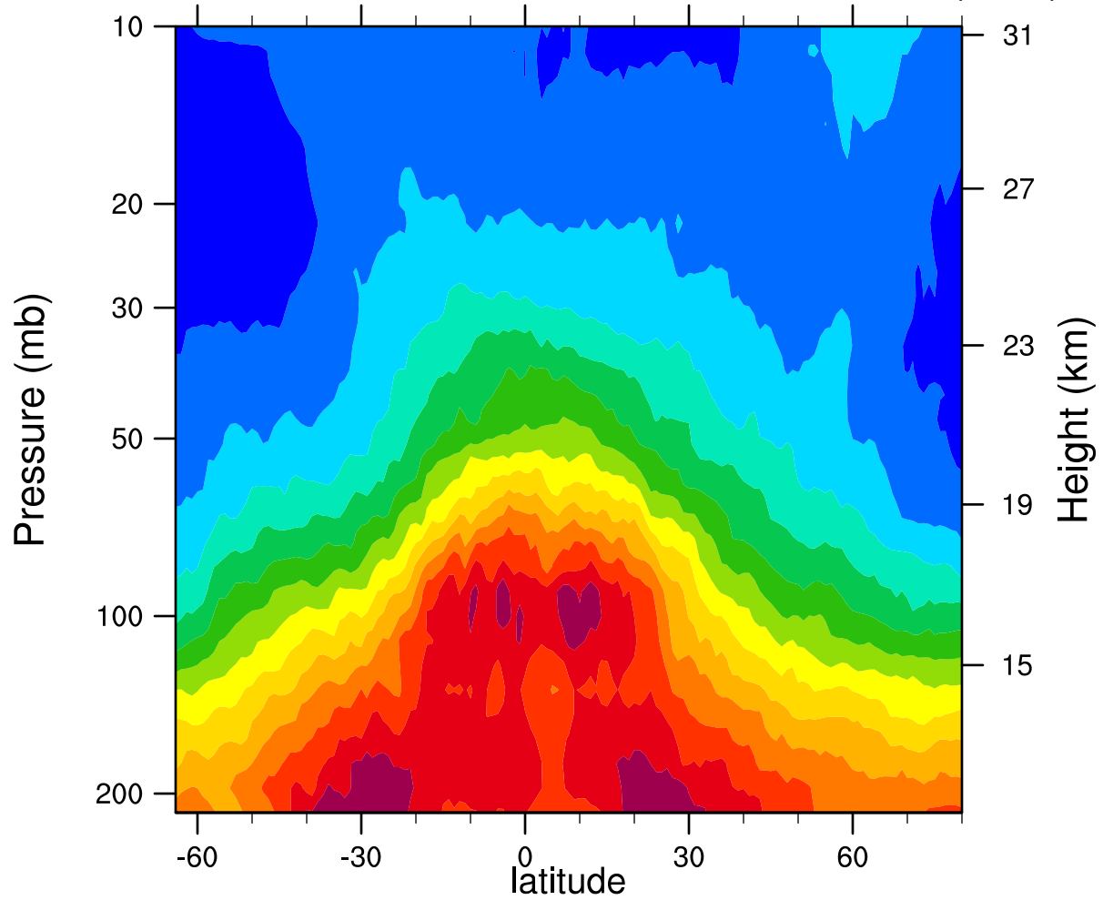
2005d322 12.1MicronExtinction_Combined (km -1 )
