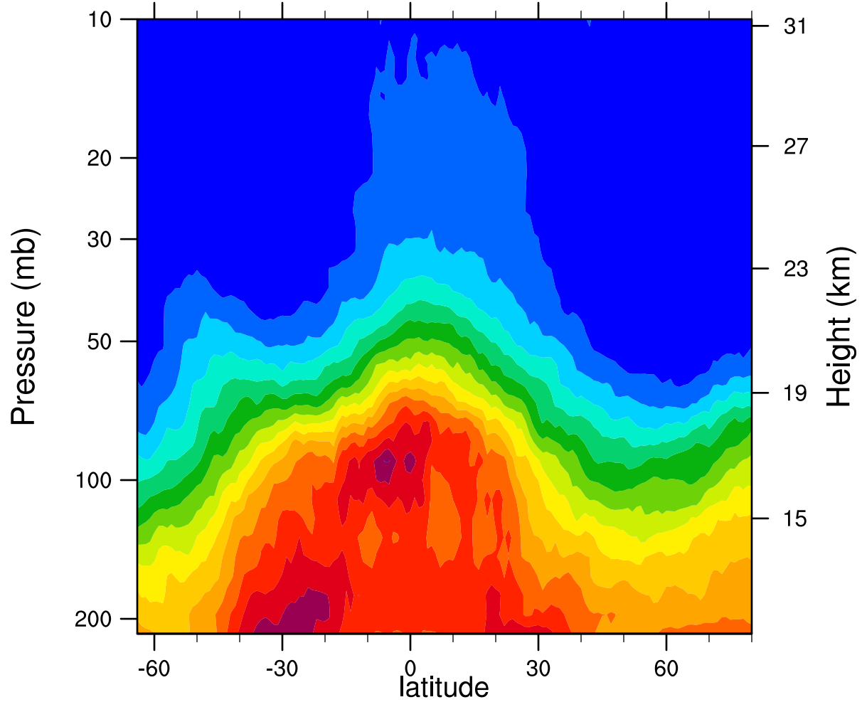
2006d338 12.1MicronExtinction_Combined ( \text{km}^{-1} )
