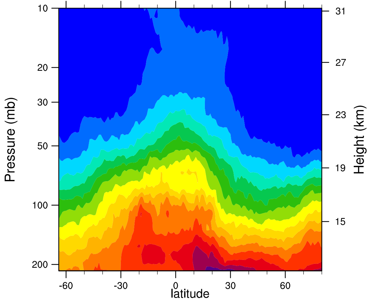
2007d083 12.1MicronExtinction_Combined (km -1 )
