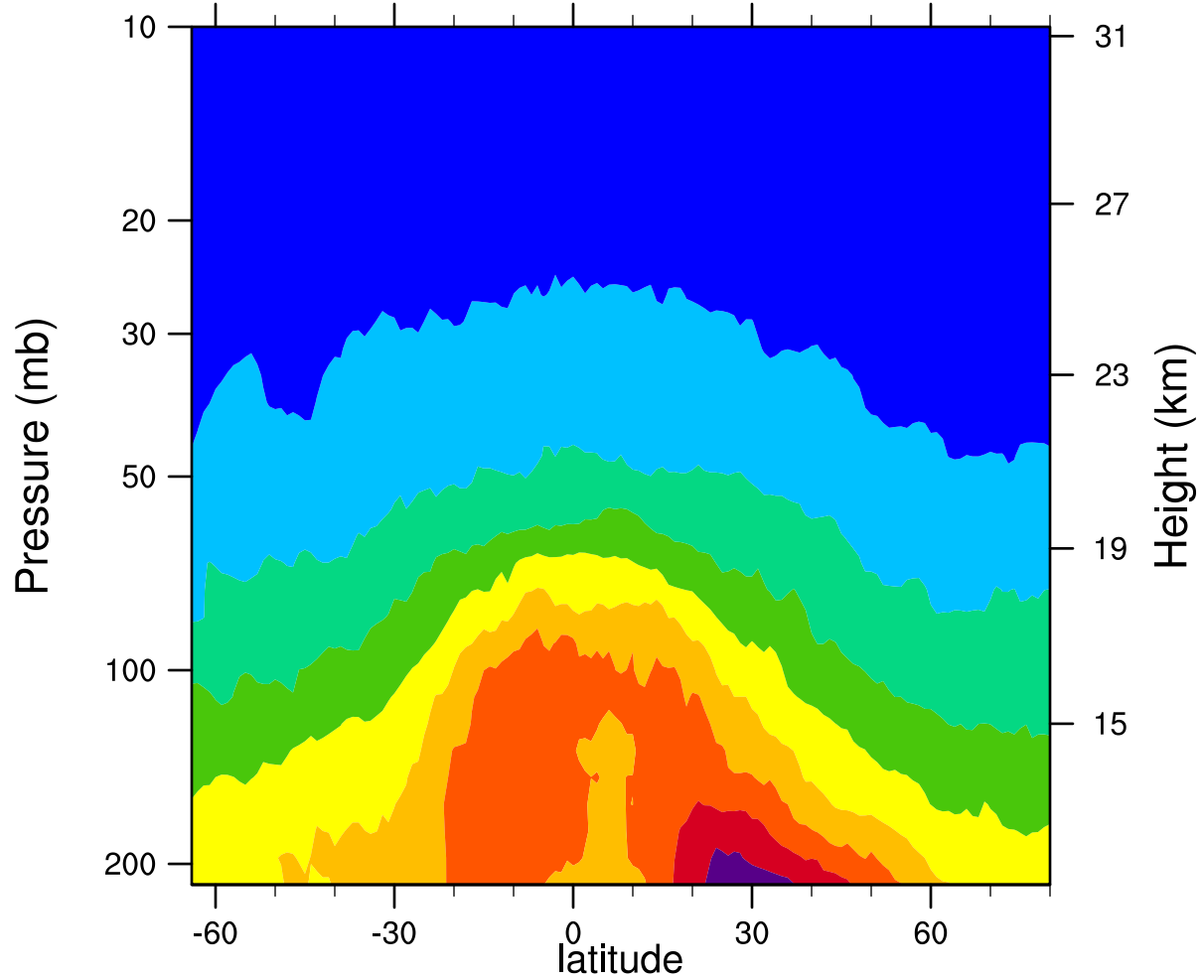
2006d136 12.1MicronExtinction_Combined (km -1 )
