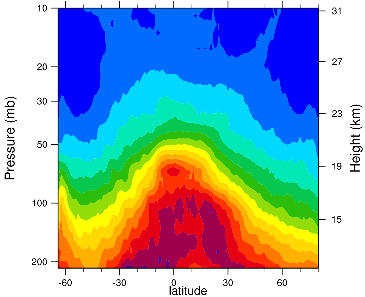
2006d270 12.1MicronExtinction_Combined (km -1 )
