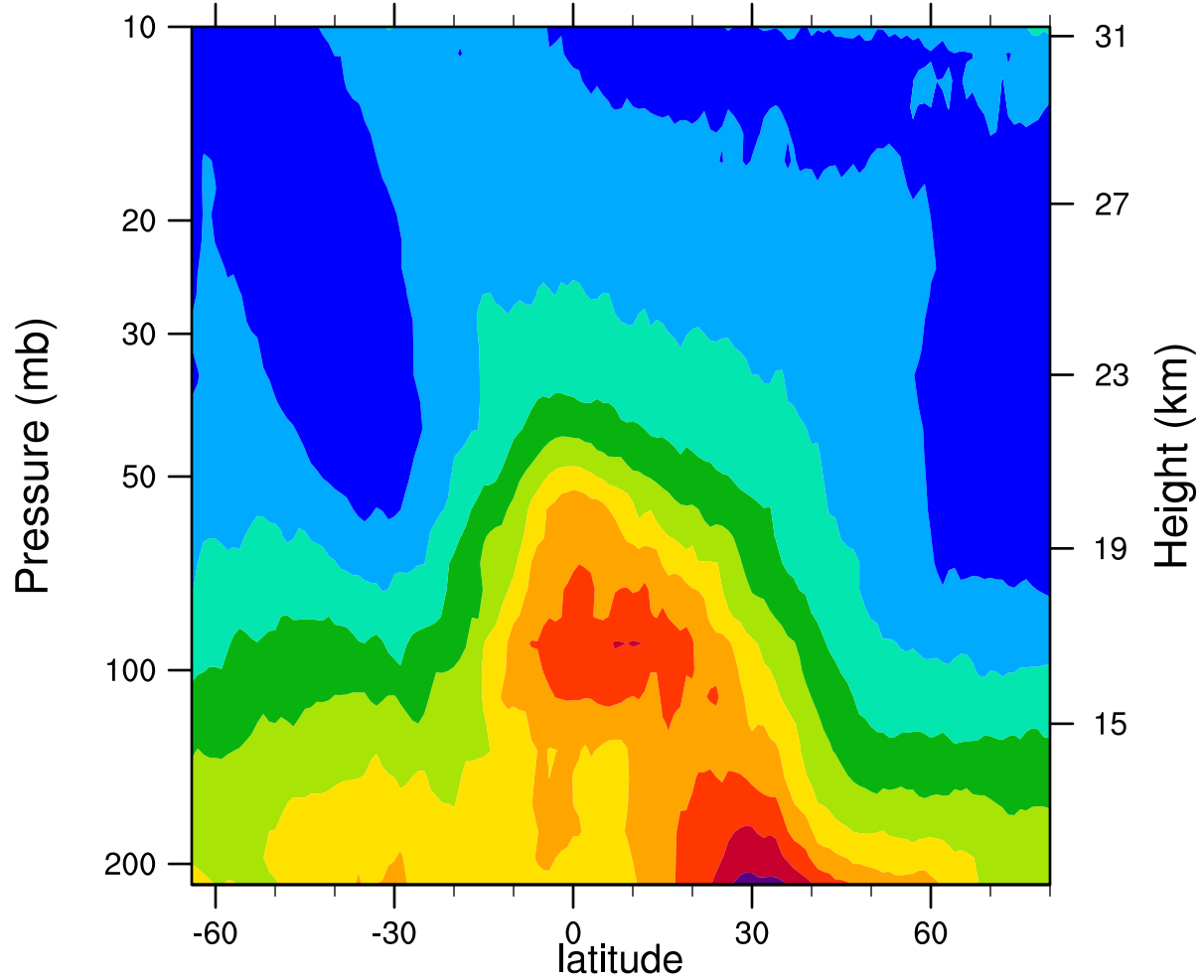
2005d140 12.1MicronExtinction_Combined (km -1 )
