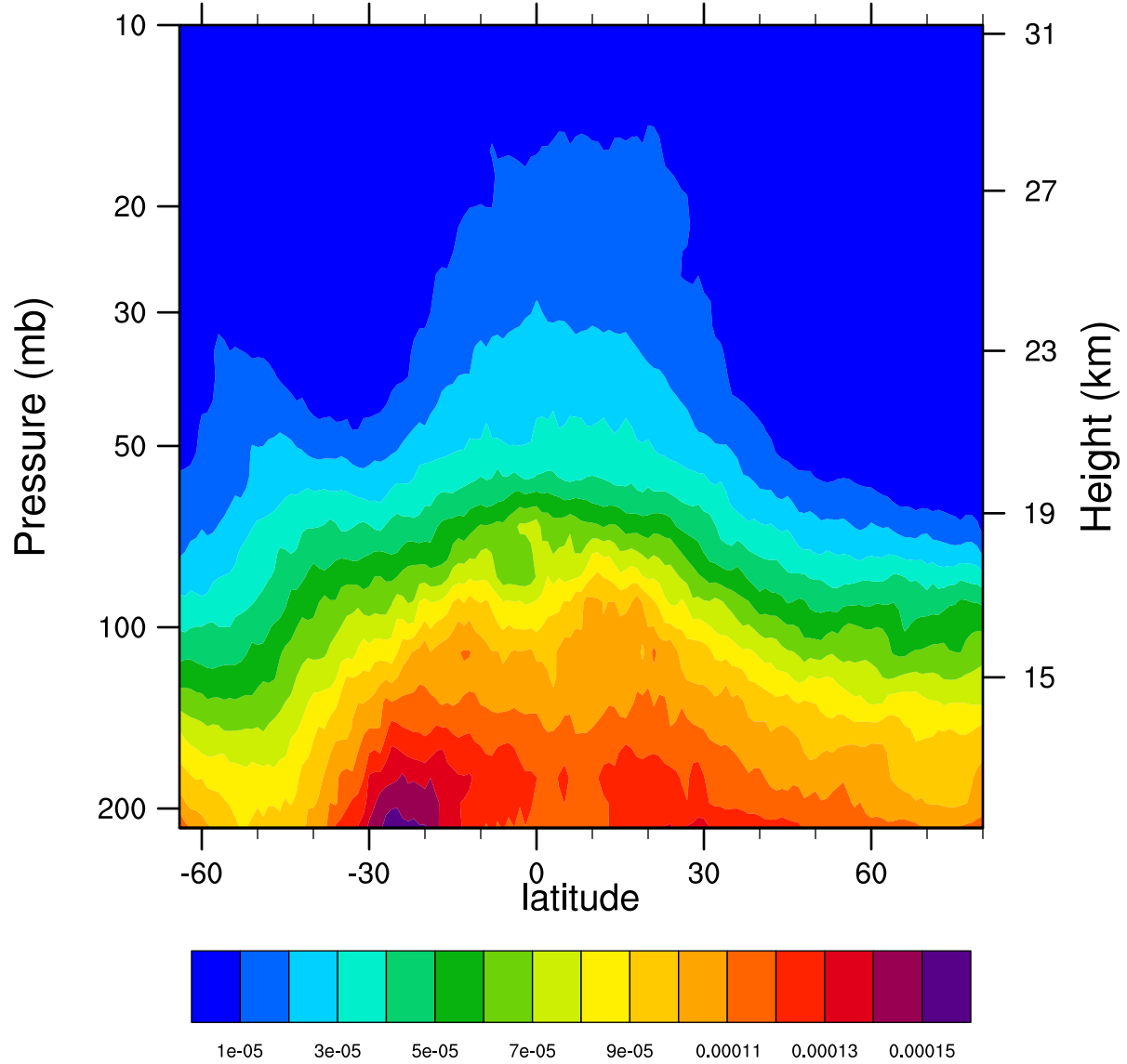
2007d310 12.1MicronExtinction_Combined (km -1 )
