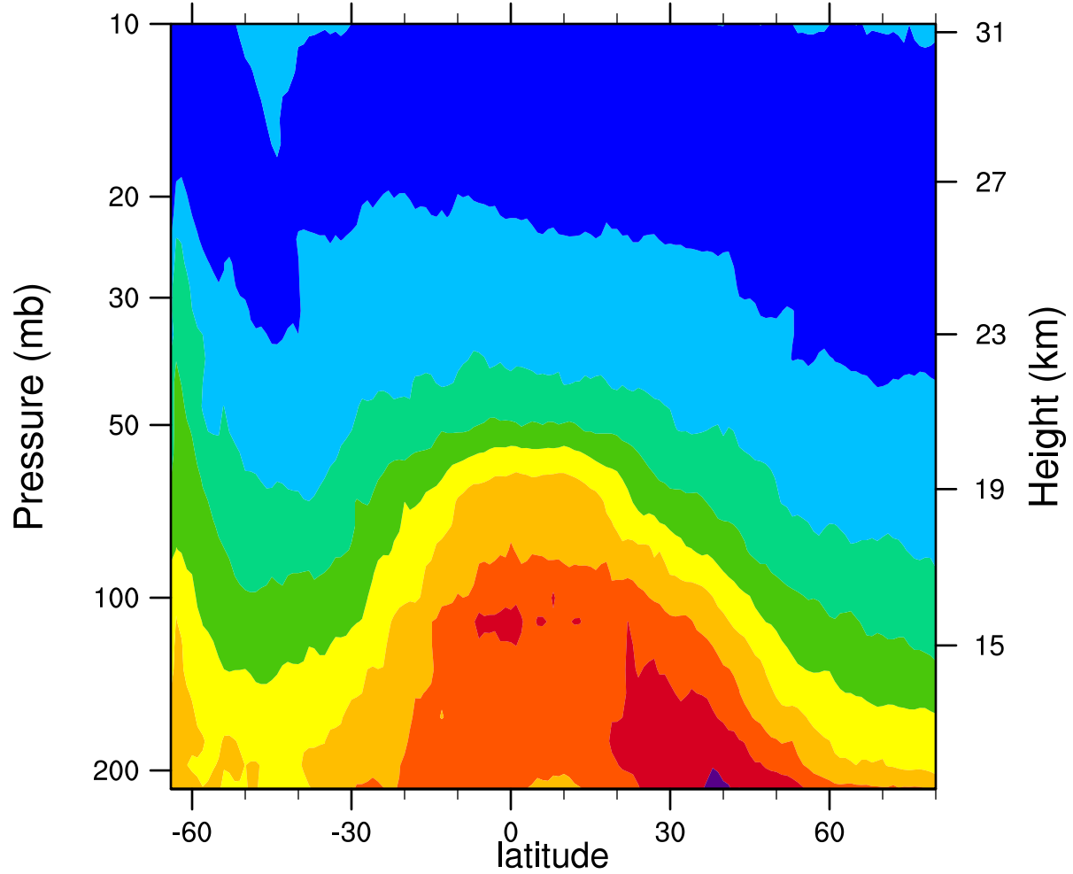
2006d217 12.1MicronExtinction_Combined ( \text{km}^{-1} )
