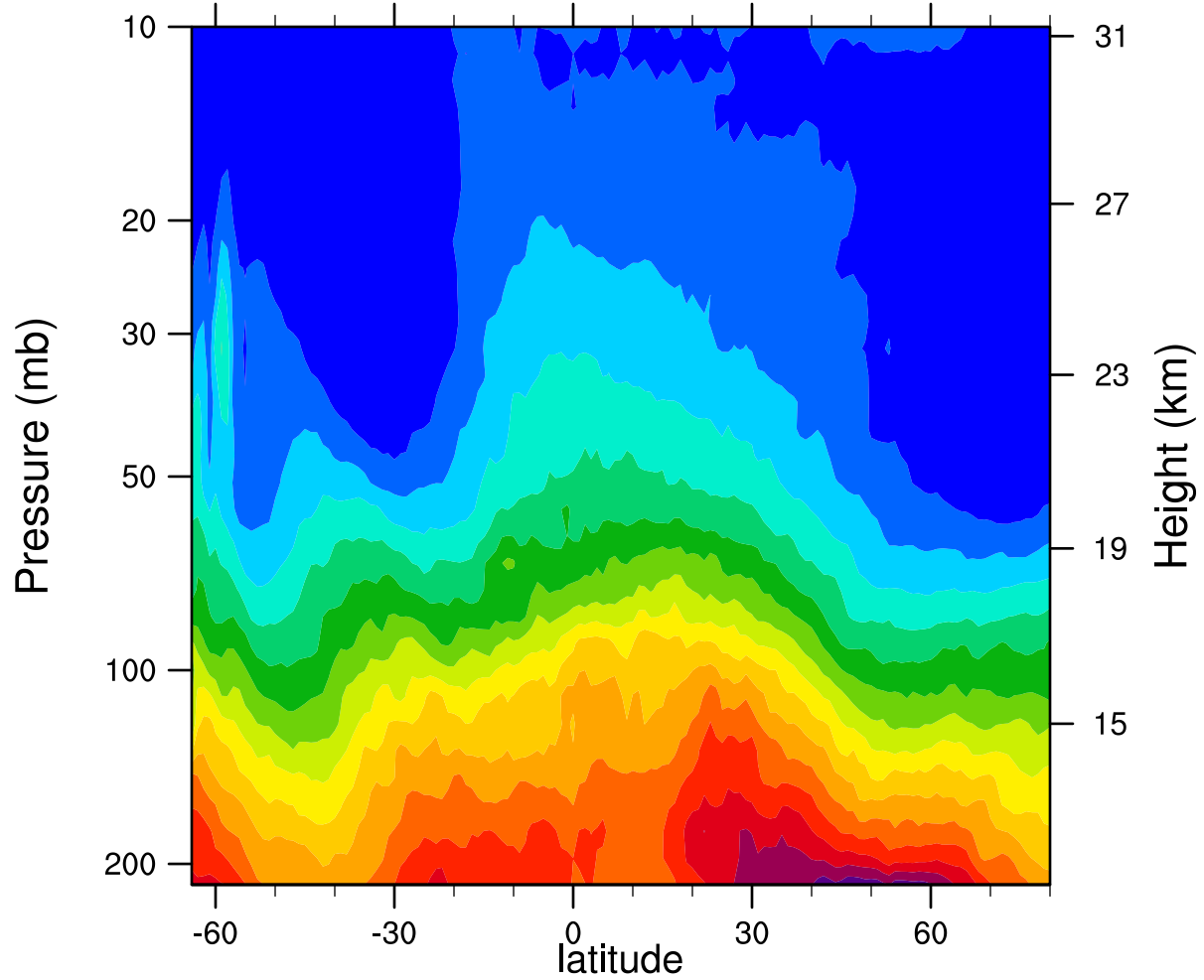
2007d230 12.1MicronExtinction_Combined (km -1 )
