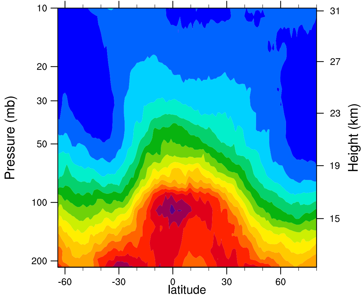
2005d262 12.1MicronExtinction_Combined (km -1 )
