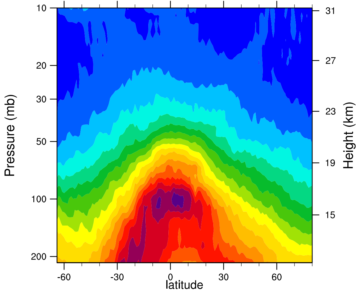
2006d299 12.1MicronExtinction_Combined ( \text{km}^{-1} )
