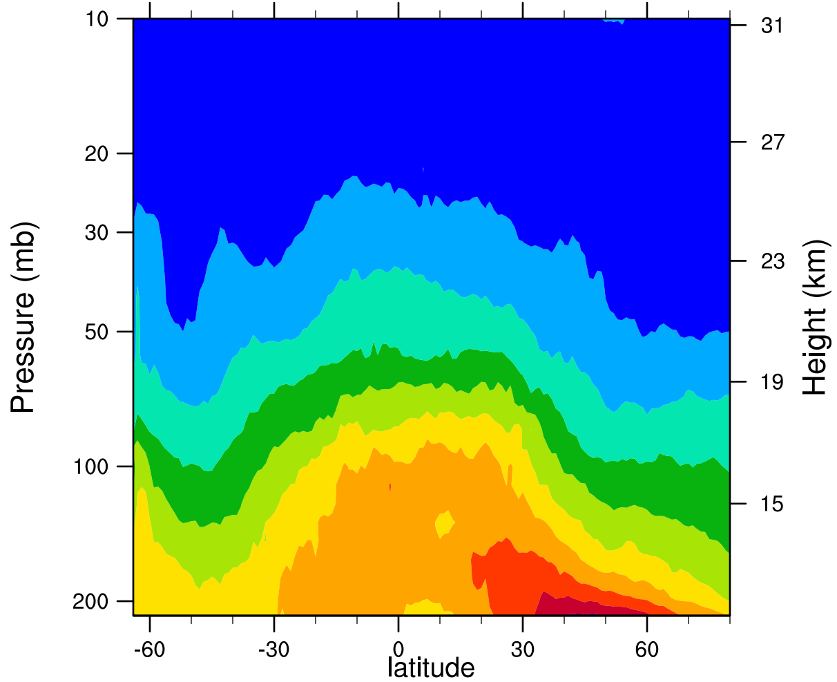
2007d193 12.1MicronExtinction_Combined ( \text{km}^{-1} )
