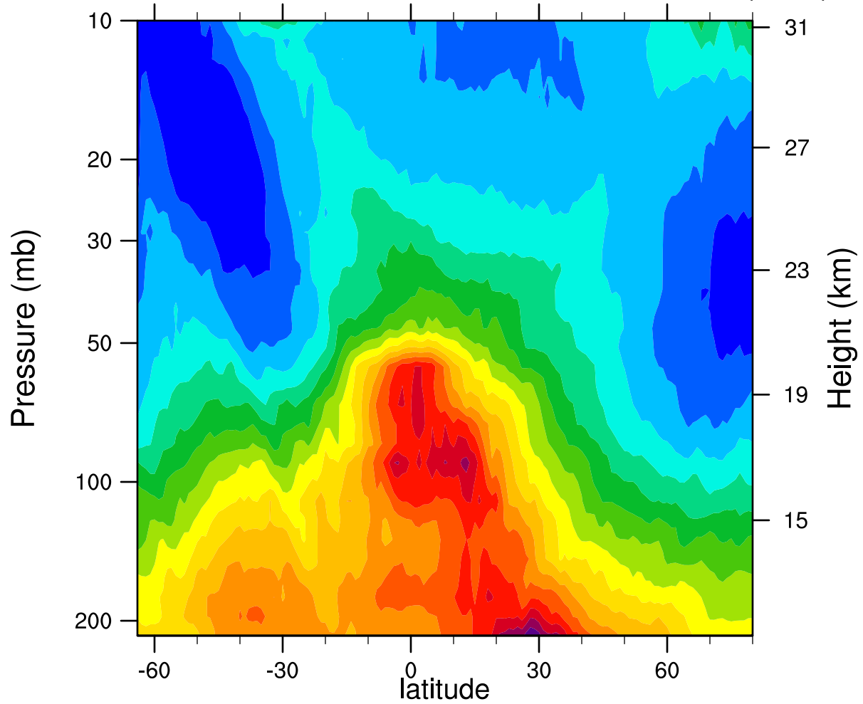
2005d102 12.1MicronExtinction_Combined (km -1 )
