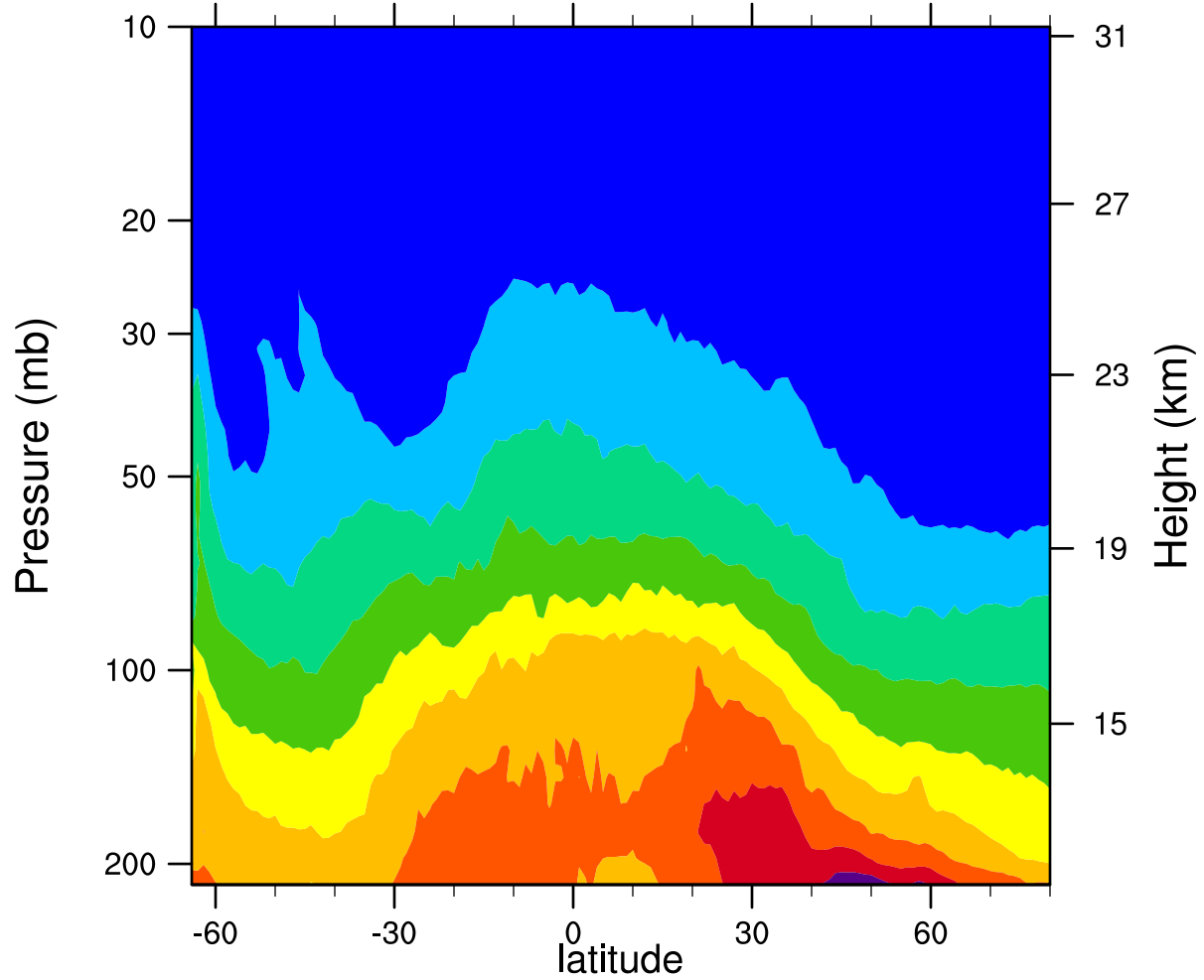
2007d208 12.1MicronExtinction_Combined (km -1 )
