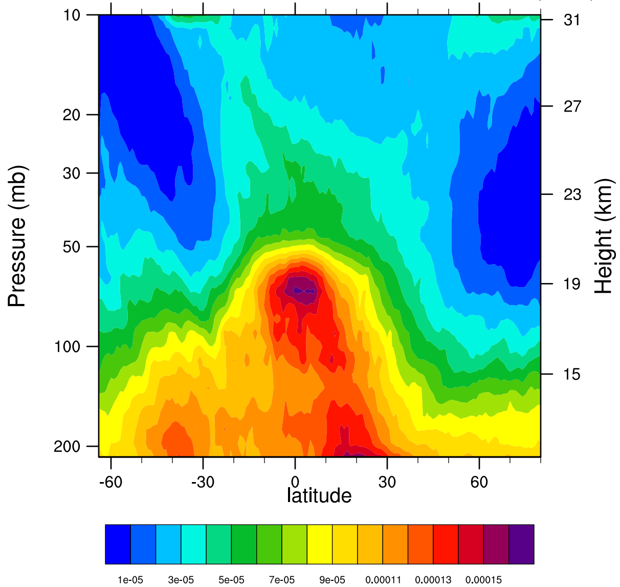
2005d074 12.1MicronExtinction_Combined (km -1 )
