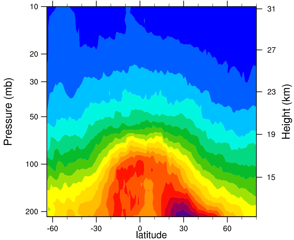
2006d142 12.1MicronExtinction_Combined (km -1 )
