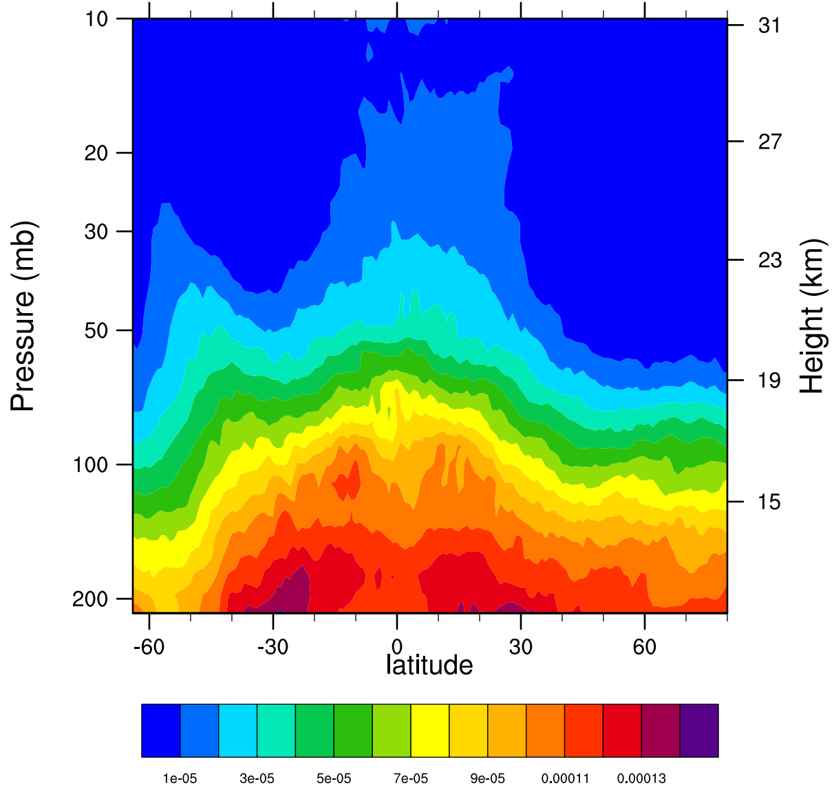
2007d326 12.1MicronExtinction_Combined (km -1 )
