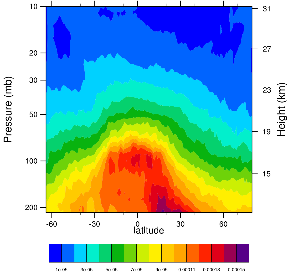
2006d088 12.1MicronExtinction_Combined ( \text{km}^{-1} )
