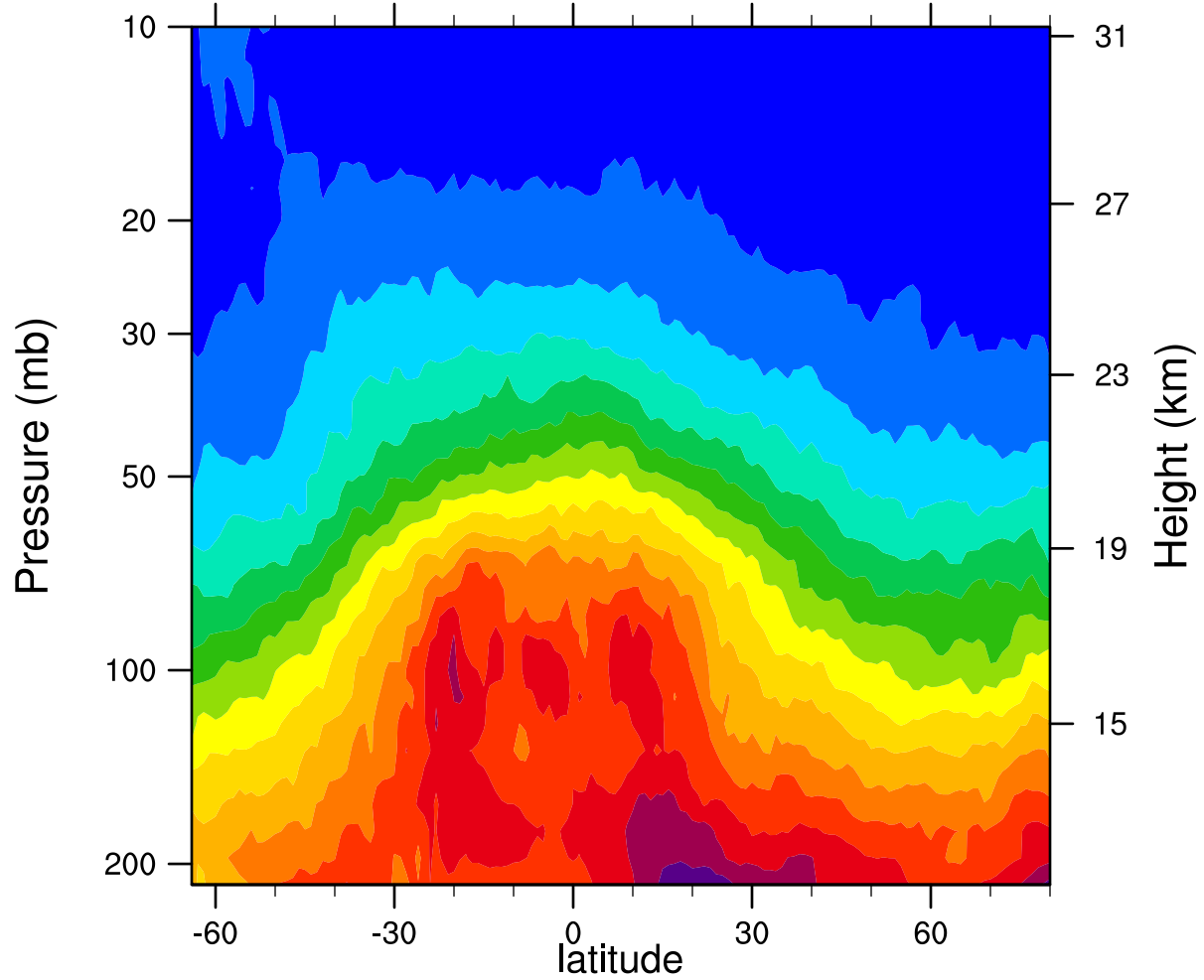
2007d071 12.1MicronExtinction_Combined (km -1 )
