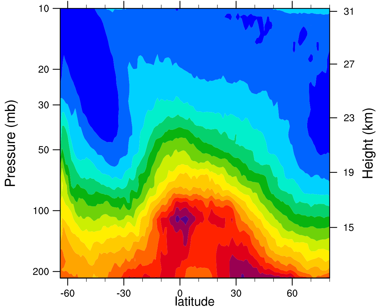
2005d218 12.1MicronExtinction_Combined (km -1 )
