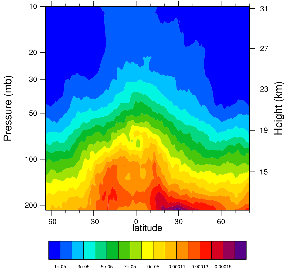
2007d105 12.1MicronExtinction_Combined ( \text{km}^{-1} )
