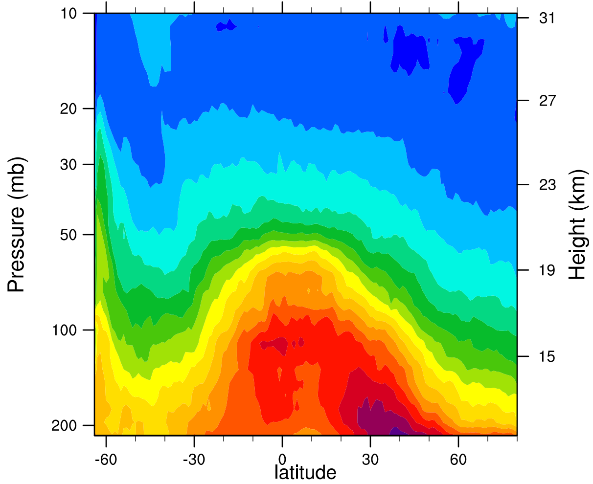
2006d215 12.1MicronExtinction_Combined (km -1 )
