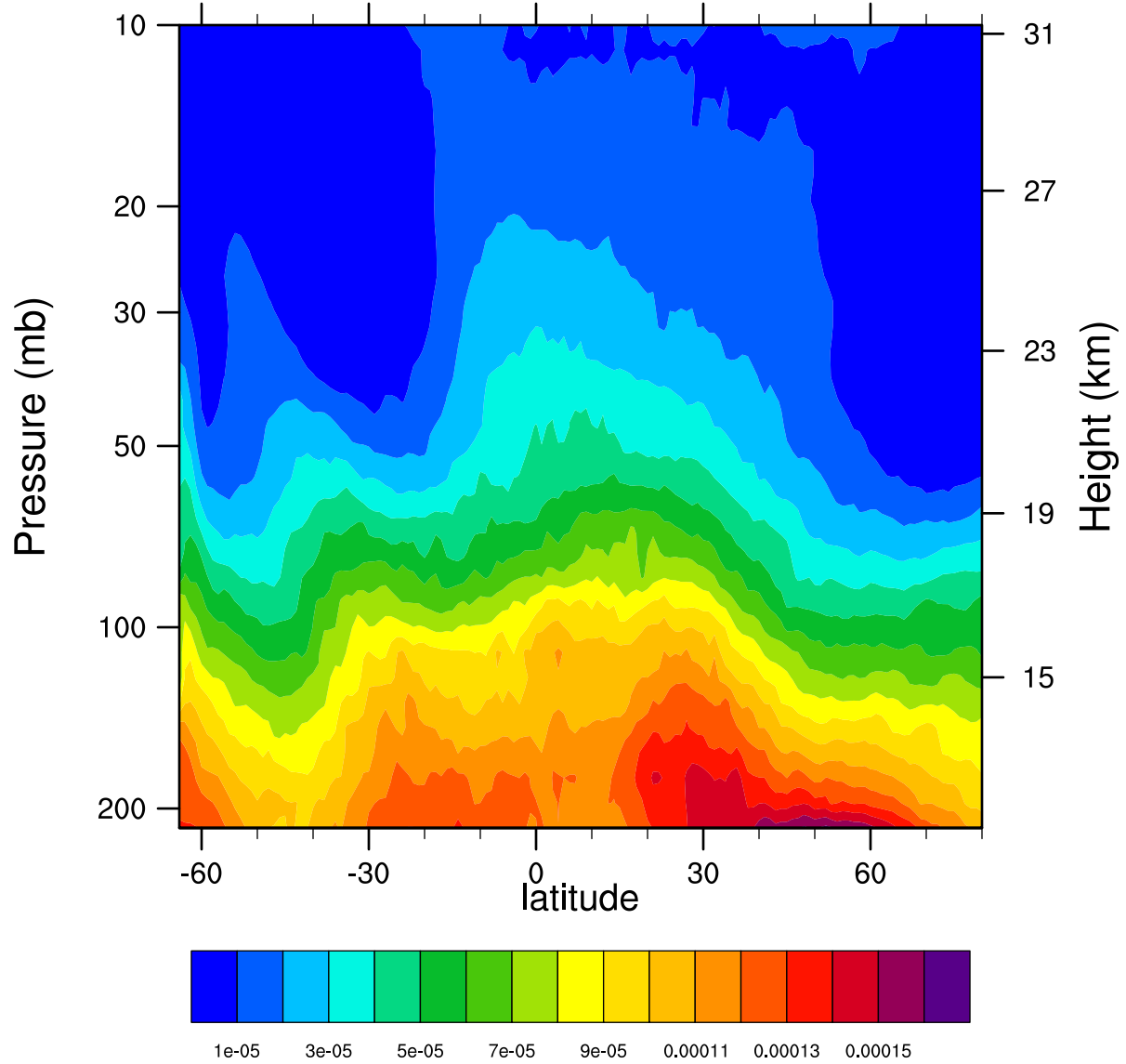
2007d223 12.1MicronExtinction_Combined ( \text{km}^{-1} )
