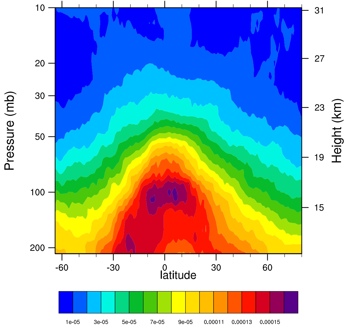
2006d296 12.1MicronExtinction_Combined (km -1 )
