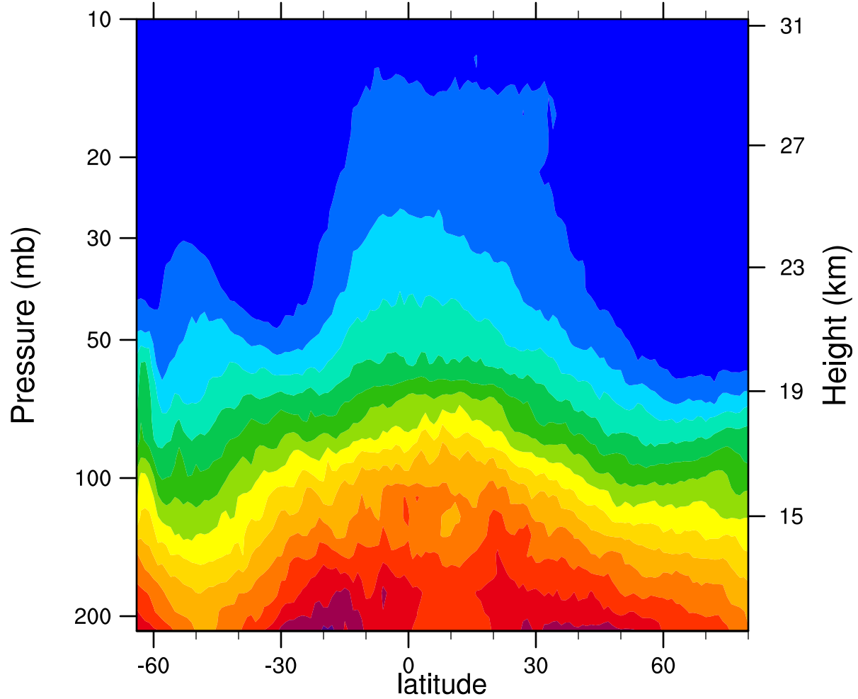
2007d267 12.1MicronExtinction_Combined (km -1 )
