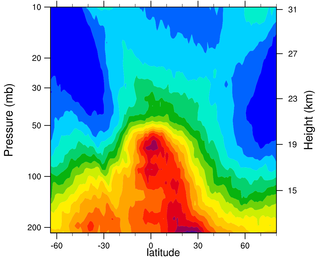
2005d089 12.1MicronExtinction_Combined (km -1 )
