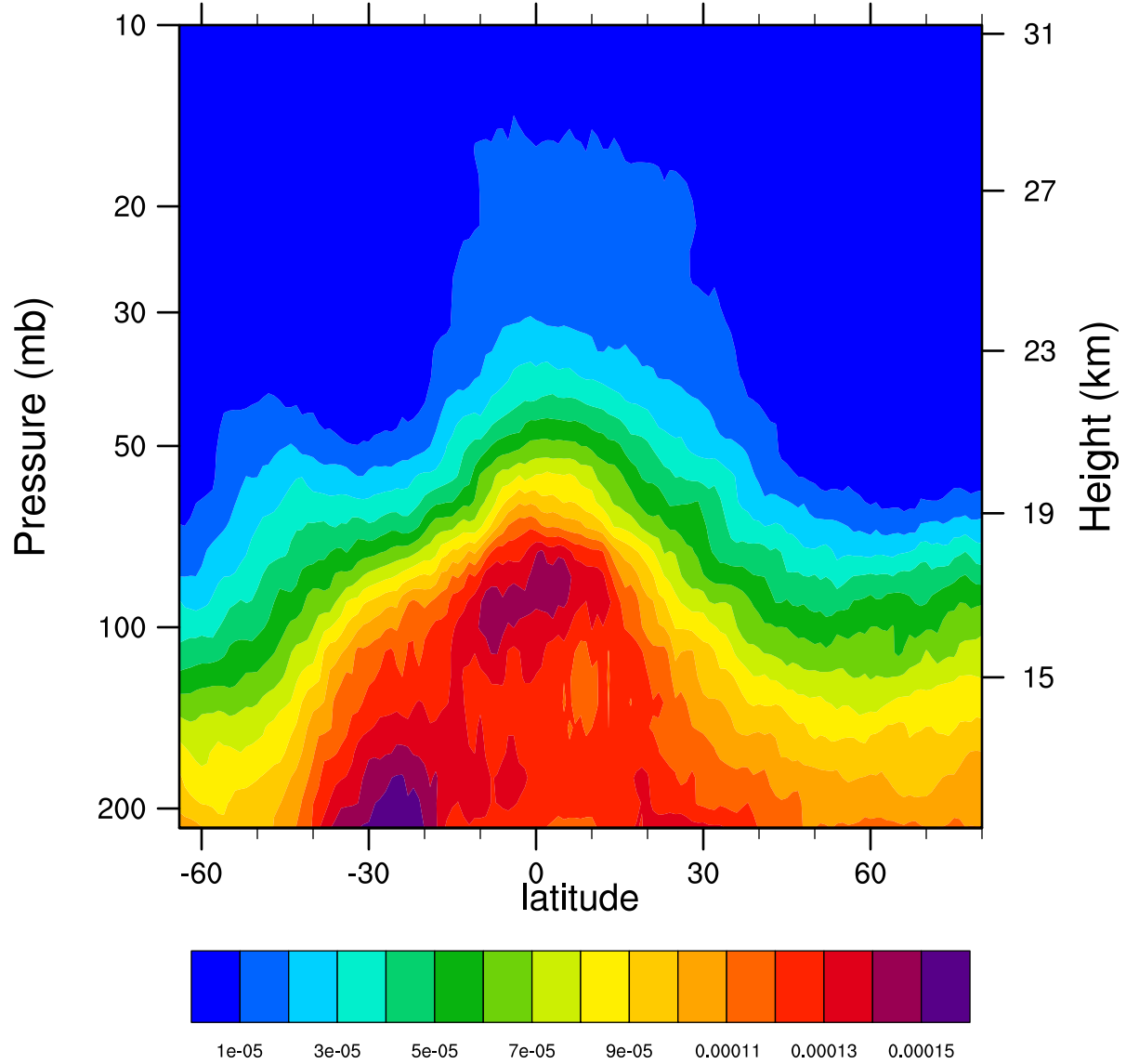
2006d327 12.1MicronExtinction_Combined (km -1 )
