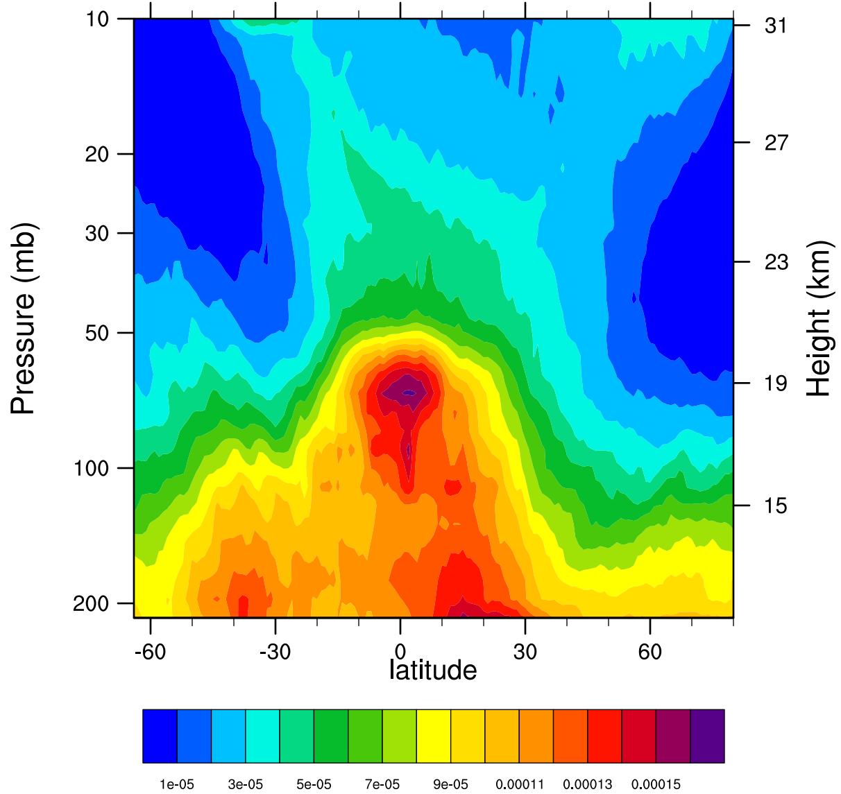
2005d069 12.1MicronExtinction_Combined (km -1 )
