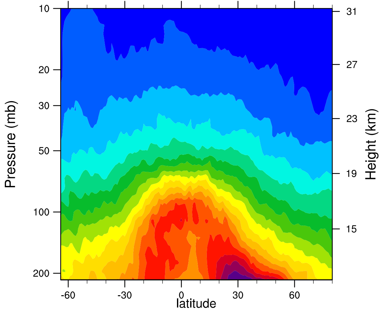
2006d146 12.1MicronExtinction_Combined (km -1 )
