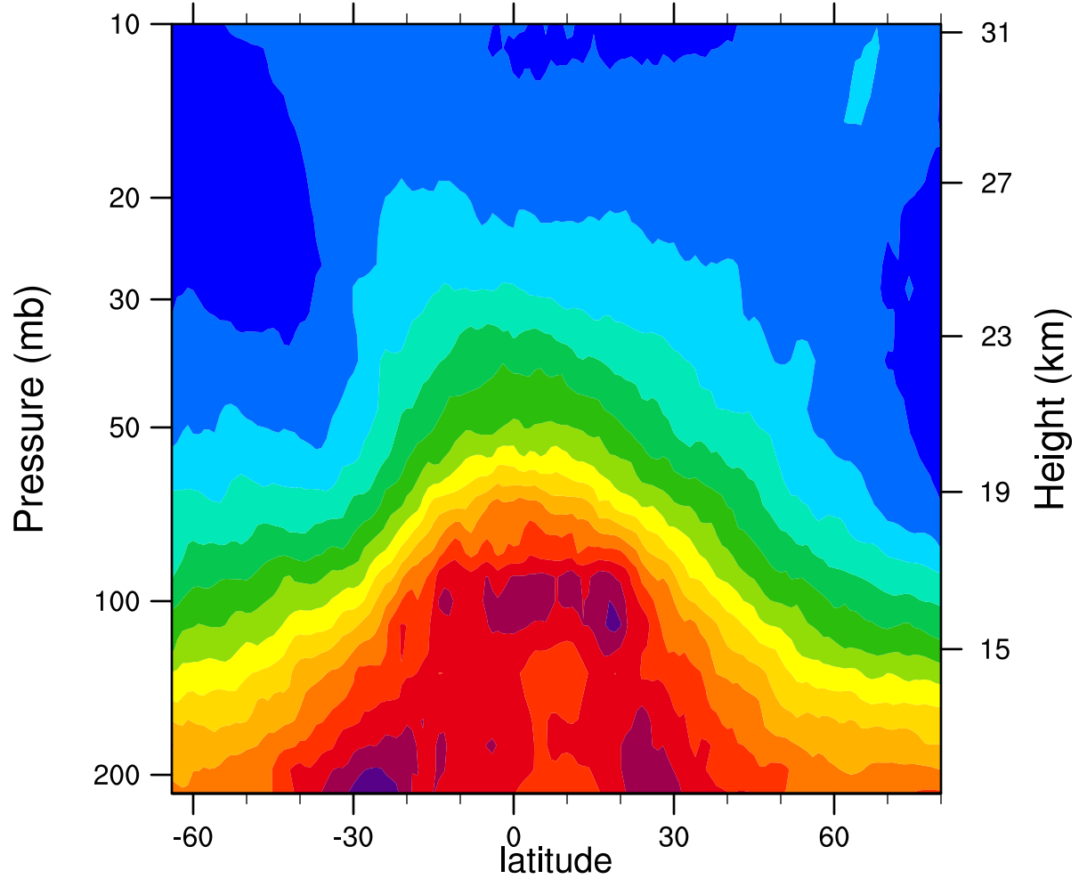
2005d306 12.1MicronExtinction_Combined (km -1 )
