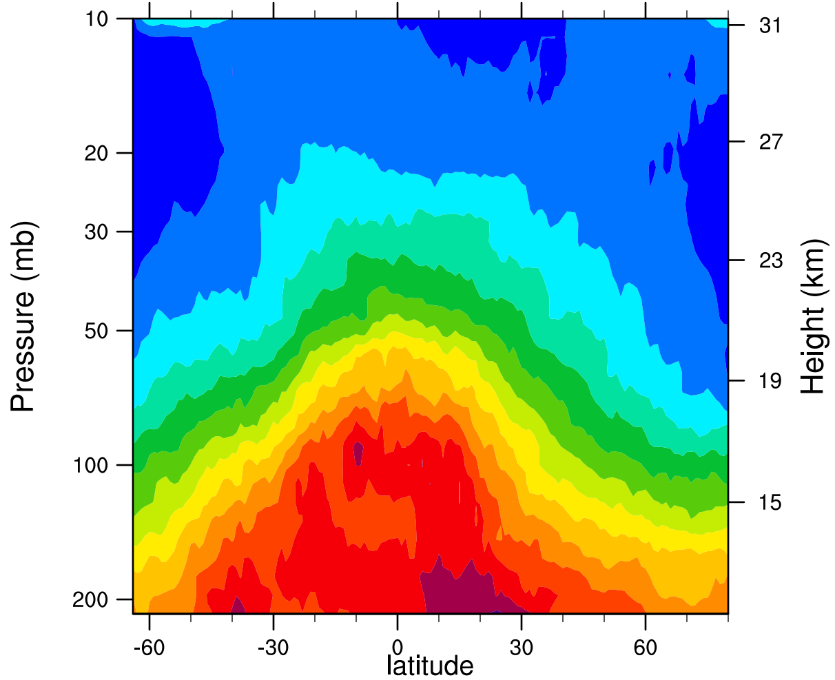
2006d023 12.1MicronExtinction_Combined (km -1 )
