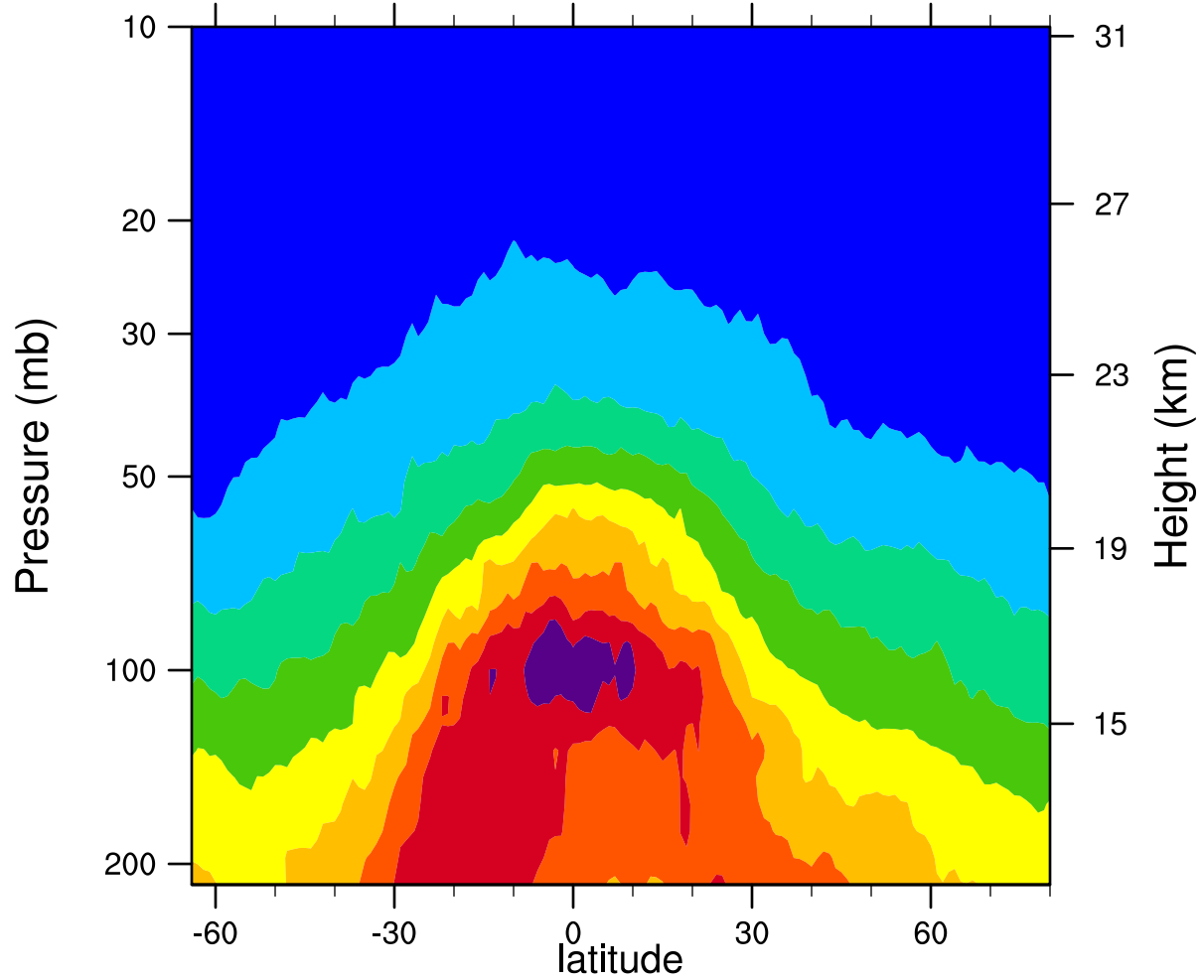
2006d306 12.1MicronExtinction_Combined (km -1 )
