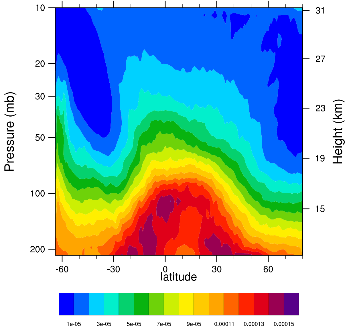
2005d236 12.1MicronExtinction_Combined (km -1 )
