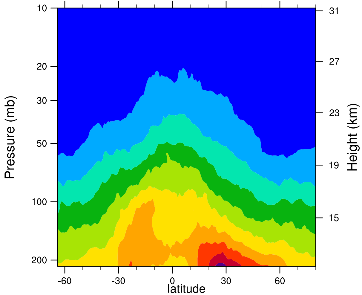
2007d116 12.1MicronExtinction_Combined (km -1 )
