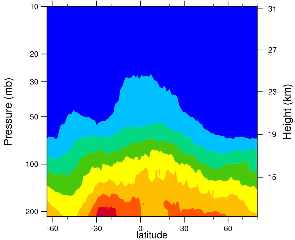
2007d279 12.1MicronExtinction_Combined (km -1 )
