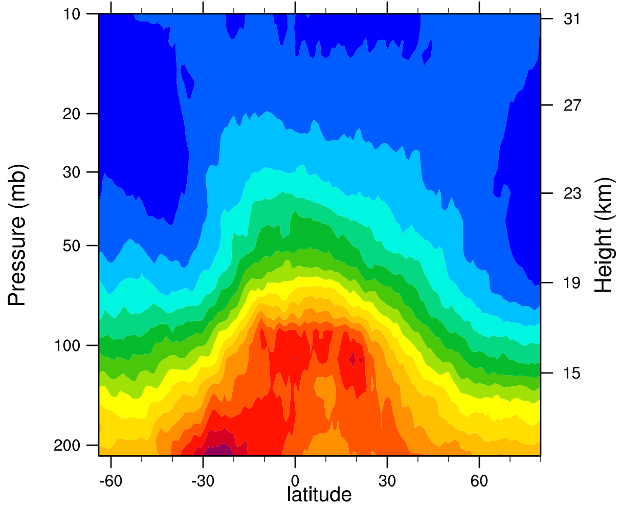
2005d291 12.1MicronExtinction_Combined (km -1 )
