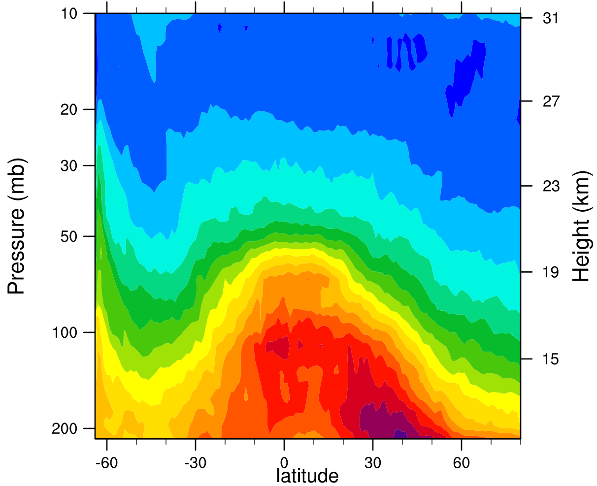
2006d218 12.1MicronExtinction_Combined (km -1 )
