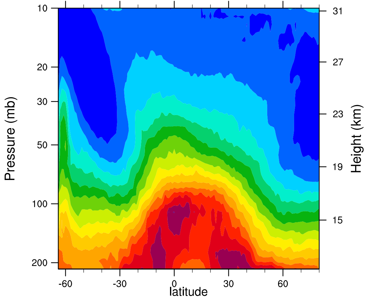
2005d231 12.1MicronExtinction_Combined (km -1 )
