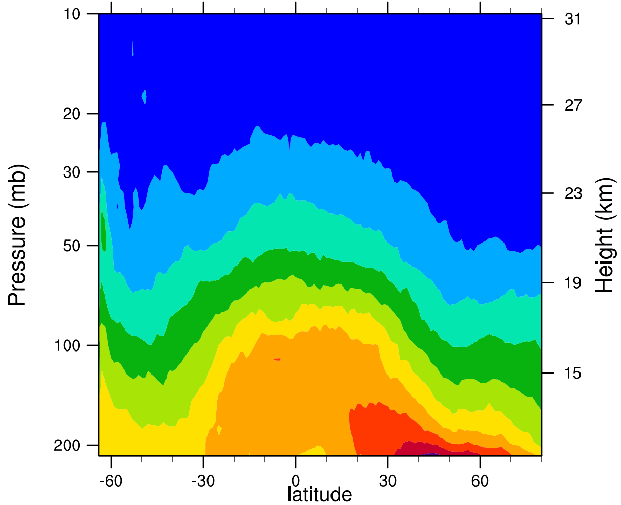
2007d182 12.1MicronExtinction_Combined (km -1 )
