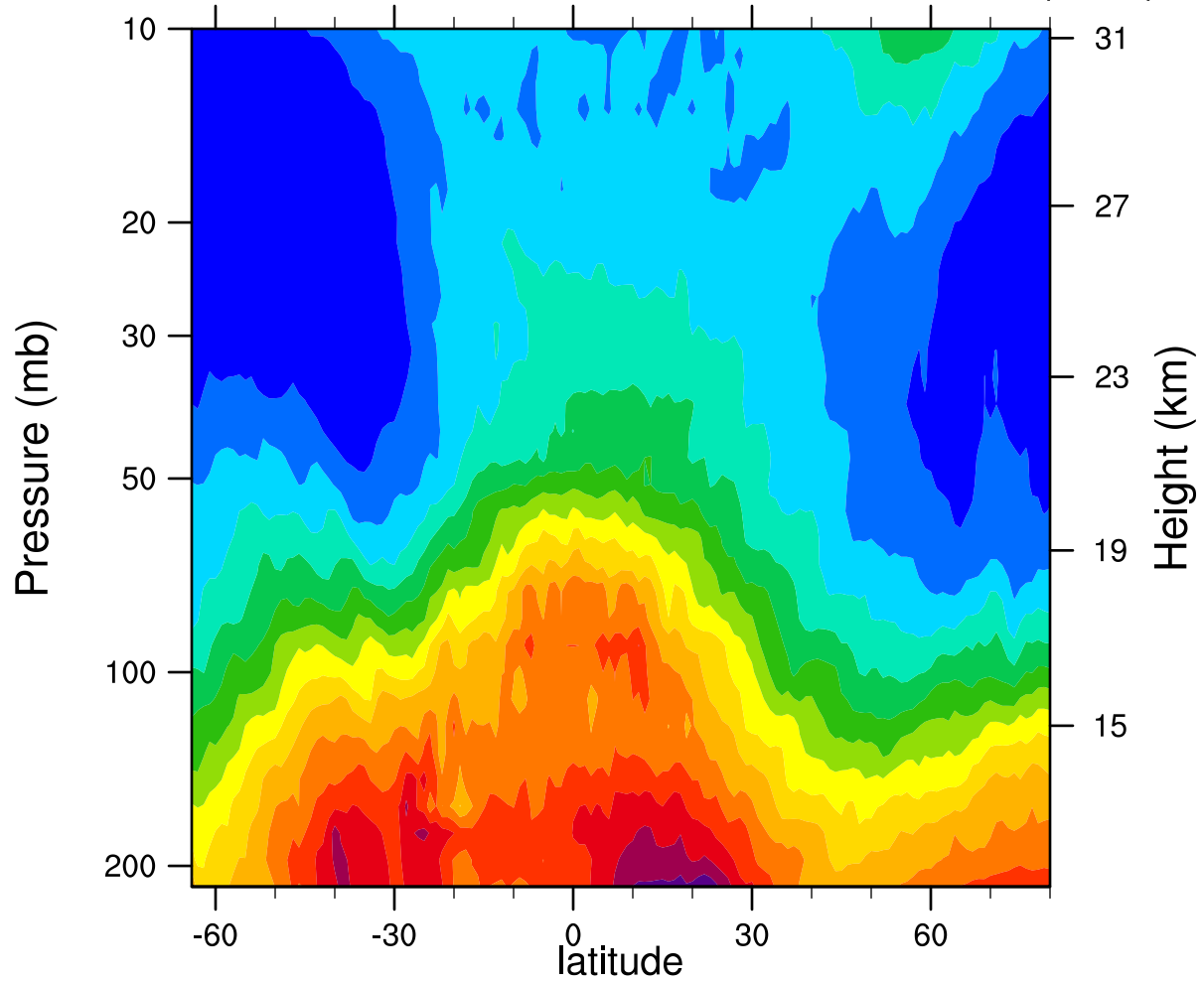
2005d033 12.1MicronExtinction_Combined (km -1 )
