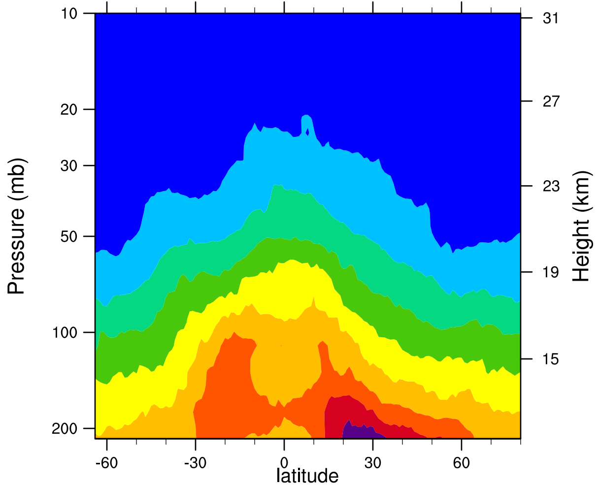
2007d111 12.1MicronExtinction_Combined (km -1 )
