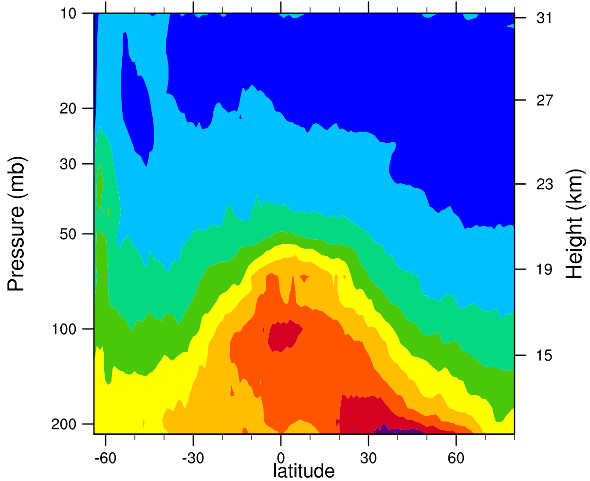
2006d182 12.1MicronExtinction_Combined (km -1 )
