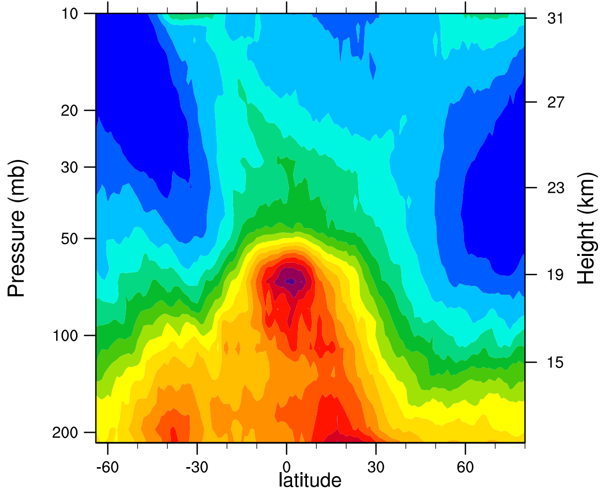
2005d072 12.1MicronExtinction_Combined (km -1 )
