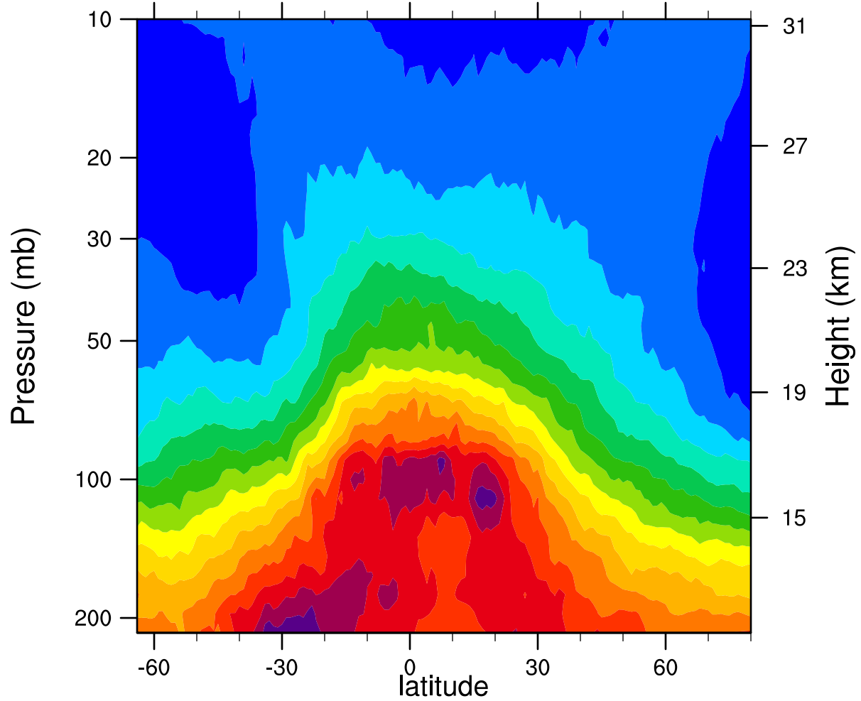
2005d300 12.1MicronExtinction_Combined ( \text{km}^{-1} )
