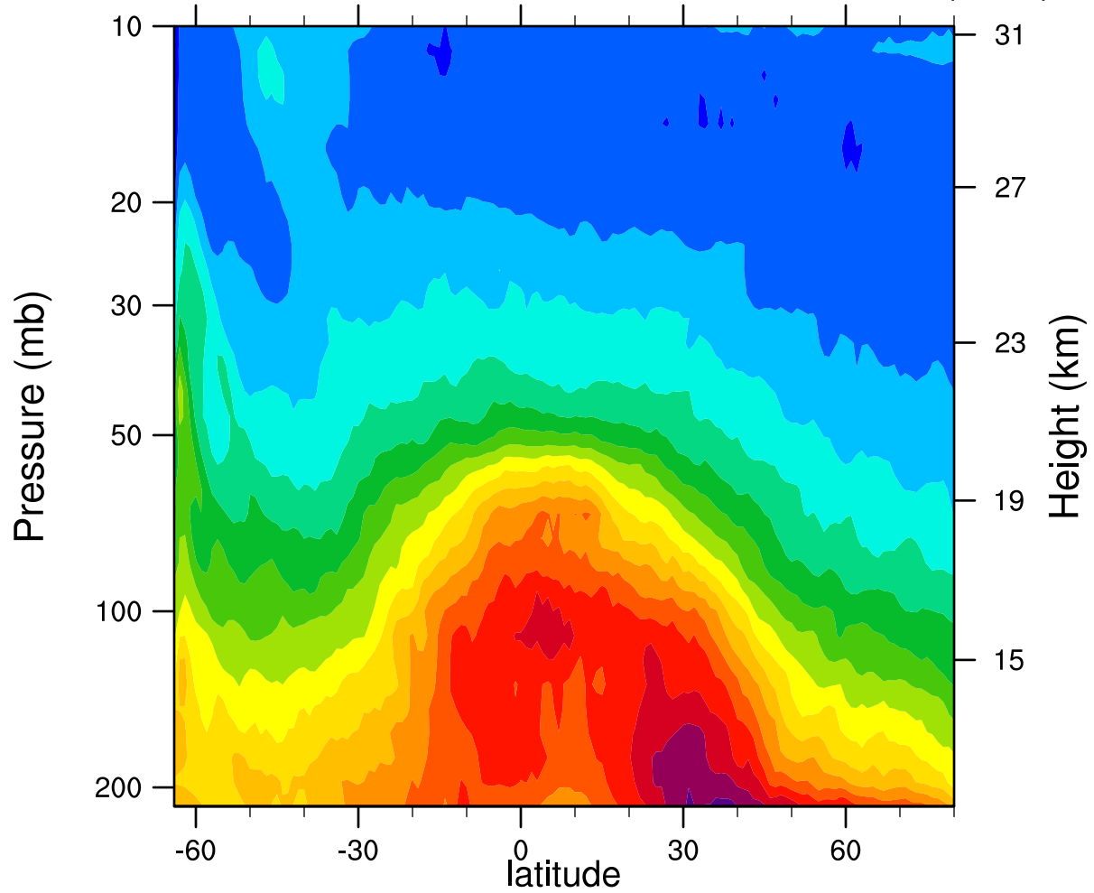
2006d205 12.1MicronExtinction_Combined (km -1 )
