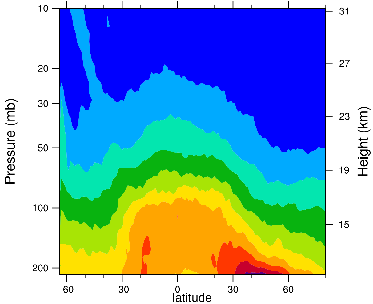
2007d170 12.1MicronExtinction_Combined (km -1 )
