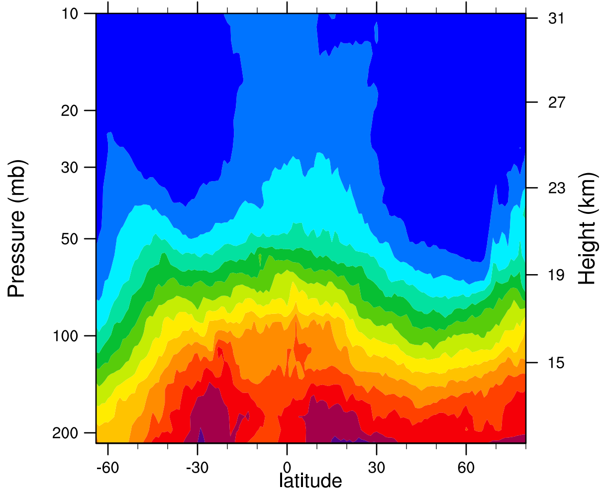
2007d359 12.1MicronExtinction_Combined (km -1 )
