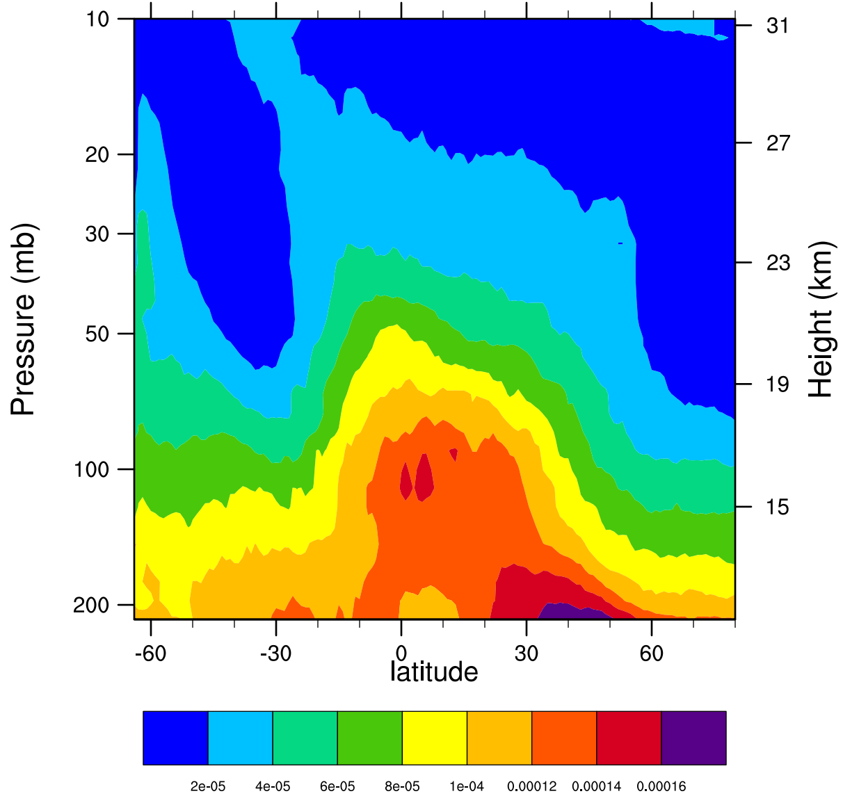
2005d179 12.1MicronExtinction_Combined (km -1 )
