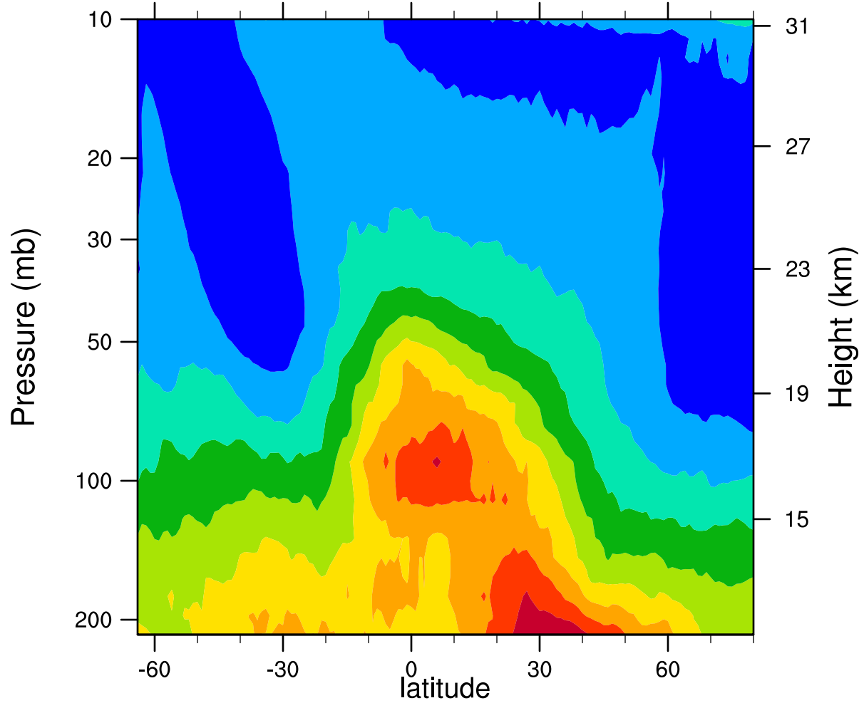
2005d148 12.1MicronExtinction_Combined (km -1 )
