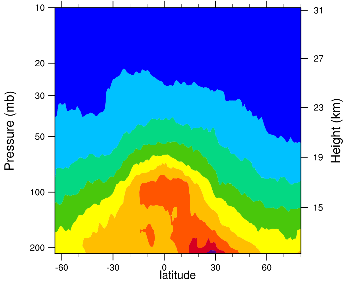
2006d097 12.1MicronExtinction_Combined (km -1 )
