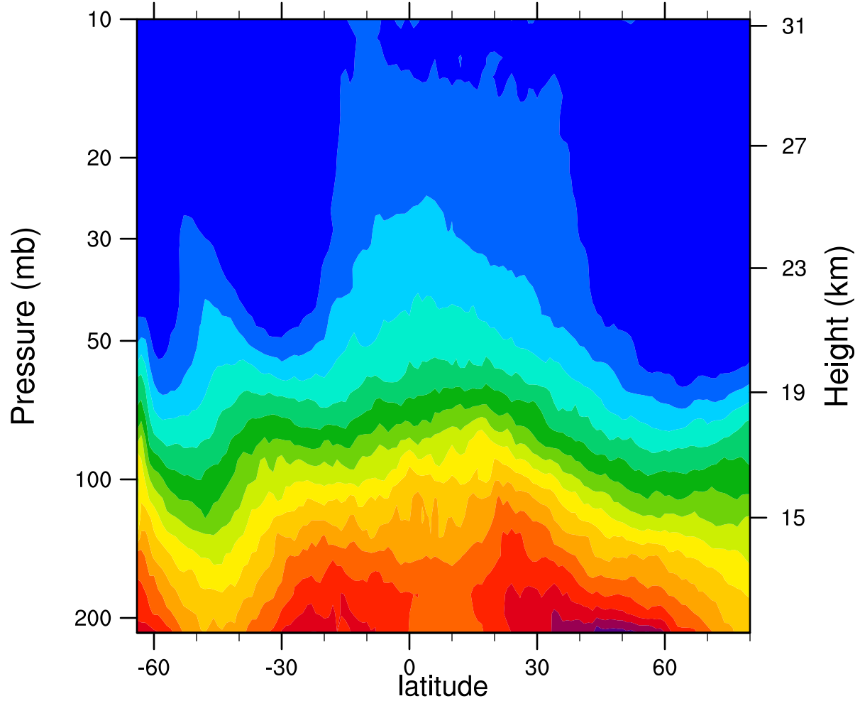
2007d245 12.1MicronExtinction_Combined (km -1 )
