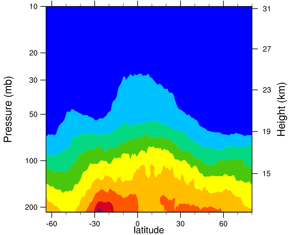
2007d280 12.1MicronExtinction_Combined (km -1 )
