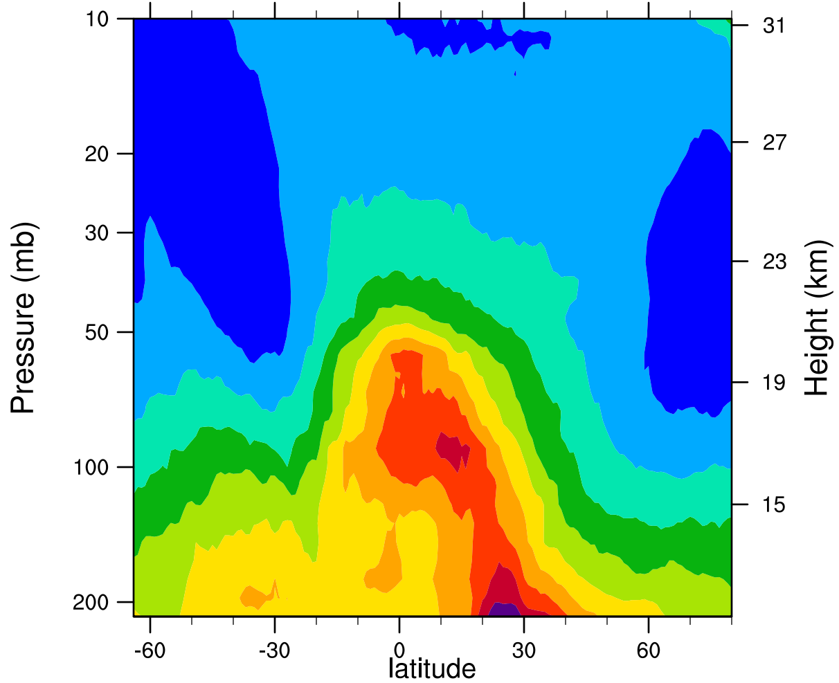
2005d121 12.1MicronExtinction_Combined (km -1 )
