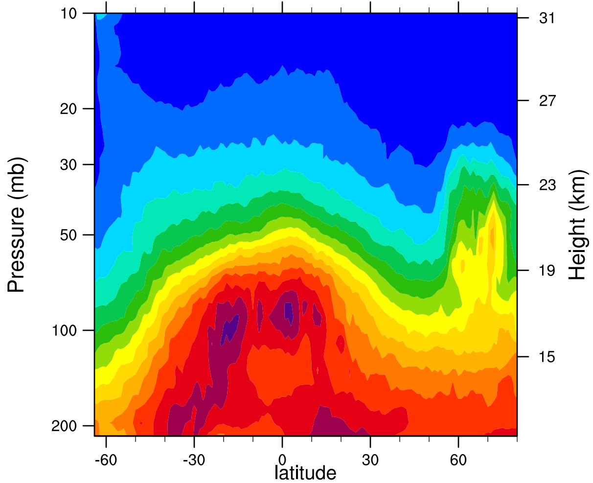
2007d024 12.1MicronExtinction_Combined ( \text{km}^{-1} )
