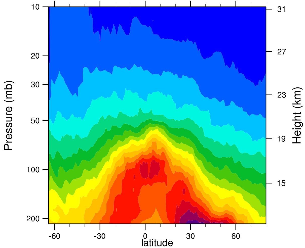
2006d159 12.1MicronExtinction_Combined (km -1 )
