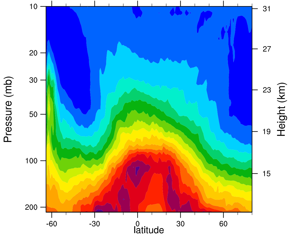
2005d246 12.1MicronExtinction_Combined (km -1 )
