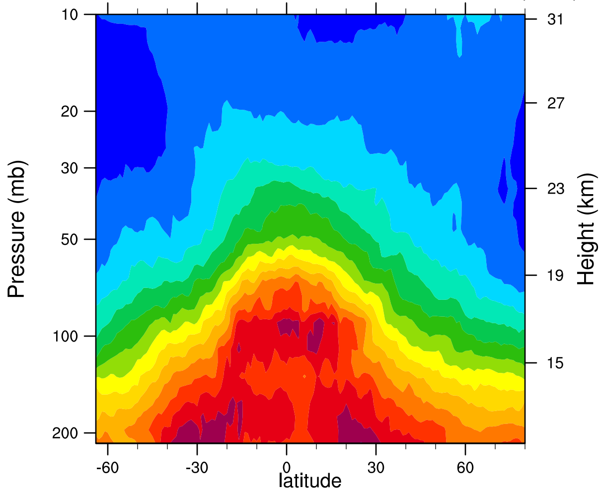
2005d331 12.1MicronExtinction_Combined ( \text{km}^{-1} )
