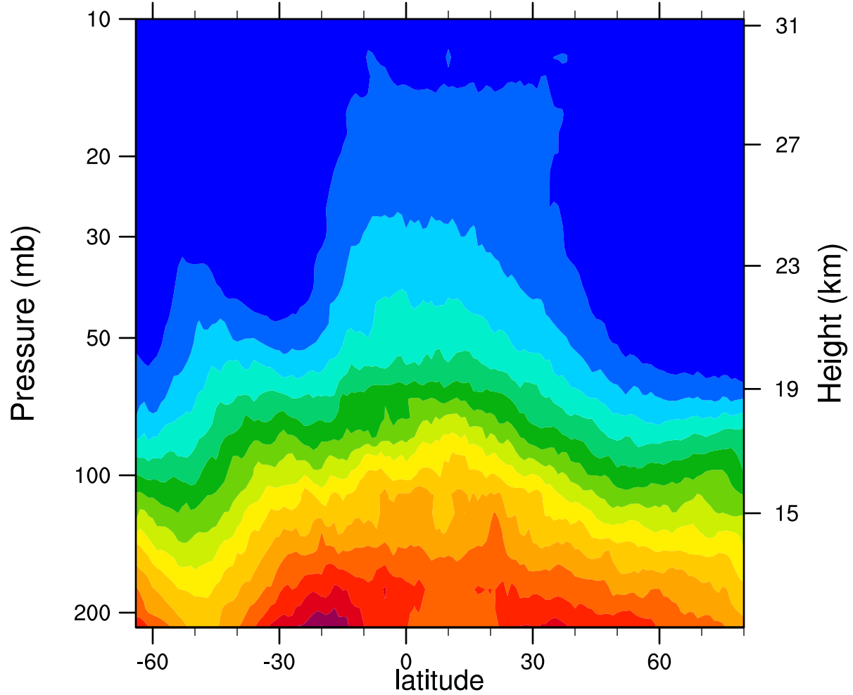
2007d273 12.1MicronExtinction_Combined (km -1 )
