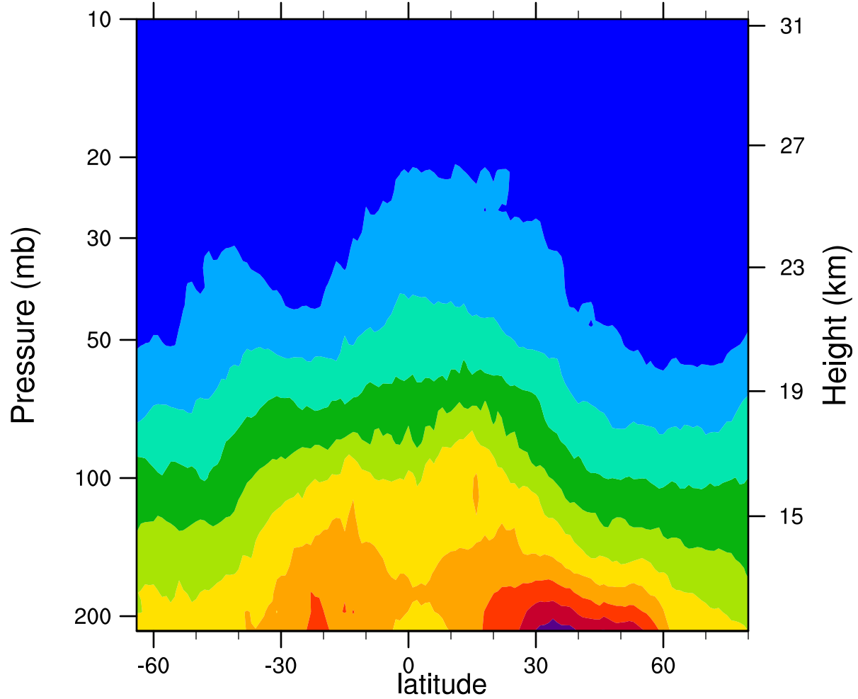
2007d141 12.1MicronExtinction_Combined ( \text{km}^{-1} )
