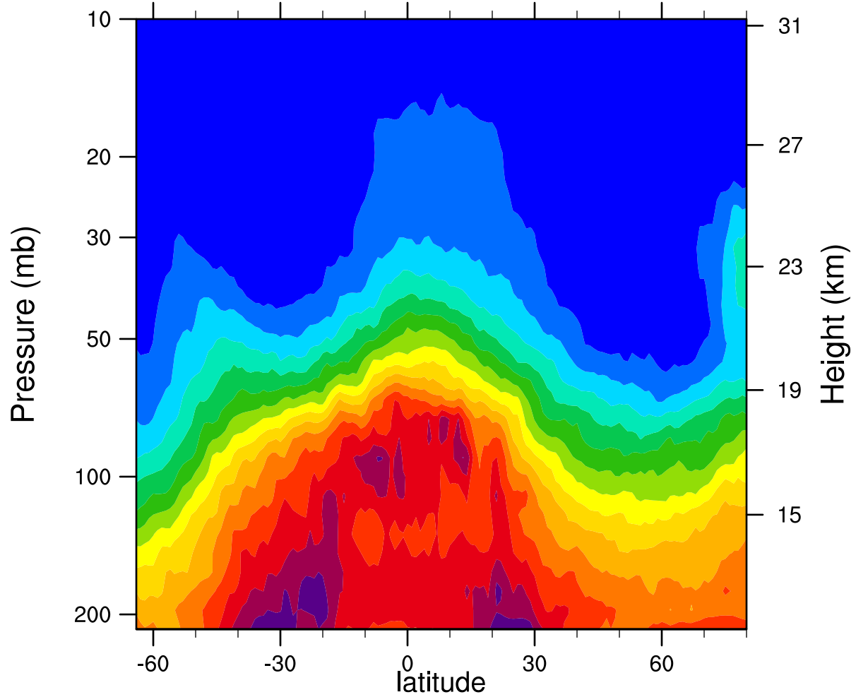
2006d347 12.1MicronExtinction_Combined (km -1 )
