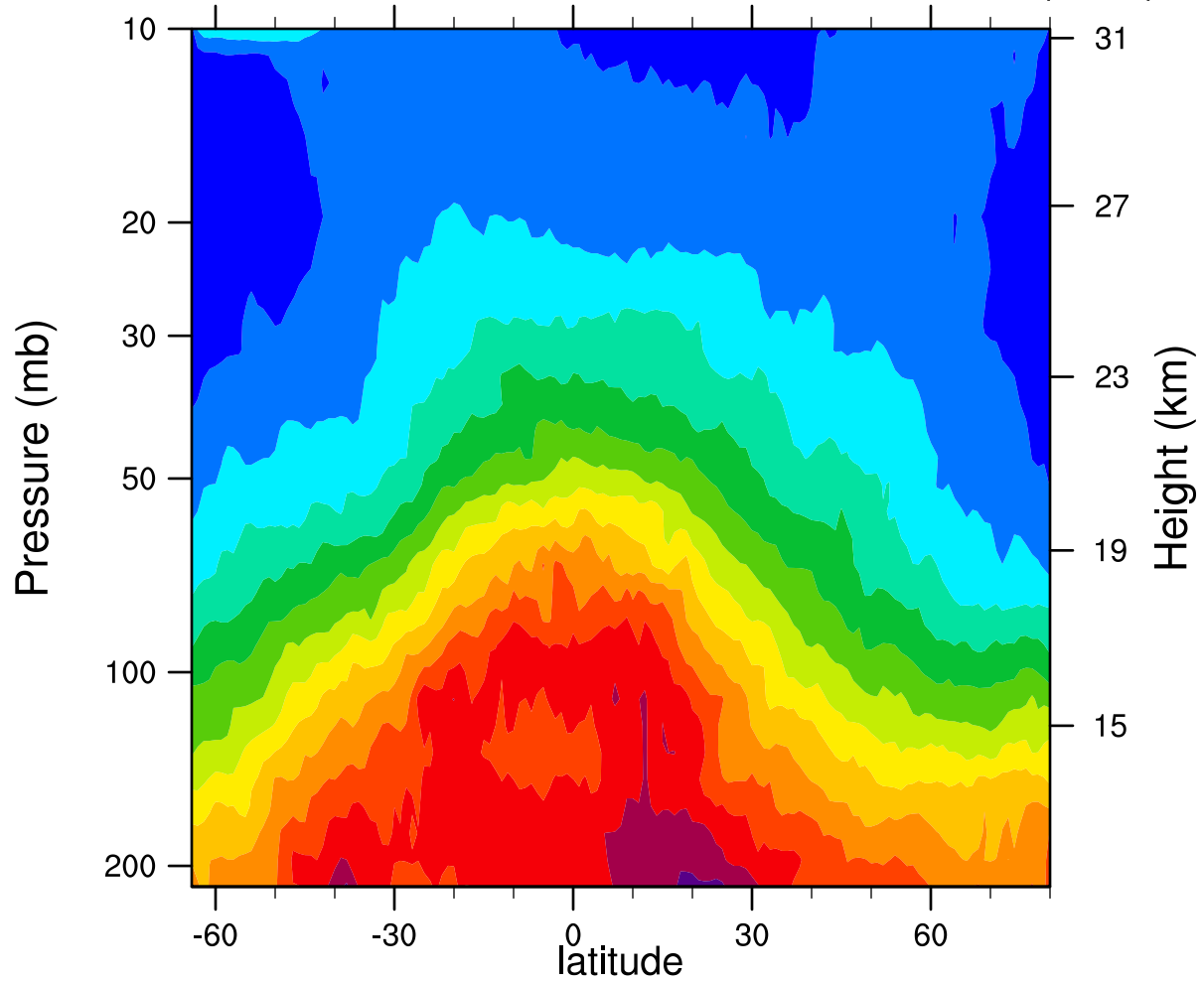
2006d020 12.1MicronExtinction_Combined (km -1 )
