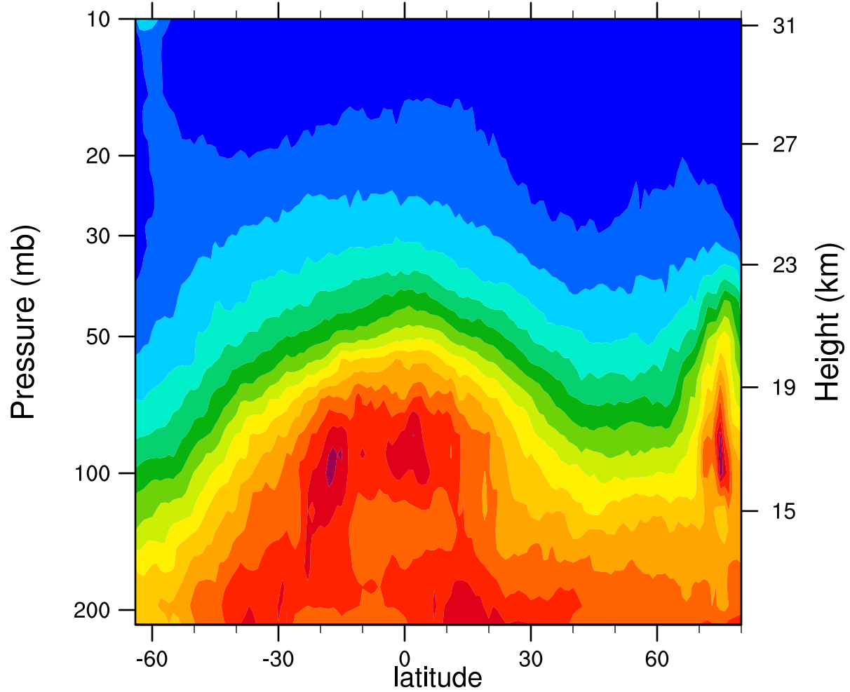
2007d030 12.1MicronExtinction_Combined (km -1 )
