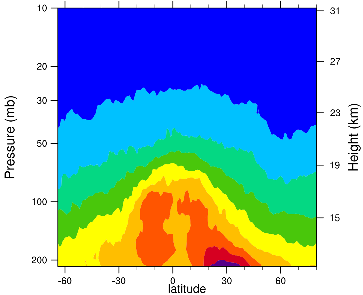
2006d122 12.1MicronExtinction_Combined (km -1 )
