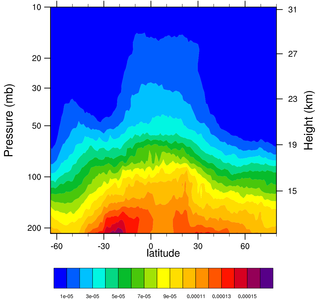
2007d298 12.1MicronExtinction_Combined (km -1 )
