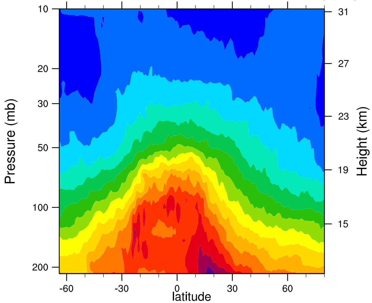
2006d056 12.1MicronExtinction_Combined (km -1 )
