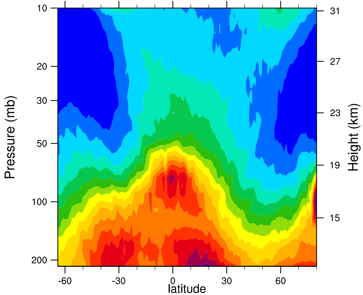
2005d043 12.1MicronExtinction_Combined (km -1 )
