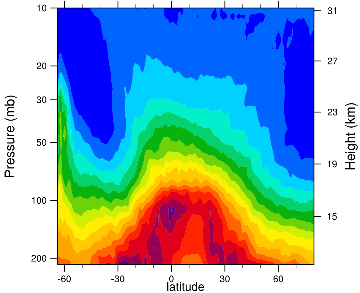
2005d247 12.1MicronExtinction_Combined (km -1 )
