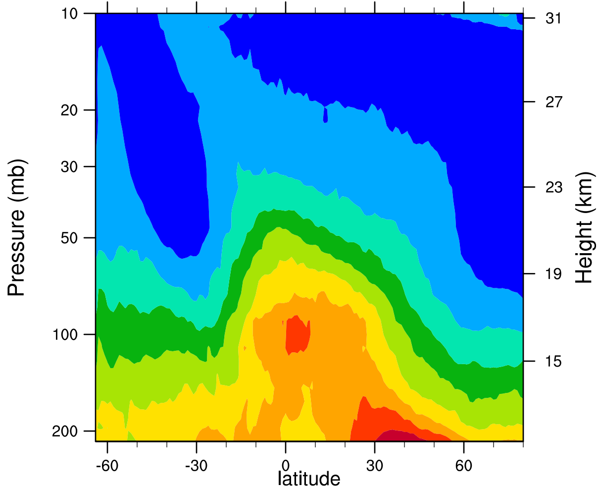
2005d171 12.1MicronExtinction_Combined (km -1 )
