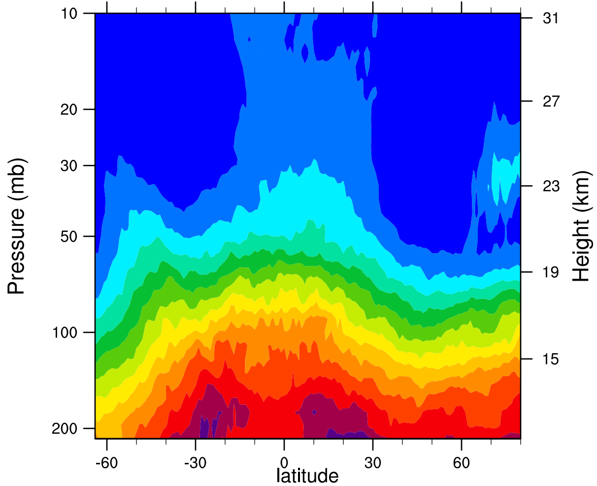
2007d350 12.1MicronExtinction_Combined (km -1 )
