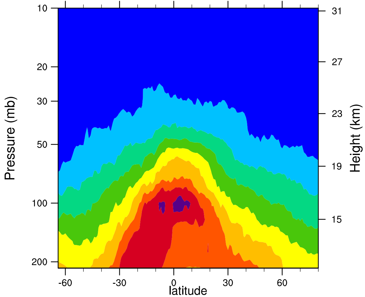
2006d302 12.1MicronExtinction_Combined (km -1 )
