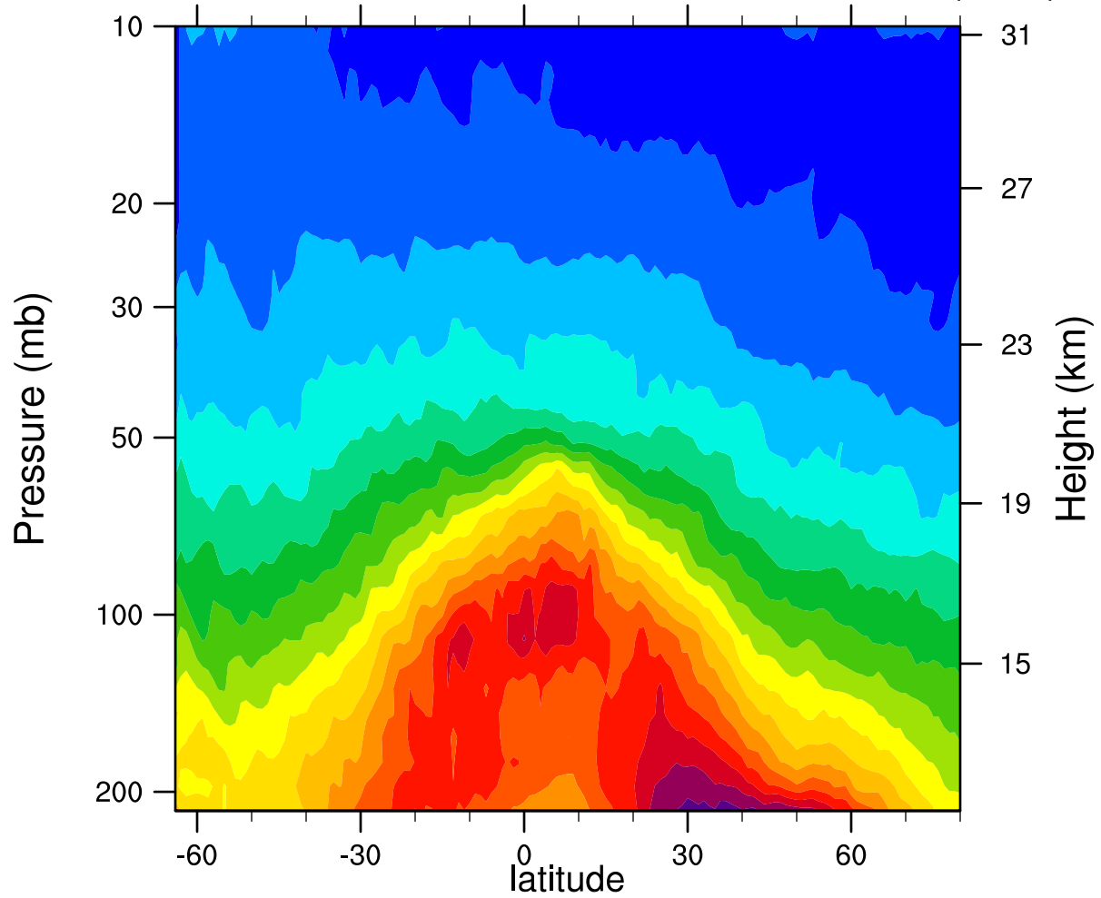
2006d164 12.1MicronExtinction_Combined ( \text{km}^{-1} )
