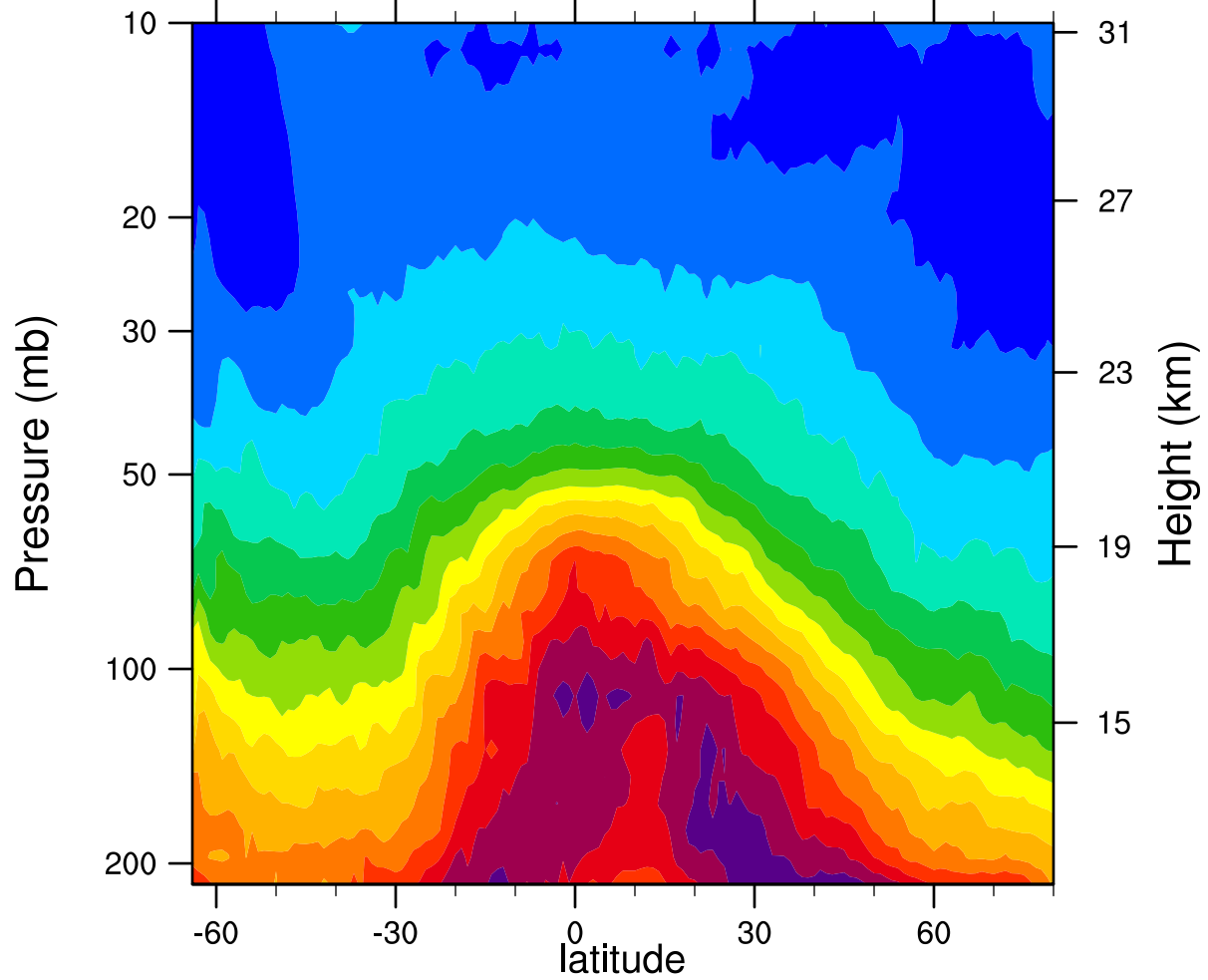
2006d239 12.1MicronExtinction_Combined (km -1 )
