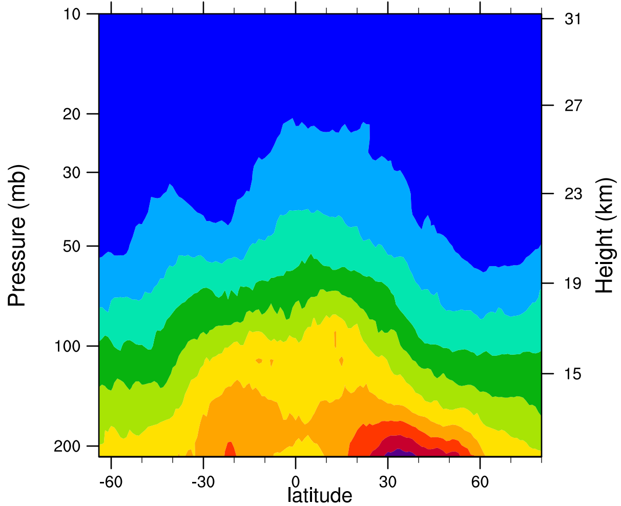
2007d138 12.1MicronExtinction_Combined (km -1 )
