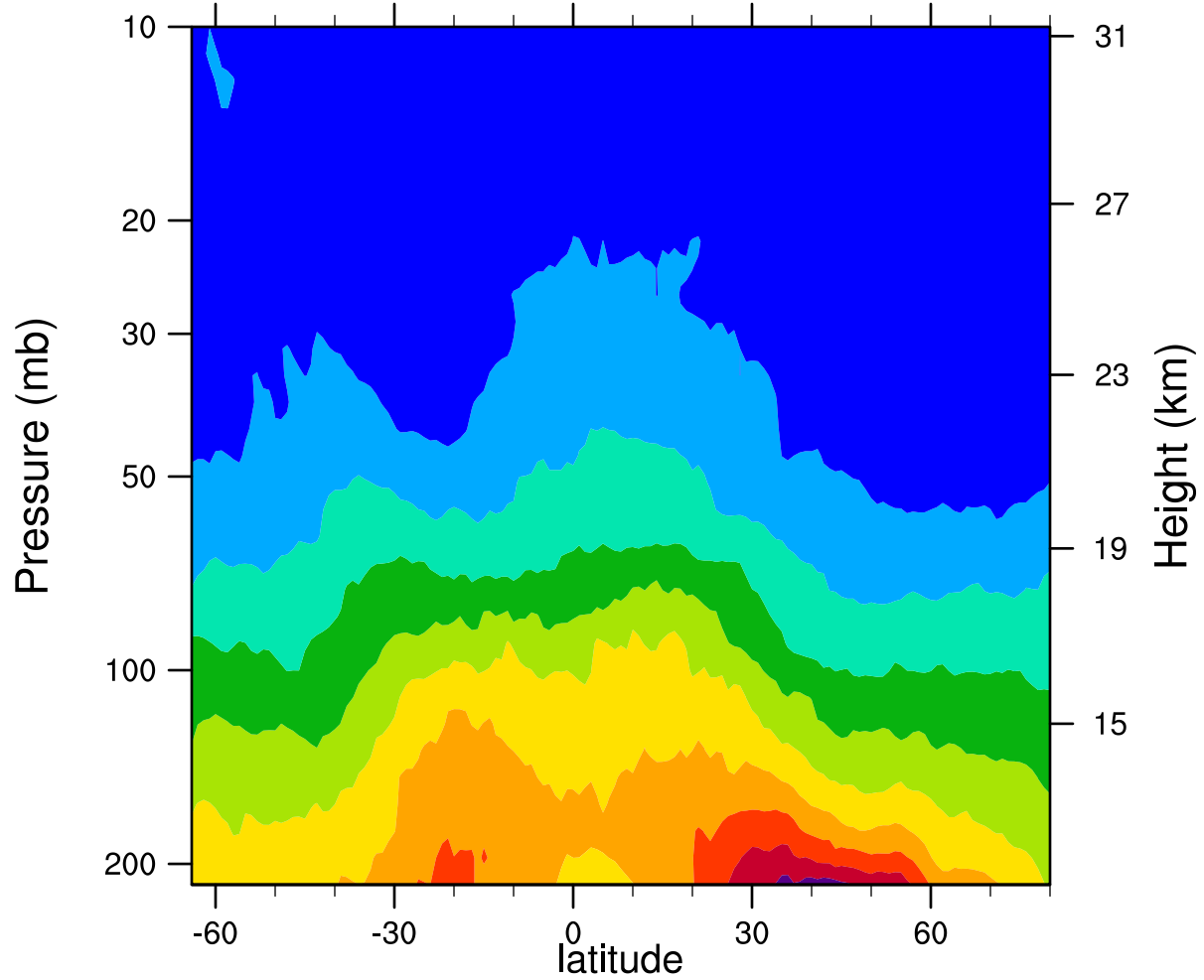
2007d151 12.1MicronExtinction_Combined ( \text{km}^{-1} )
