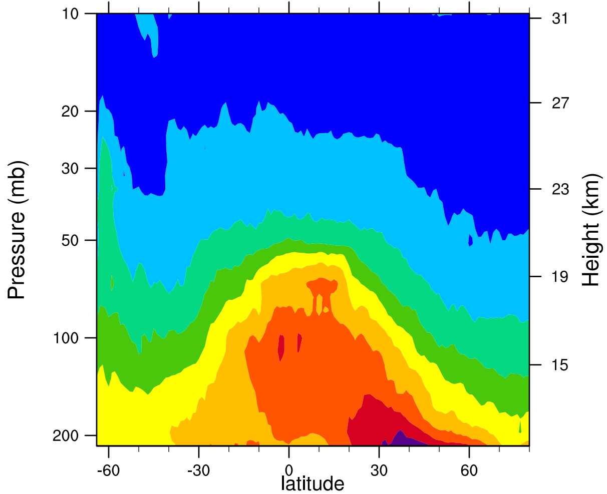
2006d188 12.1MicronExtinction_Combined (km -1 )
