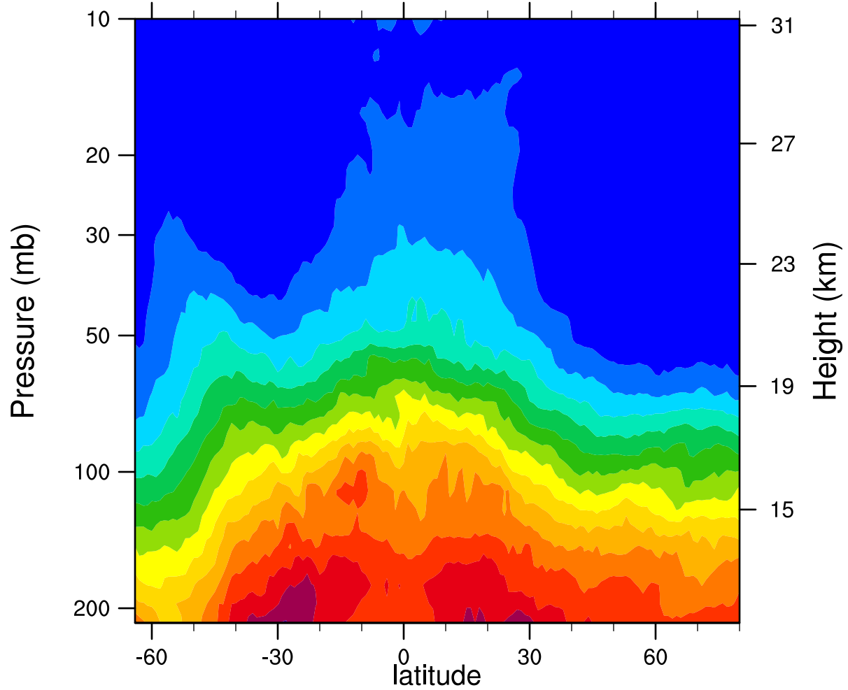
2007d327 12.1MicronExtinction_Combined (km -1 )
