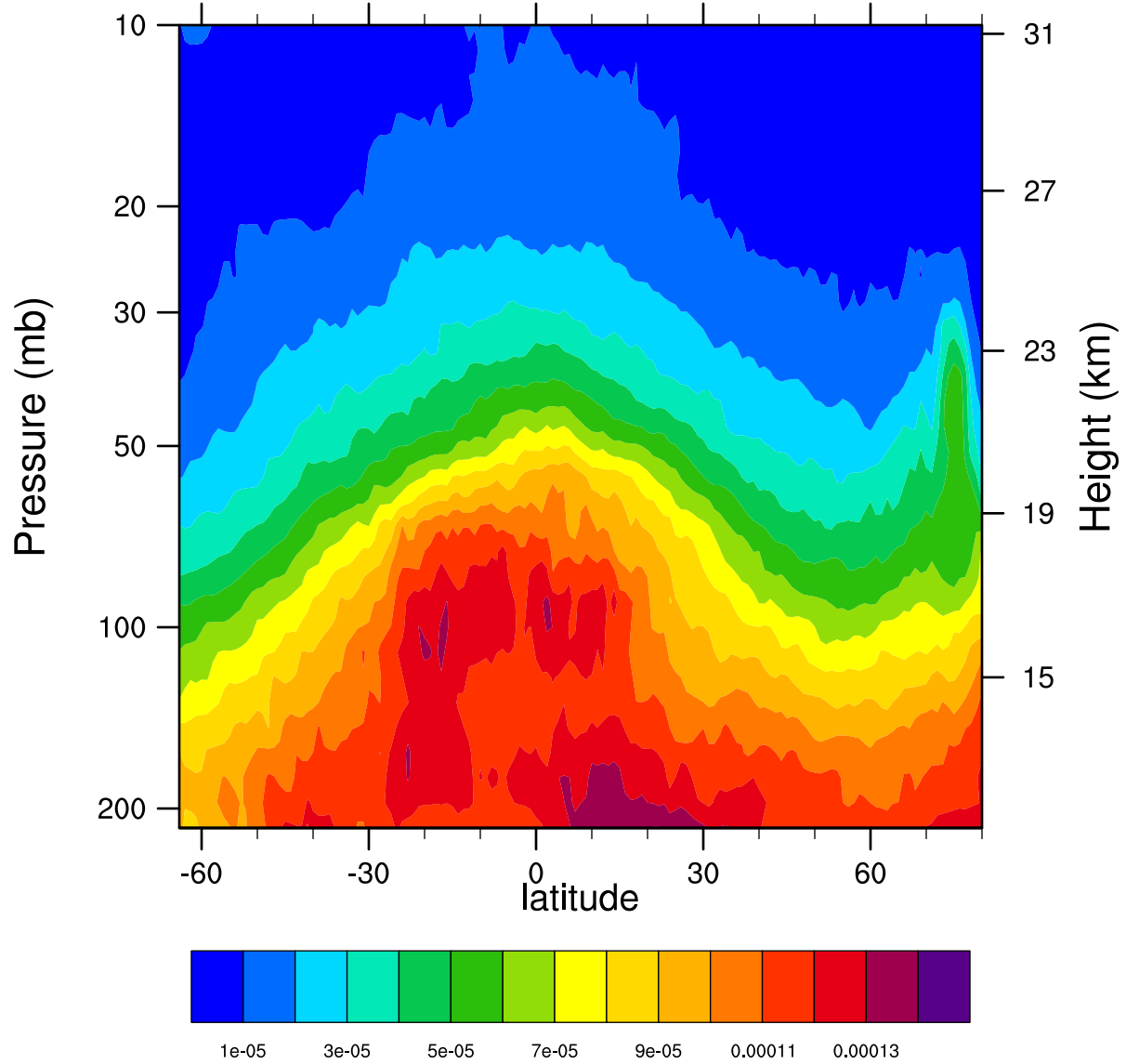
2007d041 12.1MicronExtinction_Combined (km -1 )
