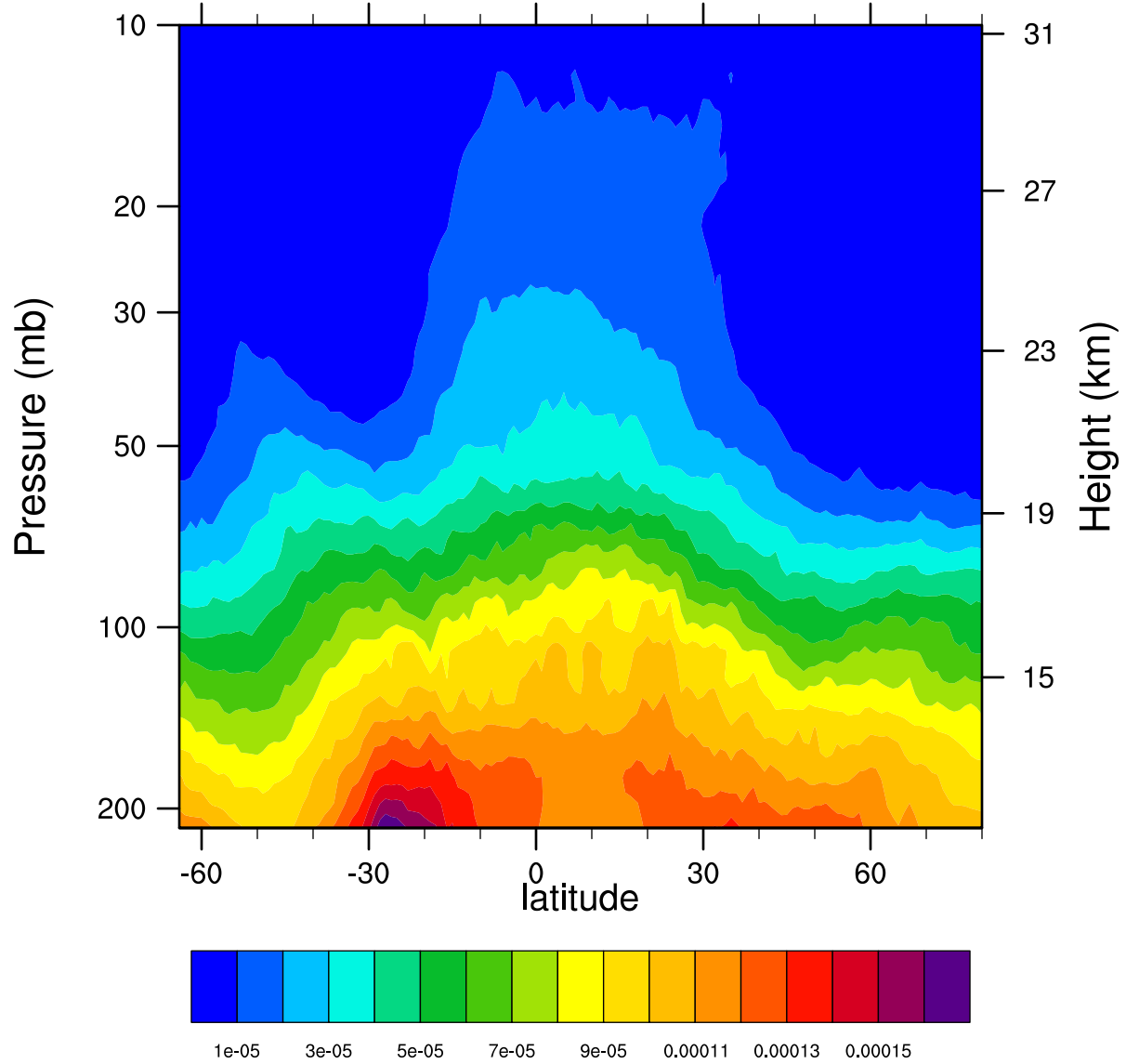
2007d281 12.1MicronExtinction_Combined (km -1 )
