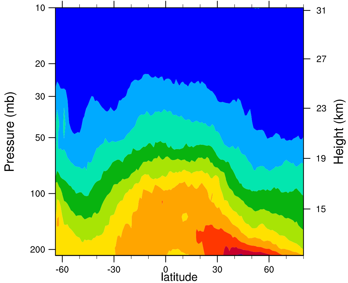
2007d192 12.1MicronExtinction_Combined (km -1 )
