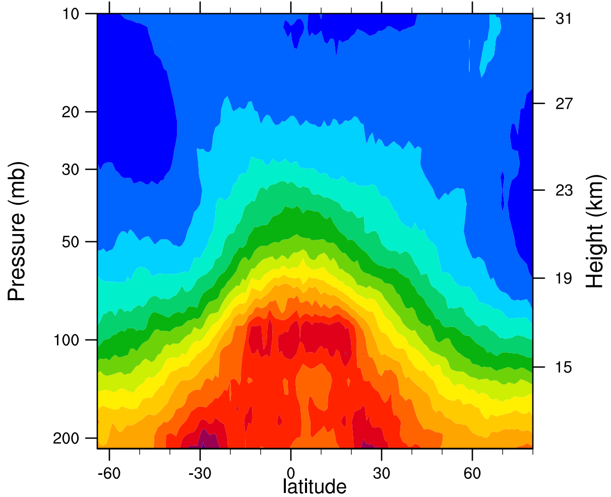
2005d310 12.1MicronExtinction_Combined (km -1 )
