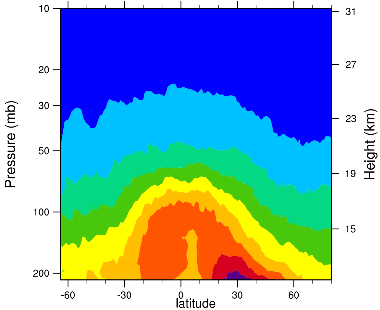
2006d141 12.1MicronExtinction_Combined (km -1 )
