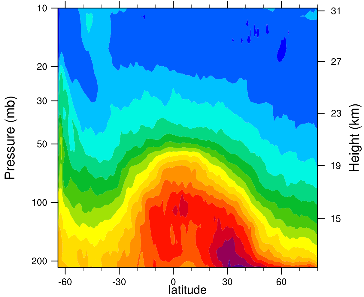
2006d208 12.1MicronExtinction_Combined (km -1 )
