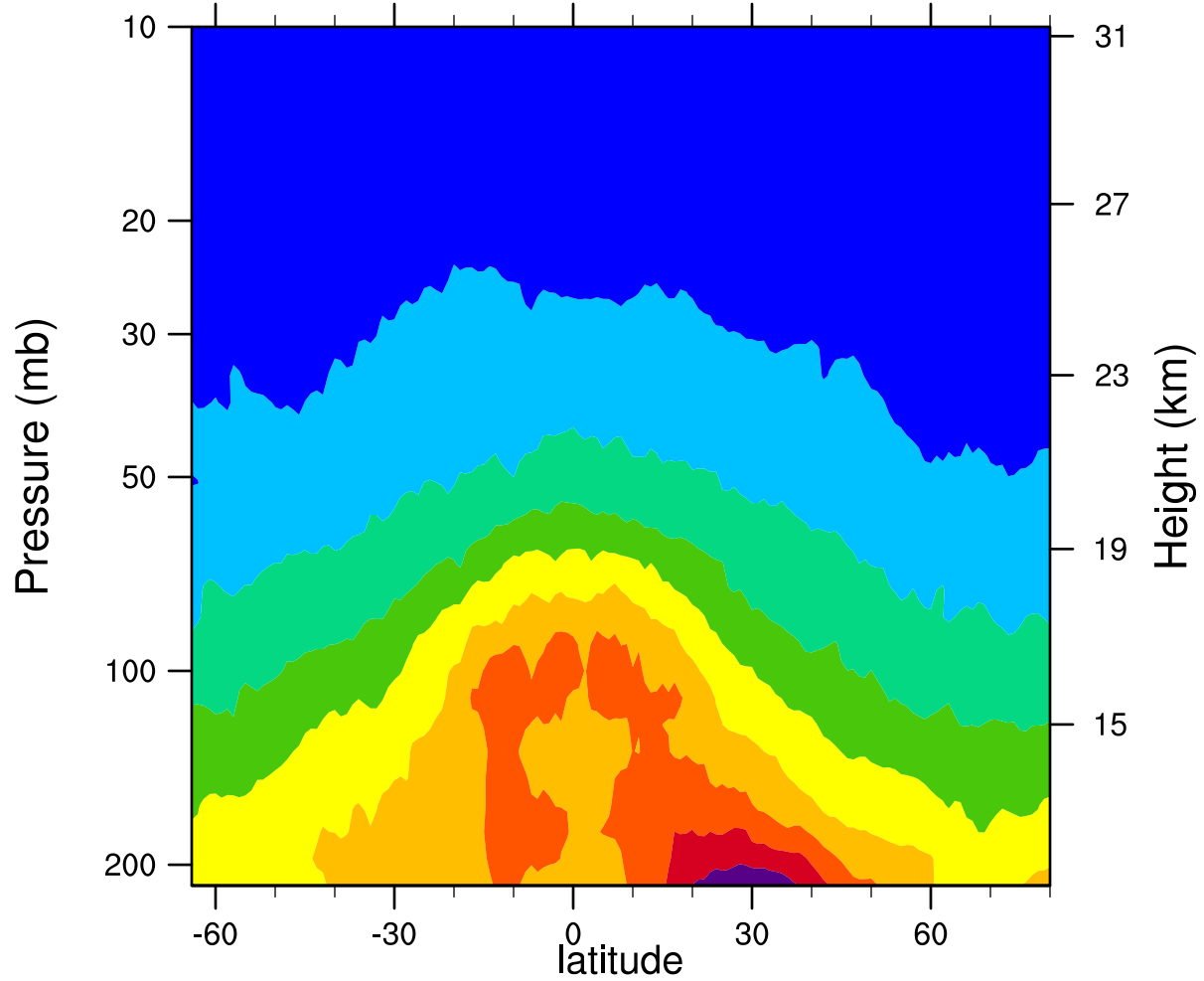
2006d115 12.1MicronExtinction_Combined (km -1 )
