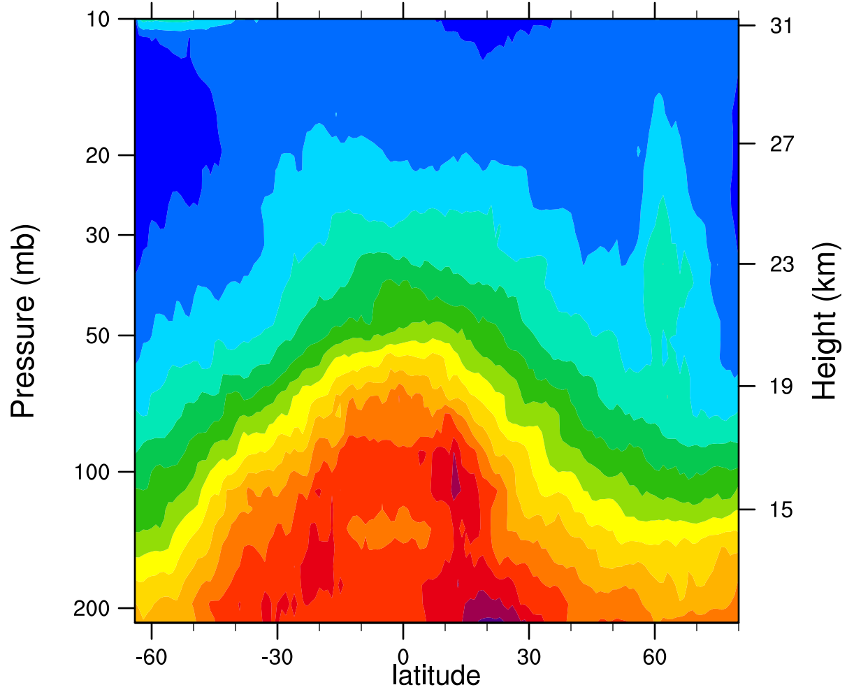
2006d010 12.1MicronExtinction_Combined (km -1 )
