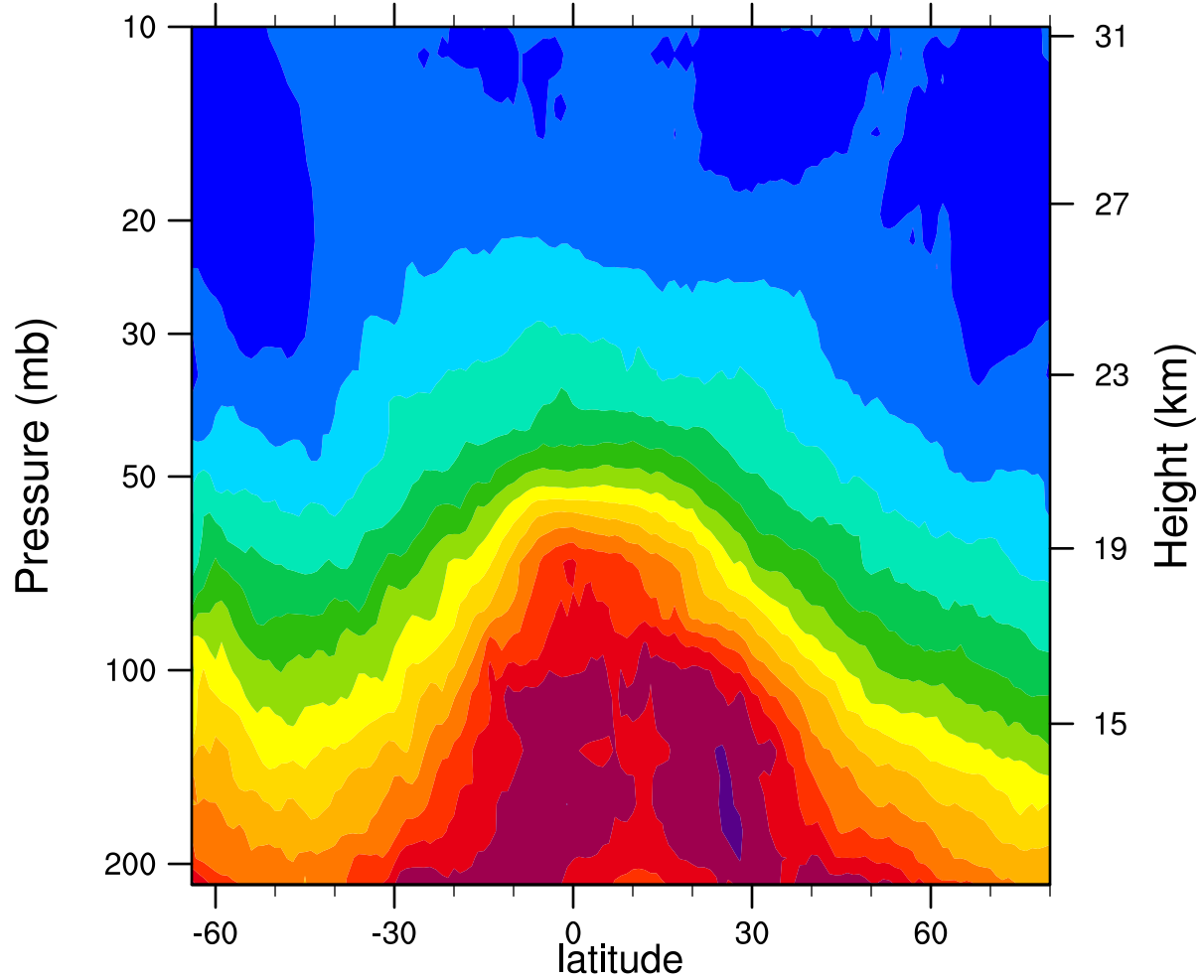
2006d257 12.1MicronExtinction_Combined ( \text{km}^{-1} )
