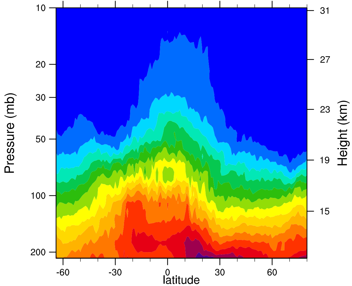
2007d079 12.1MicronExtinction_Combined (km -1 )
