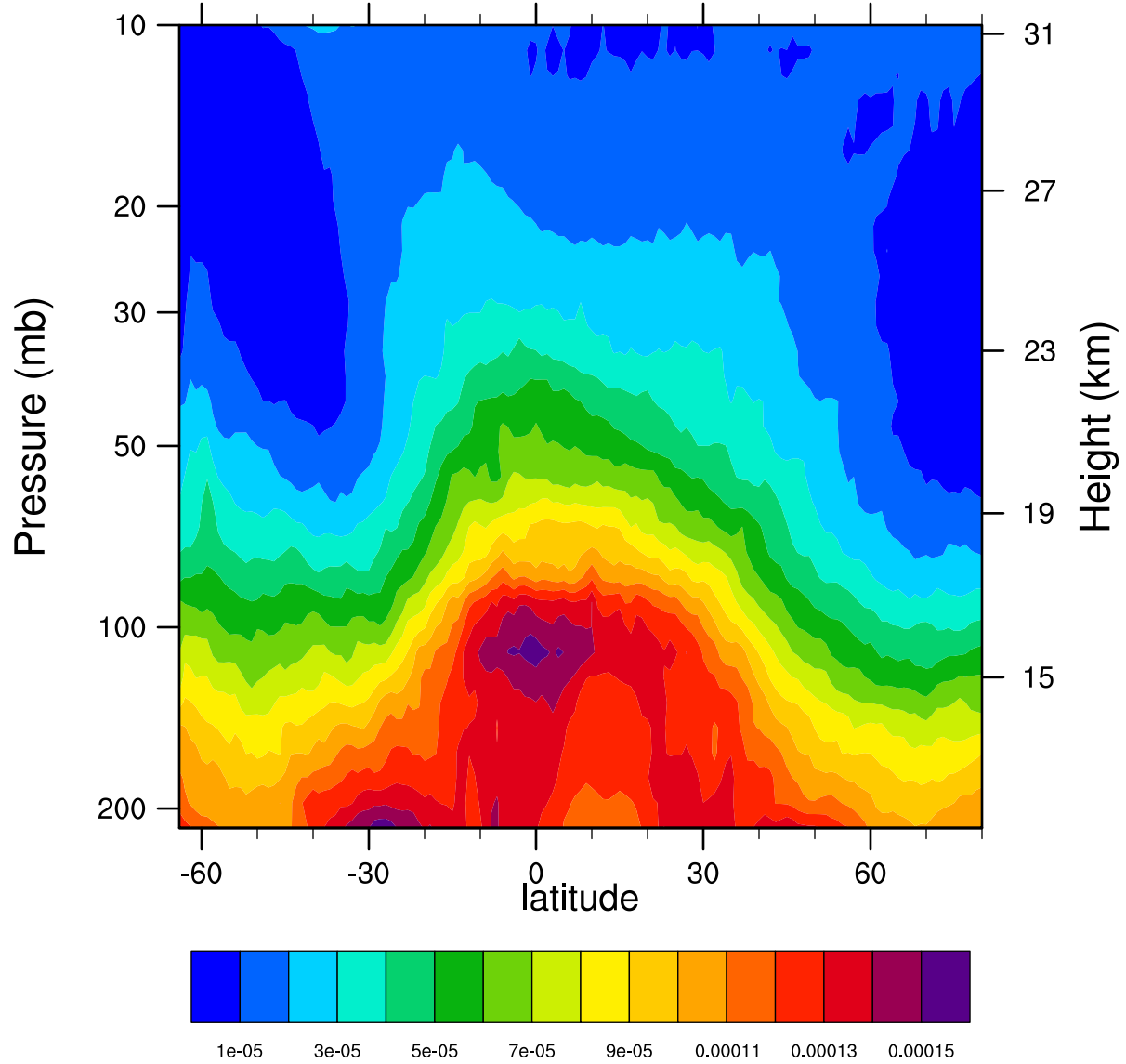
2005d260 12.1MicronExtinction_Combined ( \text{km}^{-1} )
