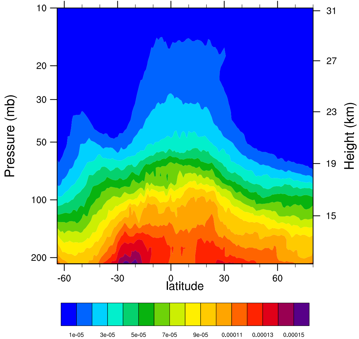
2007d305 12.1MicronExtinction_Combined (km -1 )
