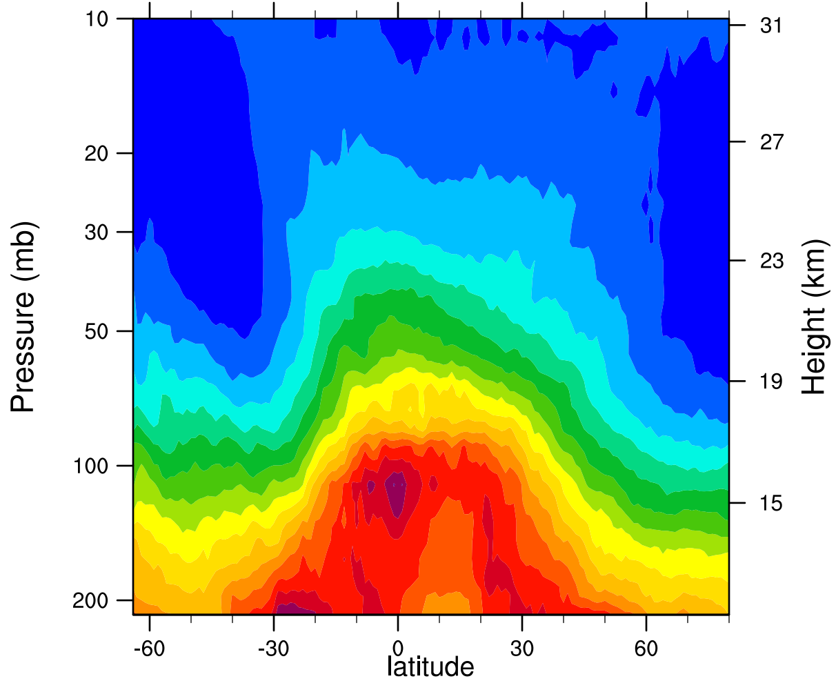
2005d251 12.1MicronExtinction_Combined (km -1 )
