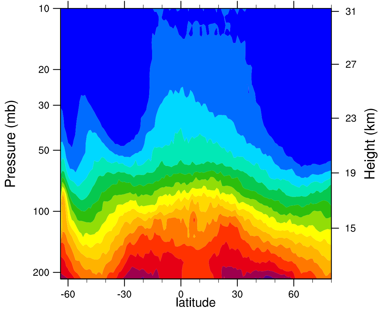
2007d253 12.1MicronExtinction_Combined (km -1 )
