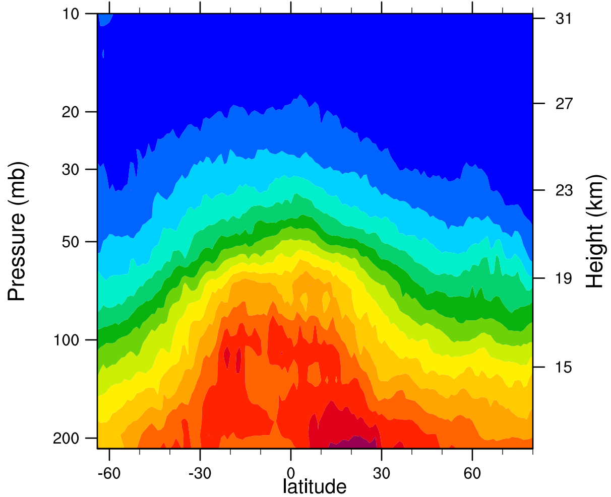
2007d054 12.1MicronExtinction_Combined ( \text{km}^{-1} )
