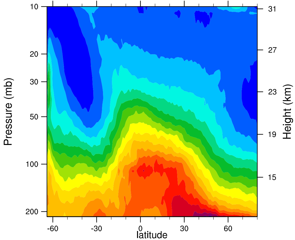
2005d198 12.1MicronExtinction_Combined (km -1 )
