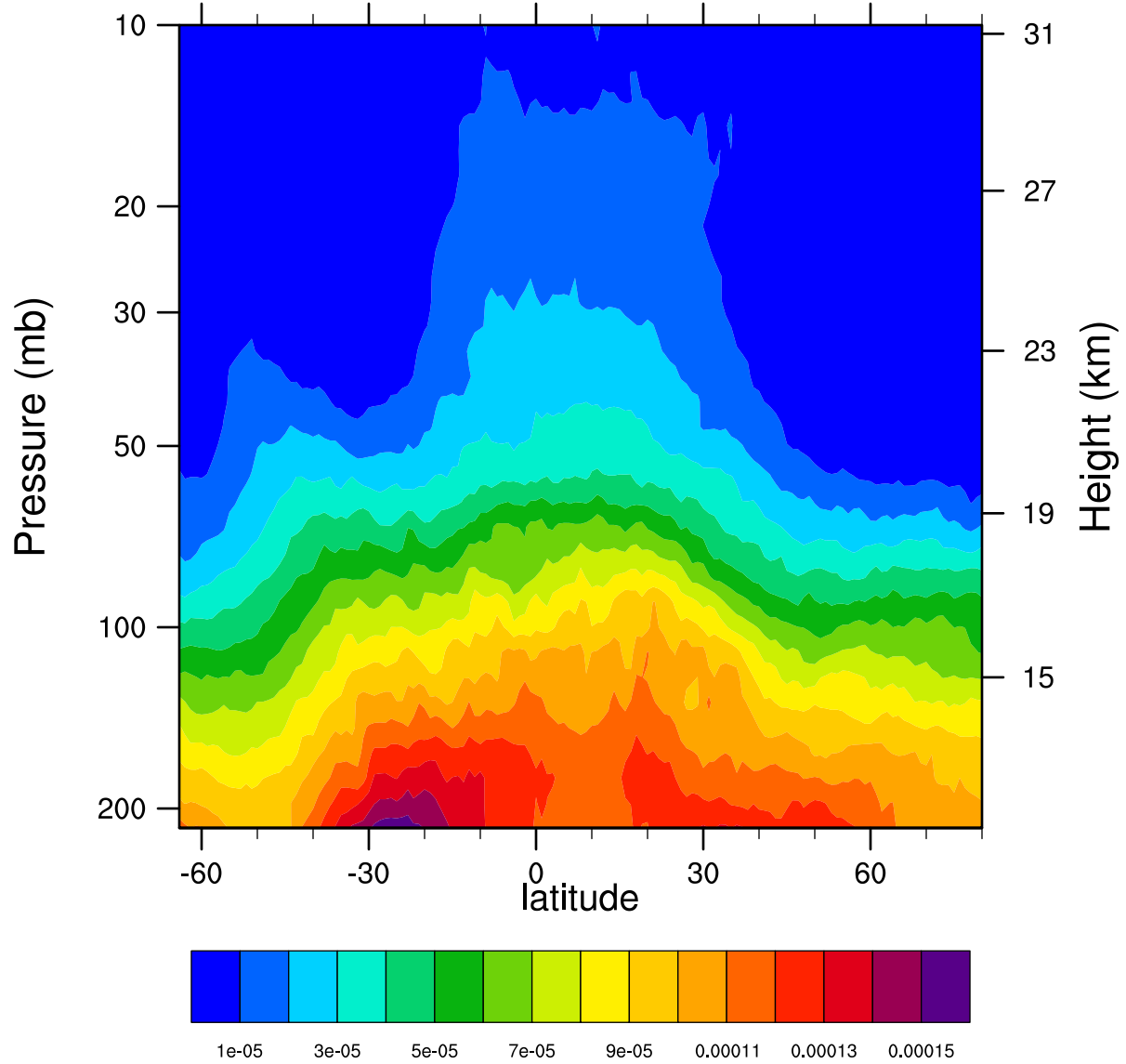
2007d290 12.1MicronExtinction_Combined (km -1 )
