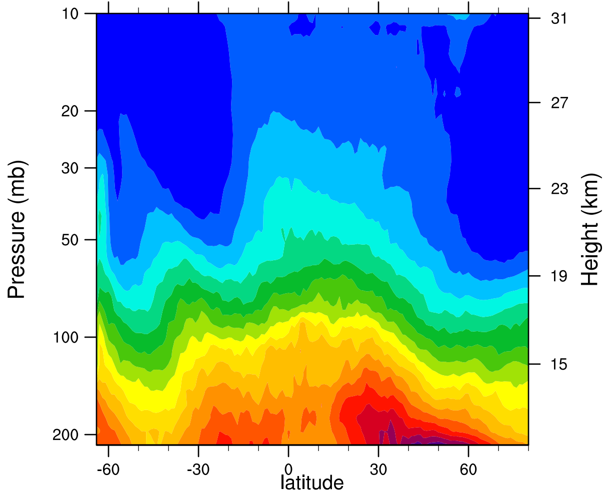
2007d218 12.1MicronExtinction_Combined (km -1 )
