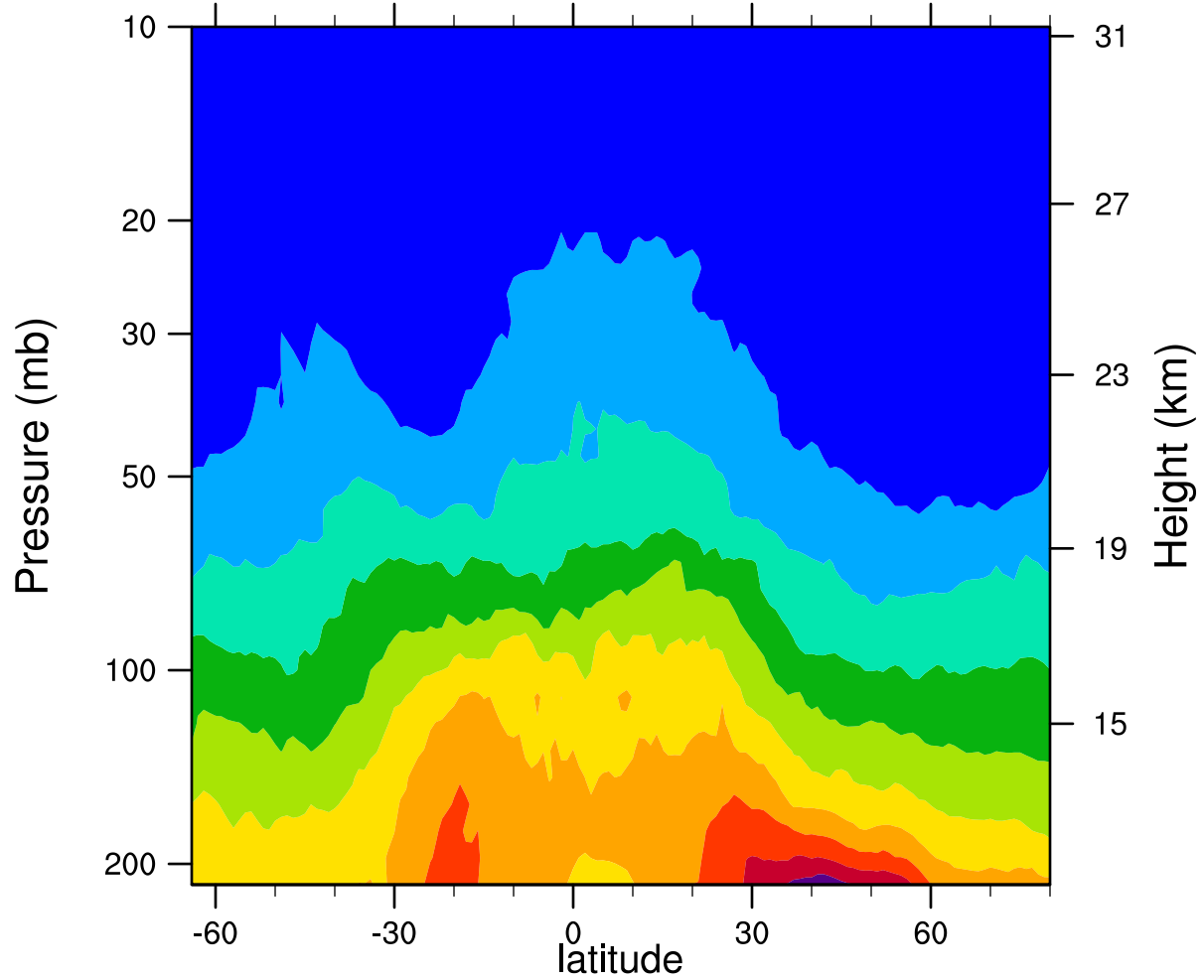
2007d158 12.1MicronExtinction_Combined (km -1 )
