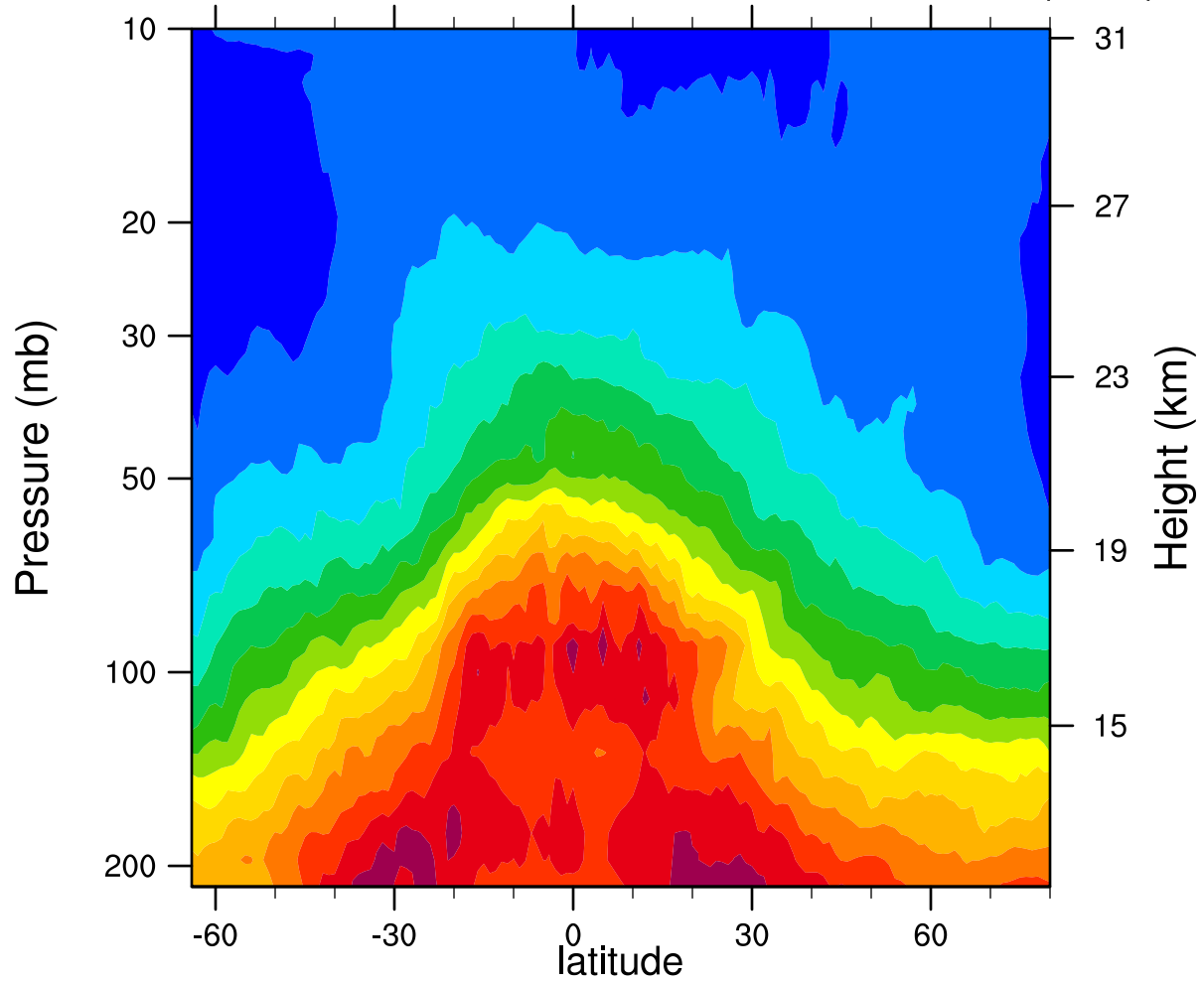
2005d337 12.1MicronExtinction_Combined (km -1 )
