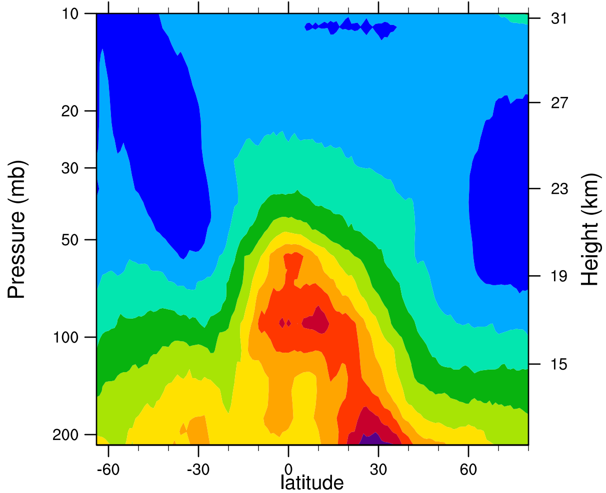
2005d131 12.1MicronExtinction_Combined (km -1 )
