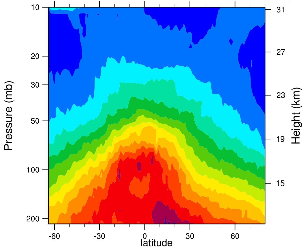
2006d039 12.1MicronExtinction_Combined ( \text{km}^{-1} )
