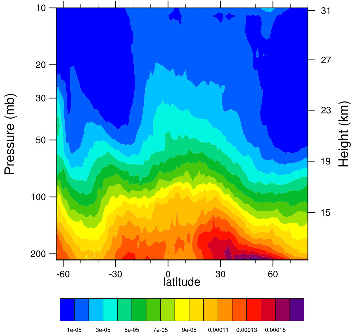
2007d217 12.1MicronExtinction_Combined (km -1 )
