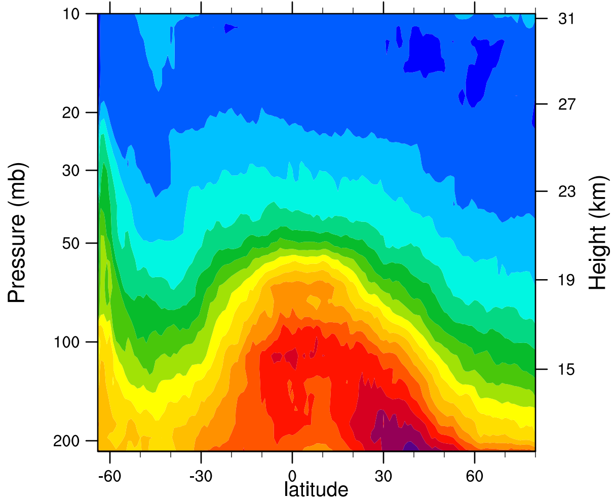
2006d216 12.1MicronExtinction_Combined (km -1 )
