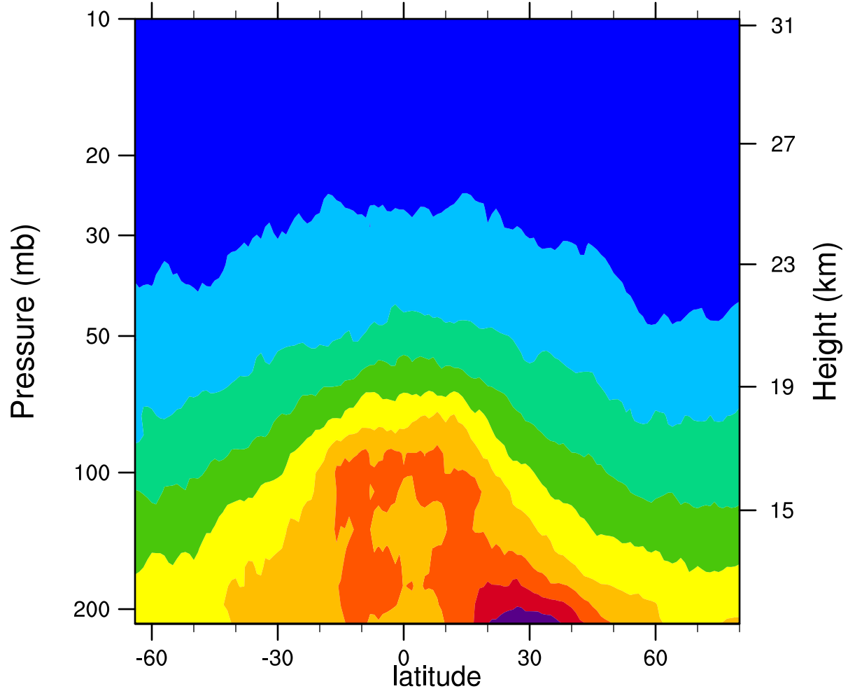
2006d118 12.1MicronExtinction_Combined ( \text{km}^{-1} )
