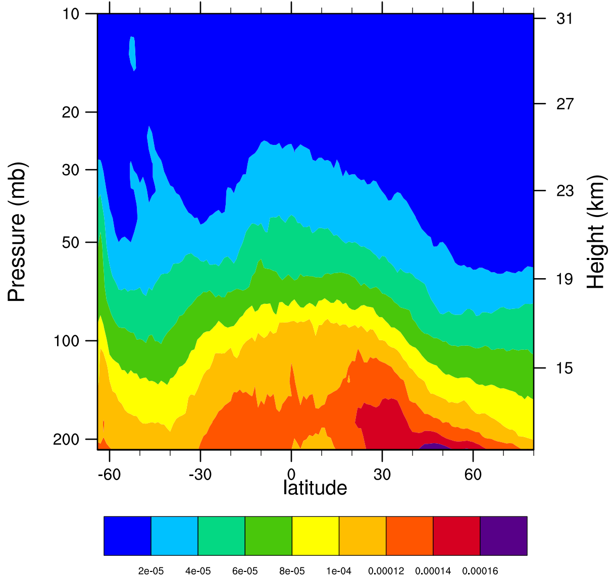
2007d209 12.1MicronExtinction_Combined ( \text{km}^{-1} )
