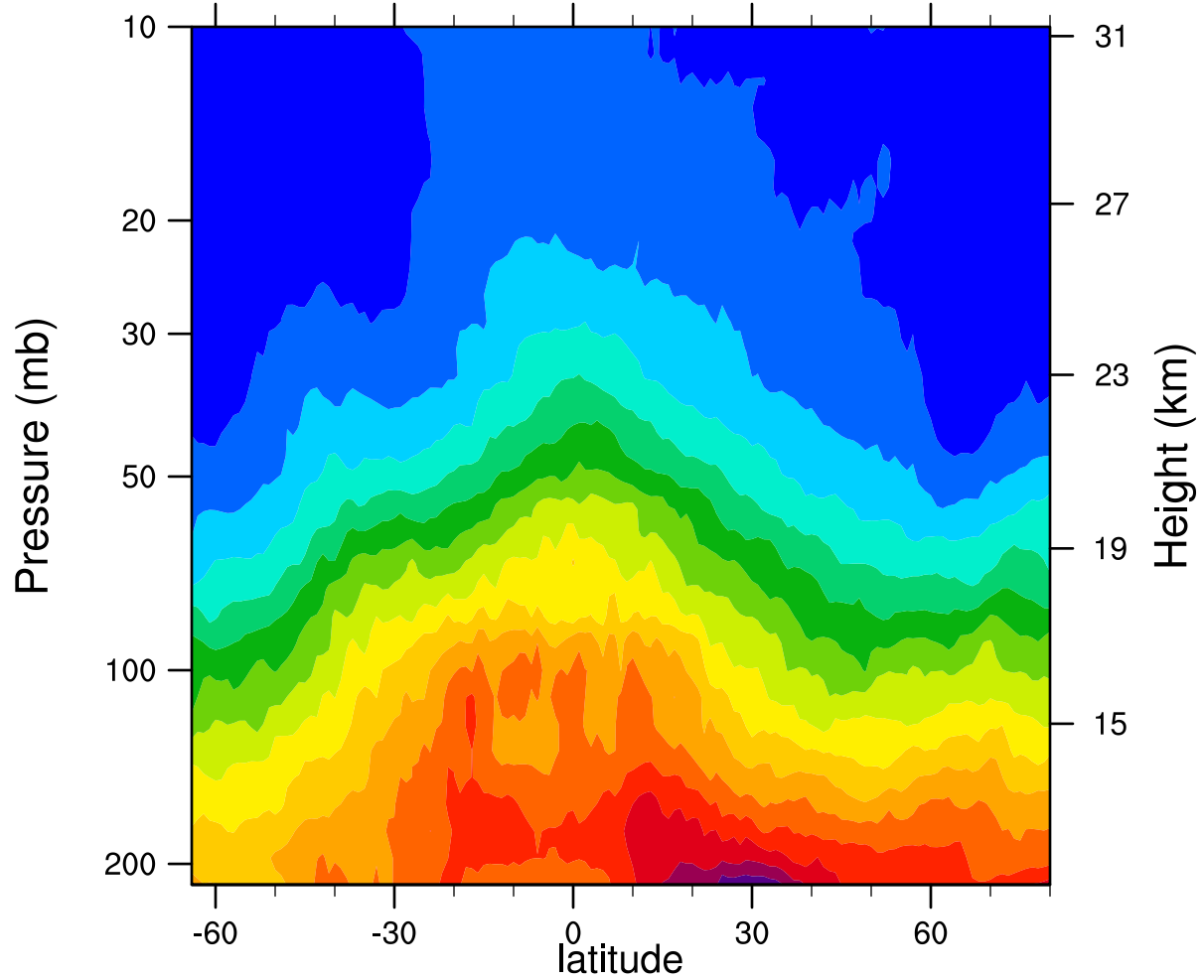
2007d092 12.1MicronExtinction_Combined (km -1 )
