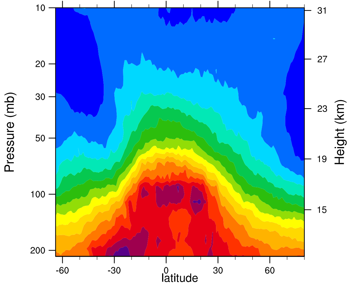
2005d302 12.1MicronExtinction_Combined (km -1 )
