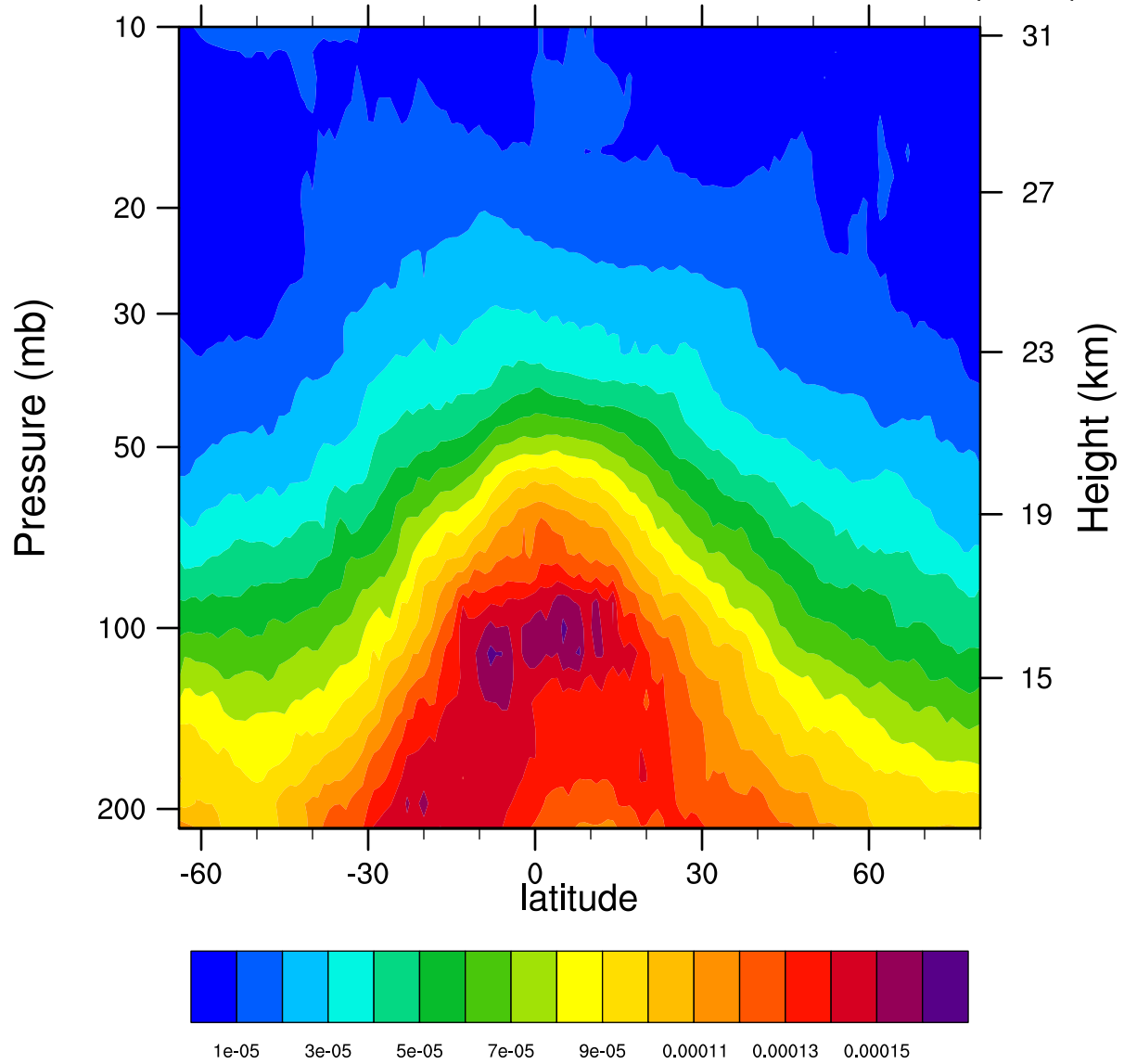
2006d293 12.1MicronExtinction_Combined ( \text{km}^{-1} )
