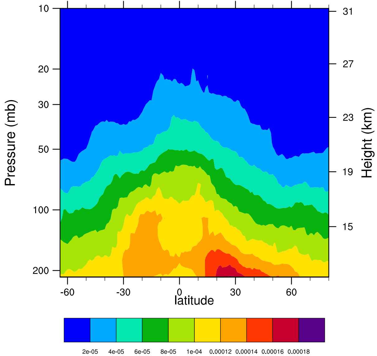
2007d112 12.1MicronExtinction_Combined (km -1 )
