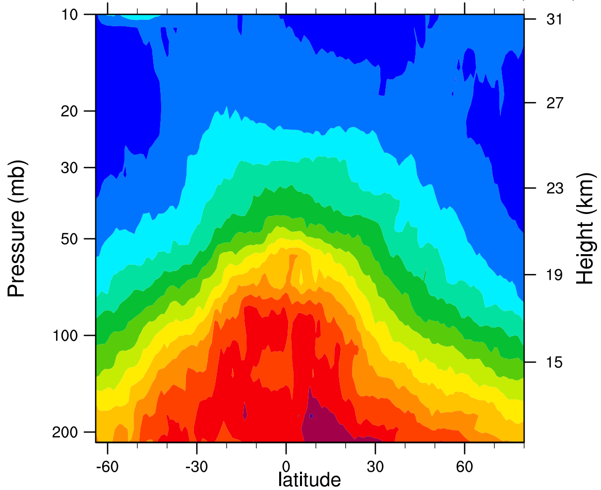
2006d032 12.1MicronExtinction_Combined ( \text{km}^{-1} )
