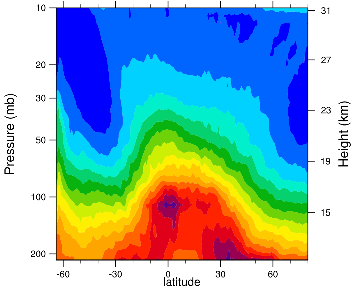
2005d220 12.1MicronExtinction_Combined (km -1 )
