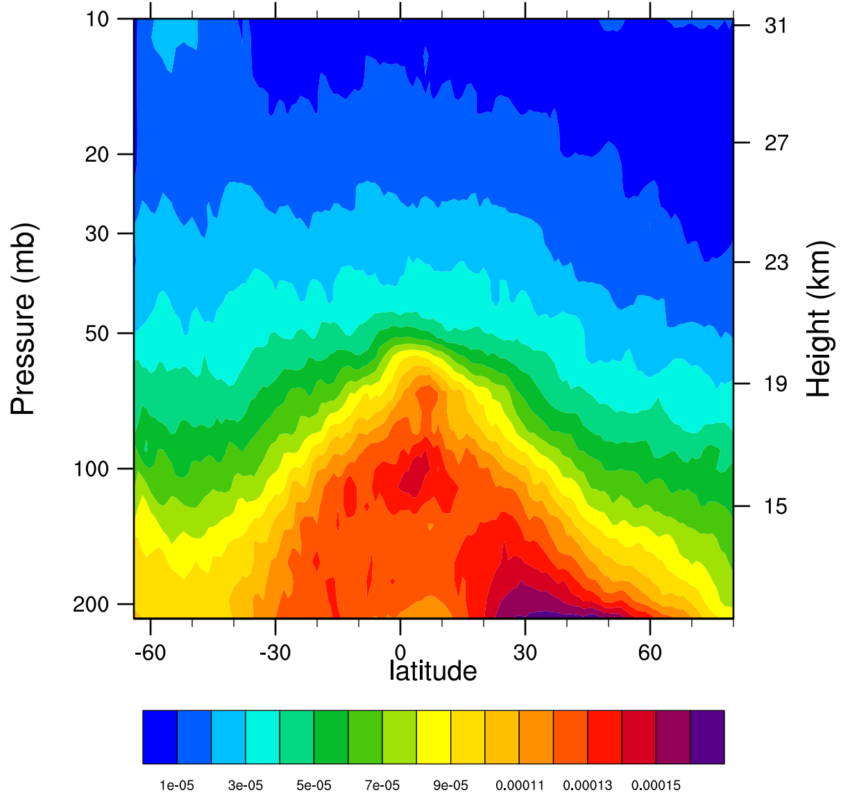
2006d171 12.1MicronExtinction_Combined ( \text{km}^{-1} )
