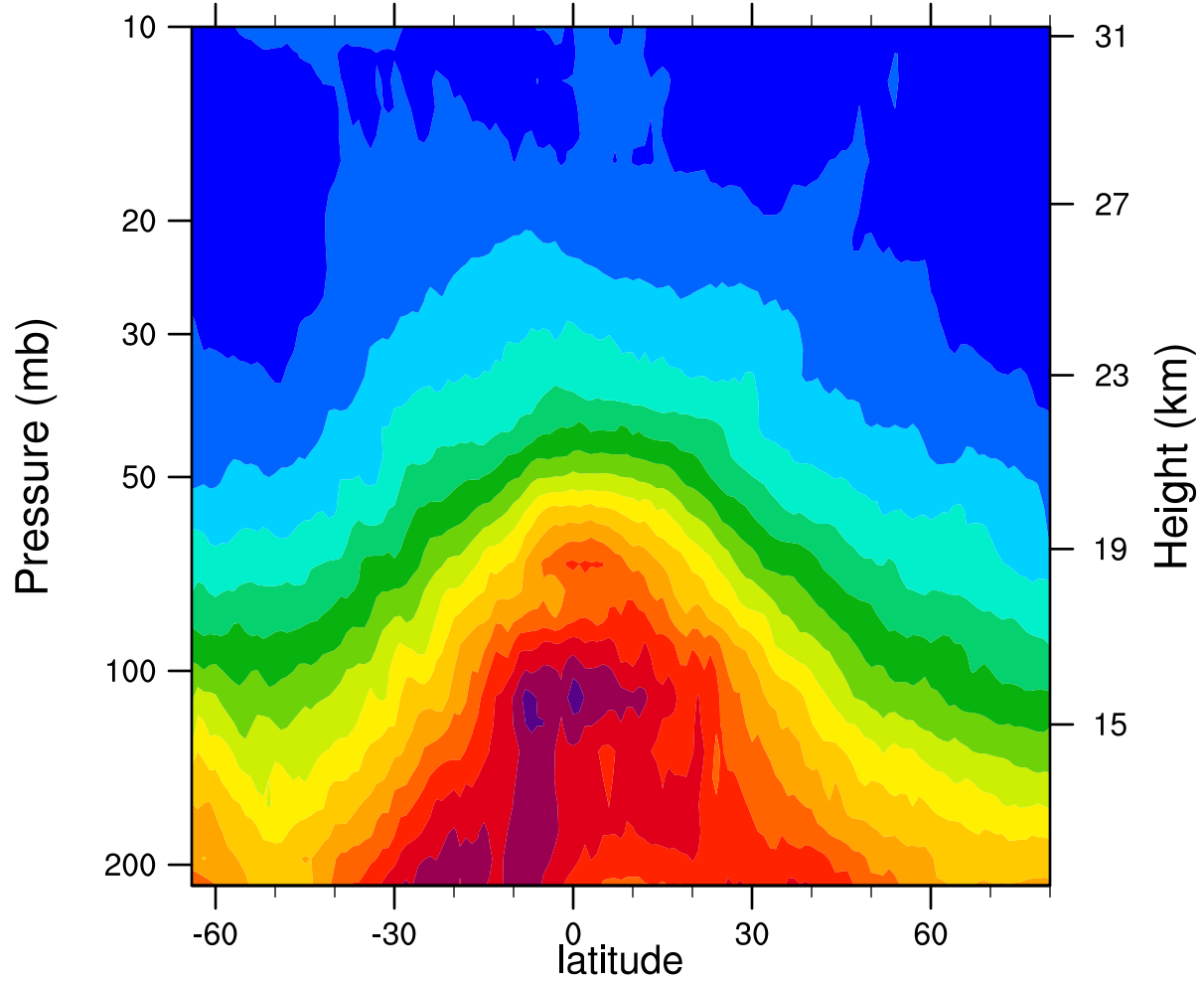
2006d286 12.1MicronExtinction_Combined (km -1 )
