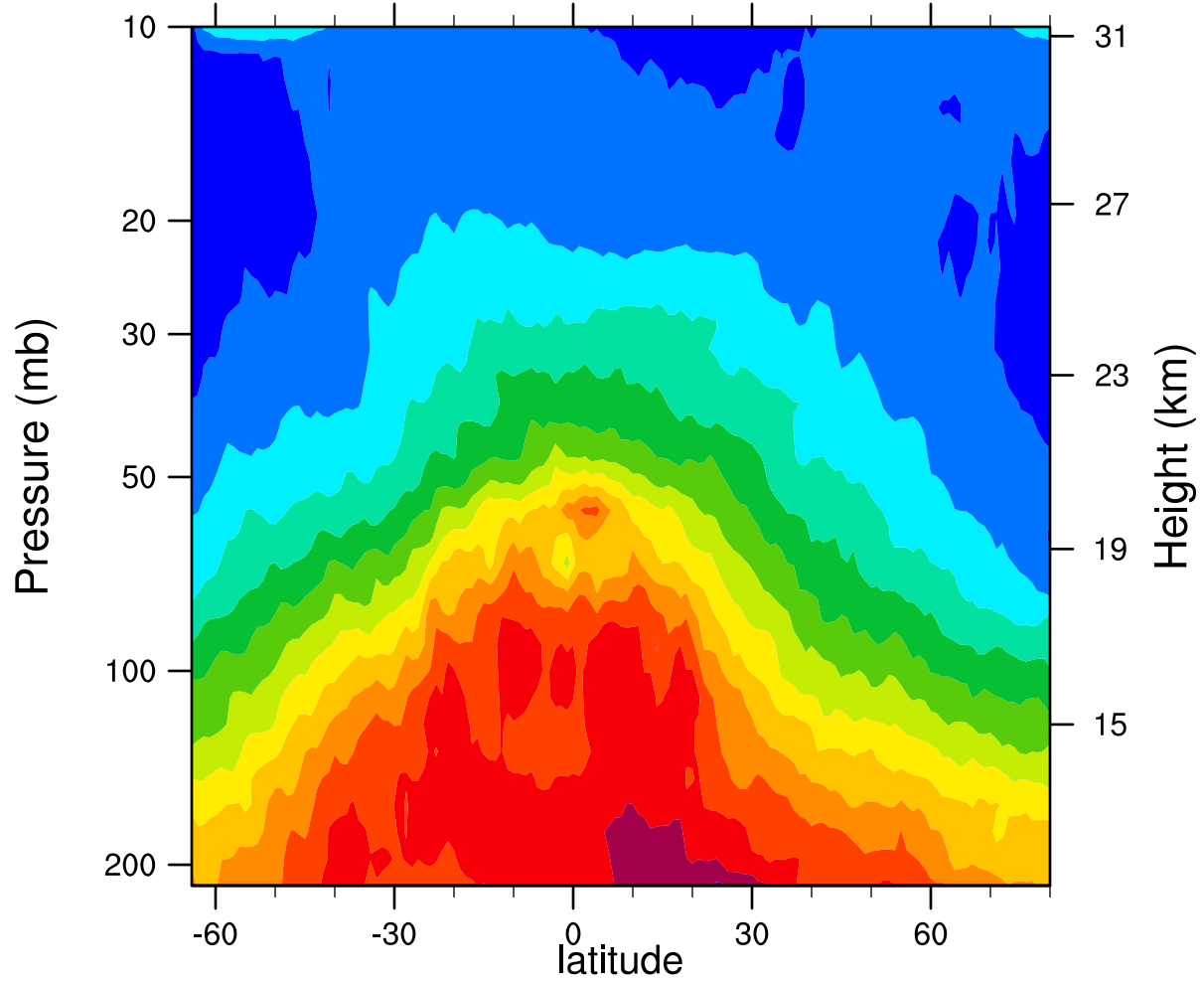
2006d027 12.1MicronExtinction_Combined (km -1 )
