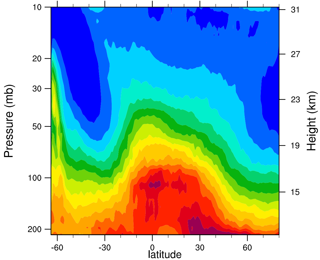
2005d210 12.1MicronExtinction_Combined ( \text{km}^{-1} )
