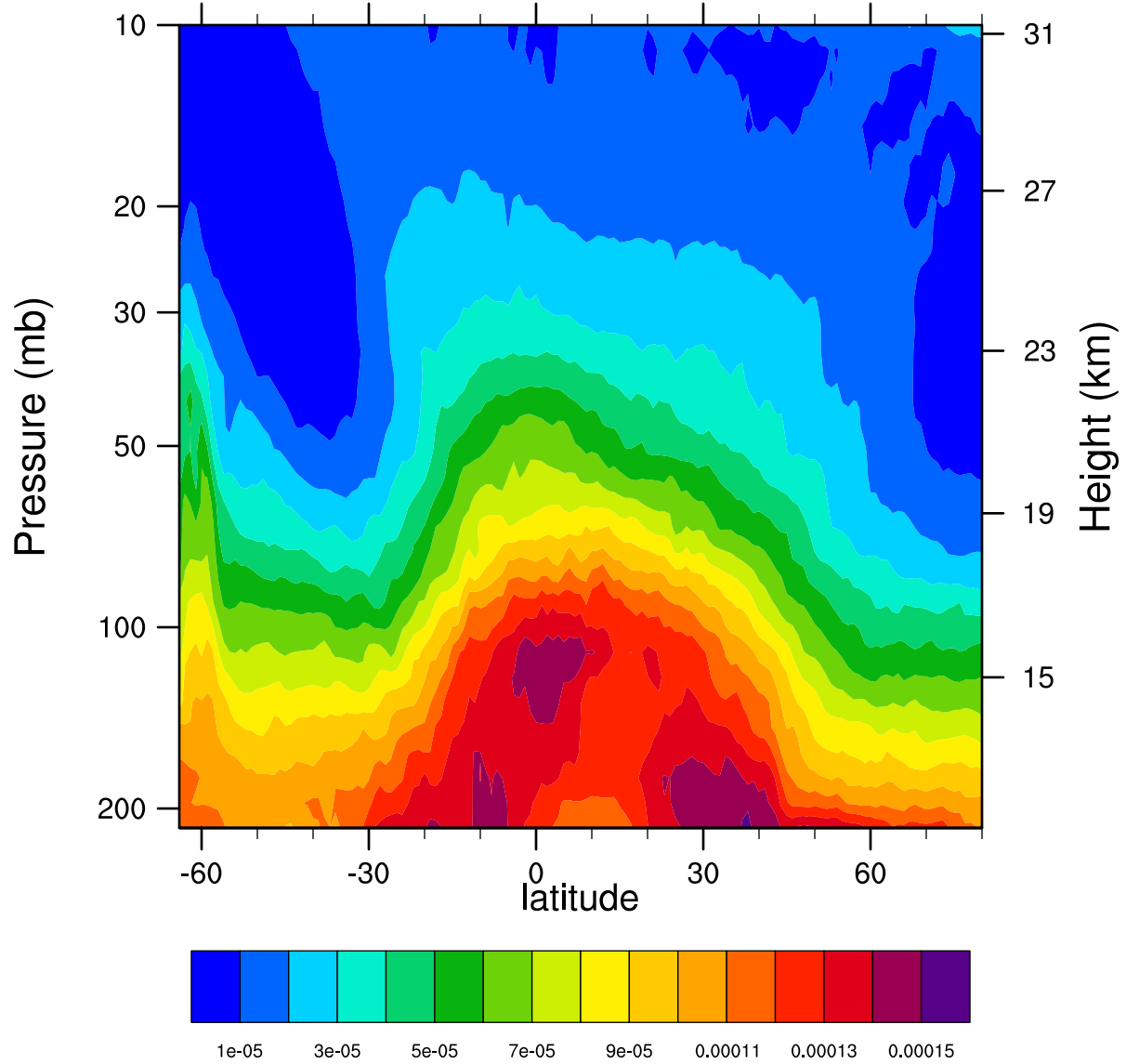
2005d228 12.1MicronExtinction_Combined (km -1 )
