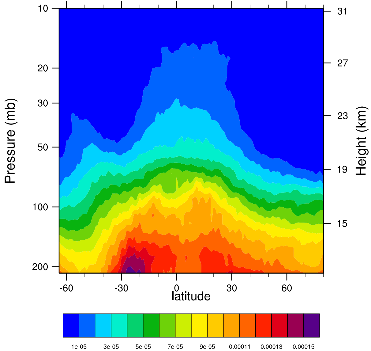
2007d309 12.1MicronExtinction_Combined (km -1 )
