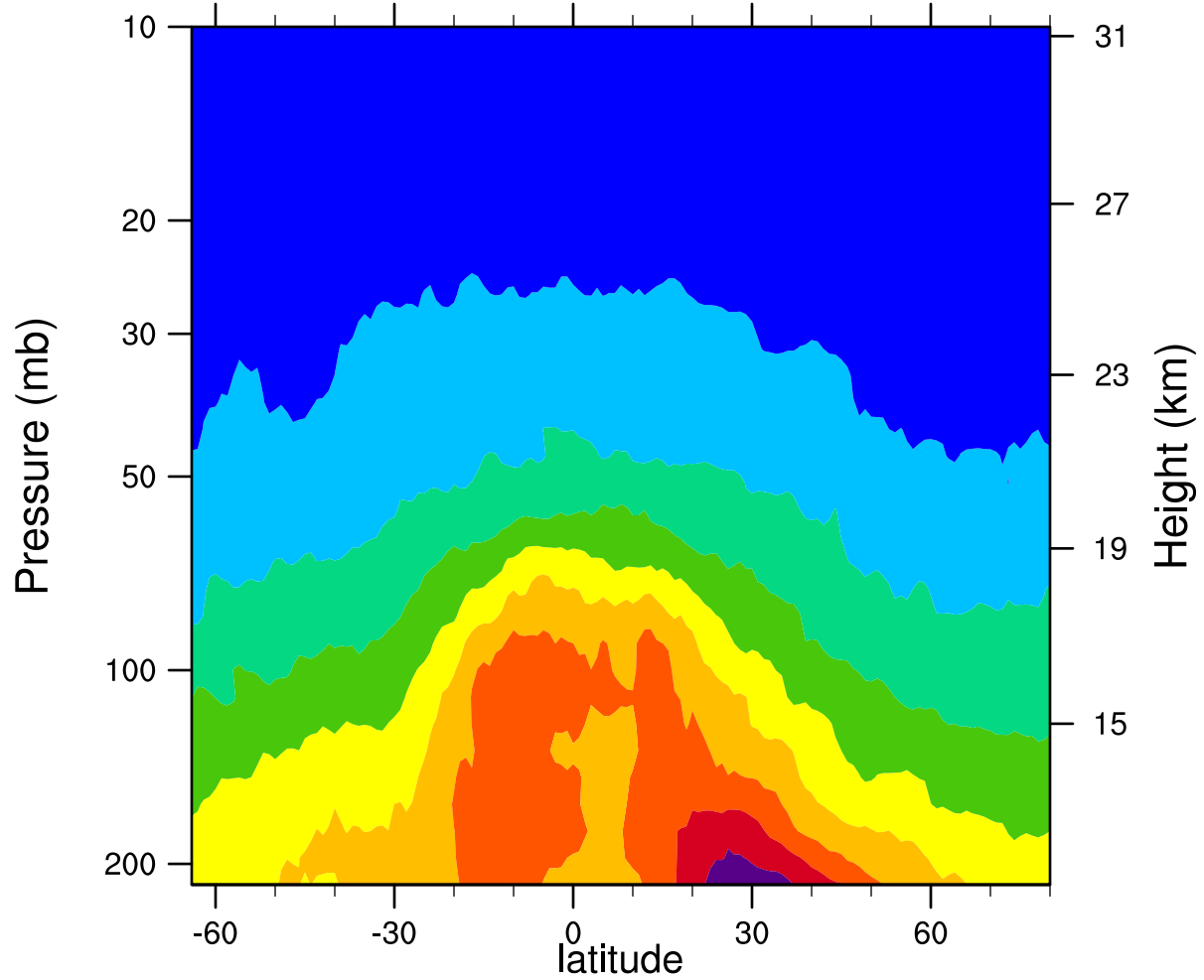
2006d131 12.1MicronExtinction_Combined (km -1 )
