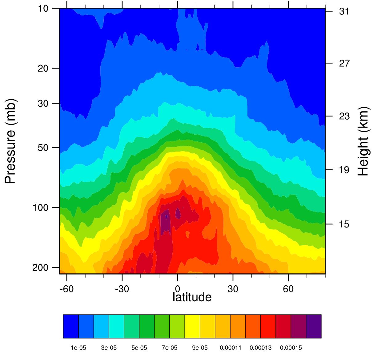
2006d288 12.1MicronExtinction_Combined ( \text{km}^{-1} )
