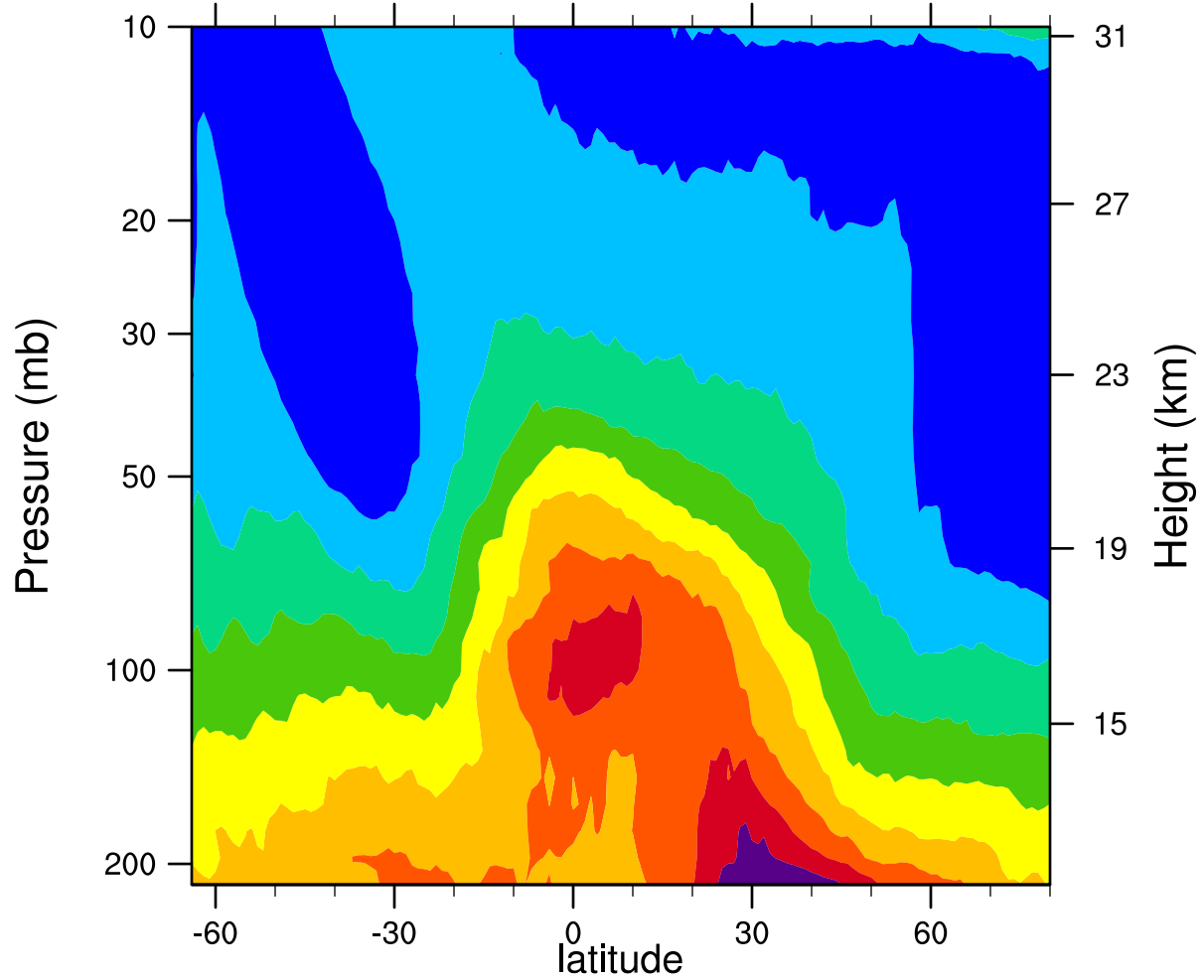
2005d159 12.1MicronExtinction_Combined (km -1 )
