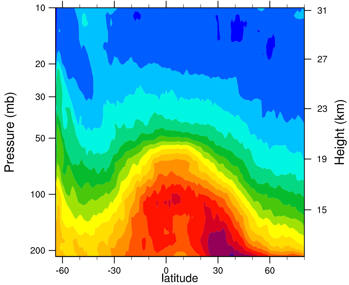
2006d211 12.1MicronExtinction_Combined (km -1 )
