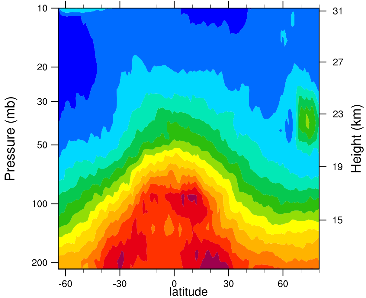
2005d363 12.1MicronExtinction_Combined (km -1 )
