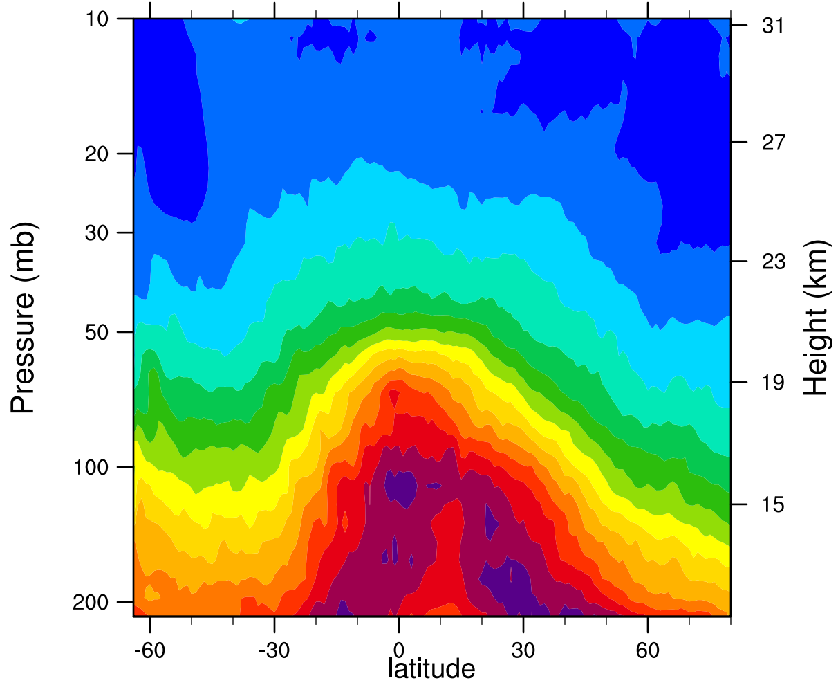
2006d241 12.1MicronExtinction_Combined (km -1 )
