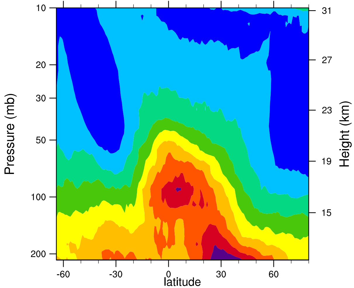
2005d150 12.1MicronExtinction_Combined ( \text{km}^{-1} )
