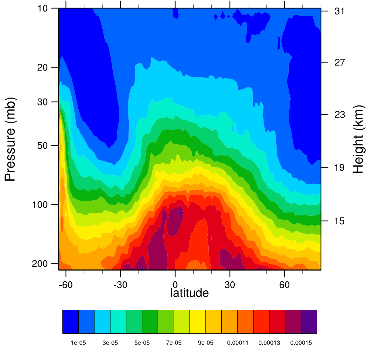
2005d240 12.1MicronExtinction_Combined (km -1 )
