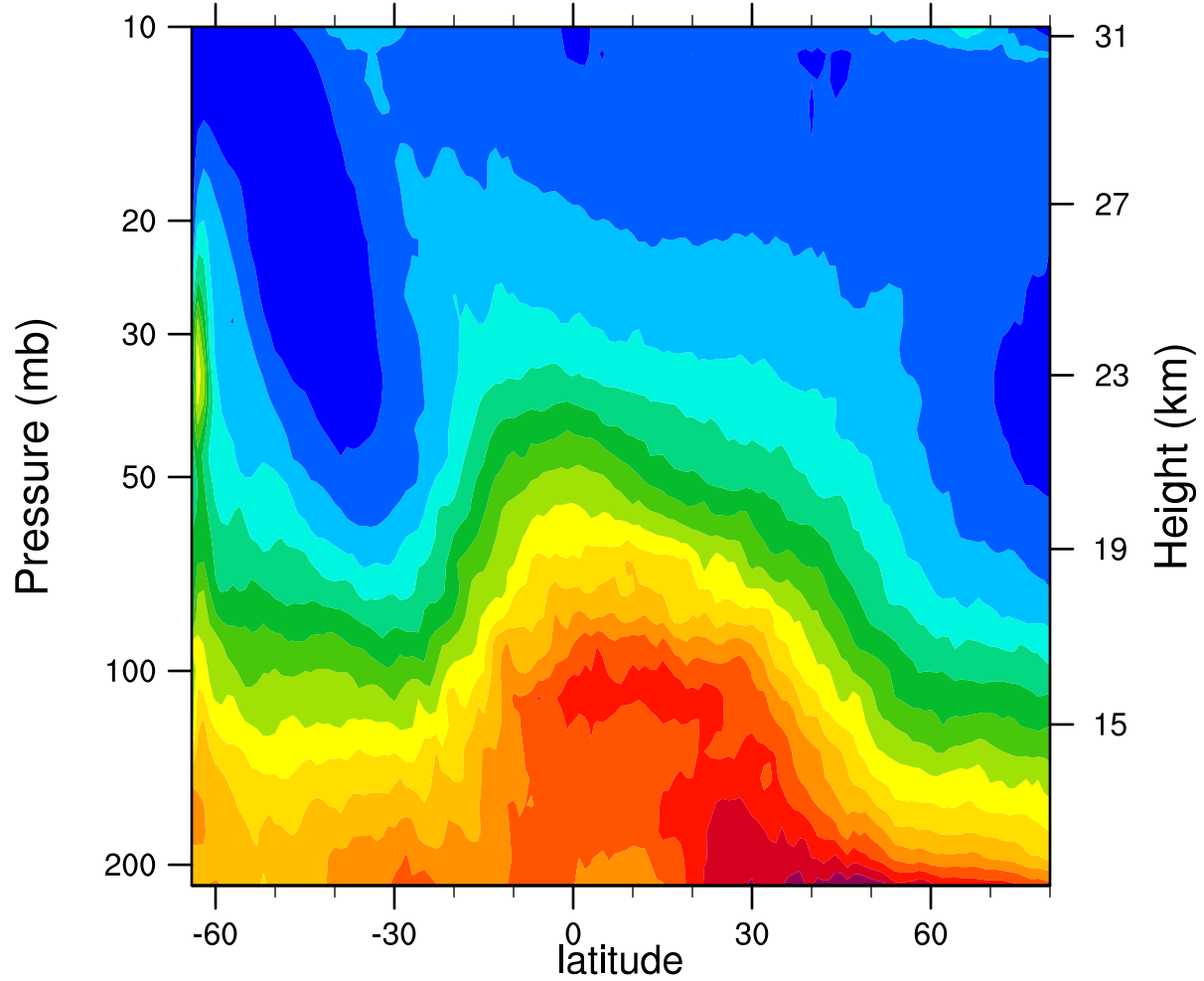
2005d201 12.1MicronExtinction_Combined (km -1 )
