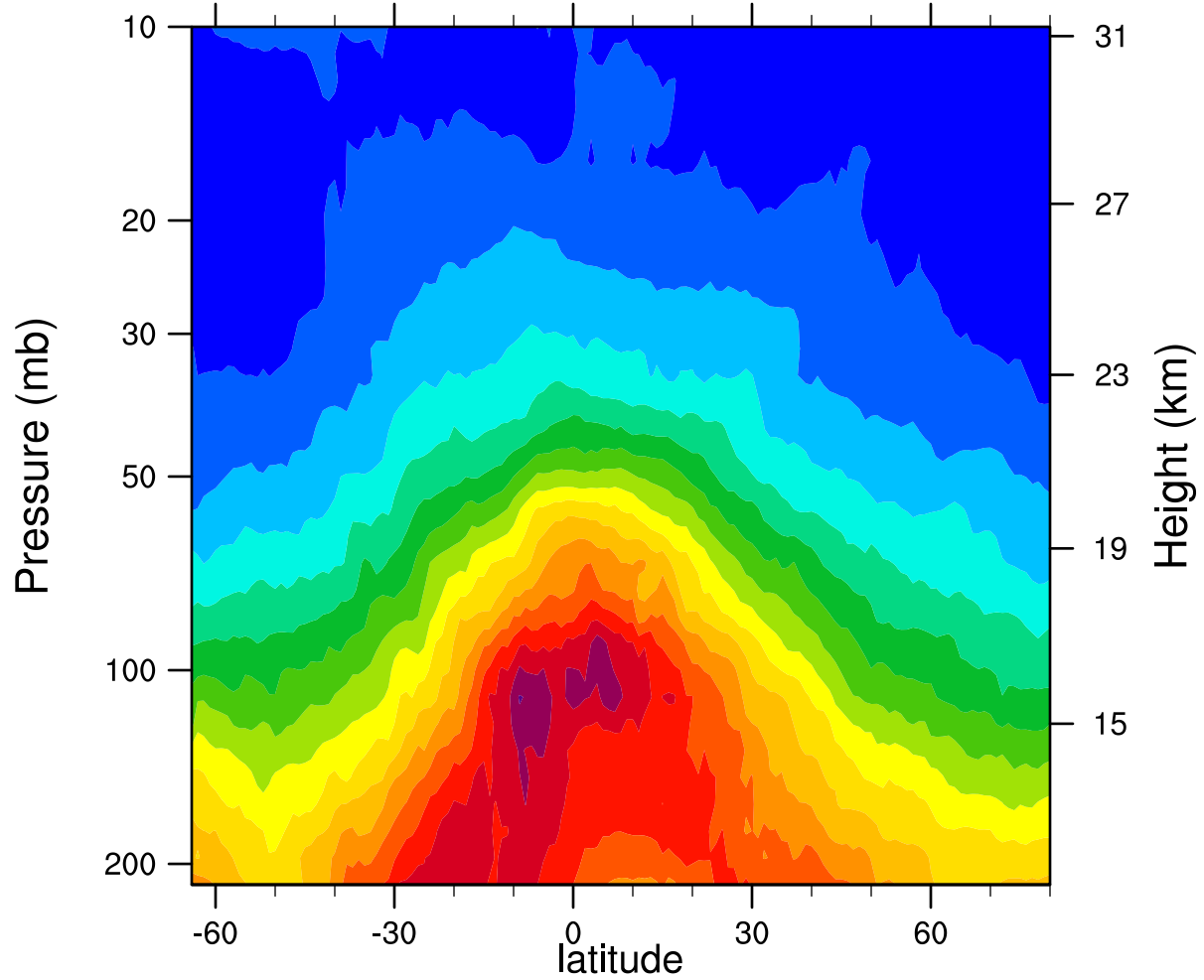
2006d291 12.1MicronExtinction_Combined (km -1 )
