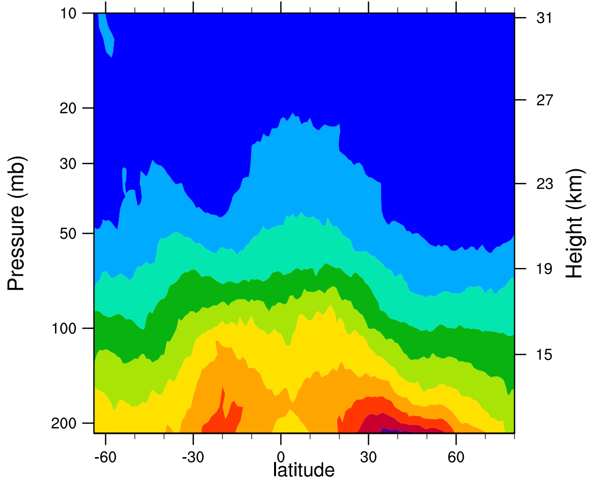
2007d149 12.1MicronExtinction_Combined (km -1 )
