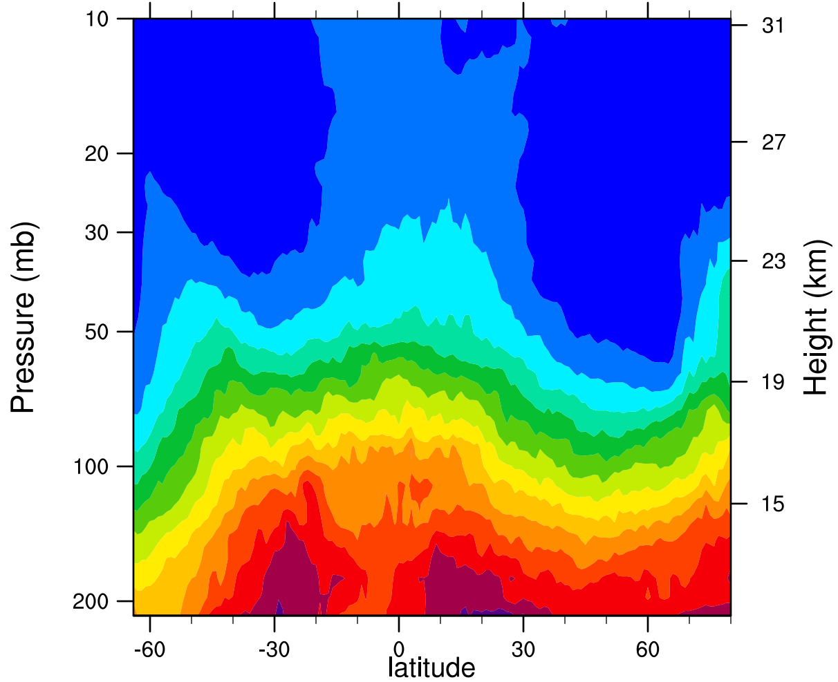
2007d360 12.1MicronExtinction_Combined ( \text{km}^{-1} )
