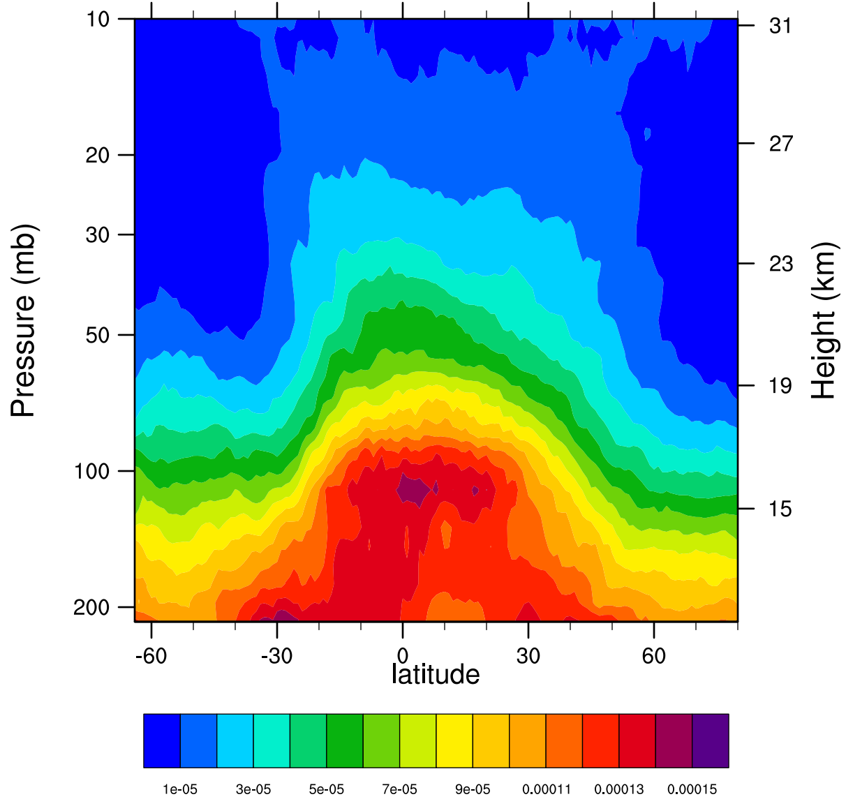
2005d270 12.1MicronExtinction_Combined (km -1 )
