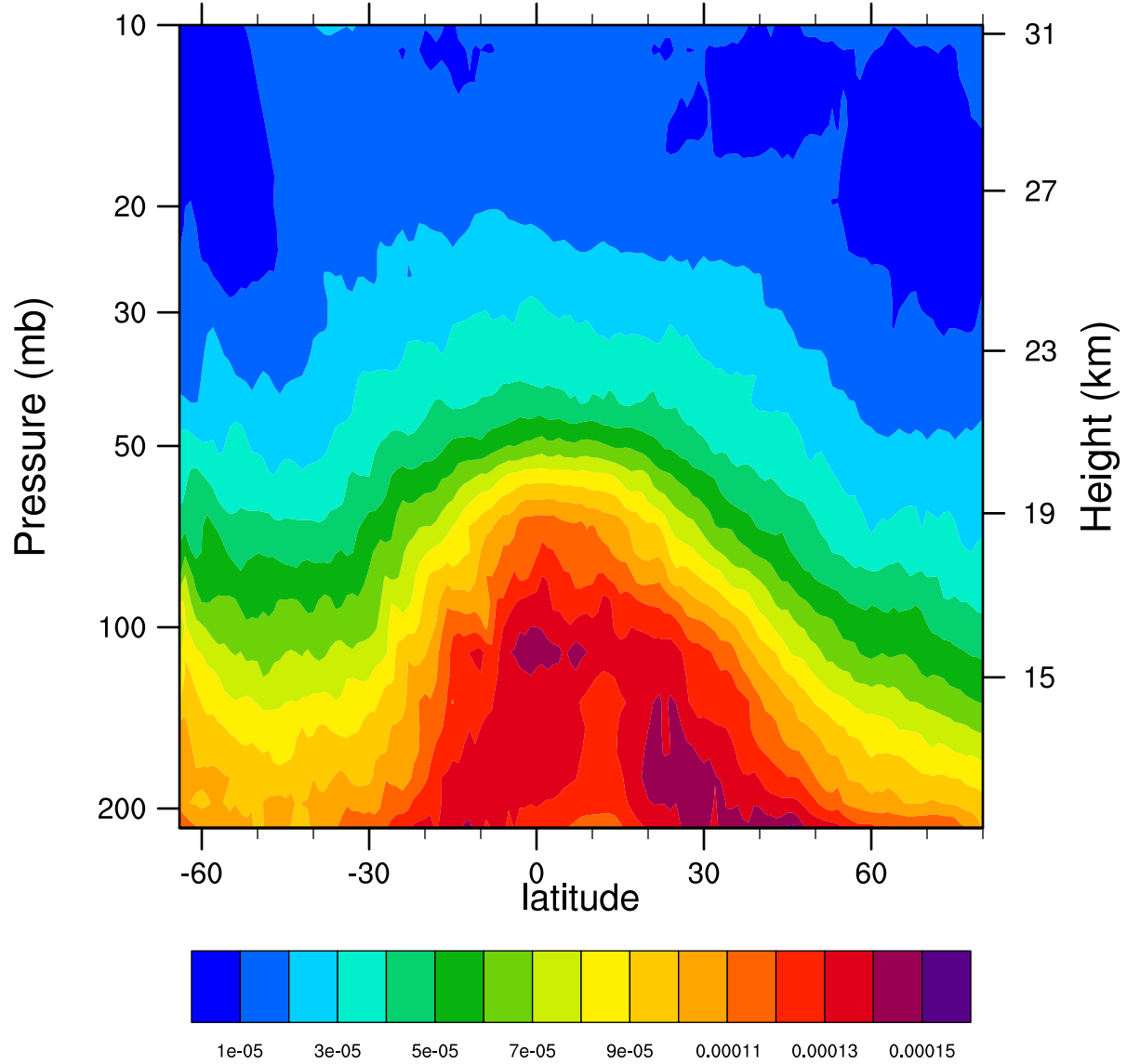
2006d237 12.1MicronExtinction_Combined (km -1 )
