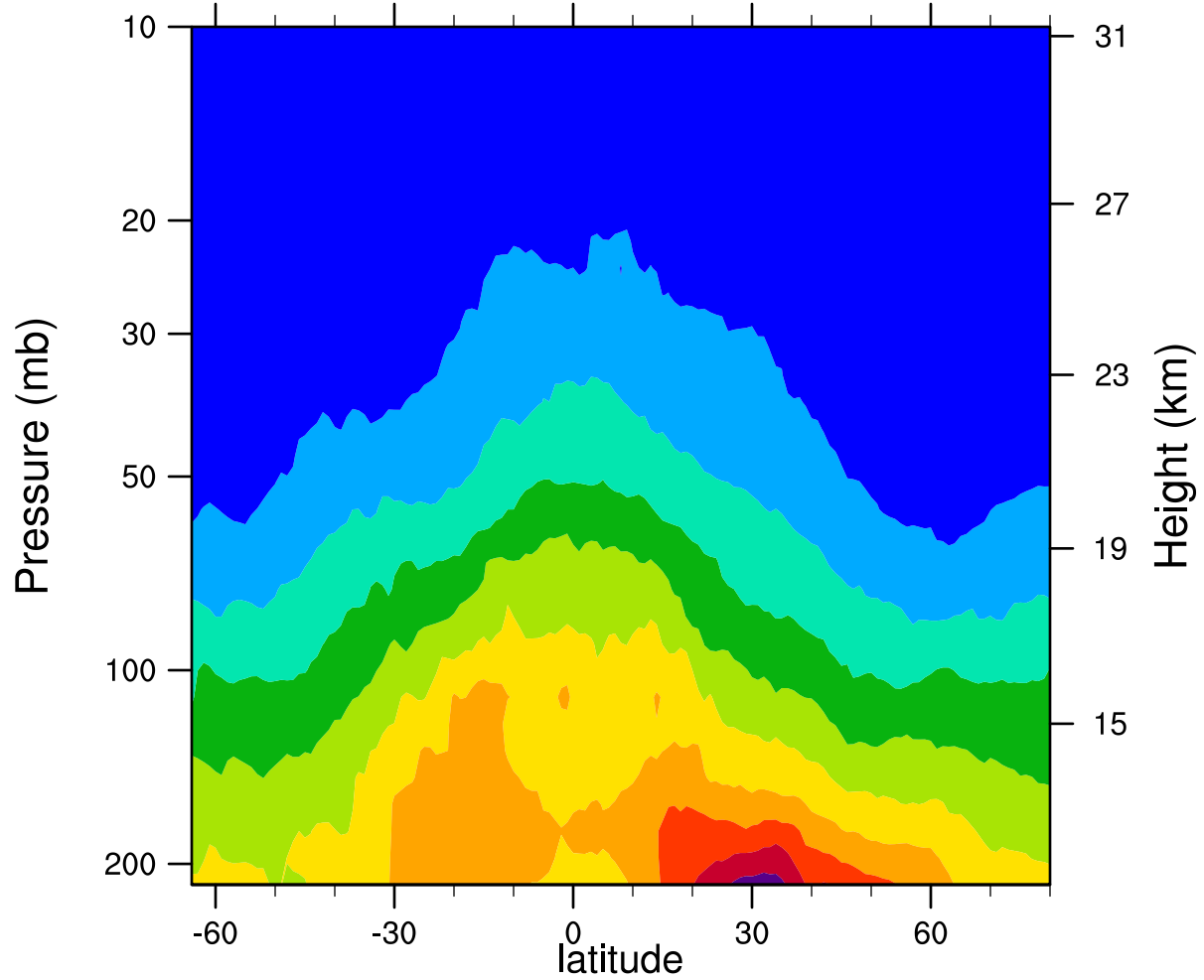
2007d120 12.1MicronExtinction_Combined (km -1 )
