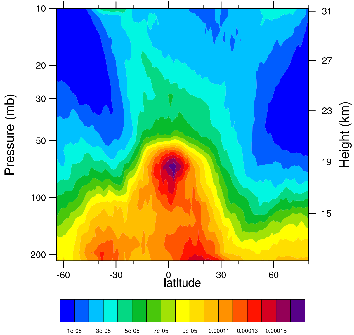
2005d065 12.1MicronExtinction_Combined ( \text{km}^{-1} )
