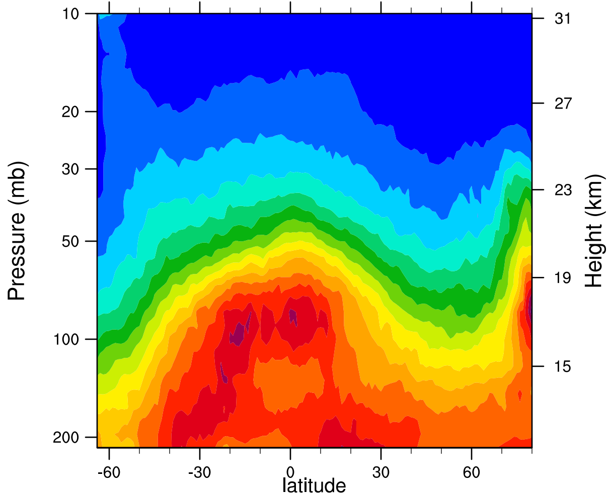
2007d021 12.1MicronExtinction_Combined (km -1 )
