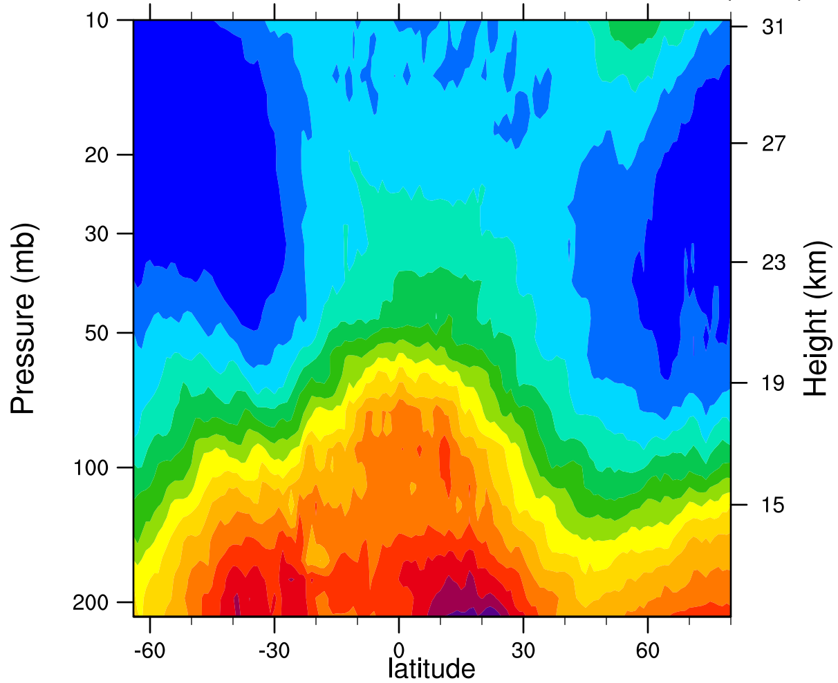
2005d032 12.1MicronExtinction_Combined (km -1 )
