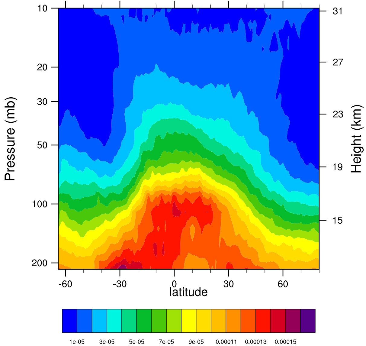
2005d275 12.1MicronExtinction_Combined (km -1 )
