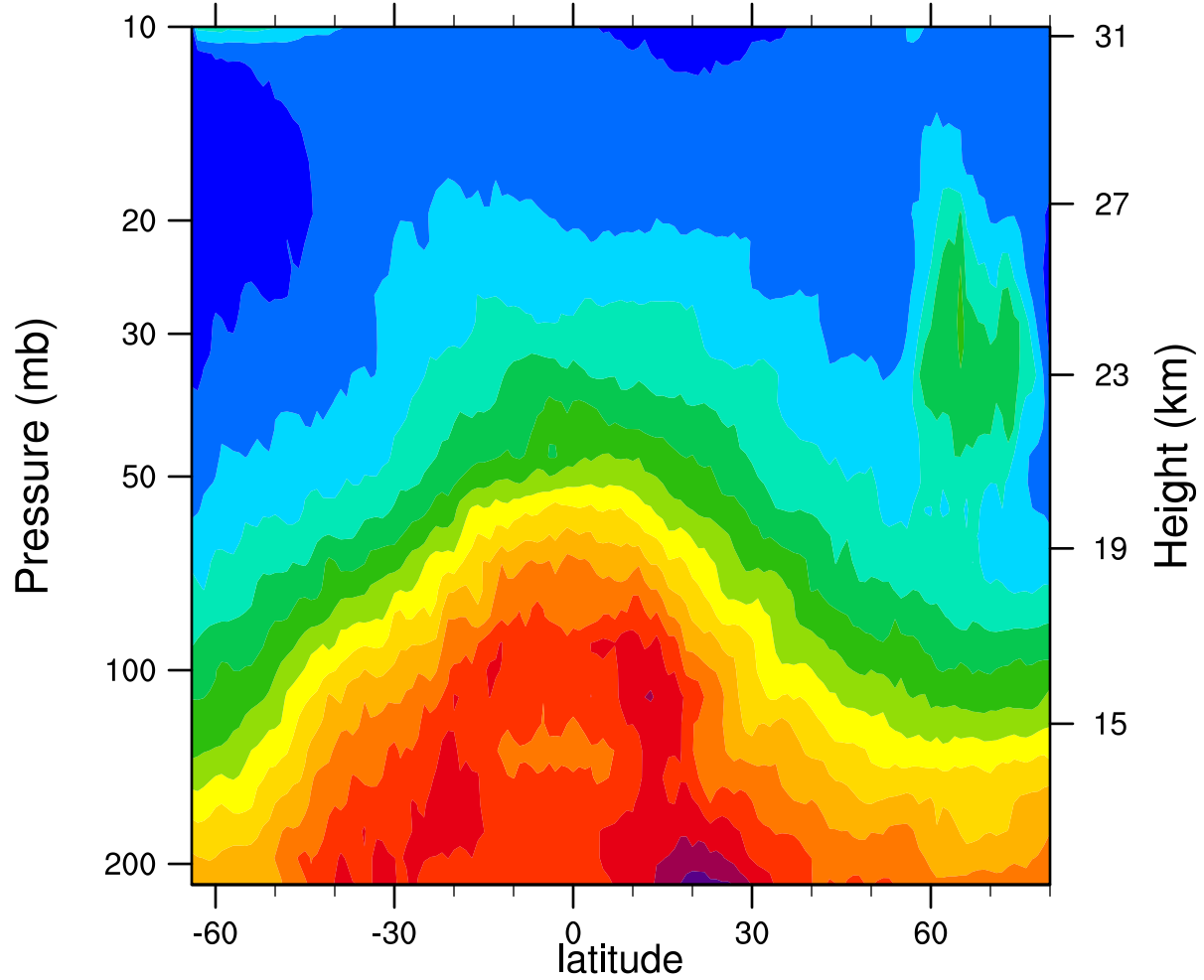
2006d008 12.1MicronExtinction_Combined (km -1 )
