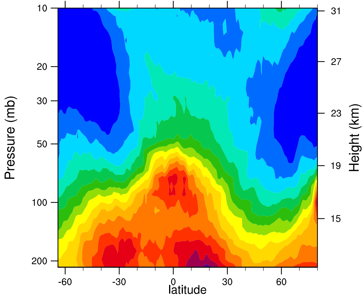
2005d041 12.1MicronExtinction_Combined (km -1 )
