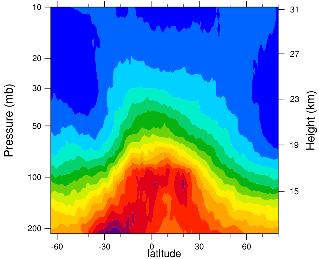
2005d288 12.1MicronExtinction_Combined (km -1 )
