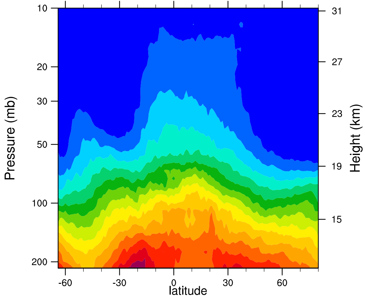
2007d271 12.1MicronExtinction_Combined (km -1 )
