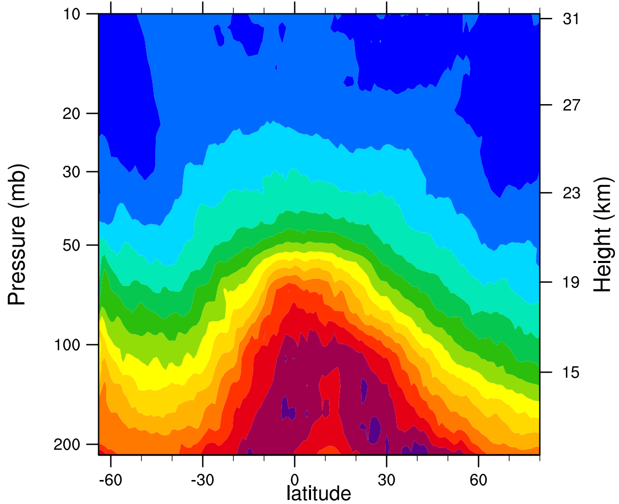
2006d249 12.1MicronExtinction_Combined (km -1 )
