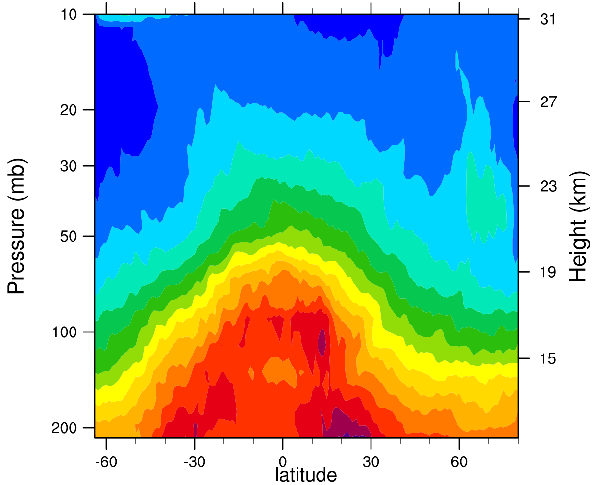
2006d003 12.1MicronExtinction_Combined (km -1 )
