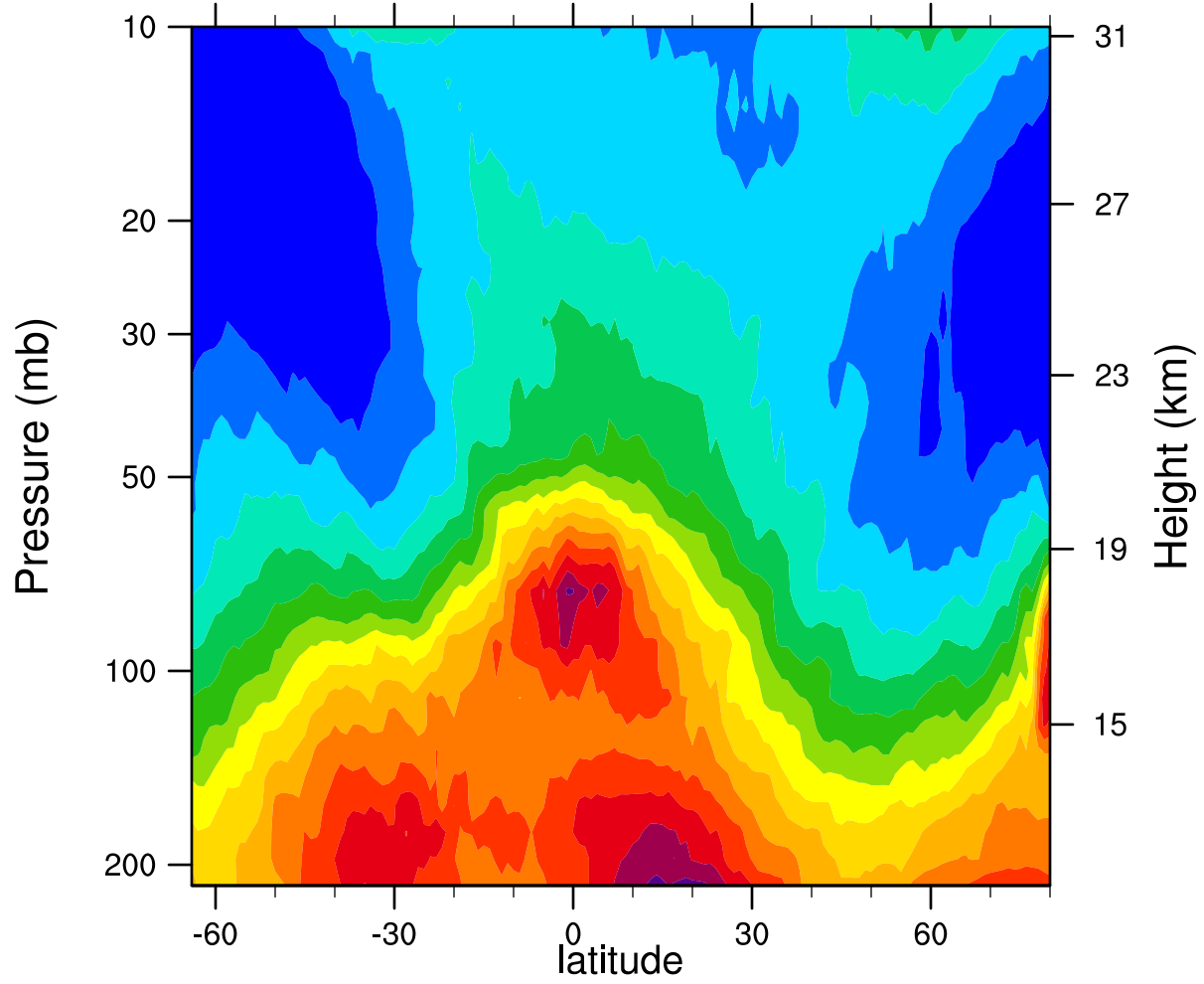
2005d044 12.1MicronExtinction_Combined (km -1 )
