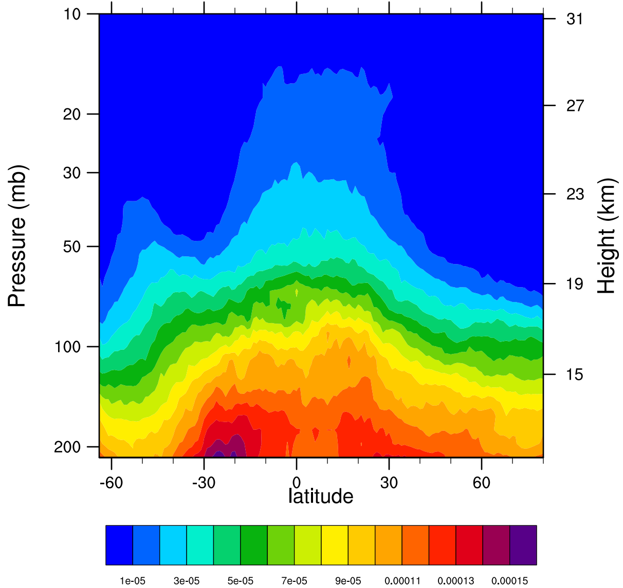
2007d306 12.1MicronExtinction_Combined (km -1 )
