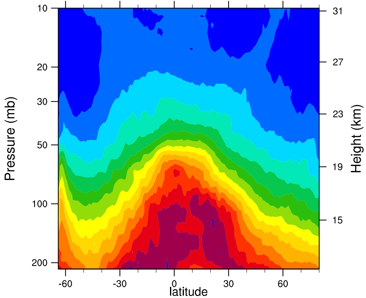
2006d267 12.1MicronExtinction_Combined (km -1 )
