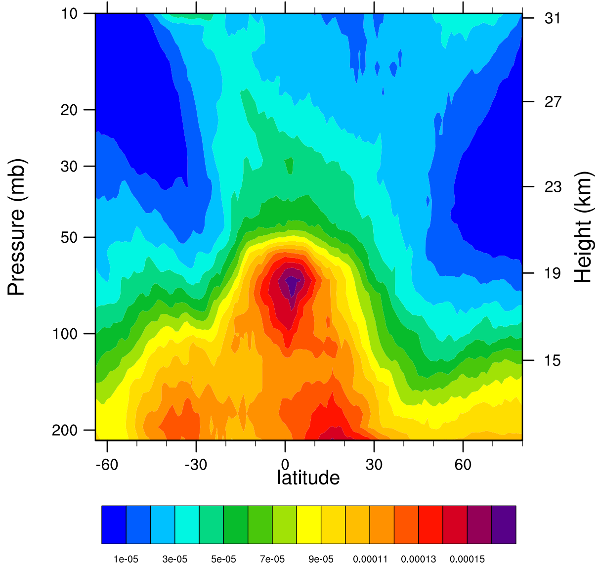
2005d063 12.1MicronExtinction_Combined (km -1 )
