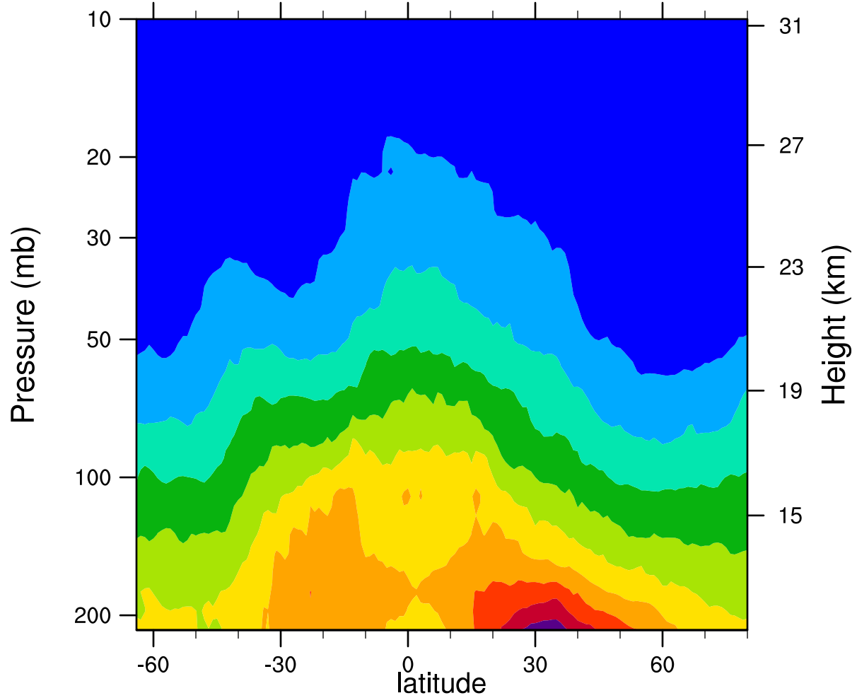
2007d127 12.1MicronExtinction_Combined (km -1 )
