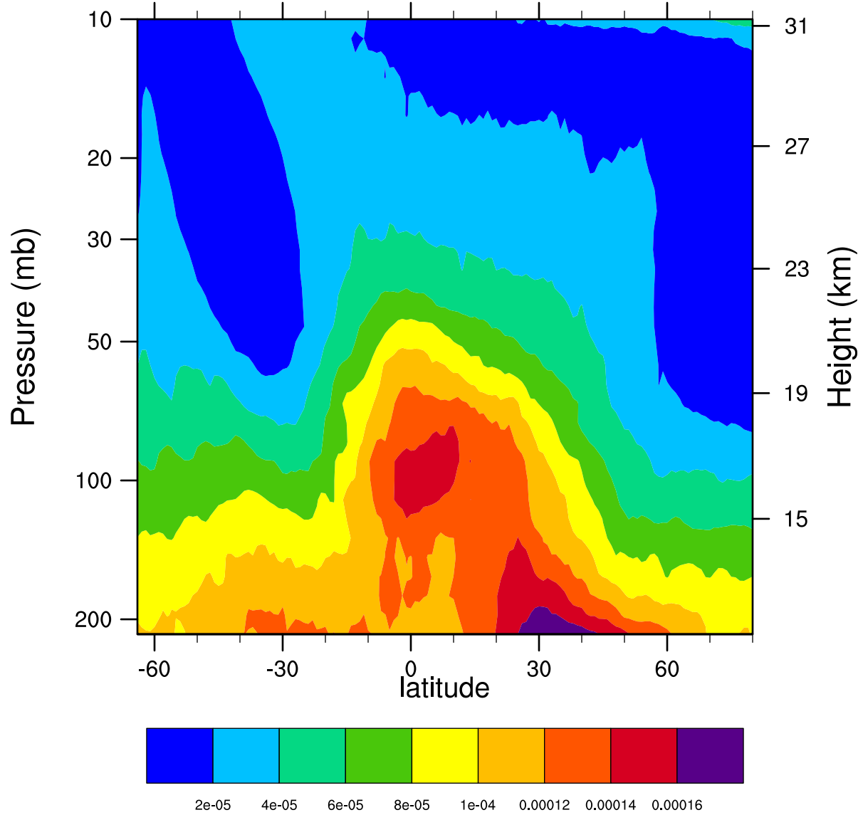
2005d156 12.1MicronExtinction_Combined (km -1 )
