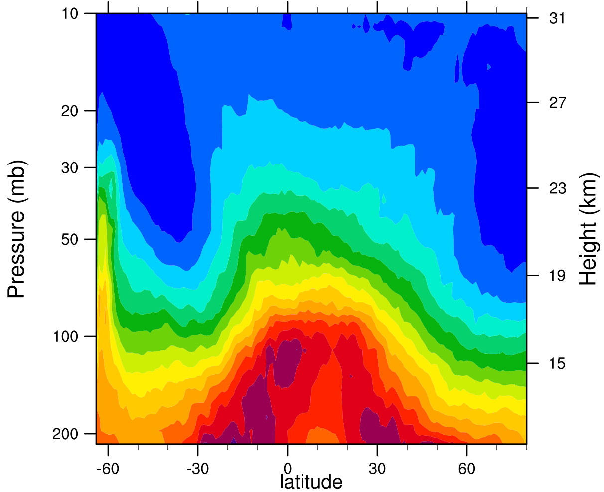
2005d241 12.1MicronExtinction_Combined (km -1 )
