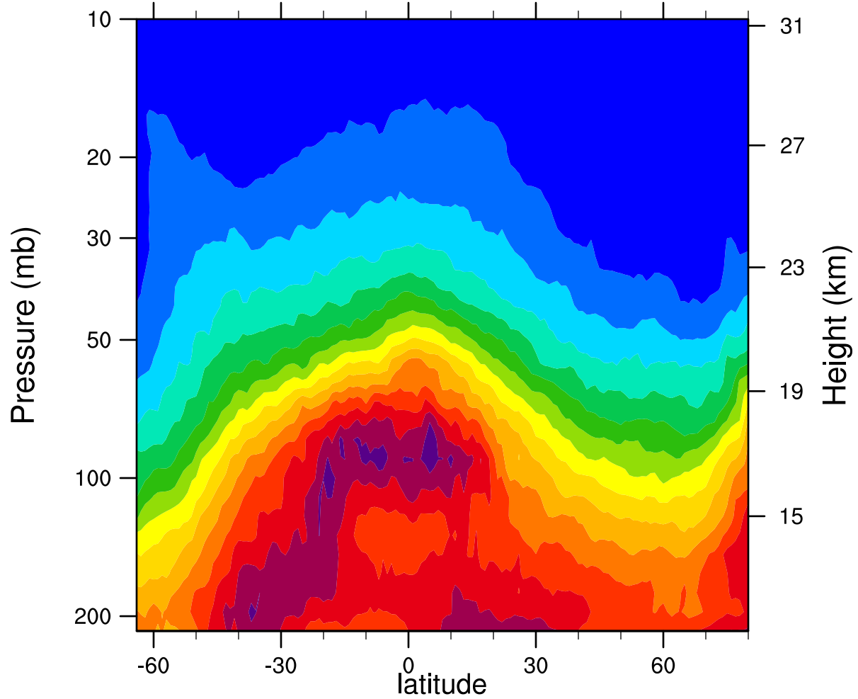
2007d013 12.1MicronExtinction_Combined (km -1 )
