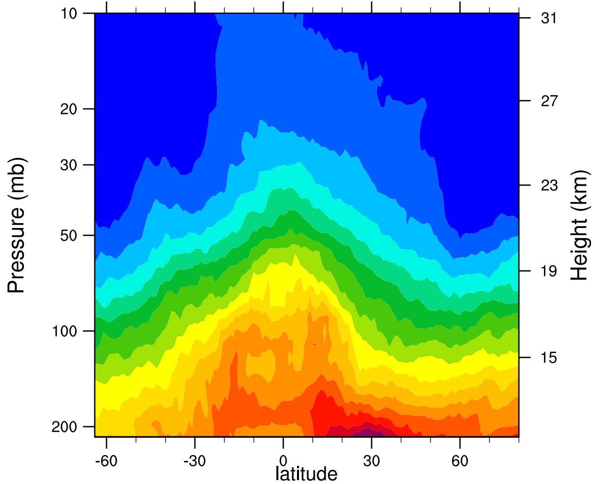
2007d097 12.1MicronExtinction_Combined (km -1 )
