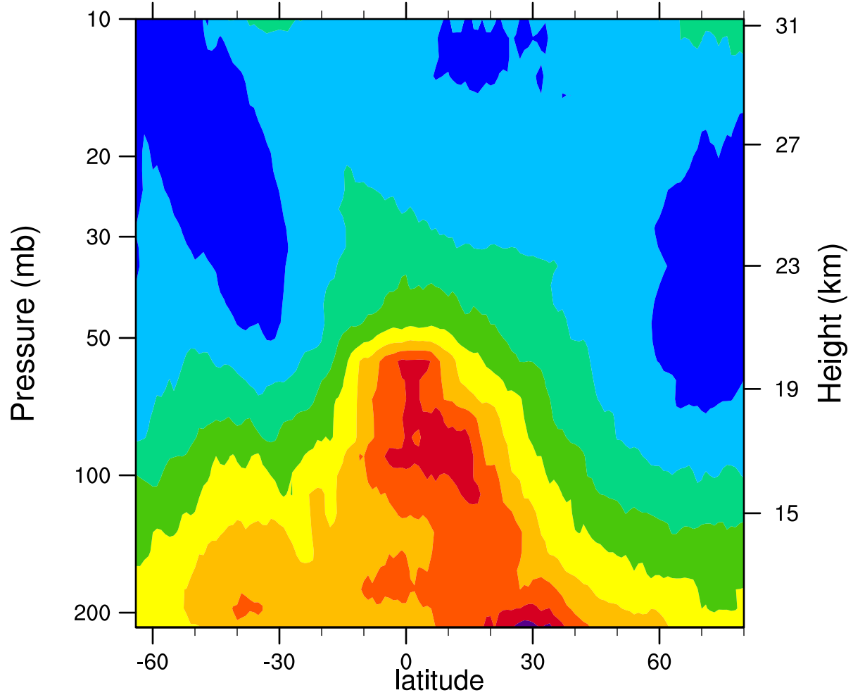
2005d105 12.1MicronExtinction_Combined (km -1 )
