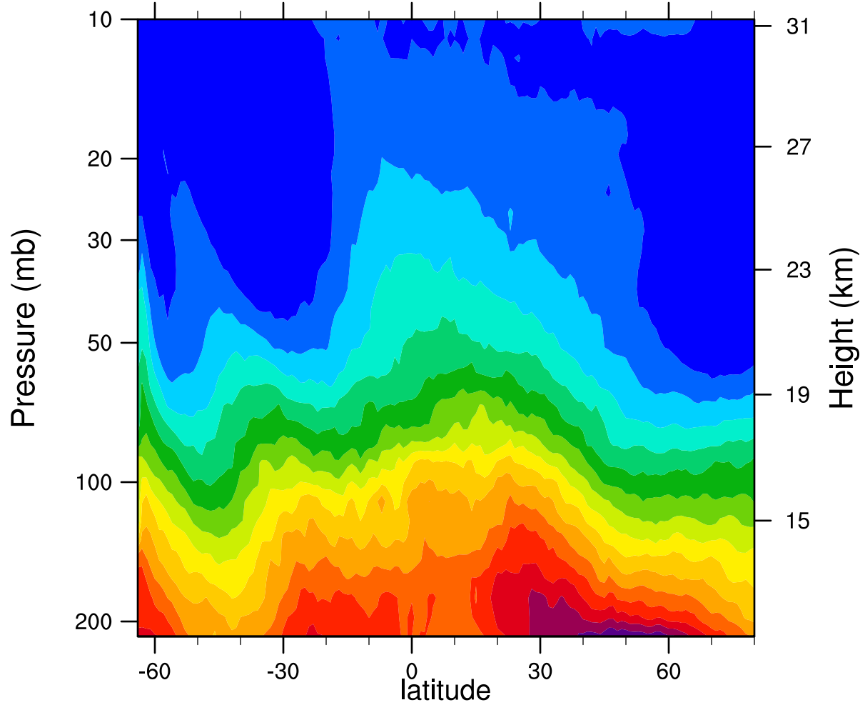
2007d226 12.1MicronExtinction_Combined (km -1 )
