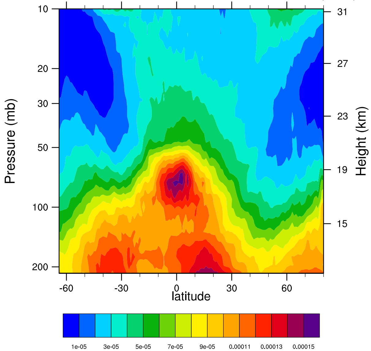
2005d048 12.1MicronExtinction_Combined (km -1 )
