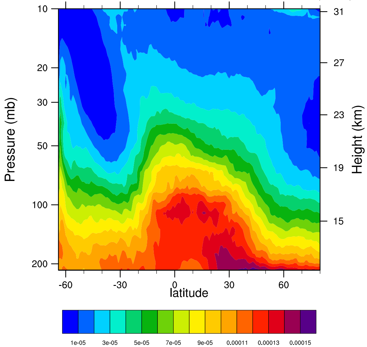
2005d204 12.1MicronExtinction_Combined ( \text{km}^{-1} )
