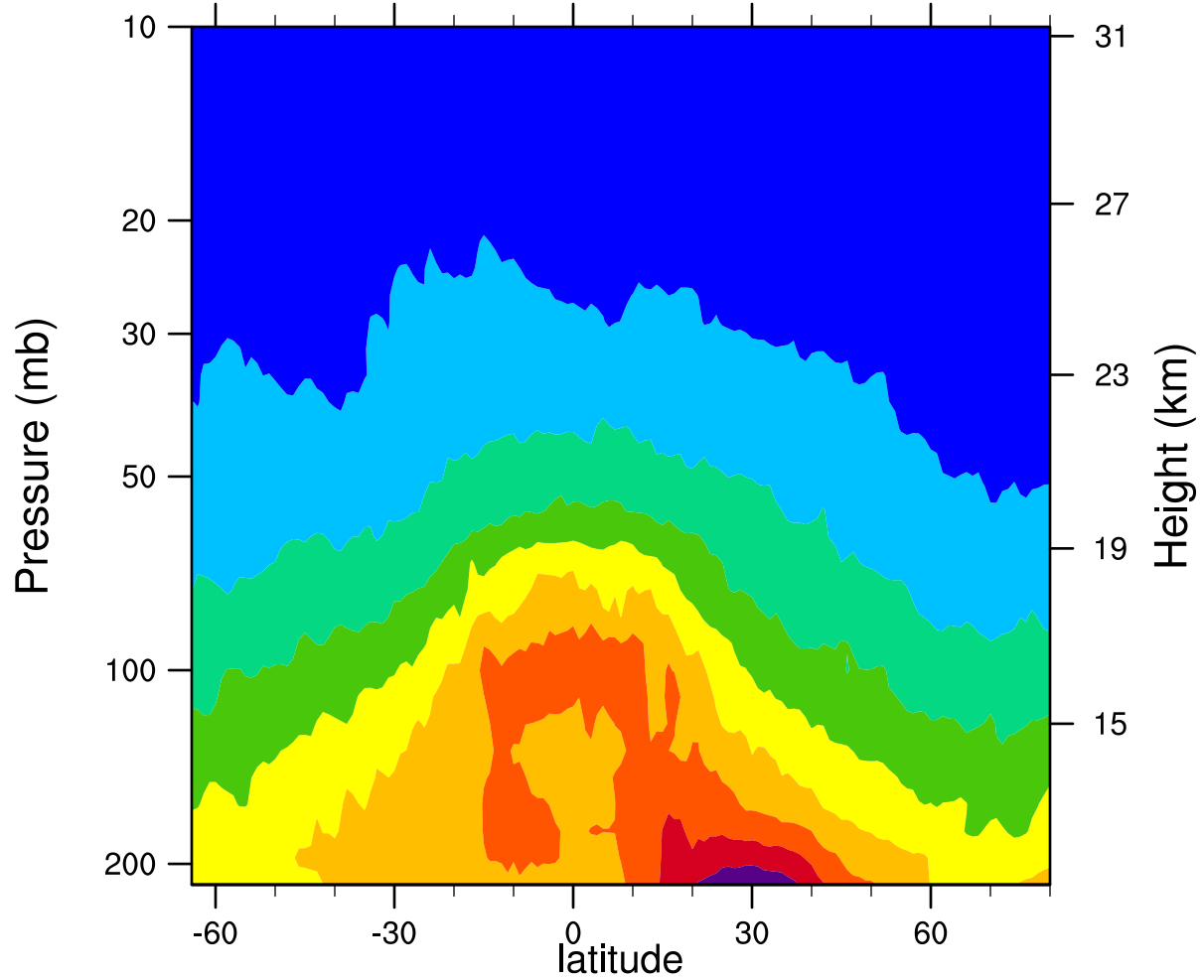
2006d110 12.1MicronExtinction_Combined (km -1 )
