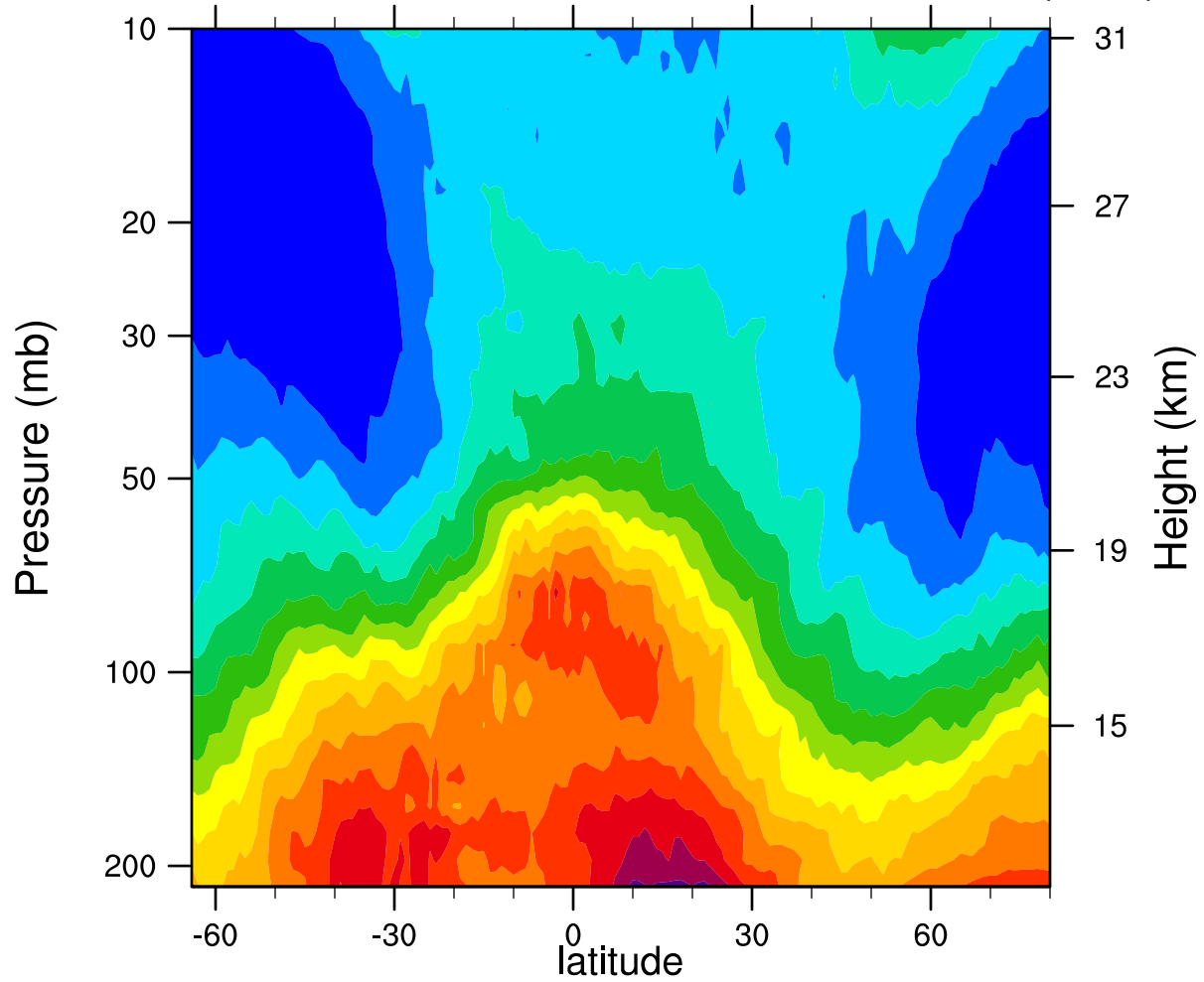
2005d038 12.1MicronExtinction_Combined (km -1 )
