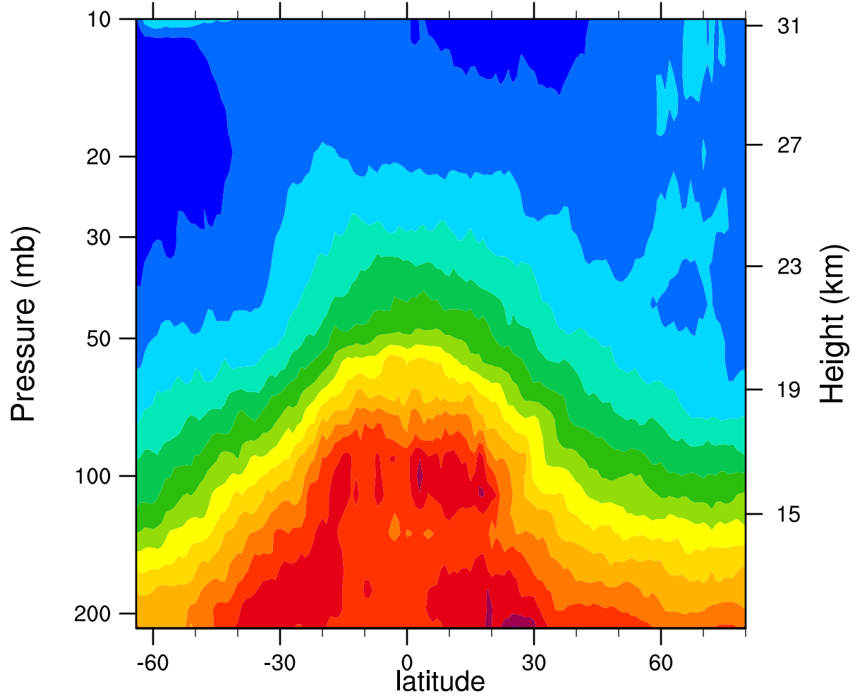
2005d353 12.1MicronExtinction_Combined (km -1 )
