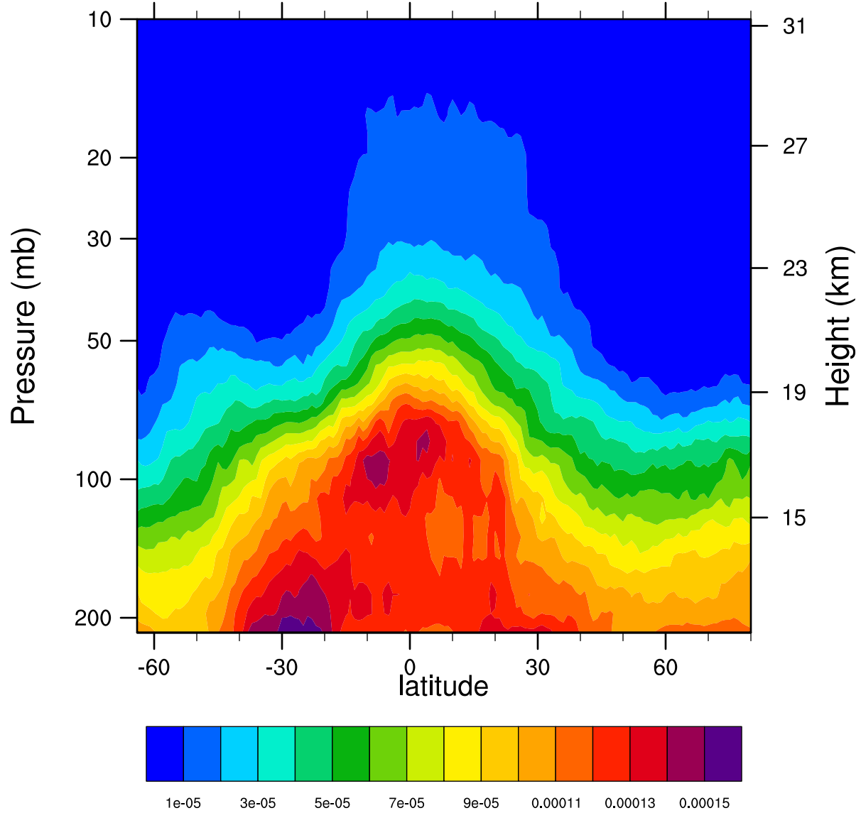
2006d331 12.1MicronExtinction_Combined (km -1 )
