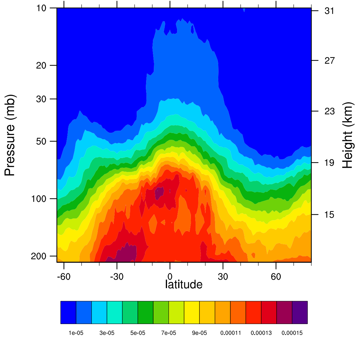
2006d337 12.1MicronExtinction_Combined (km -1 )
