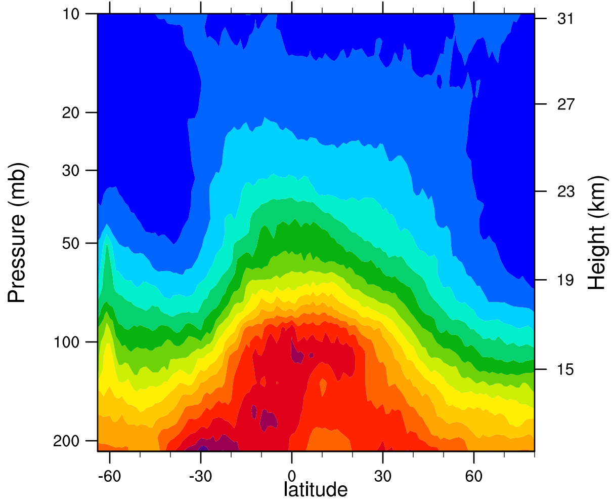
2005d277 12.1MicronExtinction_Combined (km -1 )
