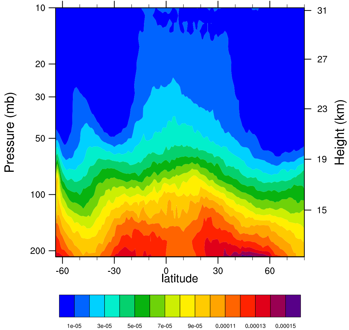
2007d246 12.1MicronExtinction_Combined (km -1 )
