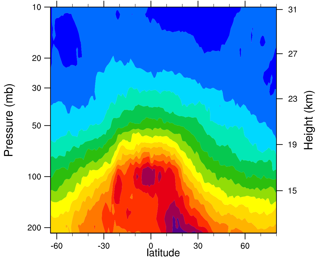
2006d077 12.1MicronExtinction_Combined ( \text{km}^{-1} )
