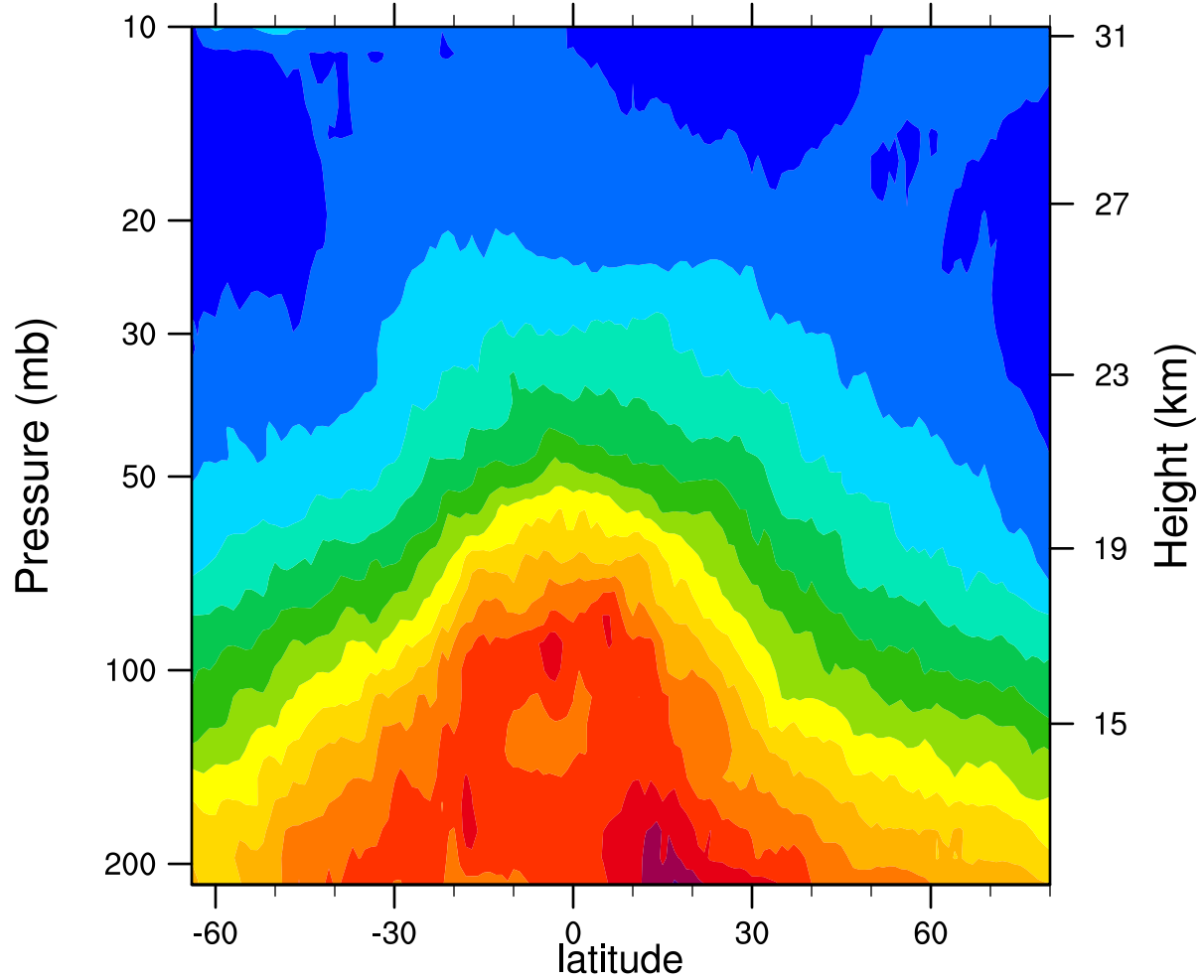
2006d044 12.1MicronExtinction_Combined ( \text{km}^{-1} )
