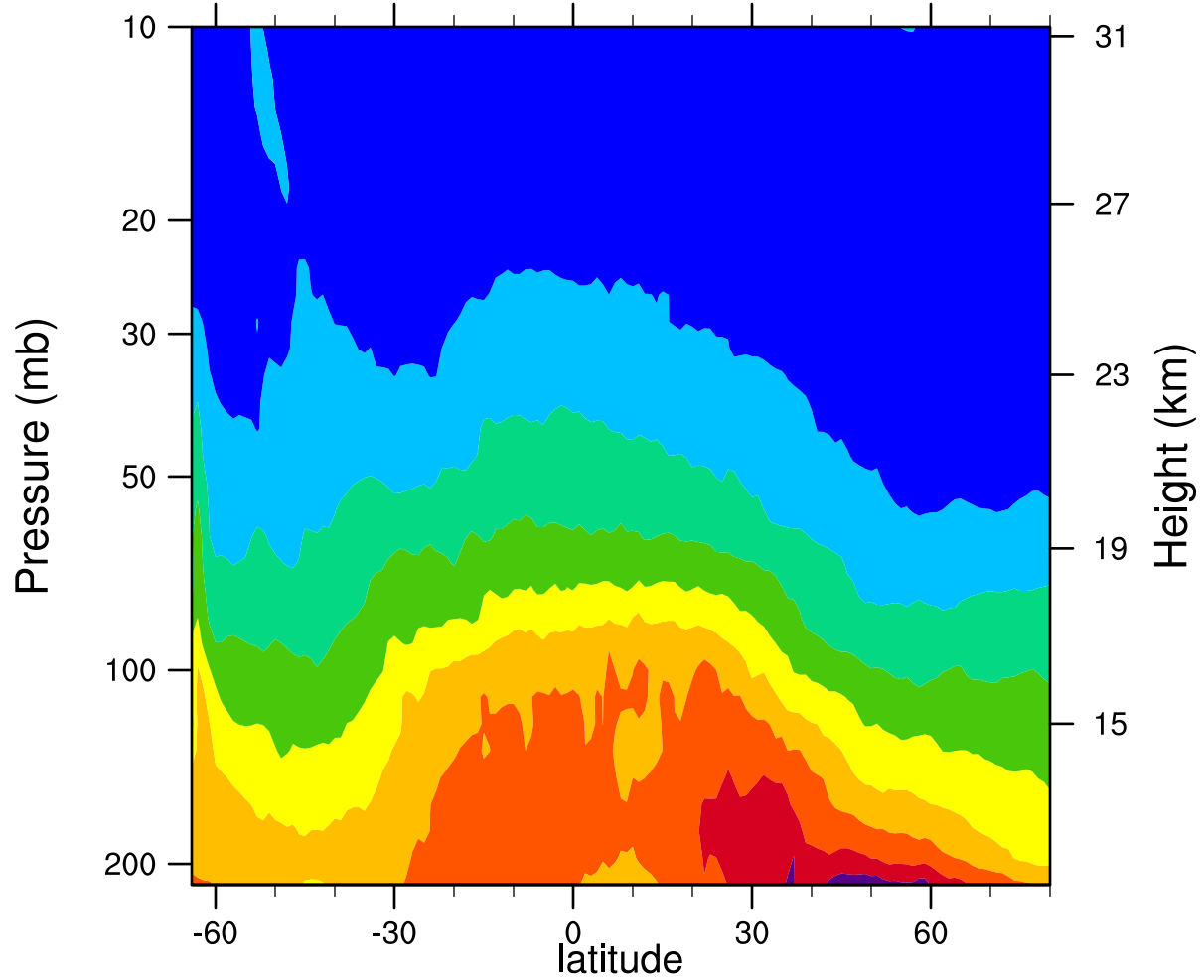
2007d203 12.1MicronExtinction_Combined (km -1 )
