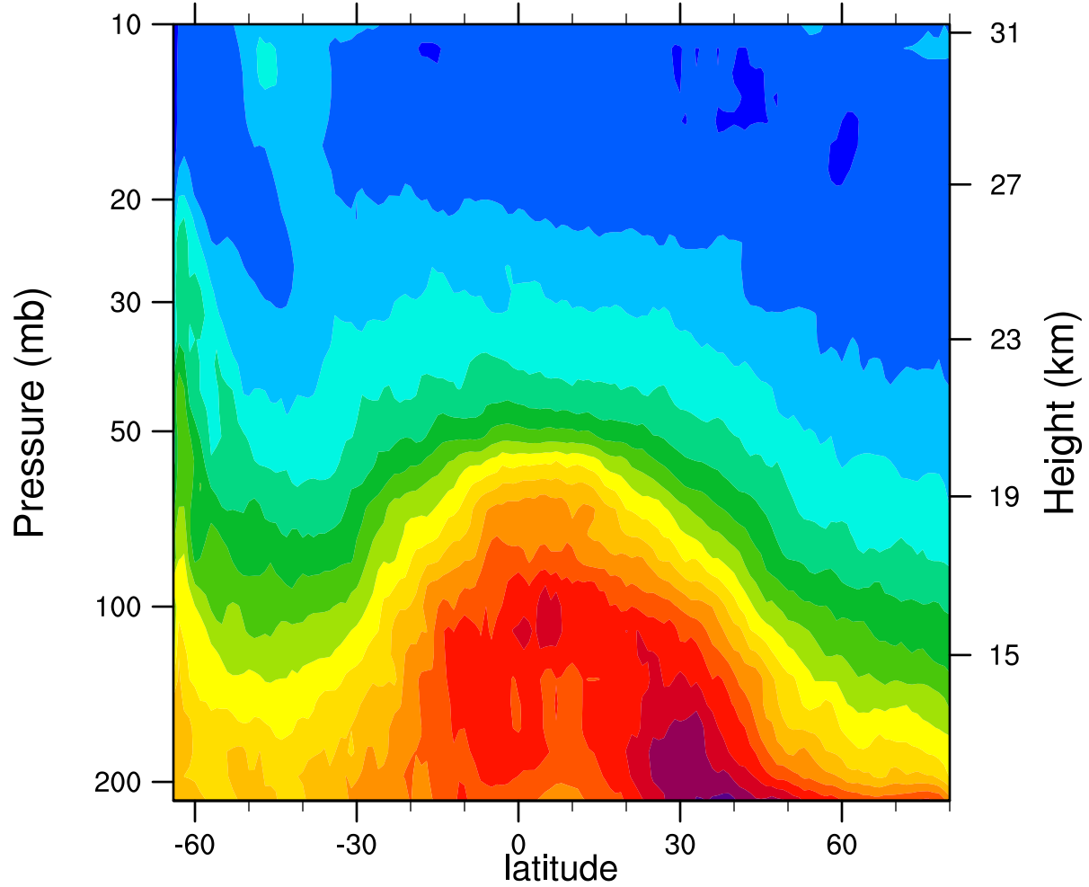
2006d209 12.1MicronExtinction_Combined ( \text{km}^{-1} )
