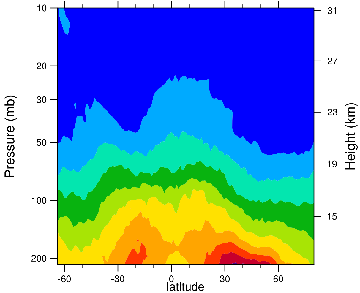
2007d146 12.1MicronExtinction_Combined (km -1 )
