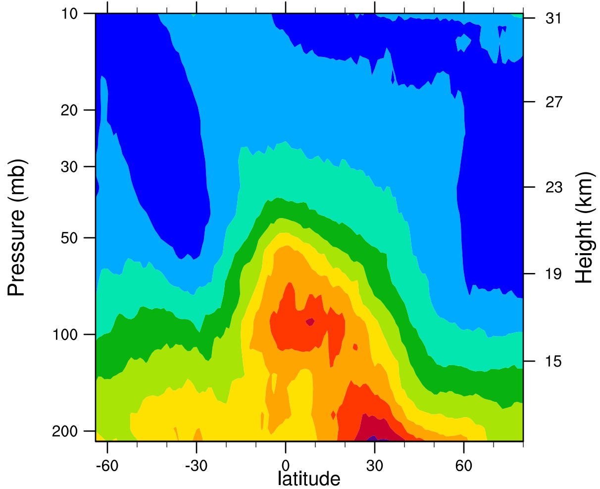
2005d141 12.1MicronExtinction_Combined (km -1 )
