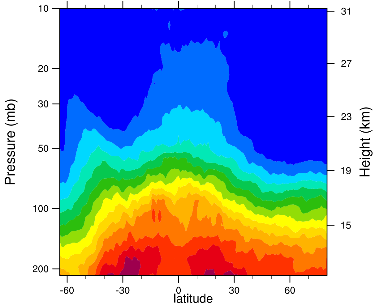
2007d330 12.1MicronExtinction_Combined (km -1 )
