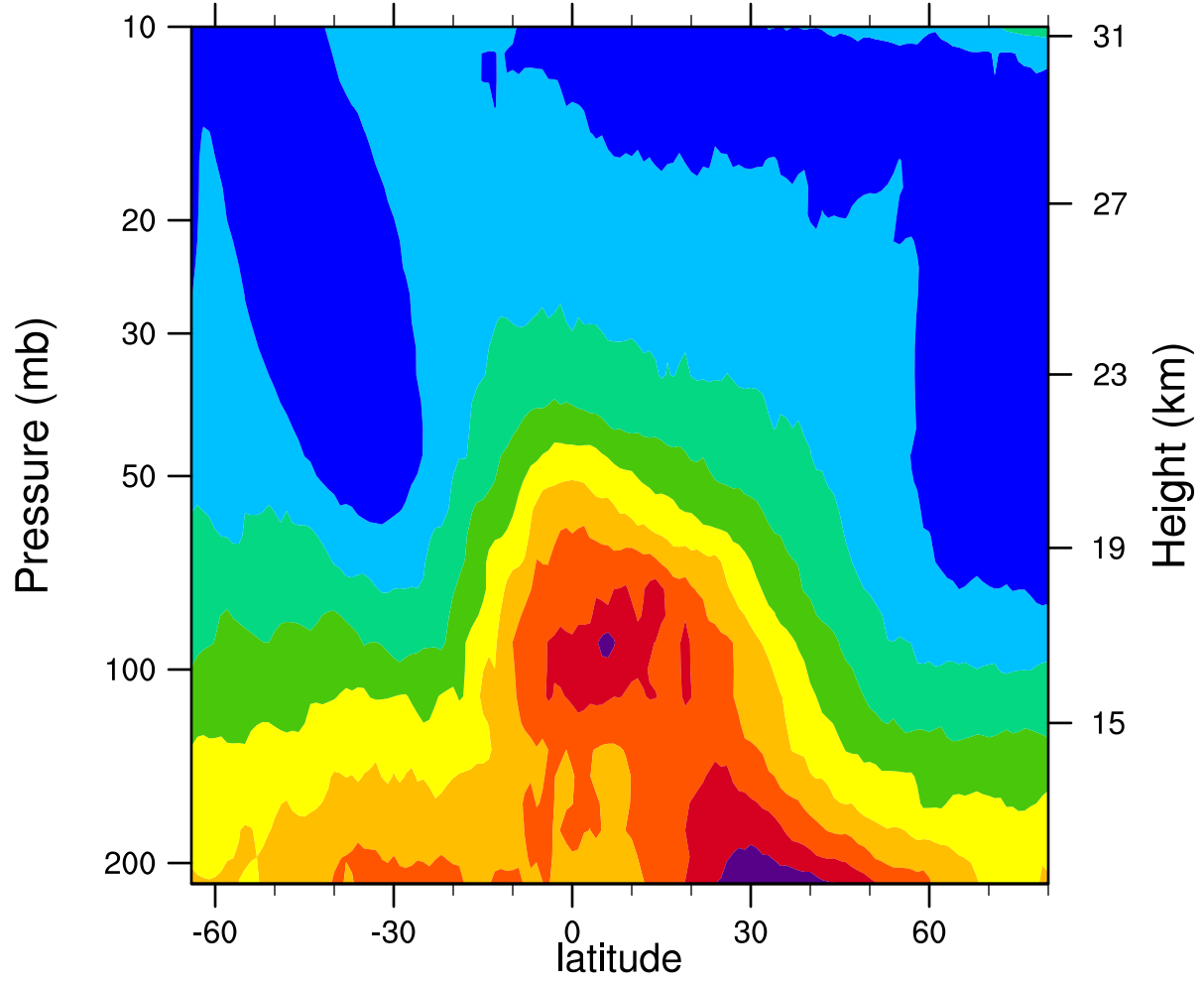
2005d153 12.1MicronExtinction_Combined (km -1 )
