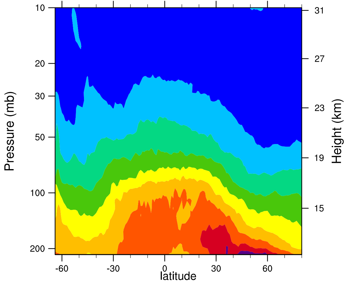
2007d202 12.1MicronExtinction_Combined (km -1 )
