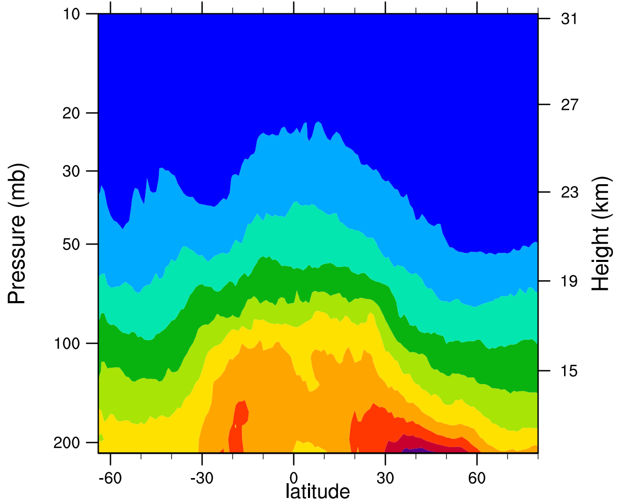
2007d163 12.1MicronExtinction_Combined (km -1 )
