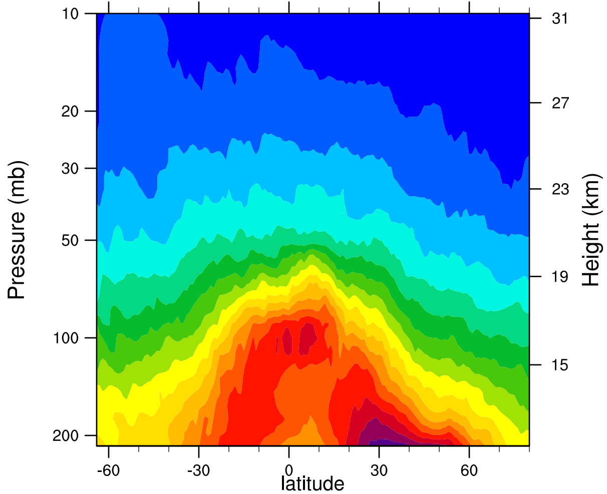
2006d157 12.1MicronExtinction_Combined (km -1 )
