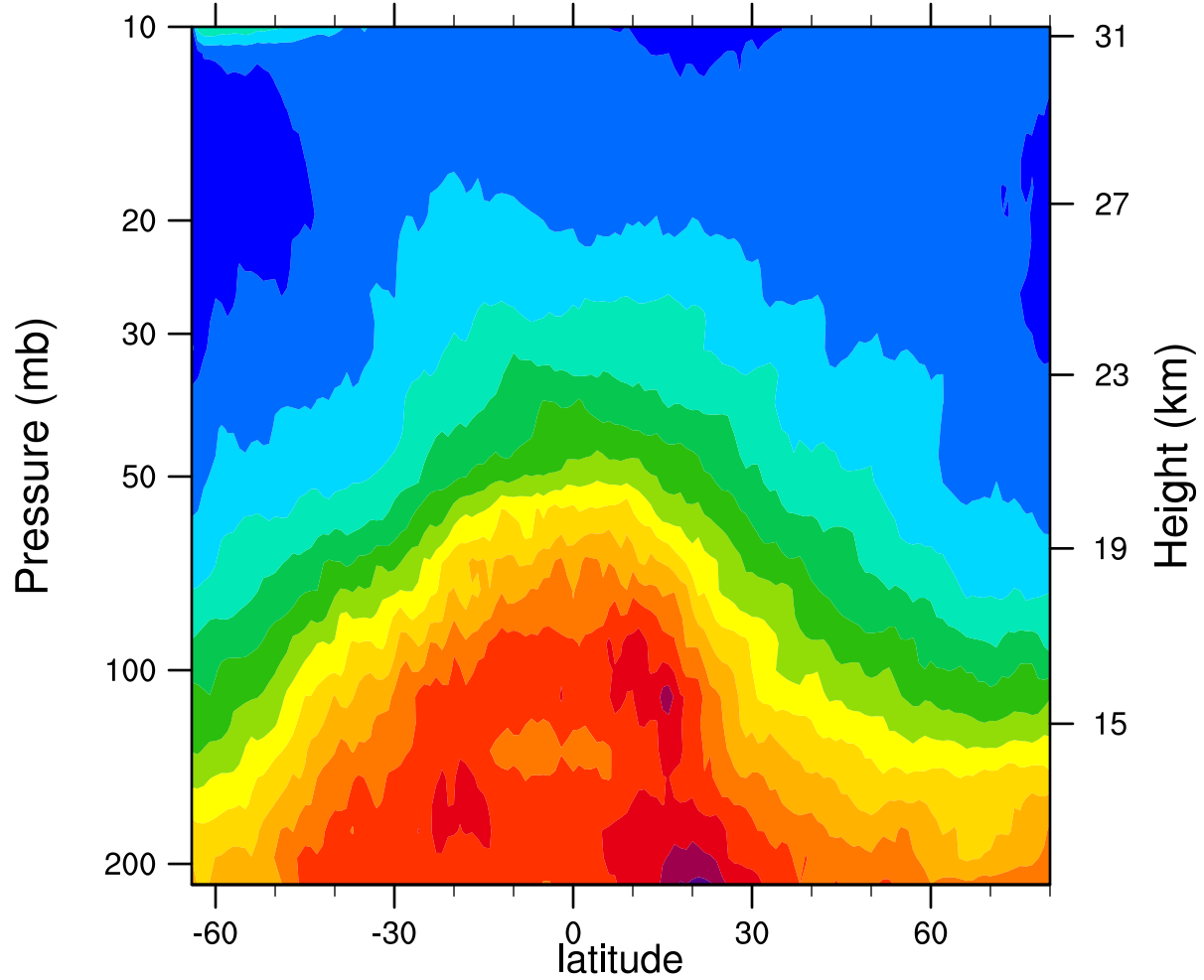
2006d014 12.1MicronExtinction_Combined (km -1 )
