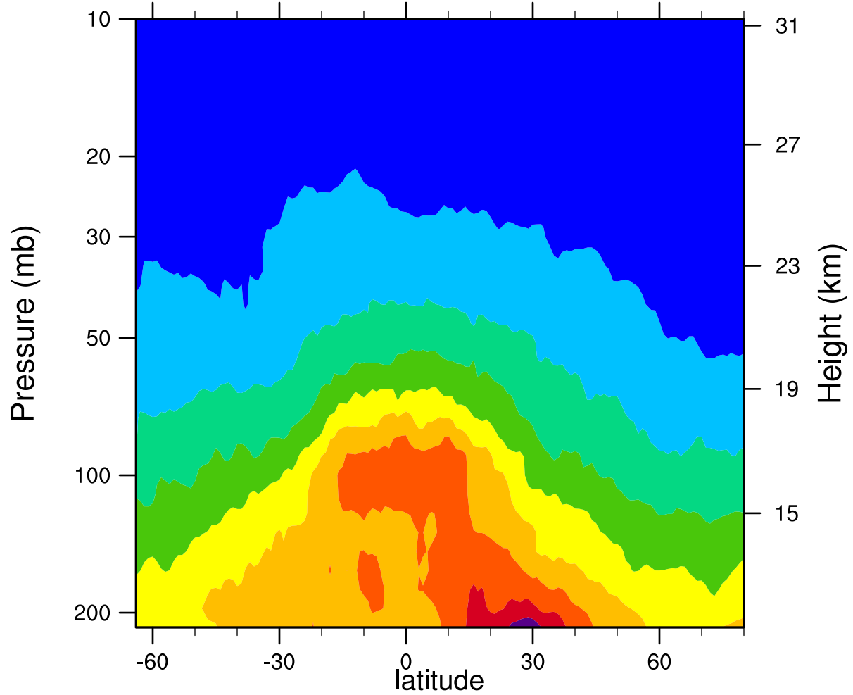
2006d100 12.1MicronExtinction_Combined (km -1 )
