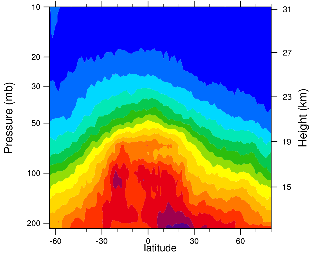
2007d057 12.1MicronExtinction_Combined (km -1 )
