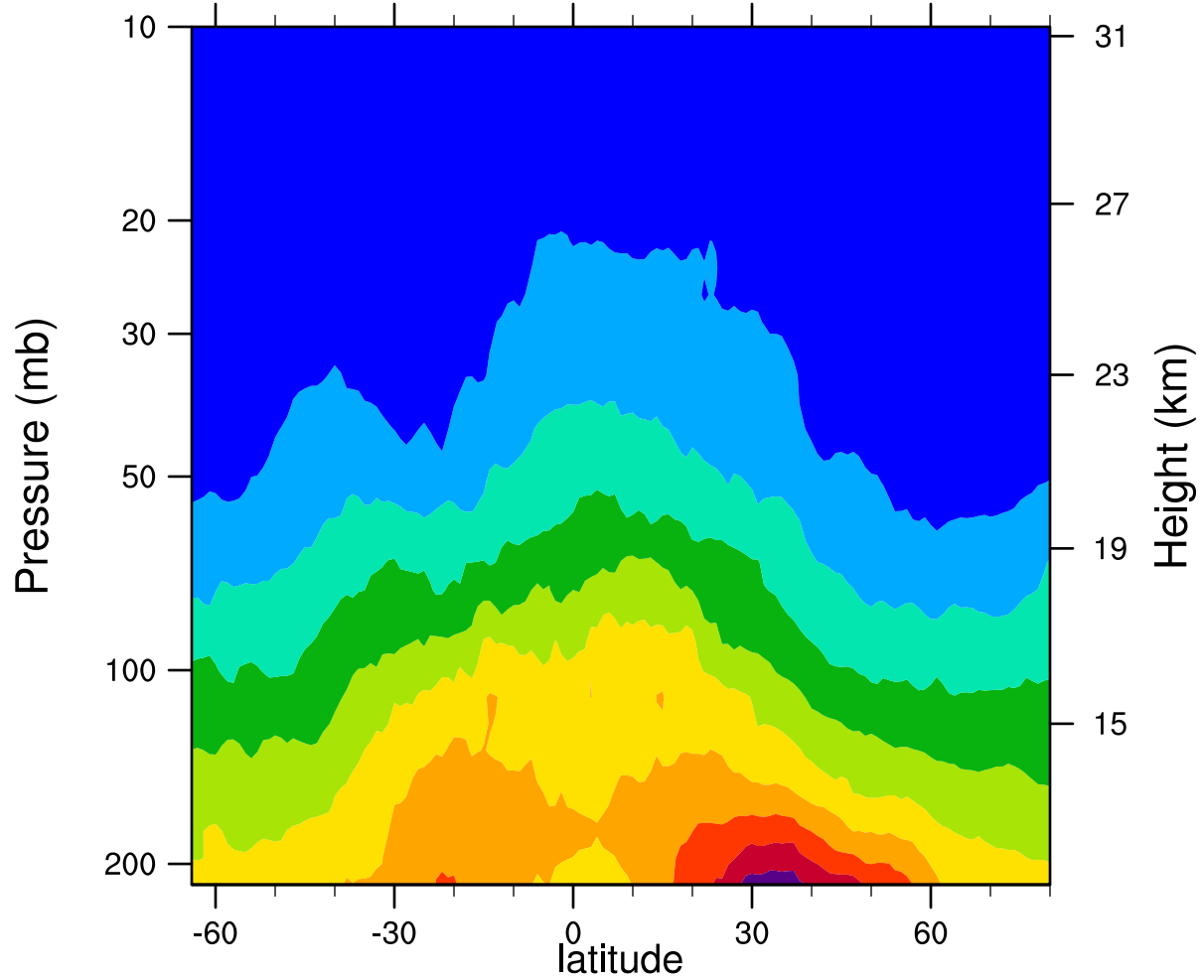
2007d136 12.1MicronExtinction_Combined (km -1 )
