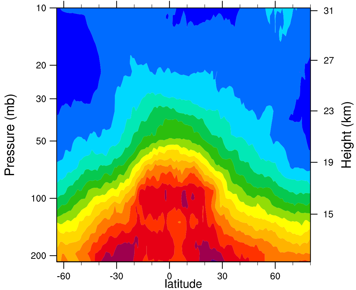
2005d326 12.1MicronExtinction_Combined (km -1 )
