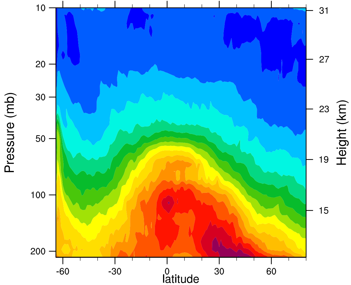
2006d226 12.1MicronExtinction_Combined (km -1 )
