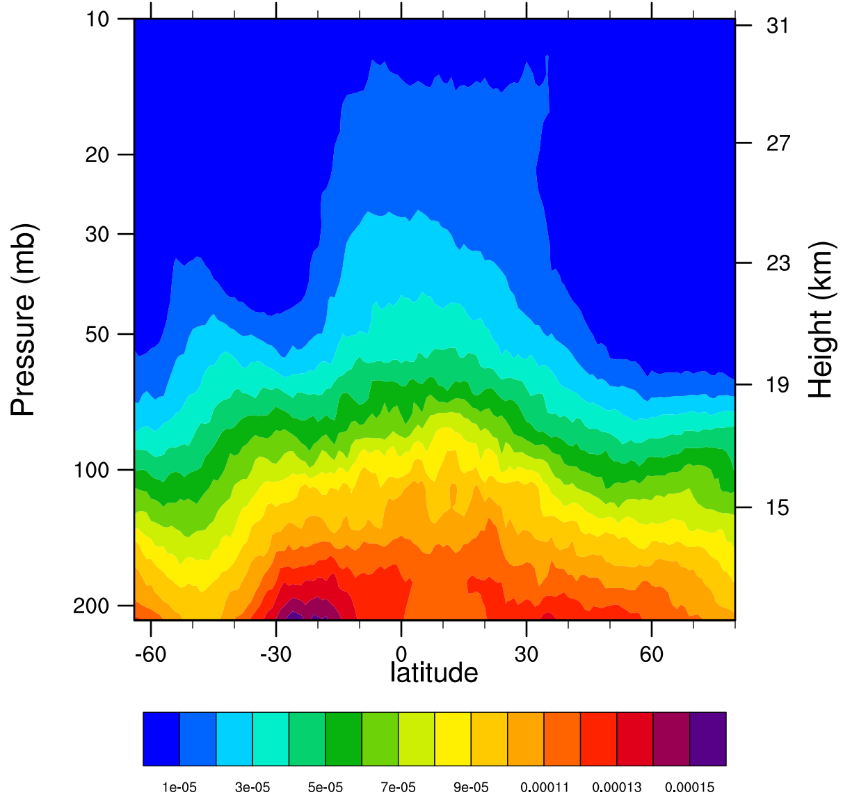
2007d277 12.1MicronExtinction_Combined (km -1 )
