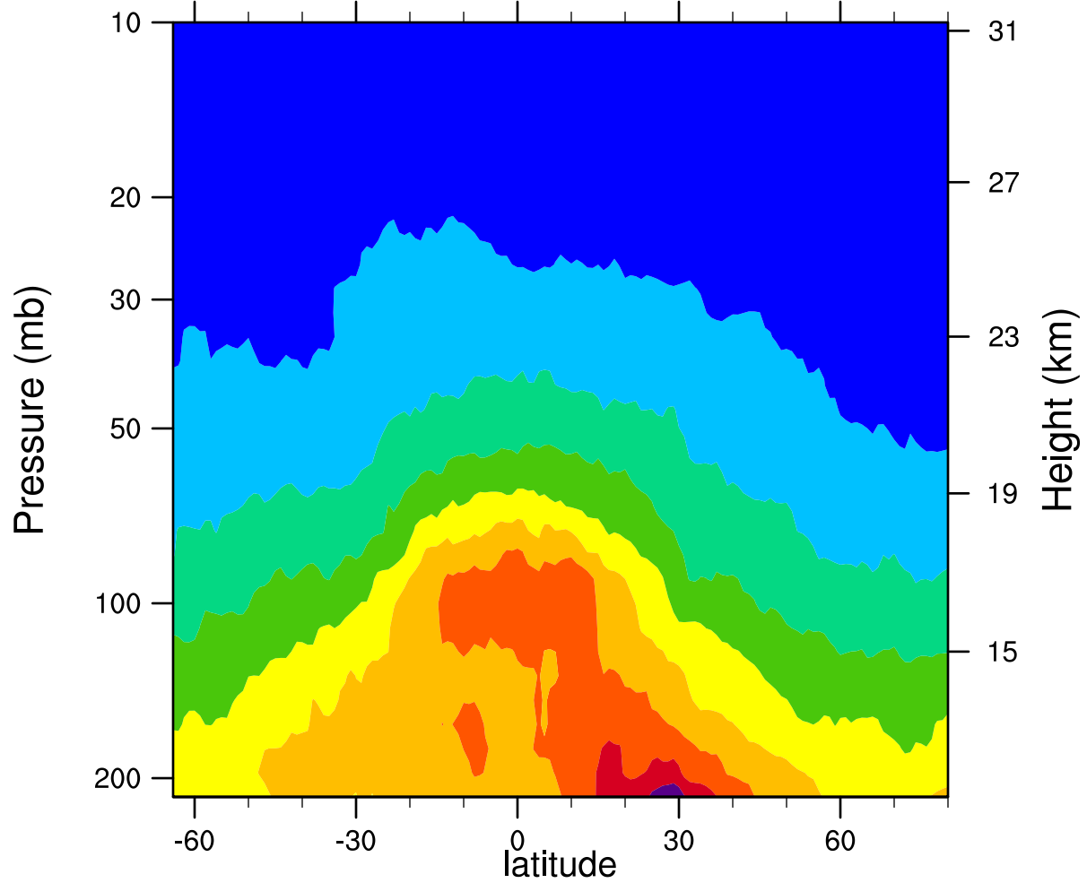
2006d098 12.1MicronExtinction_Combined (km -1 )
