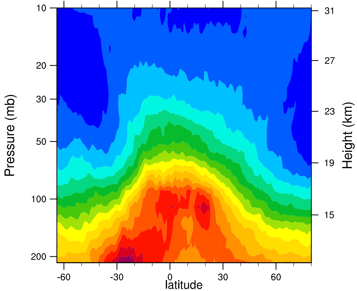
2005d290 12.1MicronExtinction_Combined (km -1 )
