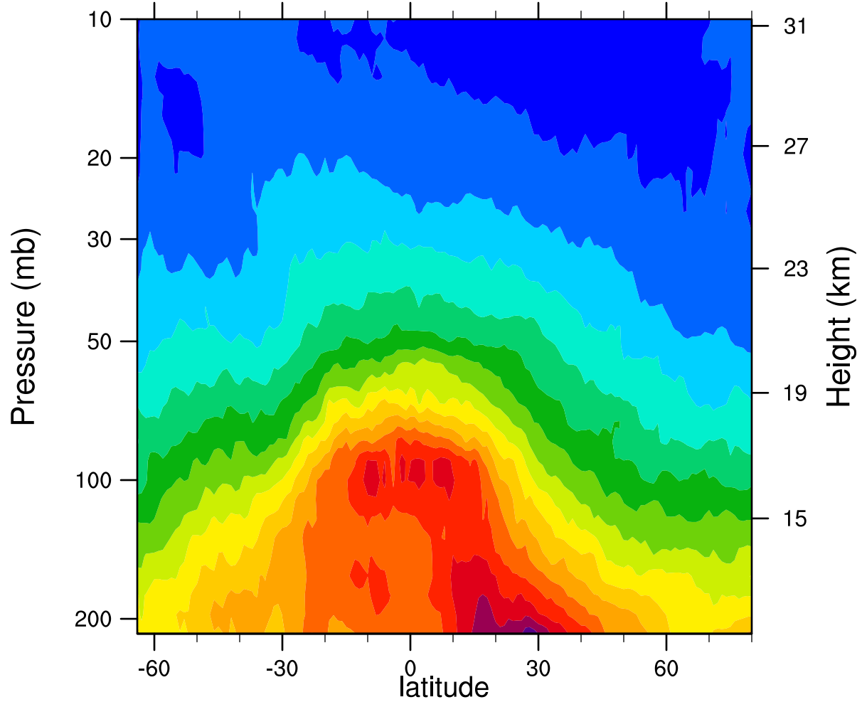
2006d093 12.1MicronExtinction_Combined (km -1 )
