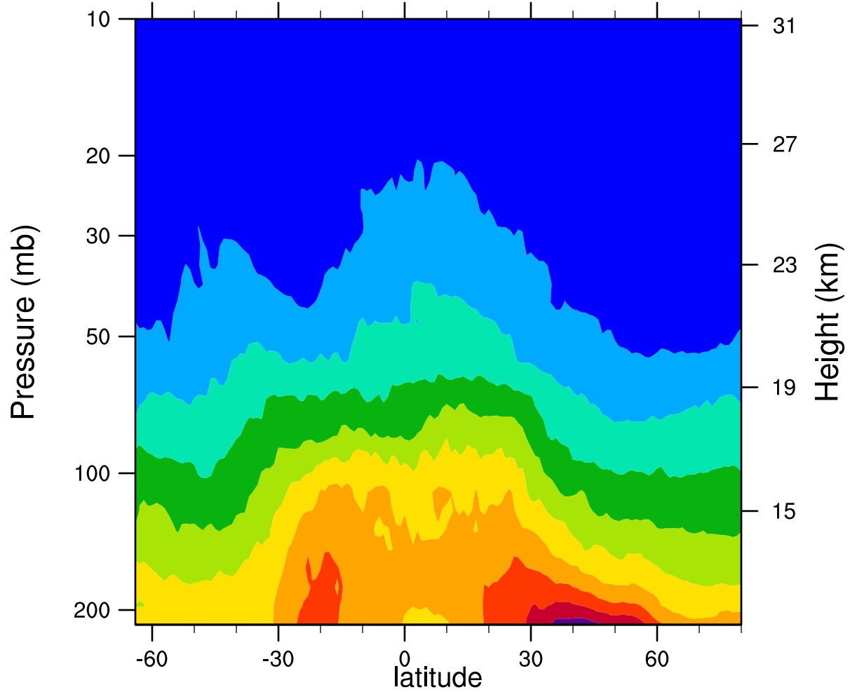
2007d161 12.1MicronExtinction_Combined (km -1 )
