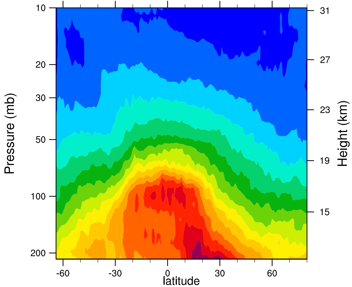
2006d090 12.1MicronExtinction_Combined (km -1 )
