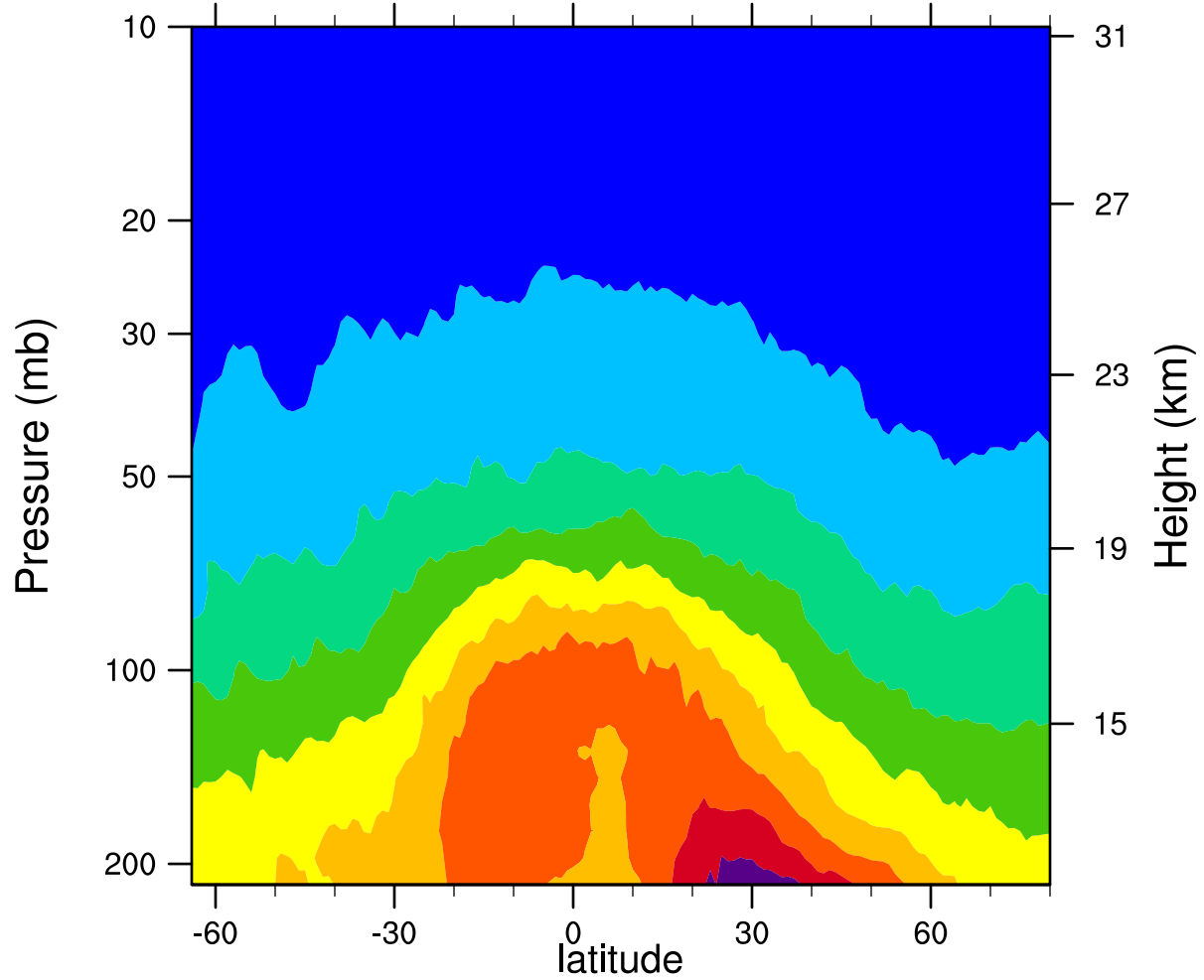
2006d140 12.1MicronExtinction_Combined (km -1 )
