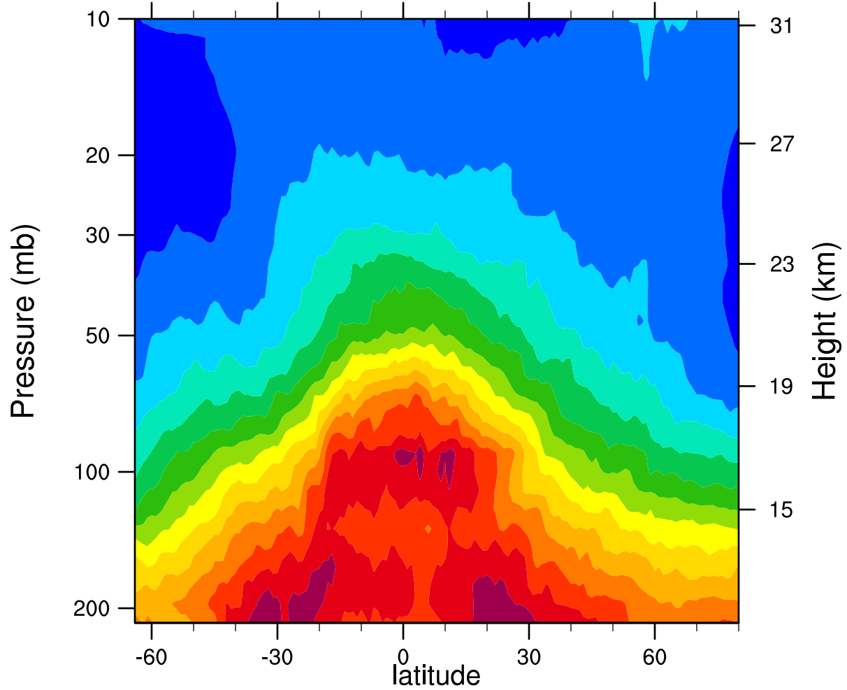
2005d333 12.1MicronExtinction_Combined ( \text{km}^{-1} )
