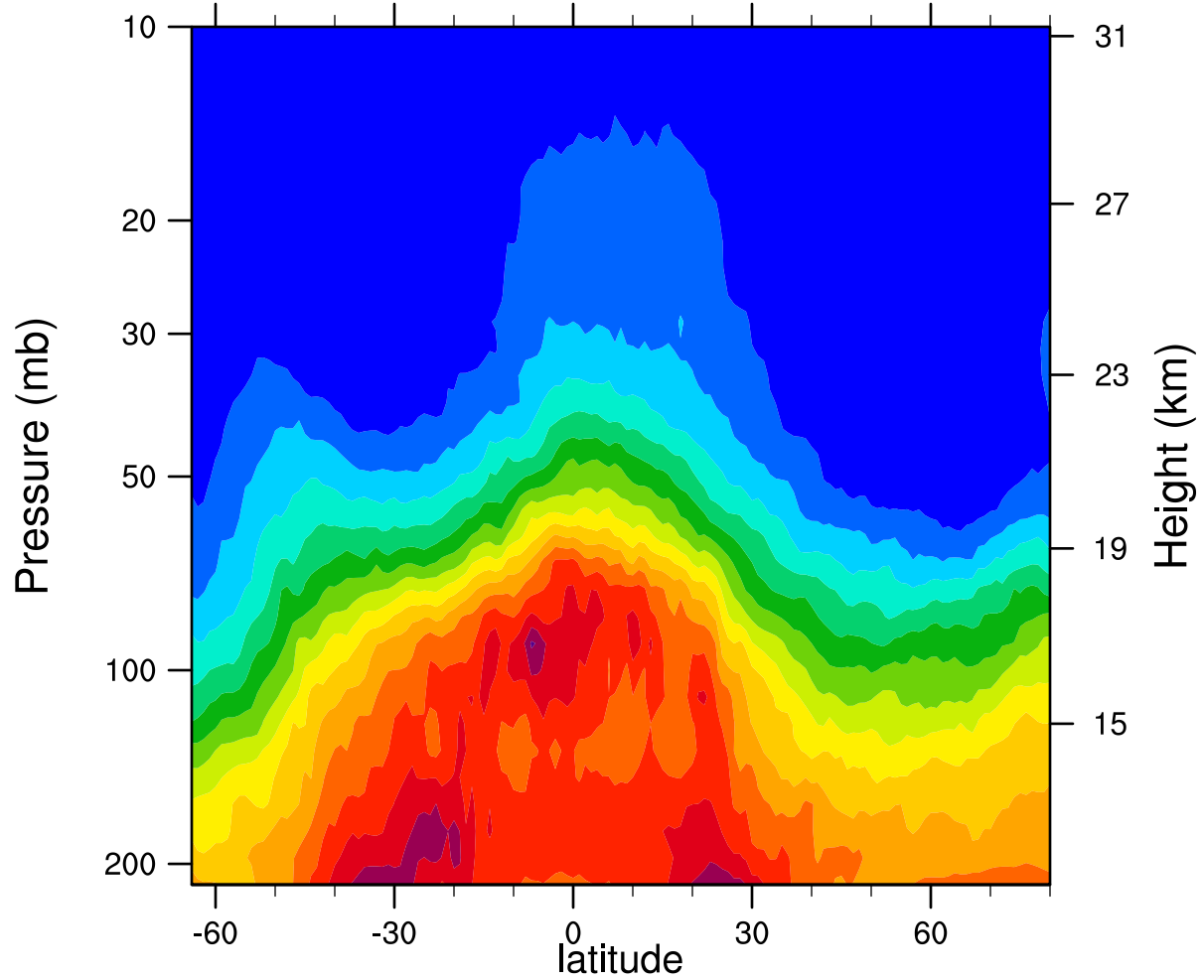
2006d343 12.1MicronExtinction_Combined (km -1 )
