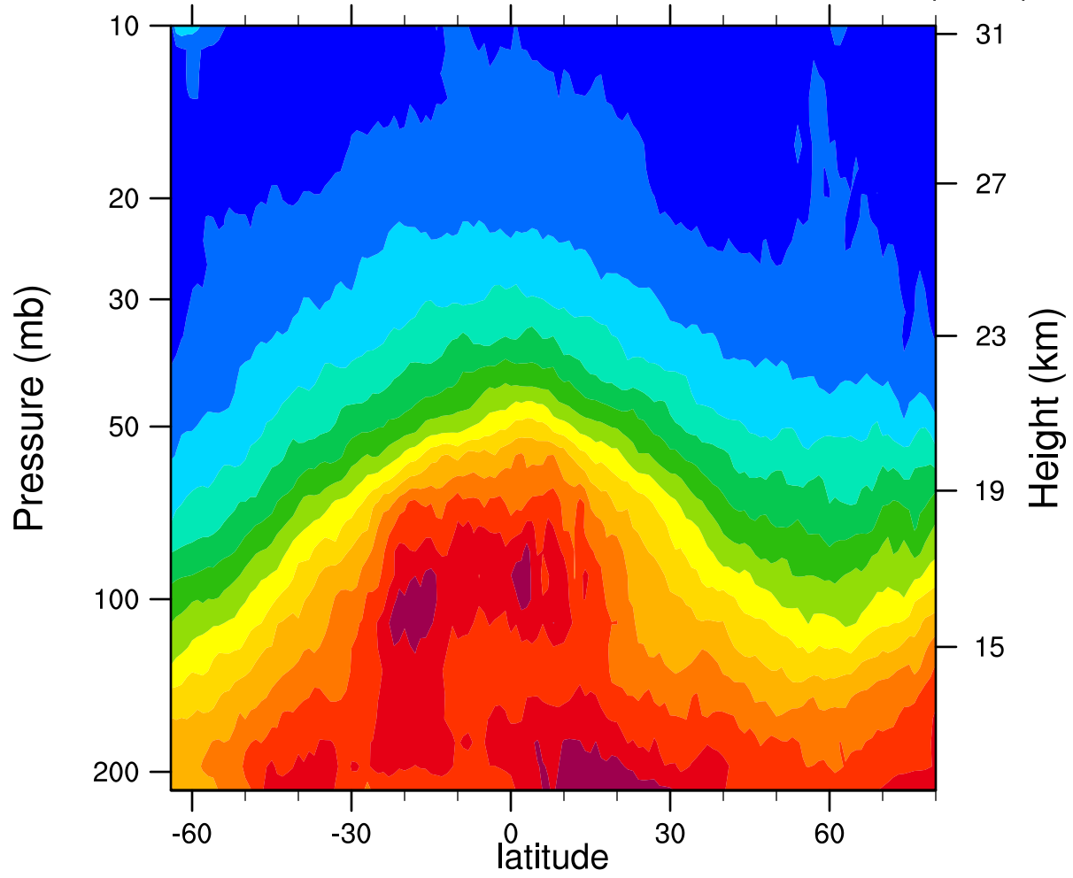
2007d037 12.1MicronExtinction_Combined ( \text{km}^{-1} )
