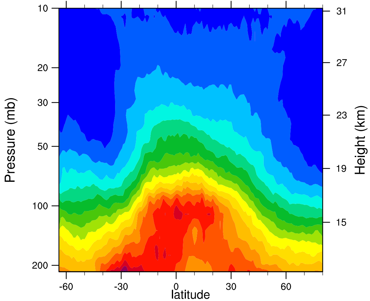
2005d274 12.1MicronExtinction_Combined (km -1 )
