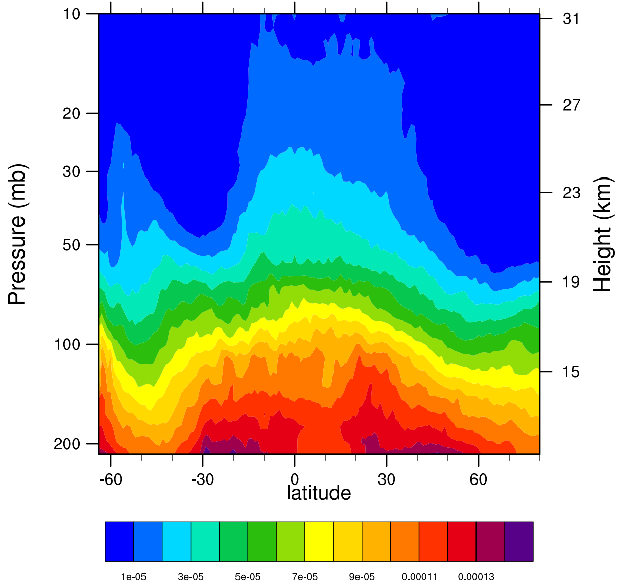
2007d258 12.1MicronExtinction_Combined ( \text{km}^{-1} )
