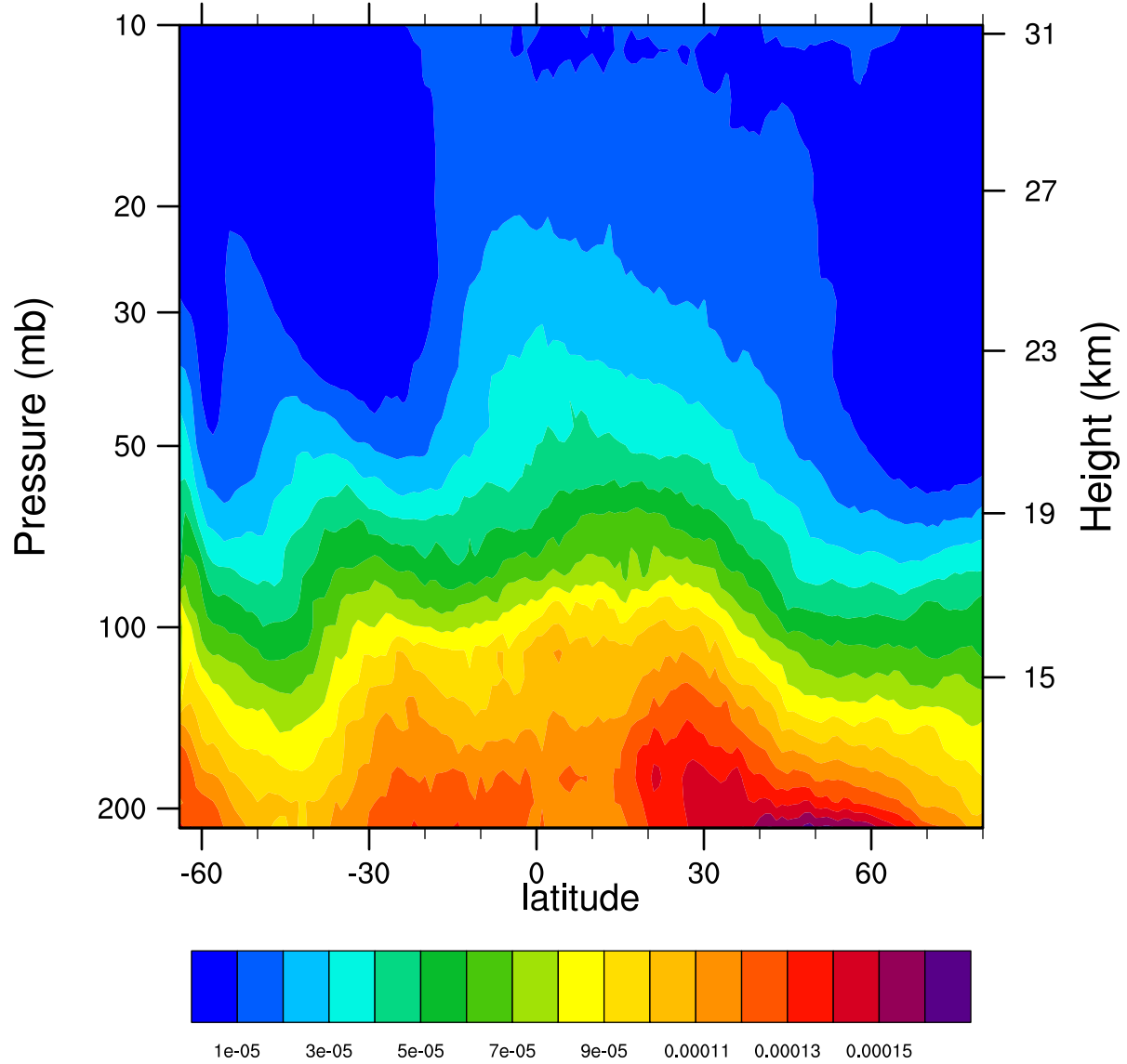
2007d222 12.1MicronExtinction_Combined (km -1 )
