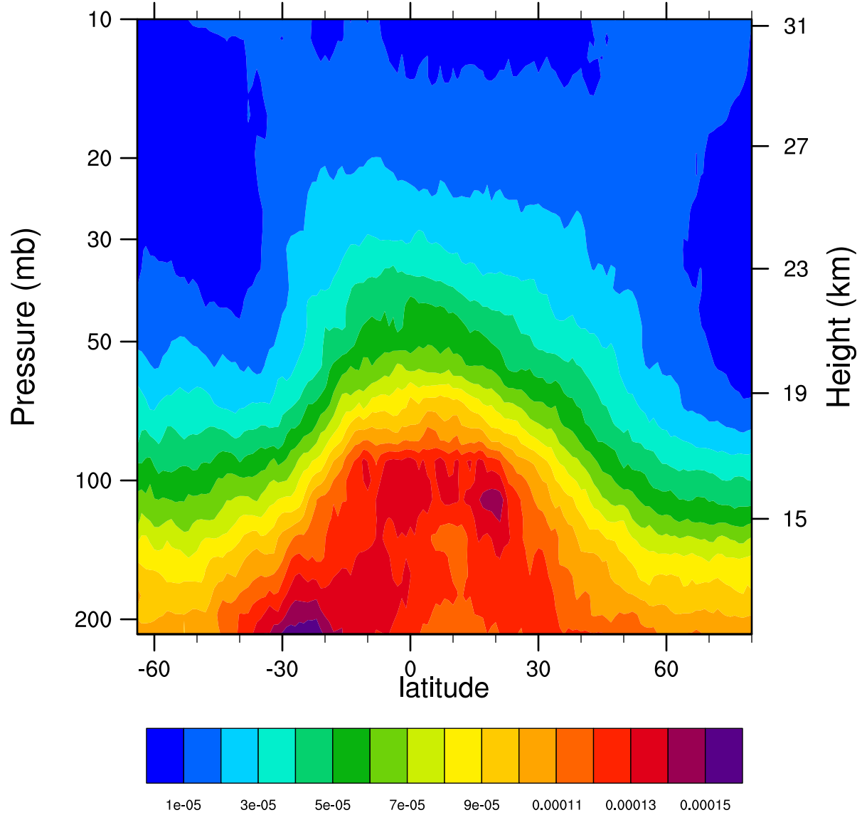
2005d292 12.1MicronExtinction_Combined (km -1 )
