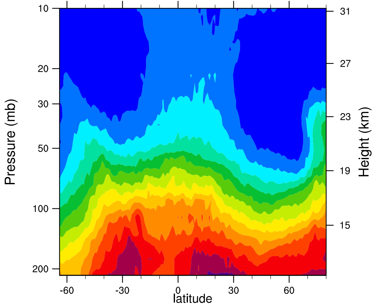
2007d362 12.1MicronExtinction_Combined (km -1 )
