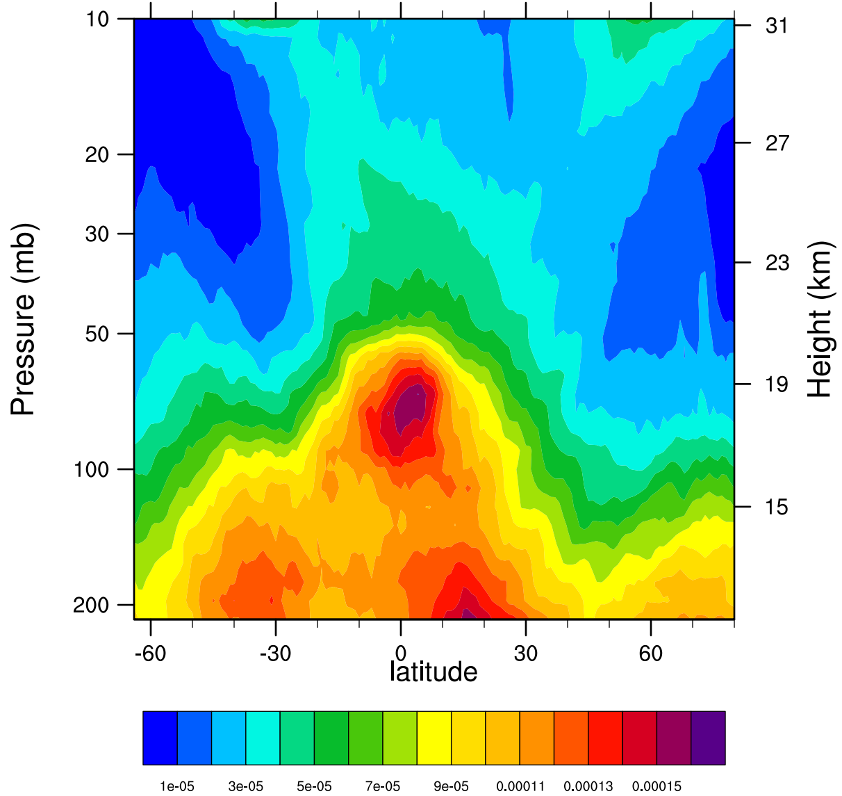
2005d053 12.1MicronExtinction_Combined ( \text{km}^{-1} )
