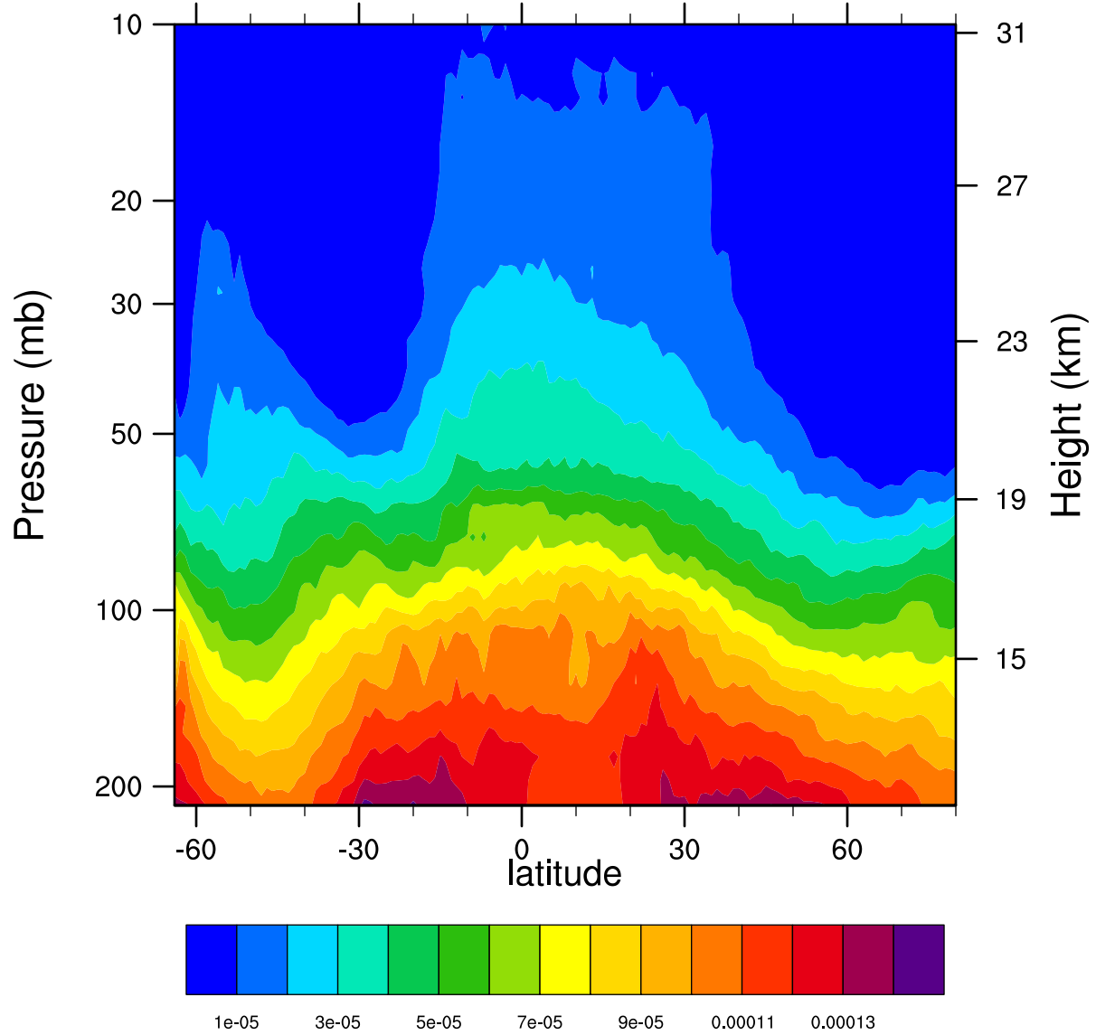
2007d260 12.1MicronExtinction_Combined (km -1 )
