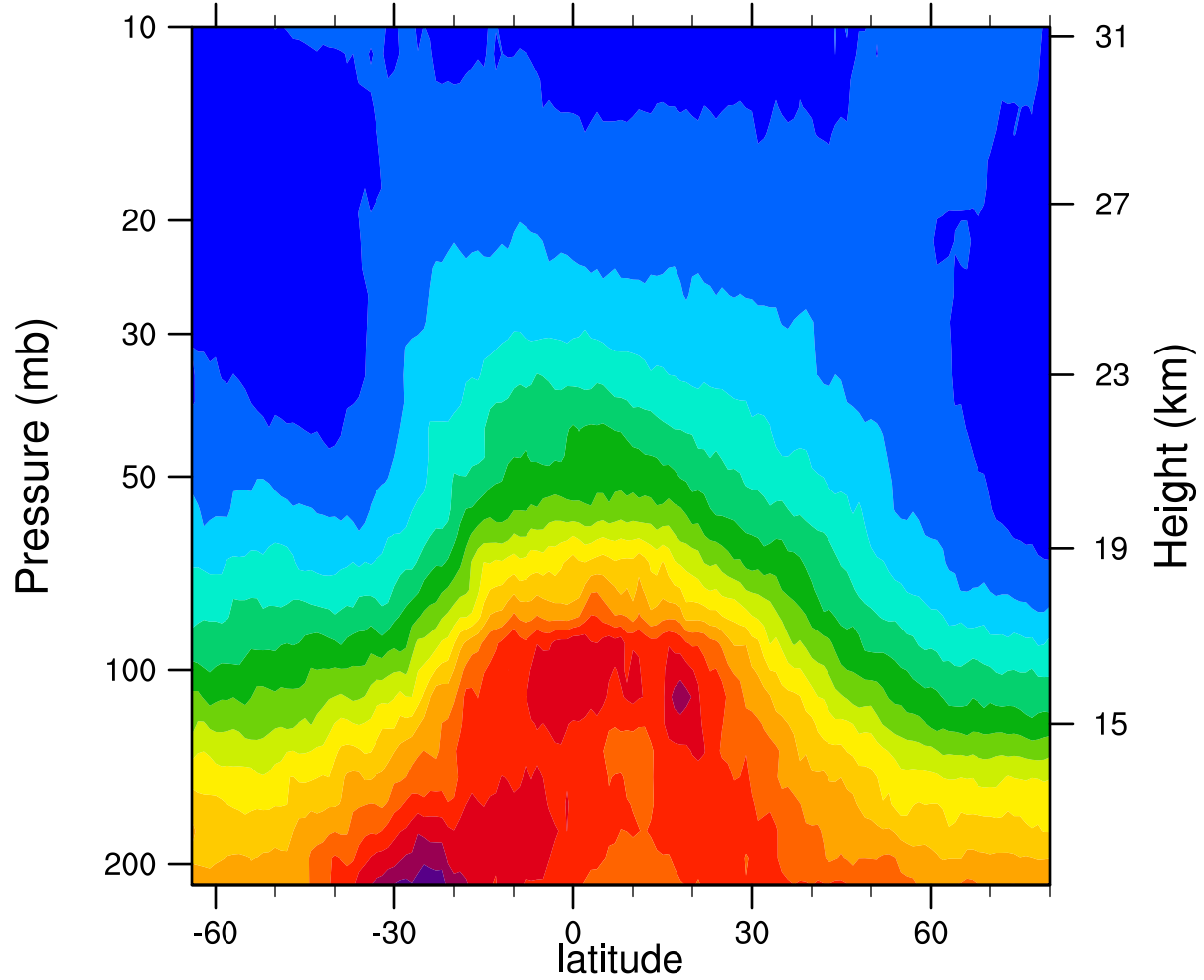
2005d294 12.1MicronExtinction_Combined (km -1 )
