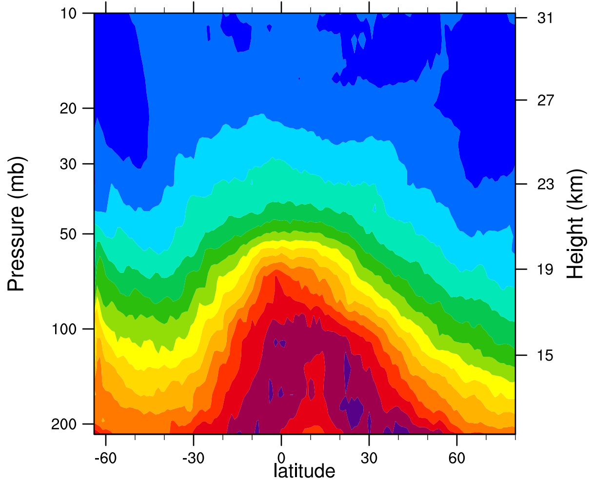
2006d248 12.1MicronExtinction_Combined ( \text{km}^{-1} )
