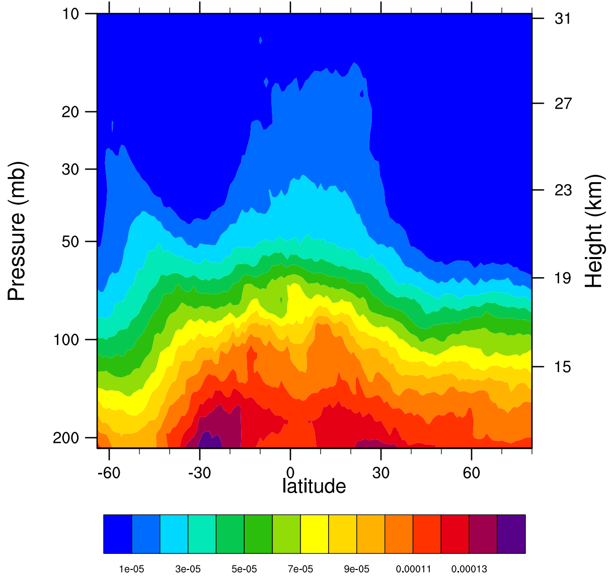
2007d319 12.1MicronExtinction_Combined (km -1 )
