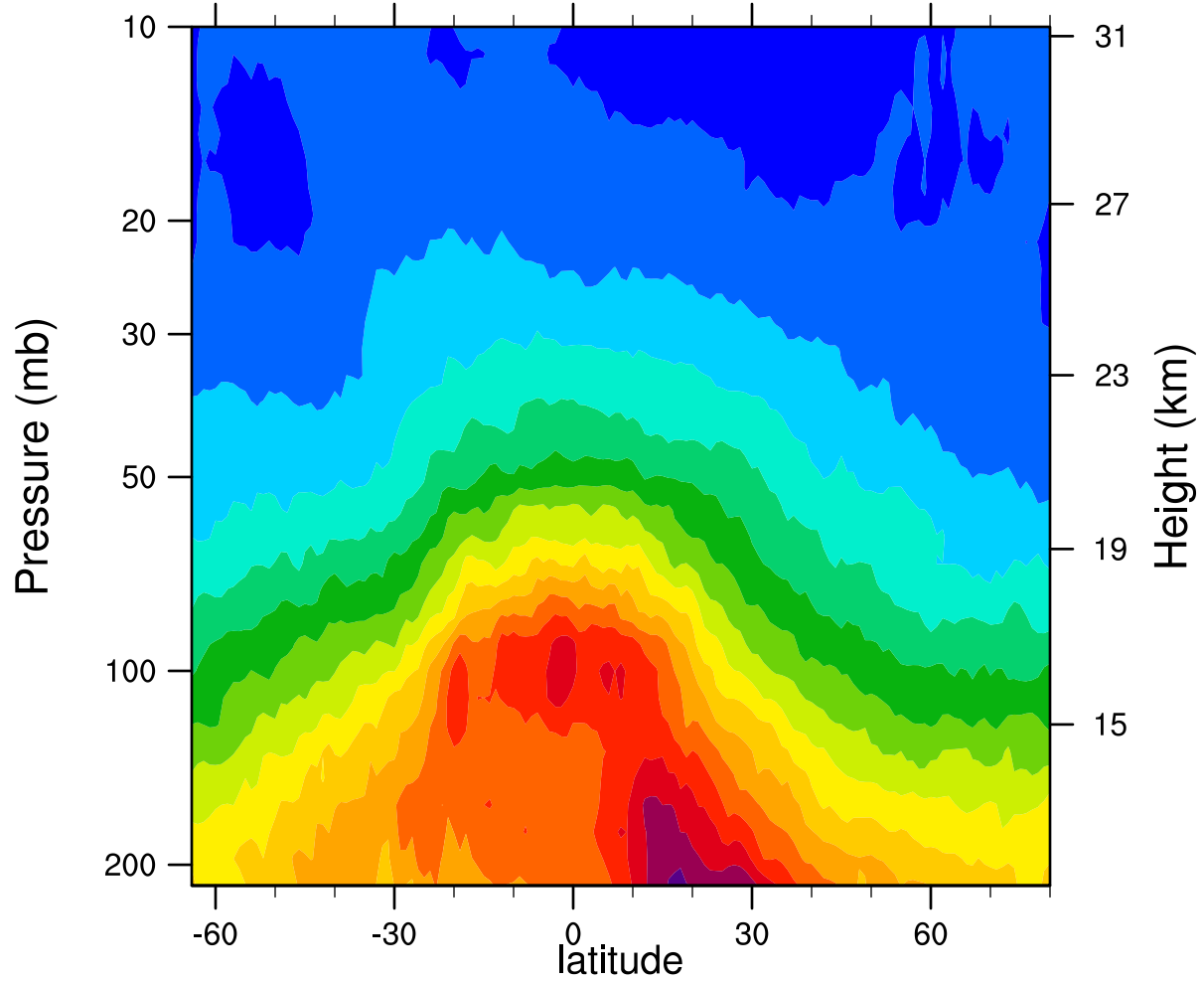
2006d083 12.1MicronExtinction_Combined (km -1 )
