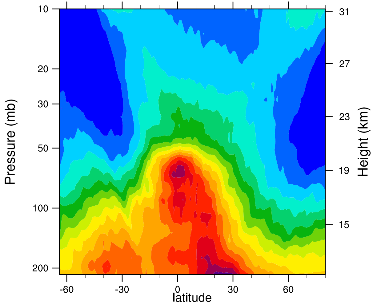
2005d088 12.1MicronExtinction_Combined (km -1 )
