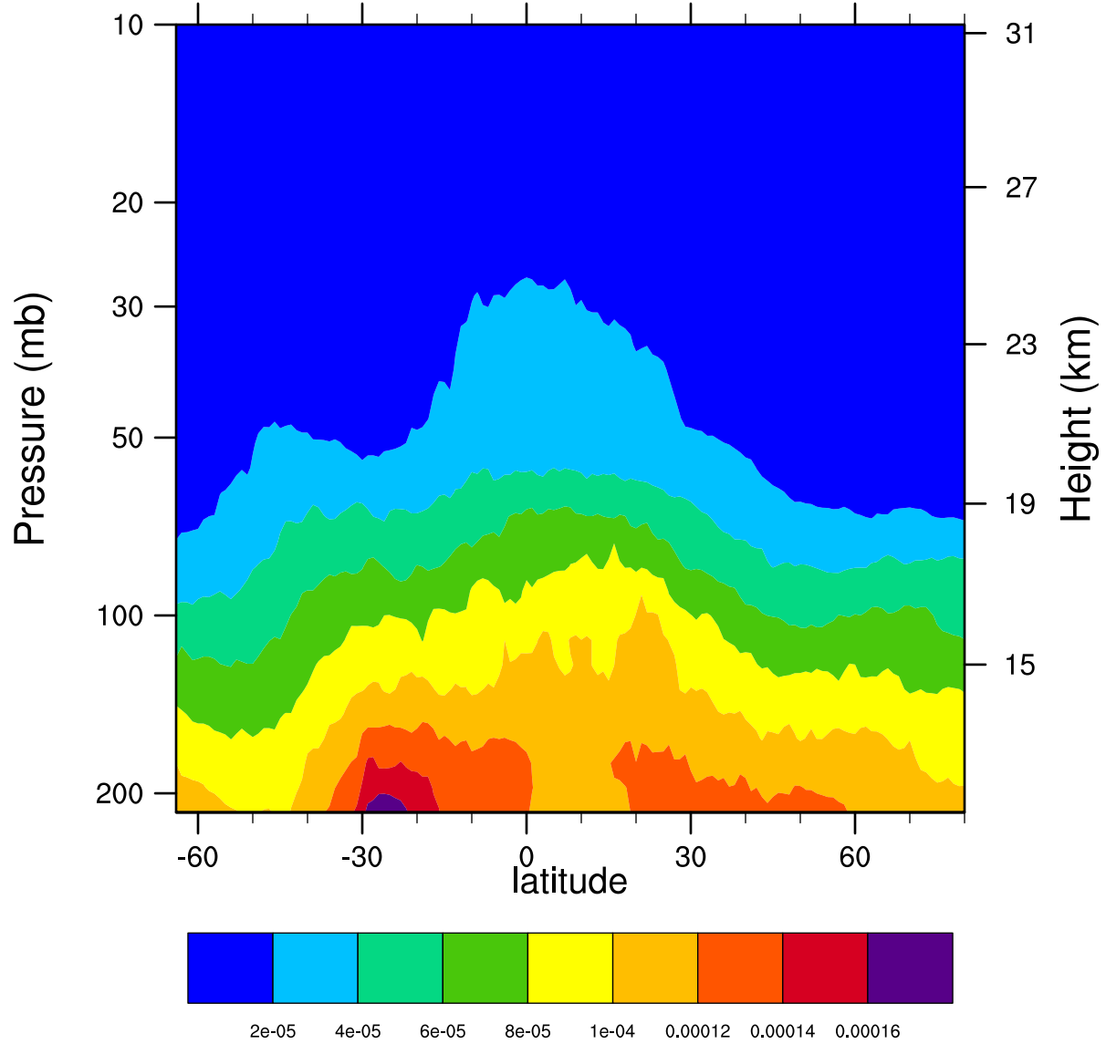
2007d283 12.1MicronExtinction_Combined (km -1 )
