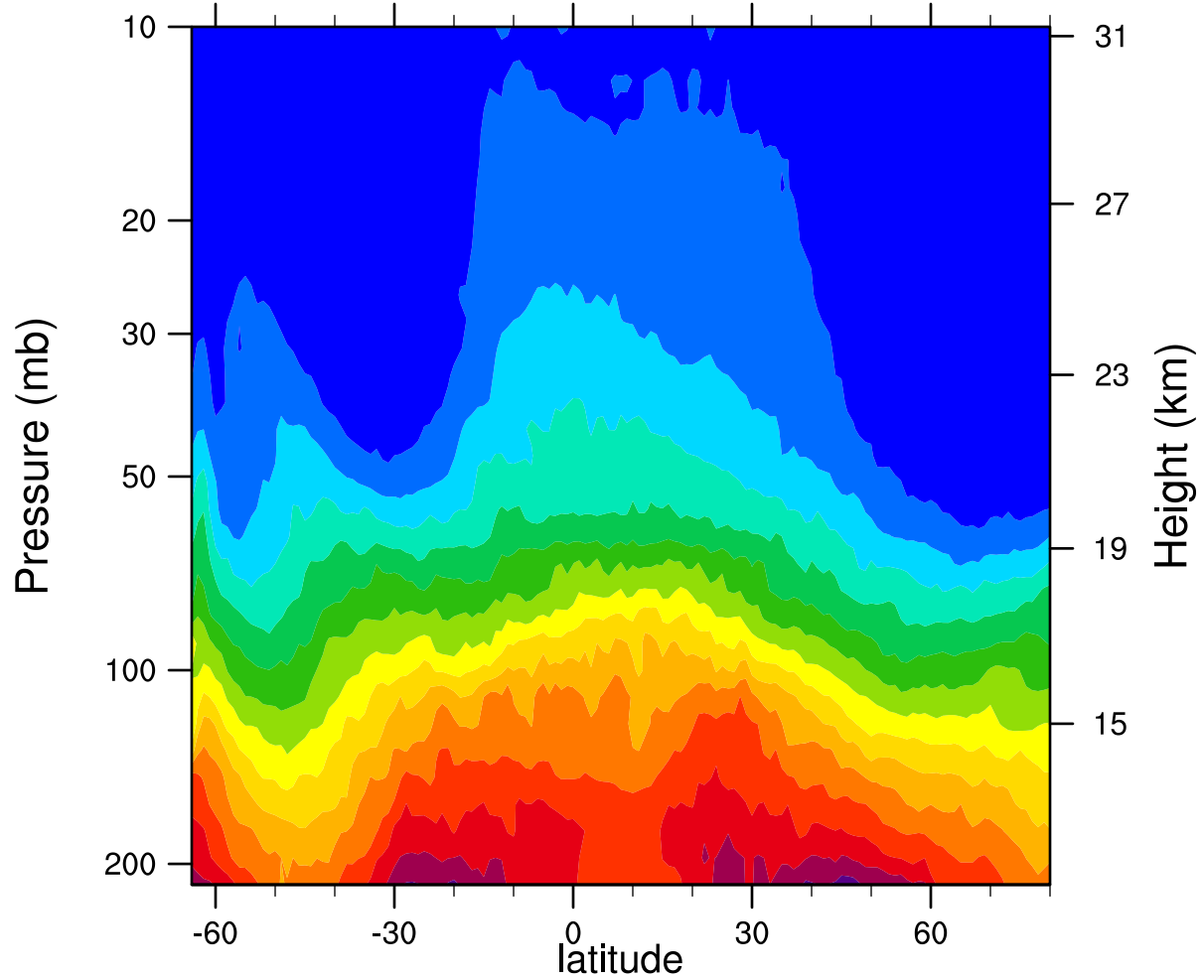
2007d255 12.1MicronExtinction_Combined (km -1 )
