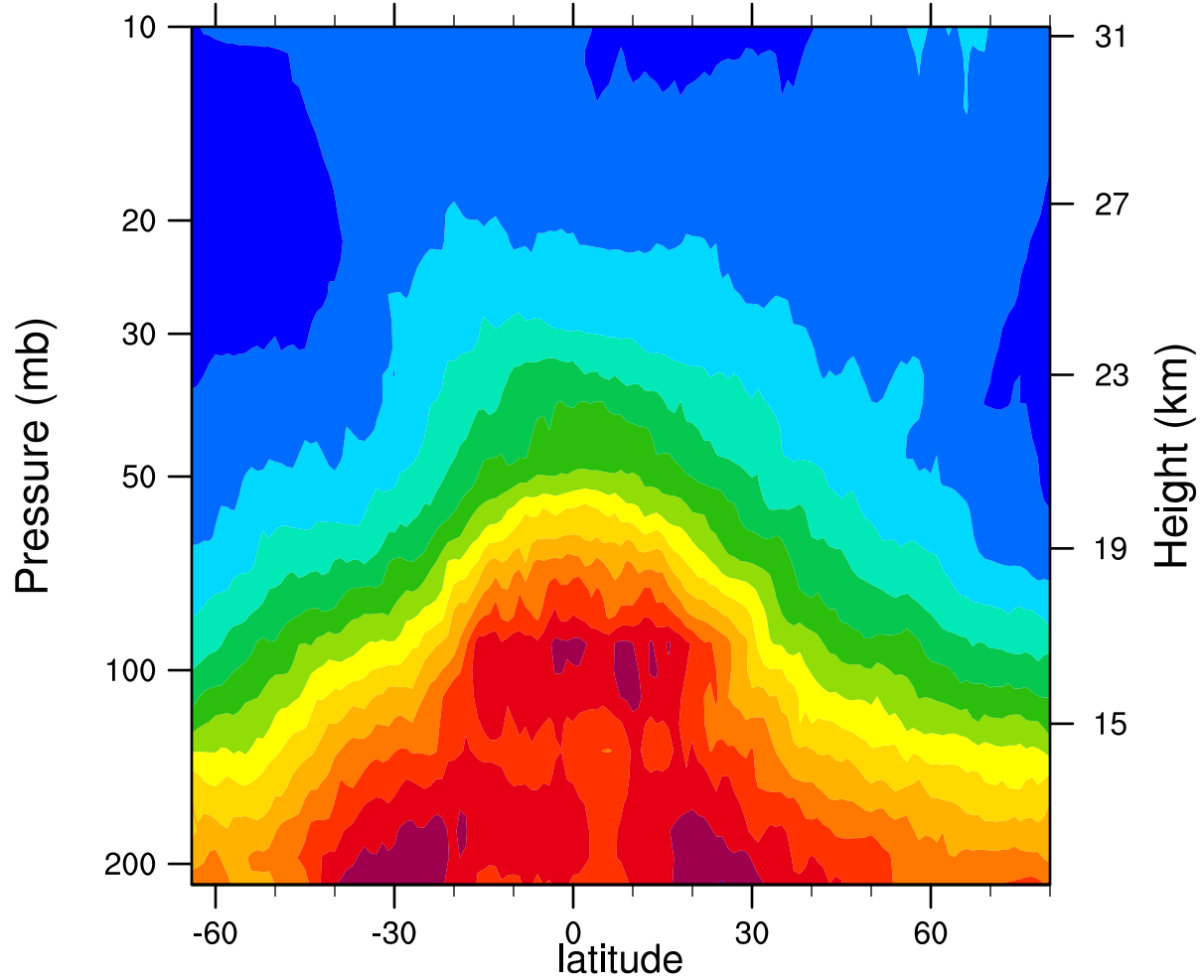
2005d328 12.1MicronExtinction_Combined (km -1 )
