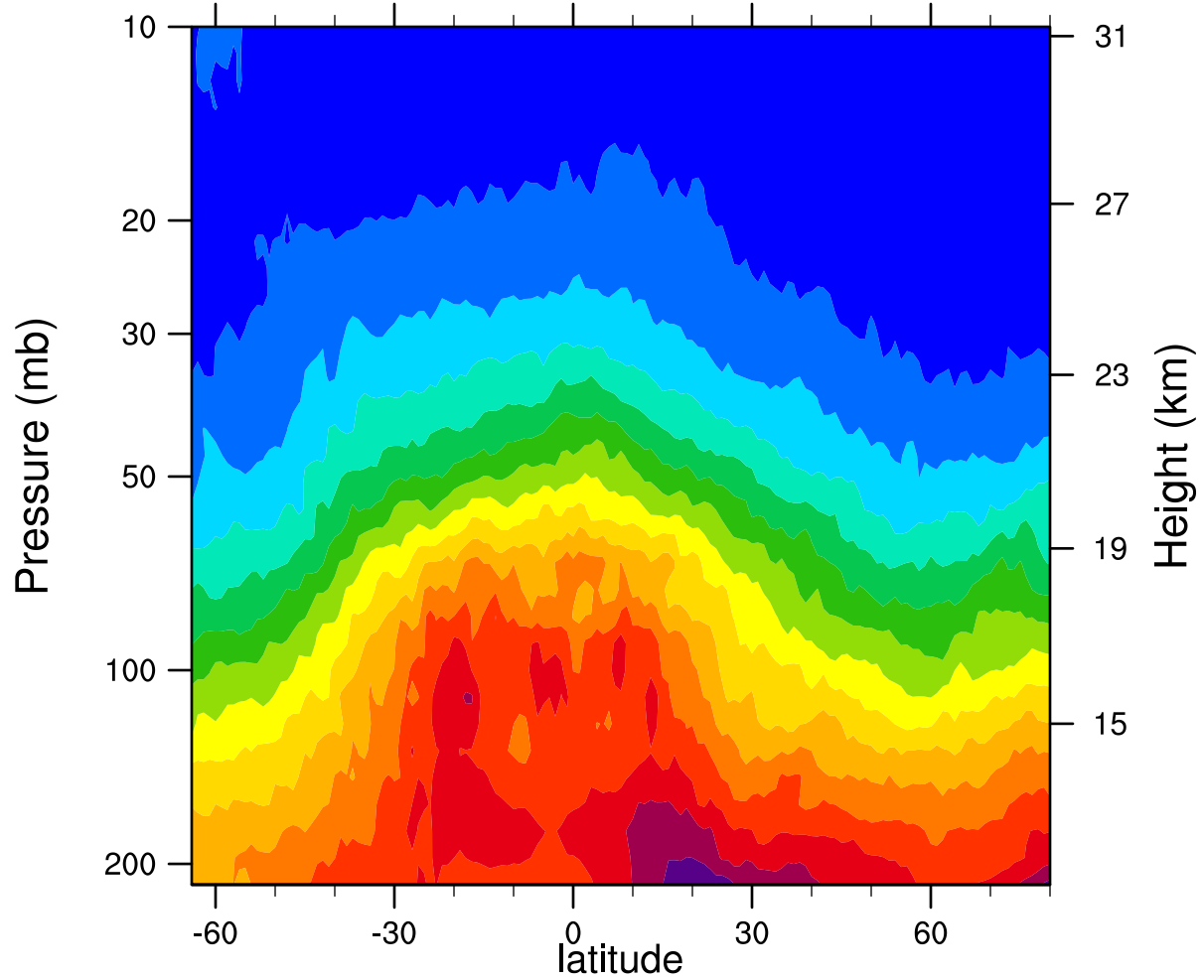
2007d074 12.1MicronExtinction_Combined (km -1 )
