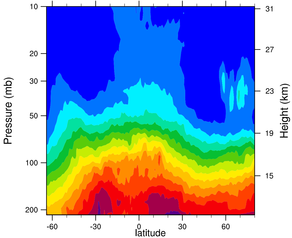
2007d354 12.1MicronExtinction_Combined (km -1 )
