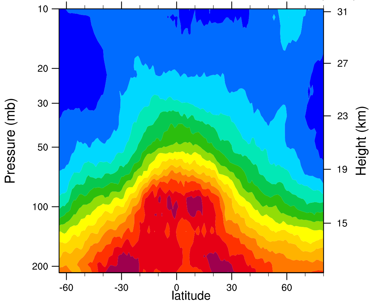
2005d321 12.1MicronExtinction_Combined ( \text{km}^{-1} )
