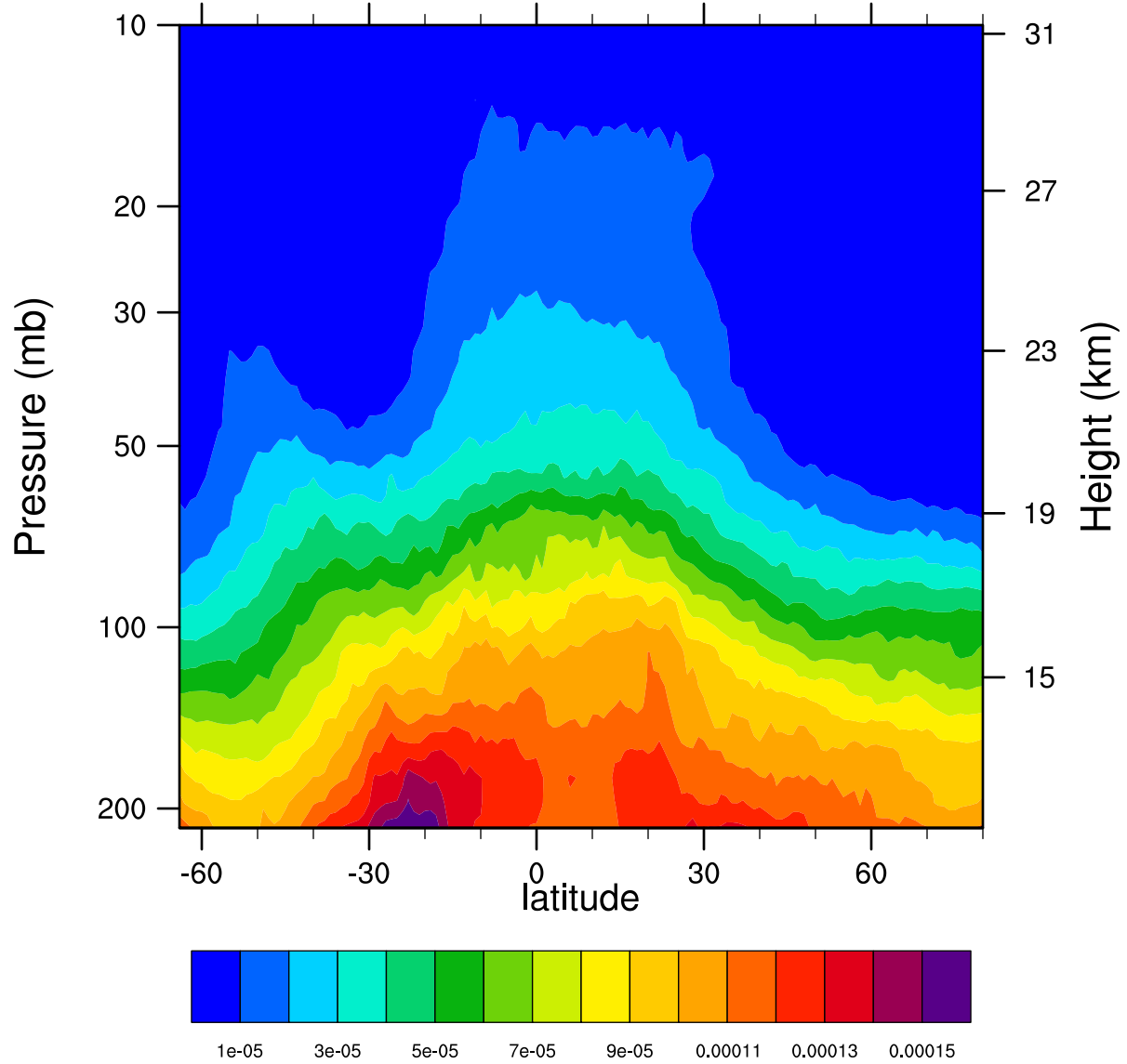
2007d302 12.1MicronExtinction_Combined (km -1 )
