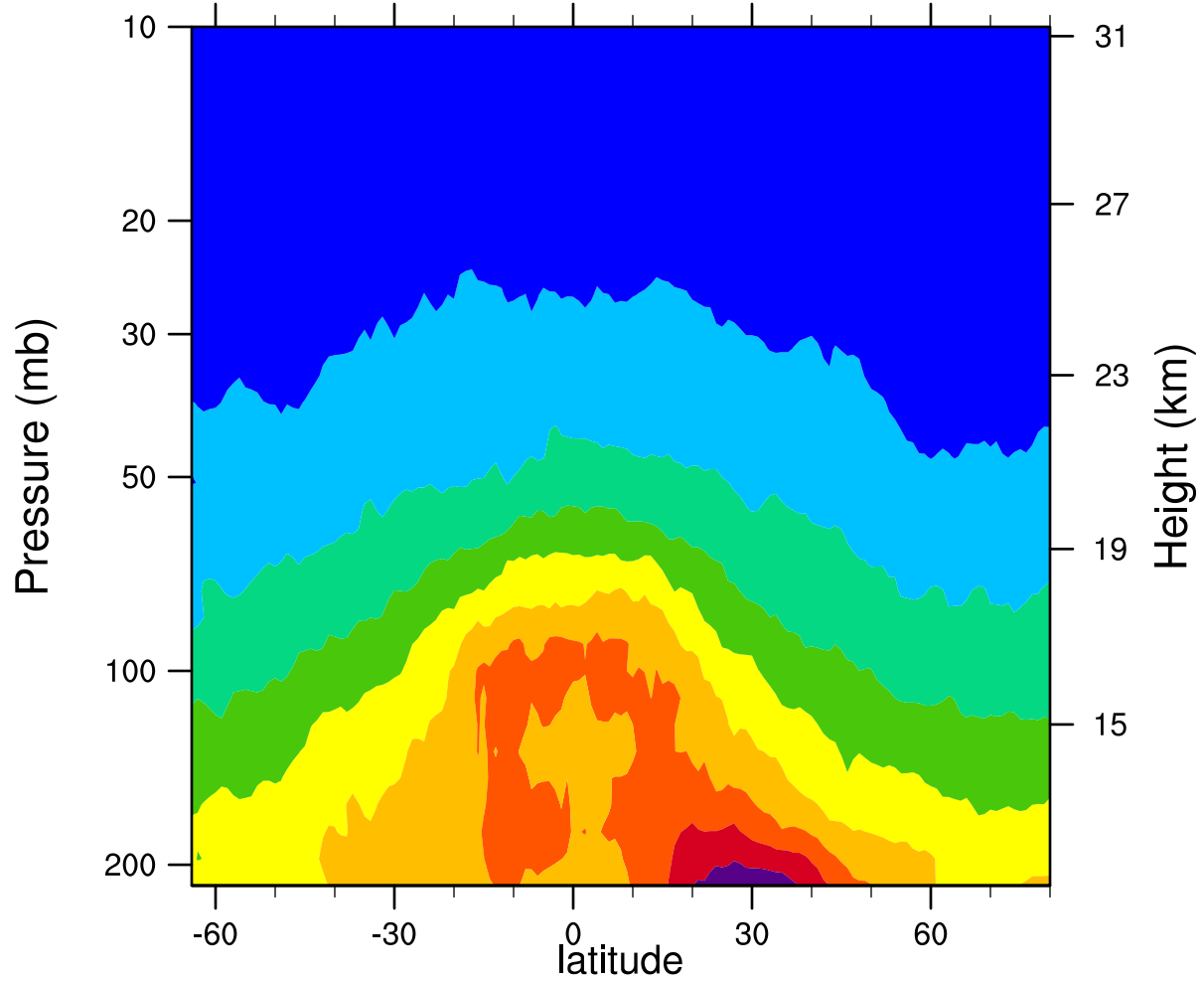
2006d117 12.1MicronExtinction_Combined (km -1 )
