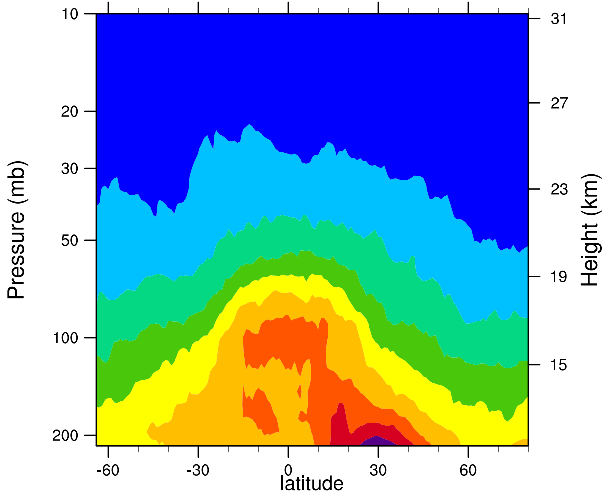
2006d105 12.1MicronExtinction_Combined (km -1 )
