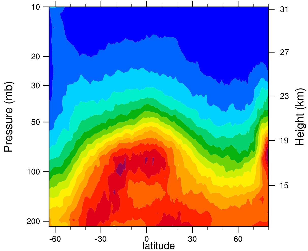
2007d020 12.1MicronExtinction_Combined (km -1 )
