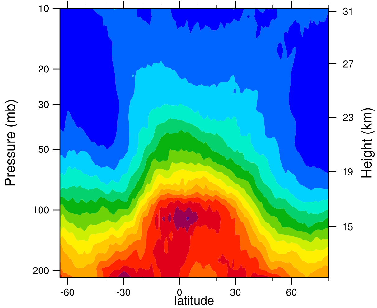
2005d264 12.1MicronExtinction_Combined (km -1 )
