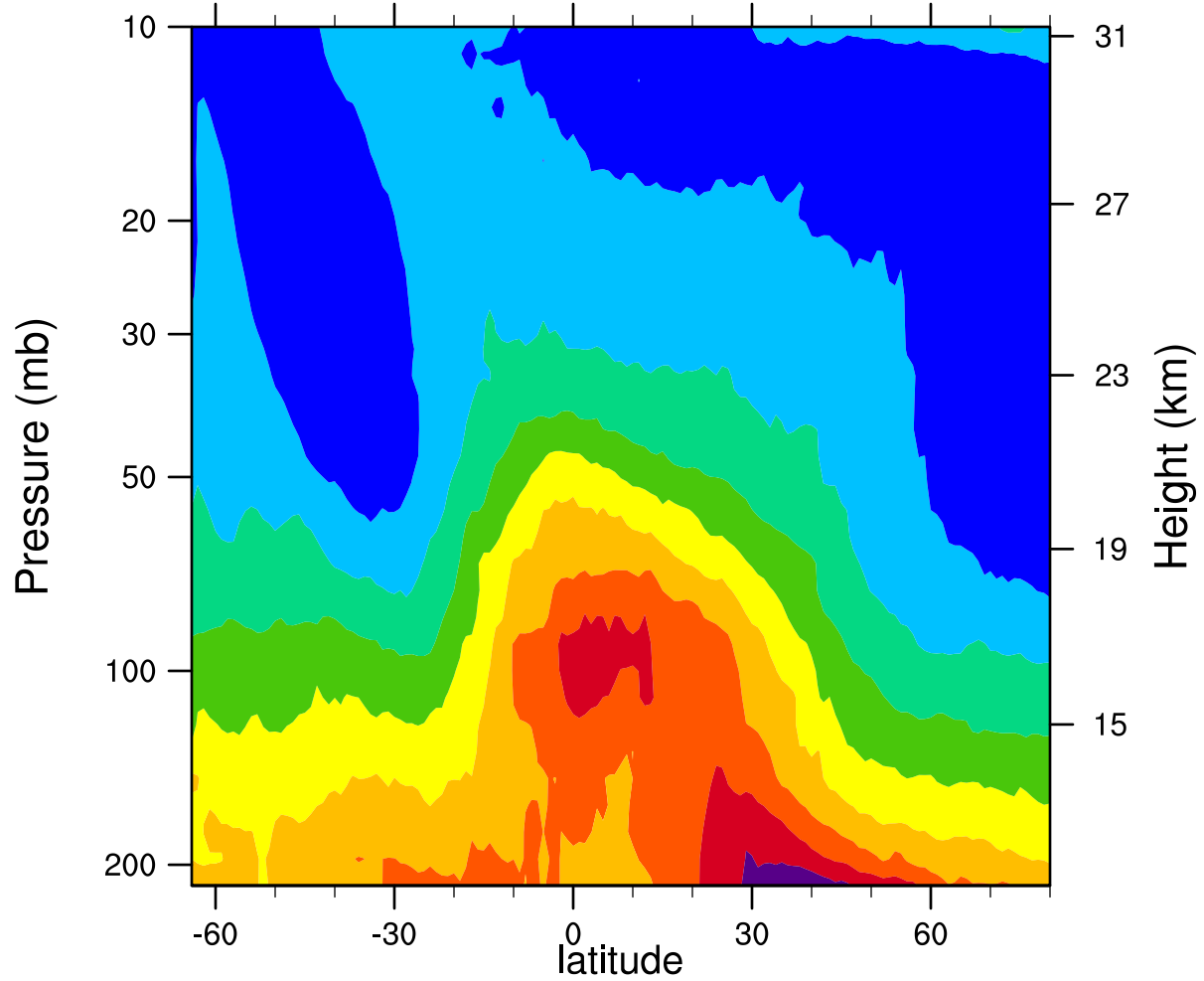
2005d165 12.1MicronExtinction_Combined (km -1 )
