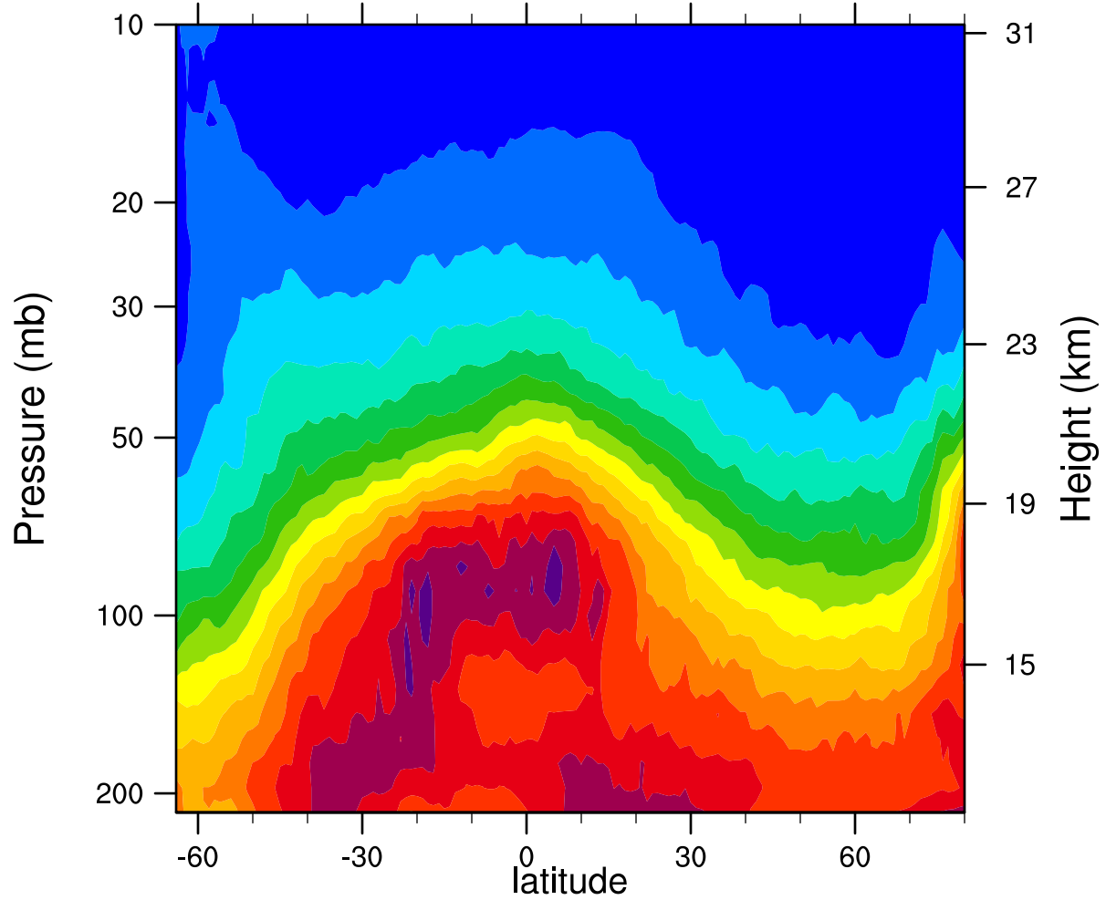
2007d017 12.1MicronExtinction_Combined (km -1 )
