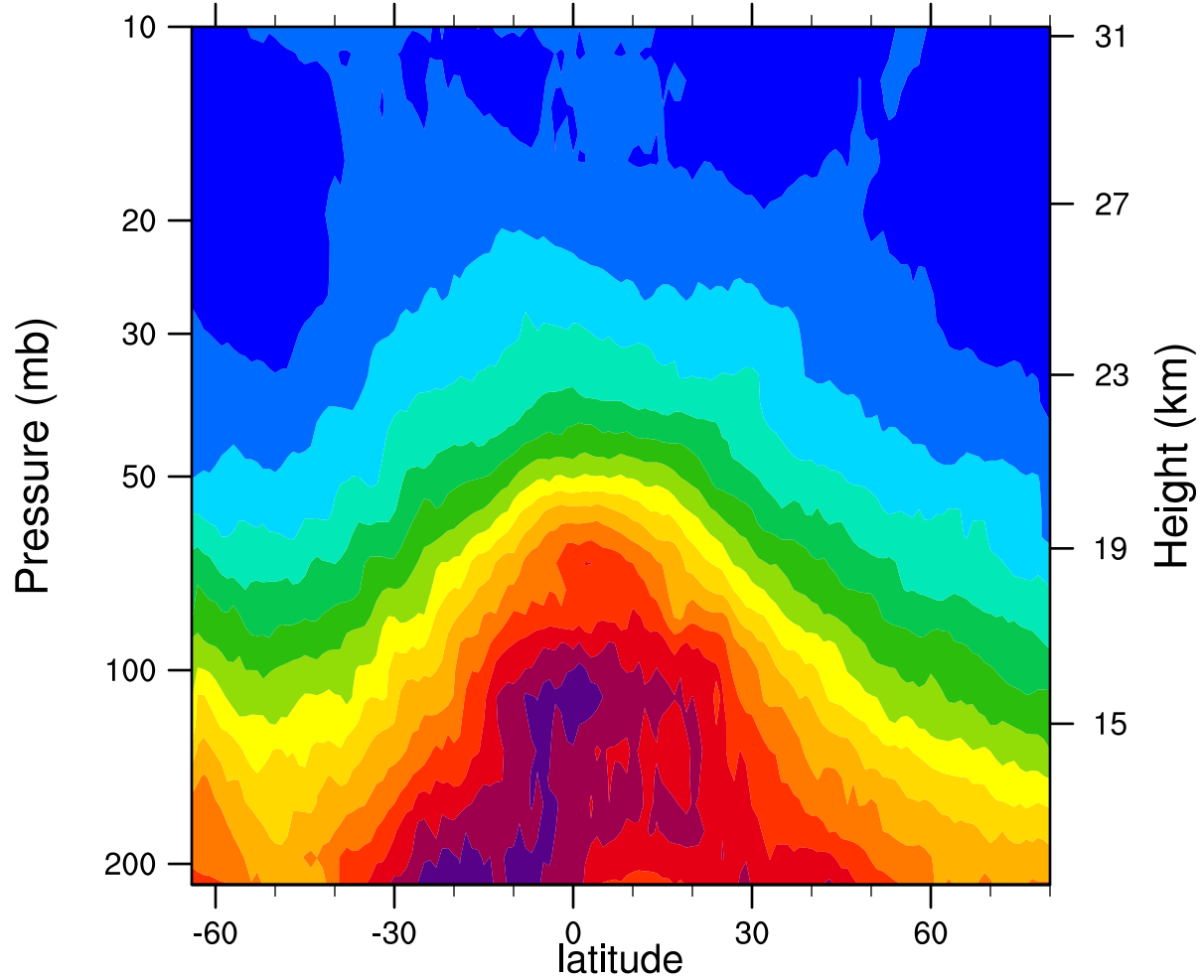
2006d283 12.1MicronExtinction_Combined (km -1 )
