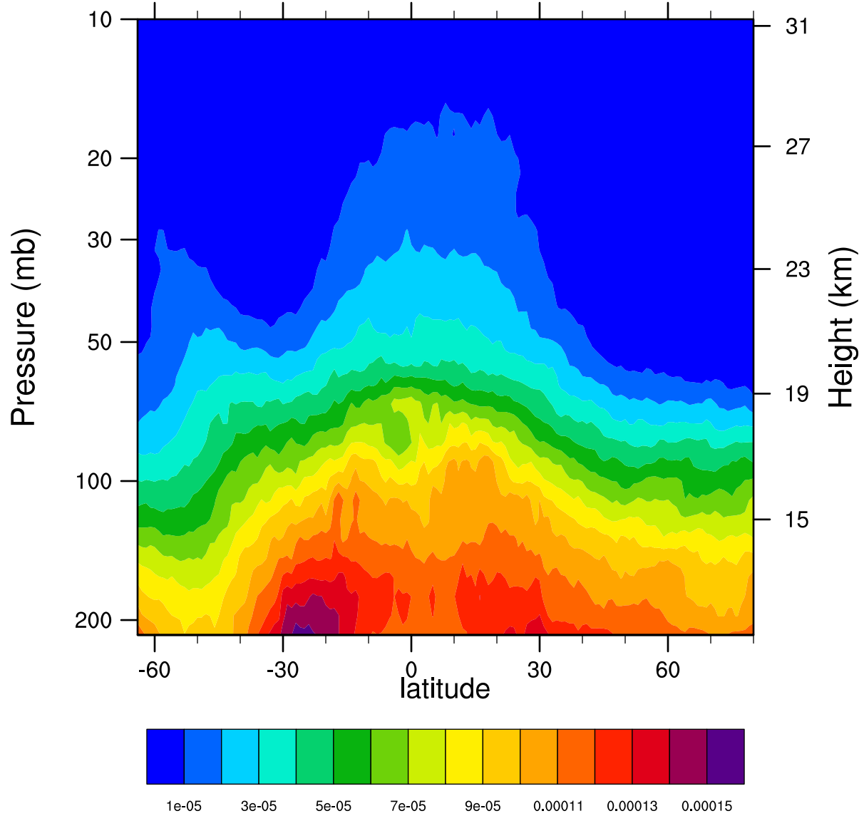
2007d312 12.1MicronExtinction_Combined ( \text{km}^{-1} )
