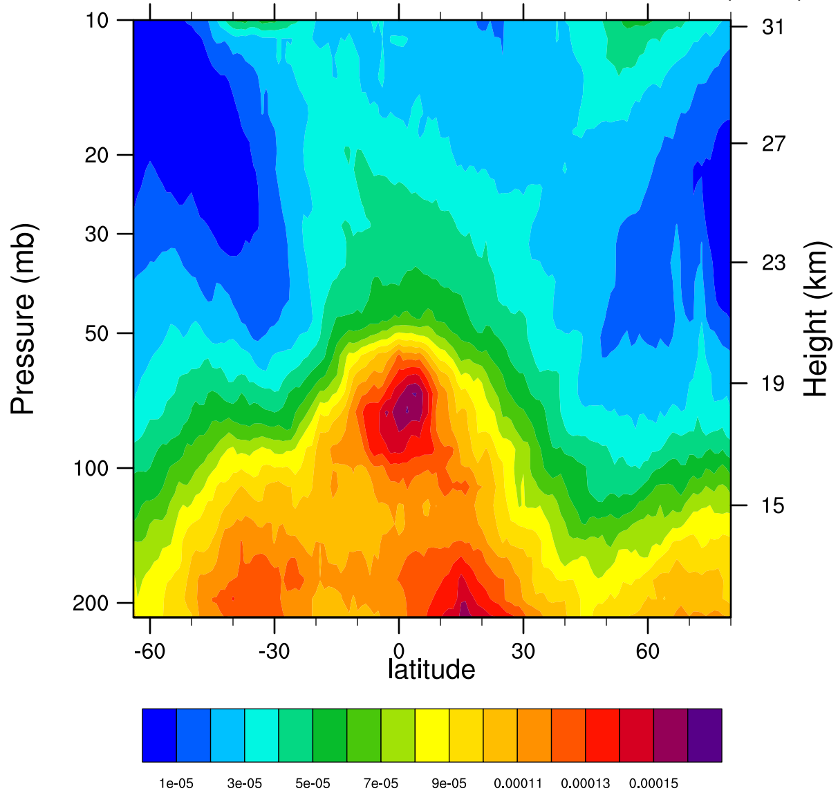
2005d052 12.1MicronExtinction_Combined ( \text{km}^{-1} )
