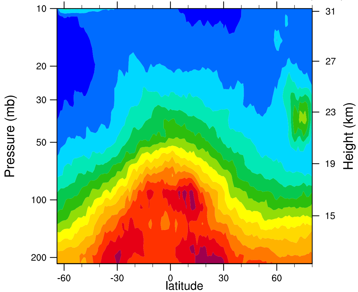
2005d364 12.1MicronExtinction_Combined ( \text{km}^{-1} )
