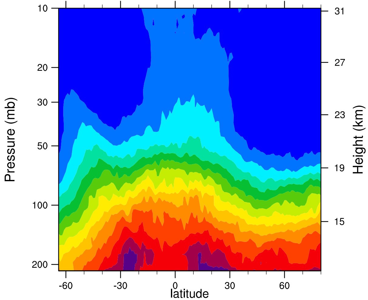
2007d348 12.1MicronExtinction_Combined ( \text{km}^{-1} )
