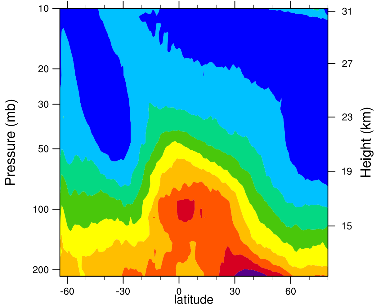
2005d170 12.1MicronExtinction_Combined (km -1 )
