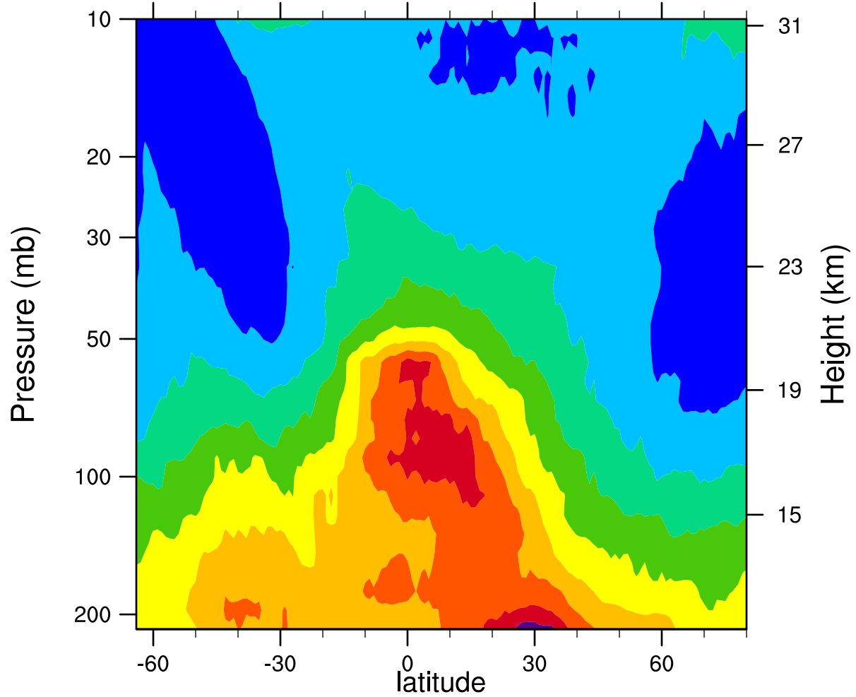
2005d107 12.1MicronExtinction_Combined (km -1 )
