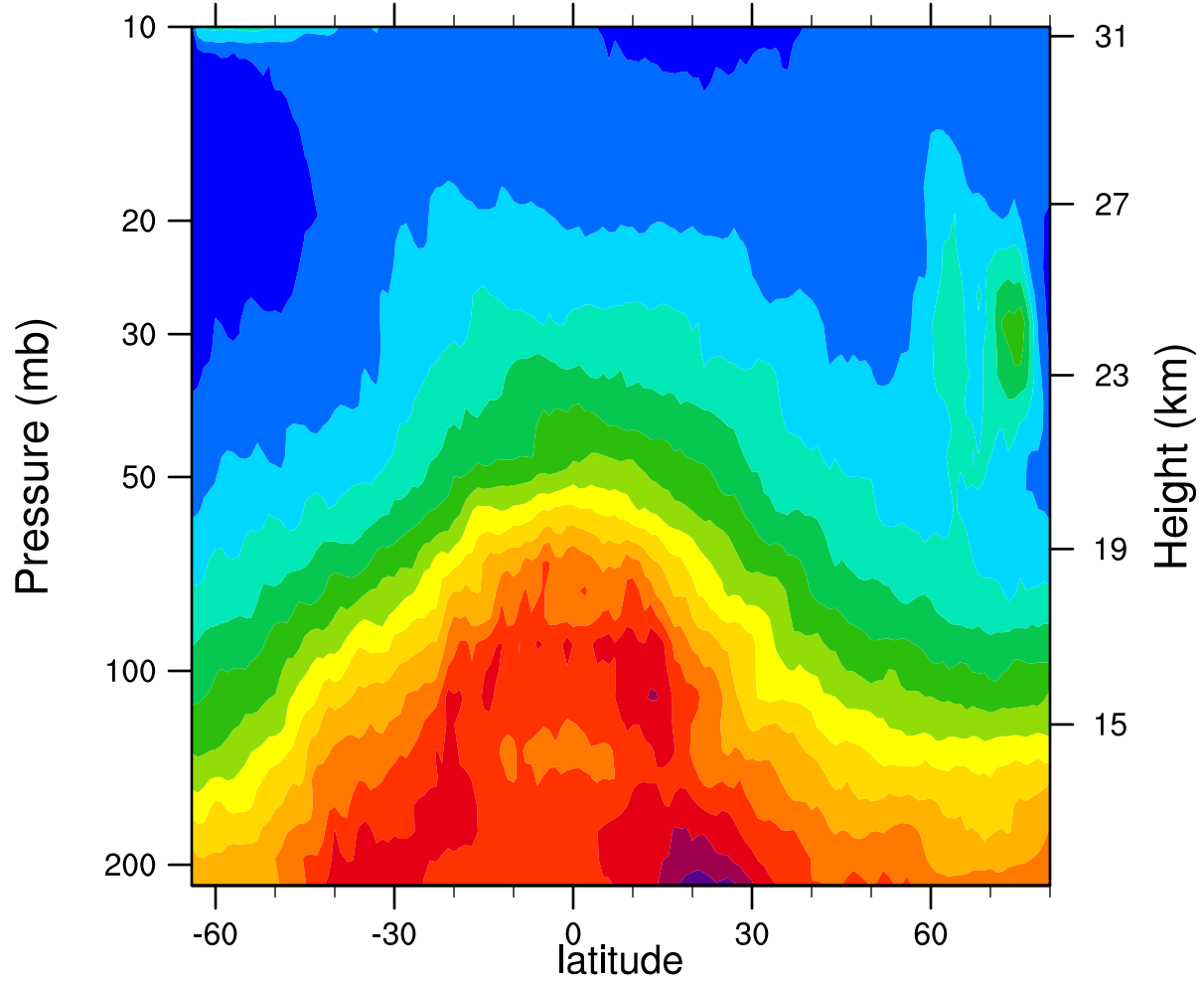
2006d006 12.1MicronExtinction_Combined ( \text{km}^{-1} )
