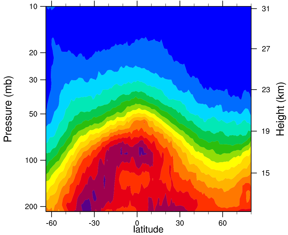
2007d007 12.1MicronExtinction_Combined (km -1 )
