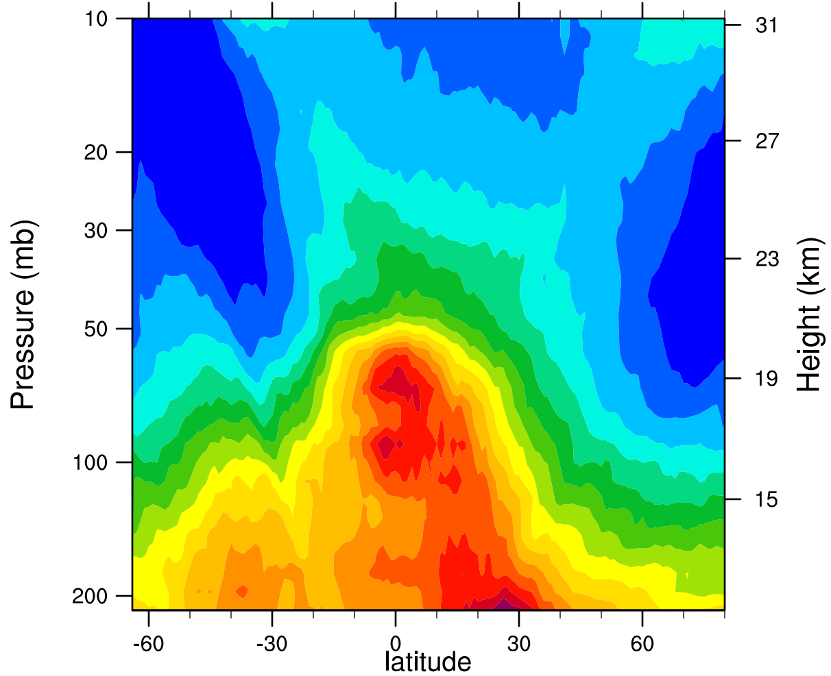
2005d094 12.1MicronExtinction_Combined (km -1 )
