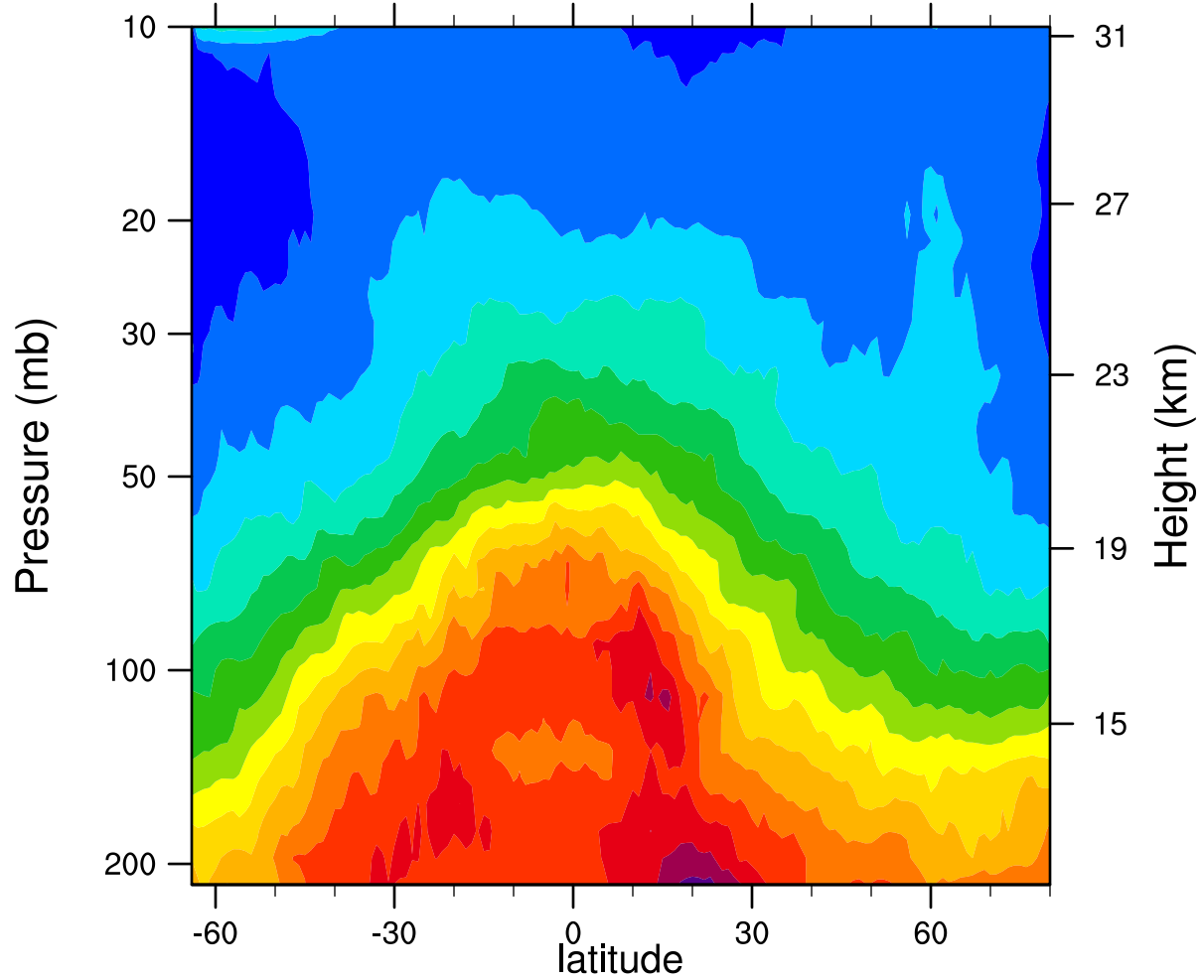
2006d011 12.1MicronExtinction_Combined ( \text{km}^{-1} )
