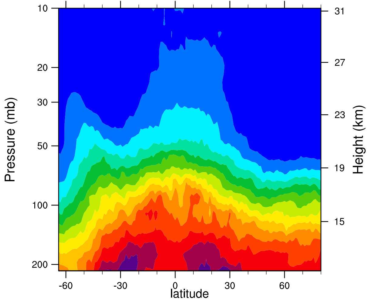
2007d332 12.1MicronExtinction_Combined ( \text{km}^{-1} )
