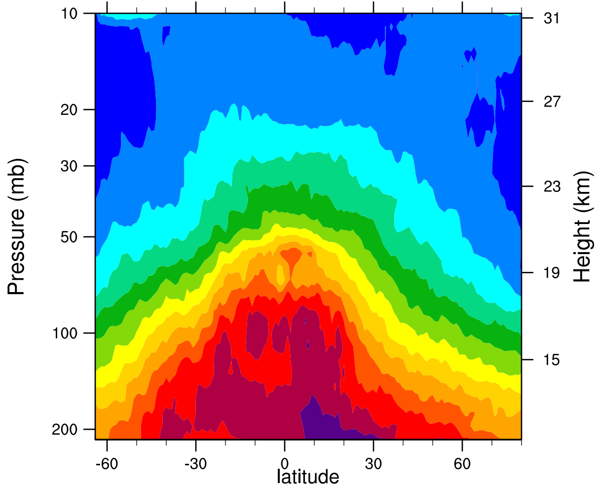
2006d028 12.1MicronExtinction_Combined ( \text{km}^{-1} )
