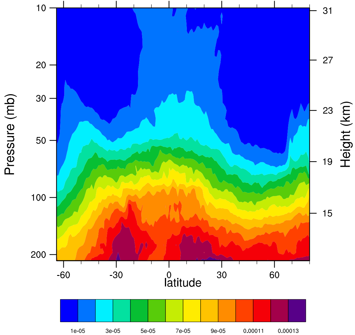
2007d358 12.1MicronExtinction_Combined ( \text{km}^{-1} )
