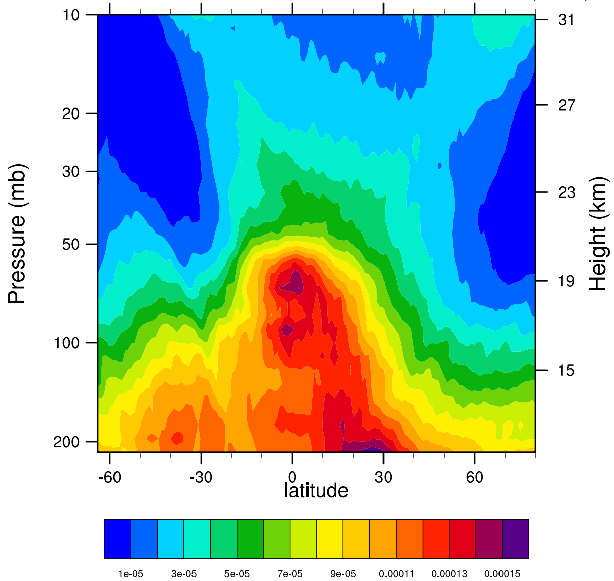
2005d091 12.1MicronExtinction_Combined ( \text{km}^{-1} )
