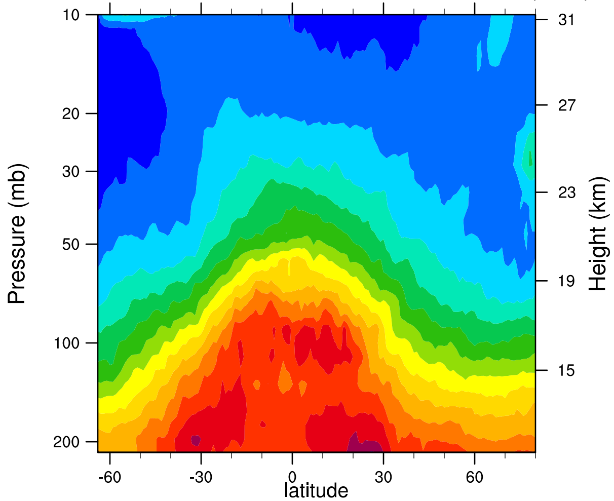
2005d357 12.1MicronExtinction_Combined (km -1 )
