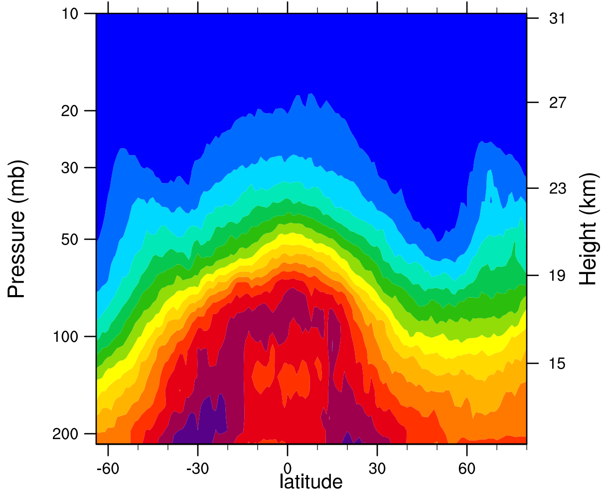
2006d356 12.1MicronExtinction_Combined (km -1 )
