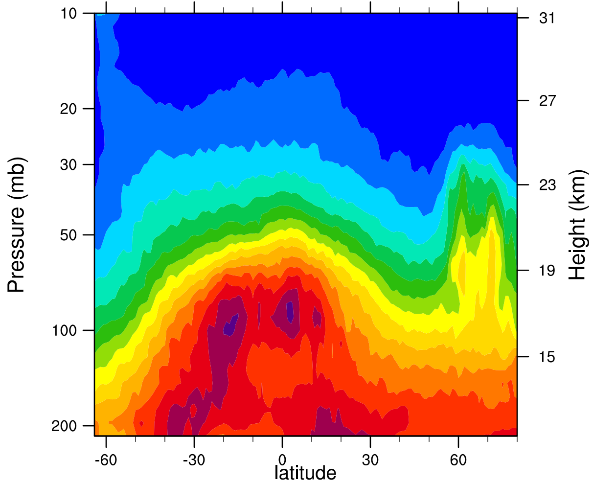
2007d025 12.1MicronExtinction_Combined (km -1 )
