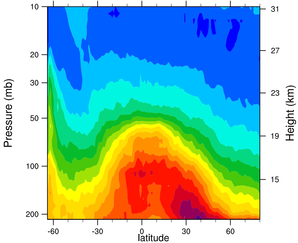
2006d214 12.1MicronExtinction_Combined (km -1 )
