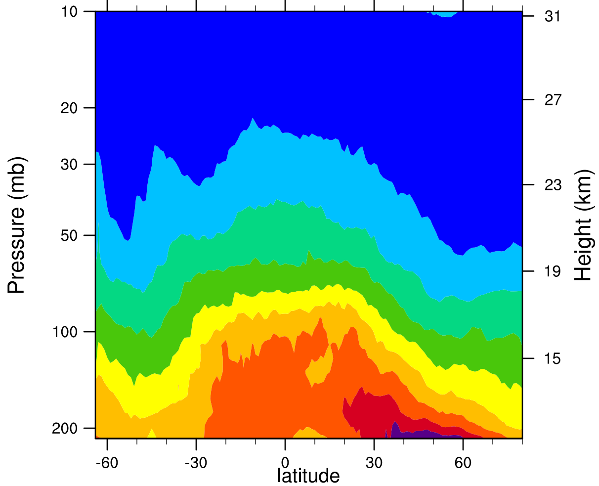
2007d199 12.1MicronExtinction_Combined (km -1 )
