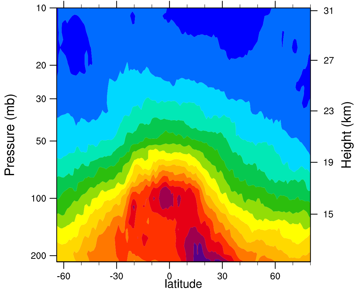
2006d078 12.1MicronExtinction_Combined (km -1 )
