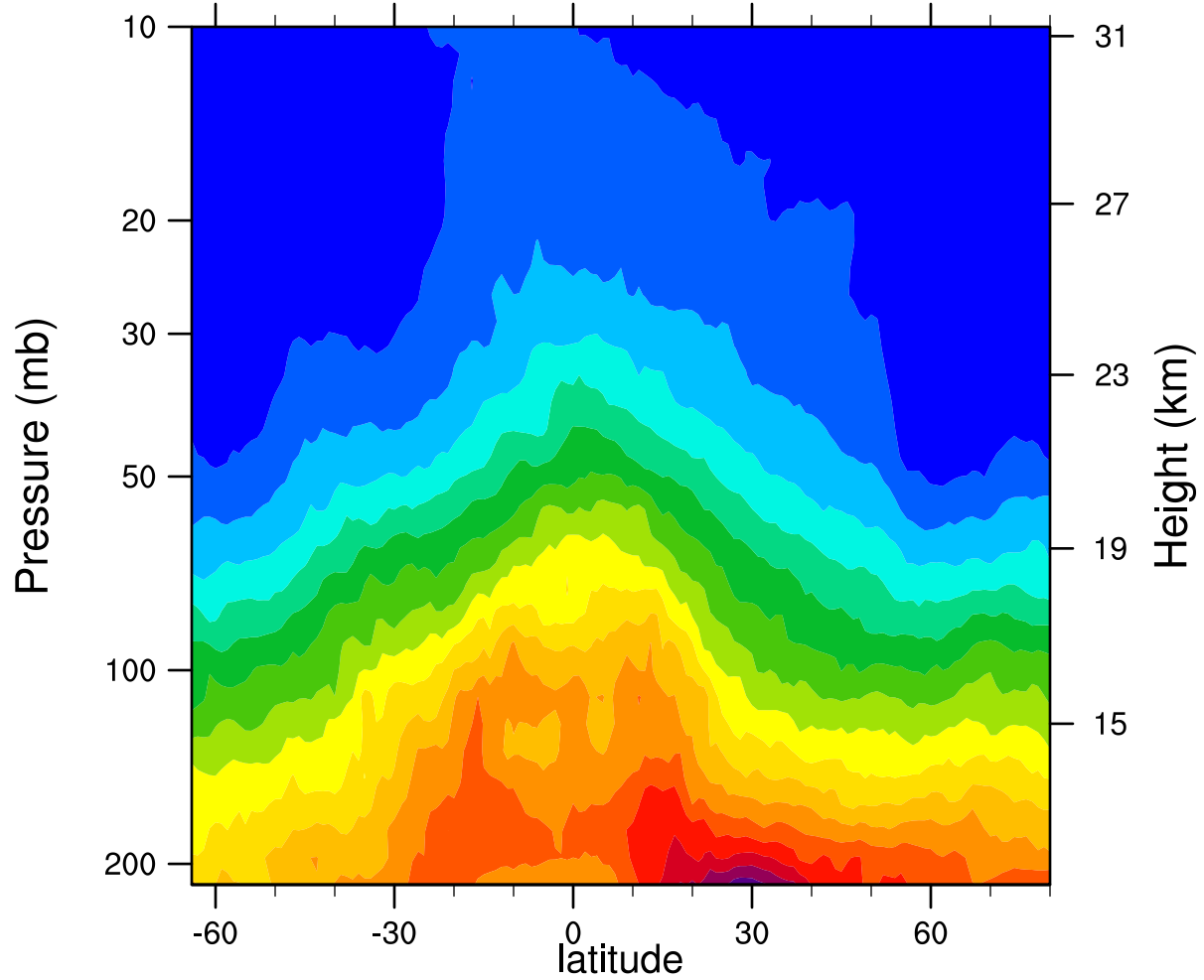
2007d100 12.1MicronExtinction_Combined (km -1 )
