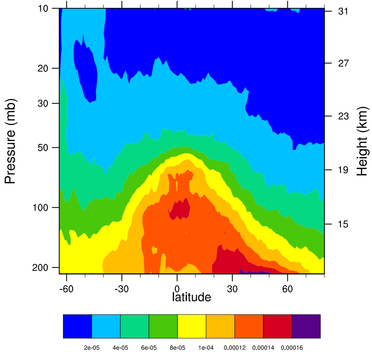
2006d177 12.1MicronExtinction_Combined (km -1 )
