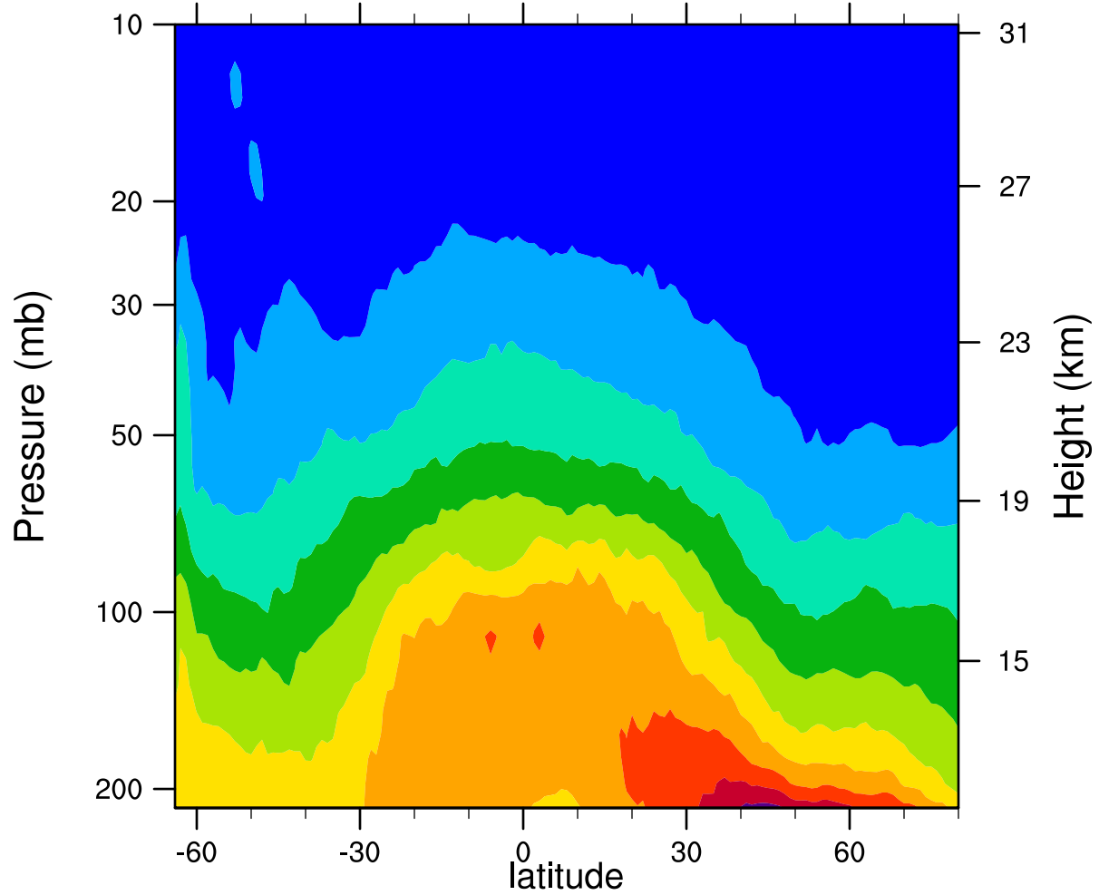
2007d181 12.1MicronExtinction_Combined (km -1 )
