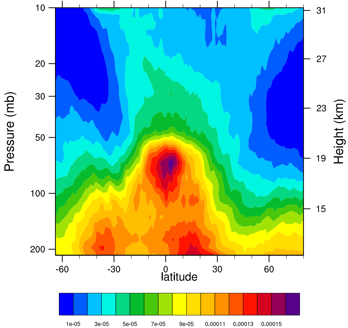
2005d059 12.1MicronExtinction_Combined (km -1 )
