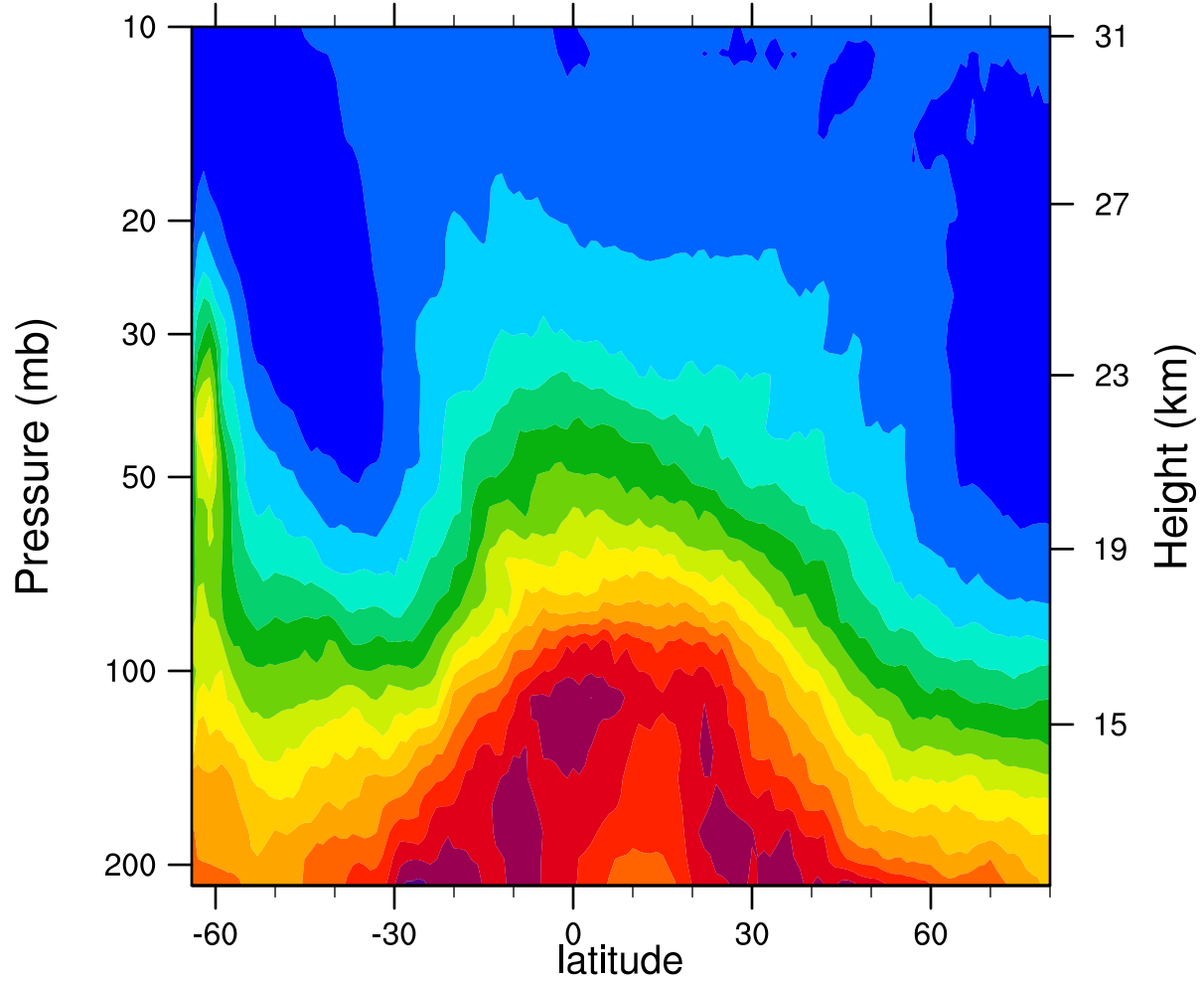
2005d244 12.1MicronExtinction_Combined (km -1 )
