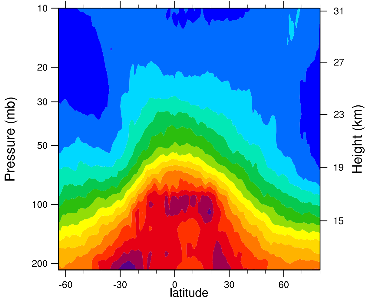
2005d305 12.1MicronExtinction_Combined (km -1 )
