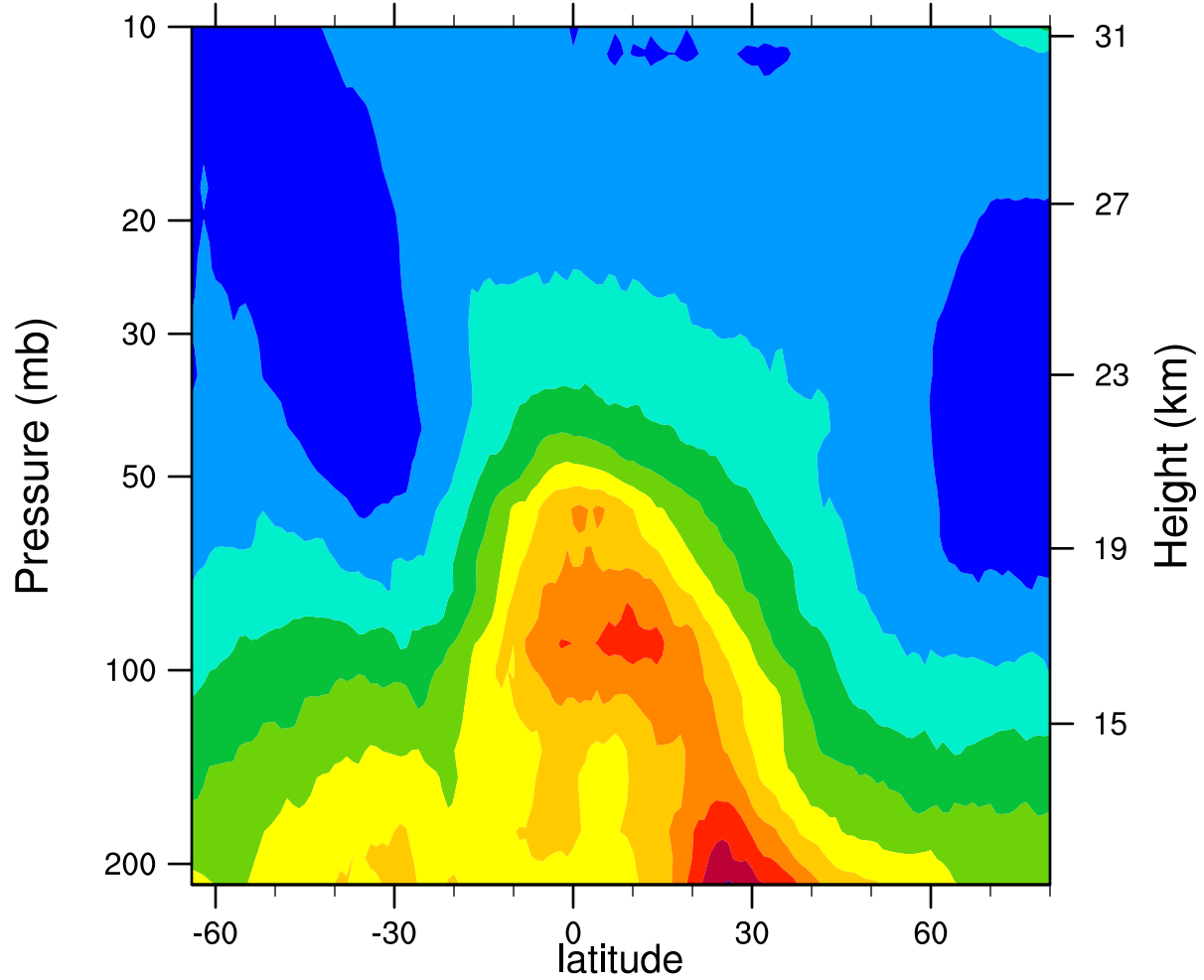
2005d128 12.1MicronExtinction_Combined (km -1 )
