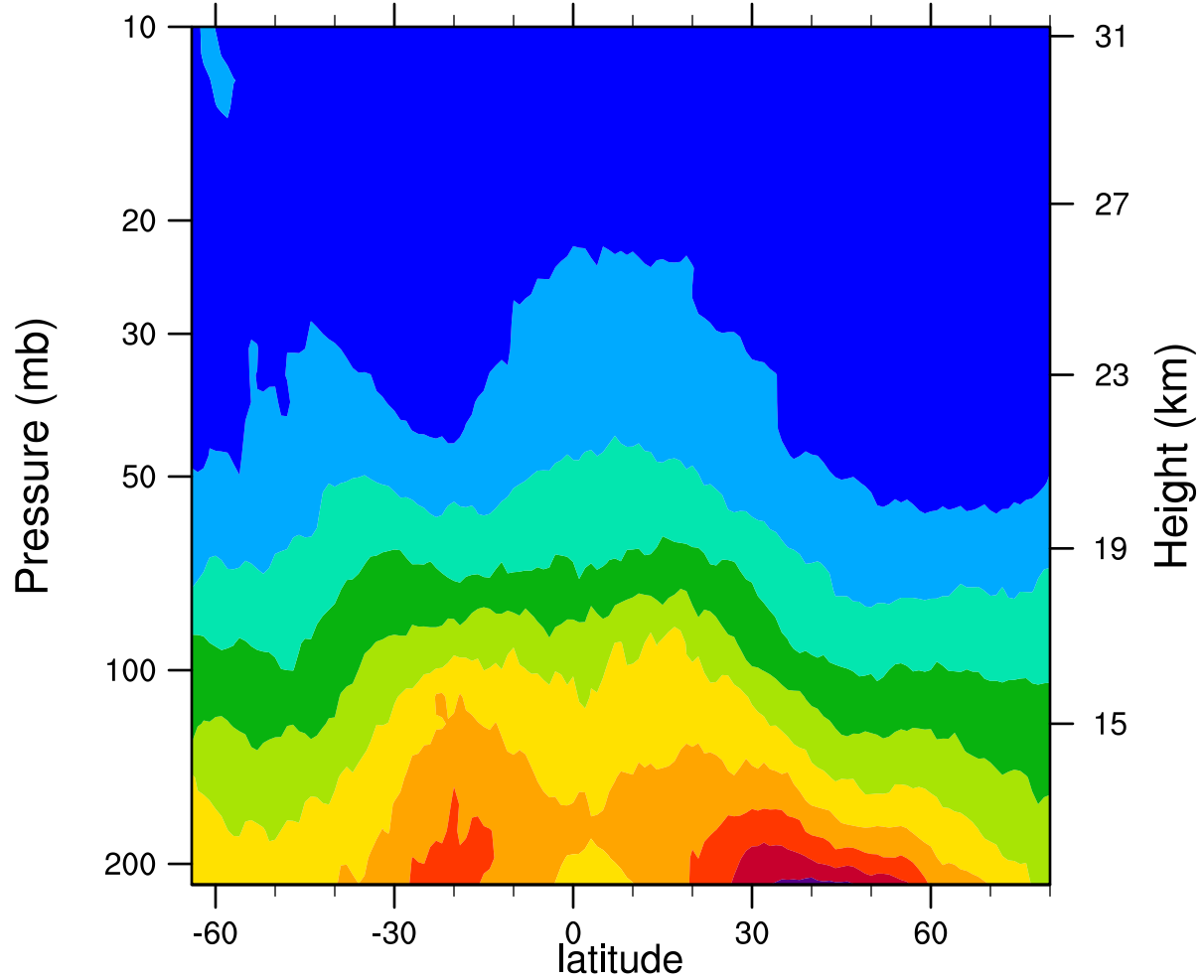
2007d148 12.1MicronExtinction_Combined (km -1 )
