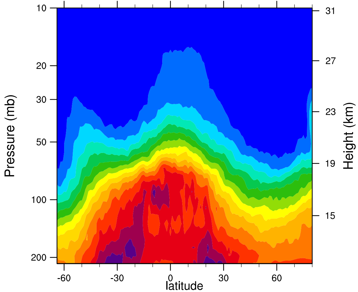
2006d350 12.1MicronExtinction_Combined (km -1 )
