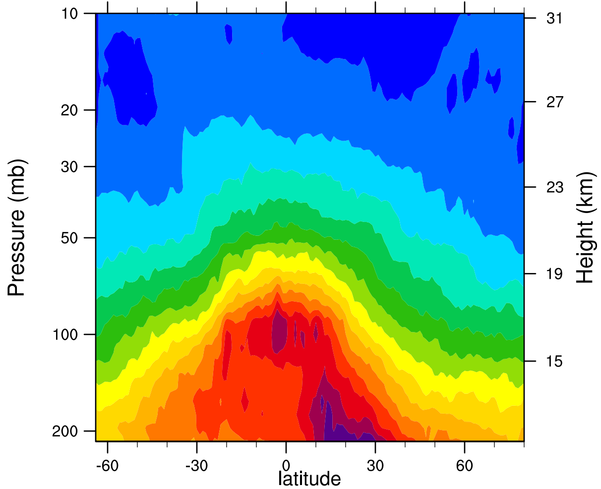
2006d081 12.1MicronExtinction_Combined (km -1 )
