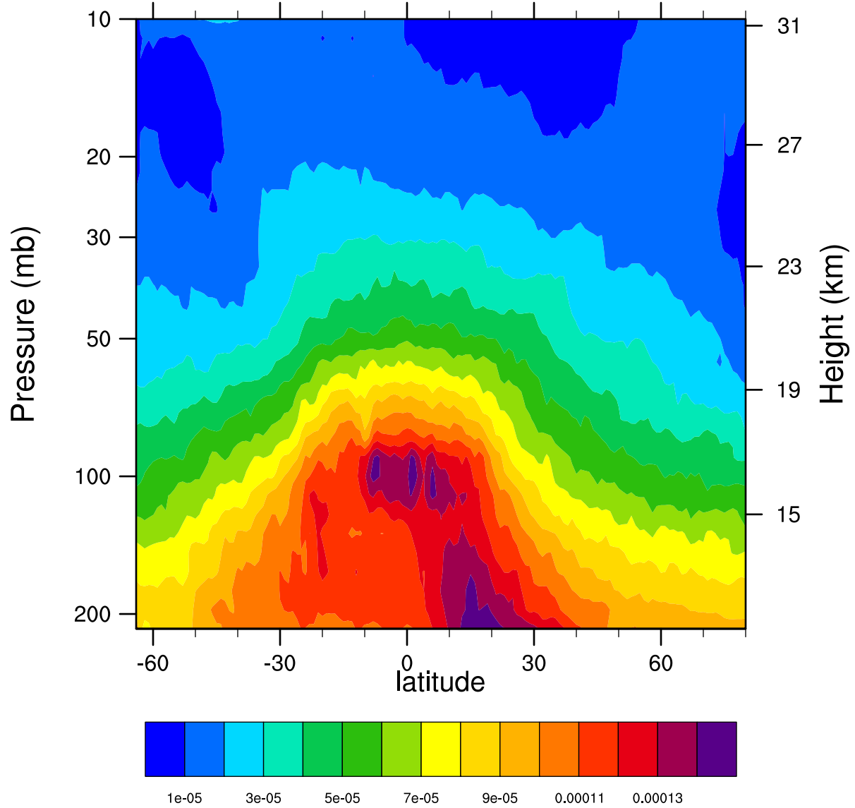
2006d071 12.1MicronExtinction_Combined (km -1 )
