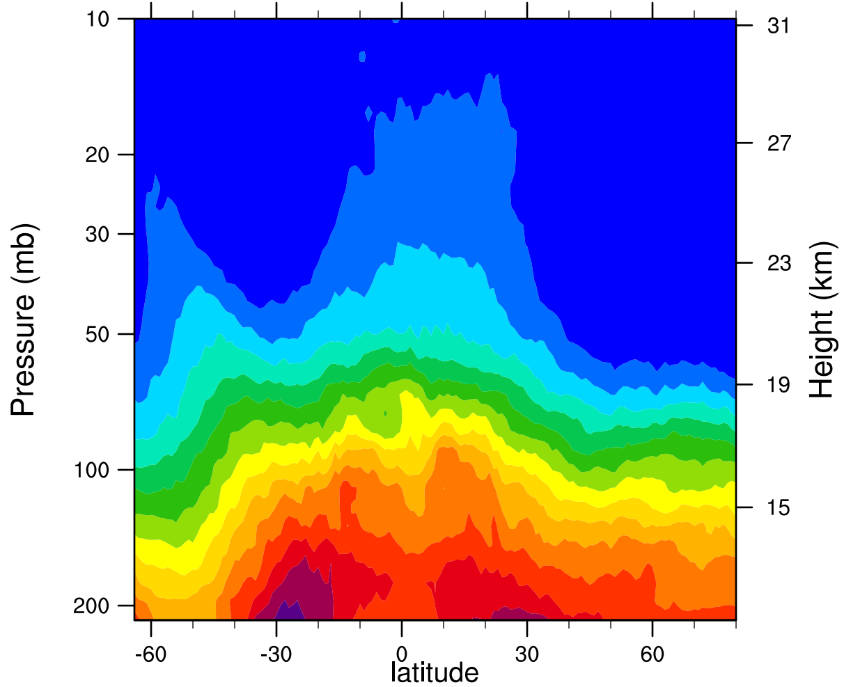
2007d320 12.1MicronExtinction_Combined (km -1 )
