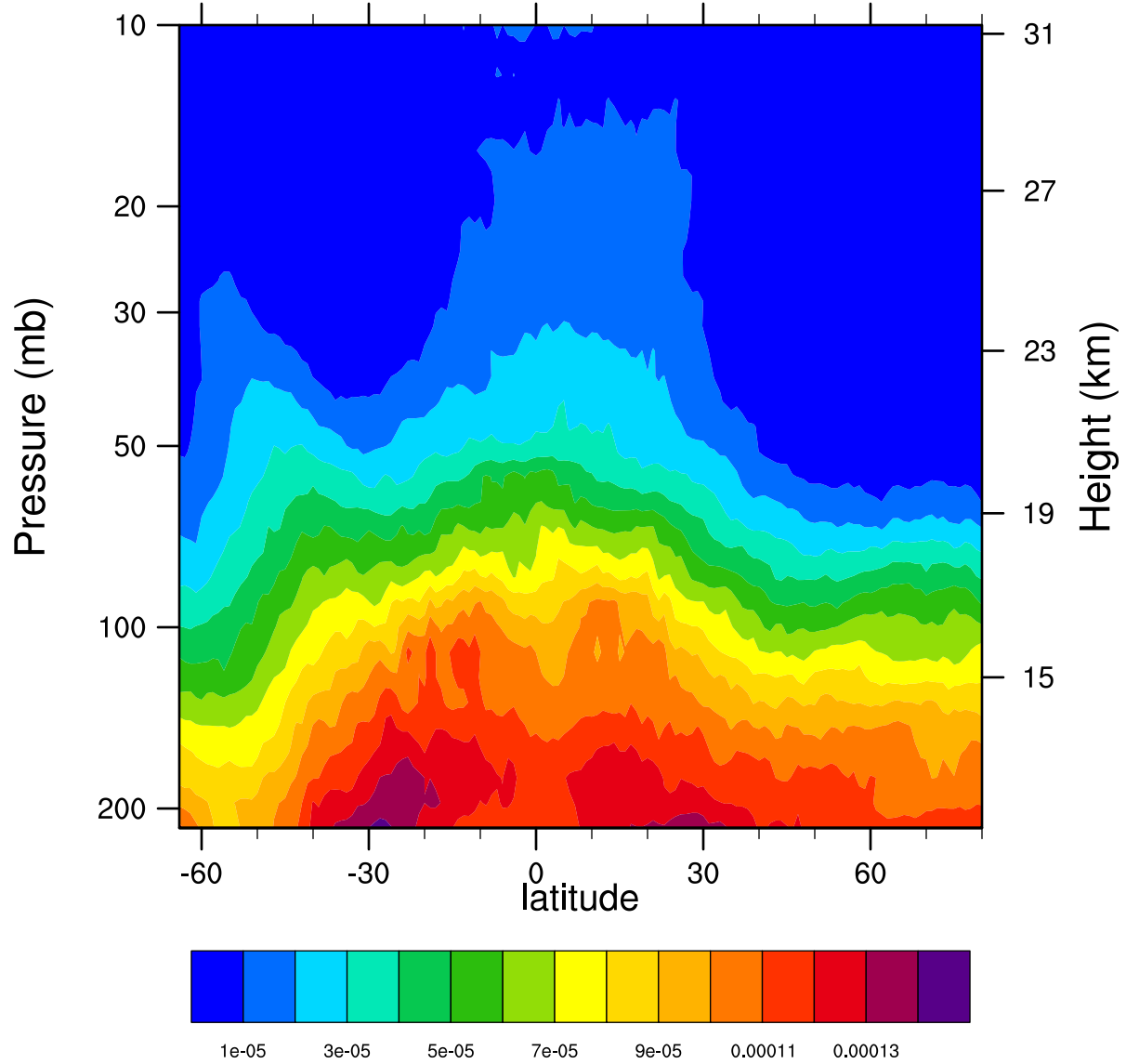
2007d324 12.1MicronExtinction_Combined (km -1 )
