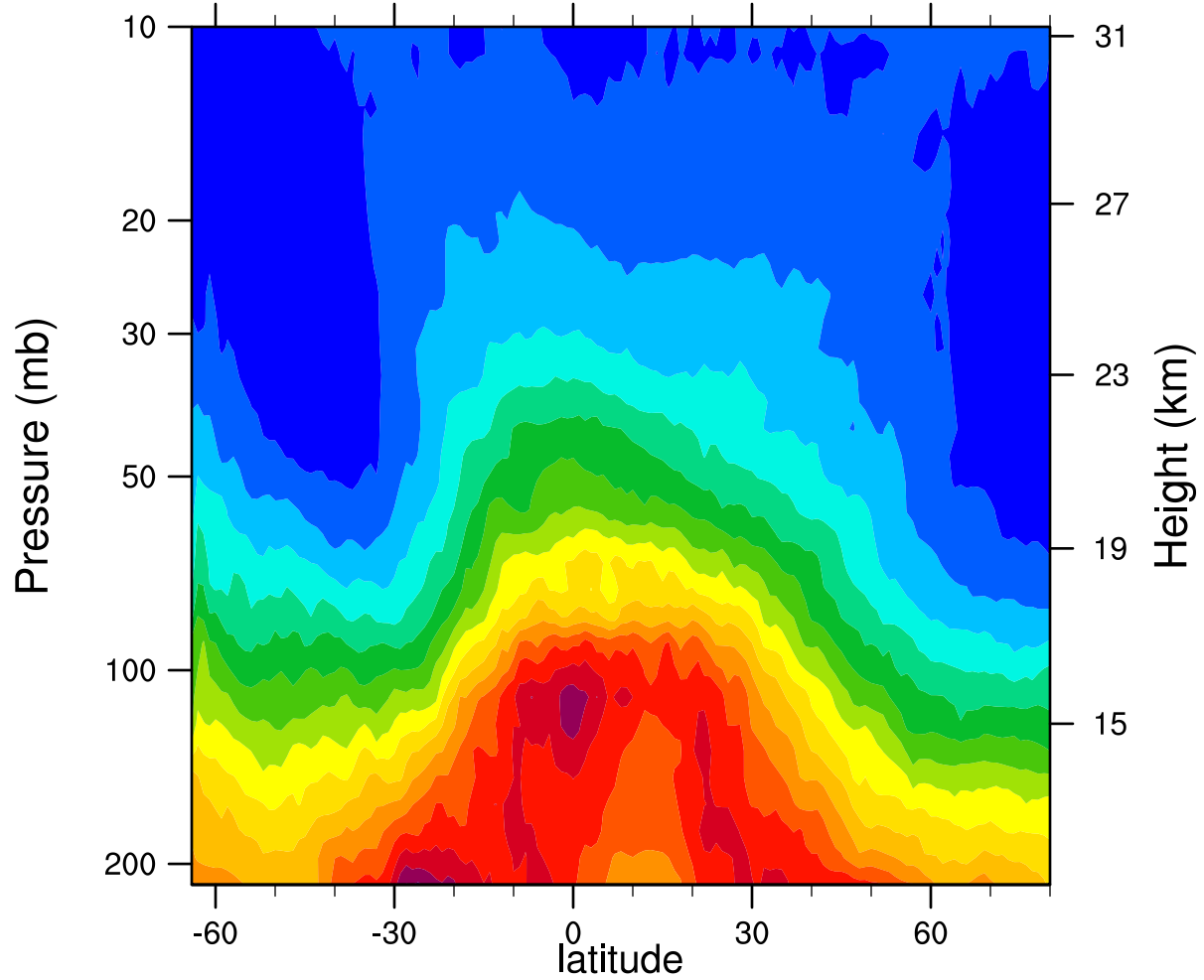
2005d250 12.1MicronExtinction_Combined ( \text{km}^{-1} )
