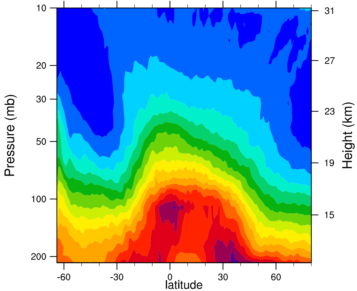
2005d224 12.1MicronExtinction_Combined (km -1 )
