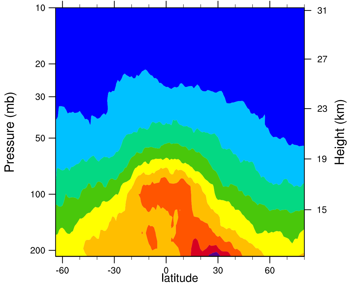
2006d099 12.1MicronExtinction_Combined (km -1 )
