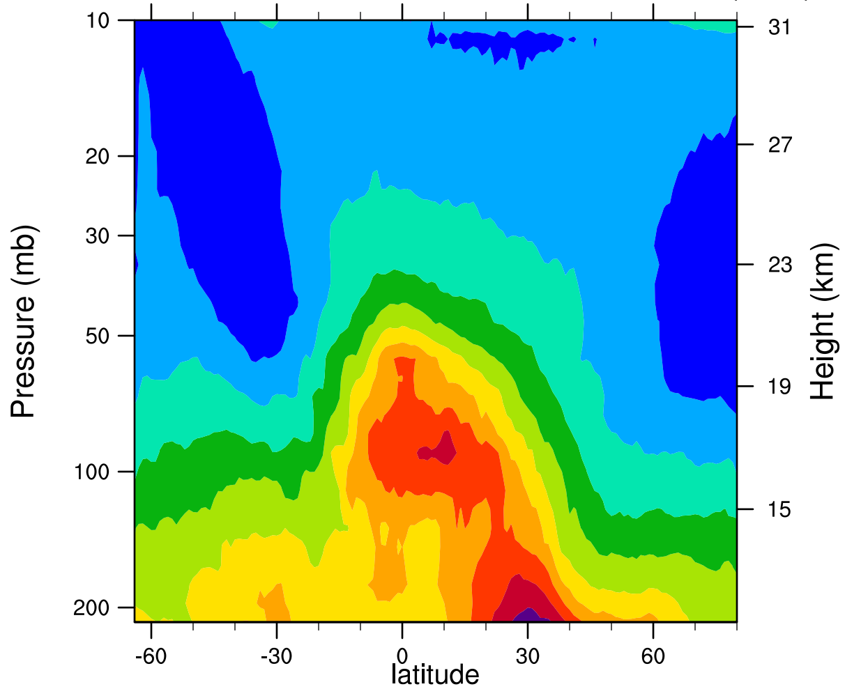
2005d135 12.1MicronExtinction_Combined (km -1 )
