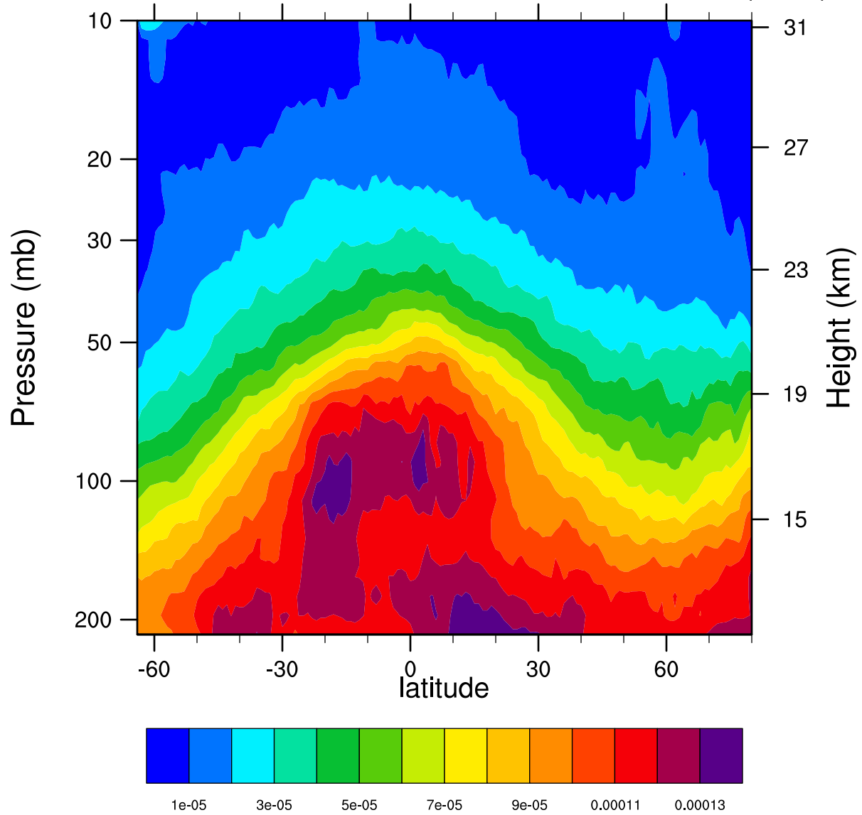
2007d036 12.1MicronExtinction_Combined ( \text{km}^{-1} )
