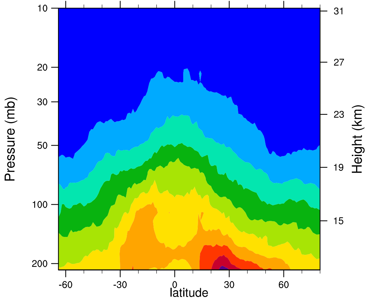
2007d114 12.1MicronExtinction_Combined (km -1 )
