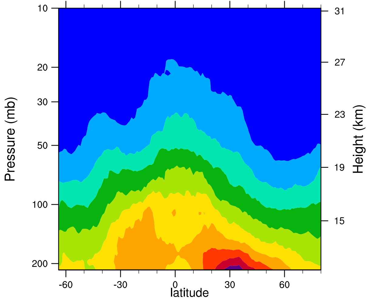
2007d126 12.1MicronExtinction_Combined (km -1 )
