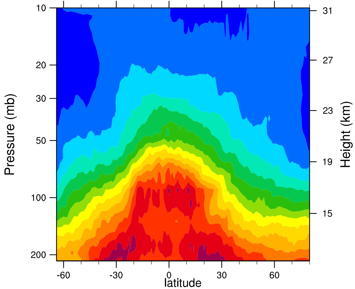
2005d338 12.1MicronExtinction_Combined (km -1 )
