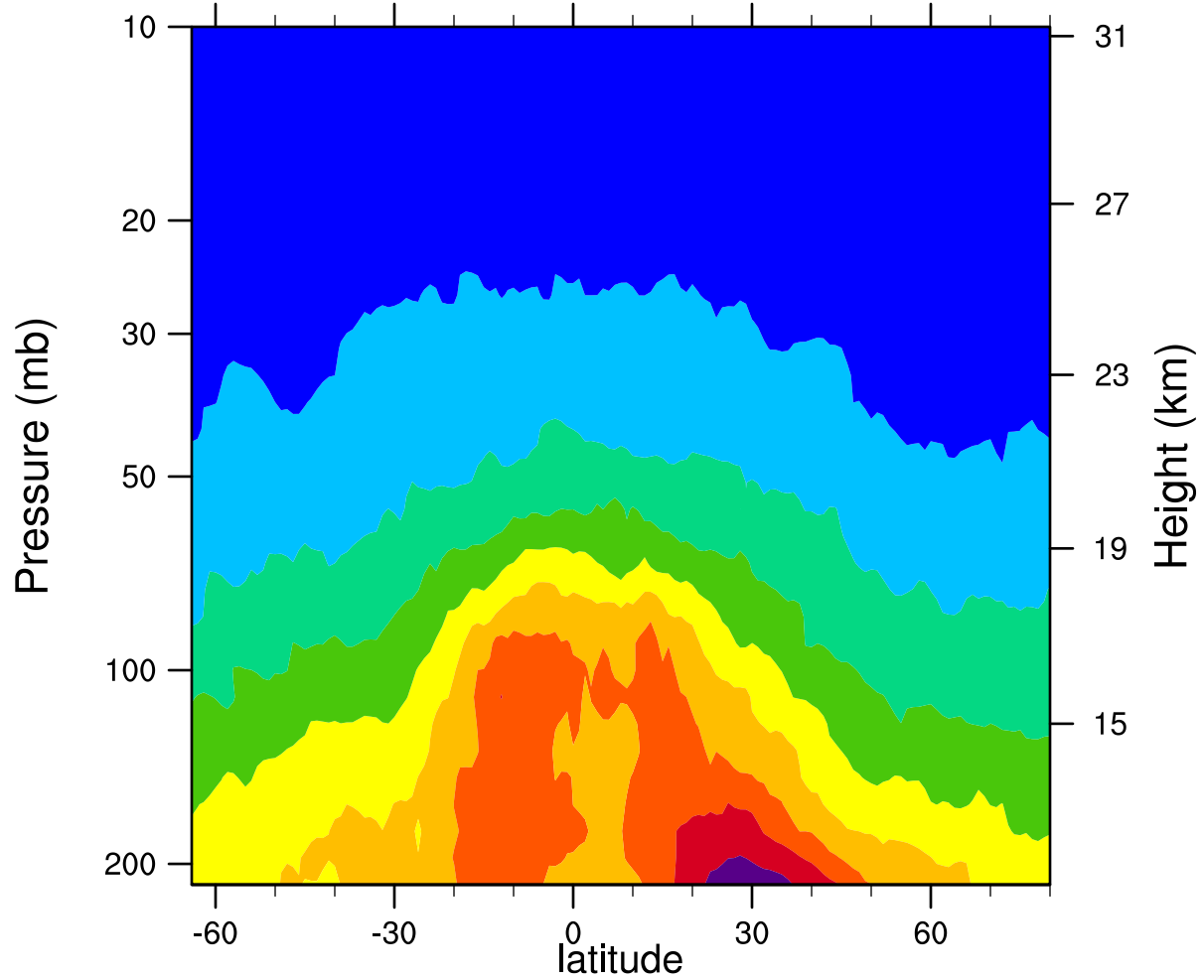
2006d129 12.1MicronExtinction_Combined (km -1 )
