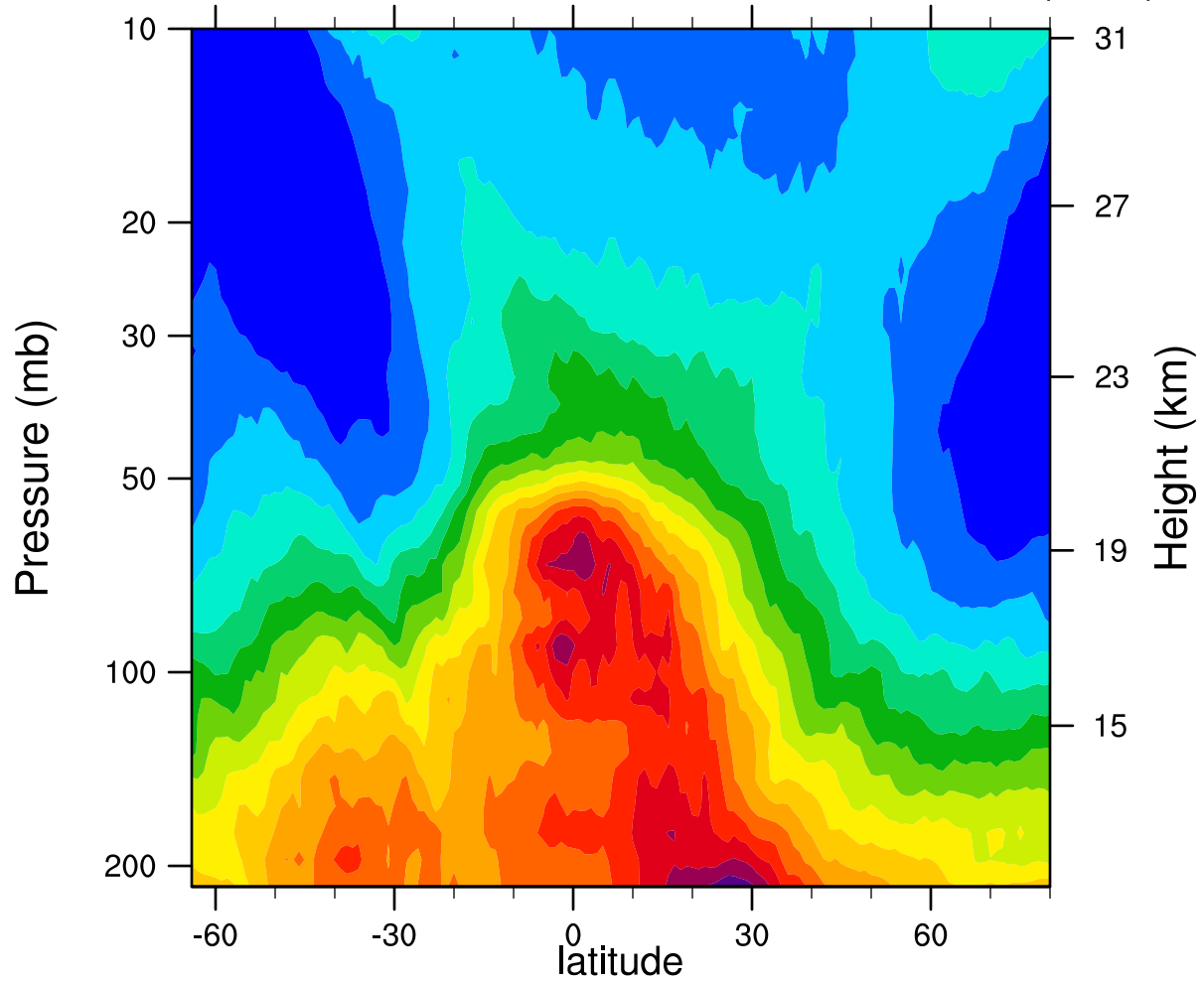
2005d092 12.1MicronExtinction_Combined (km -1 )
