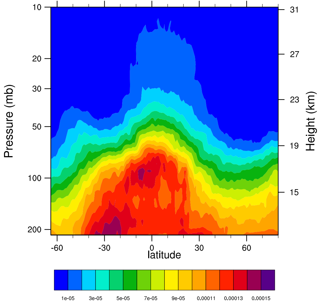
2006d335 12.1MicronExtinction_Combined (km -1 )
