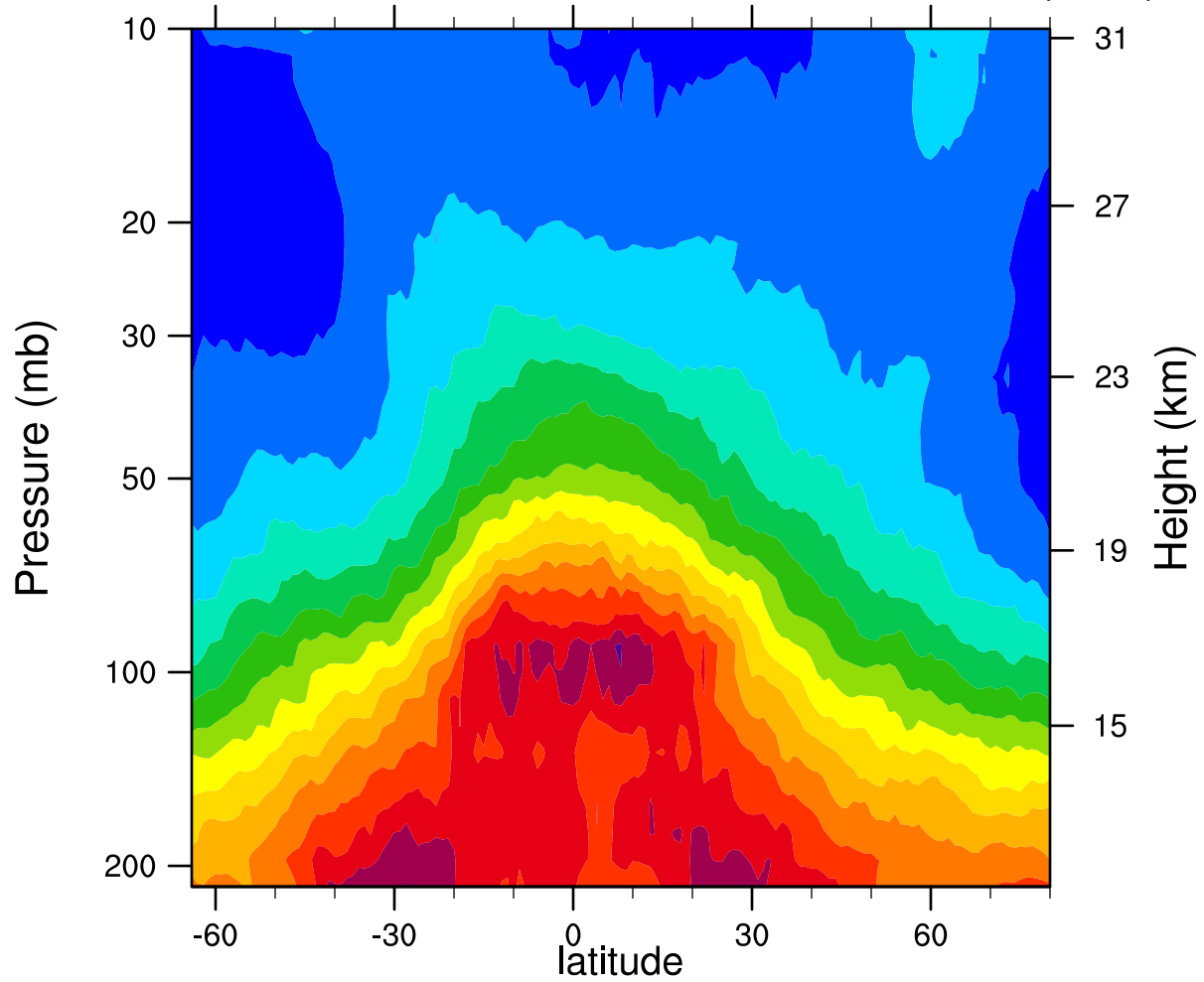
2005d318 12.1MicronExtinction_Combined ( \text{km}^{-1} )
