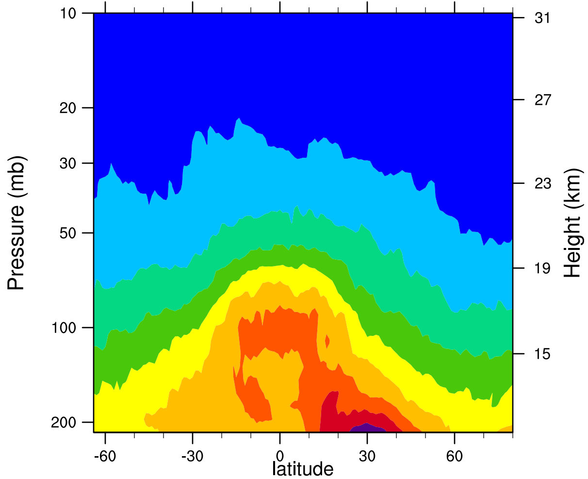
2006d107 12.1MicronExtinction_Combined (km -1 )
