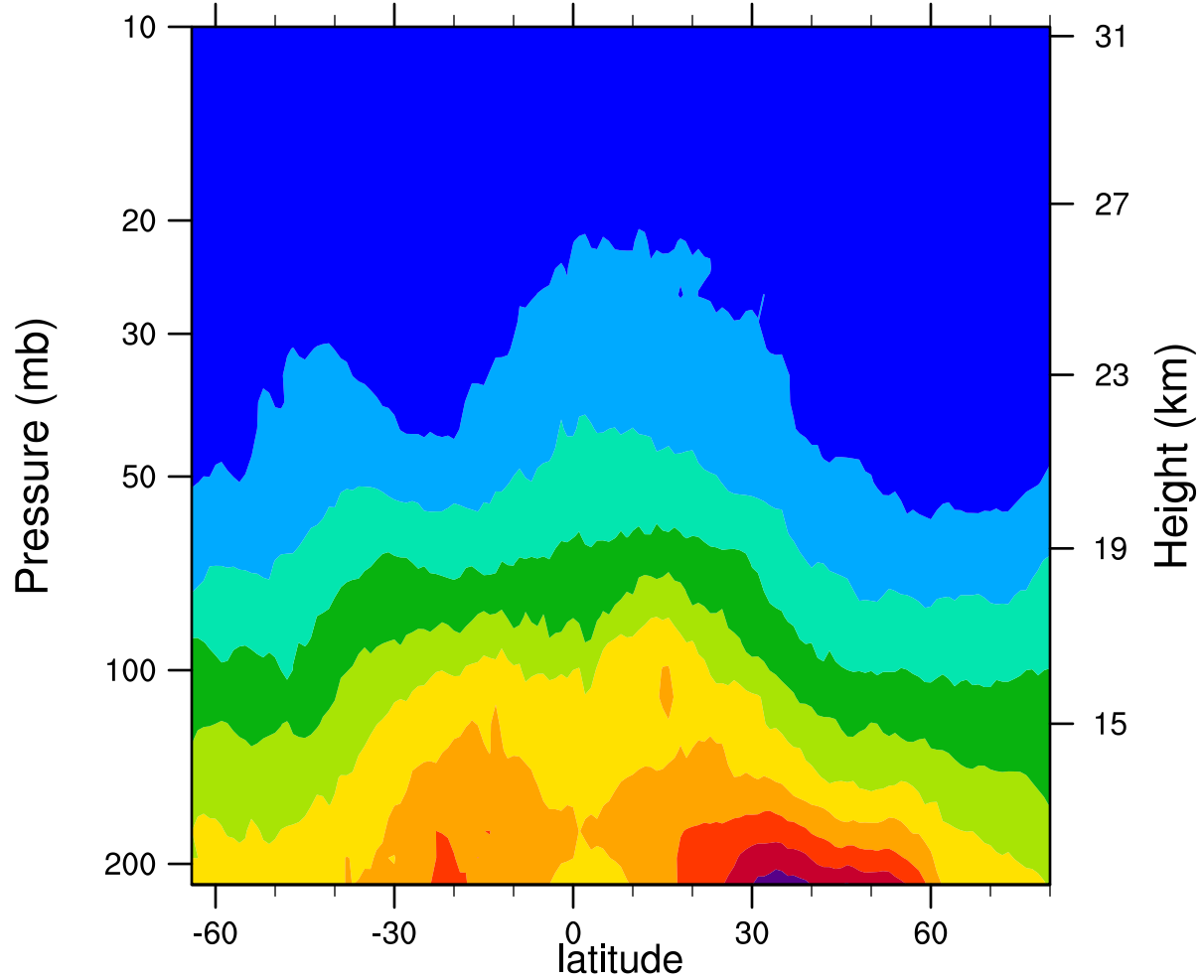
2007d142 12.1MicronExtinction_Combined (km -1 )
