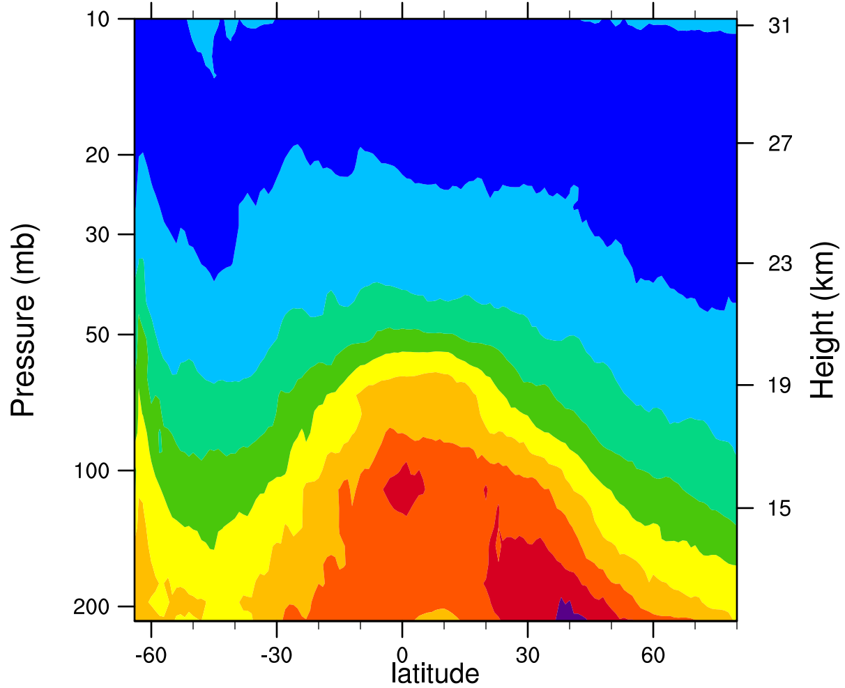
2006d222 12.1MicronExtinction_Combined (km -1 )
