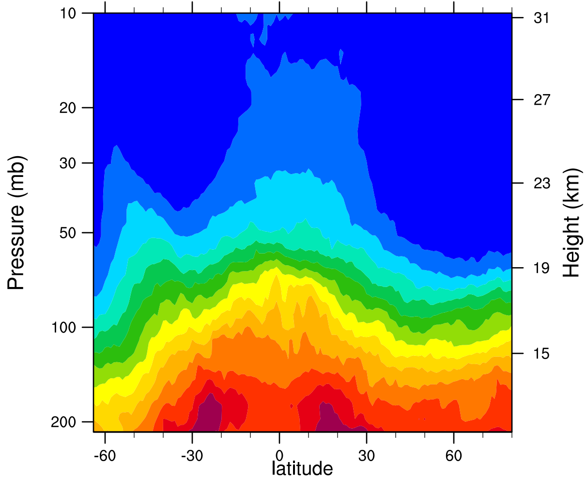
2007d339 12.1MicronExtinction_Combined ( \text{km}^{-1} )
