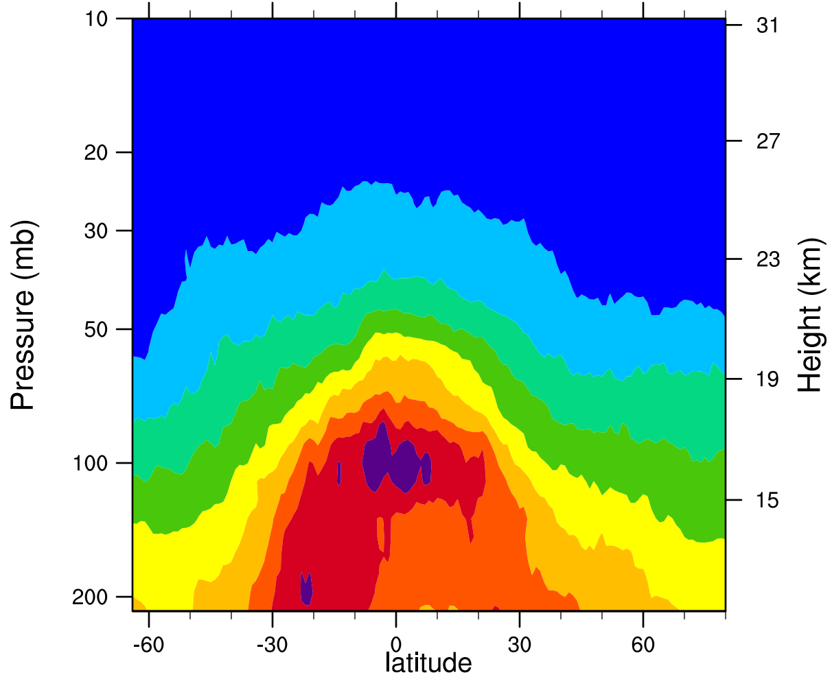
2006d308 12.1MicronExtinction_Combined (km -1 )
