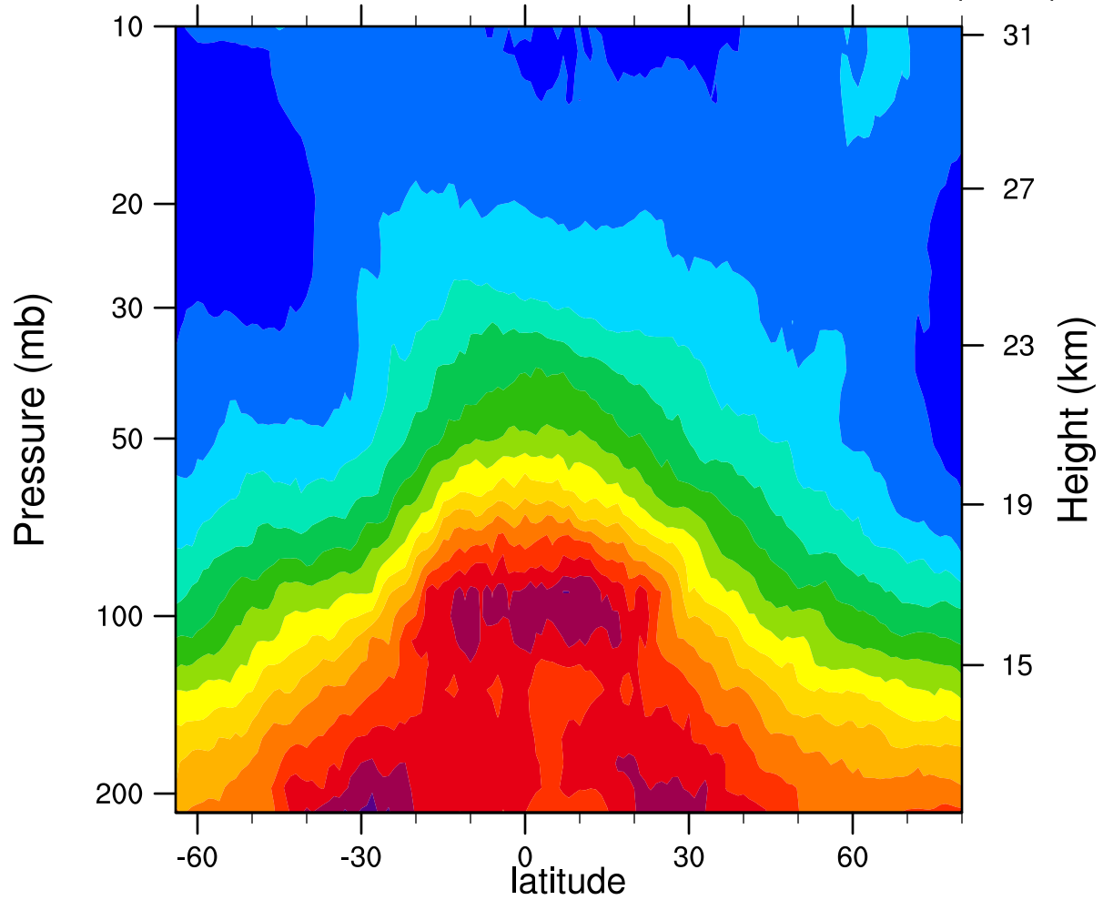
2005d316 12.1MicronExtinction_Combined (km -1 )
