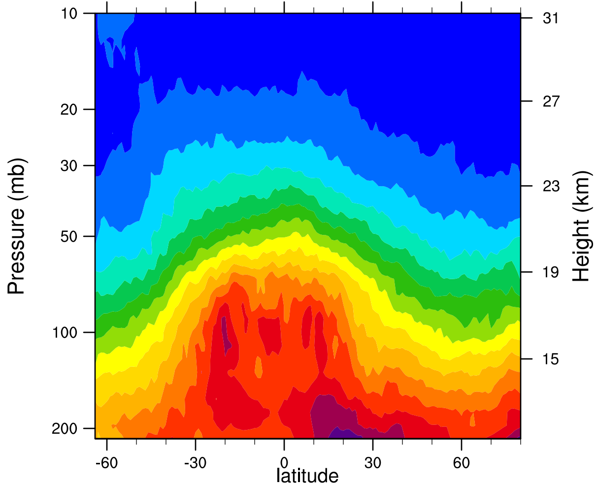
2007d072 12.1MicronExtinction_Combined ( \text{km}^{-1} )
