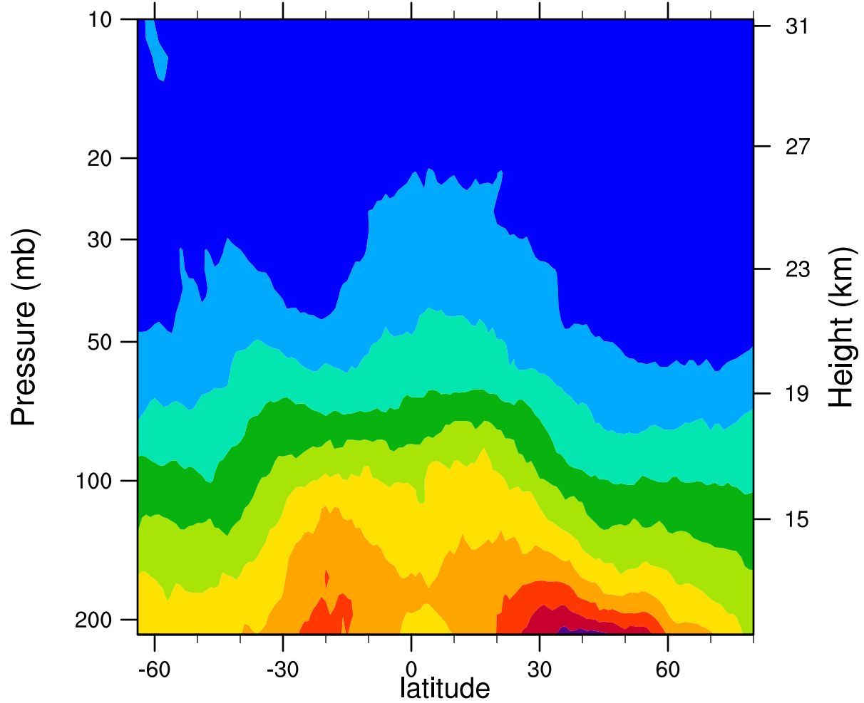
2007d150 12.1MicronExtinction_Combined ( \text{km}^{-1} )
