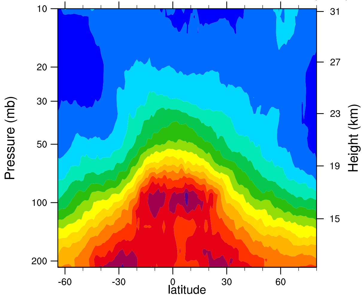
2005d317 12.1MicronExtinction_Combined (km -1 )
