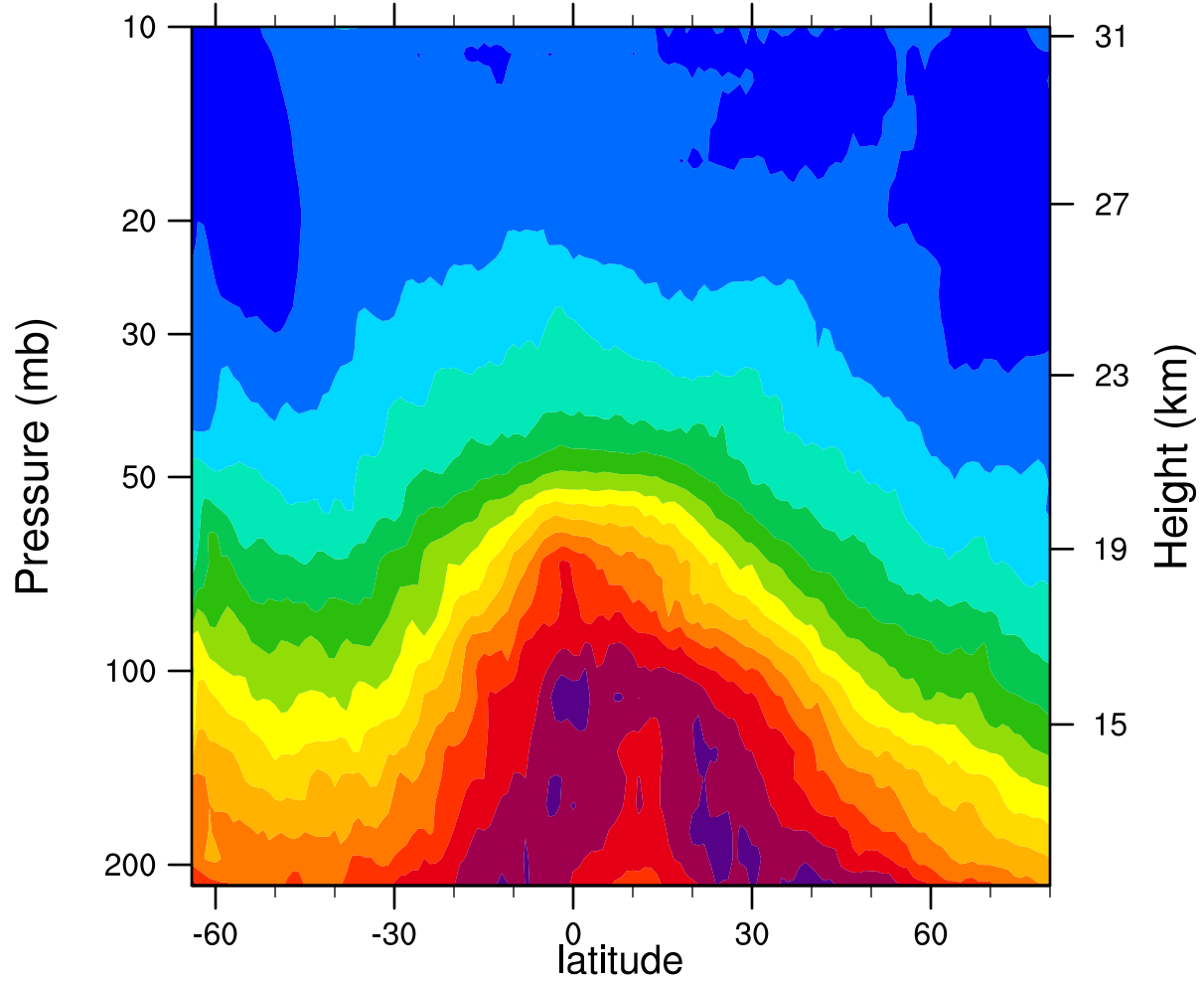
2006d245 12.1MicronExtinction_Combined (km -1 )
