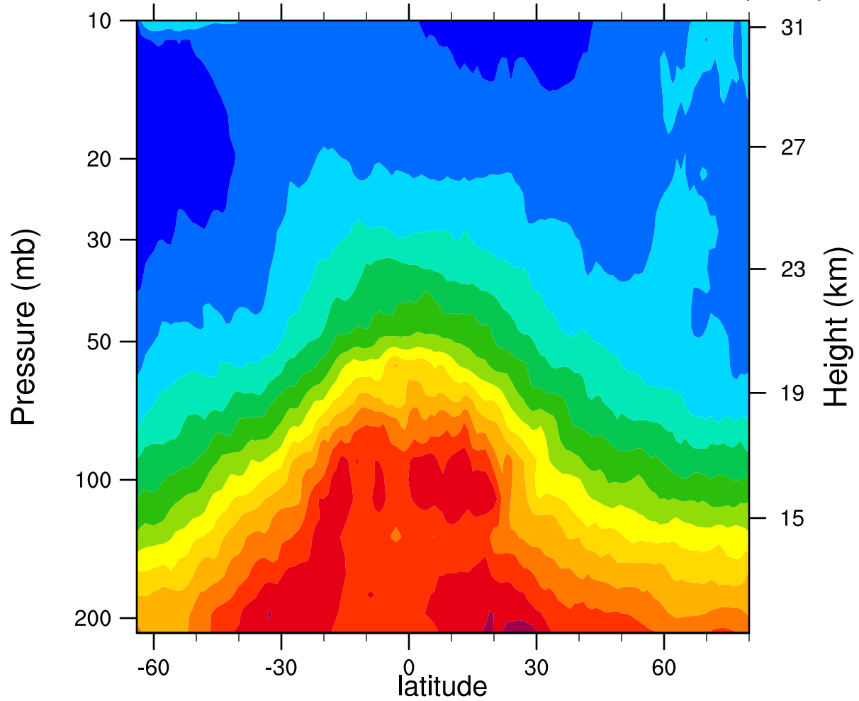
2005d350 12.1MicronExtinction_Combined ( \text{km}^{-1} )
