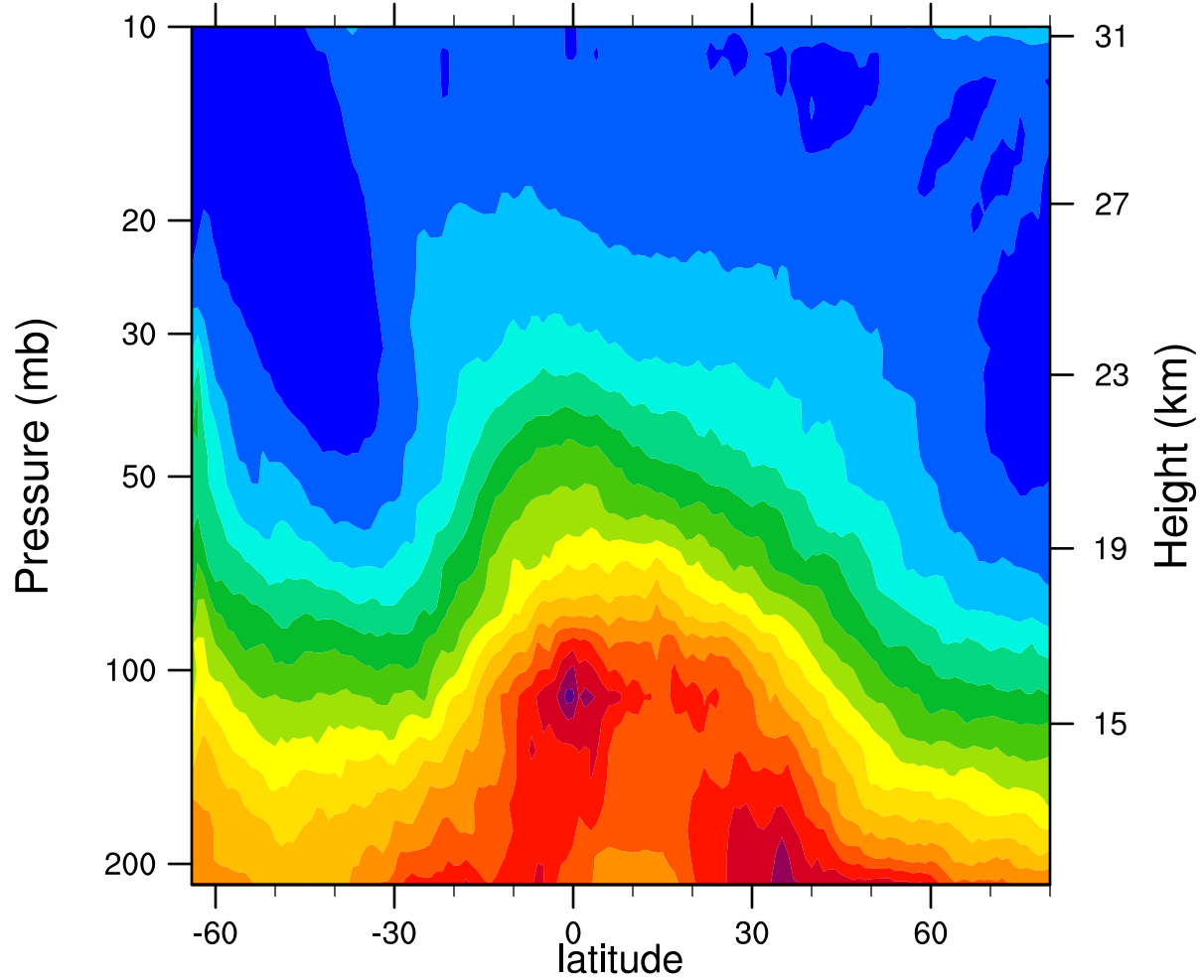
2005d221 12.1MicronExtinction_Combined (km -1 )
