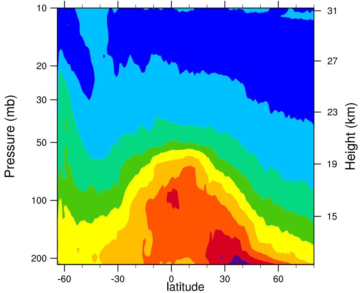
2006d192 12.1MicronExtinction_Combined (km -1 )
