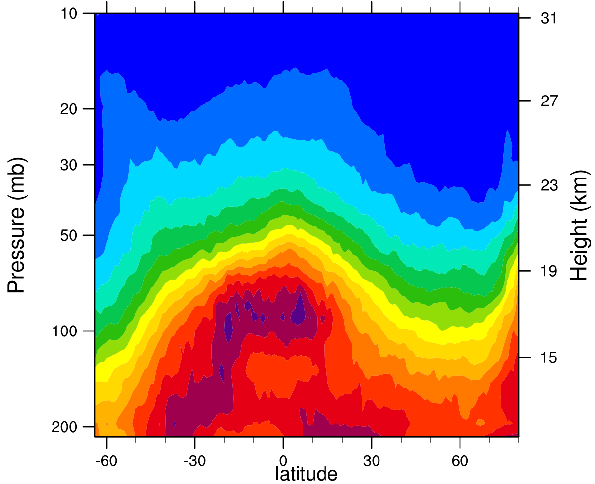
2007d015 12.1MicronExtinction_Combined ( \text{km}^{-1} )
