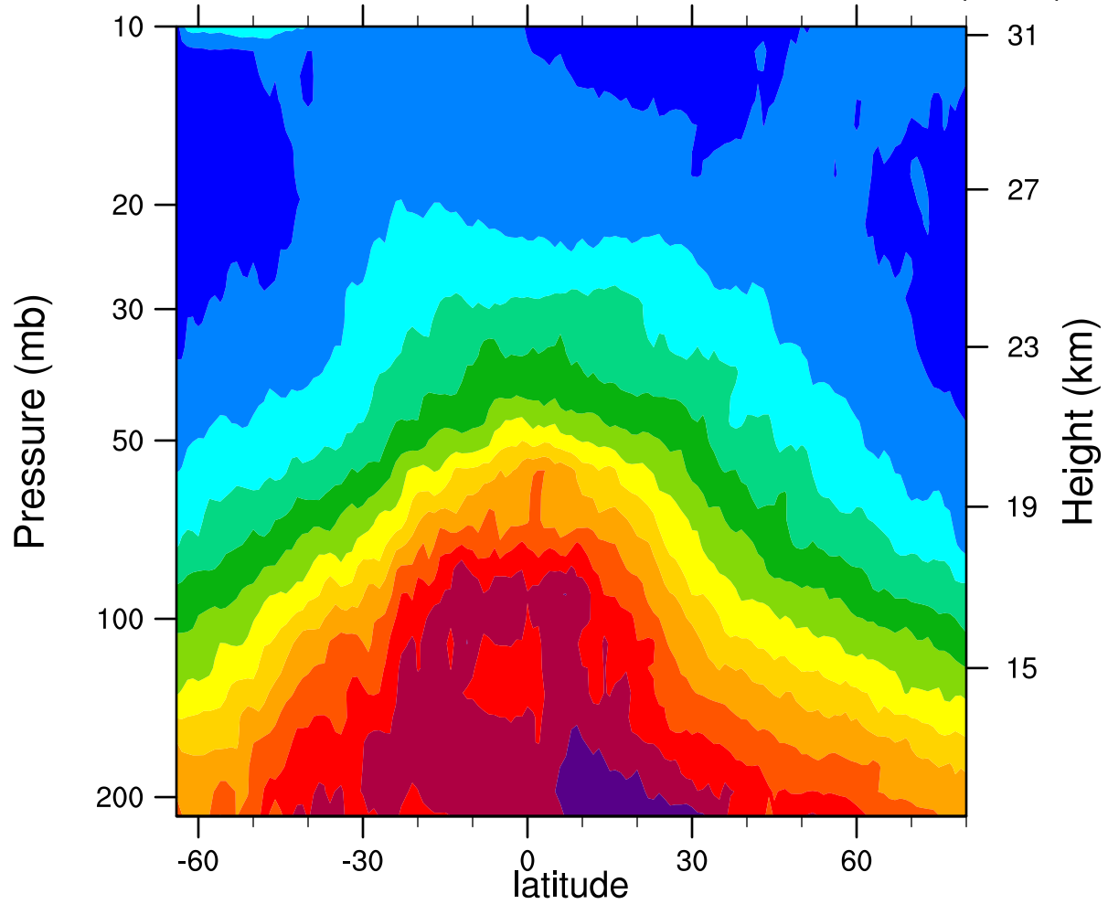
2006d034 12.1MicronExtinction_Combined (km -1 )
