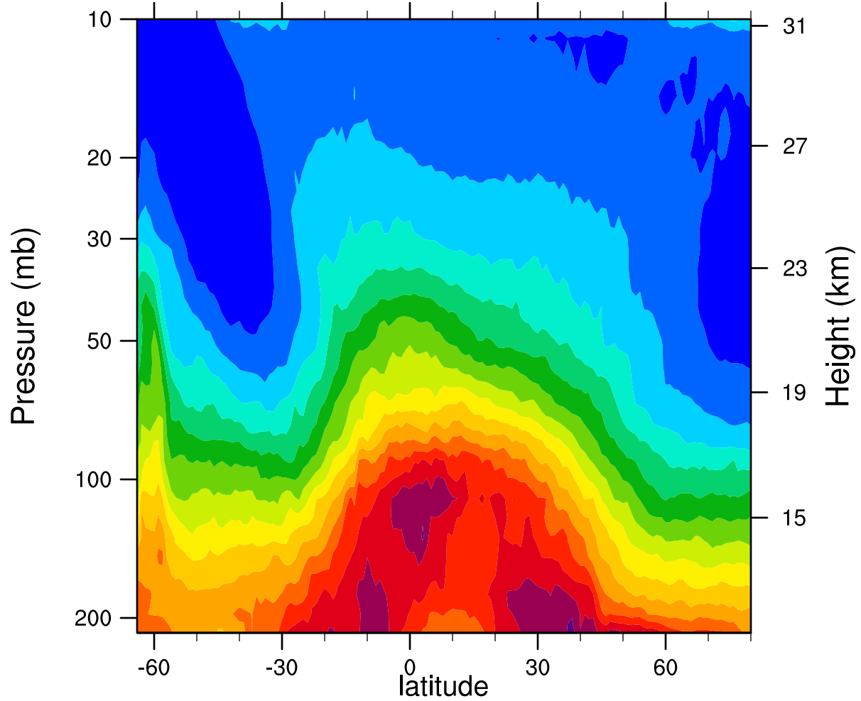
2005d229 12.1MicronExtinction_Combined (km -1 )
