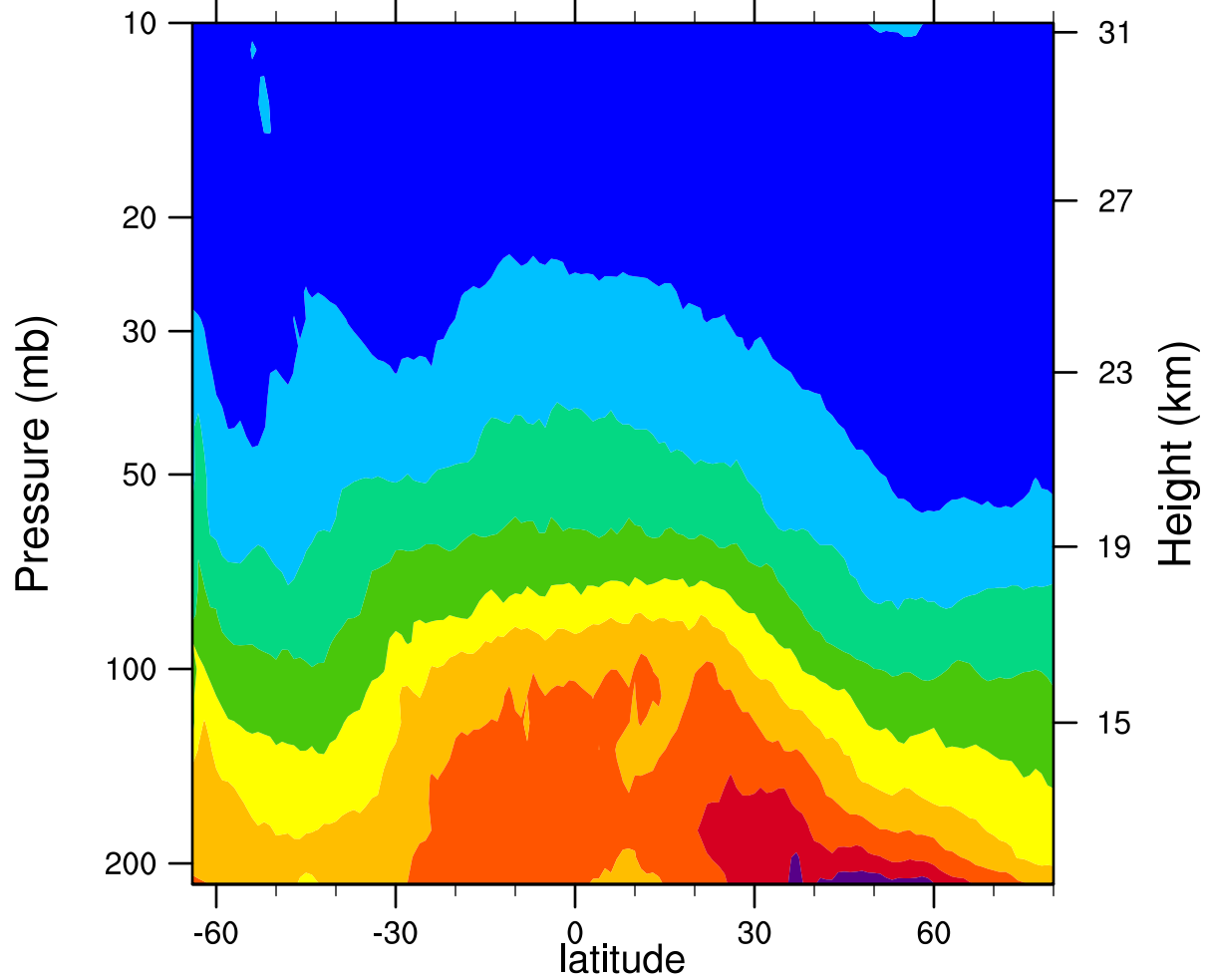
2007d201 12.1MicronExtinction_Combined (km -1 )
