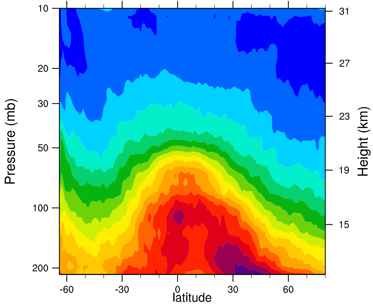
2006d229 12.1MicronExtinction_Combined (km -1 )
