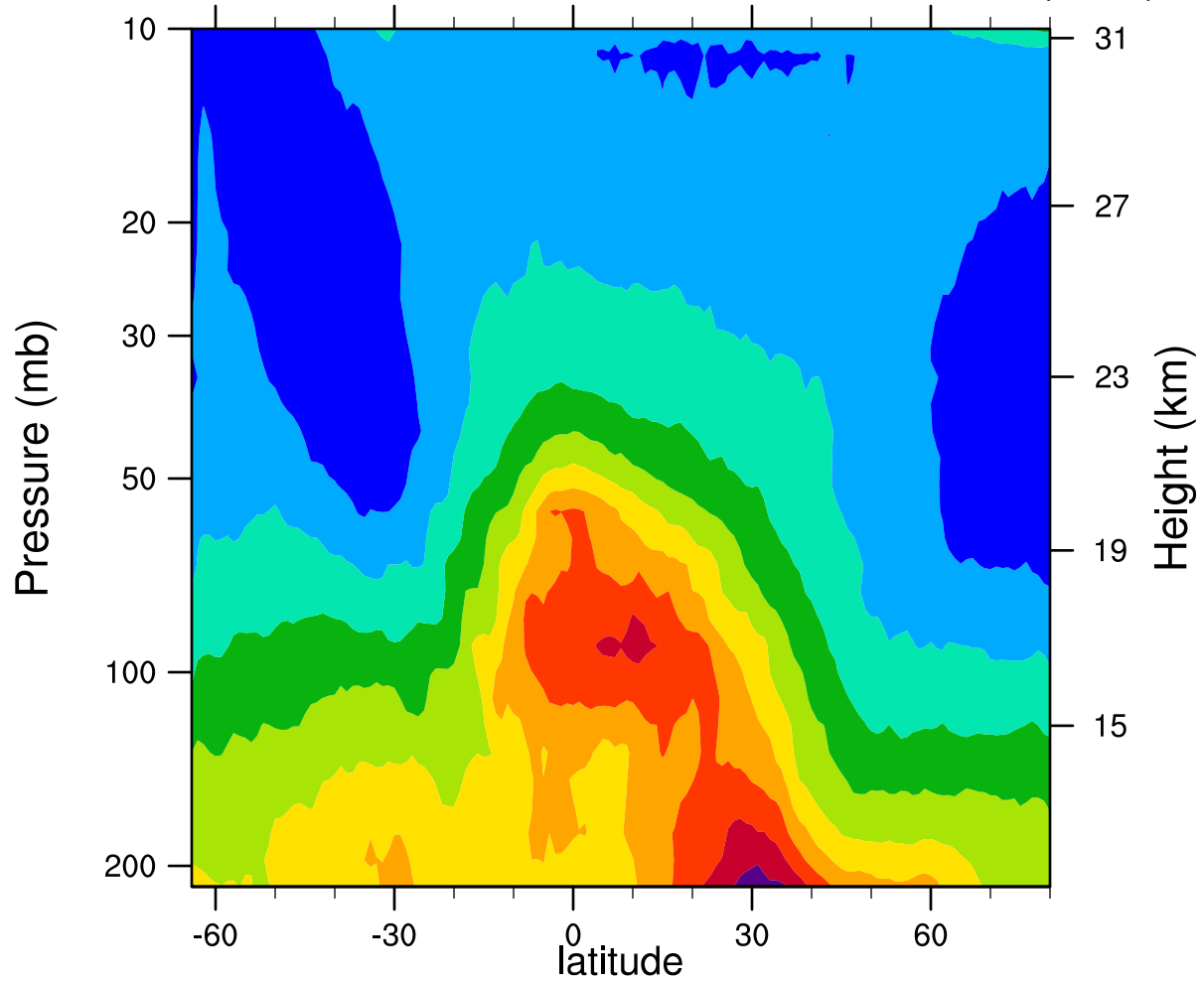
2005d136 12.1MicronExtinction_Combined (km -1 )
