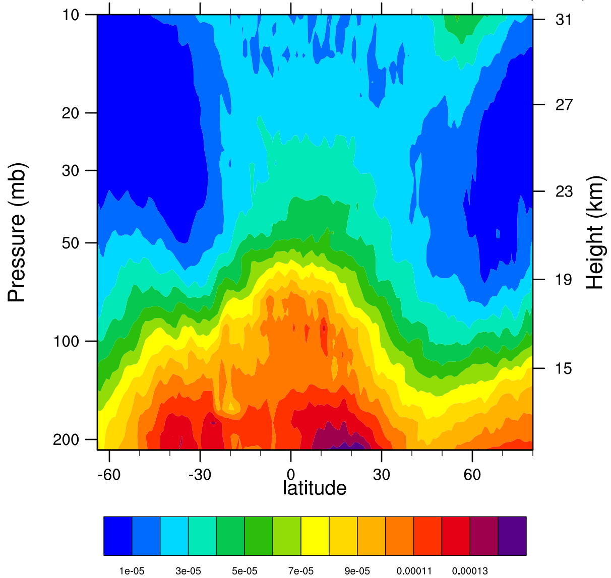
2005d031 12.1MicronExtinction_Combined ( \text{km}^{-1} )
