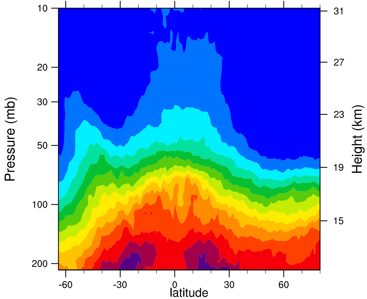
2007d334 12.1MicronExtinction_Combined ( \text{km}^{-1} )
