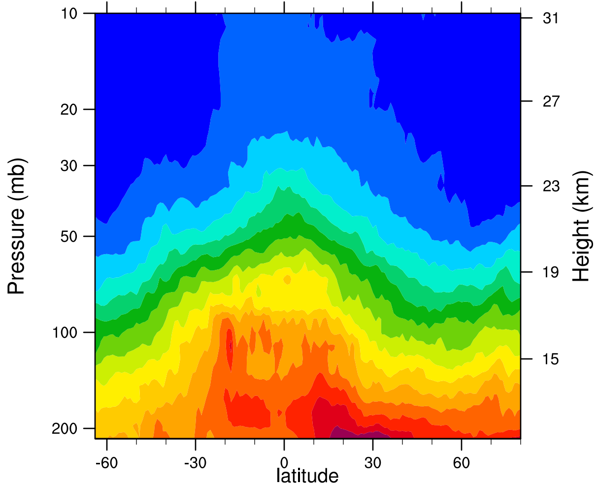
2007d086 12.1MicronExtinction_Combined (km -1 )
