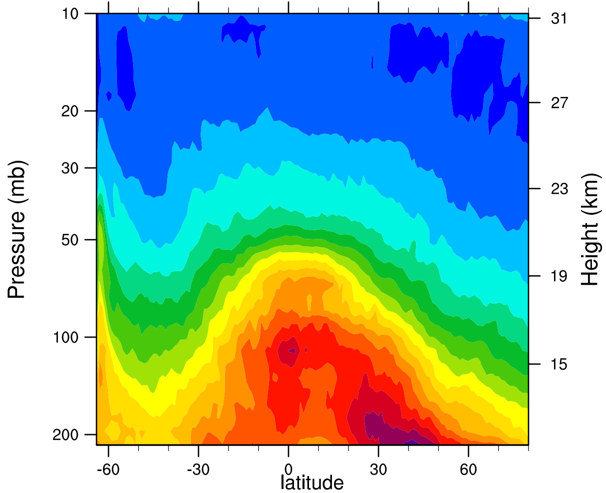
2006d225 12.1MicronExtinction_Combined (km -1 )
