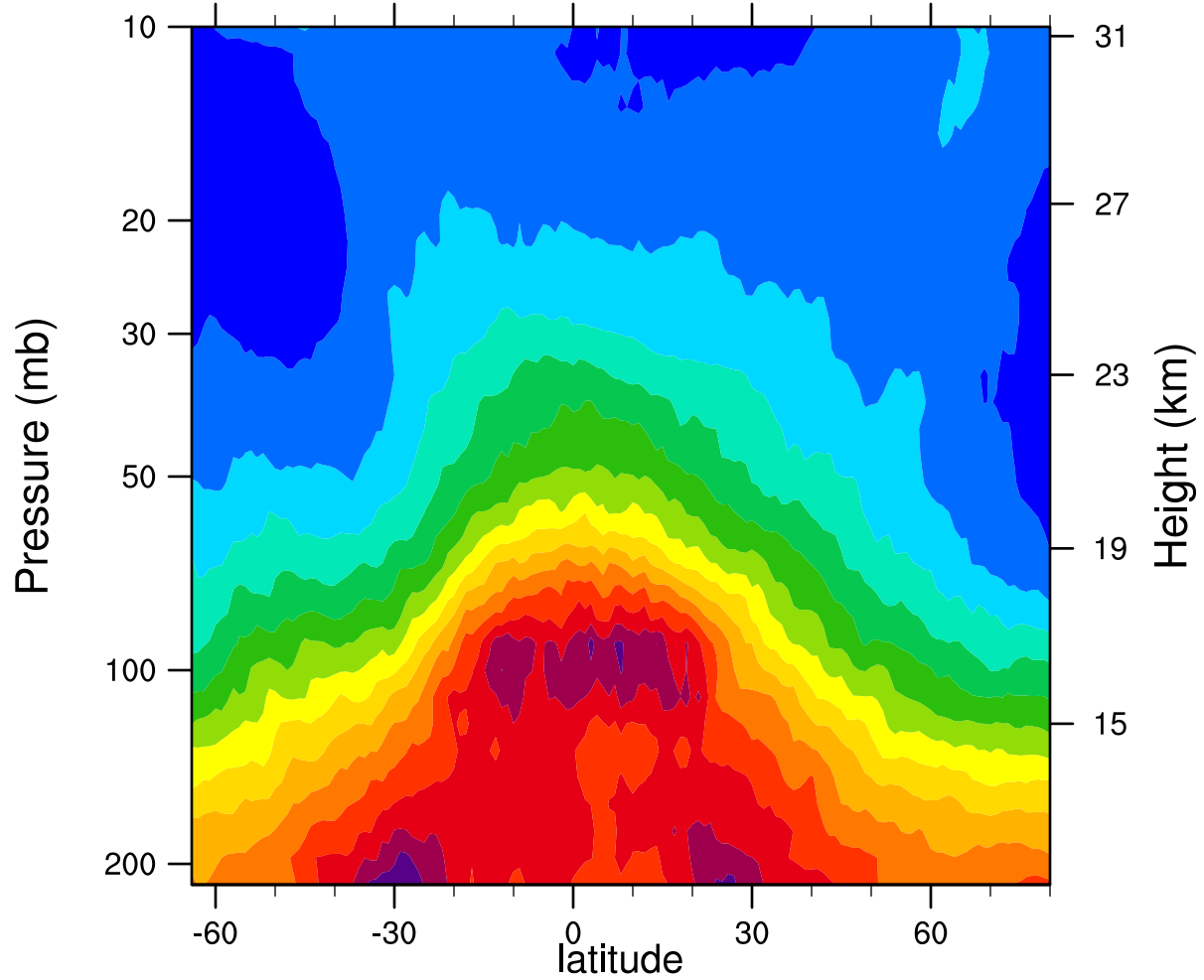
2005d313 12.1MicronExtinction_Combined (km -1 )
