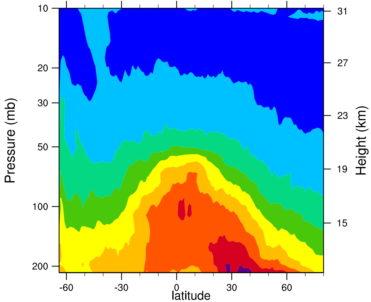
2006d197 12.1MicronExtinction_Combined (km -1 )
