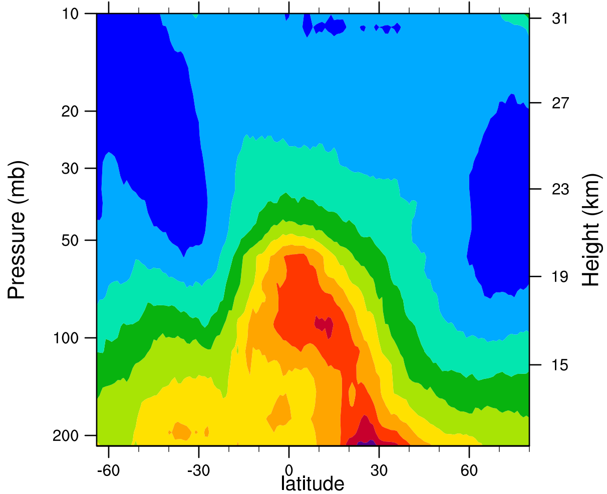
2005d119 12.1MicronExtinction_Combined ( \text{km}^{-1} )
