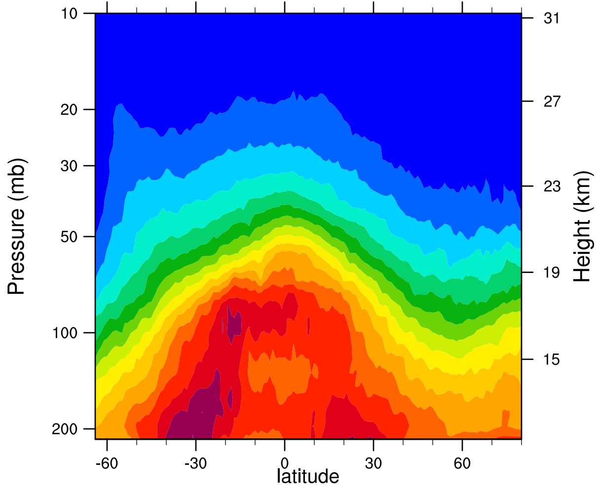
2006d365 12.1MicronExtinction_Combined (km -1 )
