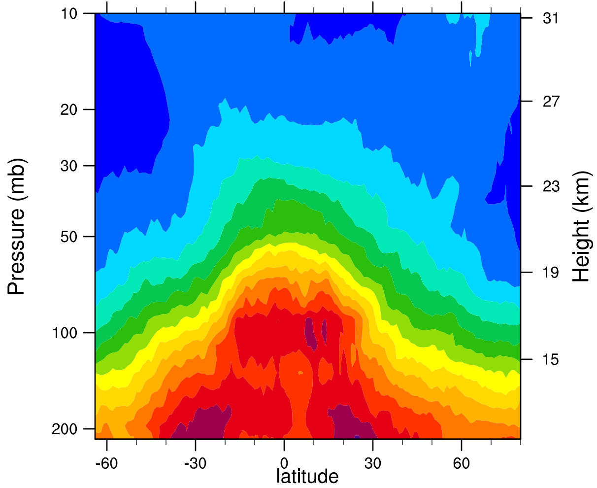
2005d327 12.1MicronExtinction_Combined (km -1 )
