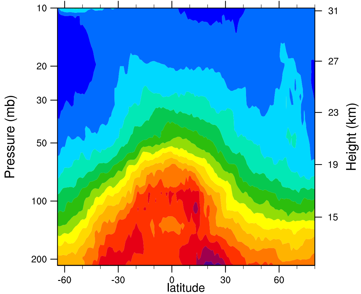
2006d004 12.1MicronExtinction_Combined ( \text{km}^{-1} )
