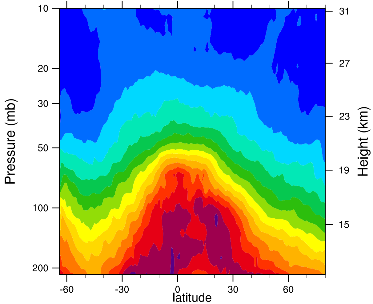
2006d265 12.1MicronExtinction_Combined (km -1 )
