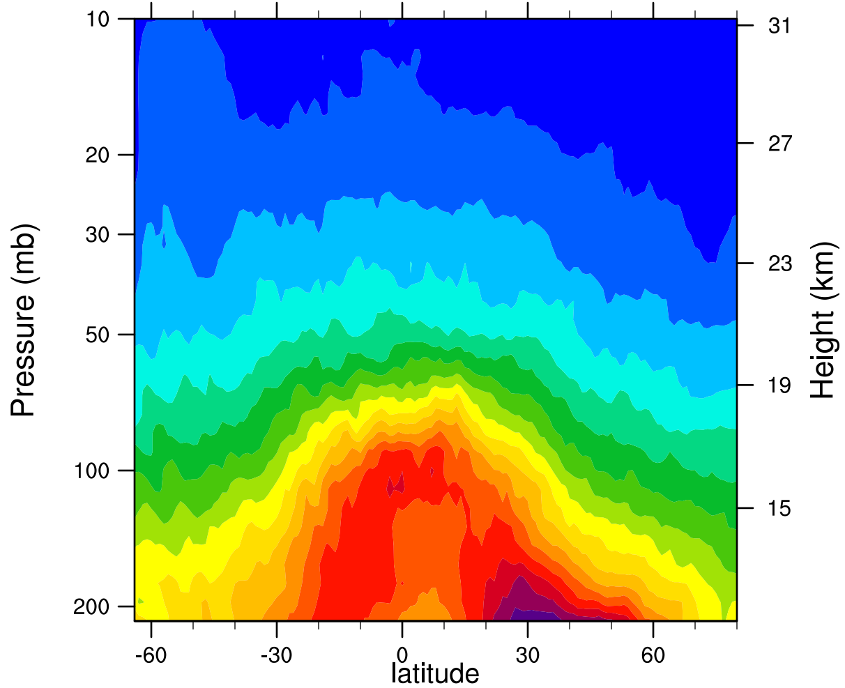
2006d152 12.1MicronExtinction_Combined (km -1 )
