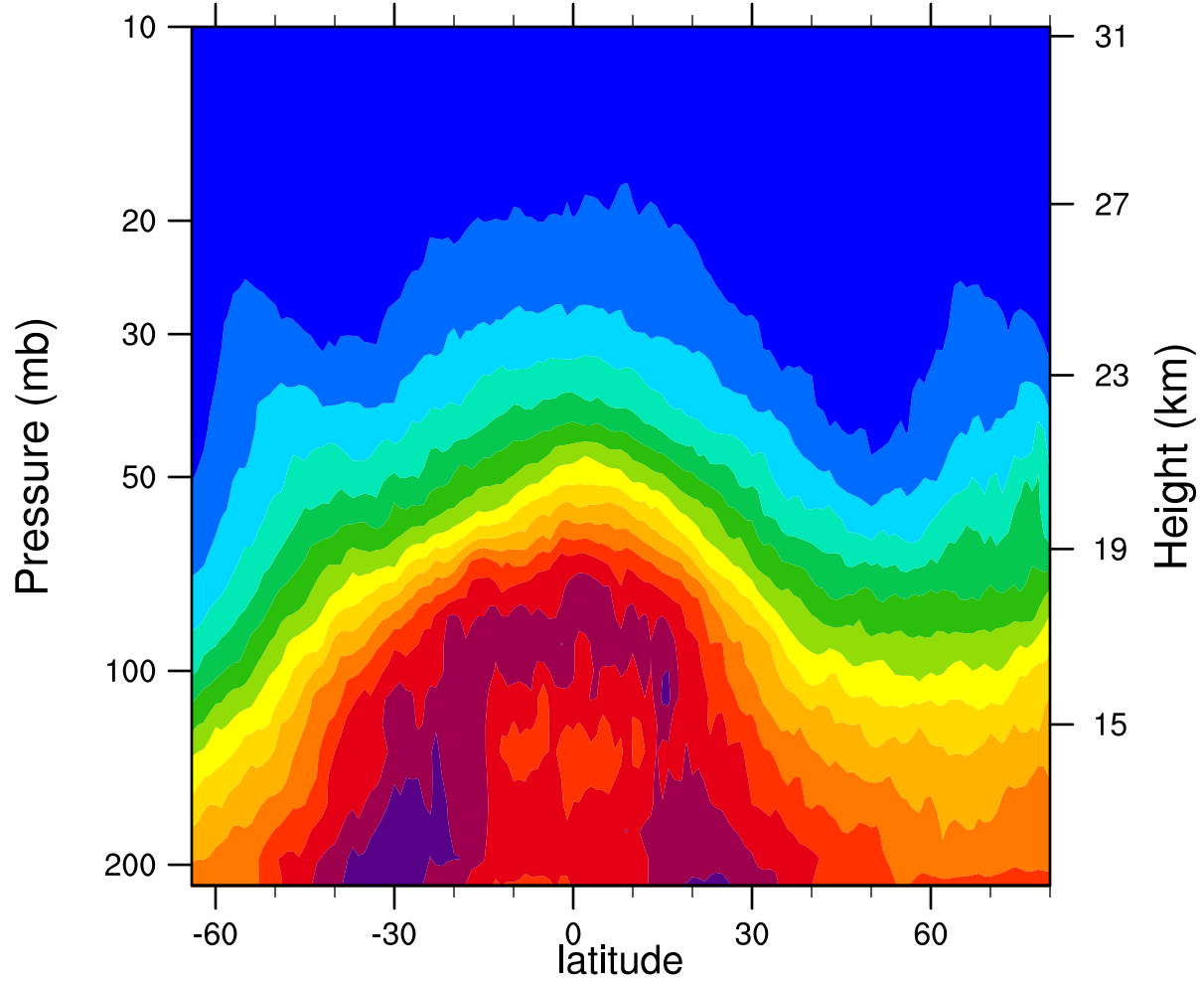
2006d357 12.1MicronExtinction_Combined (km -1 )
