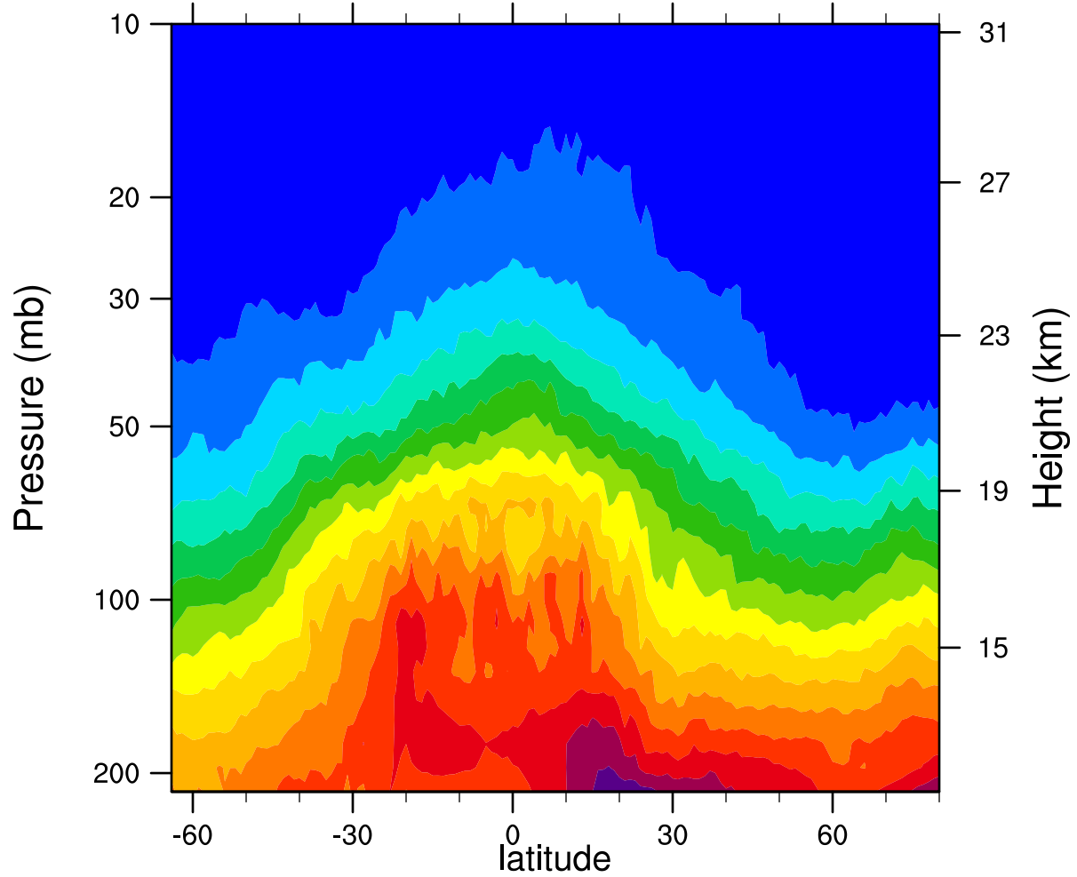
2007d076 12.1MicronExtinction_Combined (km -1 )
