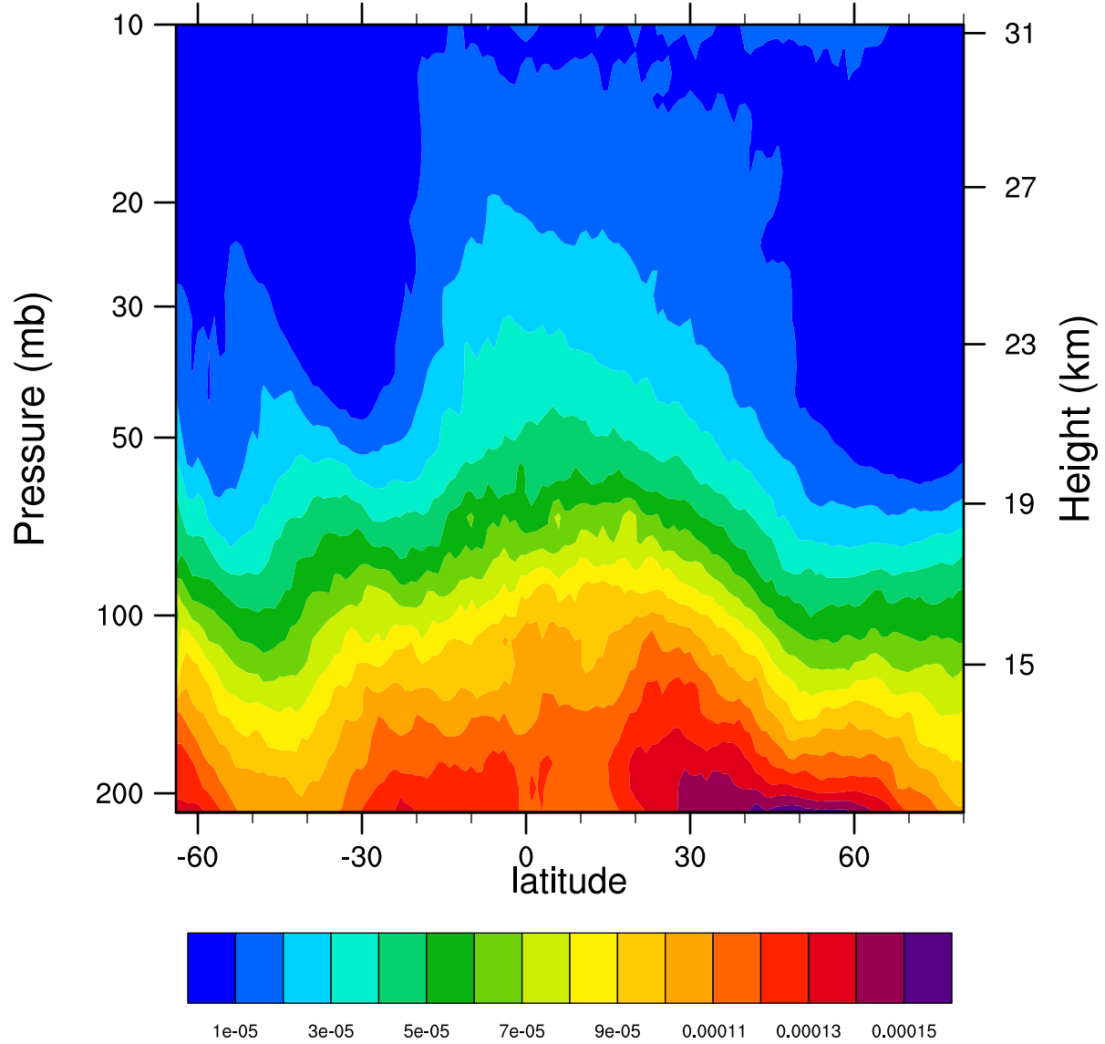
2007d232 12.1MicronExtinction_Combined (km -1 )
