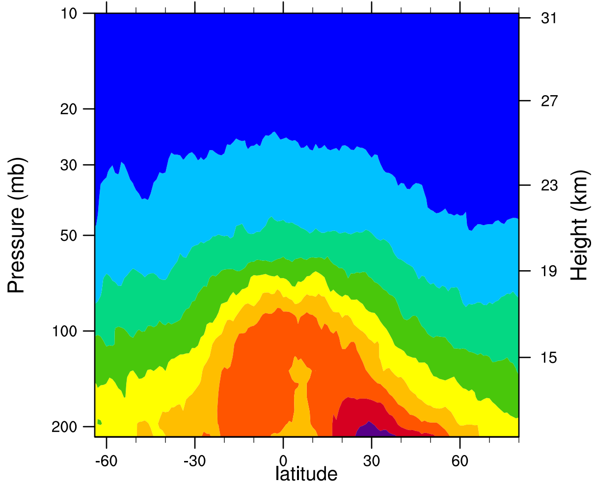
2006d144 12.1MicronExtinction_Combined (km -1 )
