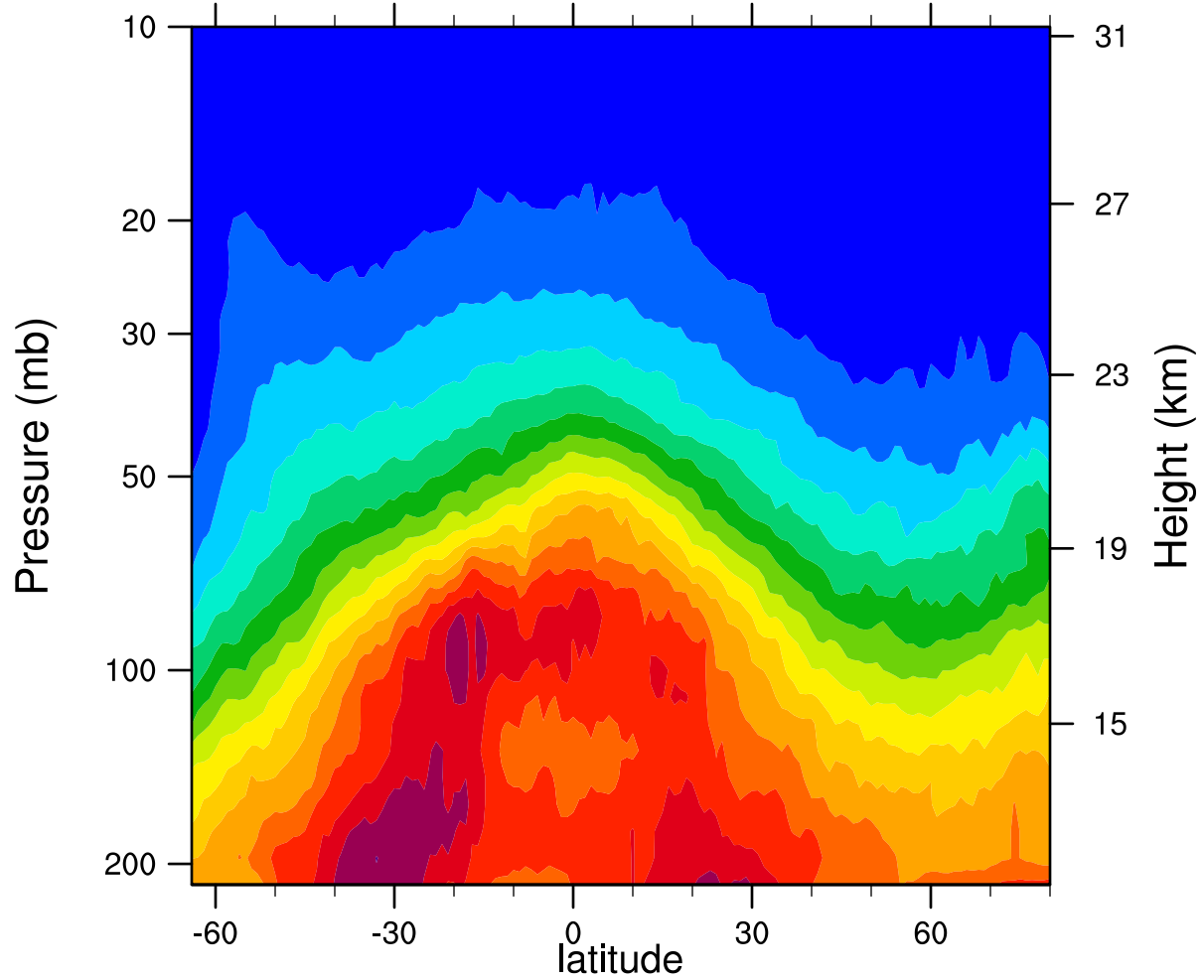
2006d364 12.1MicronExtinction_Combined (km -1 )
