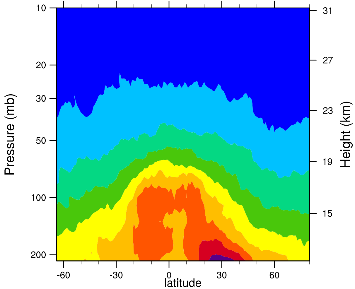
2006d125 12.1MicronExtinction_Combined (km -1 )
