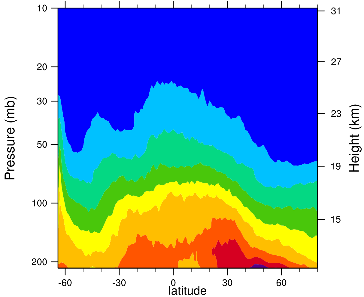
2007d211 12.1MicronExtinction_Combined (km -1 )
