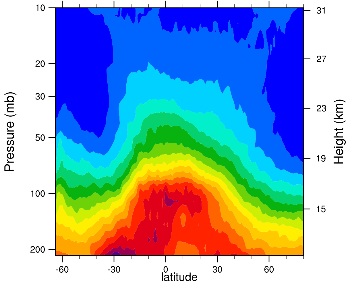
2005d276 12.1MicronExtinction_Combined (km -1 )
