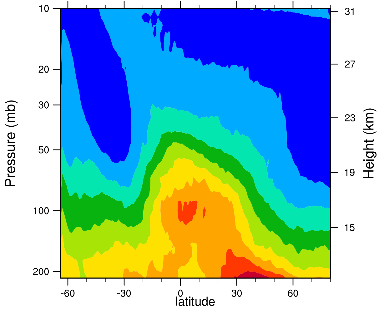
2005d169 12.1MicronExtinction_Combined (km -1 )
