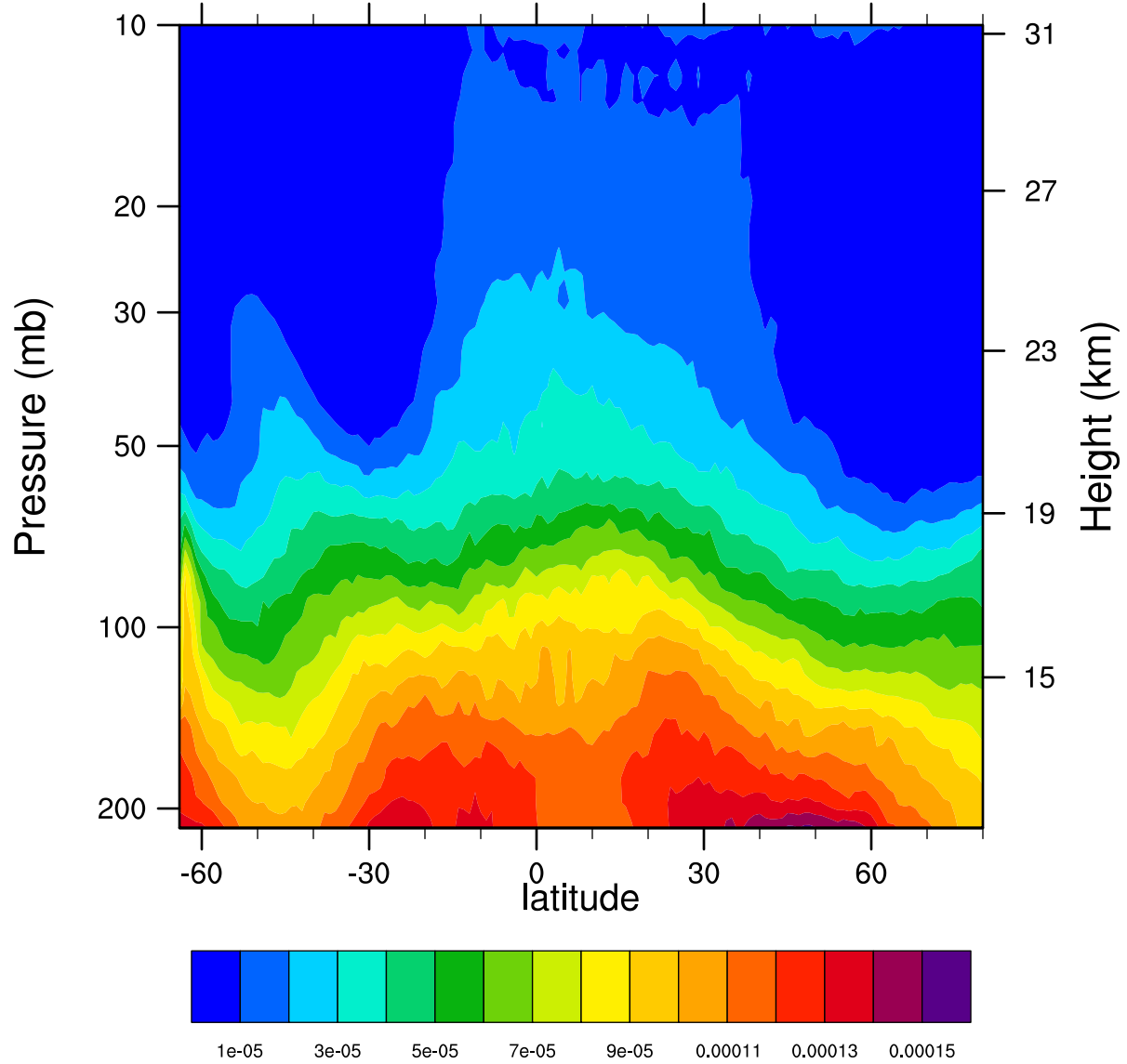
2007d248 12.1MicronExtinction_Combined (km -1 )
