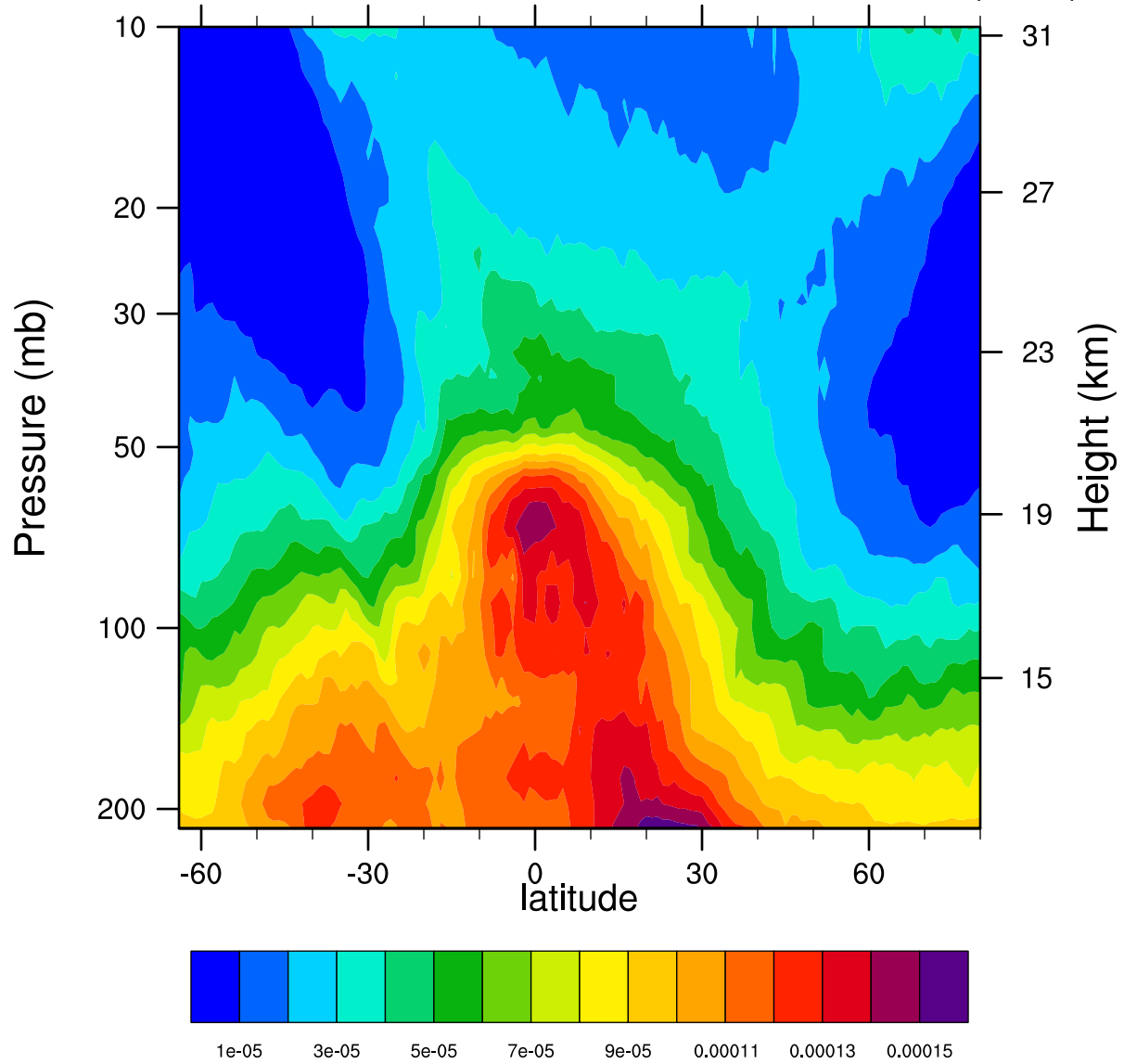
2005d086 12.1MicronExtinction_Combined (km -1 )
