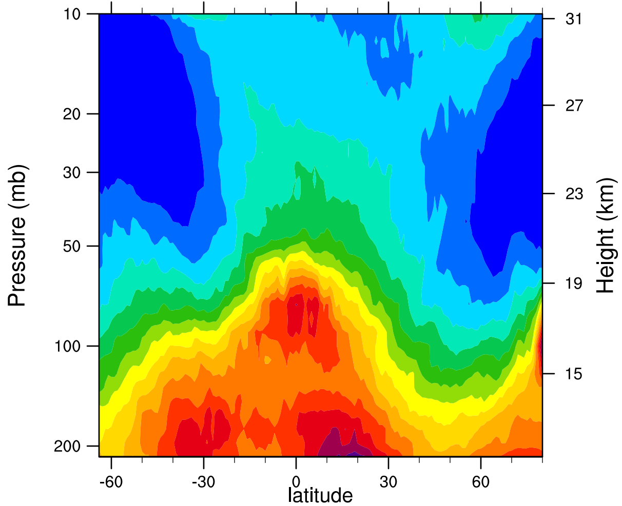
2005d042 12.1MicronExtinction_Combined (km -1 )
