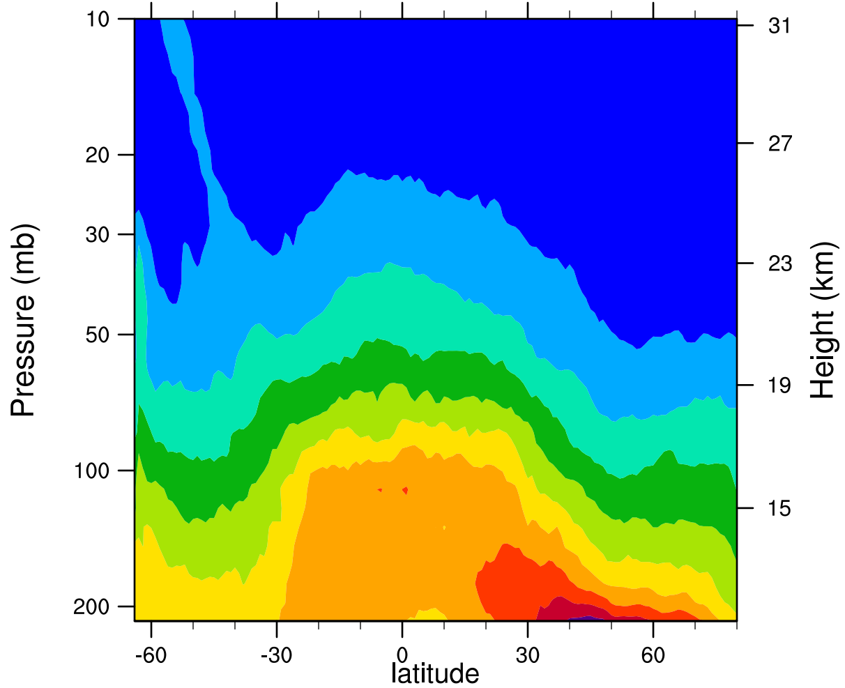
2007d177 12.1MicronExtinction_Combined (km -1 )
