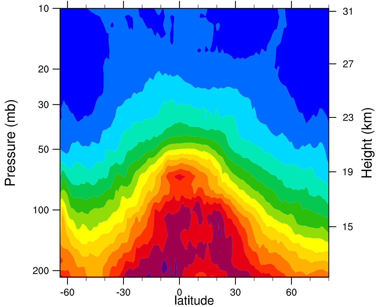
2006d273 12.1MicronExtinction_Combined (km -1 )
