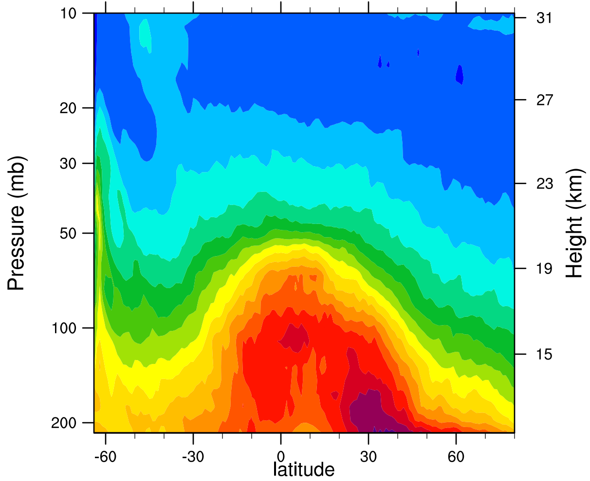
2006d204 12.1MicronExtinction_Combined (km -1 )
