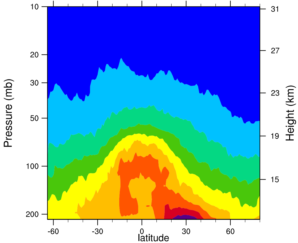
2006d112 12.1MicronExtinction_Combined (km -1 )
