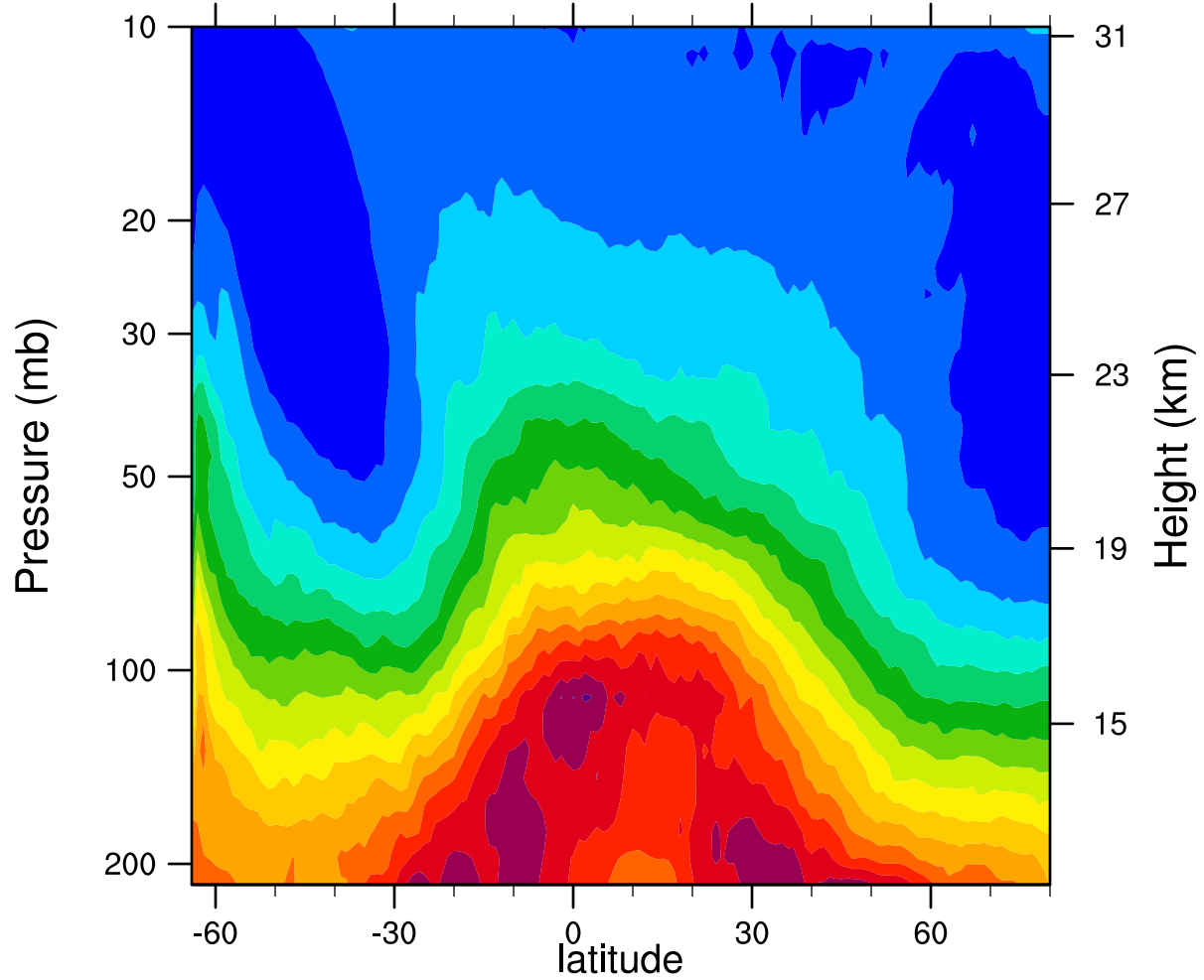
2005d237 12.1MicronExtinction_Combined (km -1 )
