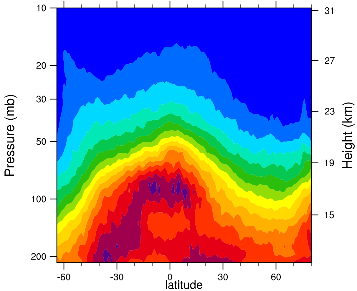
2007d011 12.1MicronExtinction_Combined (km -1 )
