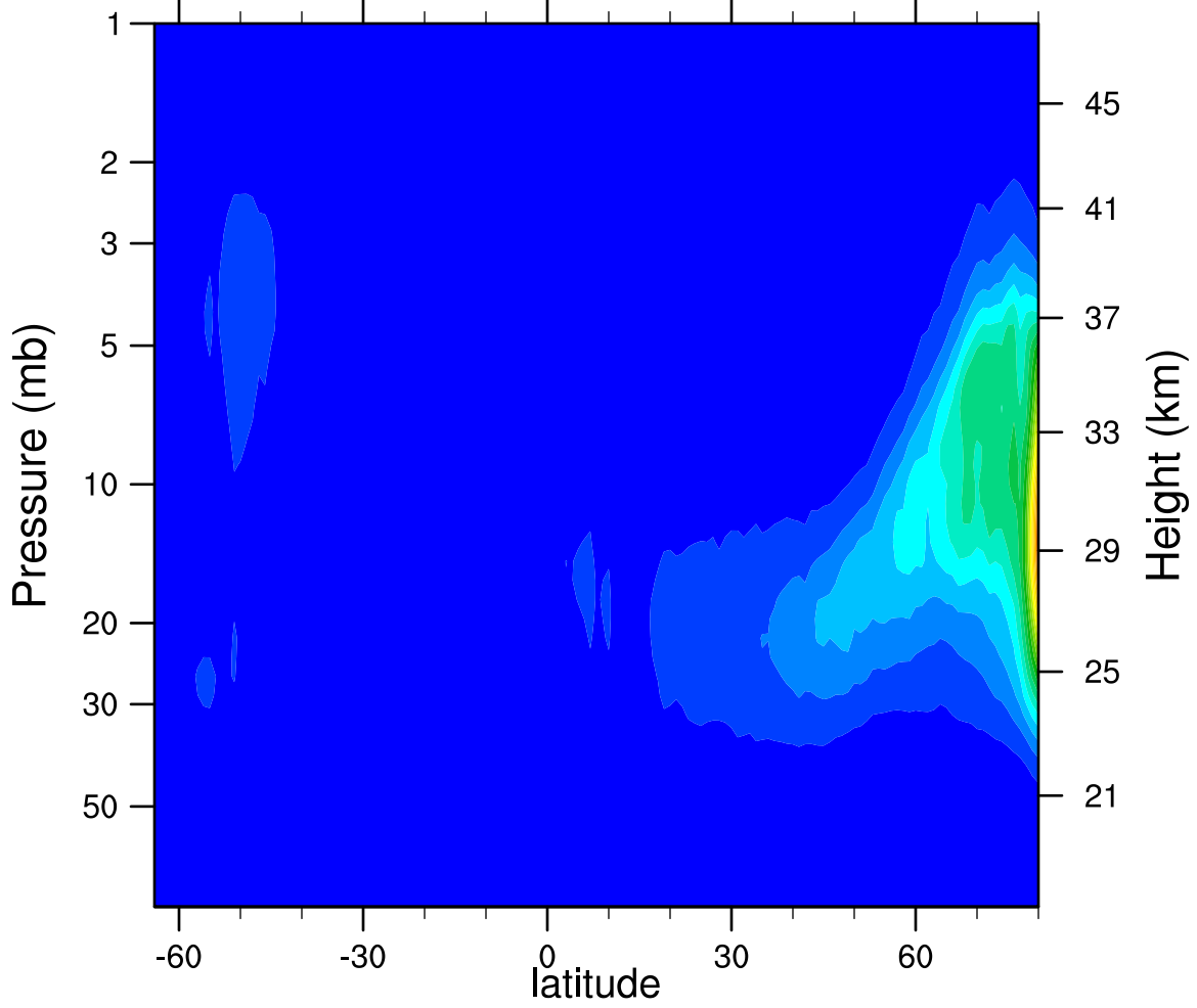
2007d059 N2O5_Ascending (ppbv)
