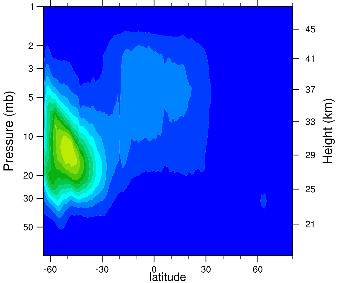
2007d226 N2O5_Ascending (ppbv)
