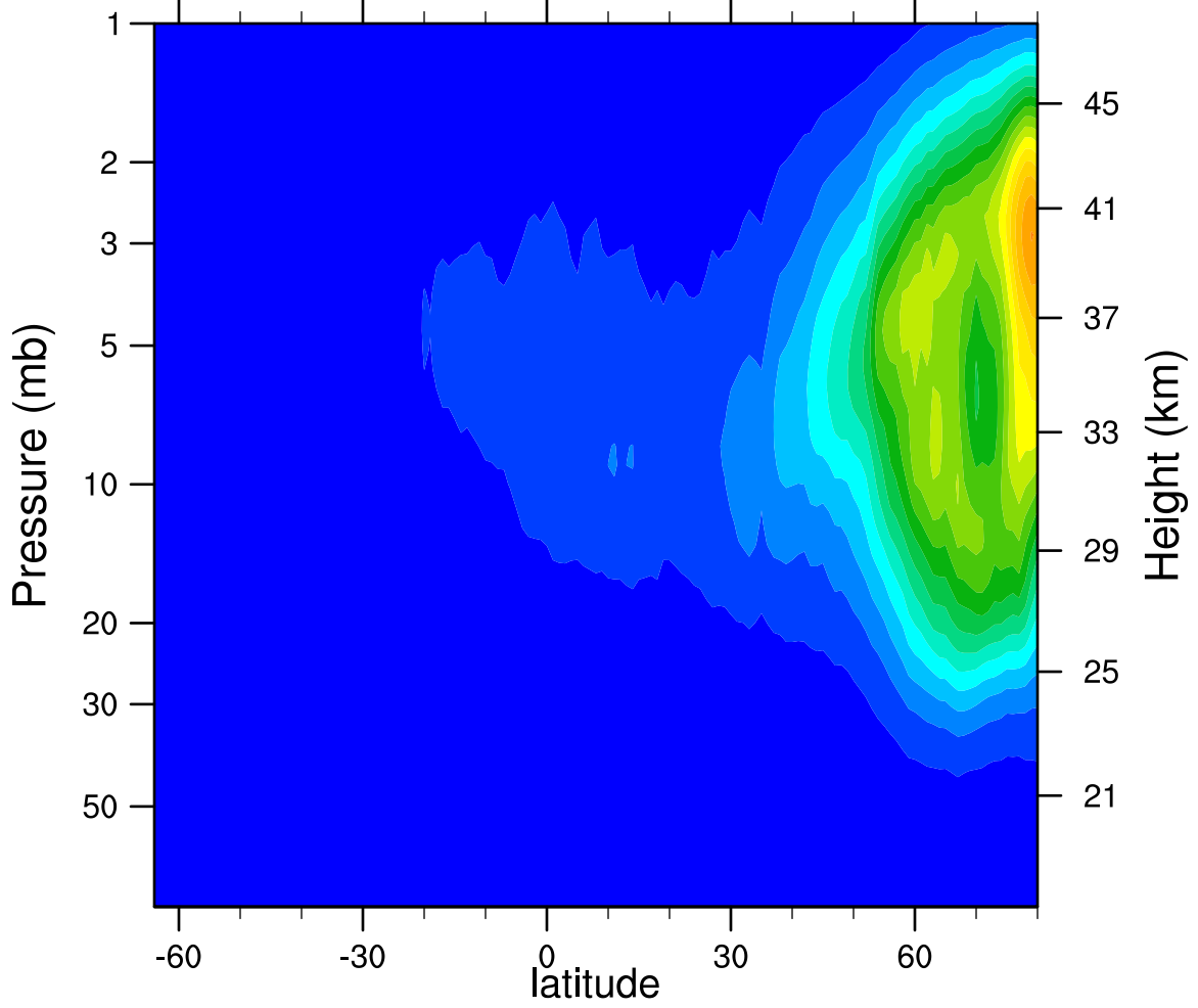
2005d324 N2O5_Ascending (ppbv)
