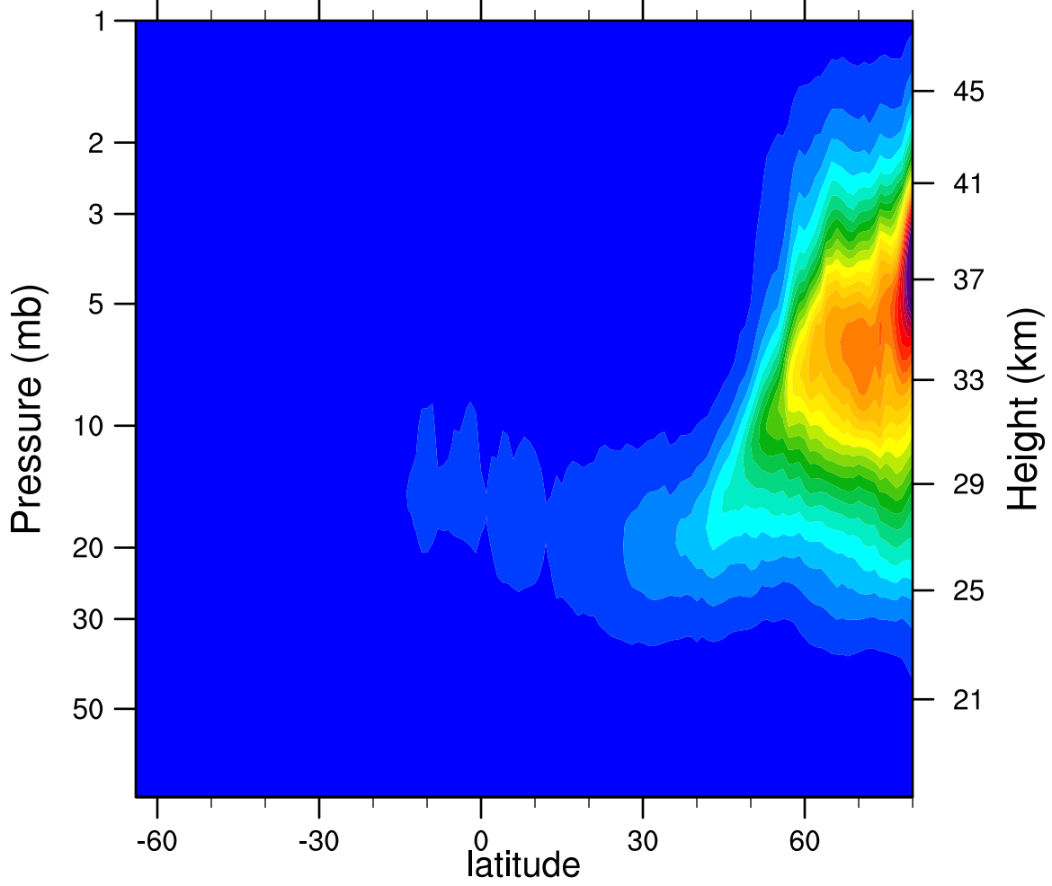
2007d033 N2O5_Ascending (ppbv)
