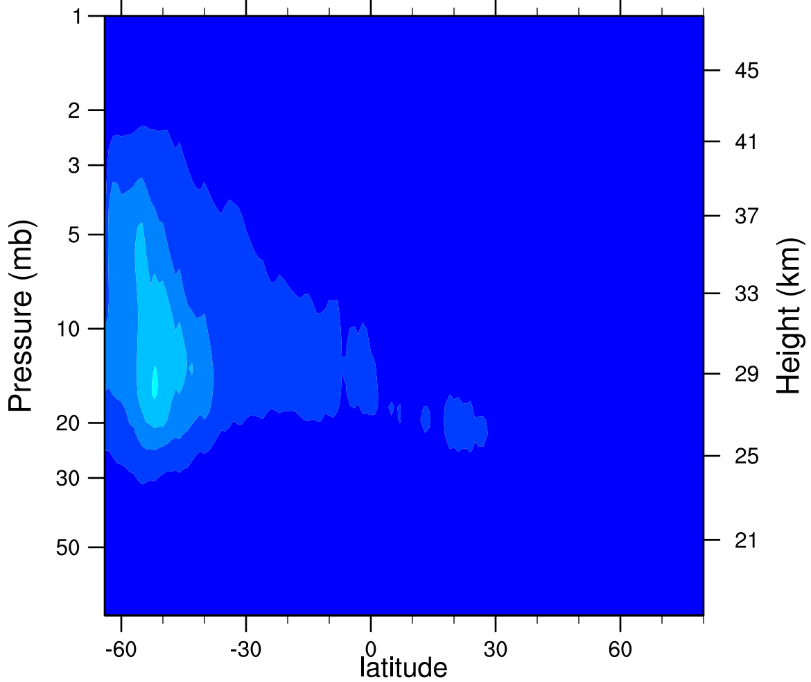
2007d188 N2O5_Ascending (ppbv)
