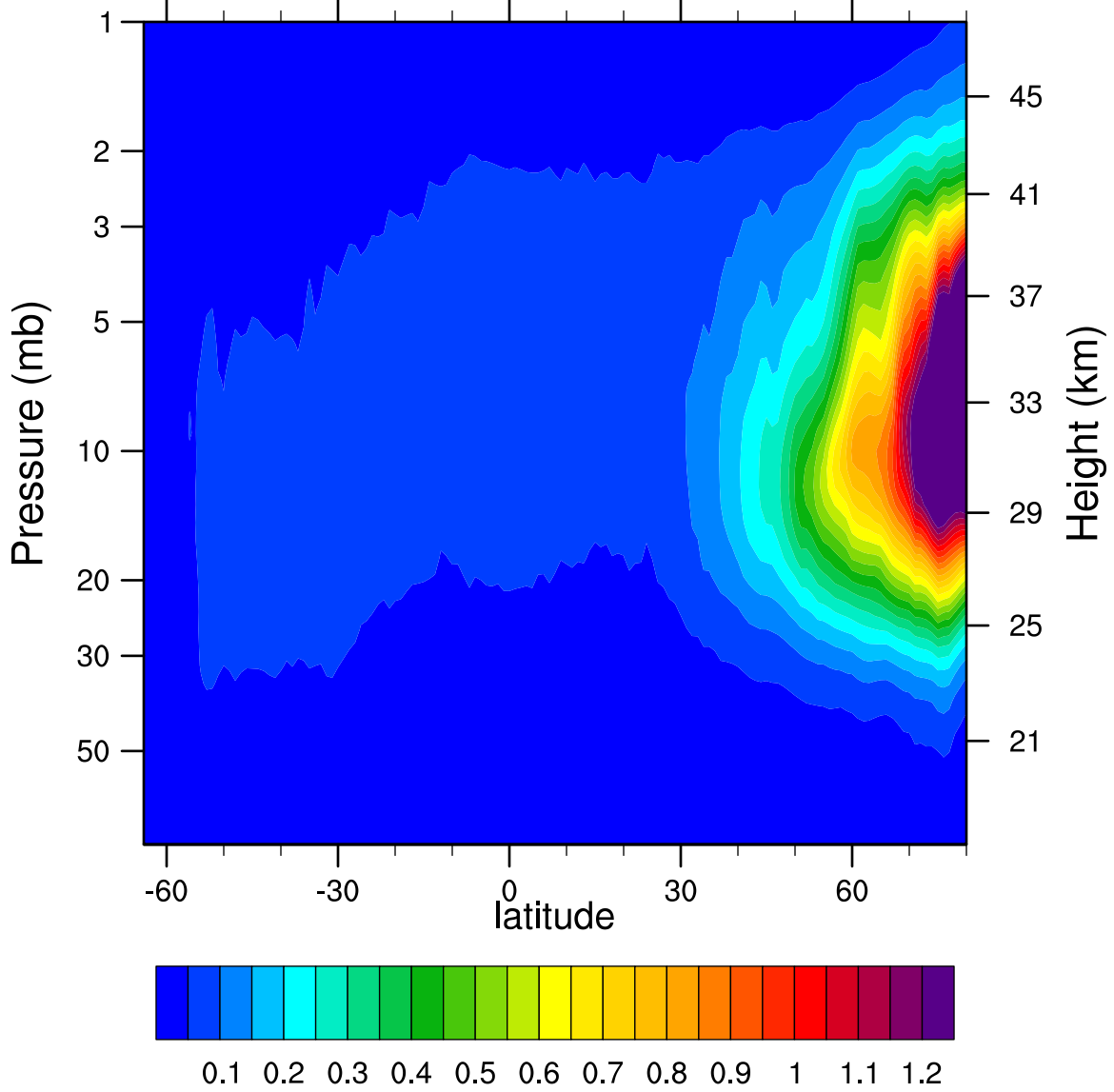
2007d347 N2O5_Ascending (ppbv)
