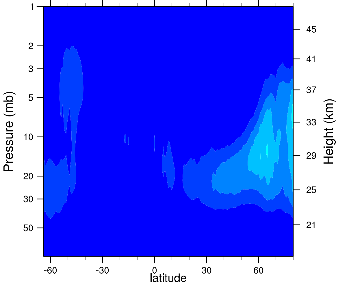
2007d072 N2O5_Ascending (ppbv)
