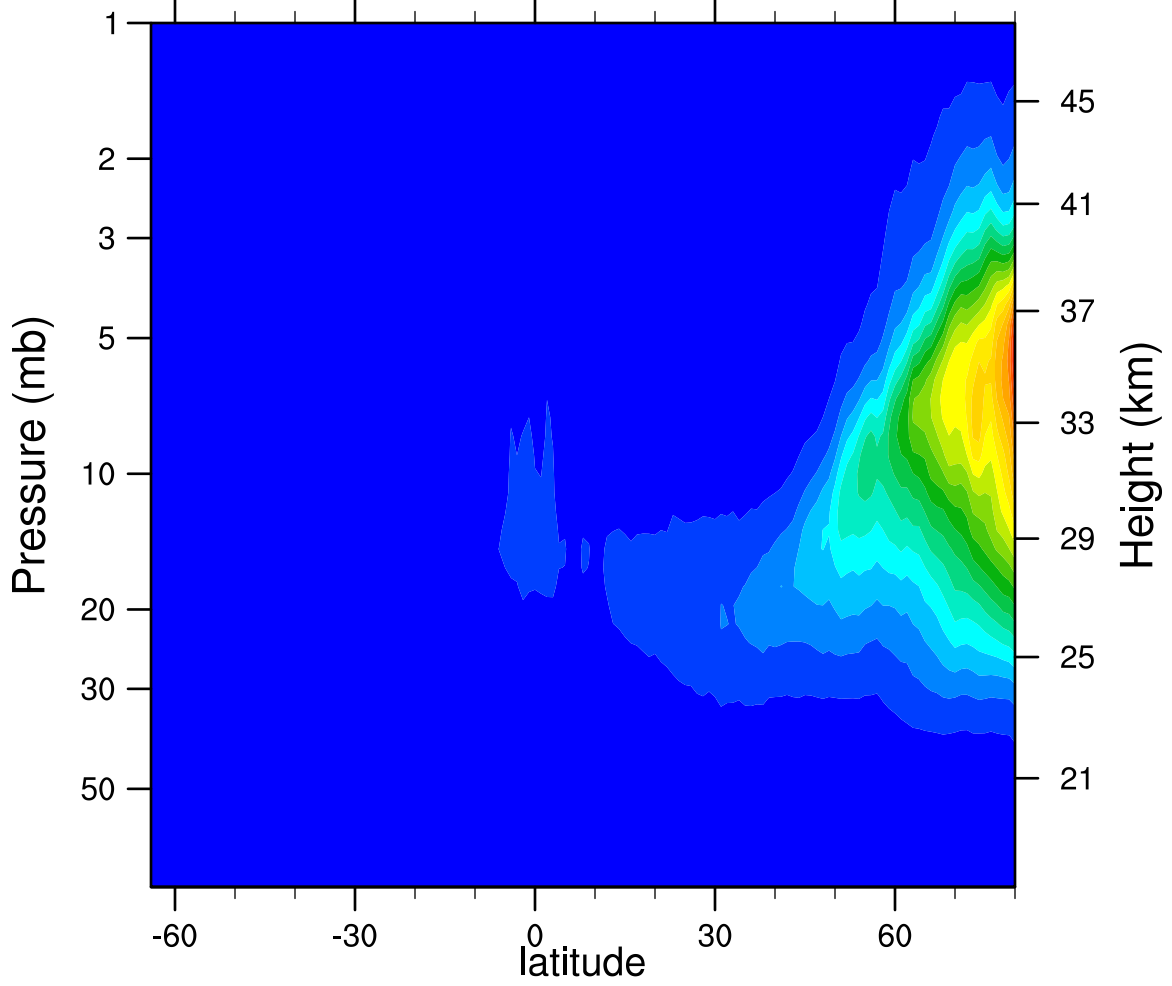
2007d040 N2O5_Ascending (ppbv)
