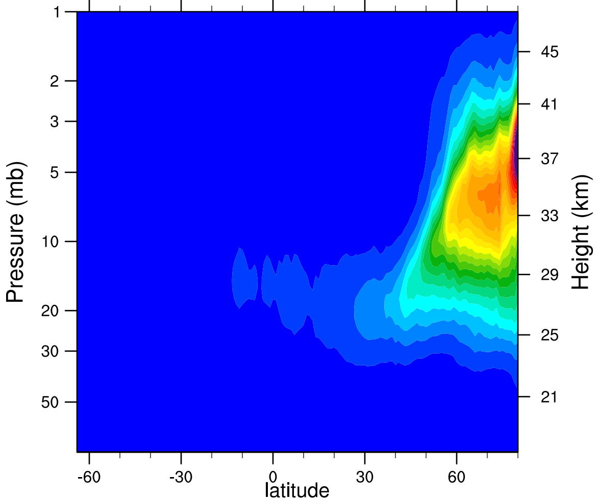
2007d032 N2O5_Ascending (ppbv)
