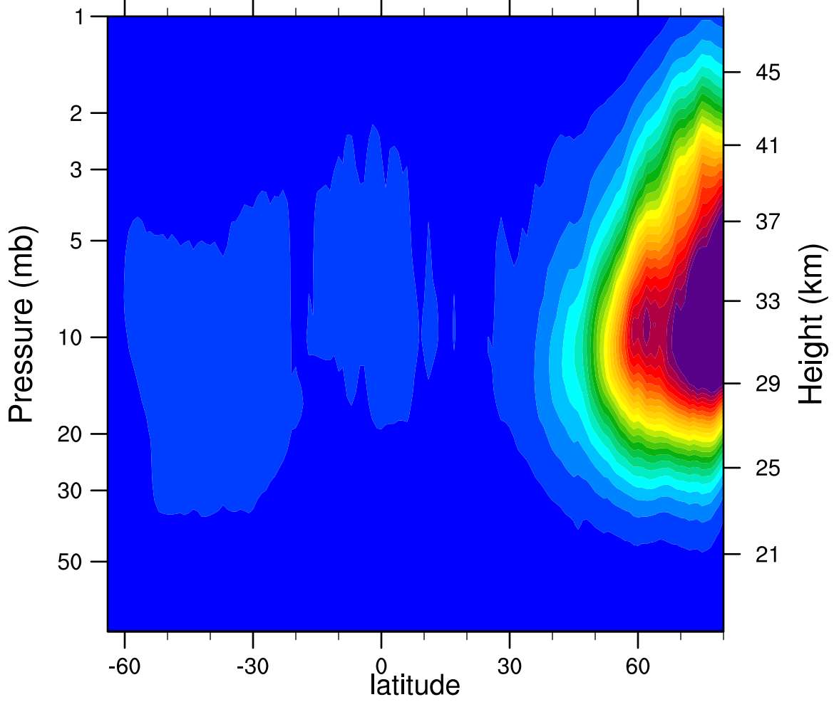
2007d361 N2O5_Ascending (ppbv)
