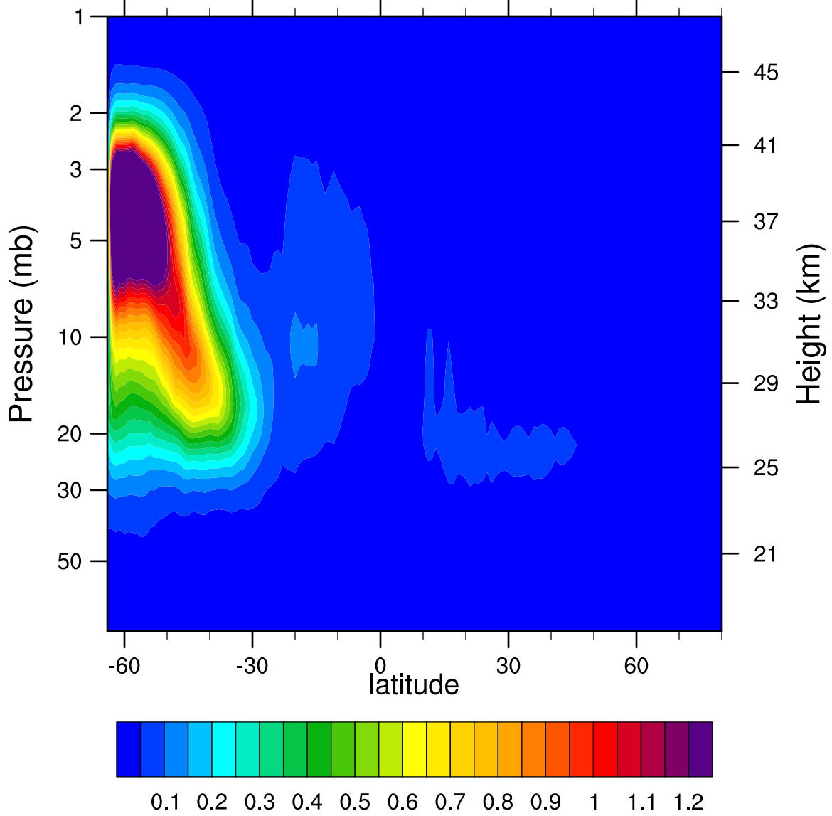
2007d159 N2O5_Ascending (ppbv)
