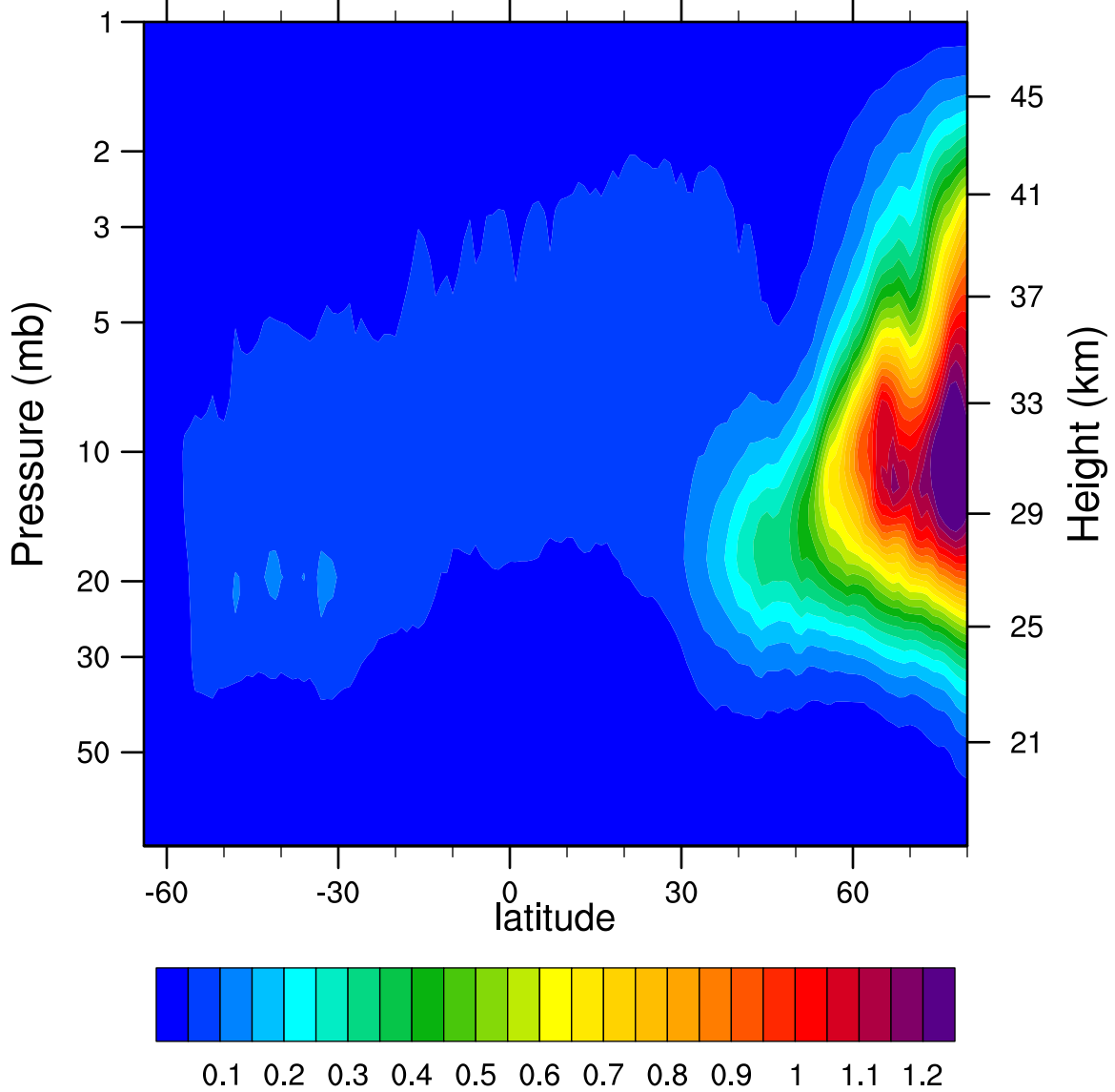
2007d322 N2O5_Ascending (ppbv)
