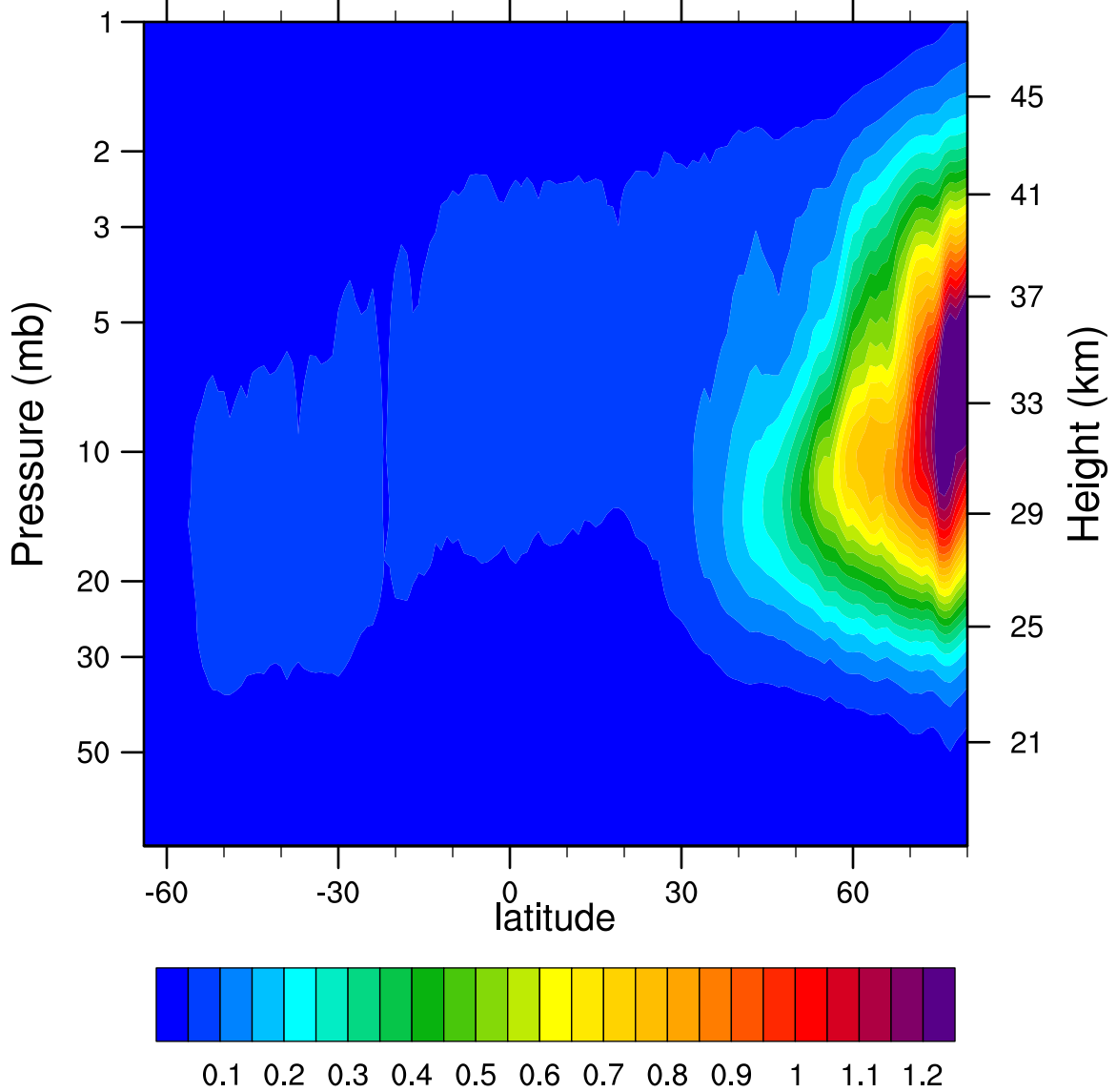
2007d341 N2O5_Ascending (ppbv)
