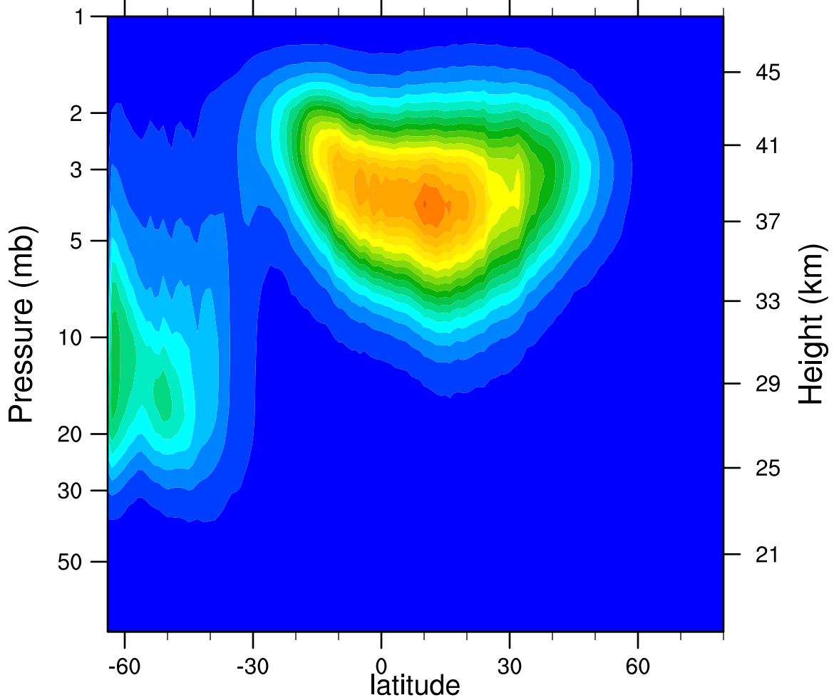
2005d123 N2O5_Ascending (ppbv)
