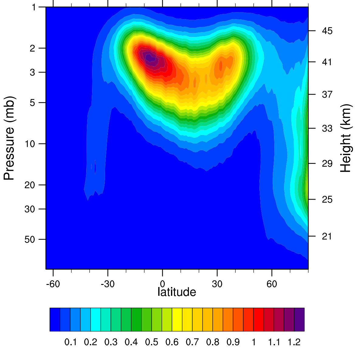
2005d057 N2O5_Ascending (ppbv)
