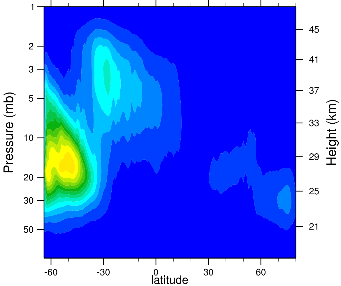
2007d105 N2O5_Ascending (ppbv)
