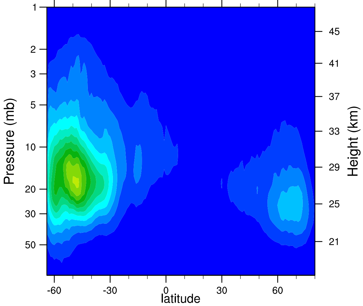
2007d246 N2O5_Ascending (ppbv)
