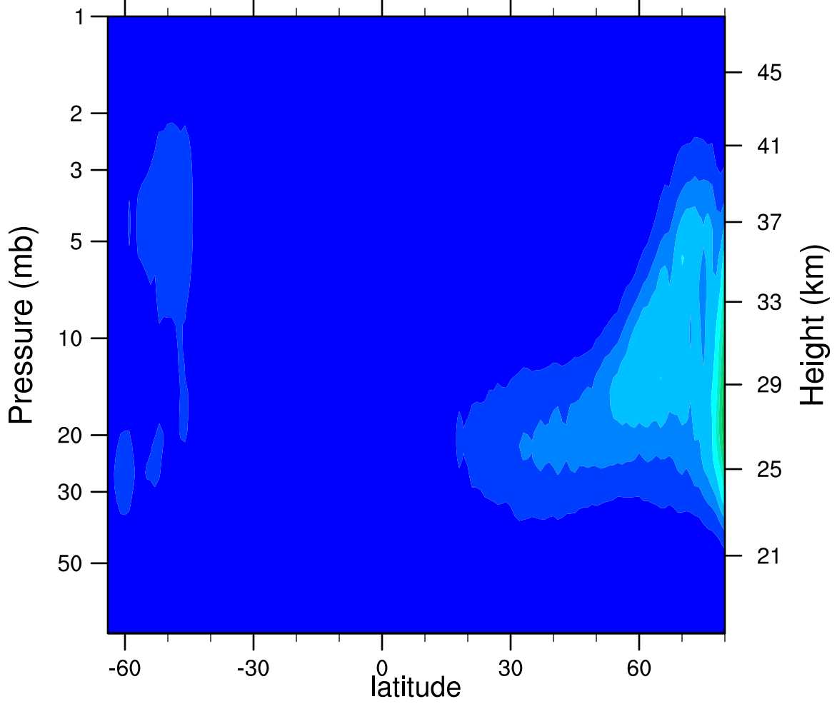
2007d065 N2O5_Ascending (ppbv)
