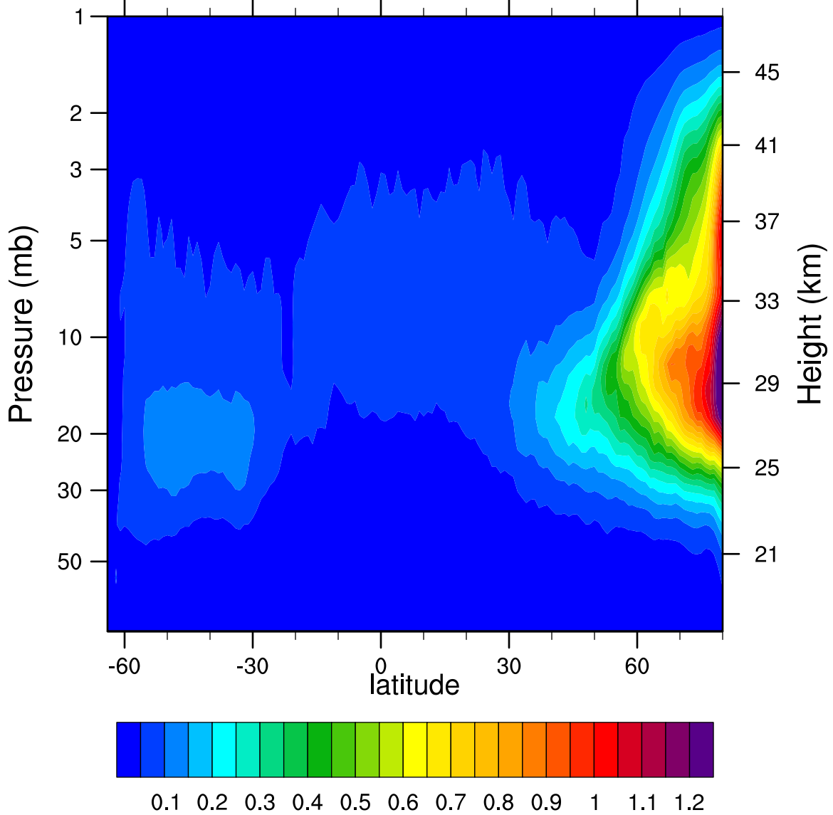
2007d312 N2O5_Ascending (ppbv)
