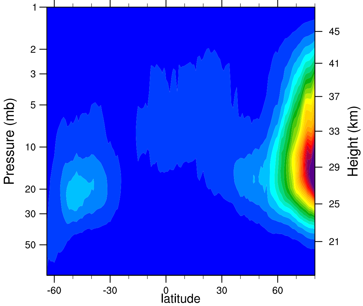
2007d300 N2O5_Ascending (ppbv)
