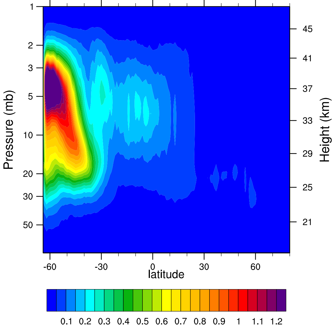
2007d140 N2O5_Ascending (ppbv)
