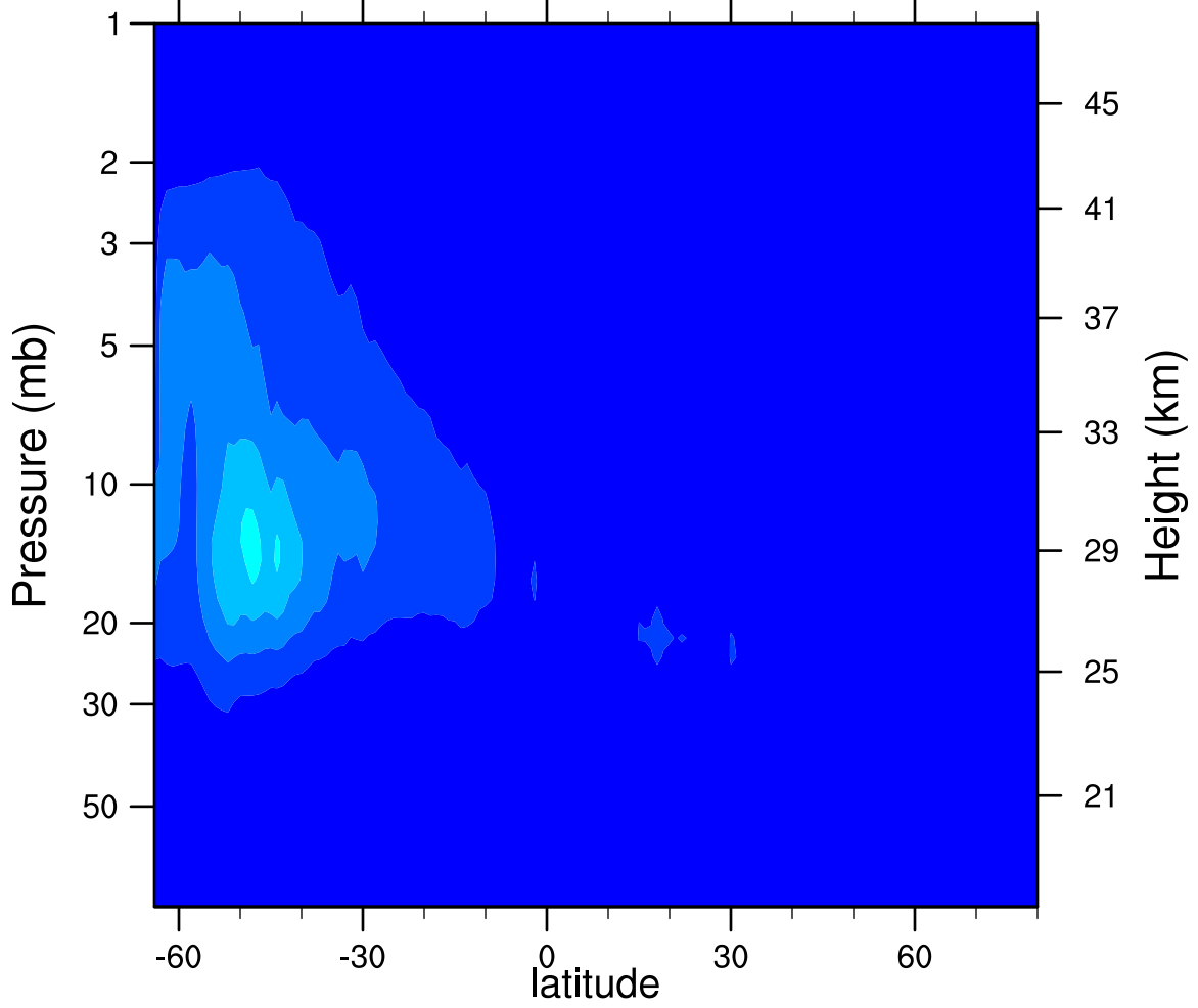
2007d181 N2O5_Ascending (ppbv)
