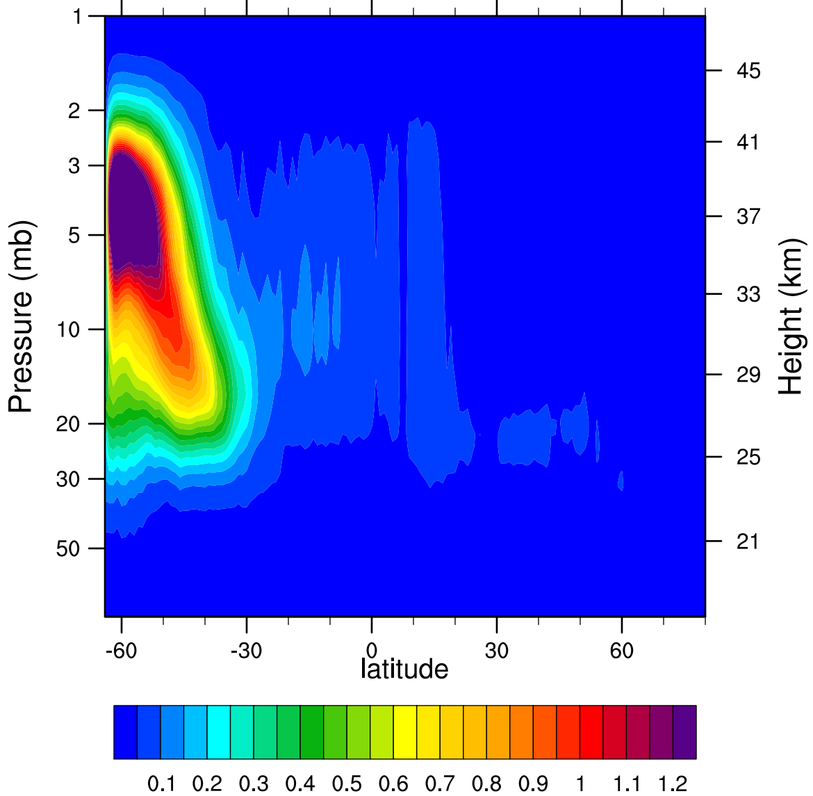
2007d143 N2O5_Ascending (ppbv)
