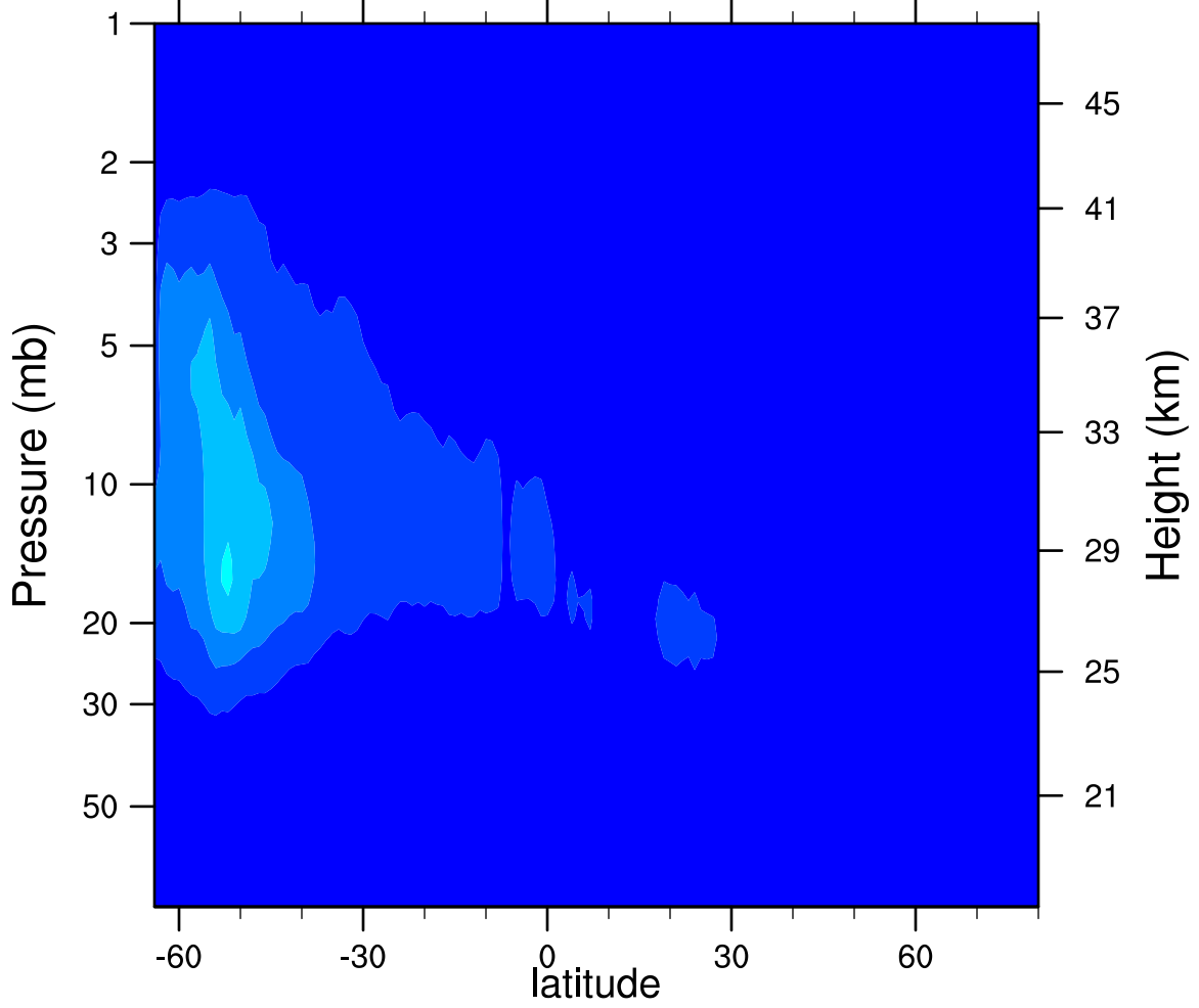
2007d189 N2O5_Ascending (ppbv)
