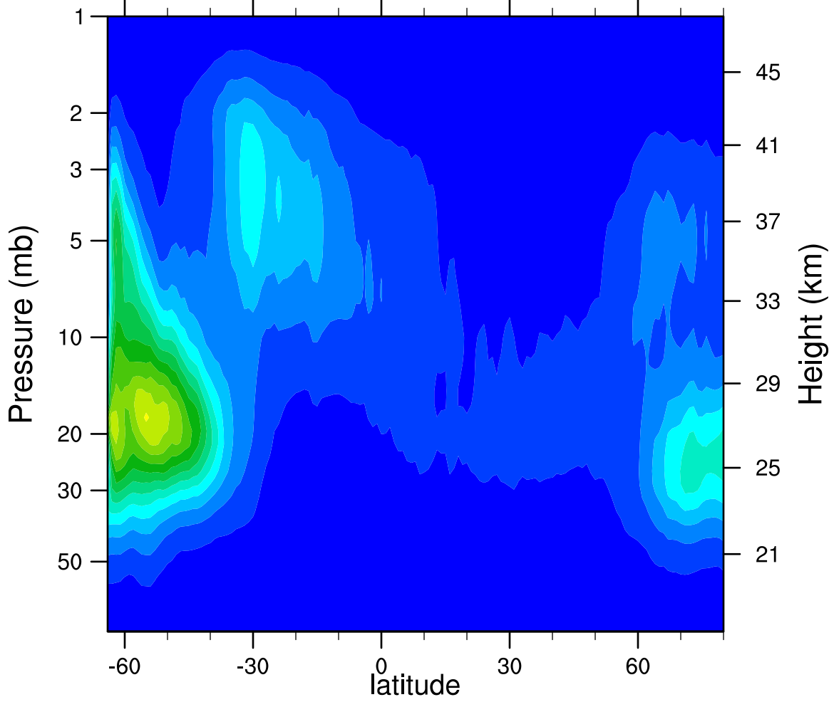
2007d089 N2O5_Ascending (ppbv)
