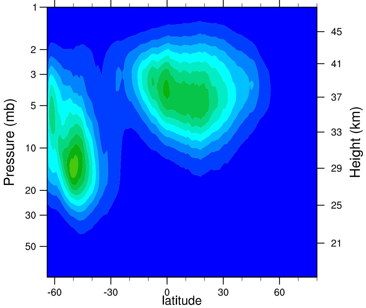
2005d172 N2O5_Ascending (ppbv)
