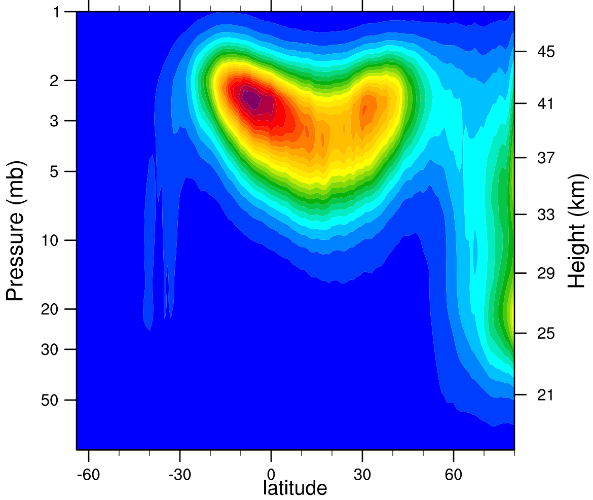
2005d053 N2O5_Ascending (ppbv)
