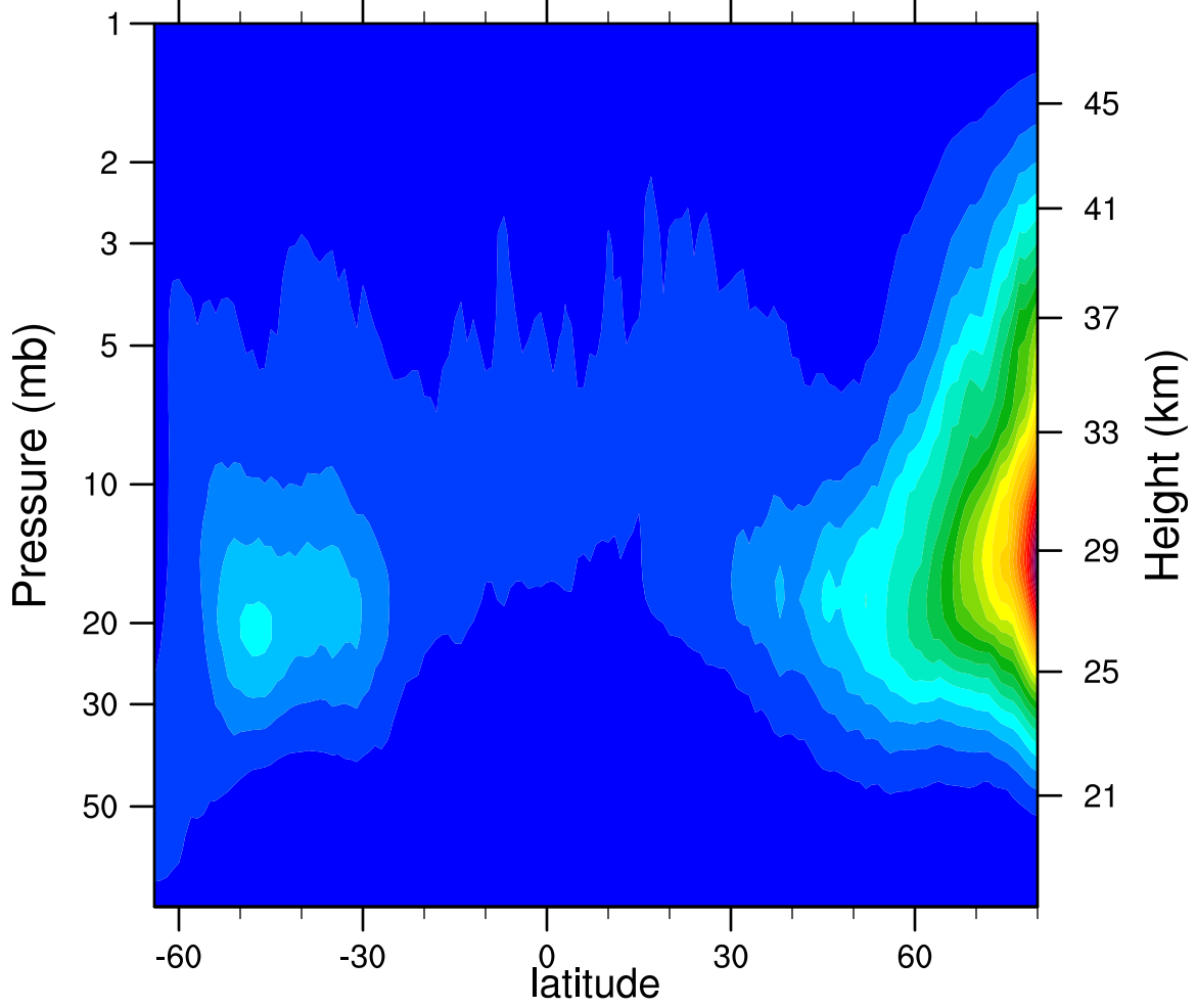
2007d291 N2O5_Ascending (ppbv)
