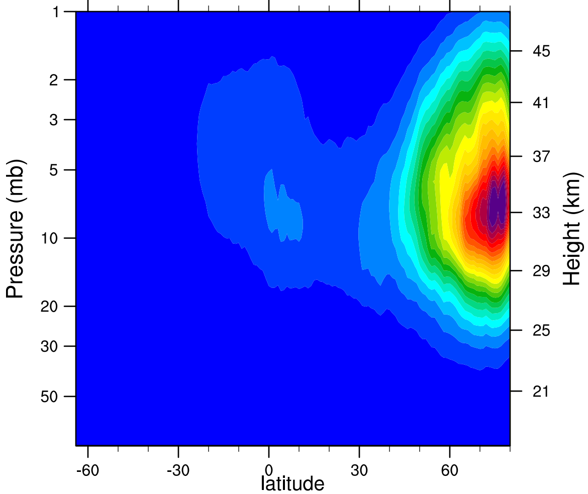
2005d361 N2O5_Ascending (ppbv)
