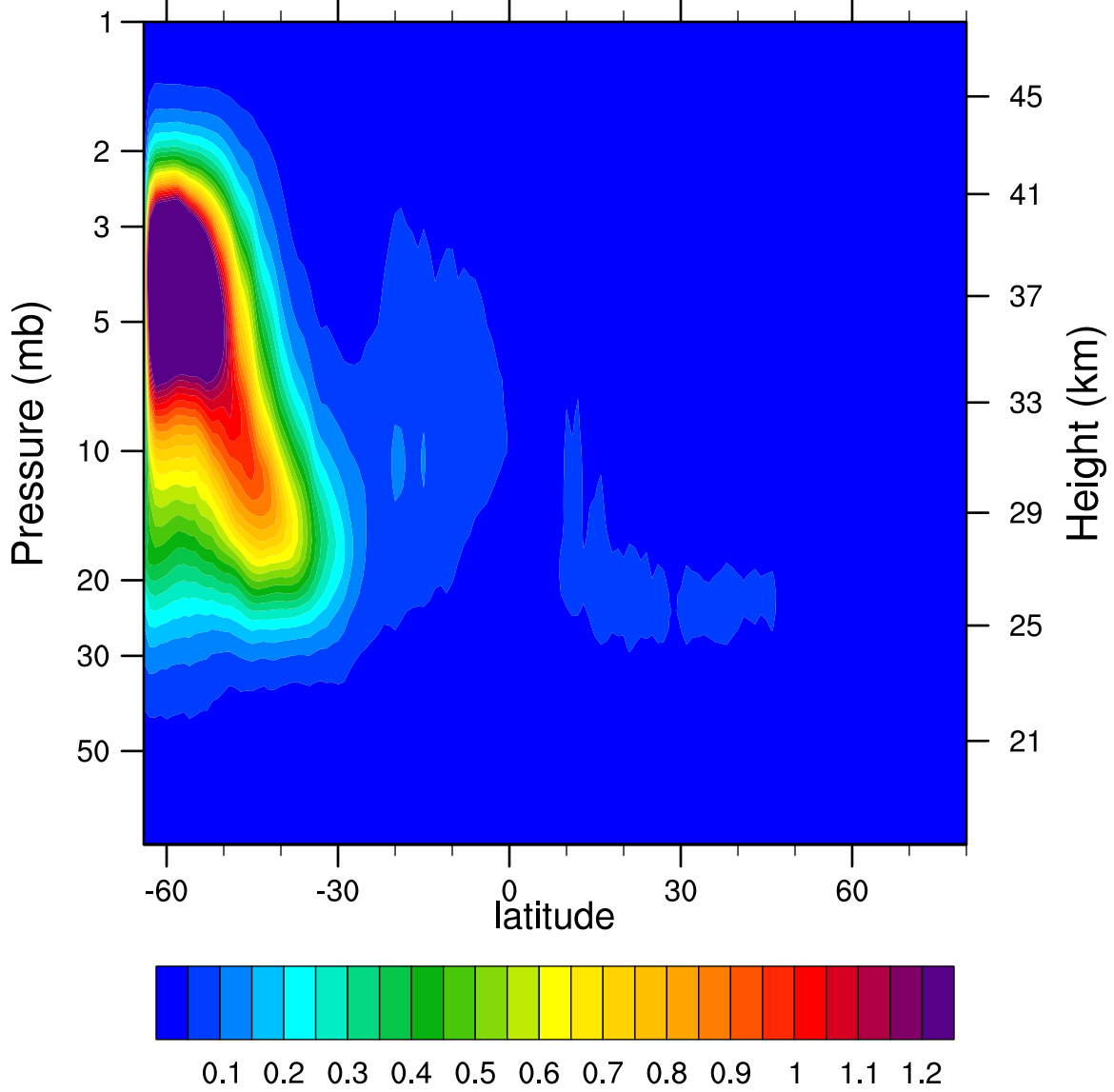
2007d158 N2O5_Ascending (ppbv)
