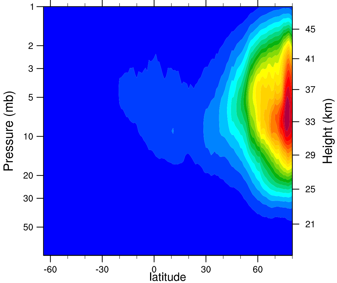
2005d328 N2O5_Ascending (ppbv)
