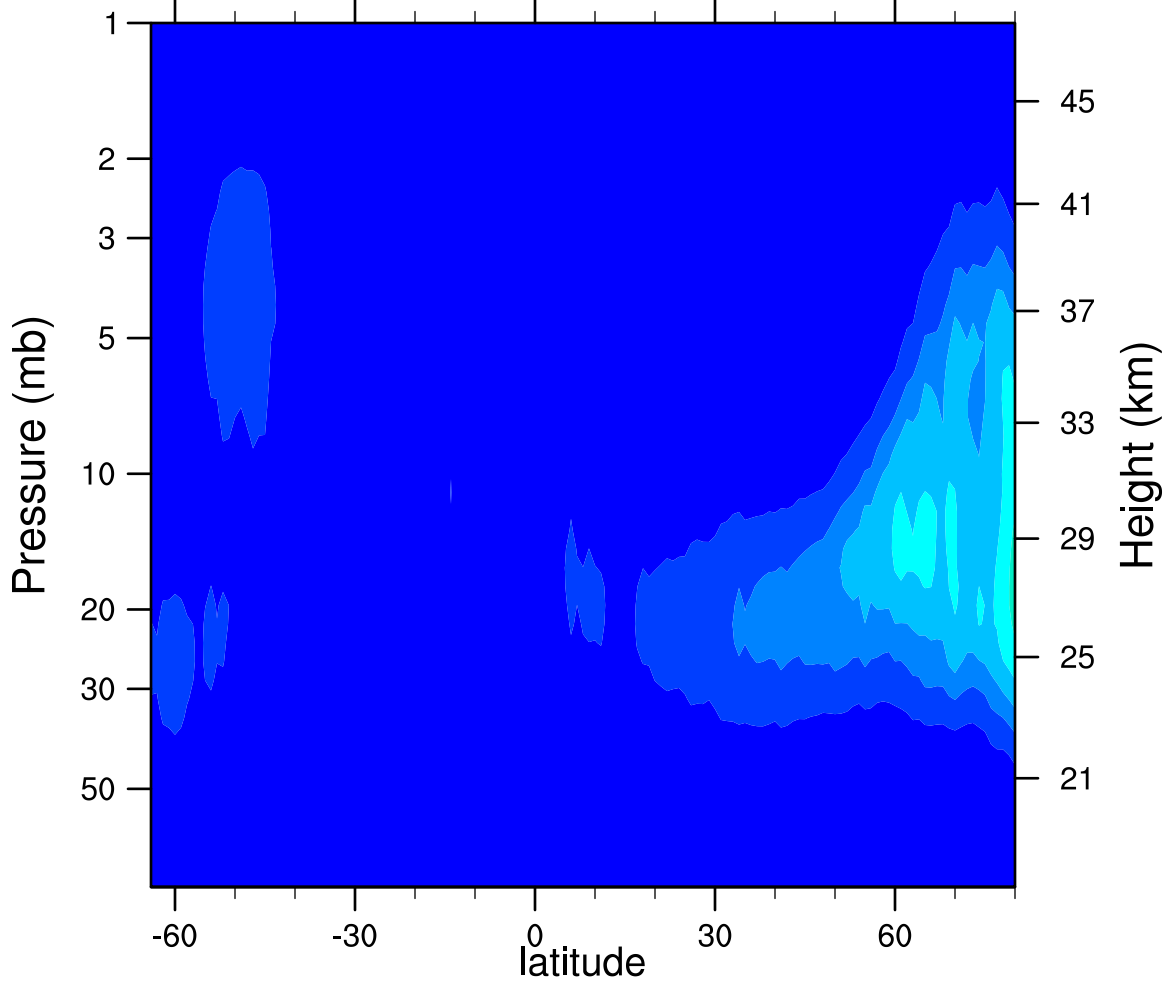
2007d068 N2O5_Ascending (ppbv)
