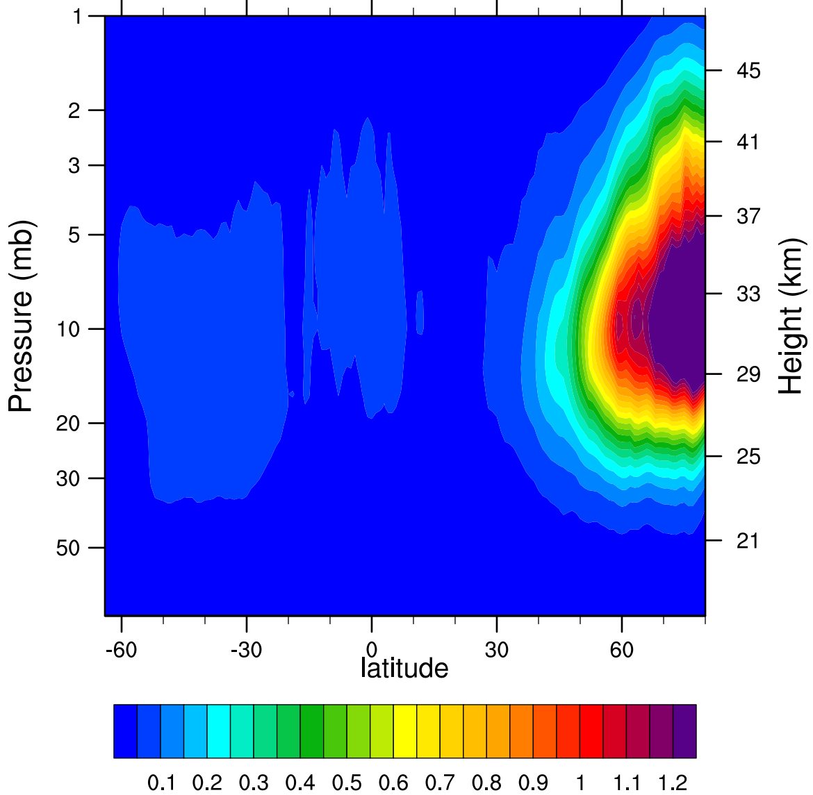
2007d363 N2O5_Ascending (ppbv)
