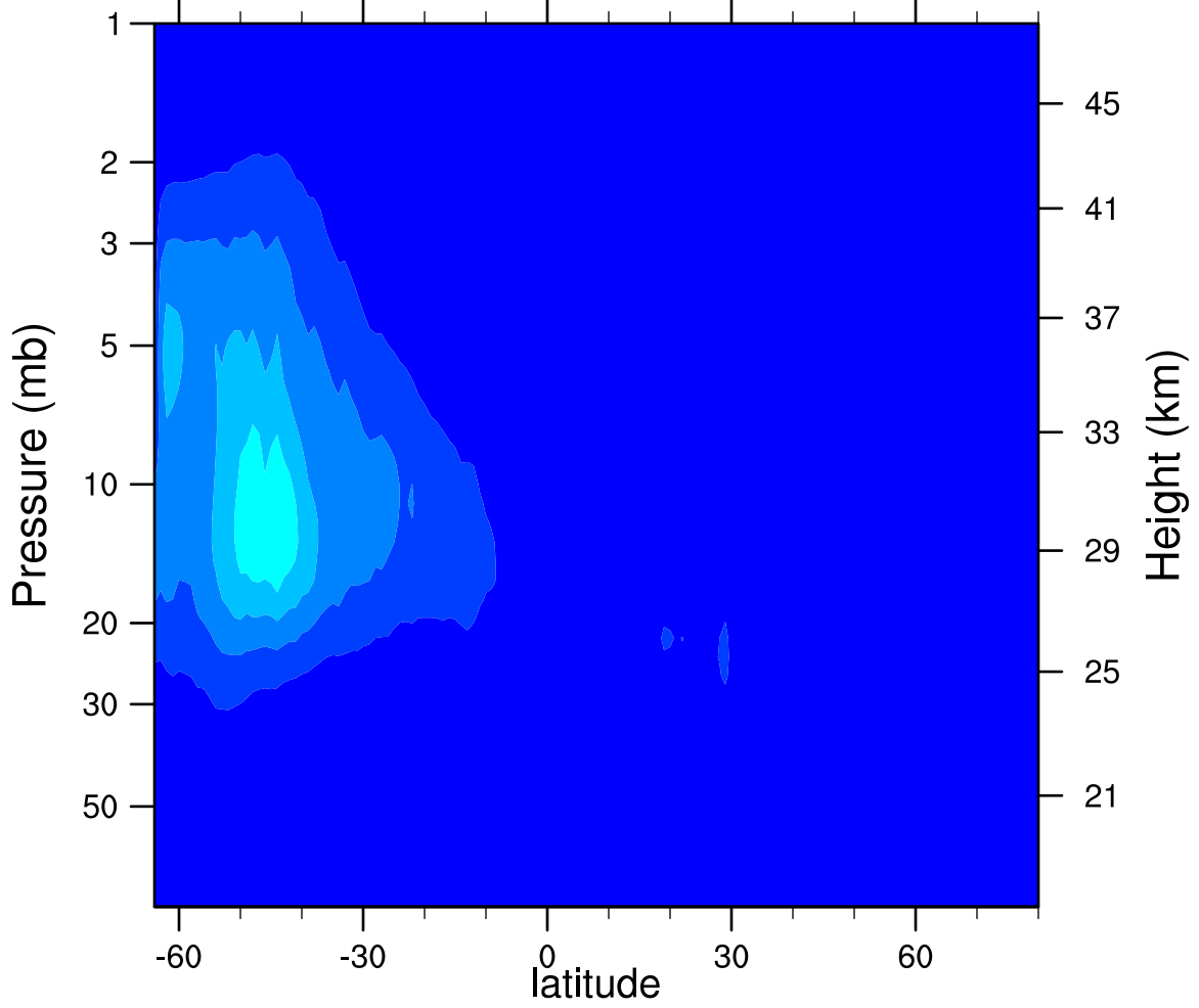
2007d178 N2O5_Ascending (ppbv)
