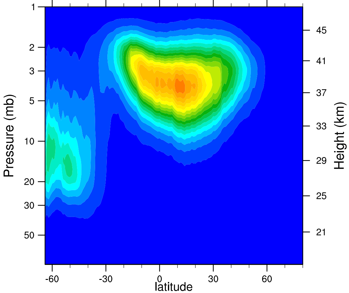
2005d121 N2O5_Ascending (ppbv)
