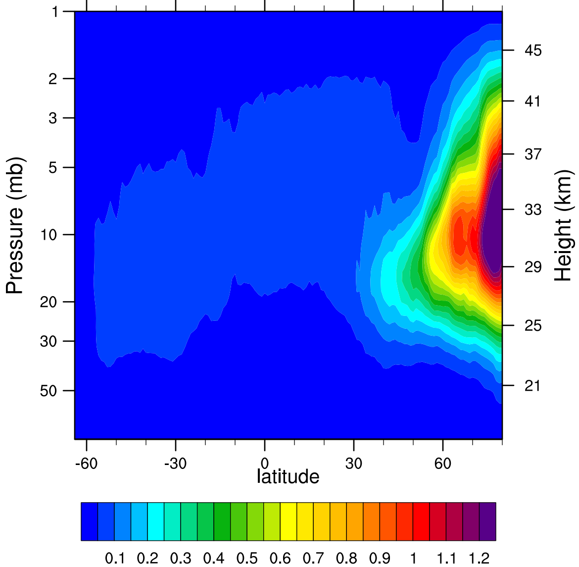
2007d325 N2O5_Ascending (ppbv)
