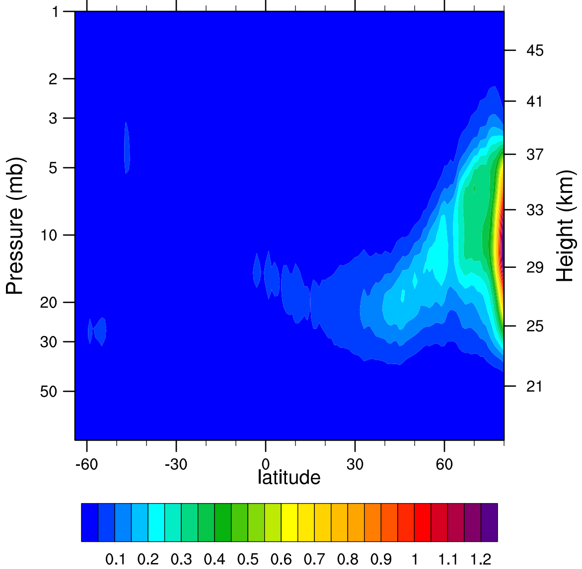
2007d055 N2O5_Ascending (ppbv)
