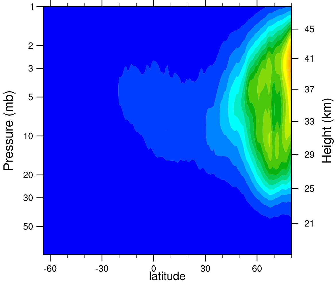
2005d320 N2O5_Ascending (ppbv)
