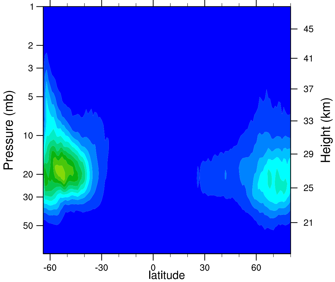
2007d081 N2O5_Ascending (ppbv)
