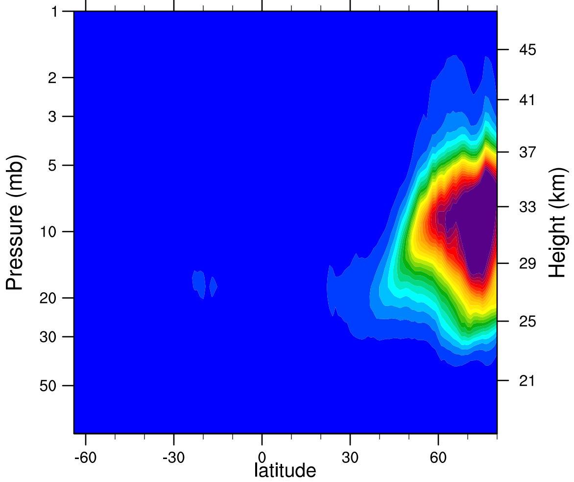
2007d003 N2O5_Ascending (ppbv)
