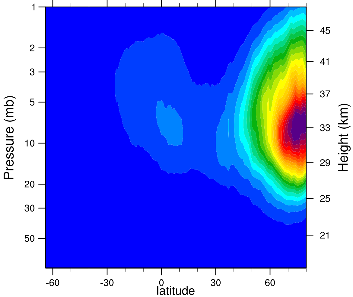
2005d364 N2O5_Ascending (ppbv)
