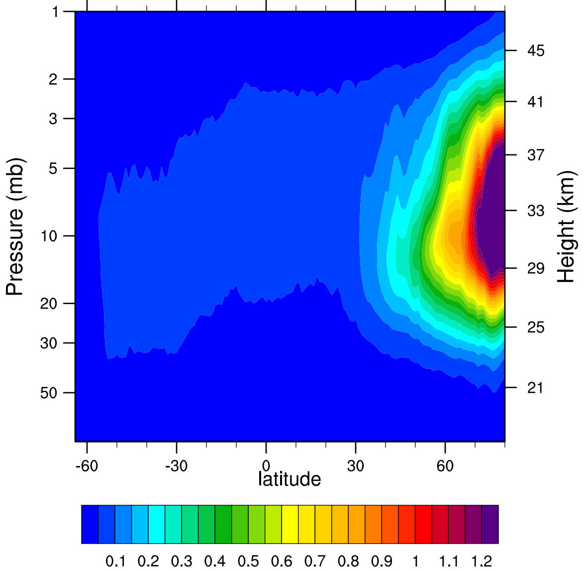
2007d344 N2O5_Ascending (ppbv)
