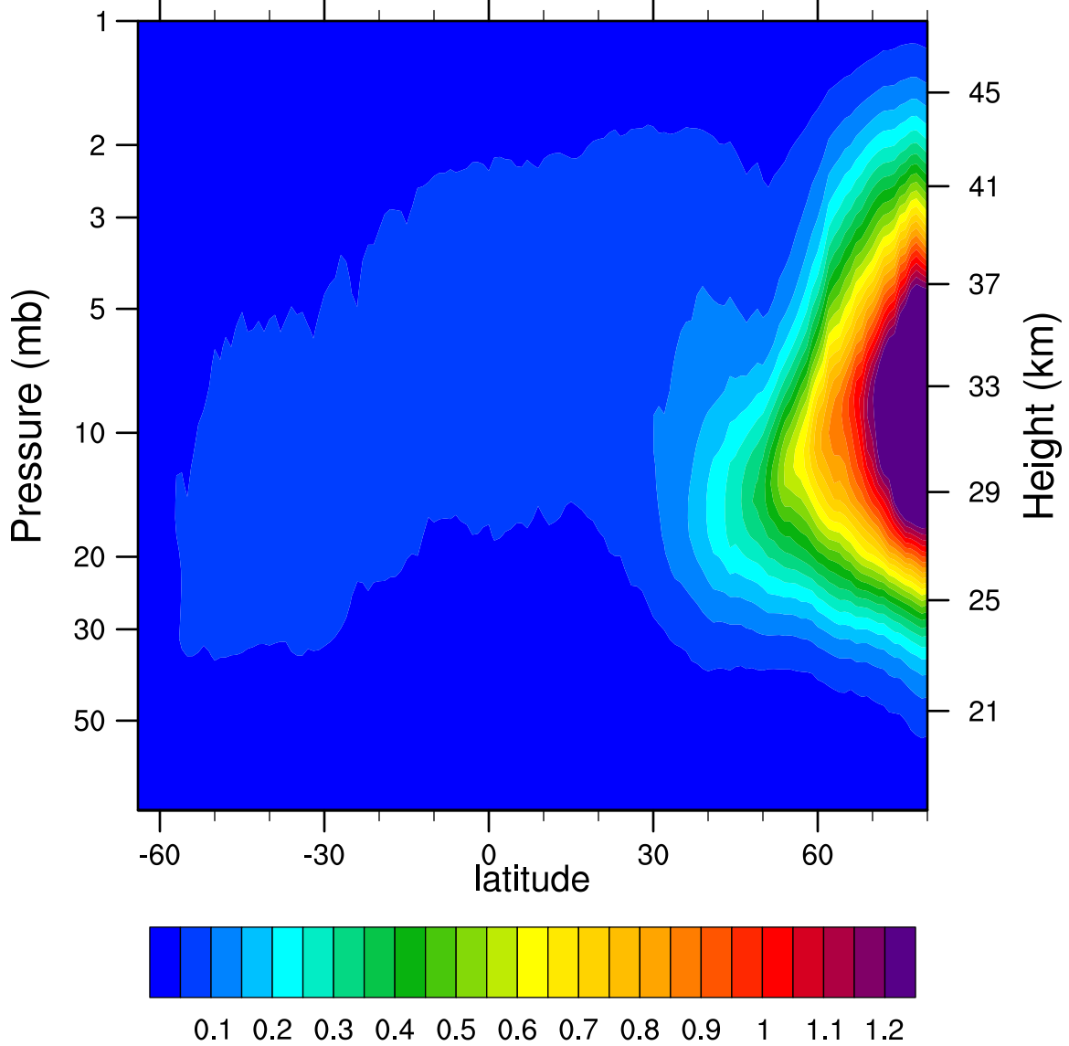
2007d333 N2O5_Ascending (ppbv)
