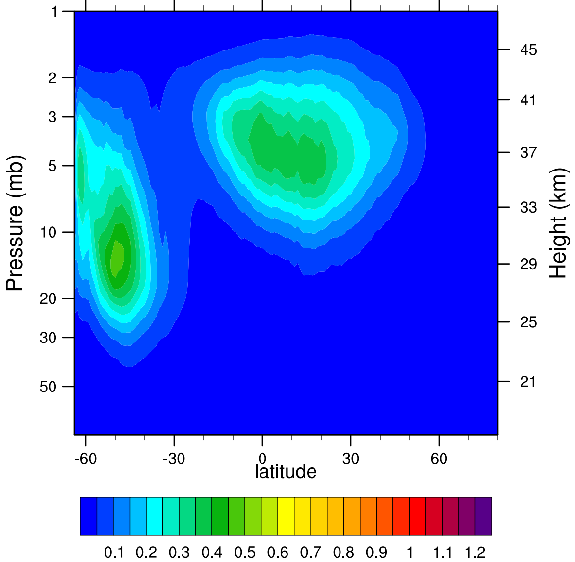
2005d174 N2O5_Ascending (ppbv)
