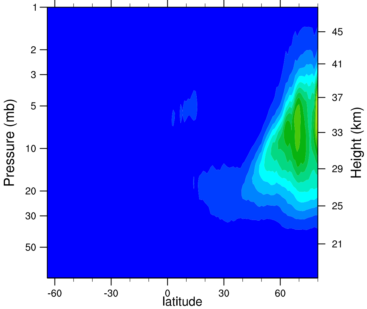
2007d045 N2O5_Ascending (ppbv)
