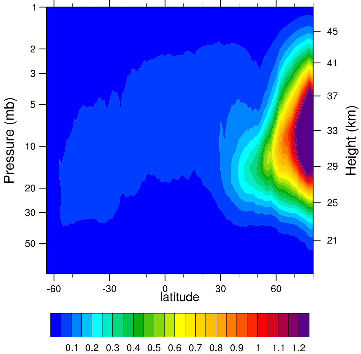
2007d331 N2O5_Ascending (ppbv)
