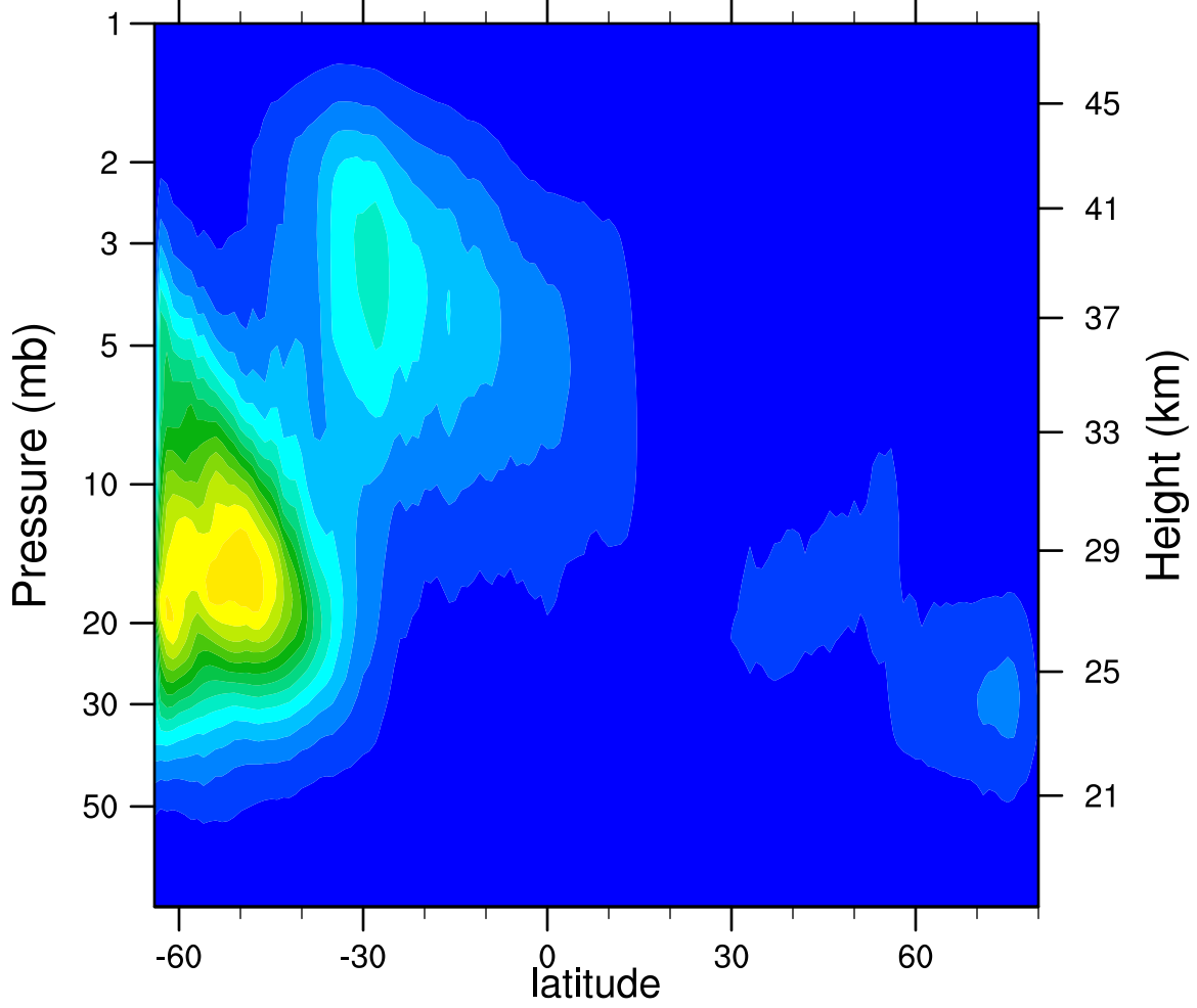
2007d106 N2O5_Ascending (ppbv)
