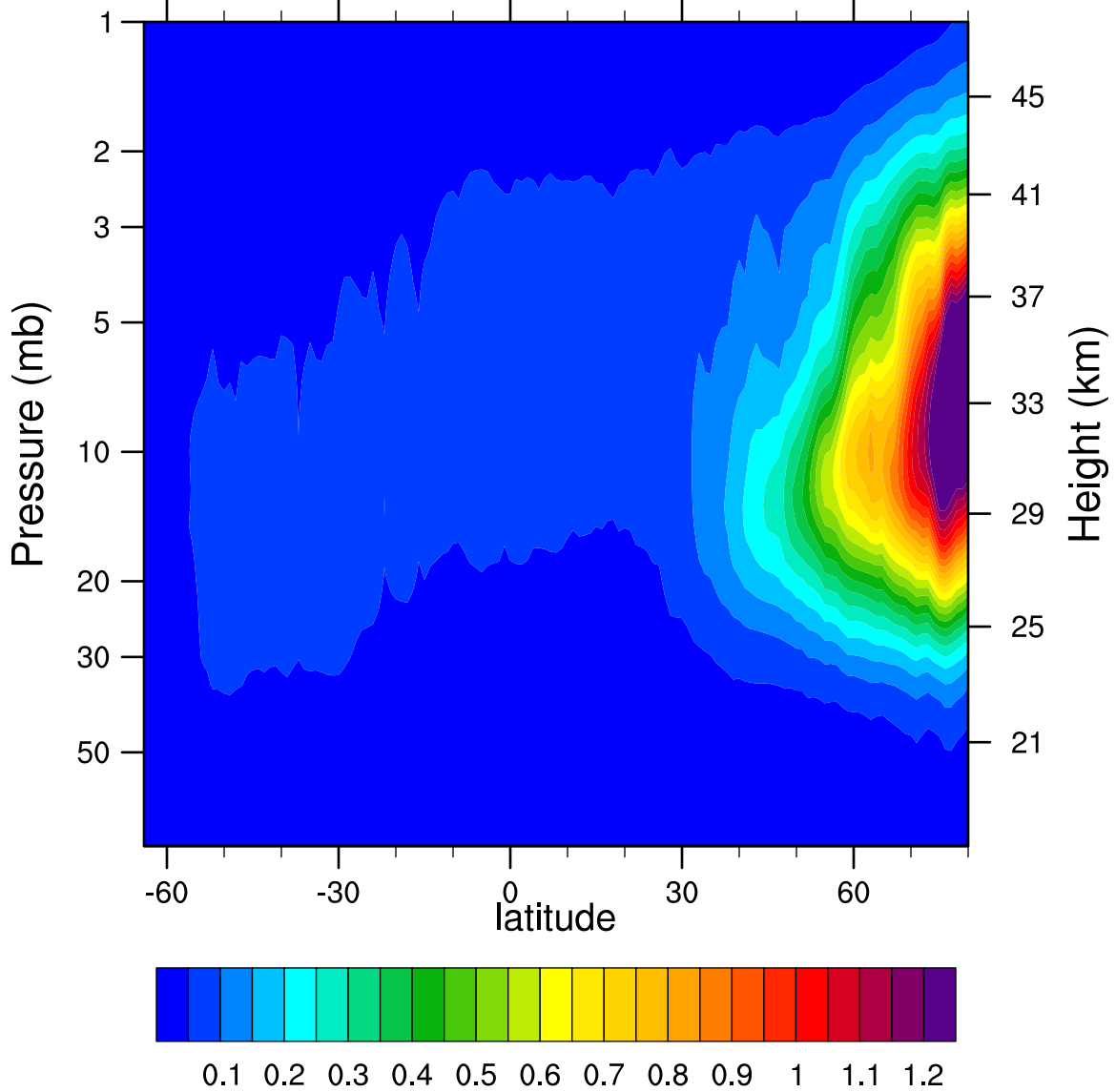
2007d342 N2O5_Ascending (ppbv)
