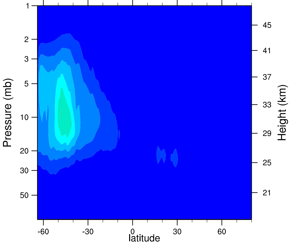
2007d174 N2O5_Ascending (ppbv)
