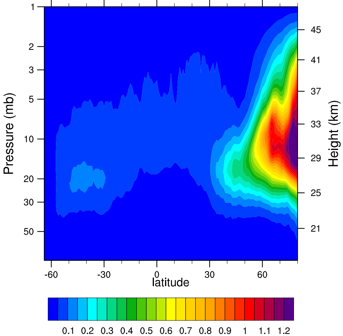
2007d319 N2O5_Ascending (ppbv)
