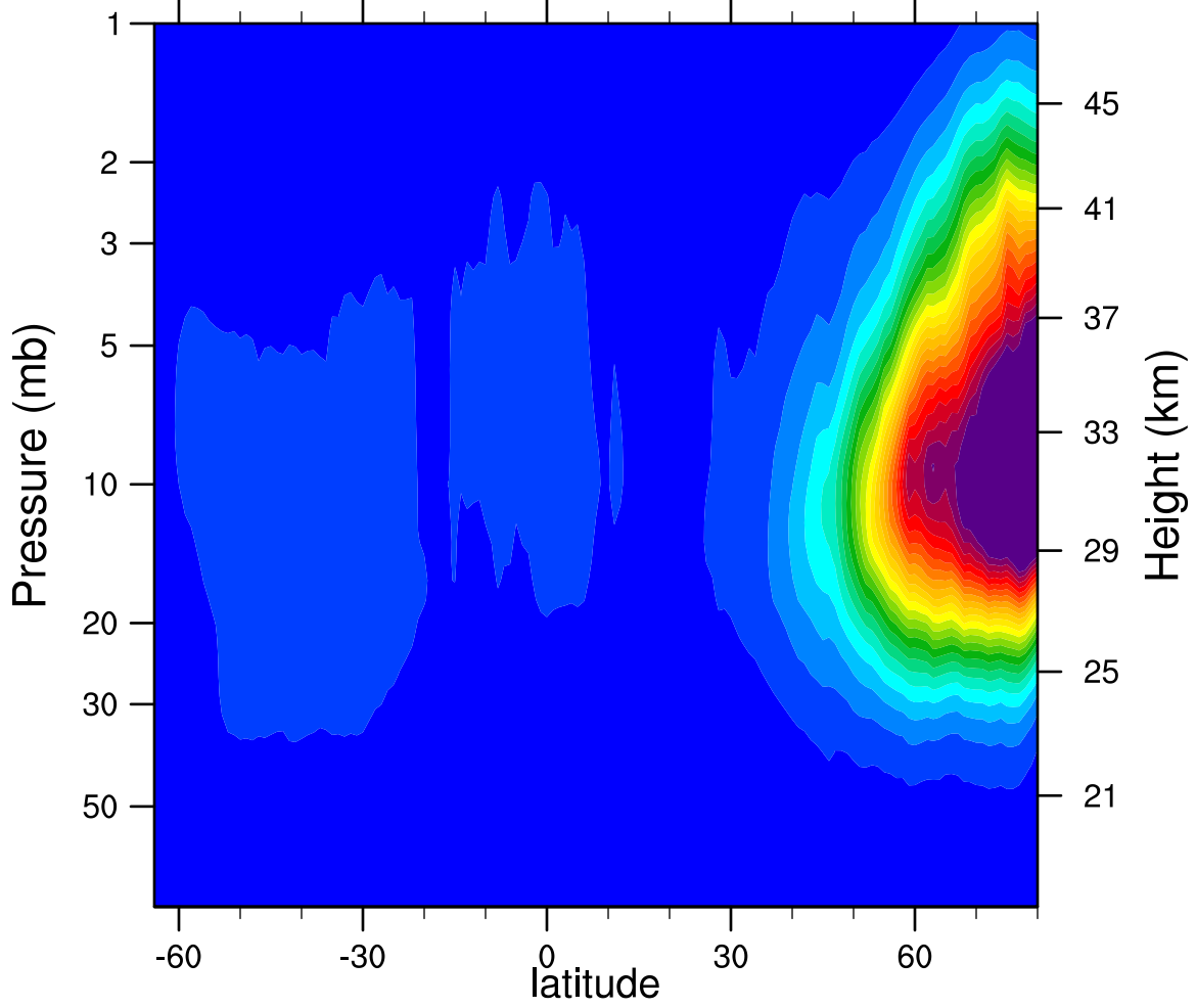
2007d362 N2O5_Ascending (ppbv)
