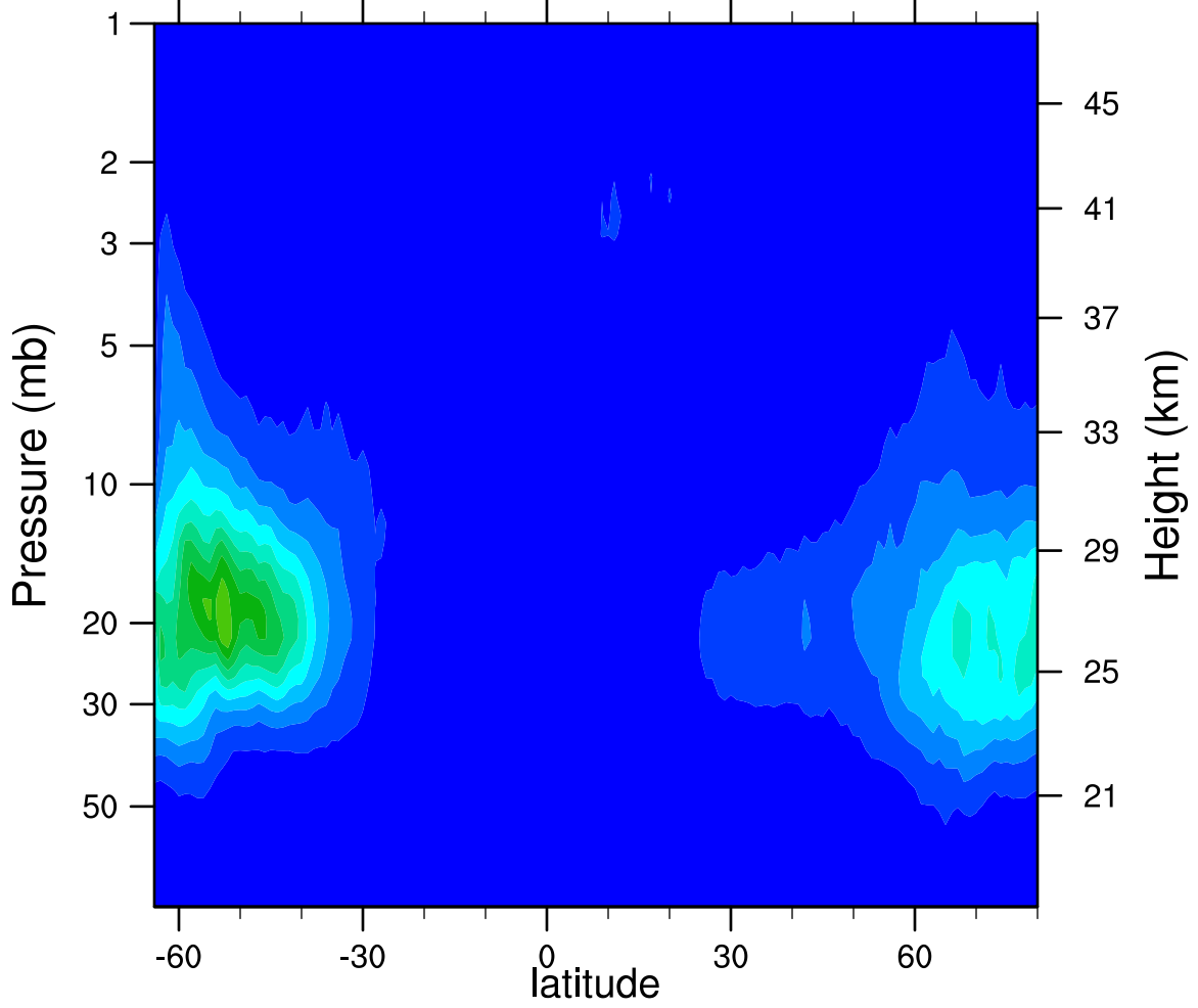
2007d080 N2O5_Ascending (ppbv)
