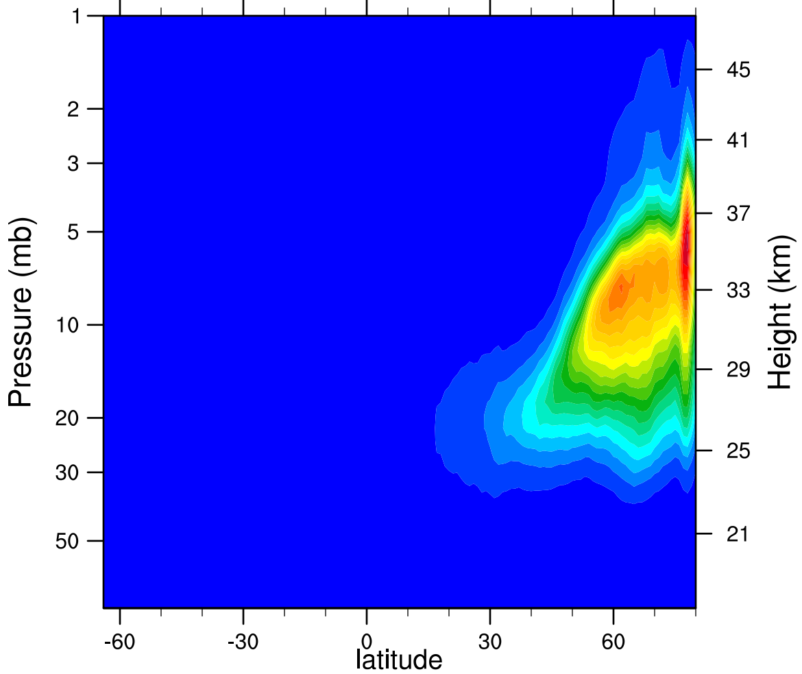
2007d020 N2O5_Ascending (ppbv)
