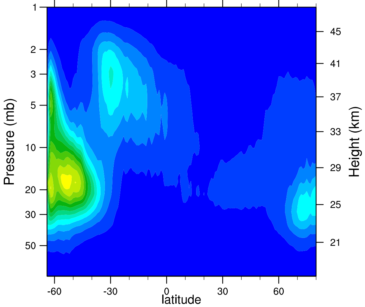
2007d094 N2O5_Ascending (ppbv)
