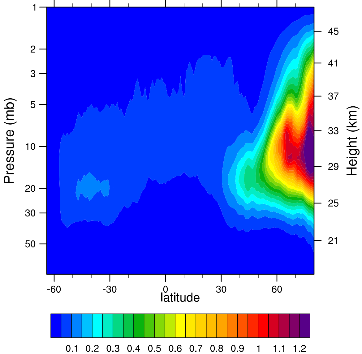
2007d320 N2O5_Ascending (ppbv)
