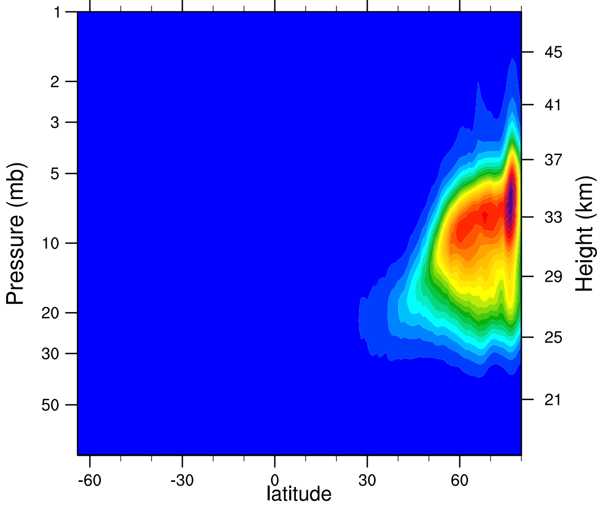
2007d010 N2O5_Ascending (ppbv)
