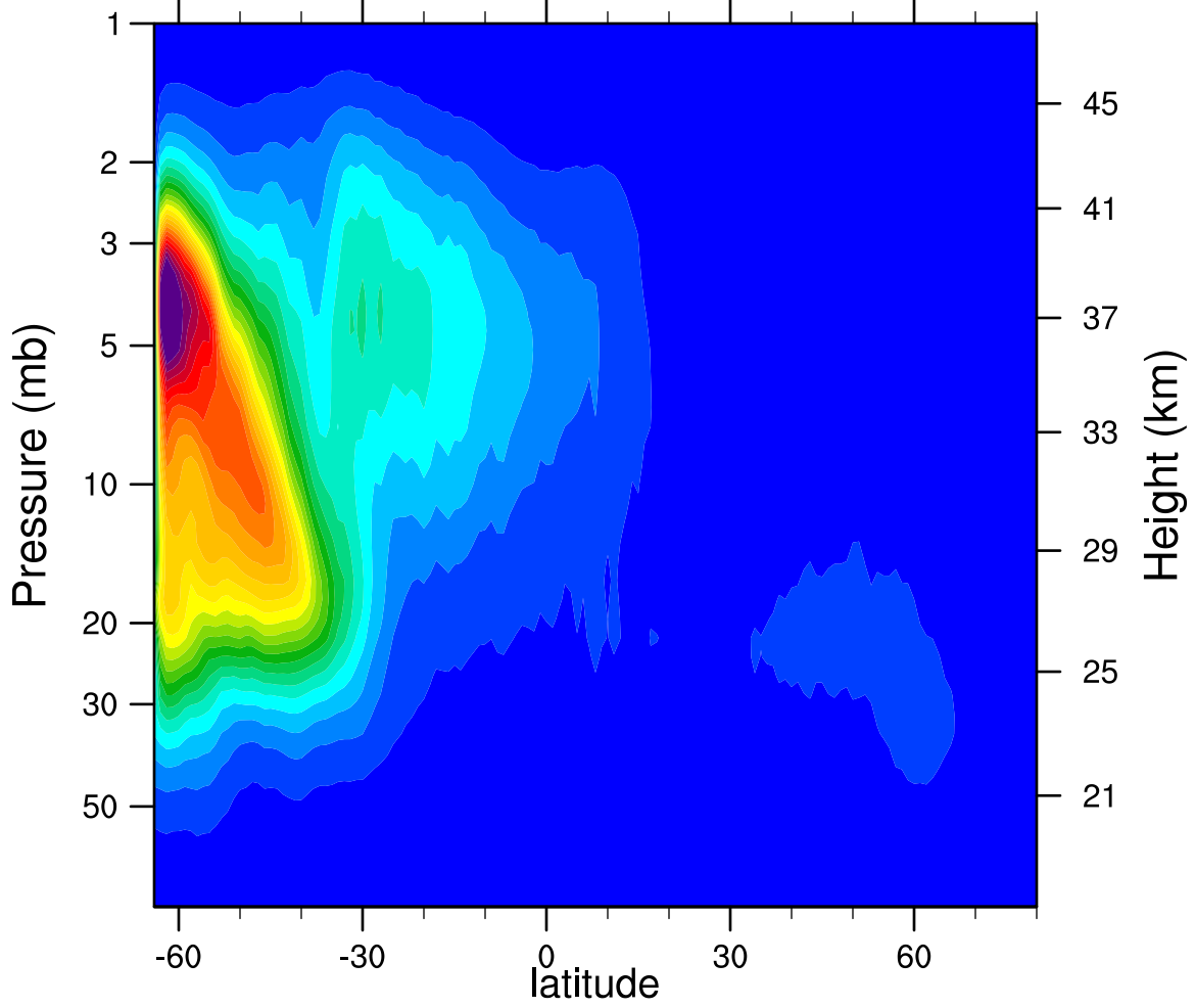
2007d129 N2O5_Ascending (ppbv)
