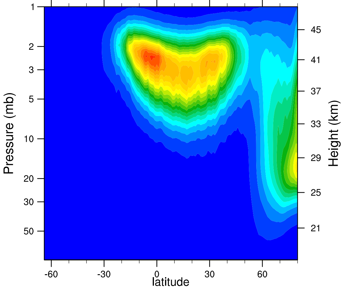
2005d044 N2O5_Ascending (ppbv)
