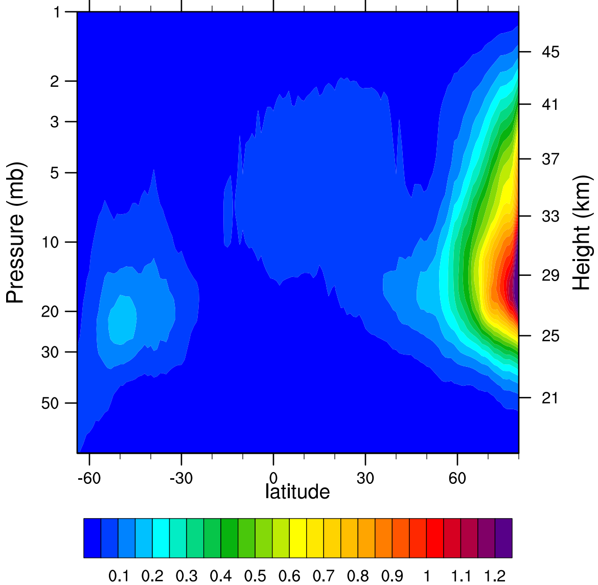
2007d304 N2O5_Ascending (ppbv)
