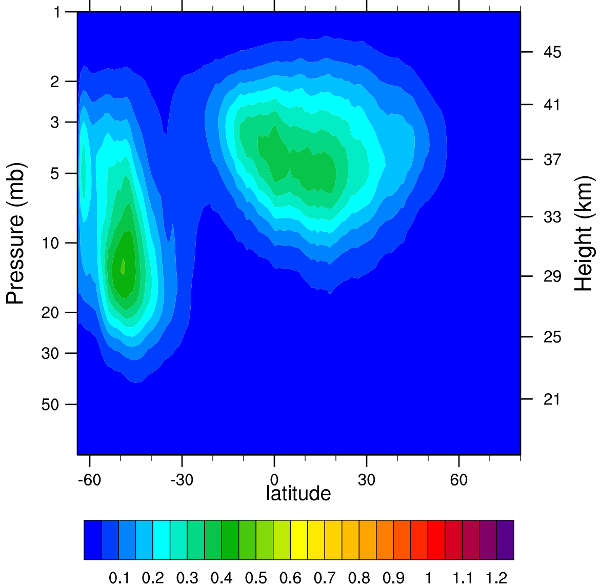
2005d178 N2O5_Ascending (ppbv)
