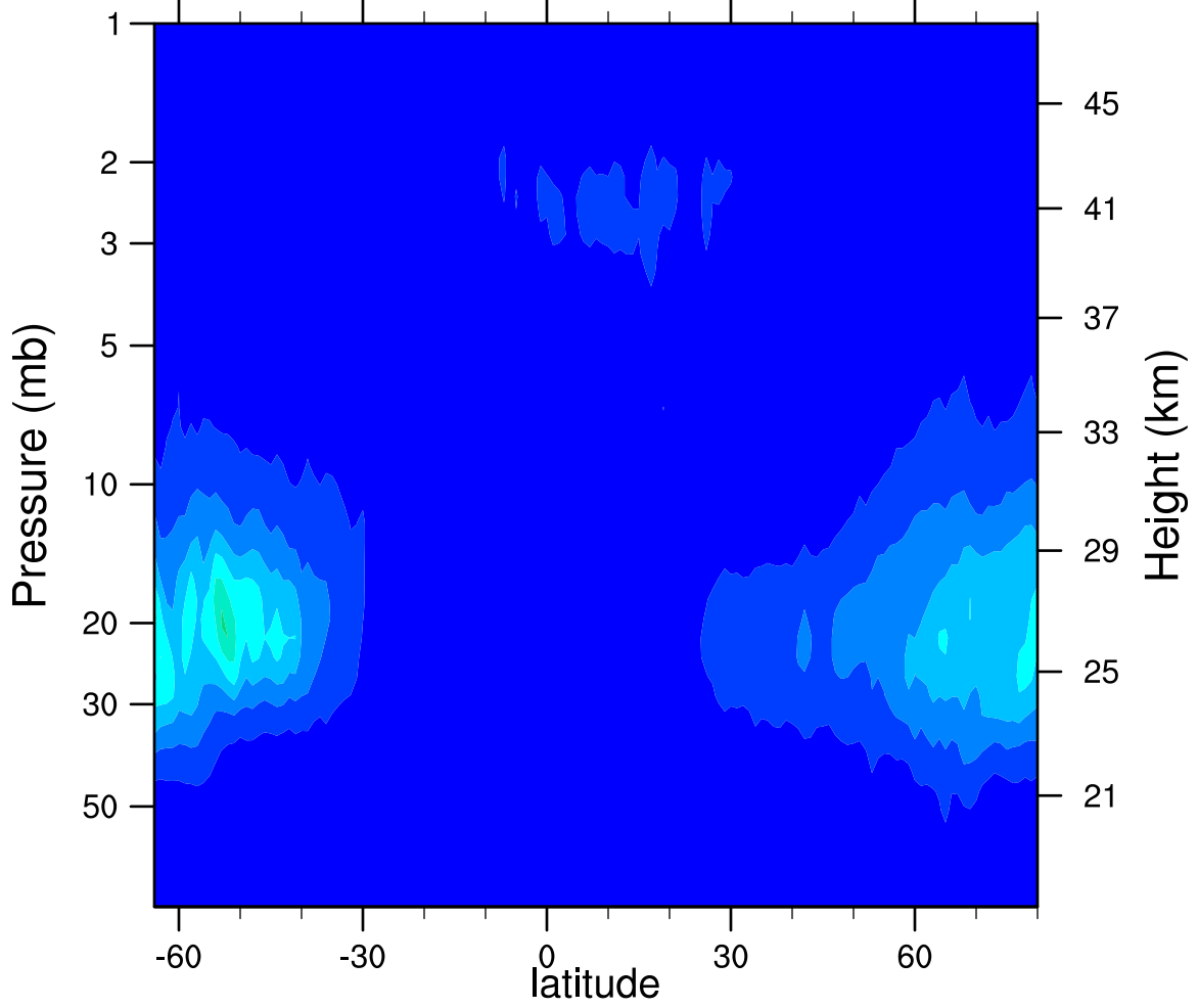
2007d078 N2O5_Ascending (ppbv)
