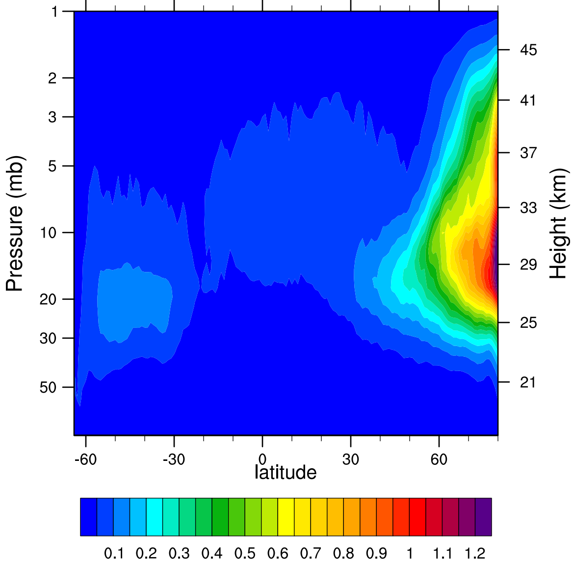
2007d311 N2O5_Ascending (ppbv)
