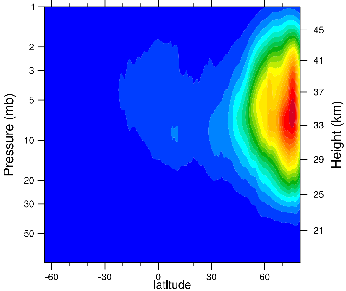
2005d338 N2O5_Ascending (ppbv)
