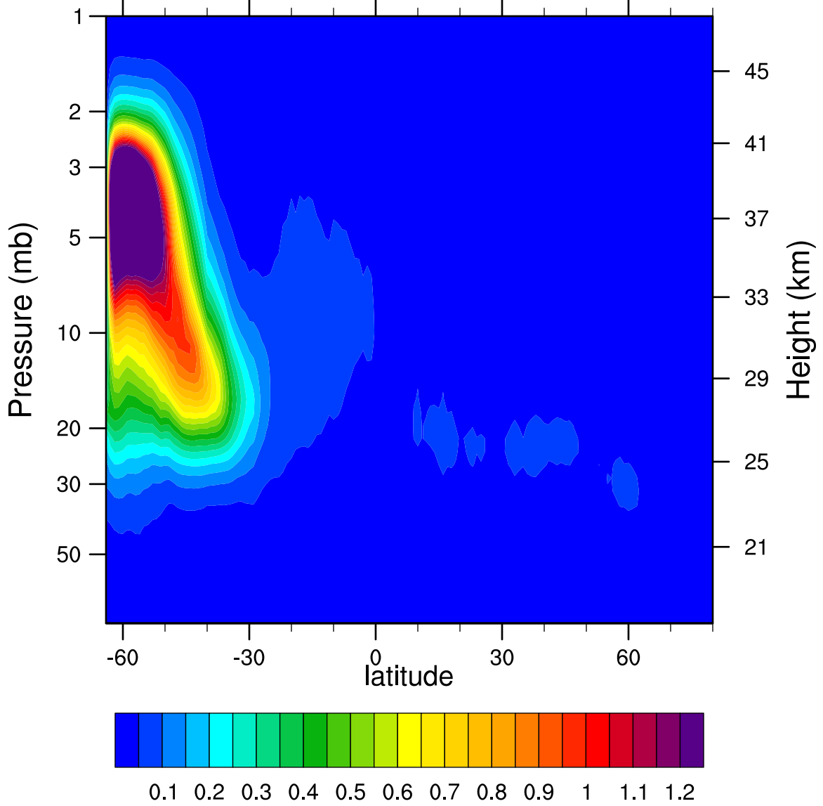
2007d154 N2O5_Ascending (ppbv)
