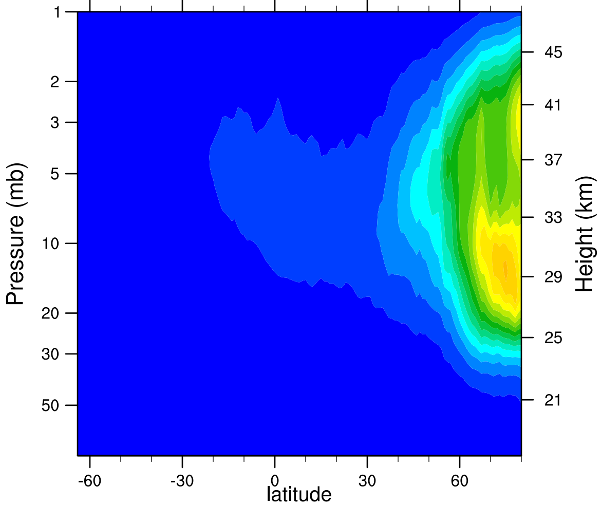
2005d316 N2O5_Ascending (ppbv)
