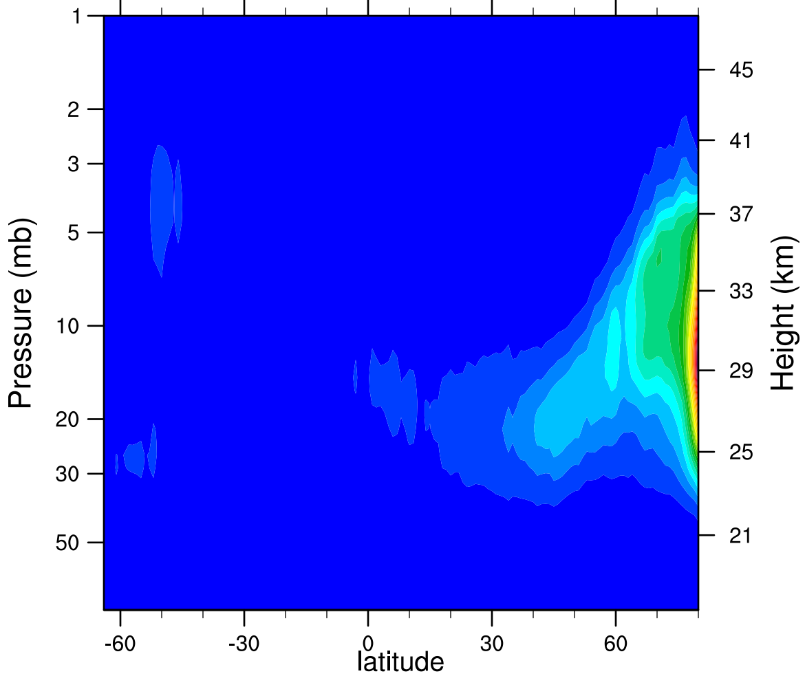
2007d057 N2O5_Ascending (ppbv)
