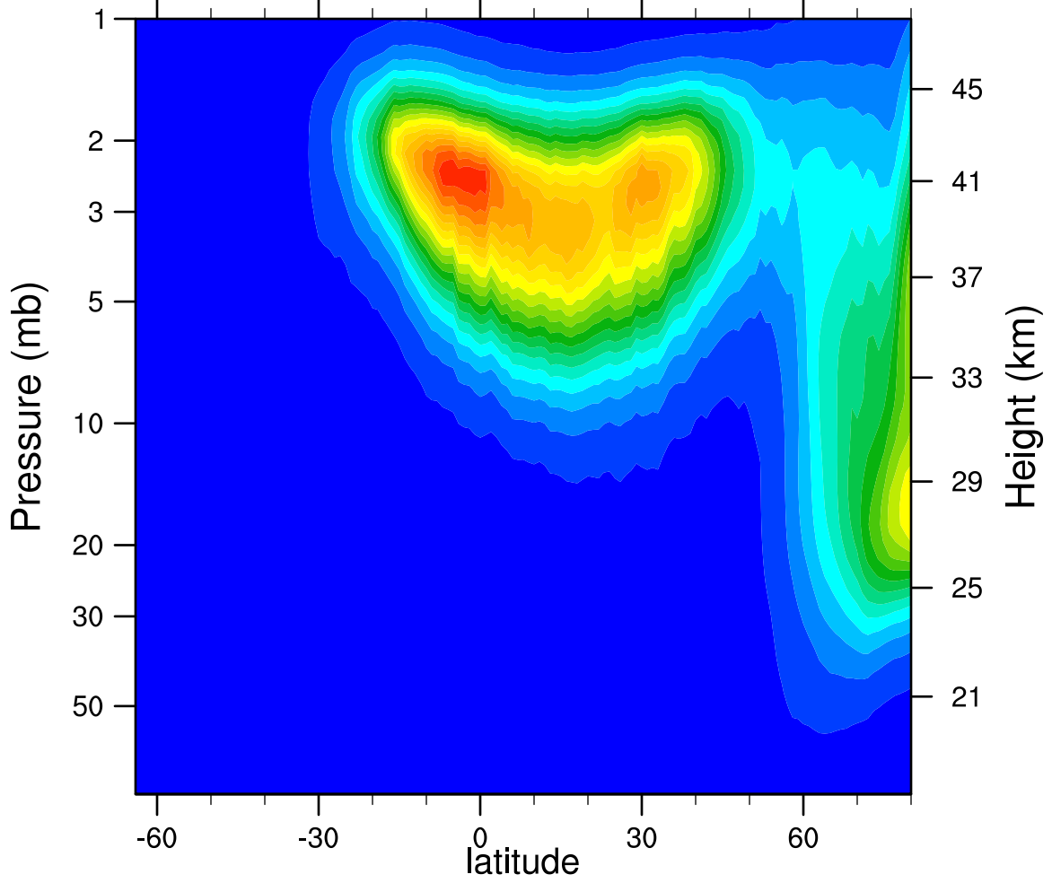
2005d045 N2O5_Ascending (ppbv)
