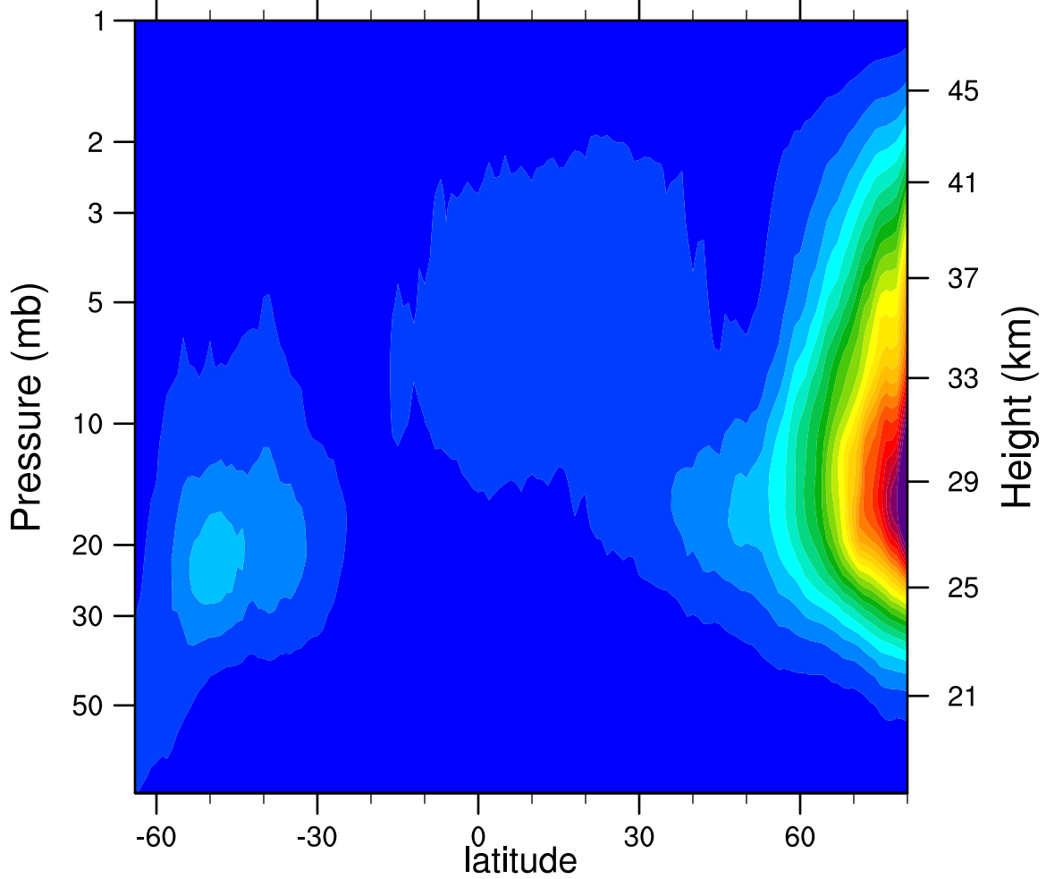
2007d303 N2O5_Ascending (ppbv)
