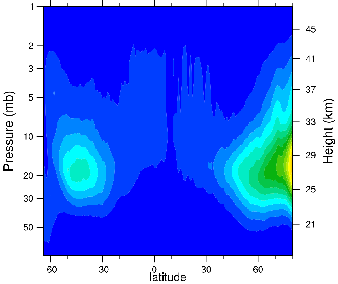
2007d278 N2O5_Ascending (ppbv)
