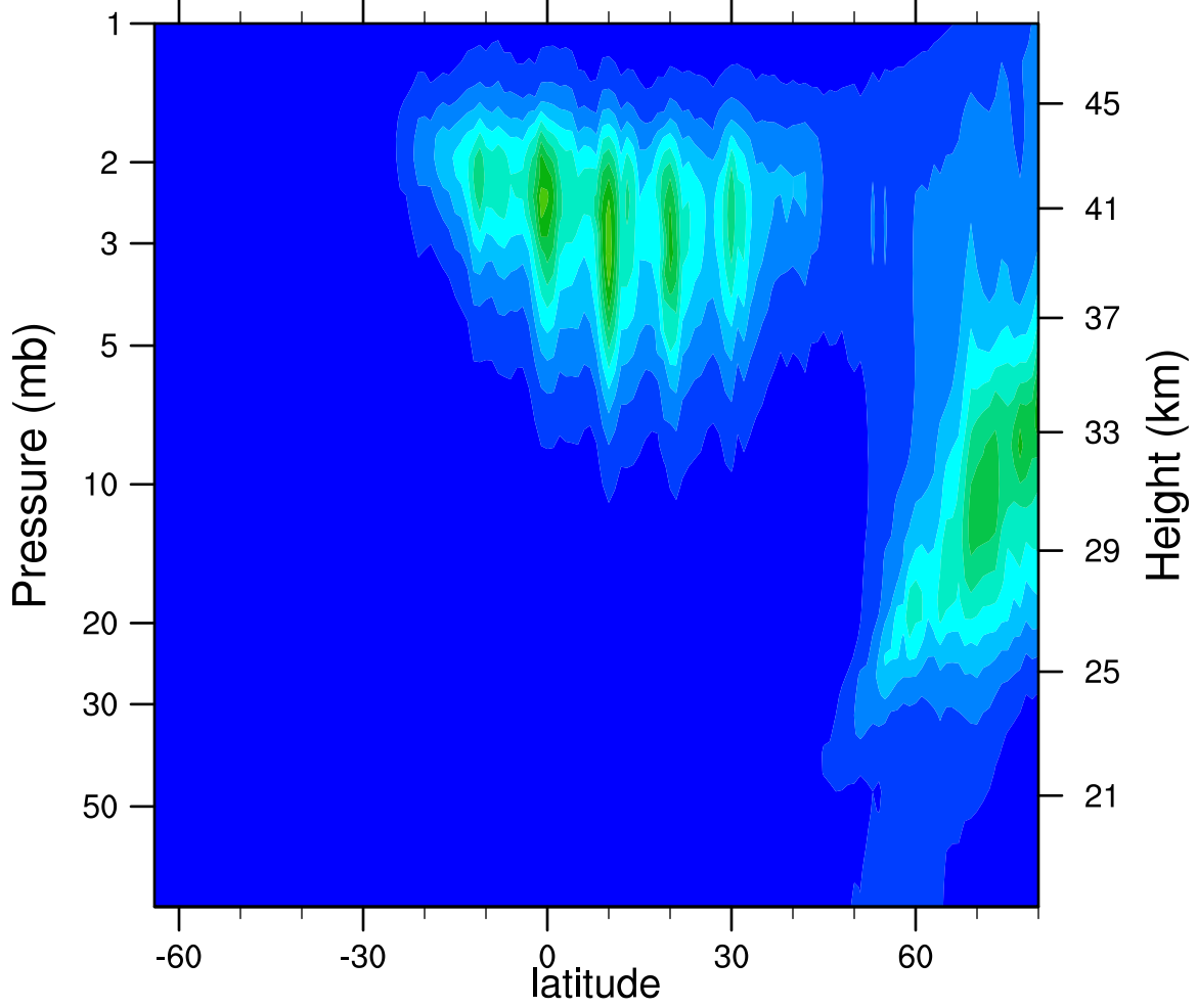
2005d025 N2O5_Ascending (ppbv)
