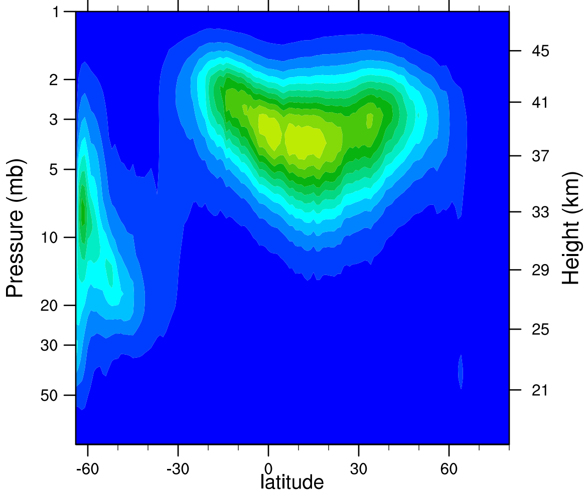
2005d106 N2O5_Ascending (ppbv)
