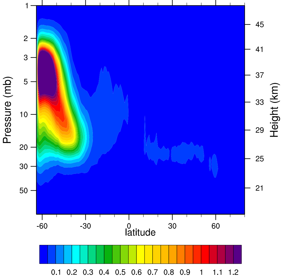
2007d150 N2O5_Ascending (ppbv)
