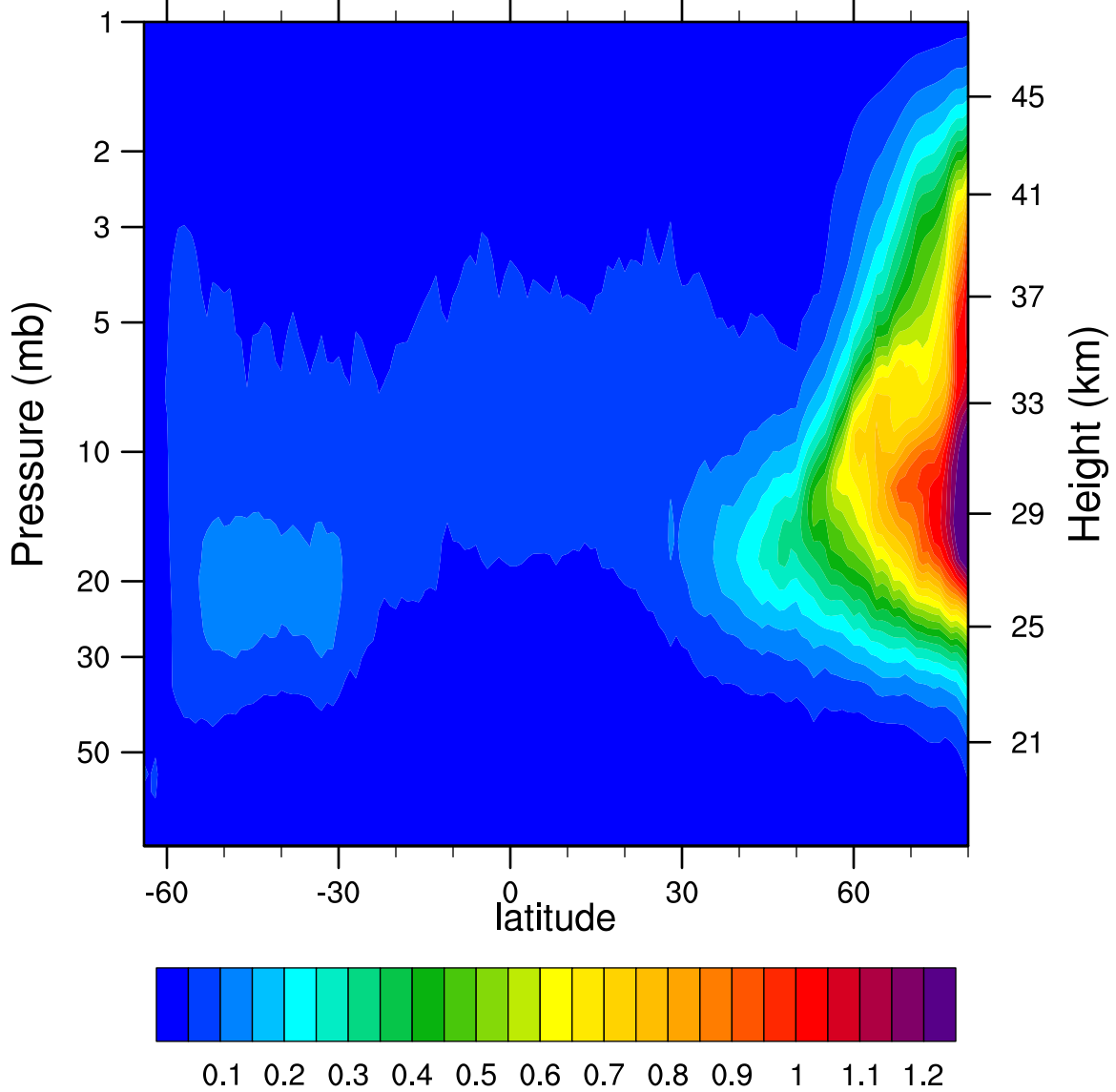
2007d313 N2O5_Ascending (ppbv)
