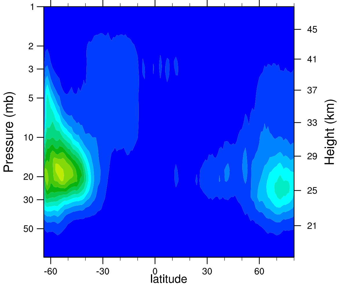
2007d084 N2O5_Ascending (ppbv)
