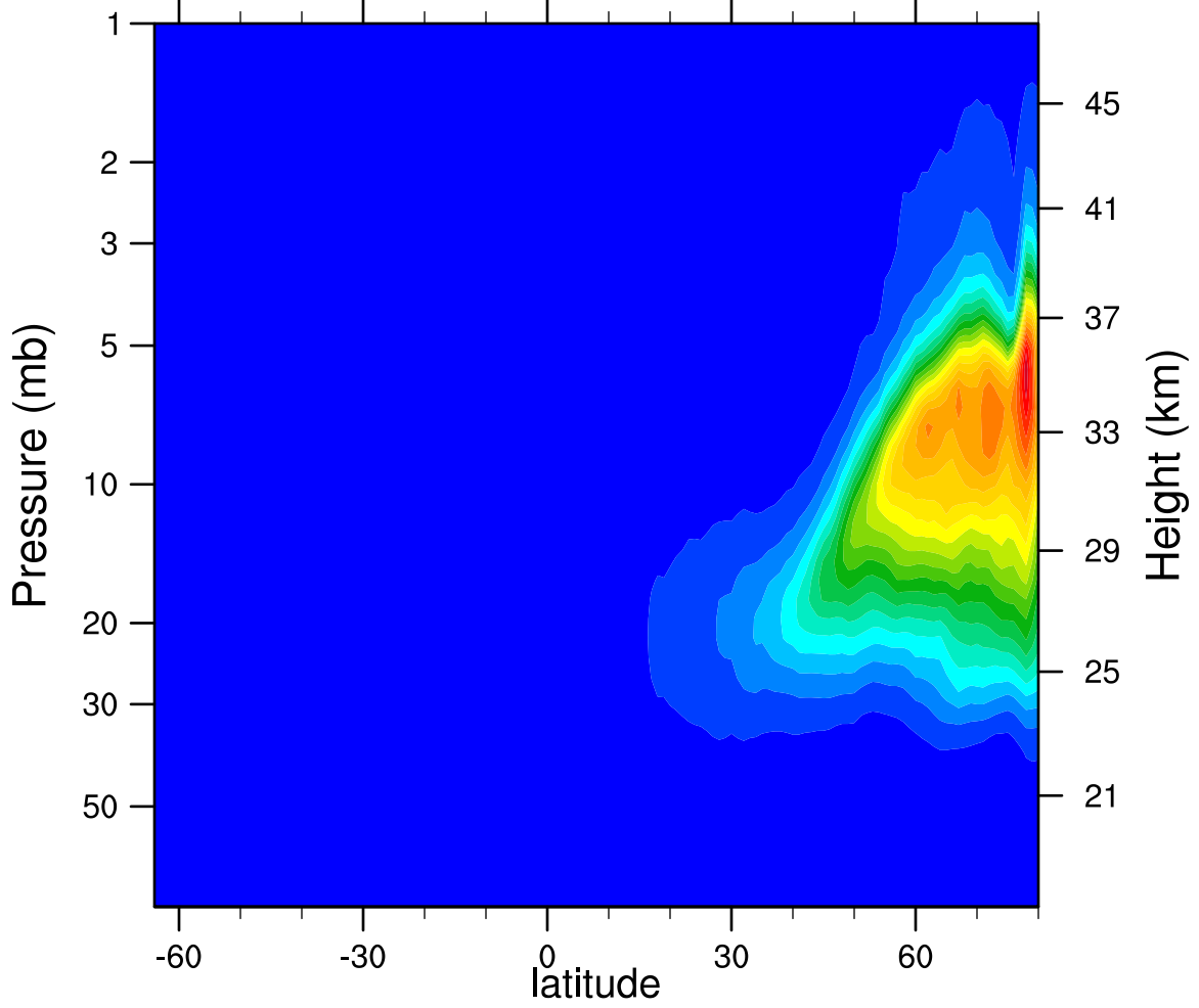
2007d024 N2O5_Ascending (ppbv)
