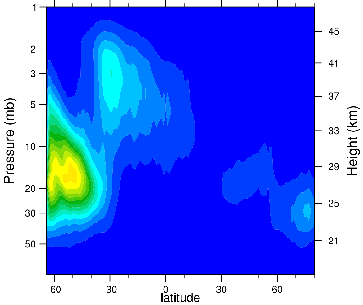
2007d102 N2O5_Ascending (ppbv)
