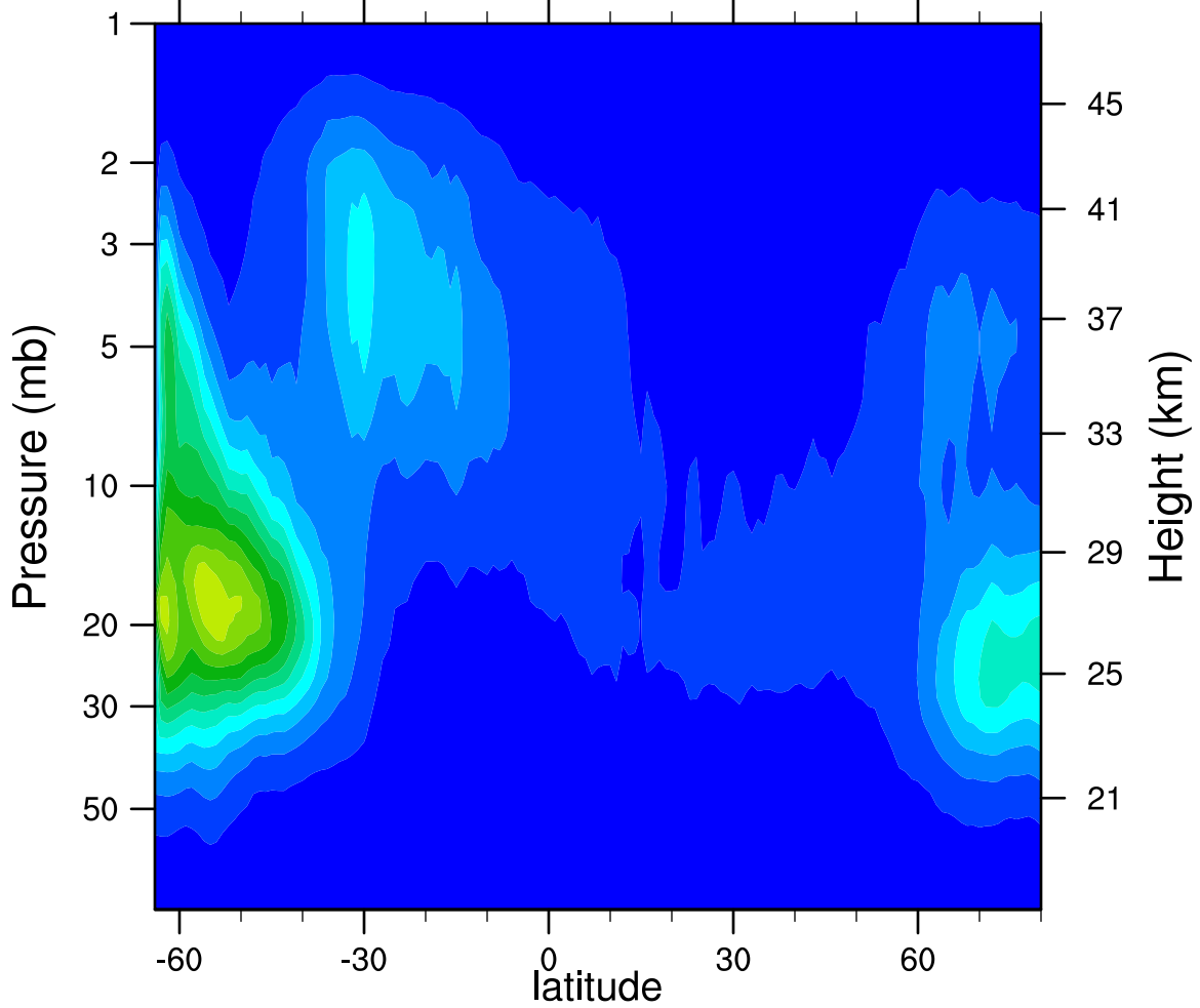
2007d088 N2O5_Ascending (ppbv)
