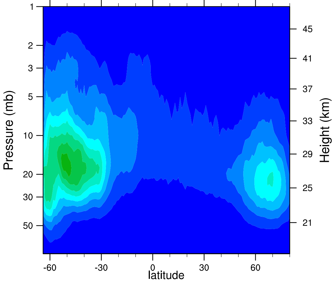
2007d254 N2O5_Ascending (ppbv)
