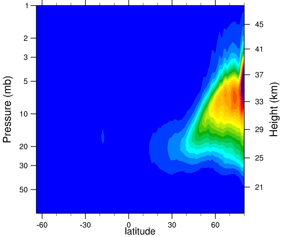
2007d028 N2O5_Ascending (ppbv)
