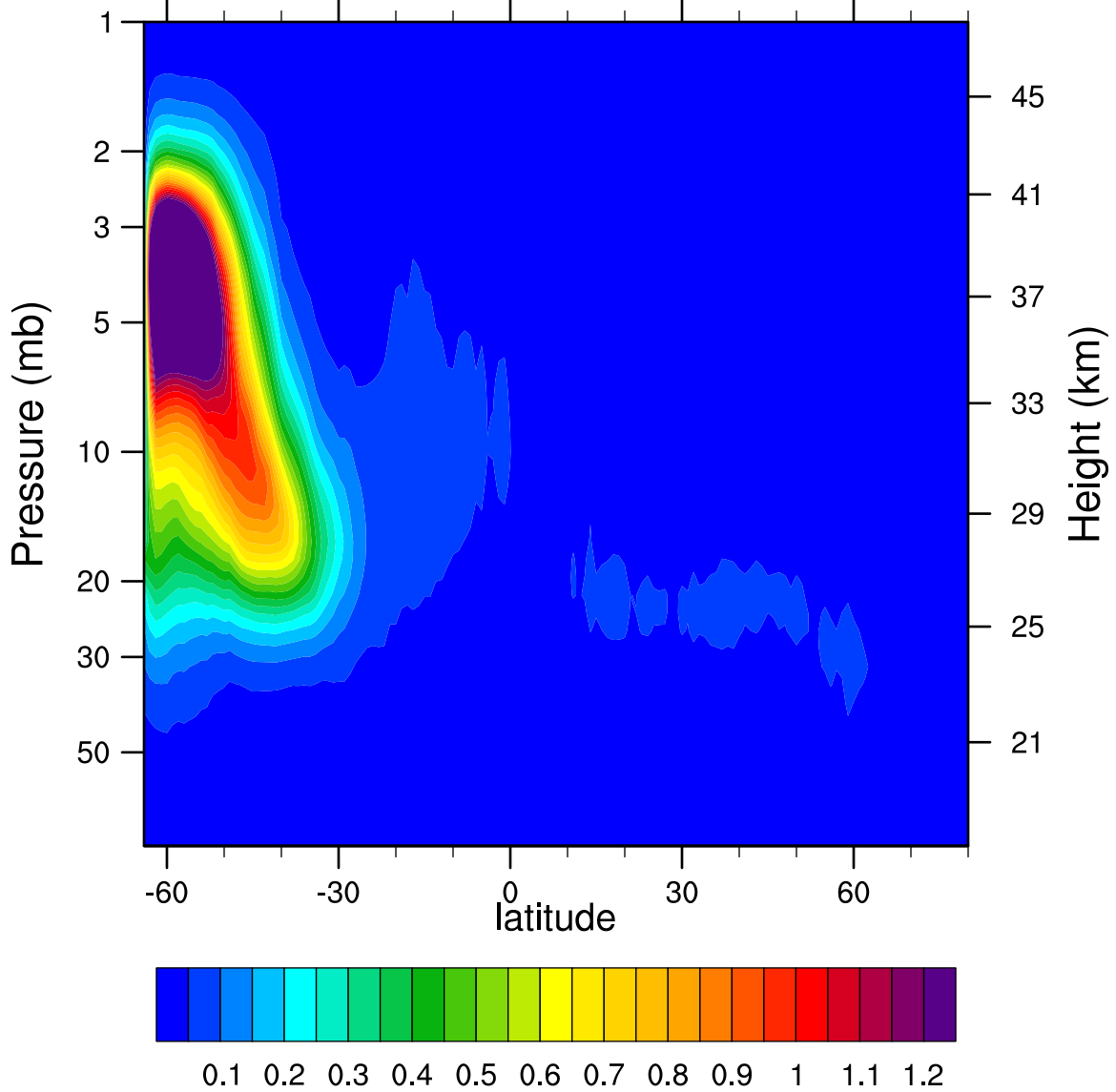
2007d151 N2O5_Ascending (ppbv)
