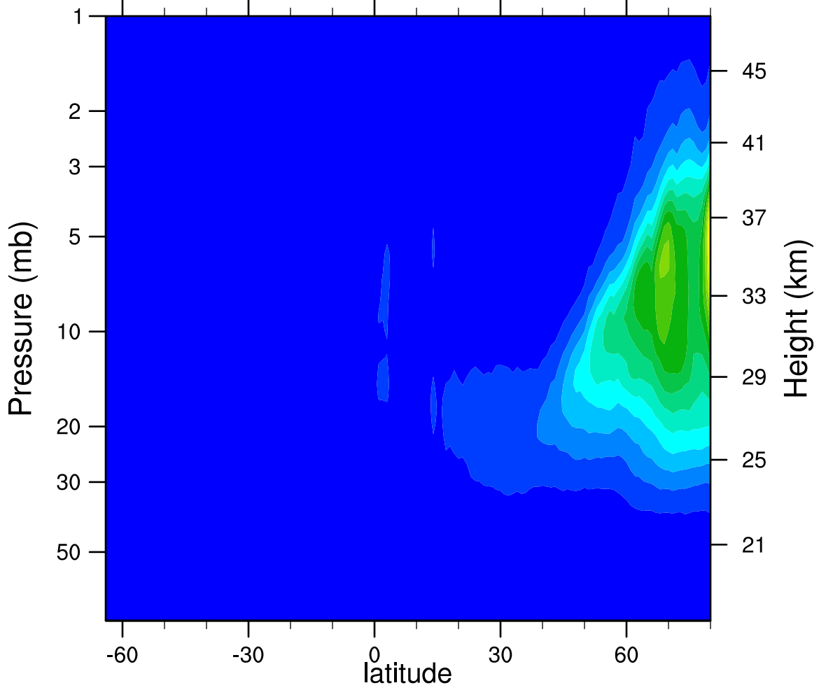
2007d044 N2O5_Ascending (ppbv)
