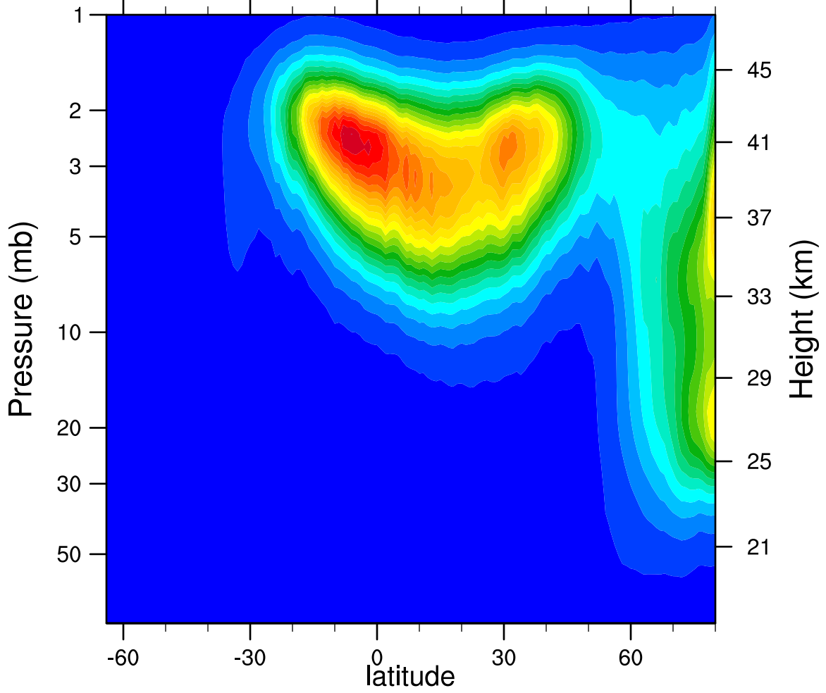
2005d049 N2O5_Ascending (ppbv)
