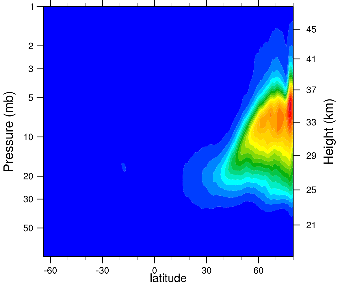
2007d025 N2O5_Ascending (ppbv)
