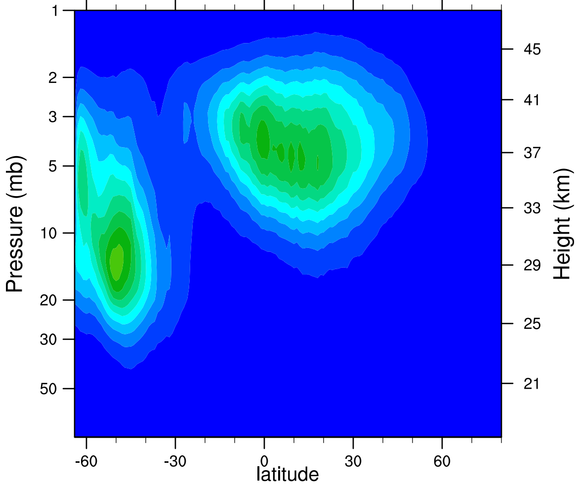
2005d171 N2O5_Ascending (ppbv)
