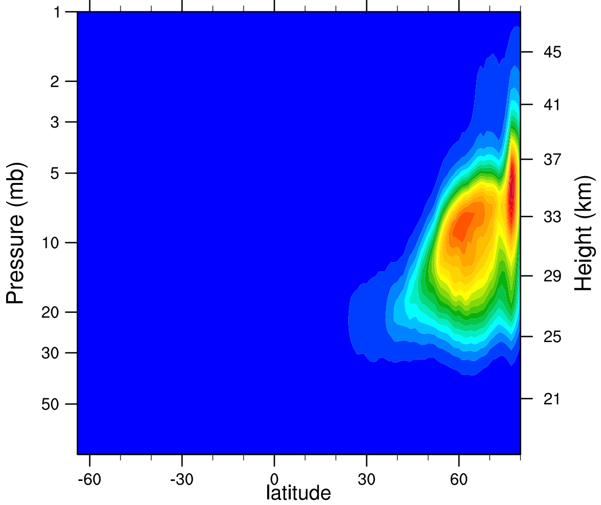
2007d014 N2O5_Ascending (ppbv)
