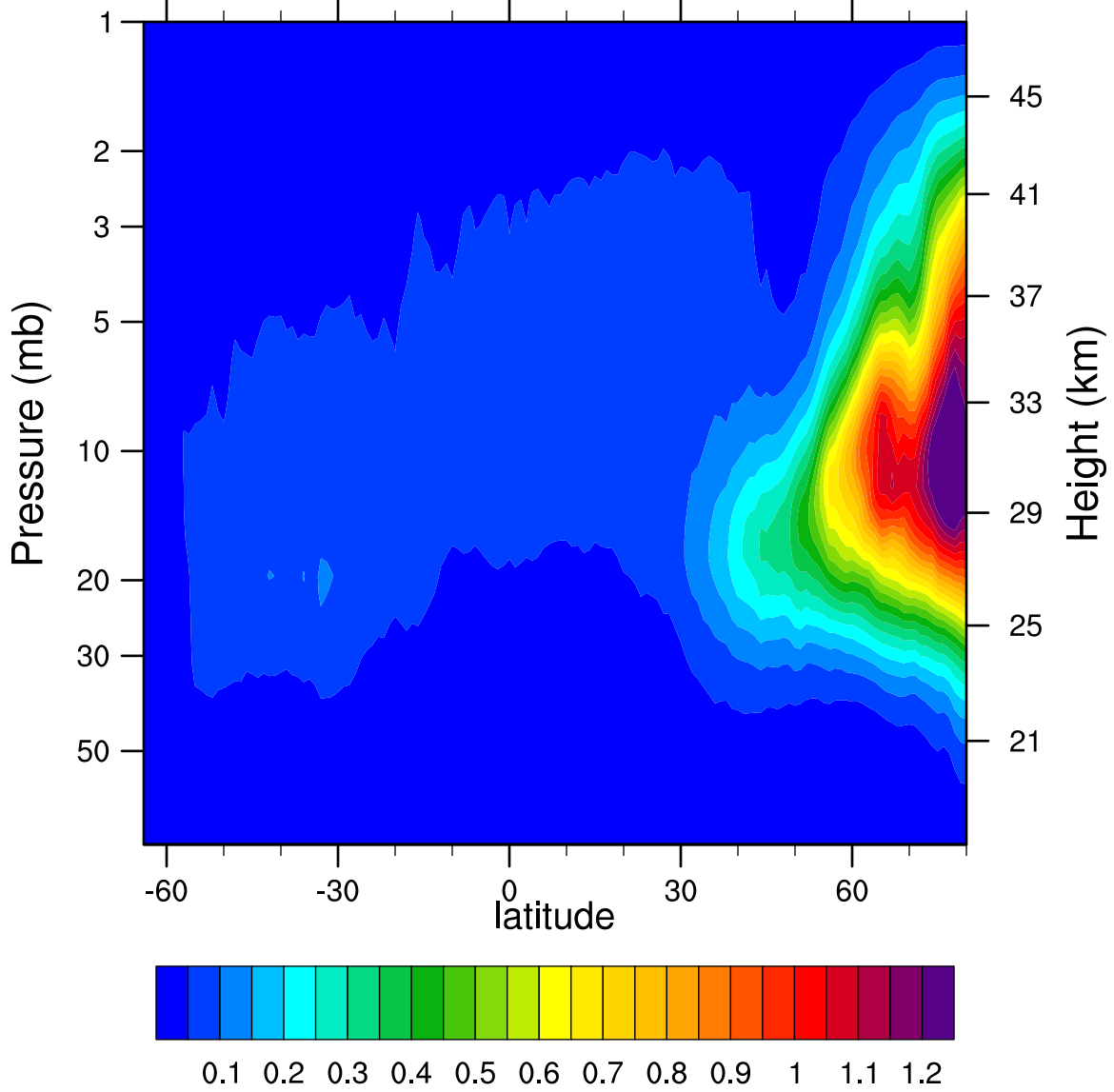
2007d323 N2O5_Ascending (ppbv)
