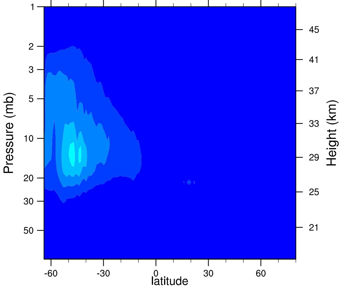
2007d180 N2O5_Ascending (ppbv)
