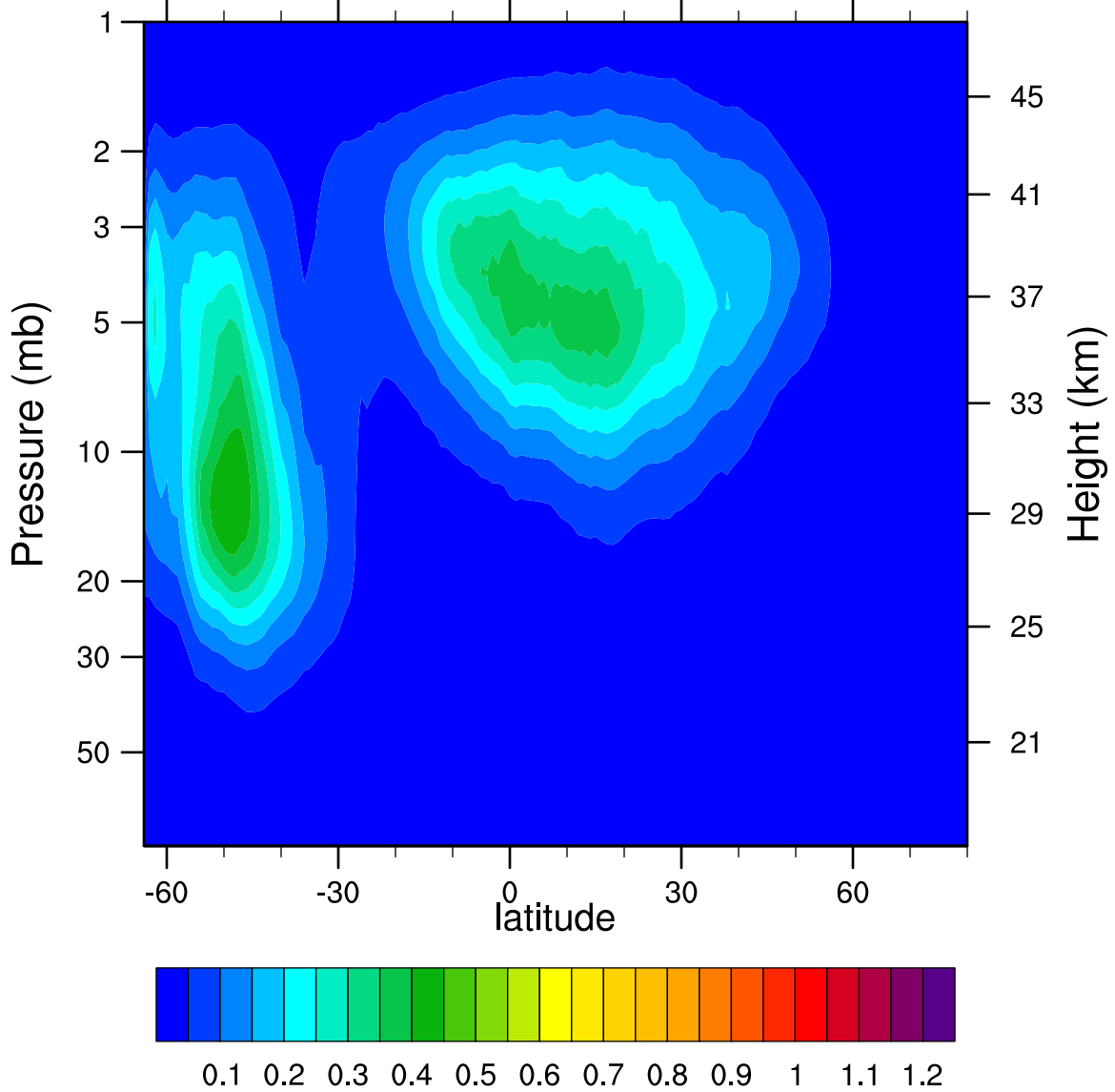
2005d179 N2O5_Ascending (ppbv)
