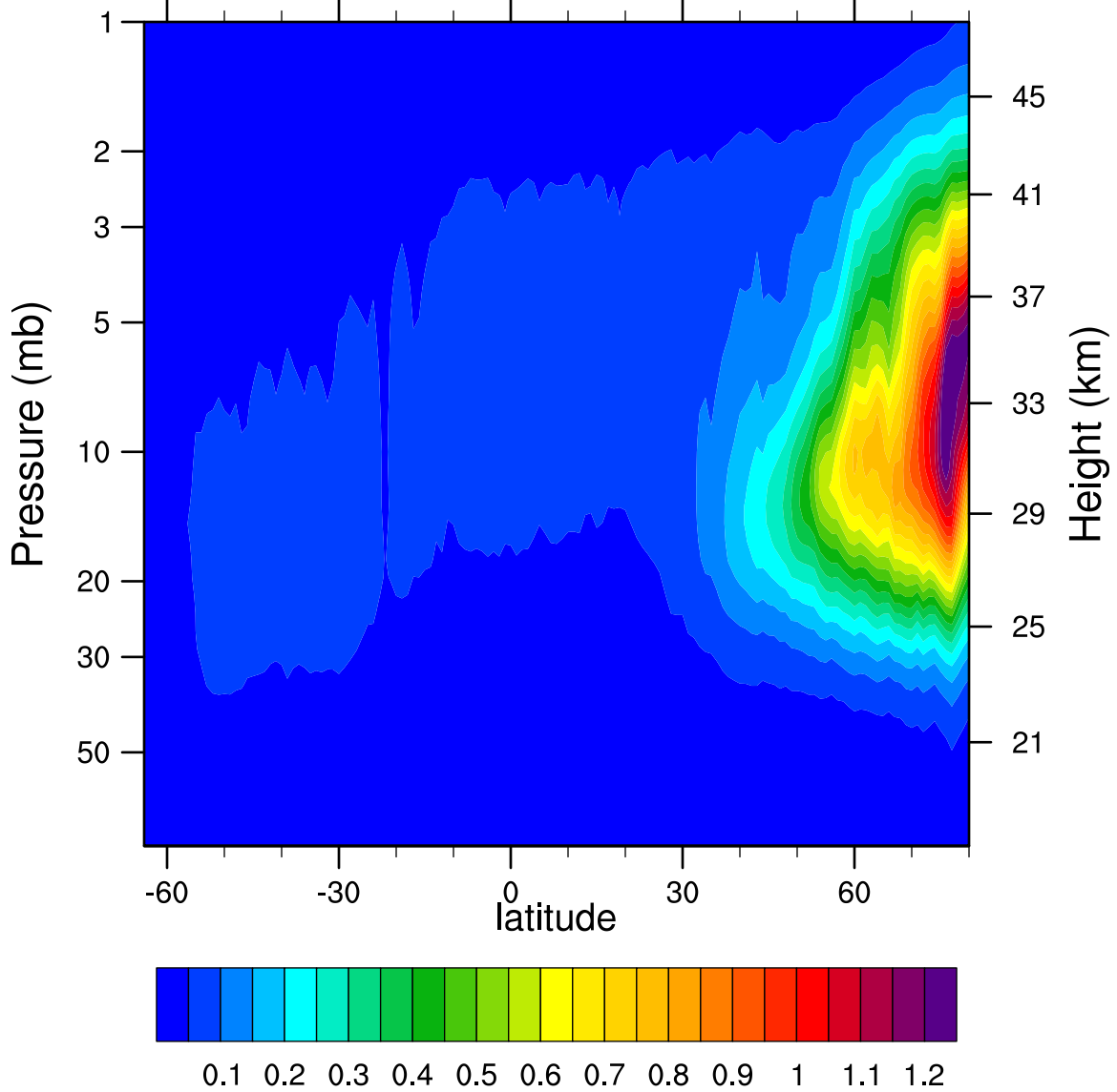
2007d340 N2O5_Ascending (ppbv)
