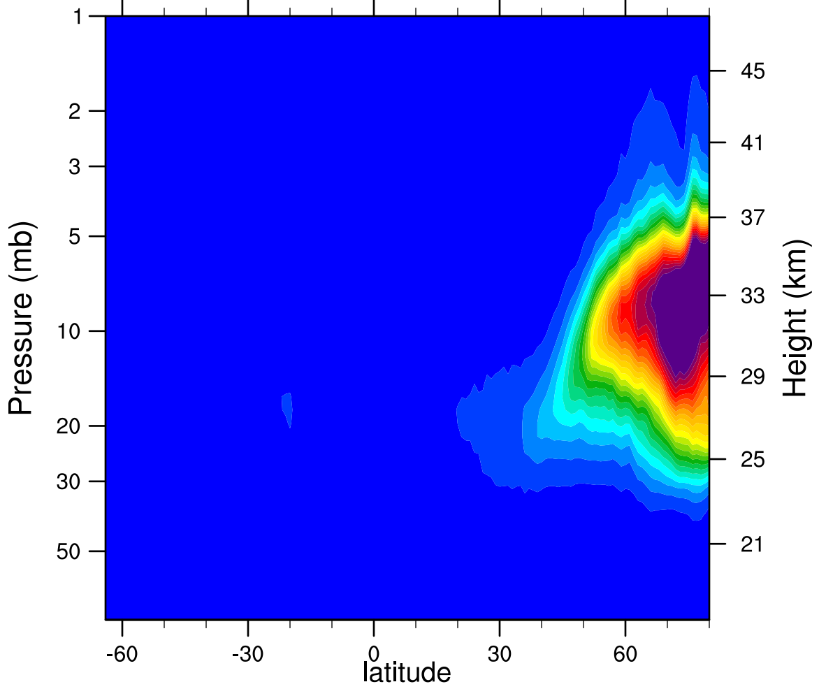
2007d006 N2O5_Ascending (ppbv)
