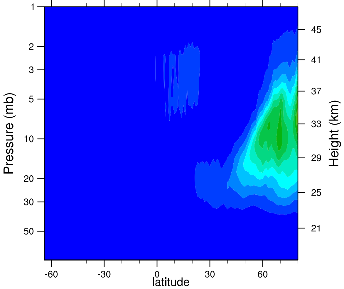
2007d048 N2O5_Ascending (ppbv)
