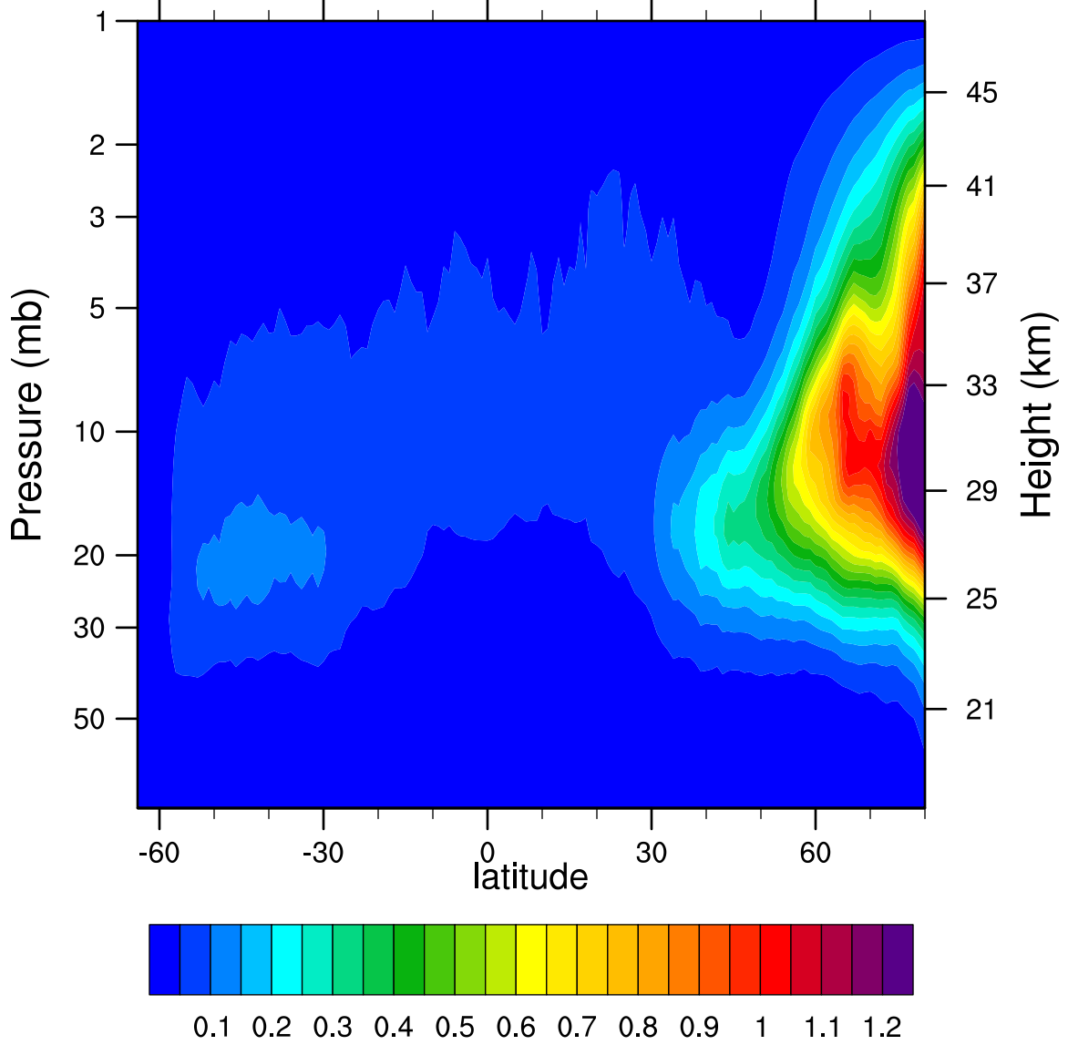
2007d318 N2O5_Ascending (ppbv)
