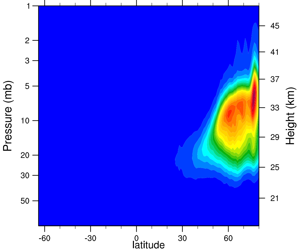
2007d012 N2O5_Ascending (ppbv)
