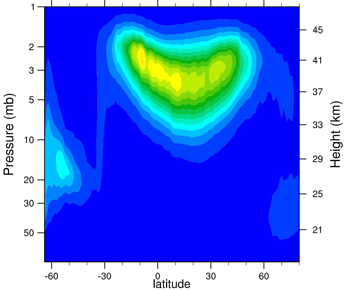
2005d090 N2O5_Ascending (ppbv)
