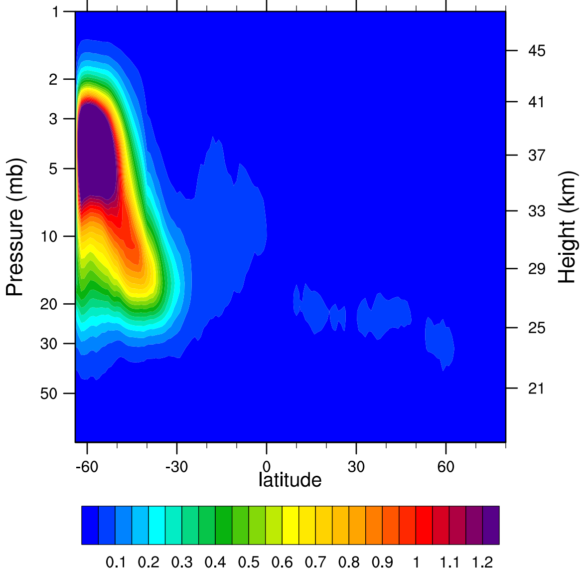
2007d153 N2O5_Ascending (ppbv)
