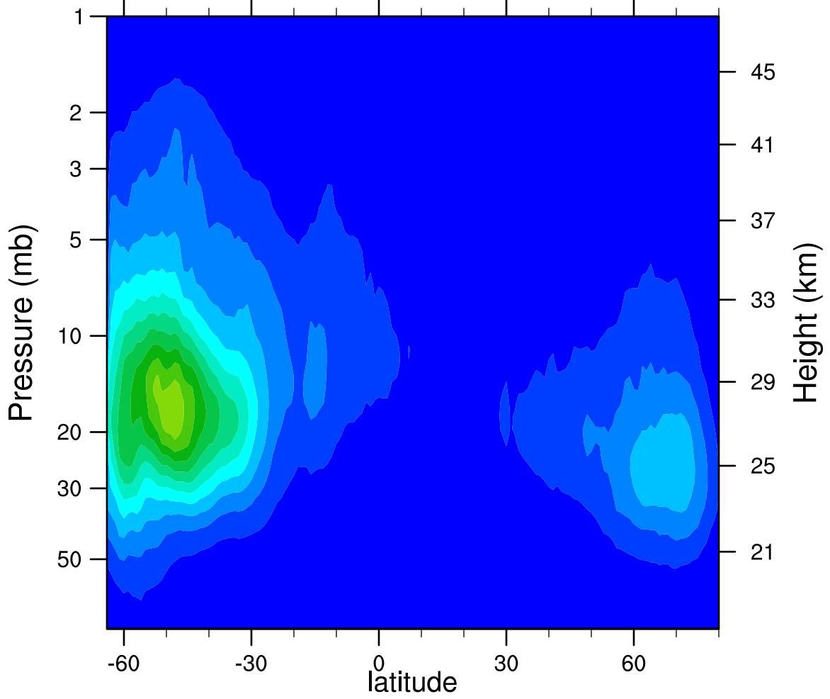
2007d247 N2O5_Ascending (ppbv)
