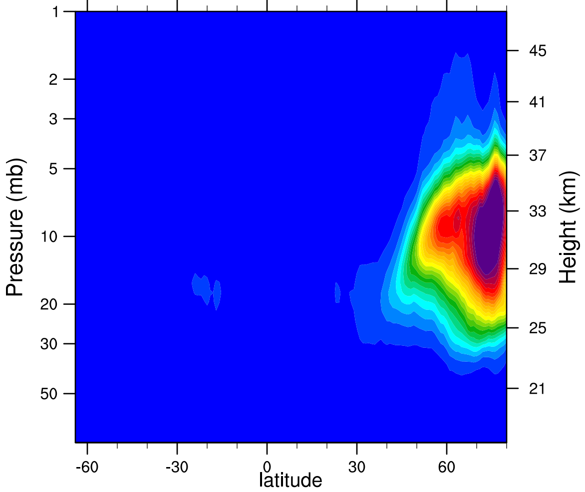
2007d001 N2O5_Ascending (ppbv)
