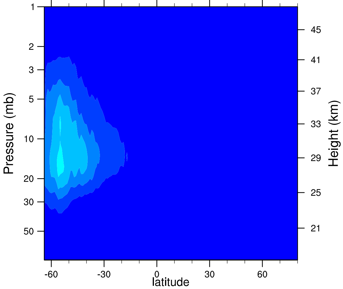
2007d198 N2O5_Ascending (ppbv)
