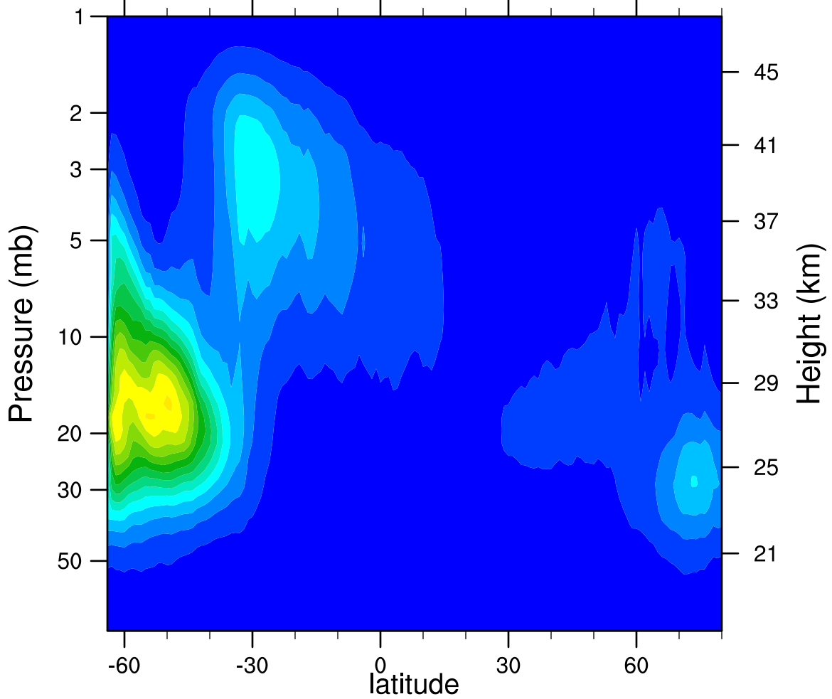
2007d098 N2O5_Ascending (ppbv)
