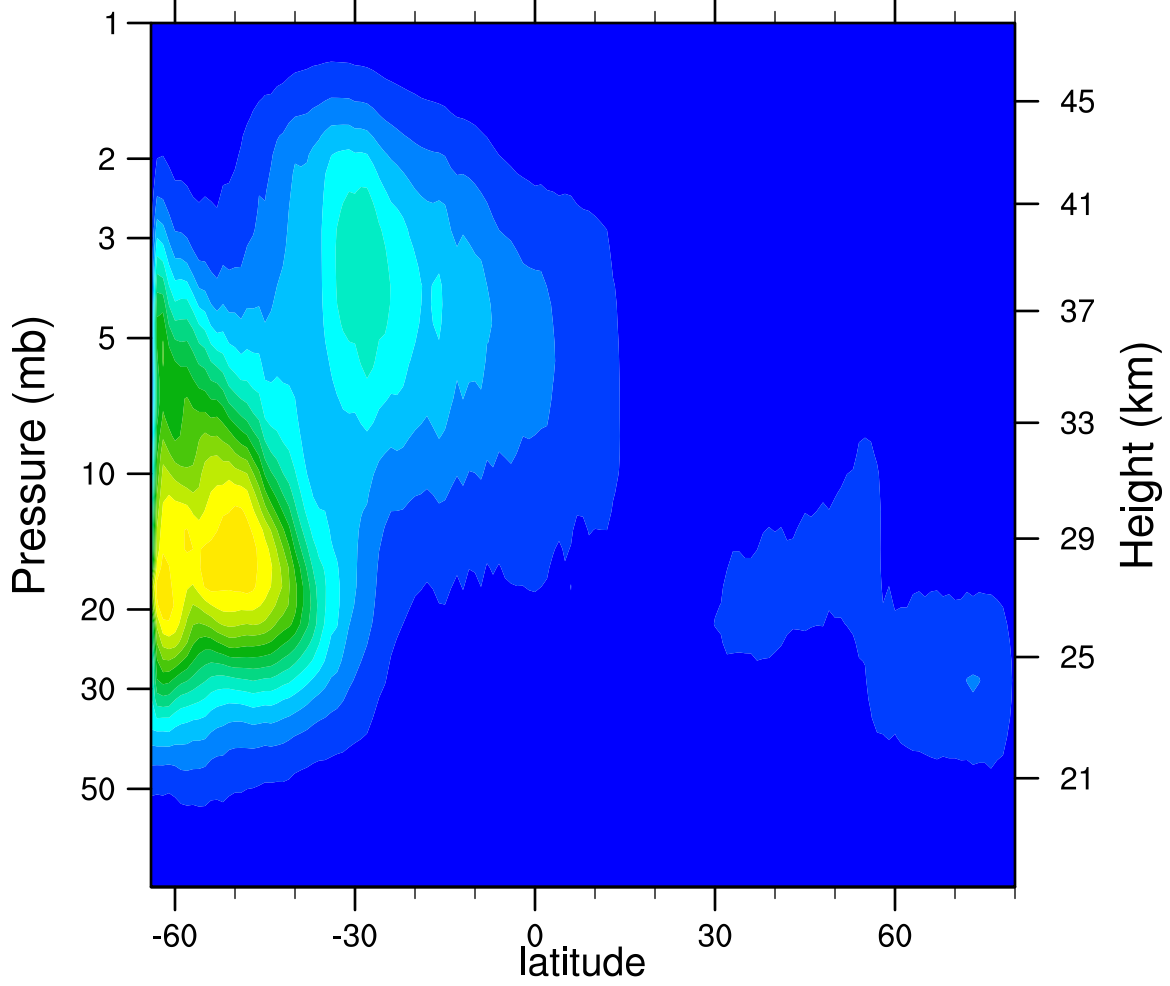
2007d108 N2O5_Ascending (ppbv)
