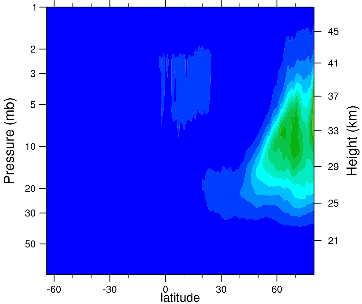
2007d047 N2O5_Ascending (ppbv)
