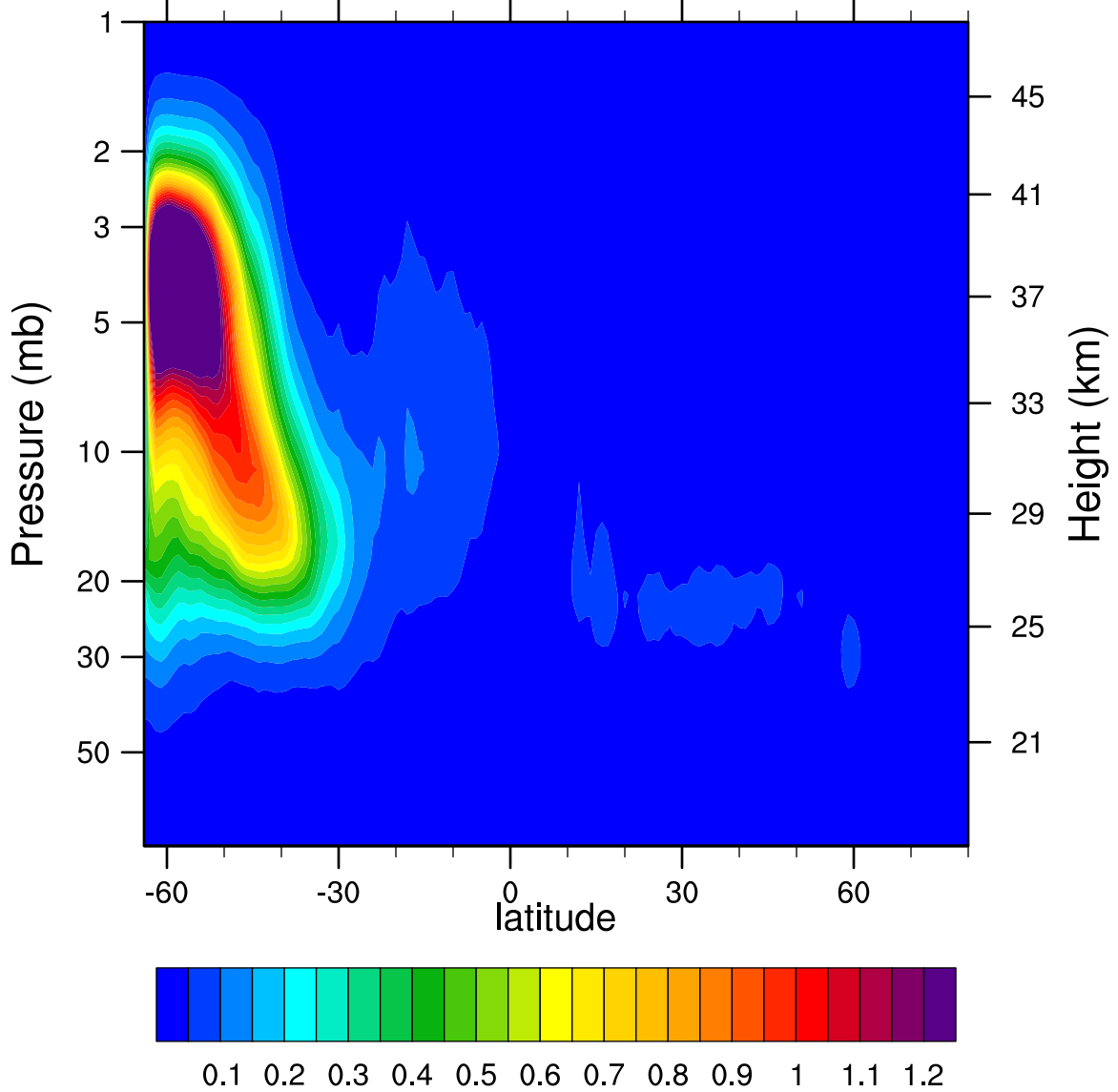
2007d147 N2O5_Ascending (ppbv)
