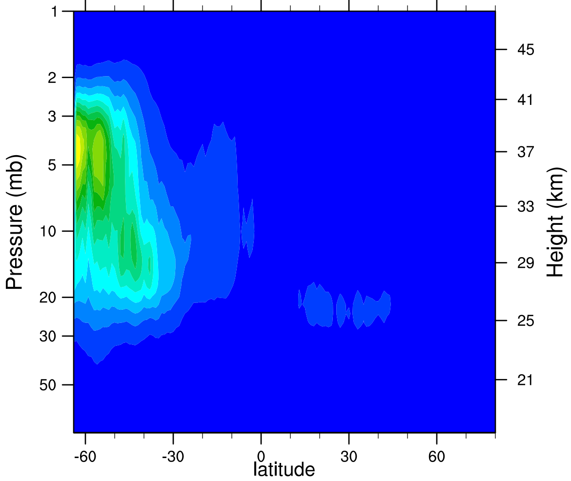
2007d163 N2O5_Ascending (ppbv)
