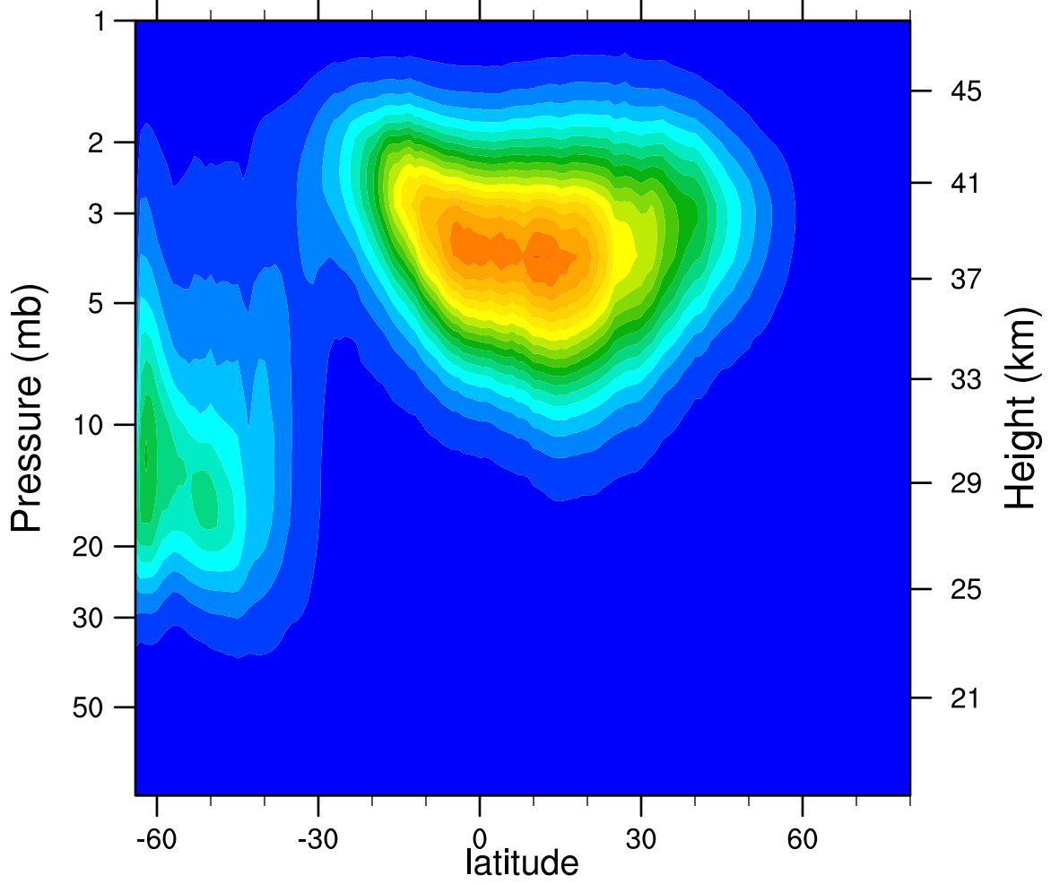
2005d125 N2O5_Ascending (ppbv)
