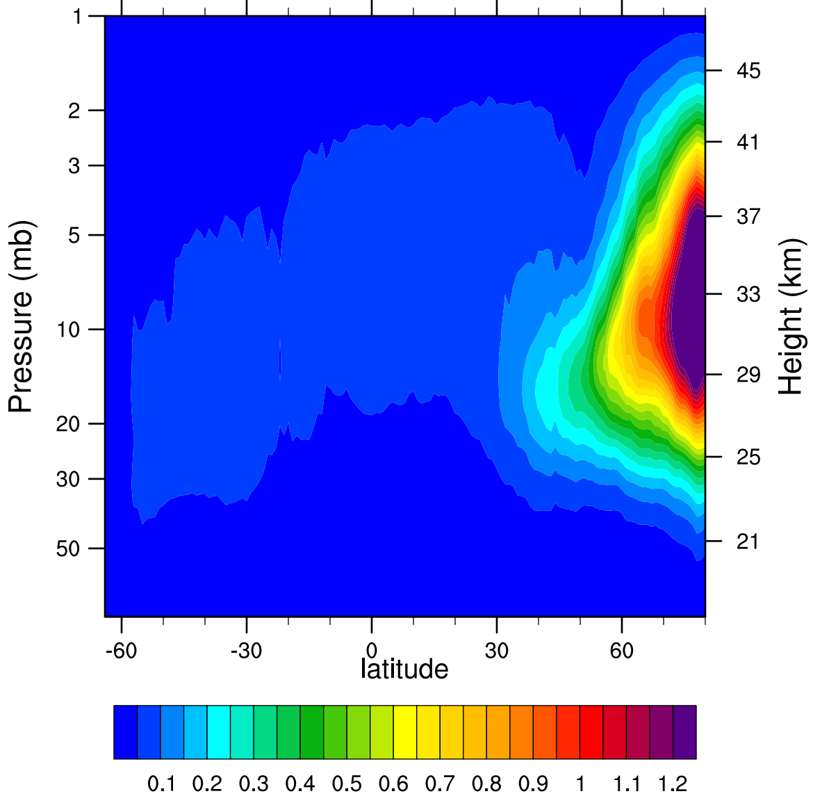
2007d328 N2O5_Ascending (ppbv)
