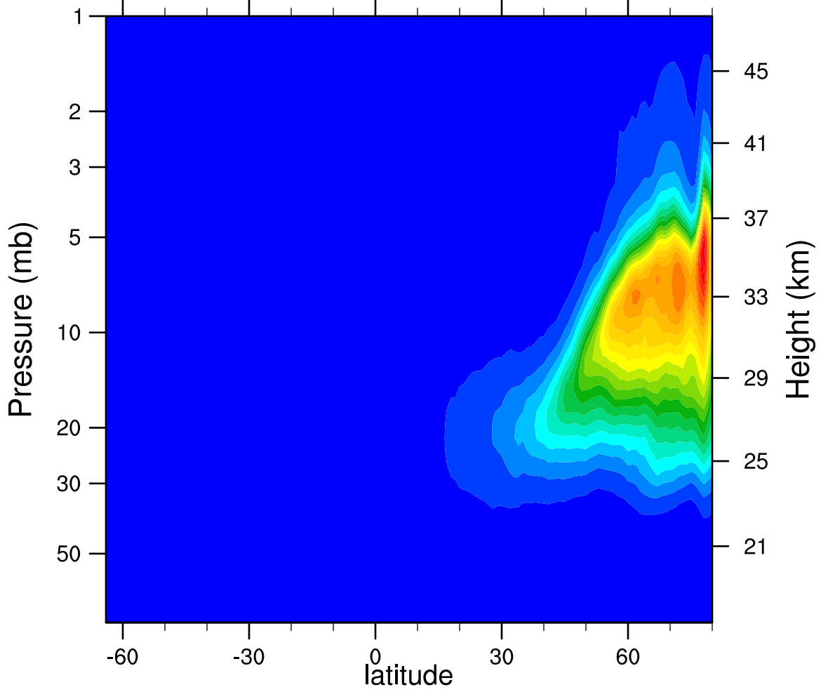
2007d023 N2O5_Ascending (ppbv)
