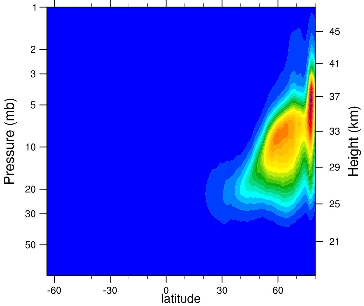
2007d017 N2O5_Ascending (ppbv)
