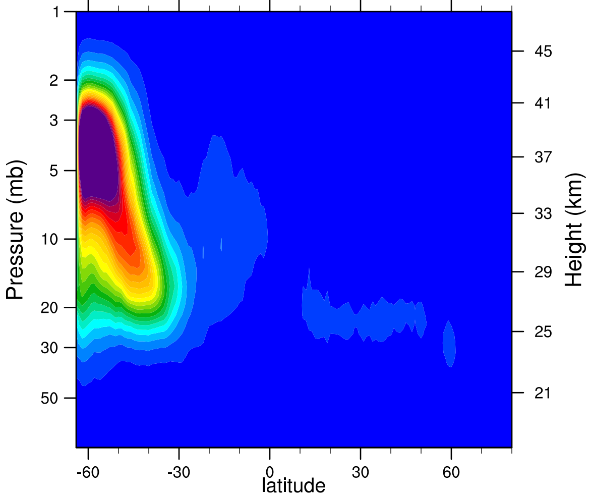
2007d149 N2O5_Ascending (ppbv)
