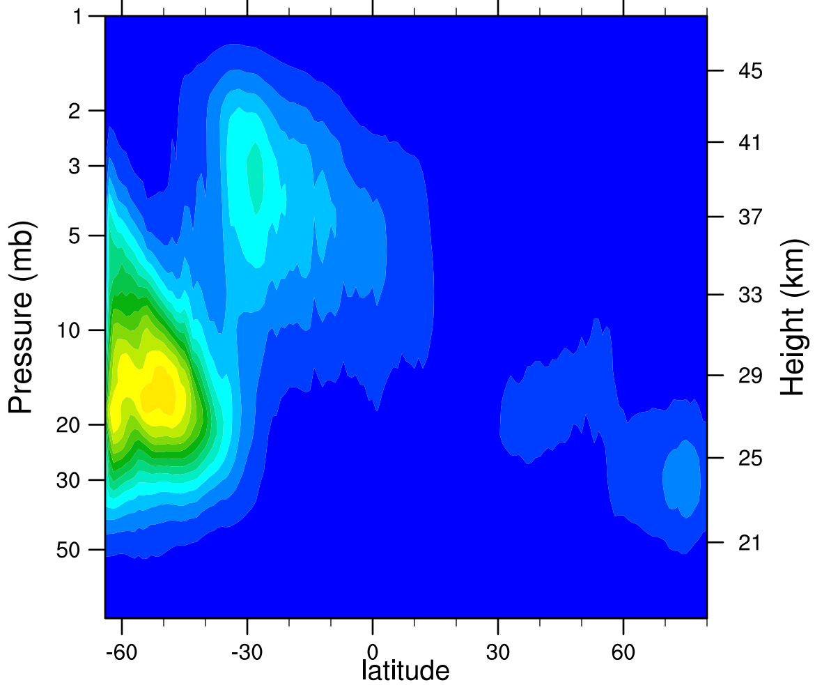
2007d104 N2O5_Ascending (ppbv)
