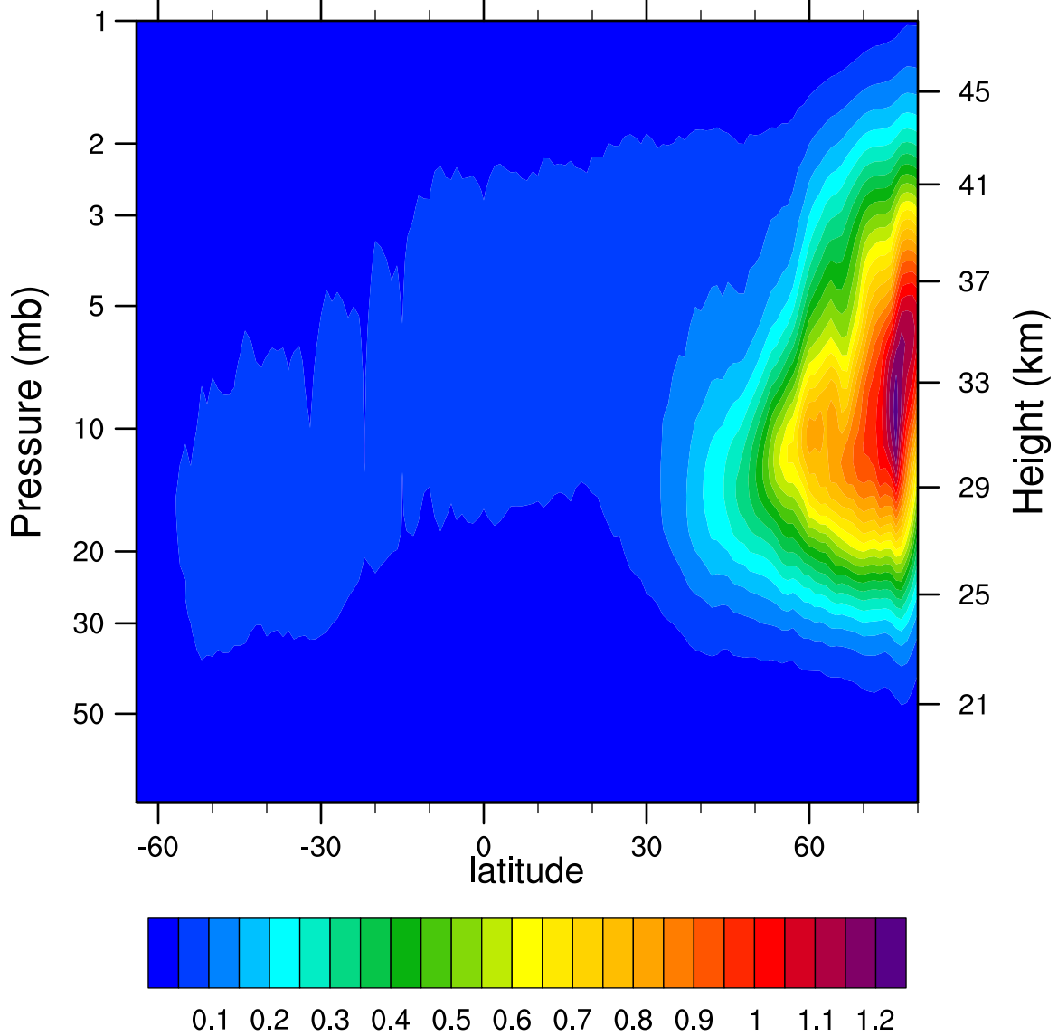
2007d338 N2O5_Ascending (ppbv)
