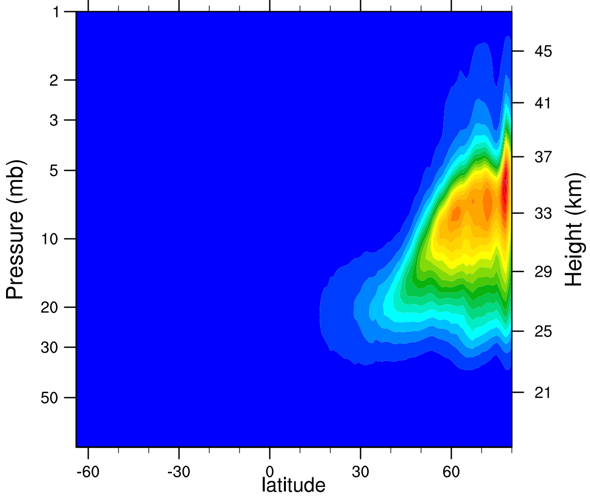
2007d022 N2O5_Ascending (ppbv)
