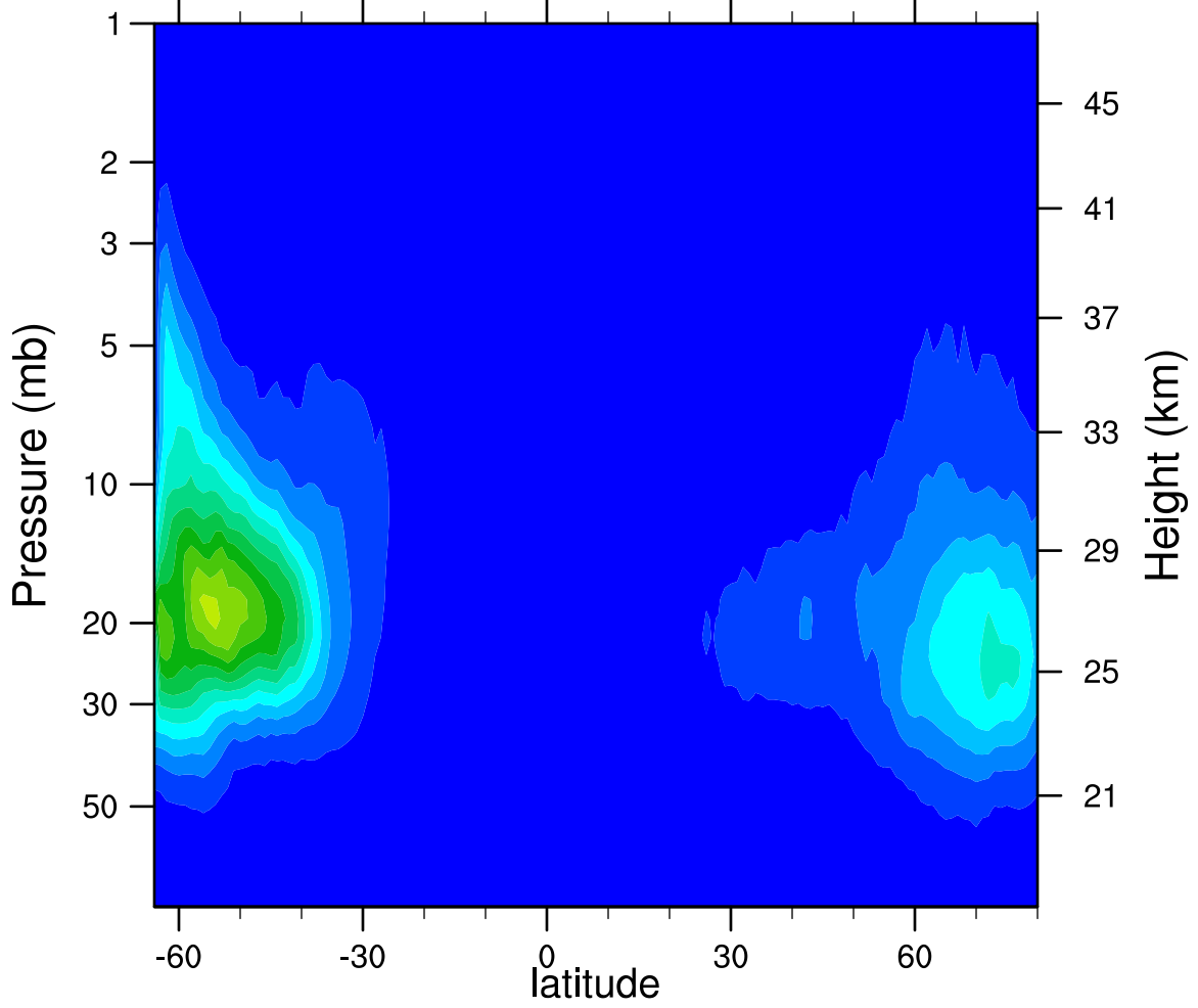
2007d082 N2O5_Ascending (ppbv)
