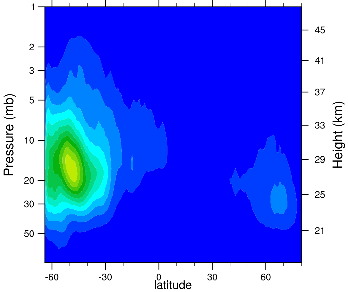
2007d240 N2O5_Ascending (ppbv)
