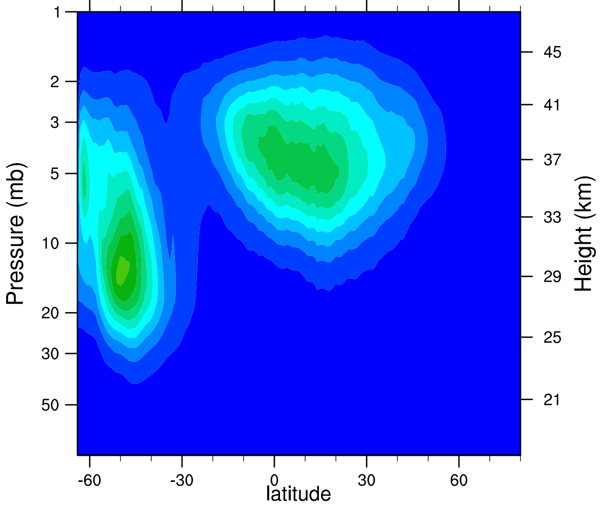
2005d176 N2O5_Ascending (ppbv)
