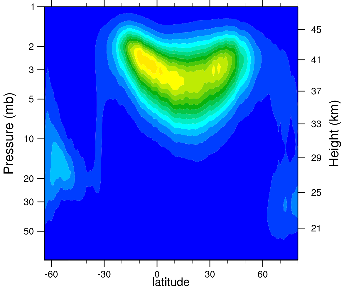
2005d086 N2O5_Ascending (ppbv)
