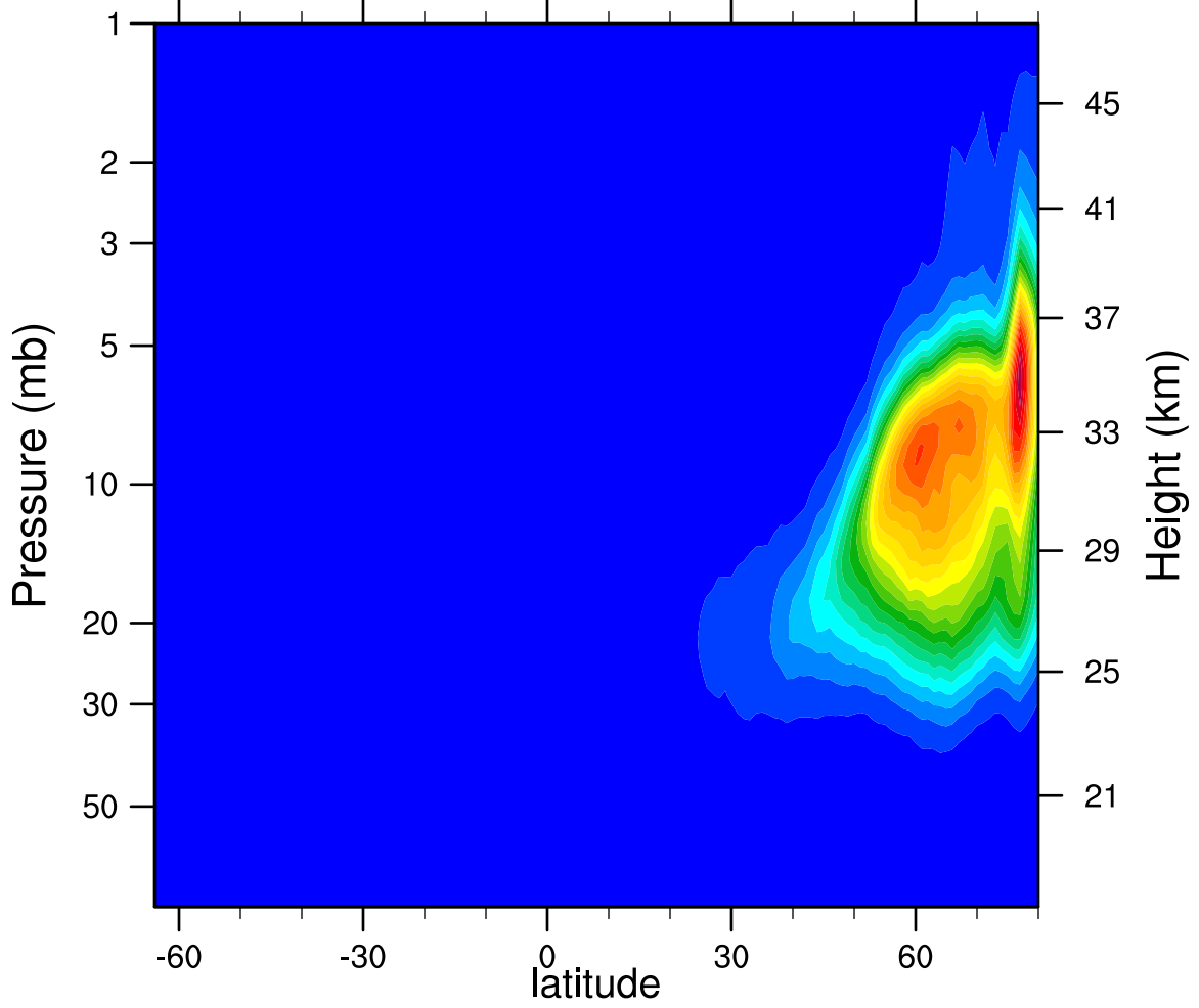
2007d013 N2O5_Ascending (ppbv)
