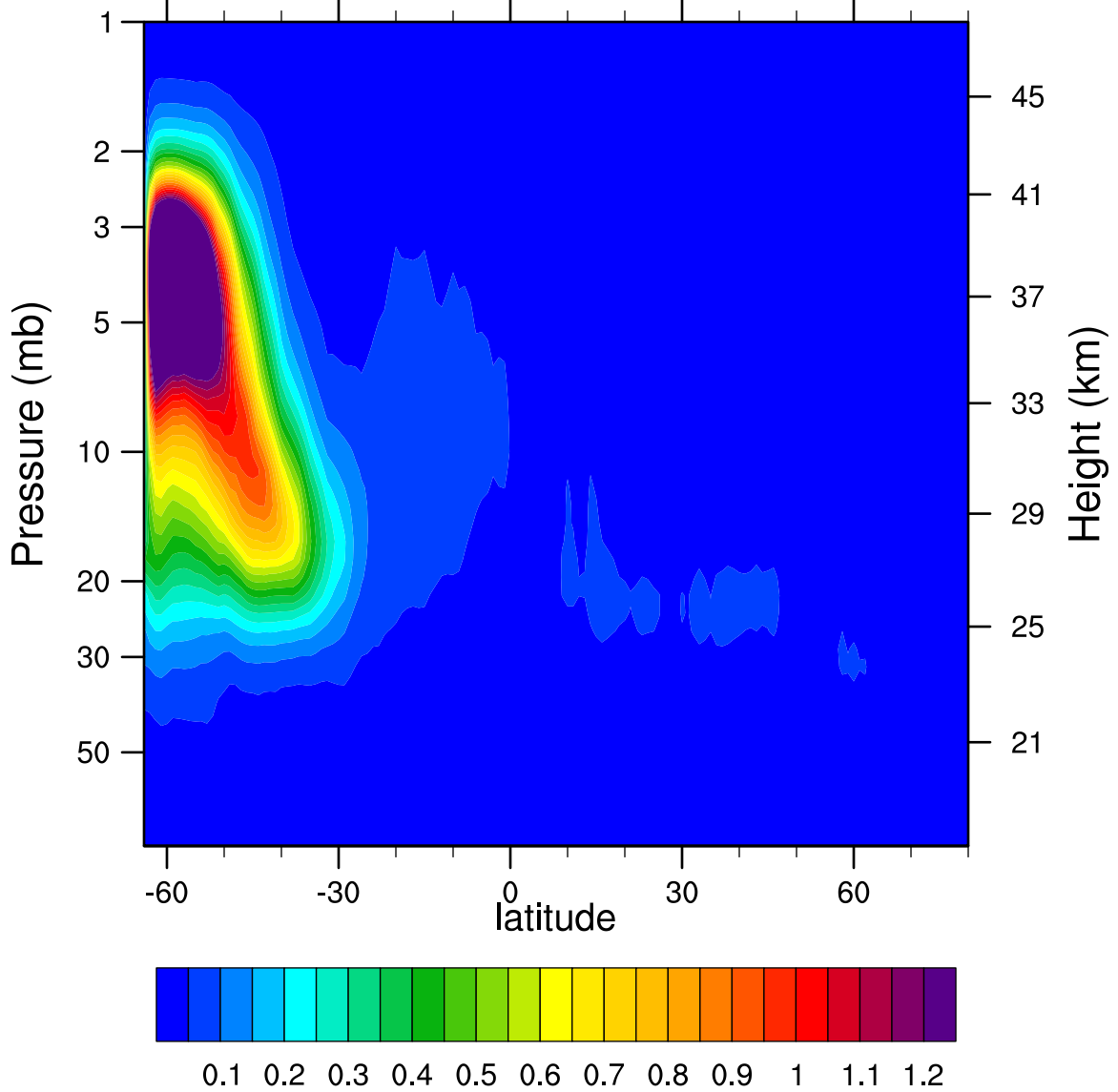
2007d155 N2O5_Ascending (ppbv)
