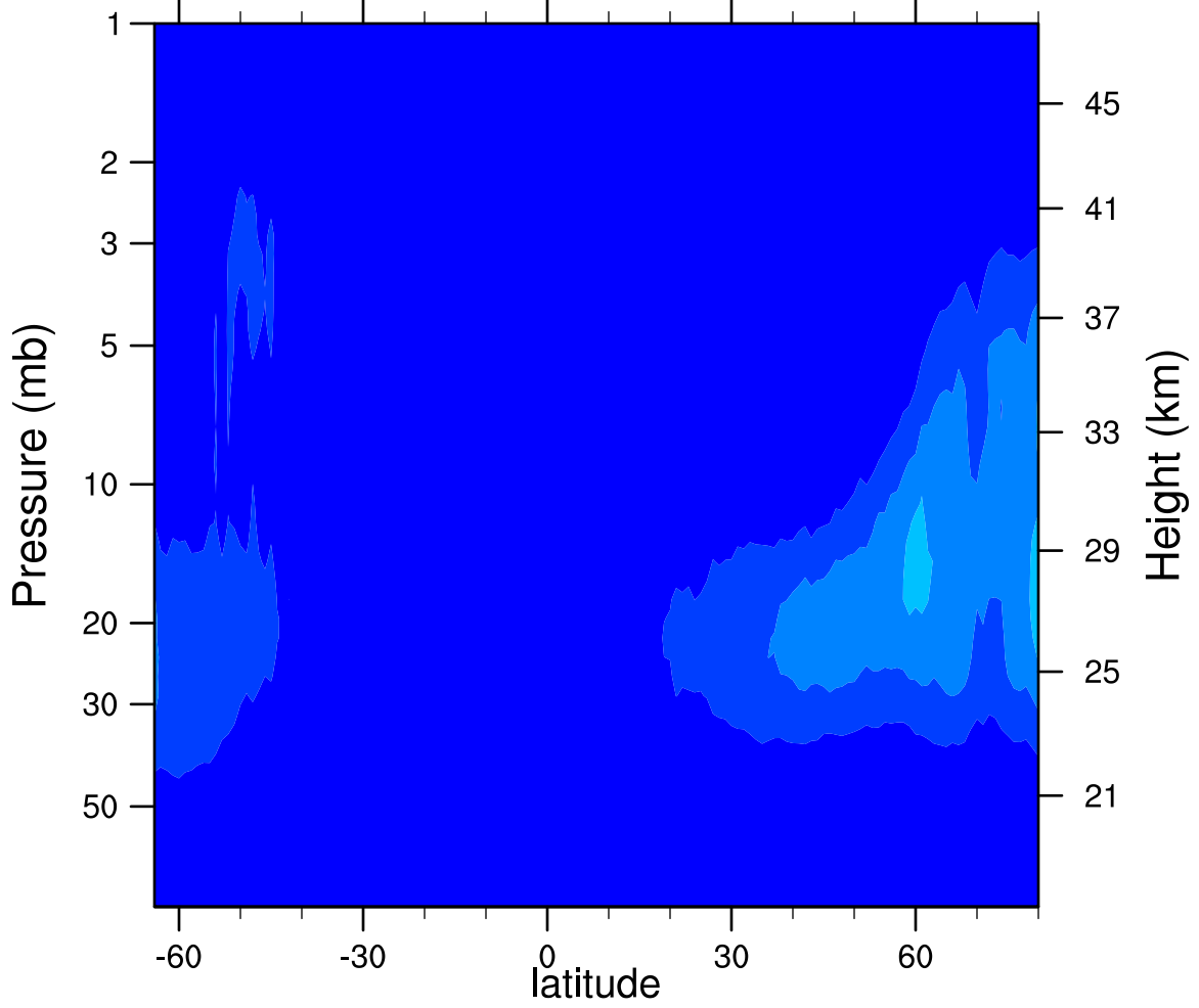
2007d074 N2O5_Ascending (ppbv)
