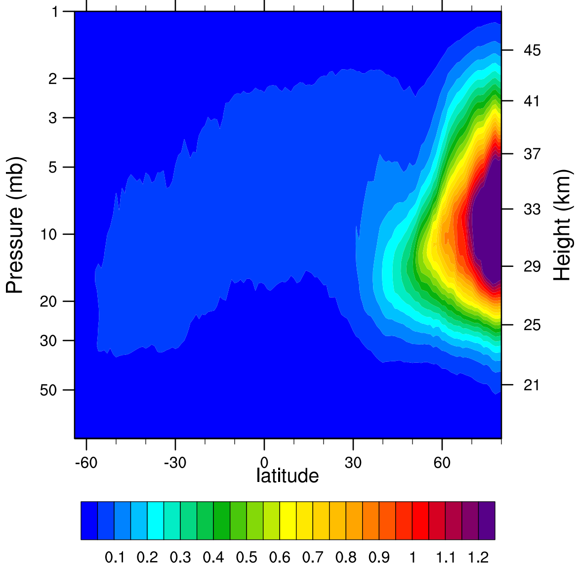
2007d334 N2O5_Ascending (ppbv)
