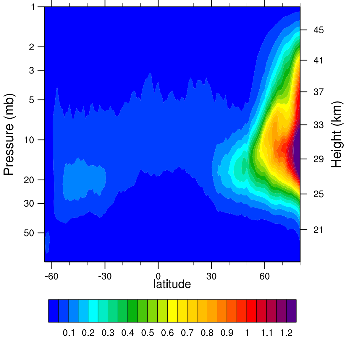
2007d315 N2O5_Ascending (ppbv)
