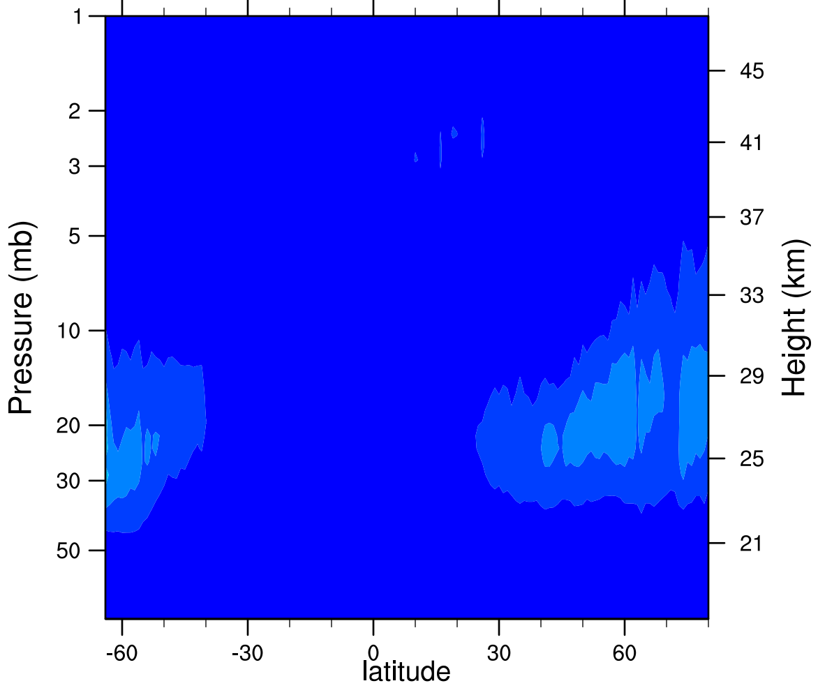
2007d076 N2O5_Ascending (ppbv)
