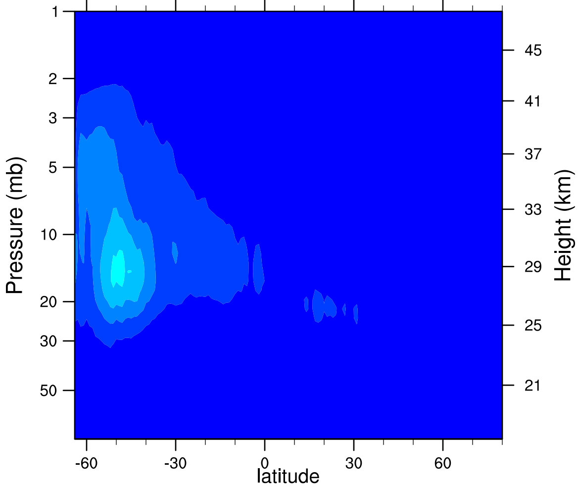
2007d183 N2O5_Ascending (ppbv)
