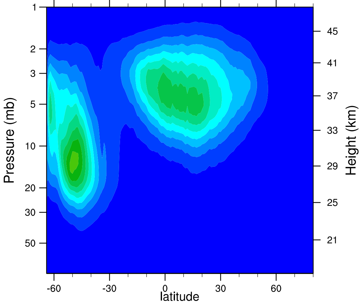
2005d175 N2O5_Ascending (ppbv)
