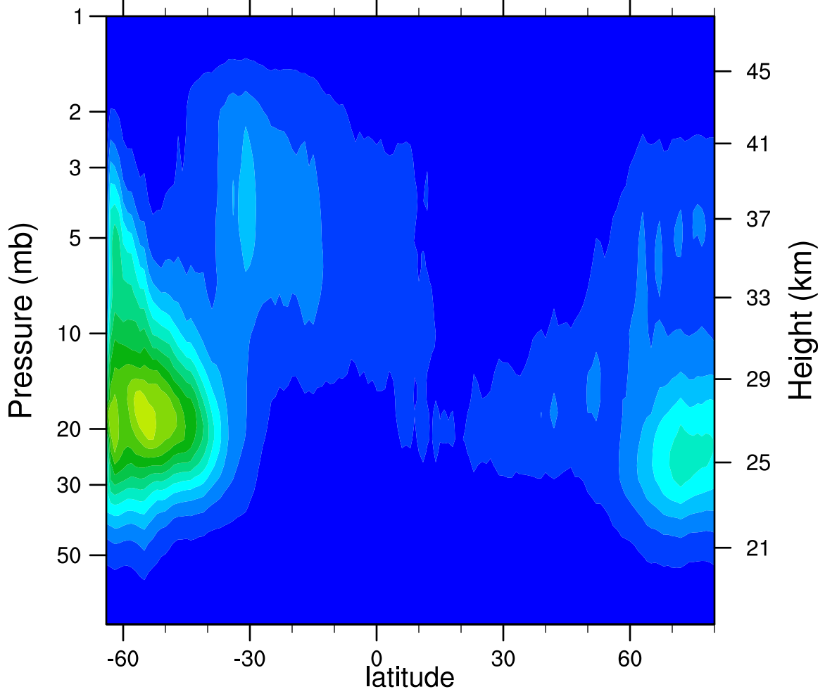
2007d086 N2O5_Ascending (ppbv)
