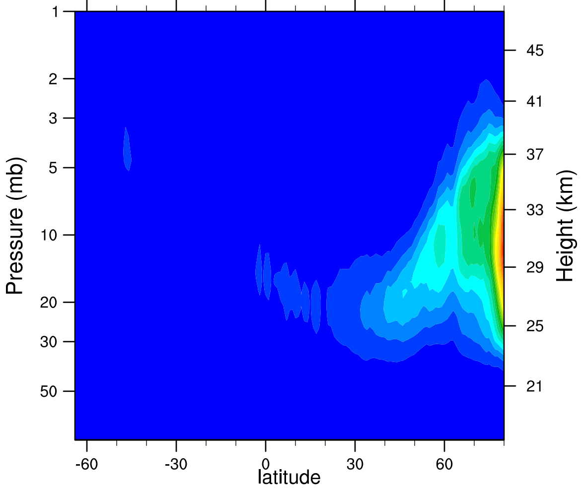
2007d053 N2O5_Ascending (ppbv)
