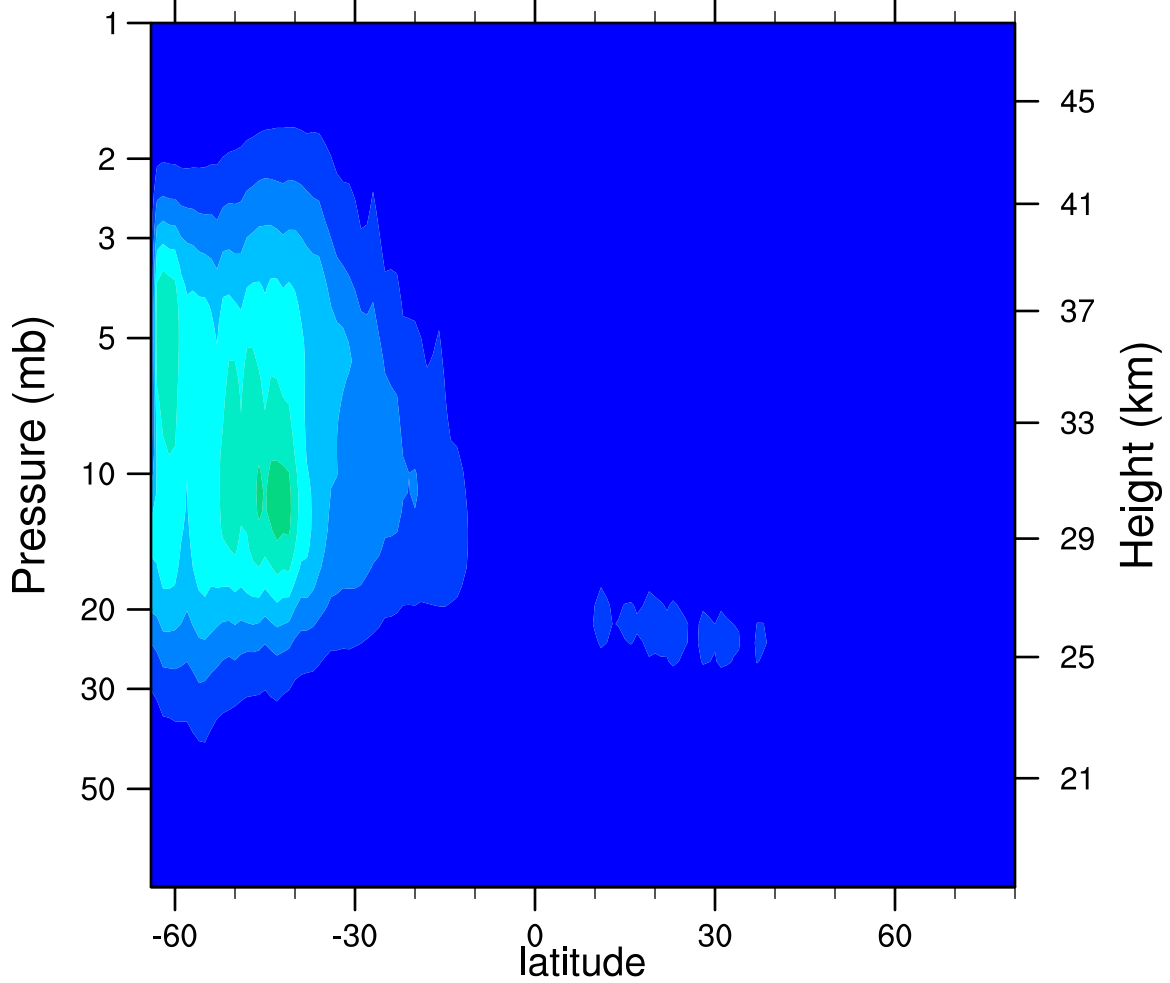
2007d167 N2O5_Ascending (ppbv)
