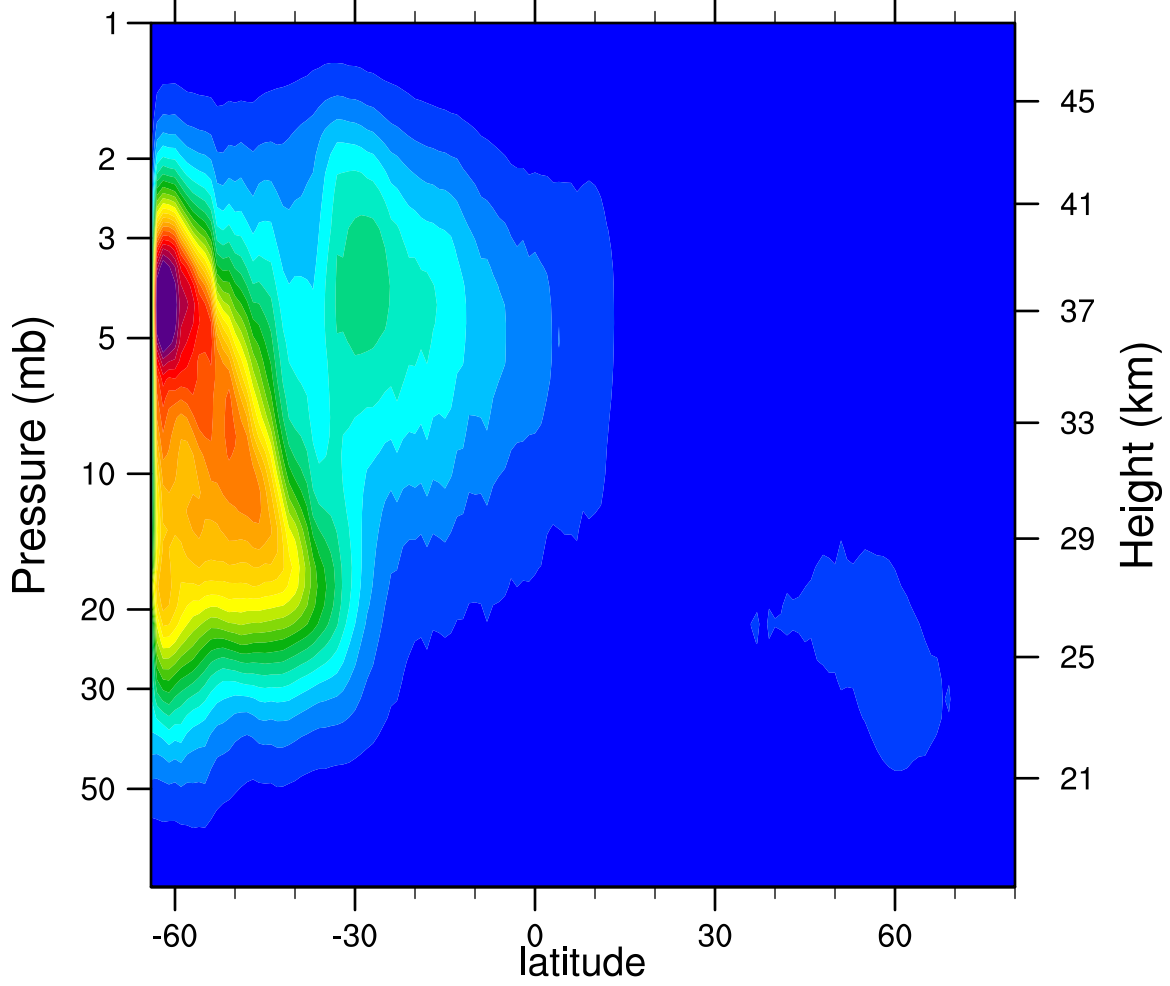
2007d125 N2O5_Ascending (ppbv)
