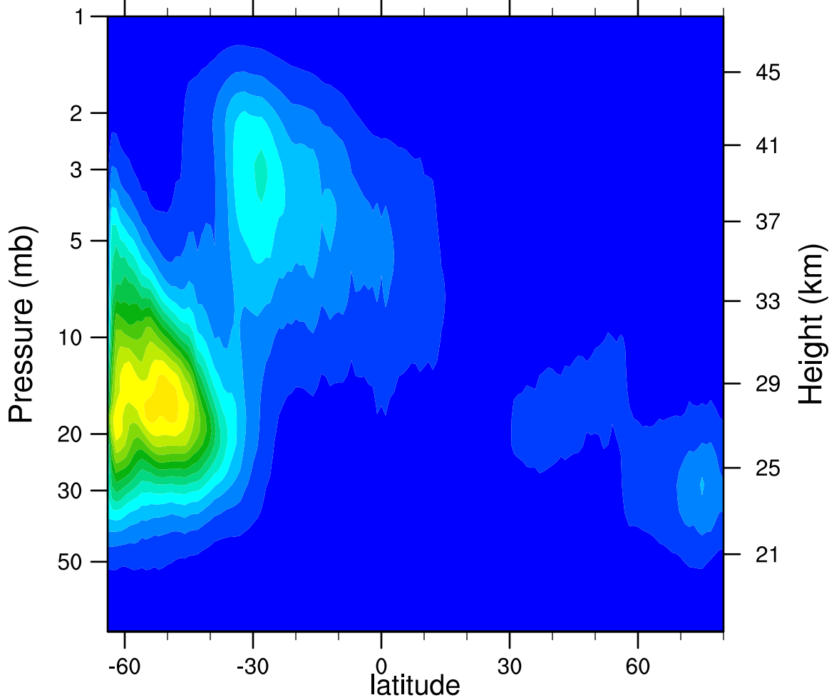
2007d103 N2O5_Ascending (ppbv)
