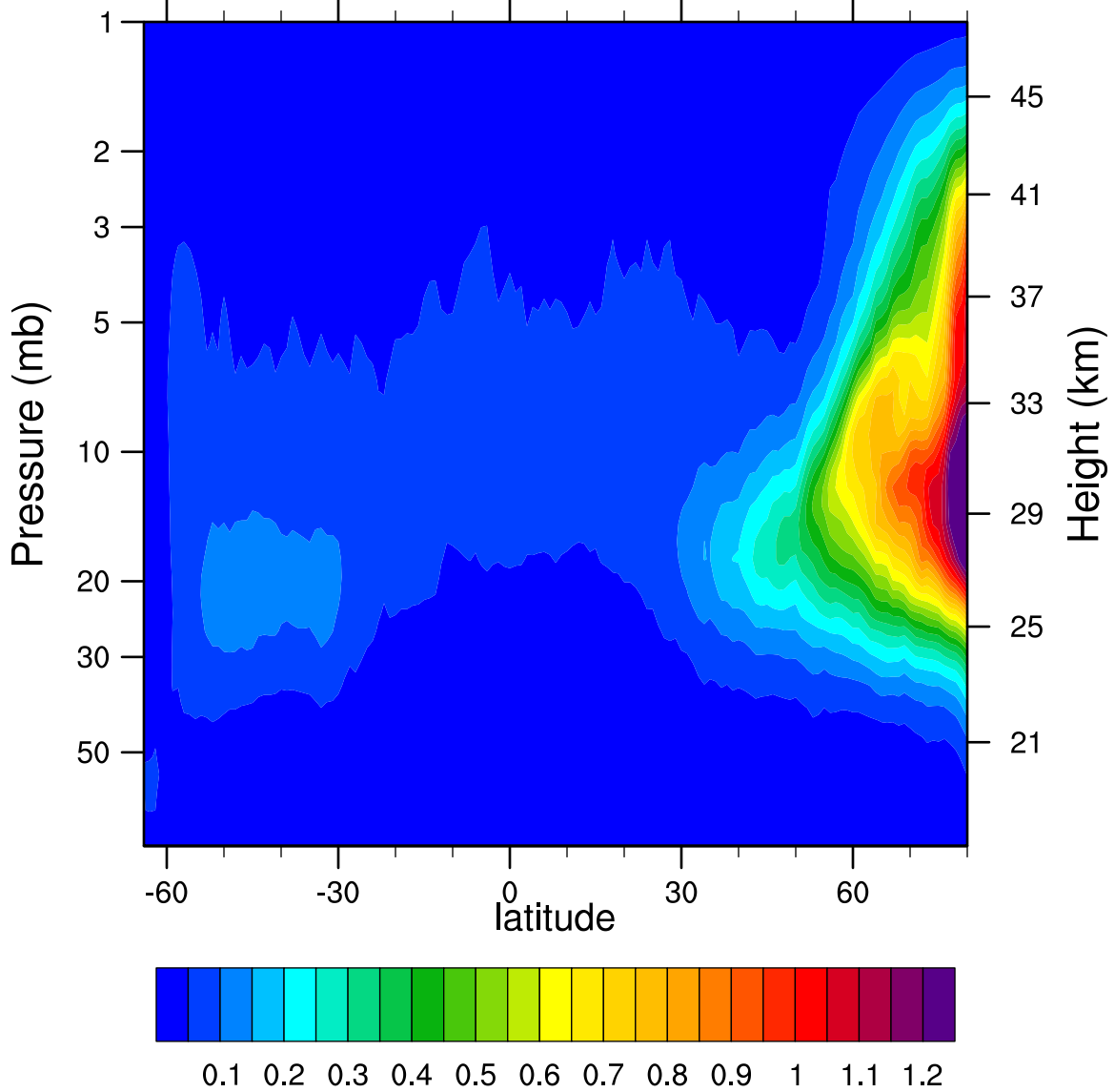
2007d314 N2O5_Ascending (ppbv)
