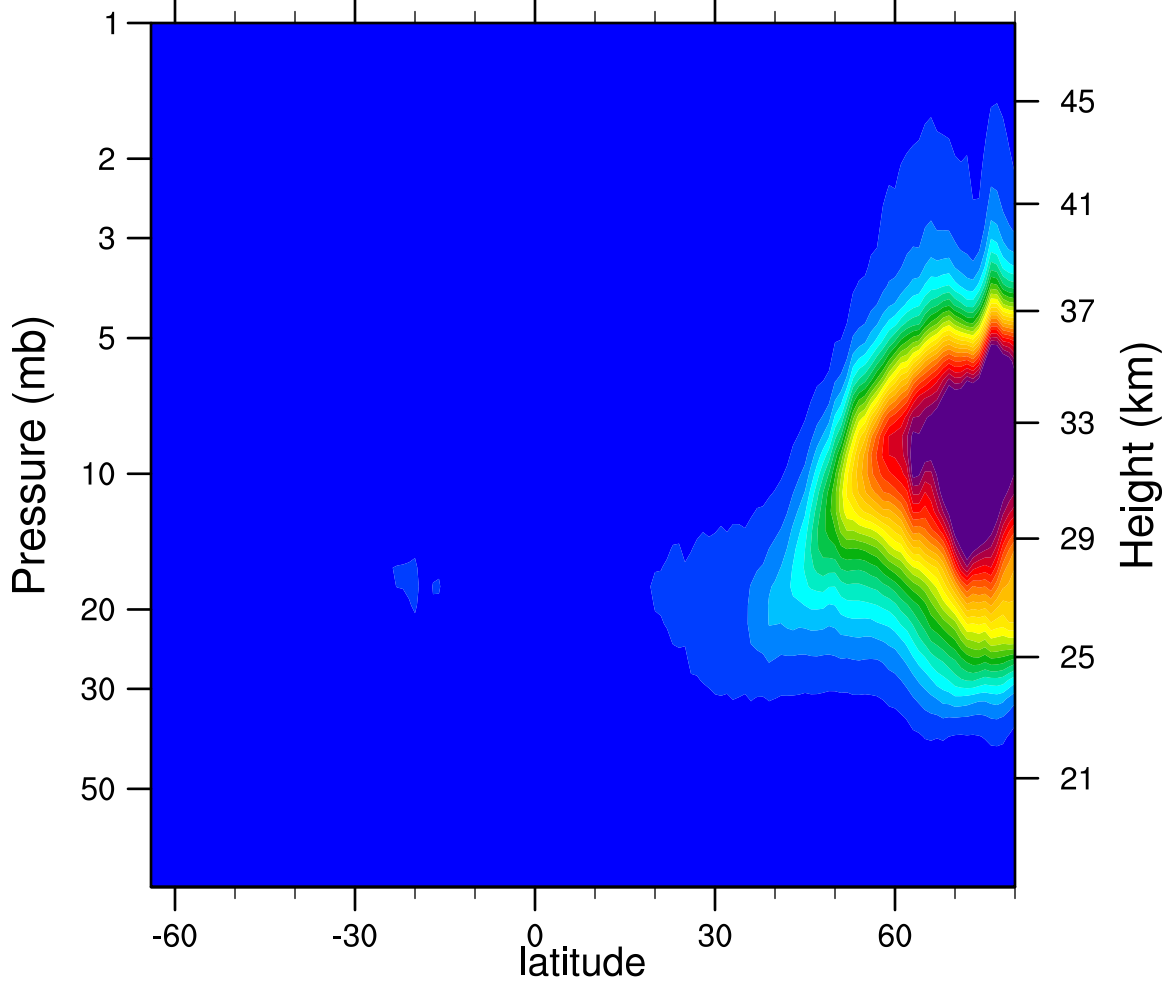
2007d005 N2O5_Ascending (ppbv)
