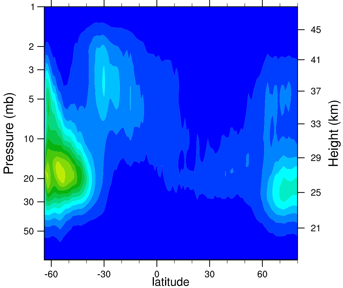
2007d087 N2O5_Ascending (ppbv)
