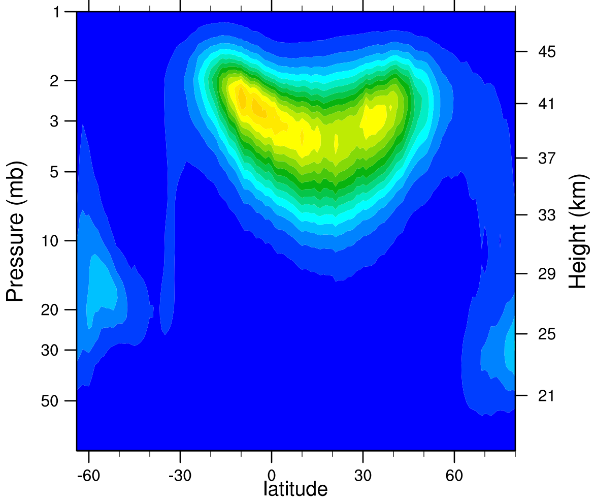
2005d084 N2O5_Ascending (ppbv)
