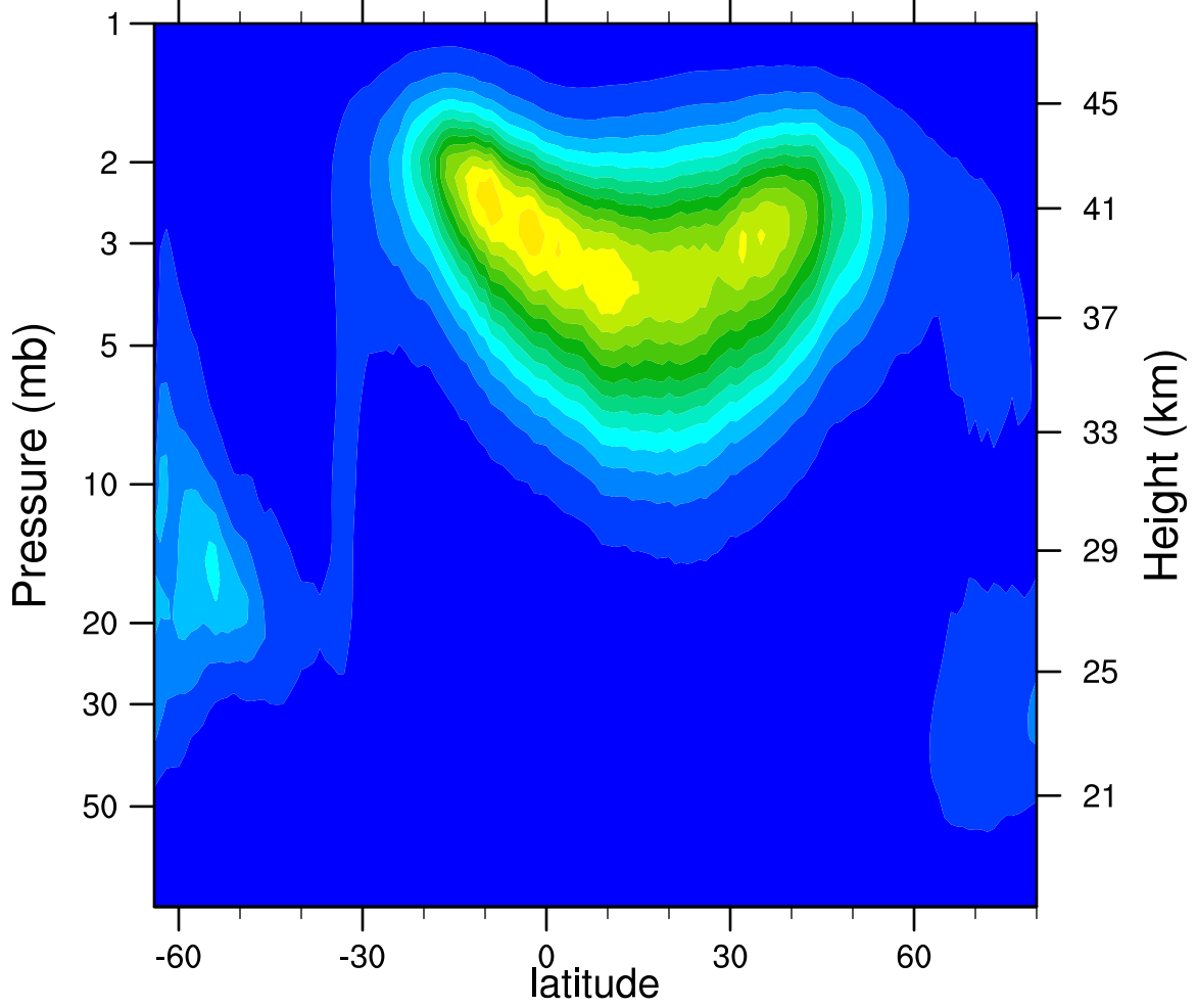
2005d087 N2O5_Ascending (ppbv)
