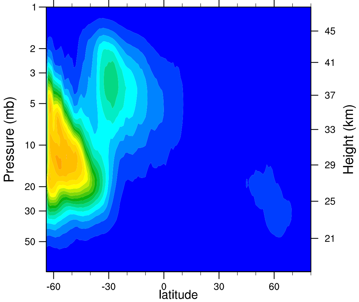
2007d120 N2O5_Ascending (ppbv)
