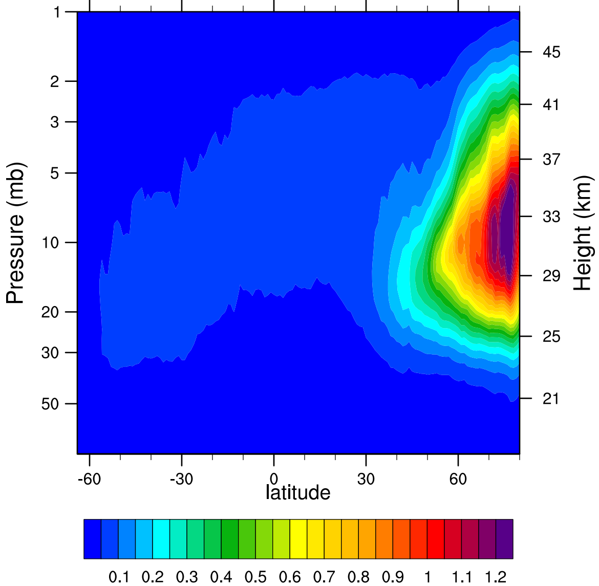
2007d336 N2O5_Ascending (ppbv)
