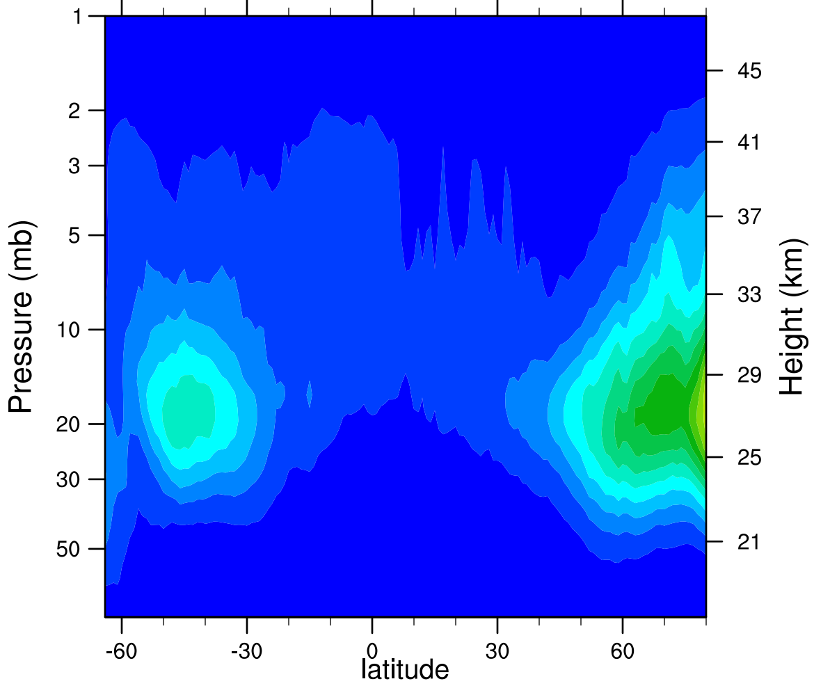
2007d275 N2O5_Ascending (ppbv)
