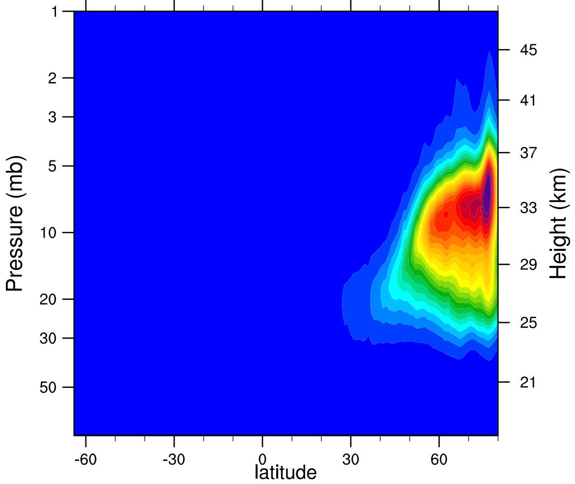
2007d009 N2O5_Ascending (ppbv)
