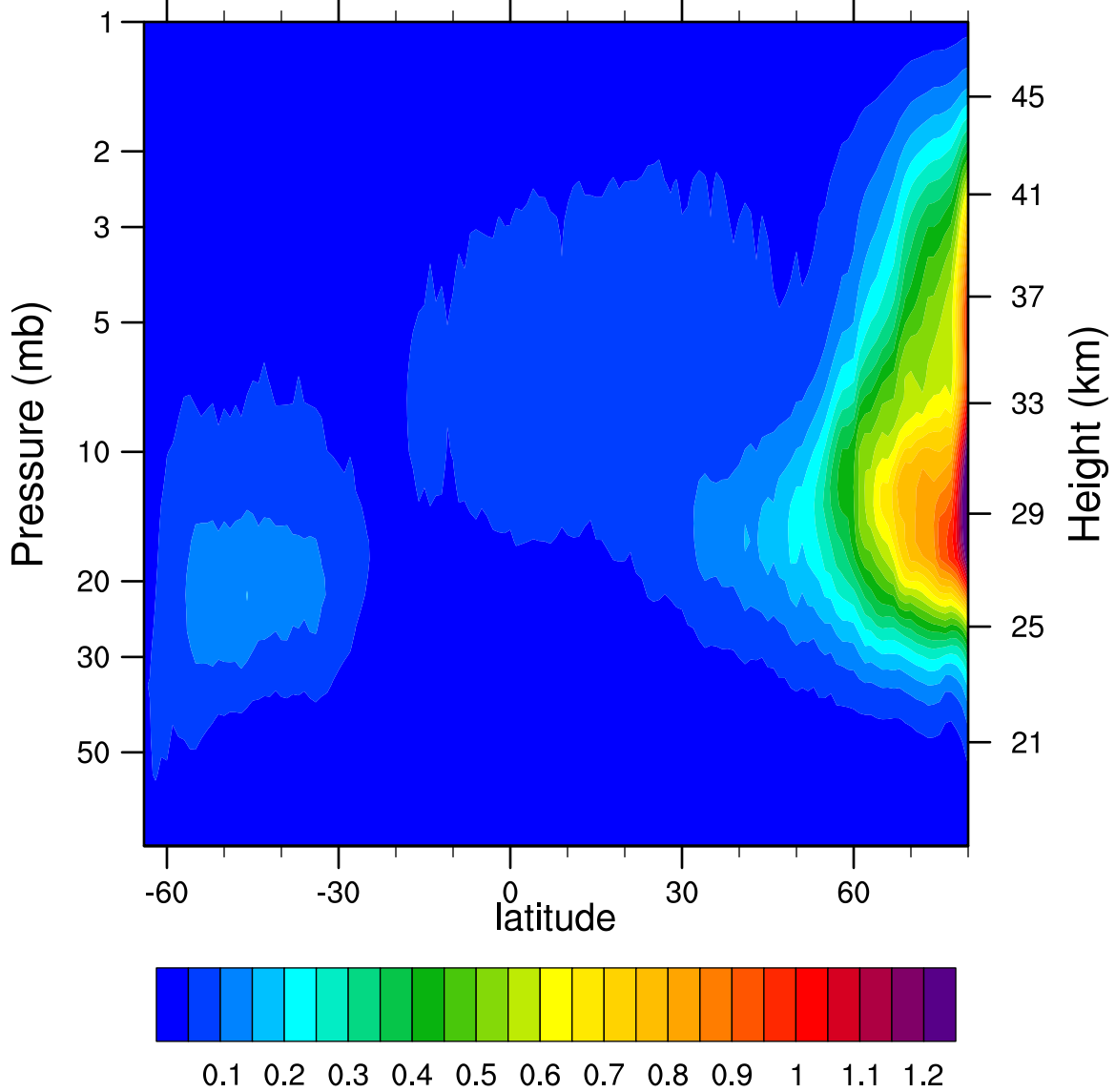
2007d310 N2O5_Ascending (ppbv)
