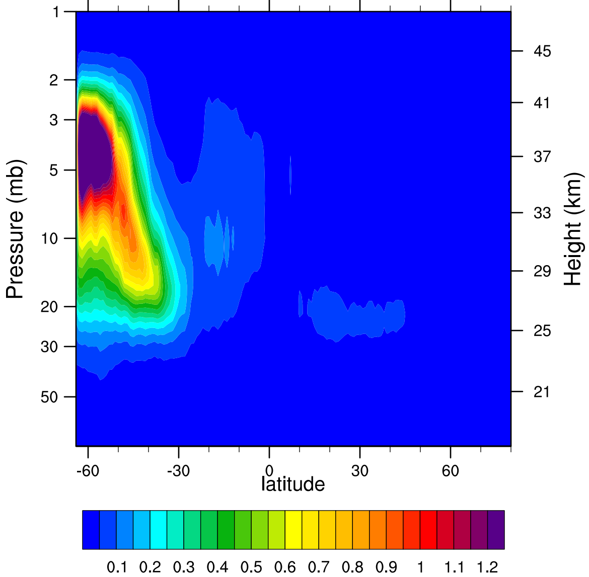
2007d161 N2O5_Ascending (ppbv)
