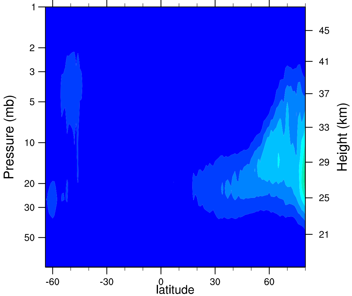
2007d066 N2O5_Ascending (ppbv)
