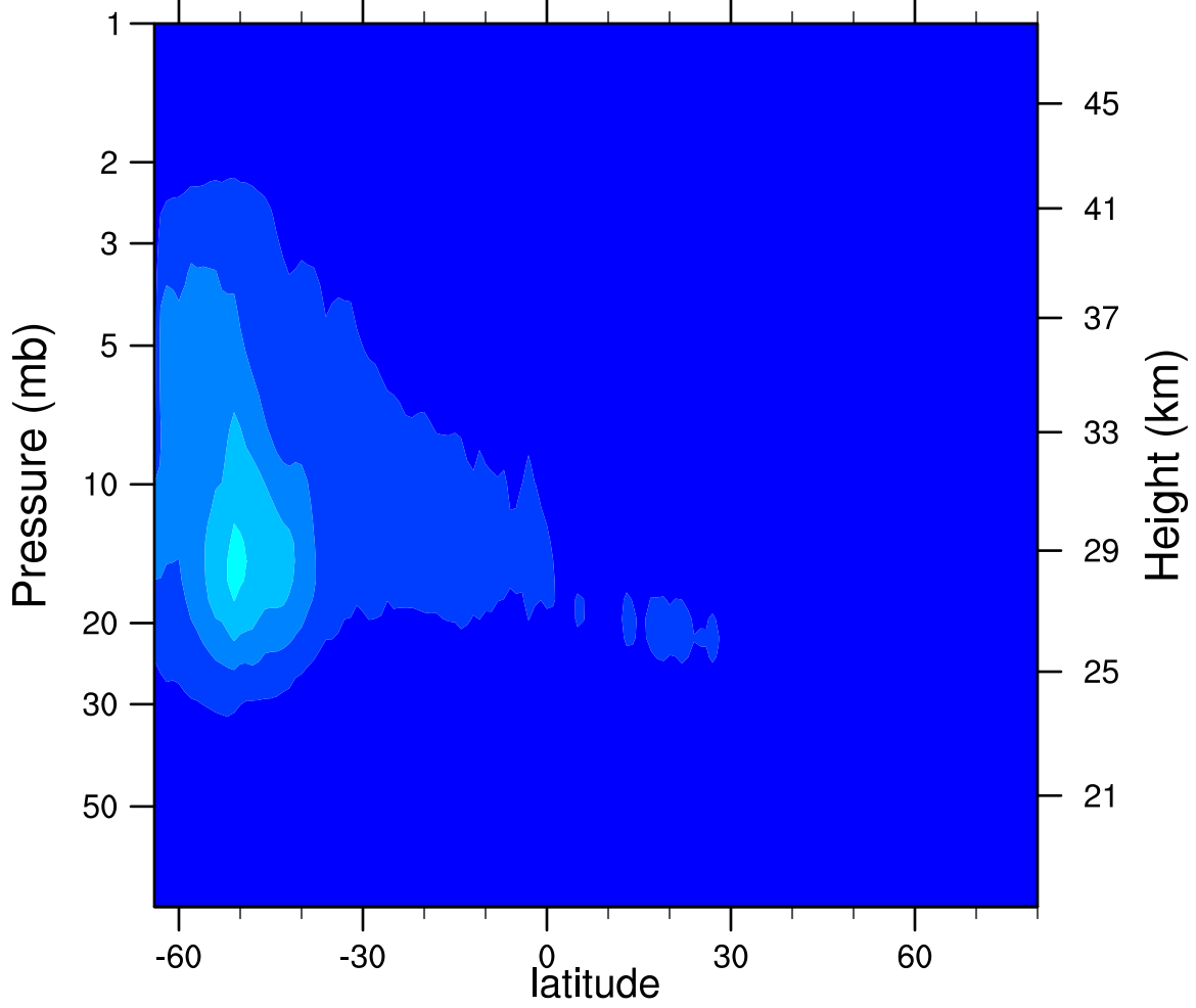
2007d185 N2O5_Ascending (ppbv)
