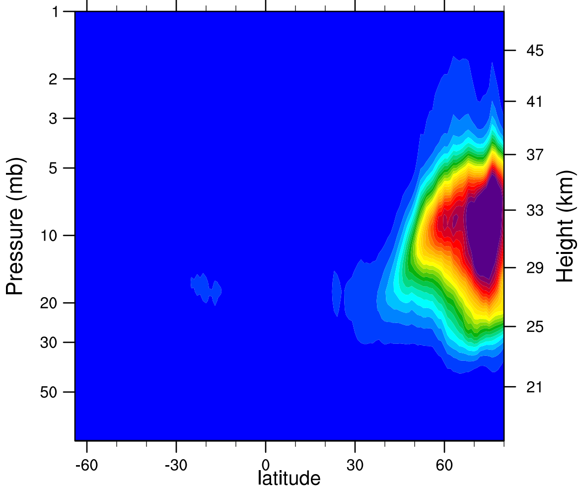
2007d002 N2O5_Ascending (ppbv)
