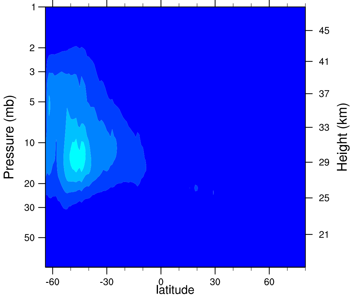
2007d179 N2O5_Ascending (ppbv)
