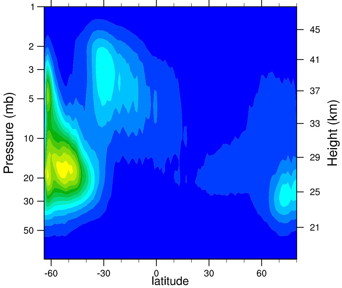
2007d095 N2O5_Ascending (ppbv)
