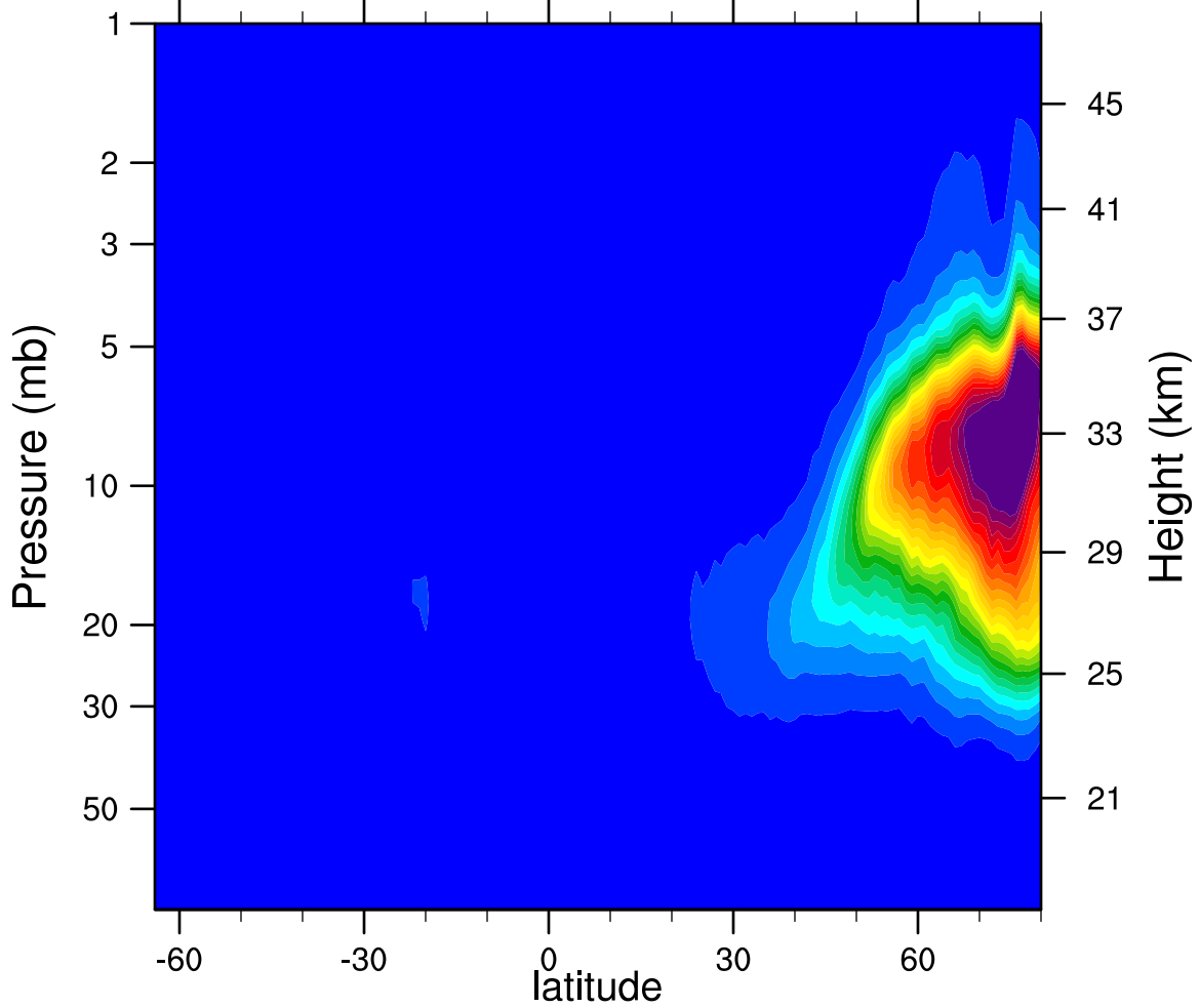
2007d007 N2O5_Ascending (ppbv)
