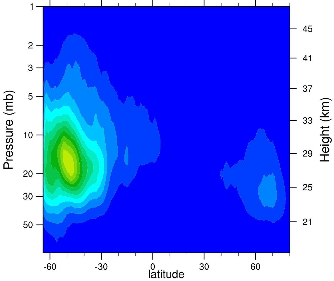
2007d241 N2O5_Ascending (ppbv)
