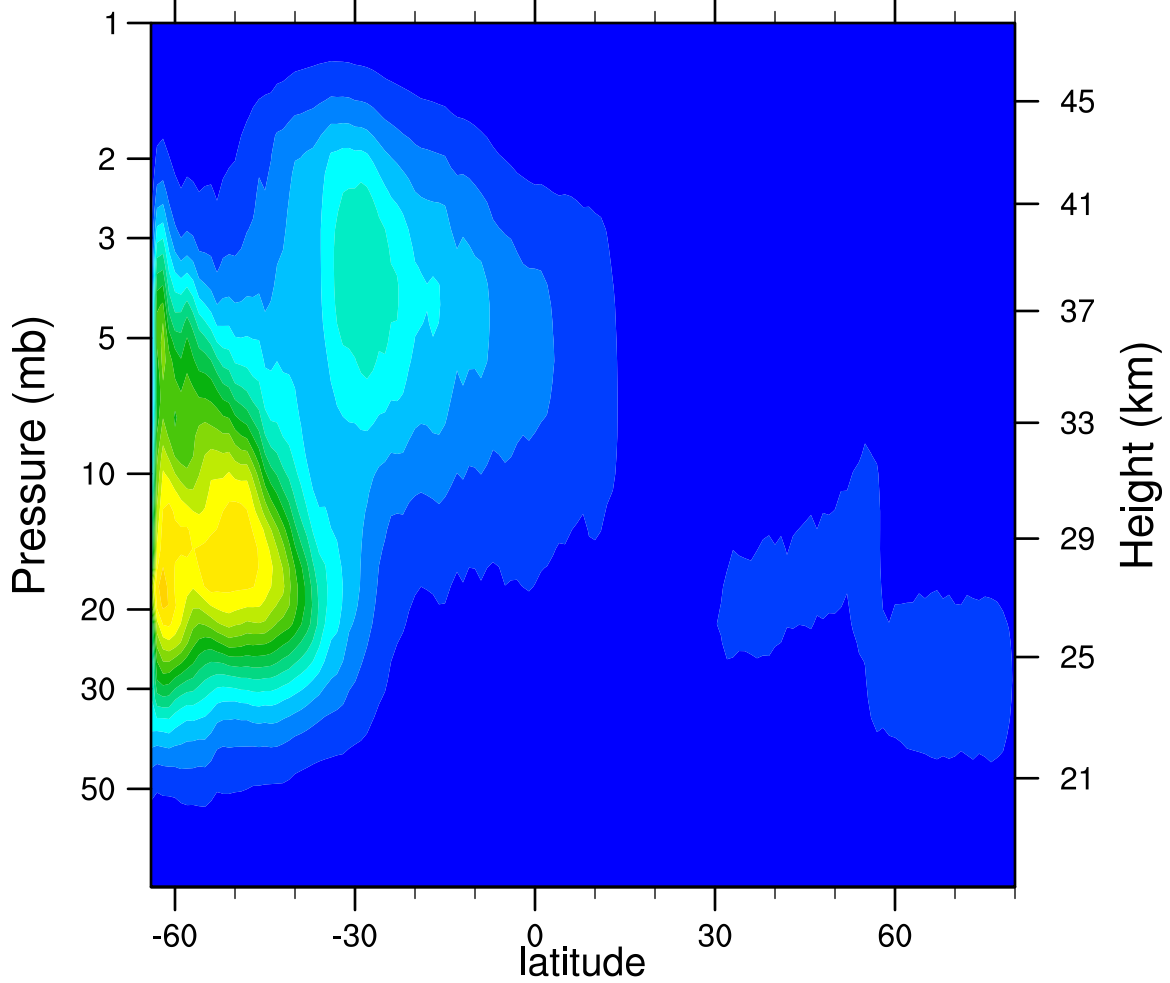
2007d109 N2O5_Ascending (ppbv)
