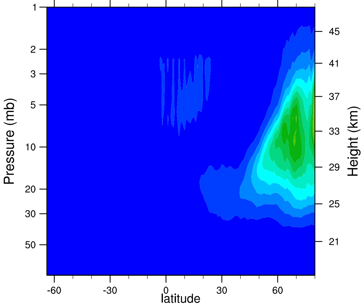
2007d046 N2O5_Ascending (ppbv)
