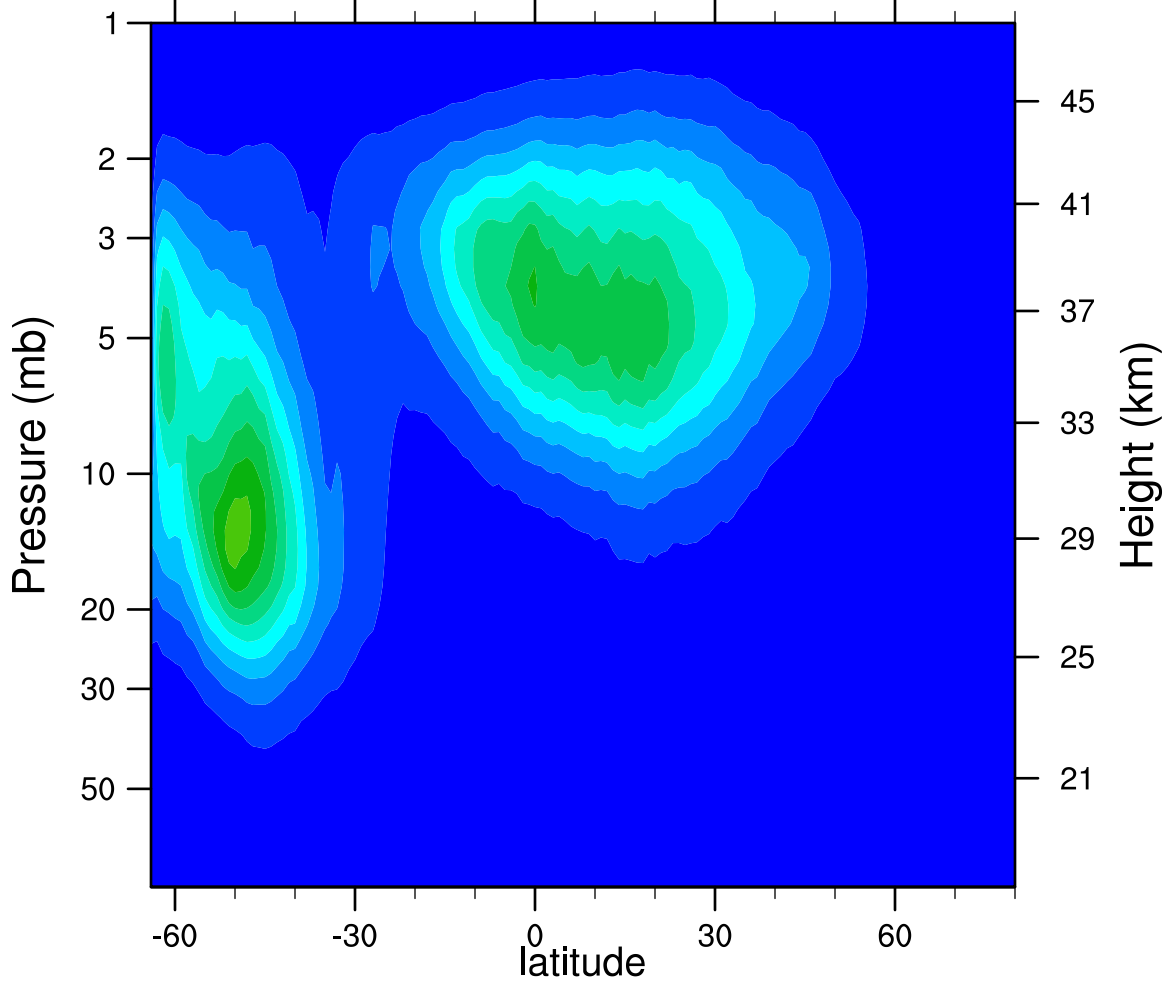
2005d173 N2O5_Ascending (ppbv)
