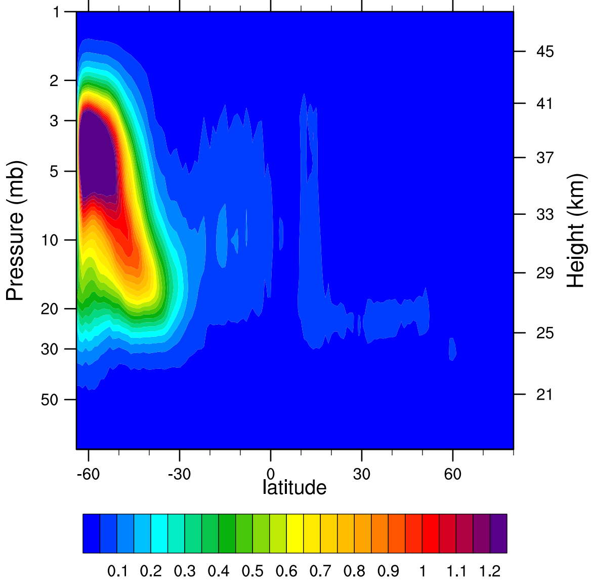
2007d144 N2O5_Ascending (ppbv)
