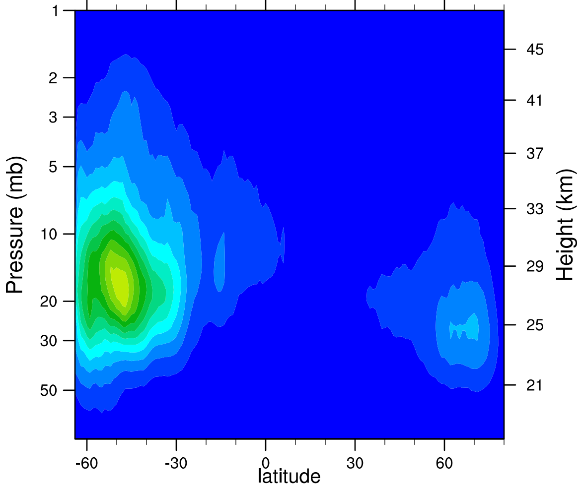
2007d244 N2O5_Ascending (ppbv)
