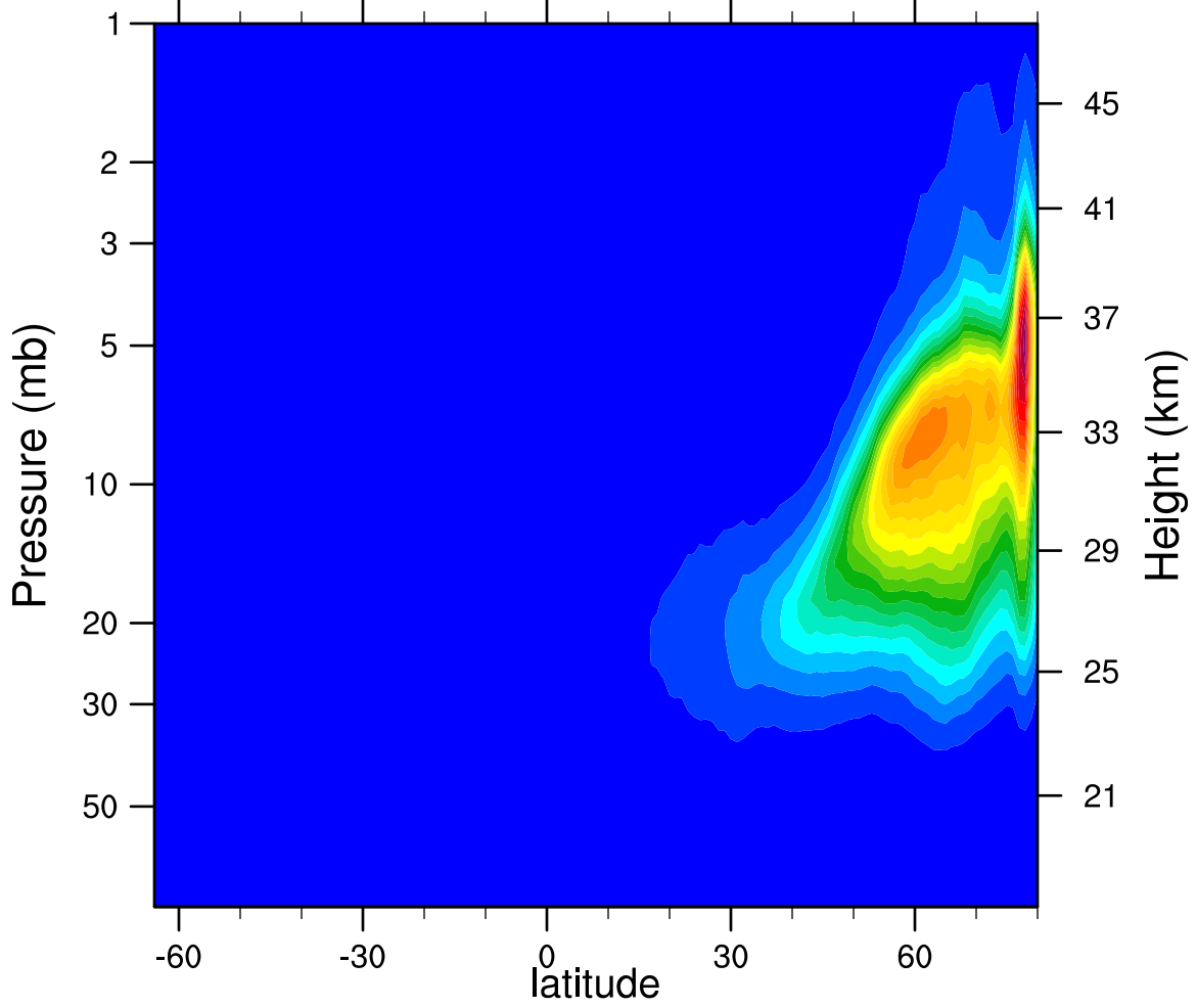
2007d019 N2O5_Ascending (ppbv)
