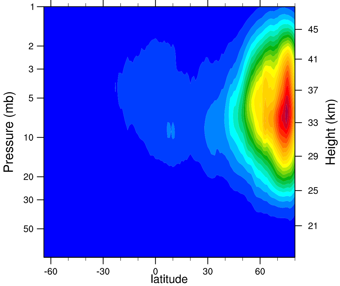
2005d339 N2O5_Ascending (ppbv)
