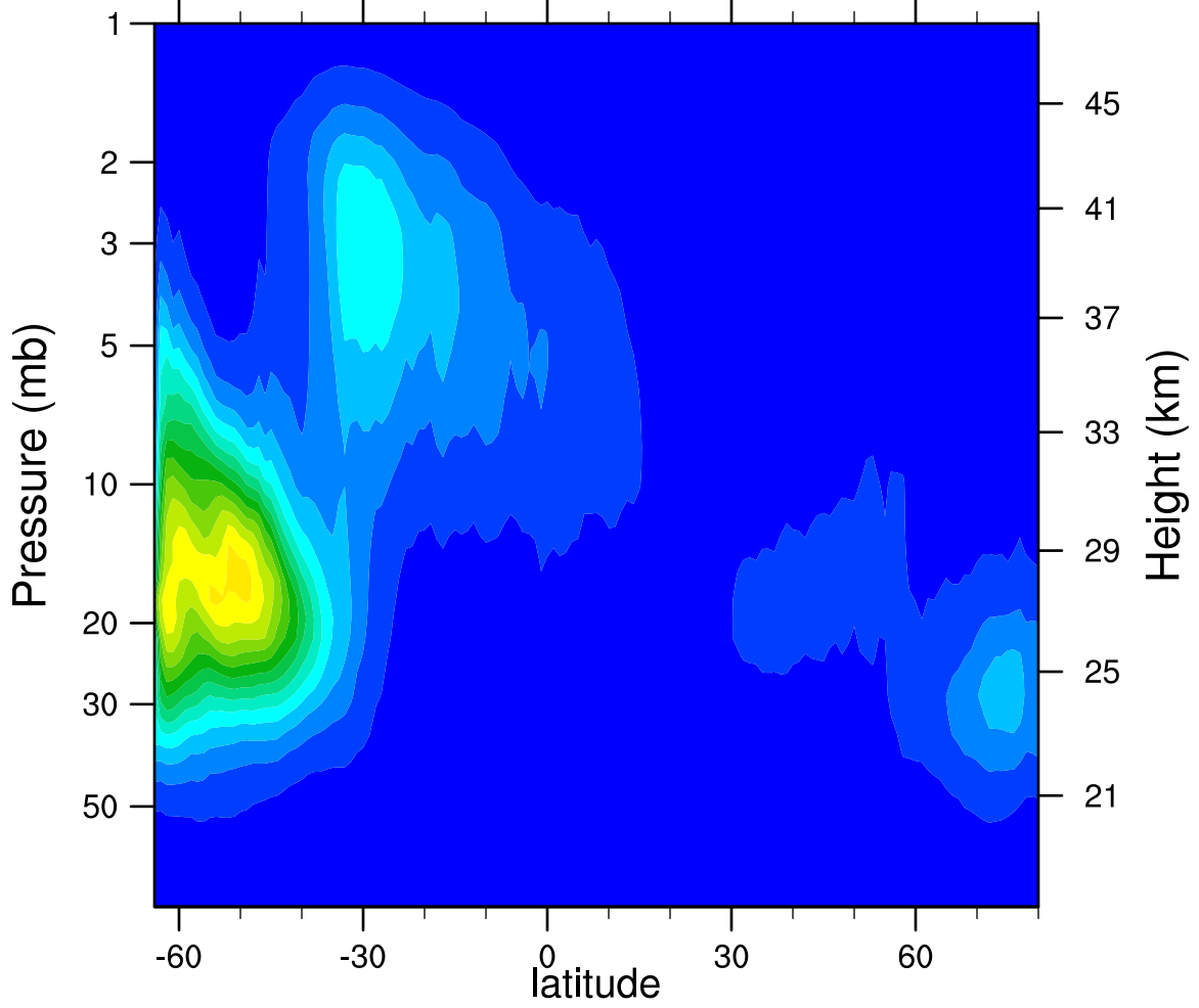
2007d100 N2O5_Ascending (ppbv)
