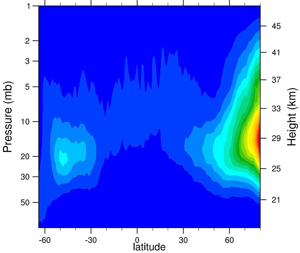
2007d292 N2O5_Ascending (ppbv)
