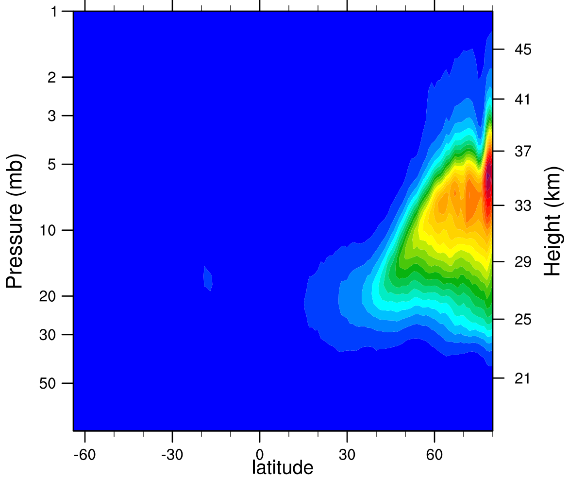
2007d026 N2O5_Ascending (ppbv)
