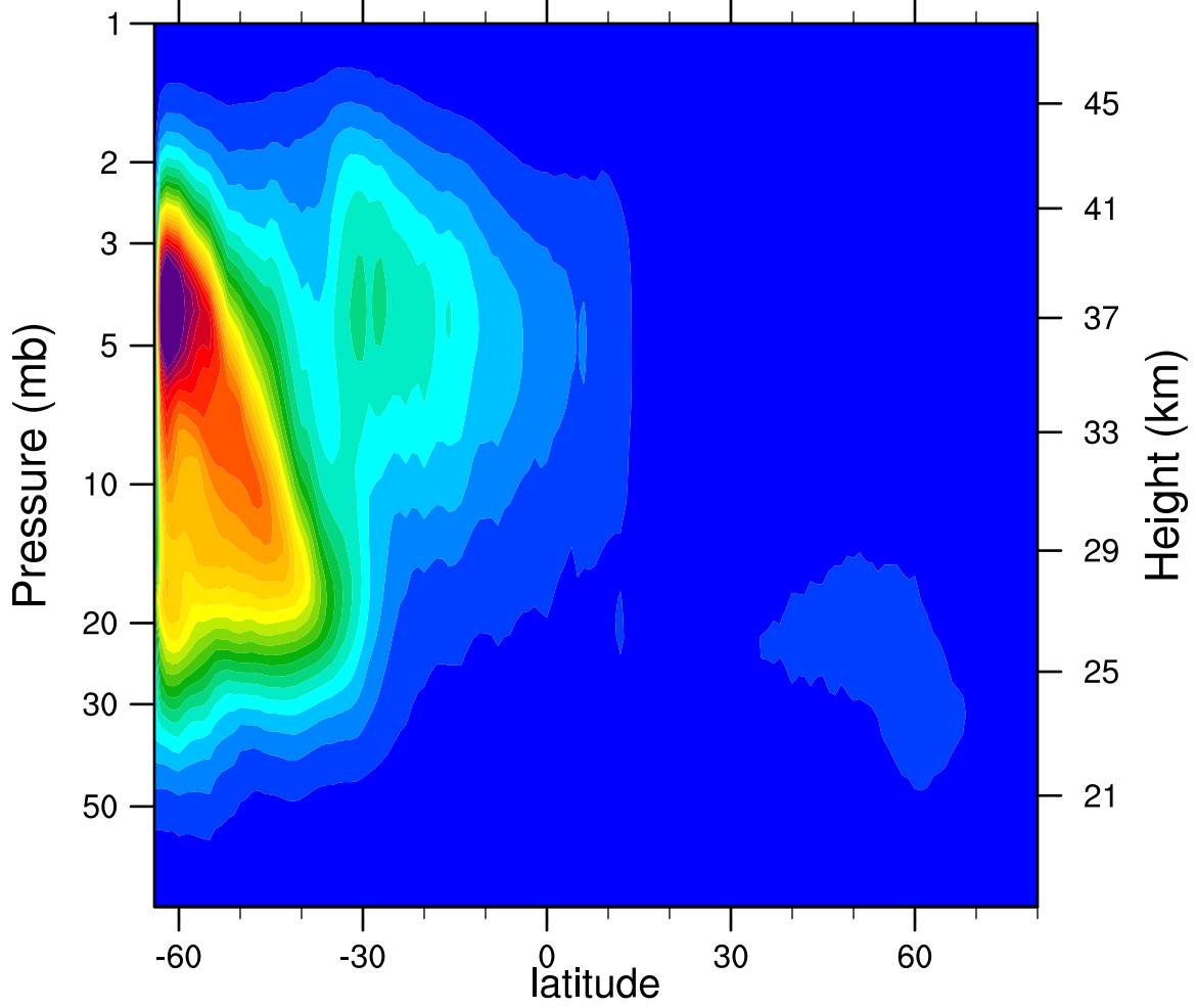
2007d127 N2O5_Ascending (ppbv)
