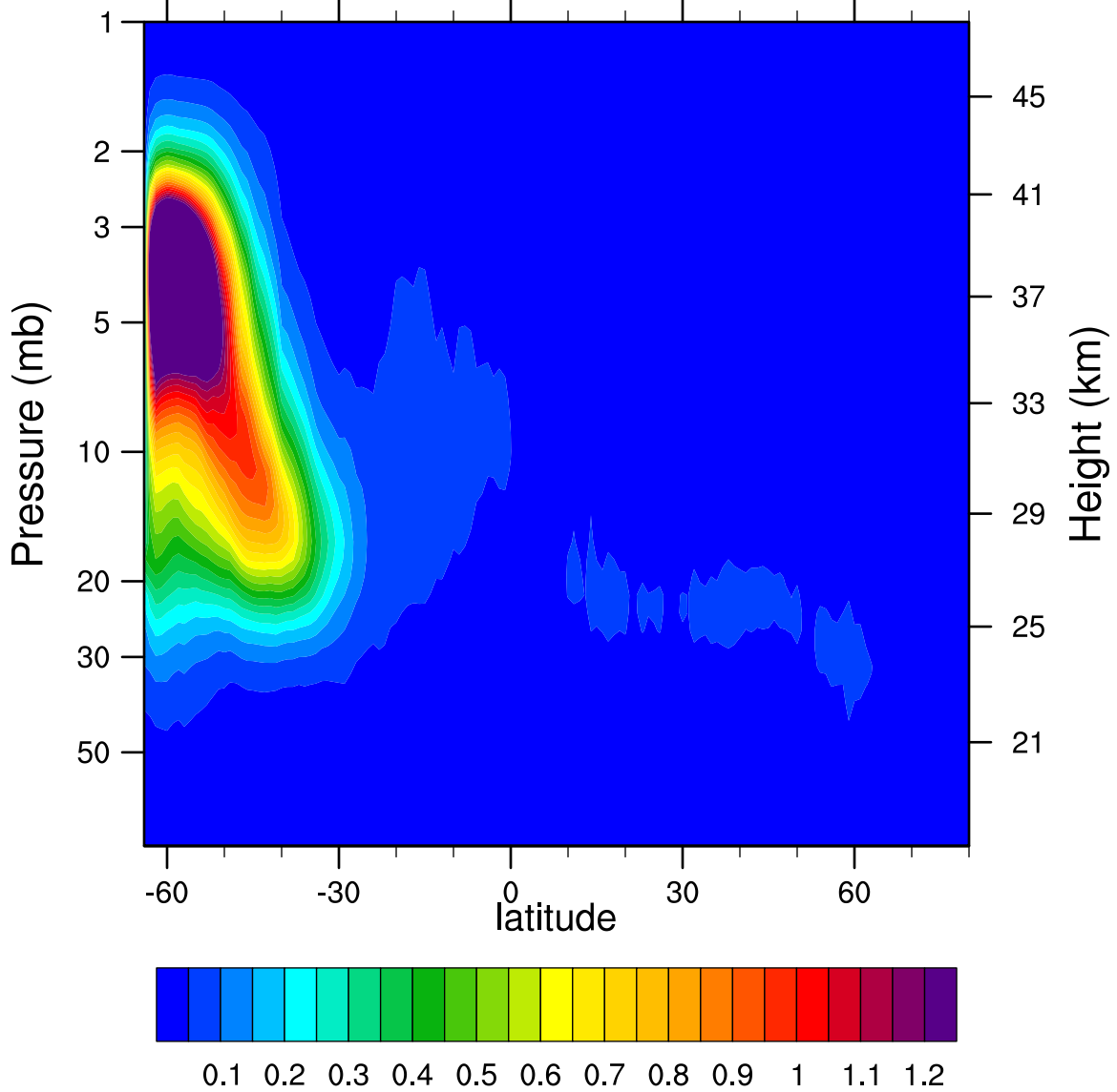
2007d152 N2O5_Ascending (ppbv)
