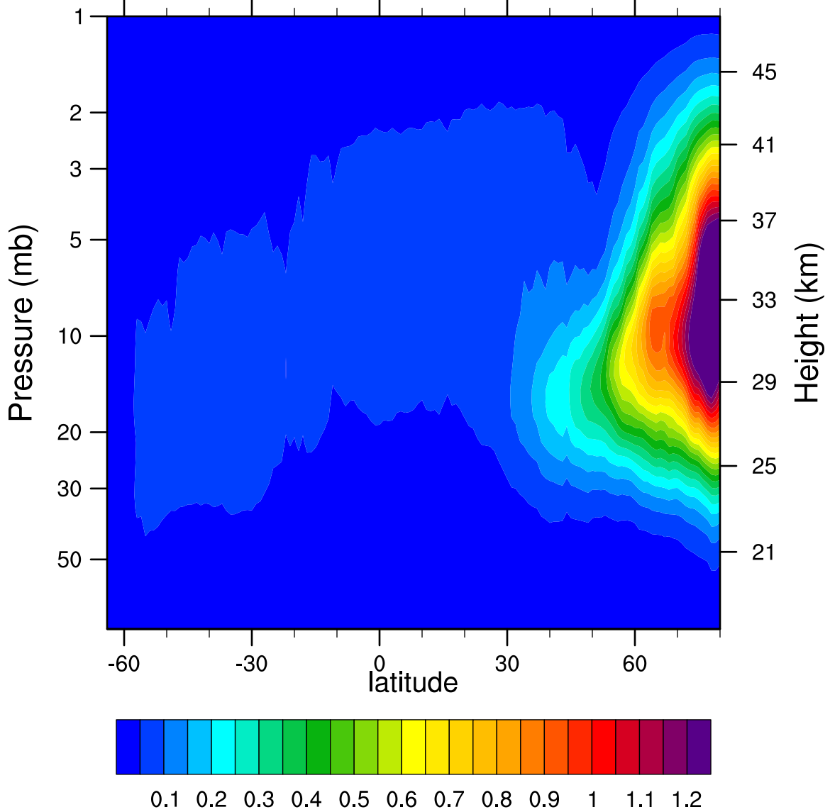
2007d327 N2O5_Ascending (ppbv)
