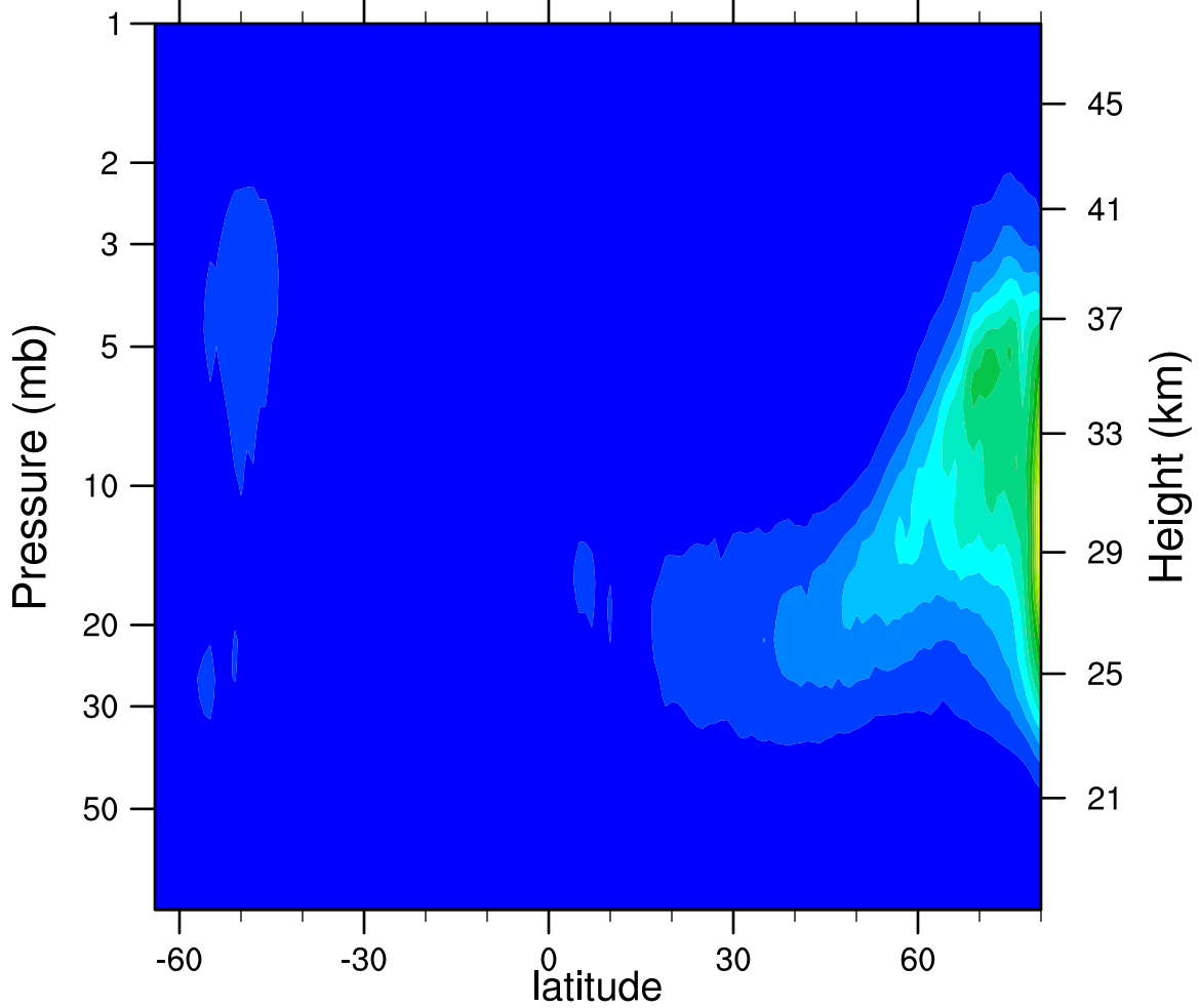
2007d060 N2O5_Ascending (ppbv)
