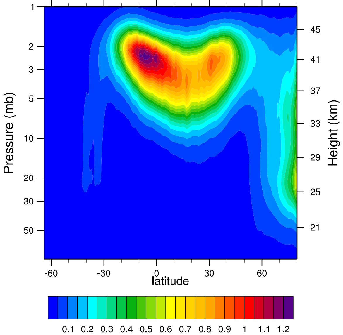
2005d055 N2O5_Ascending (ppbv)
