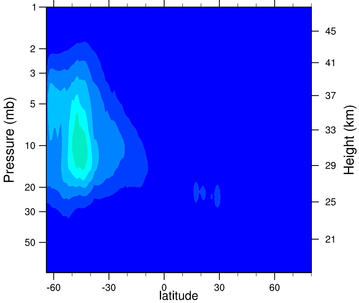
2007d175 N2O5_Ascending (ppbv)
