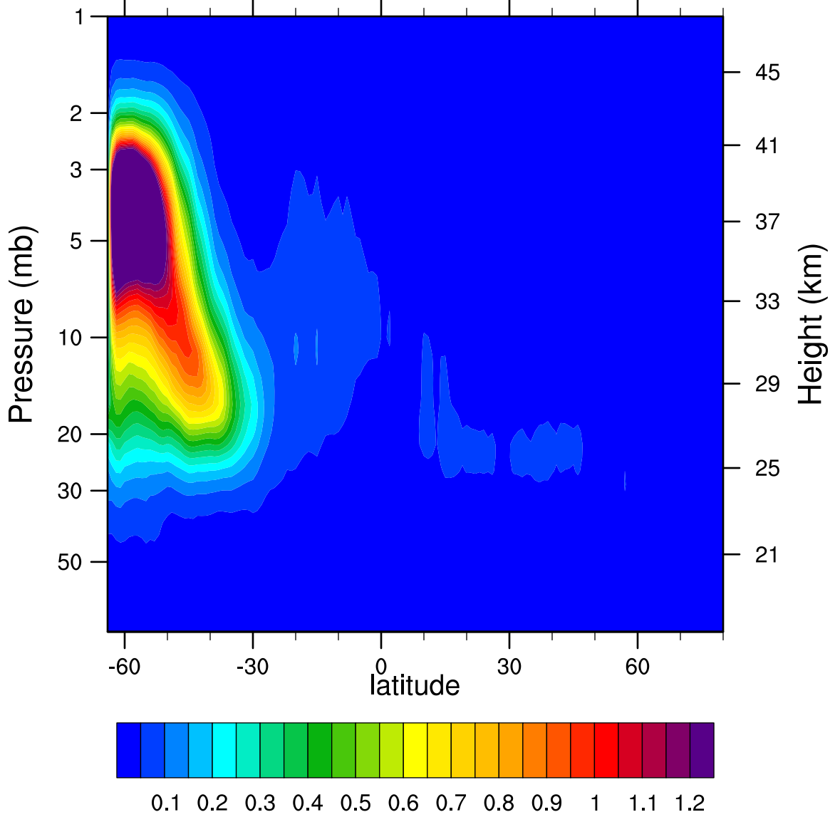
2007d156 N2O5_Ascending (ppbv)
