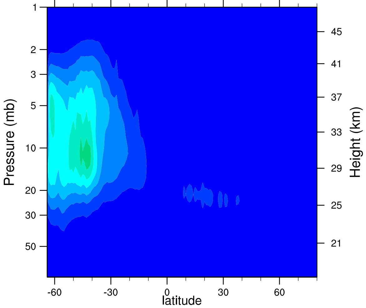
2007d168 N2O5_Ascending (ppbv)
