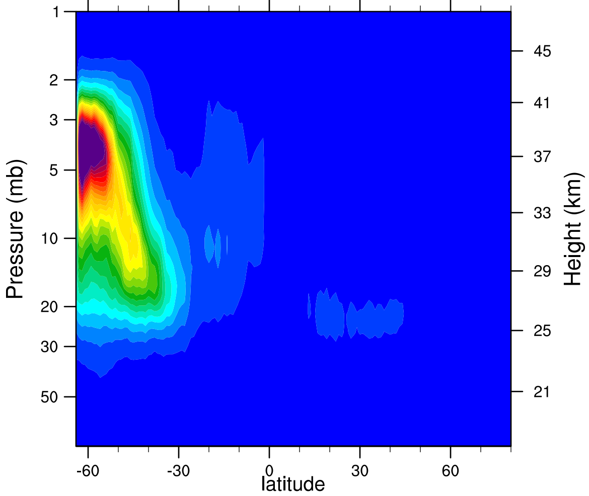
2007d162 N2O5_Ascending (ppbv)
