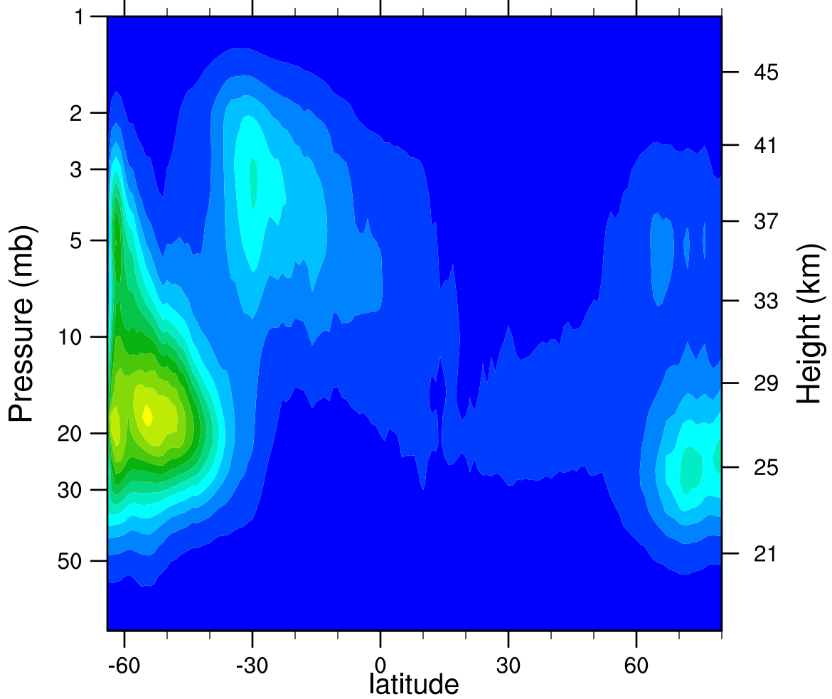
2007d091 N2O5_Ascending (ppbv)
