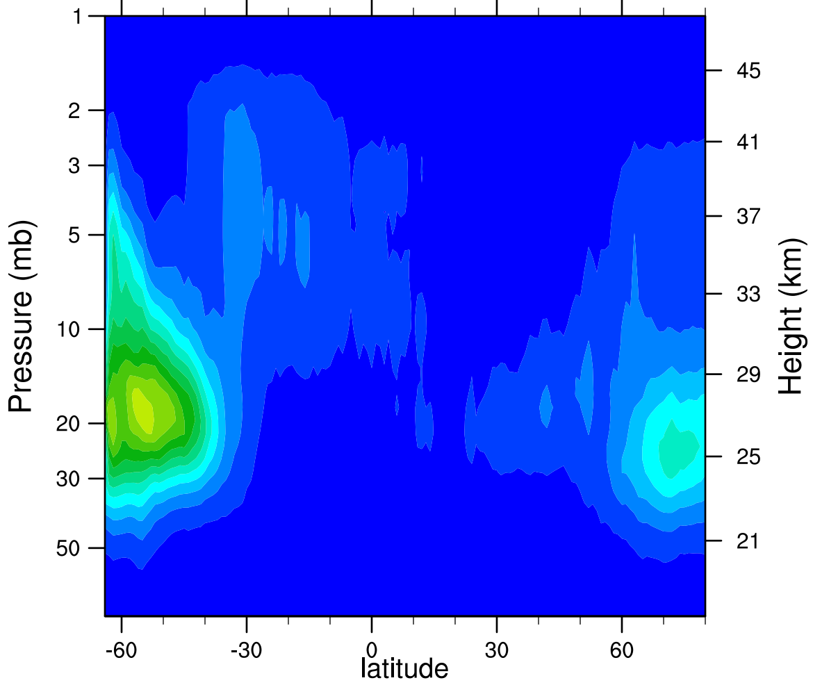
2007d085 N2O5_Ascending (ppbv)
