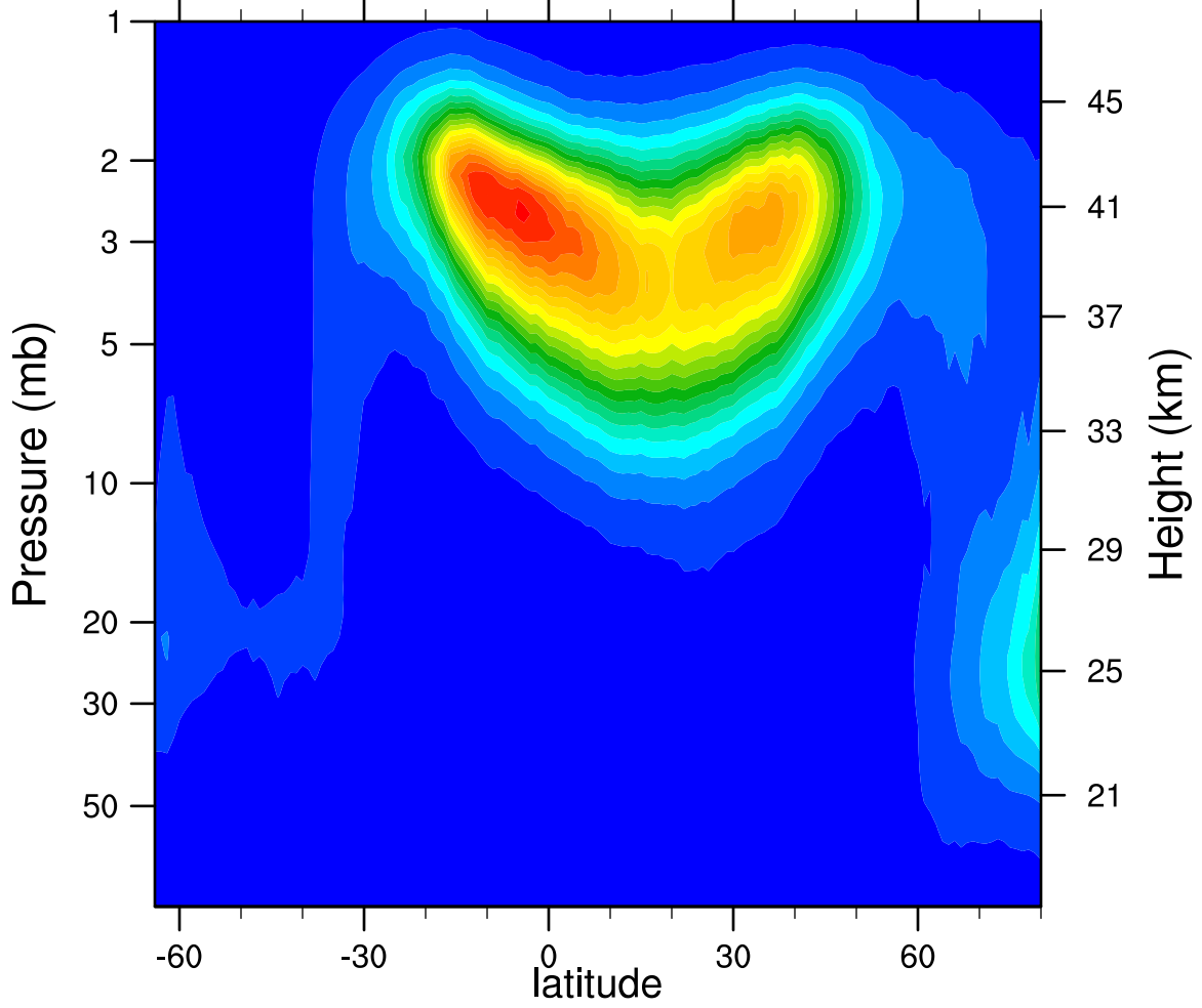
2005d069 N2O5_Ascending (ppbv)
