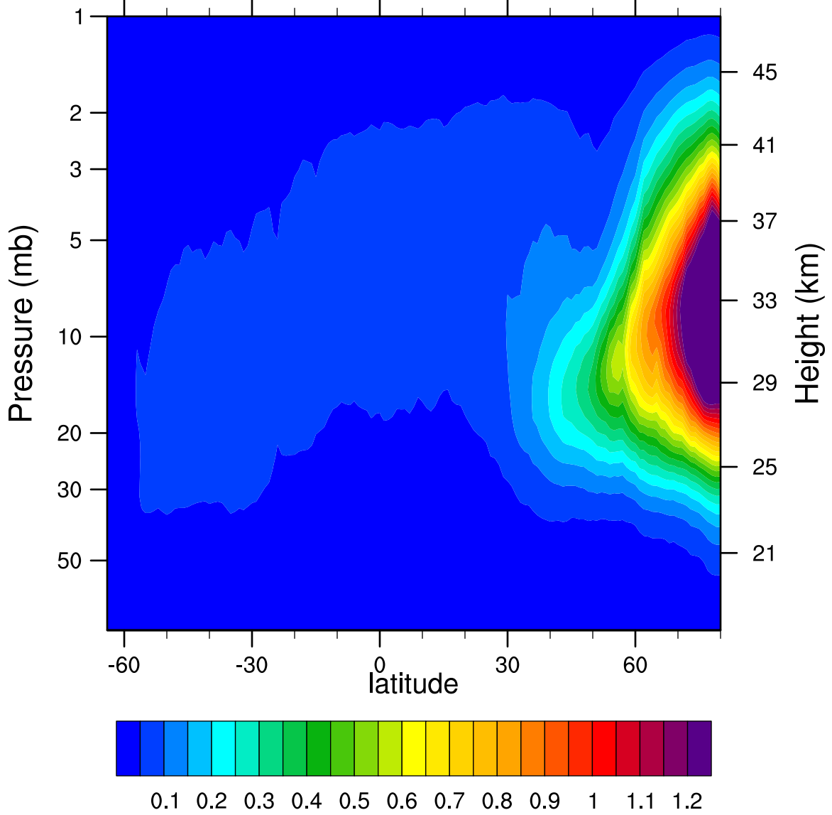
2007d332 N2O5_Ascending (ppbv)
