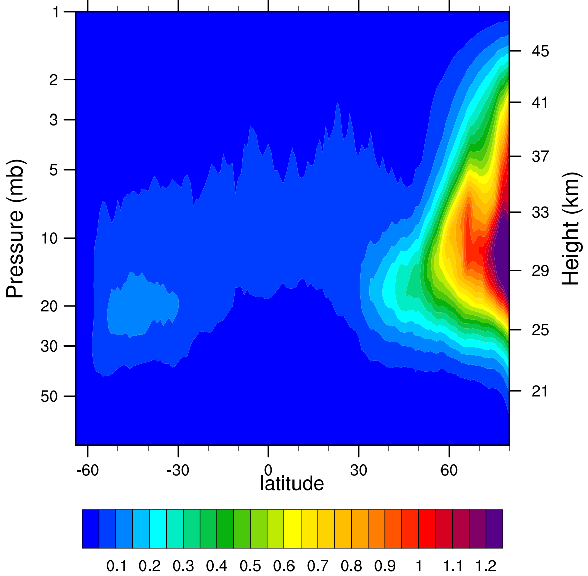
2007d317 N2O5_Ascending (ppbv)
