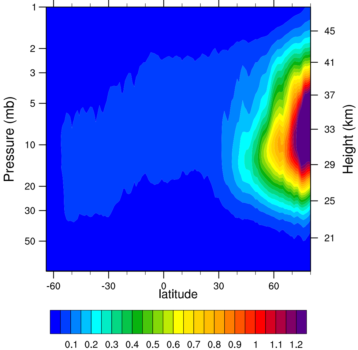
2007d343 N2O5_Ascending (ppbv)
