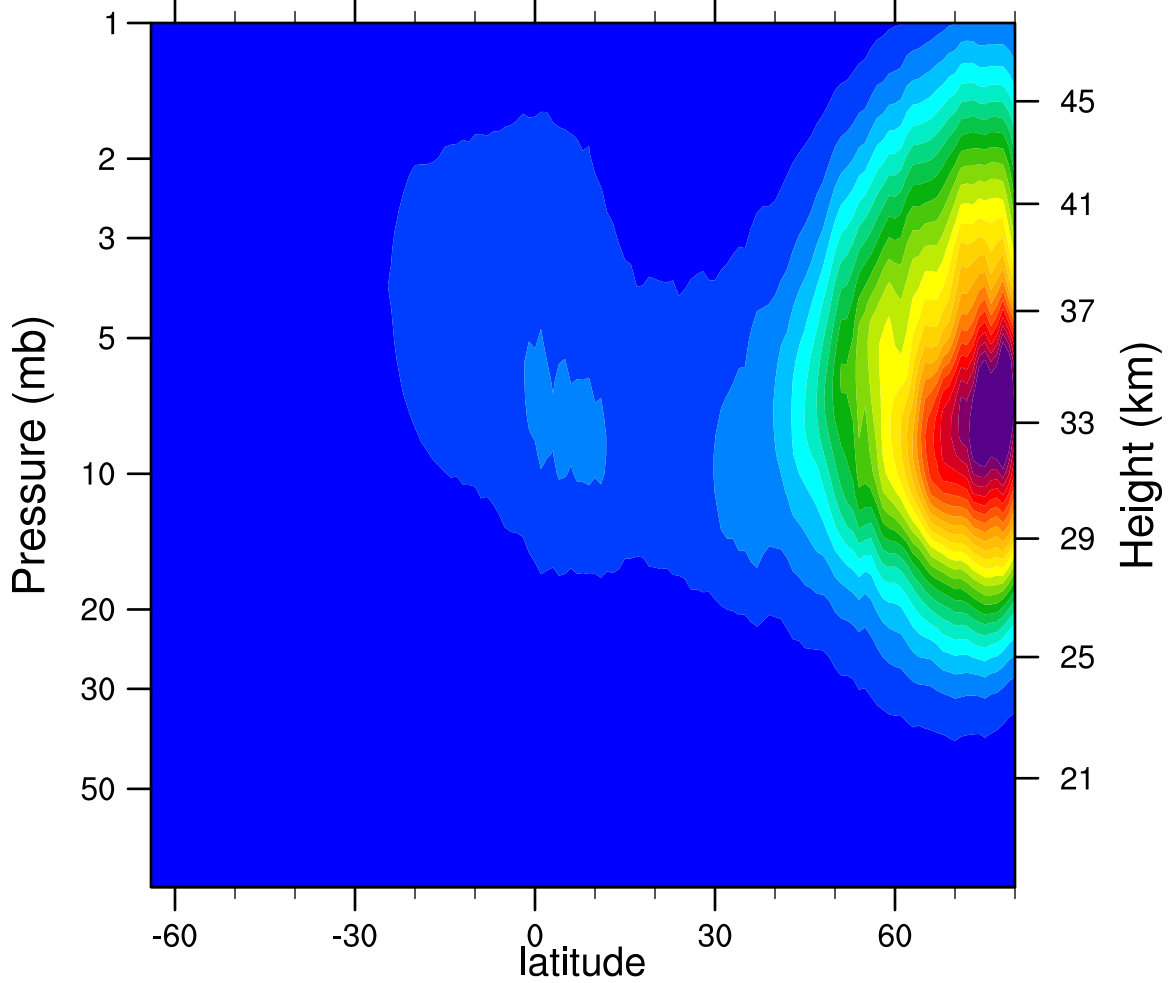
2005d362 N2O5_Ascending (ppbv)
