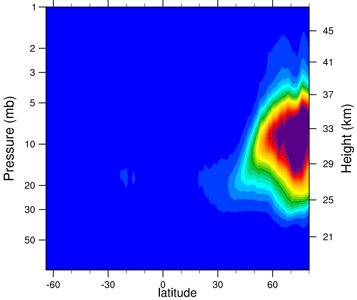
2007d004 N2O5_Ascending (ppbv)
