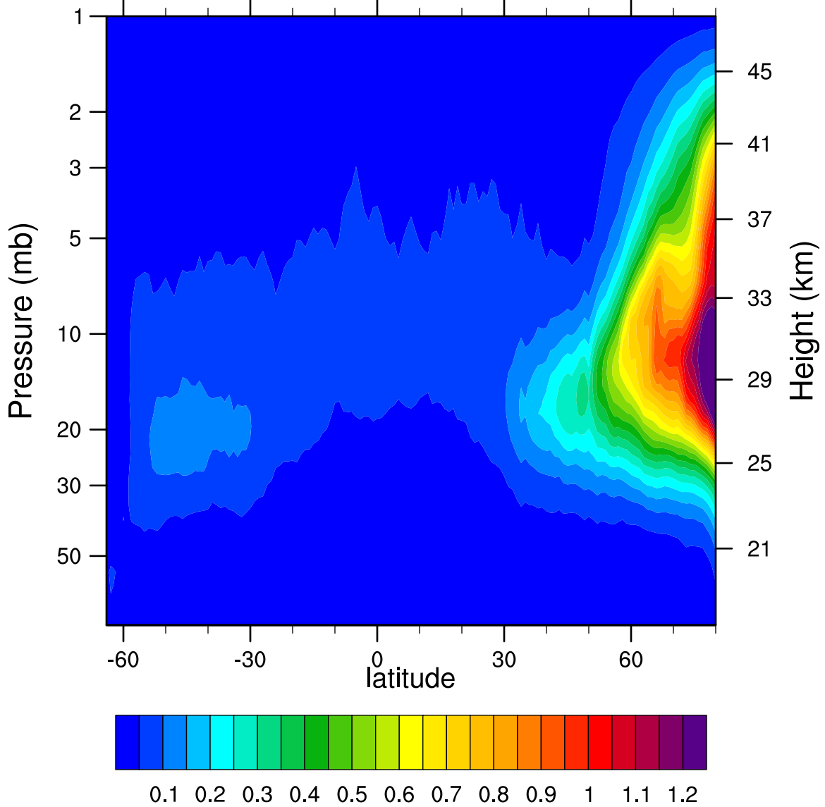
2007d316 N2O5_Ascending (ppbv)
