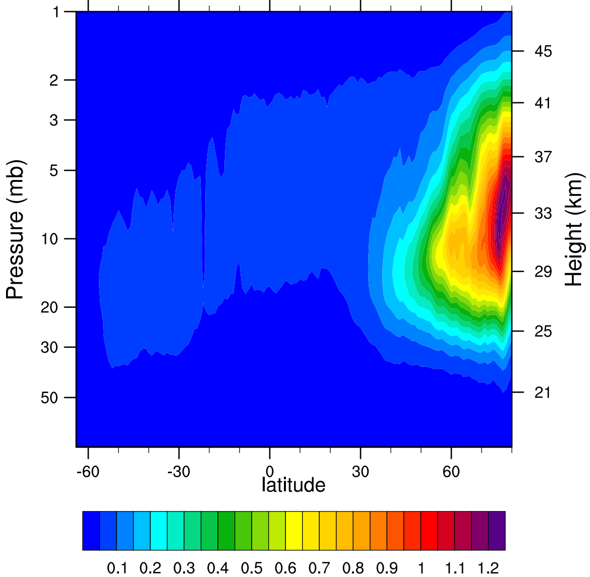
2007d339 N2O5_Ascending (ppbv)
