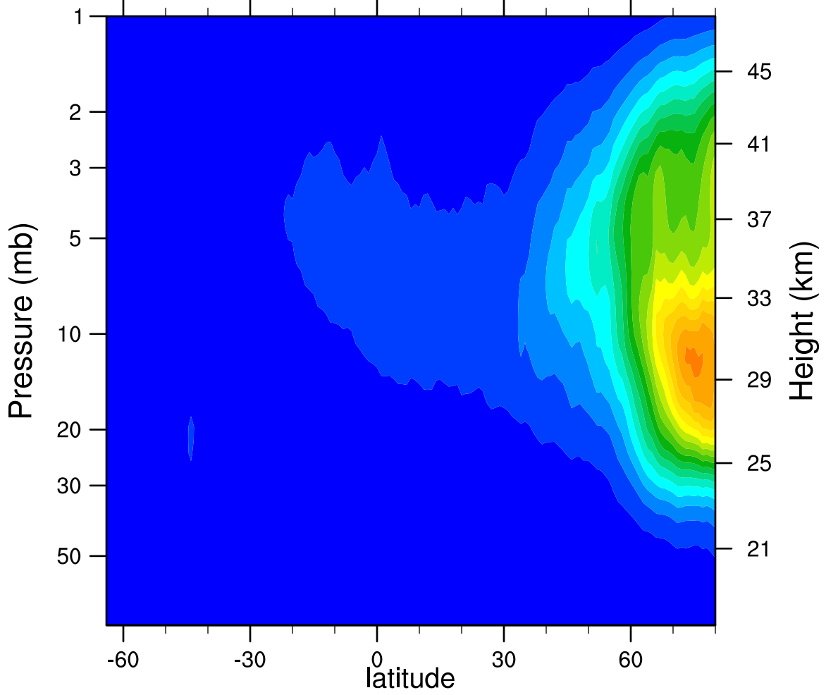
2005d314 N2O5_Ascending (ppbv)
