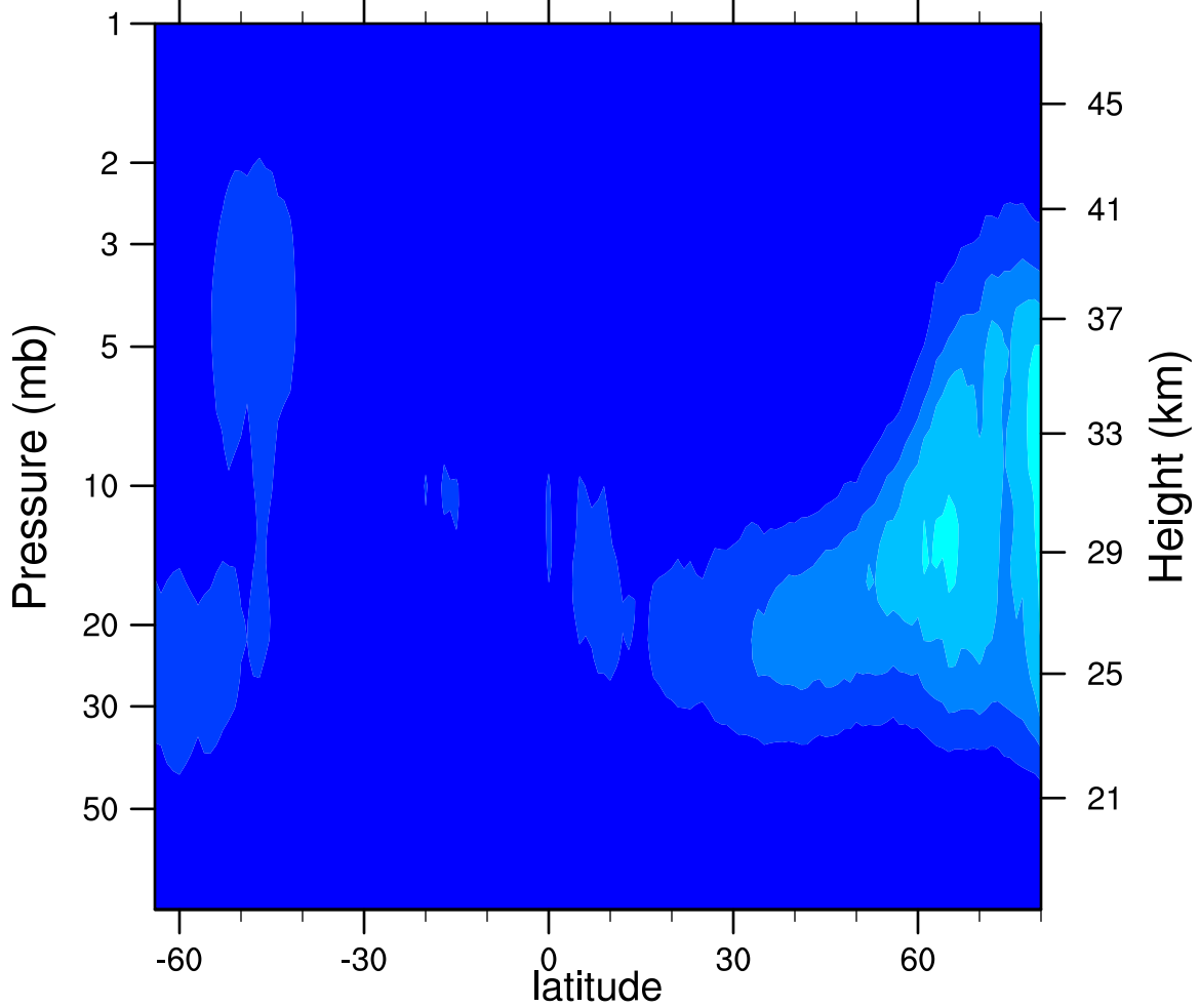
2007d071 N2O5_Ascending (ppbv)
