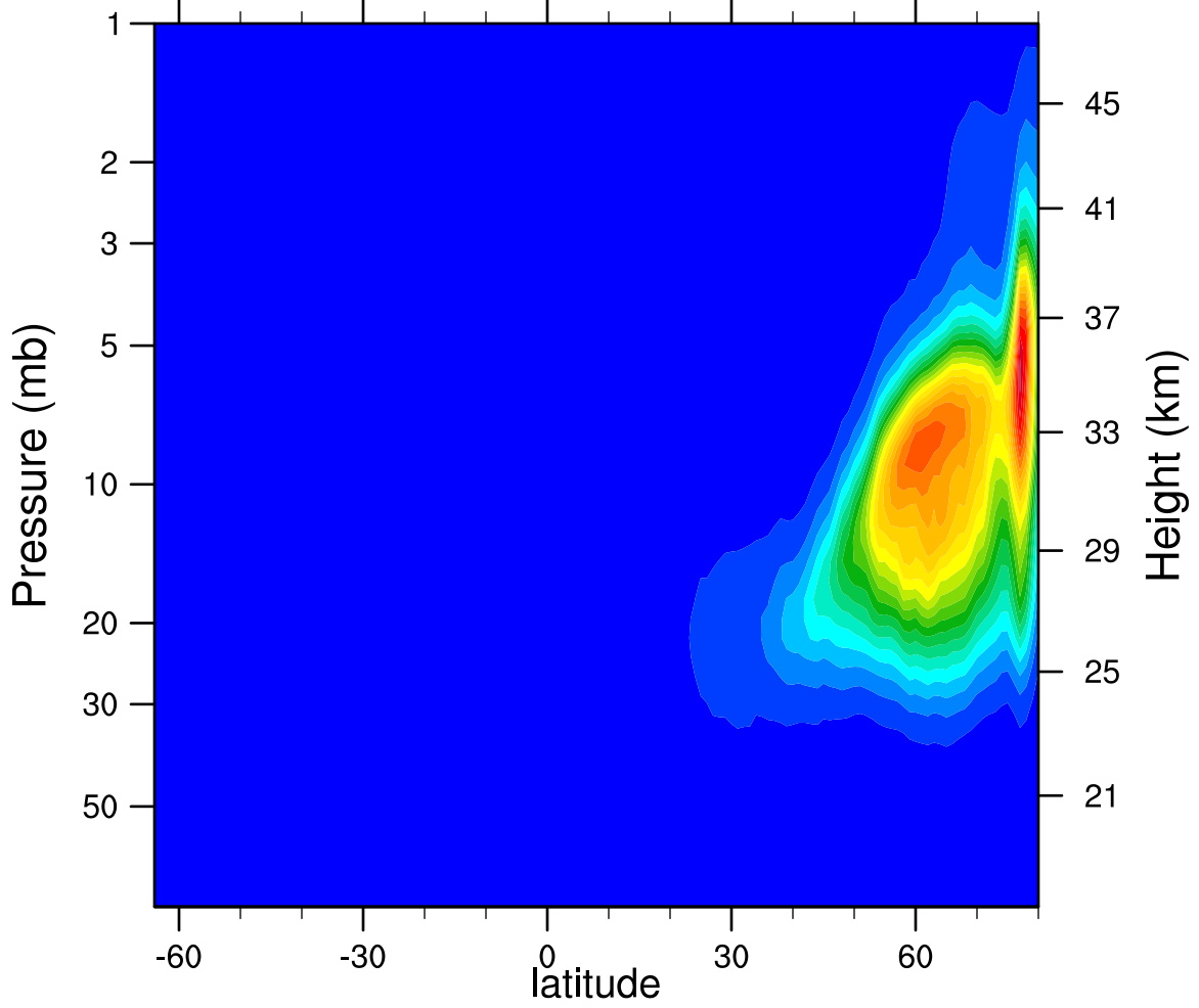
2007d015 N2O5_Ascending (ppbv)
