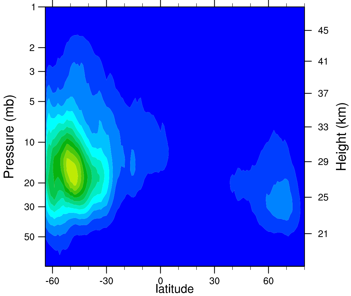
2007d242 N2O5_Ascending (ppbv)
