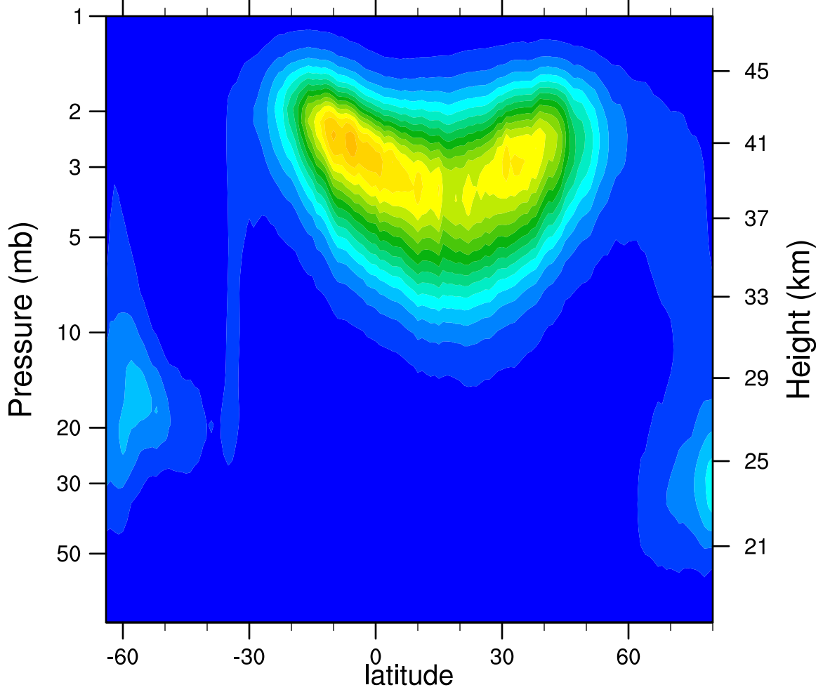
2005d082 N2O5_Ascending (ppbv)
