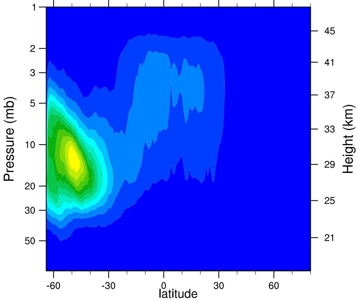
2007d220 N2O5_Ascending (ppbv)
