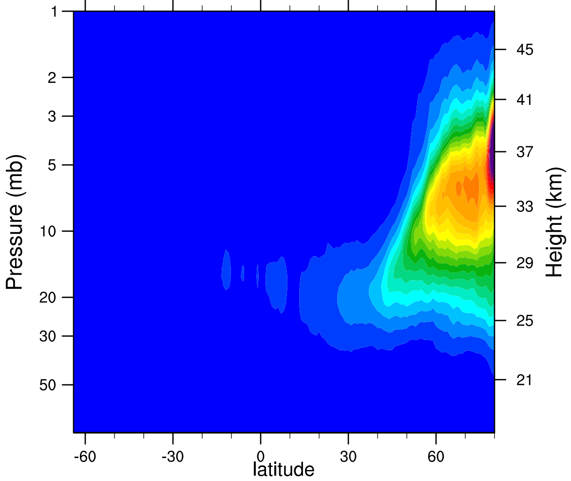
2007d031 N2O5_Ascending (ppbv)
