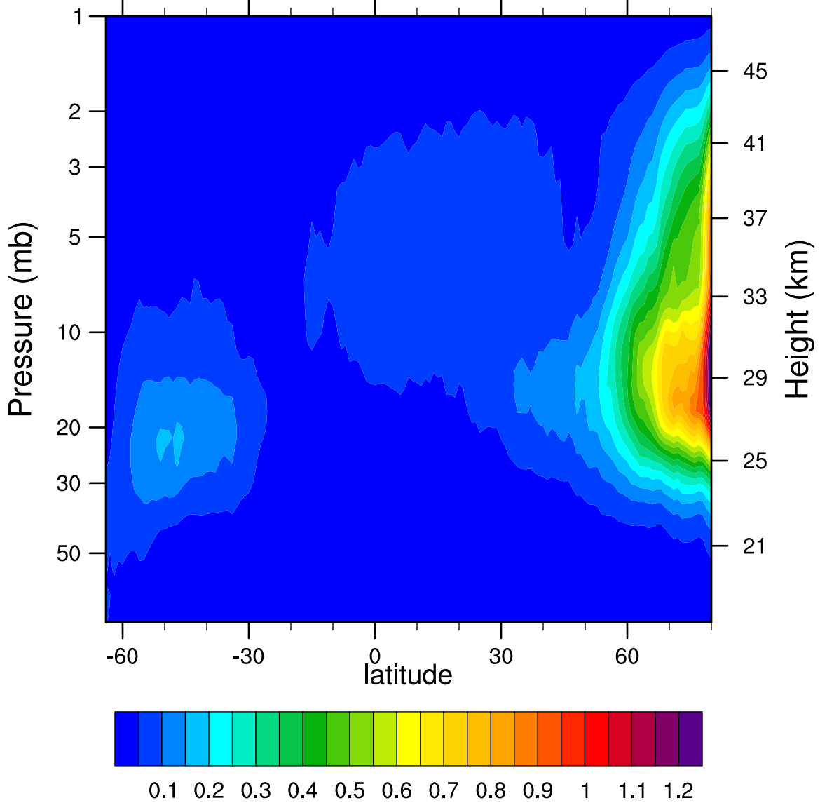
2007d308 N2O5_Ascending (ppbv)
