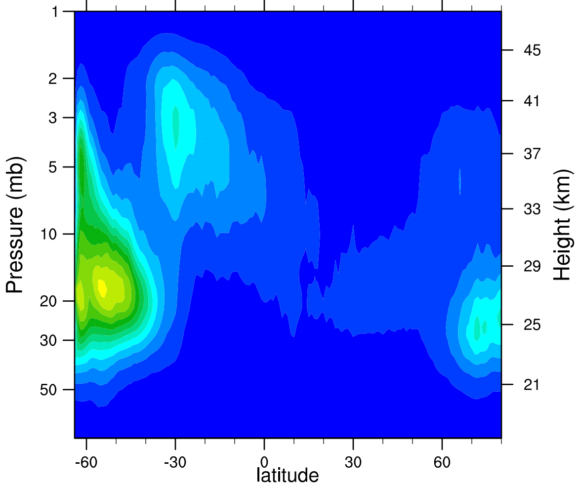
2007d092 N2O5_Ascending (ppbv)
