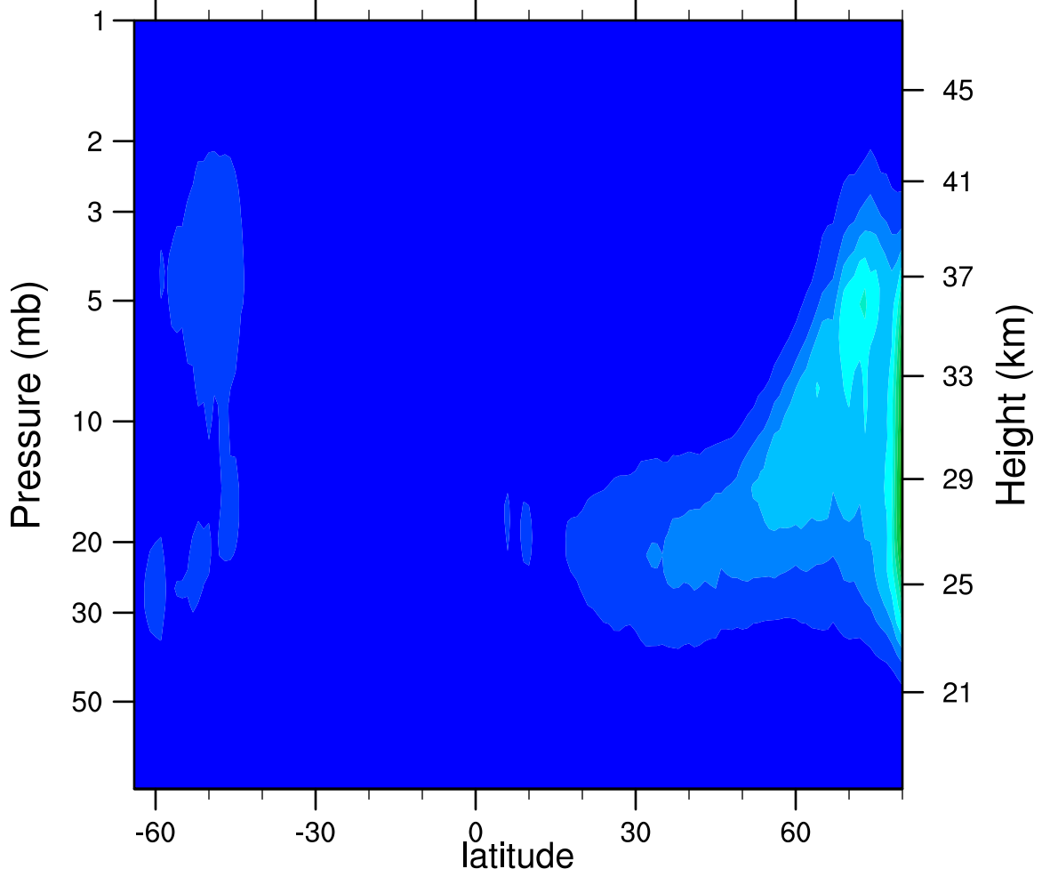
2007d064 N2O5_Ascending (ppbv)
