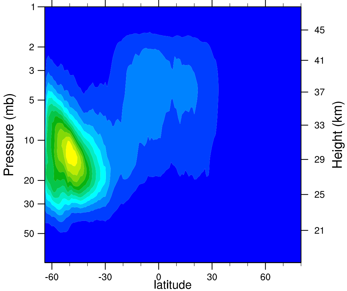
2007d222 N2O5_Ascending (ppbv)
