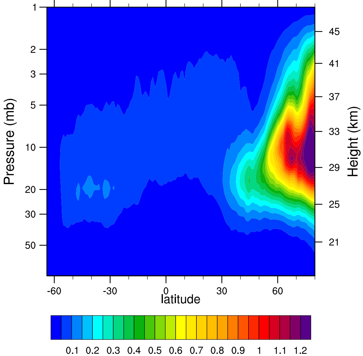
2007d321 N2O5_Ascending (ppbv)
