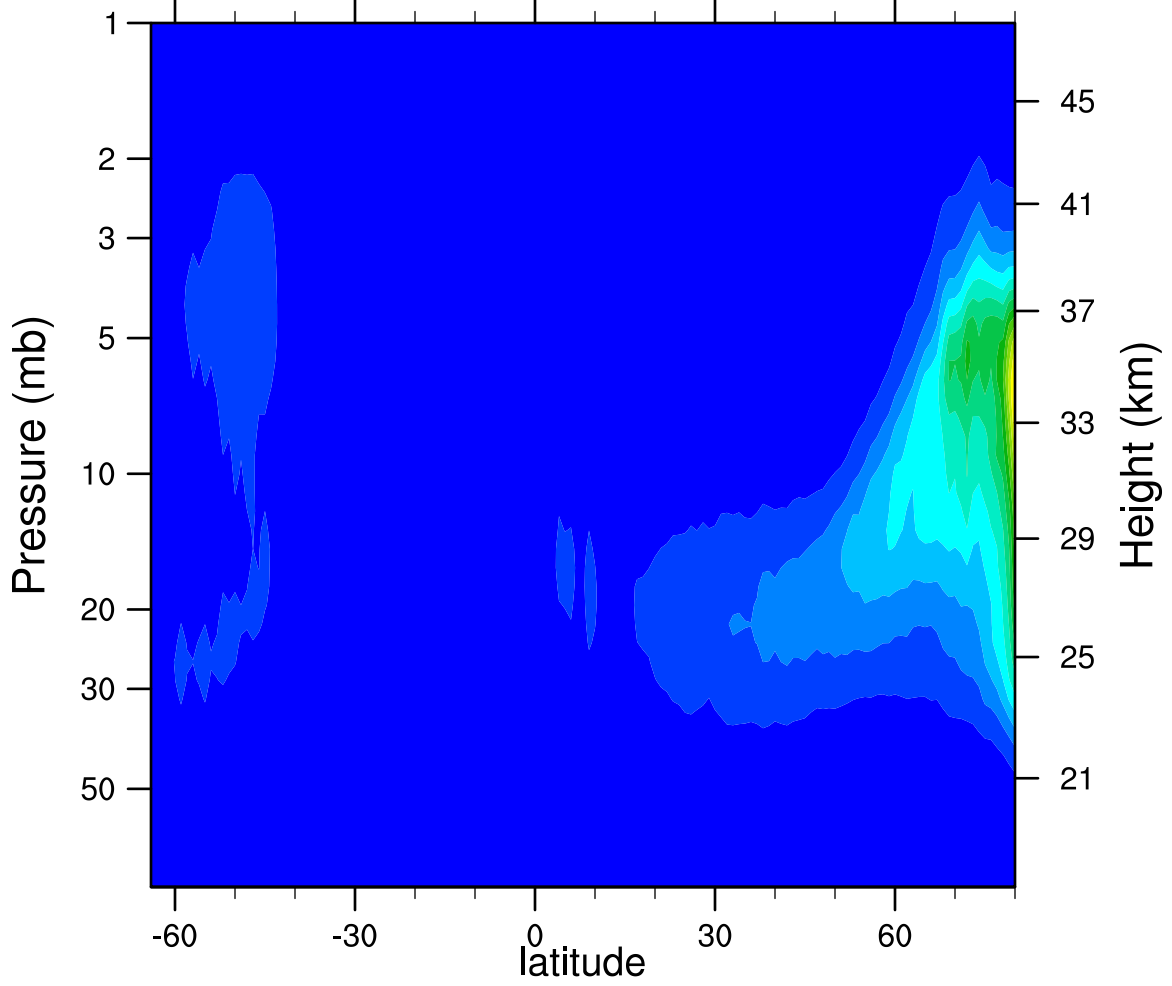
2007d062 N2O5_Ascending (ppbv)
