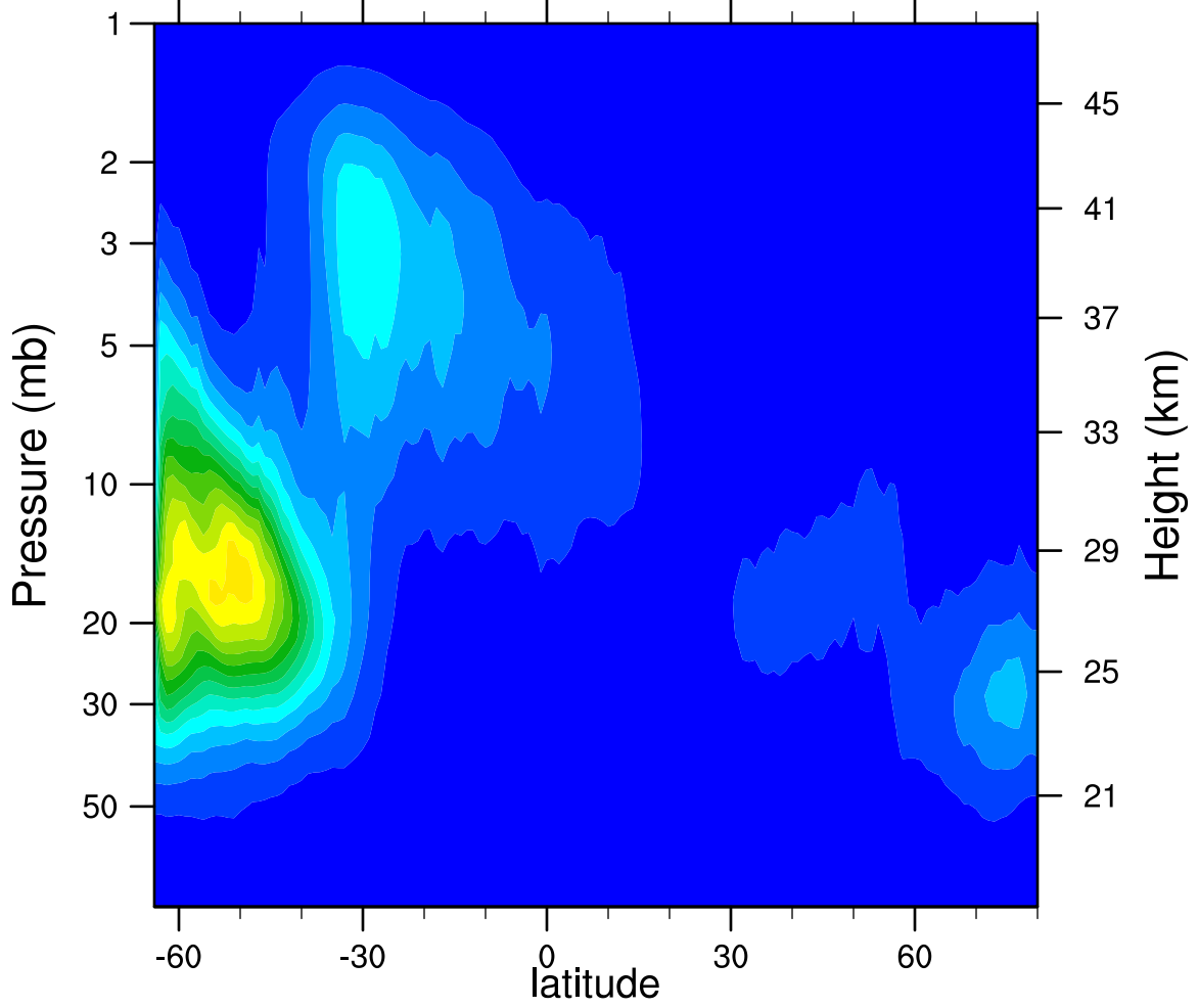
2007d101 N2O5_Ascending (ppbv)
