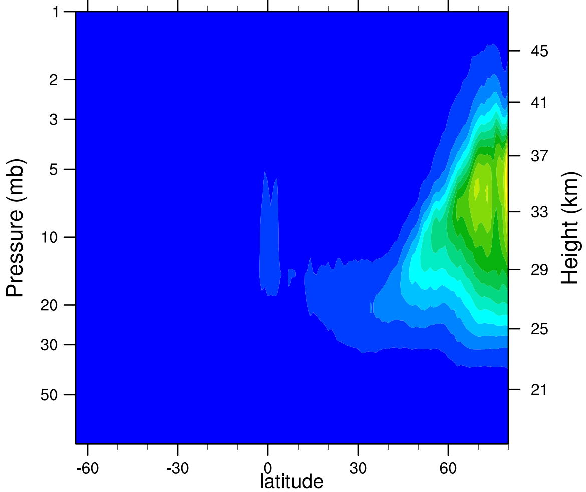
2007d042 N2O5_Ascending (ppbv)
