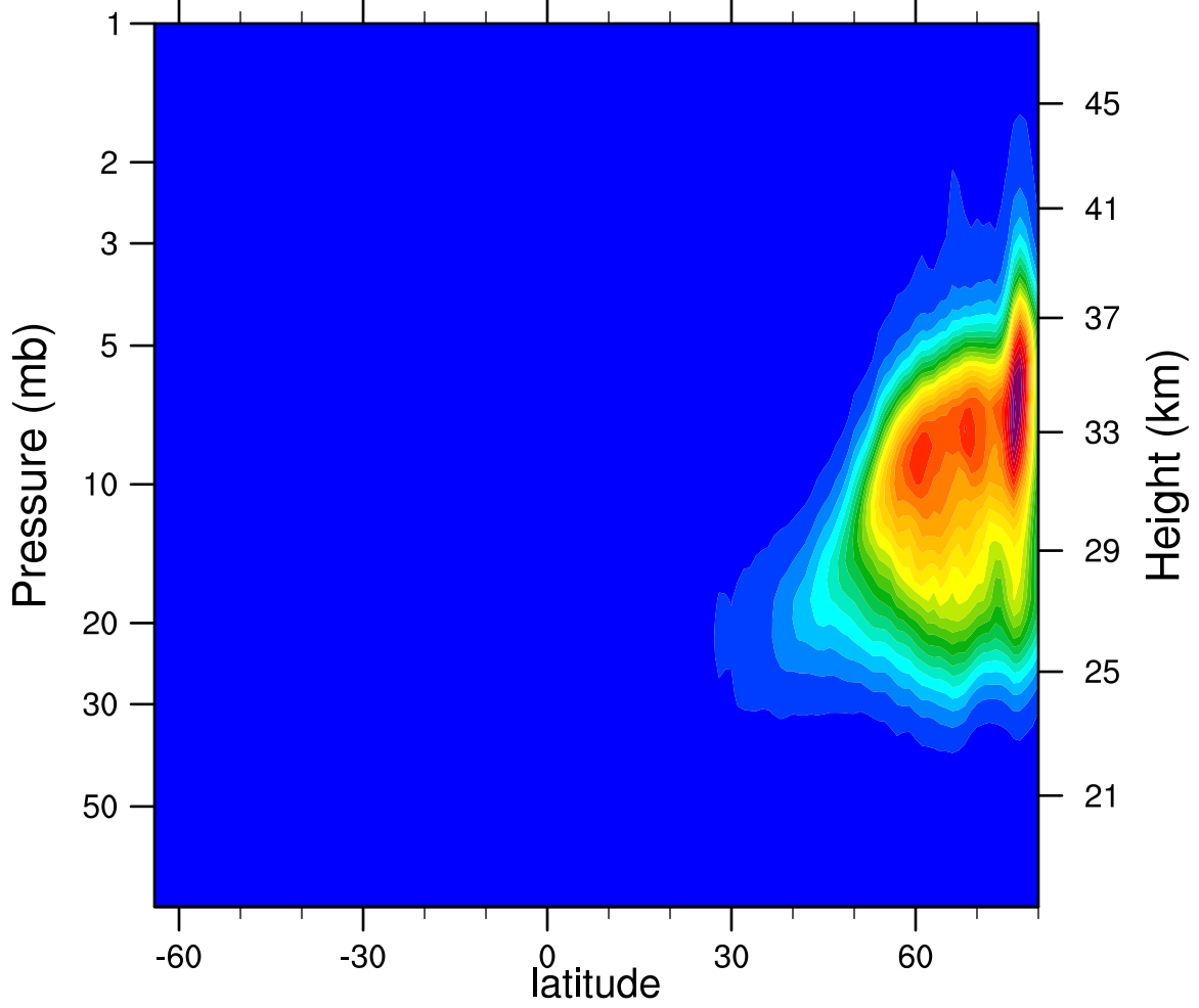
2007d011 N2O5_Ascending (ppbv)
