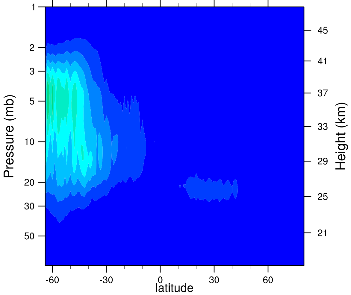
2007d164 N2O5_Ascending (ppbv)
