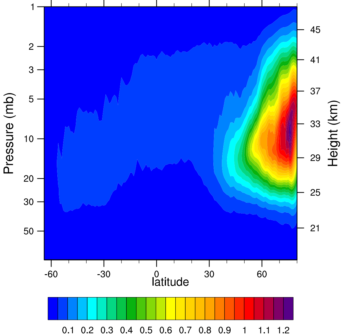
2007d337 N2O5_Ascending (ppbv)
