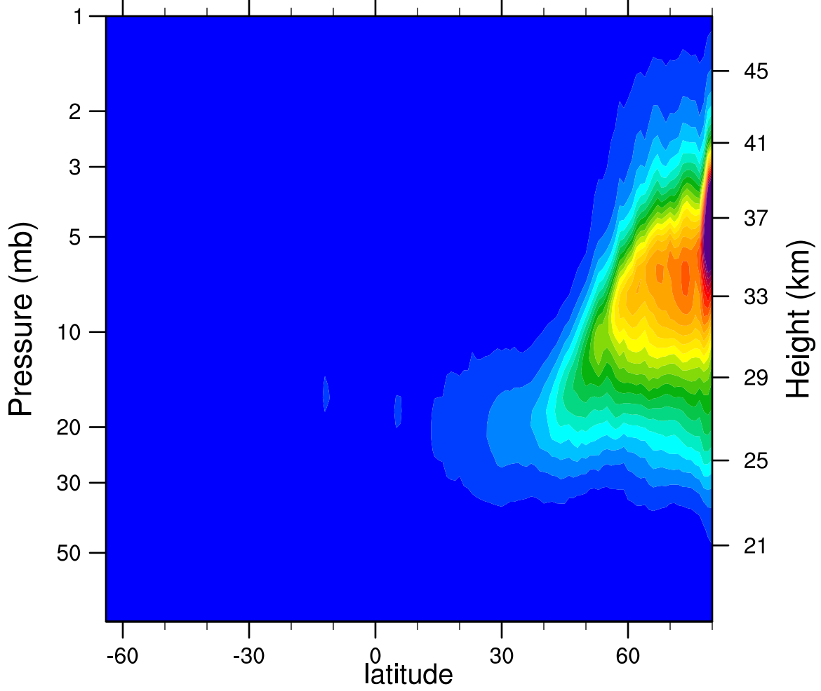
2007d030 N2O5_Ascending (ppbv)
