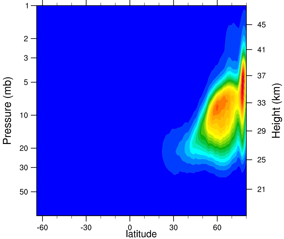
2007d016 N2O5_Ascending (ppbv)
