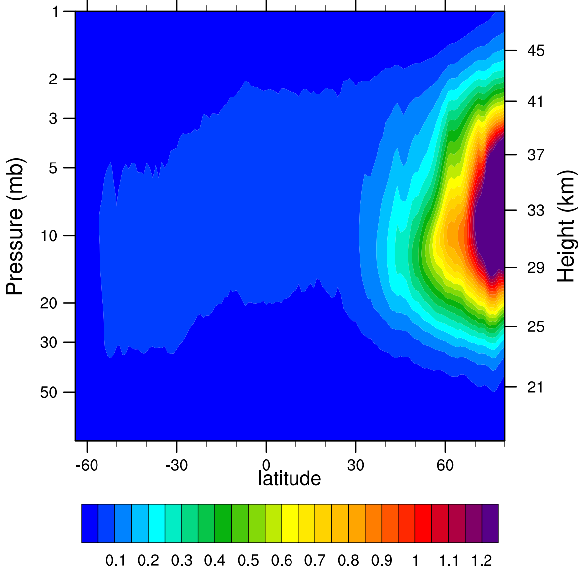
2007d345 N2O5_Ascending (ppbv)
