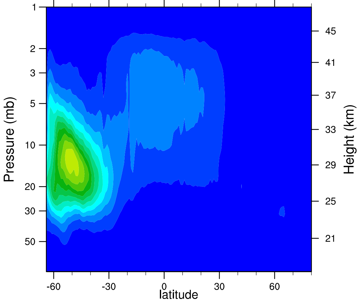
2007d228 N2O5_Ascending (ppbv)
