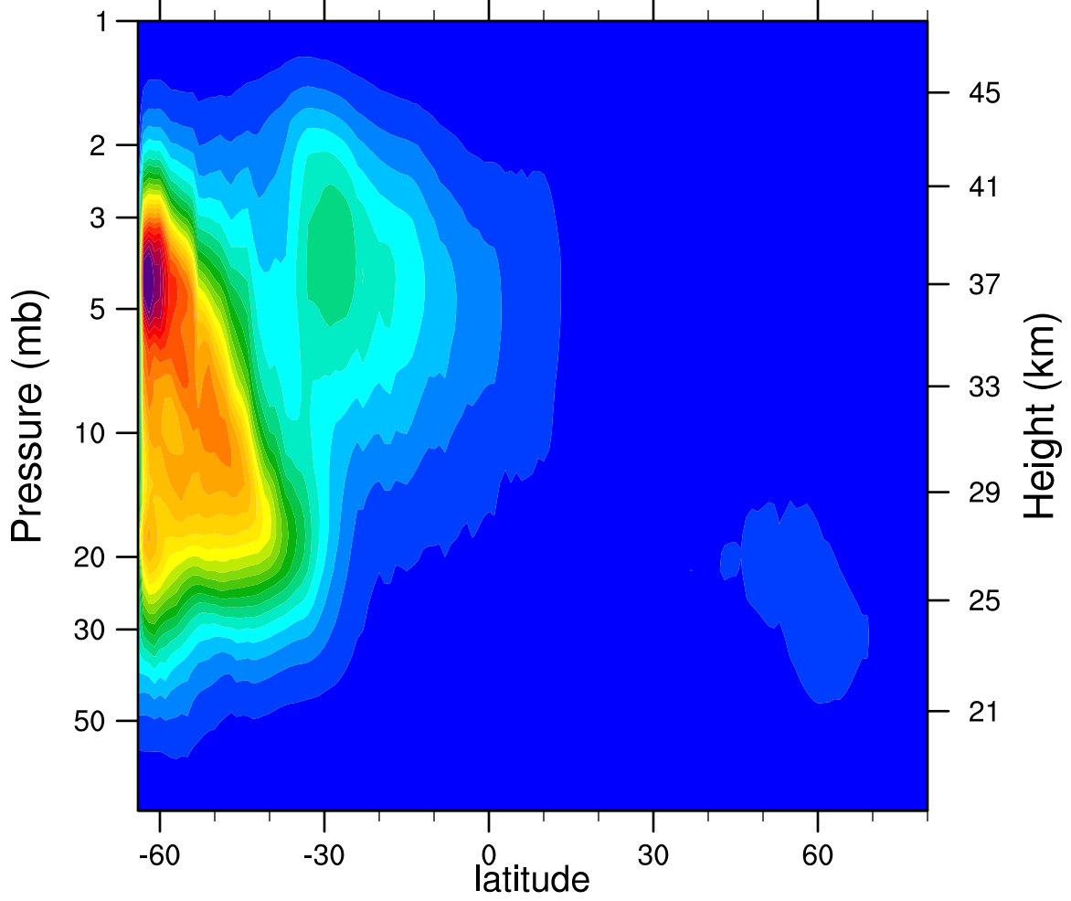
2007d124 N2O5_Ascending (ppbv)
