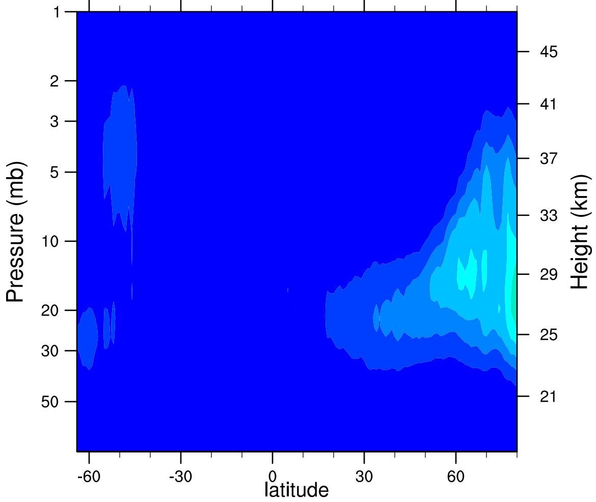
2007d067 N2O5_Ascending (ppbv)
