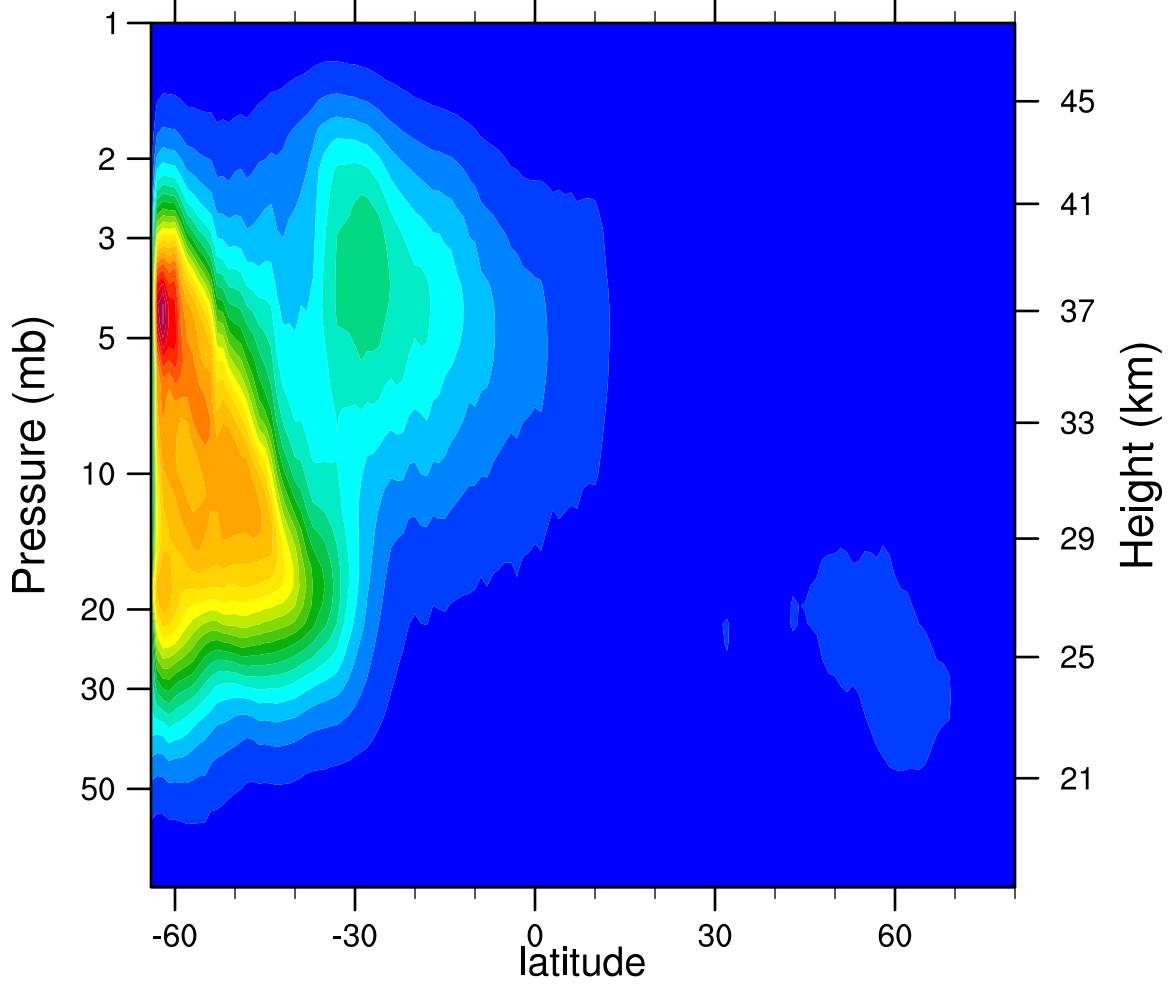
2007d123 N2O5_Ascending (ppbv)
