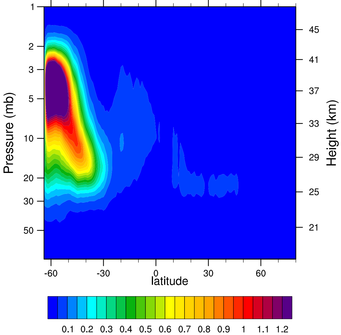
2007d157 N2O5_Ascending (ppbv)
