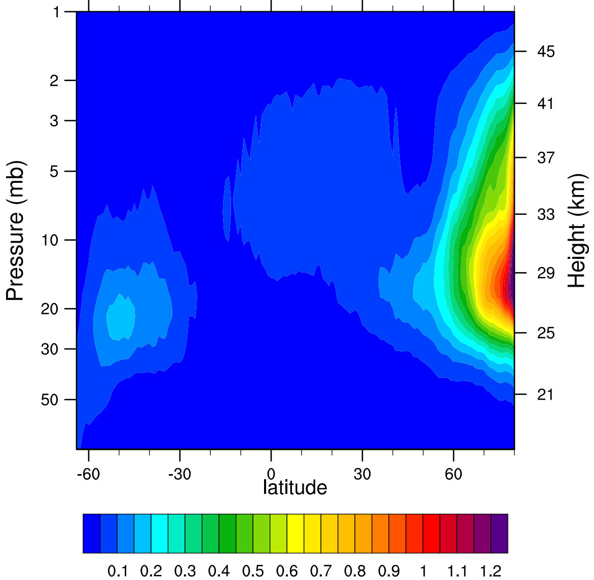
2007d305 N2O5_Ascending (ppbv)
