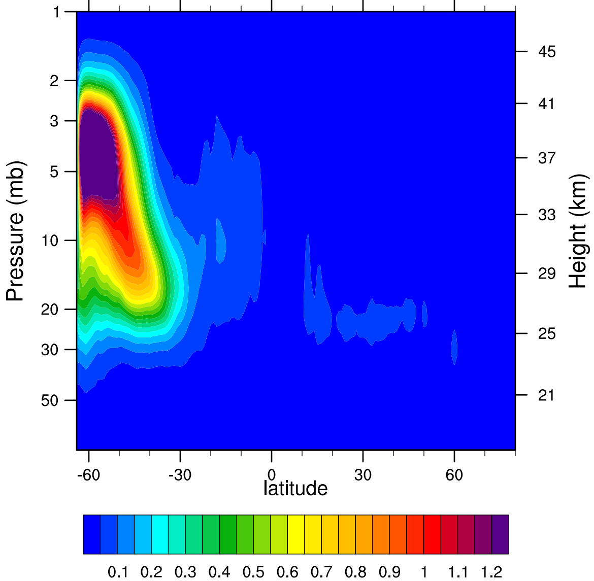
2007d146 N2O5_Ascending (ppbv)
