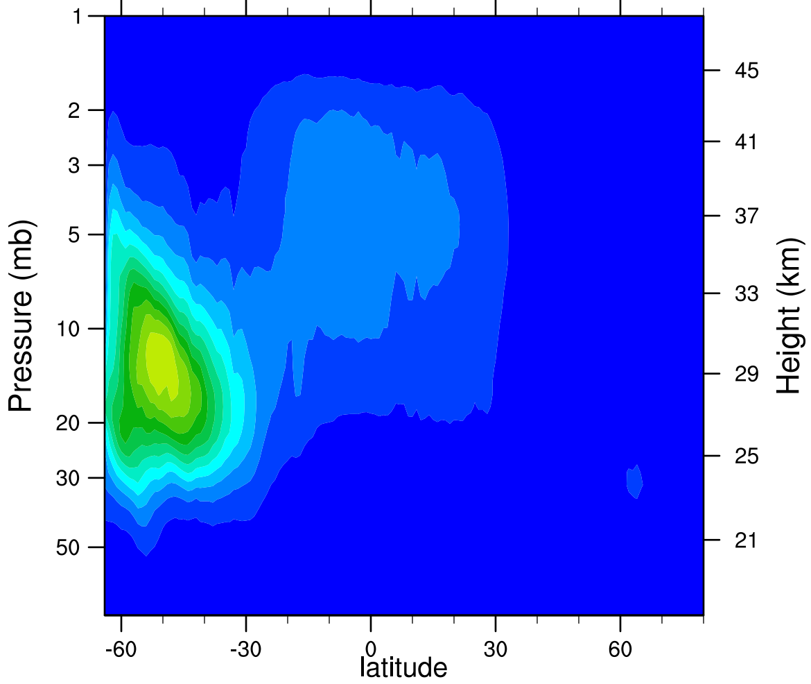
2007d227 N2O5_Ascending (ppbv)
