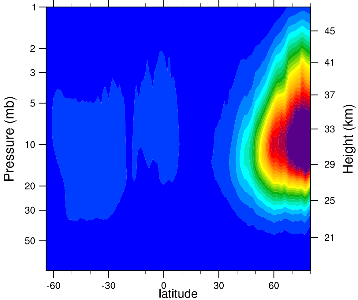
2007d364 N2O5_Ascending (ppbv)
