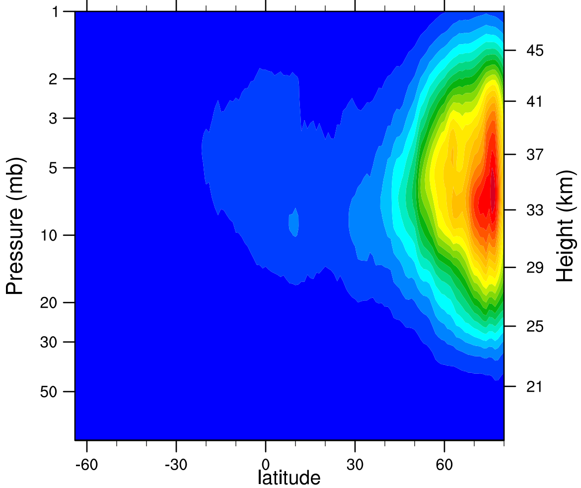
2005d337 N2O5_Ascending (ppbv)
