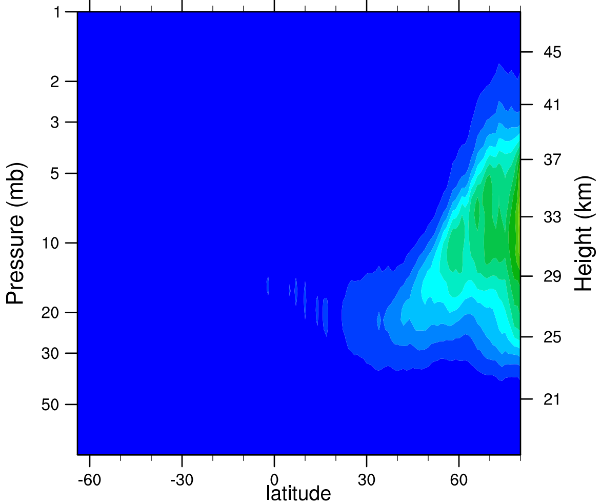
2007d051 N2O5_Ascending (ppbv)
