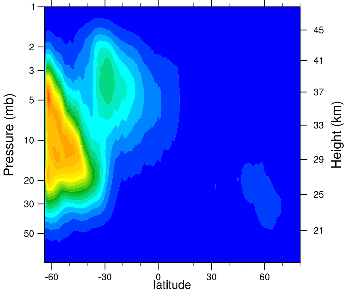
2007d122 N2O5_Ascending (ppbv)
