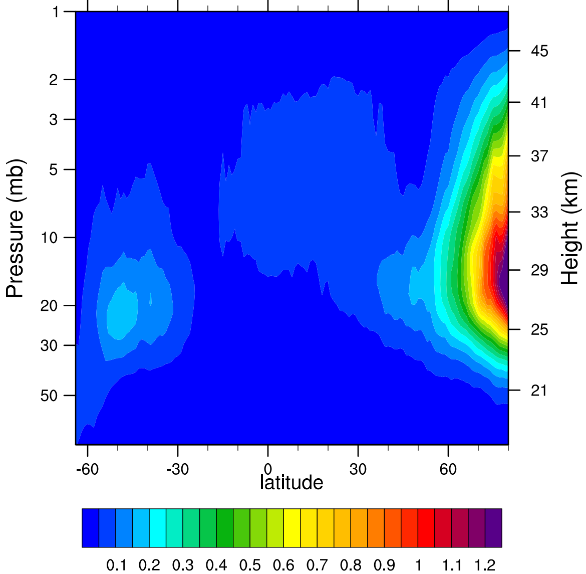
2007d302 N2O5_Ascending (ppbv)
