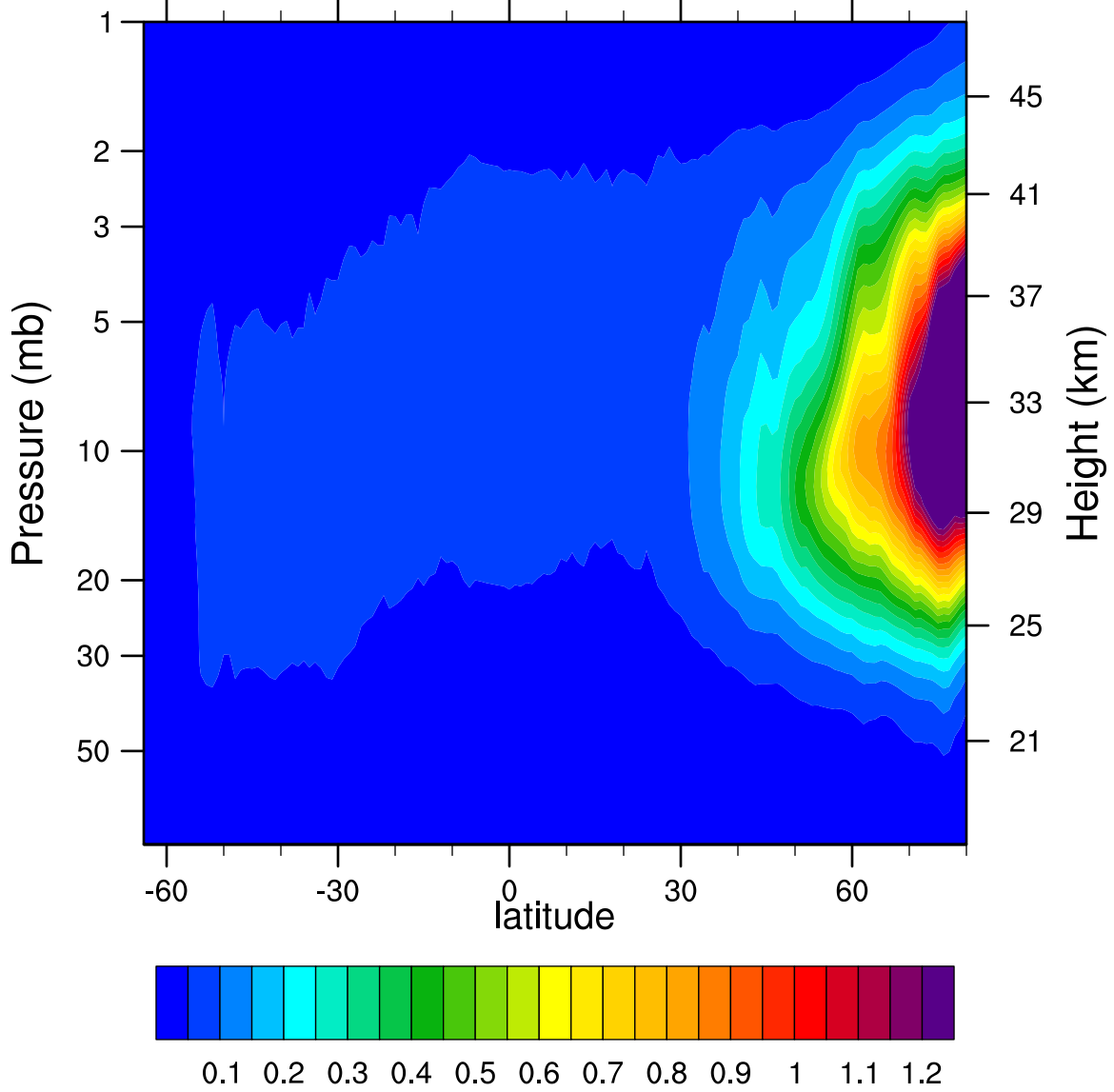
2007d346 N2O5_Ascending (ppbv)
