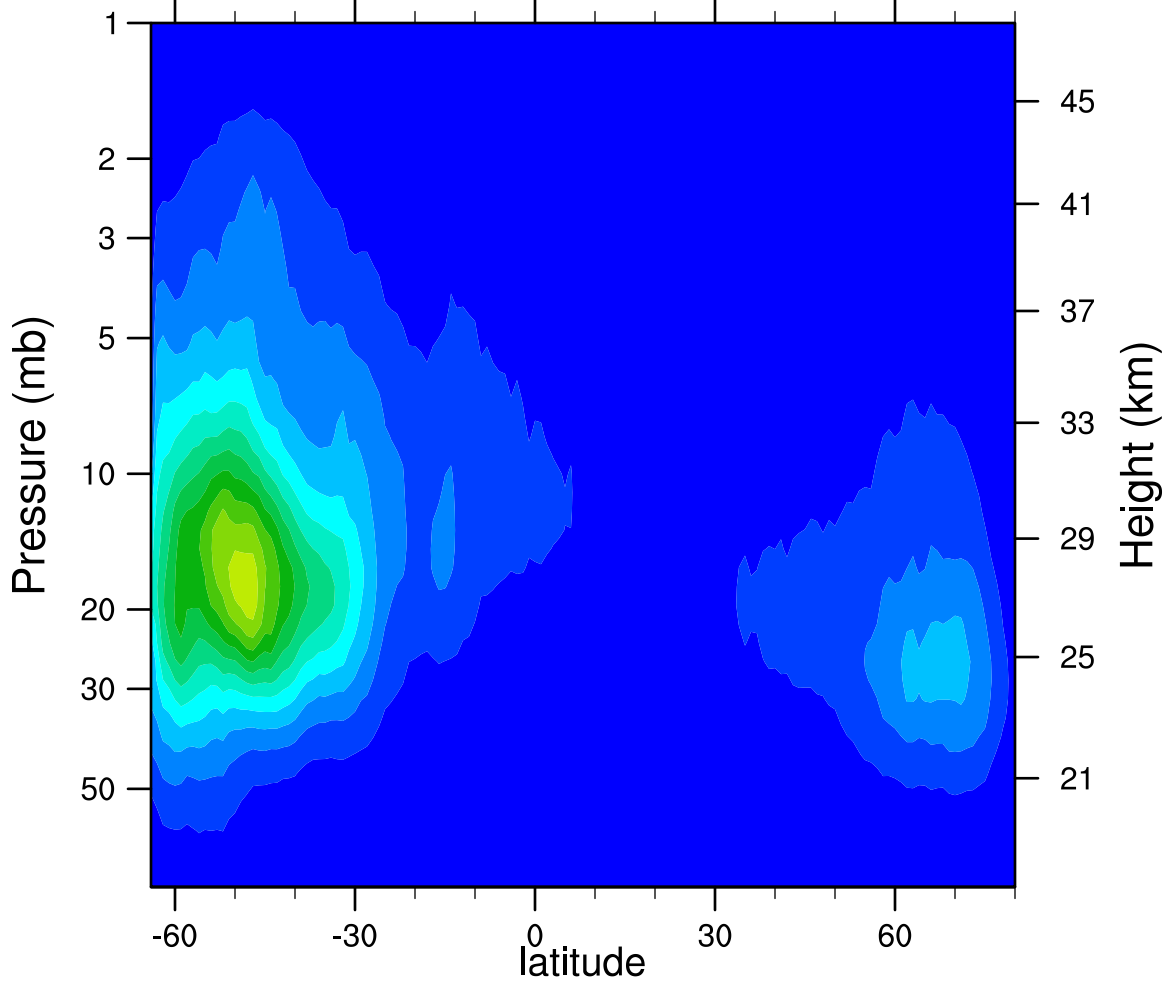
2007d245 N2O5_Ascending (ppbv)
