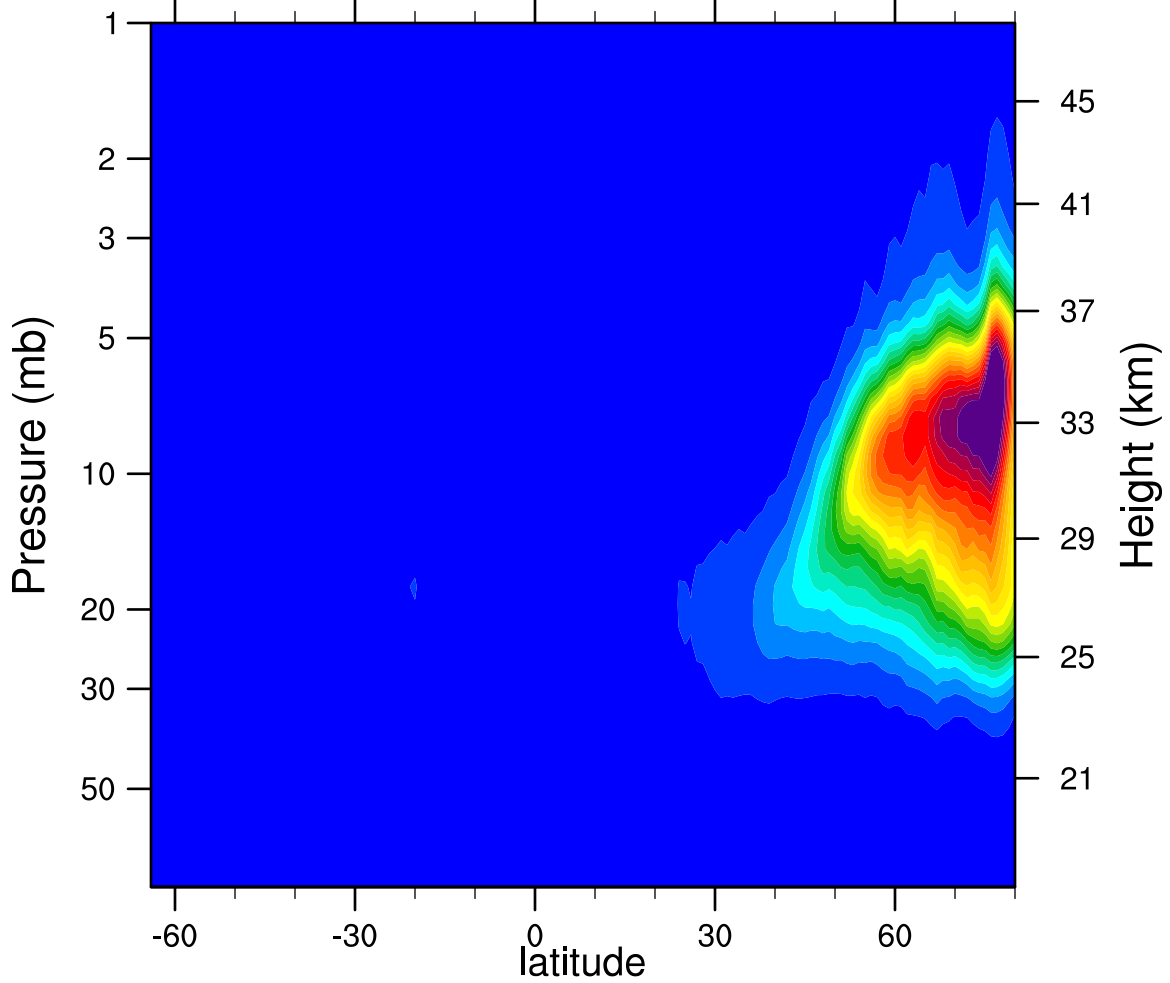
2007d008 N2O5_Ascending (ppbv)
