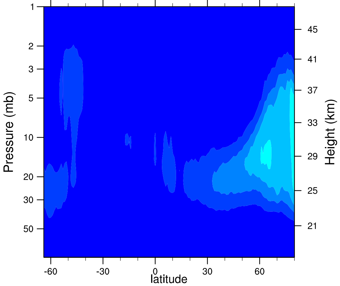
2007d070 N2O5_Ascending (ppbv)
