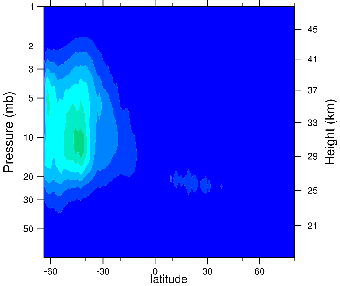
2007d169 N2O5_Ascending (ppbv)
