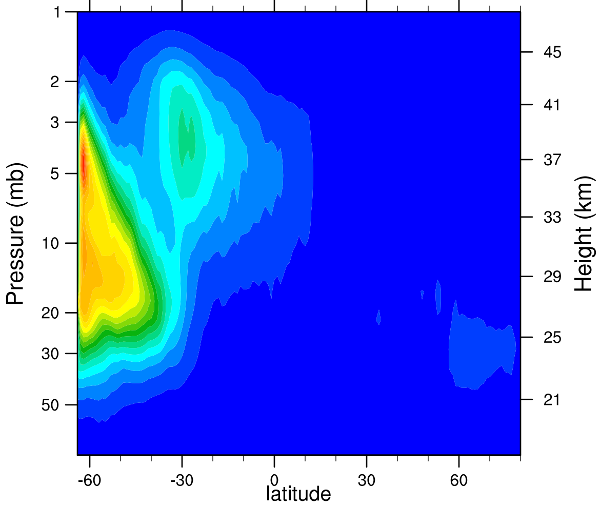
2007d114 N2O5_Ascending (ppbv)
