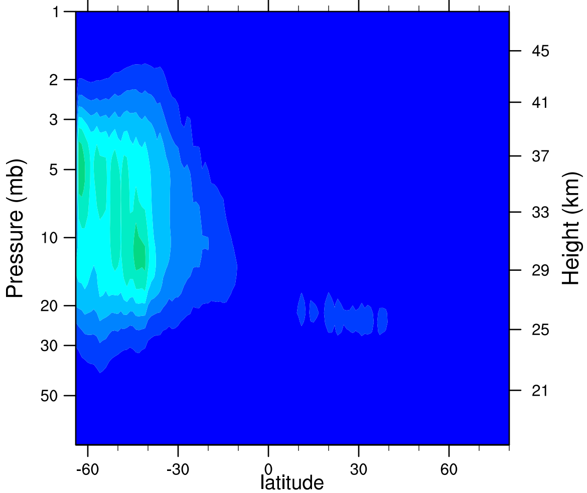
2007d166 N2O5_Ascending (ppbv)
