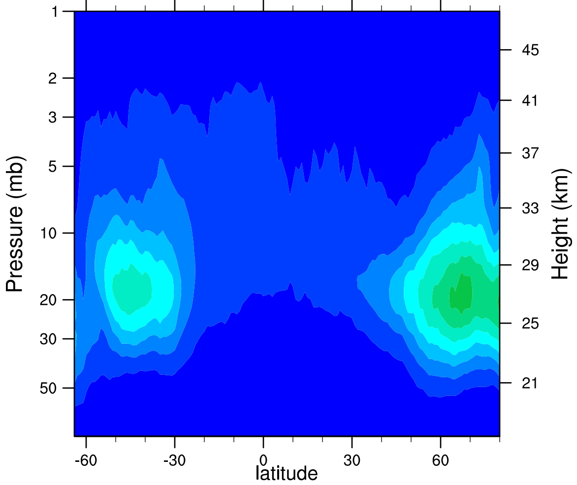
2007d270 N2O5_Ascending (ppbv)
