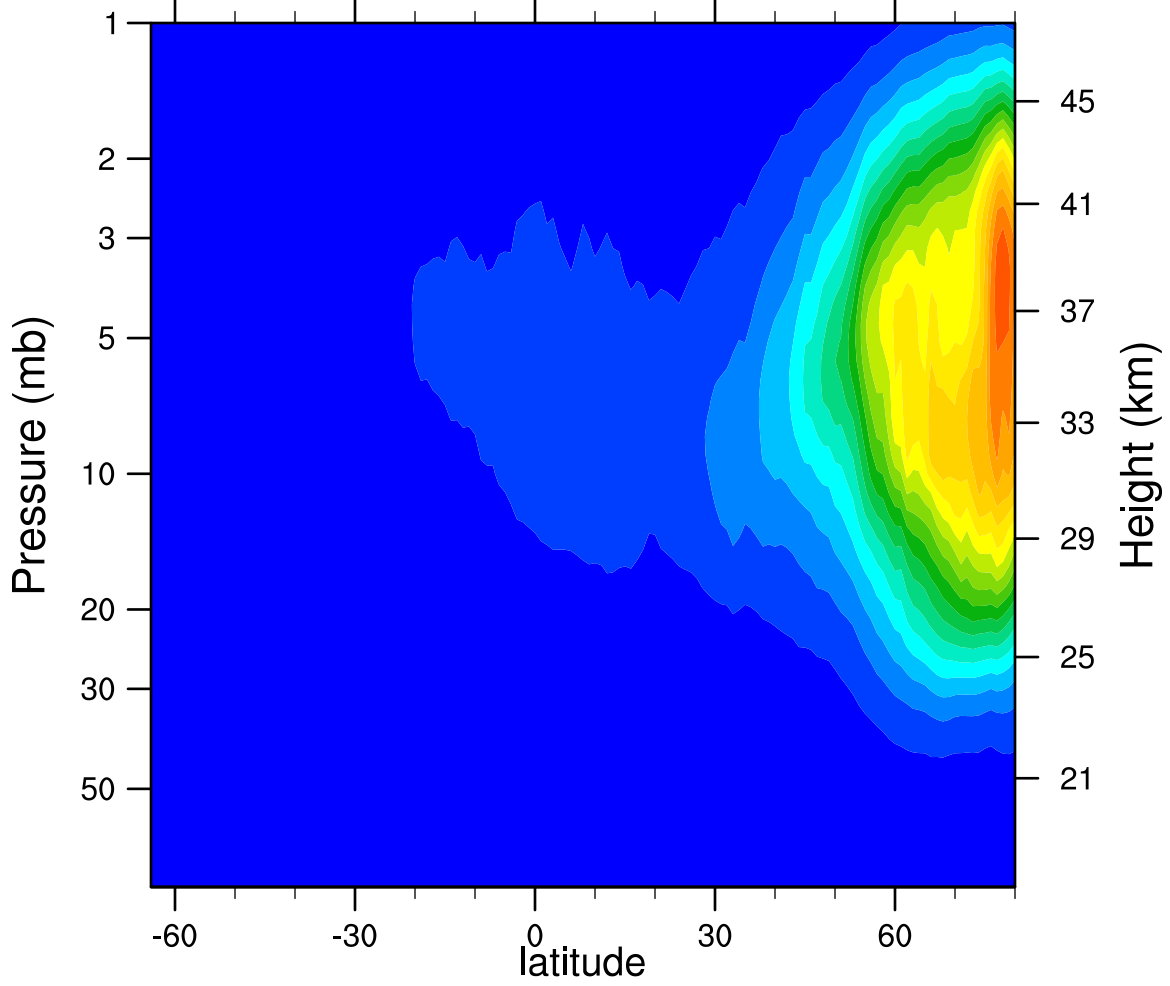
2005d327 N2O5_Ascending (ppbv)
