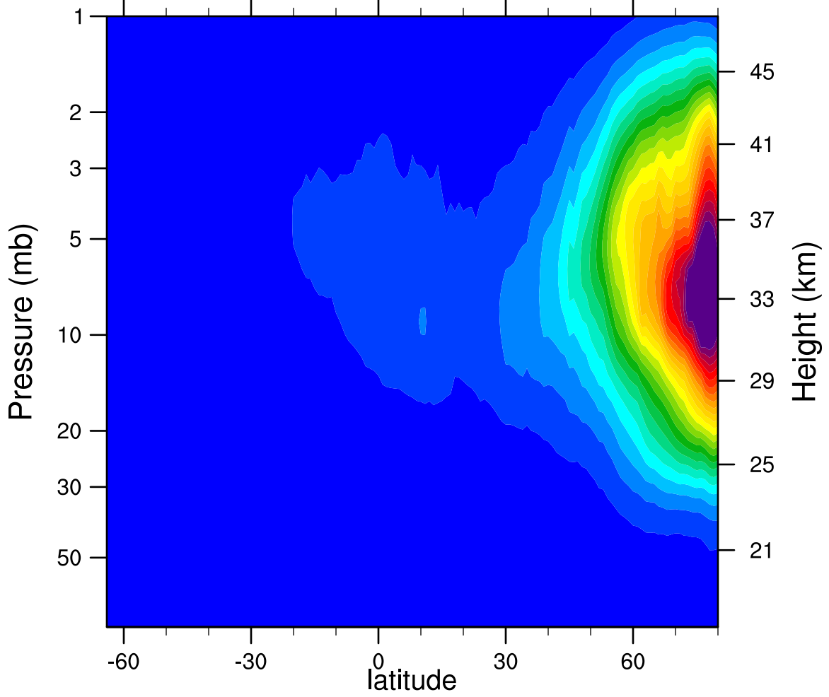
2005d329 N2O5_Ascending (ppbv)
