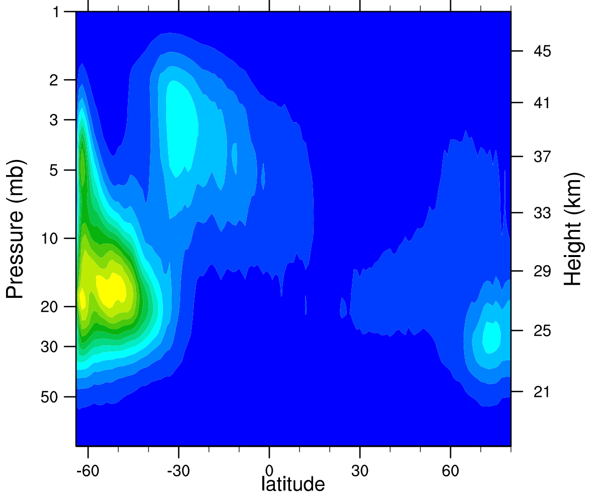
2007d096 N2O5_Ascending (ppbv)
