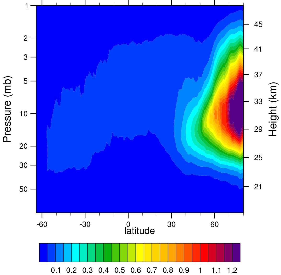
2007d335 N2O5_Ascending (ppbv)
