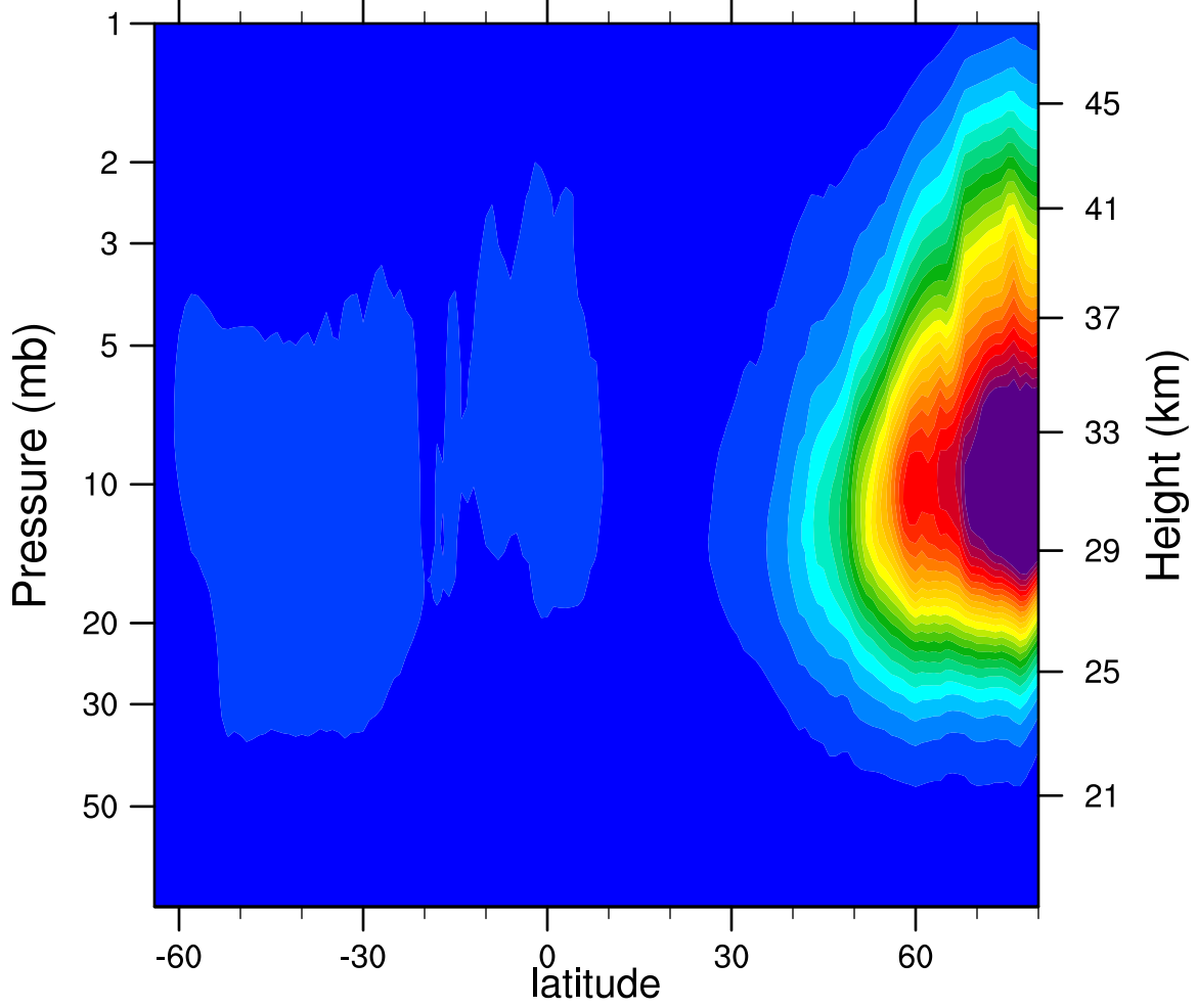
2007d365 N2O5_Ascending (ppbv)
