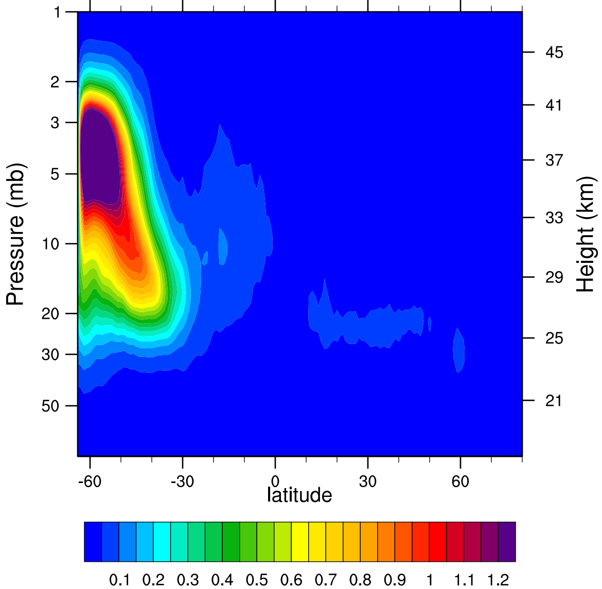
2007d148 N2O5_Ascending (ppbv)
