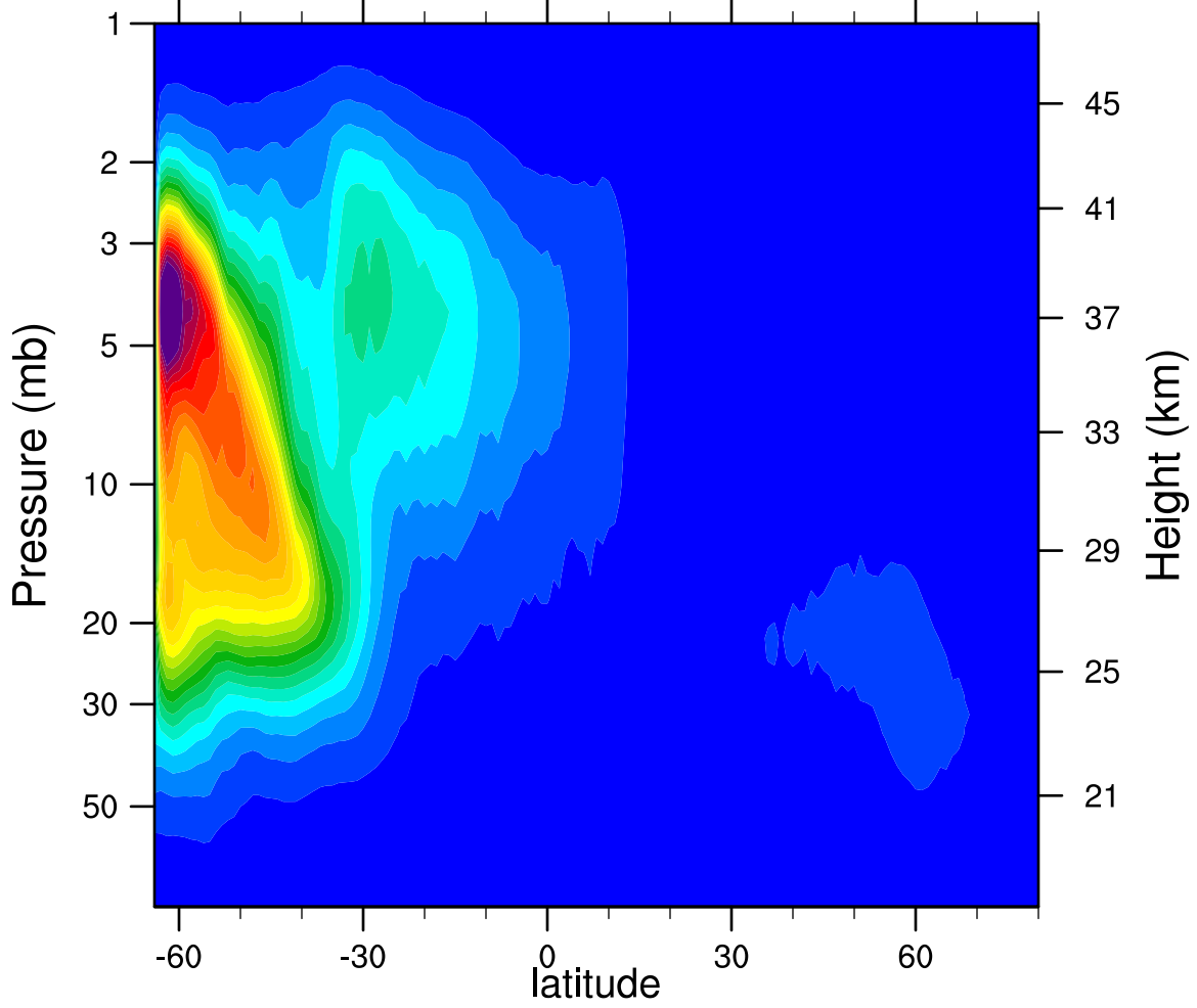
2007d126 N2O5_Ascending (ppbv)
