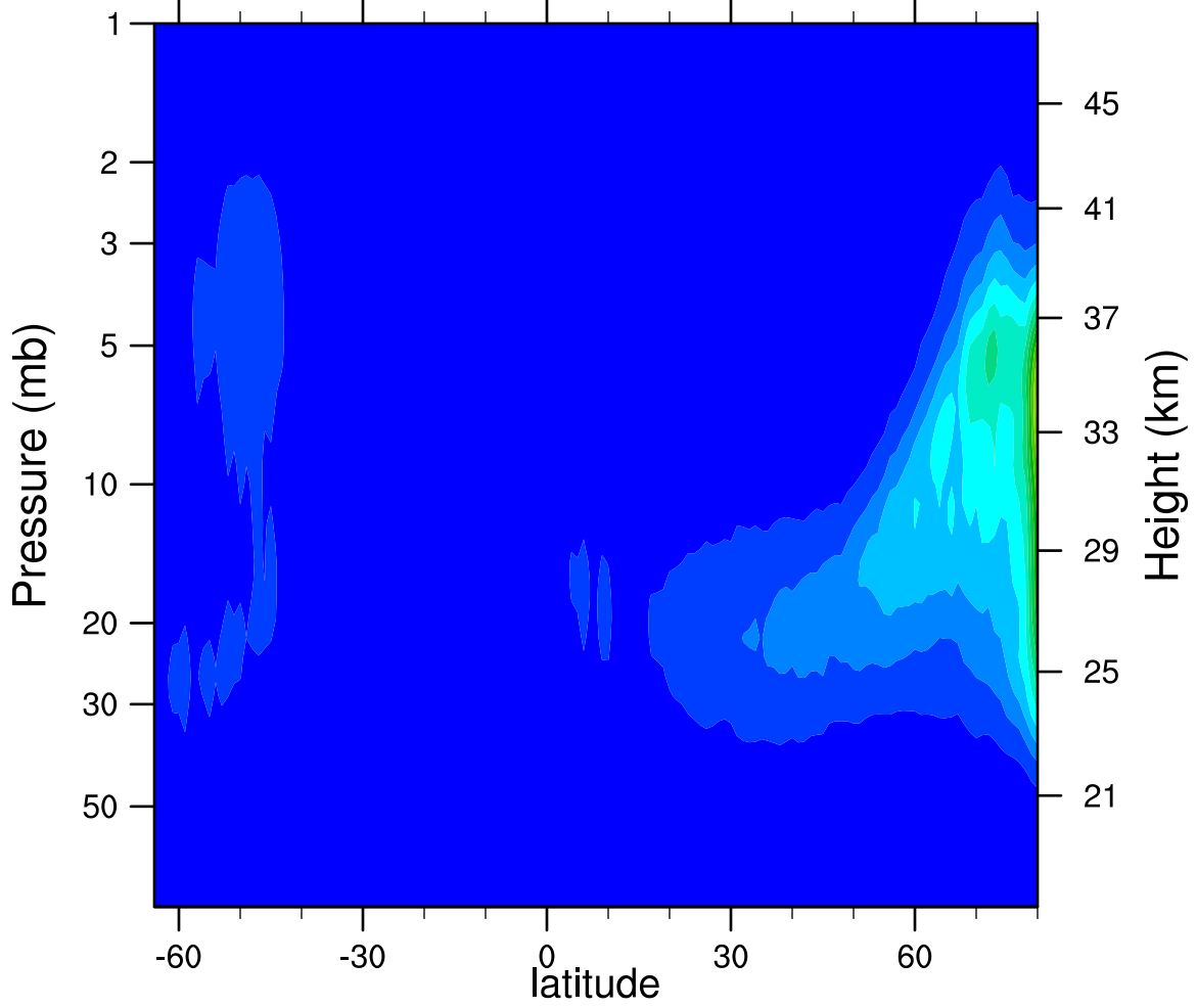
2007d063 N2O5_Ascending (ppbv)
