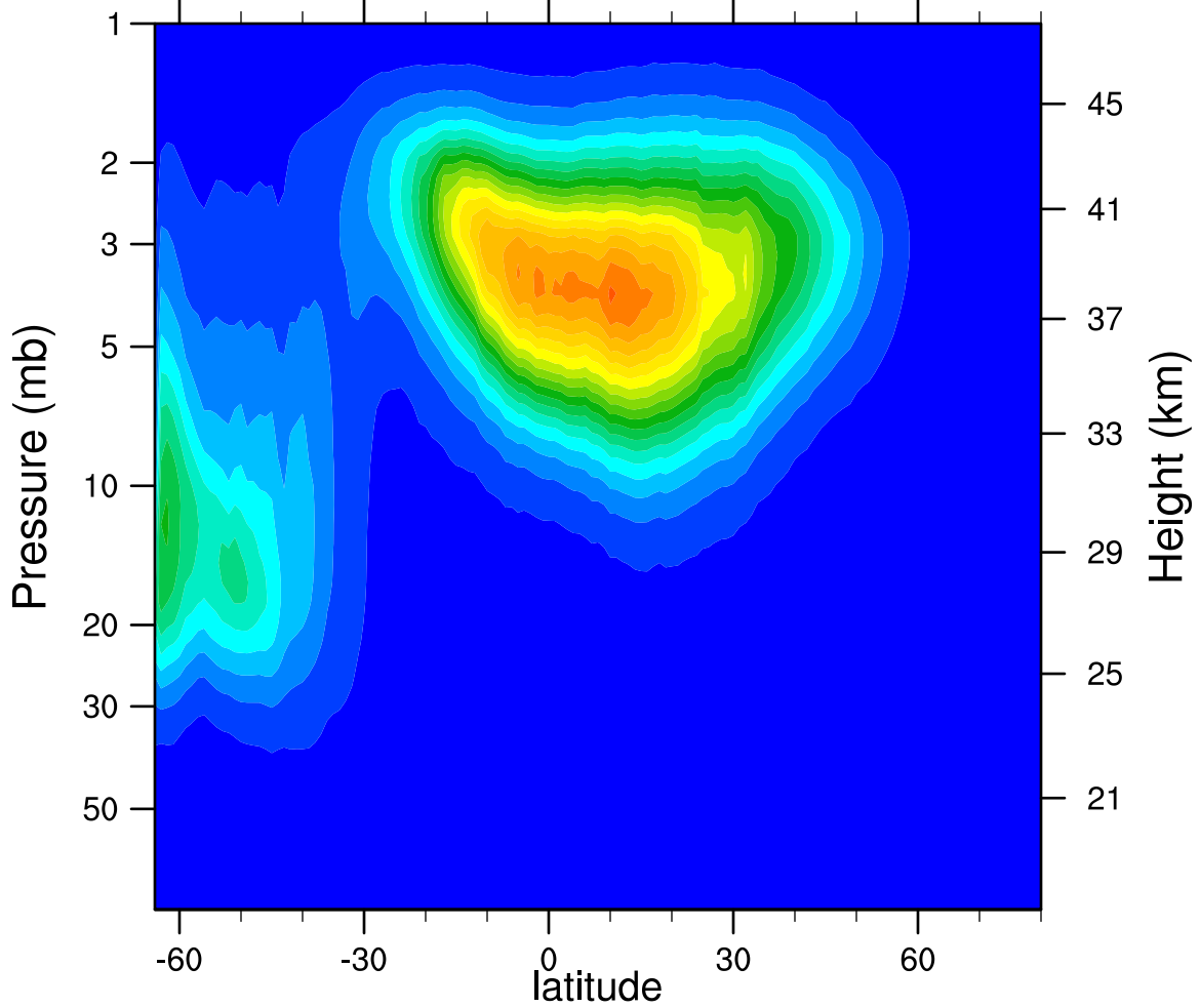
2005d124 N2O5_Ascending (ppbv)
