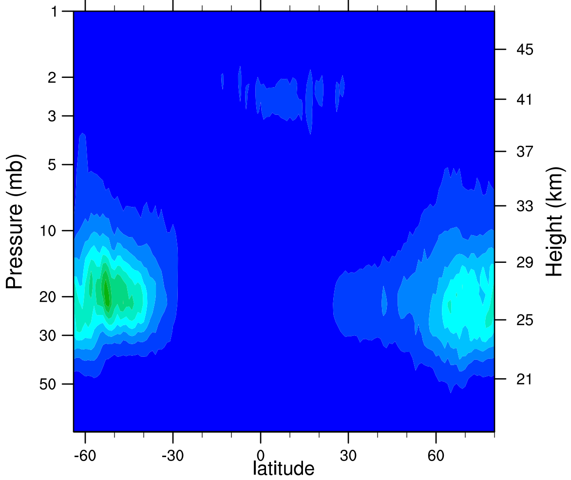
2007d079 N2O5_Ascending (ppbv)
