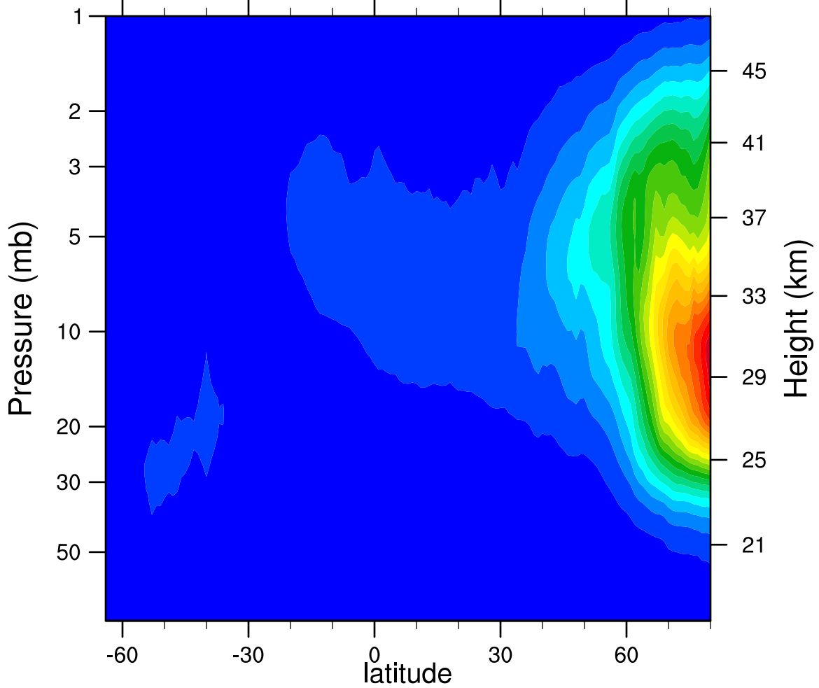
2005d310 N2O5_Ascending (ppbv)
