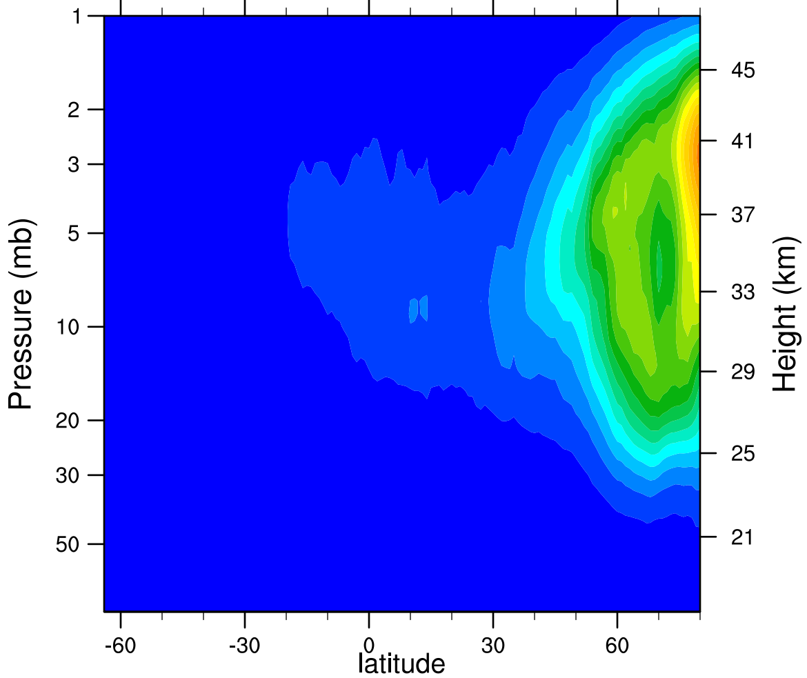
2005d322 N2O5_Ascending (ppbv)
