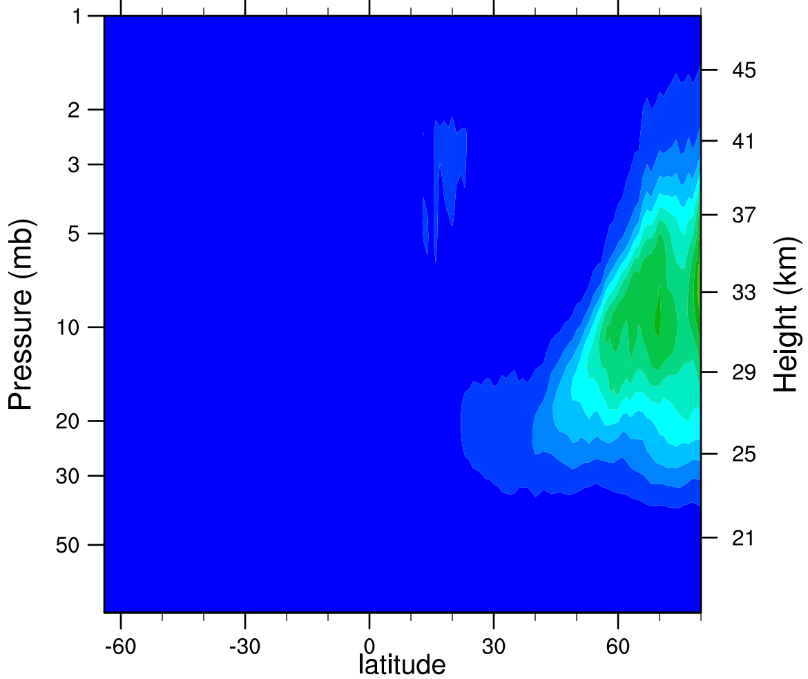
2007d049 N2O5_Ascending (ppbv)
