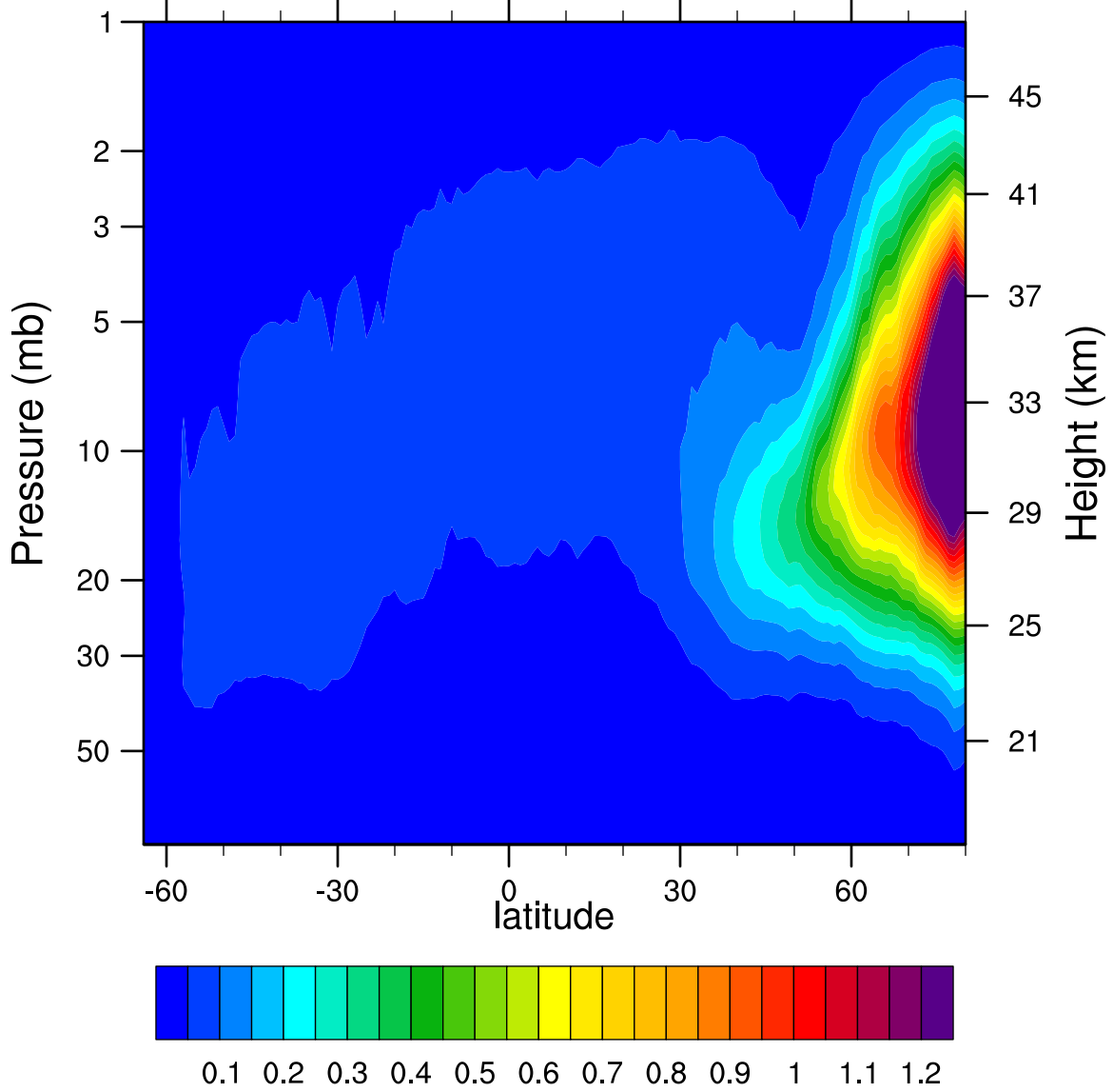
2007d329 N2O5_Ascending (ppbv)
