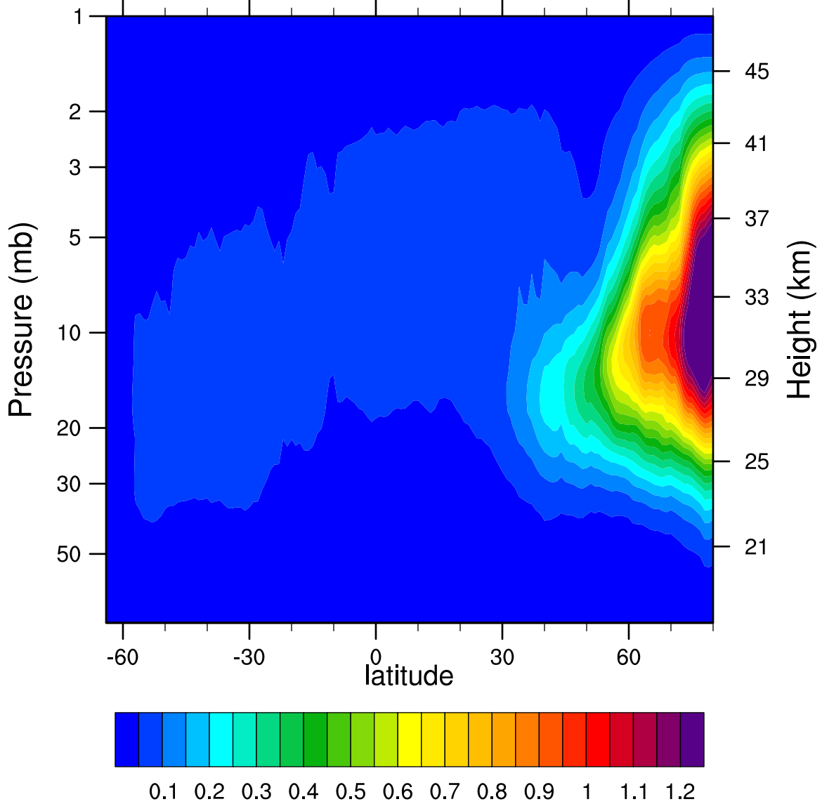
2007d326 N2O5_Ascending (ppbv)
