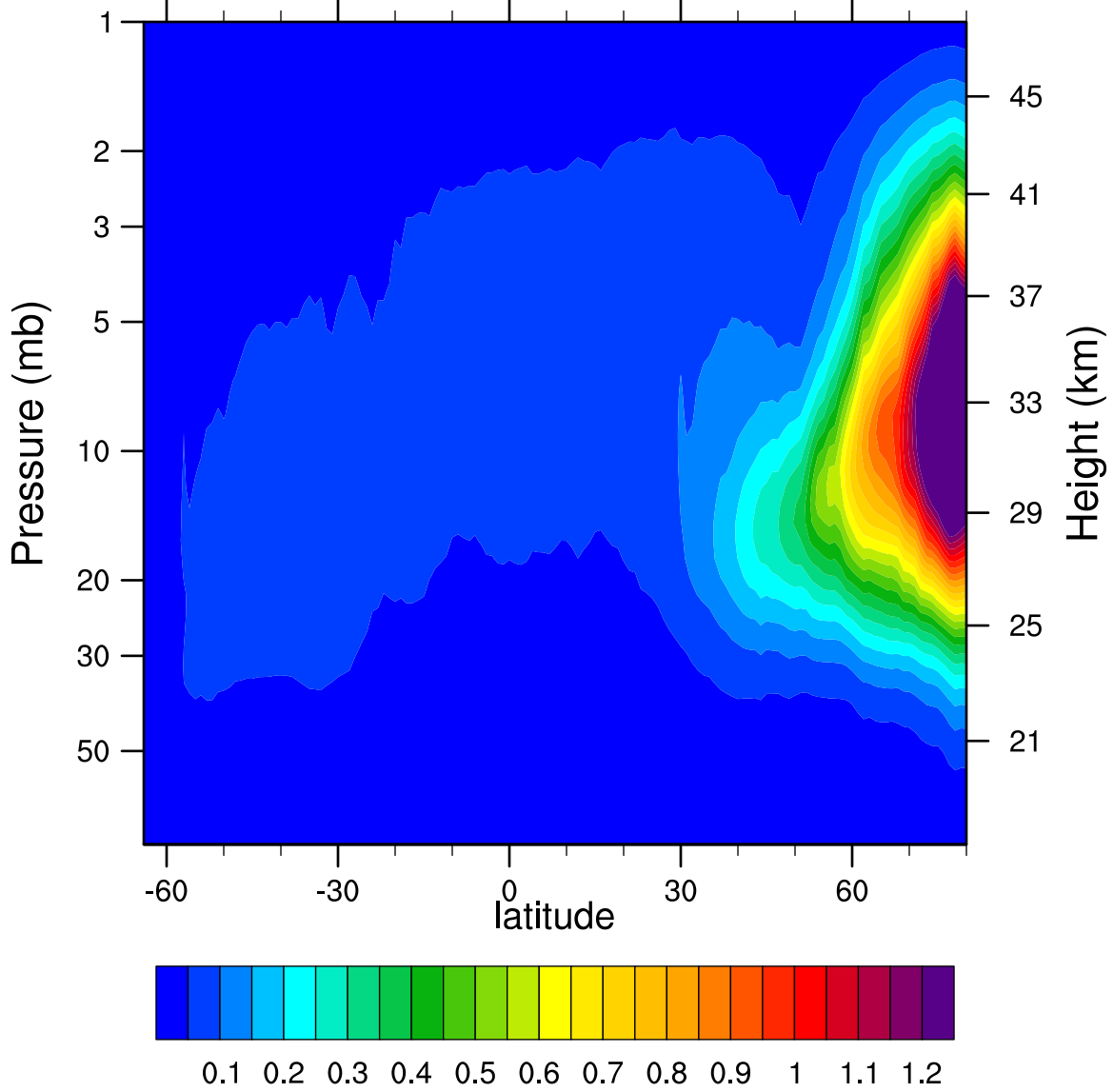
2007d330 N2O5_Ascending (ppbv)
