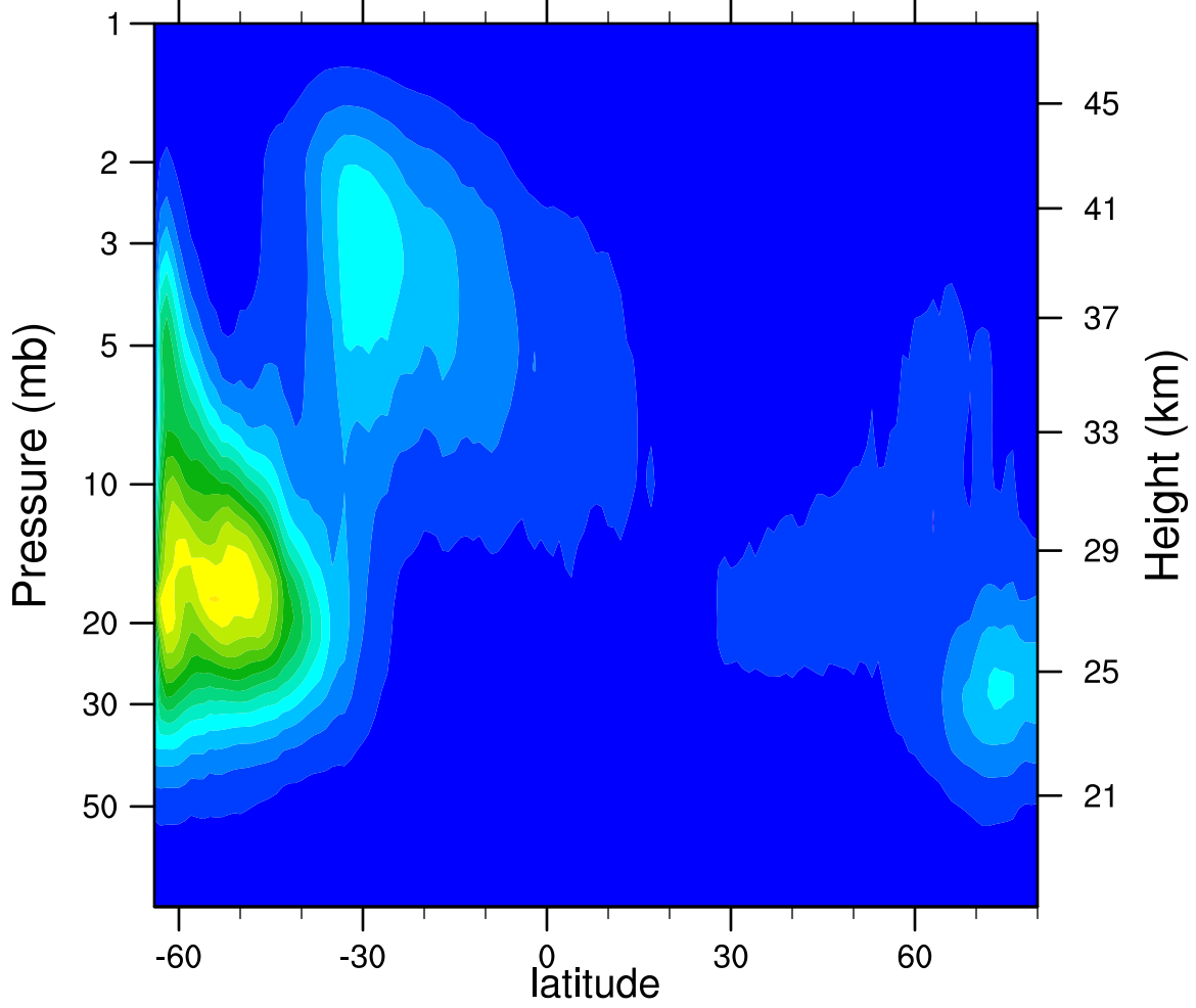
2007d097 N2O5_Ascending (ppbv)
