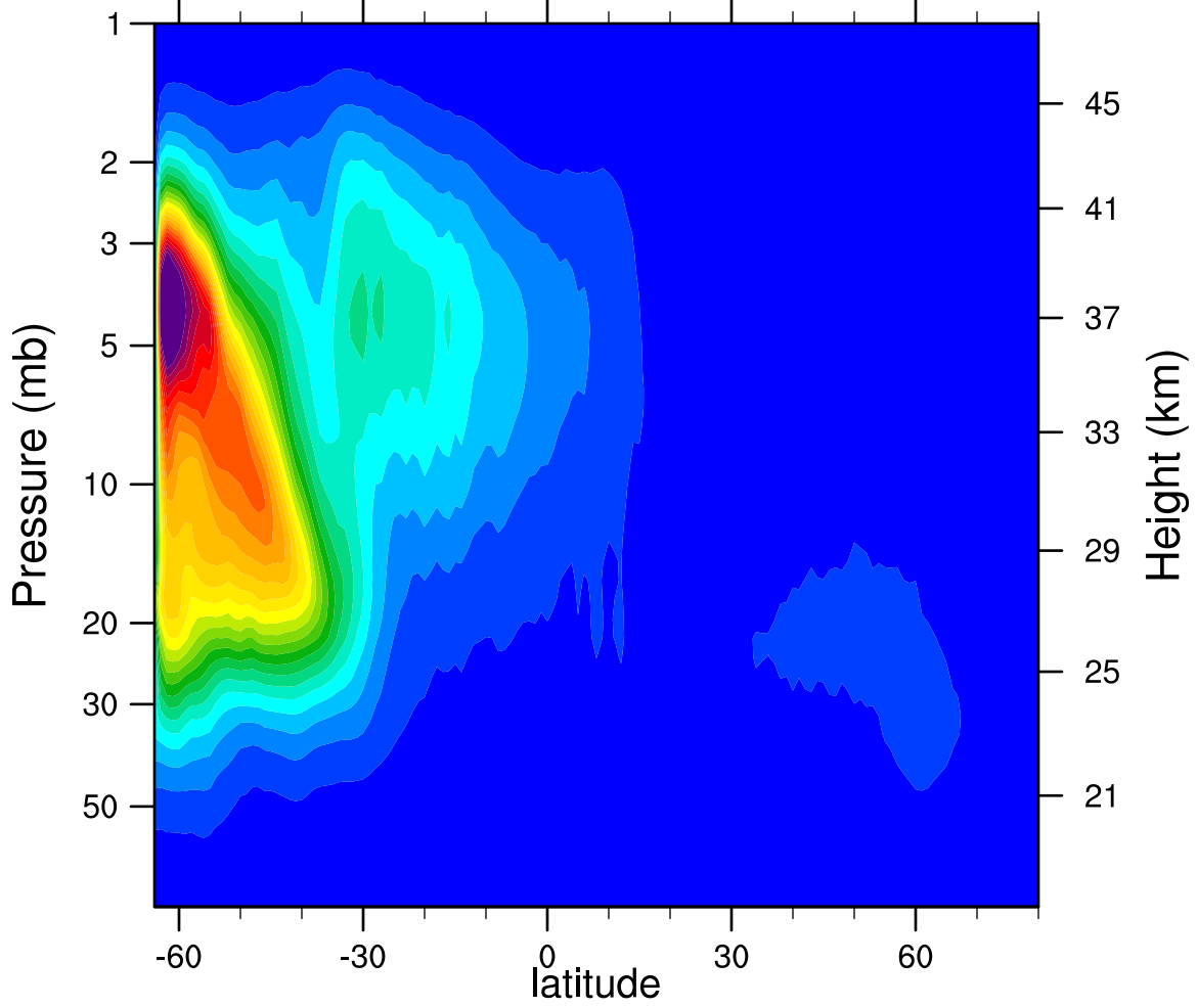
2007d128 N2O5_Ascending (ppbv)
