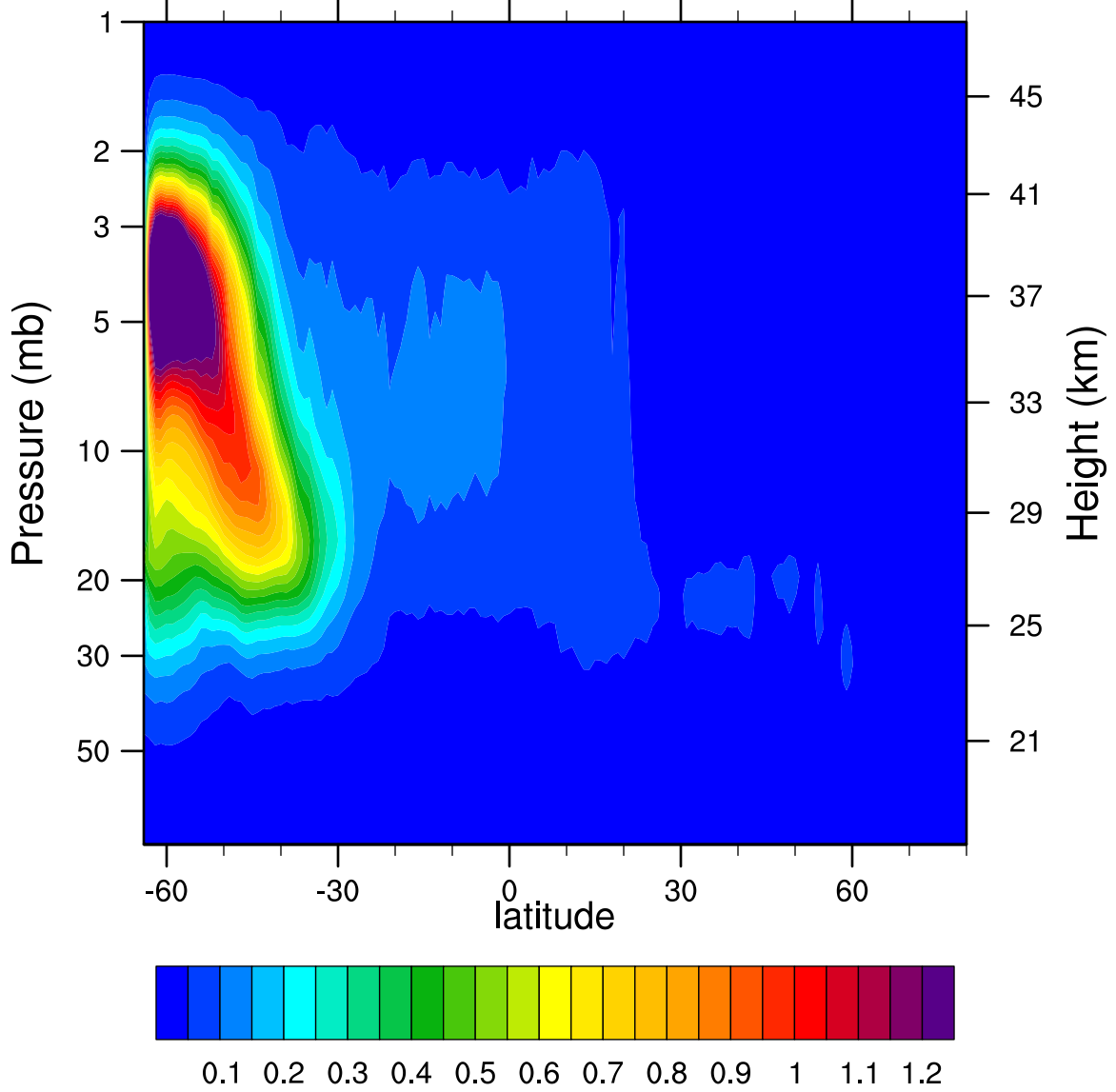
2007d142 N2O5_Ascending (ppbv)
