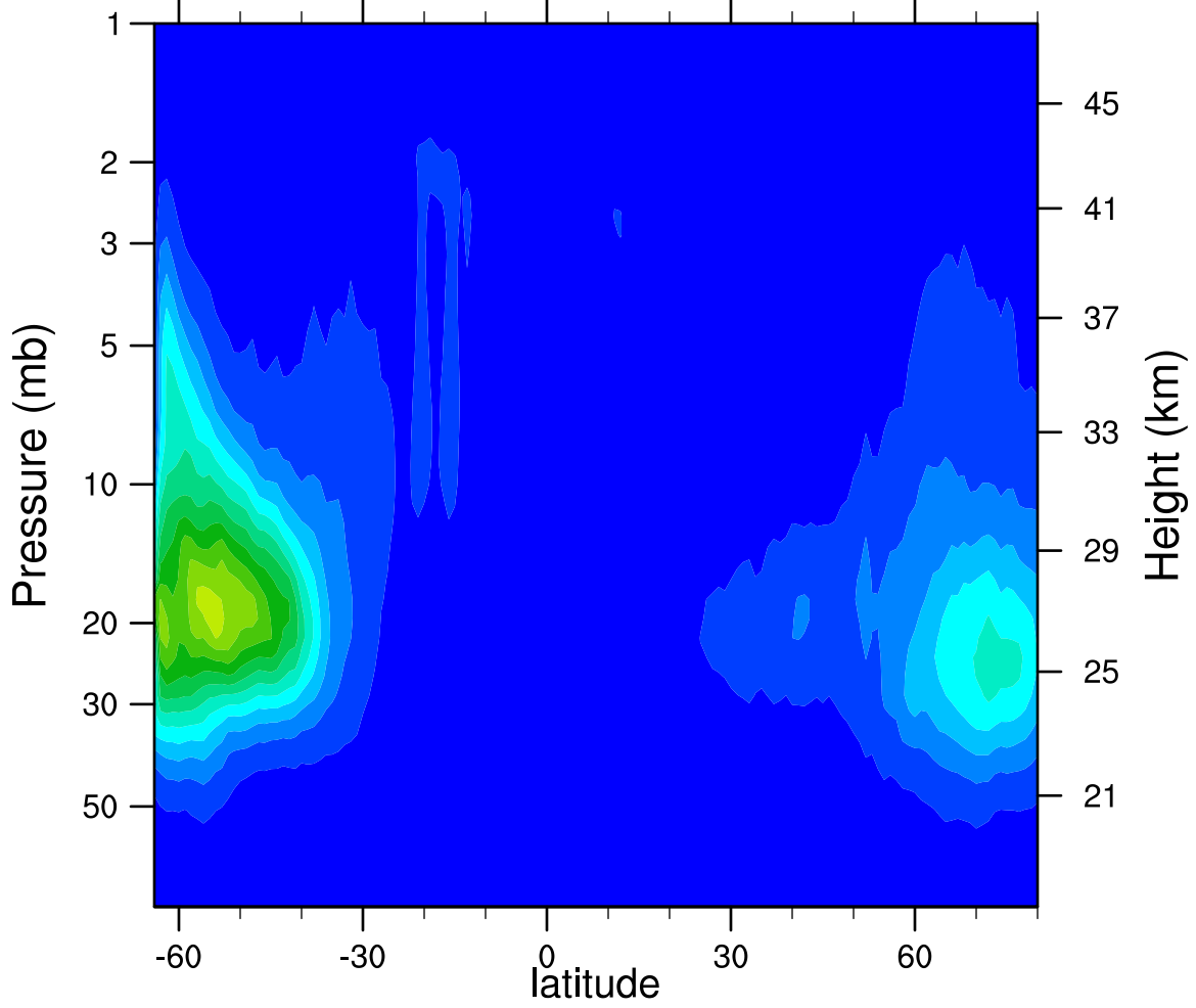
2007d083 N2O5_Ascending (ppbv)
