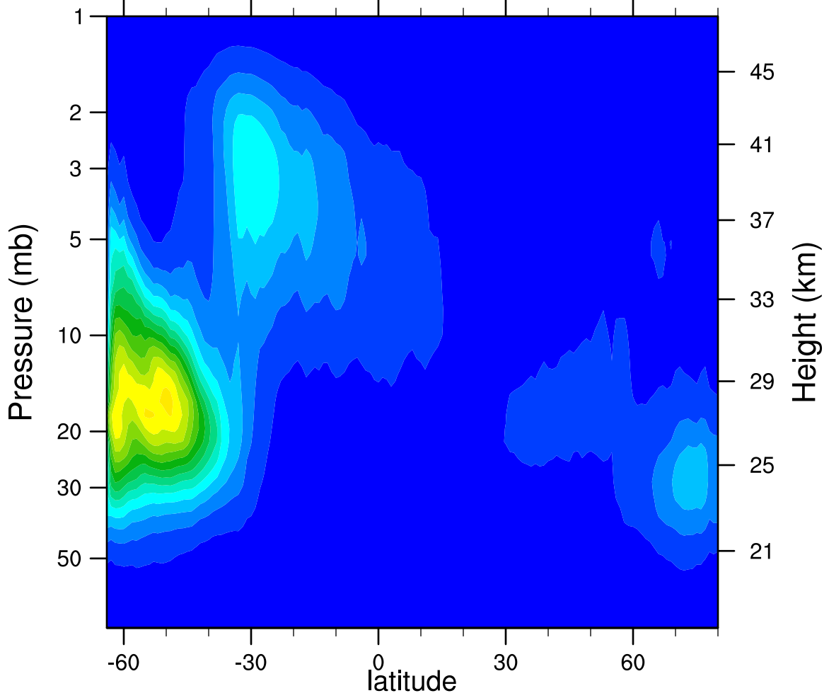
2007d099 N2O5_Ascending (ppbv)
