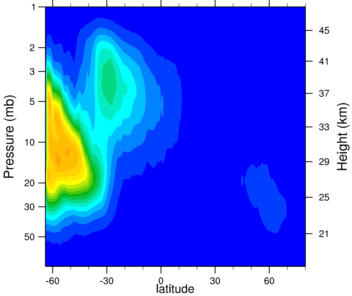
2007d121 N2O5_Ascending (ppbv)
