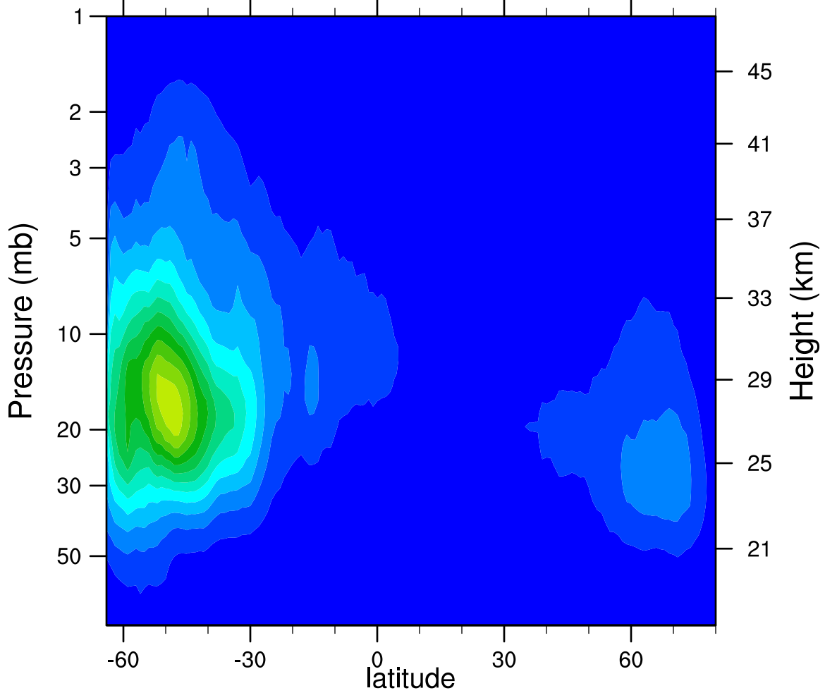
2007d243 N2O5_Ascending (ppbv)
