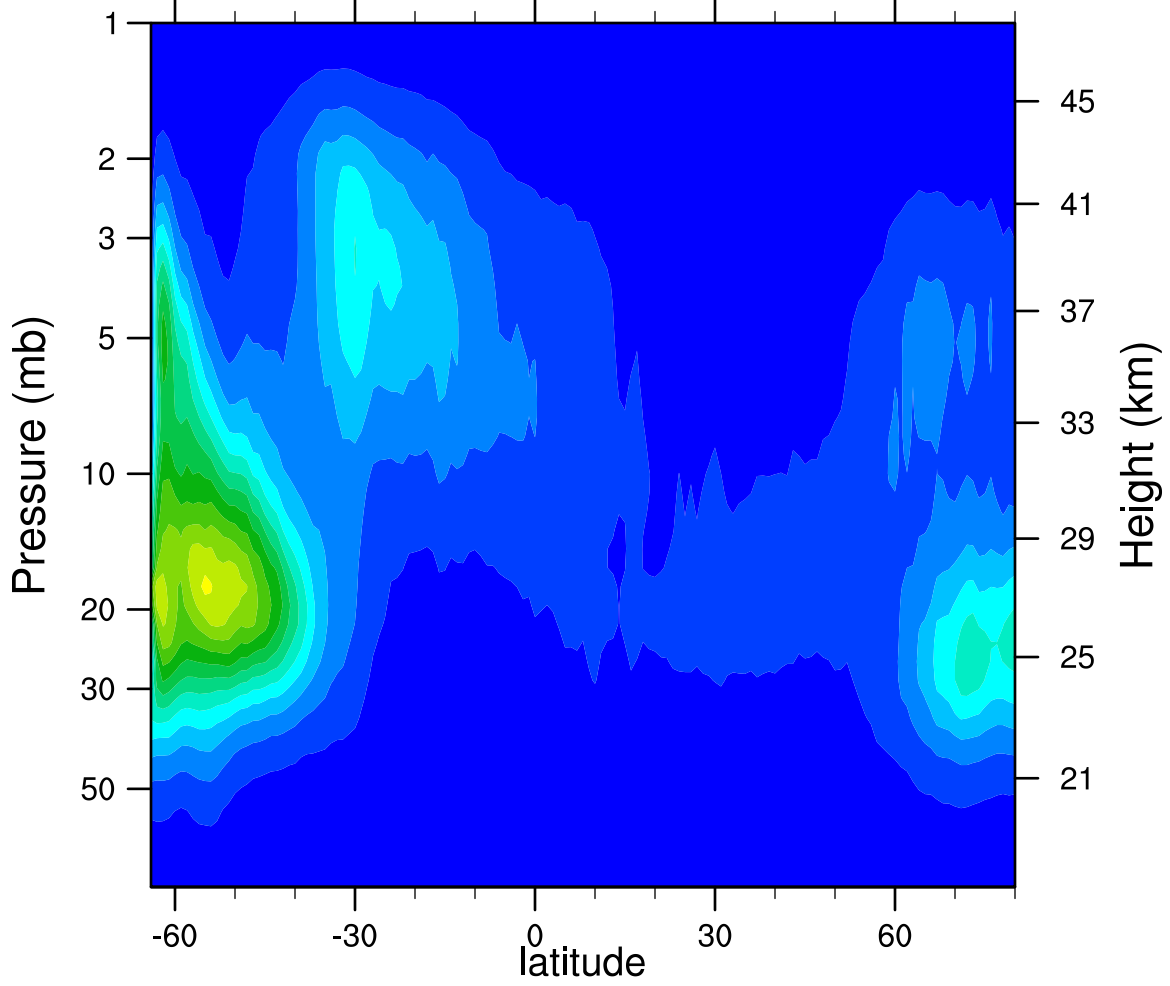
2007d090 N2O5_Ascending (ppbv)
