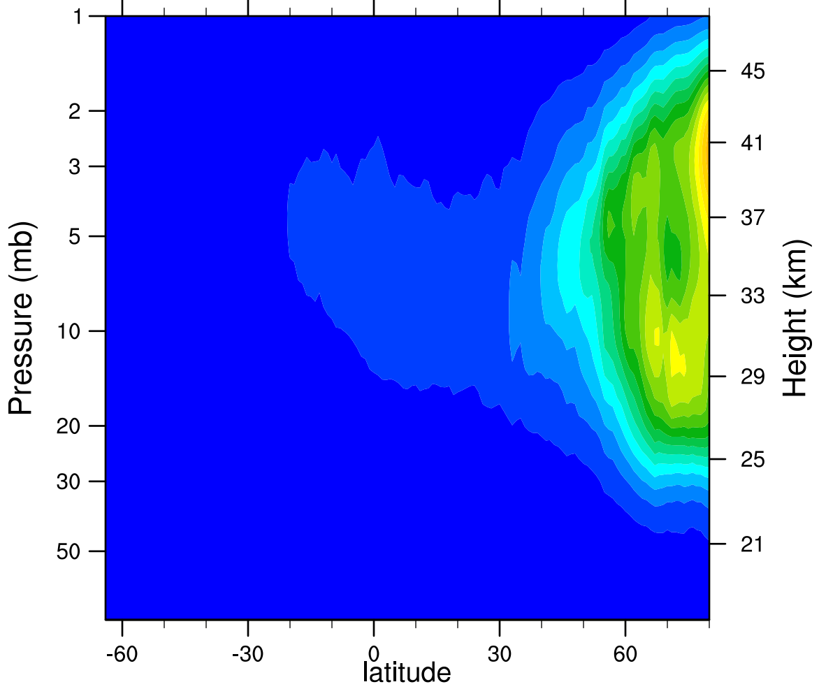
2005d318 N2O5_Ascending (ppbv)
