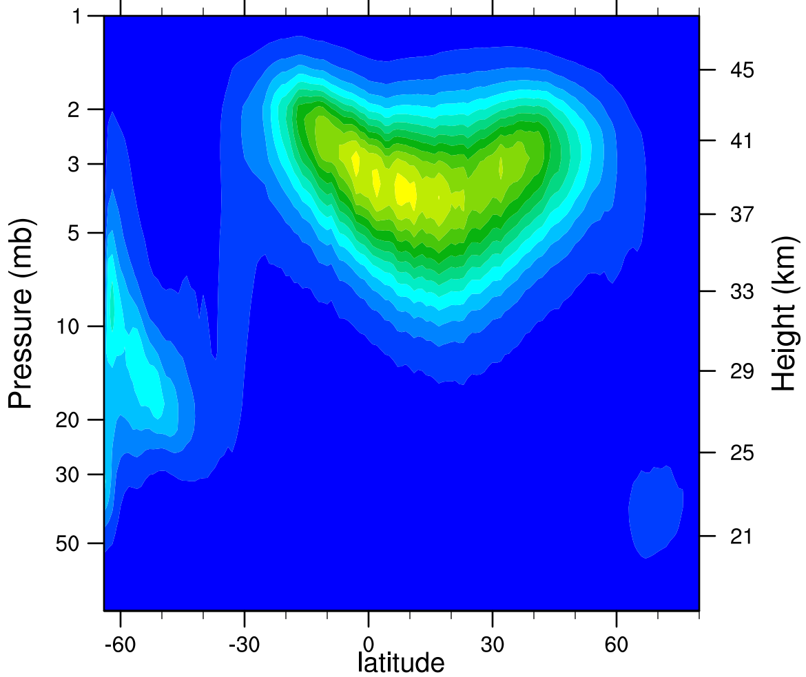
2005d099 N2O5_Ascending (ppbv)
