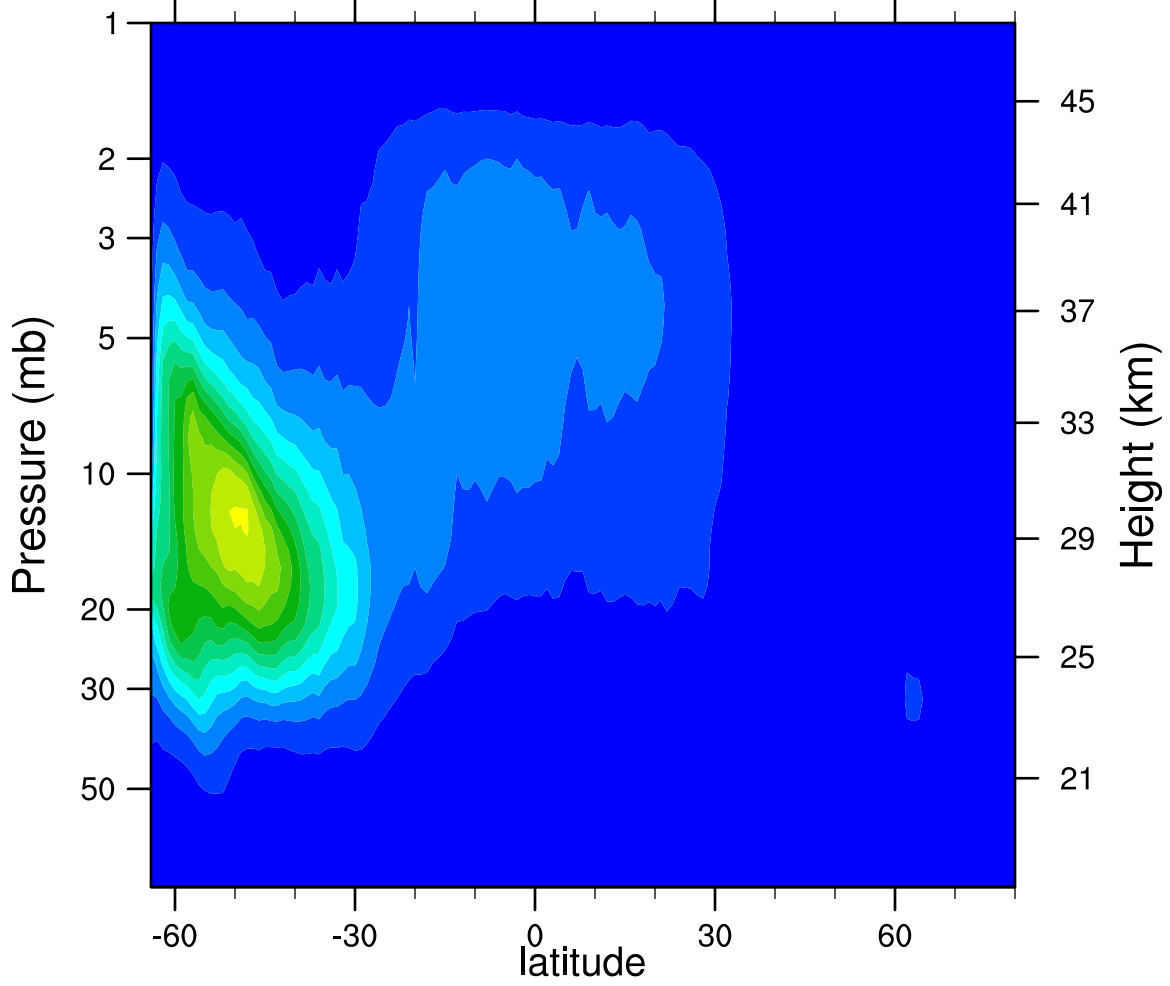
2007d225 N2O5_Ascending (ppbv)
