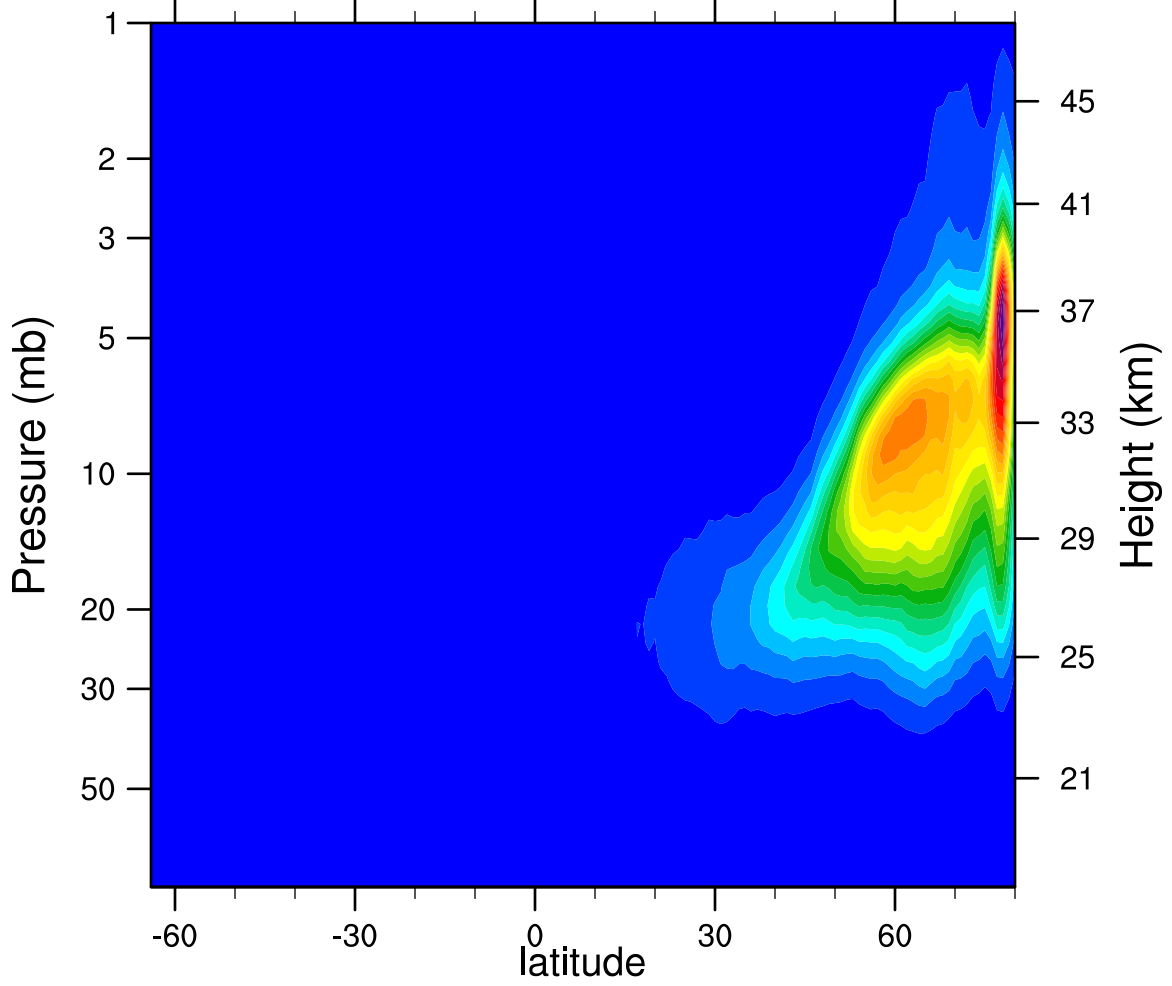
2007d018 N2O5_Ascending (ppbv)
