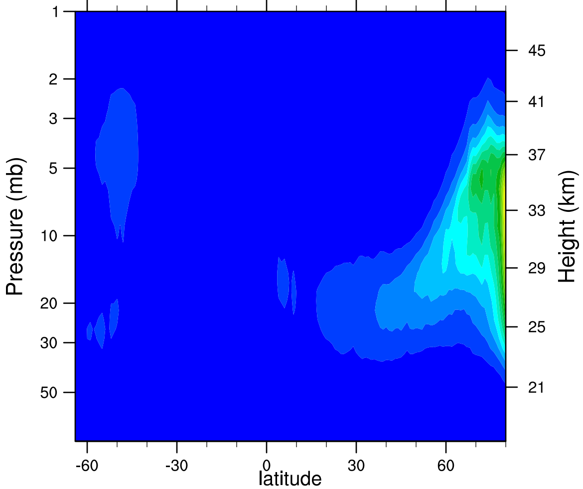
2007d061 N2O5_Ascending (ppbv)
