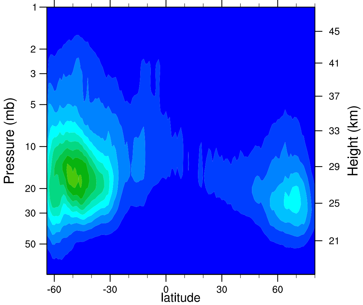
2007d249 N2O5_Ascending (ppbv)
