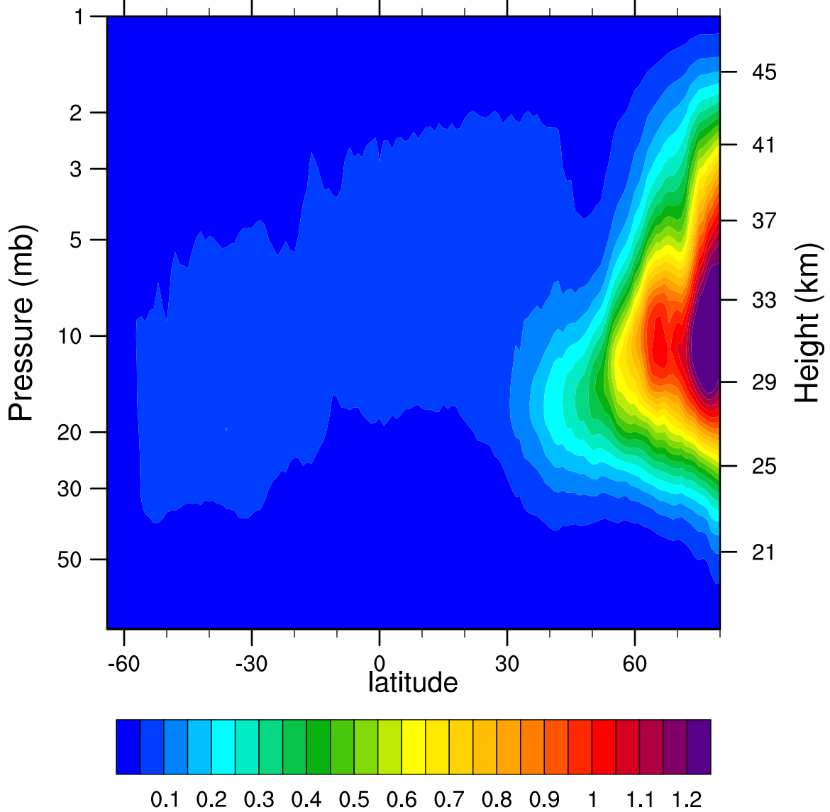
2007d324 N2O5_Ascending (ppbv)
