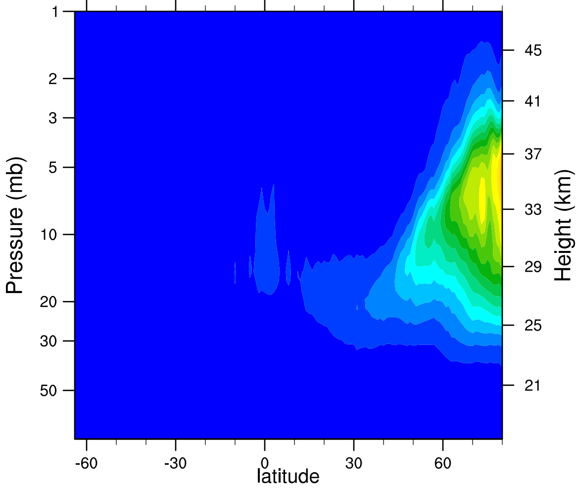
2007d041 N2O5_Ascending (ppbv)
