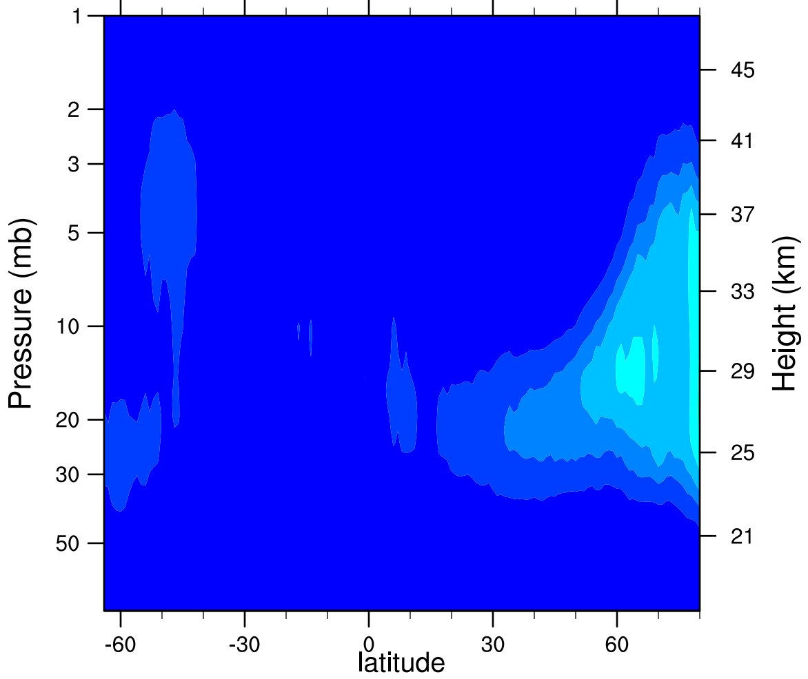
2007d069 N2O5_Ascending (ppbv)
