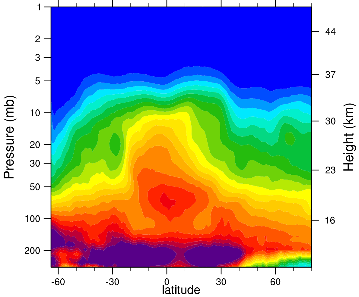
2007d159 N2O_Combined (ppbv)
