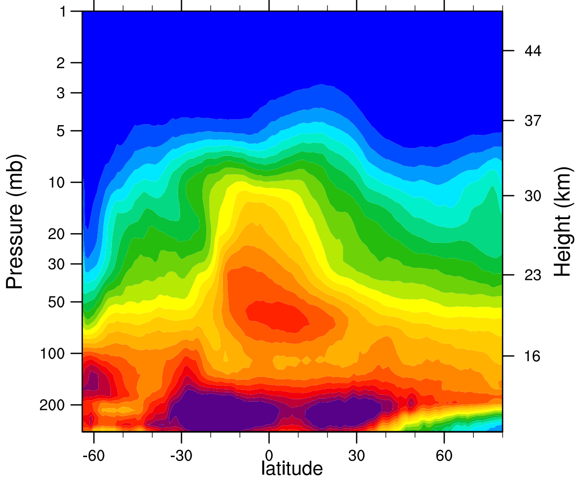
2005d177 N2O_Combined (ppbv)
