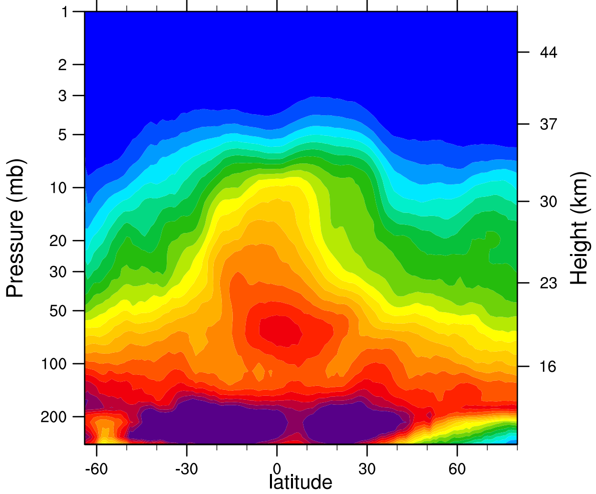
2007d137 N2O_Combined (ppbv)
