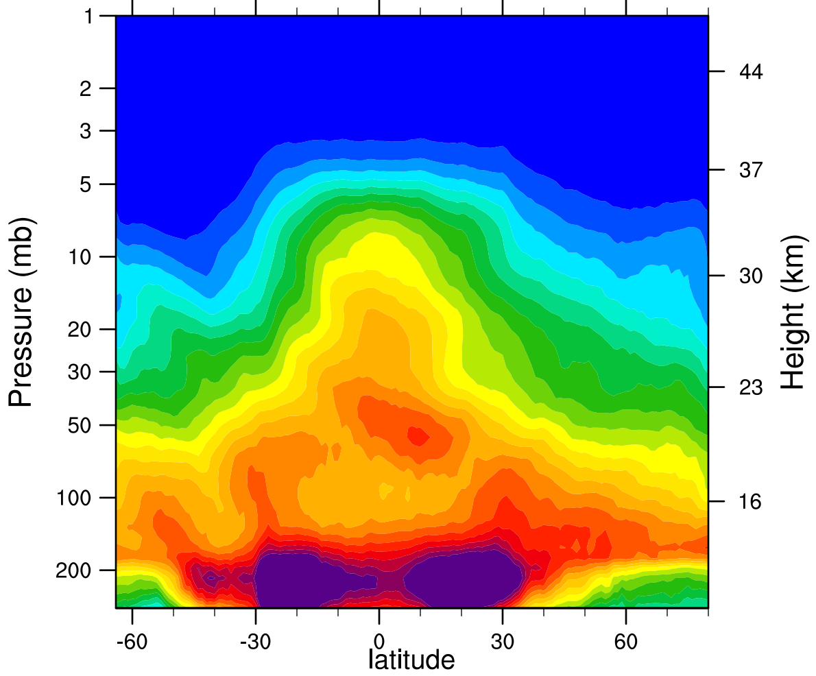
2005d090 N2O_Combined (ppbv)
