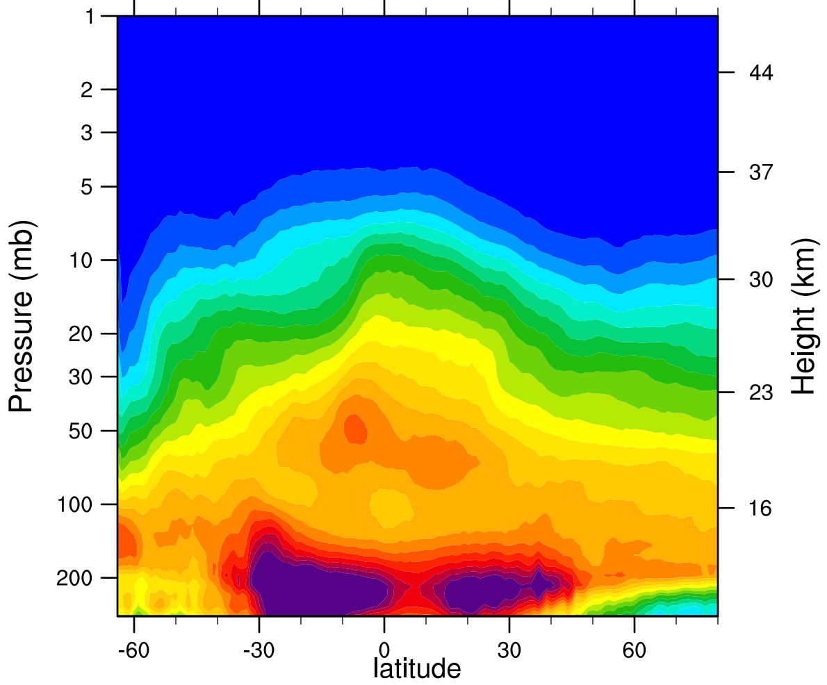
2006d176 N2O_Combined (ppbv)
