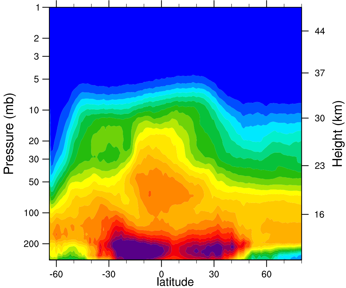
2007d208 N2O_Combined (ppbv)
