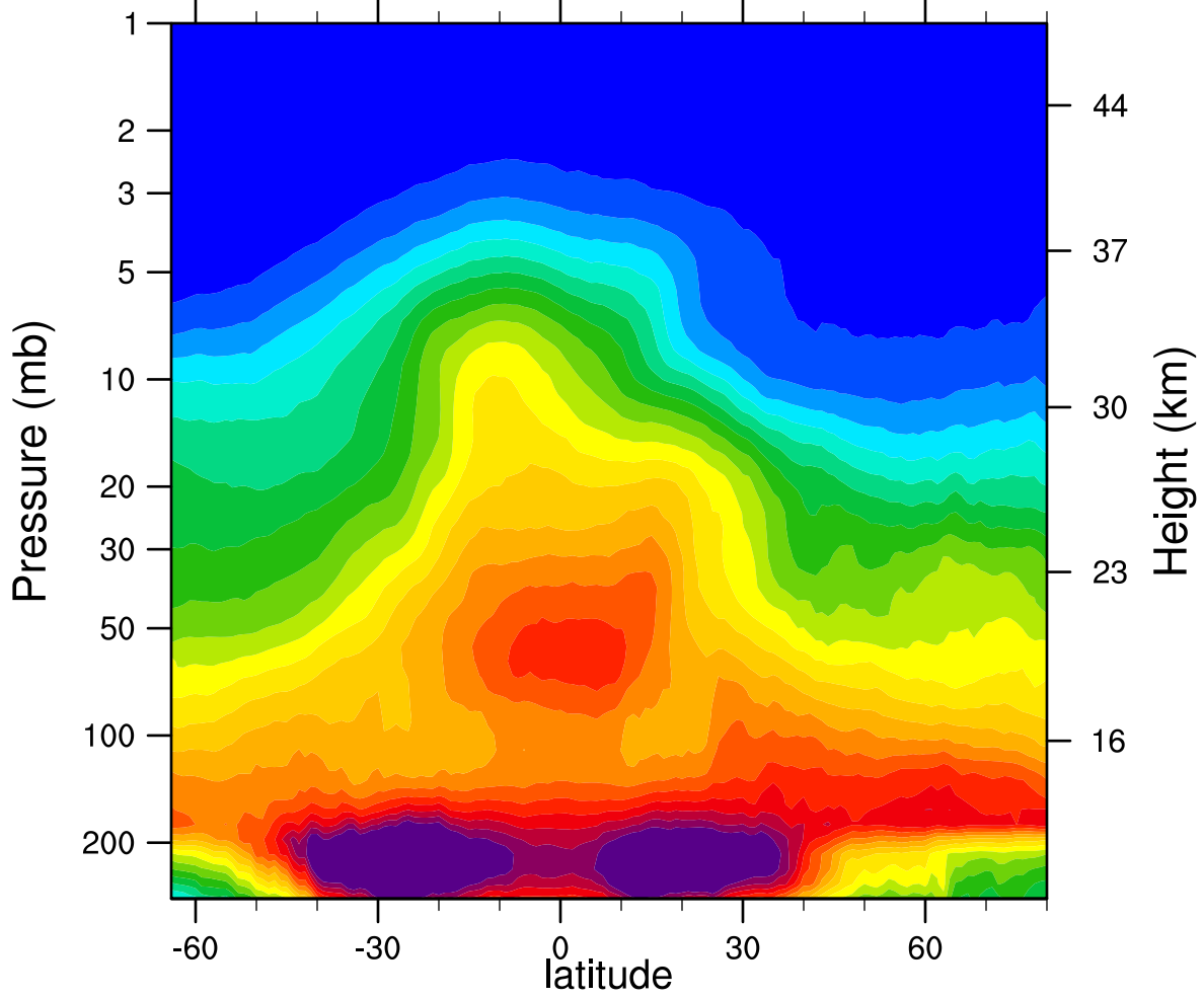
2006d042 N2O_Combined (ppbv)
