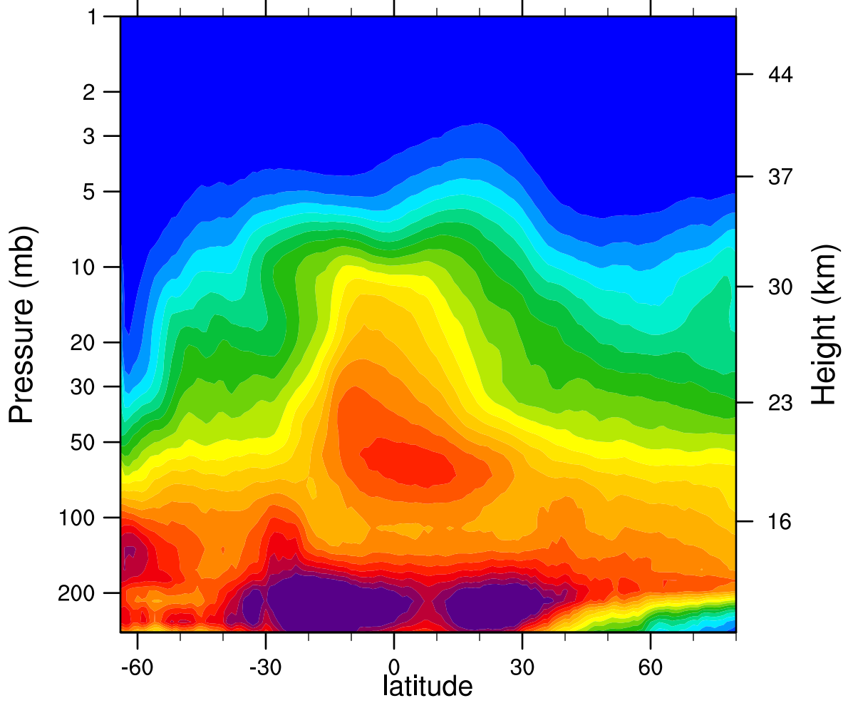
2005d172 N2O_Combined (ppbv)
