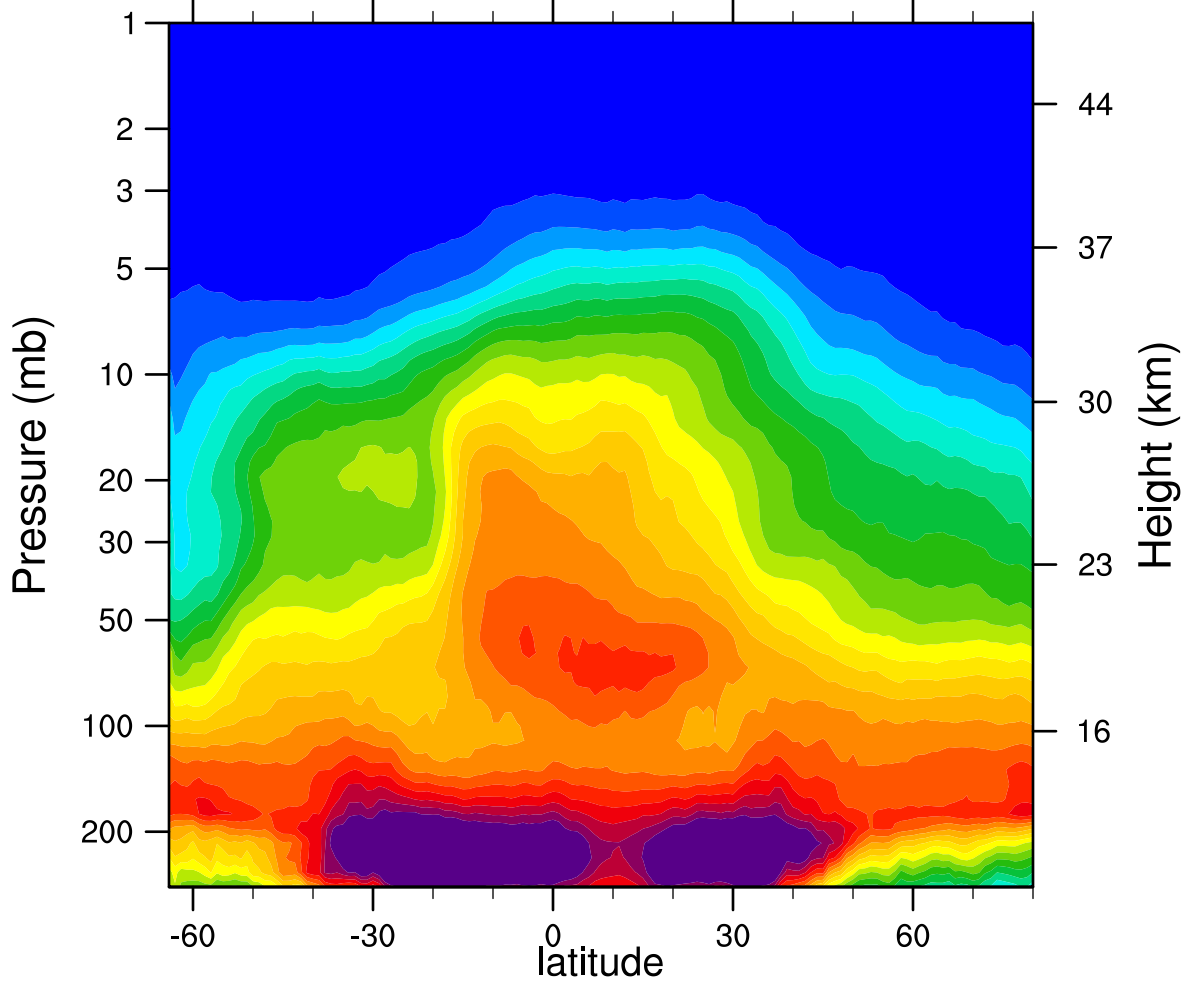
2007d276 N2O_Combined (ppbv)
