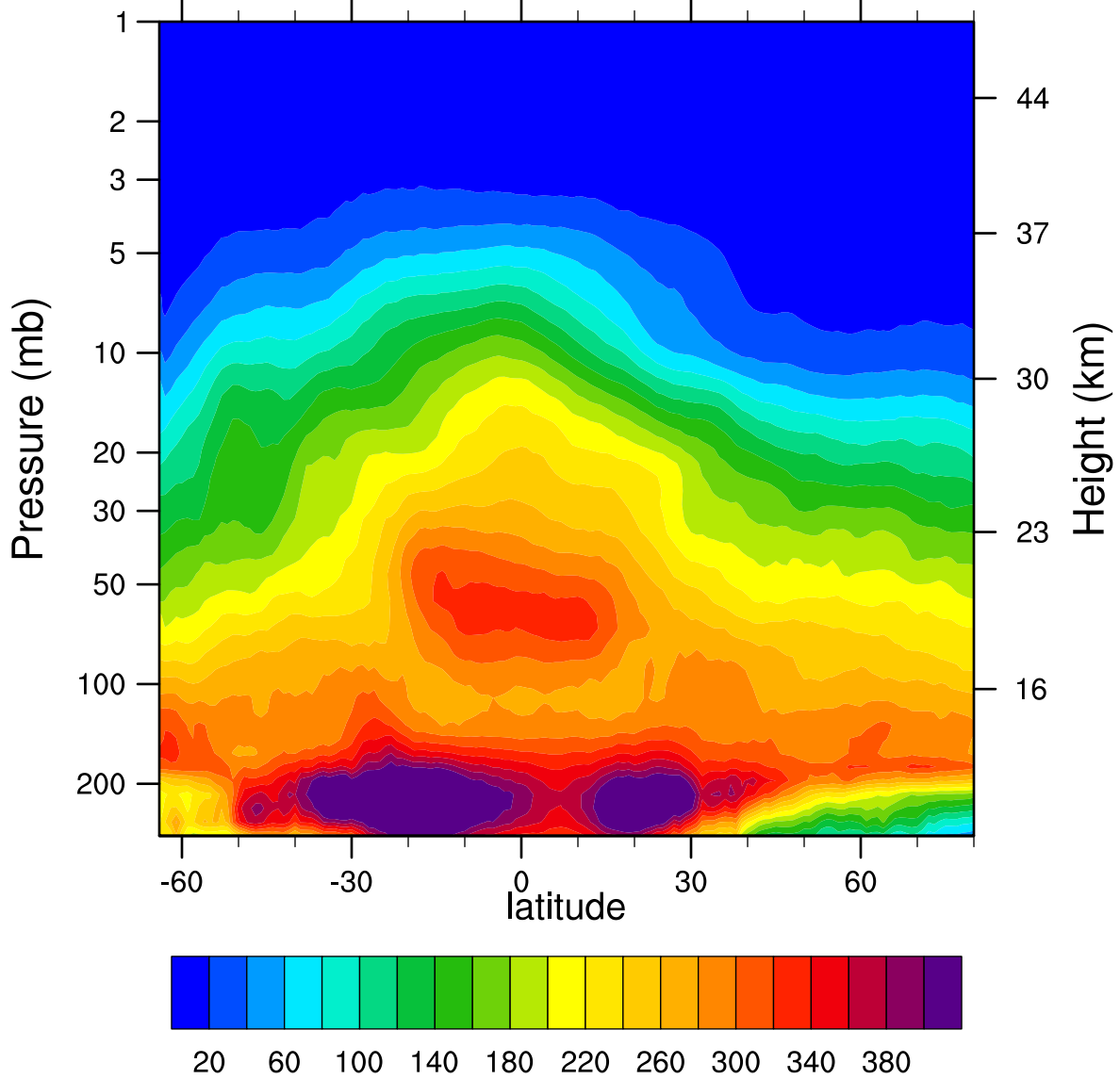
2006d132 N2O_Combined (ppbv)
