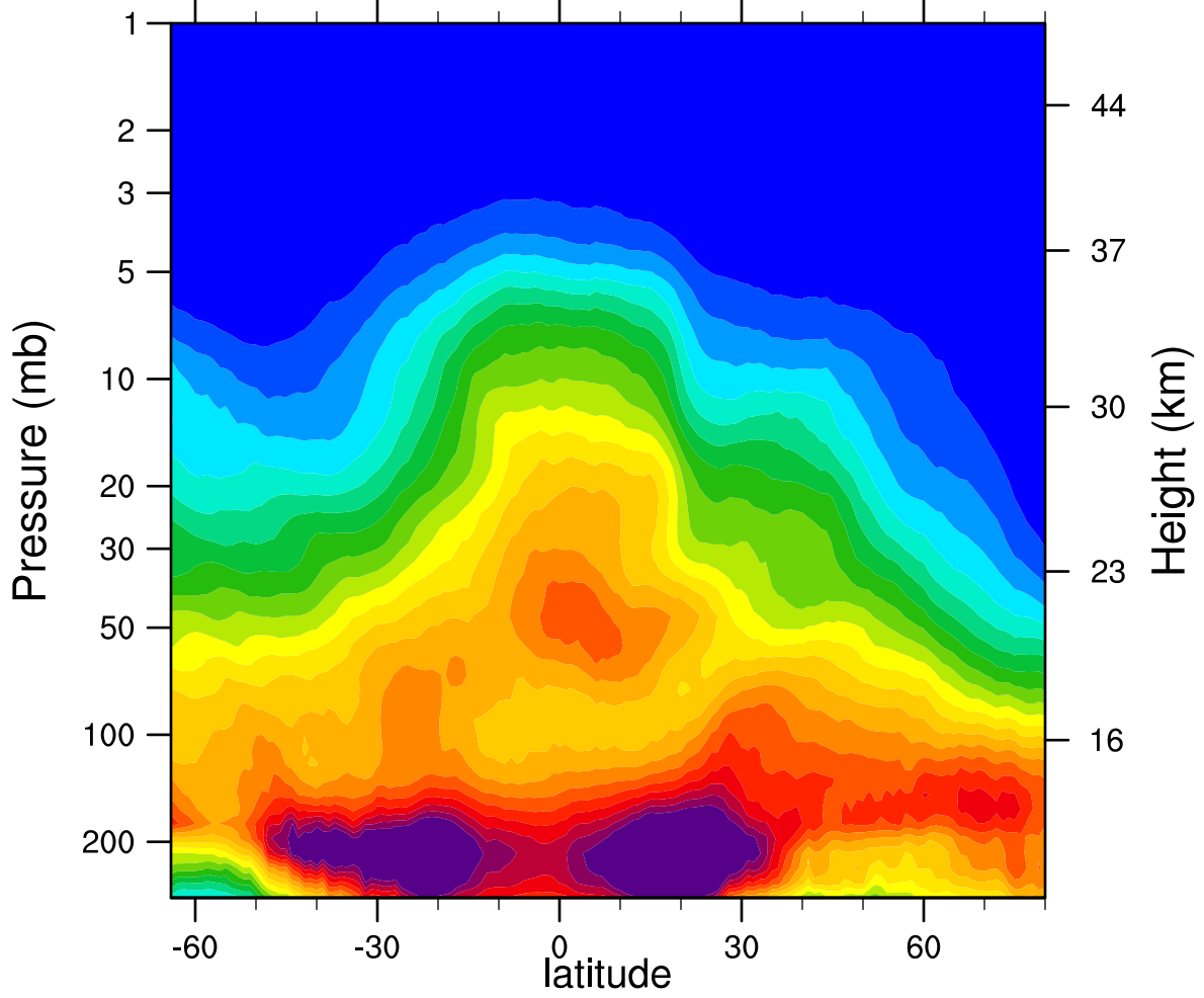
2005d046 N2O_Combined (ppbv)
