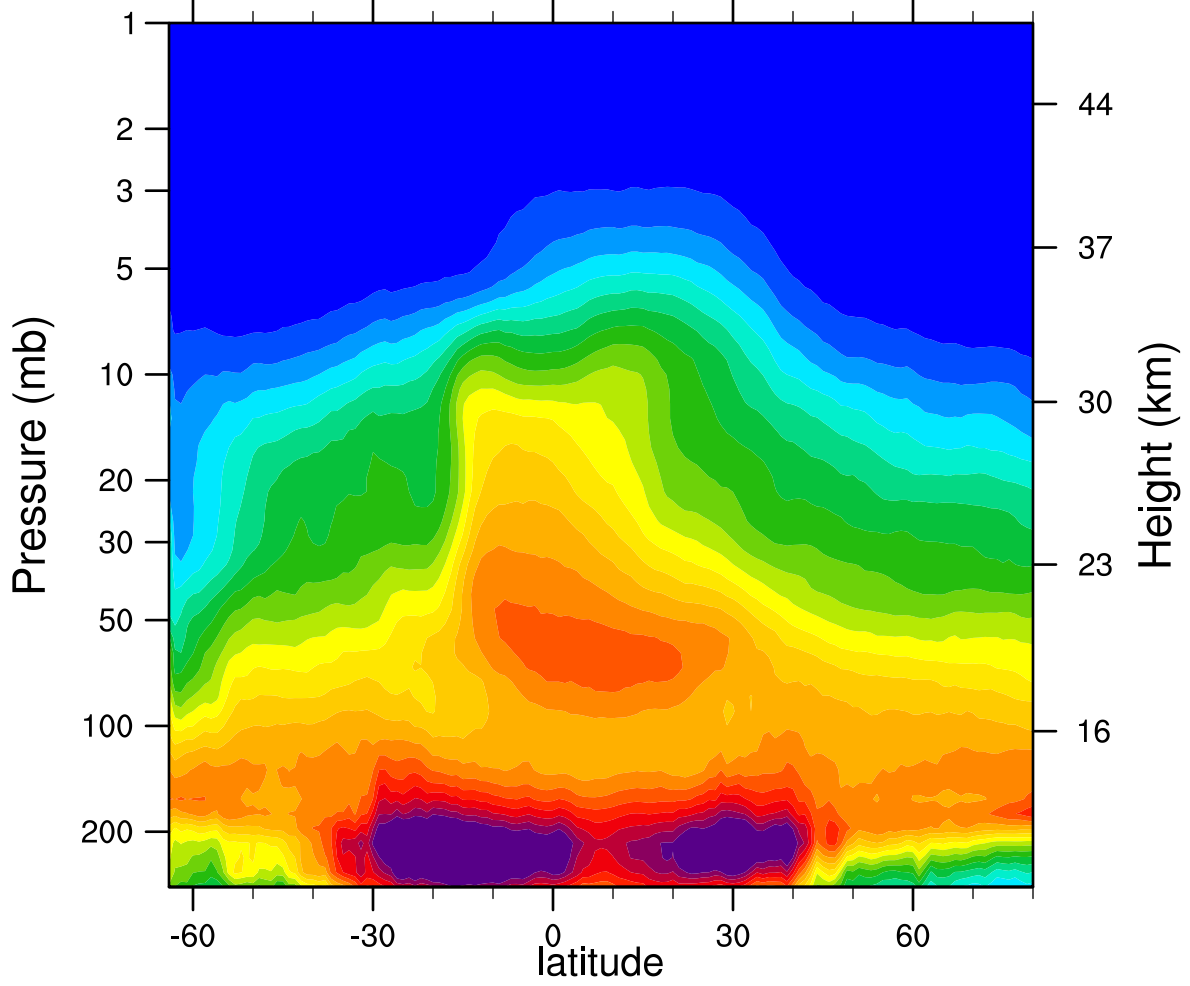
2005d248 N2O_Combined (ppbv)
