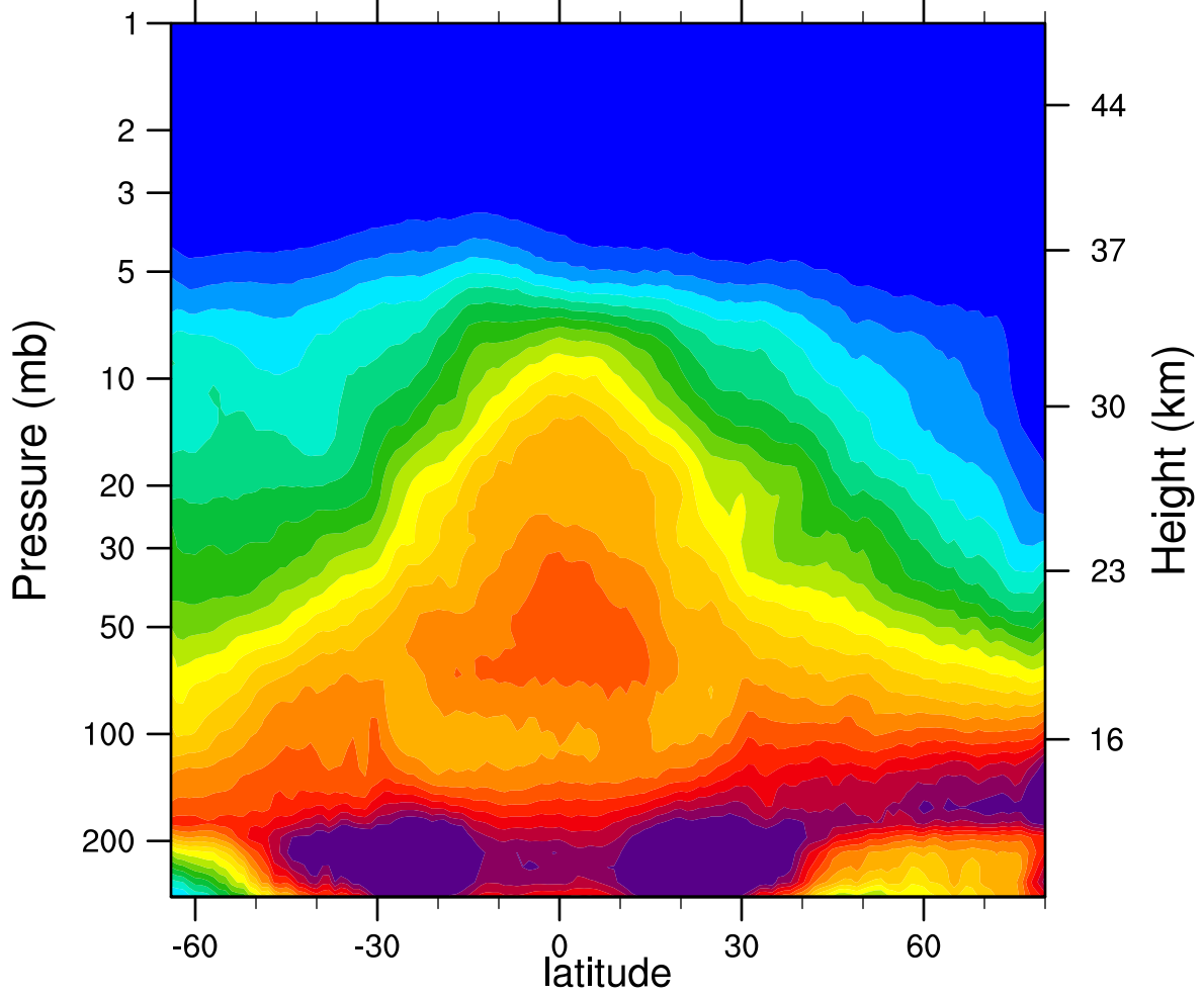
2006d355 N2O_Combined (ppbv)
