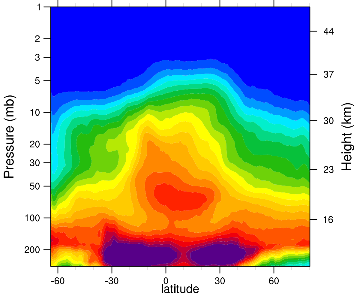
2007d264 N2O_Combined (ppbv)
