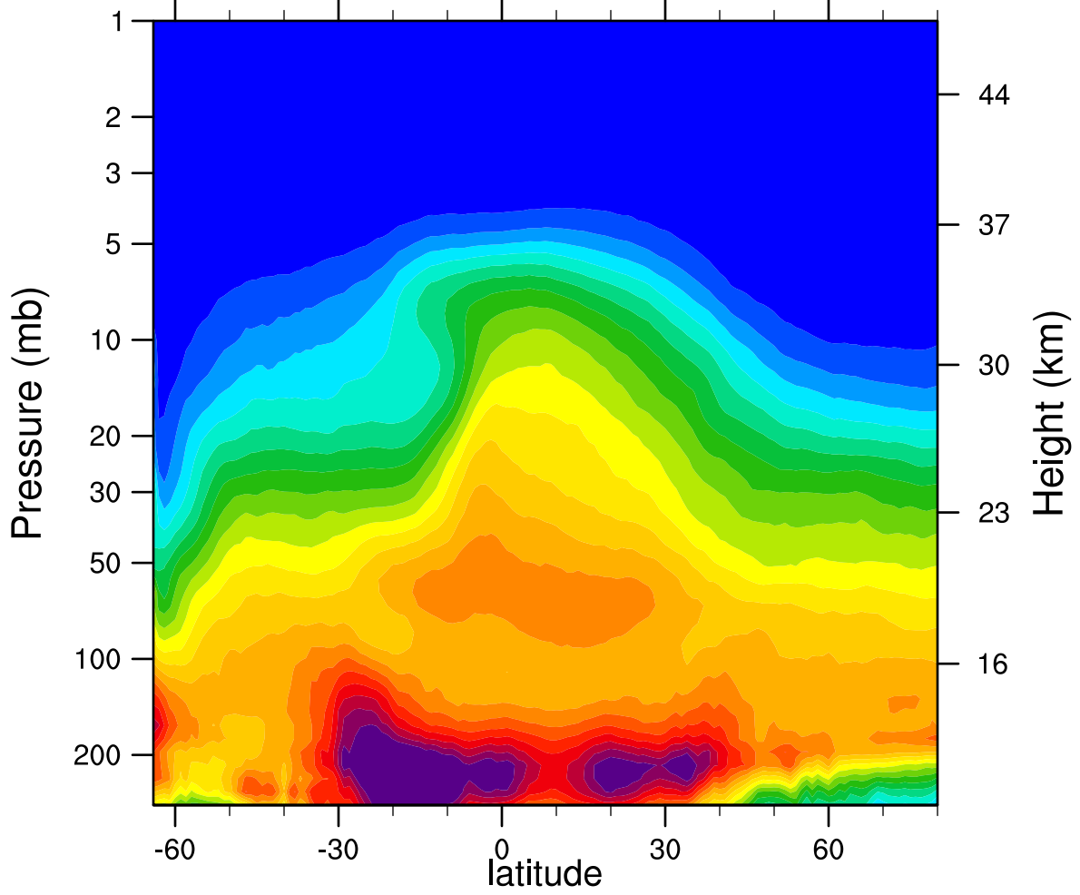
2006d251 N2O_Combined (ppbv)
