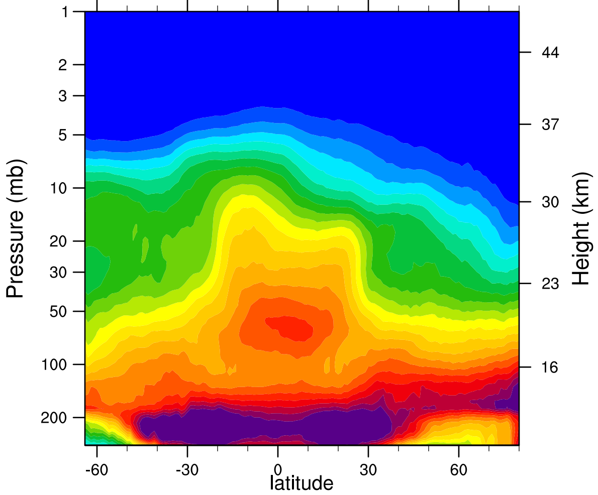
2007d346 N2O_Combined (ppbv)
