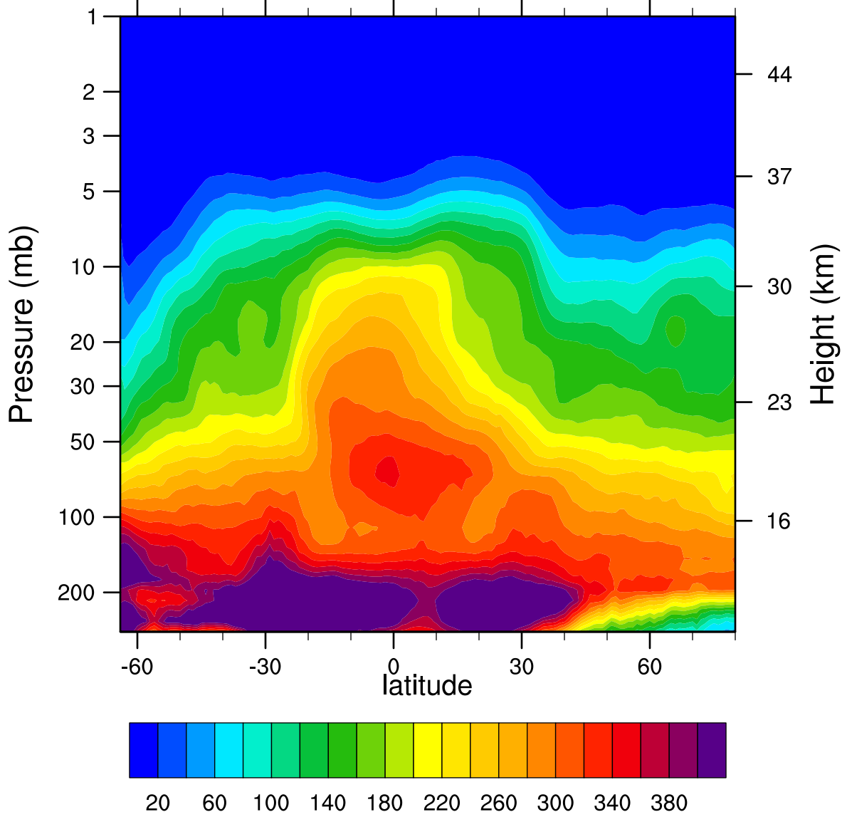
2007d153 N2O_Combined (ppbv)
