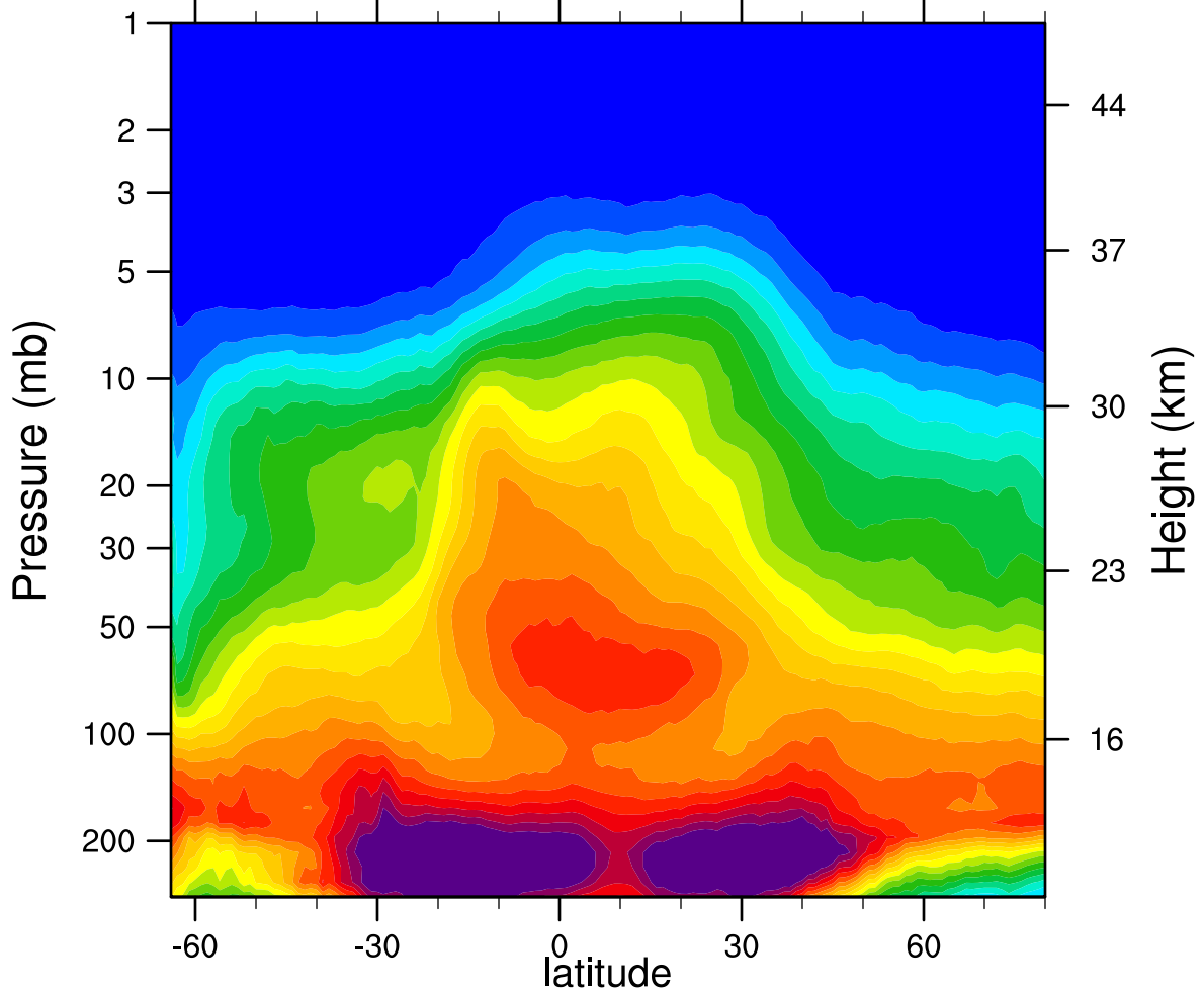
2007d261 N2O_Combined (ppbv)
