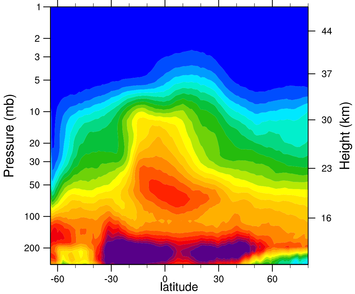
2005d199 N2O_Combined (ppbv)
