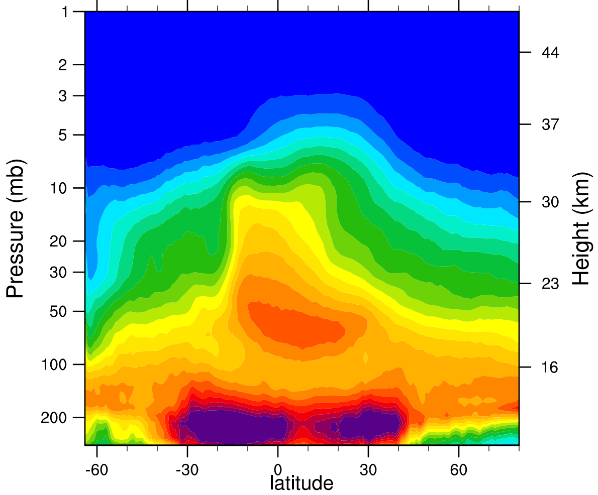
2005d247 N2O_Combined (ppbv)
