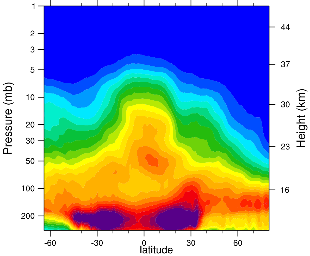
2005d036 N2O_Combined (ppbv)
