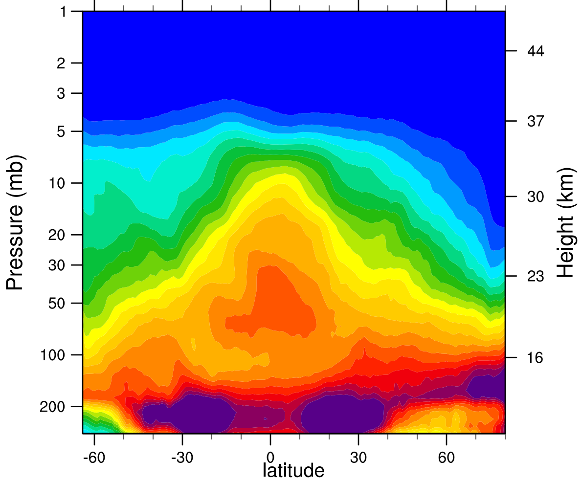
2006d347 N2O_Combined (ppbv)
