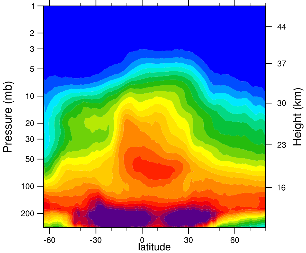
2007d270 N2O_Combined (ppbv)
