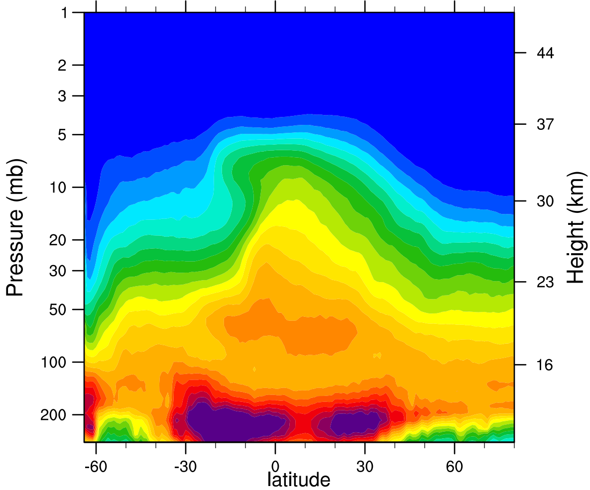
2006d261 N2O_Combined (ppbv)
