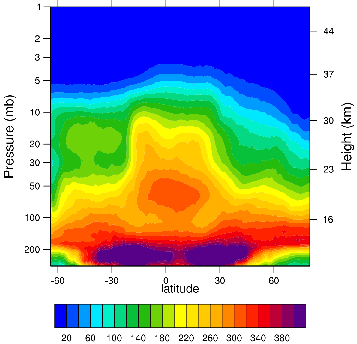
2007d307 N2O_Combined (ppbv)
