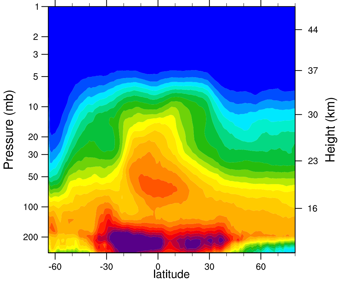
2007d178 N2O_Combined (ppbv)
