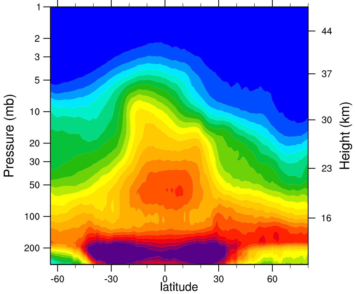
2006d019 N2O_Combined (ppbv)
