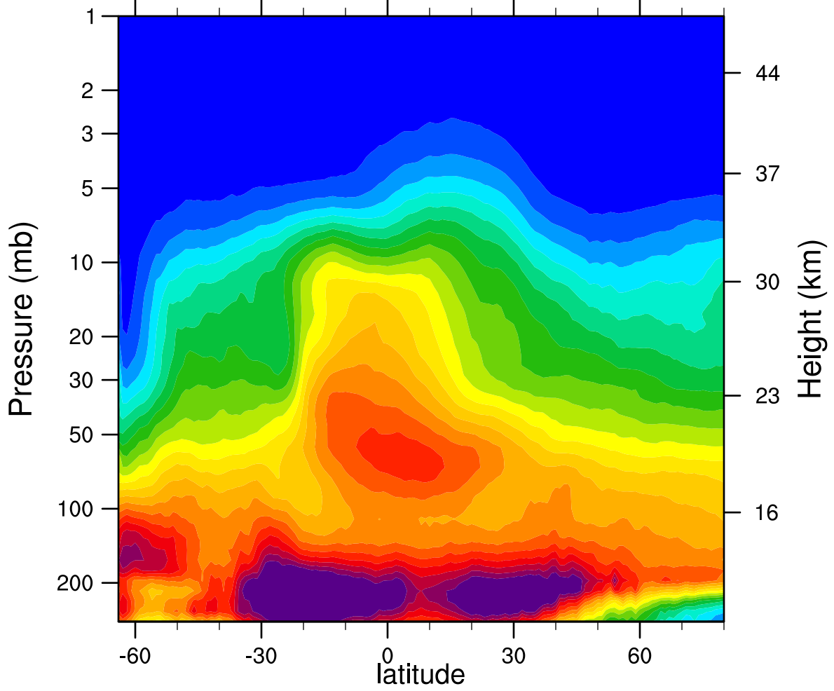
2005d192 N2O_Combined (ppbv)
