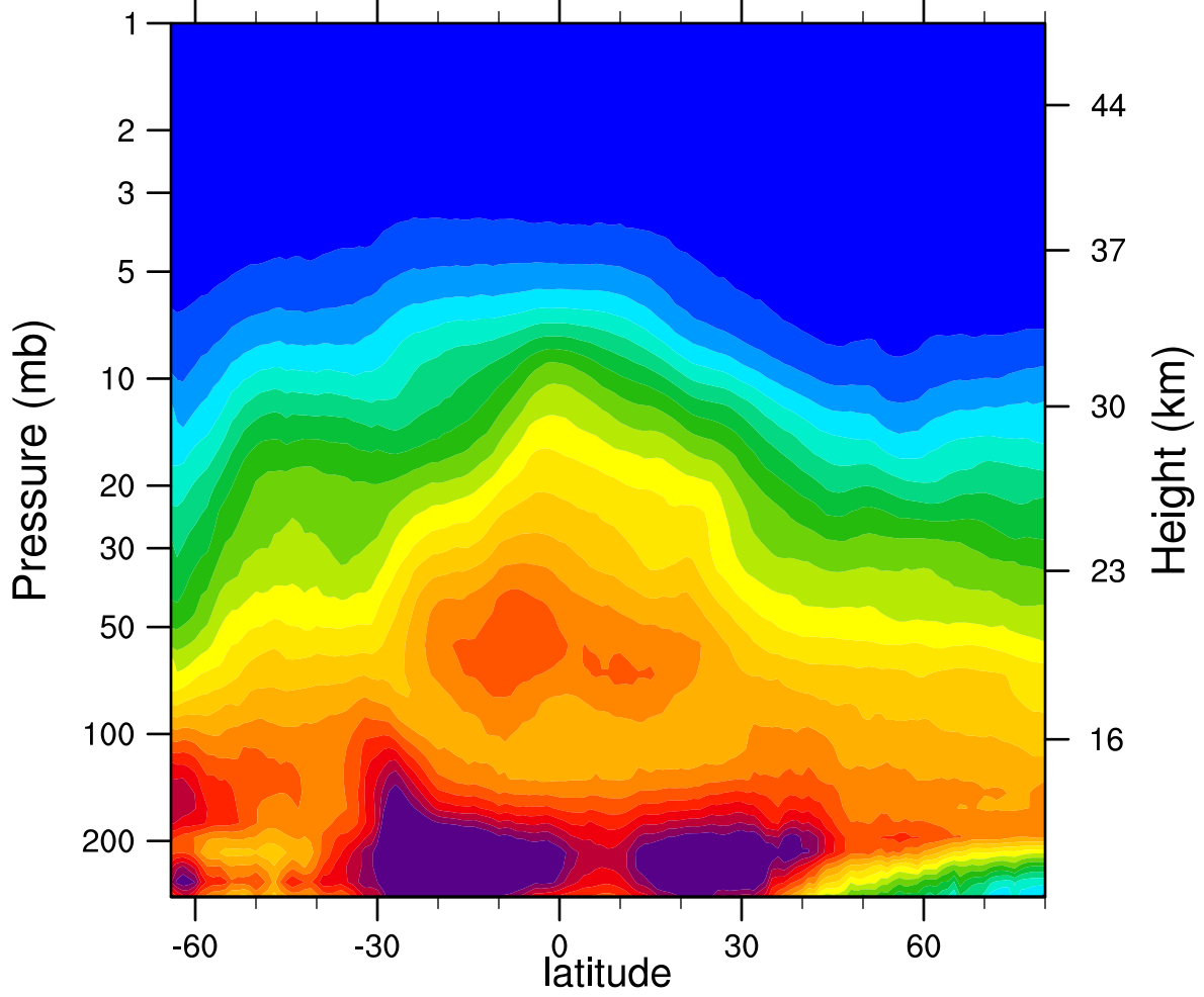
2006d166 N2O_Combined (ppbv)
