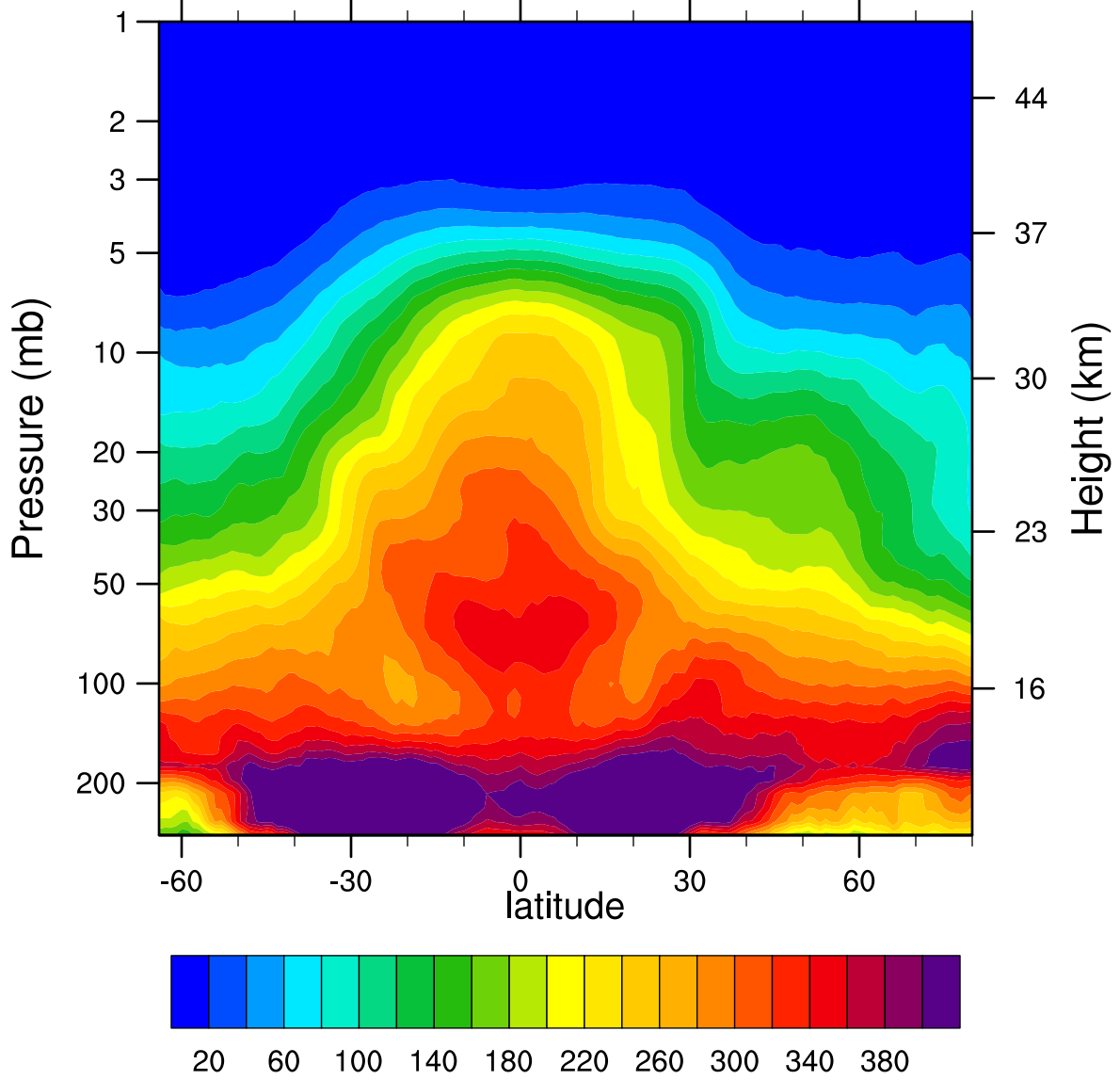
2007d091 N2O_Combined (ppbv)
