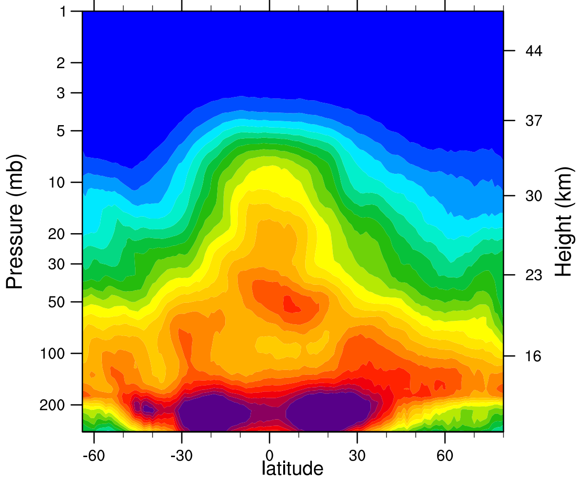
2005d081 N2O_Combined (ppbv)
