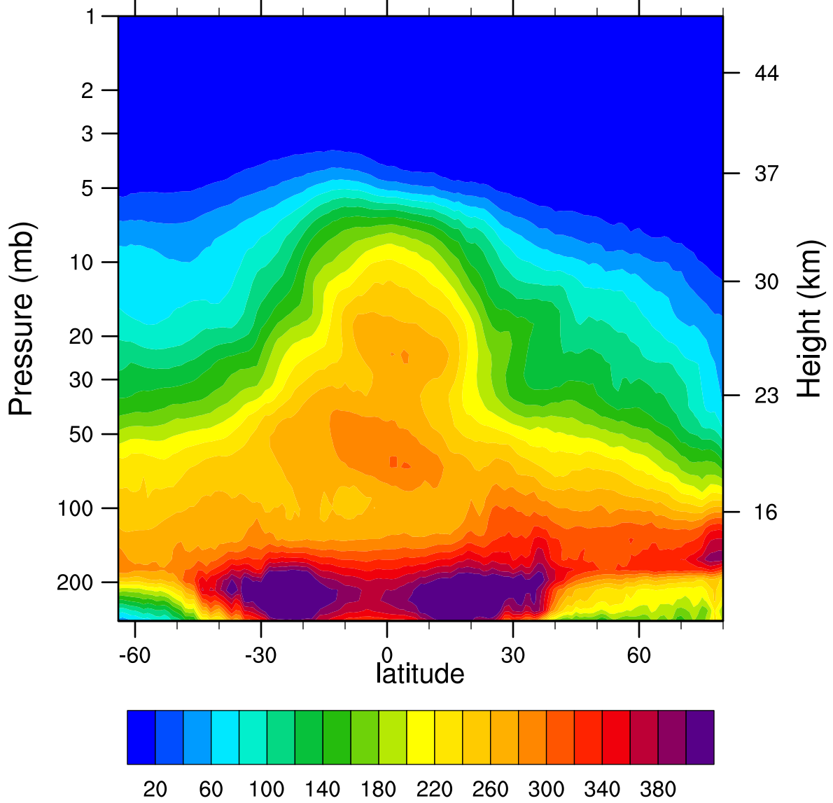
2007d026 N2O_Combined (ppbv)
