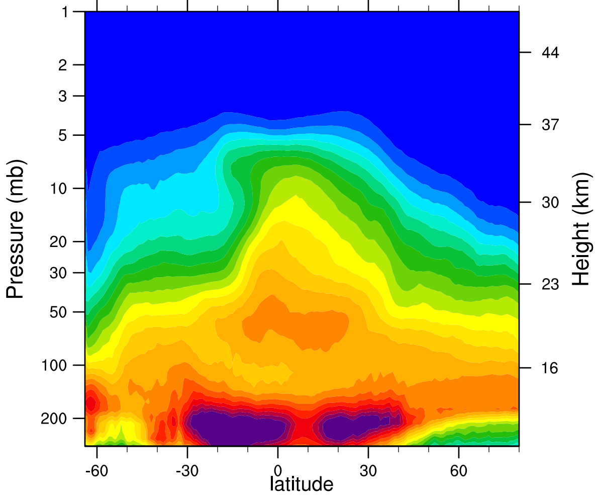
2006d281 N2O_Combined (ppbv)
