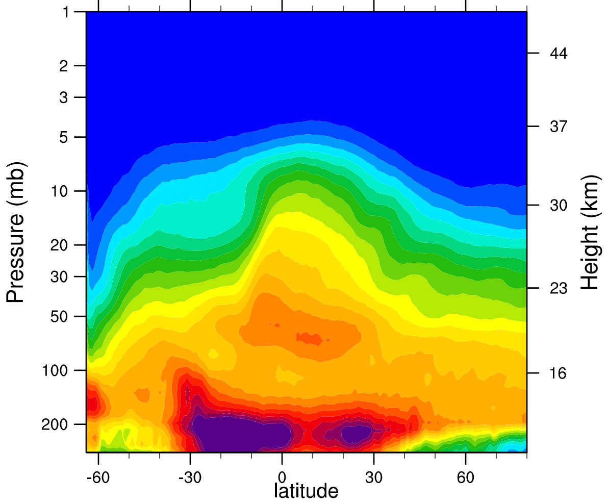
2006d228 N2O_Combined (ppbv)
