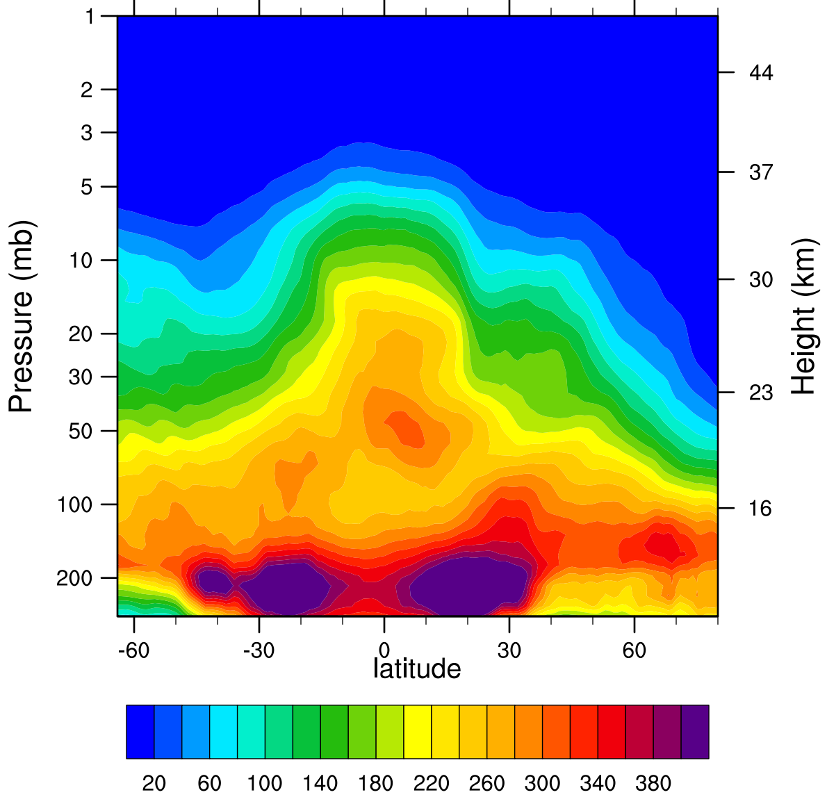
2005d040 N2O_Combined (ppbv)
