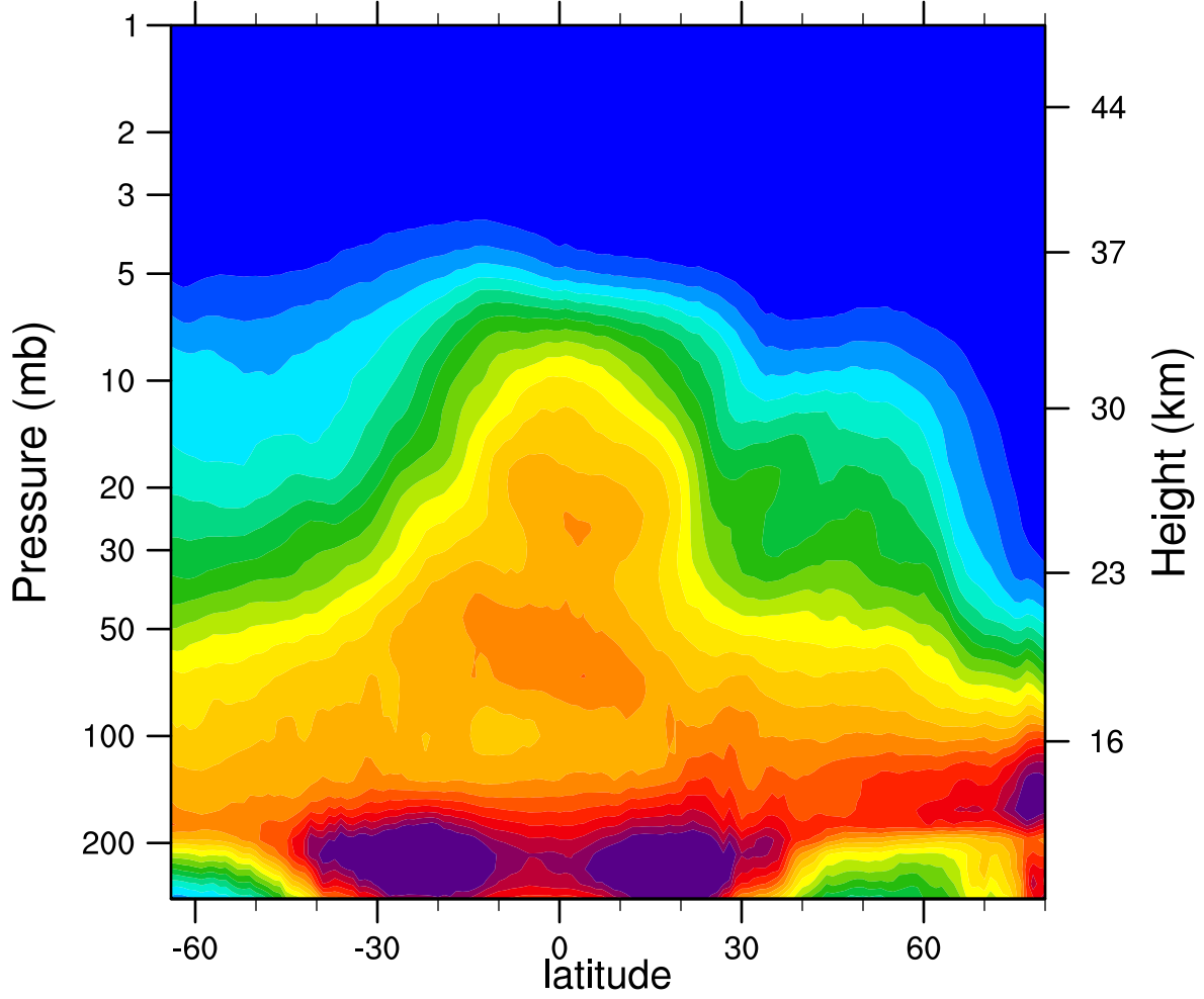
2007d019 N2O_Combined (ppbv)
