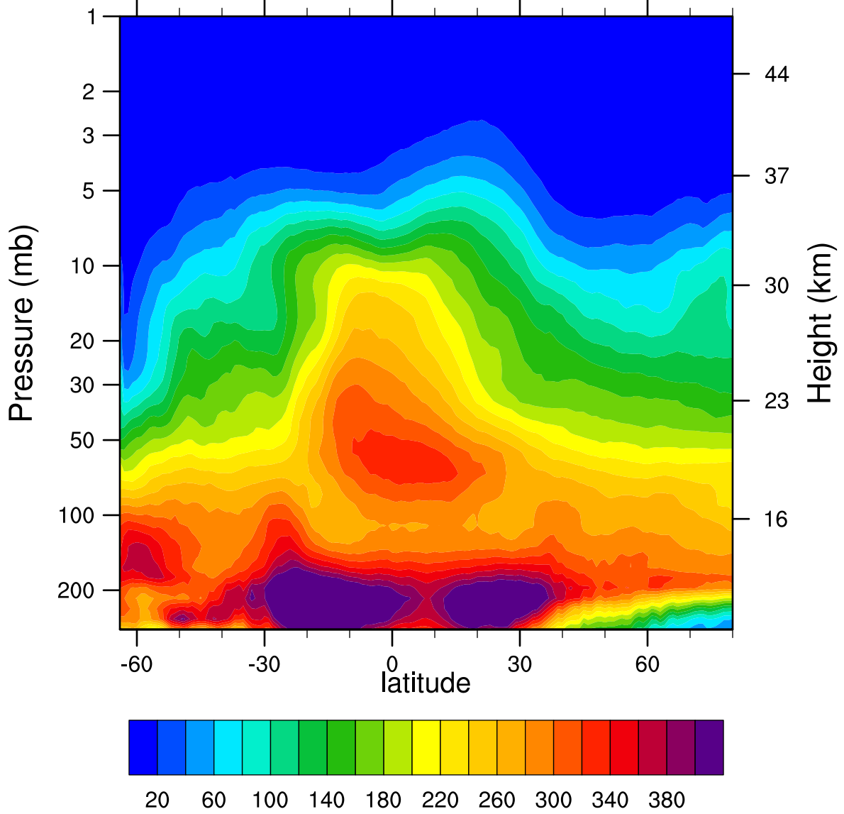
2005d168 N2O_Combined (ppbv)
