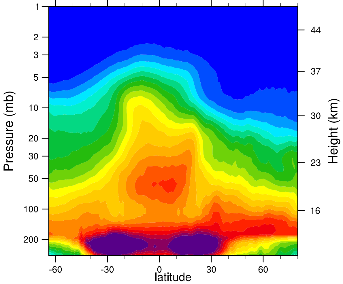
2006d031 N2O_Combined (ppbv)
