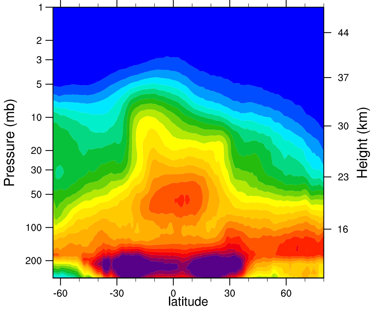
2005d343 N2O_Combined (ppbv)
