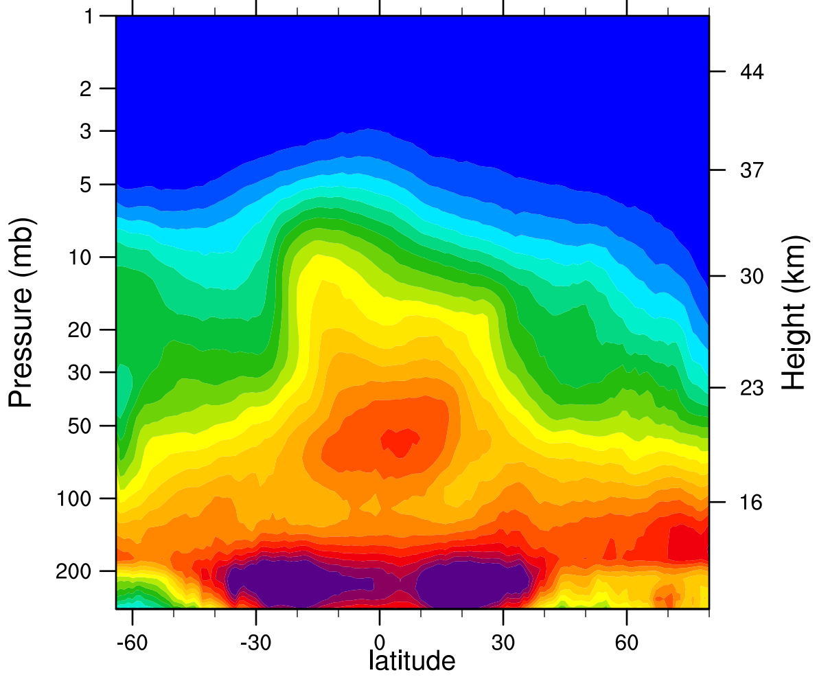
2005d338 N2O_Combined (ppbv)
