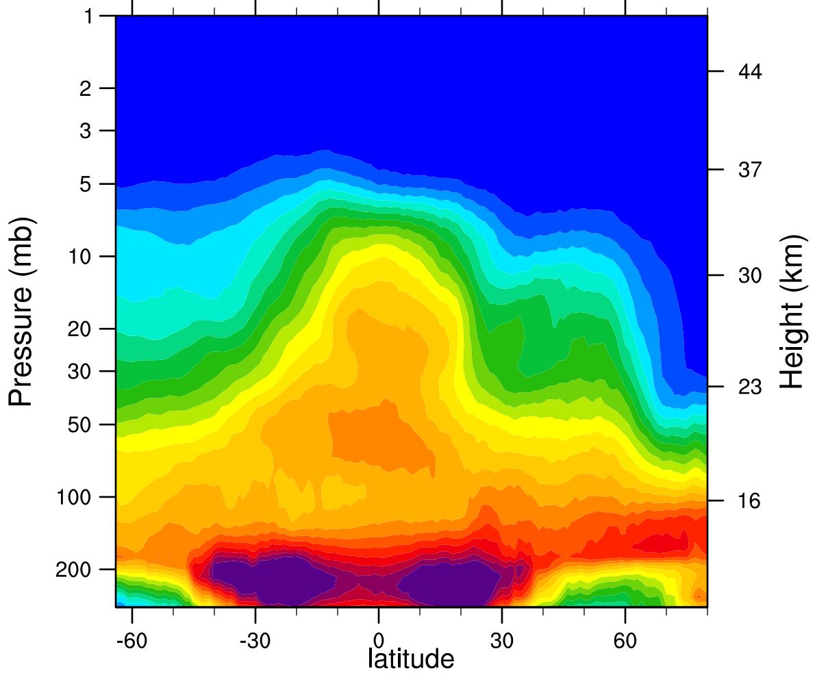
2007d013 N2O_Combined (ppbv)
