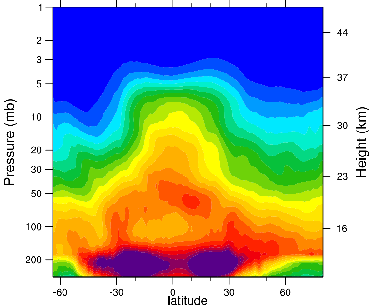
2005d105 N2O_Combined (ppbv)
