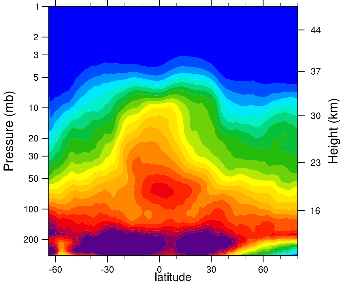
2007d139 N2O_Combined (ppbv)
