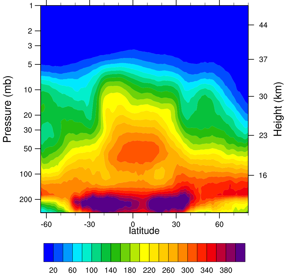
2005d324 N2O_Combined (ppbv)
