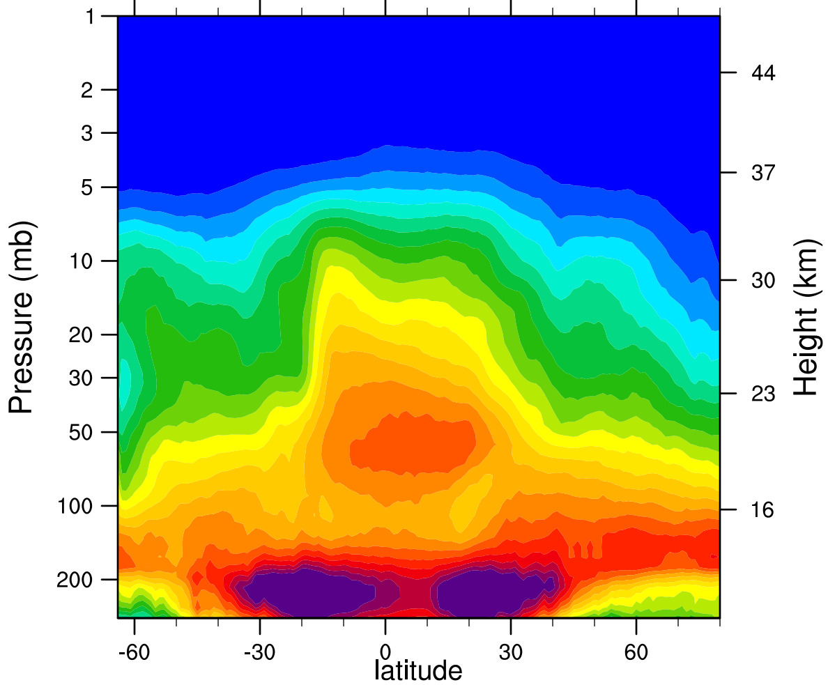
2005d308 N2O_Combined (ppbv)
