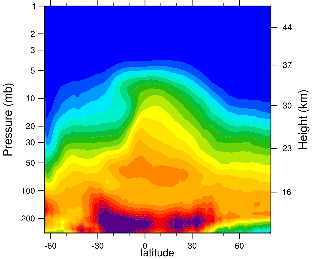
2006d254 N2O_Combined (ppbv)
