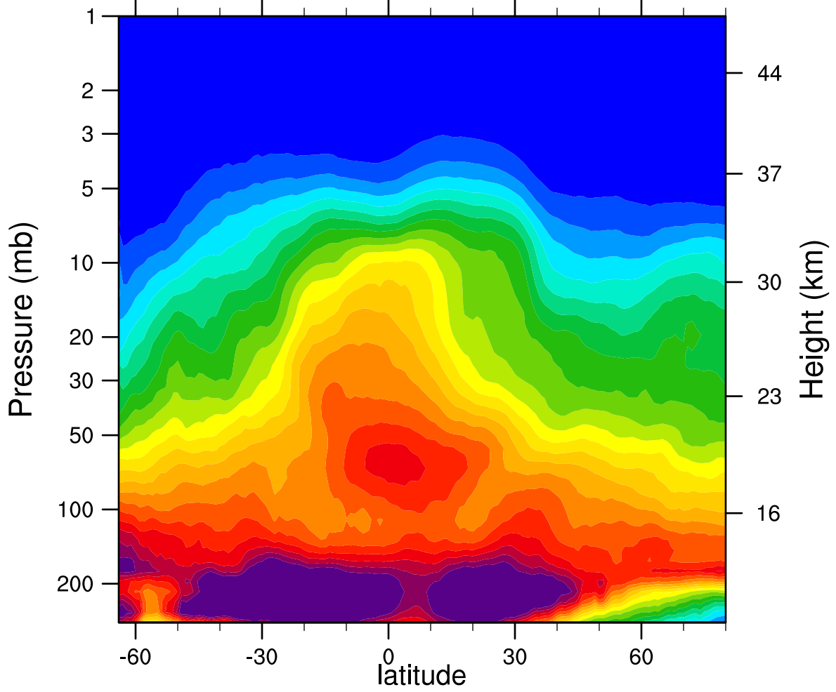
2007d138 N2O_Combined (ppbv)
