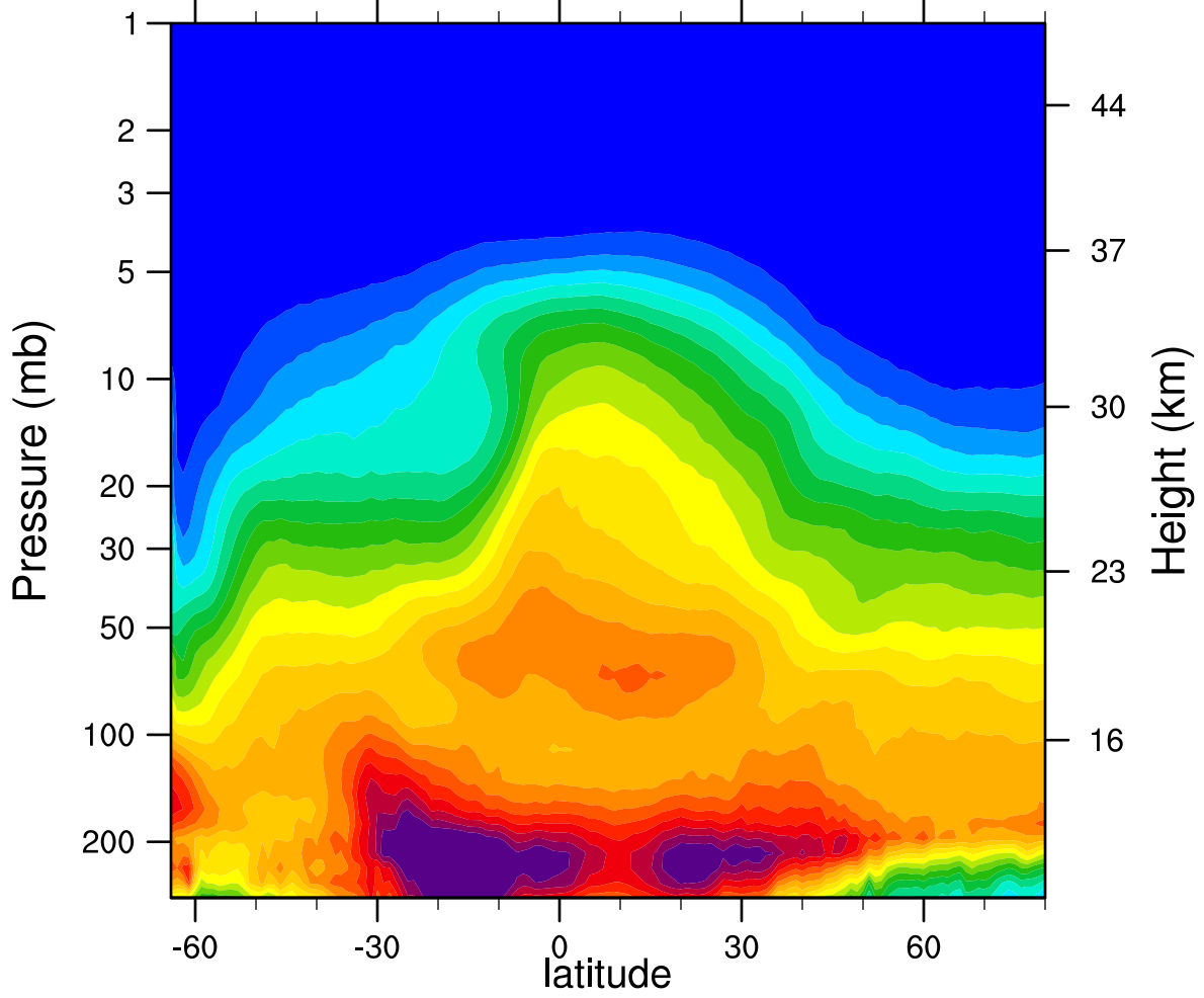
2006d247 N2O_Combined (ppbv)
