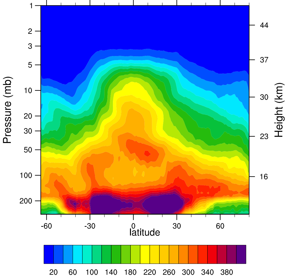
2005d089 N2O_Combined (ppbv)
