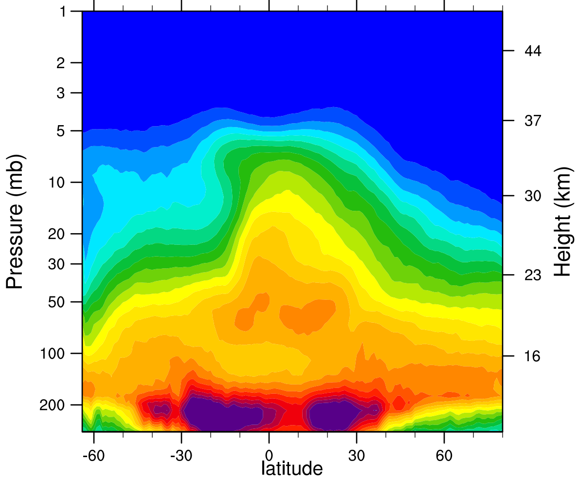
2006d291 N2O_Combined (ppbv)
