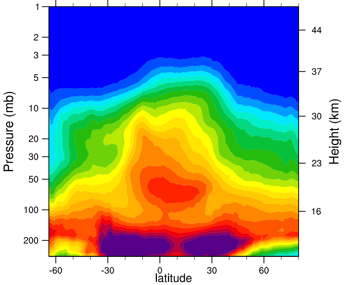
2007d263 N2O_Combined (ppbv)
