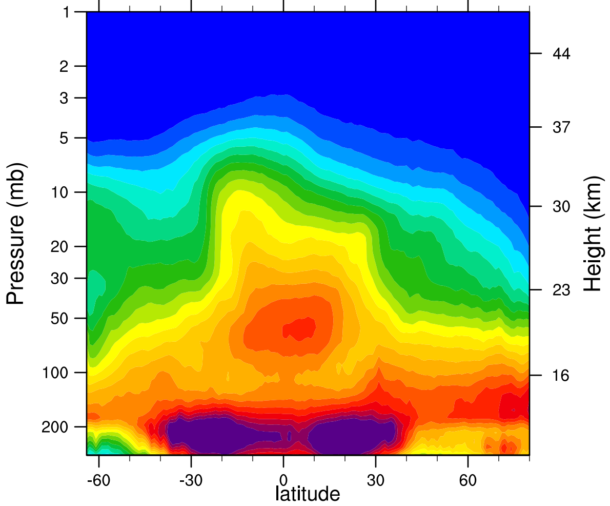
2005d341 N2O_Combined (ppbv)
