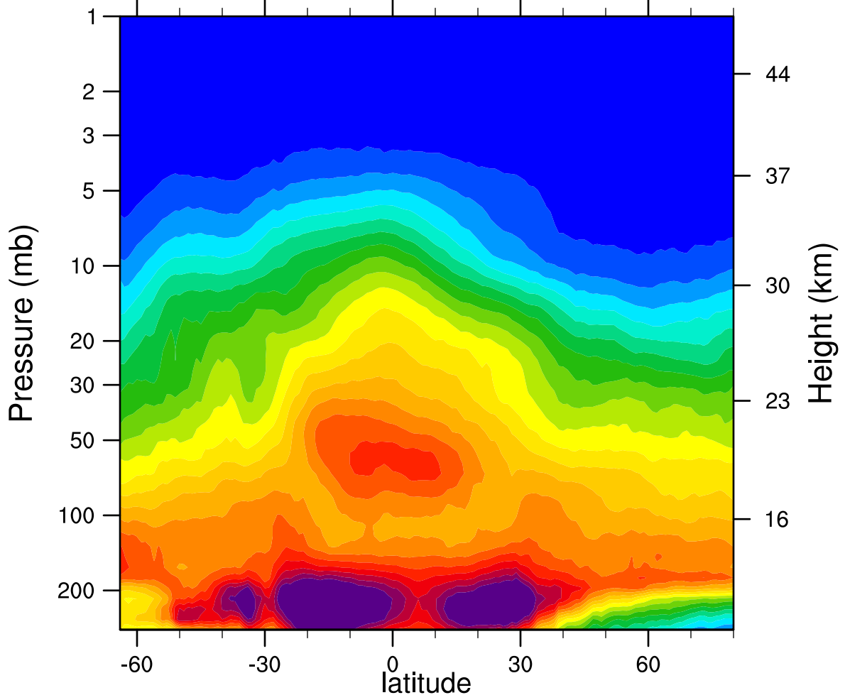
2006d139 N2O_Combined (ppbv)
