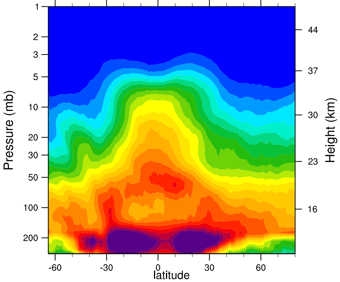
2005d115 N2O_Combined (ppbv)
