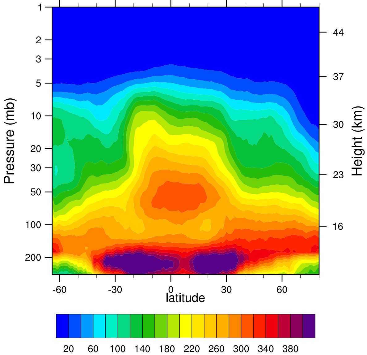
2005d318 N2O_Combined (ppbv)
