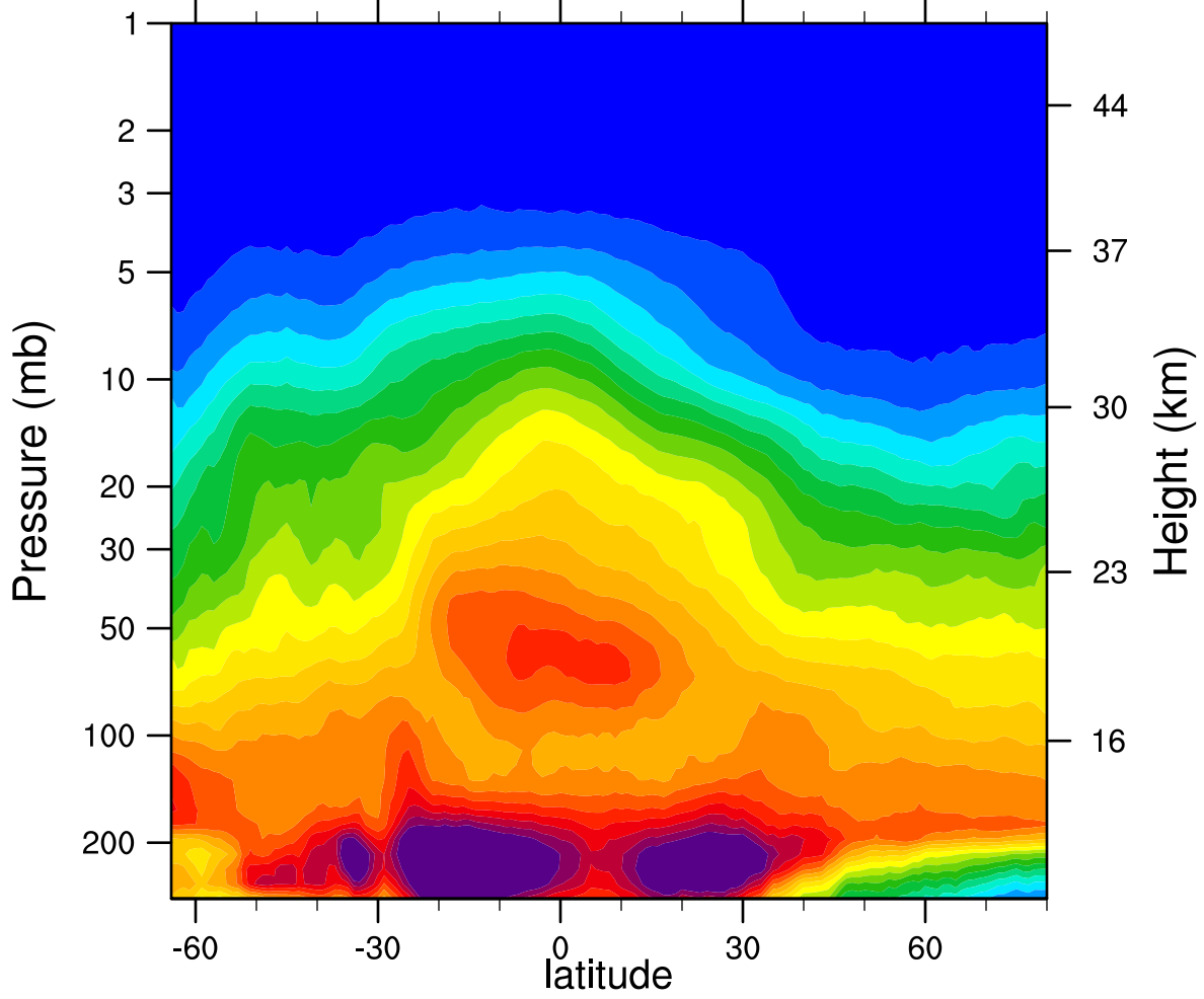
2006d141 N2O_Combined (ppbv)
