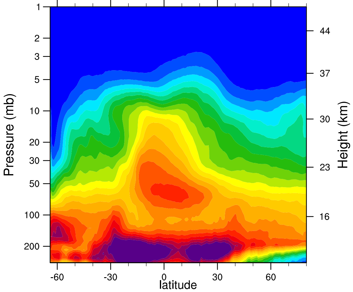
2005d175 N2O_Combined (ppbv)
