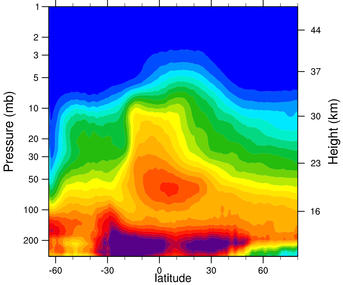
2005d227 N2O_Combined (ppbv)
