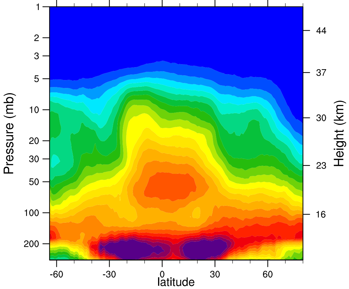
2005d319 N2O_Combined (ppbv)
