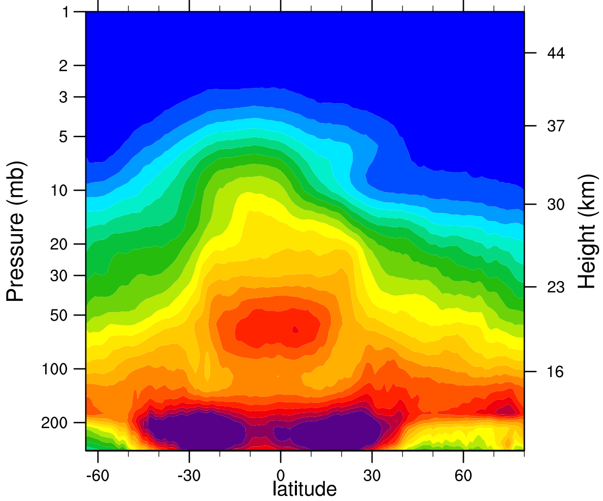
2006d078 N2O_Combined (ppbv)
