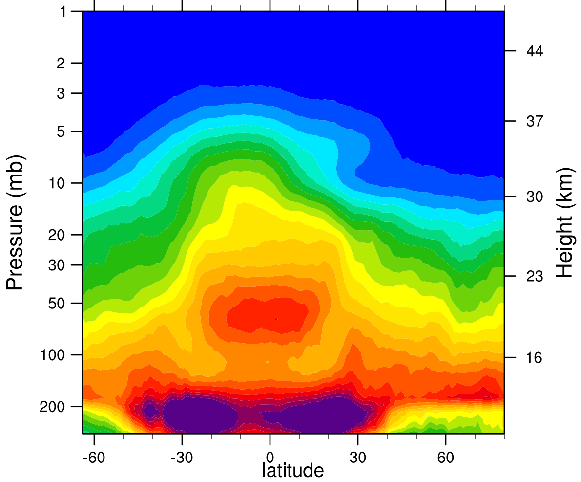
2006d082 N2O_Combined (ppbv)
