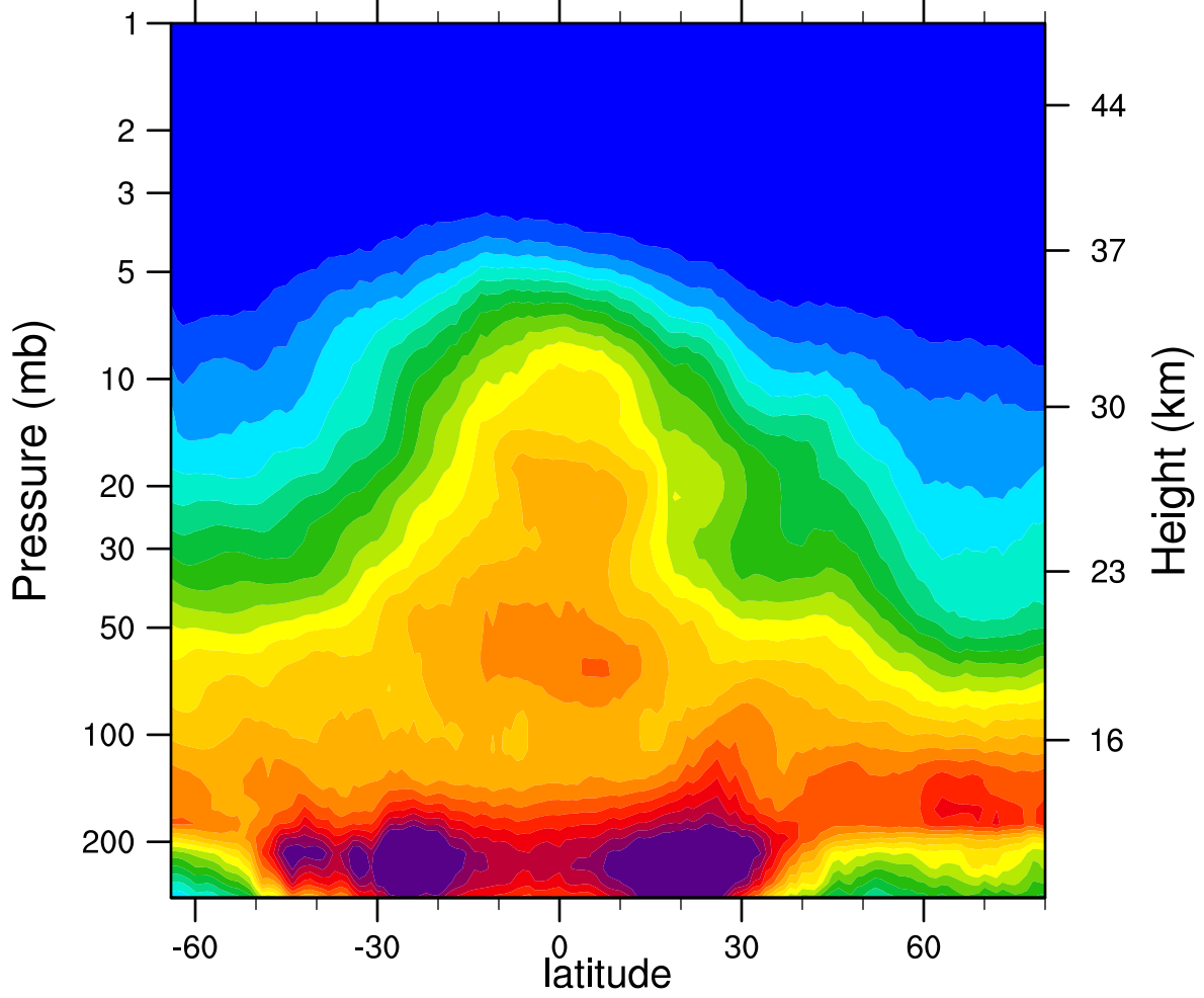
2007d054 N2O_Combined (ppbv)
