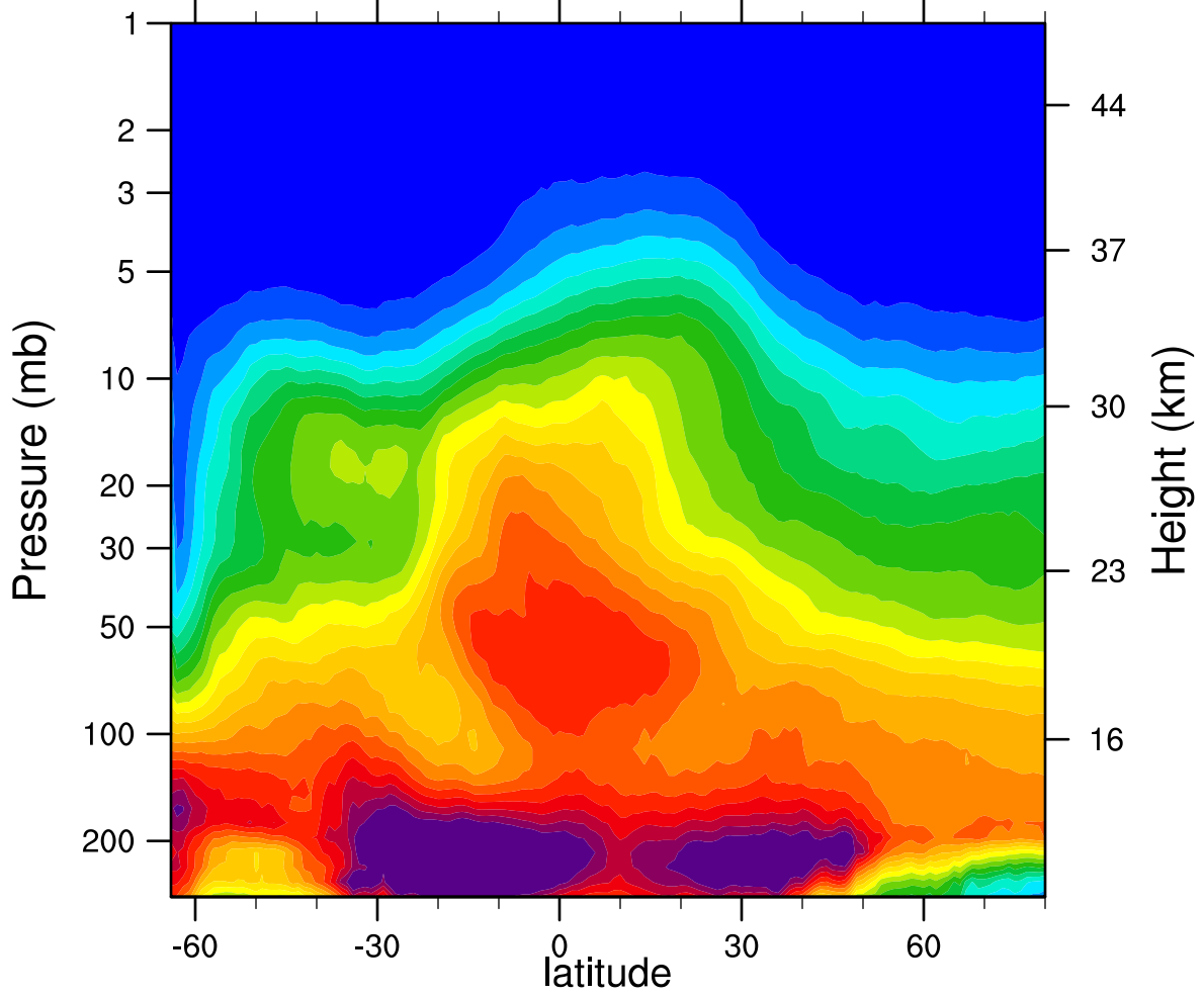
2007d216 N2O_Combined (ppbv)
