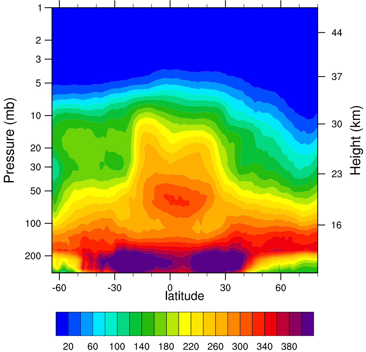
2007d316 N2O_Combined (ppbv)
