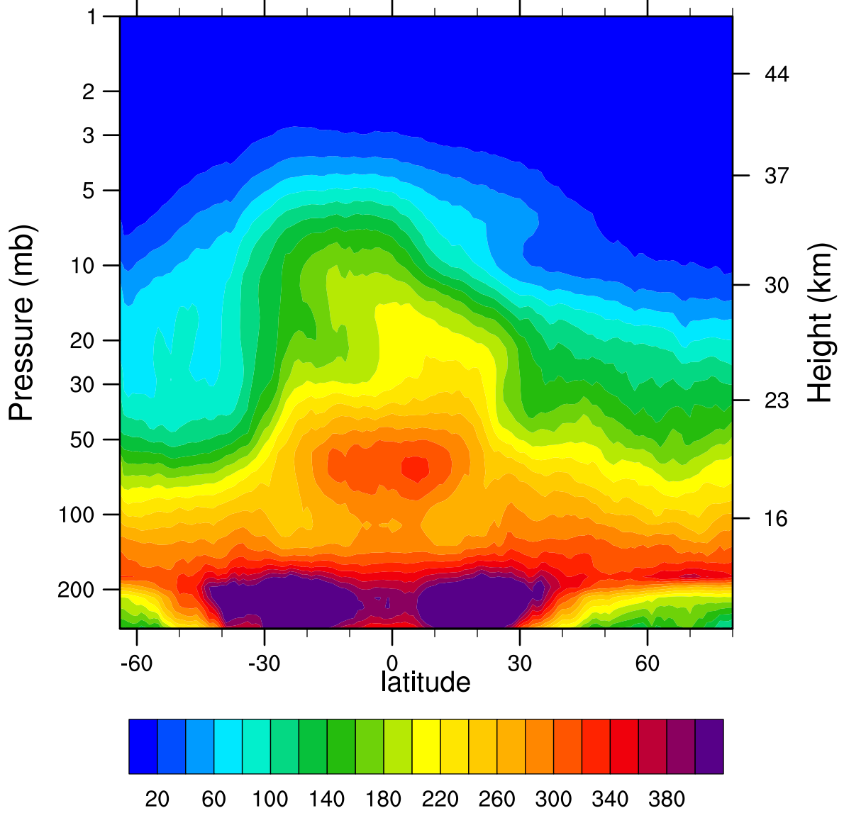
2006d093 N2O_Combined (ppbv)
