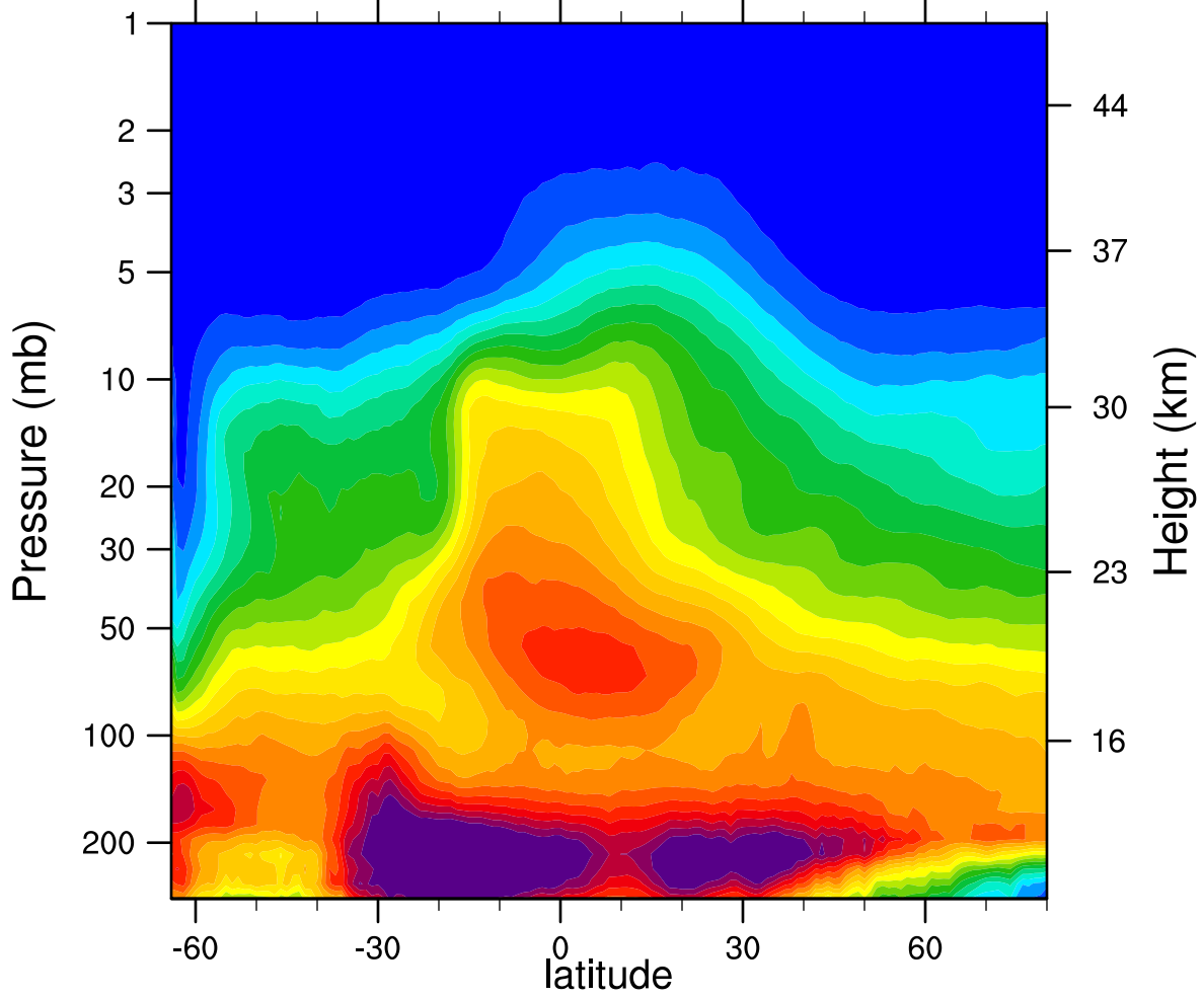
2005d218 N2O_Combined (ppbv)
