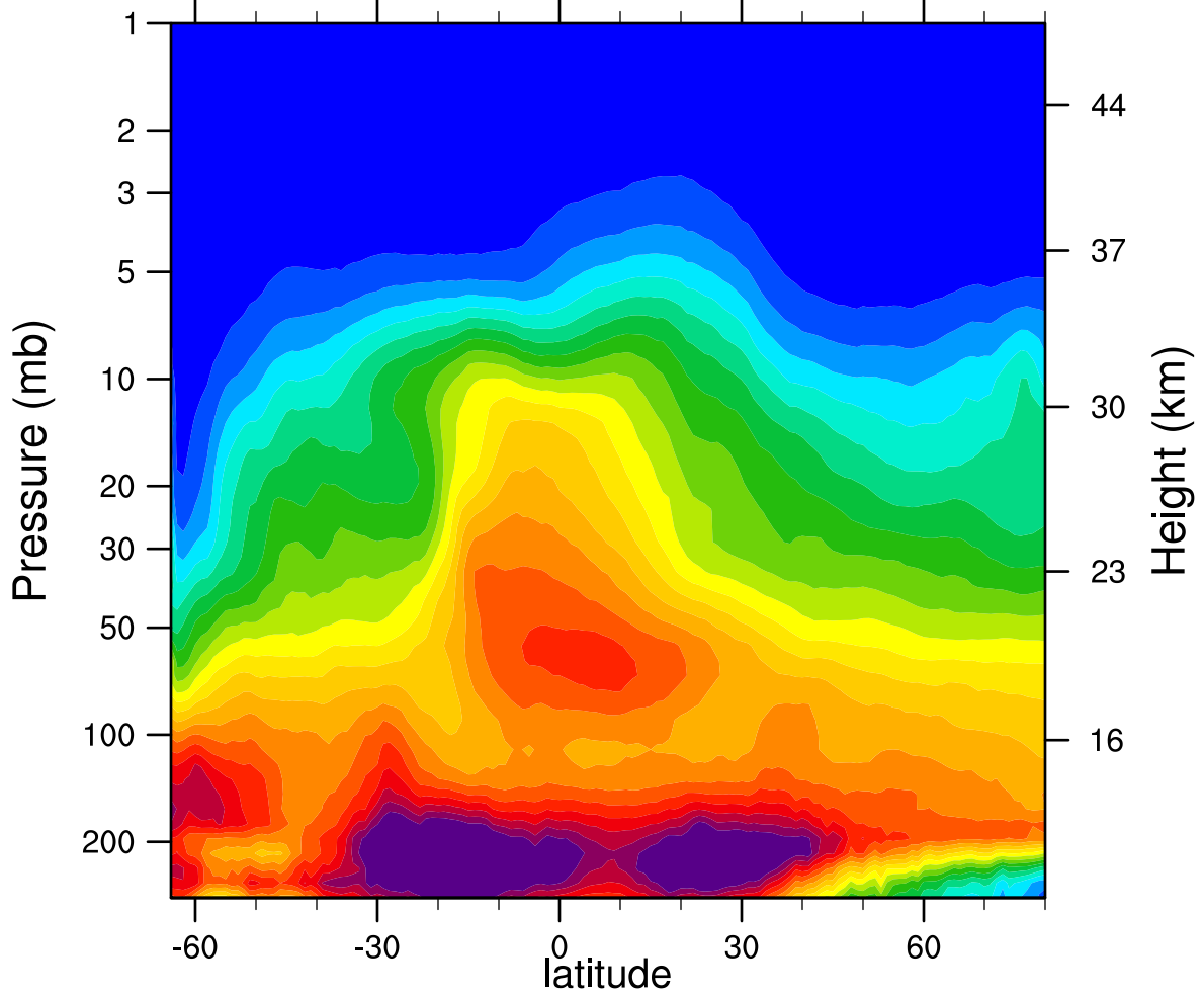
2005d180 N2O_Combined (ppbv)
