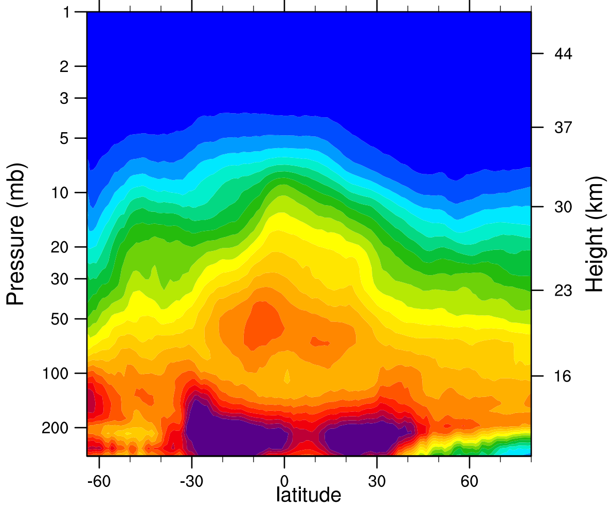
2006d169 N2O_Combined (ppbv)
