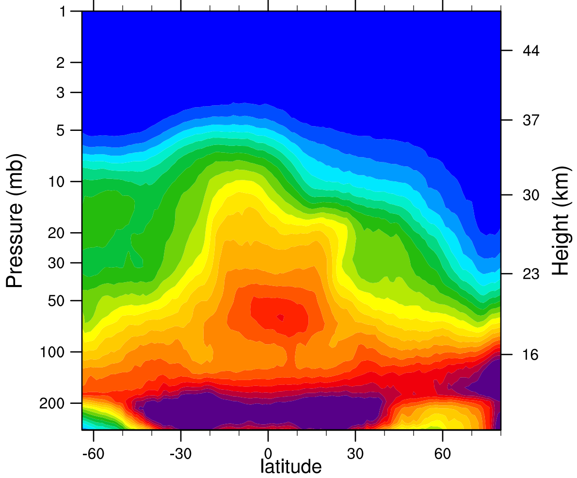
2007d363 N2O_Combined (ppbv)
