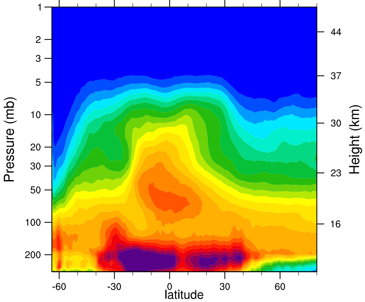
2007d176 N2O_Combined (ppbv)
