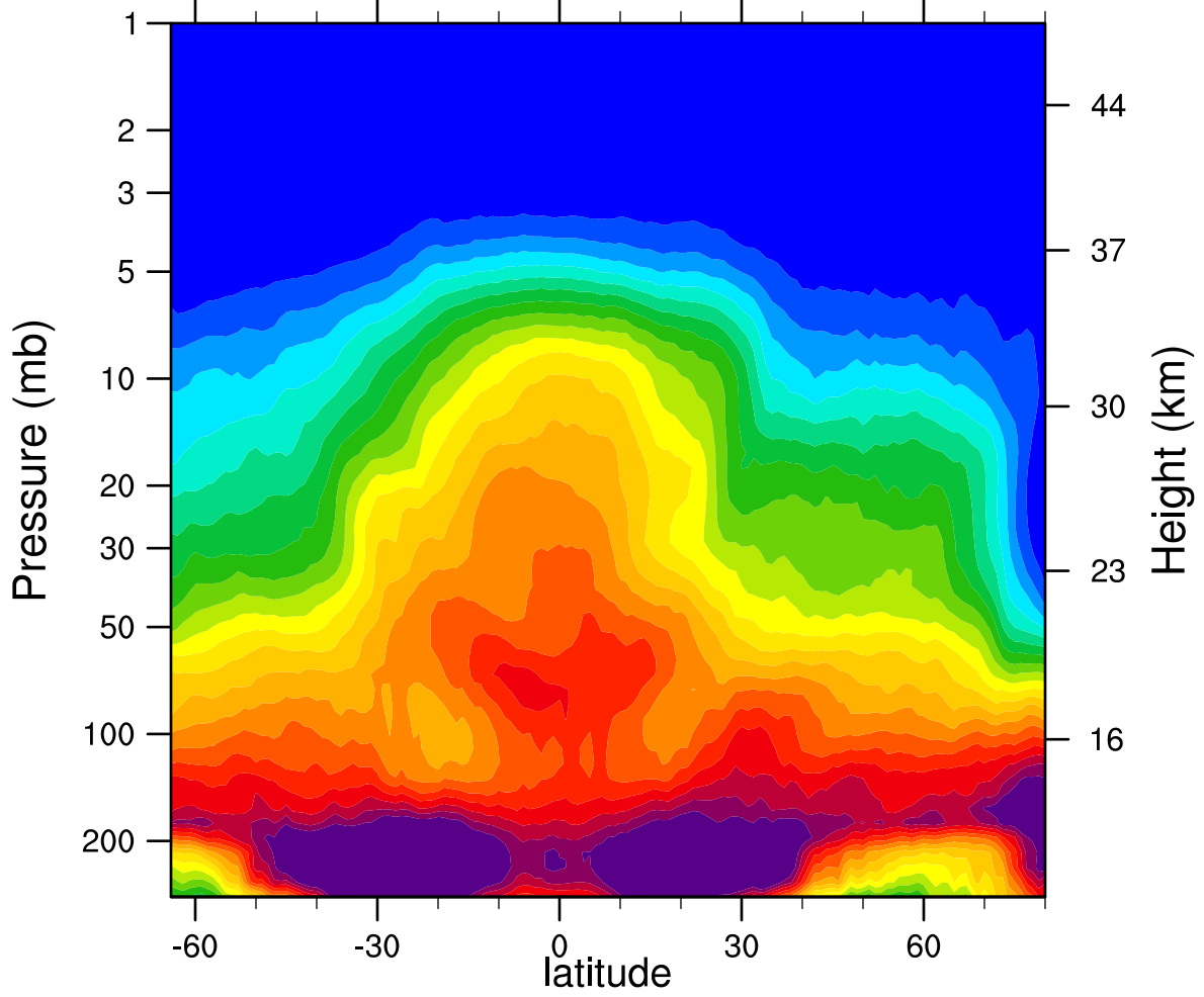
2007d082 N2O_Combined (ppbv)
