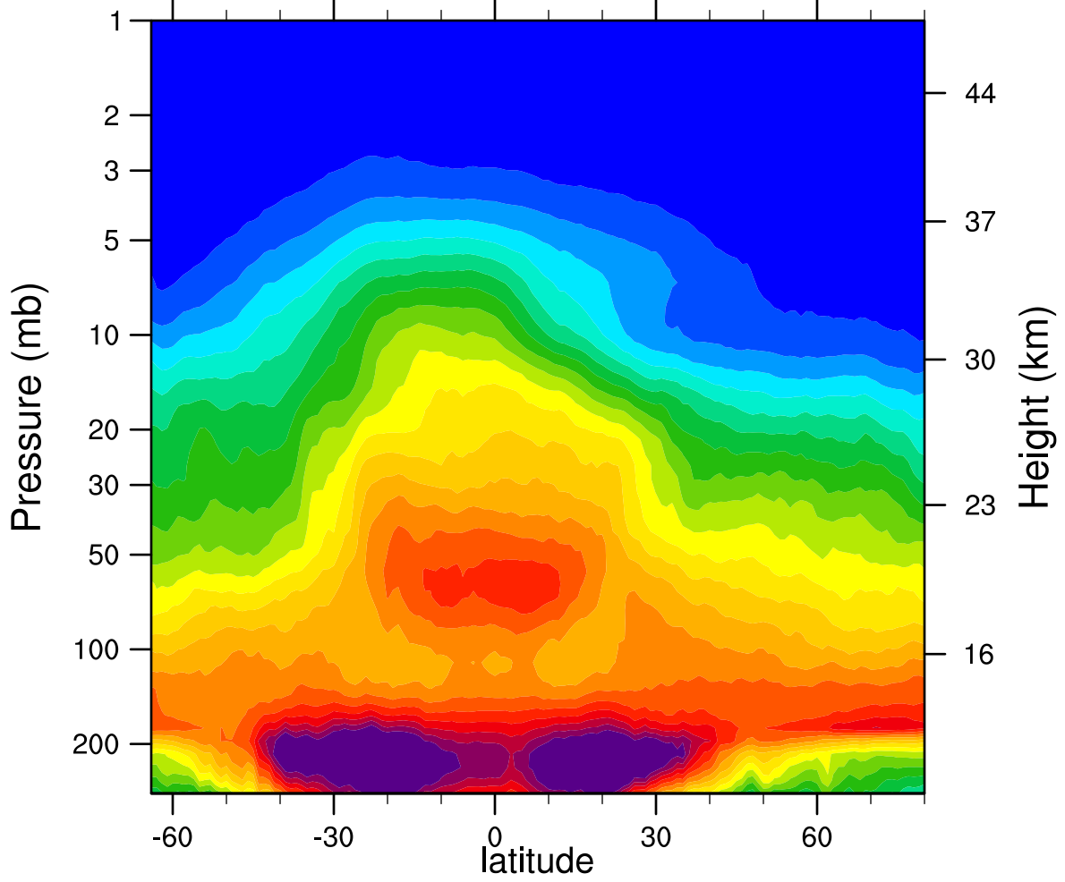
2006d096 N2O_Combined (ppbv)
