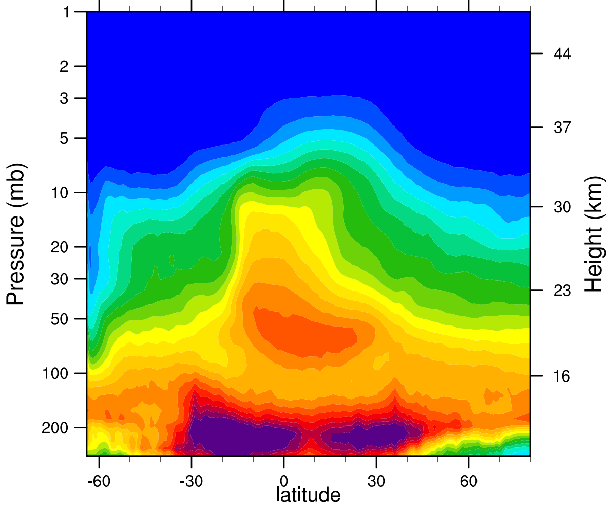
2005d242 N2O_Combined (ppbv)
