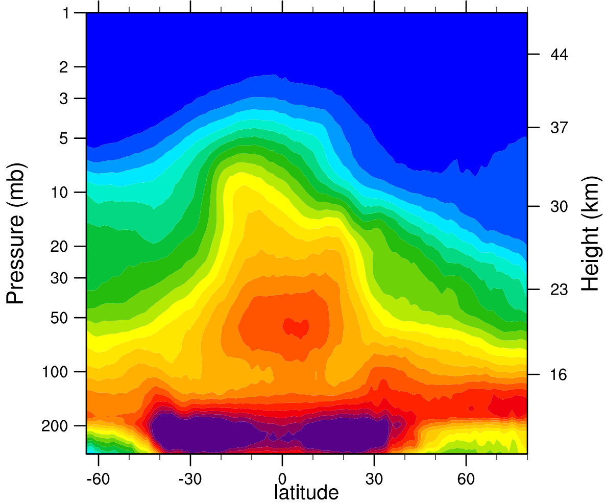
2006d022 N2O_Combined (ppbv)
