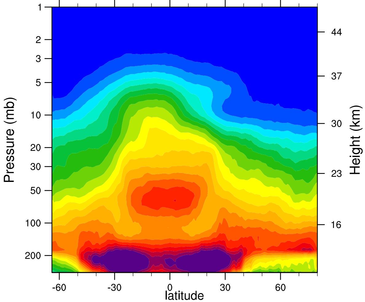
2006d080 N2O_Combined (ppbv)
