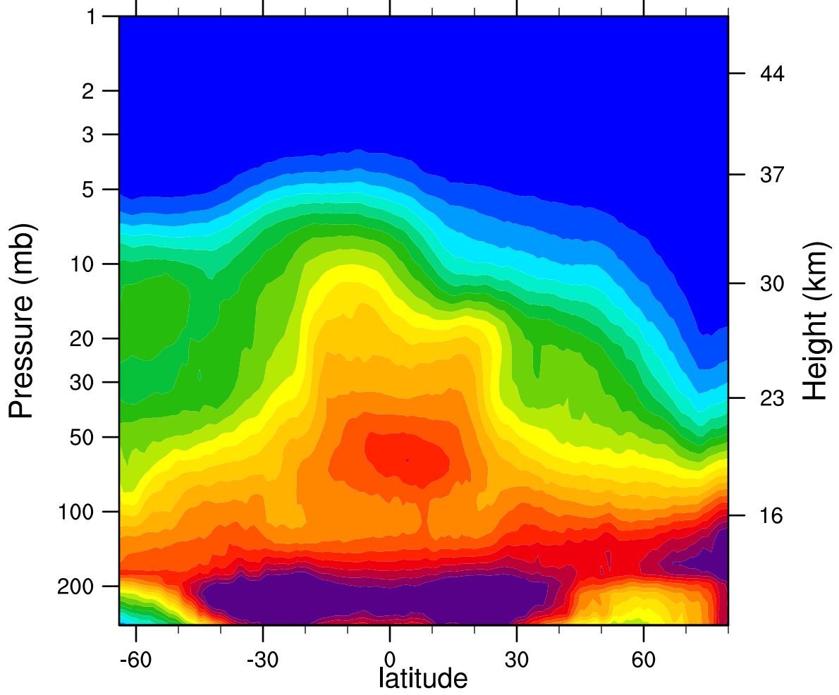
2007d361 N2O_Combined (ppbv)
