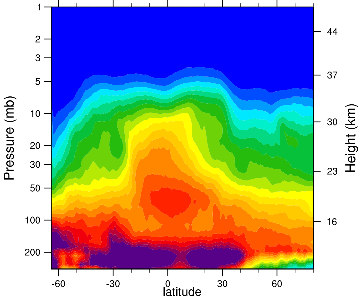
2007d161 N2O_Combined (ppbv)
