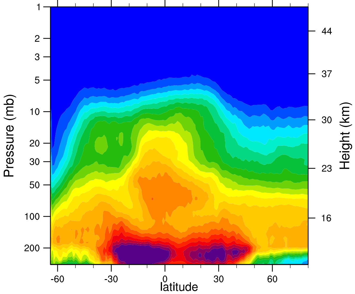
2007d210 N2O_Combined (ppbv)
