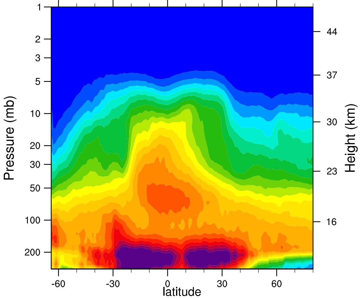
2007d164 N2O_Combined (ppbv)
