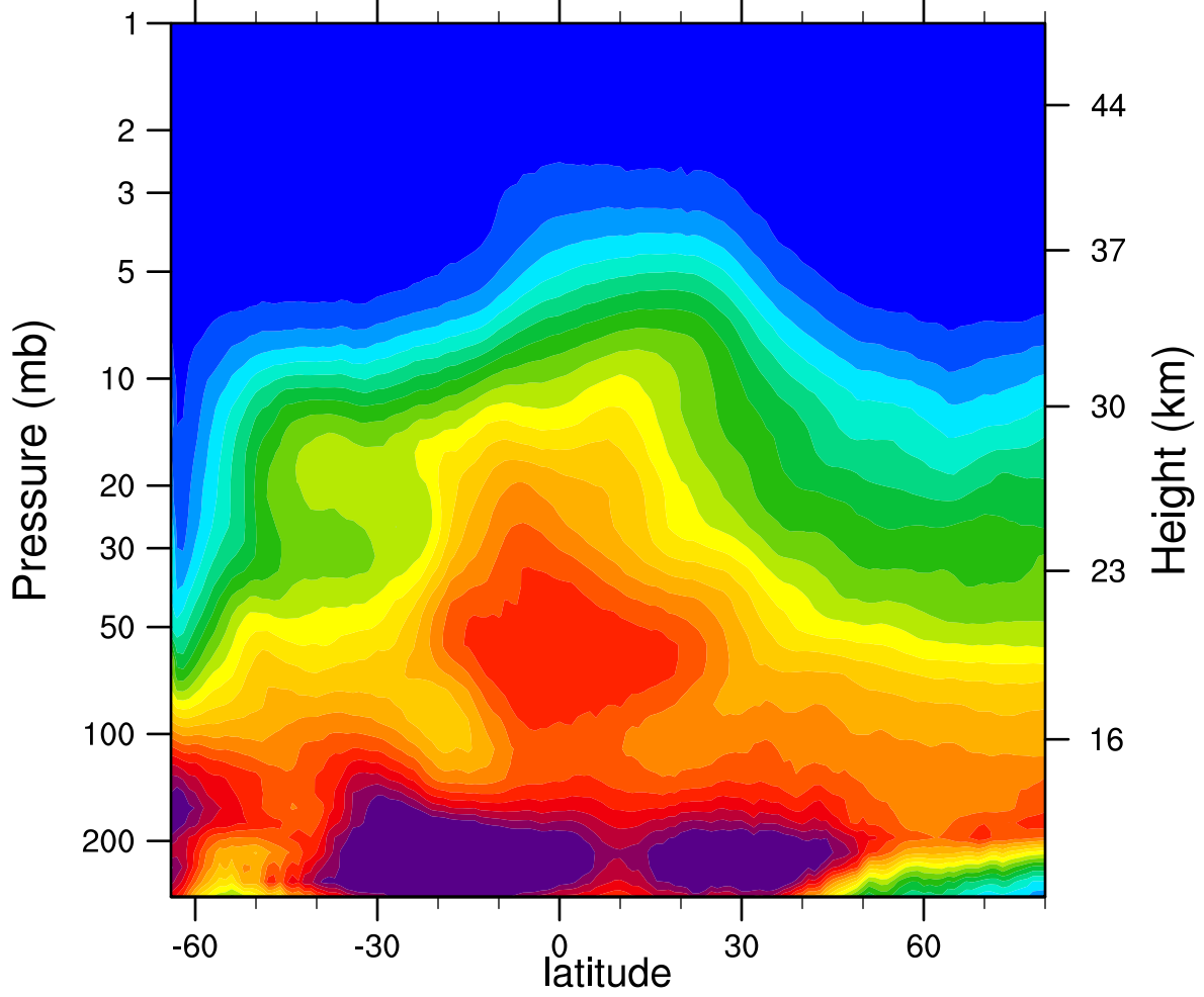
2007d233 N2O_Combined (ppbv)
