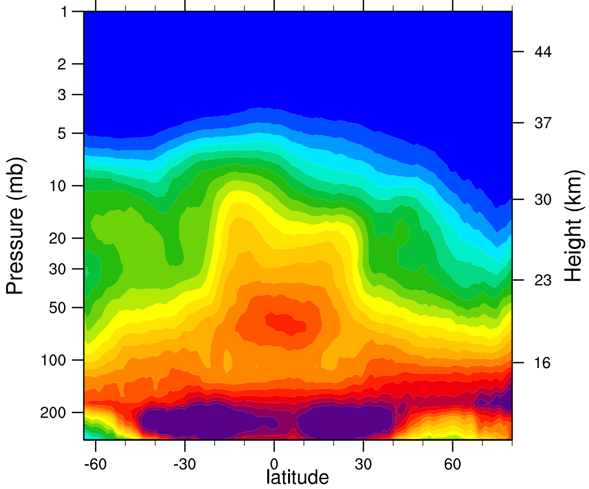
2007d339 N2O_Combined (ppbv)
