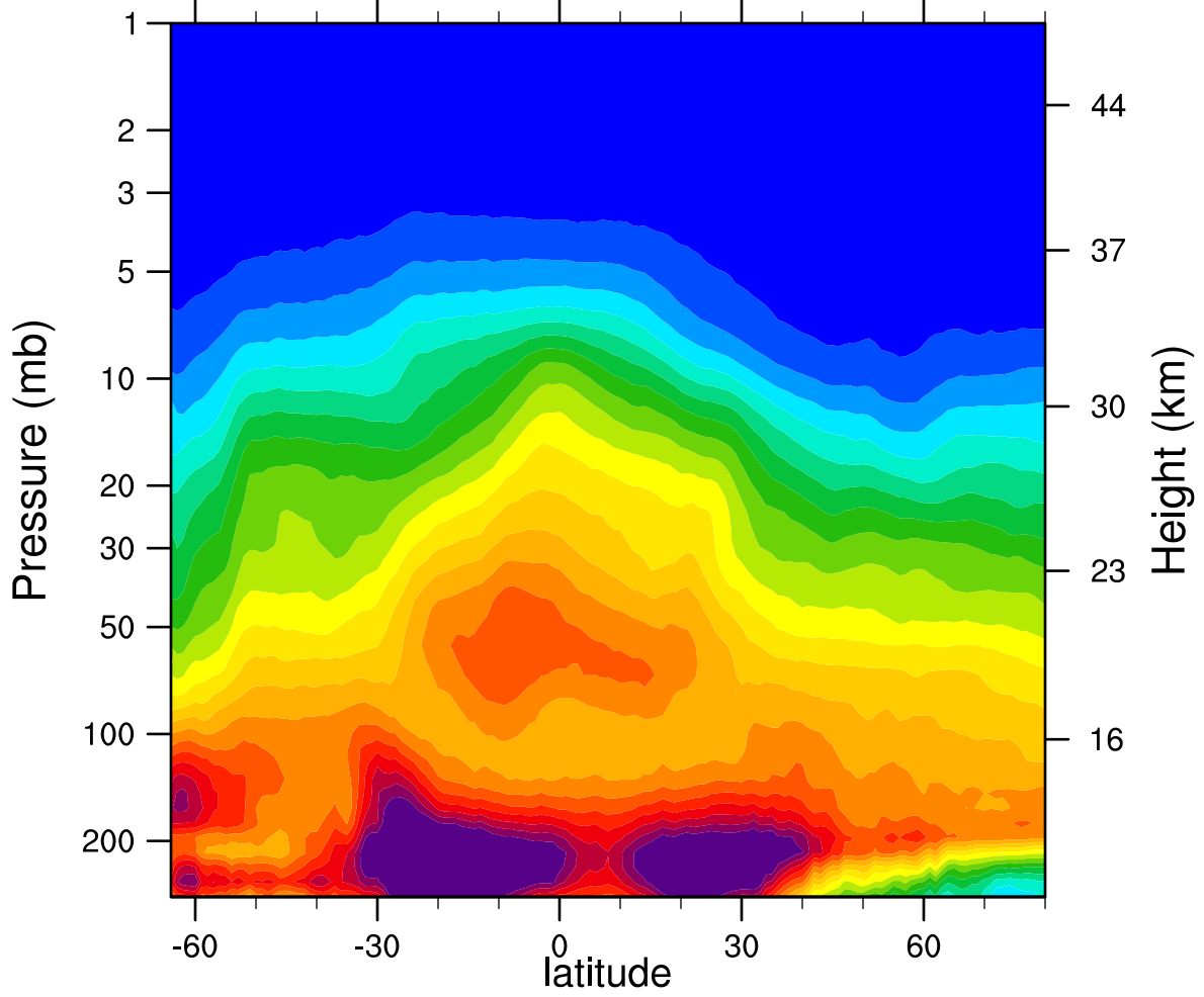
2006d163 N2O_Combined (ppbv)
