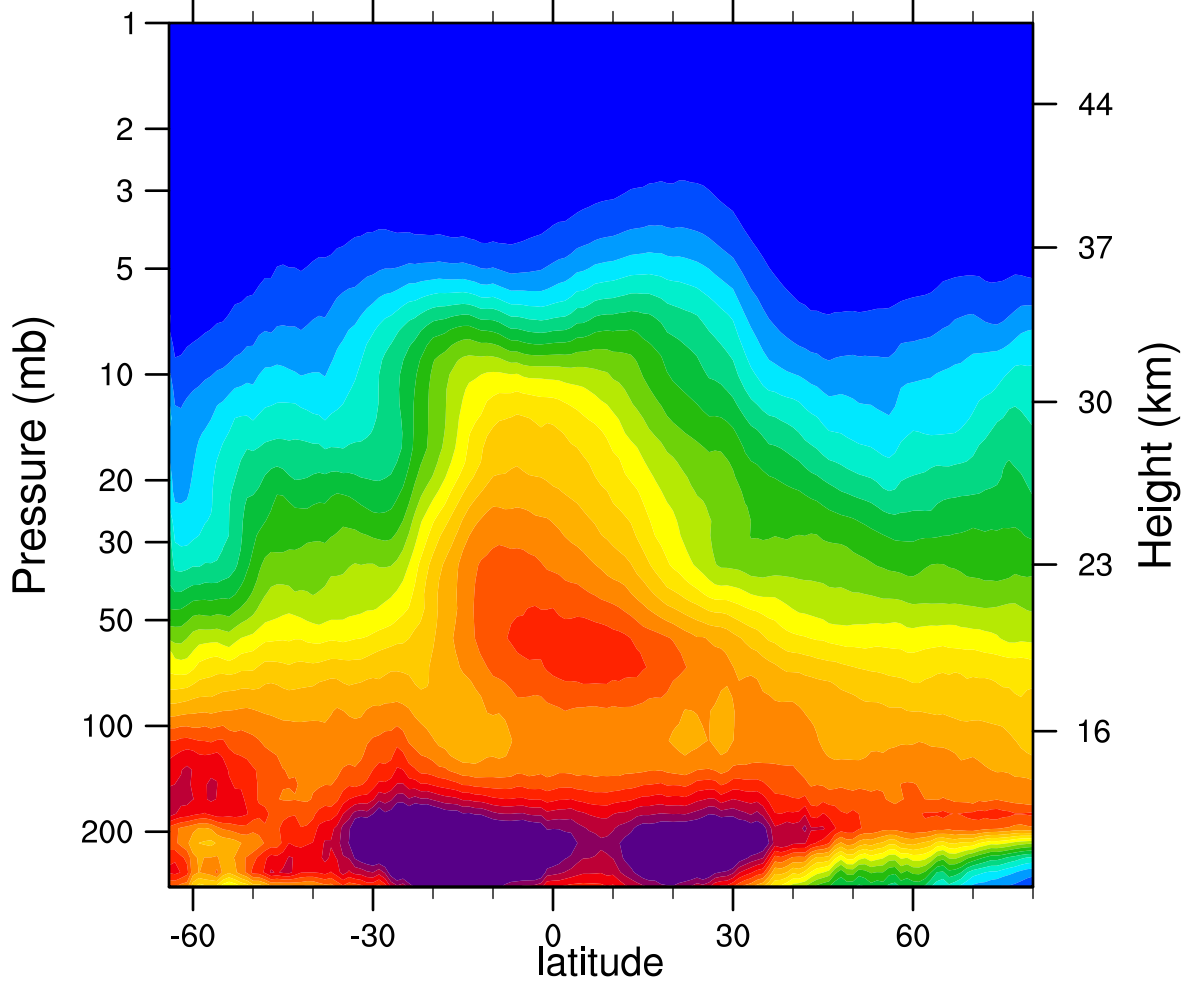
2005d159 N2O_Combined (ppbv)
