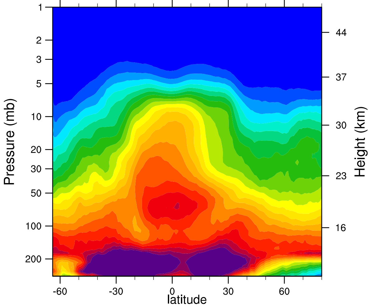
2007d125 N2O_Combined (ppbv)
