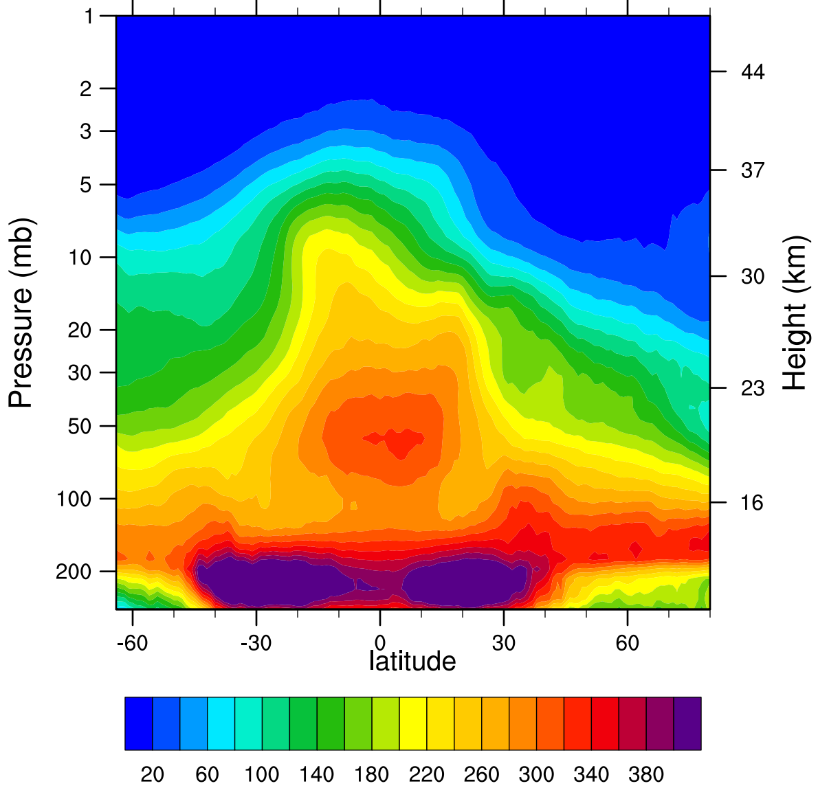
2006d025 N2O_Combined (ppbv)
