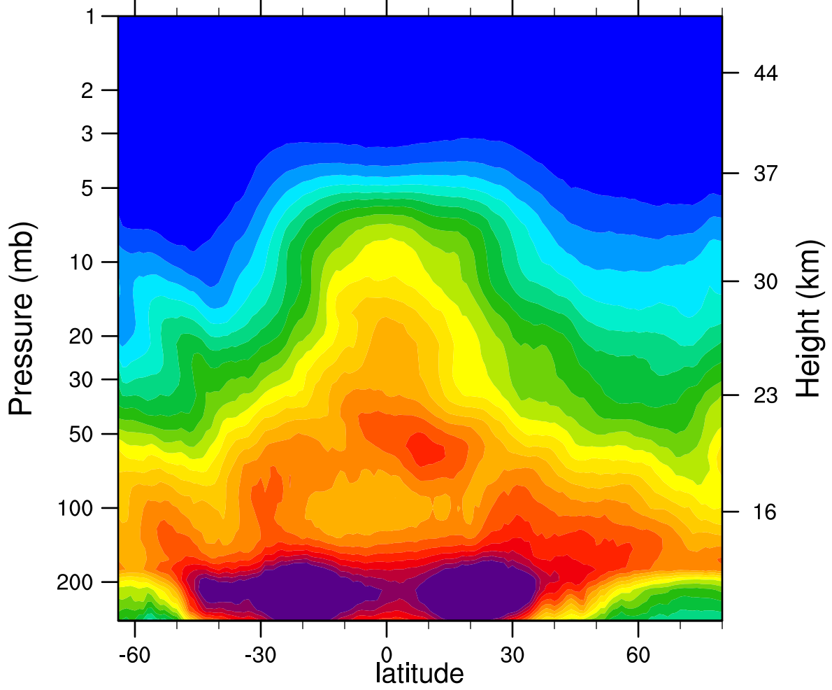
2005d097 N2O_Combined (ppbv)
