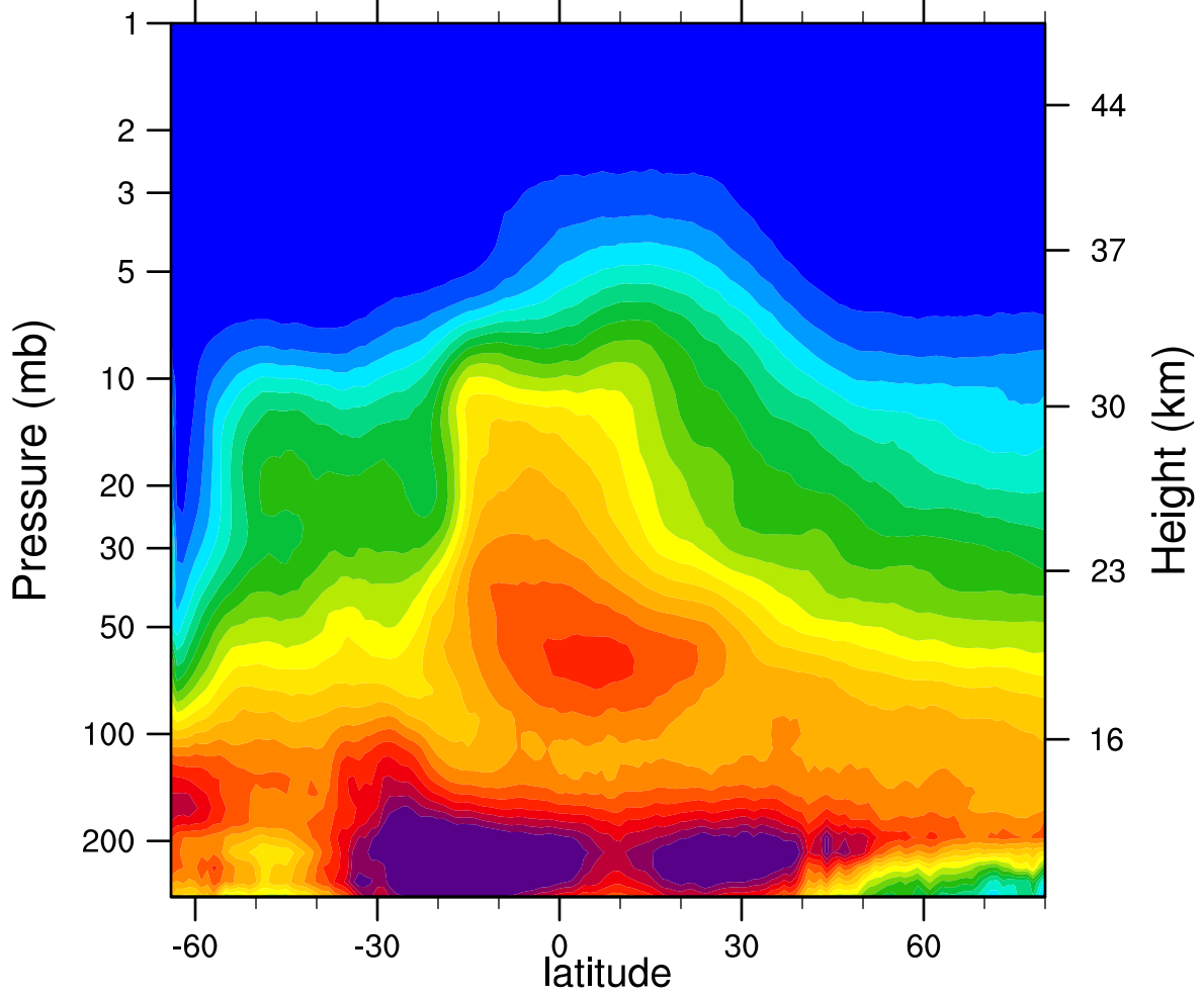
2005d225 N2O_Combined (ppbv)
