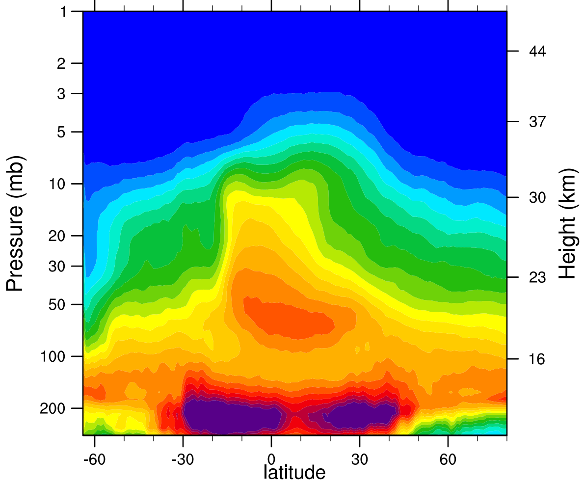
2005d249 N2O_Combined (ppbv)
