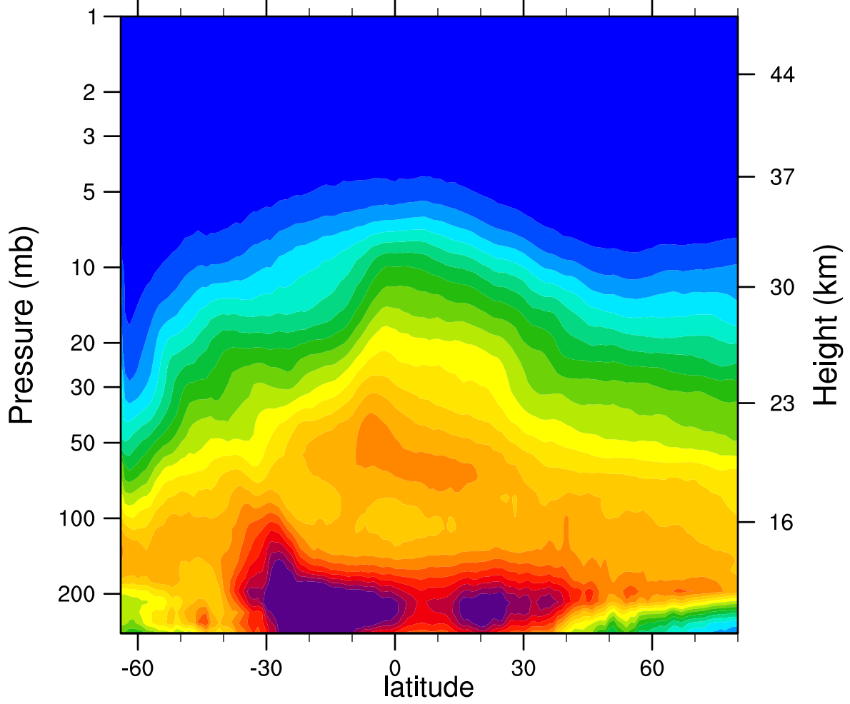
2006d184 N2O_Combined (ppbv)
