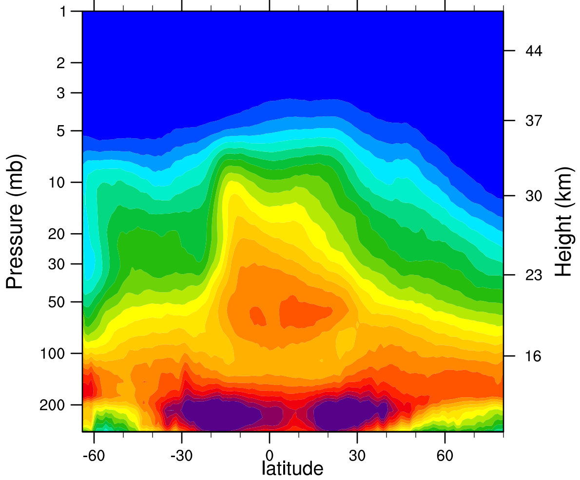
2005d291 N2O_Combined (ppbv)
