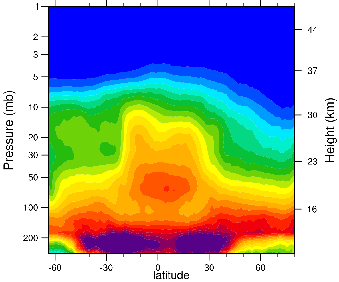
2007d321 N2O_Combined (ppbv)
