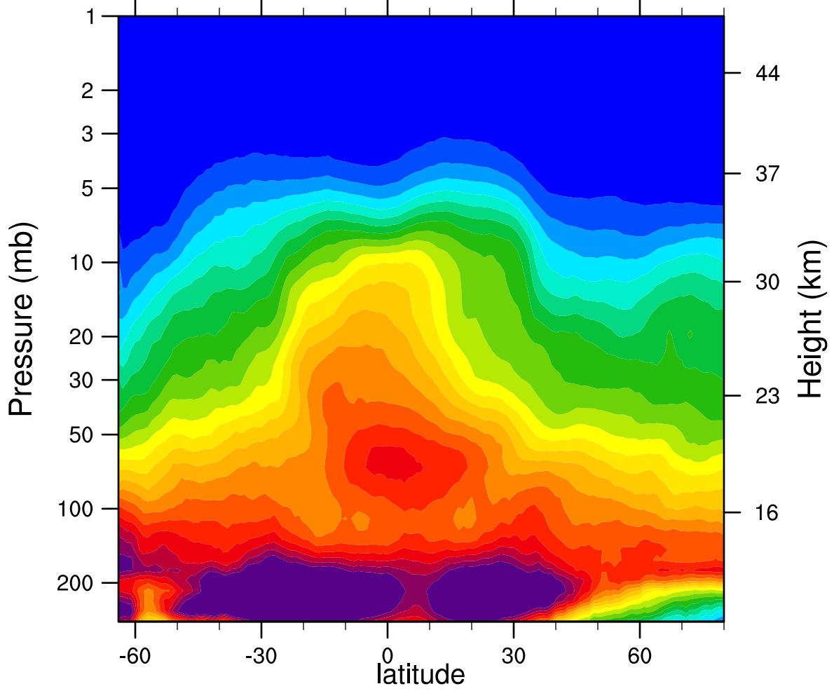
2007d140 N2O_Combined (ppbv)
