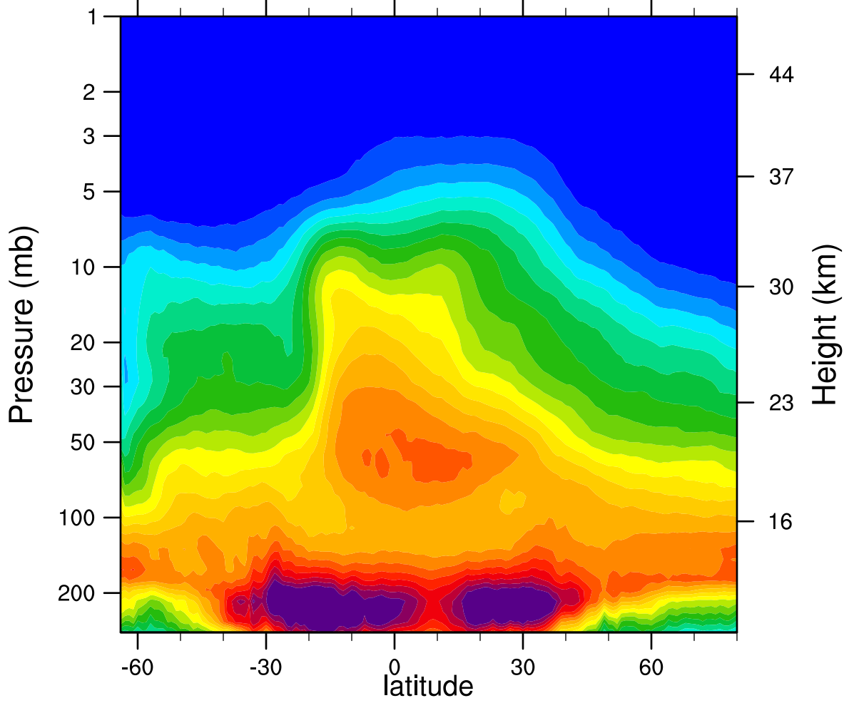
2005d273 N2O_Combined (ppbv)
