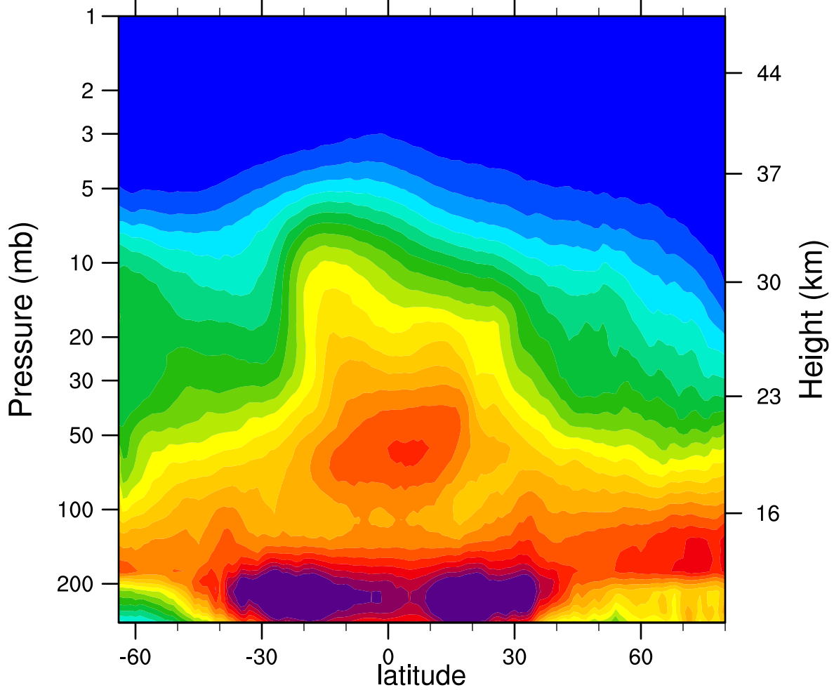
2005d336 N2O_Combined (ppbv)
