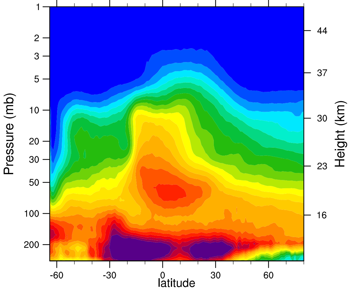
2005d223 N2O_Combined (ppbv)
