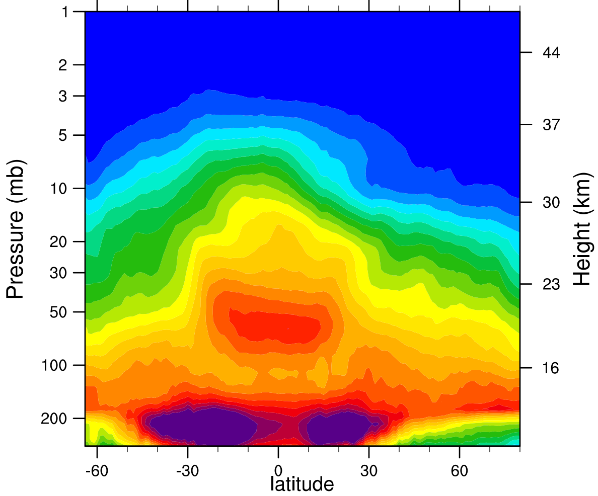
2006d112 N2O_Combined (ppbv)
