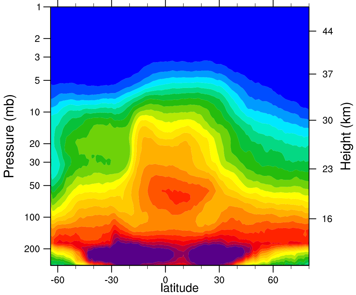
2007d292 N2O_Combined (ppbv)
