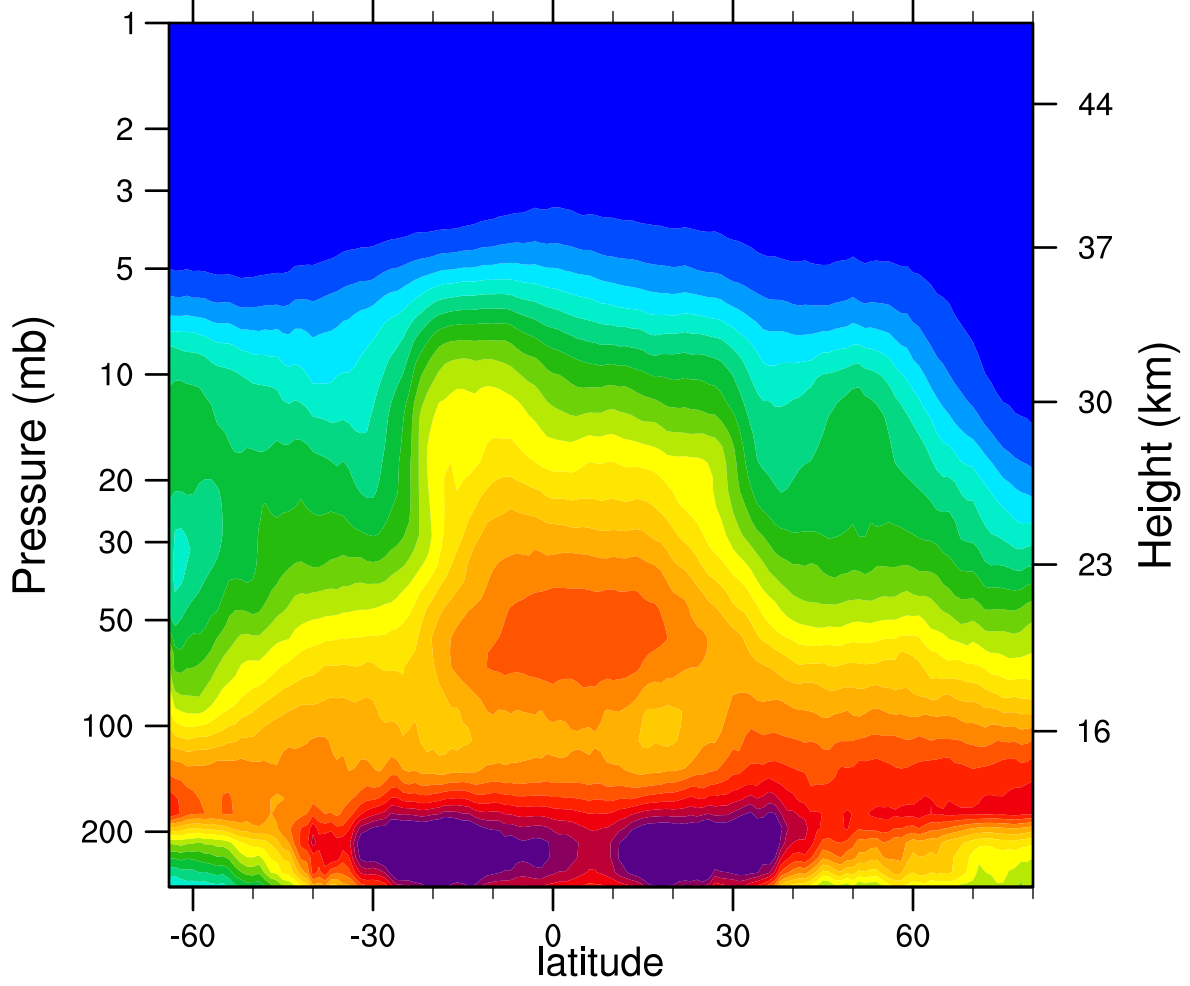
2005d322 N2O_Combined (ppbv)
