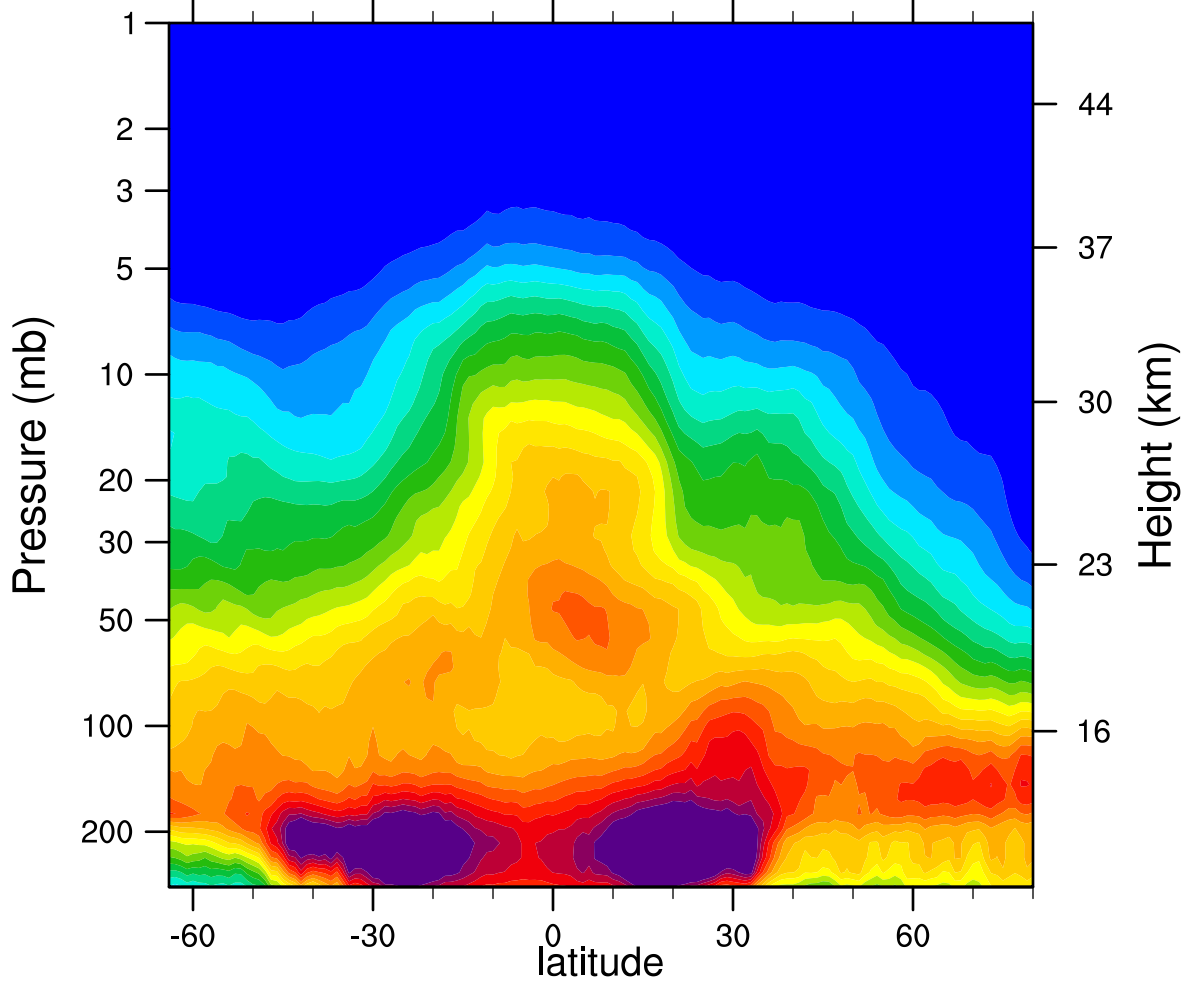
2005d037 N2O_Combined (ppbv)
