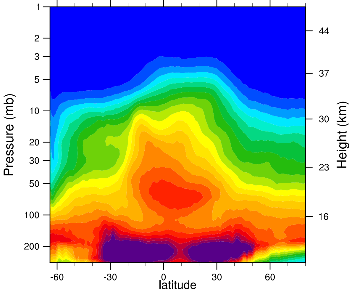
2007d256 N2O_Combined (ppbv)
