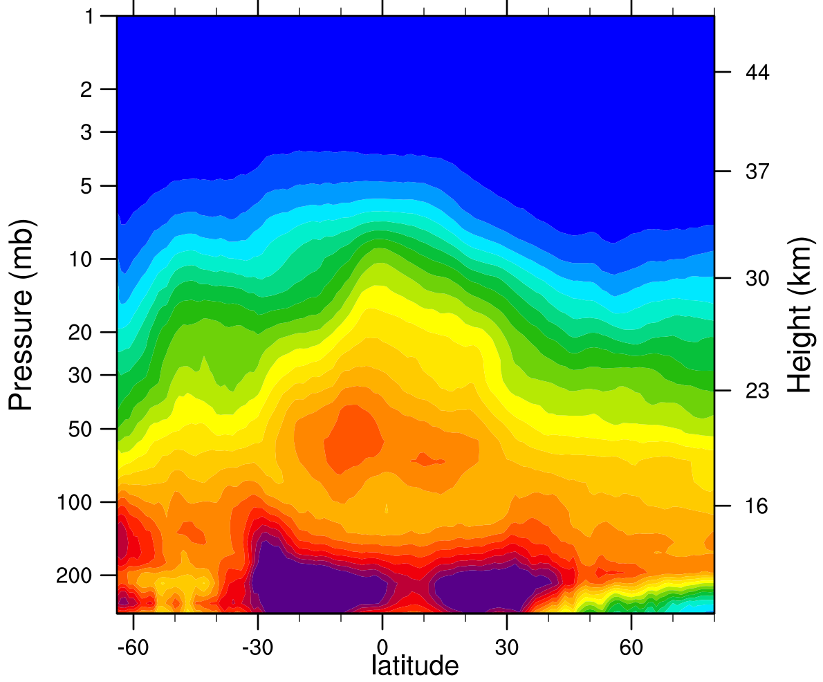
2006d168 N2O_Combined (ppbv)
