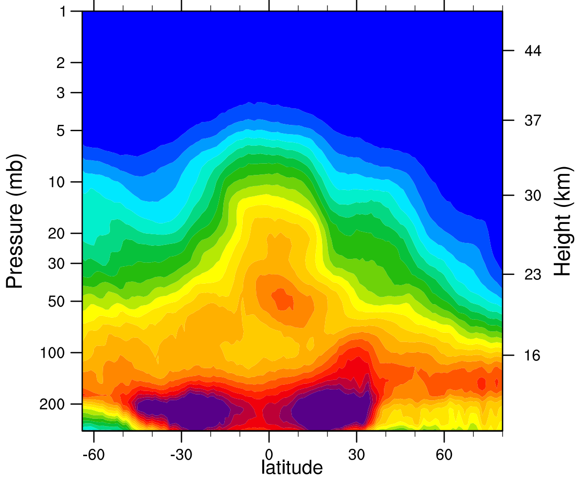
2005d035 N2O_Combined (ppbv)
