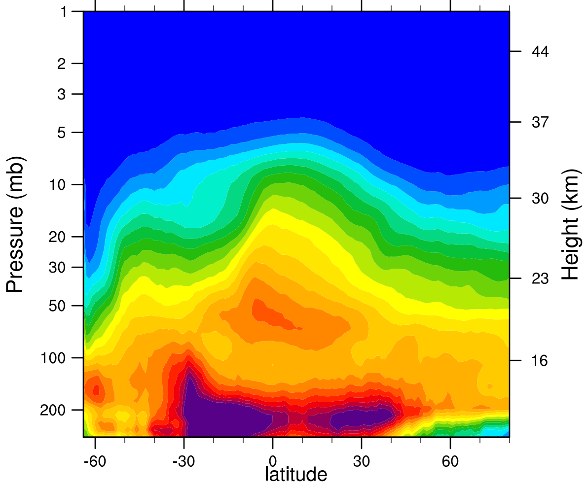
2006d211 N2O_Combined (ppbv)
