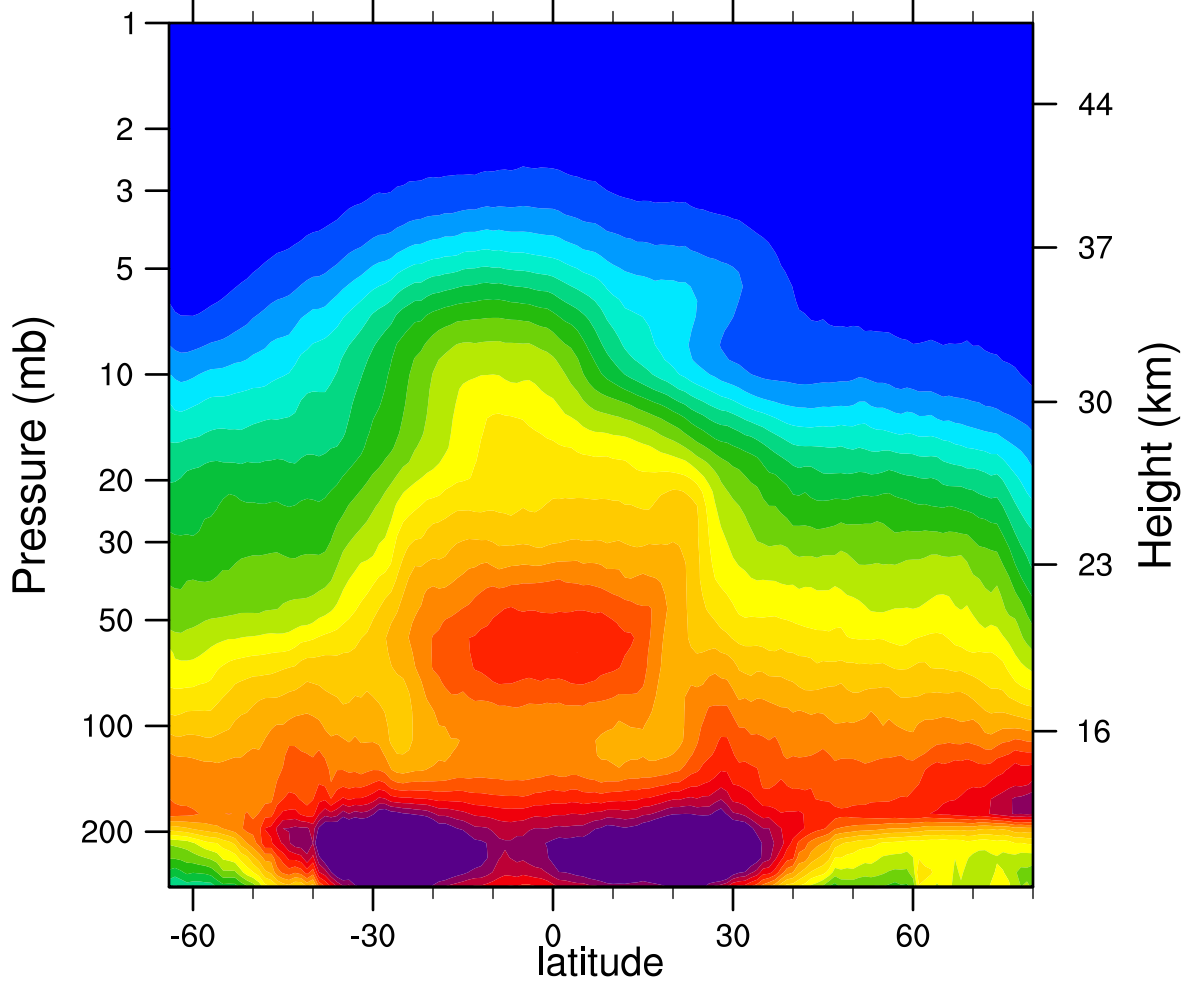
2006d071 N2O_Combined (ppbv)
