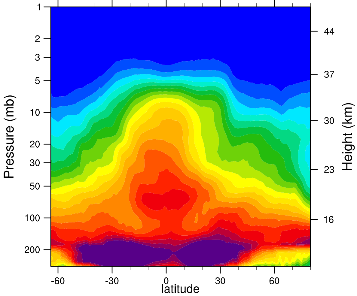
2007d107 N2O_Combined (ppbv)
