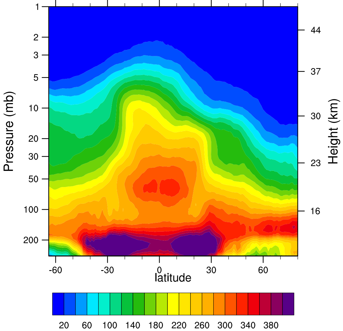
2006d010 N2O_Combined (ppbv)
