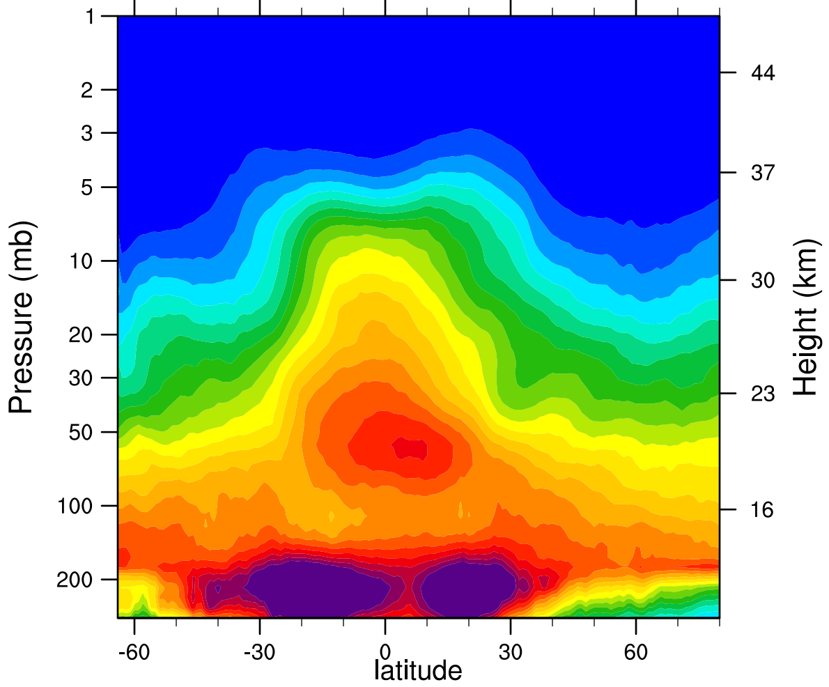
2005d122 N2O_Combined (ppbv)
