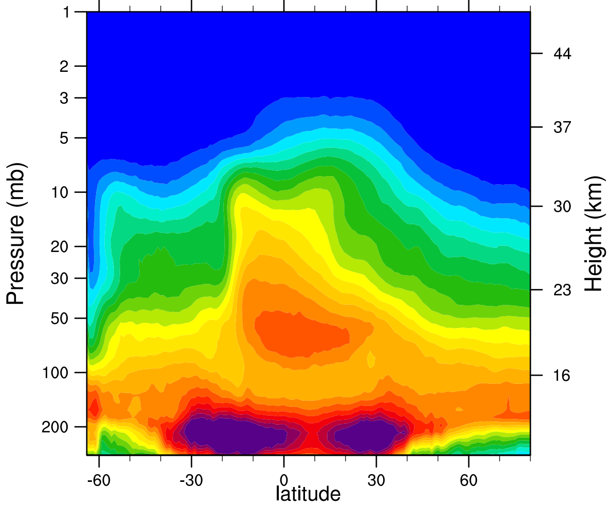
2005d261 N2O_Combined (ppbv)
