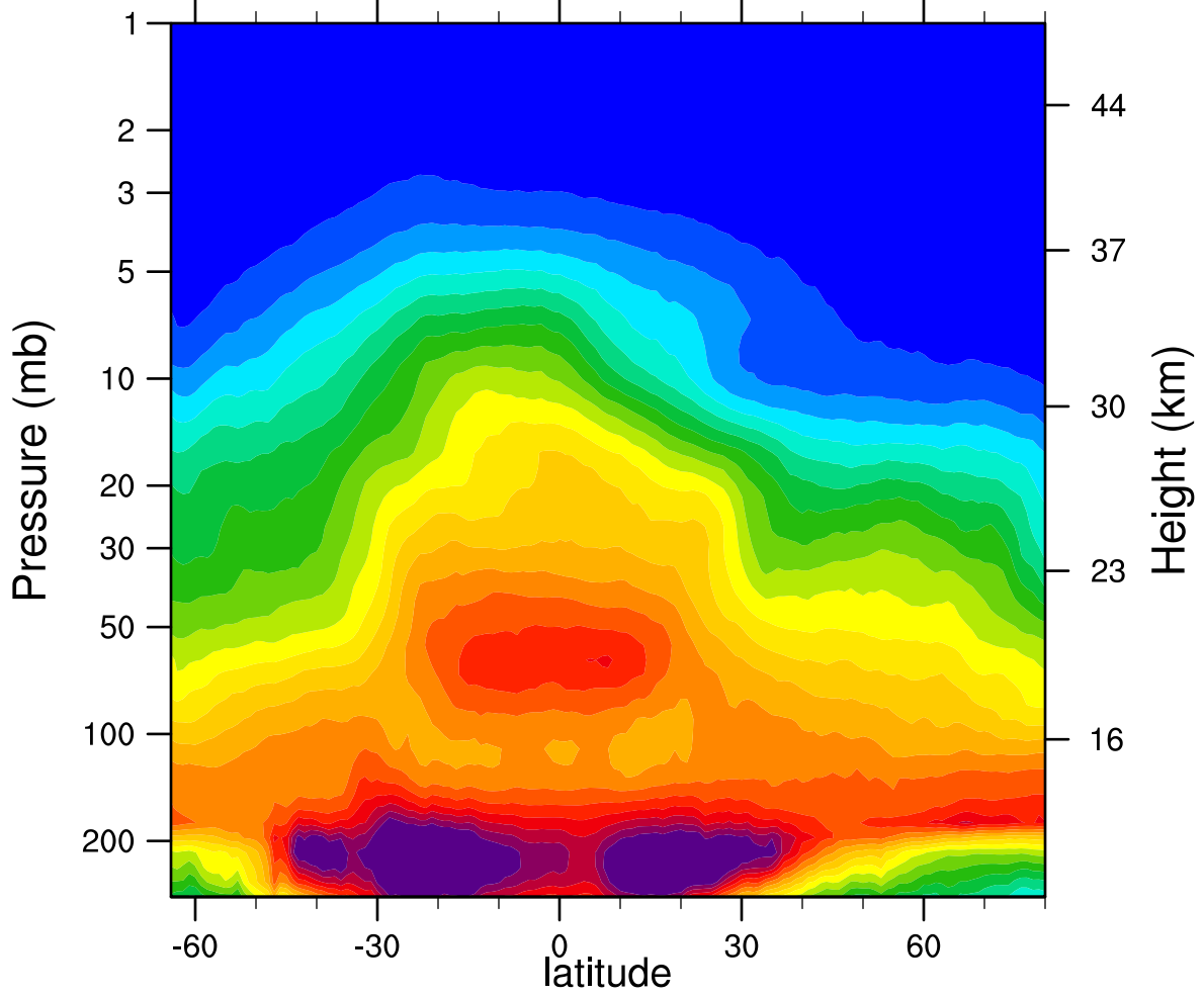
2006d102 N2O_Combined (ppbv)
