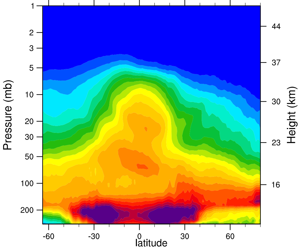
2007d027 N2O_Combined (ppbv)
