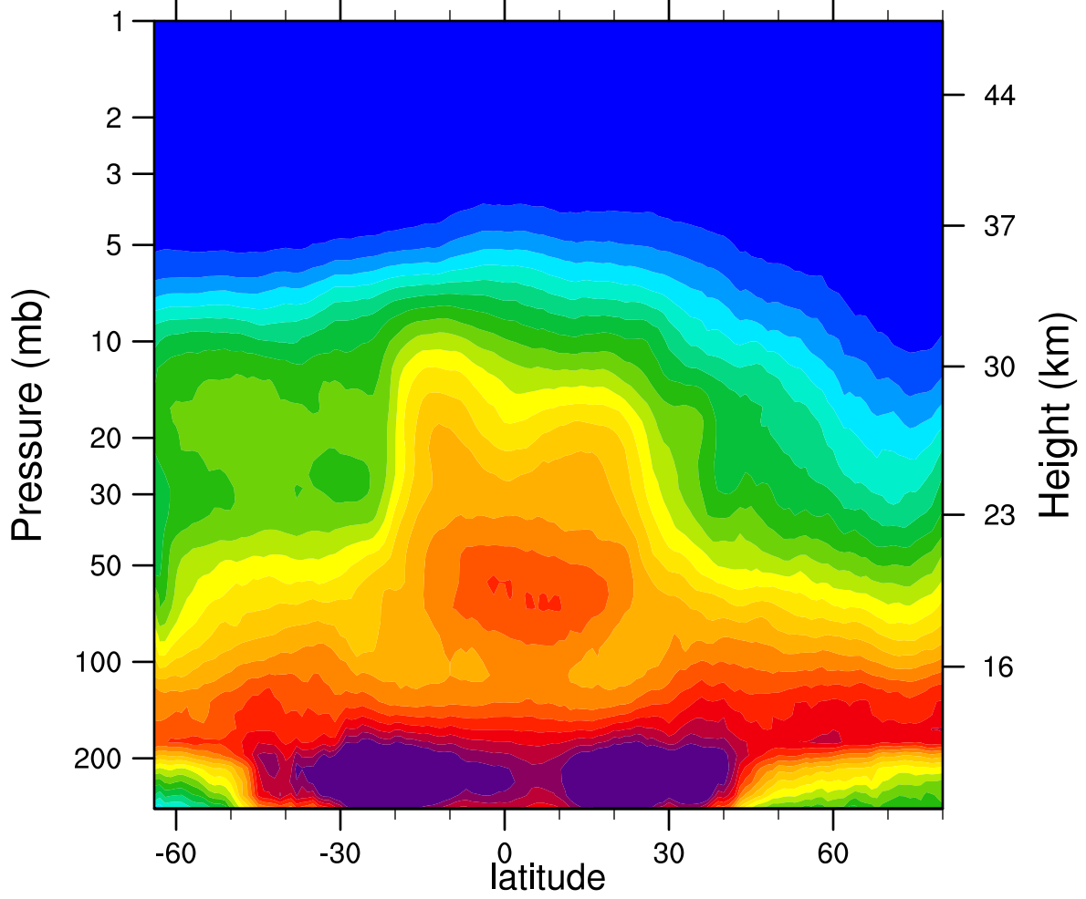
2007d318 N2O_Combined (ppbv)
