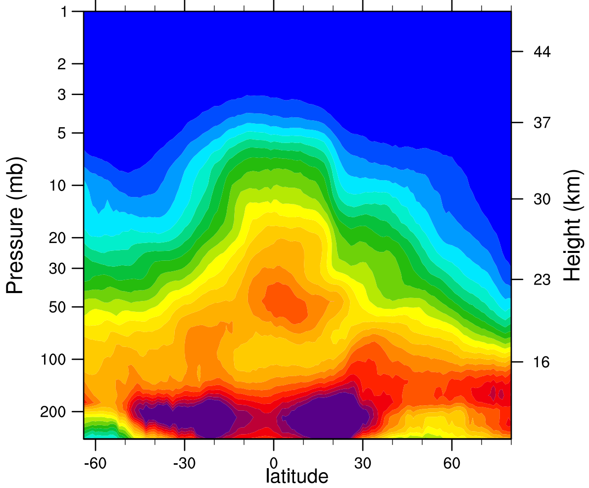
2005d048 N2O_Combined (ppbv)
