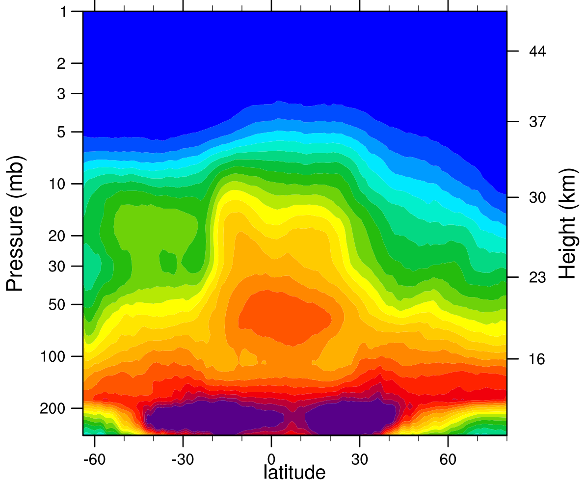
2007d304 N2O_Combined (ppbv)
