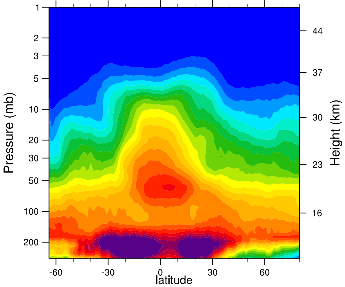
2005d140 N2O_Combined (ppbv)
