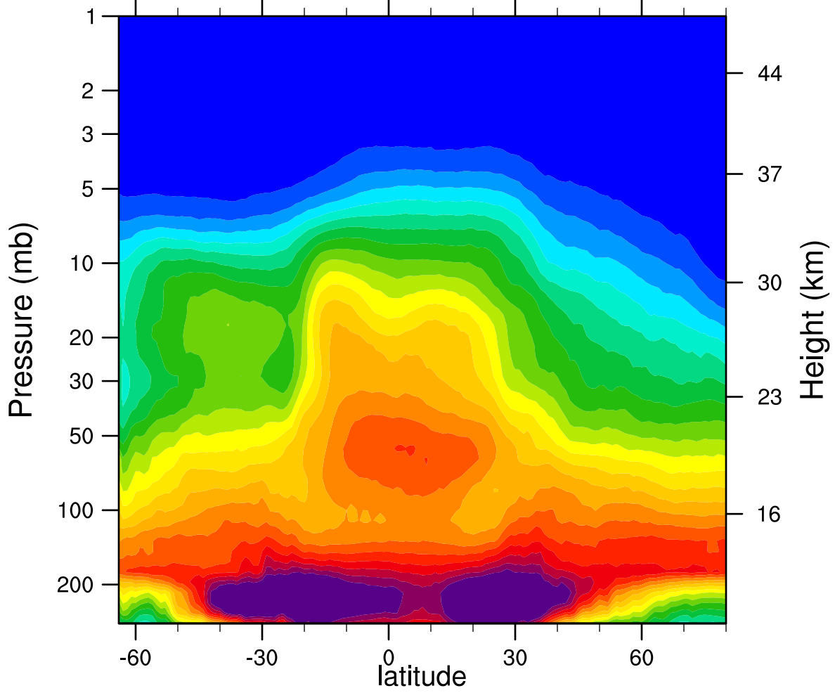
2007d300 N2O_Combined (ppbv)
