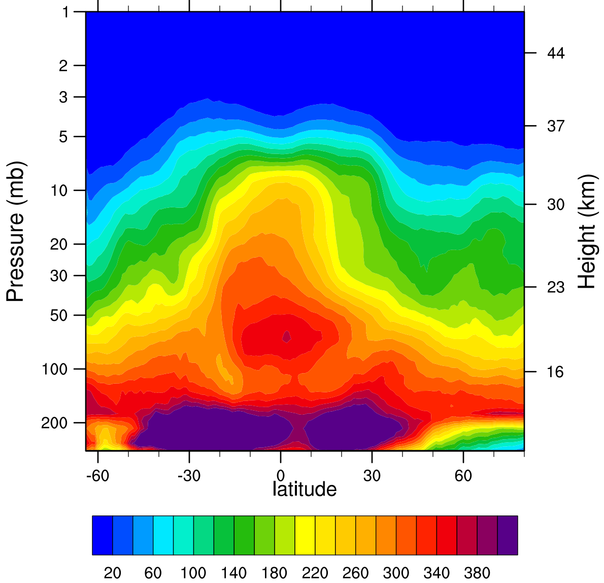
2007d127 N2O_Combined (ppbv)
