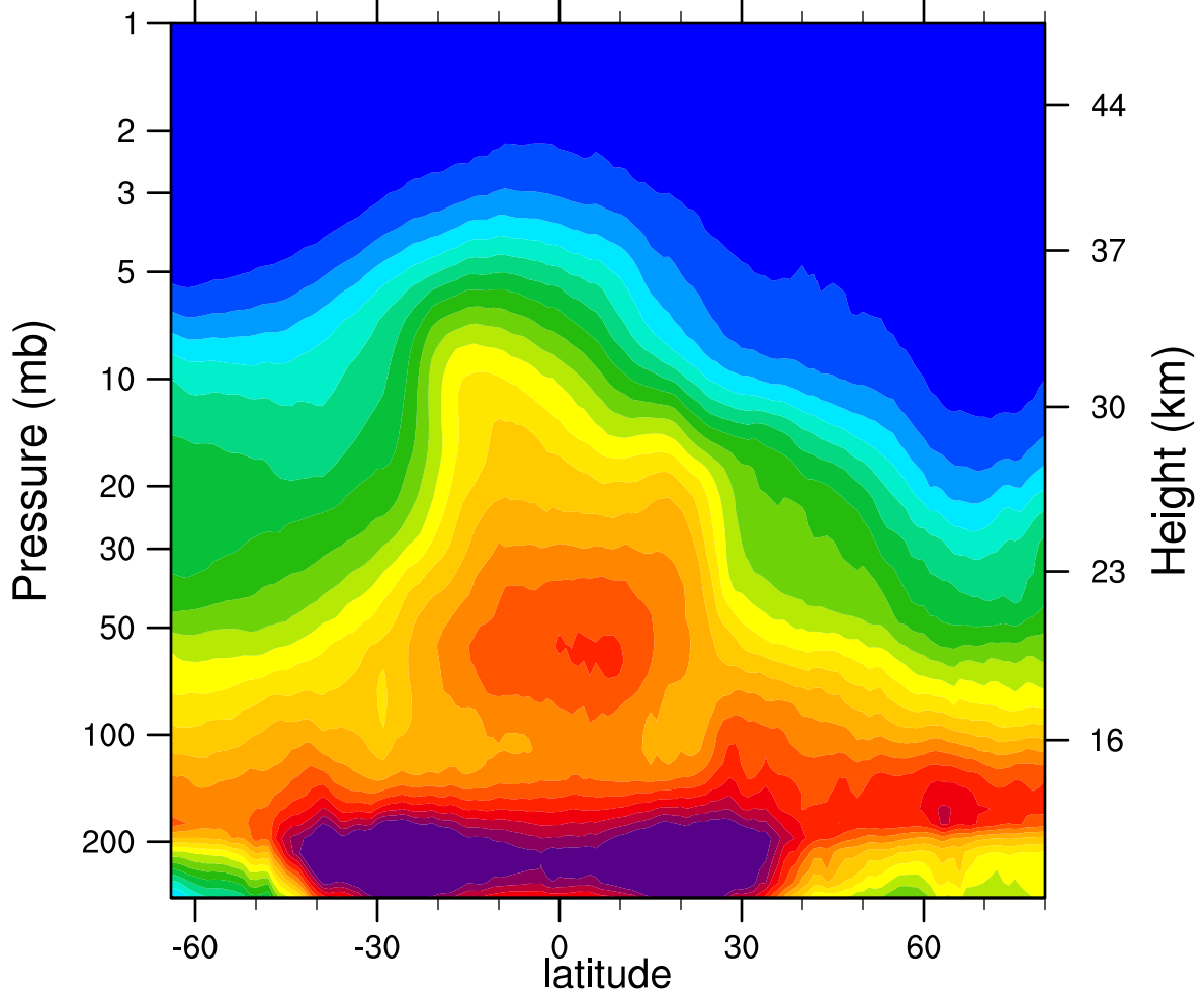
2006d017 N2O_Combined (ppbv)
