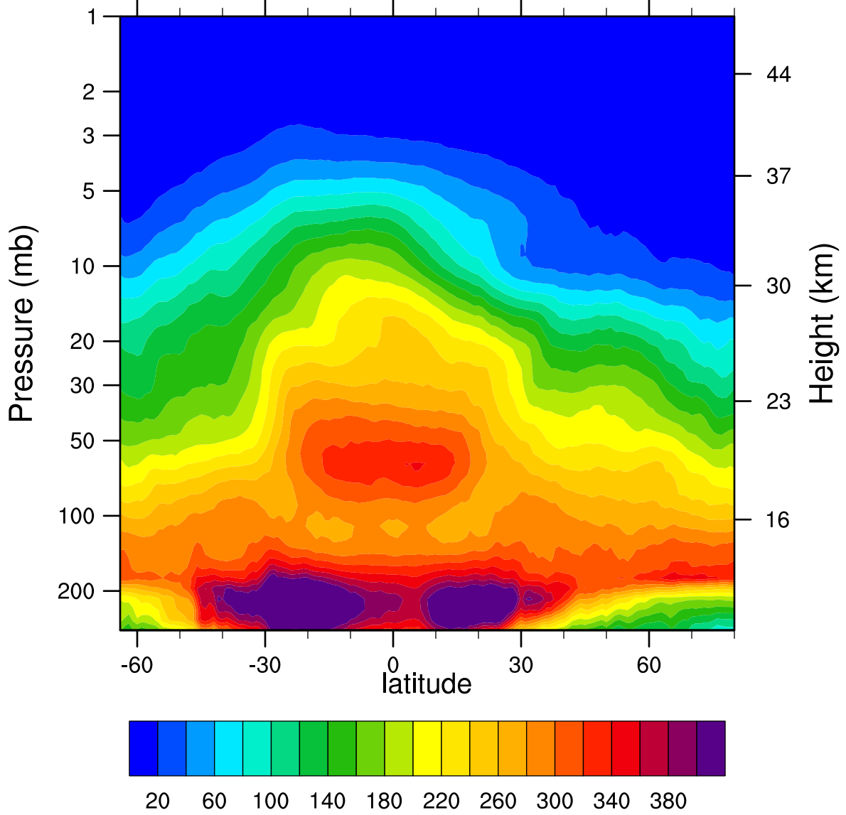
2006d107 N2O_Combined (ppbv)
