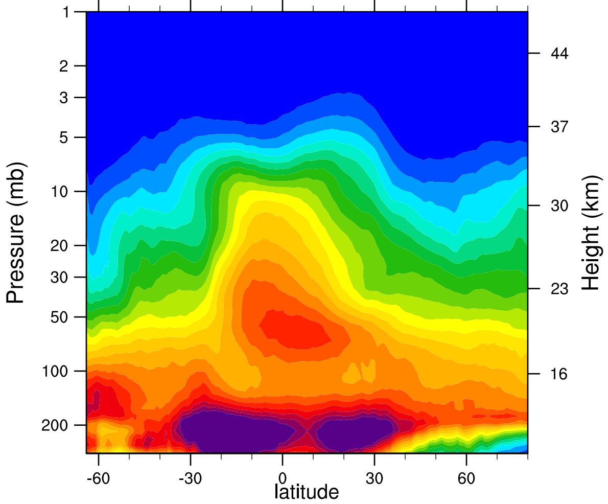
2005d158 N2O_Combined (ppbv)
