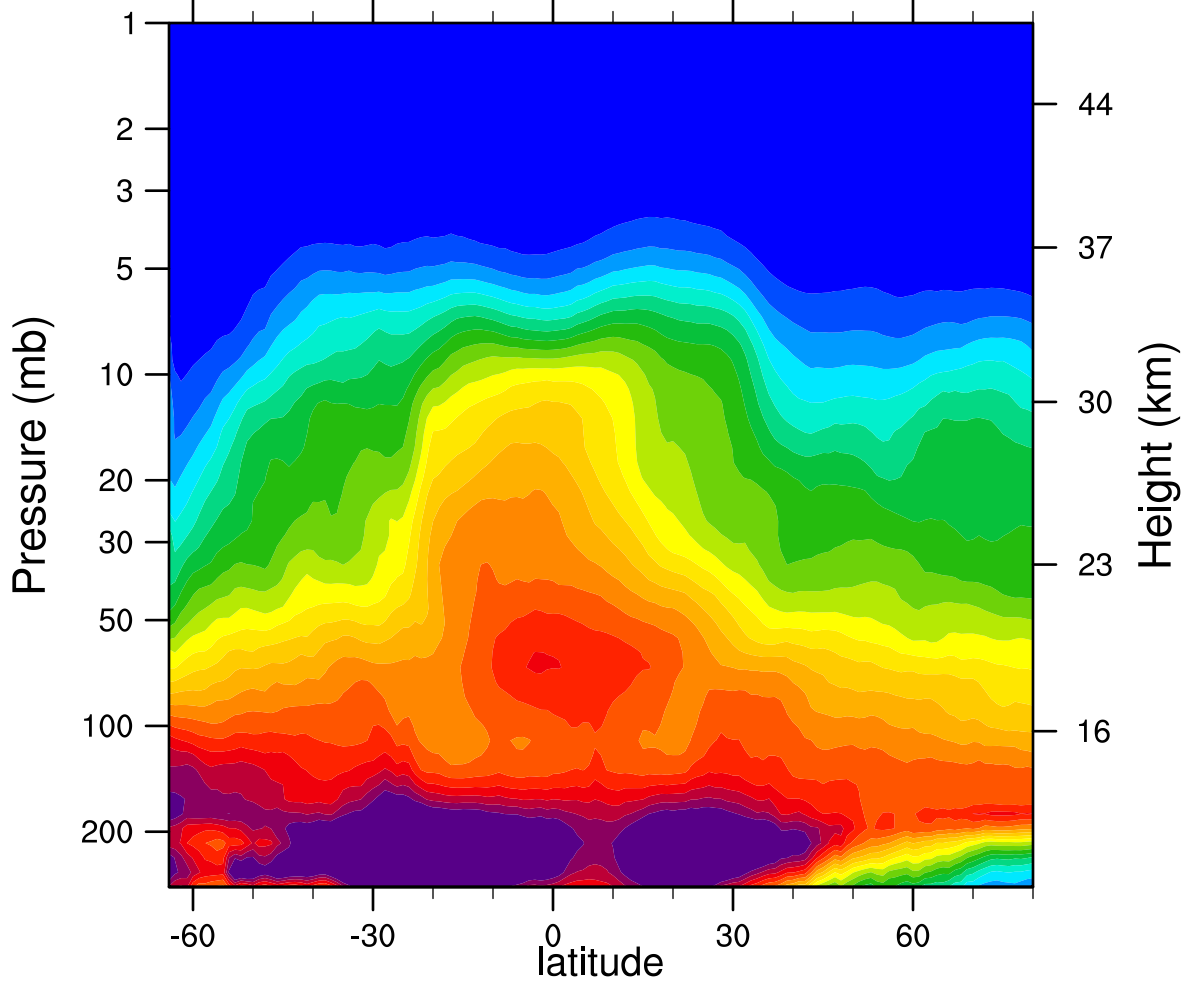
2007d148 N2O_Combined (ppbv)
