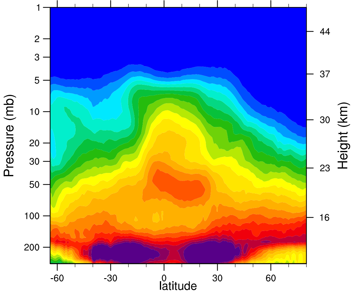
2006d317 N2O_Combined (ppbv)
