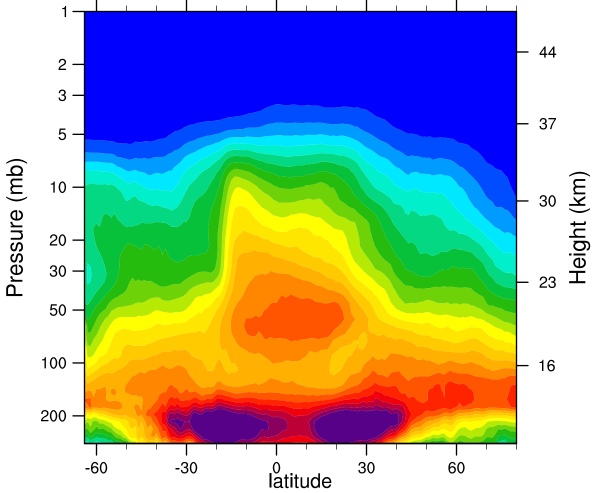
2005d305 N2O_Combined (ppbv)
