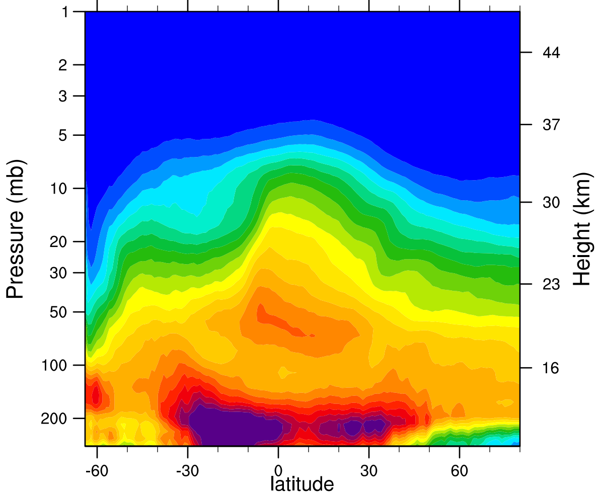
2006d219 N2O_Combined (ppbv)
