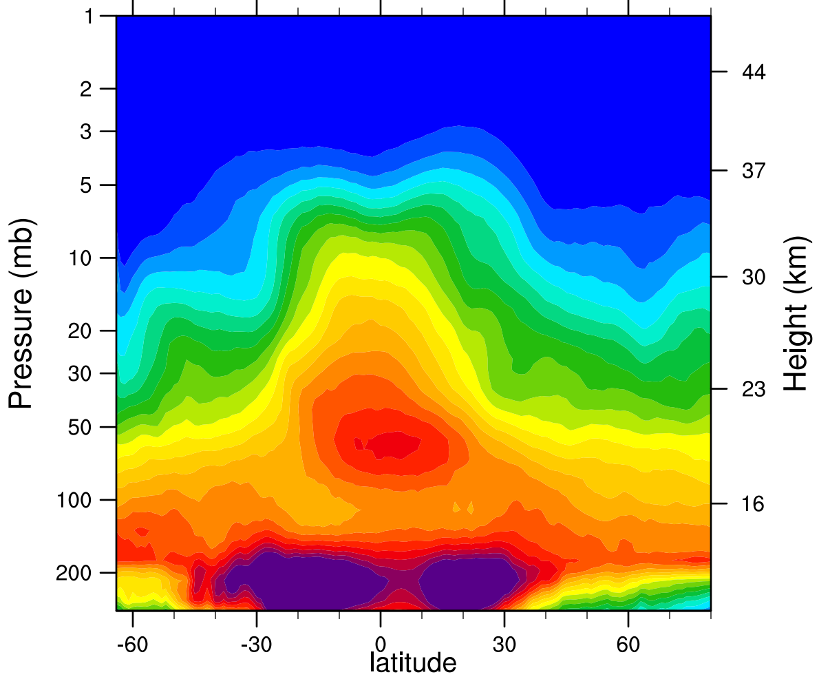
2005d132 N2O_Combined (ppbv)
