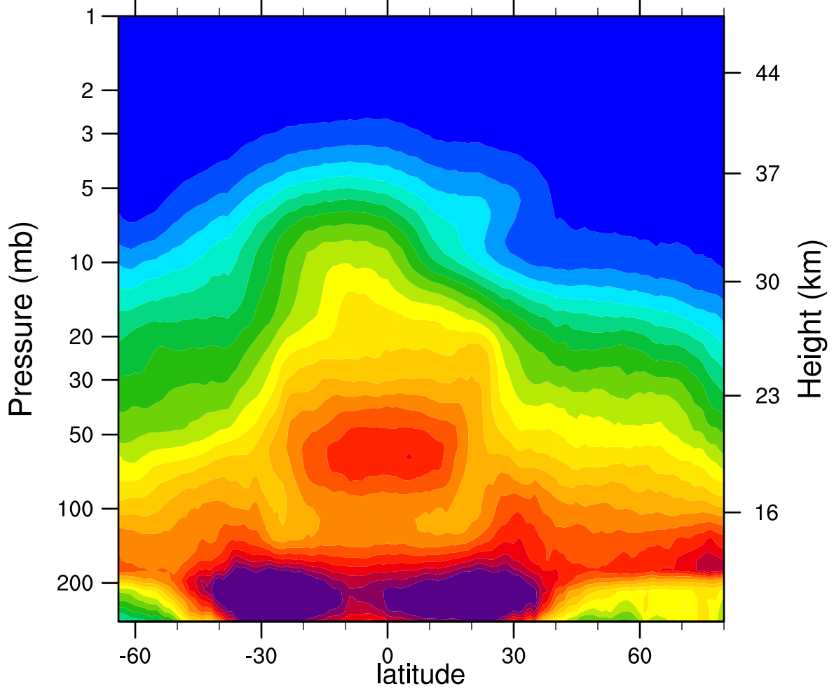
2006d073 N2O_Combined (ppbv)
