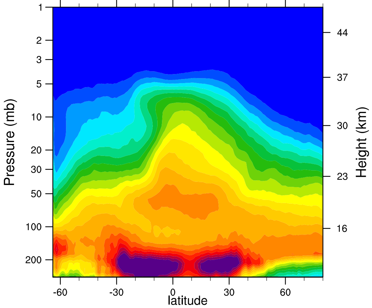
2006d276 N2O_Combined (ppbv)
