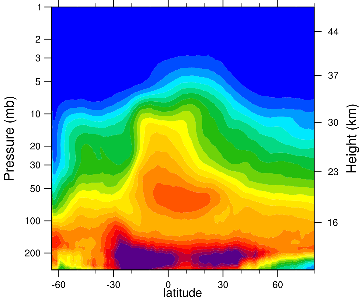
2005d233 N2O_Combined (ppbv)
