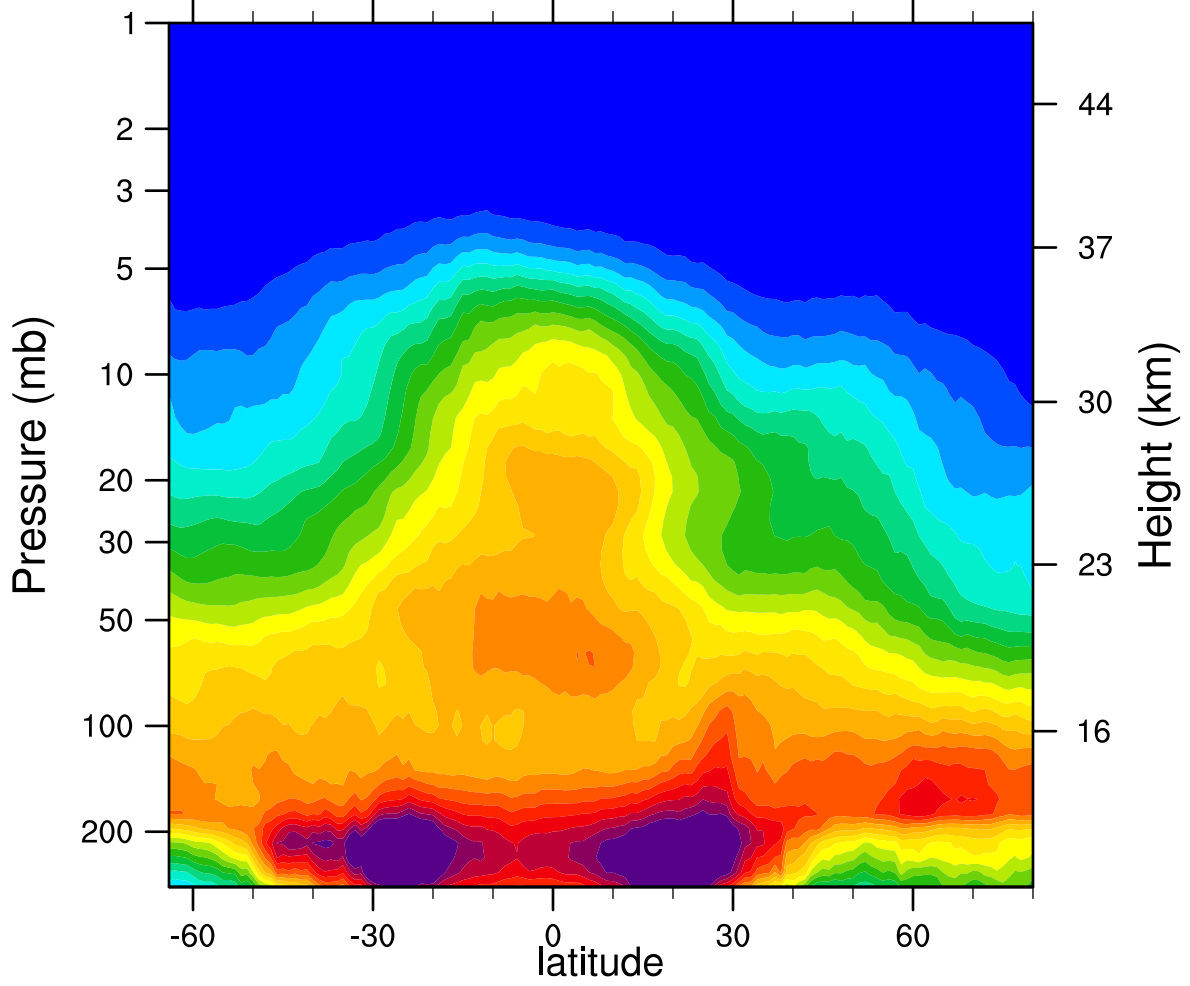
2007d052 N2O_Combined (ppbv)
