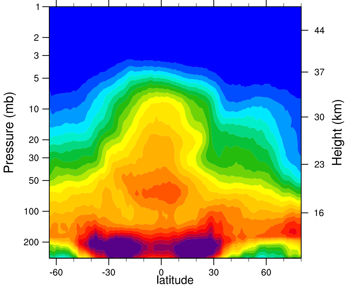
2007d073 N2O_Combined (ppbv)
