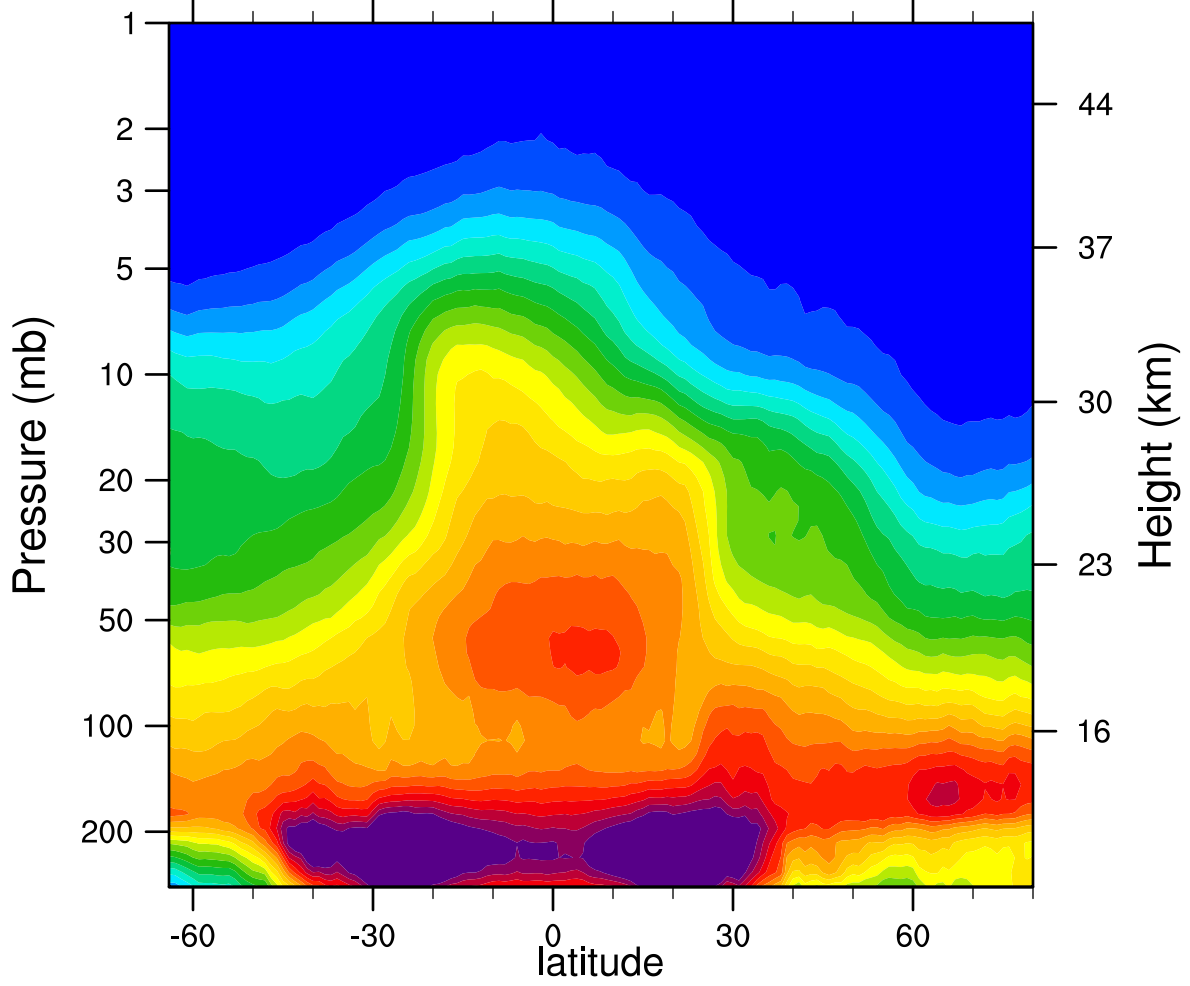
2006d015 N2O_Combined (ppbv)
