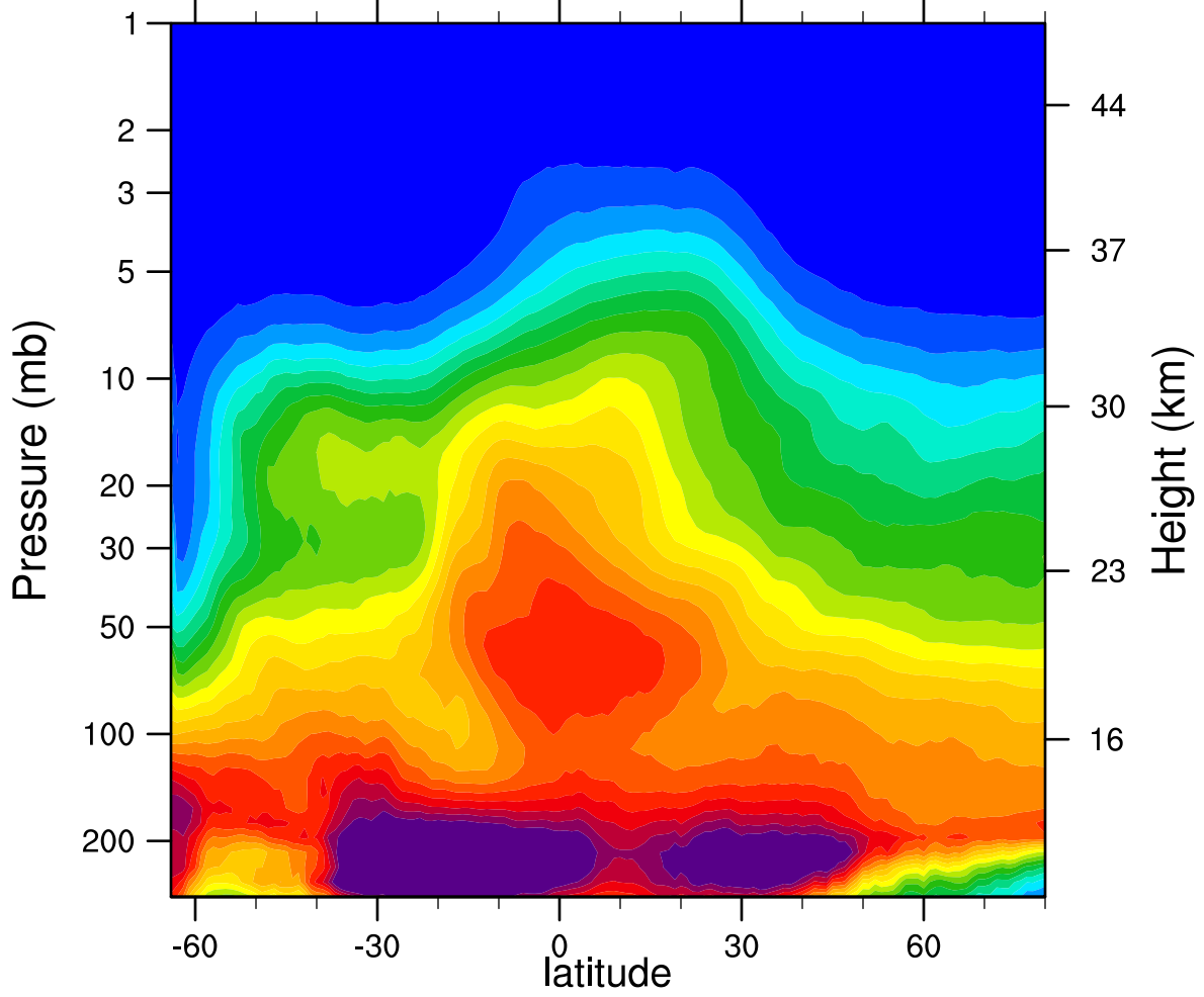
2007d223 N2O_Combined (ppbv)
