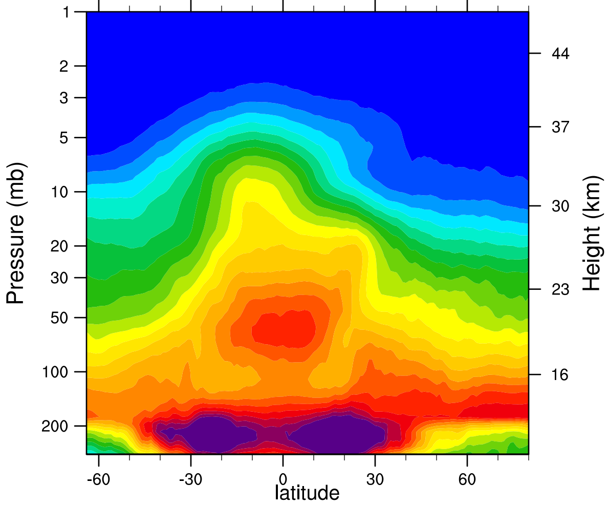
2006d054 N2O_Combined (ppbv)
