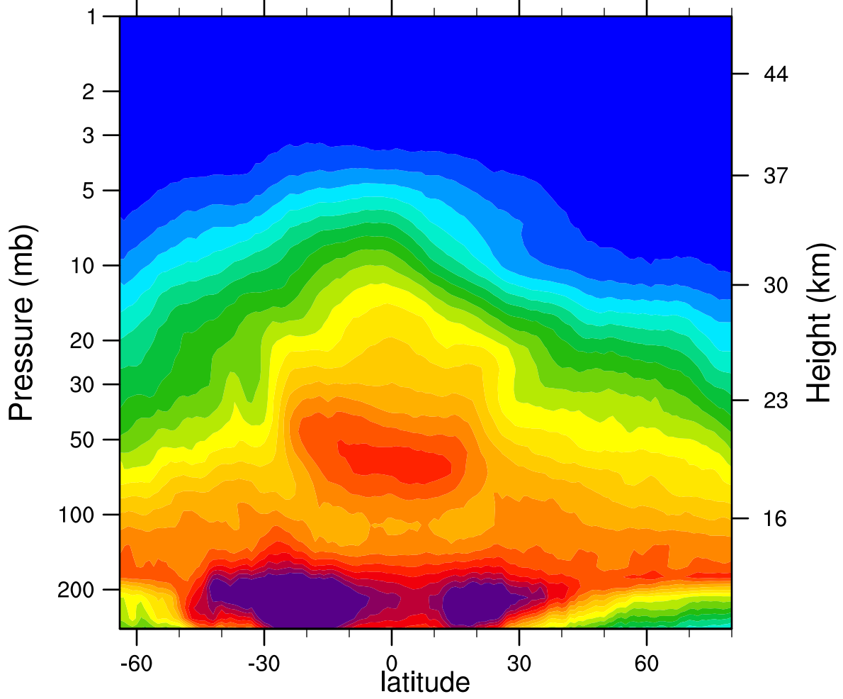
2006d120 N2O_Combined (ppbv)
