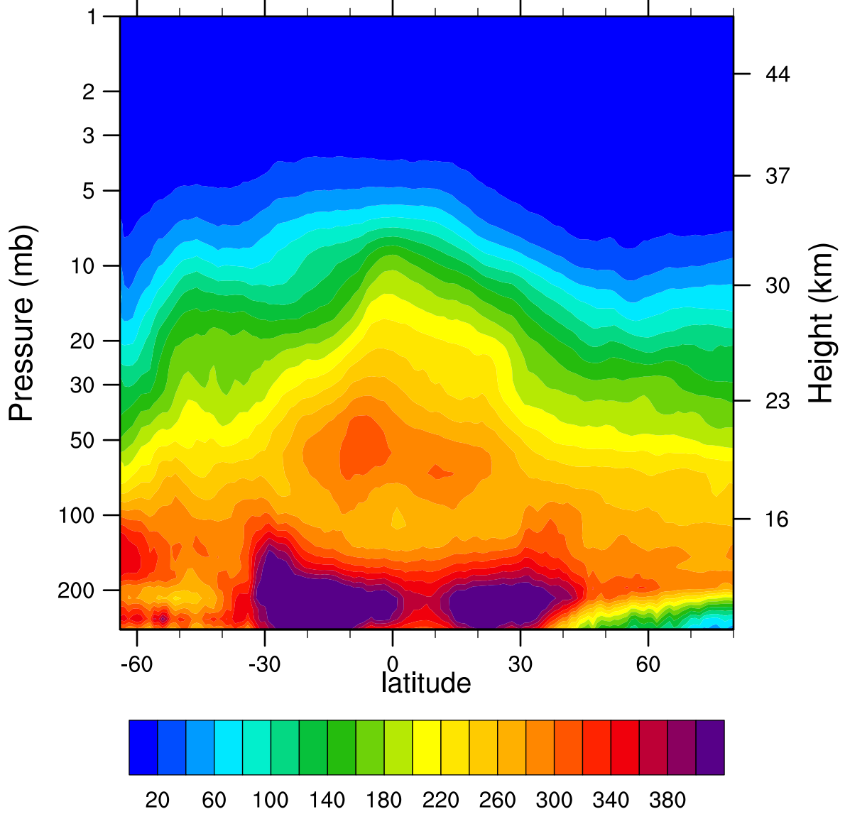
2006d170 N2O_Combined (ppbv)
