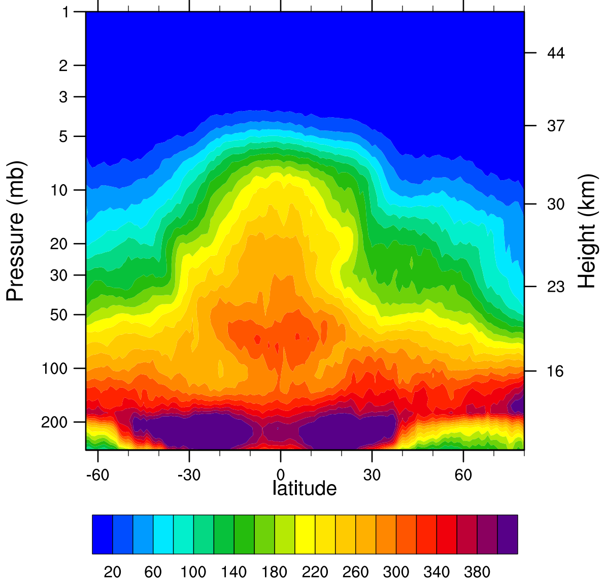
2007d078 N2O_Combined (ppbv)
