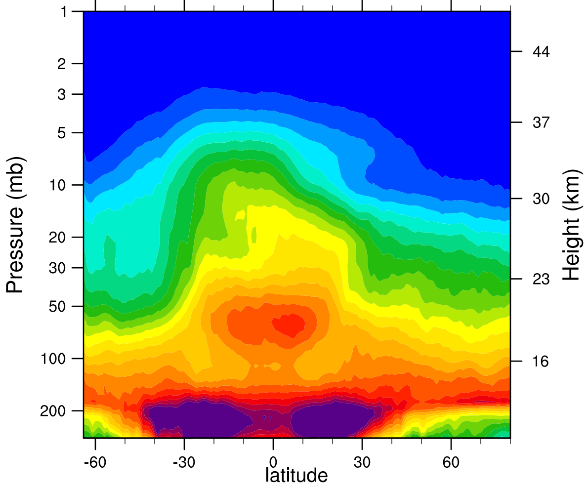
2006d094 N2O_Combined (ppbv)
