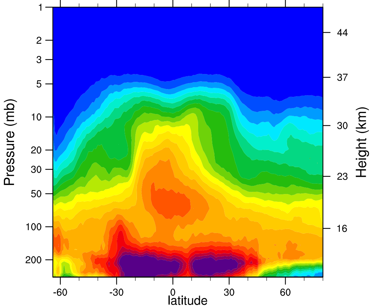
2007d165 N2O_Combined (ppbv)
