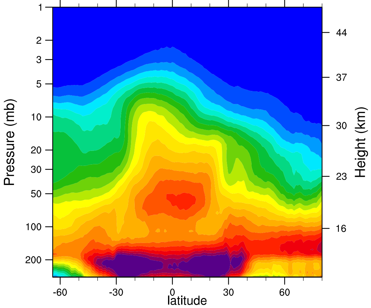
2005d364 N2O_Combined (ppbv)
