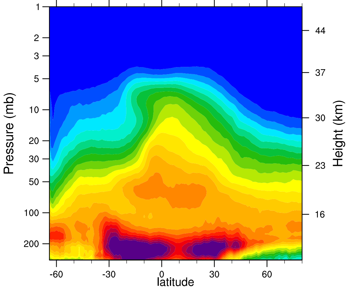
2006d267 N2O_Combined (ppbv)
