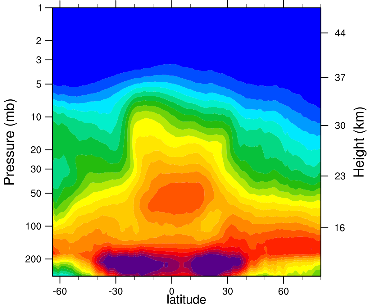
2005d329 N2O_Combined (ppbv)
