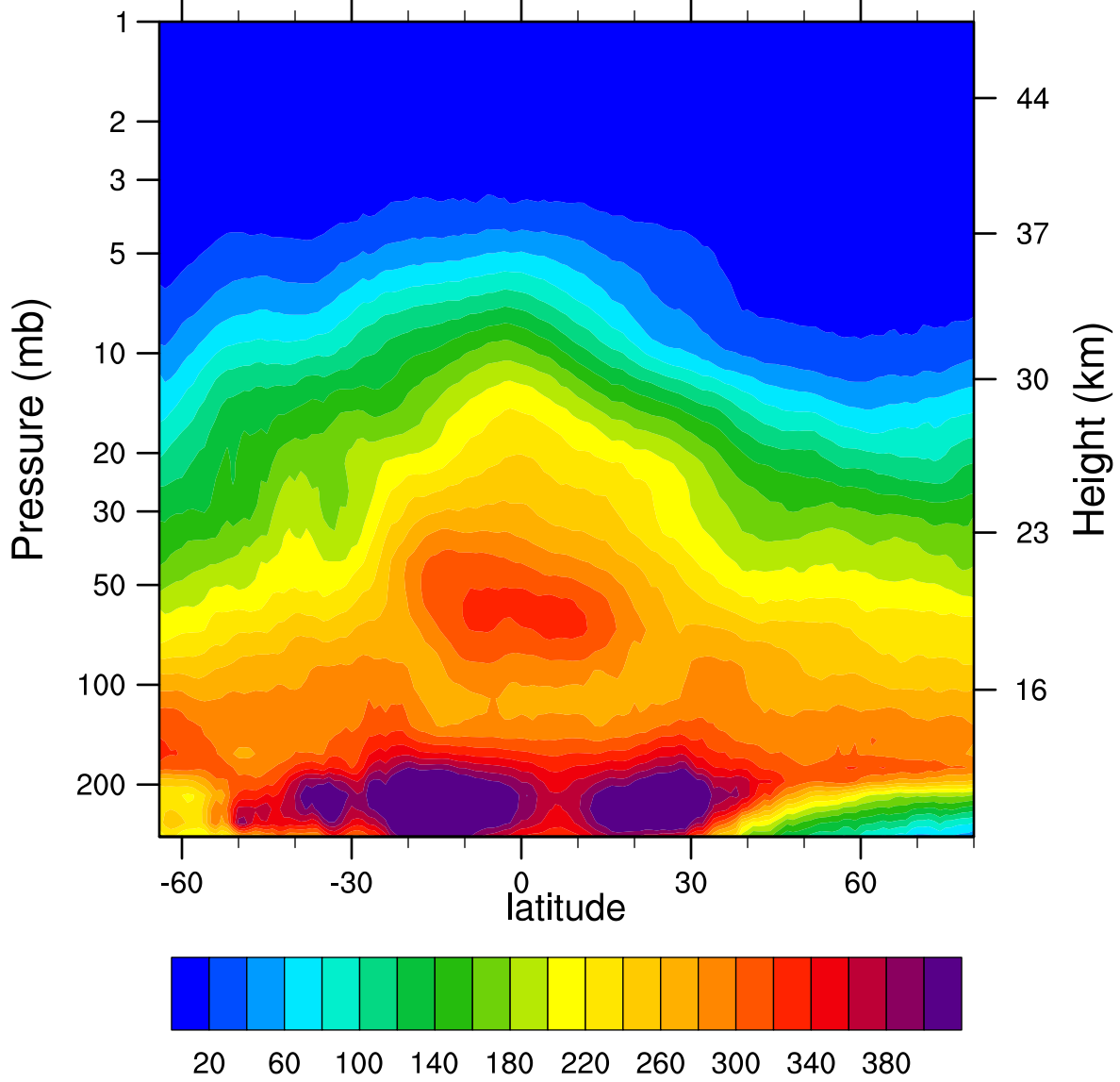
2006d138 N2O_Combined (ppbv)
