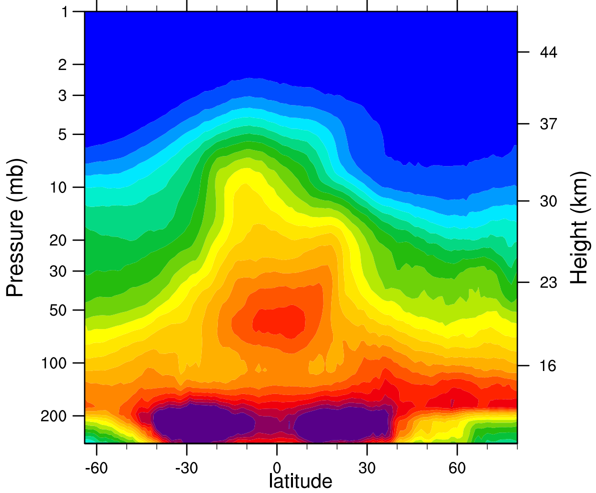
2006d039 N2O_Combined (ppbv)
