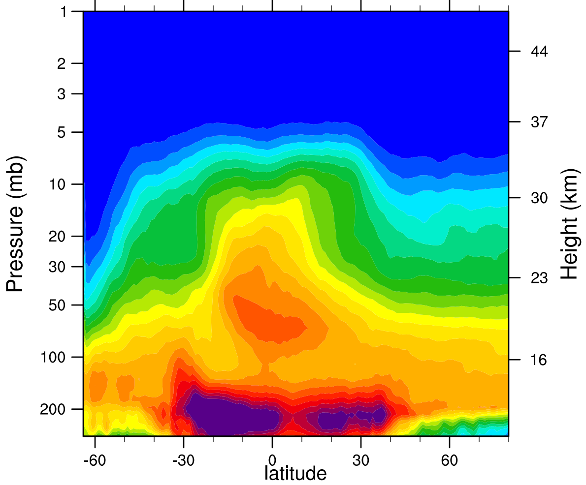
2007d181 N2O_Combined (ppbv)
