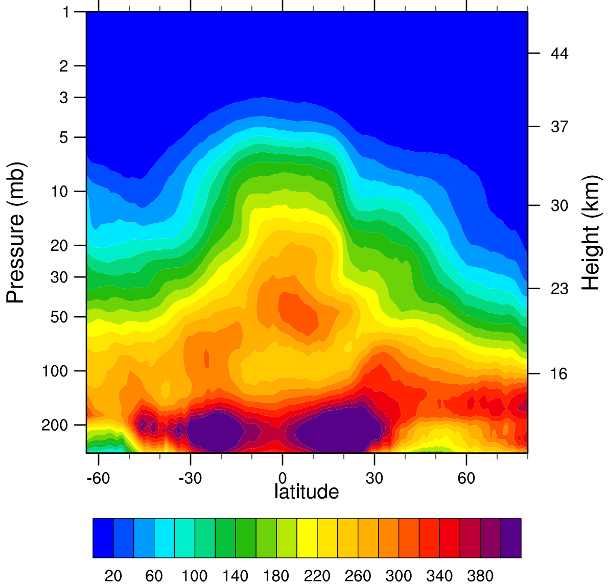
2005d051 N2O_Combined (ppbv)
