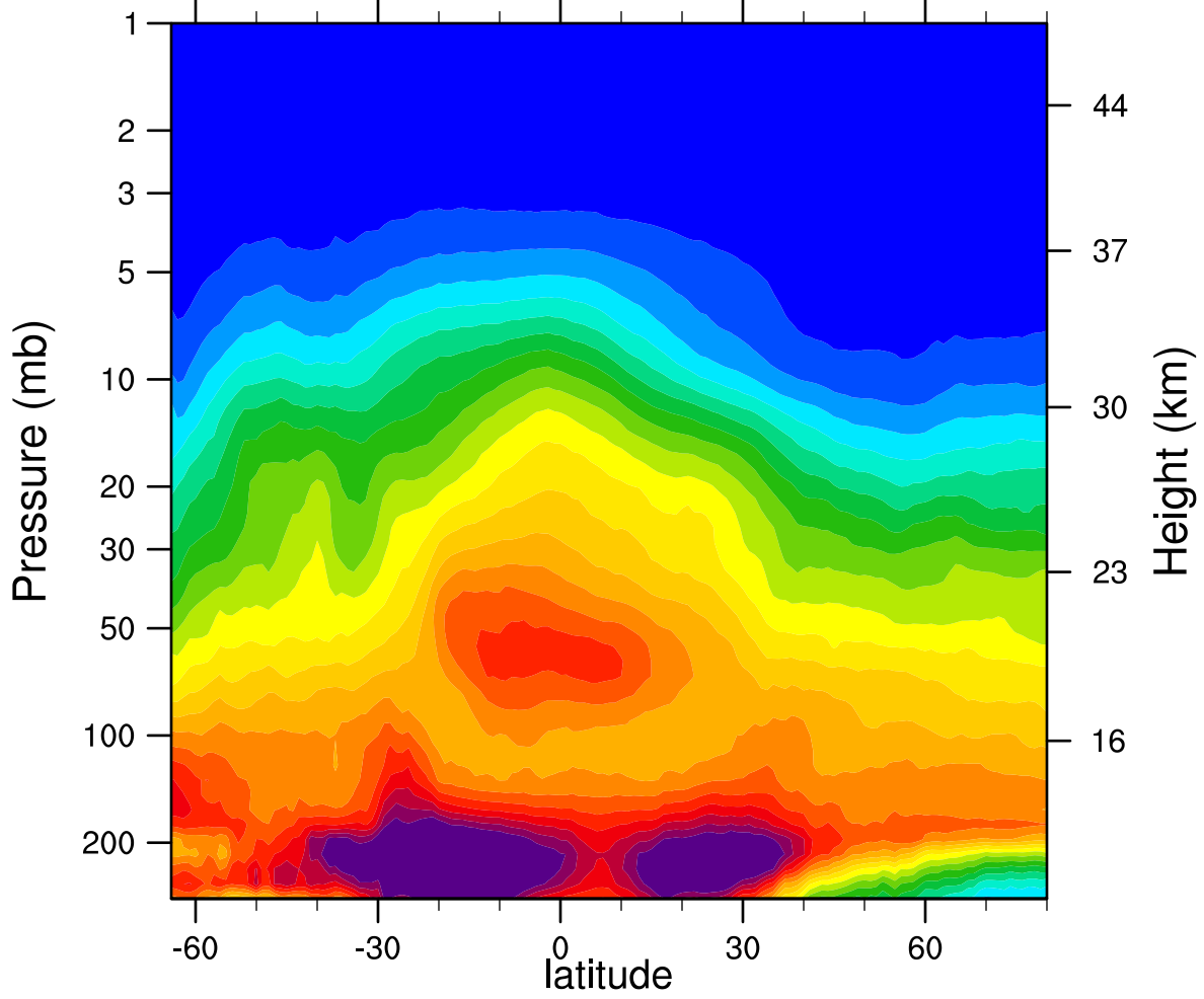
2006d146 N2O_Combined (ppbv)
