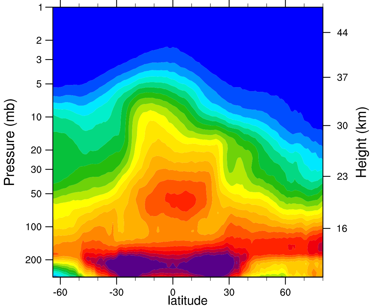
2006d001 N2O_Combined (ppbv)
