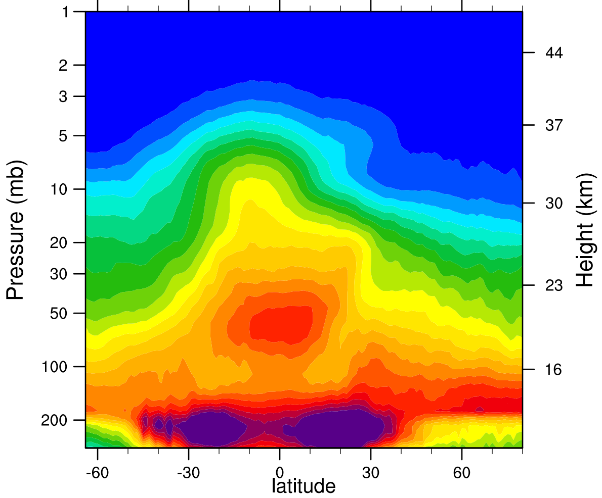
2006d059 N2O_Combined (ppbv)
