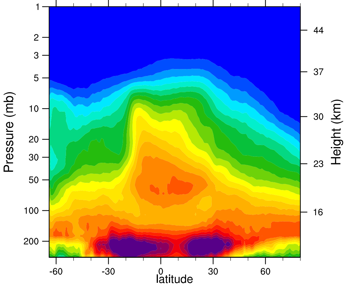
2005d287 N2O_Combined (ppbv)
