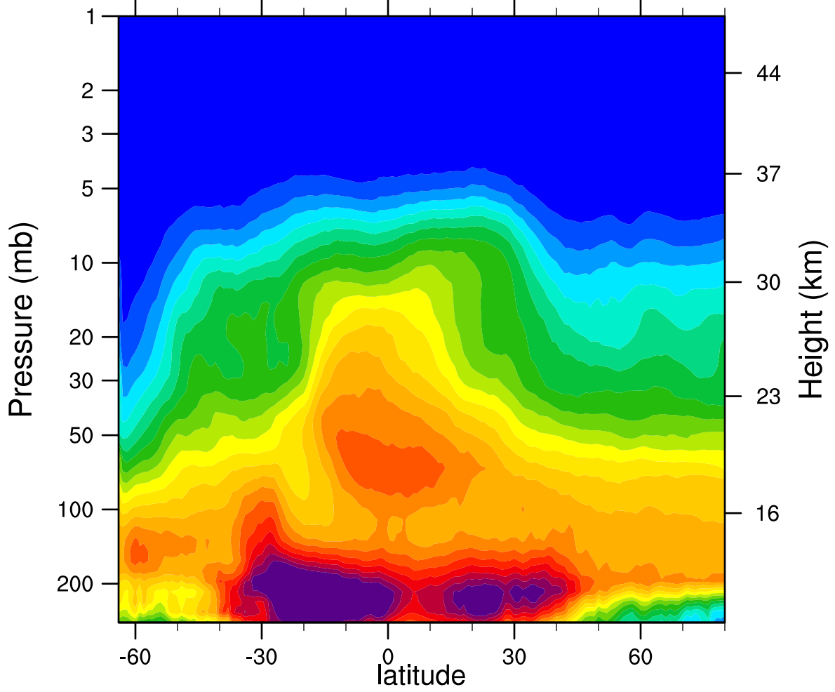
2007d188 N2O_Combined (ppbv)
