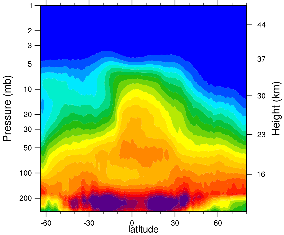
2006d309 N2O_Combined (ppbv)
