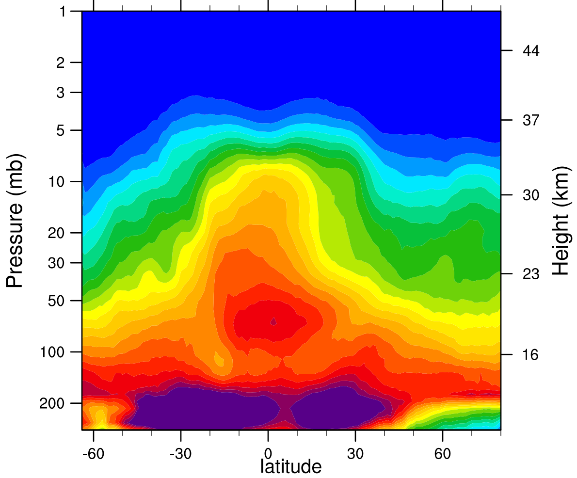
2007d129 N2O_Combined (ppbv)
