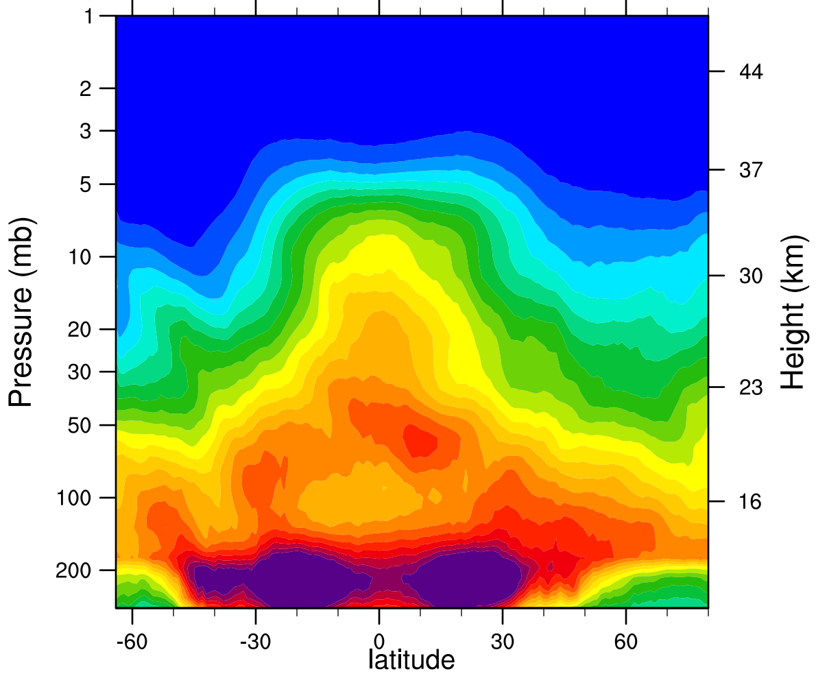
2005d099 N2O_Combined (ppbv)
