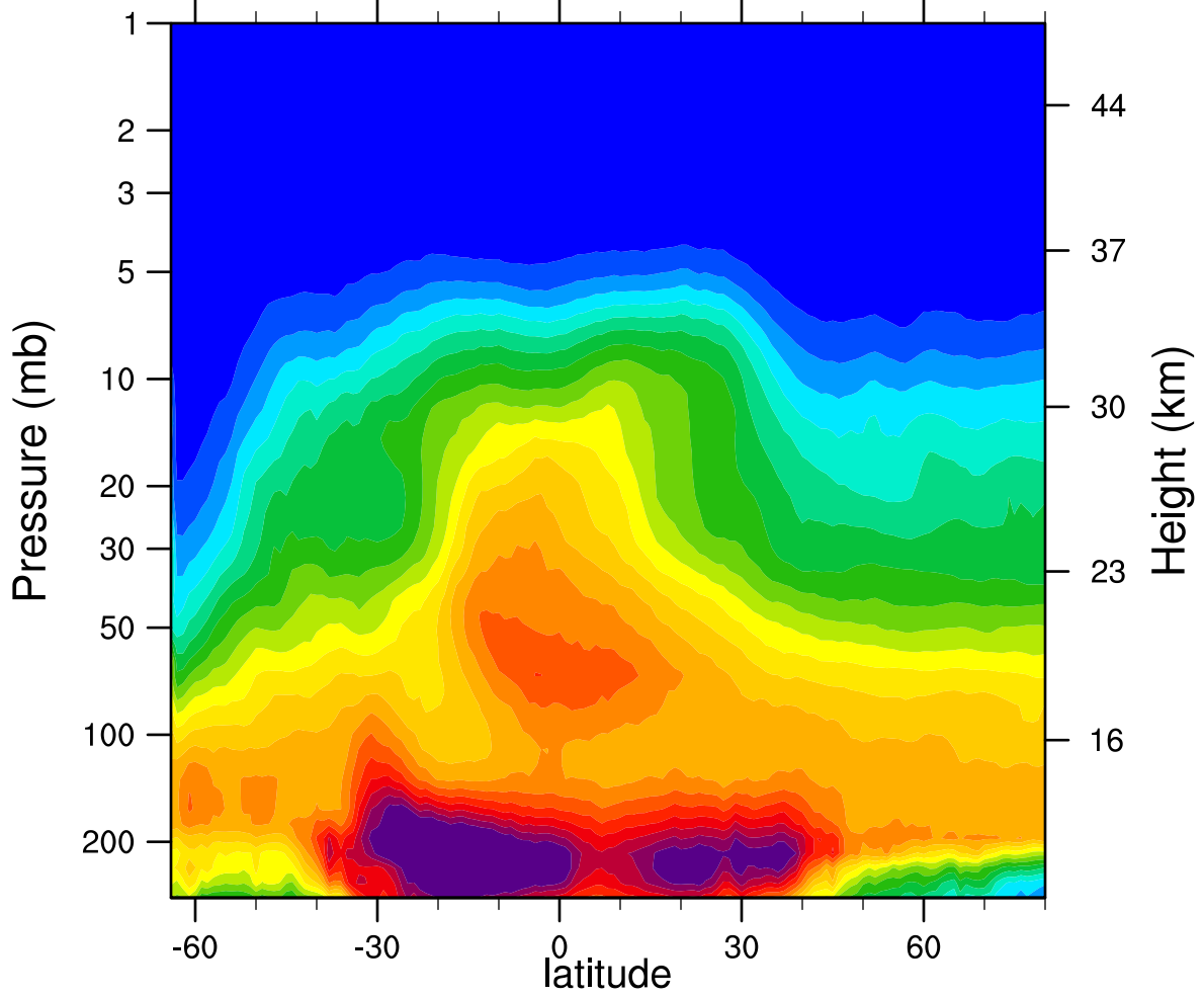
2007d183 N2O_Combined (ppbv)
