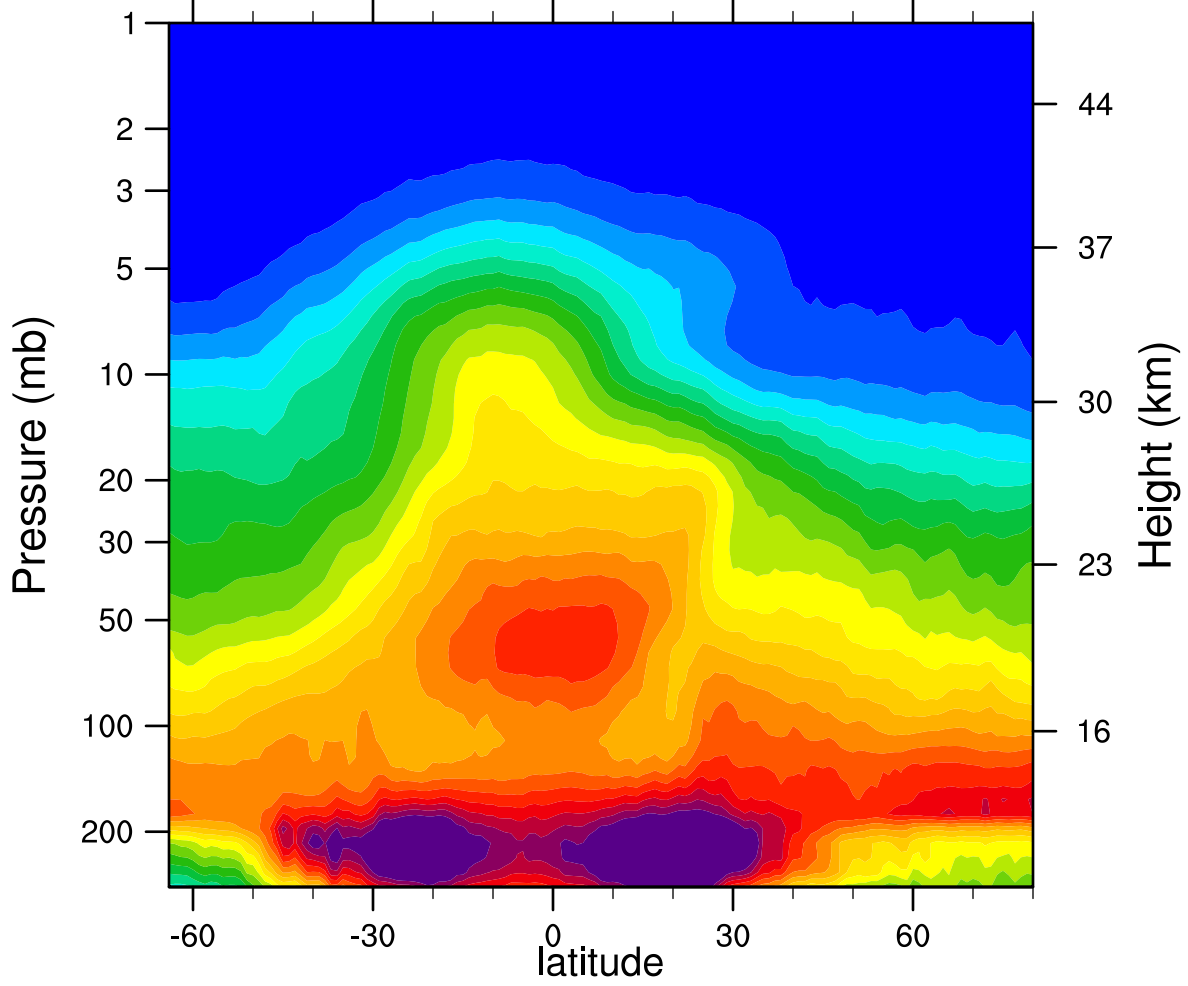
2006d058 N2O_Combined (ppbv)
