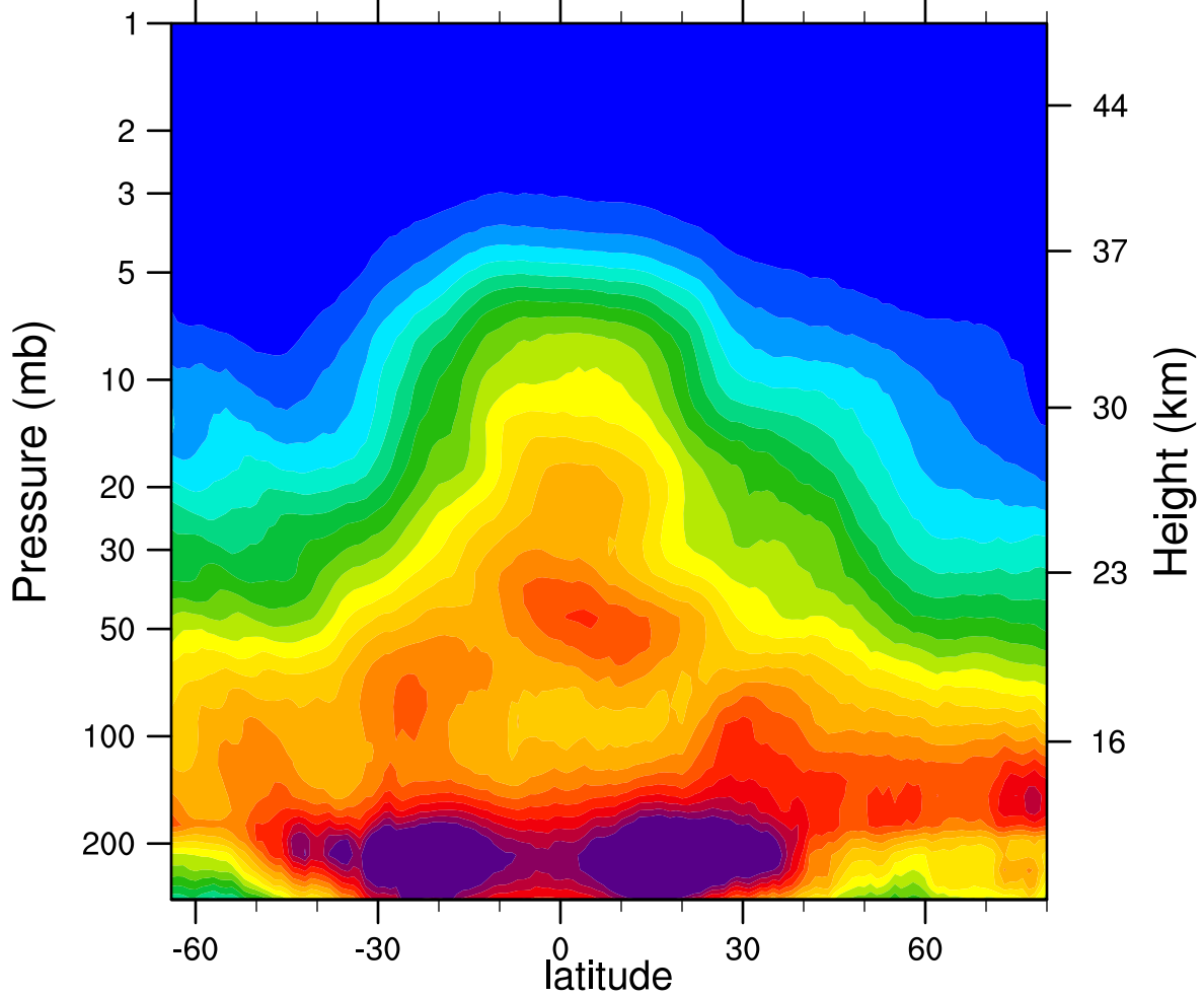
2005d070 N2O_Combined (ppbv)
