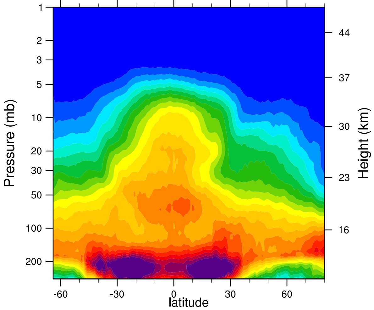
2007d075 N2O_Combined (ppbv)
