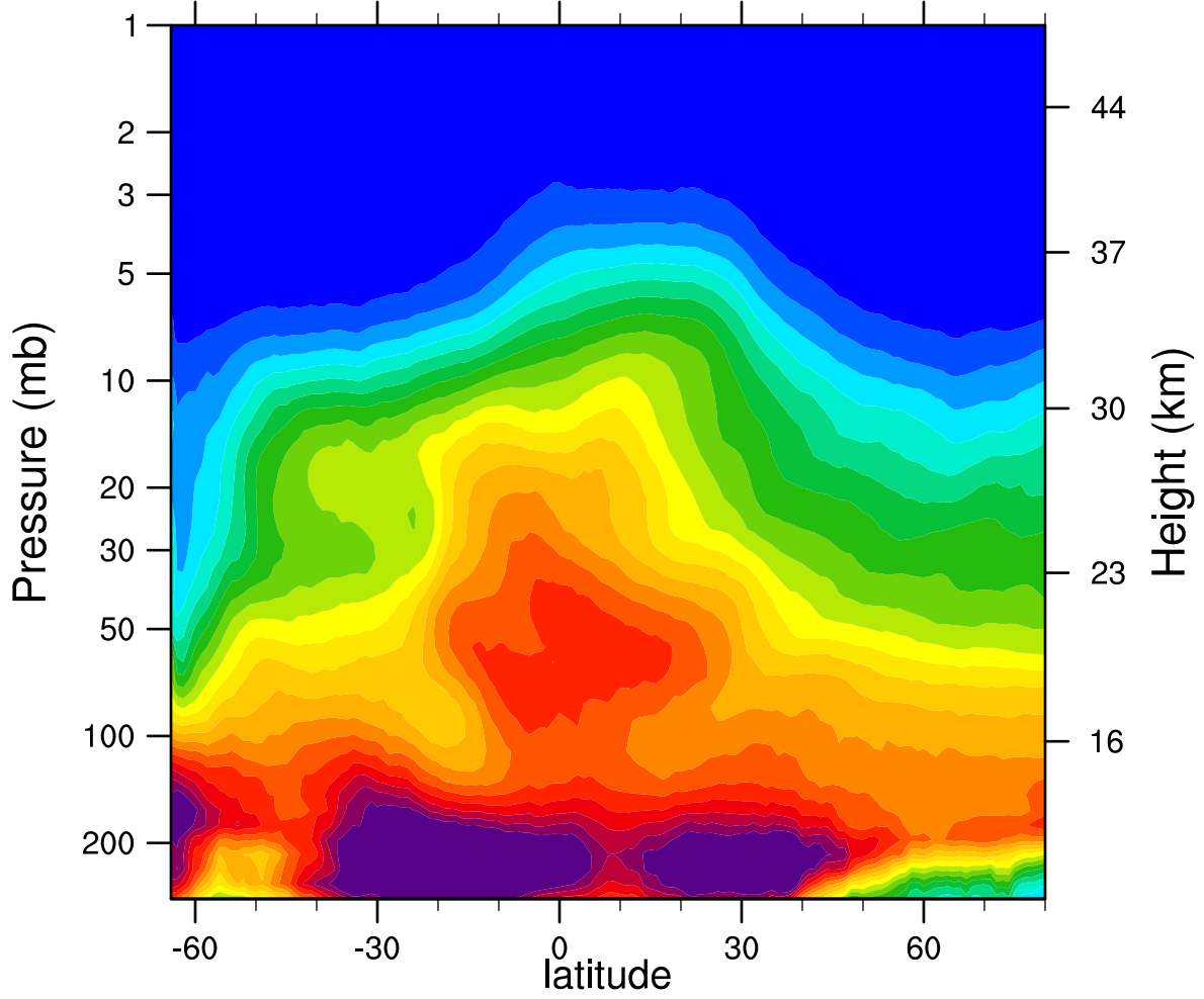
2007d237 N2O_Combined (ppbv)
