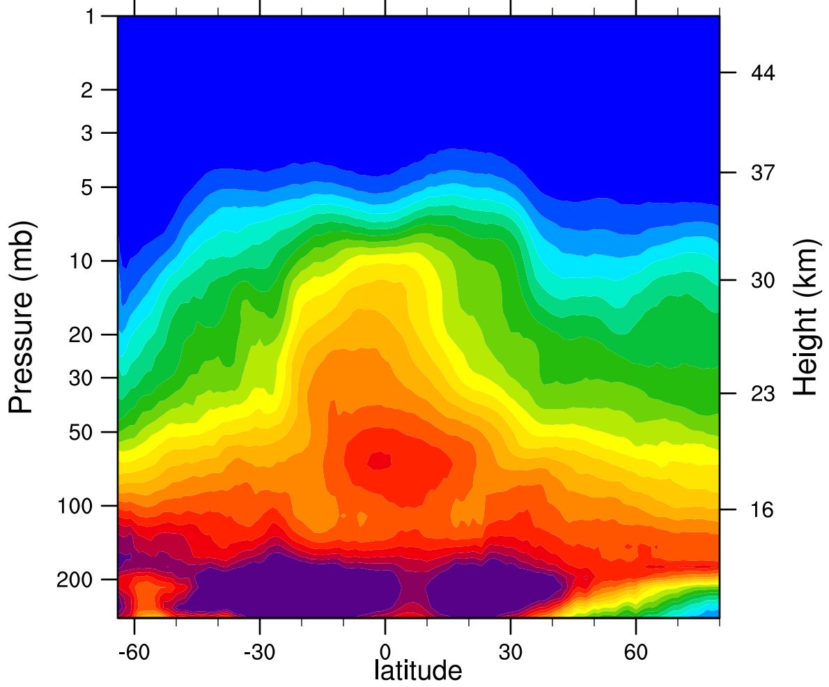
2007d144 N2O_Combined (ppbv)
