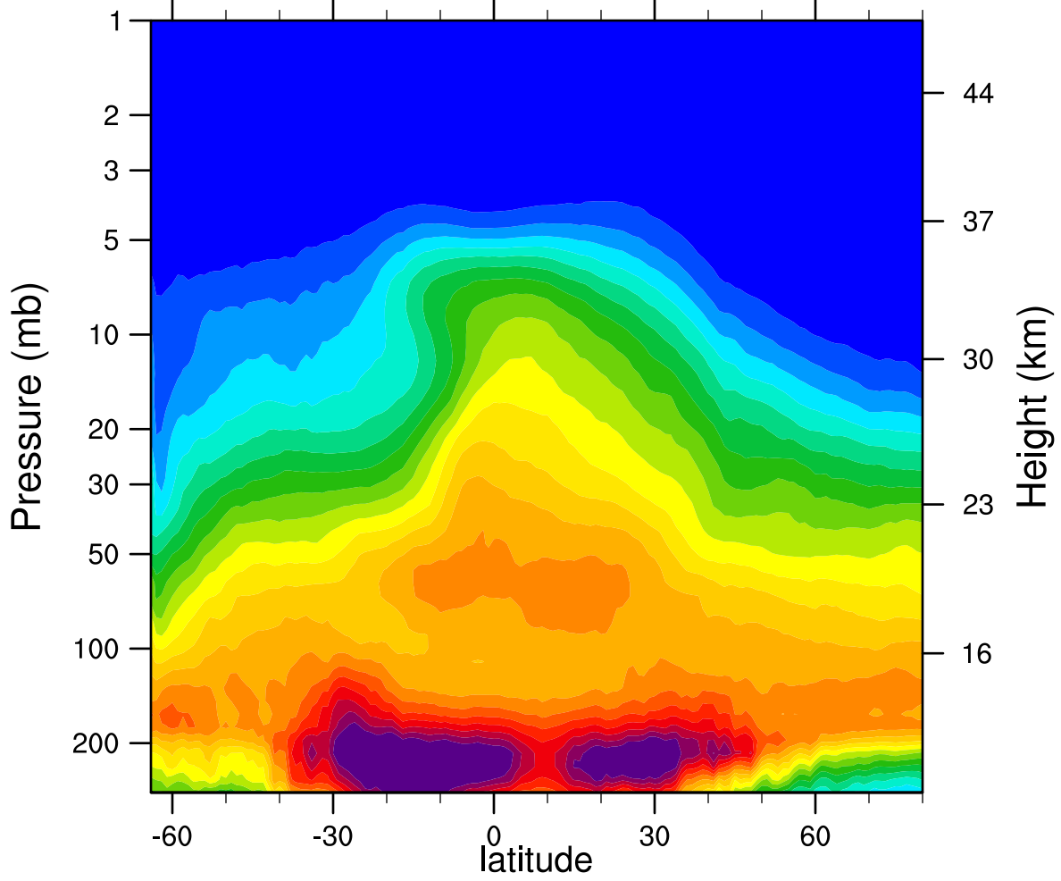
2006d271 N2O_Combined (ppbv)
