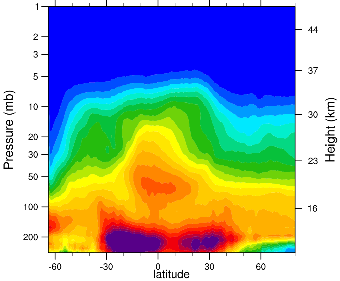
2007d196 N2O_Combined (ppbv)
