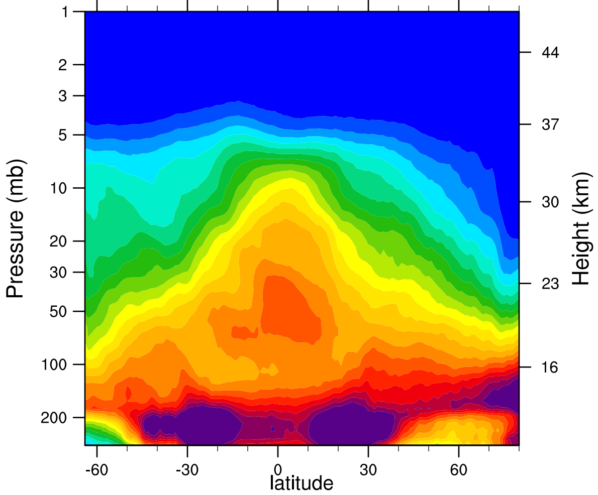
2006d349 N2O_Combined (ppbv)
