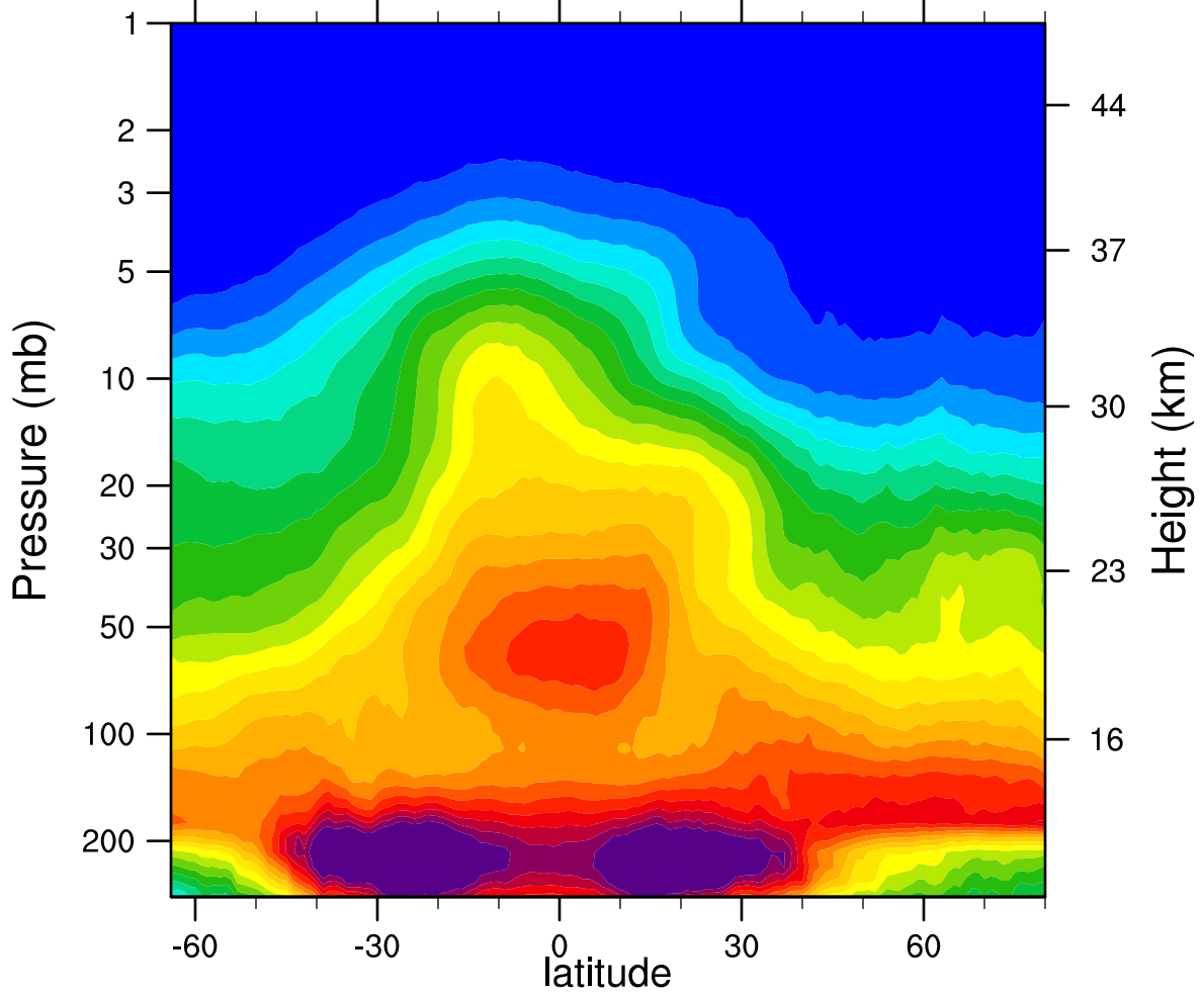
2006d045 N2O_Combined (ppbv)
