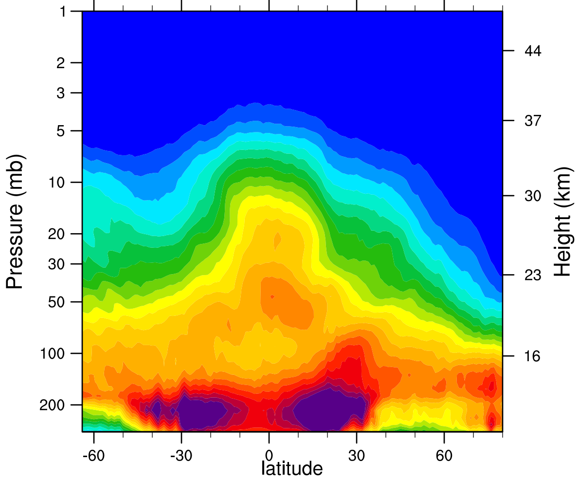
2005d030 N2O_Combined (ppbv)
