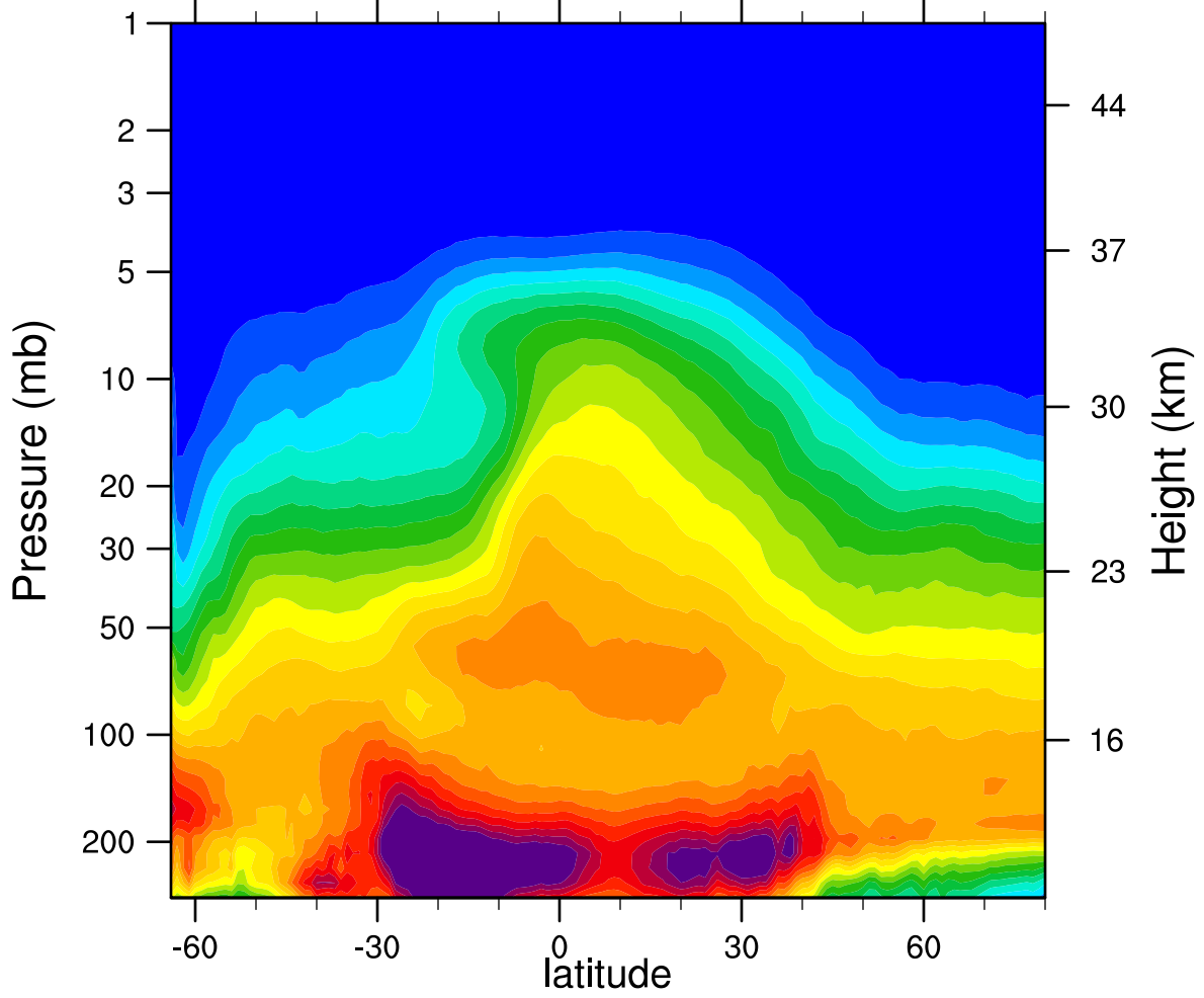
2006d256 N2O_Combined (ppbv)
