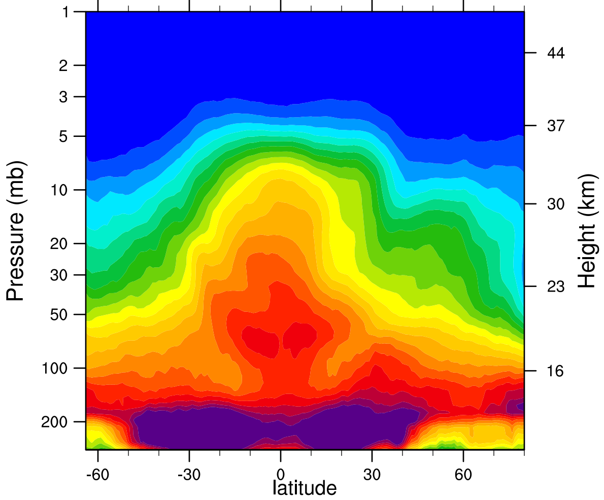
2007d098 N2O_Combined (ppbv)
