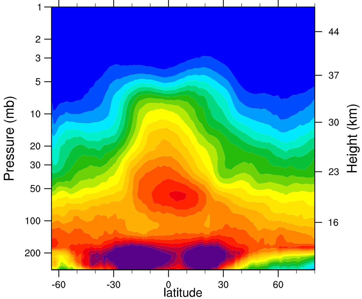
2005d124 N2O_Combined (ppbv)
