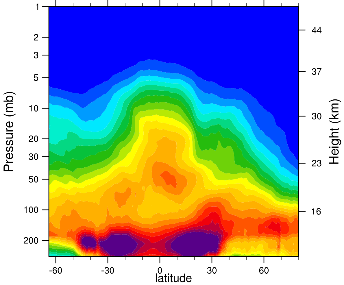
2005d039 N2O_Combined (ppbv)
