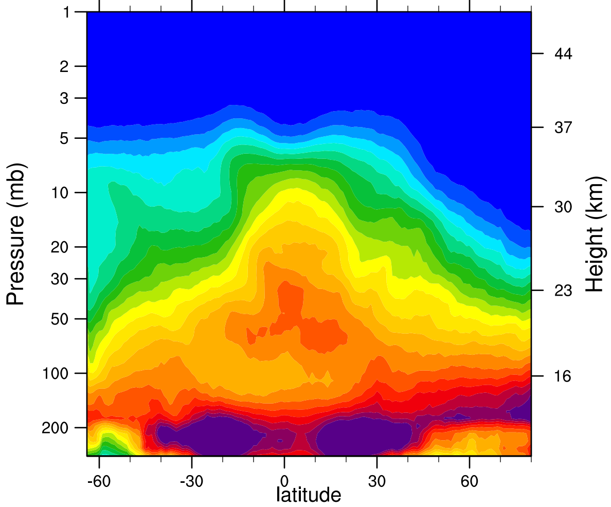
2006d330 N2O_Combined (ppbv)
