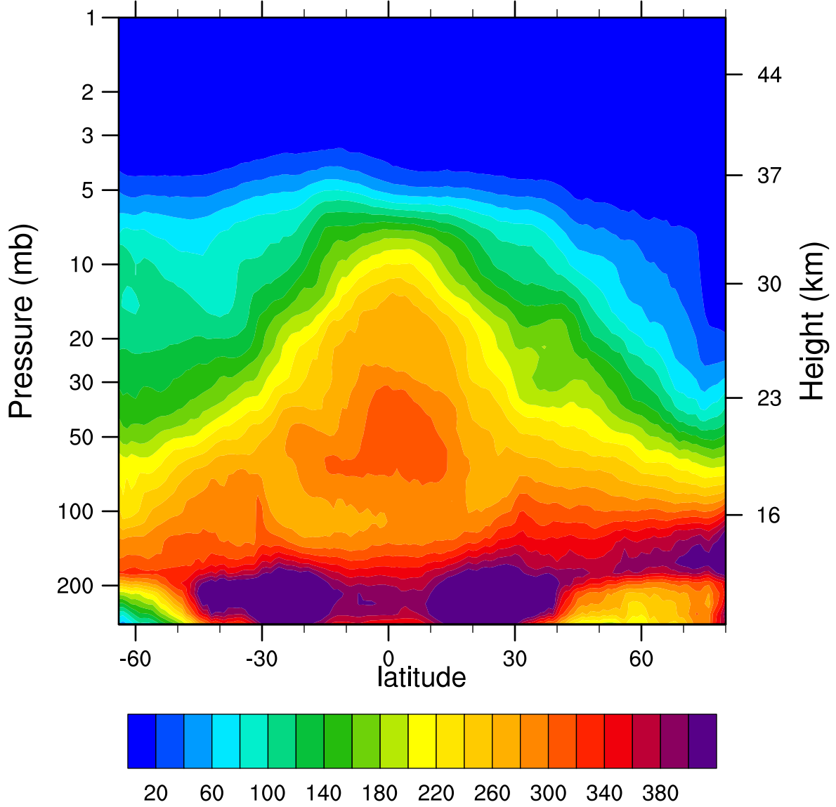
2006d353 N2O_Combined (ppbv)
