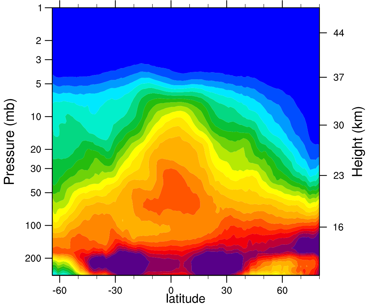
2006d346 N2O_Combined (ppbv)
