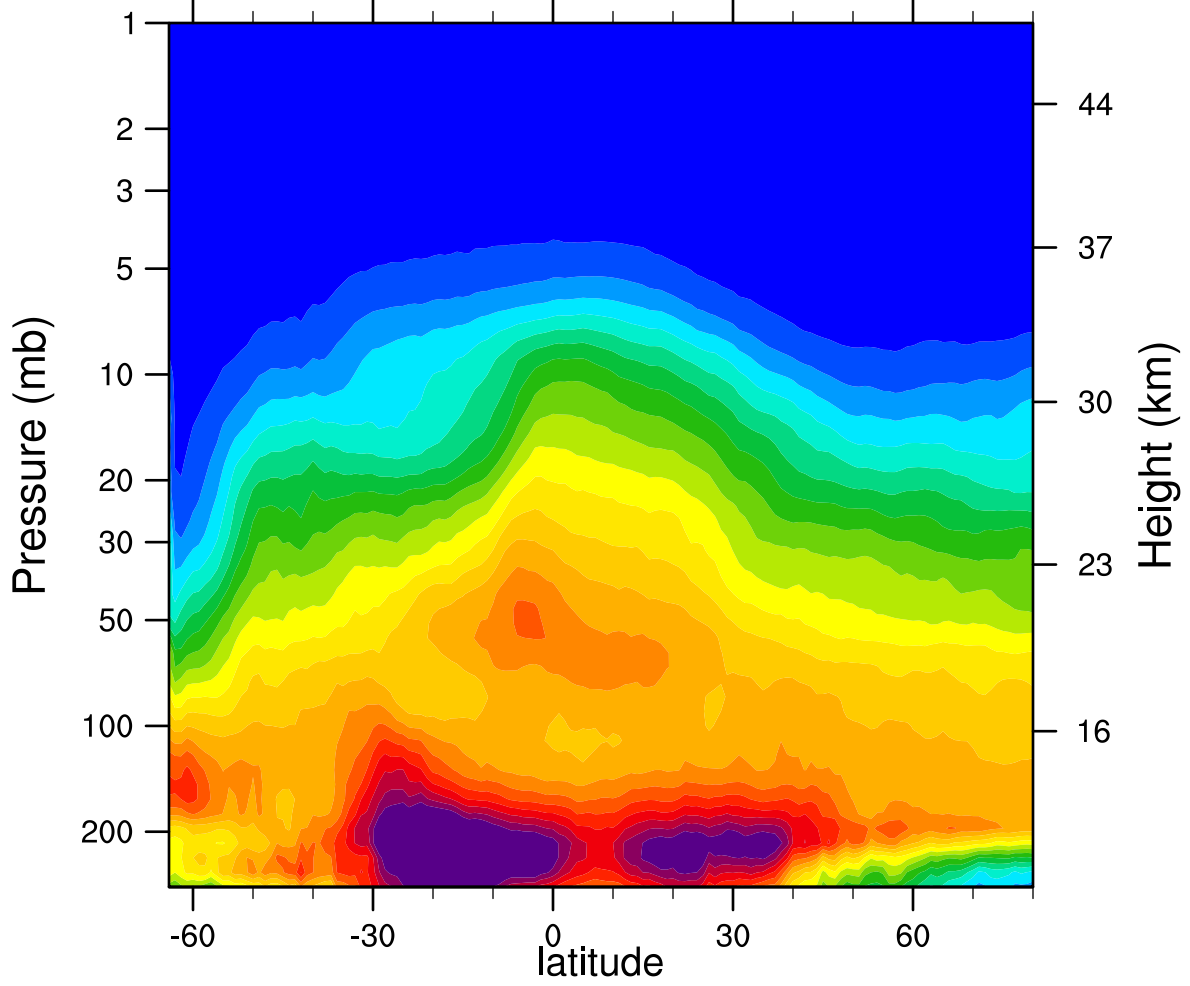
2006d194 N2O_Combined (ppbv)
