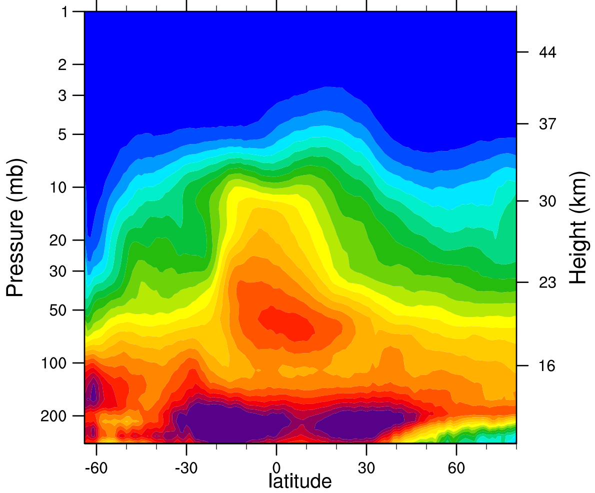
2005d183 N2O_Combined (ppbv)
