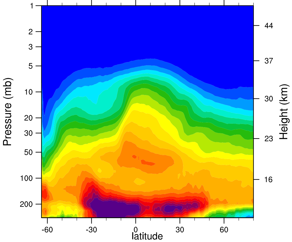
2006d223 N2O_Combined (ppbv)
