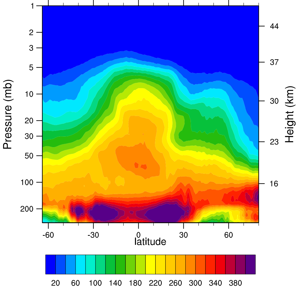
2007d036 N2O_Combined (ppbv)
