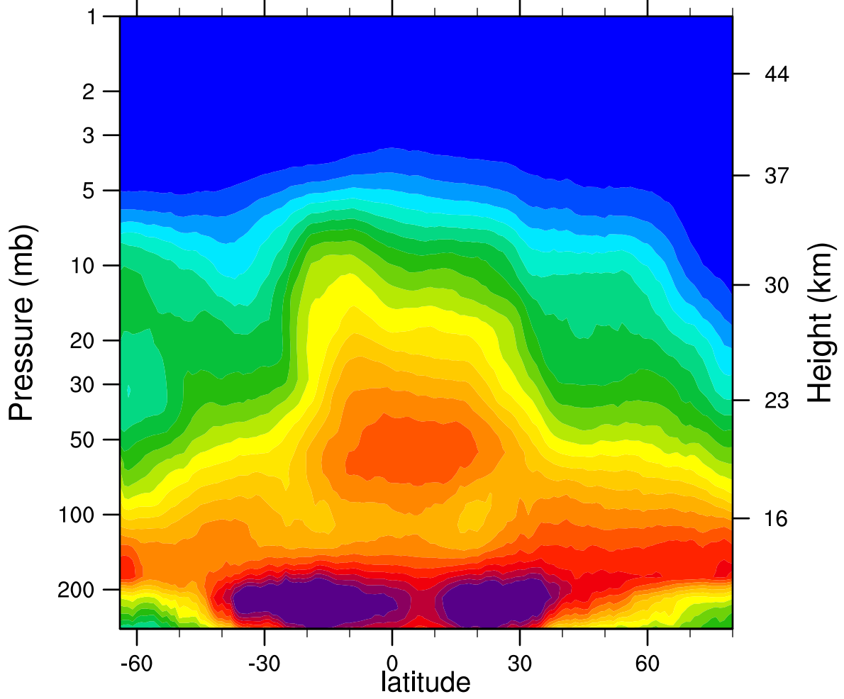
2005d317 N2O_Combined (ppbv)
