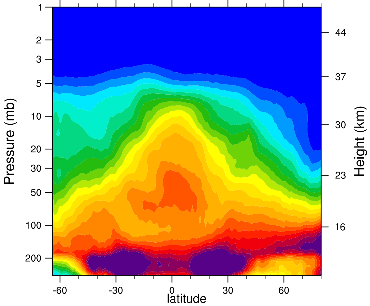
2006d351 N2O_Combined (ppbv)
