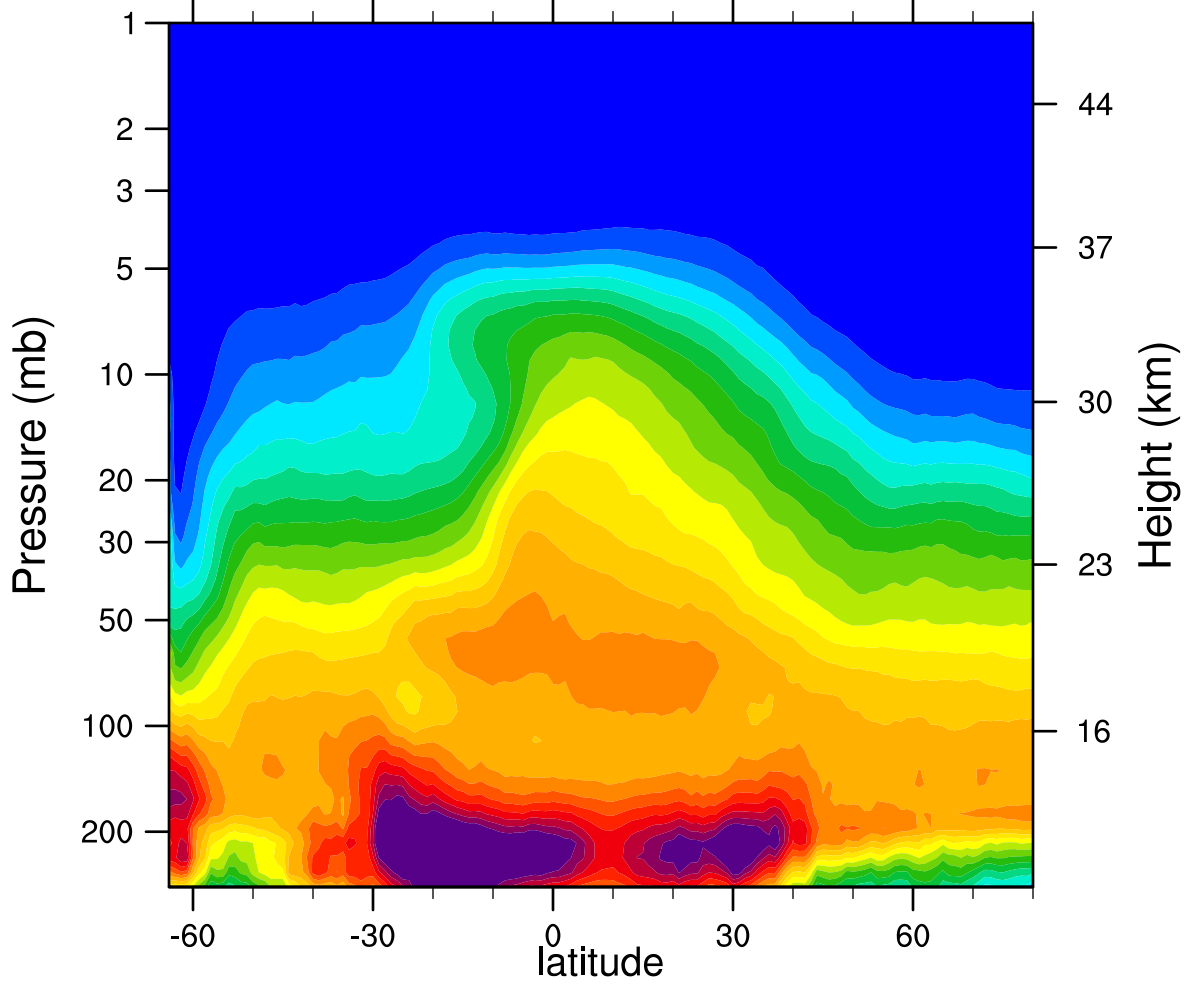
2006d258 N2O_Combined (ppbv)
