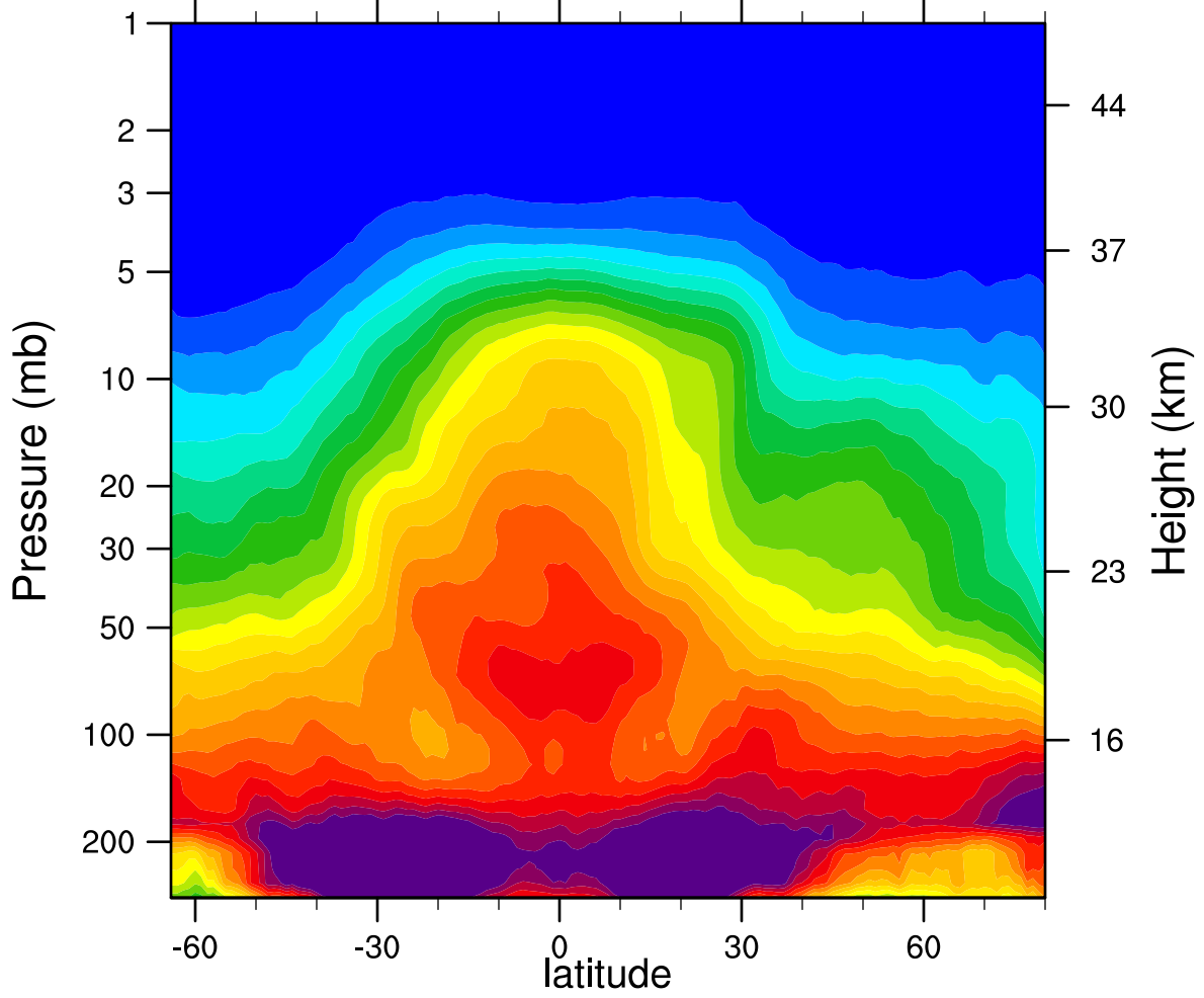
2007d090 N2O_Combined (ppbv)
