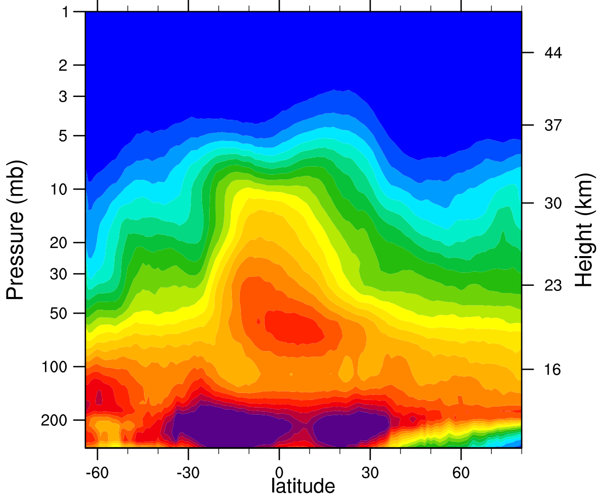
2005d161 N2O_Combined (ppbv)
