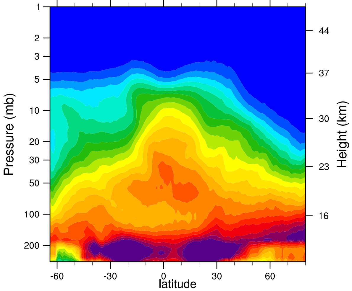
2006d328 N2O_Combined (ppbv)
