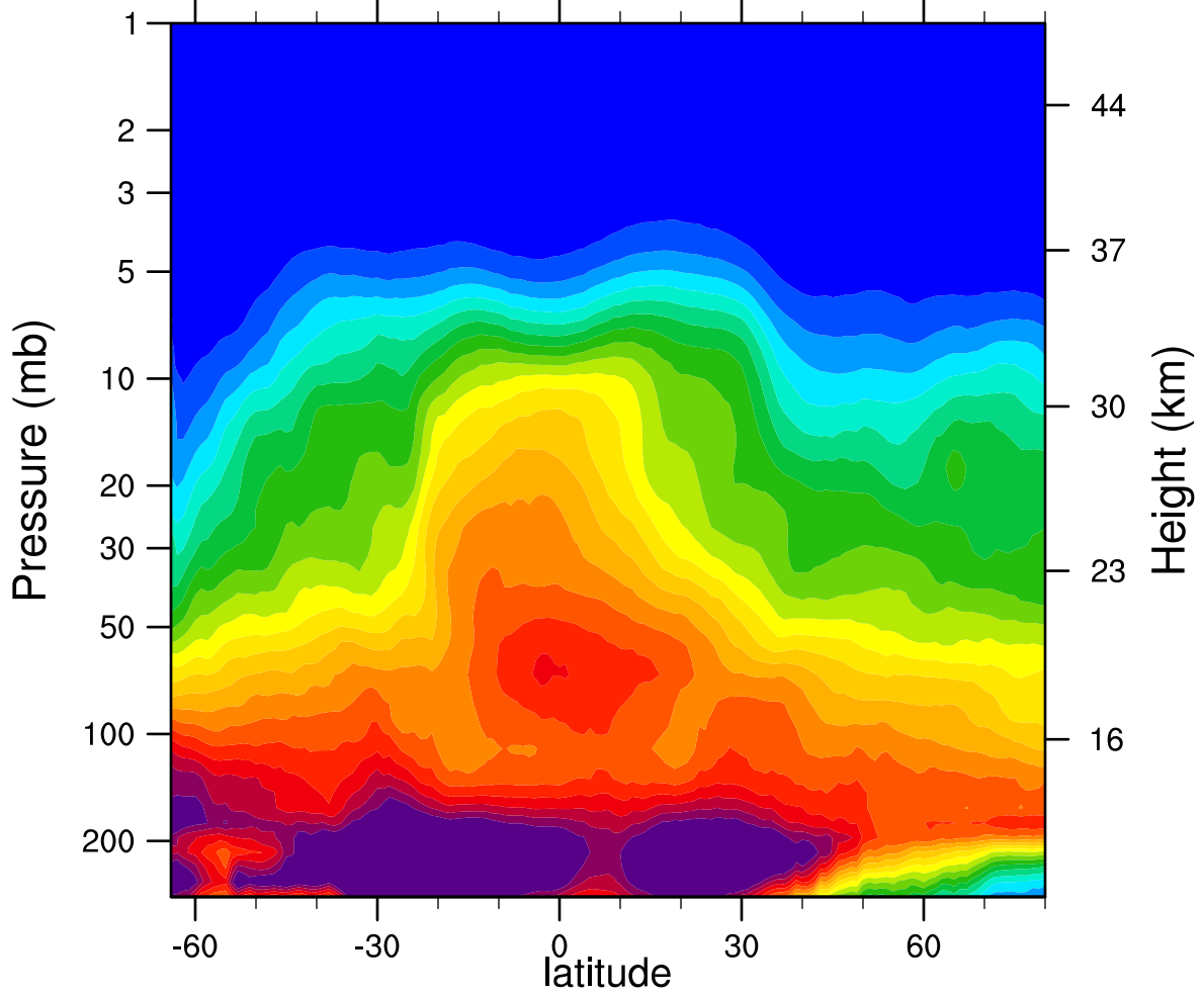
2007d150 N2O_Combined (ppbv)
