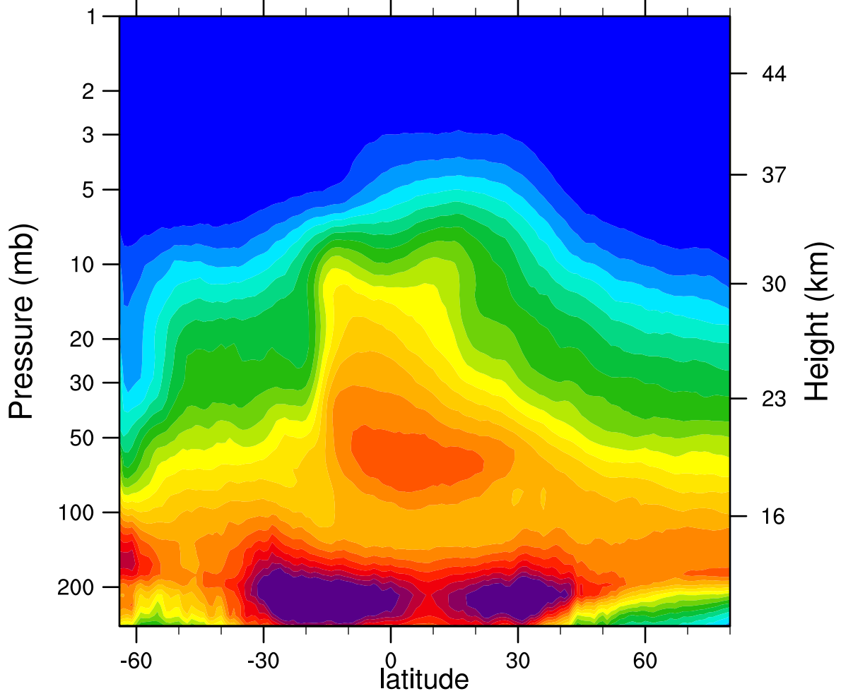
2005d257 N2O_Combined (ppbv)
