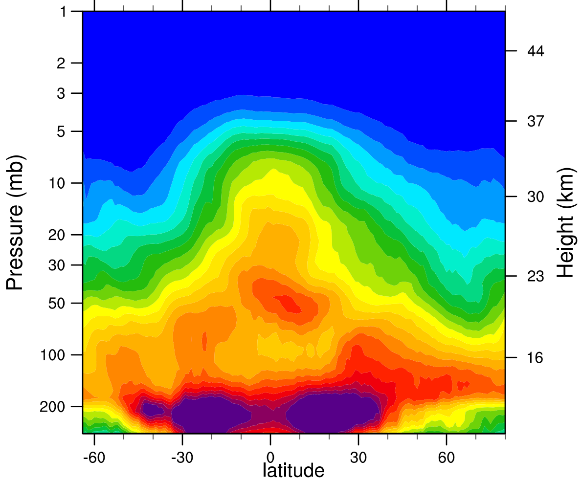
2005d077 N2O_Combined (ppbv)
