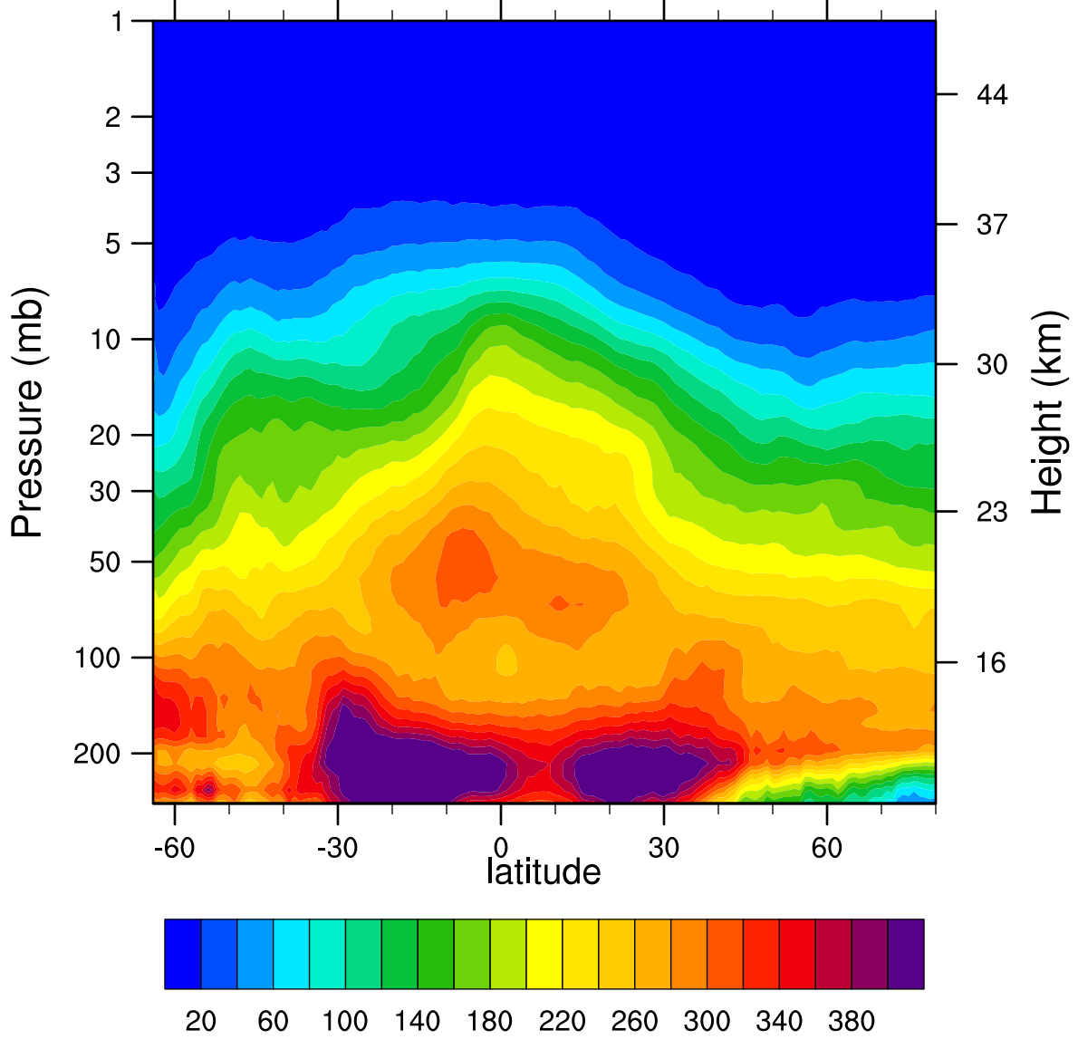
2006d171 N2O_Combined (ppbv)
