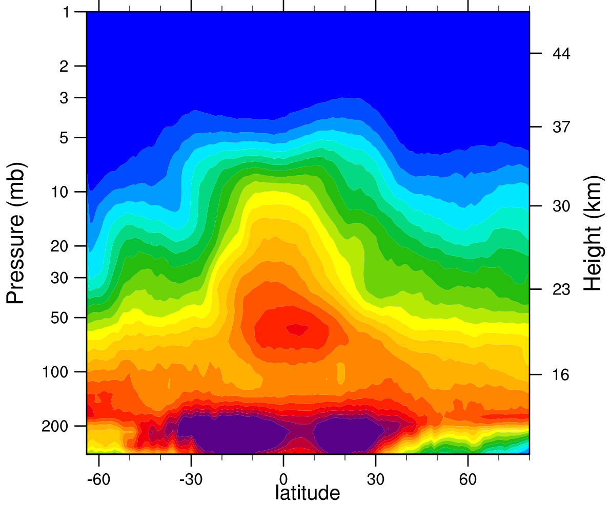
2005d141 N2O_Combined (ppbv)
