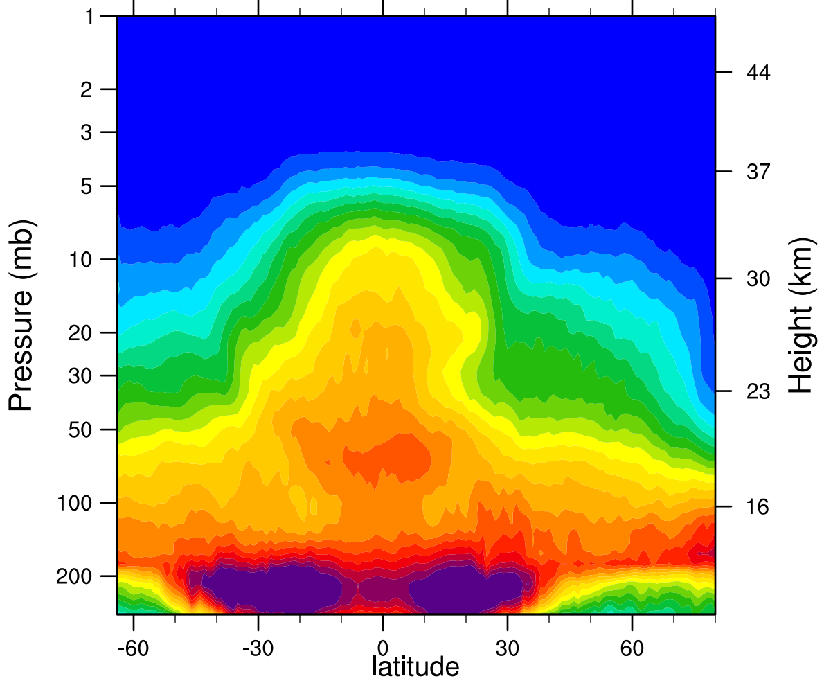
2007d077 N2O_Combined (ppbv)
