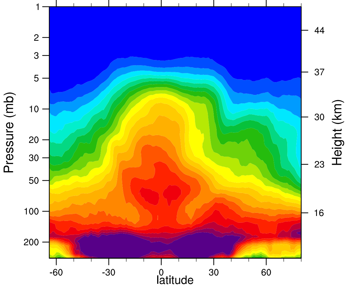
2007d099 N2O_Combined (ppbv)
