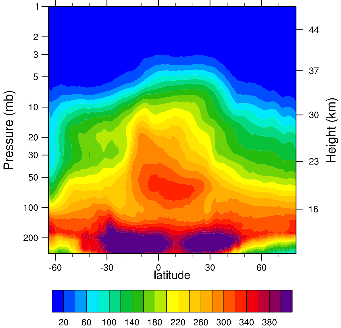
2007d269 N2O_Combined (ppbv)
