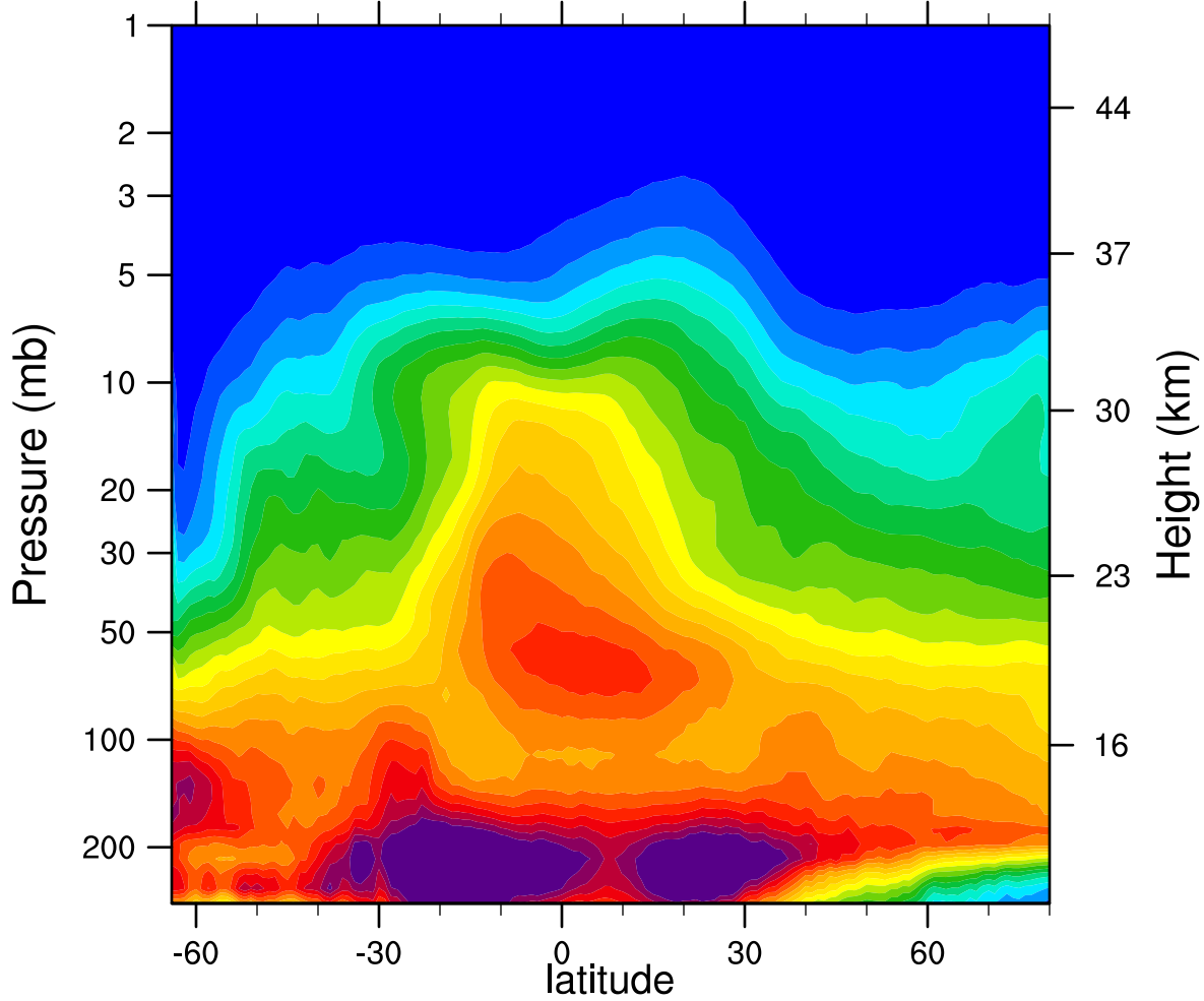
2005d171 N2O_Combined (ppbv)
