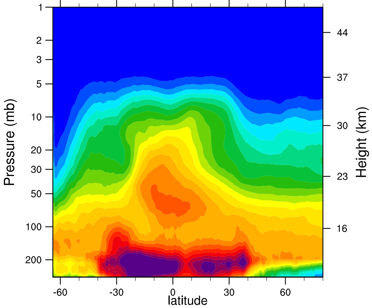
2007d174 N2O_Combined (ppbv)
