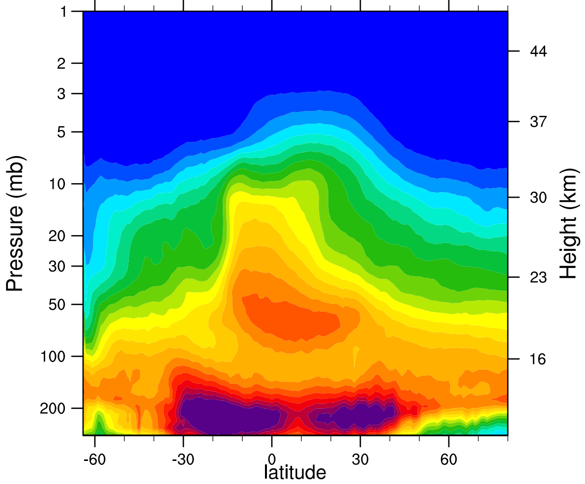
2005d244 N2O_Combined (ppbv)
