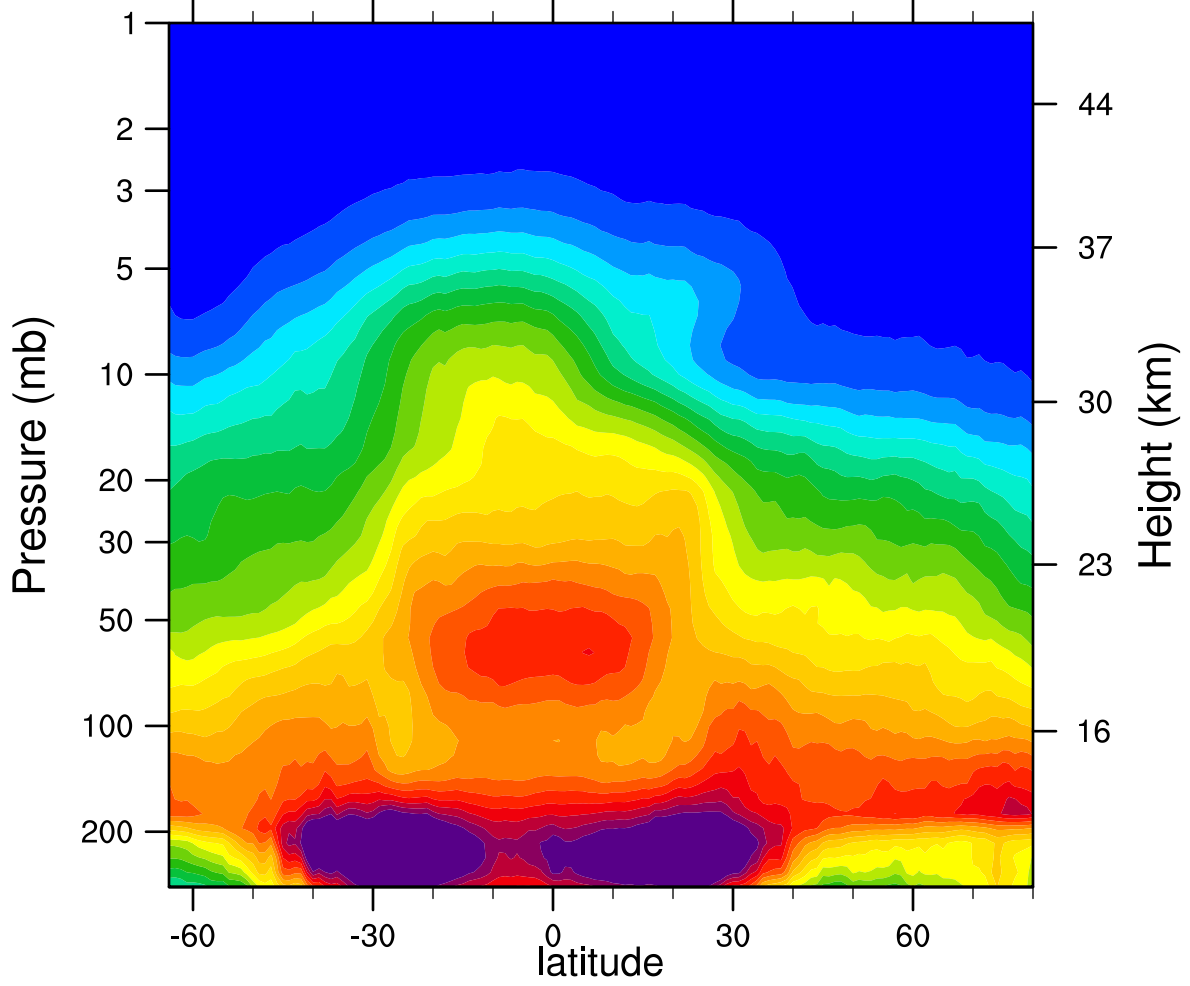
2006d075 N2O_Combined (ppbv)
