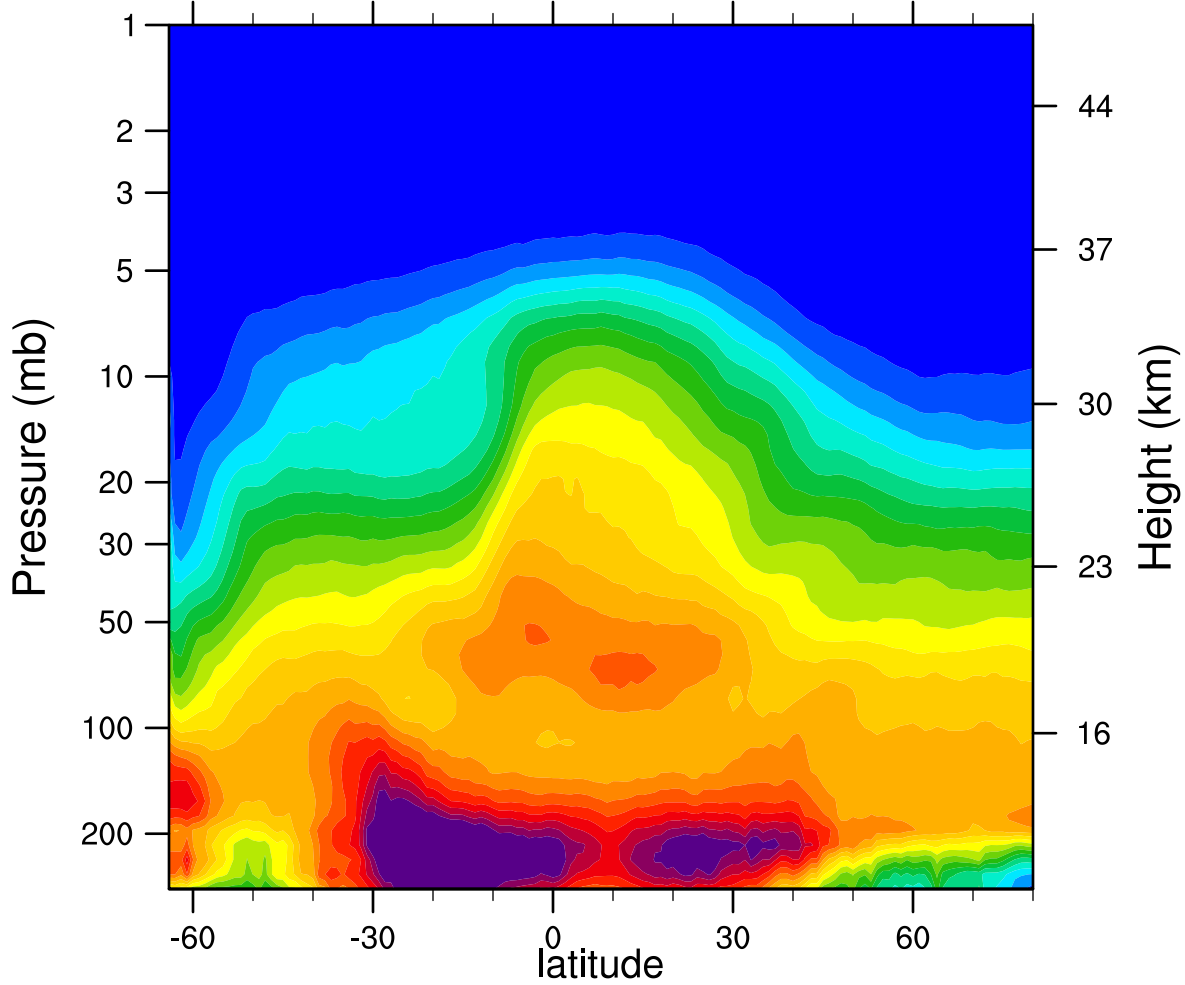
2006d237 N2O_Combined (ppbv)
