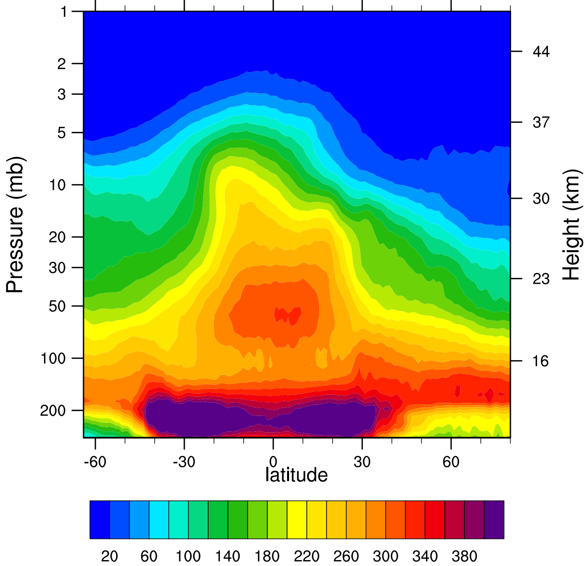
2006d021 N2O_Combined (ppbv)
