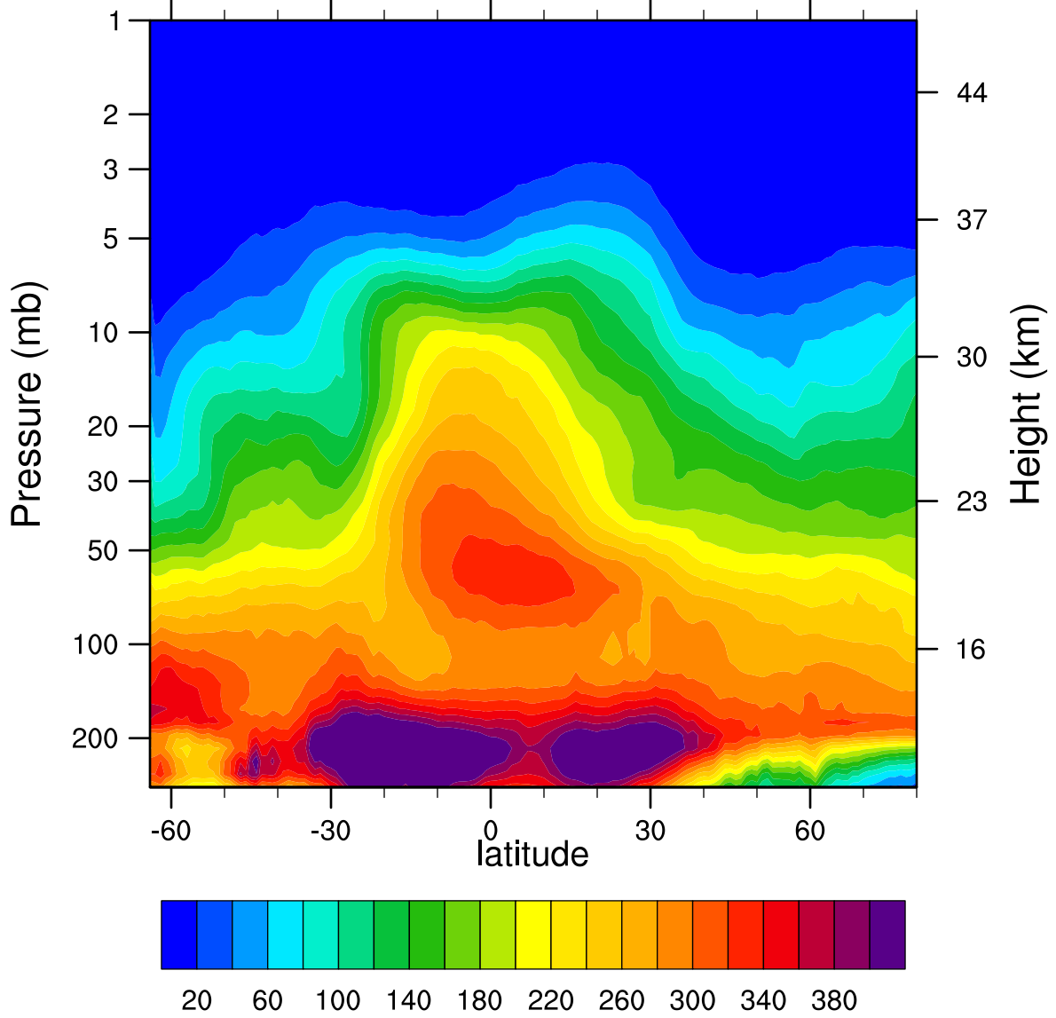
2005d156 N2O_Combined (ppbv)
