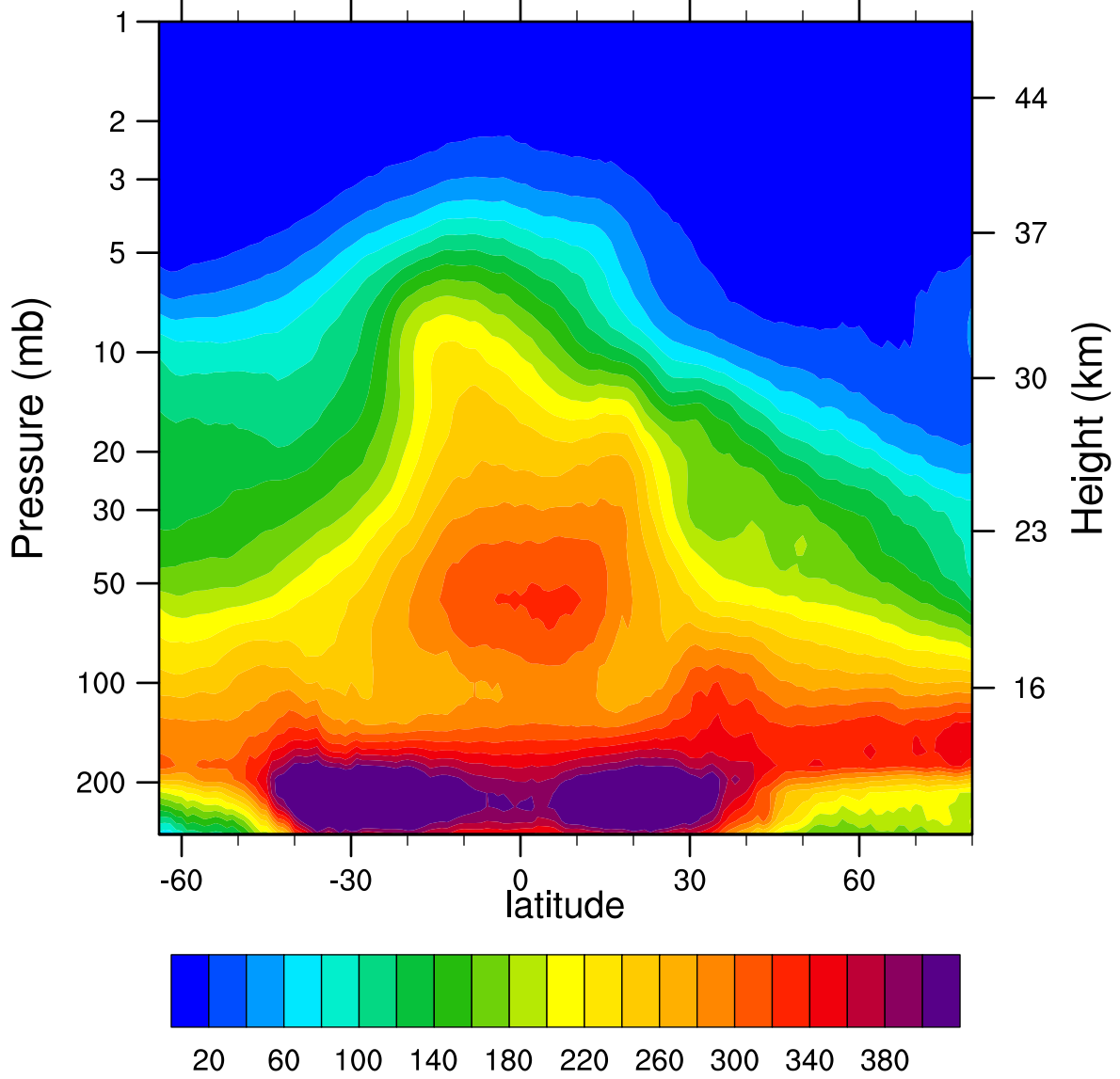
2006d024 N2O_Combined (ppbv)
