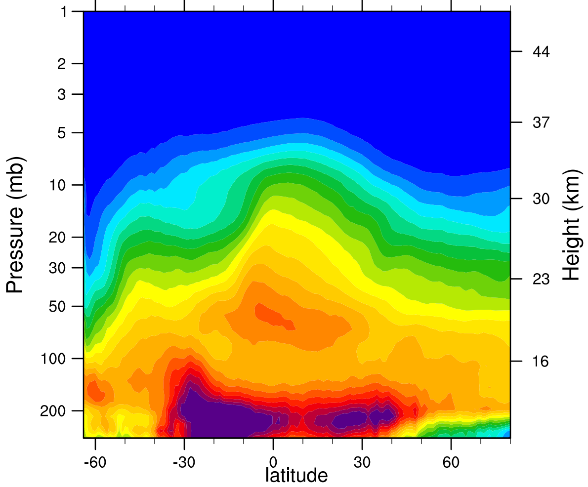
2006d213 N2O_Combined (ppbv)
