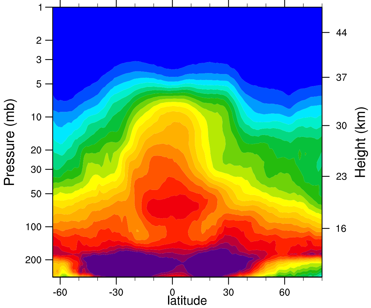
2007d112 N2O_Combined (ppbv)
