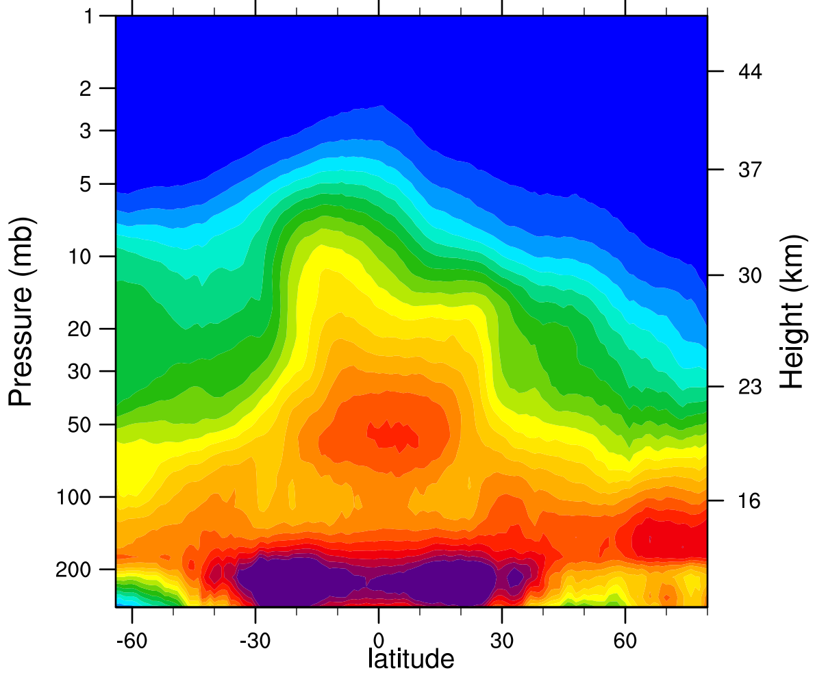
2005d357 N2O_Combined (ppbv)
