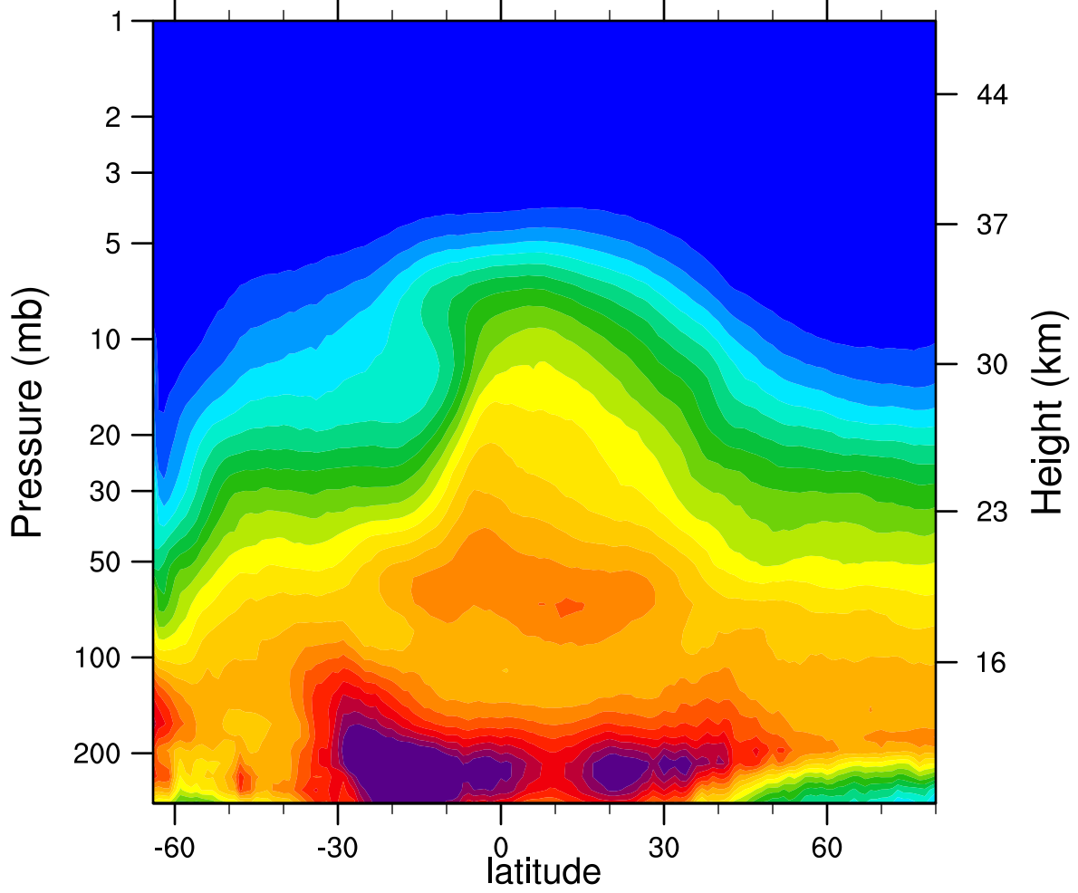
2006d249 N2O_Combined (ppbv)
