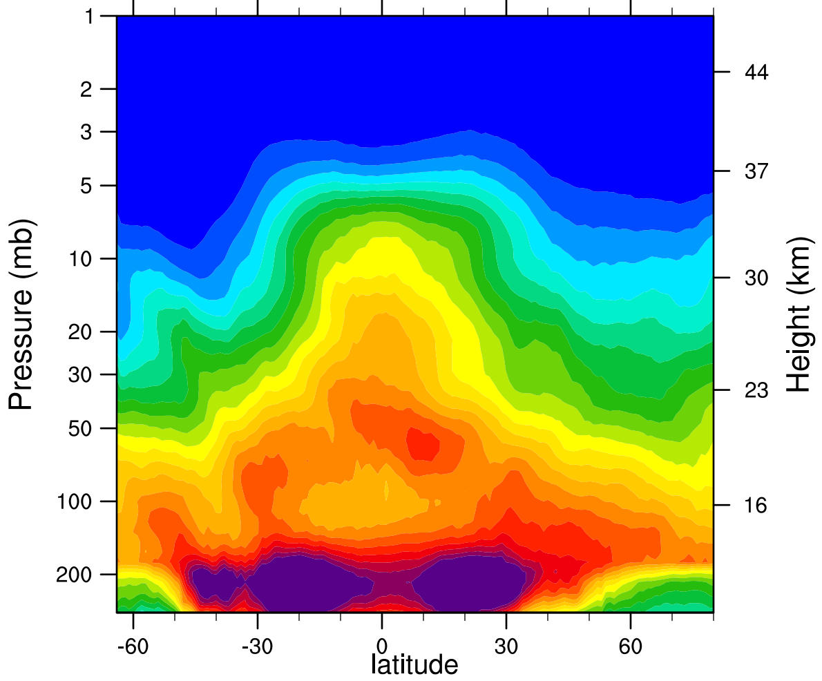
2005d100 N2O_Combined (ppbv)
