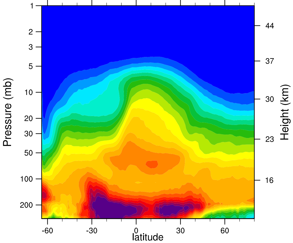
2006d242 N2O_Combined (ppbv)
