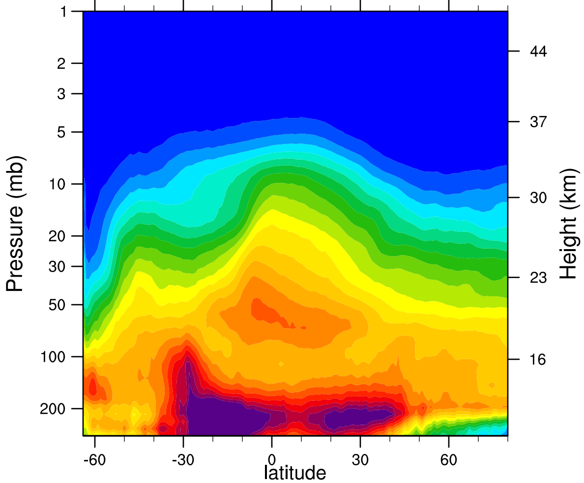
2006d208 N2O_Combined (ppbv)
