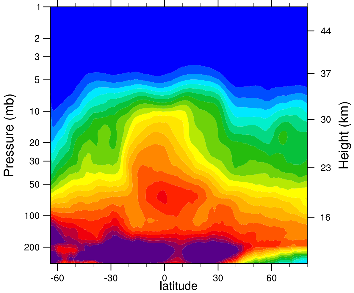
2007d154 N2O_Combined (ppbv)
