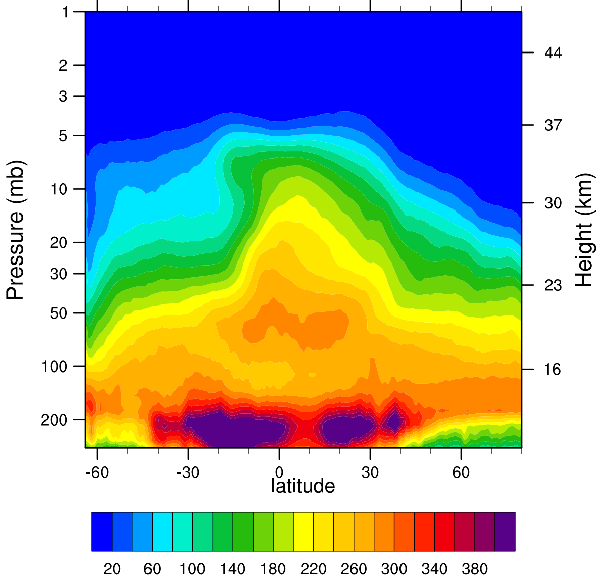
2006d284 N2O_Combined (ppbv)
