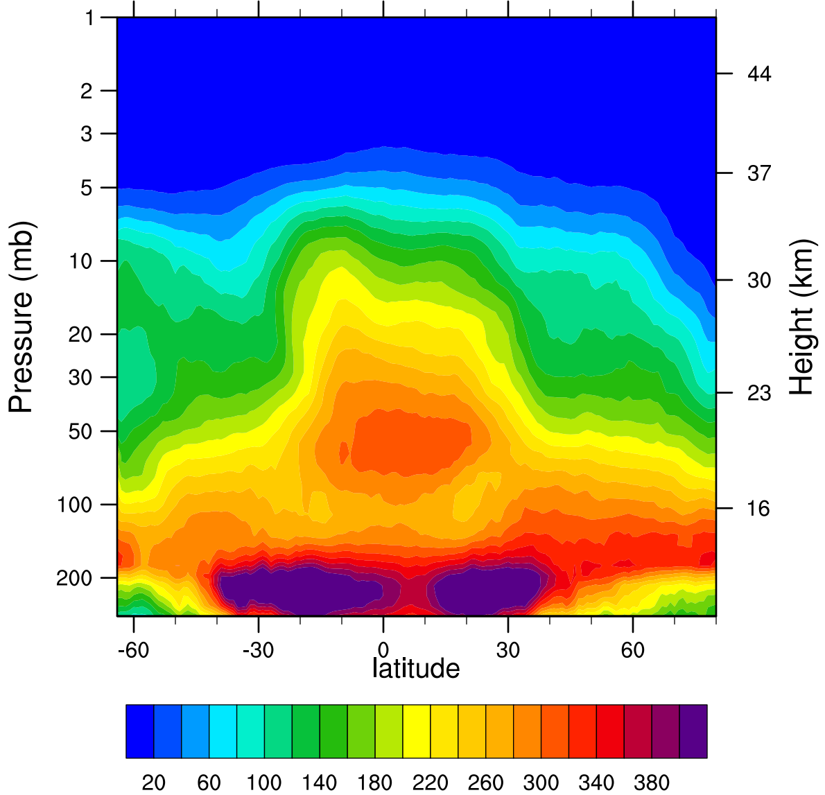
2005d315 N2O_Combined (ppbv)
