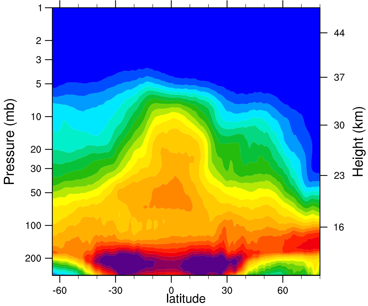
2007d008 N2O_Combined (ppbv)
