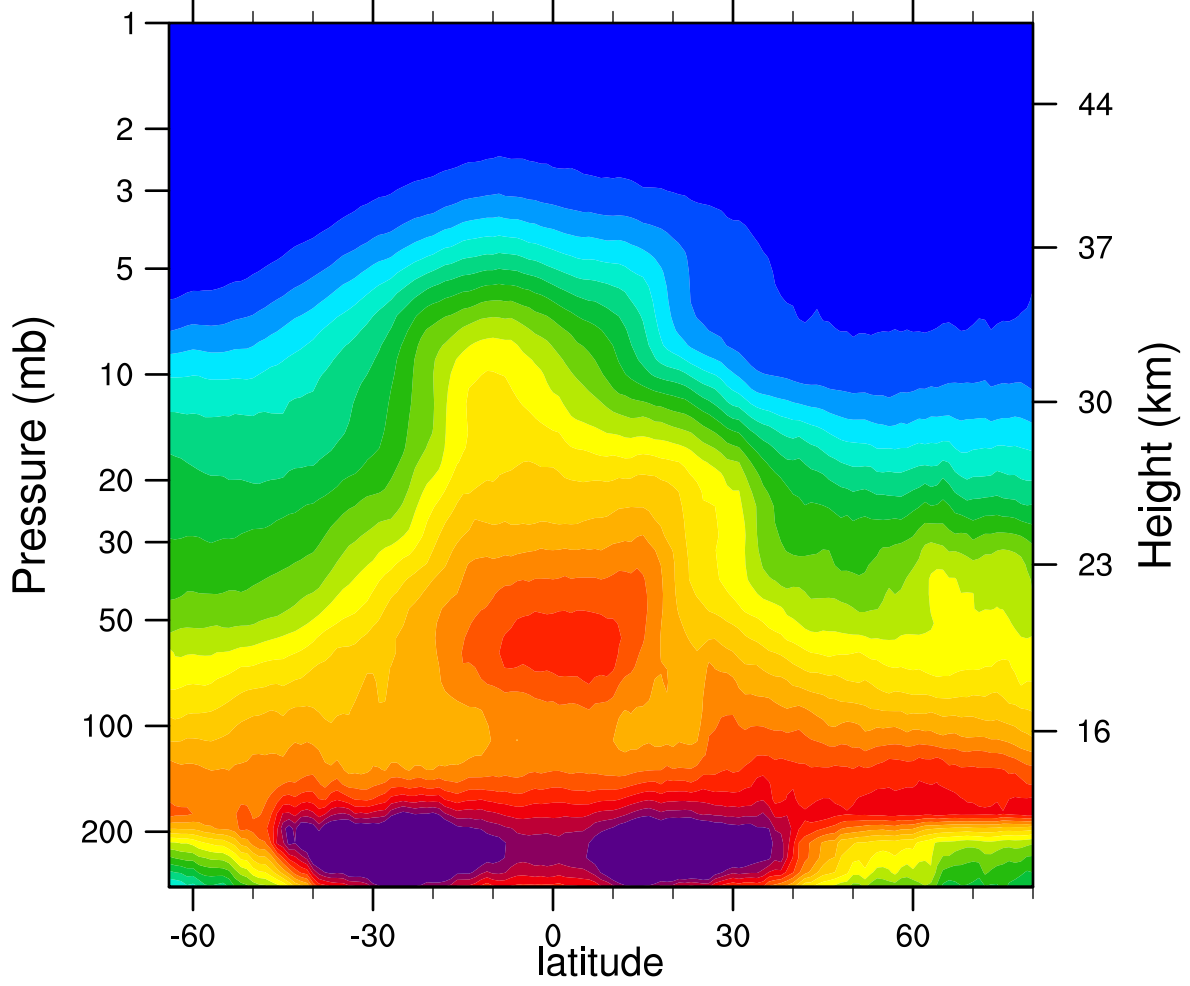
2006d043 N2O_Combined (ppbv)
