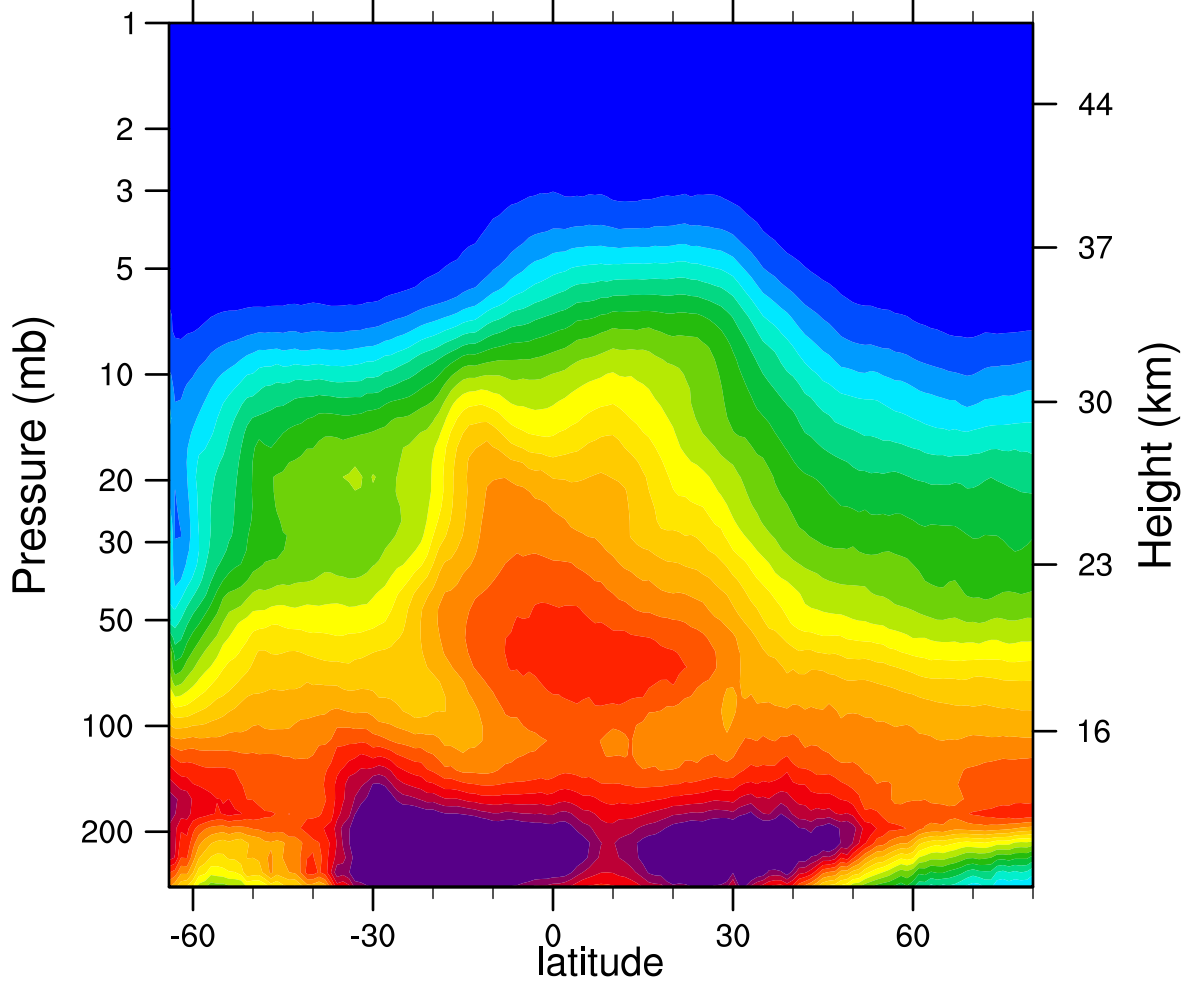
2007d253 N2O_Combined (ppbv)
