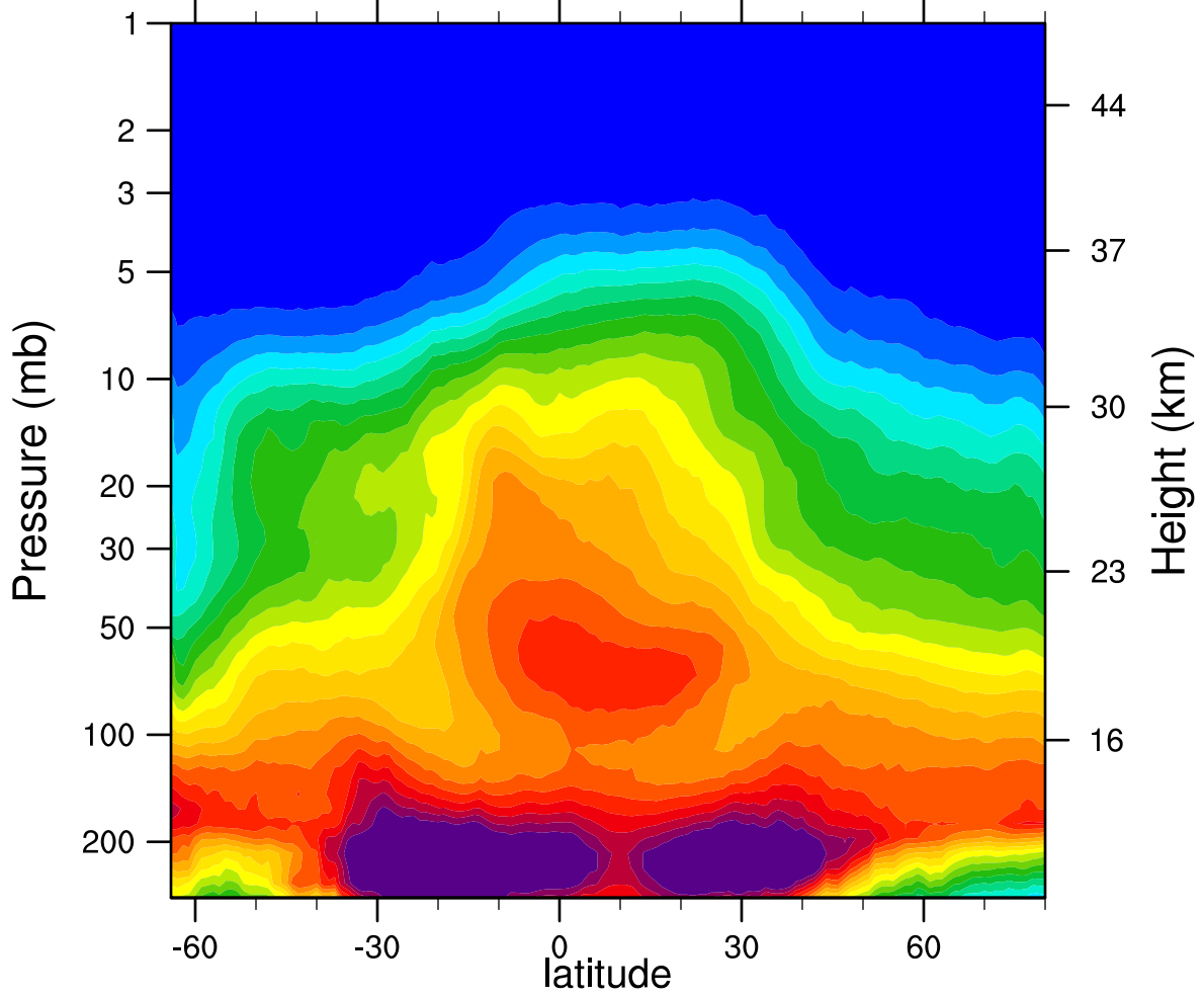
2007d265 N2O_Combined (ppbv)
