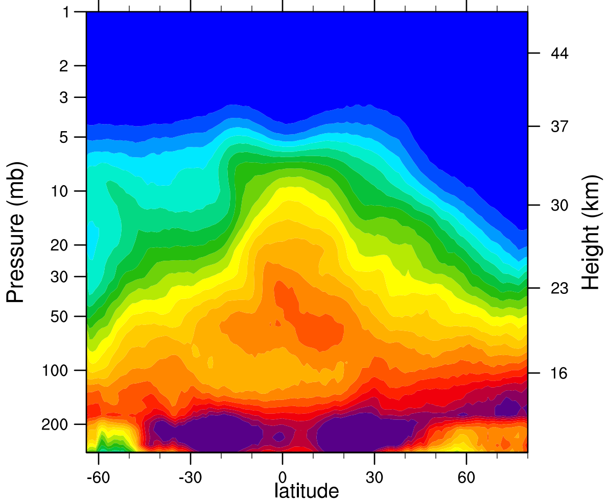
2006d327 N2O_Combined (ppbv)
