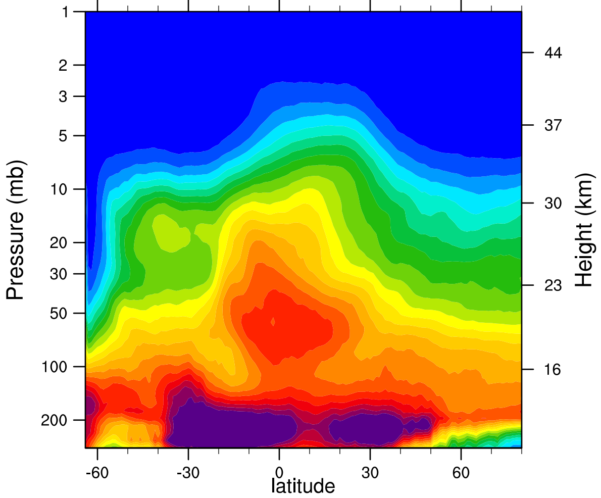
2007d225 N2O_Combined (ppbv)
