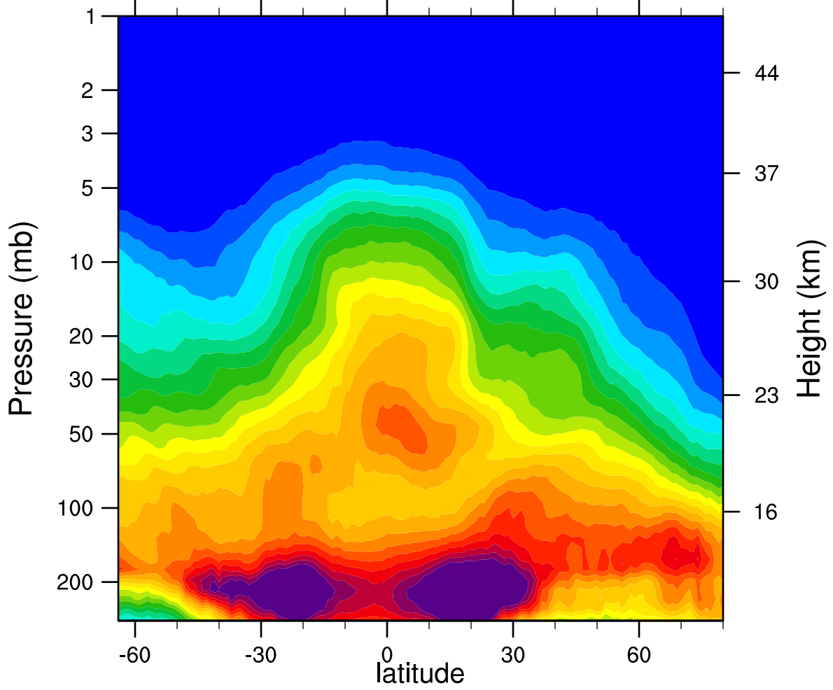
2005d044 N2O_Combined (ppbv)
