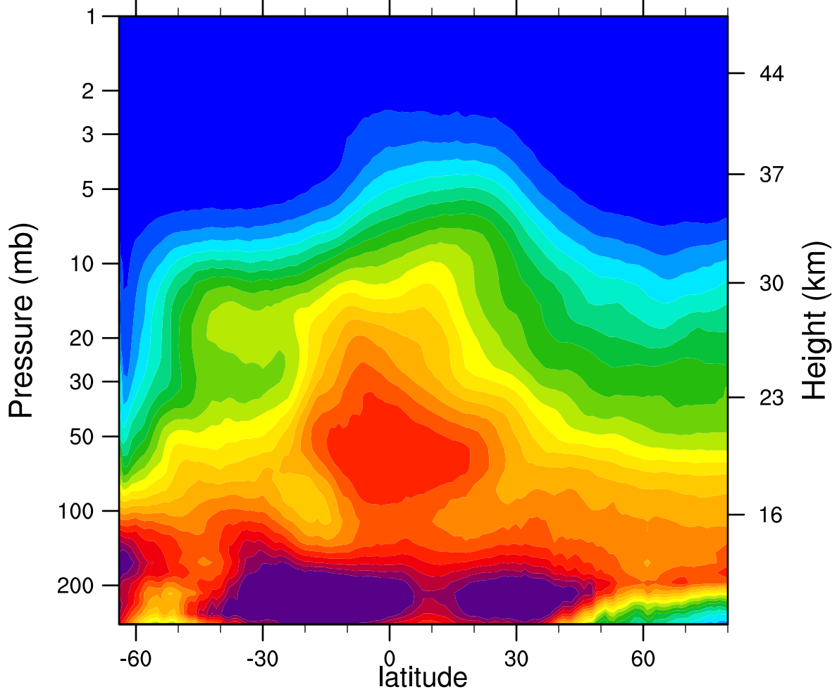
2007d231 N2O_Combined (ppbv)
