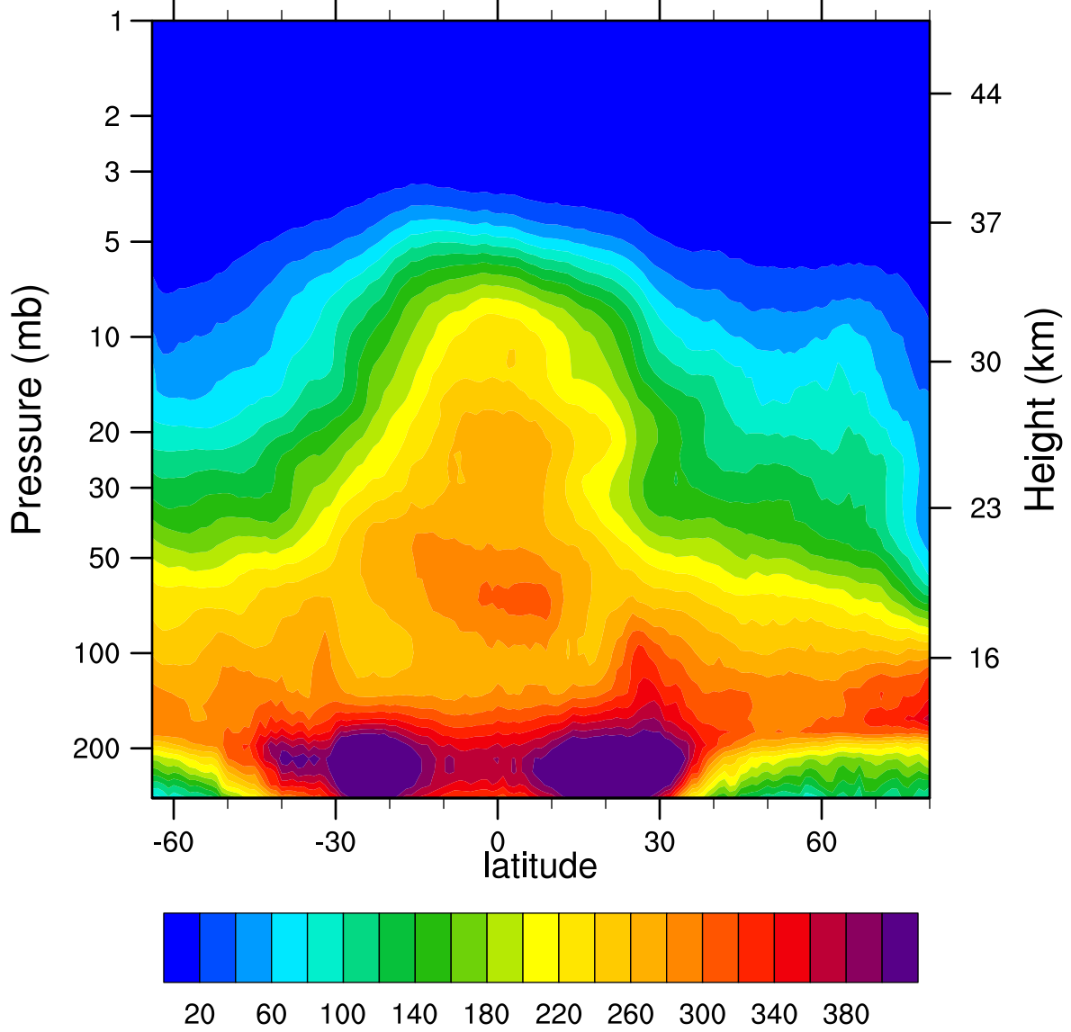
2007d061 N2O_Combined (ppbv)
