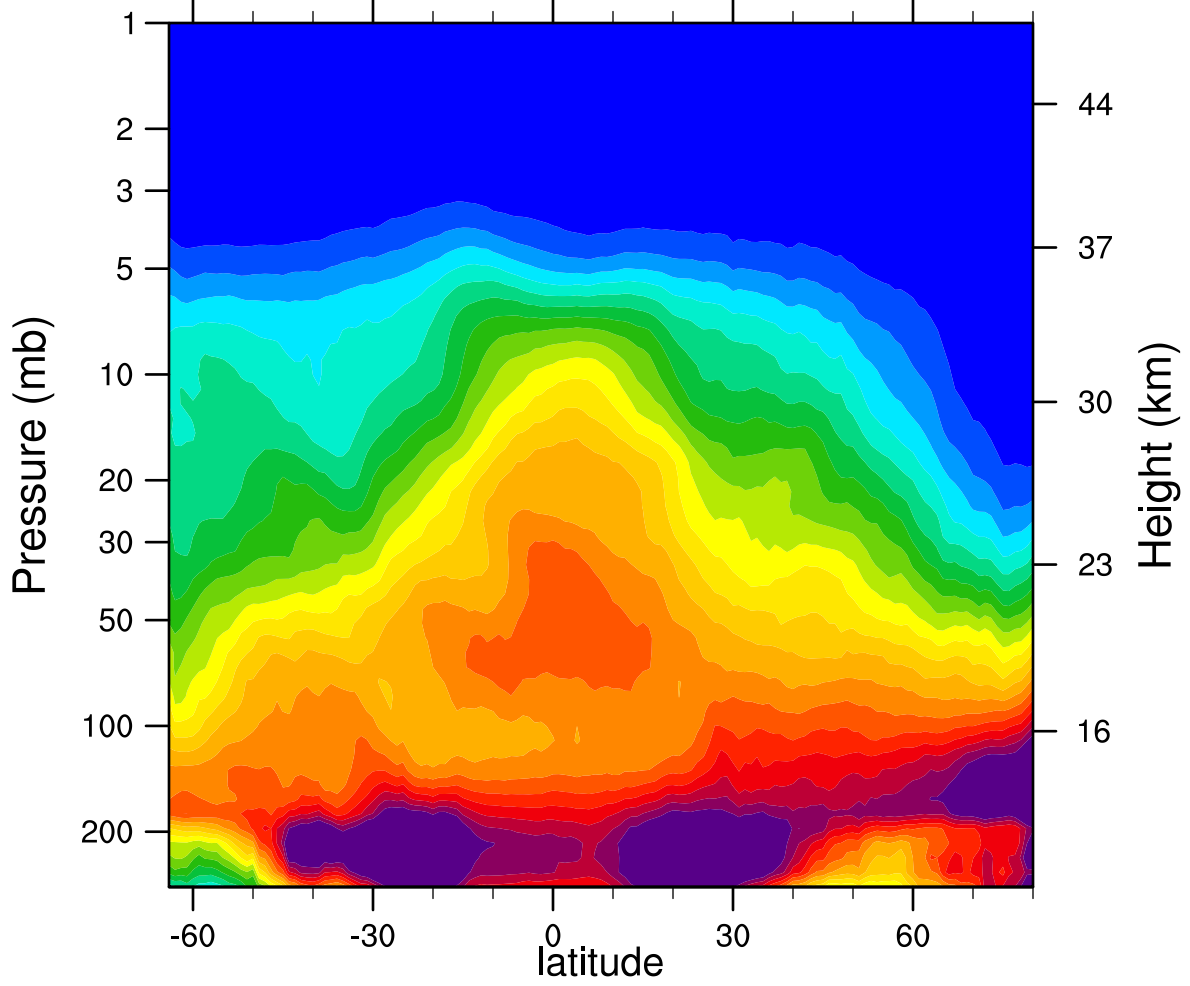
2006d344 N2O_Combined (ppbv)
