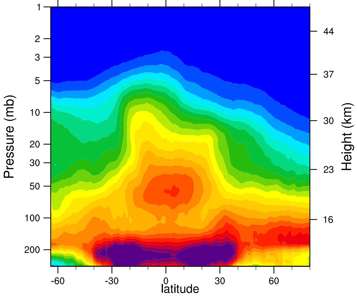
2005d348 N2O_Combined (ppbv)
