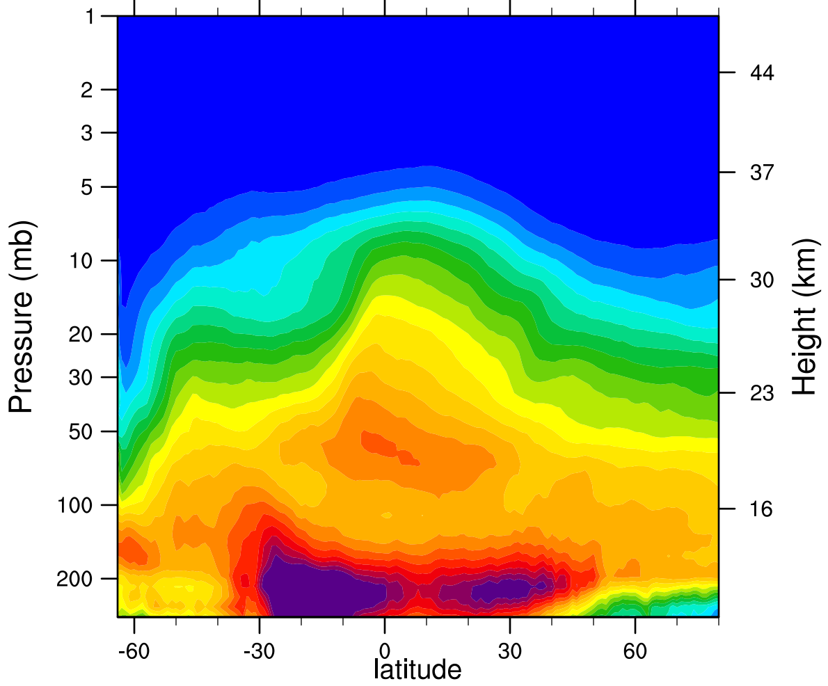
2006d216 N2O_Combined (ppbv)
