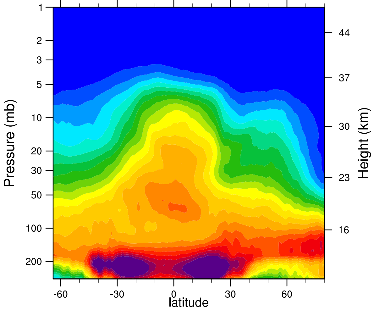
2007d034 N2O_Combined (ppbv)
