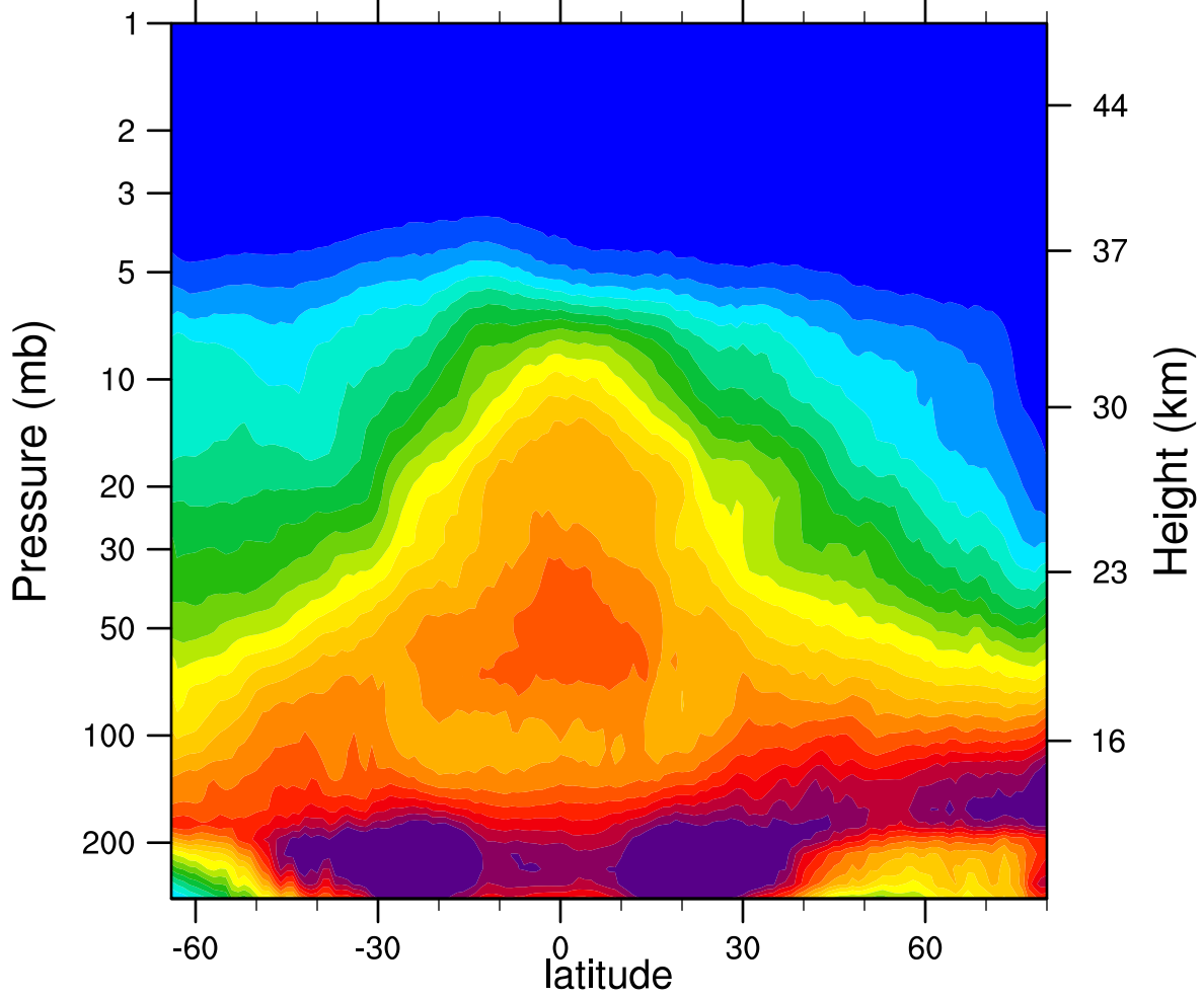
2006d356 N2O_Combined (ppbv)
