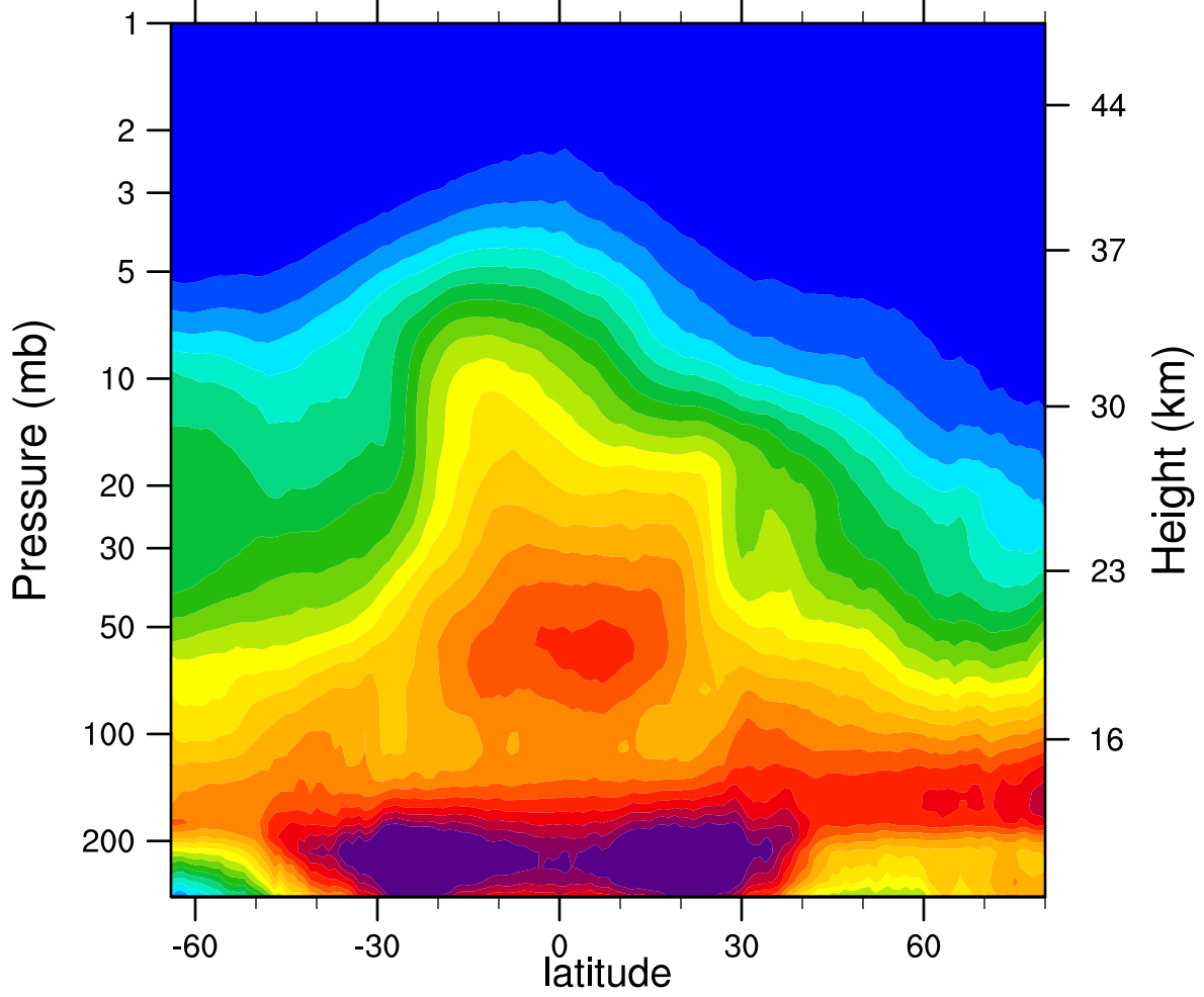
2005d365 N2O_Combined (ppbv)
