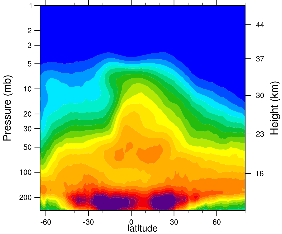
2006d289 N2O_Combined (ppbv)
