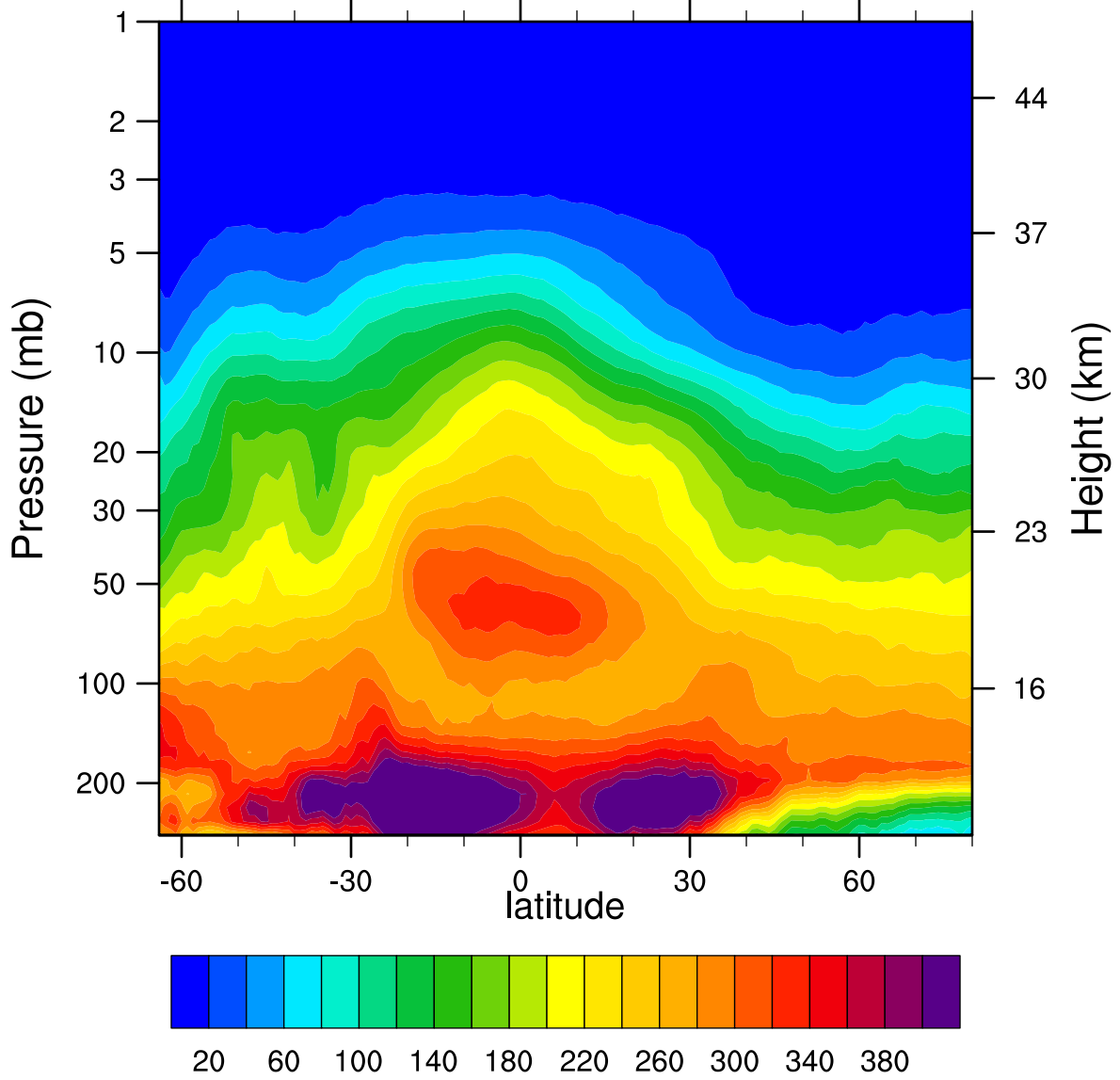
2006d144 N2O_Combined (ppbv)
