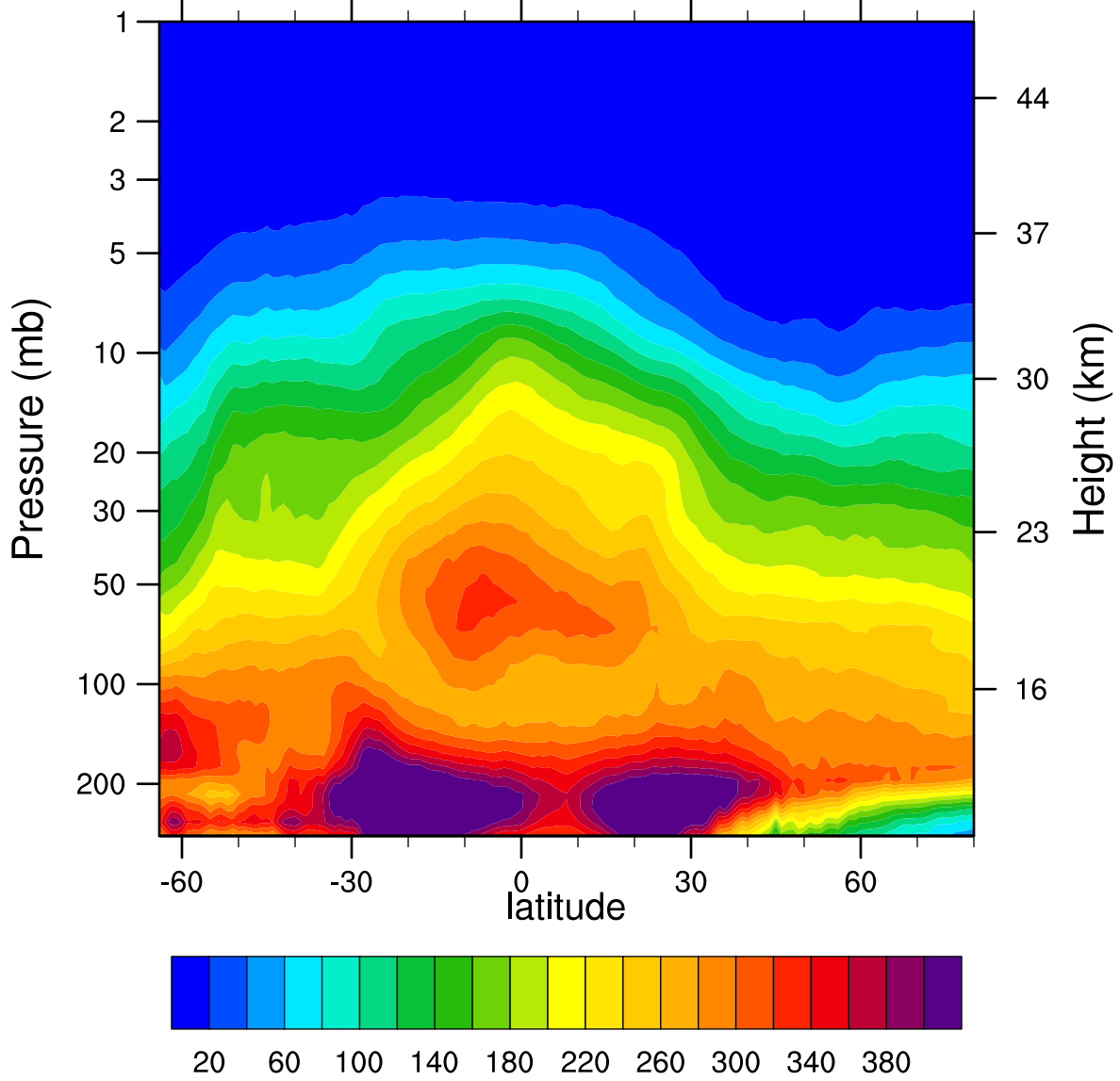
2006d159 N2O_Combined (ppbv)
