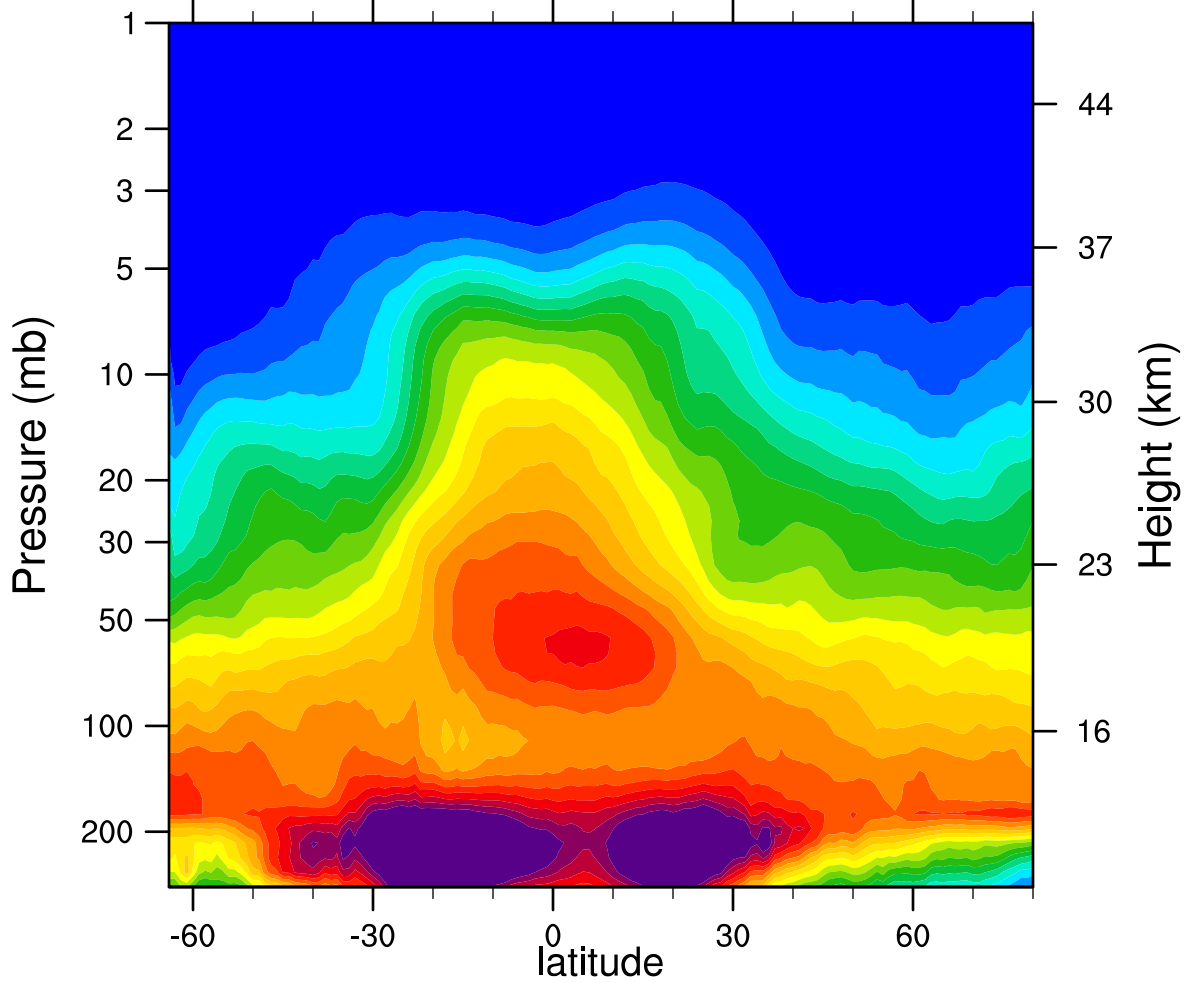
2005d128 N2O_Combined (ppbv)
