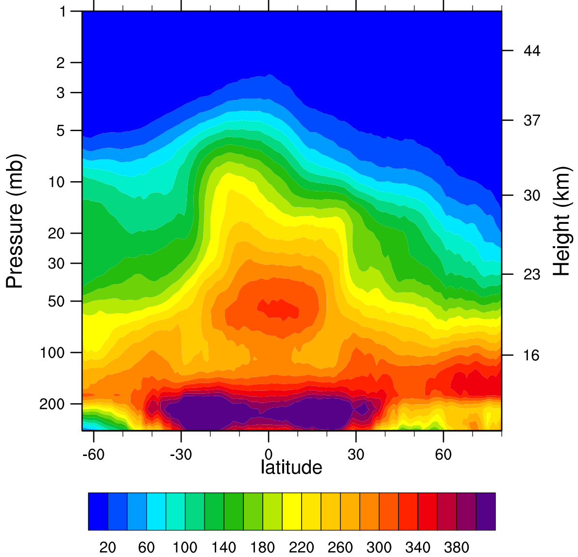
2005d358 N2O_Combined (ppbv)
