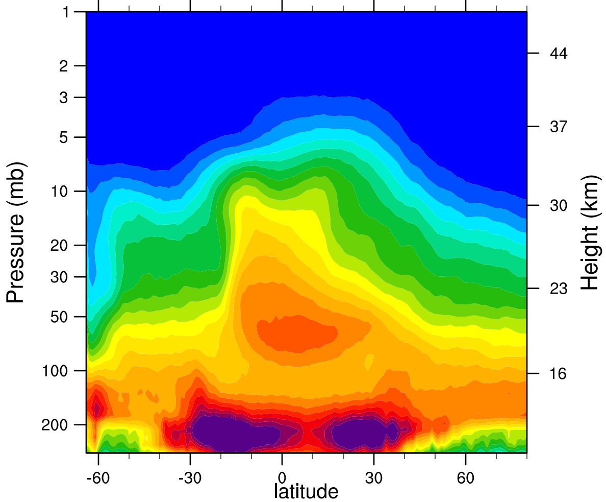
2005d266 N2O_Combined (ppbv)
