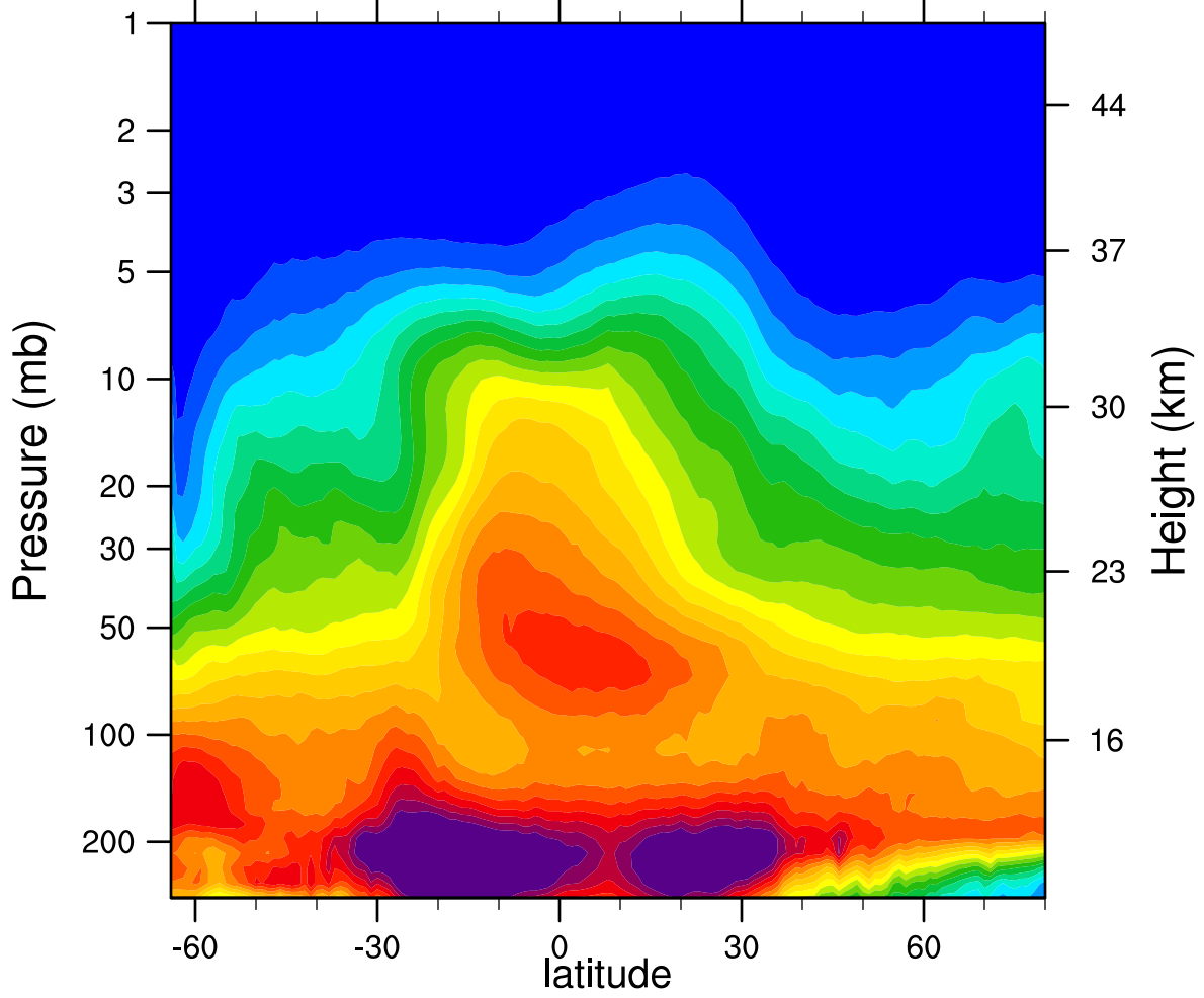
2005d165 N2O_Combined (ppbv)
