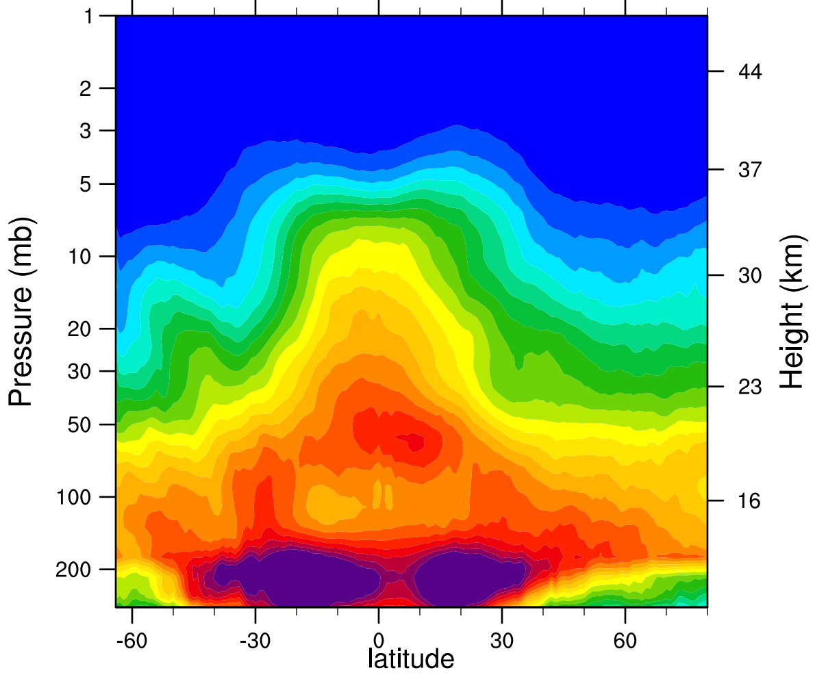
2005d117 N2O_Combined (ppbv)
