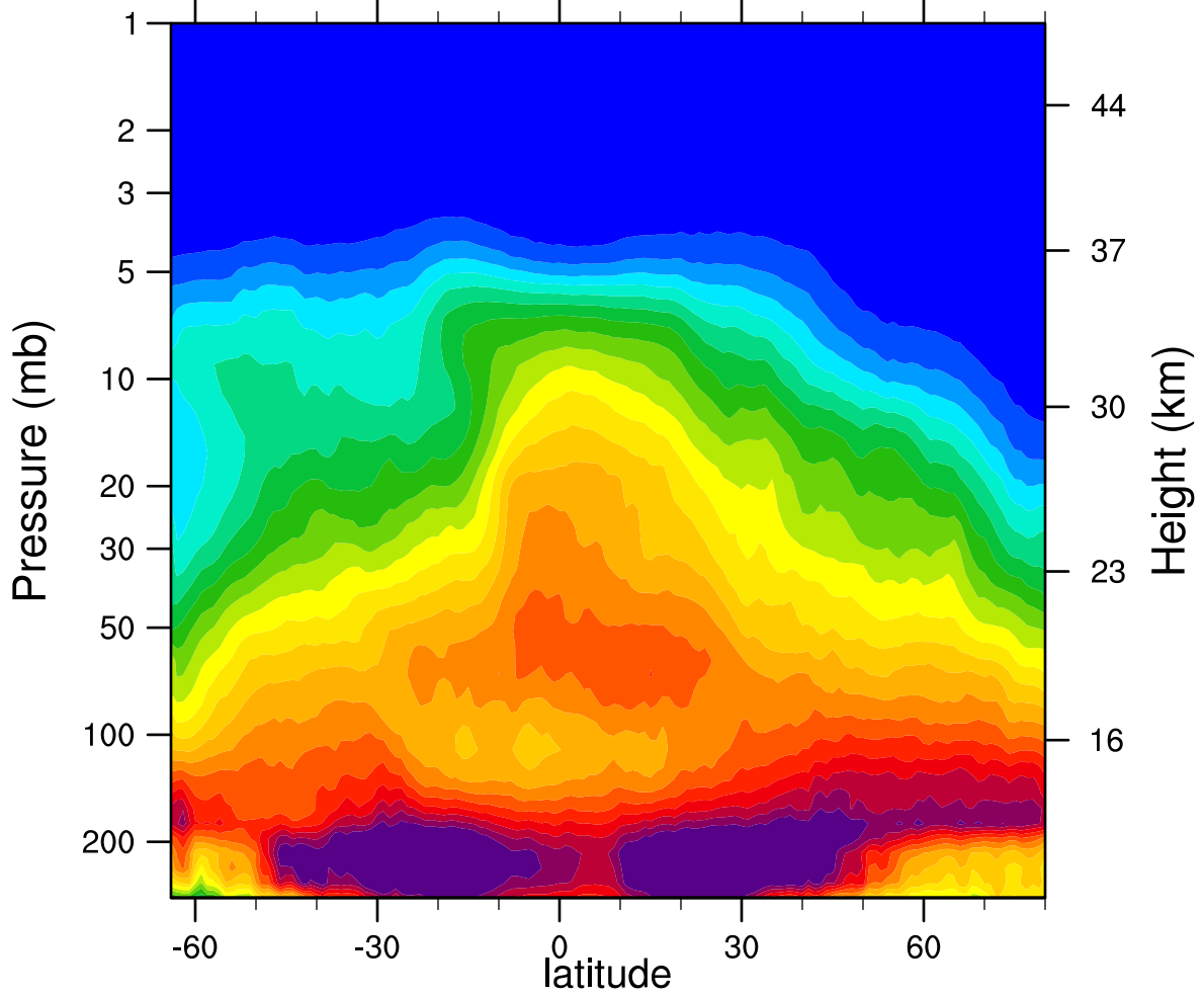
2006d312 N2O_Combined (ppbv)
