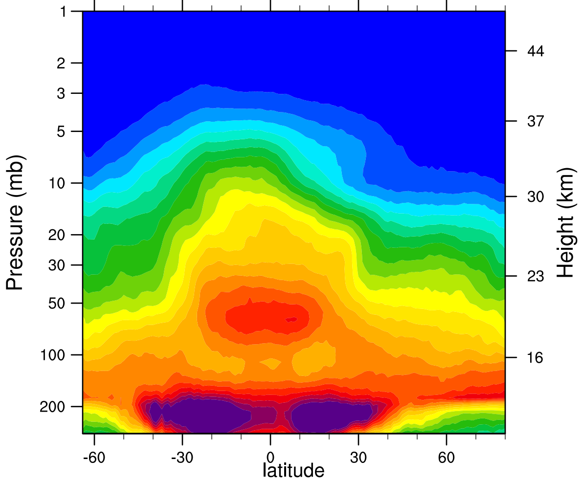
2006d099 N2O_Combined (ppbv)
