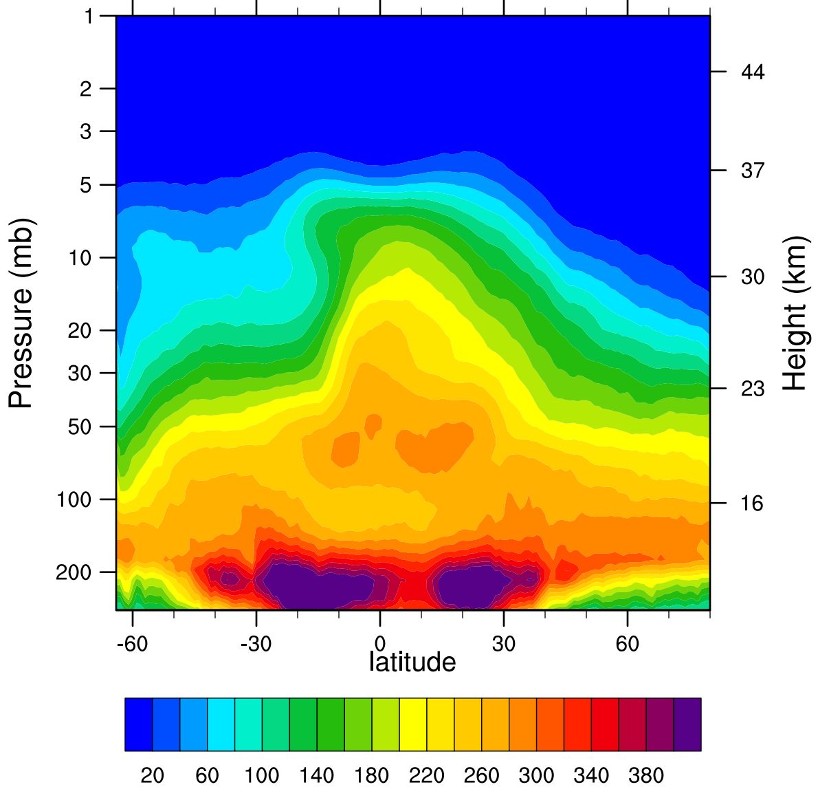
2006d290 N2O_Combined (ppbv)
