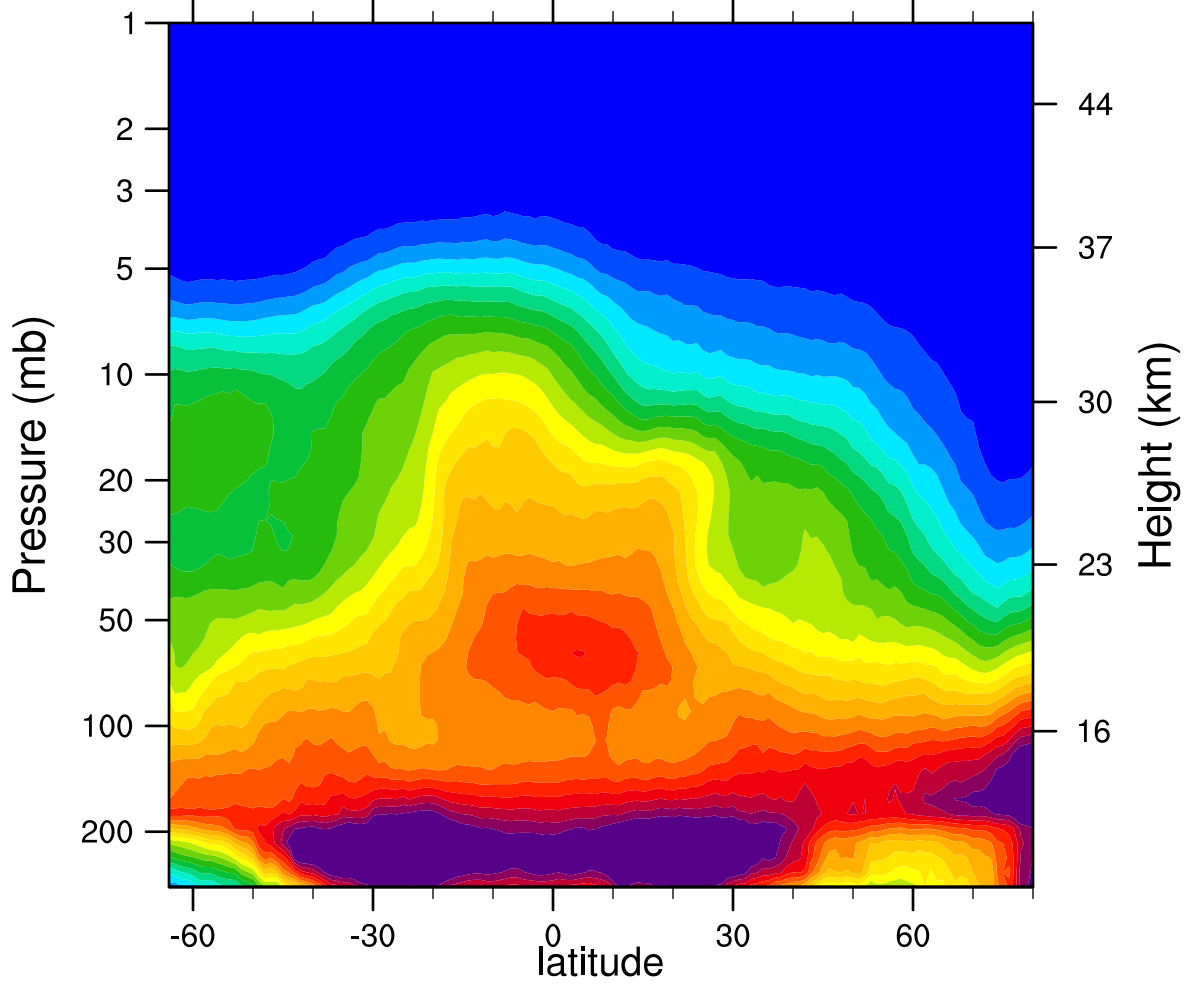
2007d362 N2O_Combined (ppbv)
