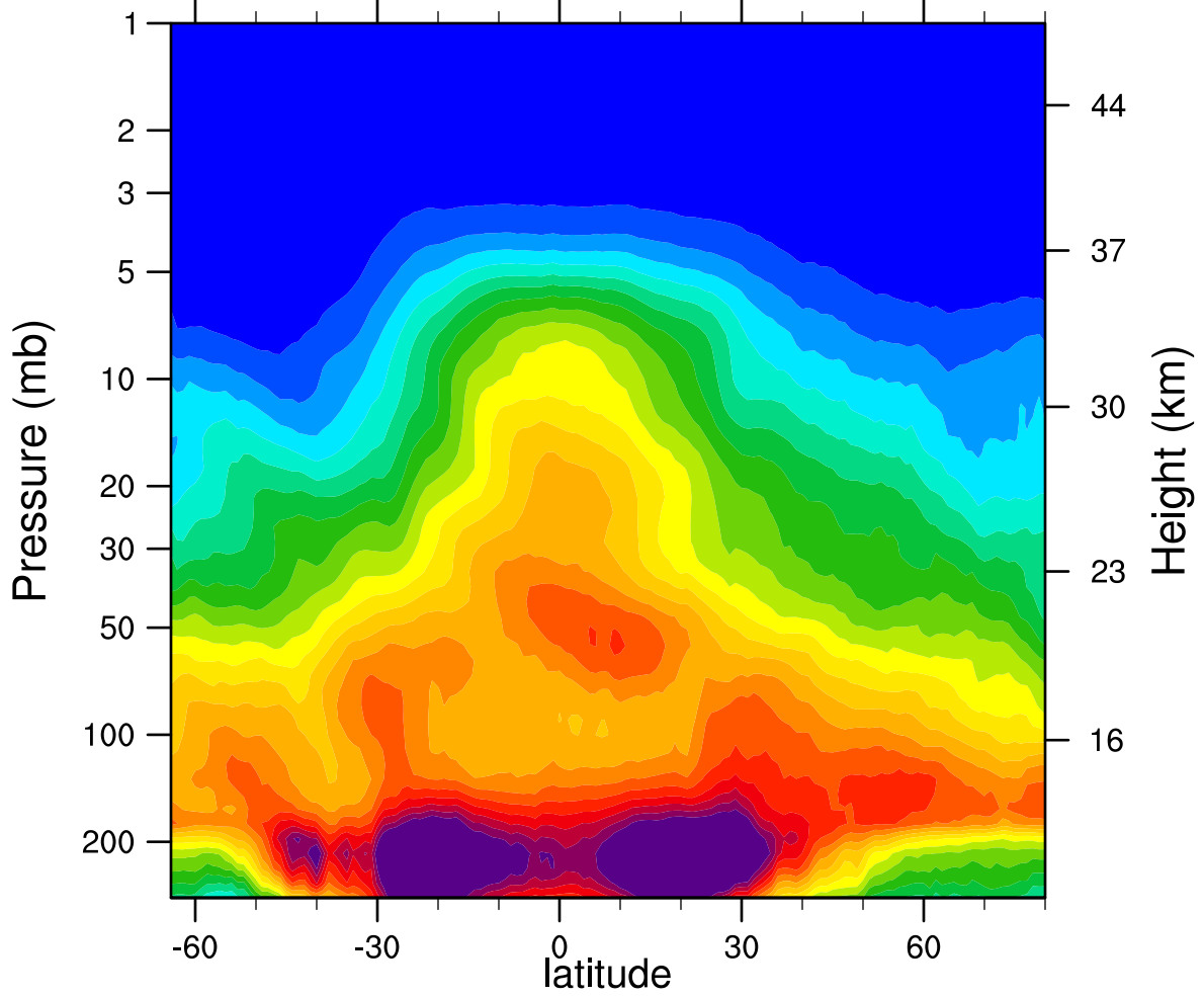
2005d087 N2O_Combined (ppbv)
