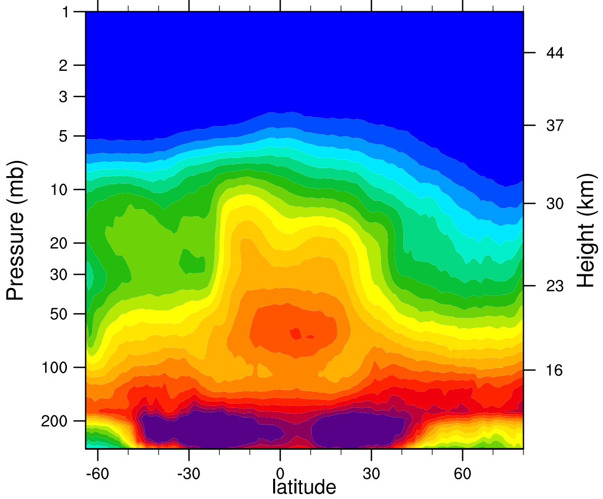
2007d323 N2O_Combined (ppbv)
