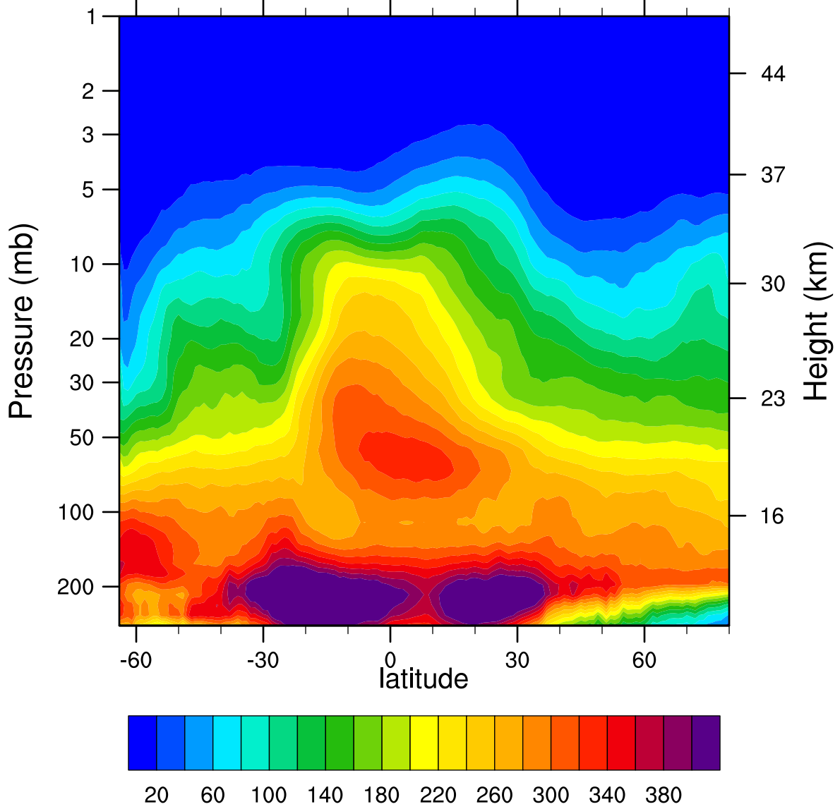
2005d163 N2O_Combined (ppbv)
