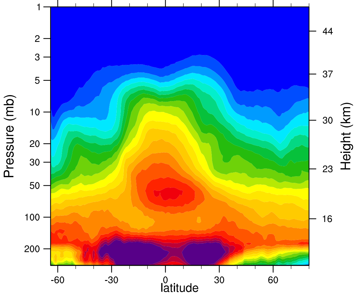
2005d133 N2O_Combined (ppbv)
