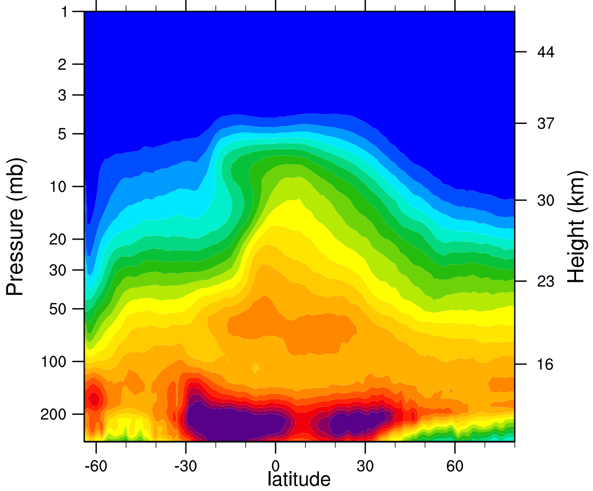
2006d264 N2O_Combined (ppbv)
