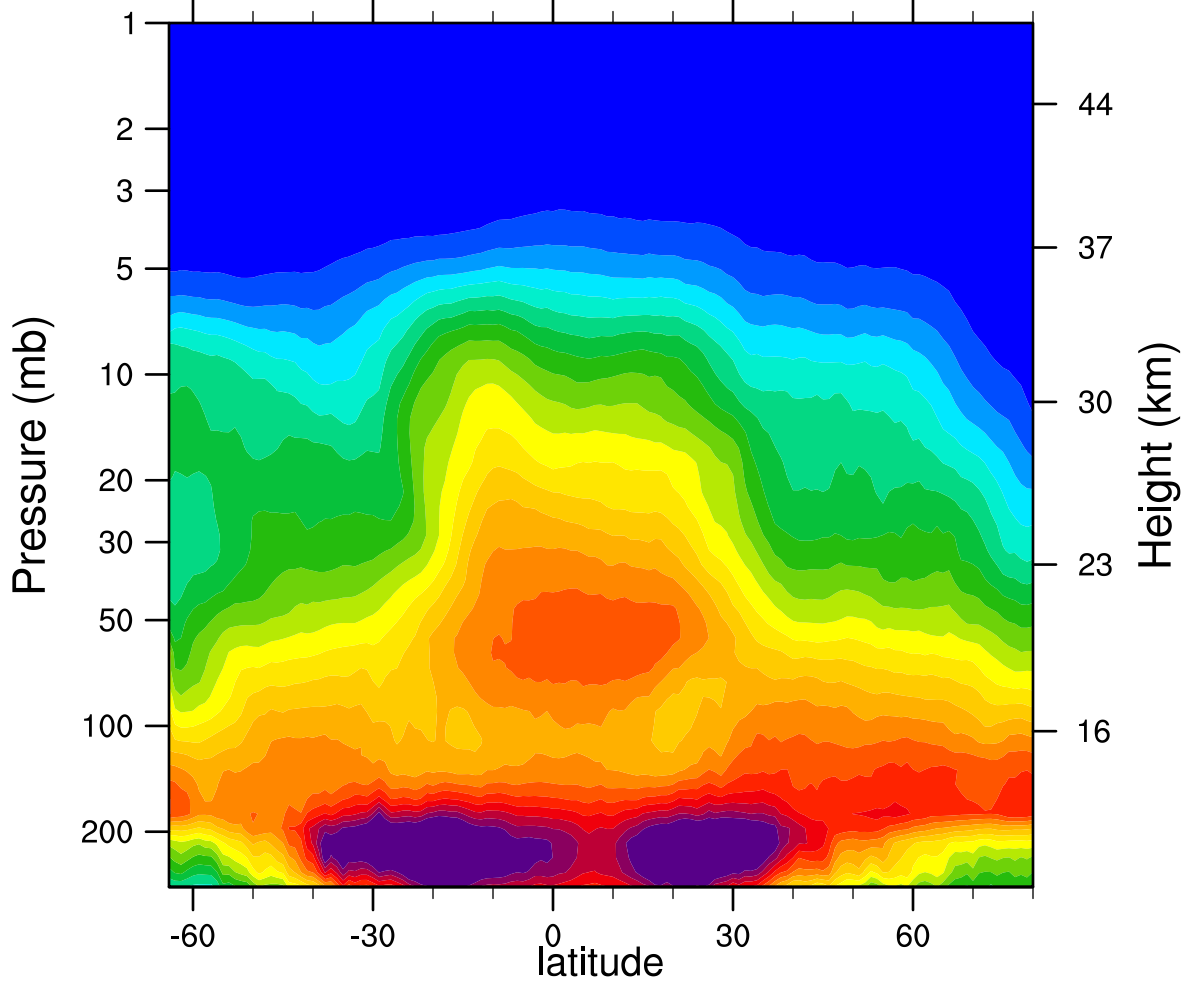
2005d314 N2O_Combined (ppbv)
