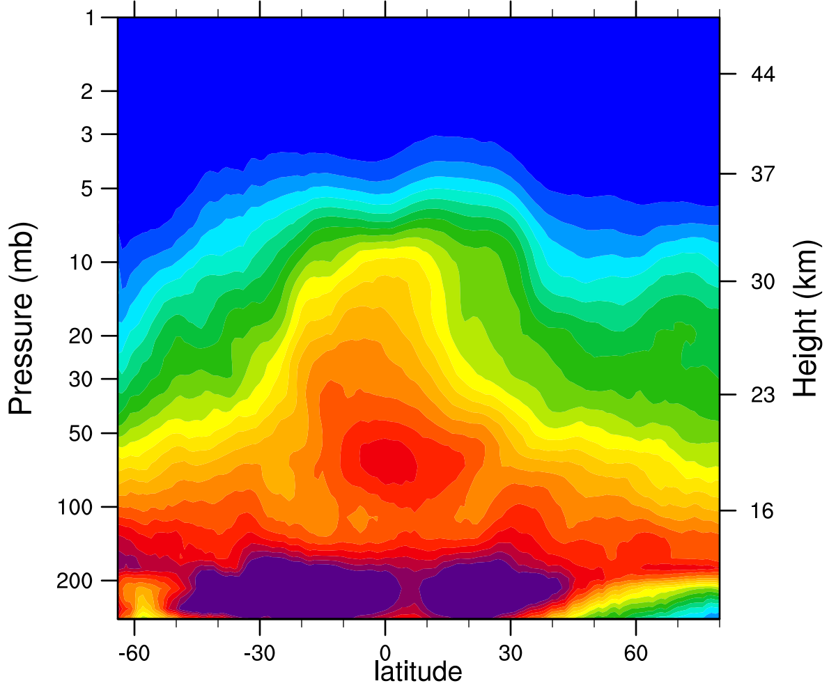
2007d136 N2O_Combined (ppbv)
