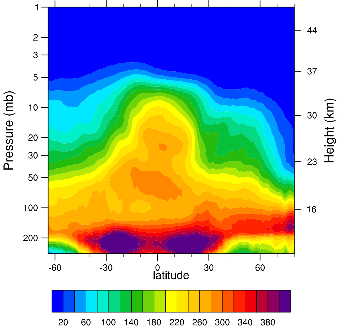
2007d022 N2O_Combined (ppbv)
