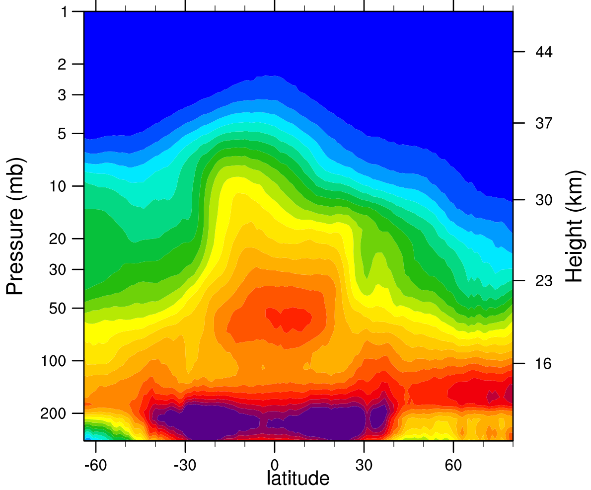
2005d363 N2O_Combined (ppbv)
