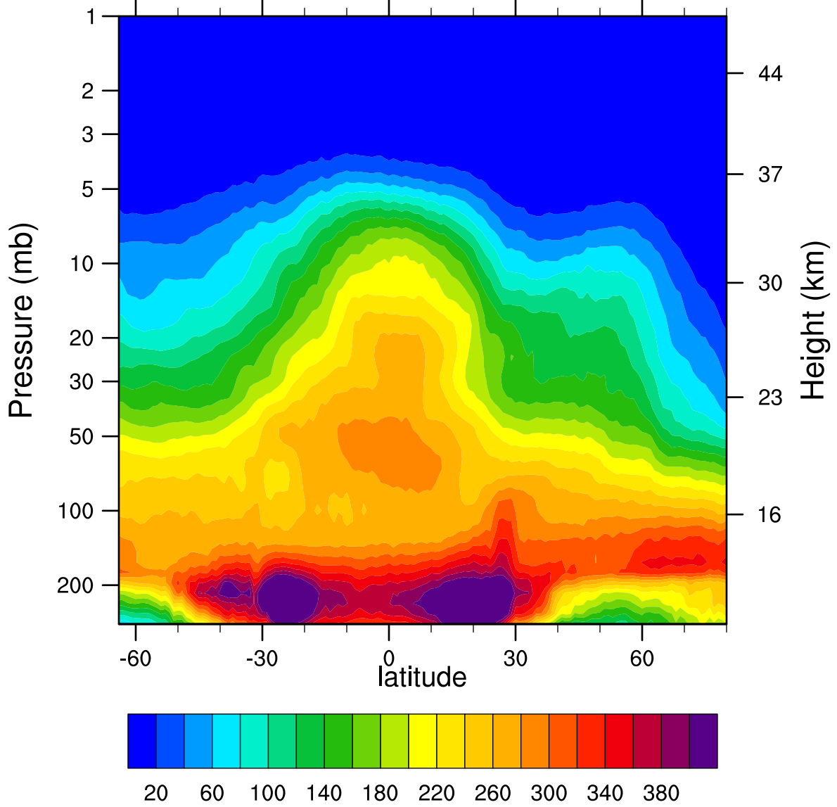
2007d048 N2O_Combined (ppbv)
