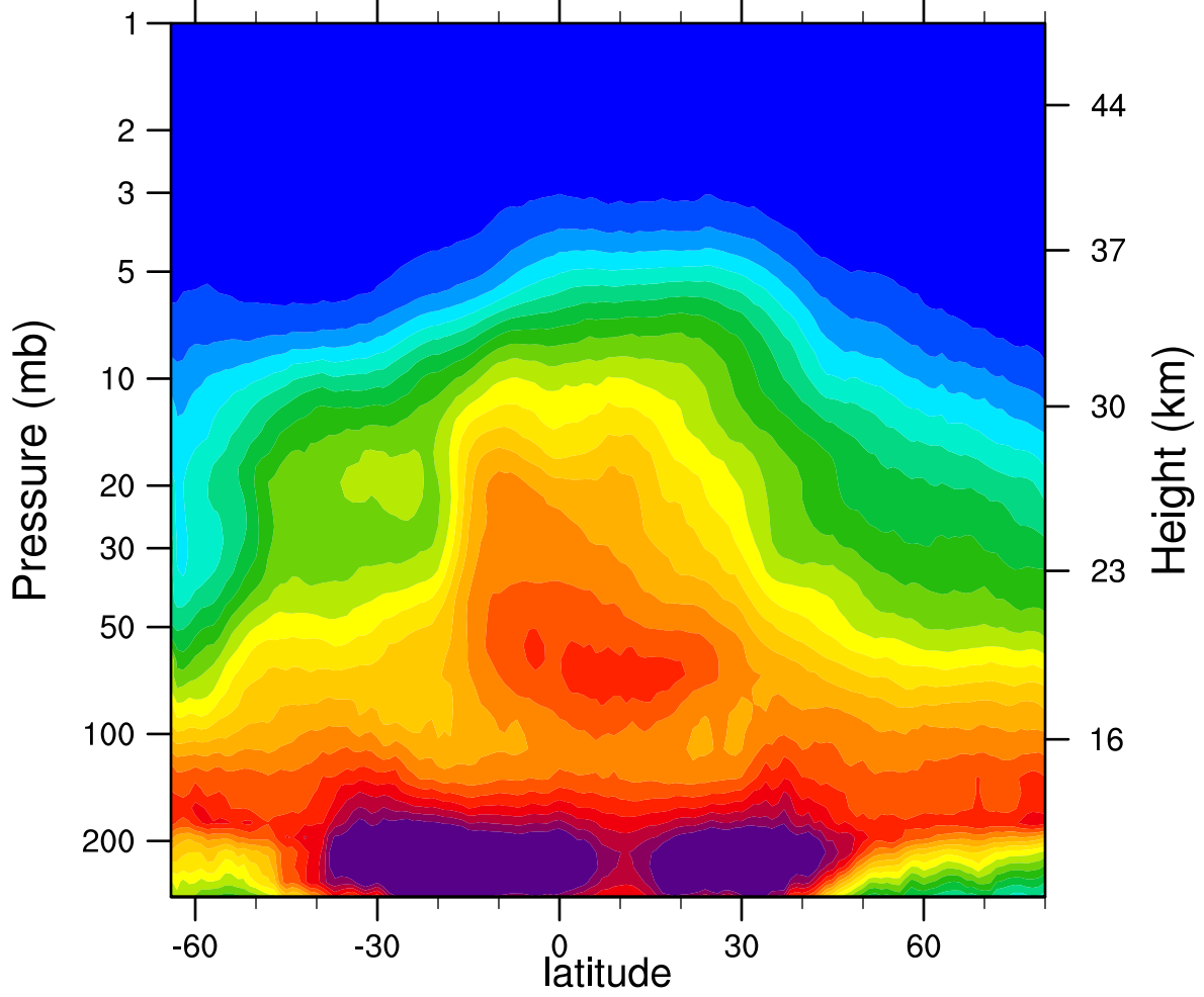
2007d275 N2O_Combined (ppbv)
