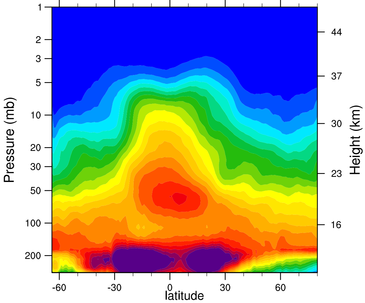
2005d126 N2O_Combined (ppbv)
