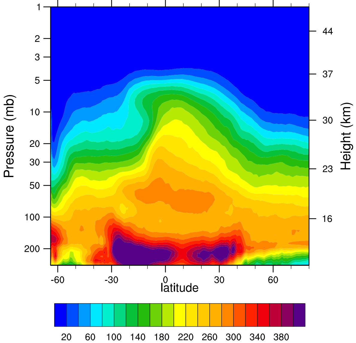
2006d257 N2O_Combined (ppbv)
