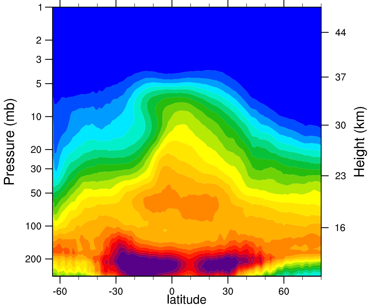
2006d270 N2O_Combined (ppbv)
