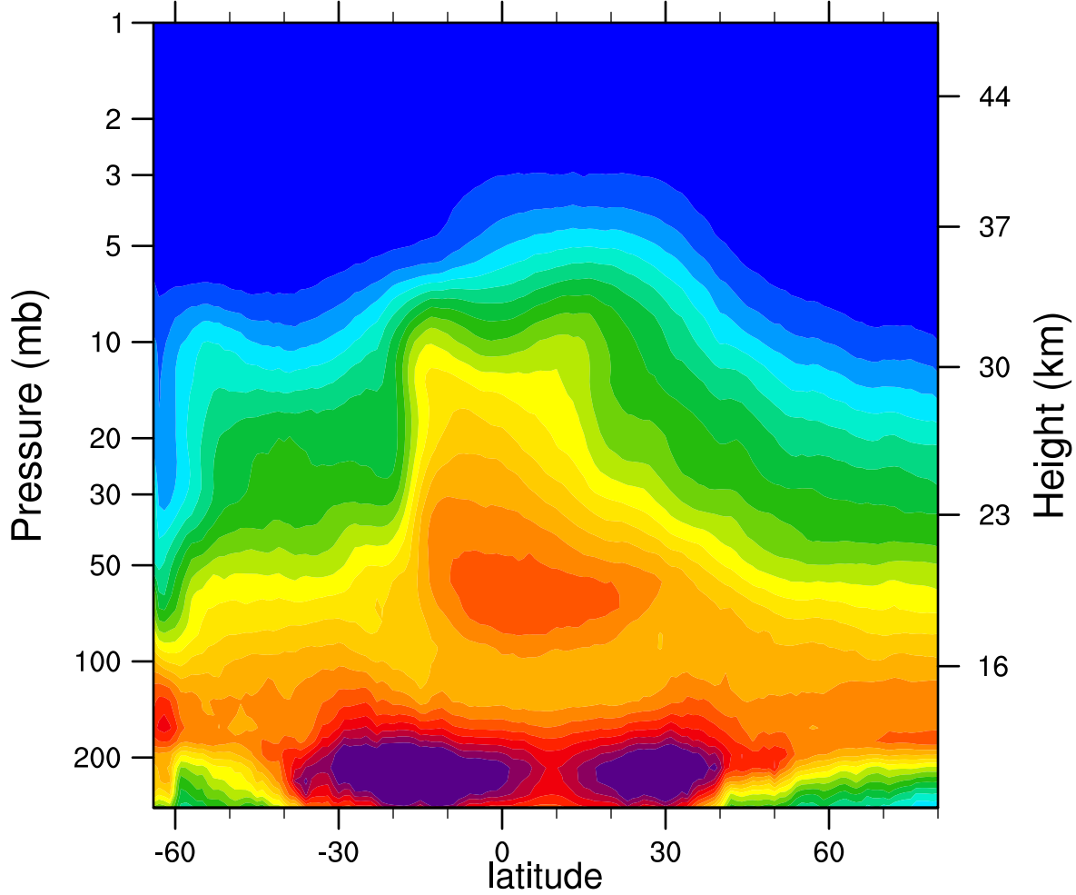
2005d260 N2O_Combined (ppbv)
