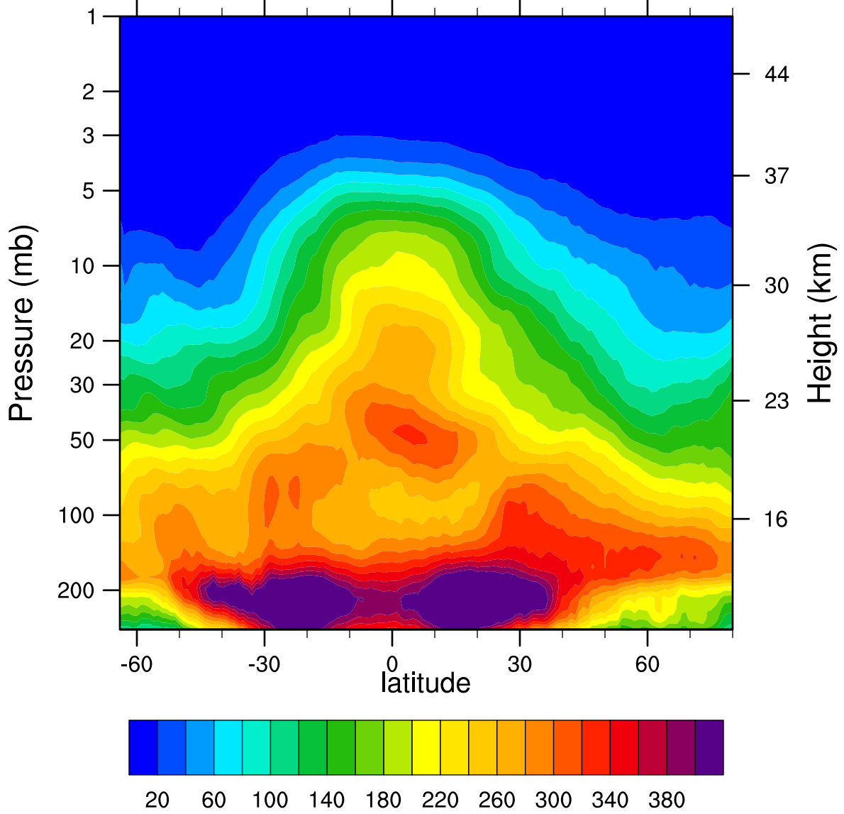
2005d074 N2O_Combined (ppbv)
