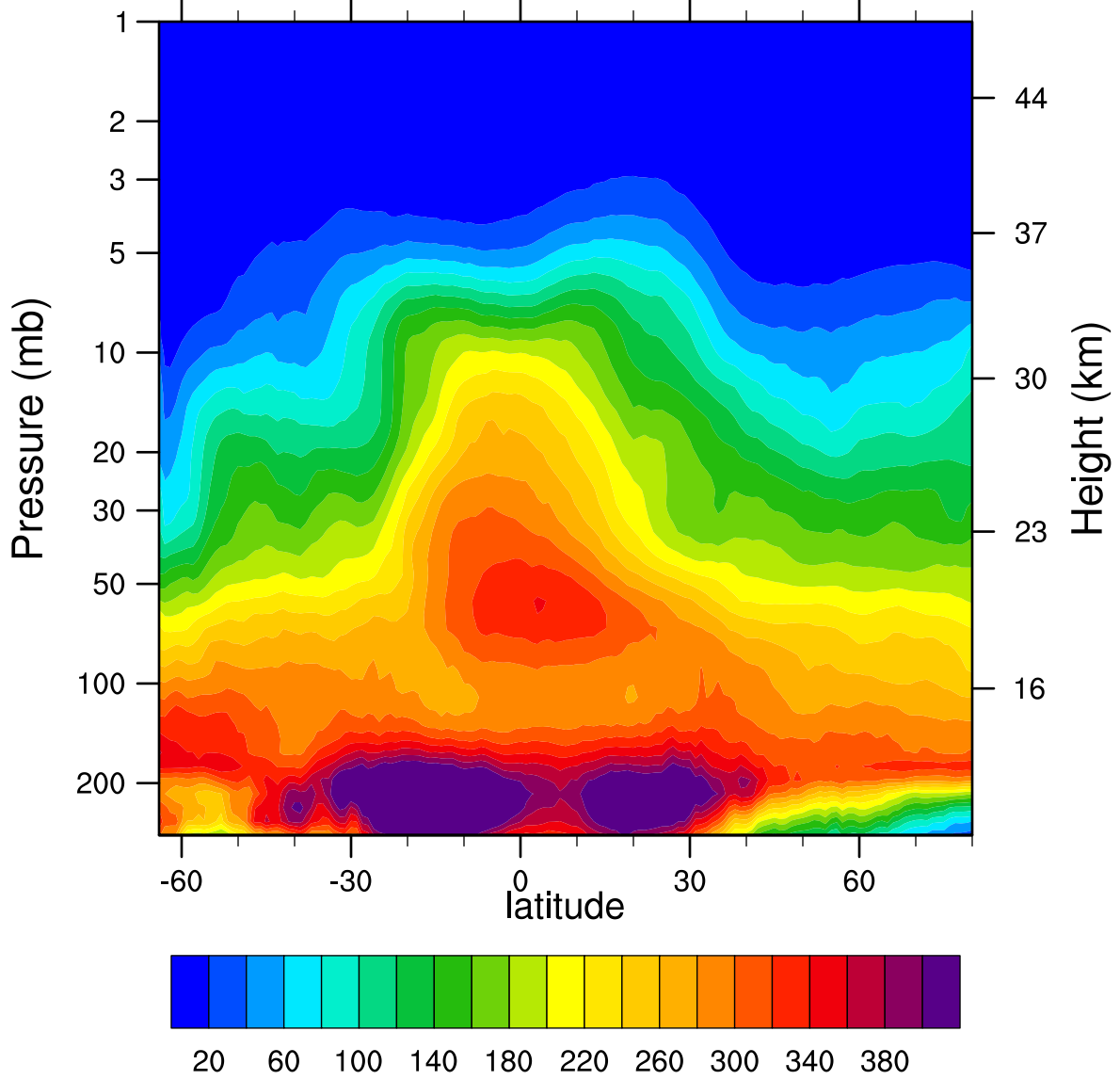
2005d149 N2O_Combined (ppbv)
