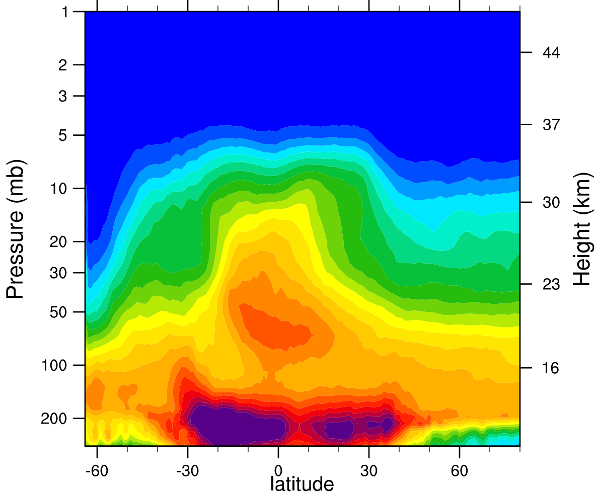
2007d180 N2O_Combined (ppbv)
