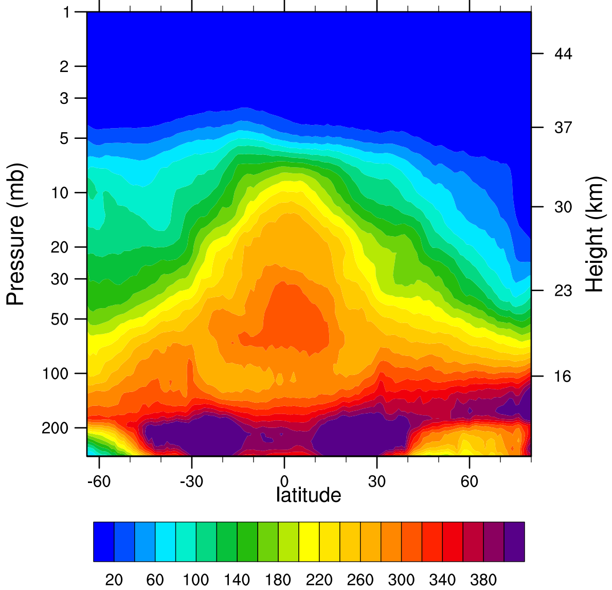
2006d354 N2O_Combined (ppbv)
