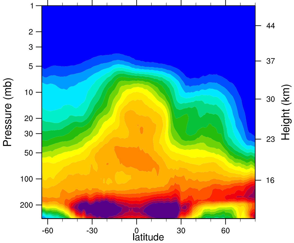
2007d016 N2O_Combined (ppbv)
