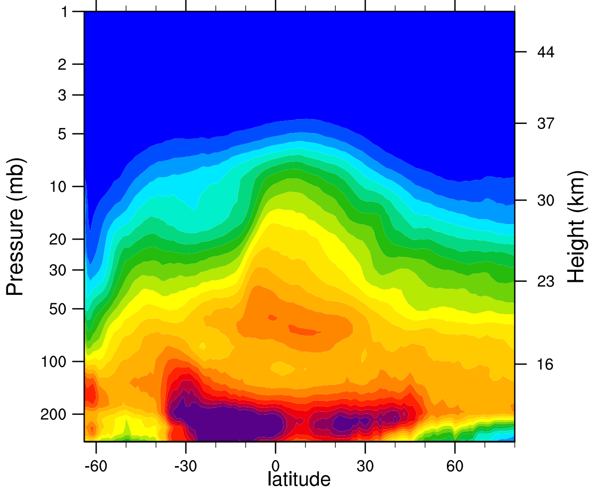
2006d224 N2O_Combined (ppbv)
