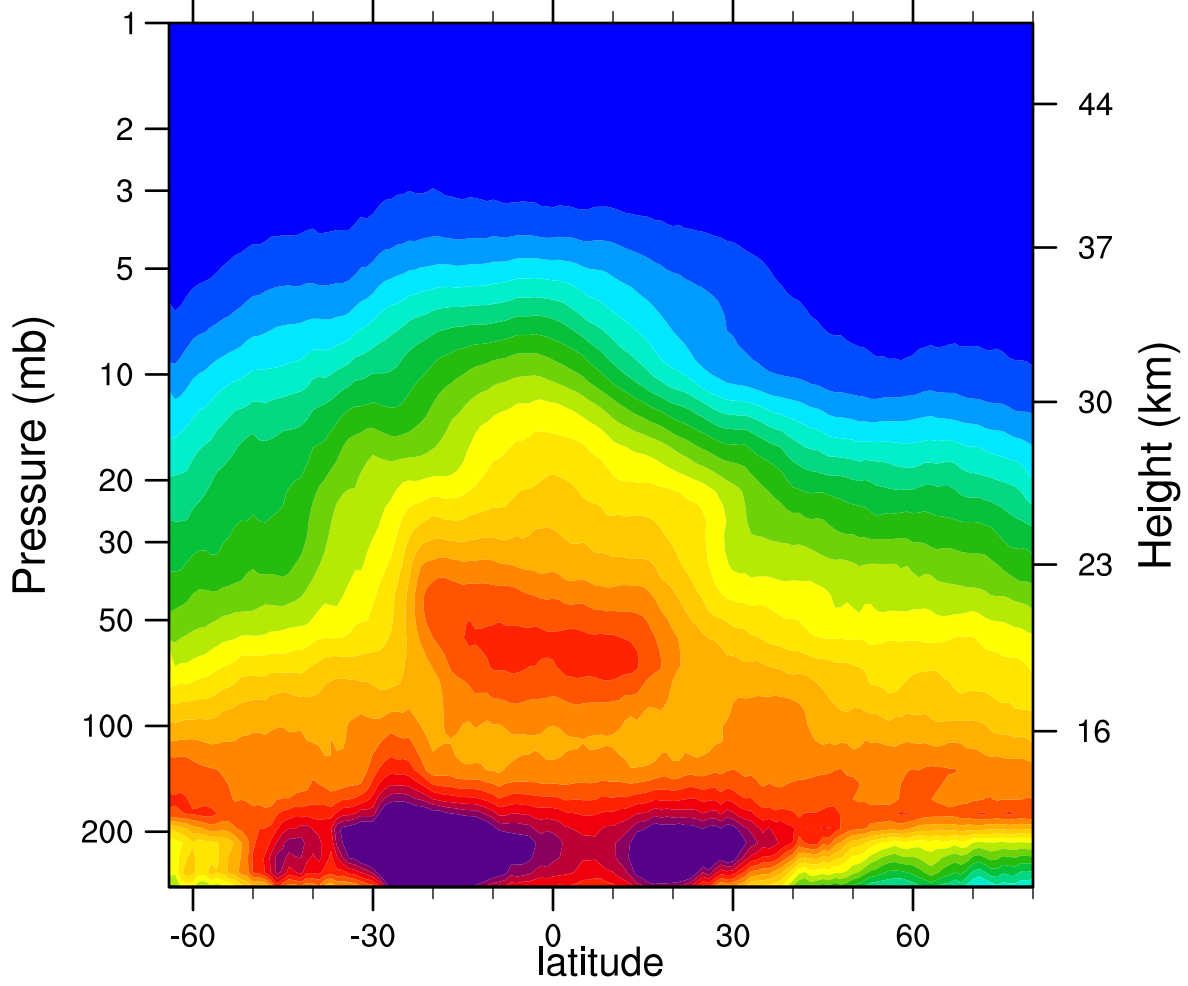
2006d126 N2O_Combined (ppbv)
