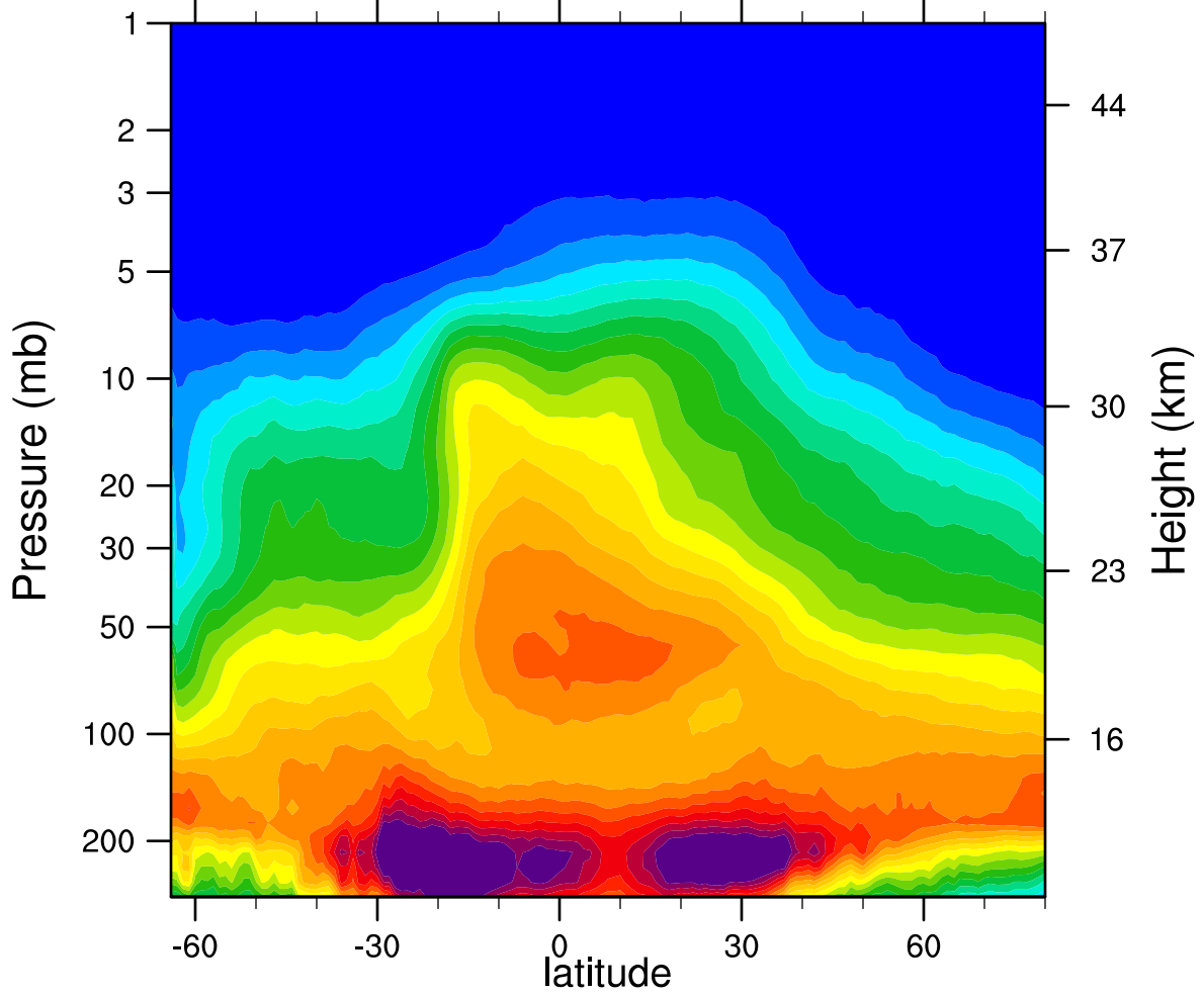
2005d276 N2O_Combined (ppbv)
