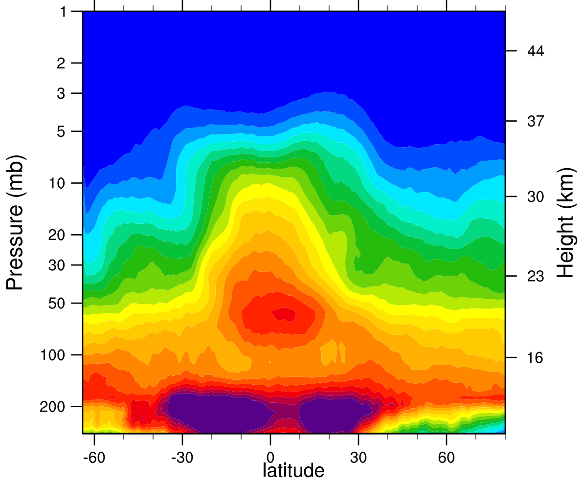
2005d139 N2O_Combined (ppbv)
