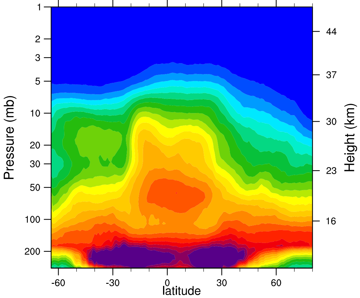
2007d302 N2O_Combined (ppbv)
