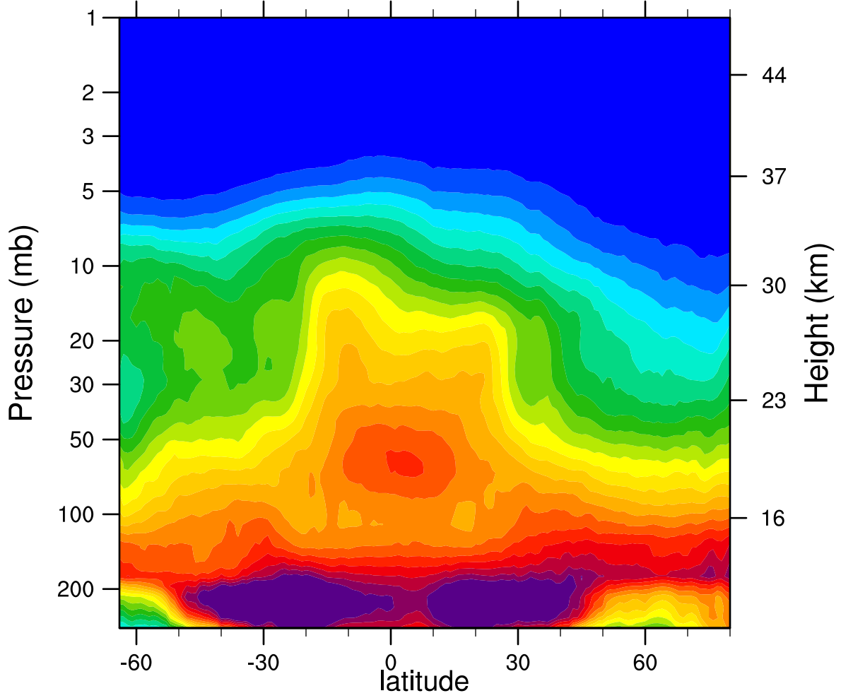
2007d334 N2O_Combined (ppbv)
