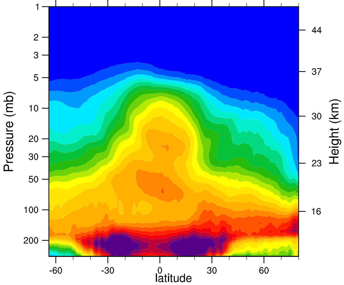
2007d025 N2O_Combined (ppbv)
