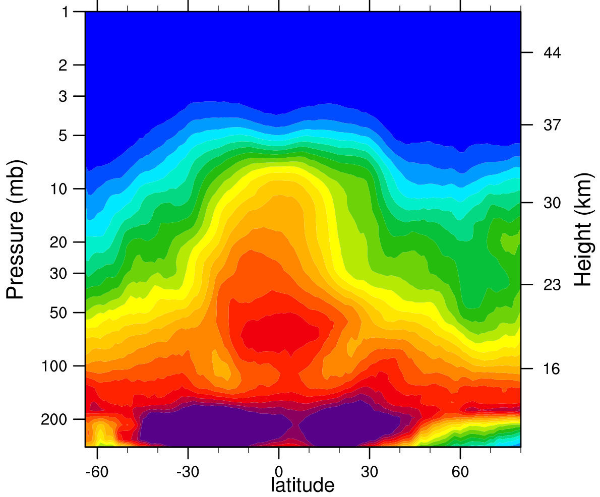
2007d120 N2O_Combined (ppbv)
