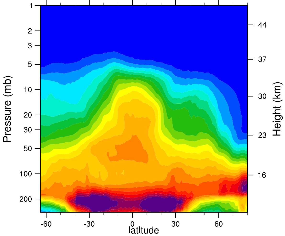
2007d006 N2O_Combined (ppbv)
