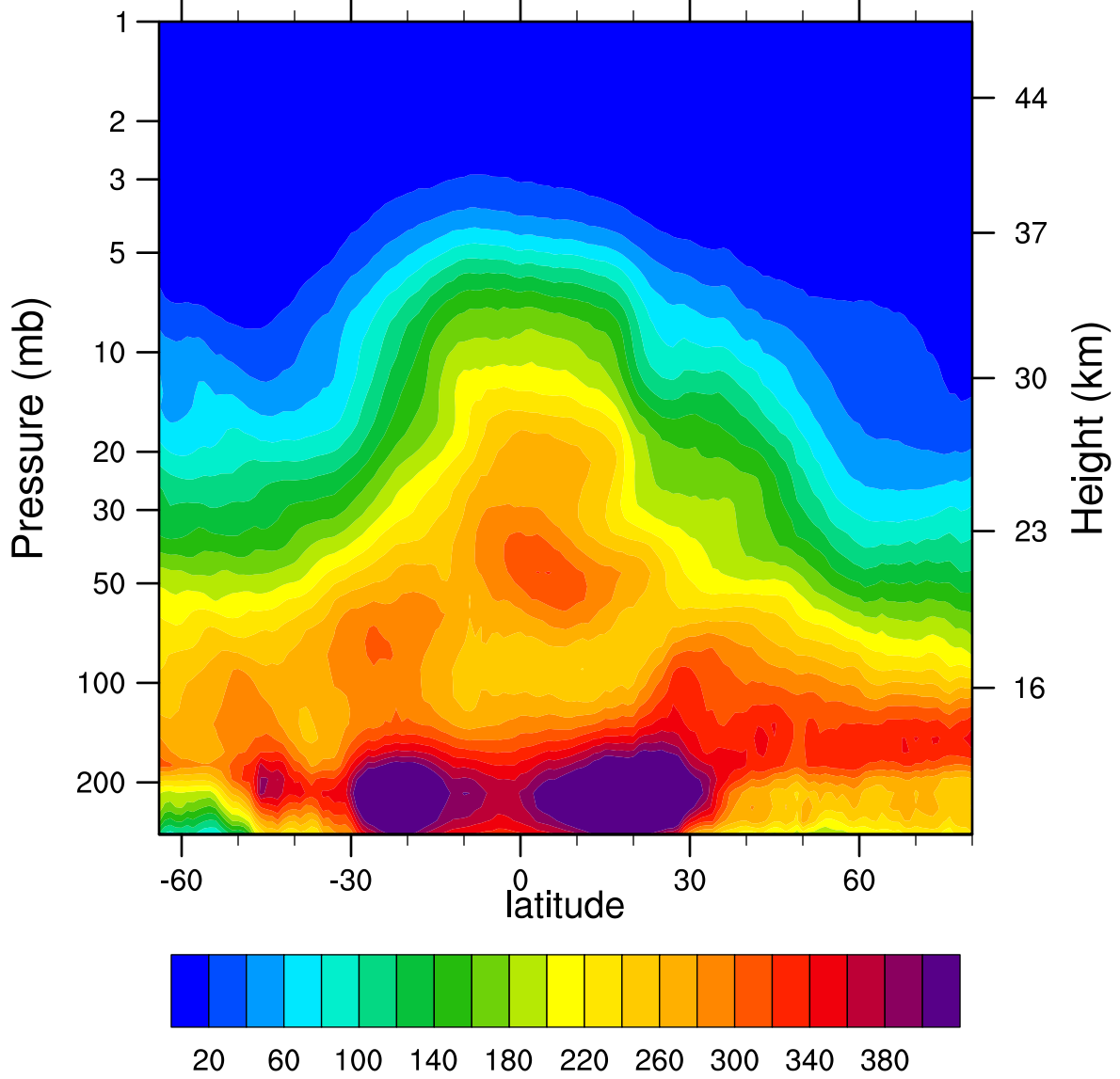
2005d058 N2O_Combined (ppbv)
