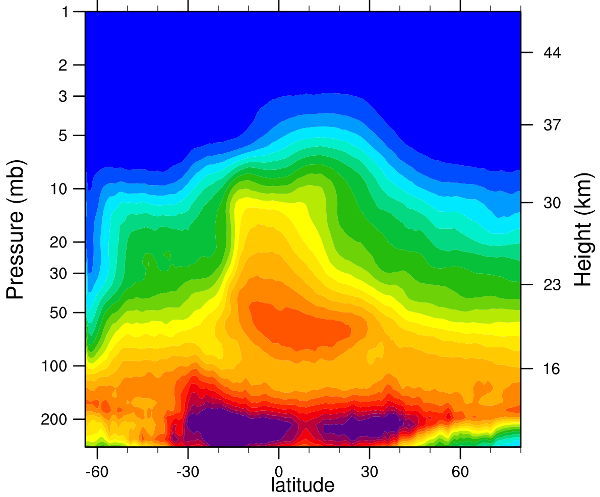
2005d241 N2O_Combined (ppbv)
