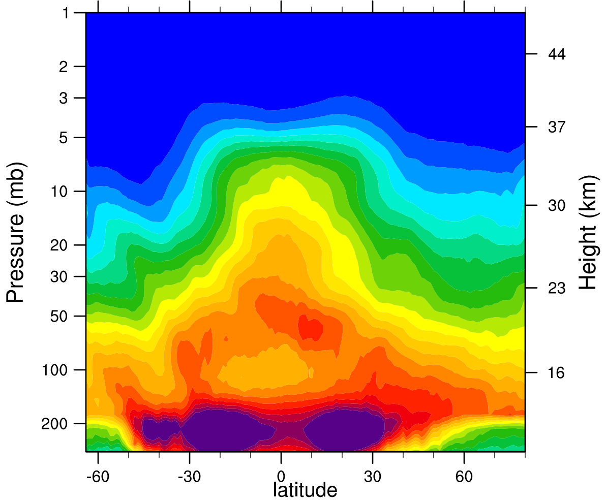
2005d102 N2O_Combined (ppbv)
