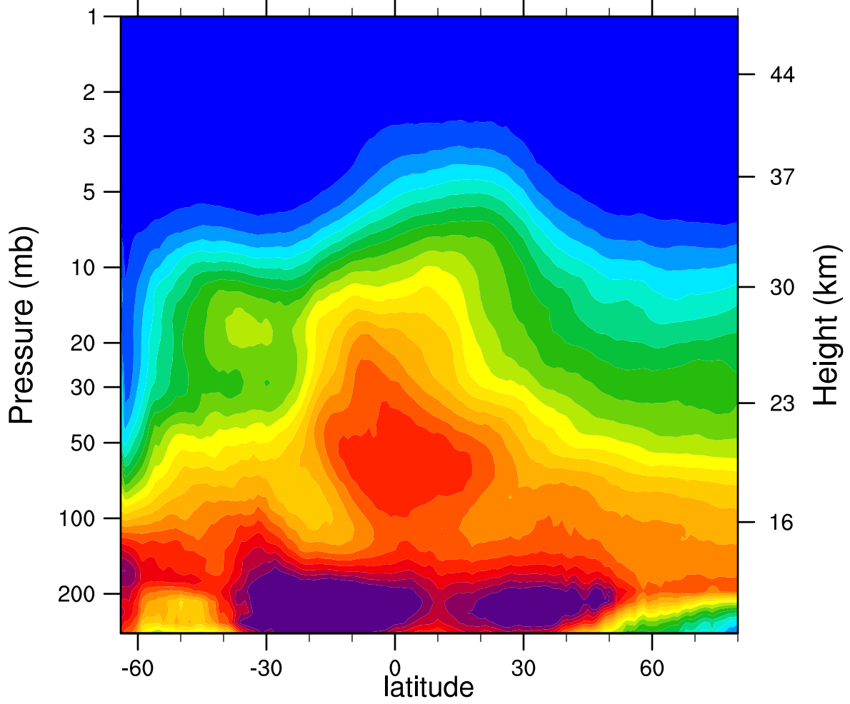
2007d218 N2O_Combined (ppbv)
