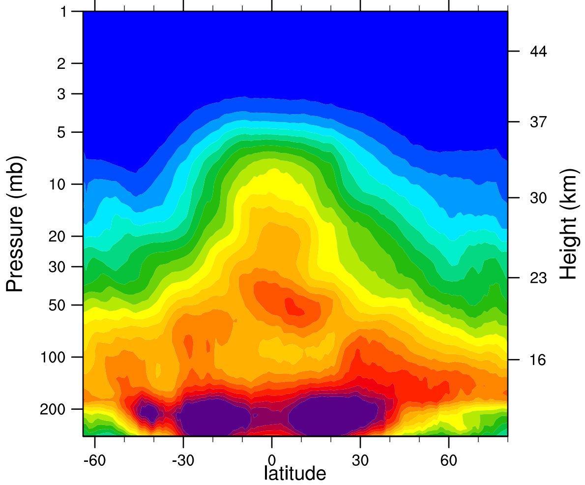
2005d079 N2O_Combined (ppbv)
