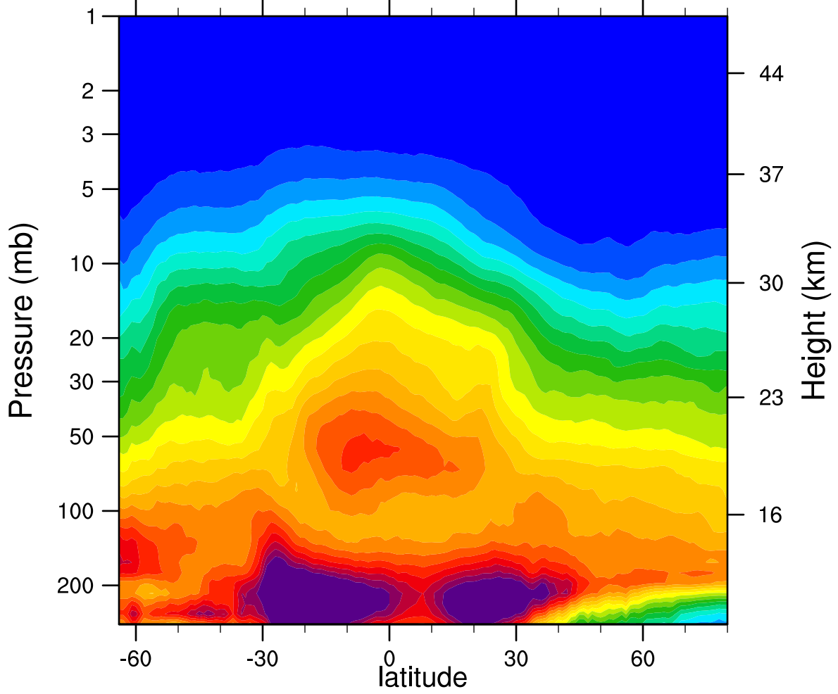
2006d156 N2O_Combined (ppbv)
