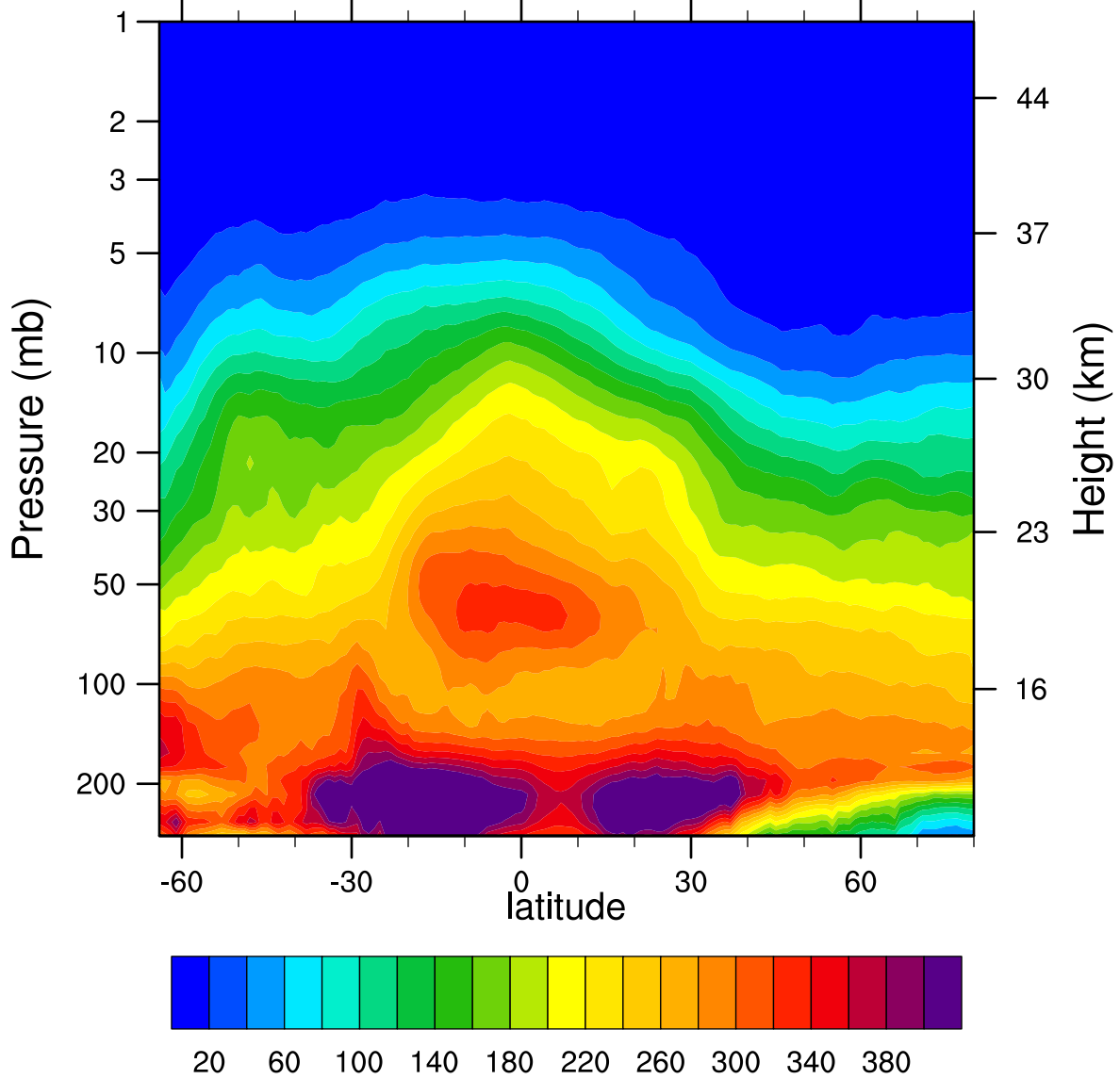
2006d150 N2O_Combined (ppbv)
