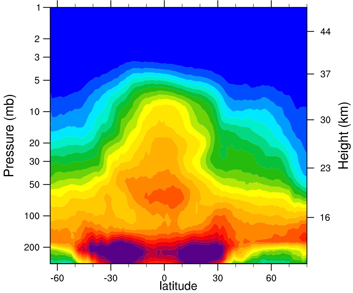
2007d070 N2O_Combined (ppbv)
