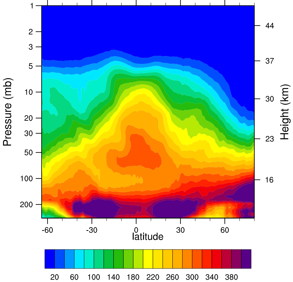
2006d341 N2O_Combined (ppbv)
