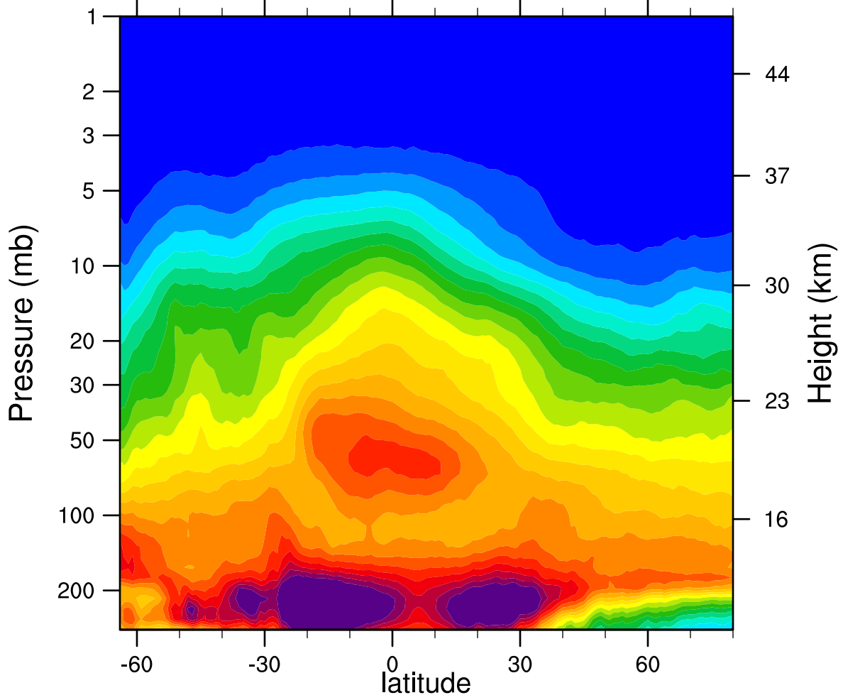
2006d143 N2O_Combined (ppbv)
