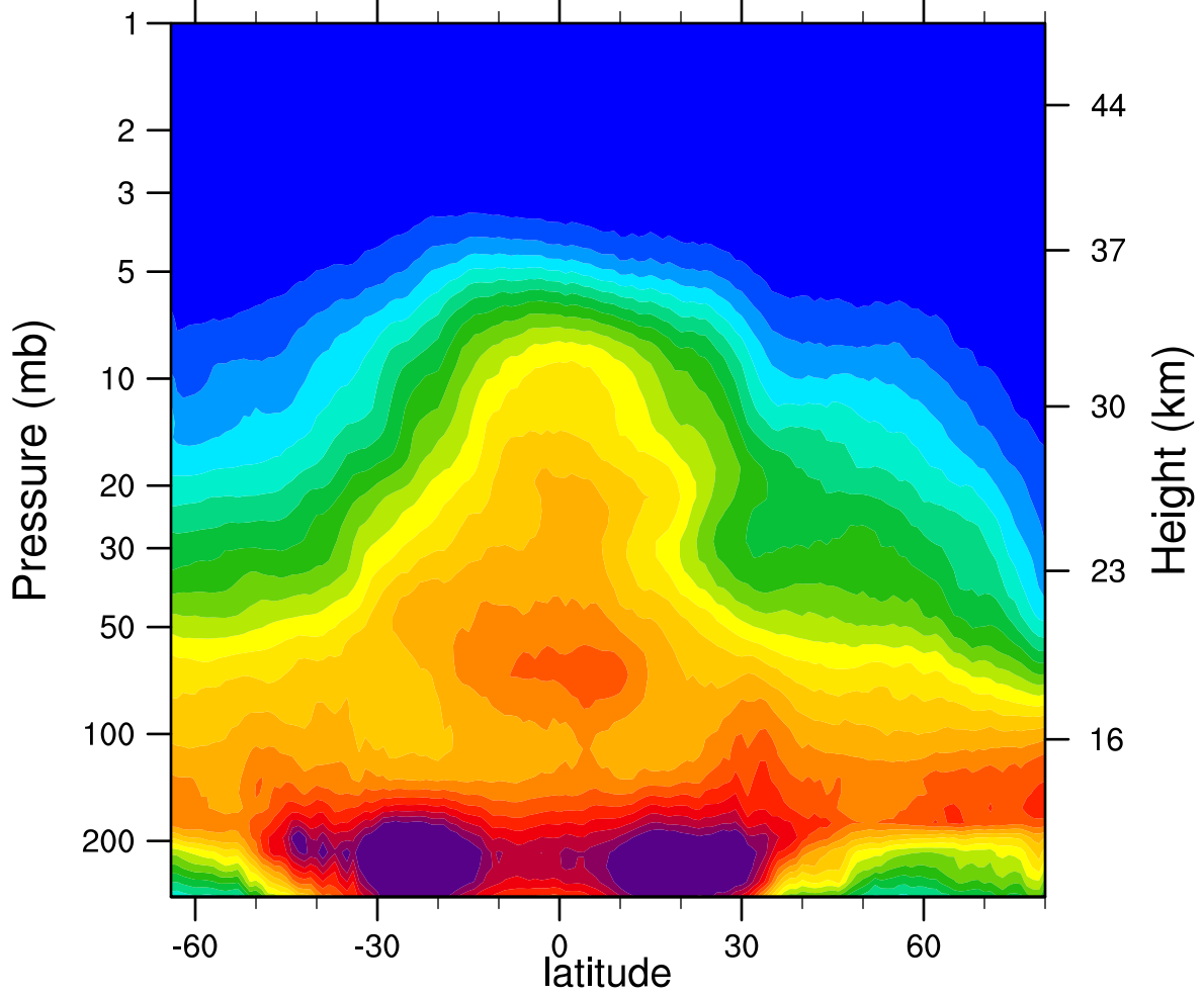
2007d067 N2O_Combined (ppbv)
