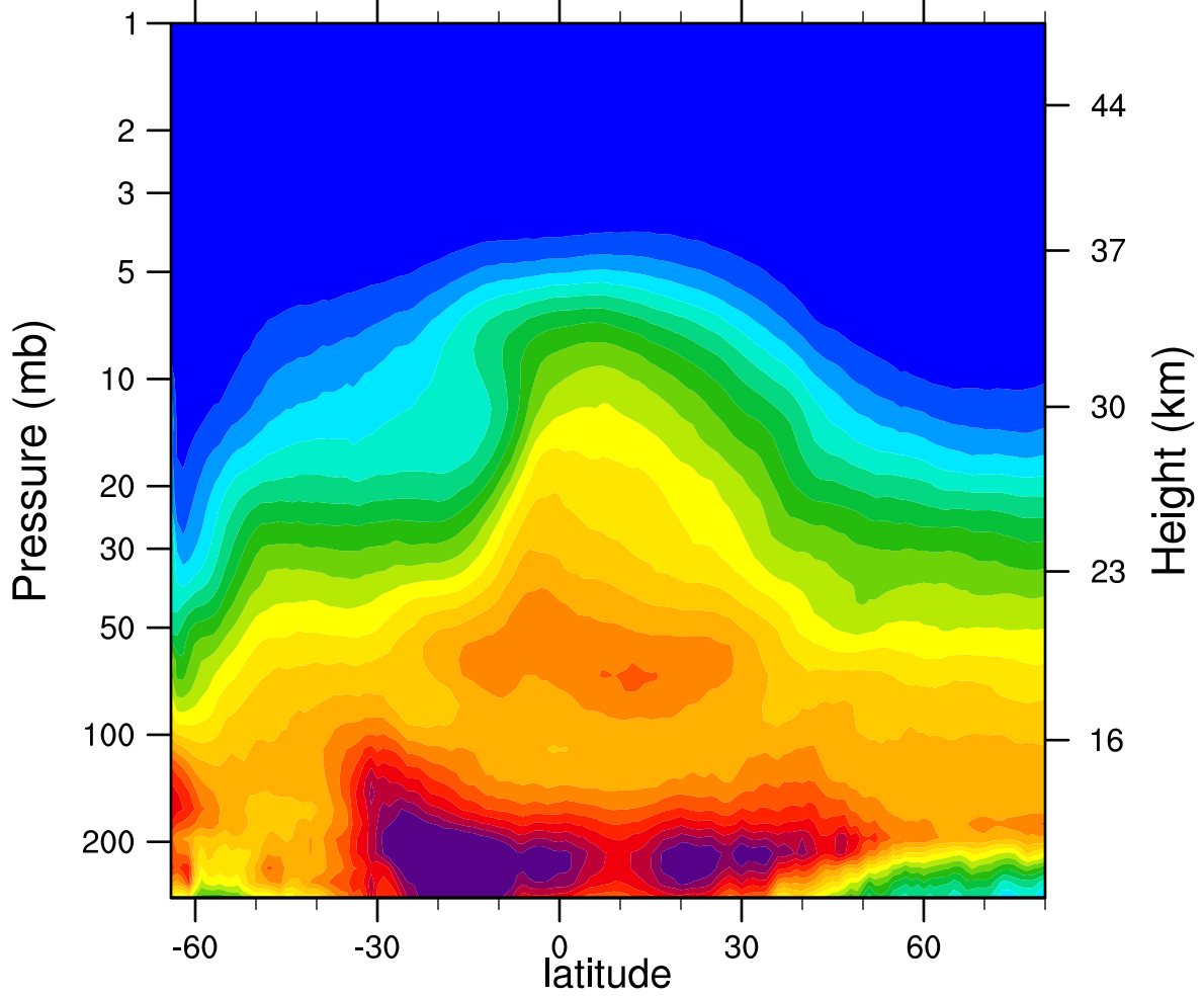
2006d248 N2O_Combined (ppbv)
