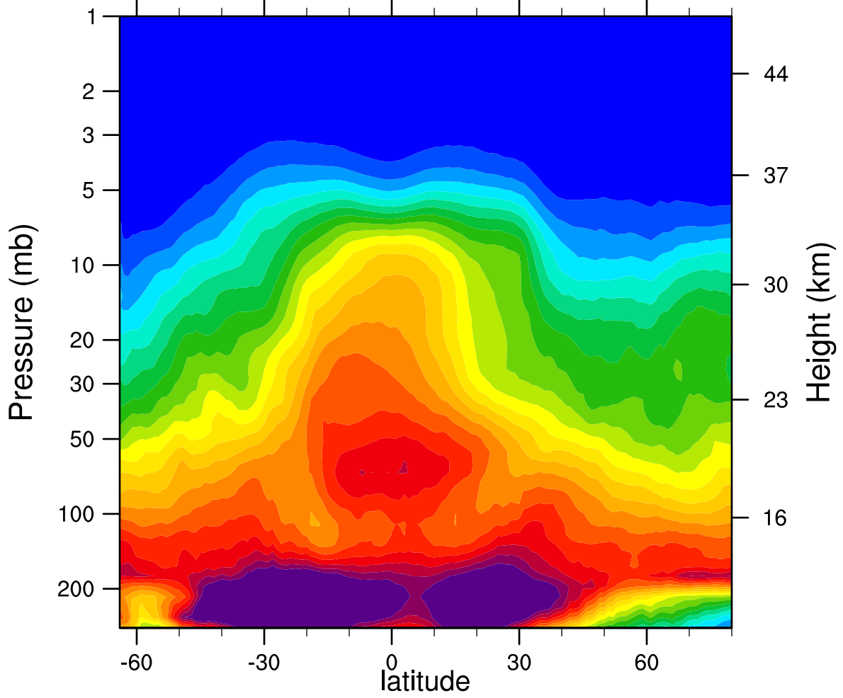
2007d124 N2O_Combined (ppbv)
