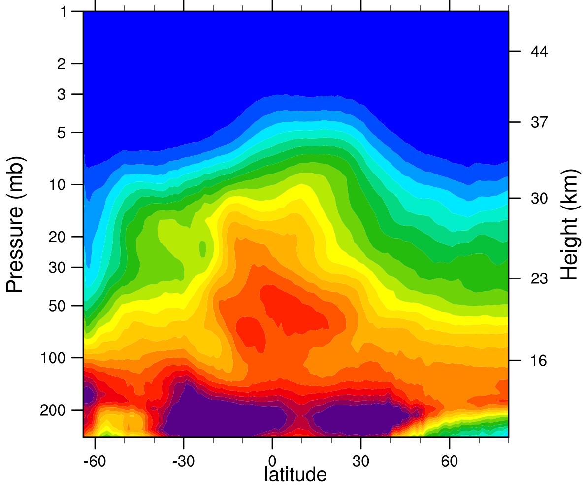
2007d241 N2O_Combined (ppbv)
