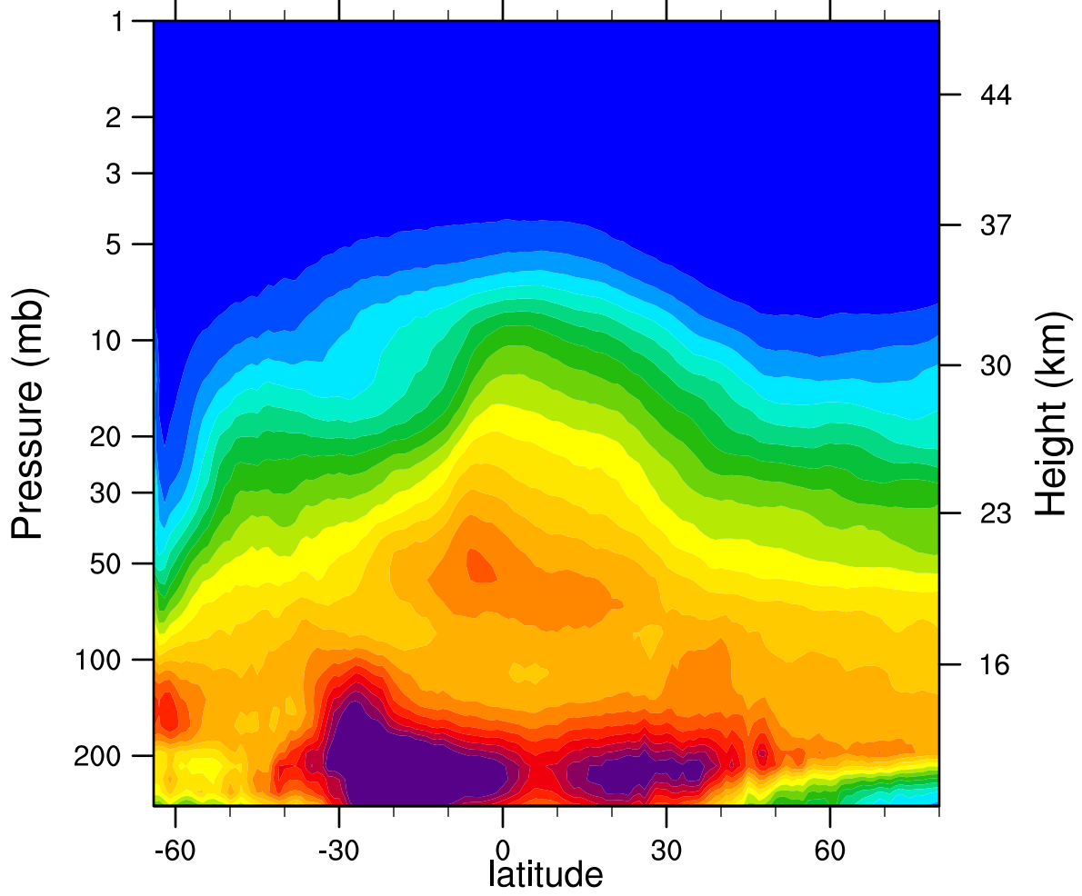
2006d198 N2O_Combined (ppbv)
