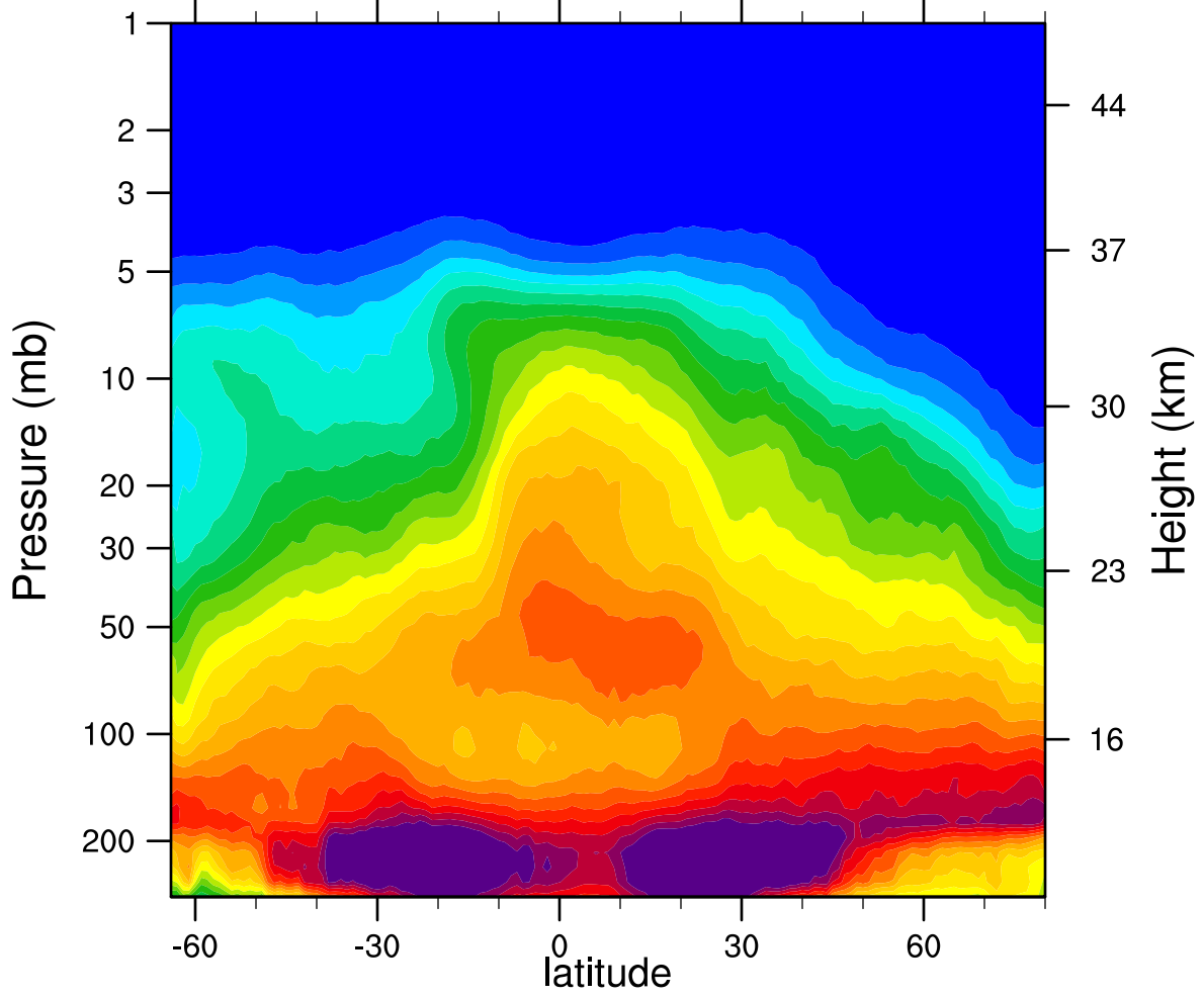
2006d314 N2O_Combined (ppbv)
