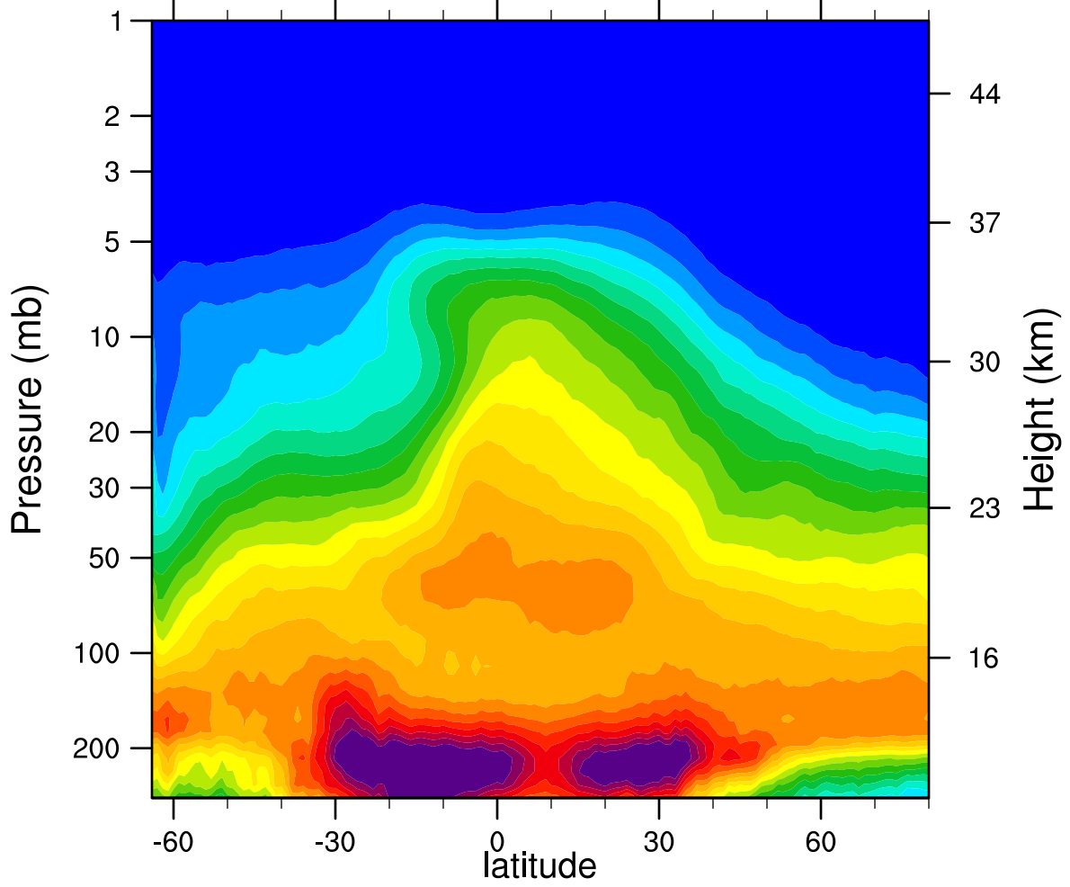
2006d273 N2O_Combined (ppbv)
