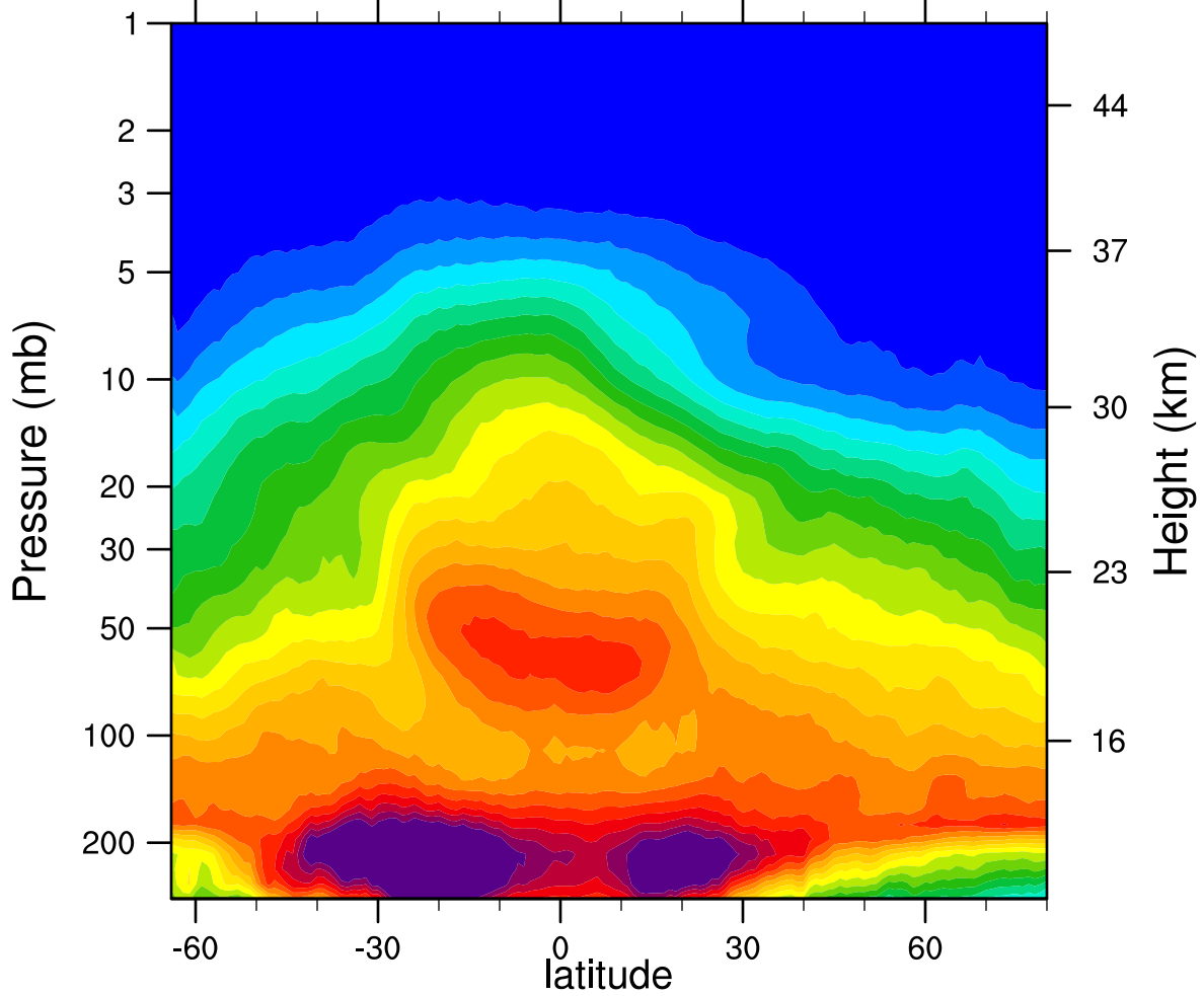
2006d117 N2O_Combined (ppbv)
