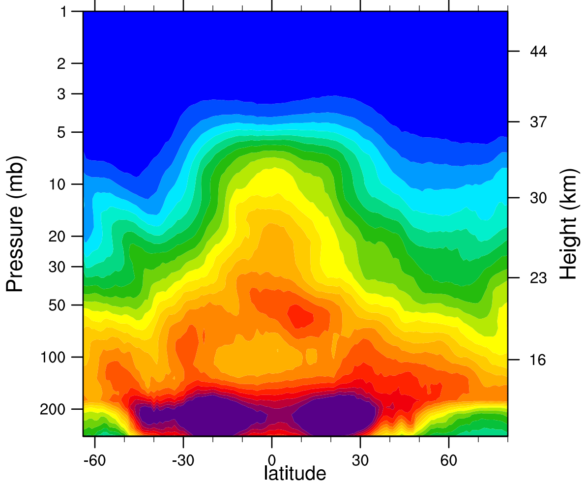
2005d098 N2O_Combined (ppbv)
