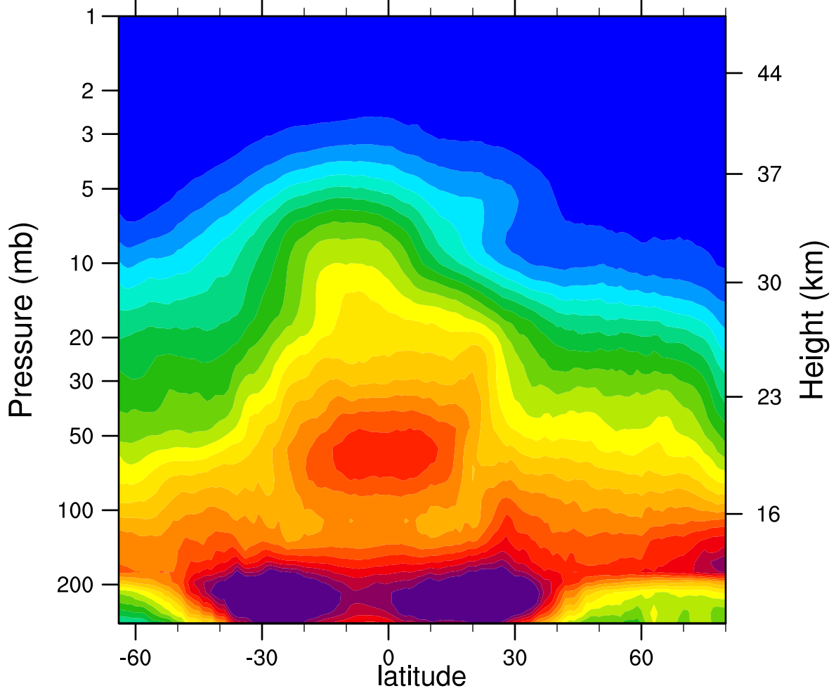
2006d069 N2O_Combined (ppbv)
