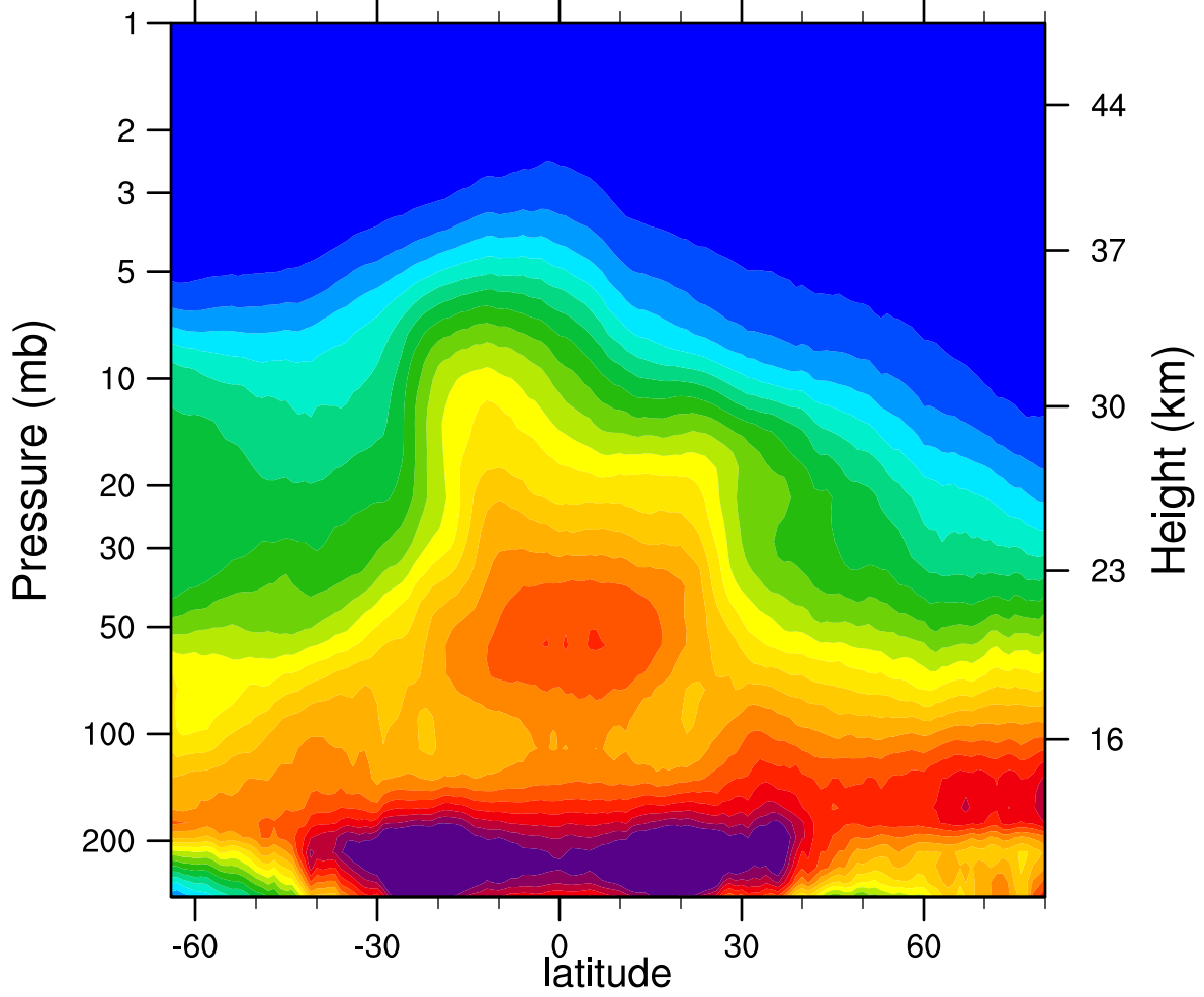
2005d353 N2O_Combined (ppbv)
