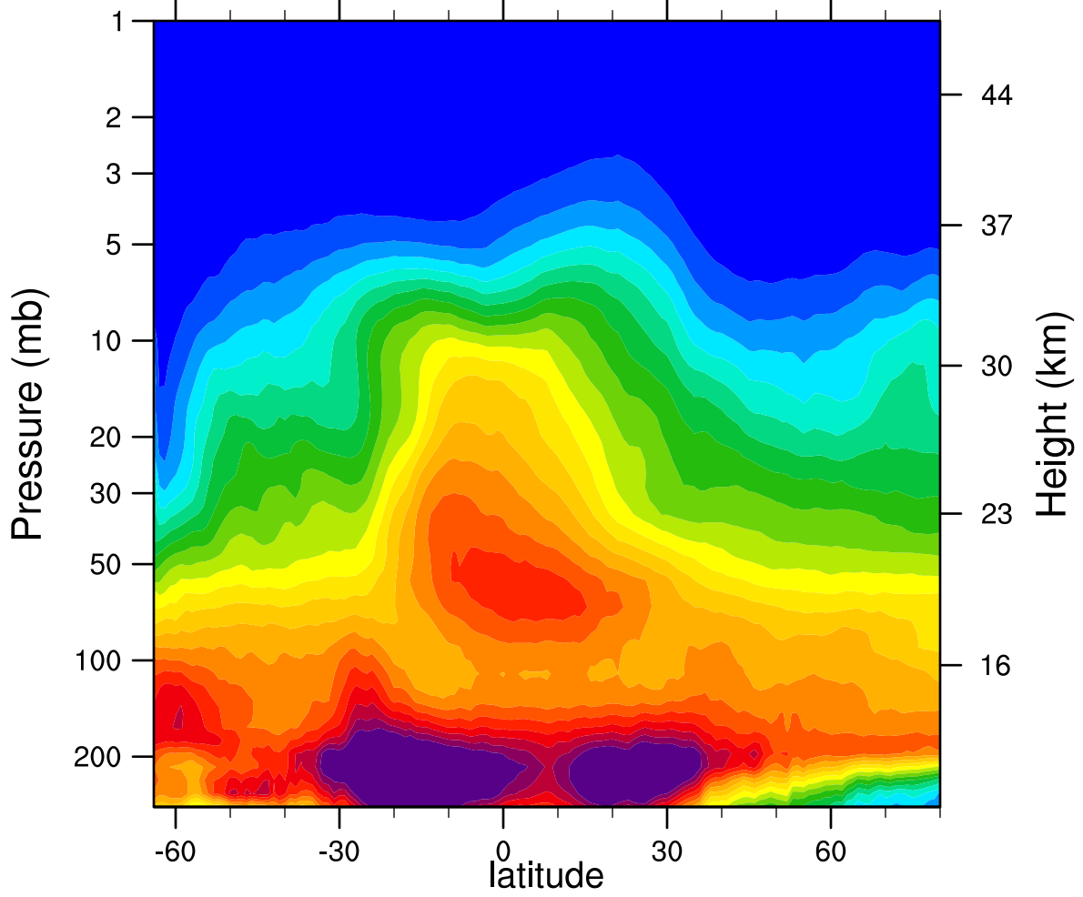
2005d166 N2O_Combined (ppbv)
