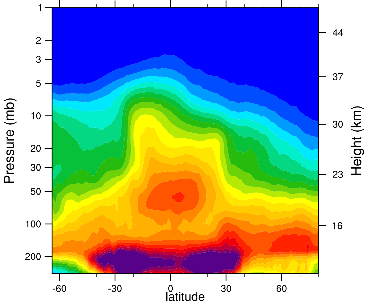
2005d345 N2O_Combined (ppbv)
