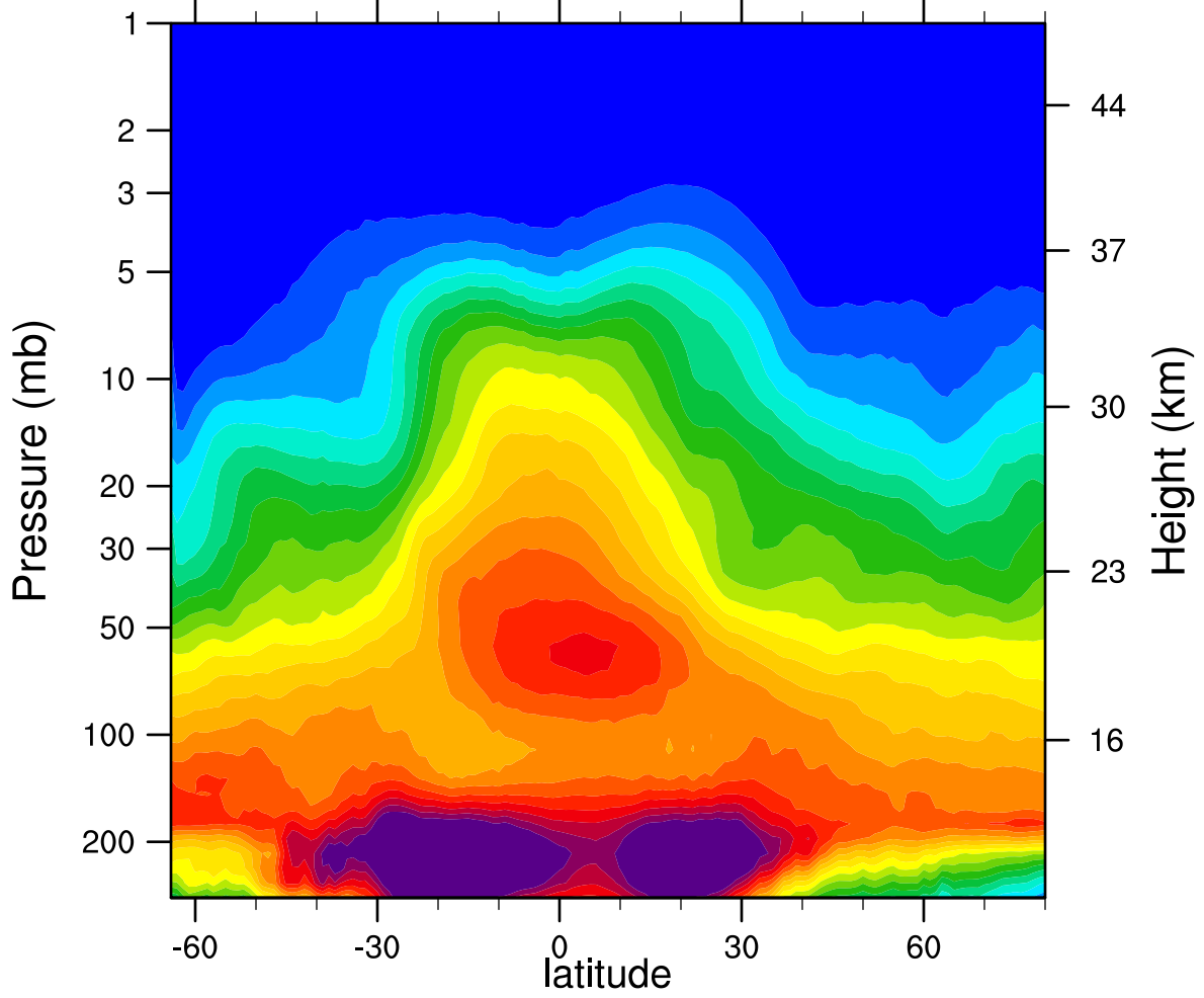
2005d131 N2O_Combined (ppbv)
