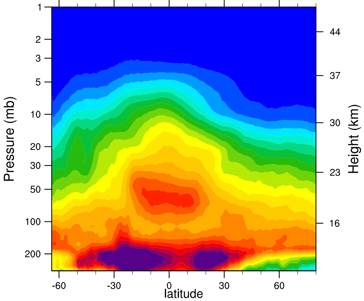
2006d130 N2O_Combined (ppbv)
