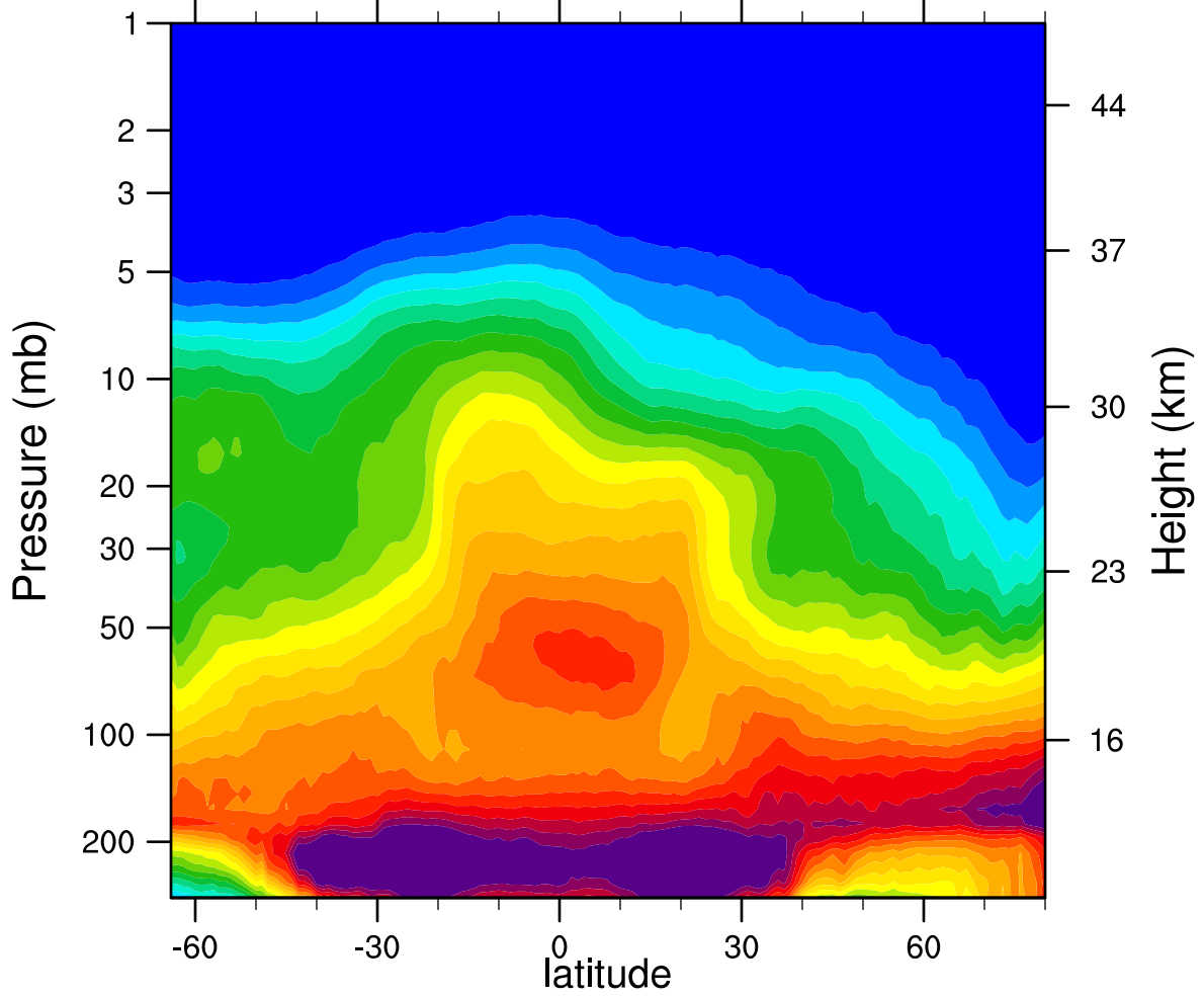
2007d351 N2O_Combined (ppbv)
