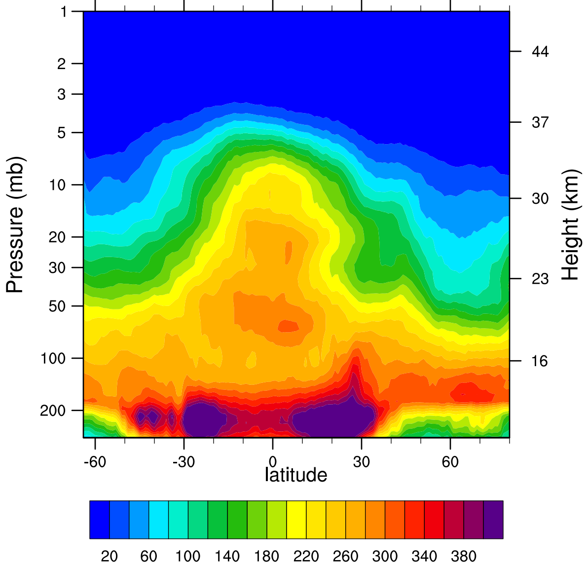
2007d056 N2O_Combined (ppbv)
