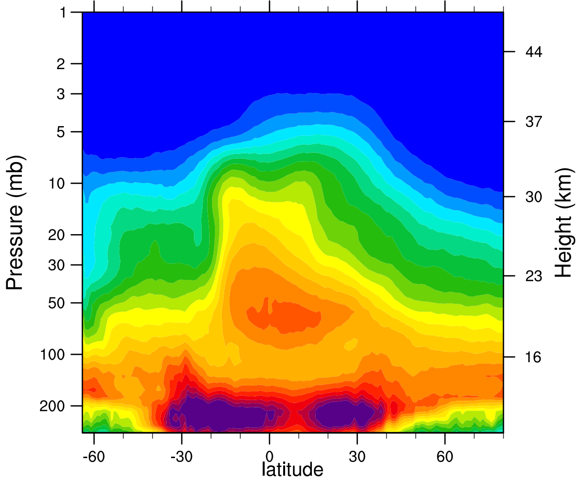
2005d270 N2O_Combined (ppbv)
