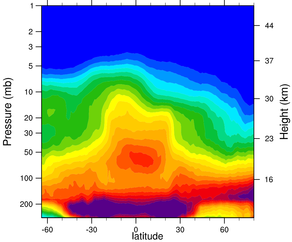
2007d355 N2O_Combined (ppbv)
