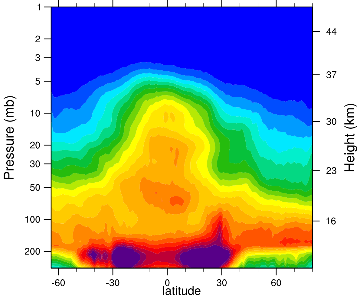
2007d058 N2O_Combined (ppbv)
