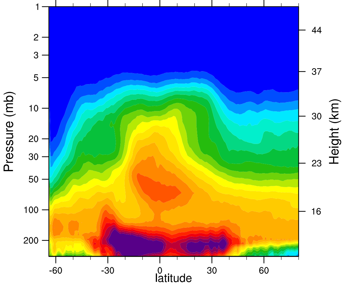
2007d182 N2O_Combined (ppbv)
