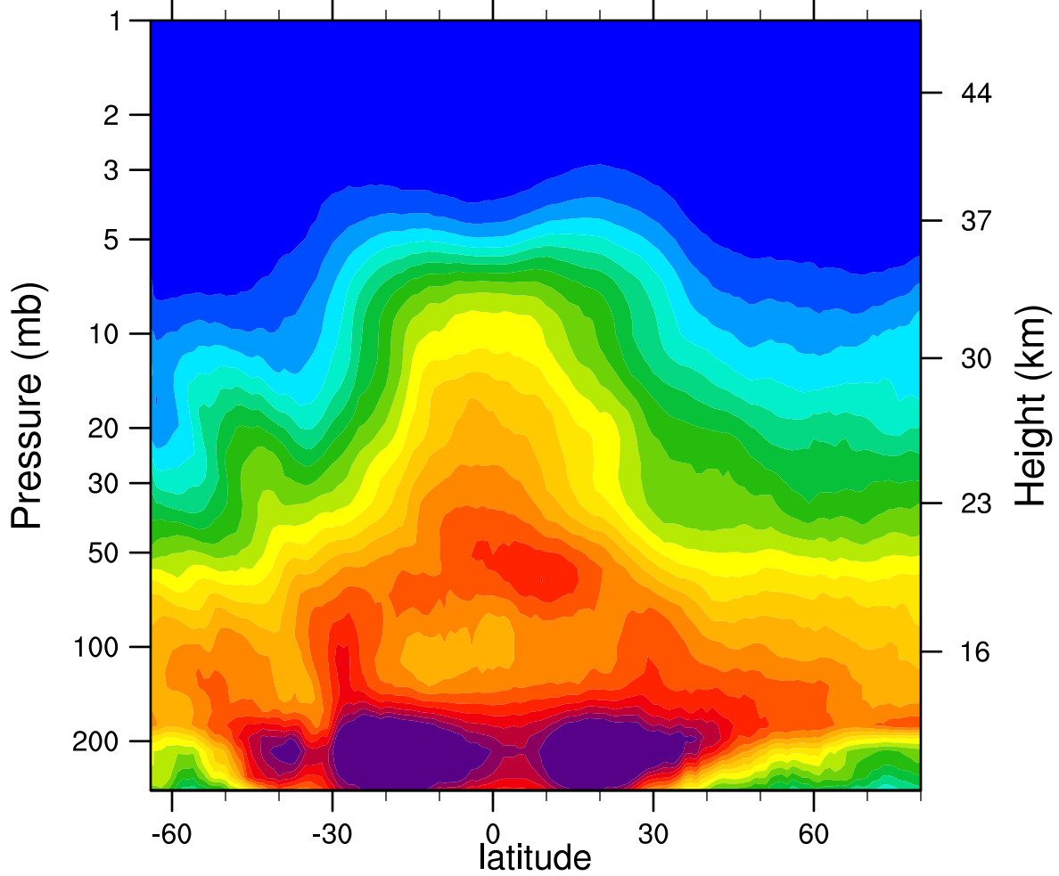
2005d114 N2O_Combined (ppbv)
