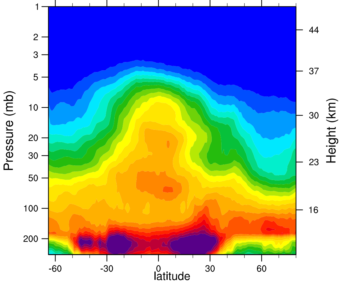
2007d055 N2O_Combined (ppbv)
