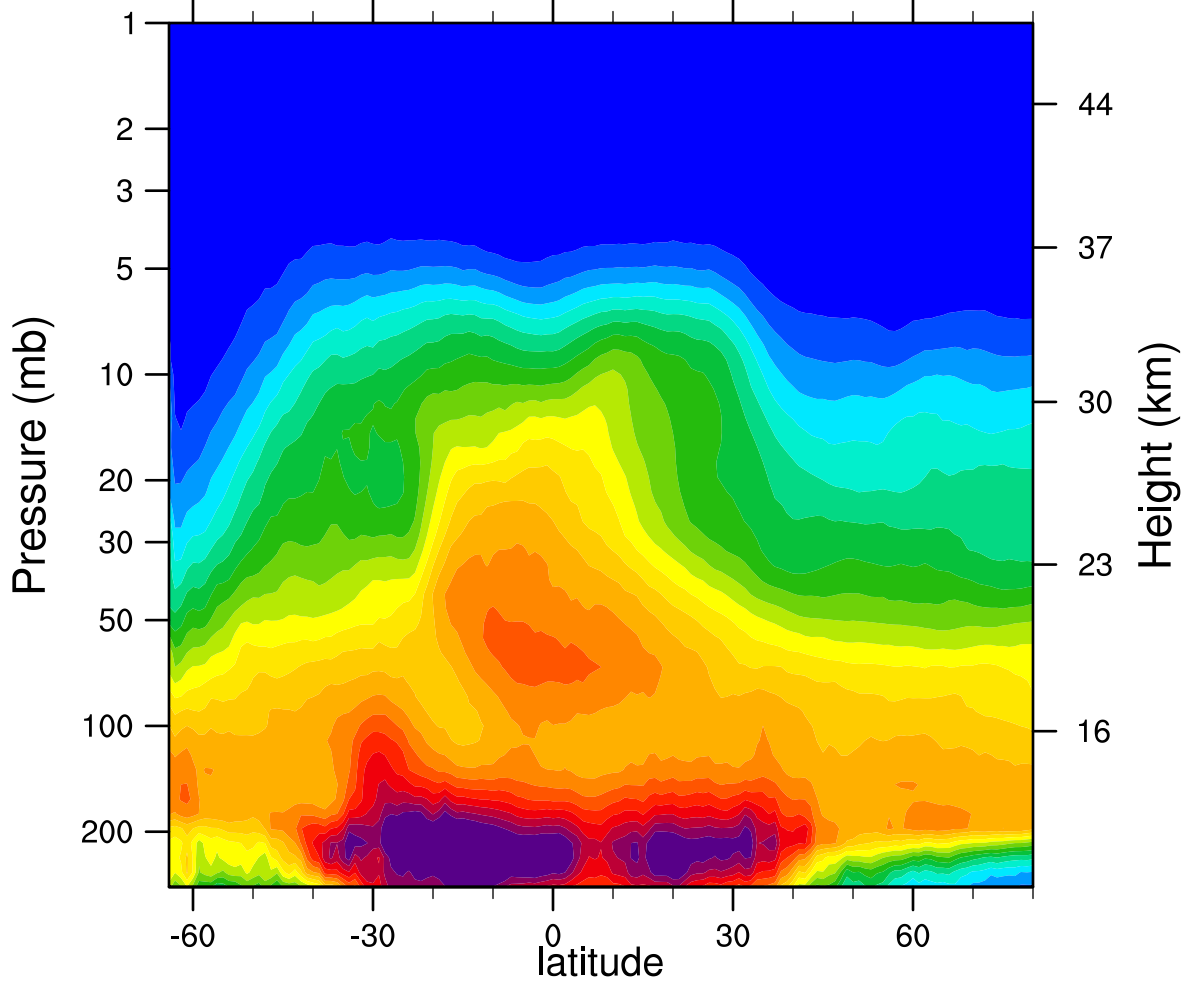
2007d170 N2O_Combined (ppbv)
