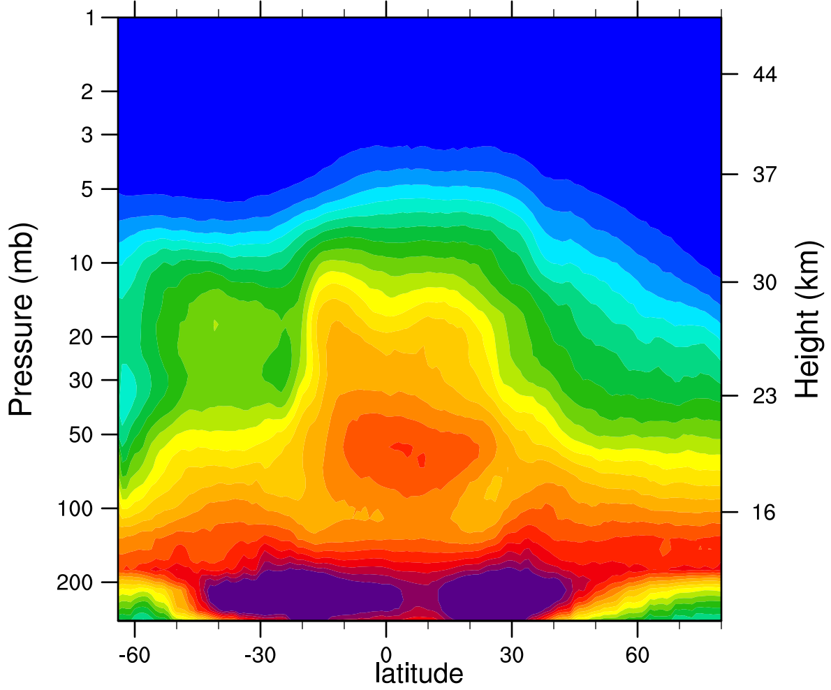
2007d298 N2O_Combined (ppbv)
