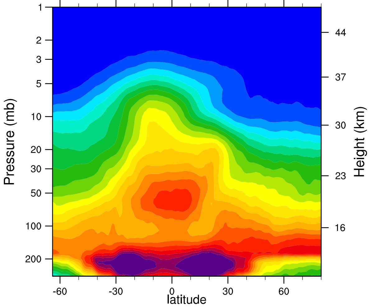
2006d053 N2O_Combined (ppbv)
