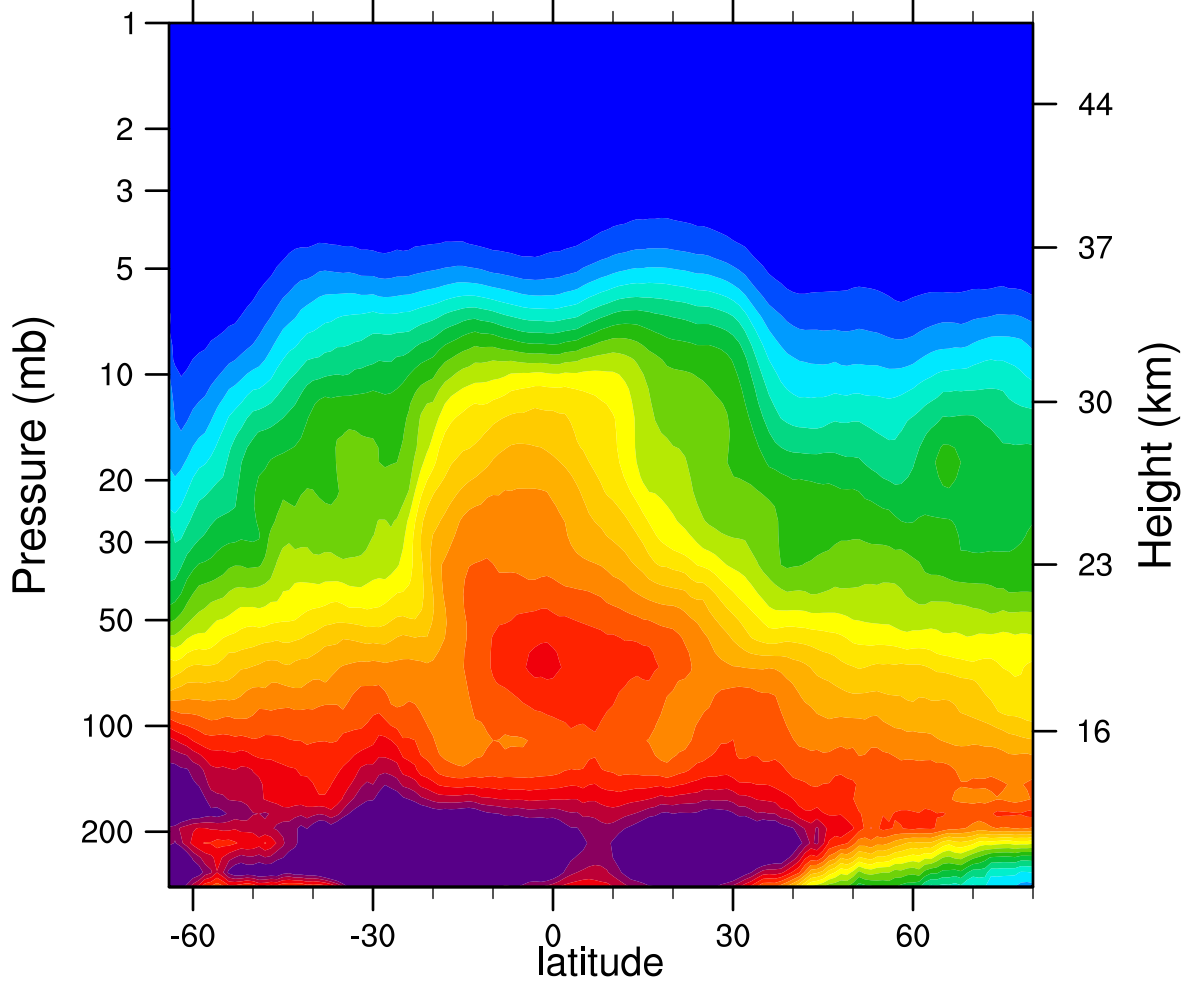
2007d152 N2O_Combined (ppbv)
