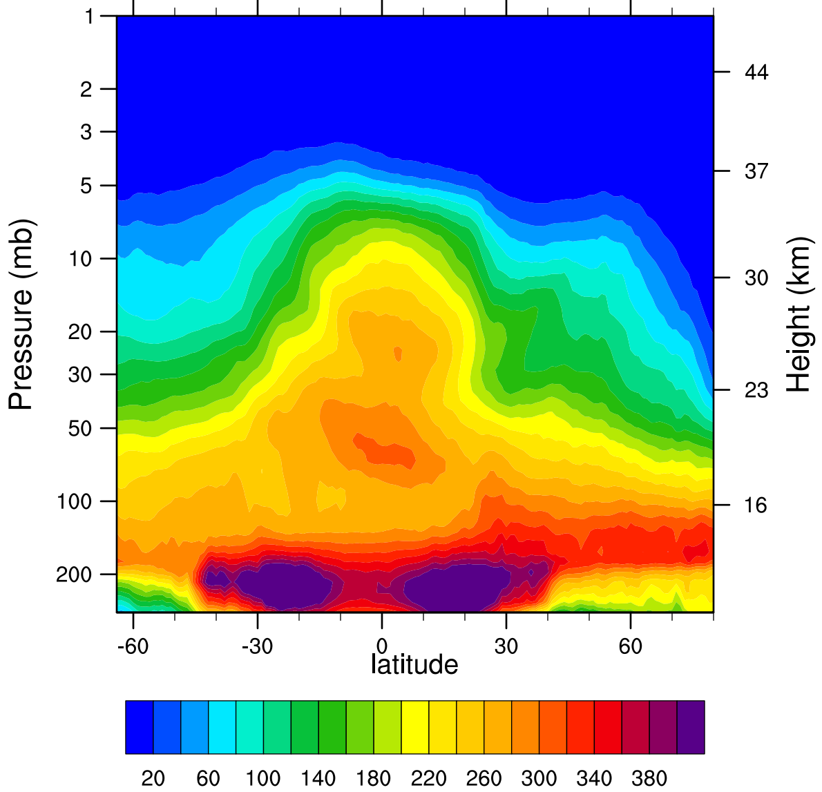
2007d031 N2O_Combined (ppbv)
