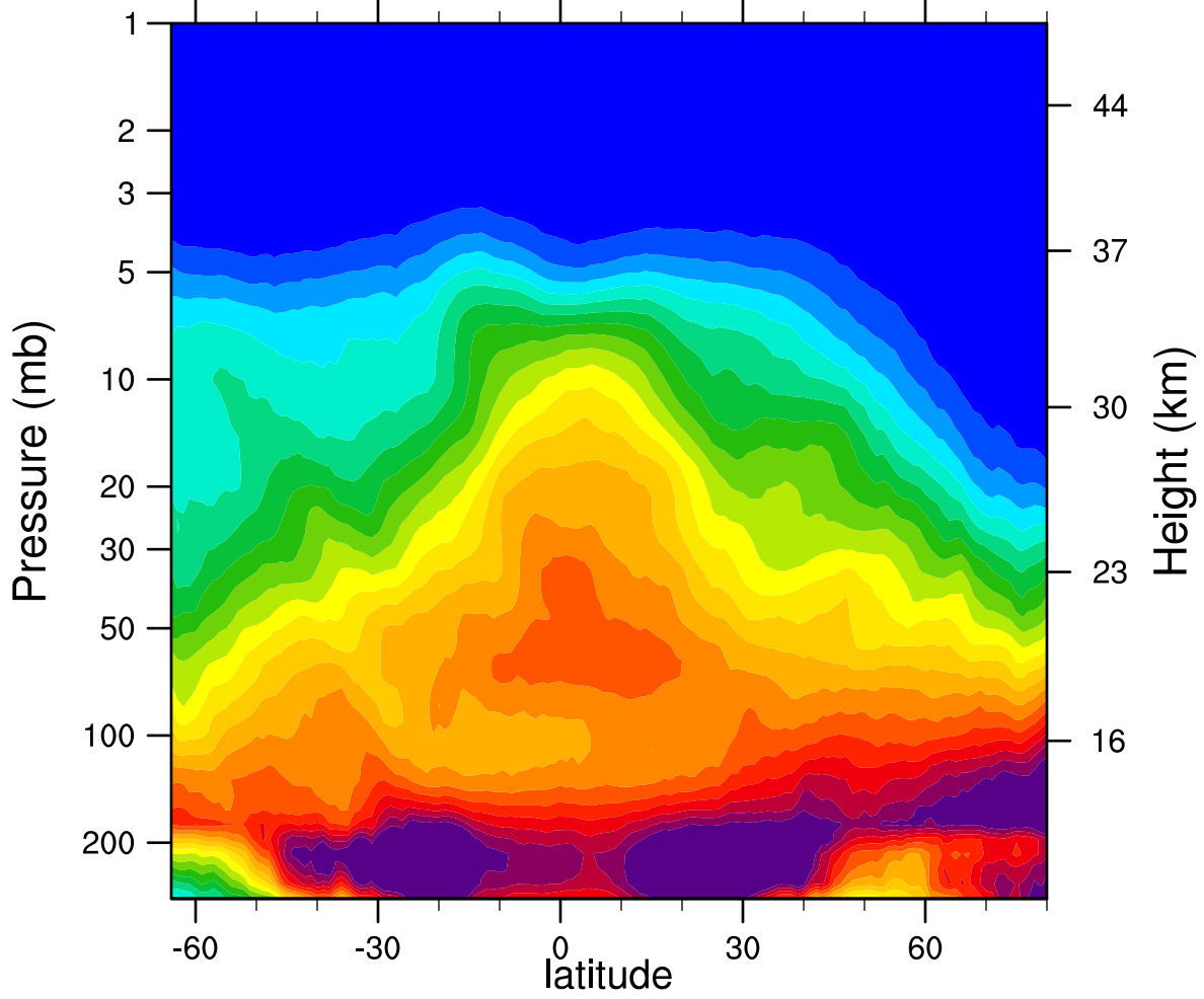
2006d338 N2O_Combined (ppbv)
