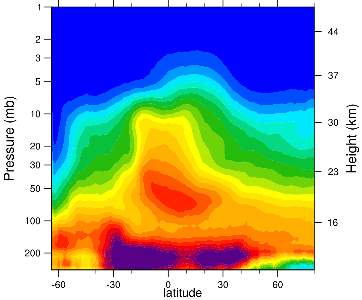
2005d209 N2O_Combined (ppbv)
