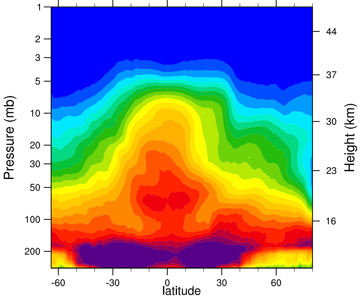
2007d105 N2O_Combined (ppbv)
