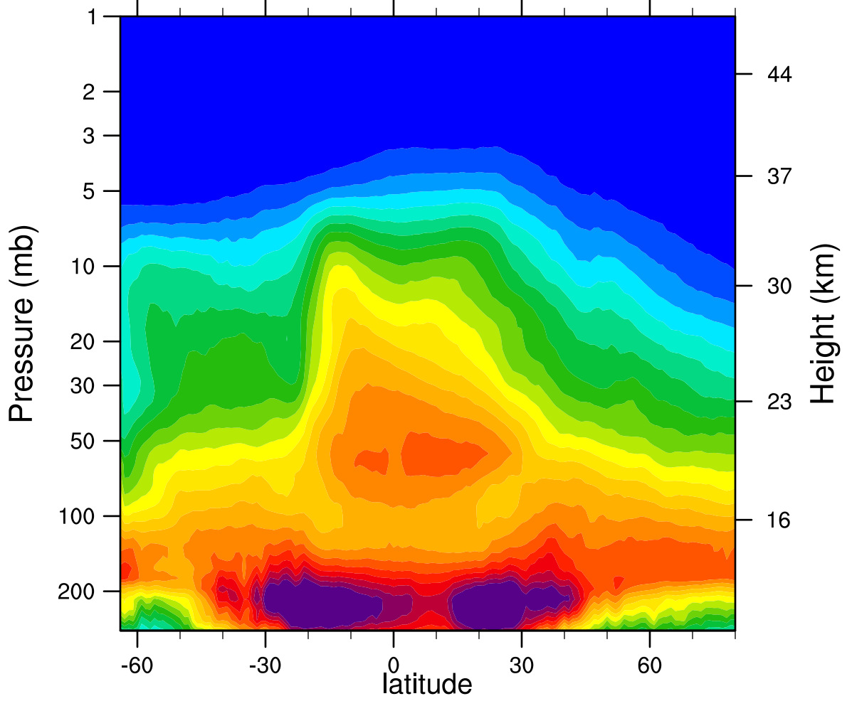
2005d296 N2O_Combined (ppbv)
