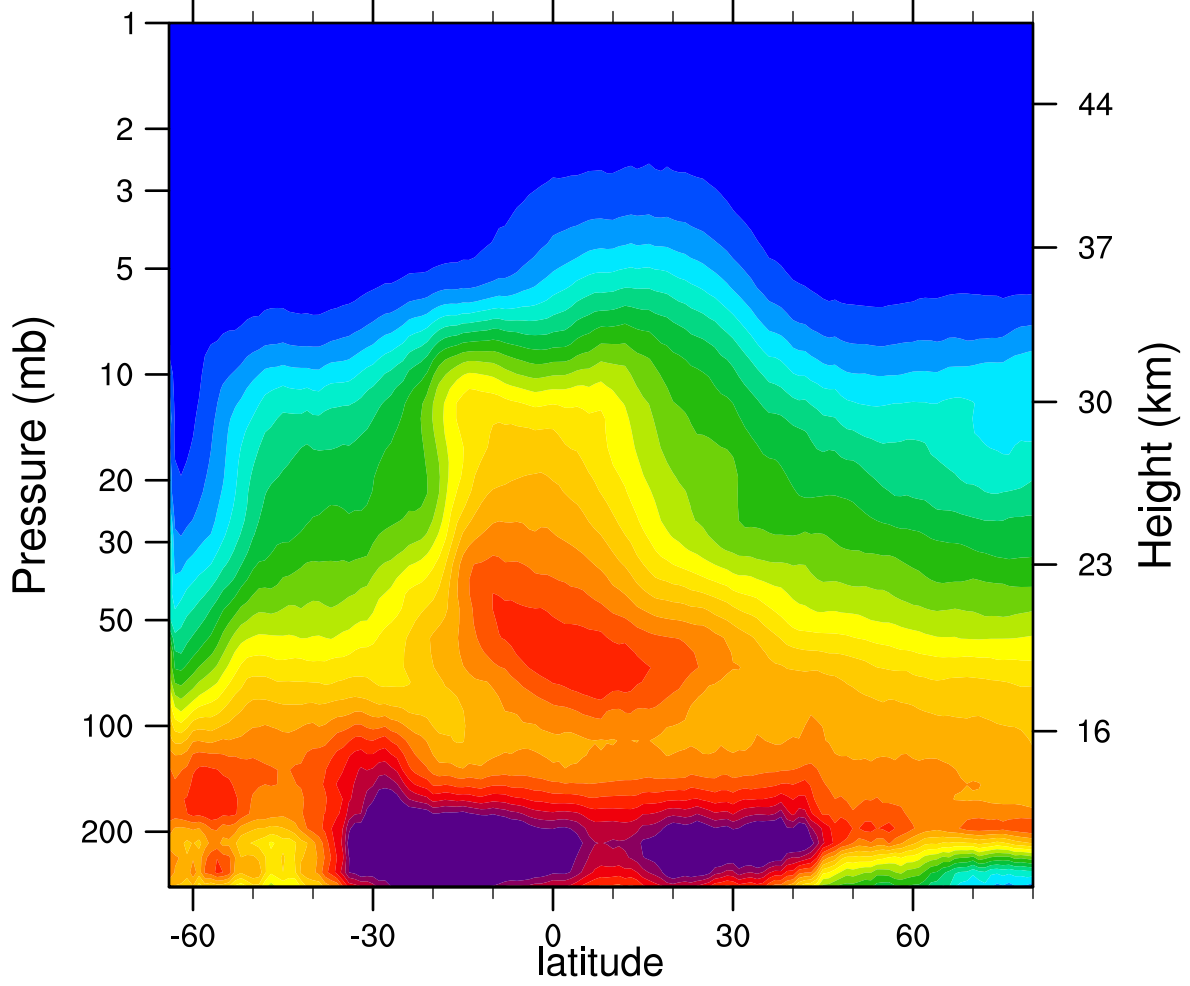
2005d208 N2O_Combined (ppbv)
