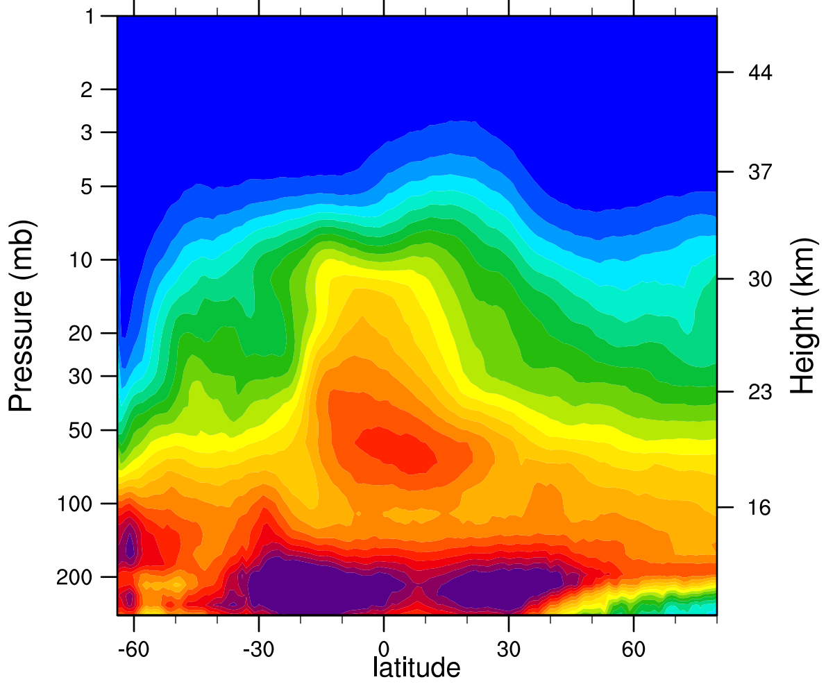
2005d184 N2O_Combined (ppbv)
