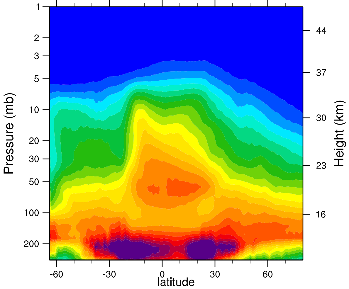
2005d295 N2O_Combined (ppbv)
