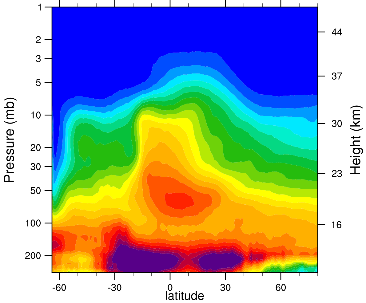
2005d224 N2O_Combined (ppbv)
