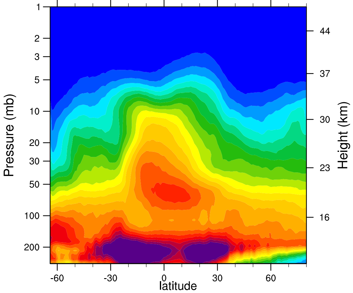
2005d162 N2O_Combined (ppbv)
