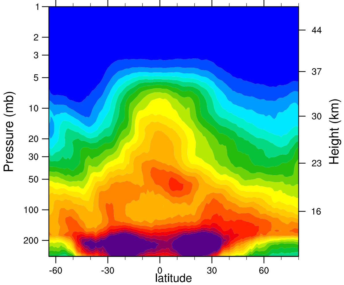
2005d094 N2O_Combined (ppbv)
