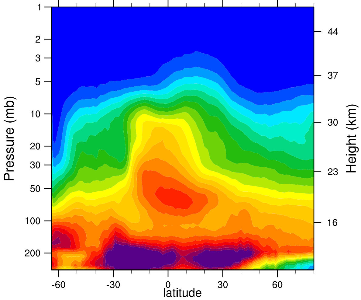
2005d191 N2O_Combined (ppbv)
