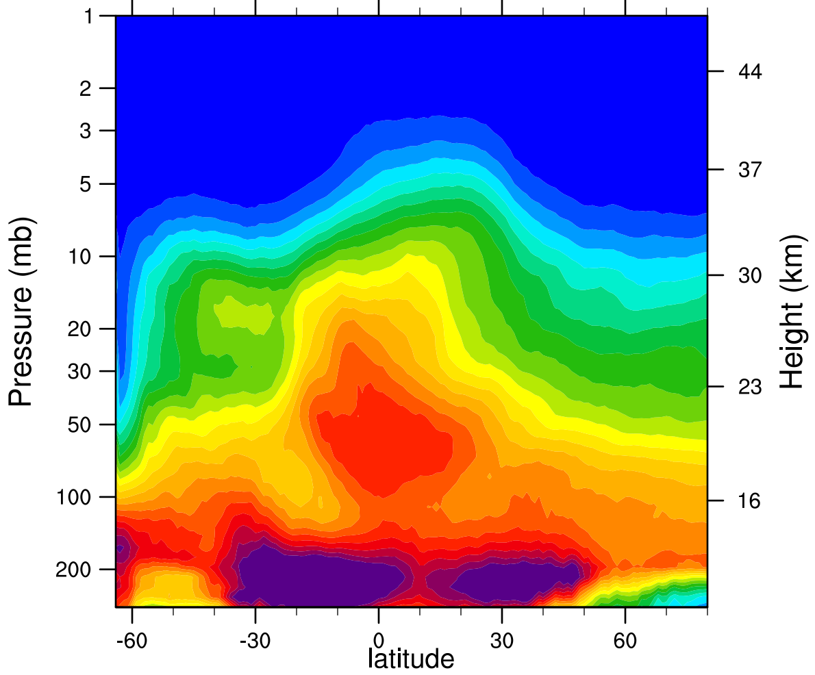
2007d217 N2O_Combined (ppbv)
