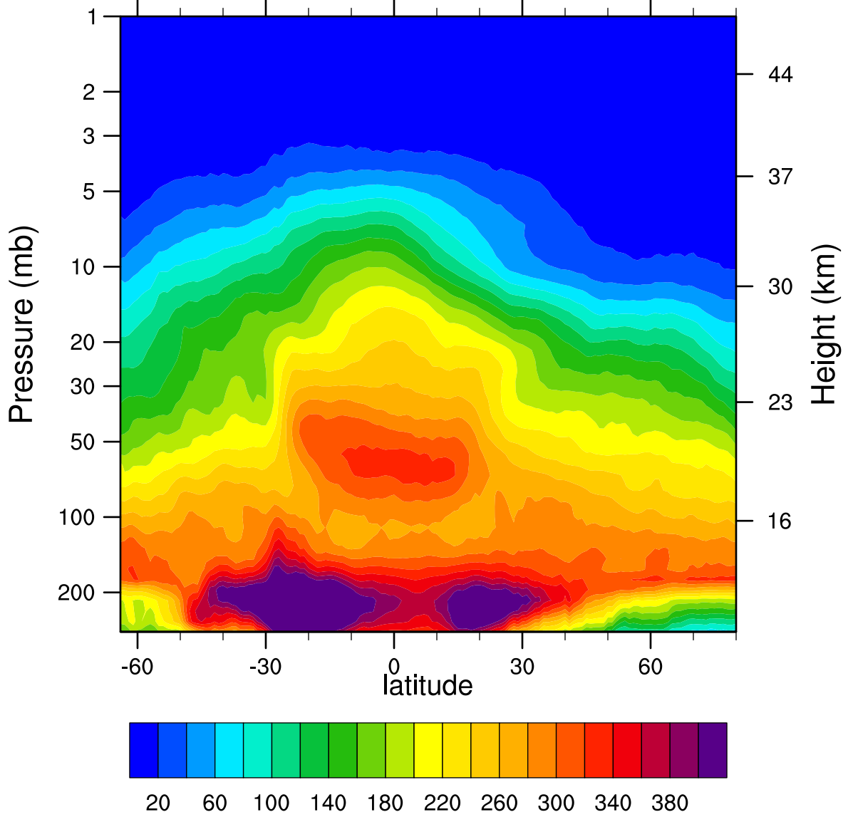
2006d122 N2O_Combined (ppbv)
