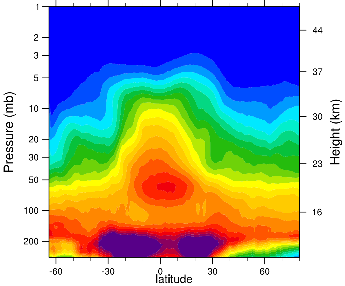
2005d137 N2O_Combined (ppbv)
