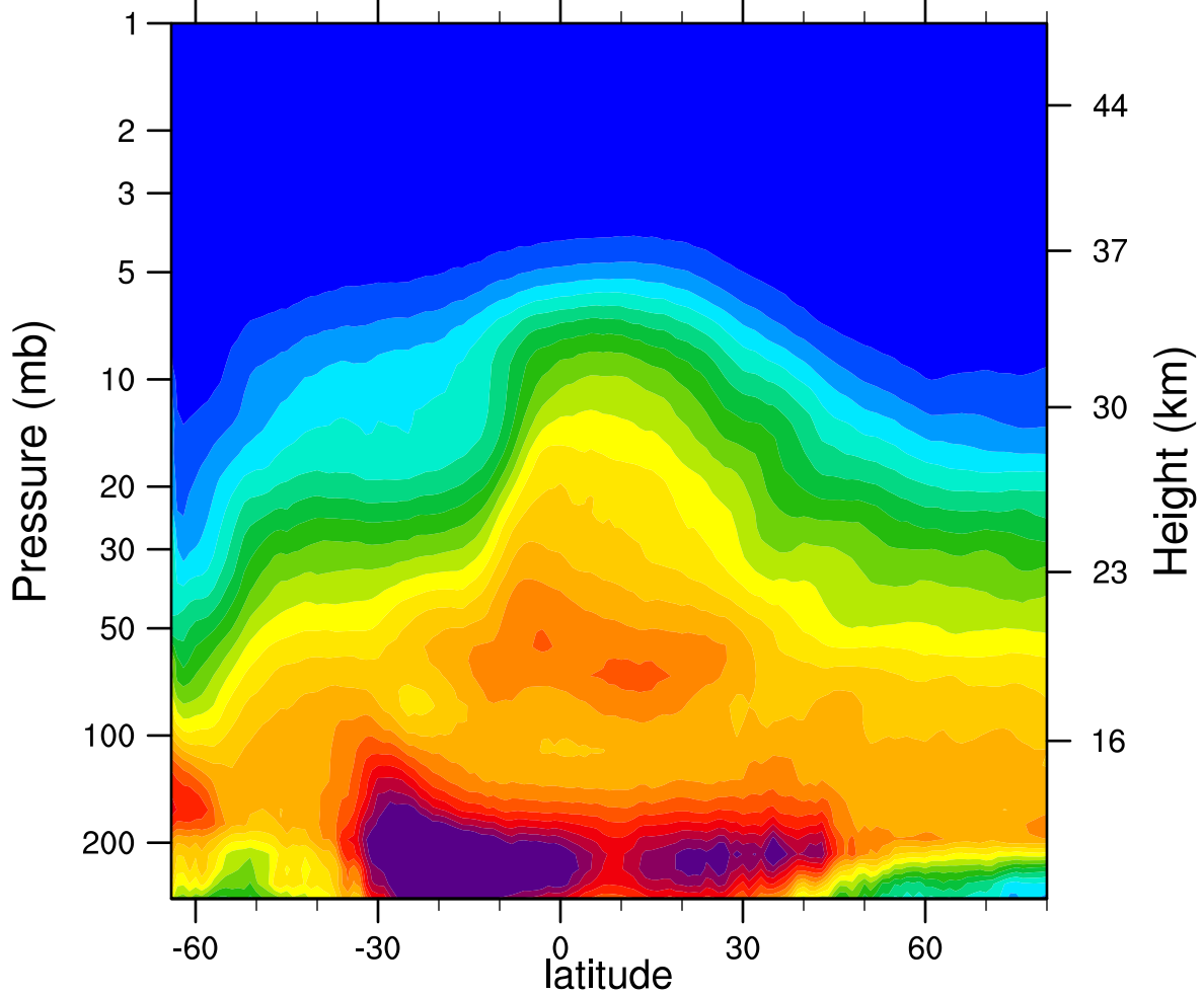
2006d233 N2O_Combined (ppbv)
