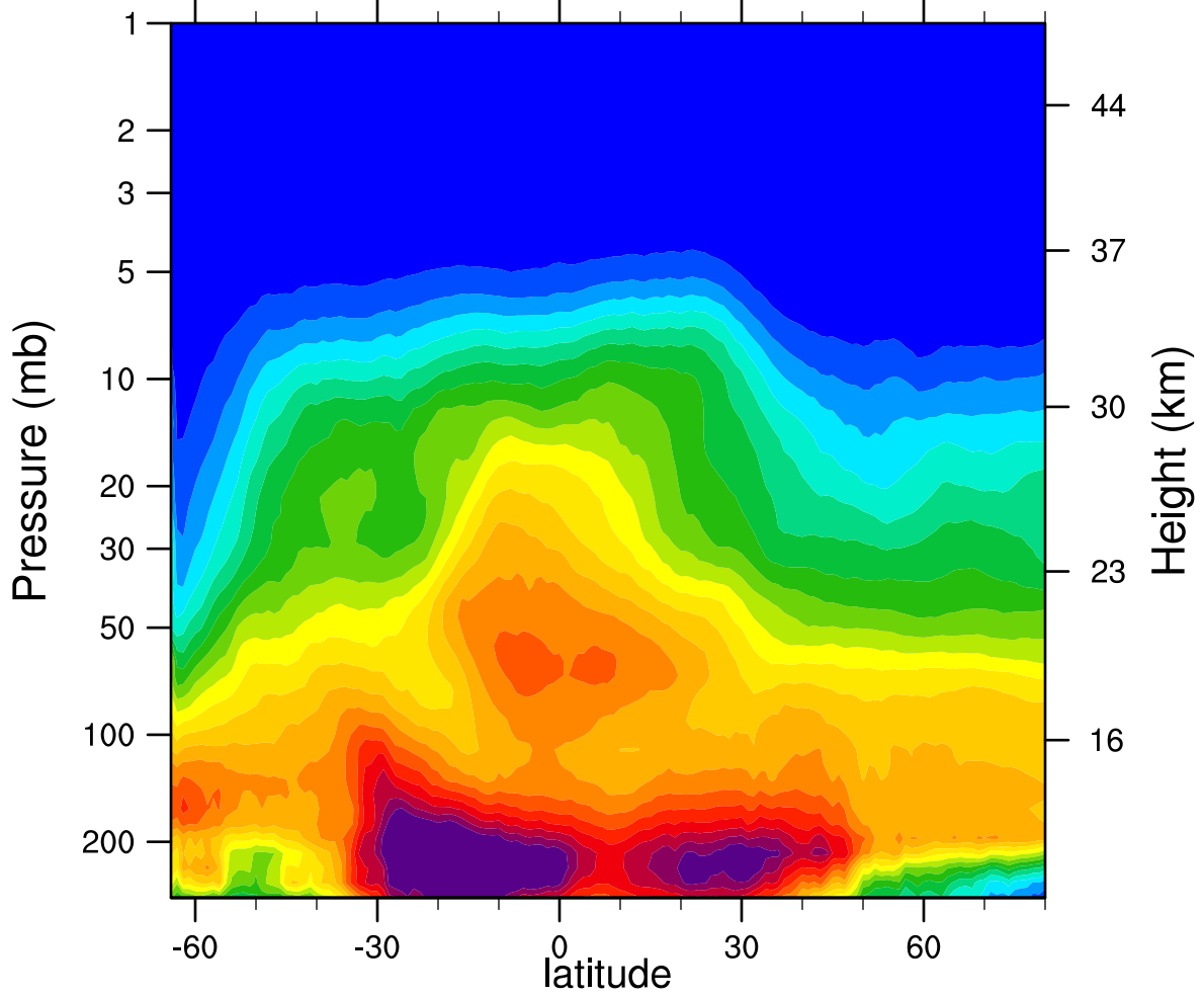
2007d200 N2O_Combined (ppbv)
