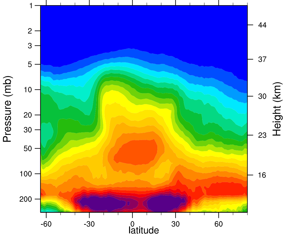
2005d330 N2O_Combined (ppbv)
