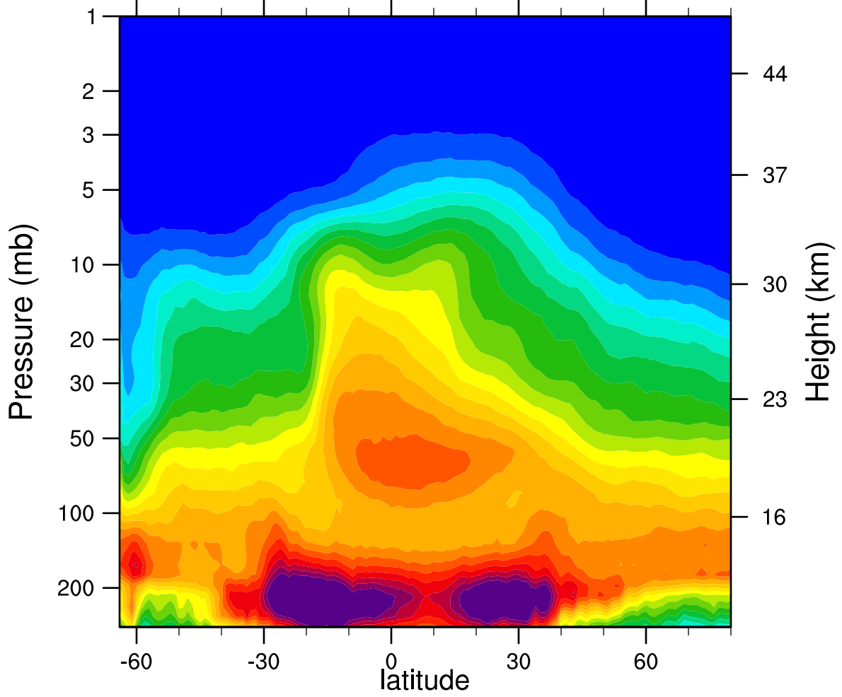
2005d265 N2O_Combined (ppbv)
