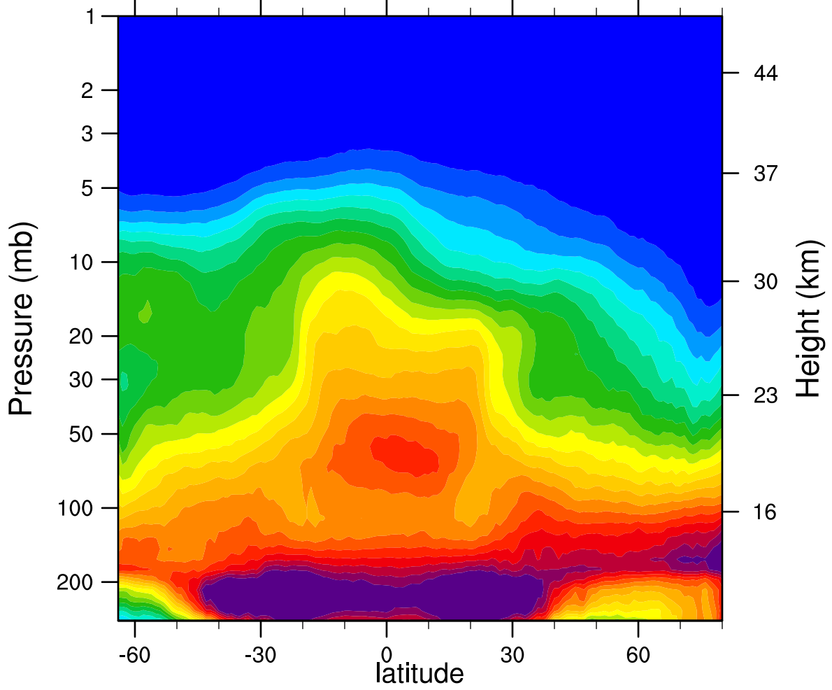
2007d350 N2O_Combined (ppbv)
