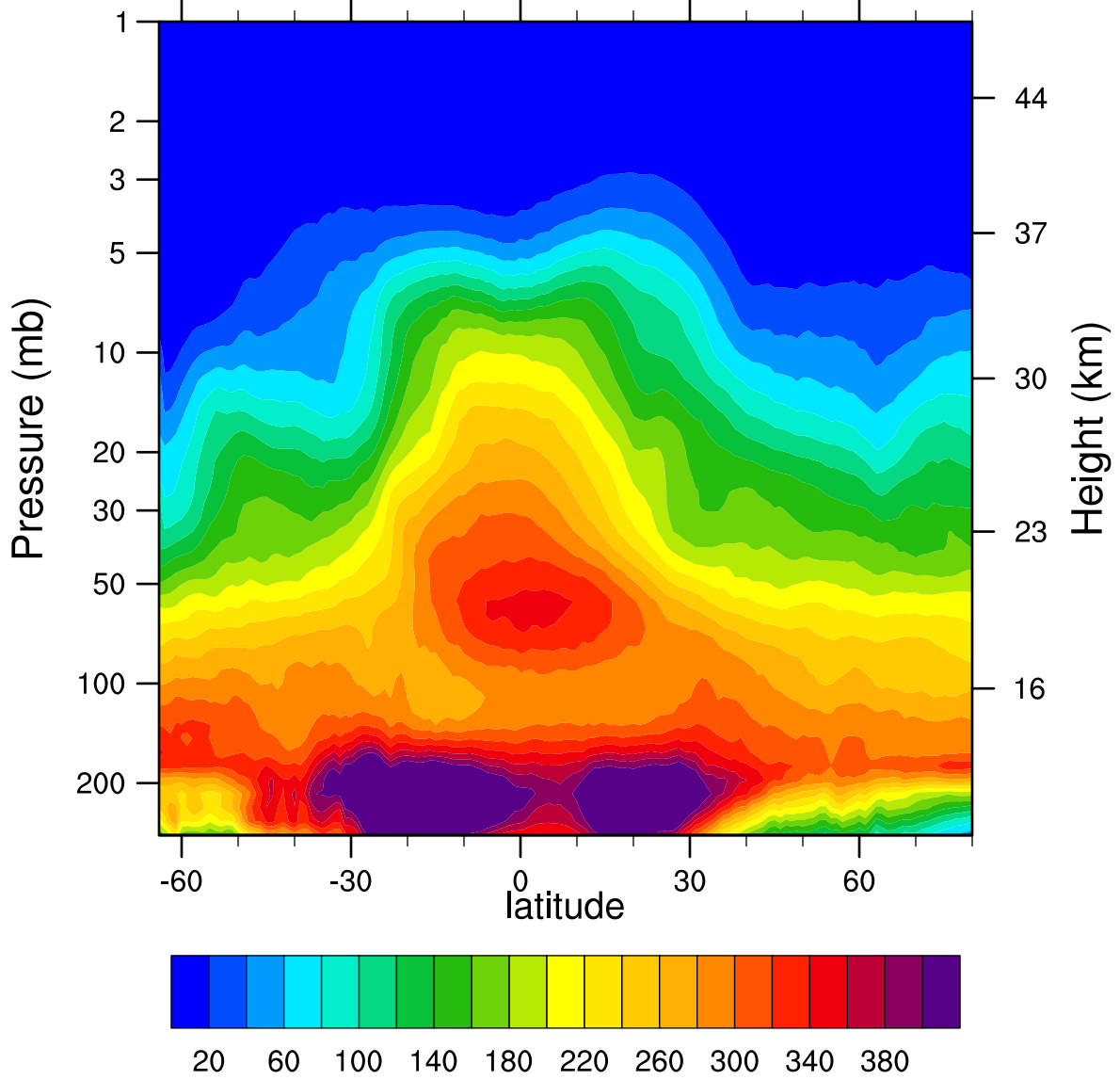
2005d134 N2O_Combined (ppbv)
