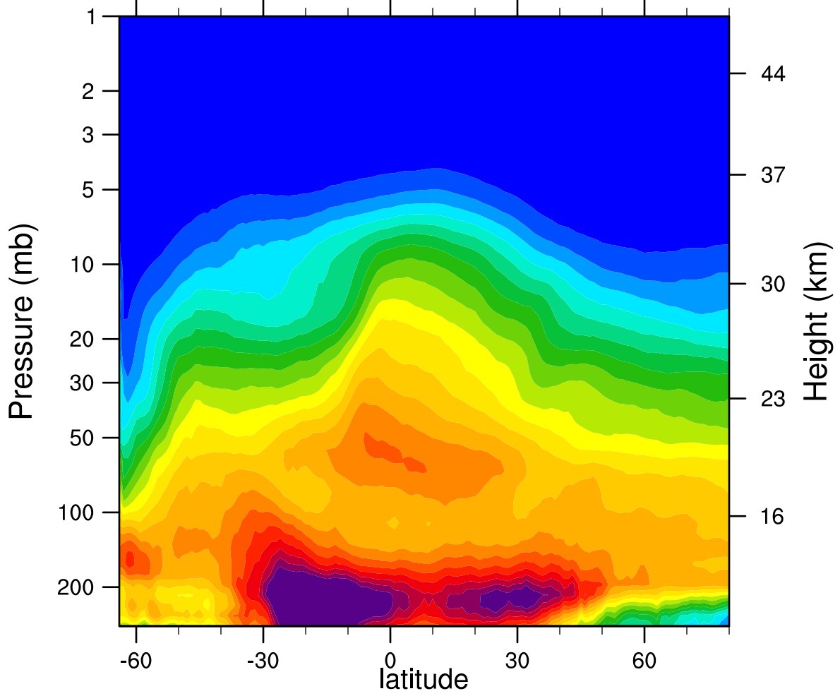
2006d217 N2O_Combined (ppbv)
