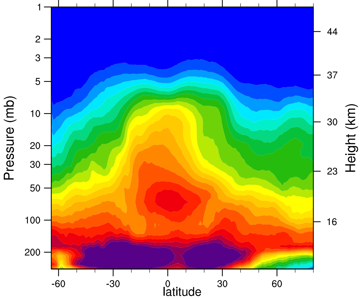
2007d133 N2O_Combined (ppbv)
