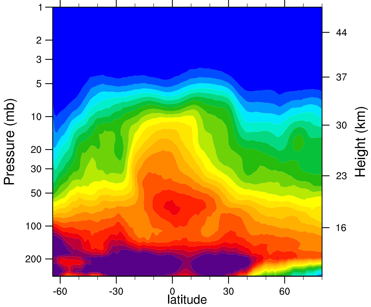
2007d156 N2O_Combined (ppbv)
