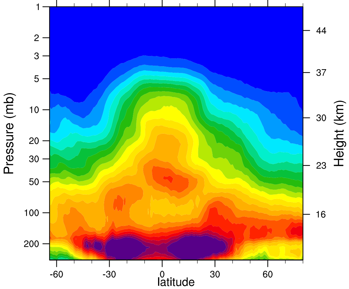
2005d071 N2O_Combined (ppbv)
