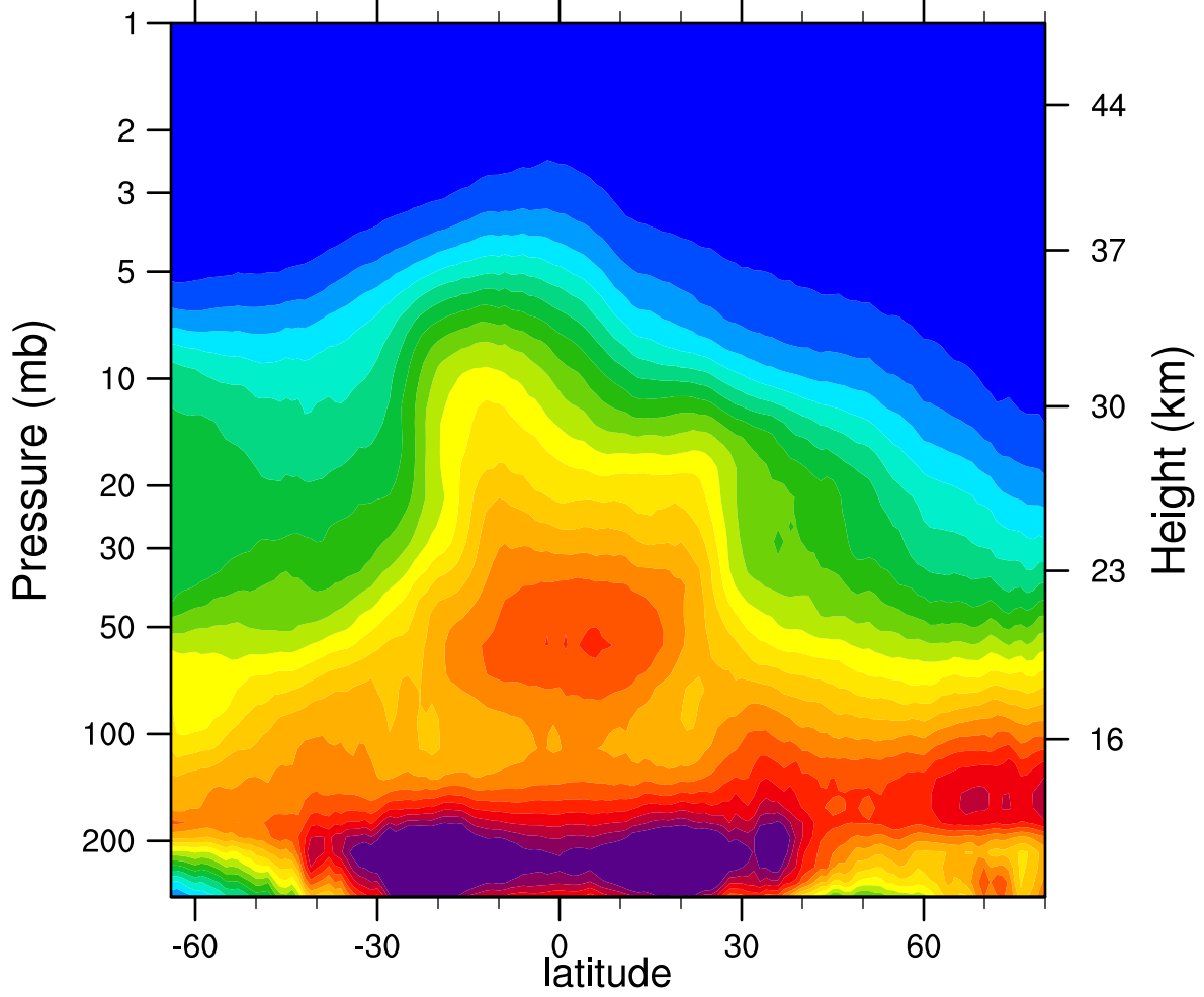
2005d354 N2O_Combined (ppbv)
