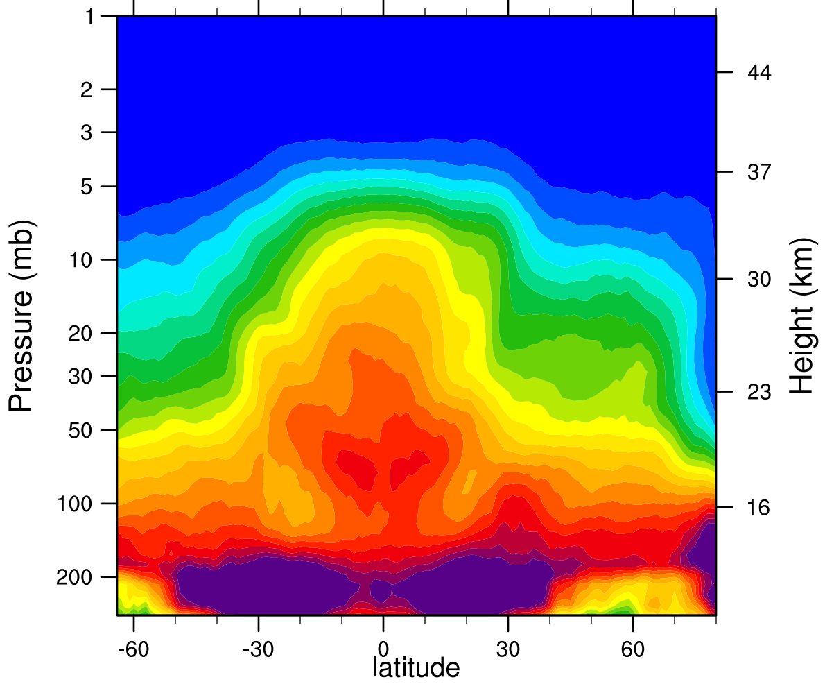
2007d085 N2O_Combined (ppbv)
