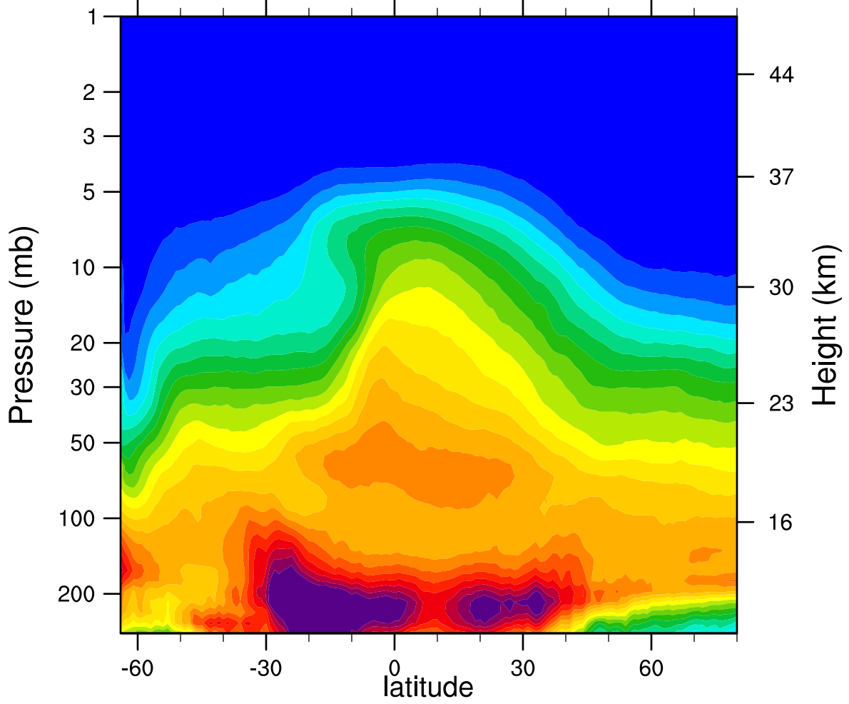
2006d253 N2O_Combined (ppbv)
