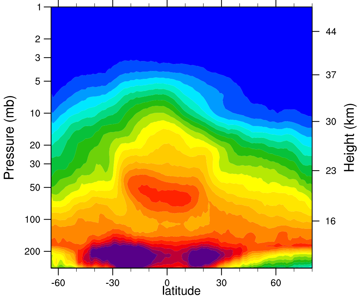
2006d118 N2O_Combined (ppbv)
