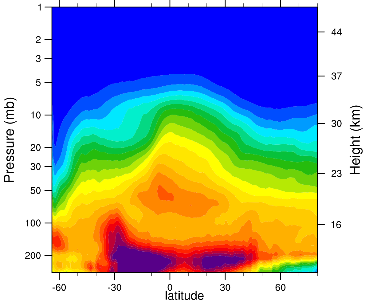
2006d205 N2O_Combined (ppbv)
