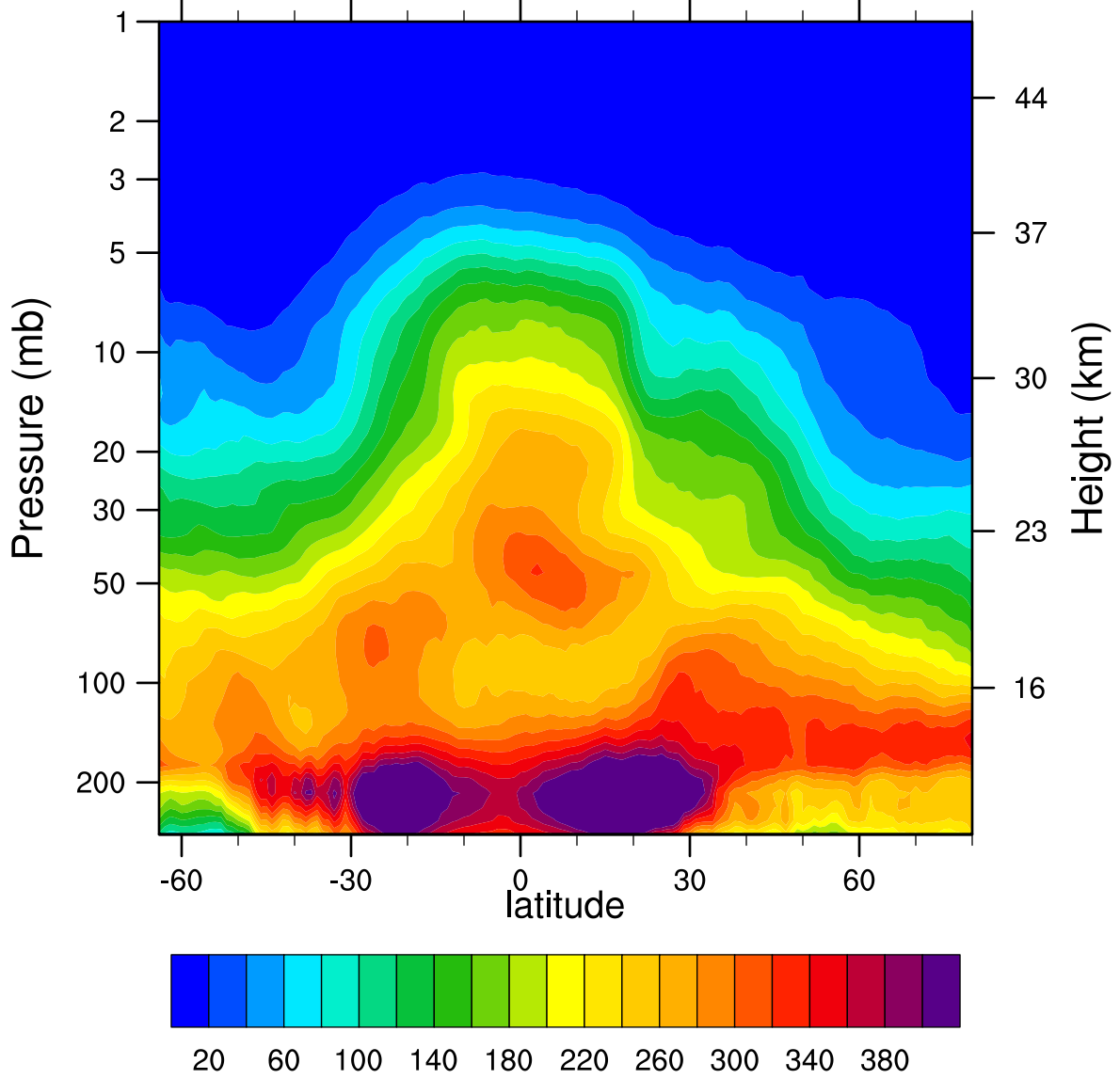
2005d060 N2O_Combined (ppbv)
