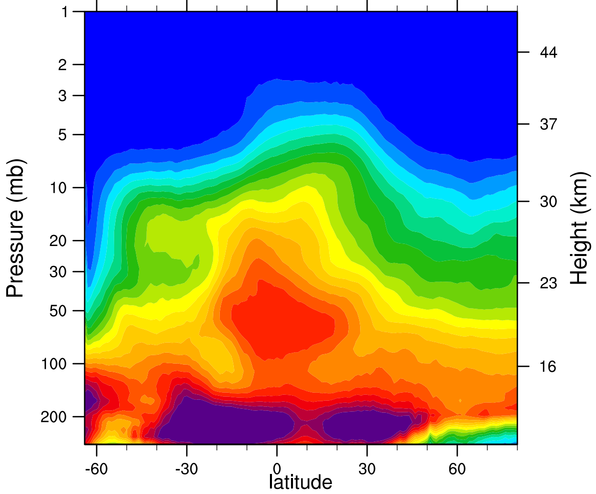
2007d232 N2O_Combined (ppbv)
