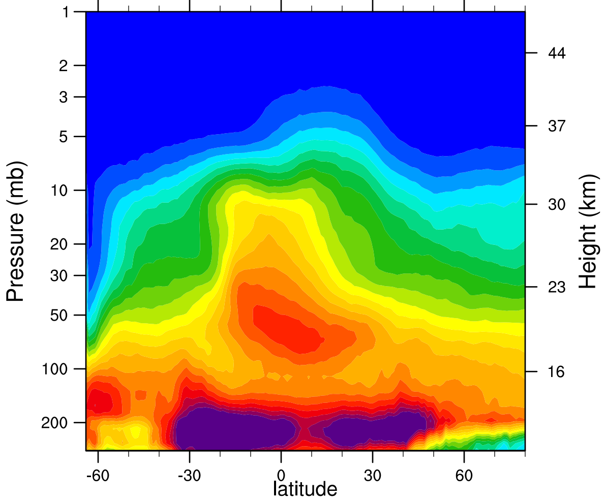
2005d200 N2O_Combined (ppbv)
