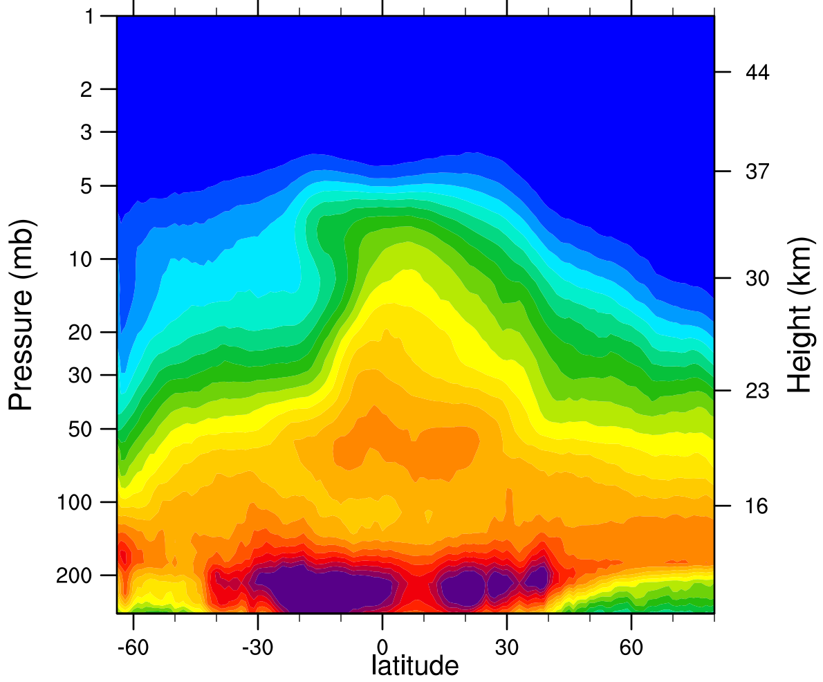
2006d283 N2O_Combined (ppbv)
