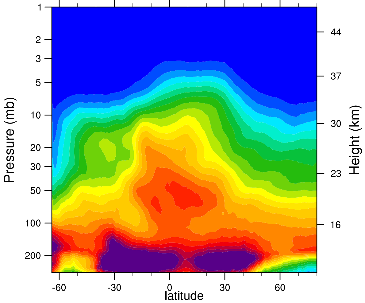
2007d247 N2O_Combined (ppbv)
