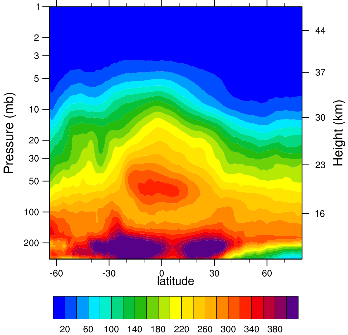
2006d145 N2O_Combined (ppbv)
