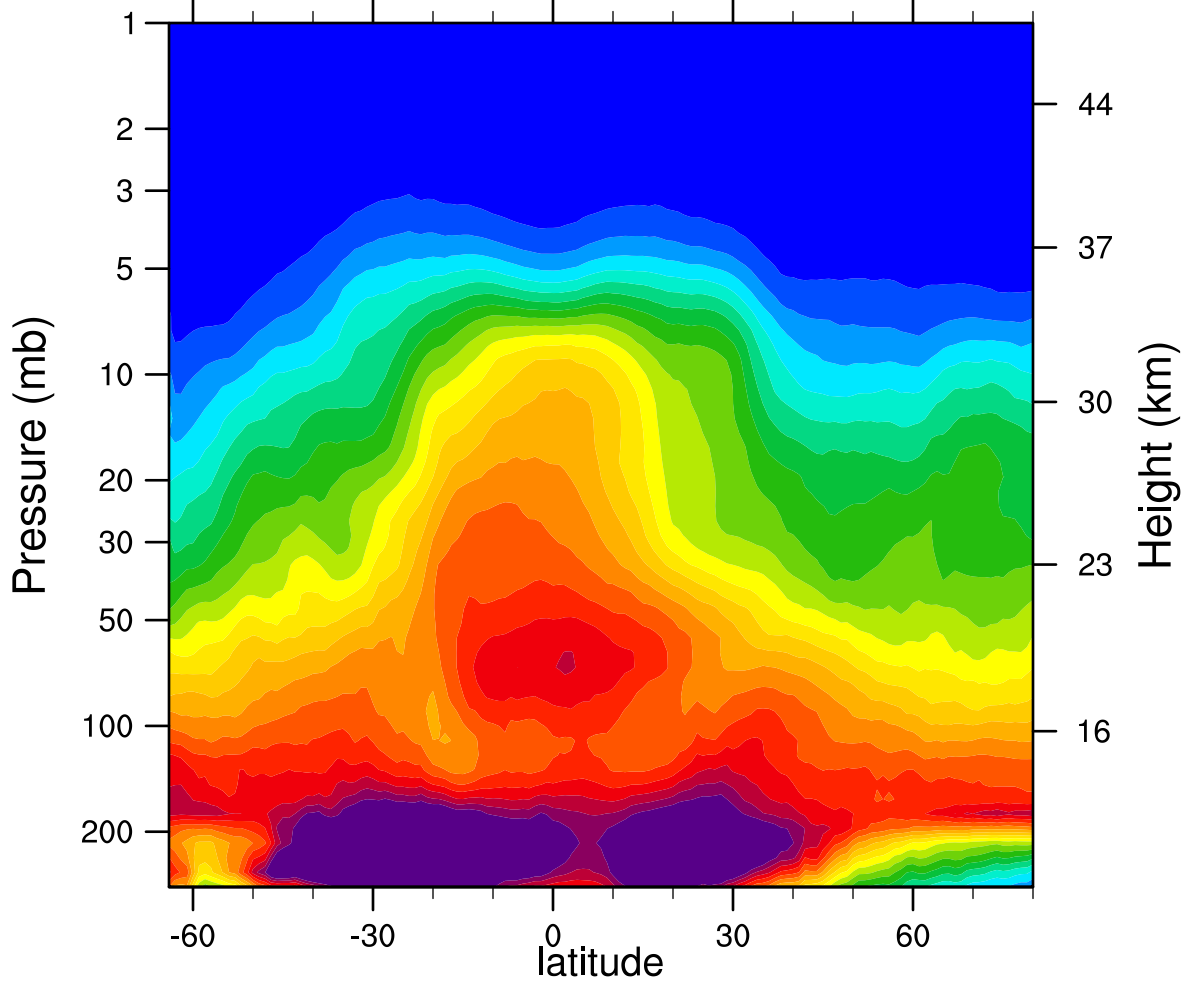
2007d126 N2O_Combined (ppbv)
