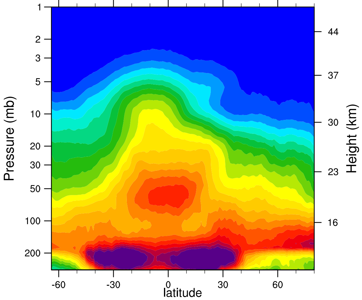
2006d063 N2O_Combined (ppbv)
