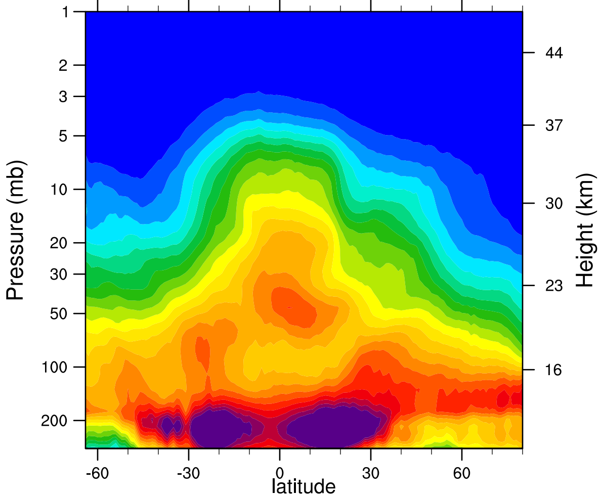
2005d062 N2O_Combined (ppbv)
