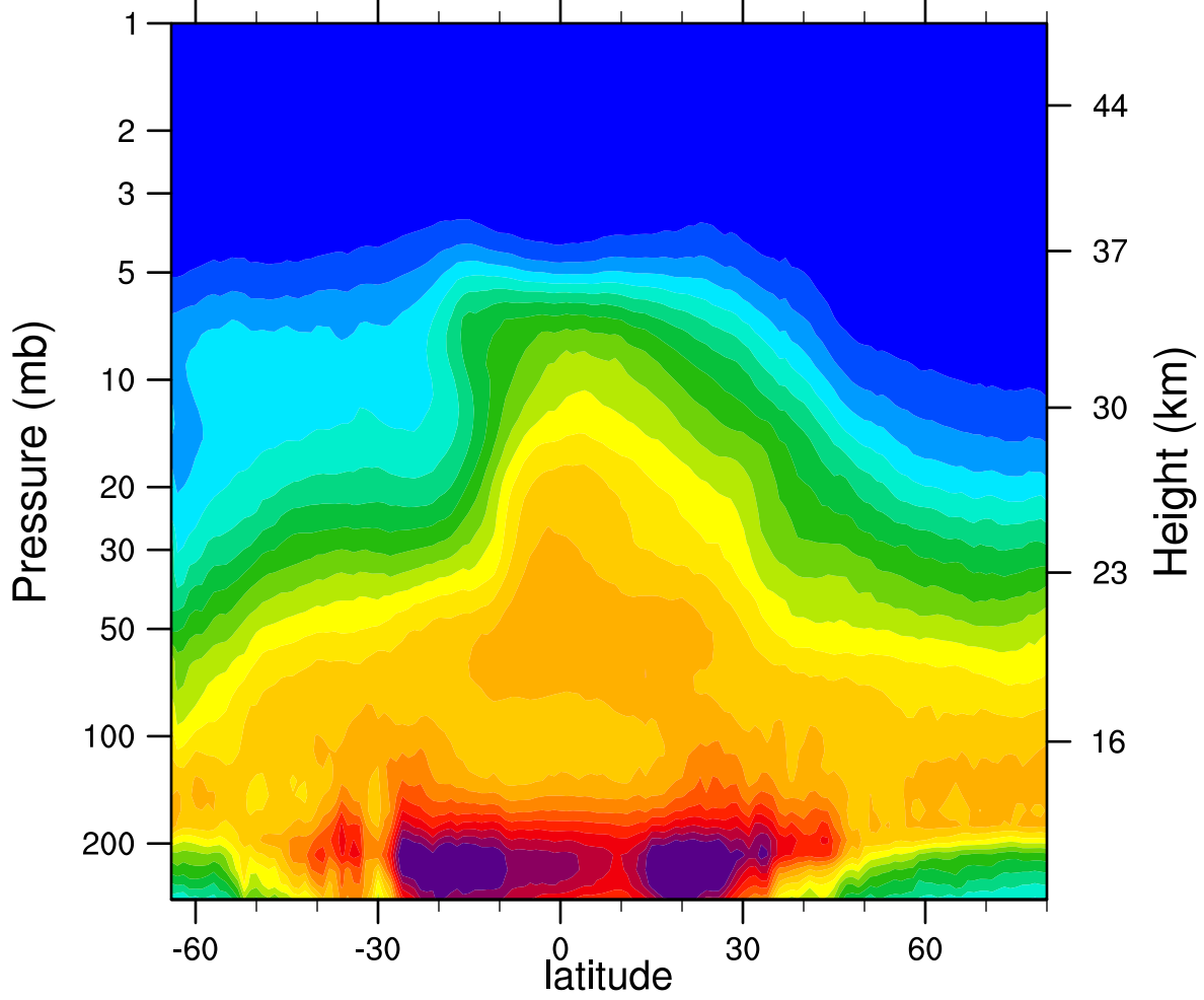
2006d300 N2O_Combined (ppbv)
