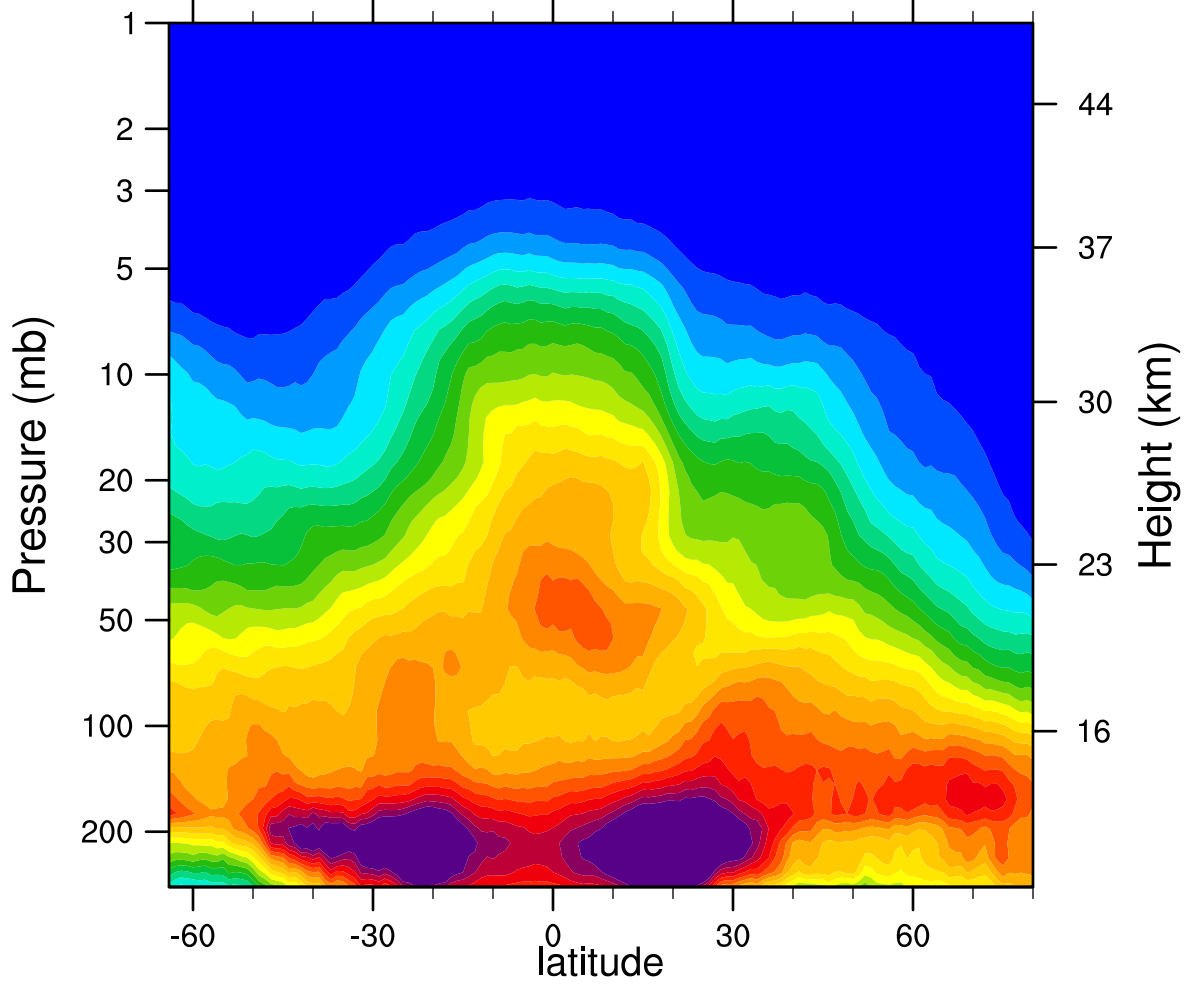
2005d045 N2O_Combined (ppbv)
