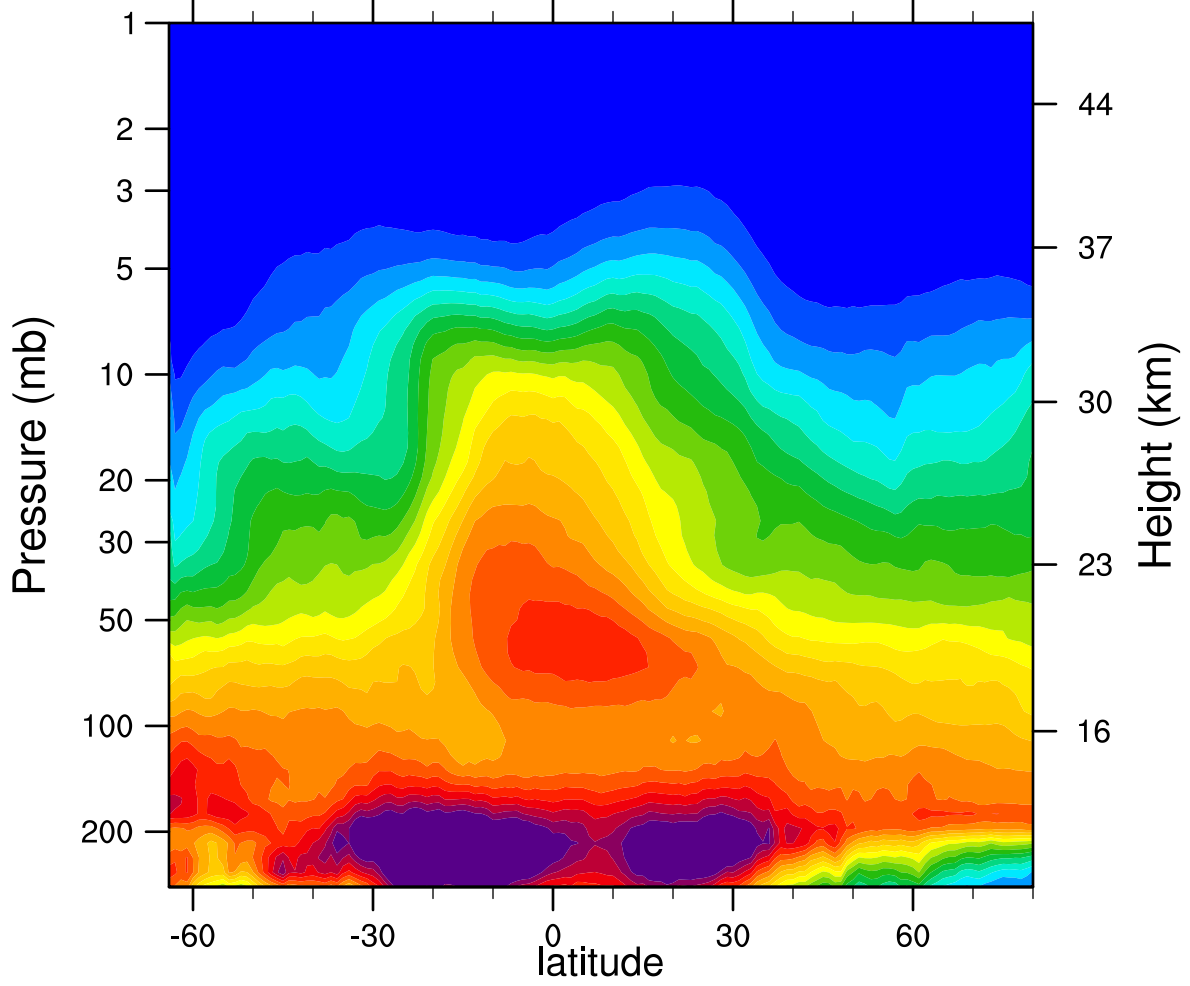
2005d153 N2O_Combined (ppbv)
