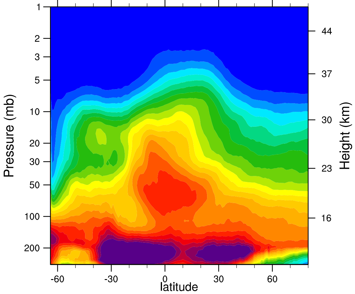
2007d220 N2O_Combined (ppbv)
