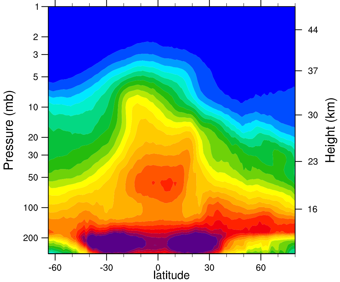
2006d028 N2O_Combined (ppbv)
