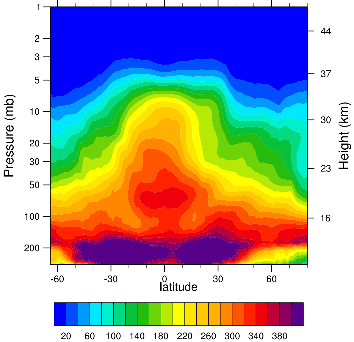
2007d108 N2O_Combined (ppbv)
