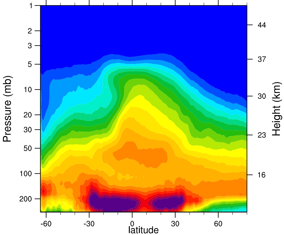
2006d275 N2O_Combined (ppbv)
