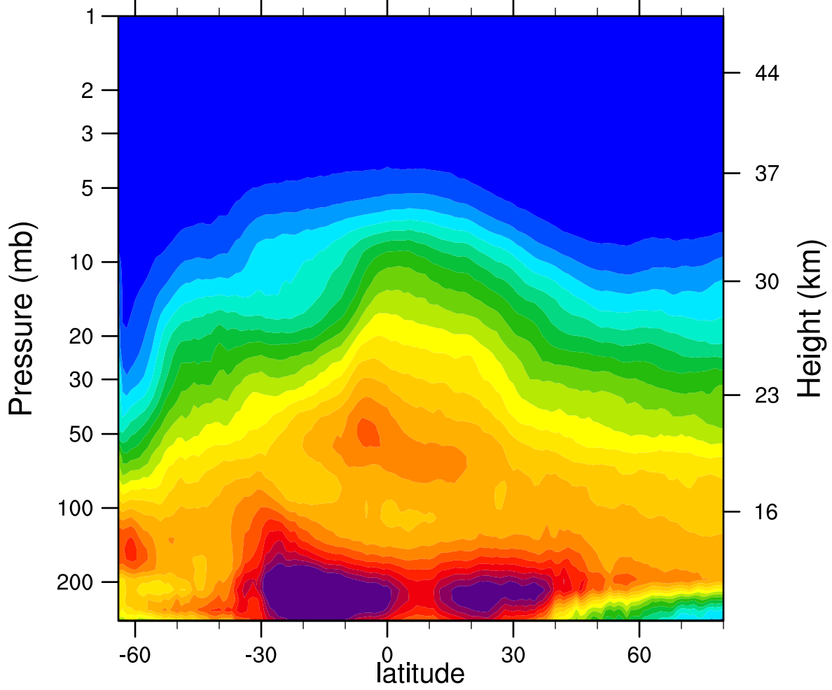
2006d193 N2O_Combined (ppbv)
