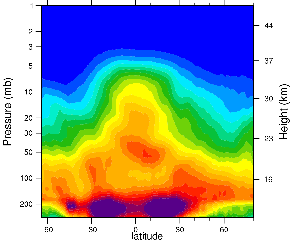
2005d082 N2O_Combined (ppbv)
