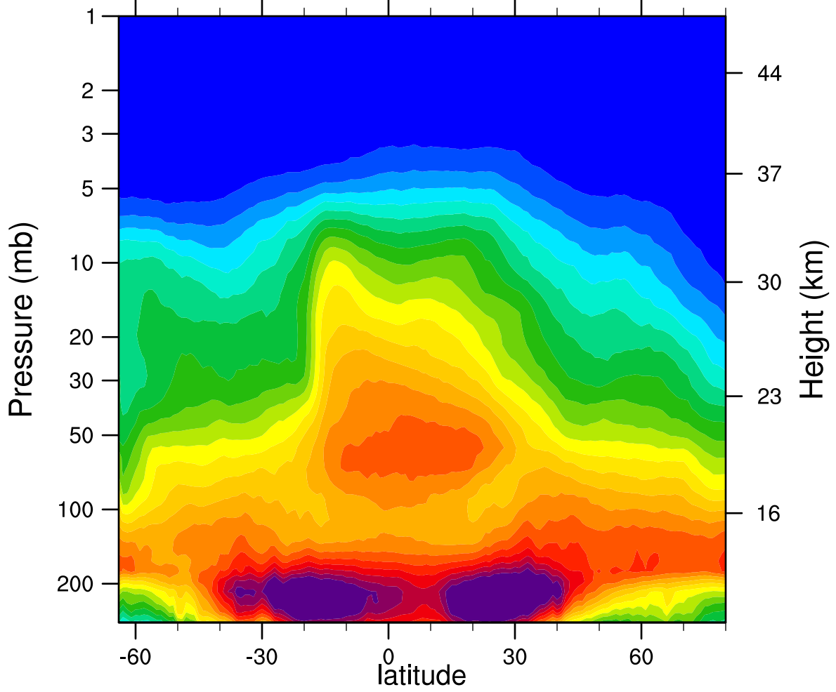
2005d302 N2O_Combined (ppbv)
