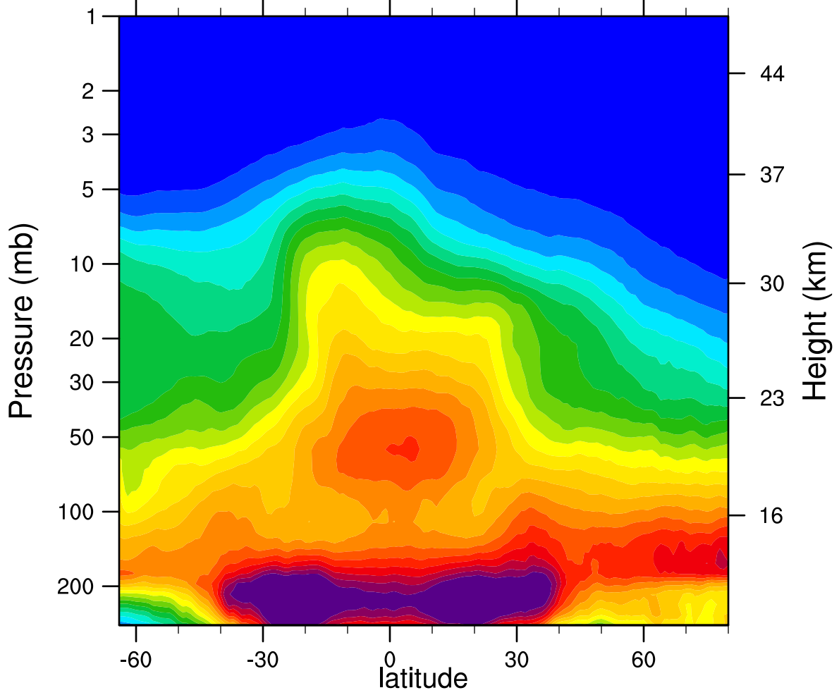
2005d349 N2O_Combined (ppbv)
