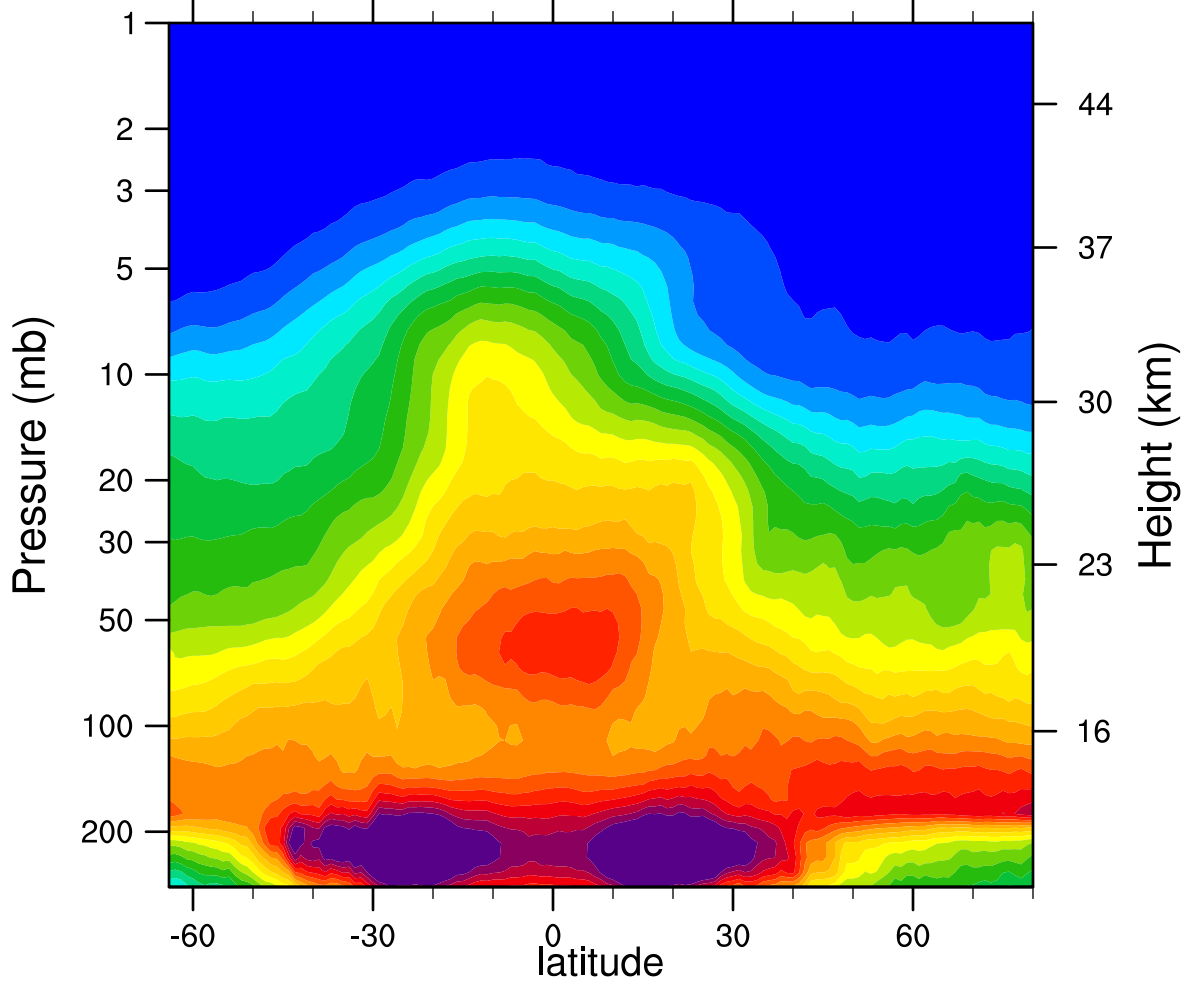
2006d047 N2O_Combined (ppbv)
