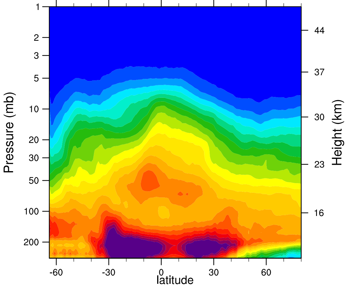
2006d173 N2O_Combined (ppbv)
