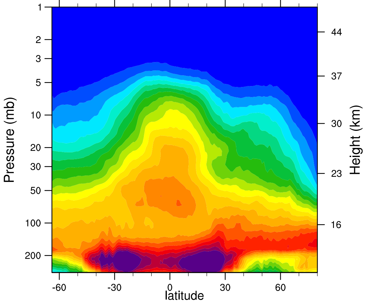
2007d044 N2O_Combined (ppbv)
