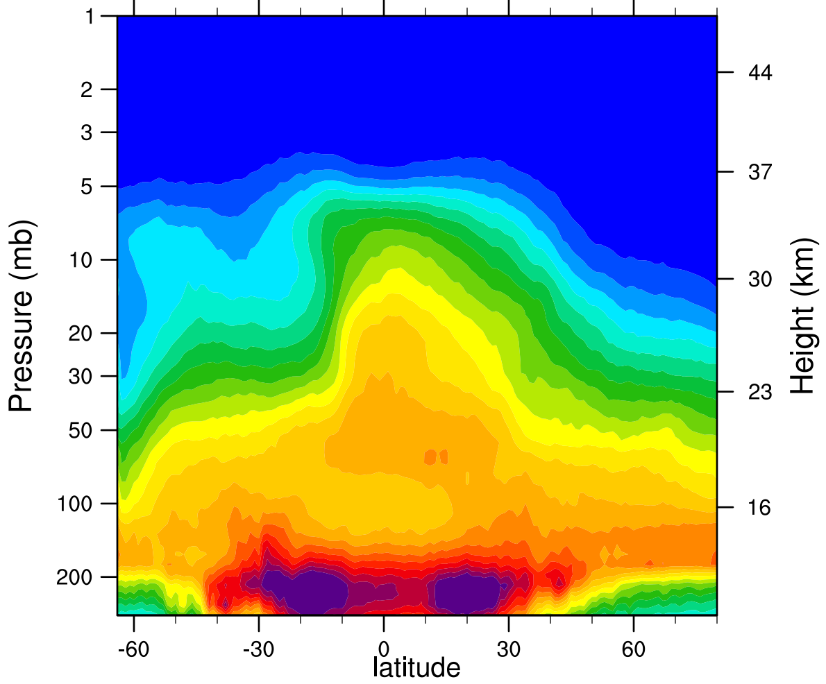
2006d304 N2O_Combined (ppbv)
