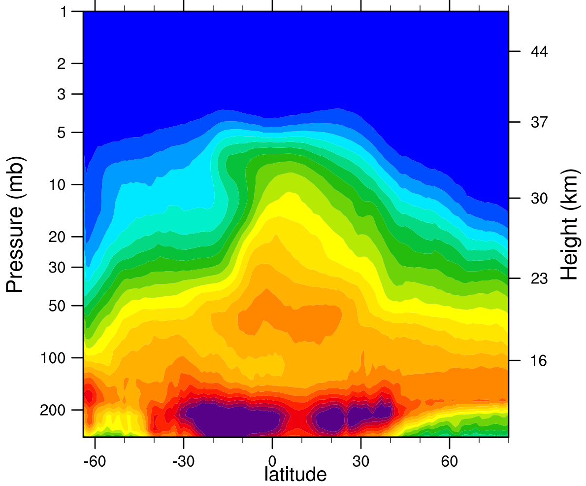
2006d282 N2O_Combined (ppbv)
