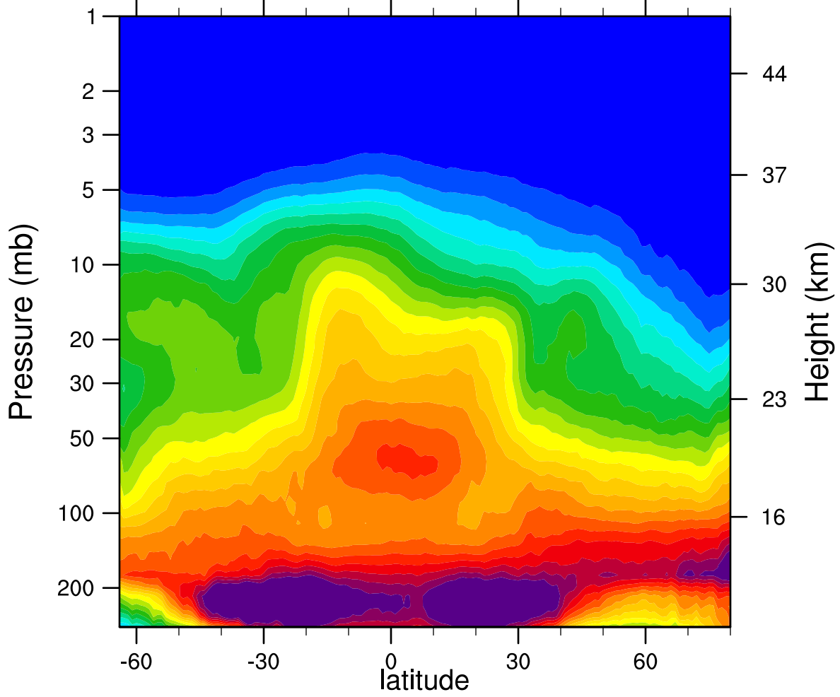
2007d340 N2O_Combined (ppbv)
