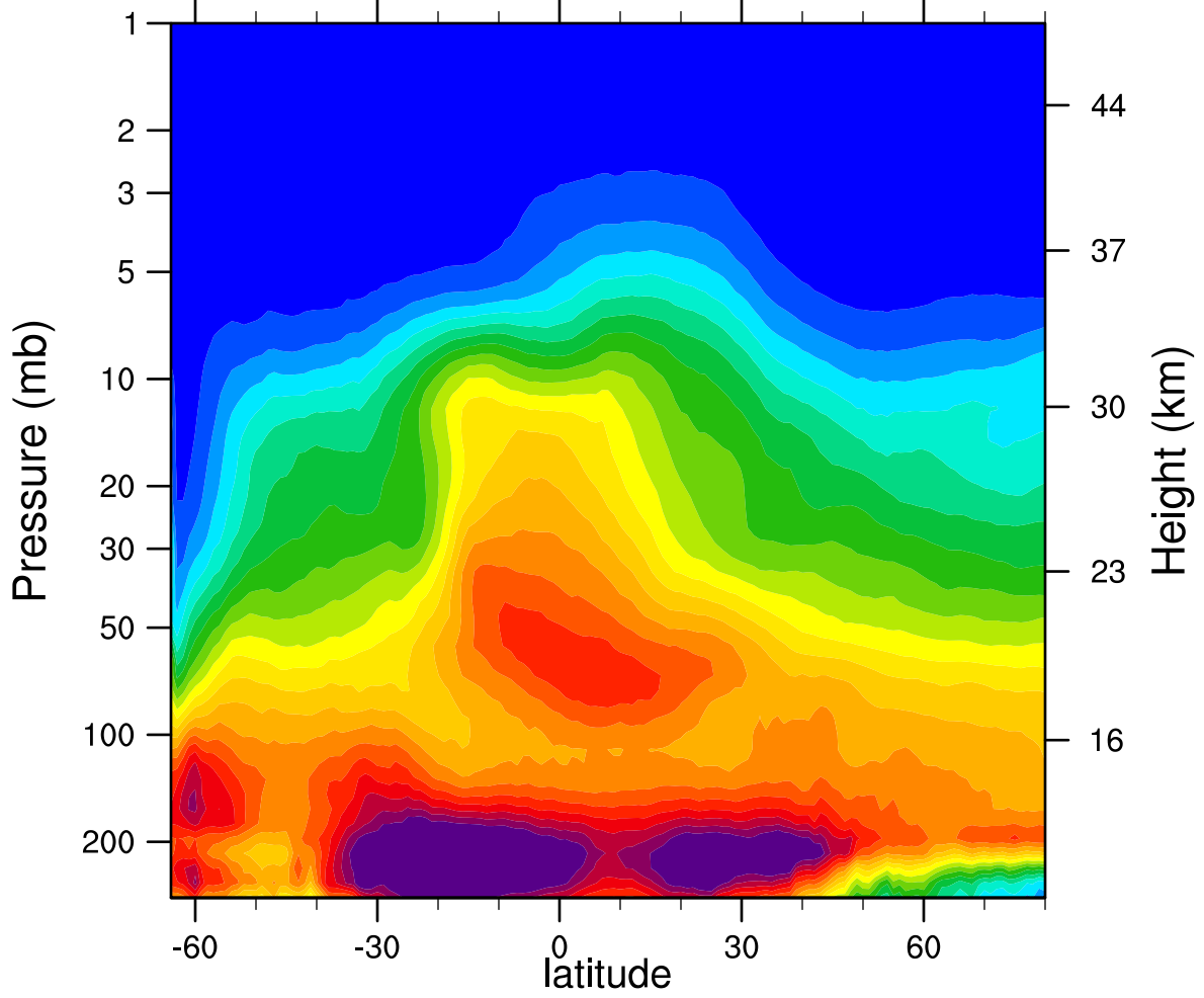
2005d204 N2O_Combined (ppbv)
