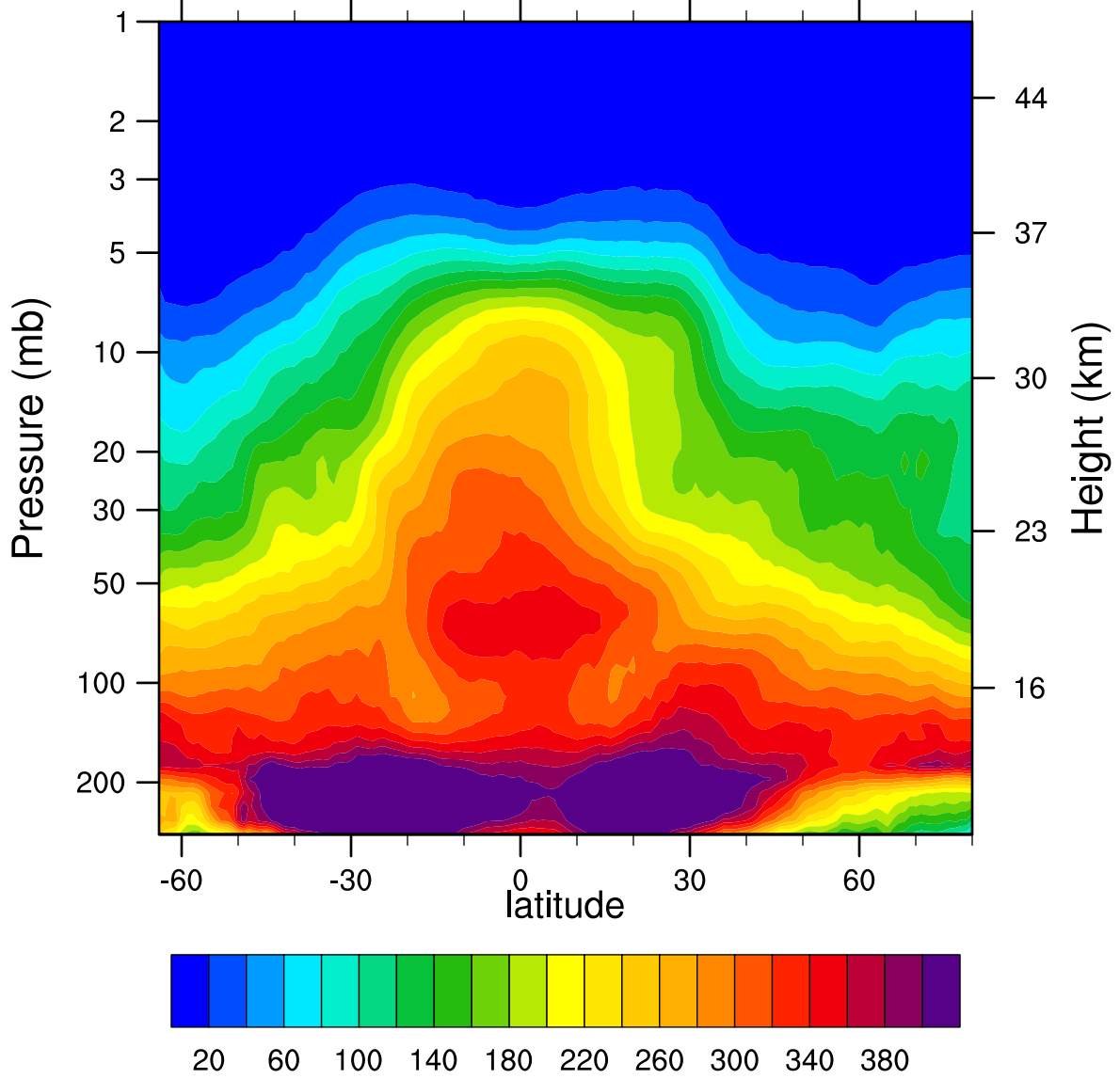
2007d111 N2O_Combined (ppbv)
