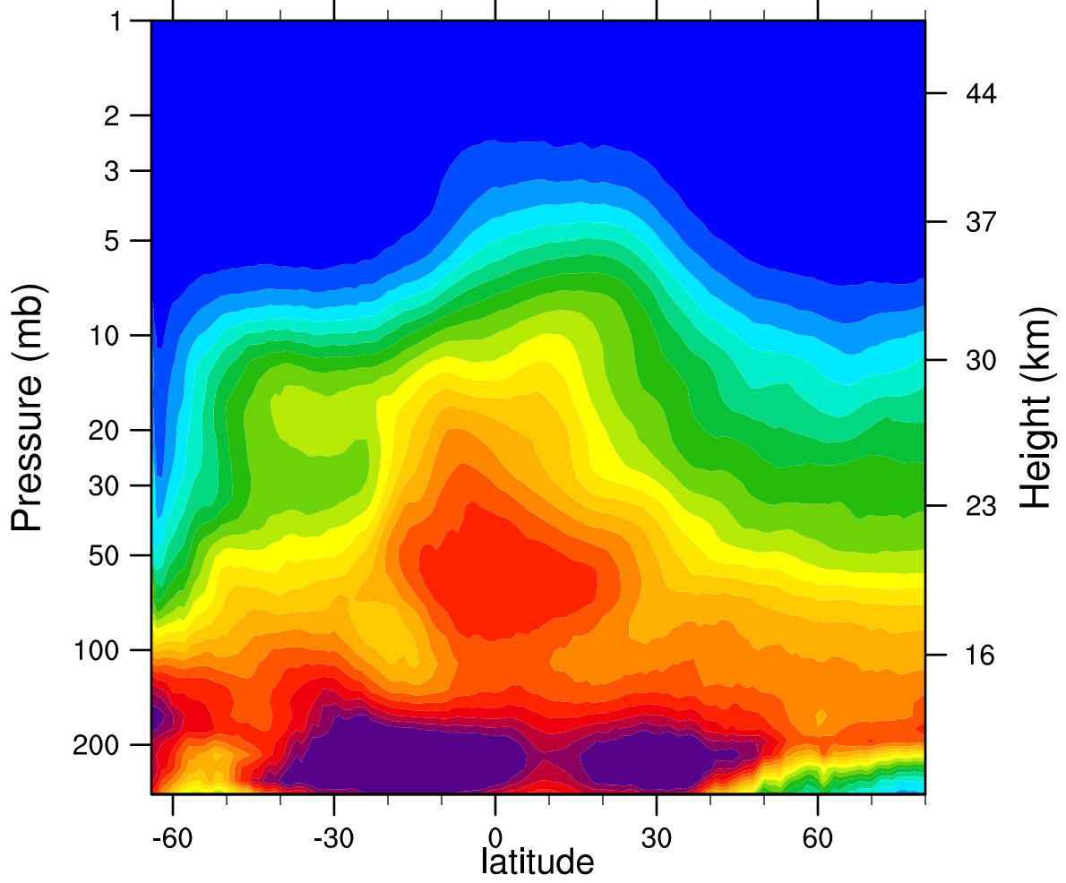
2007d230 N2O_Combined (ppbv)
