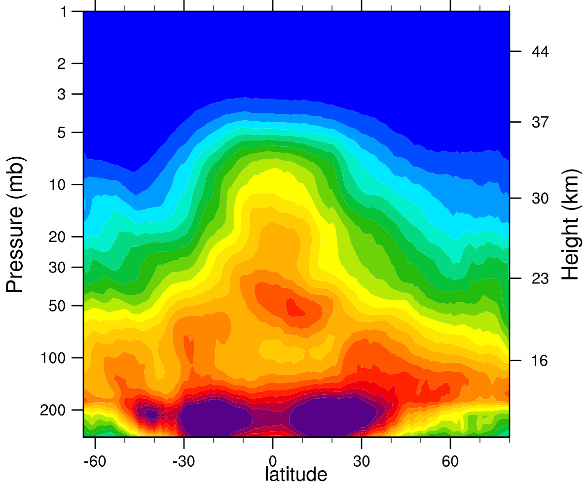
2005d080 N2O_Combined (ppbv)
