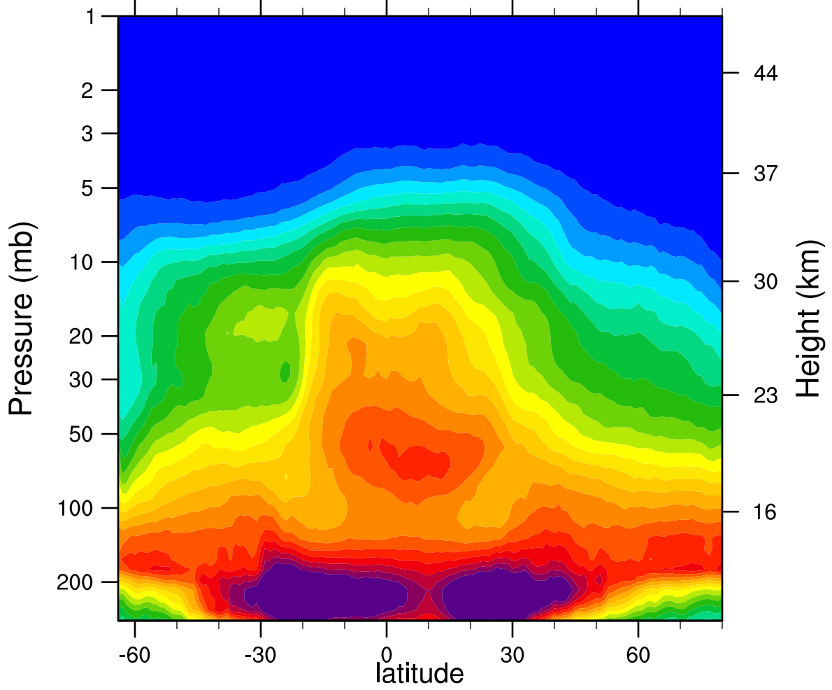
2007d286 N2O_Combined (ppbv)
