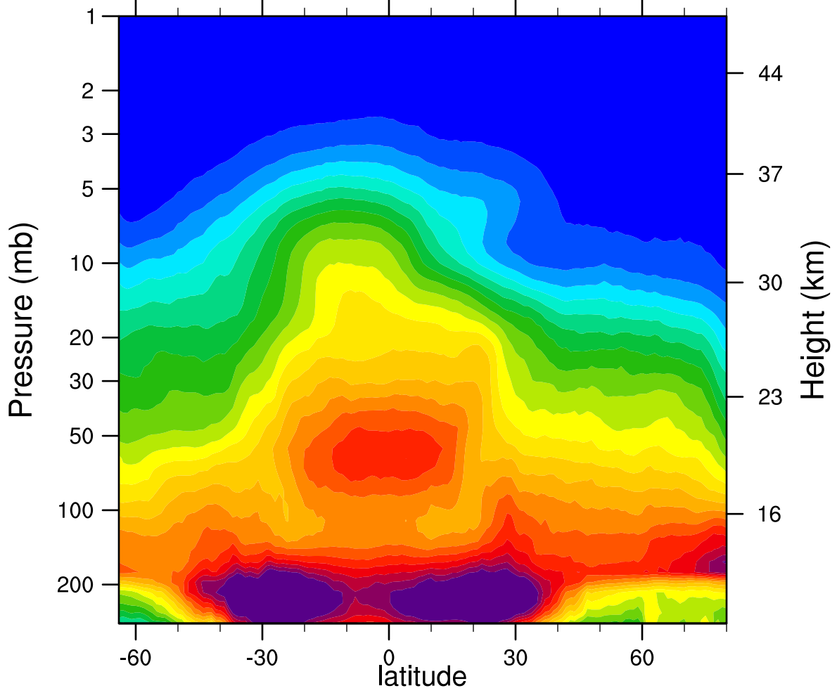
2006d070 N2O_Combined (ppbv)
