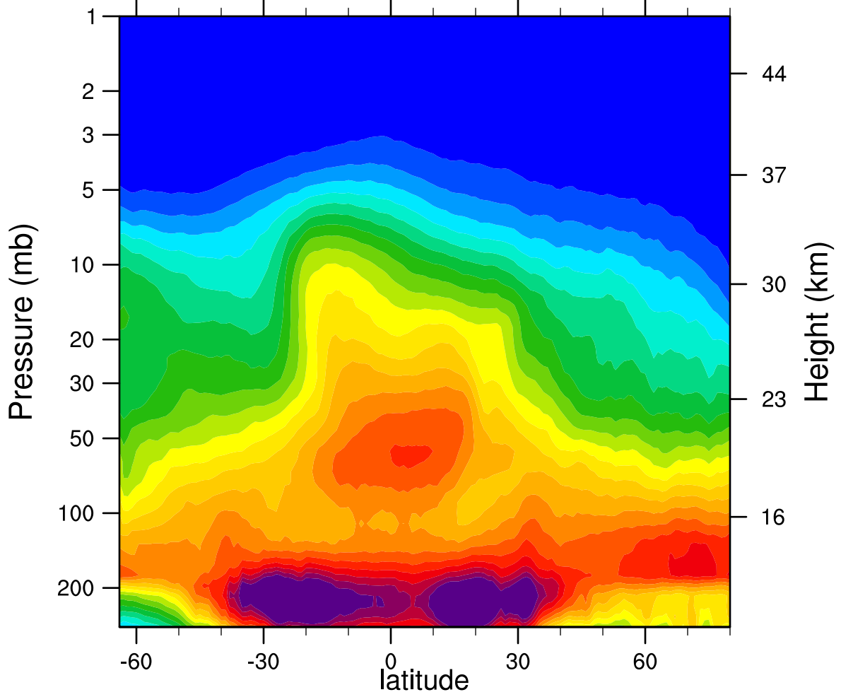
2005d335 N2O_Combined (ppbv)
