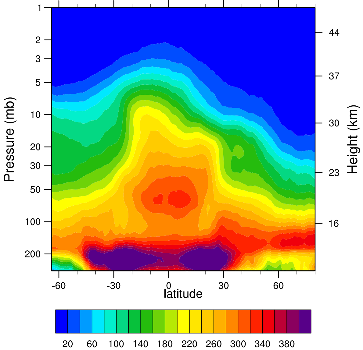
2006d012 N2O_Combined (ppbv)
