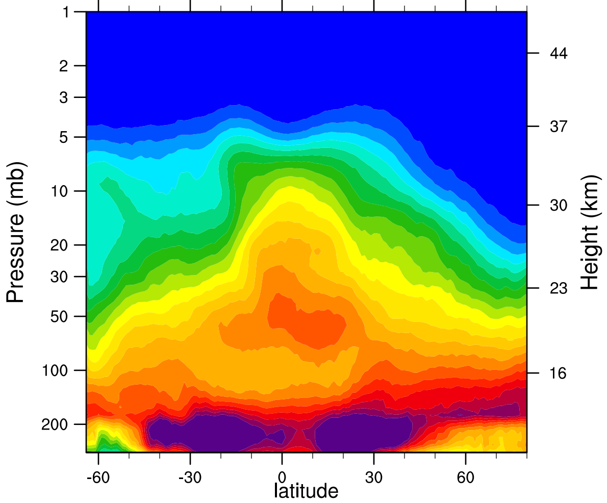
2006d324 N2O_Combined (ppbv)
