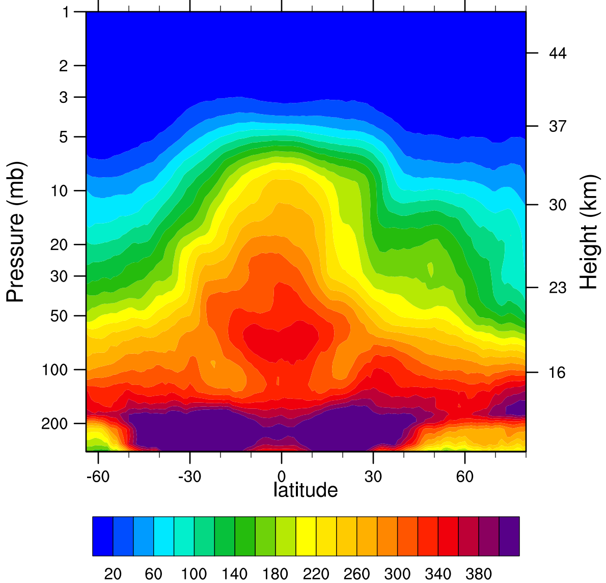
2007d093 N2O_Combined (ppbv)
