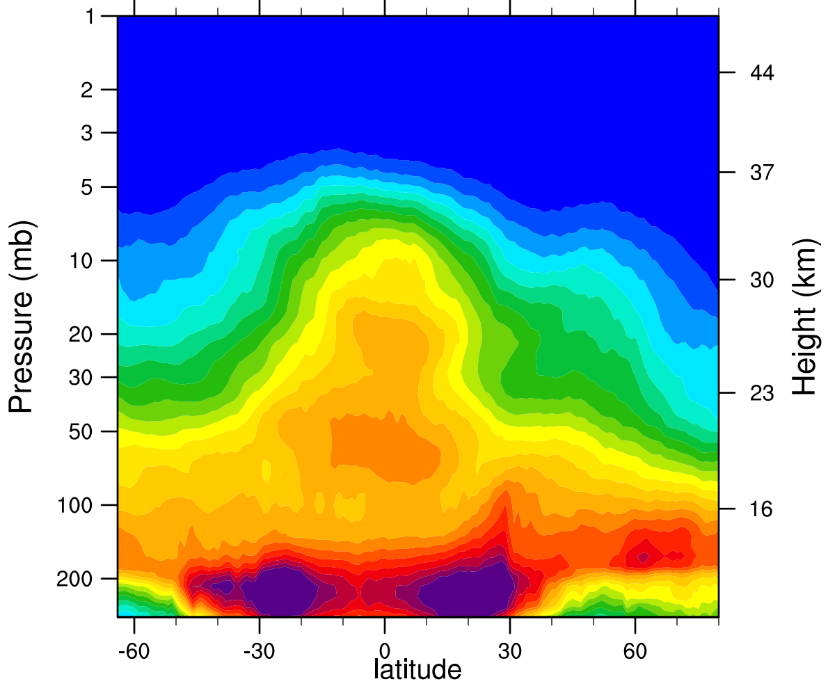
2007d051 N2O_Combined (ppbv)
