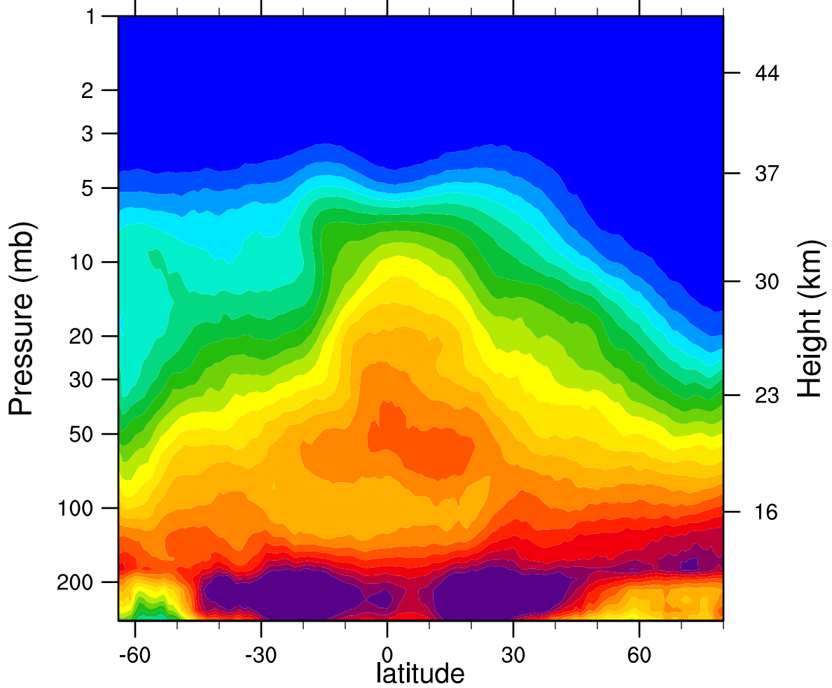
2006d325 N2O_Combined (ppbv)
