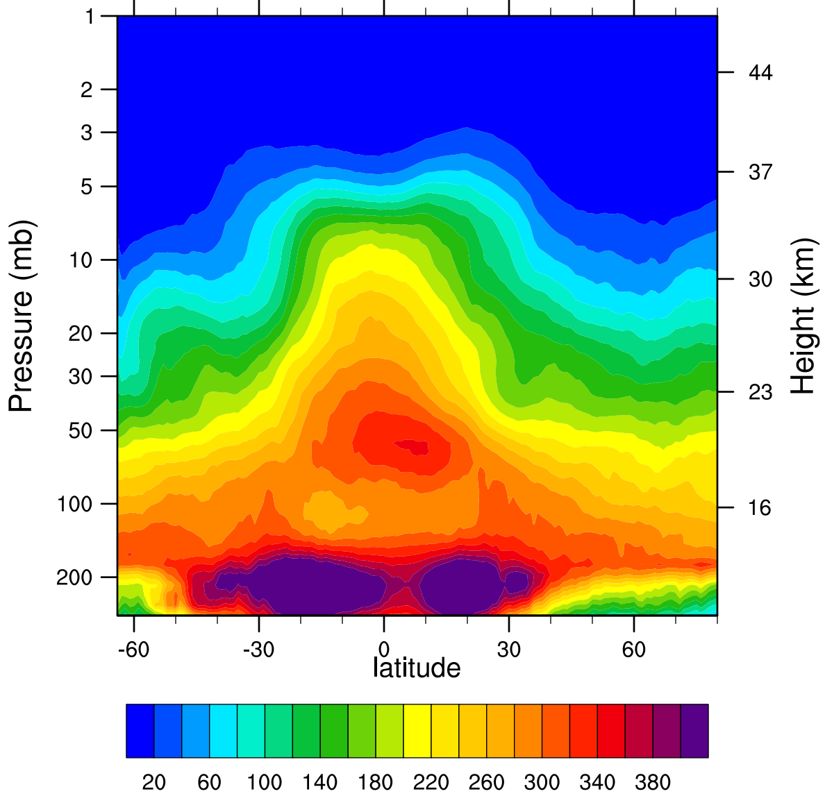
2005d119 N2O_Combined (ppbv)
