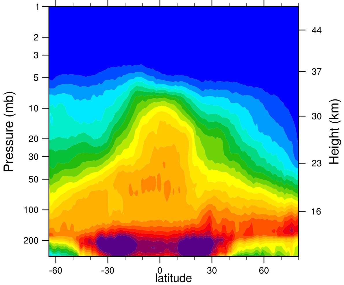
2006d359 N2O_Combined (ppbv)
