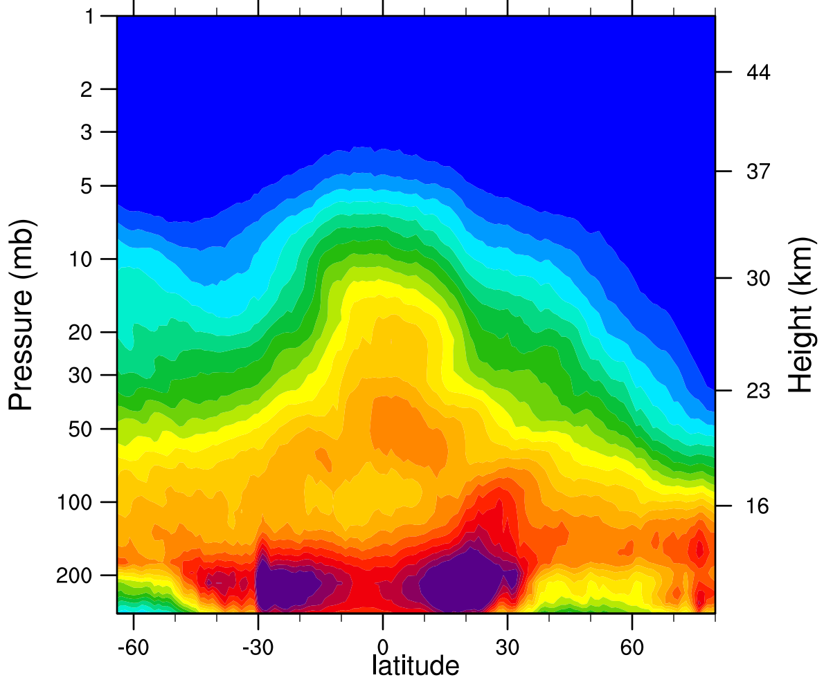
2005d029 N2O_Combined (ppbv)
