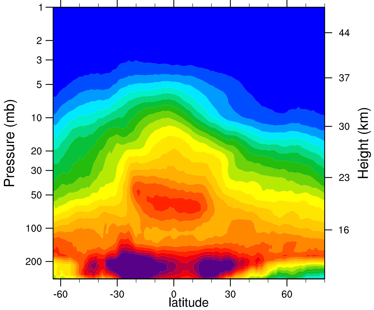
2006d125 N2O_Combined (ppbv)
