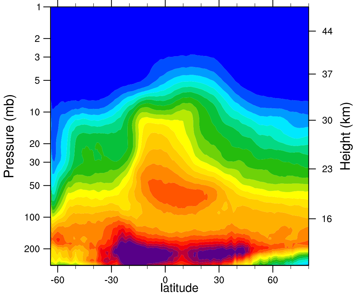
2005d239 N2O_Combined (ppbv)
