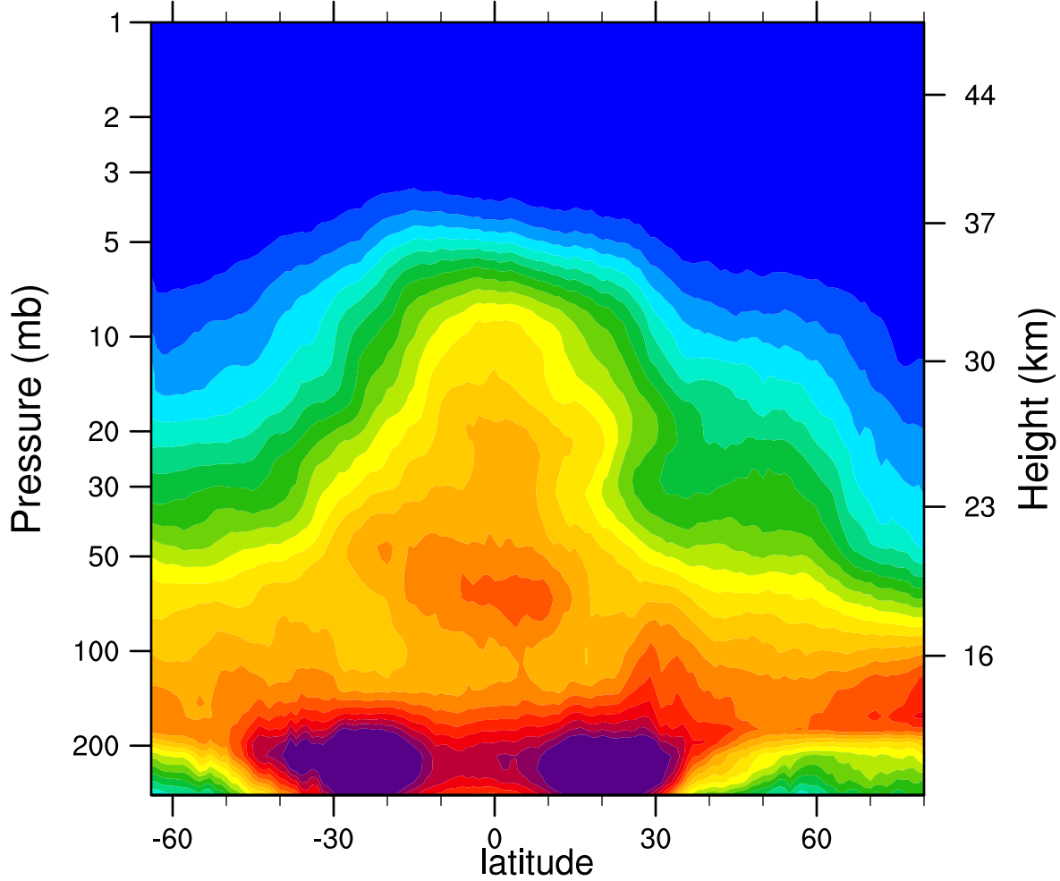
2007d065 N2O_Combined (ppbv)
