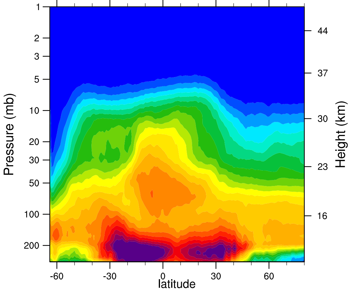
2007d207 N2O_Combined (ppbv)
