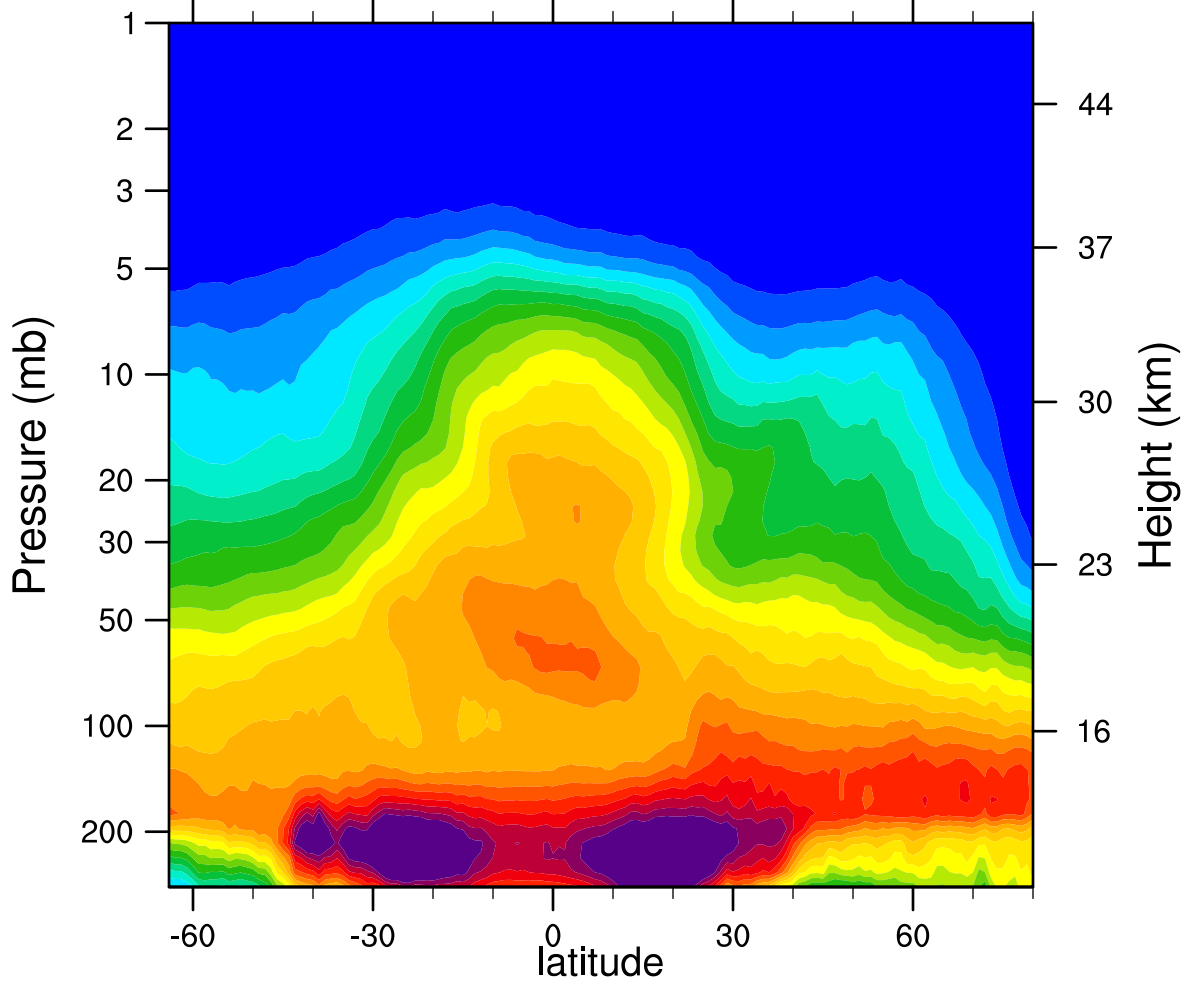
2007d032 N2O_Combined (ppbv)
