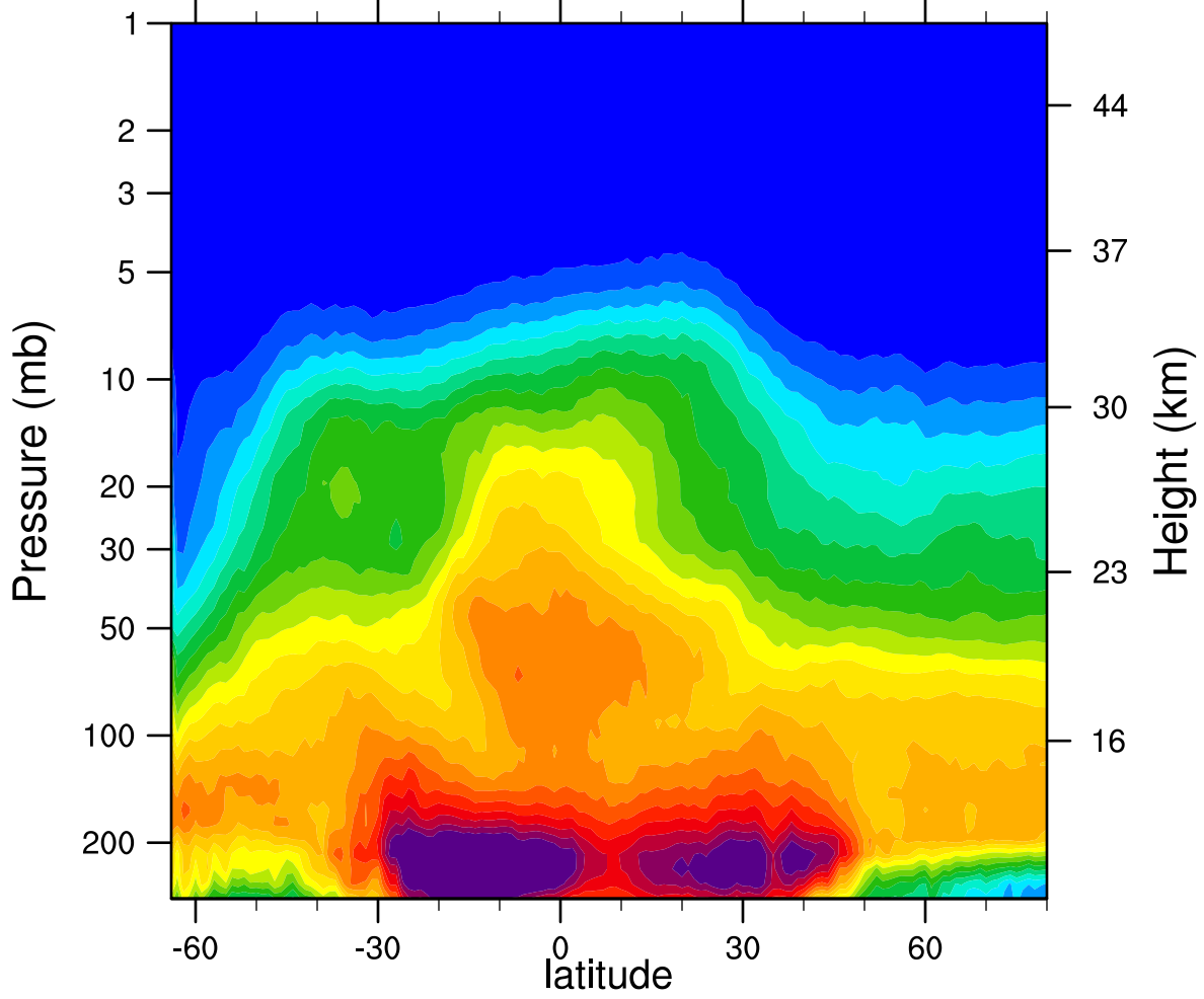
2007d211 N2O_Combined (ppbv)
