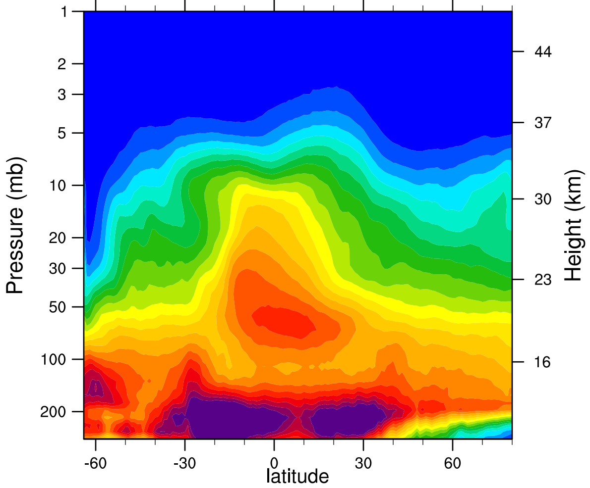
2005d174 N2O_Combined (ppbv)
