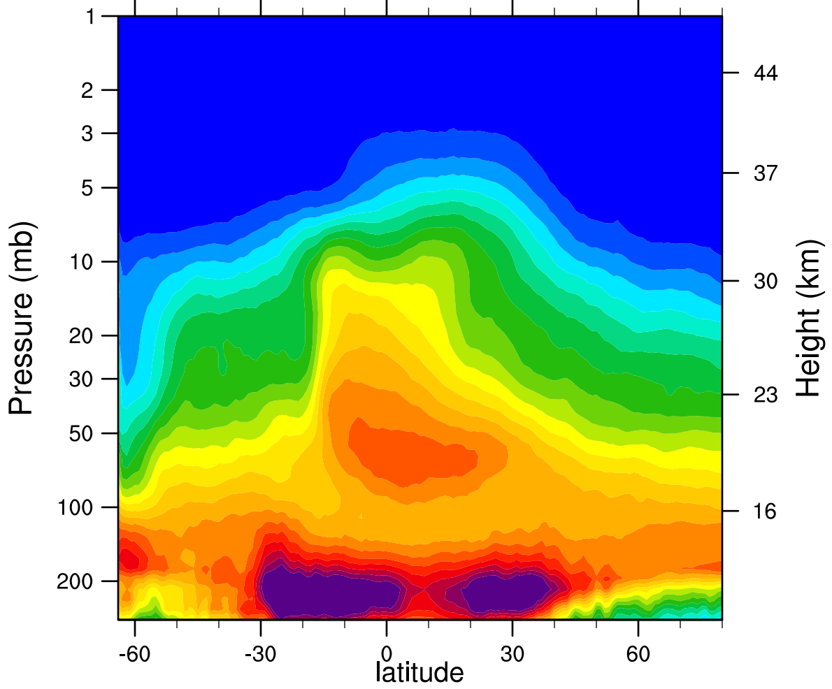
2005d254 N2O_Combined (ppbv)
