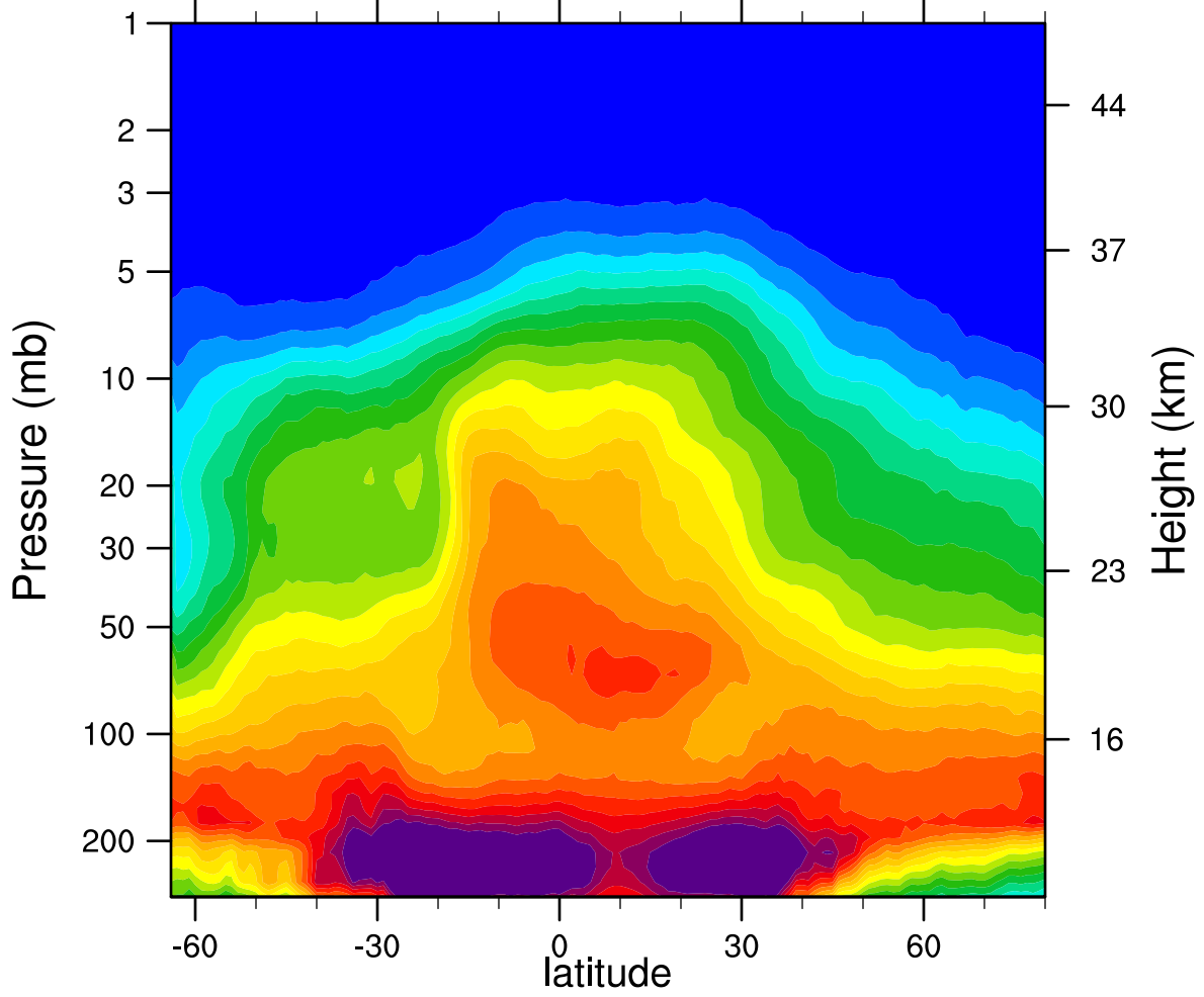
2007d278 N2O_Combined (ppbv)
