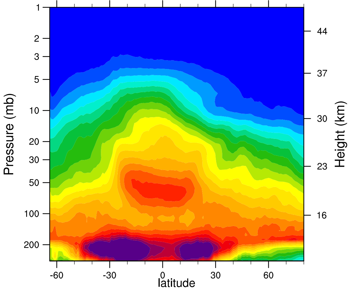
2006d114 N2O_Combined (ppbv)
