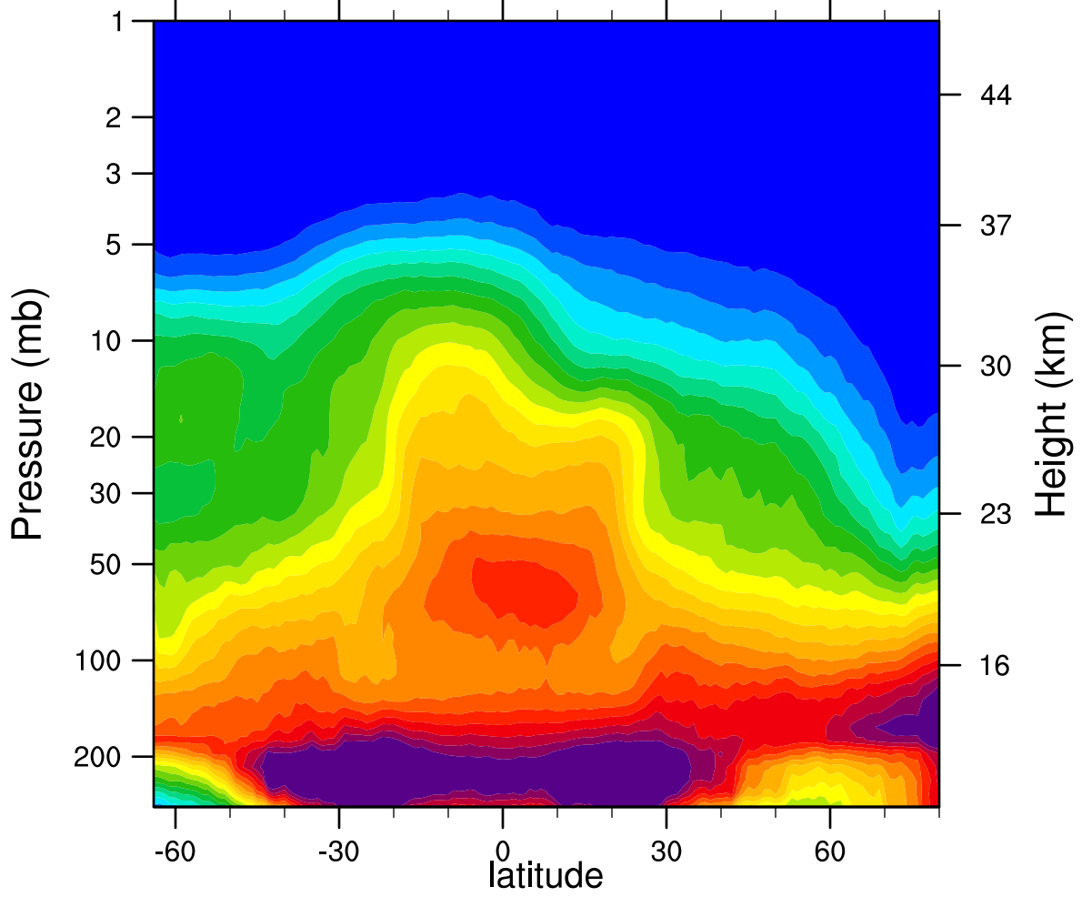
2007d360 N2O_Combined (ppbv)
