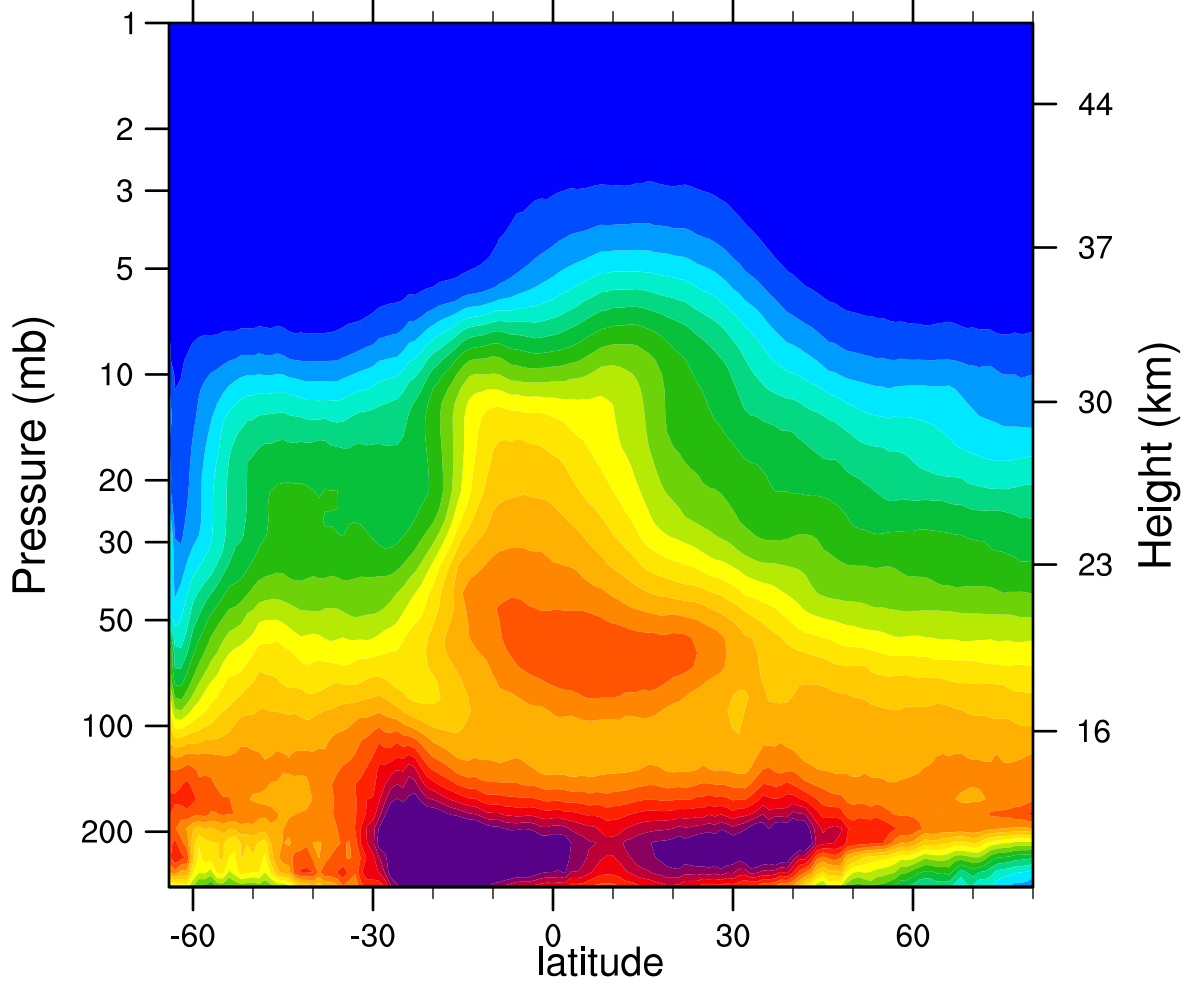
2005d236 N2O_Combined (ppbv)
