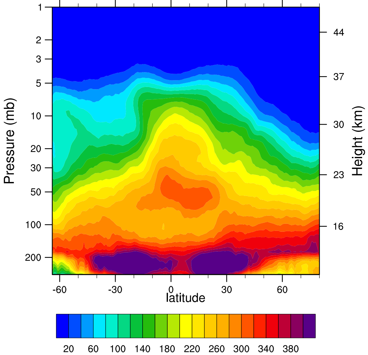
2006d321 N2O_Combined (ppbv)
