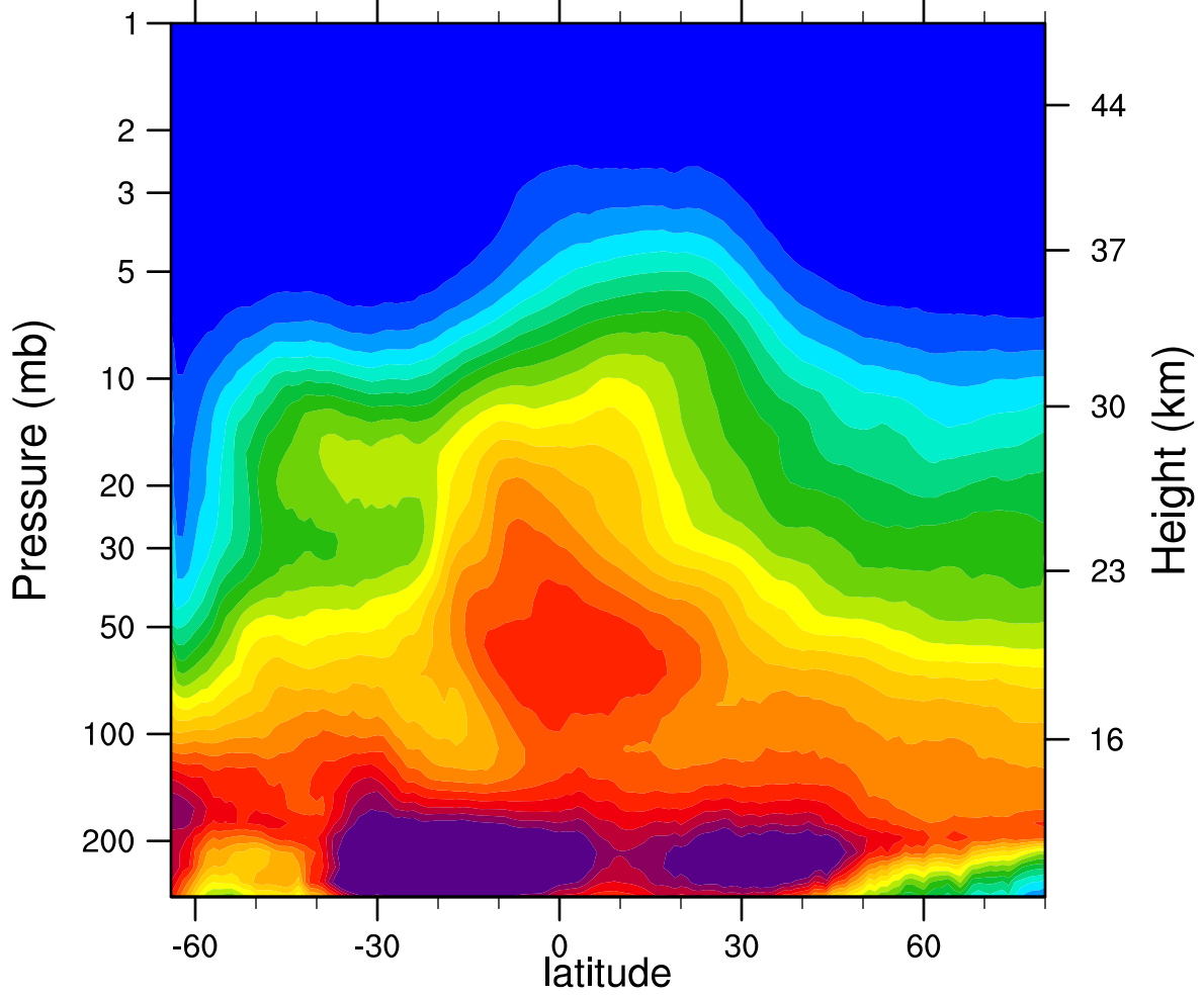
2007d222 N2O_Combined (ppbv)
