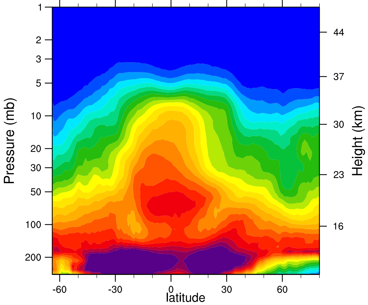
2007d121 N2O_Combined (ppbv)
