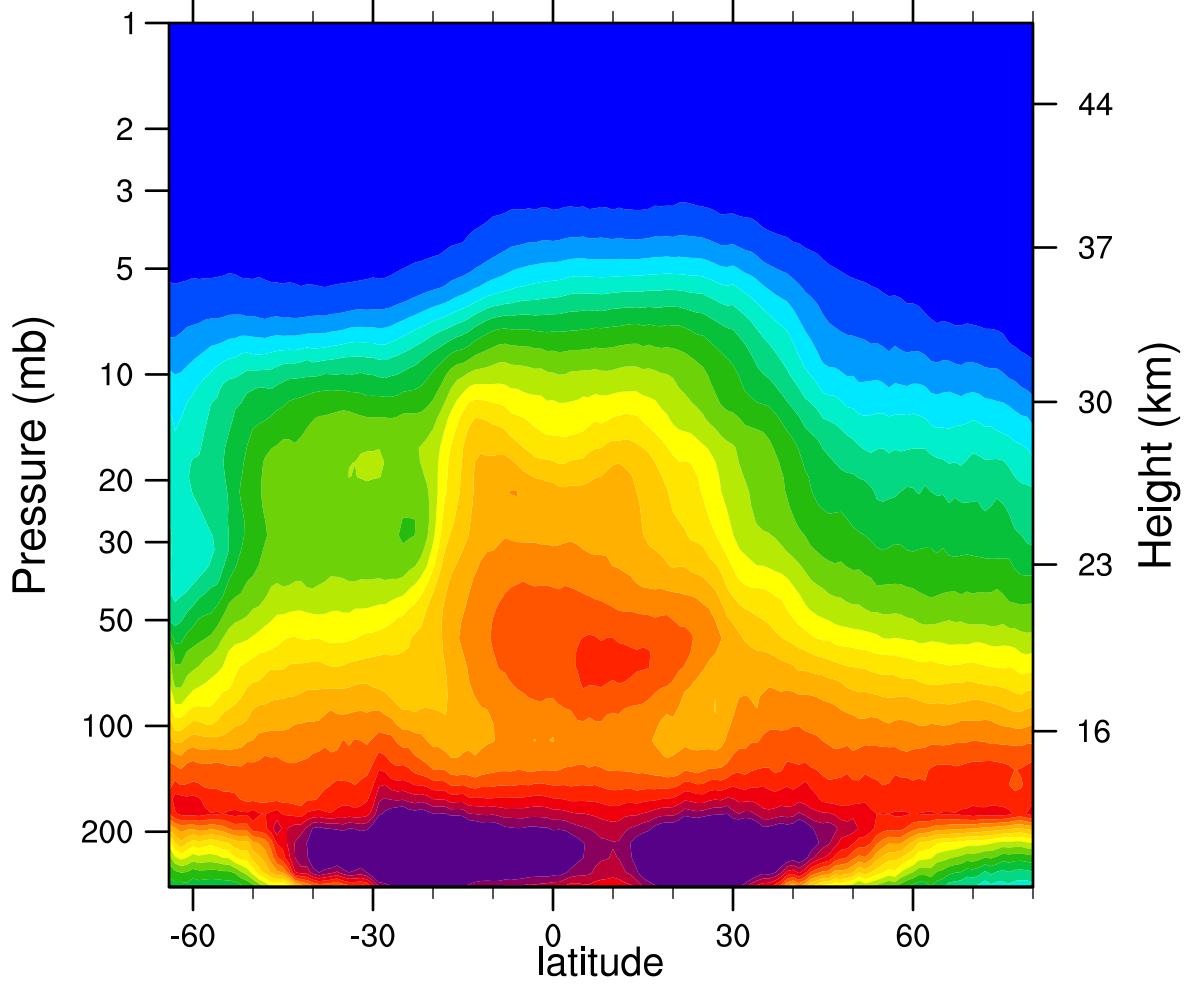
2007d289 N2O_Combined (ppbv)
