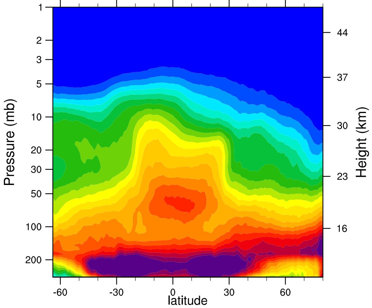
2007d344 N2O_Combined (ppbv)
