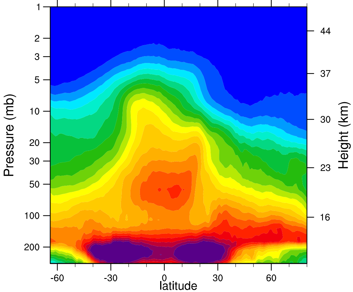
2006d029 N2O_Combined (ppbv)
