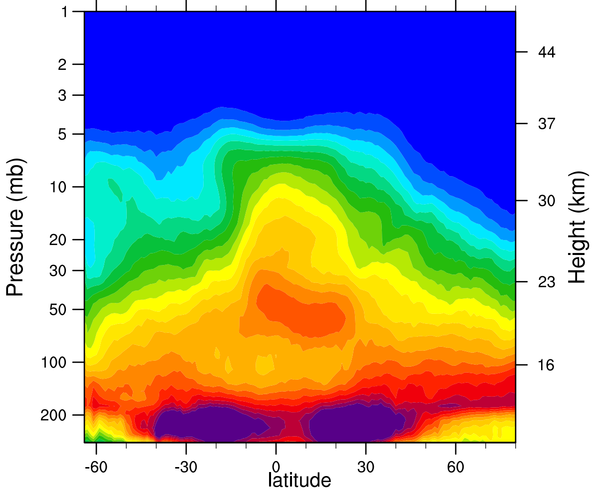
2006d316 N2O_Combined (ppbv)
