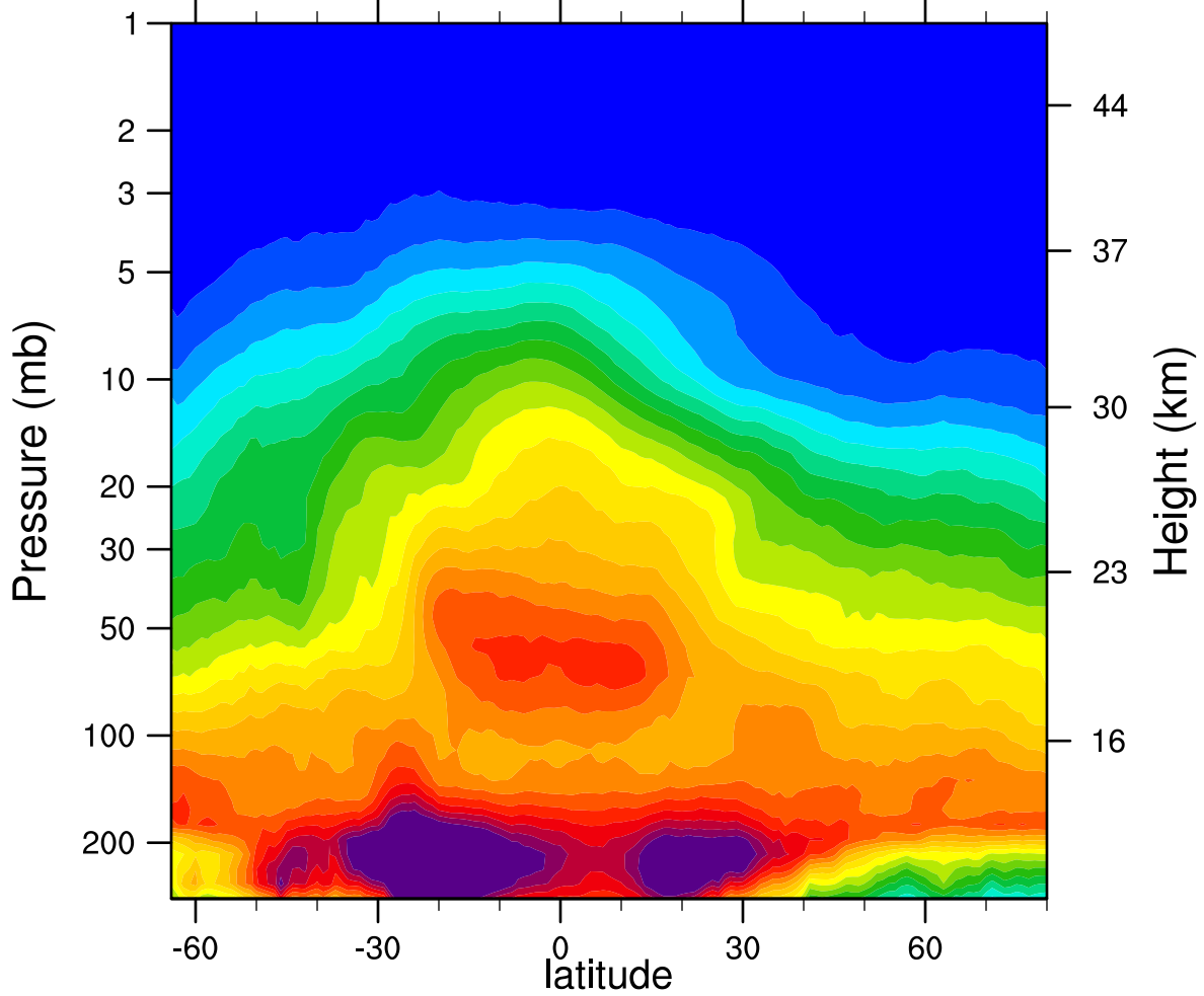
2006d127 N2O_Combined (ppbv)
