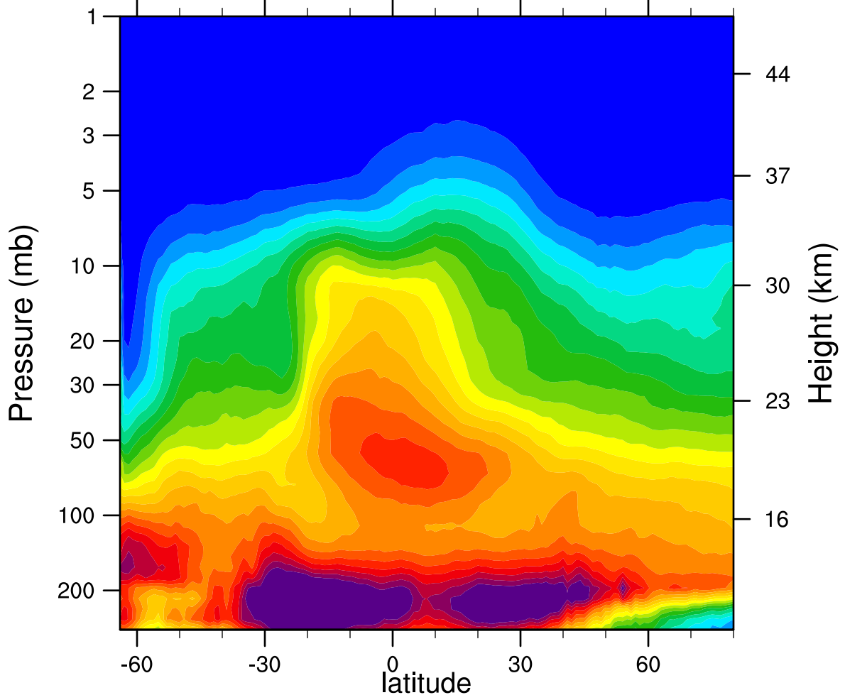
2005d193 N2O_Combined (ppbv)
