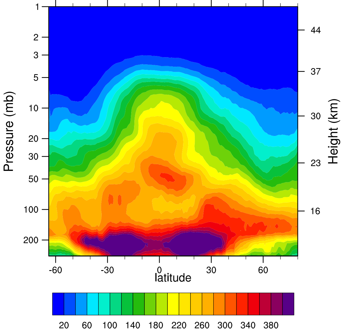
2005d075 N2O_Combined (ppbv)
