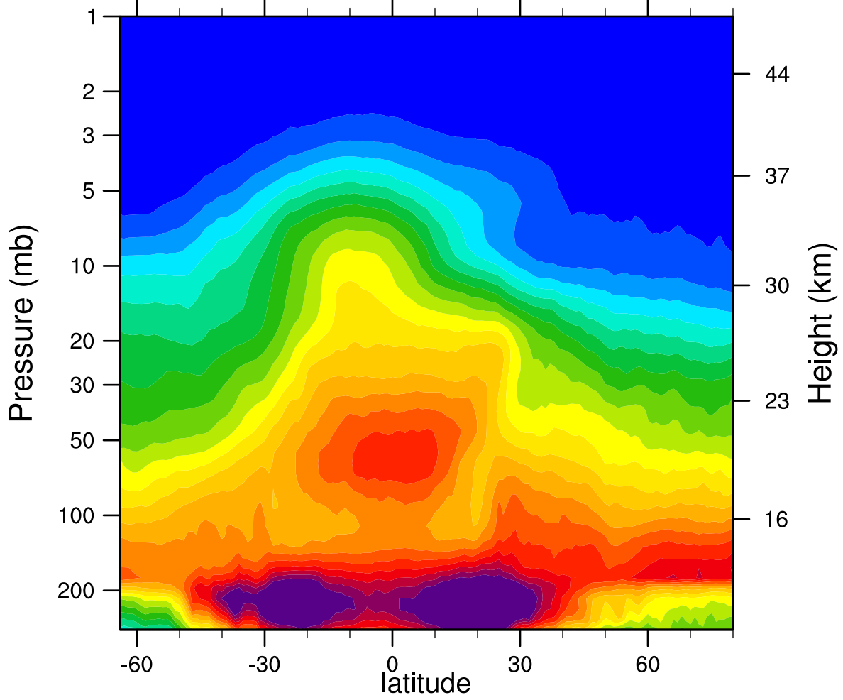
2006d057 N2O_Combined (ppbv)
