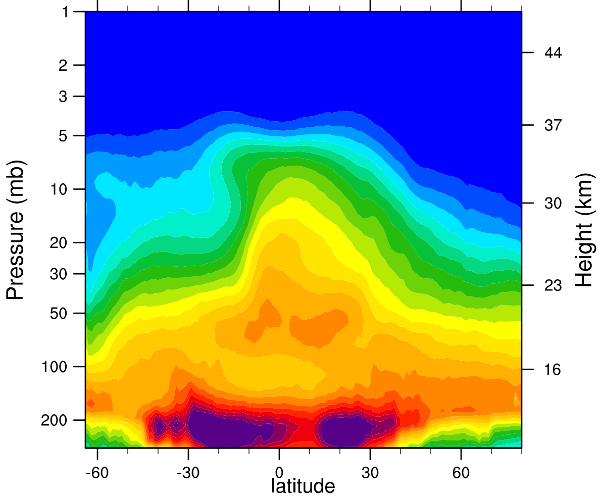
2006d293 N2O_Combined (ppbv)
