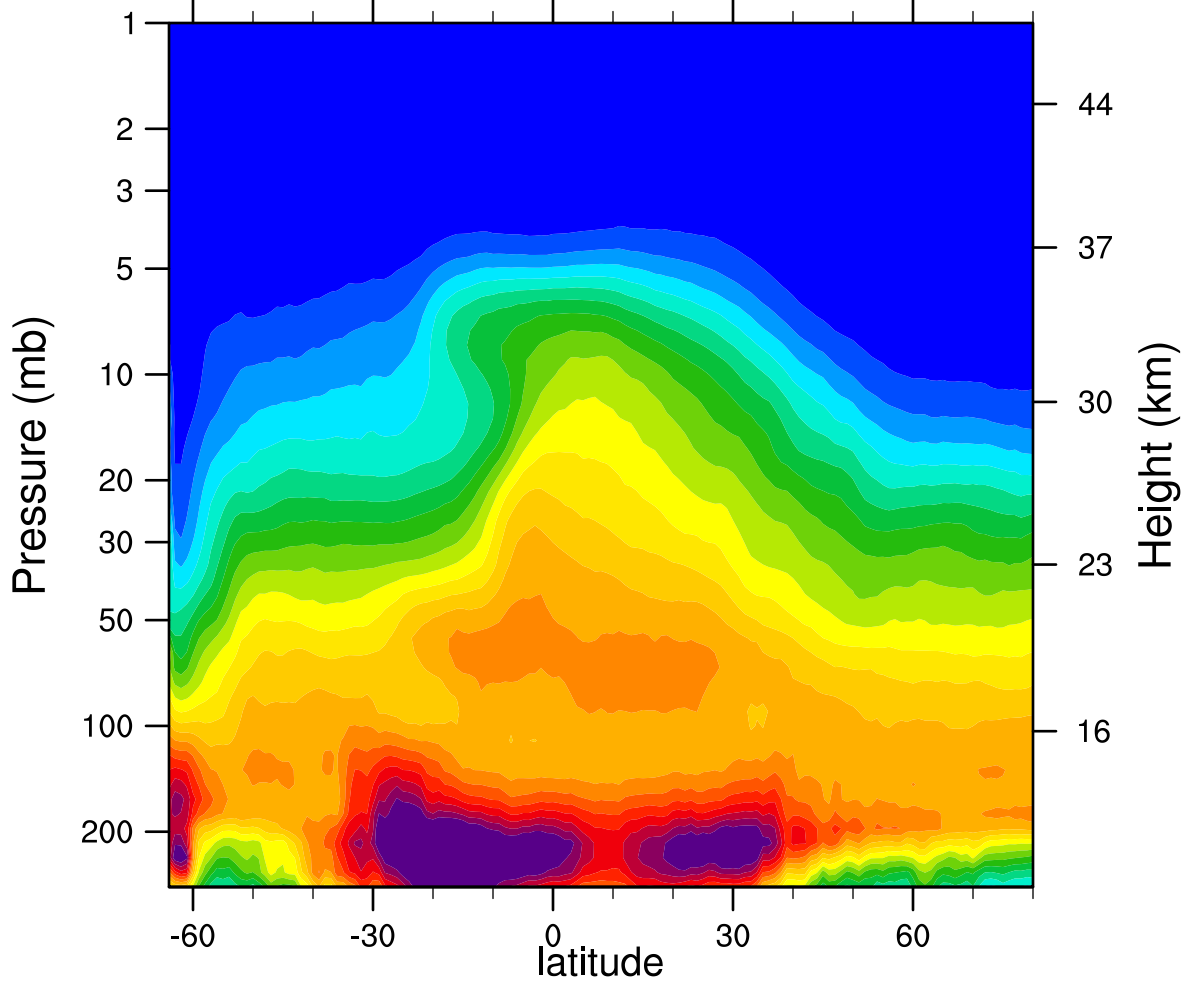
2006d260 N2O_Combined (ppbv)
