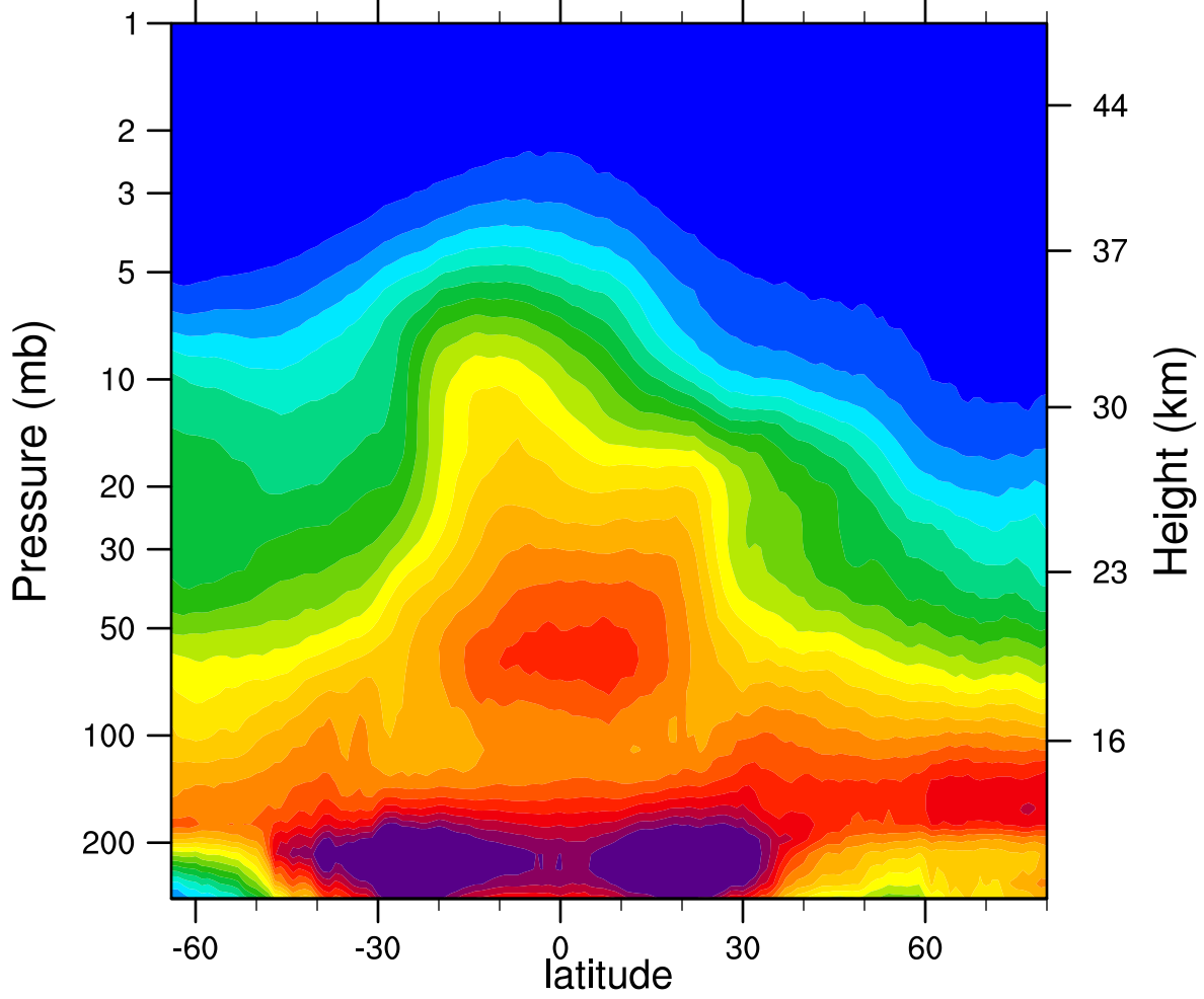
2006d005 N2O_Combined (ppbv)
