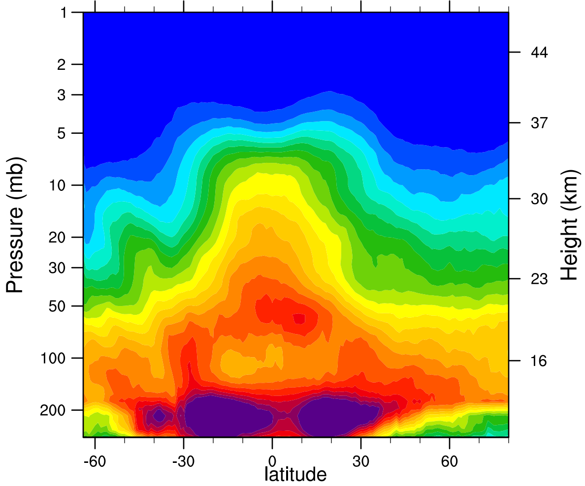
2005d116 N2O_Combined (ppbv)
