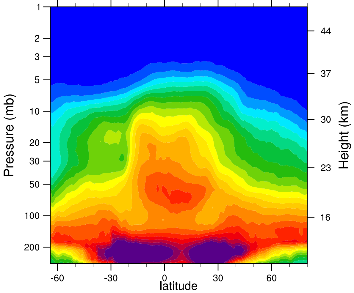
2007d285 N2O_Combined (ppbv)
