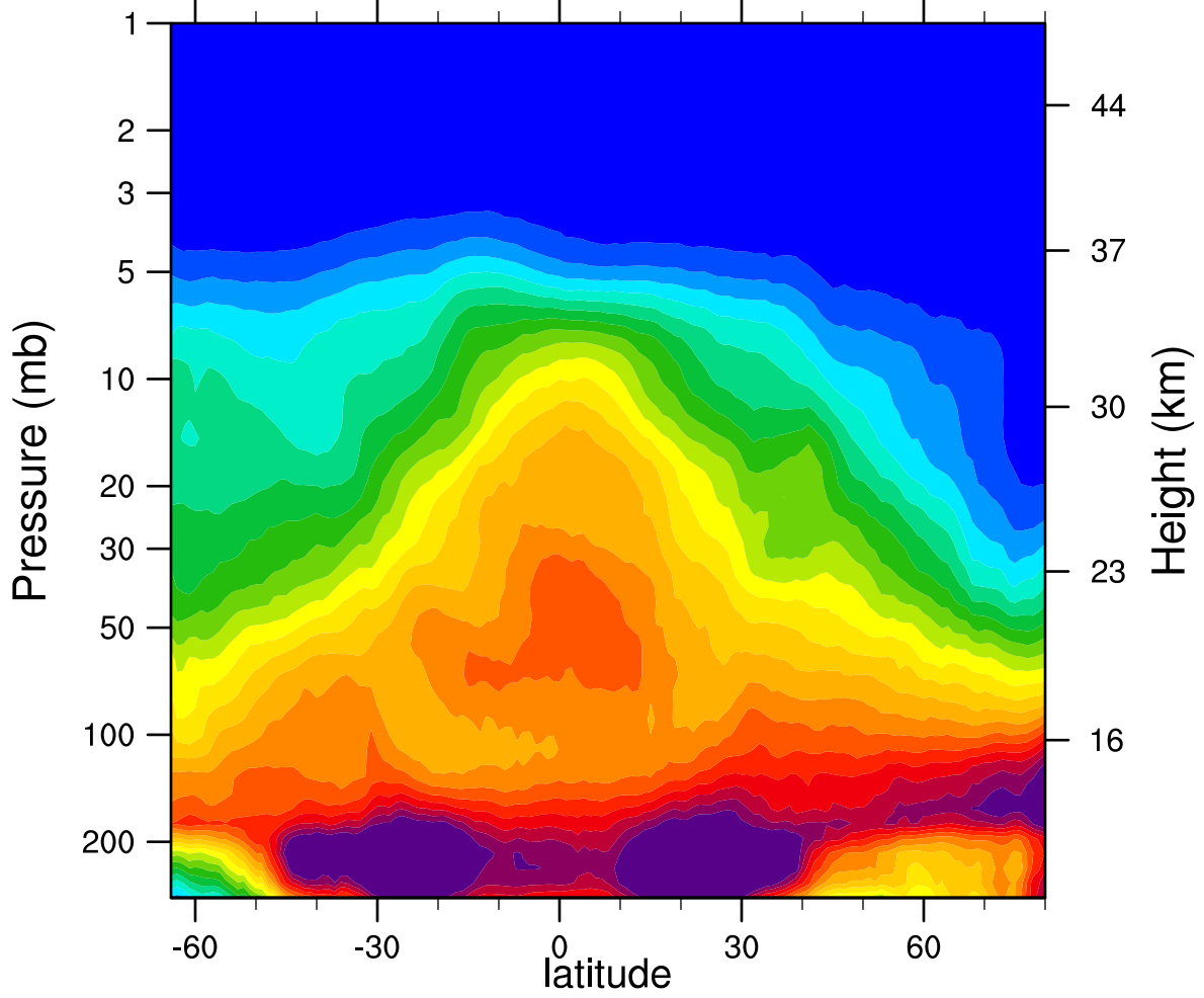
2006d352 N2O_Combined (ppbv)
