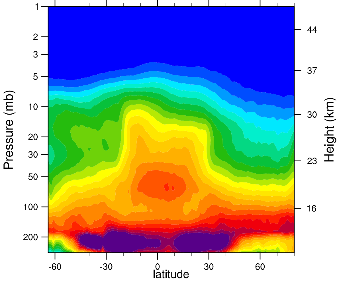
2007d329 N2O_Combined (ppbv)
