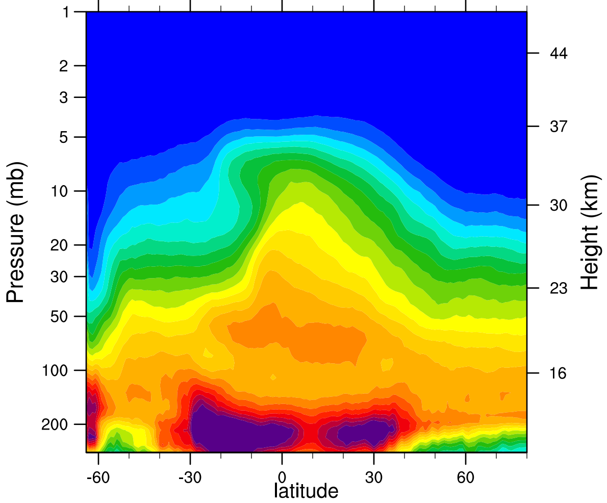
2006d259 N2O_Combined (ppbv)
