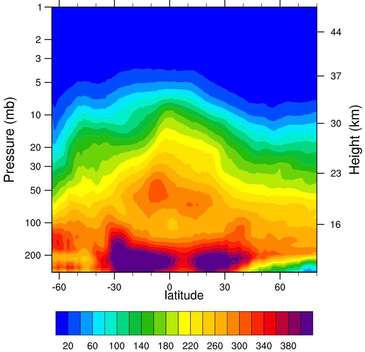
2006d172 N2O_Combined (ppbv)
