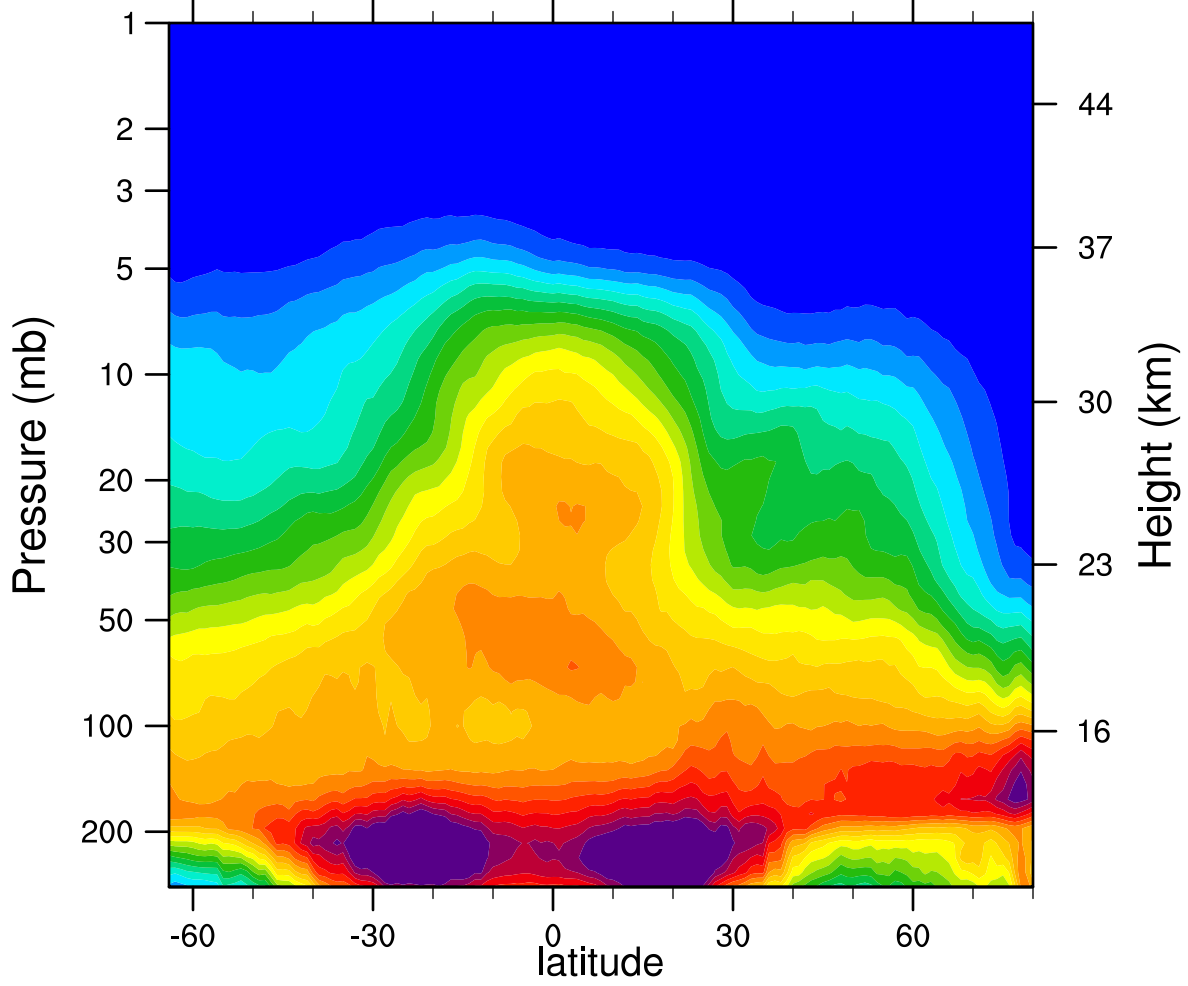
2007d021 N2O_Combined (ppbv)
