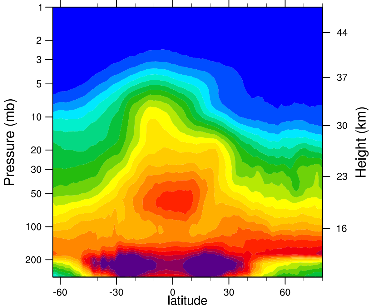
2006d048 N2O_Combined (ppbv)
