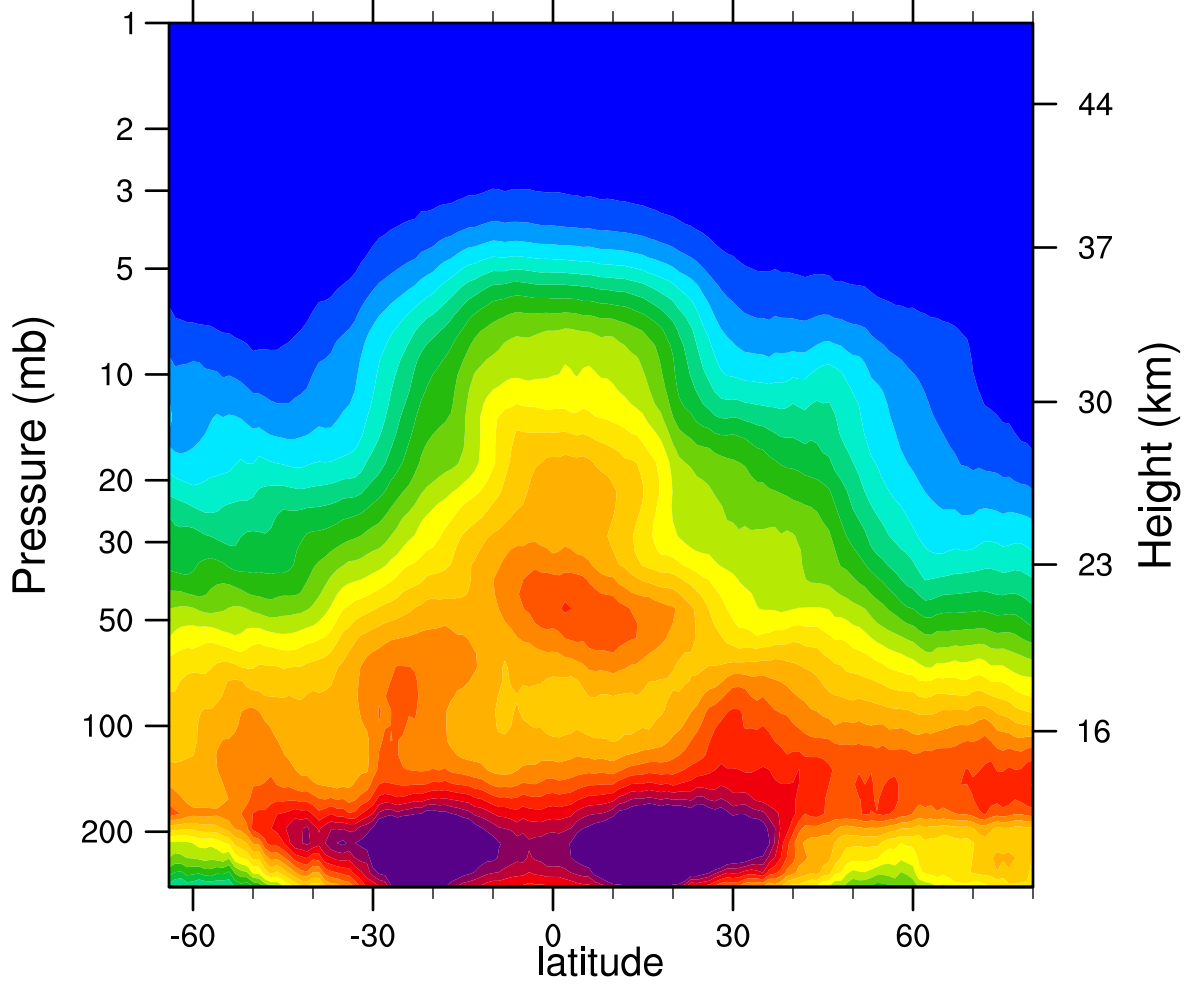
2005d068 N2O_Combined (ppbv)
