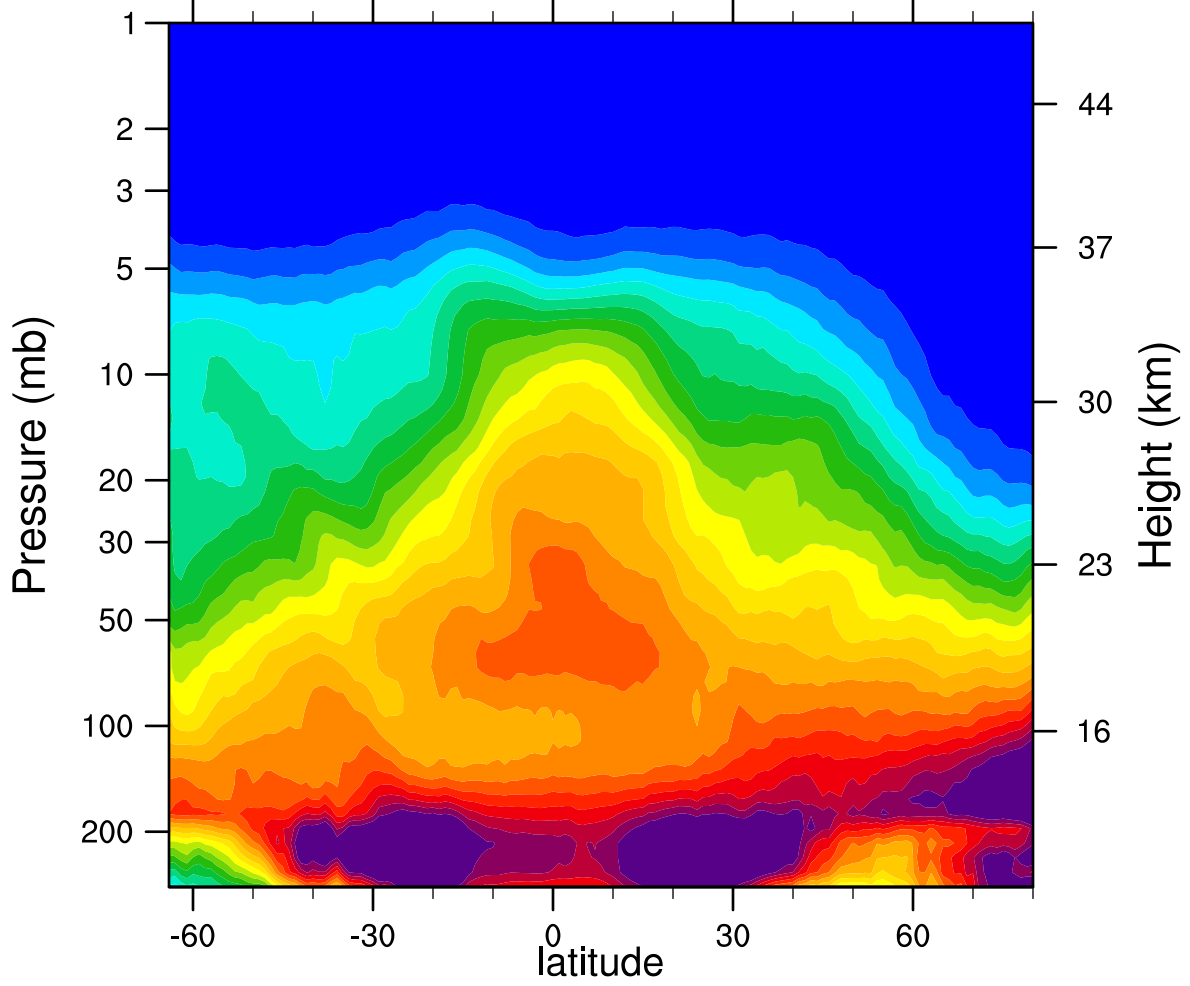
2006d340 N2O_Combined (ppbv)
