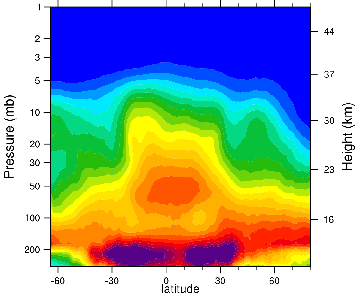
2005d323 N2O_Combined (ppbv)
