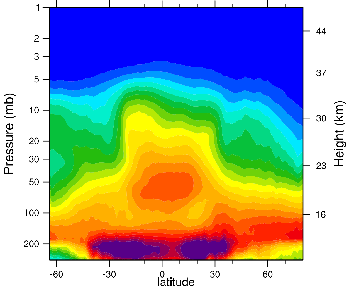
2005d327 N2O_Combined (ppbv)
