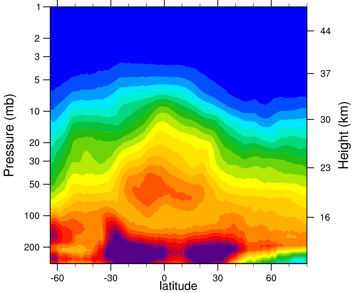
2006d164 N2O_Combined (ppbv)
