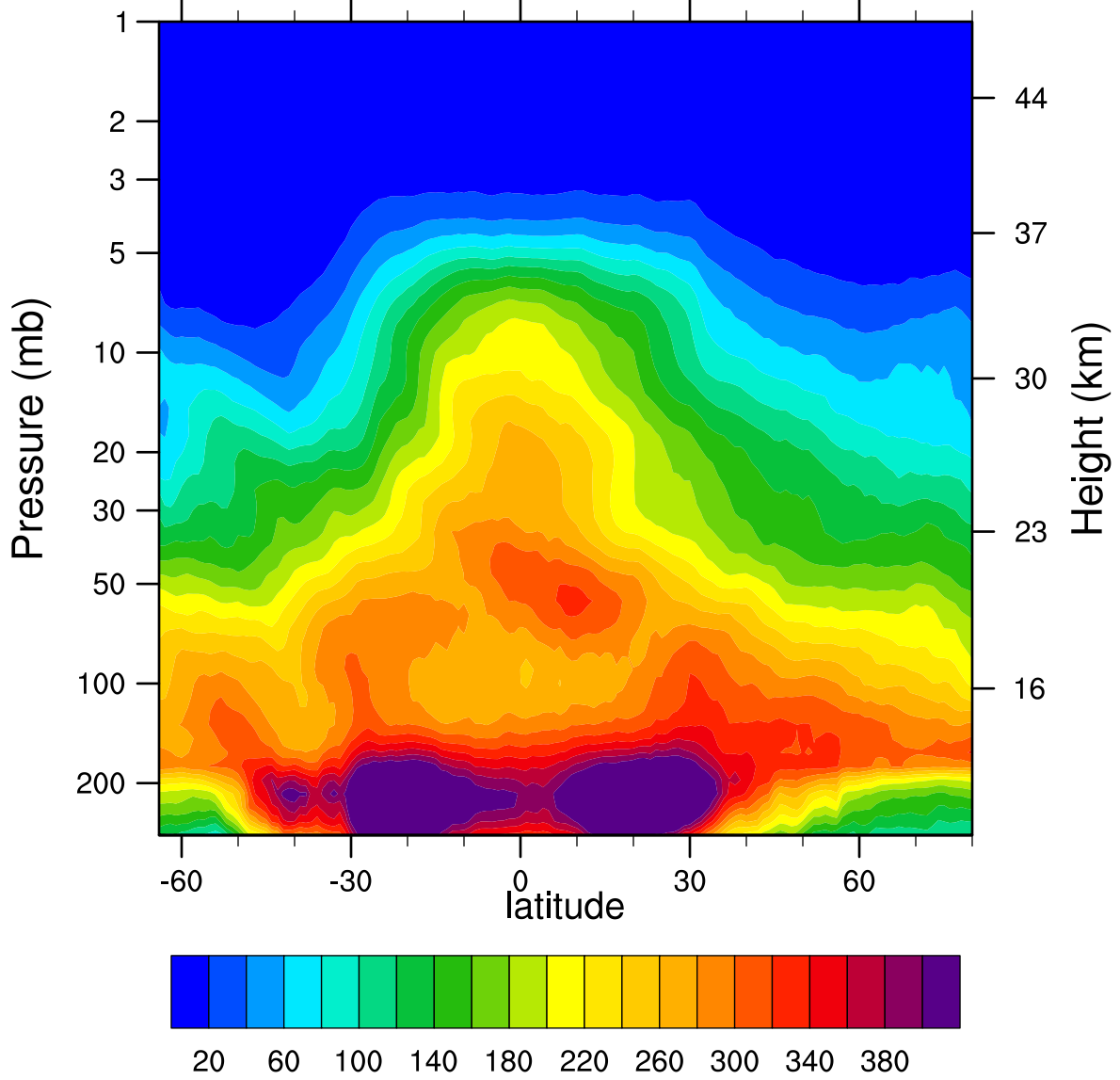
2005d091 N2O_Combined (ppbv)
