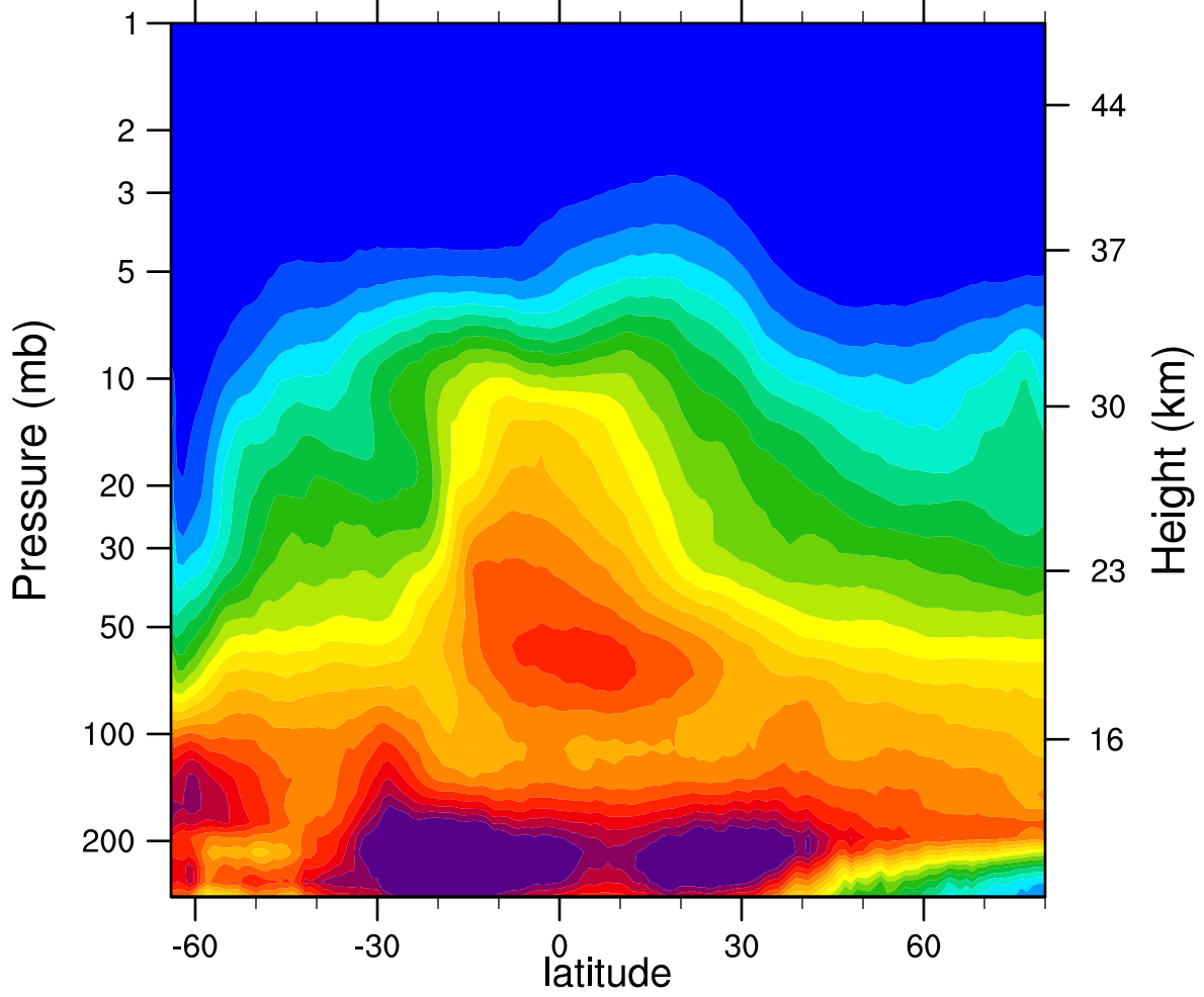
2005d178 N2O_Combined (ppbv)
