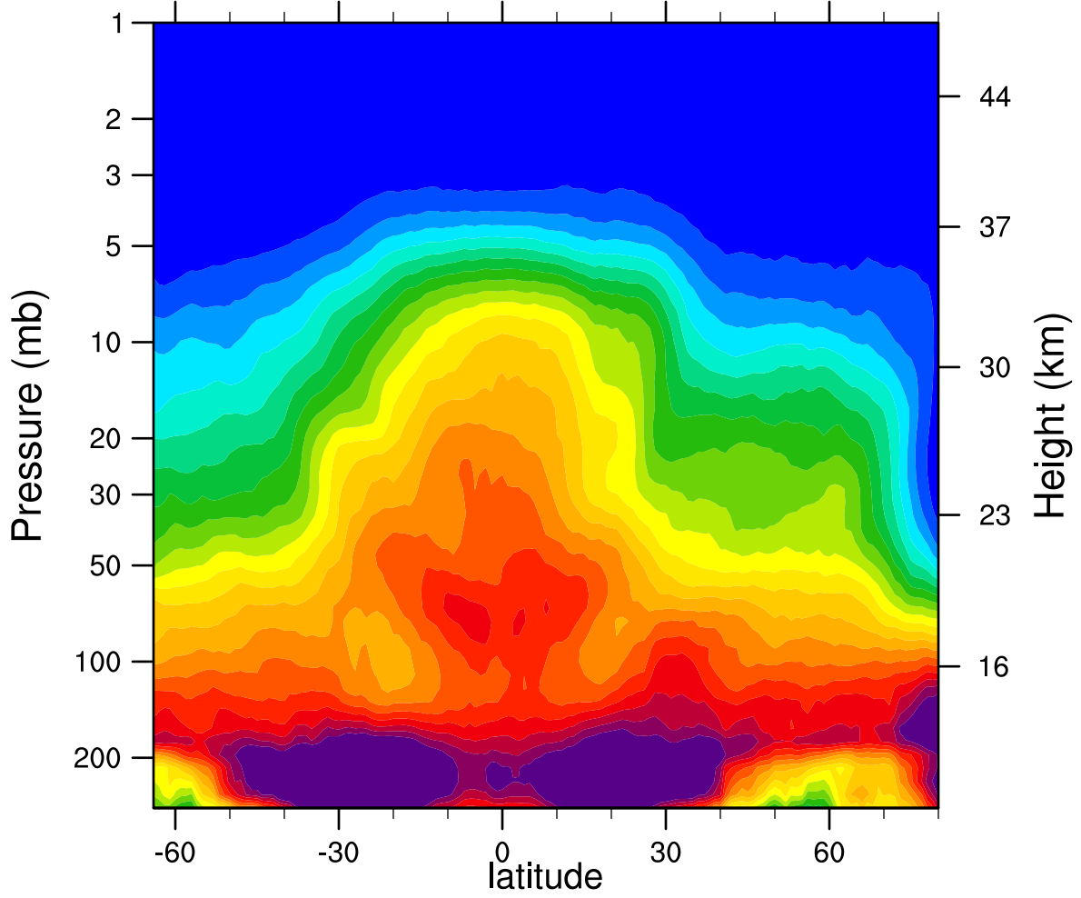
2007d084 N2O_Combined (ppbv)
