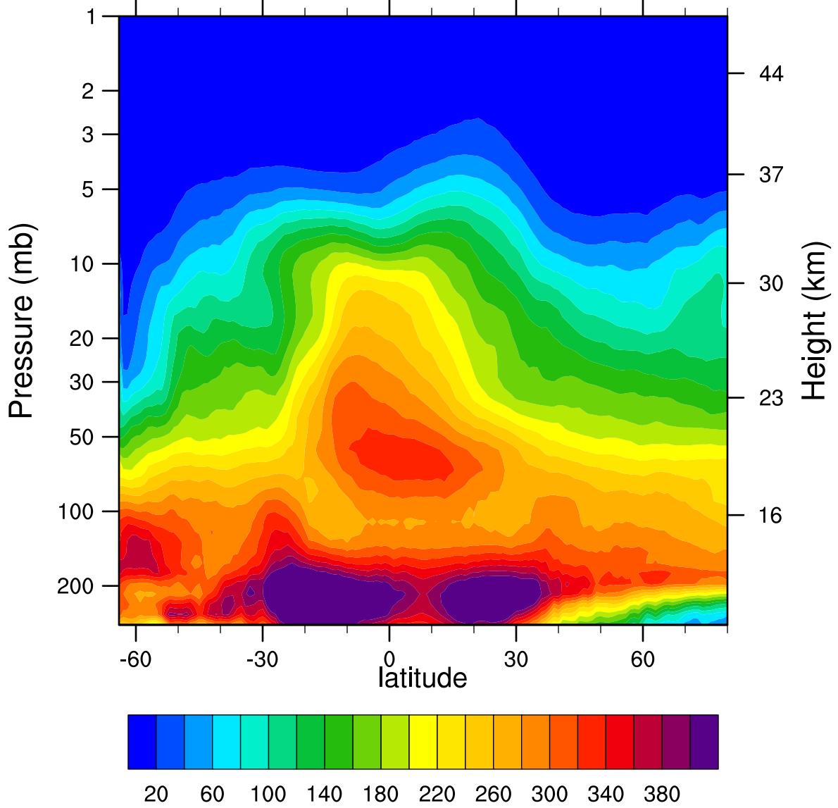
2005d169 N2O_Combined (ppbv)
