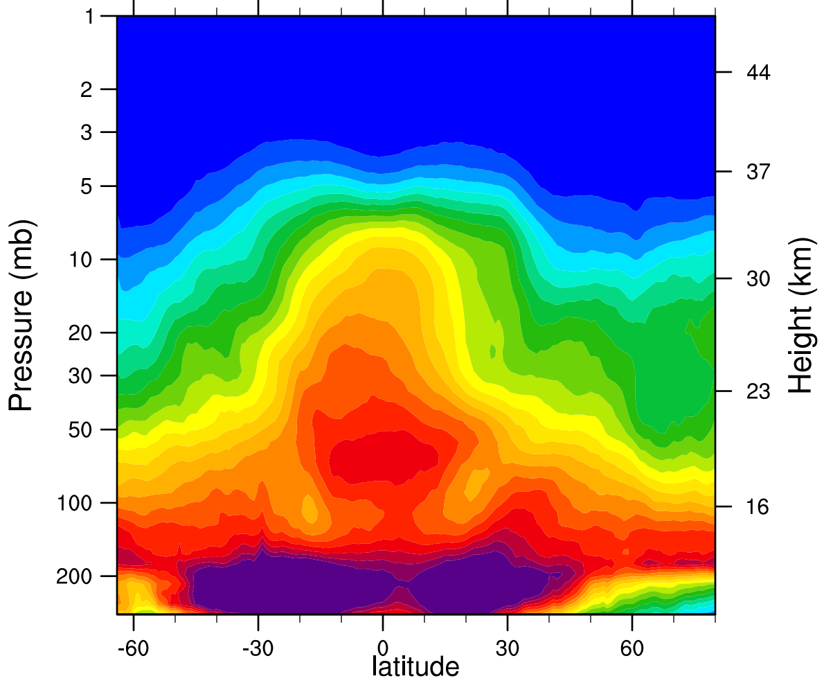
2007d118 N2O_Combined (ppbv)
