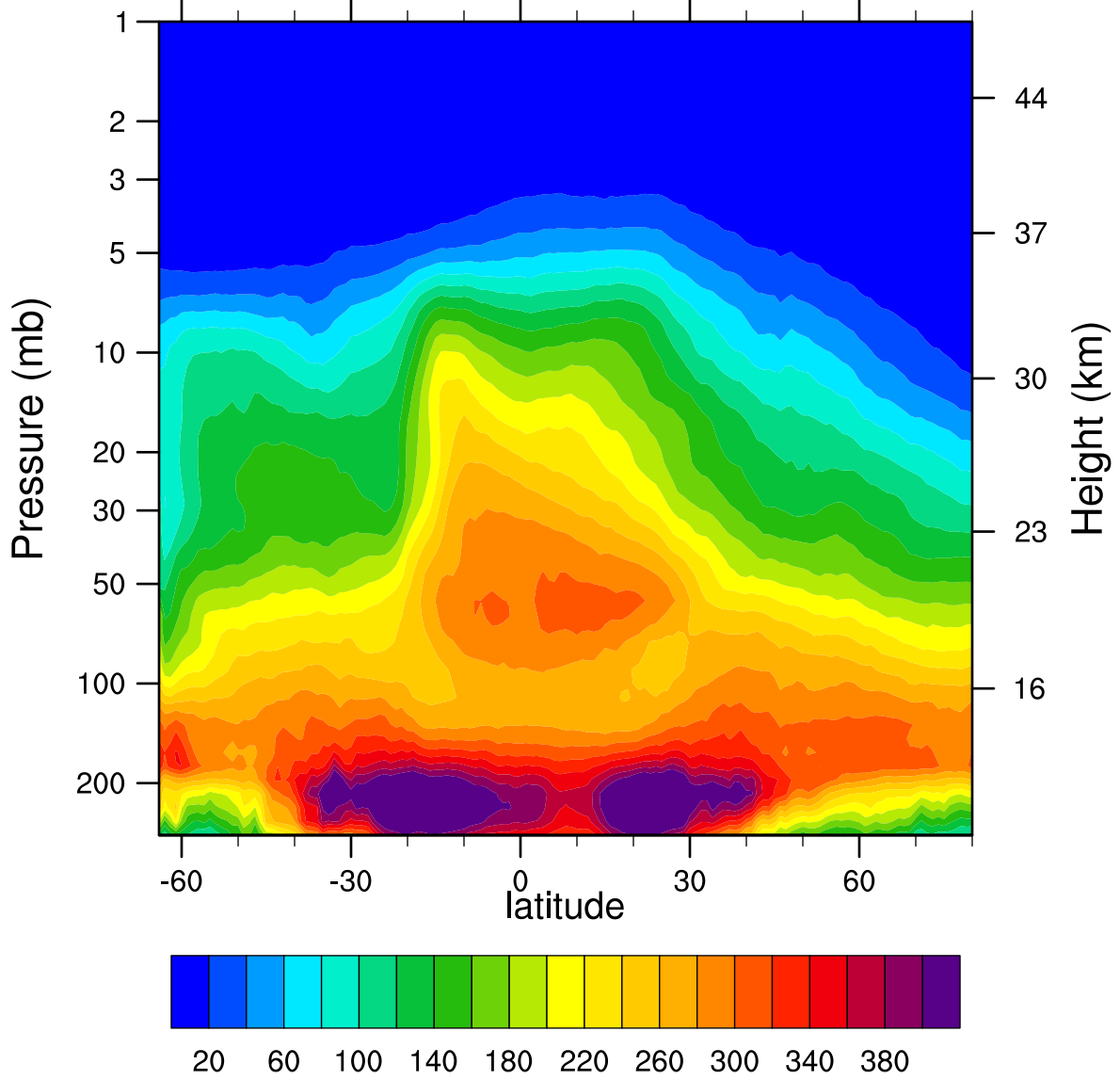
2005d294 N2O_Combined (ppbv)
