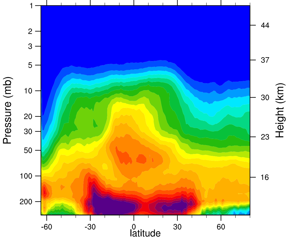
2007d204 N2O_Combined (ppbv)
