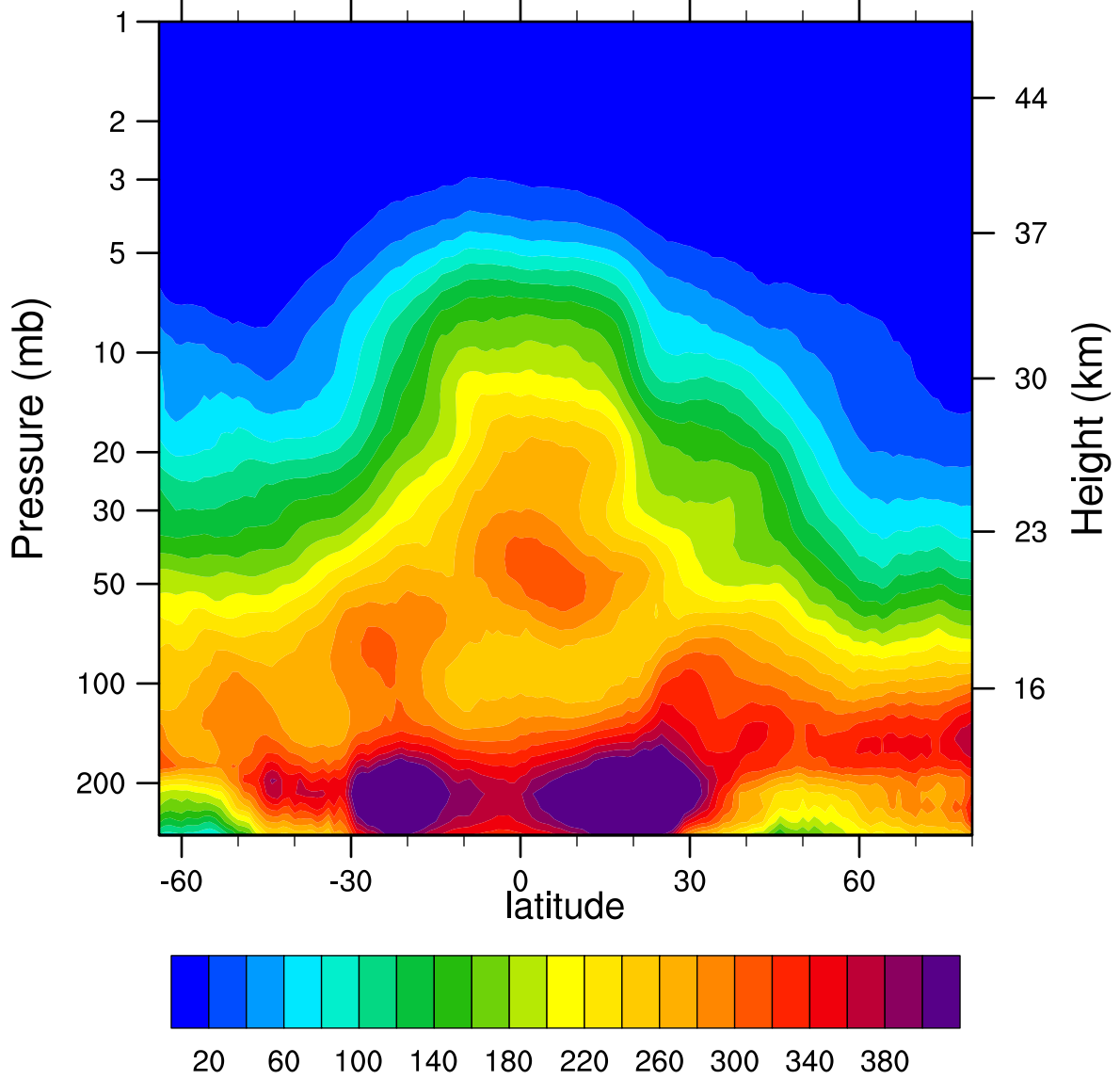
2005d055 N2O_Combined (ppbv)
