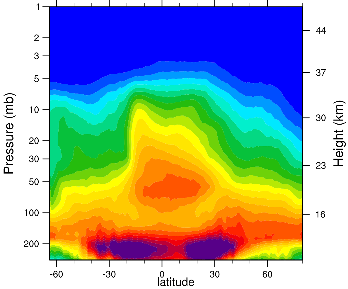
2005d301 N2O_Combined (ppbv)
