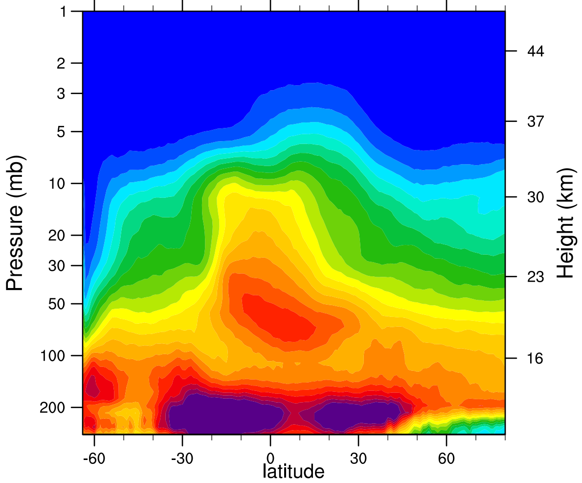
2005d203 N2O_Combined (ppbv)
