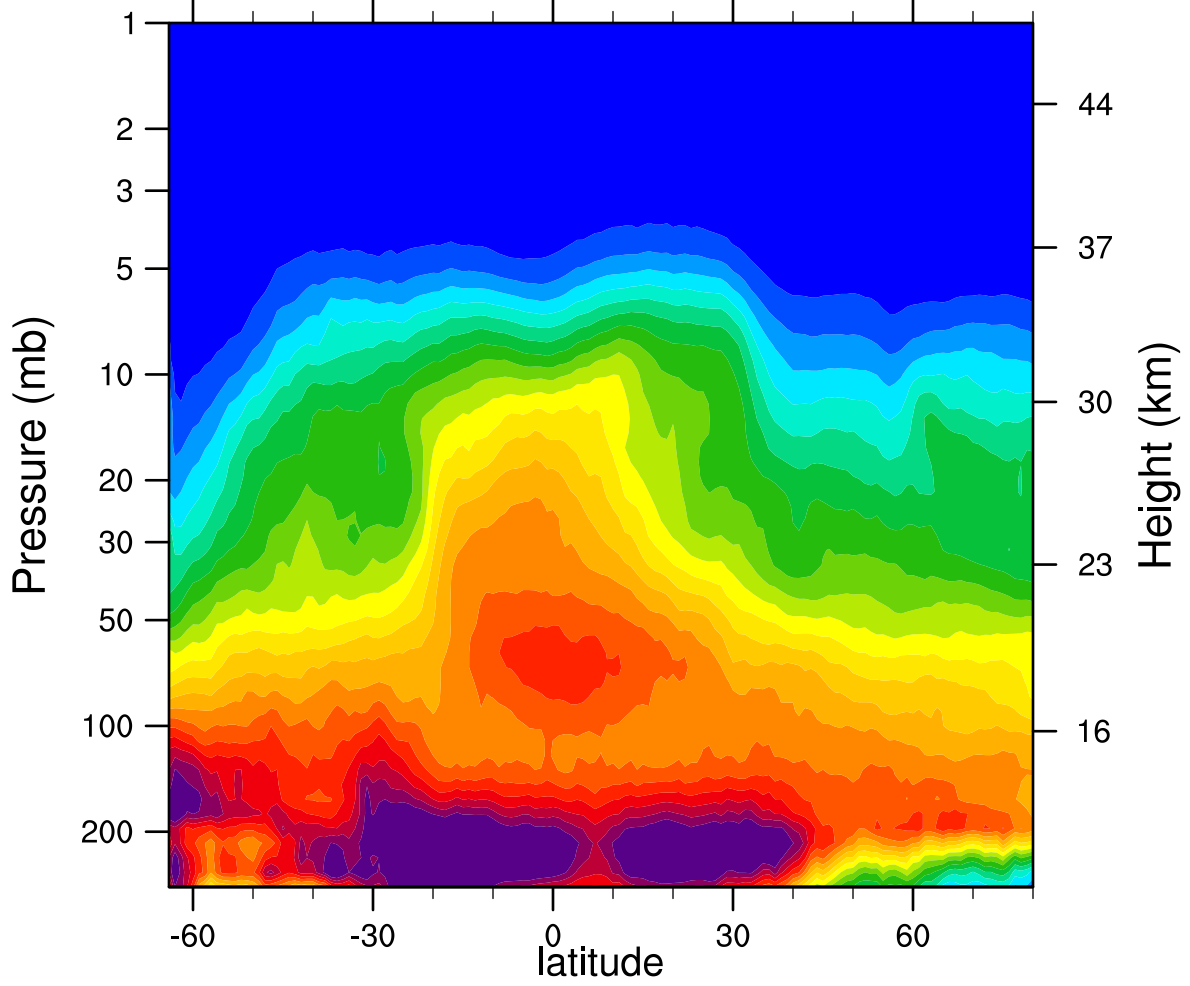
2007d162 N2O_Combined (ppbv)
