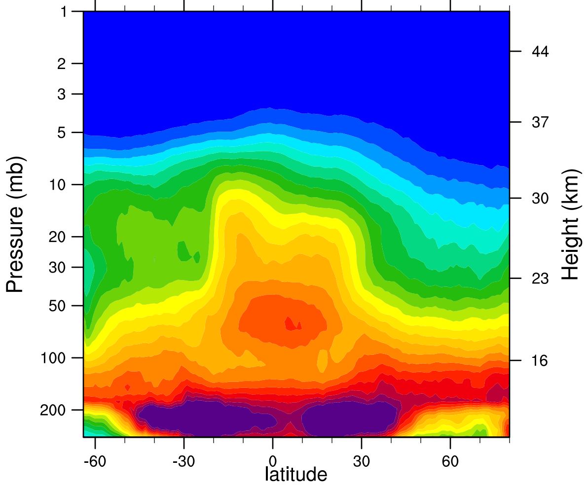
2007d327 N2O_Combined (ppbv)
