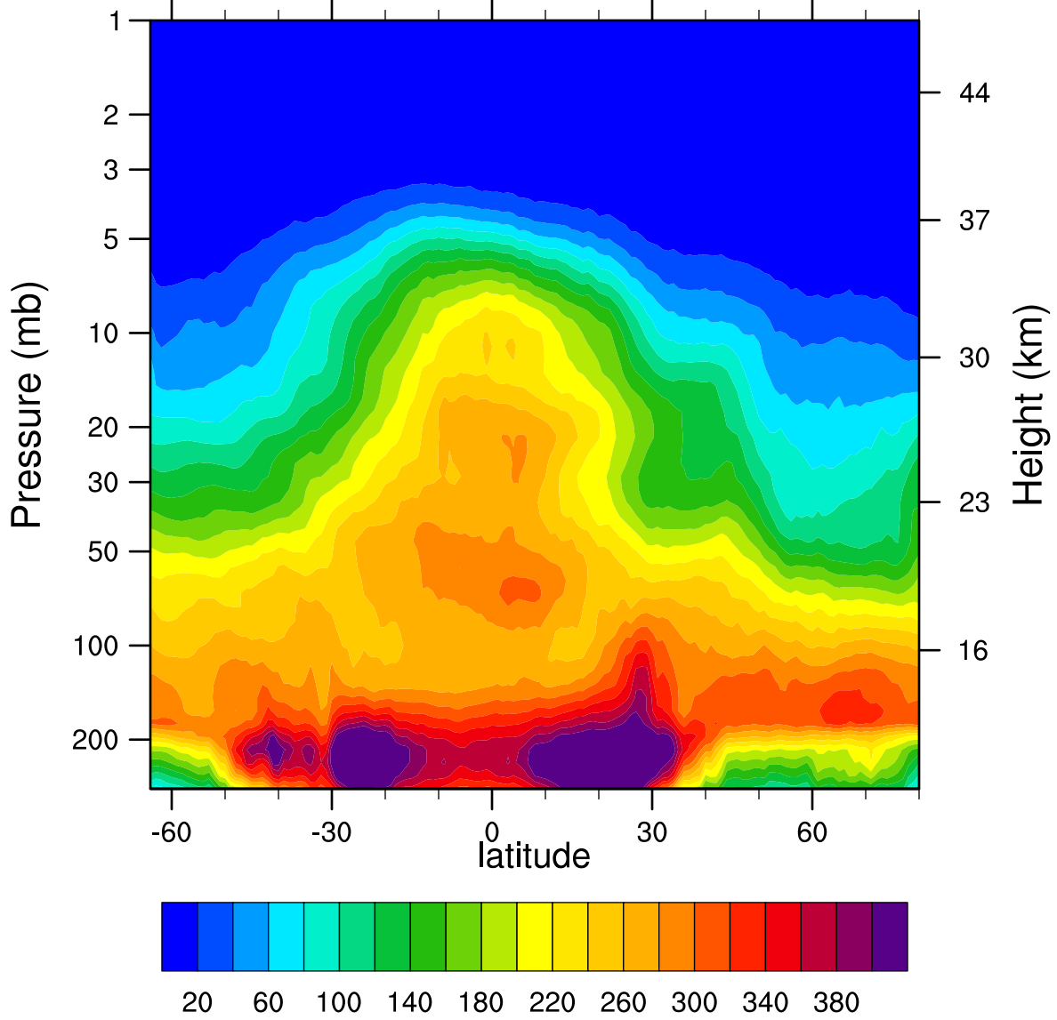
2007d057 N2O_Combined (ppbv)
