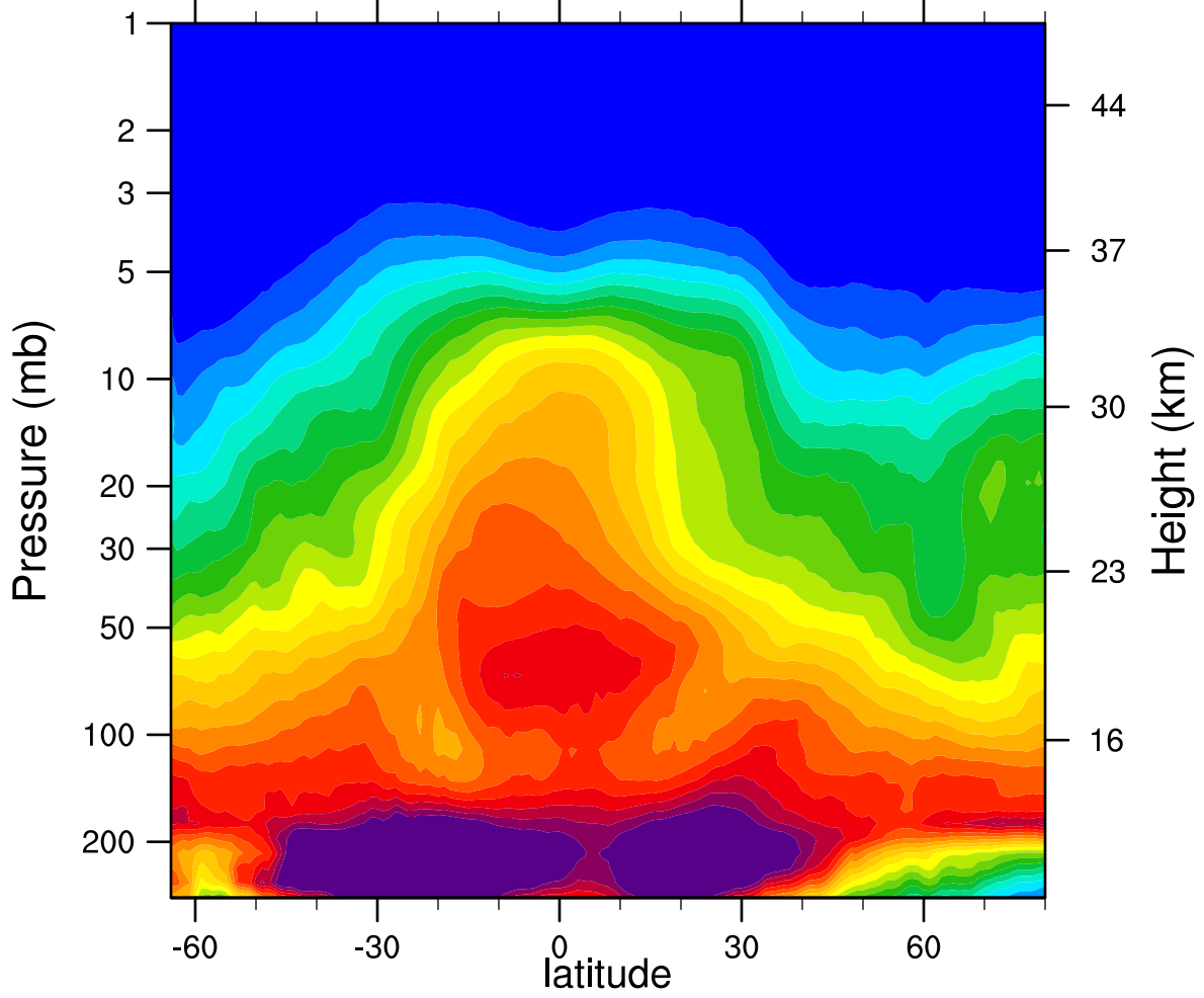
2007d122 N2O_Combined (ppbv)
