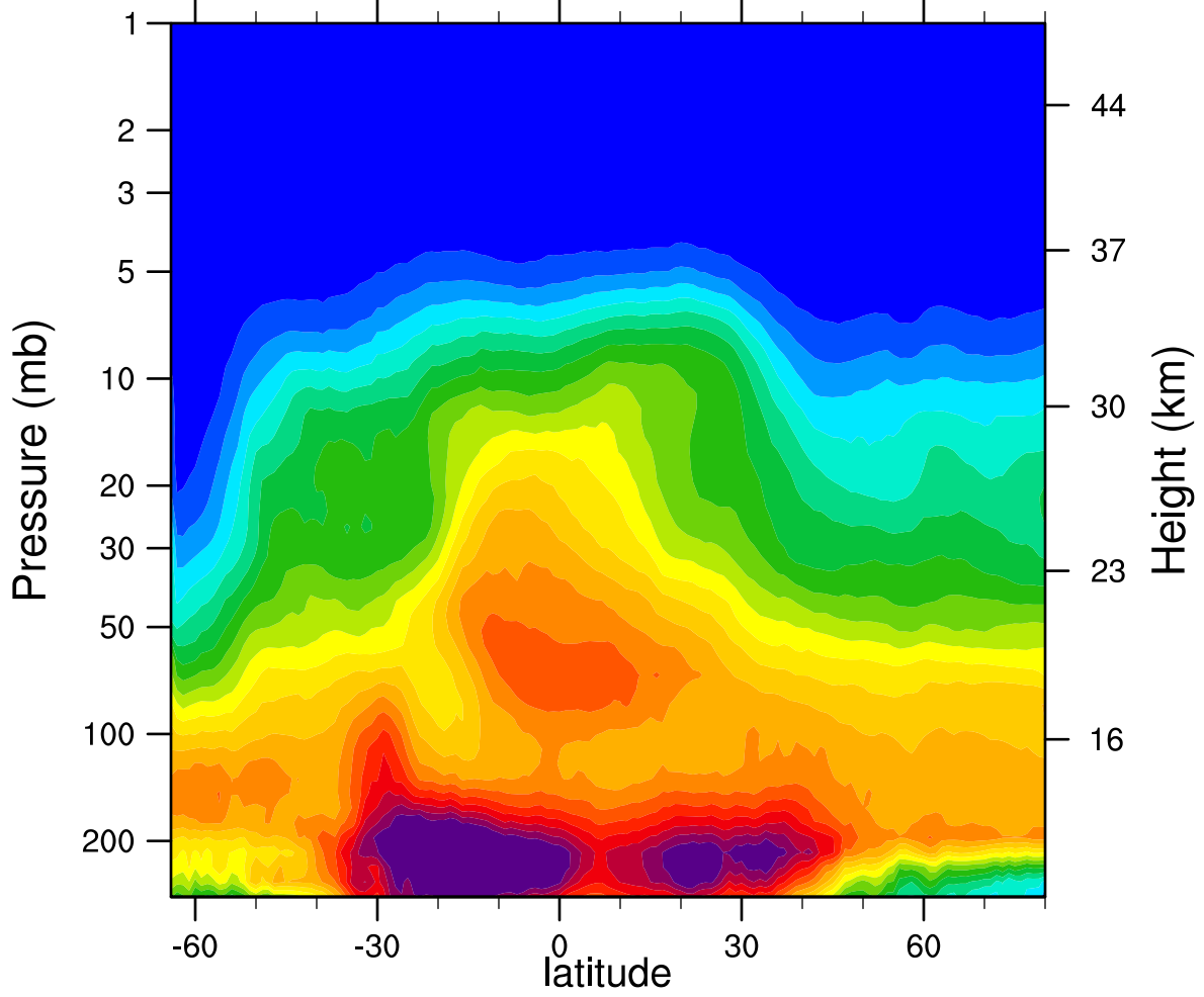
2007d190 N2O_Combined (ppbv)
