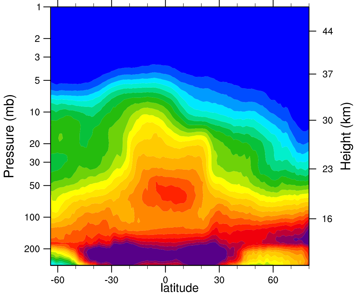
2007d357 N2O_Combined (ppbv)
