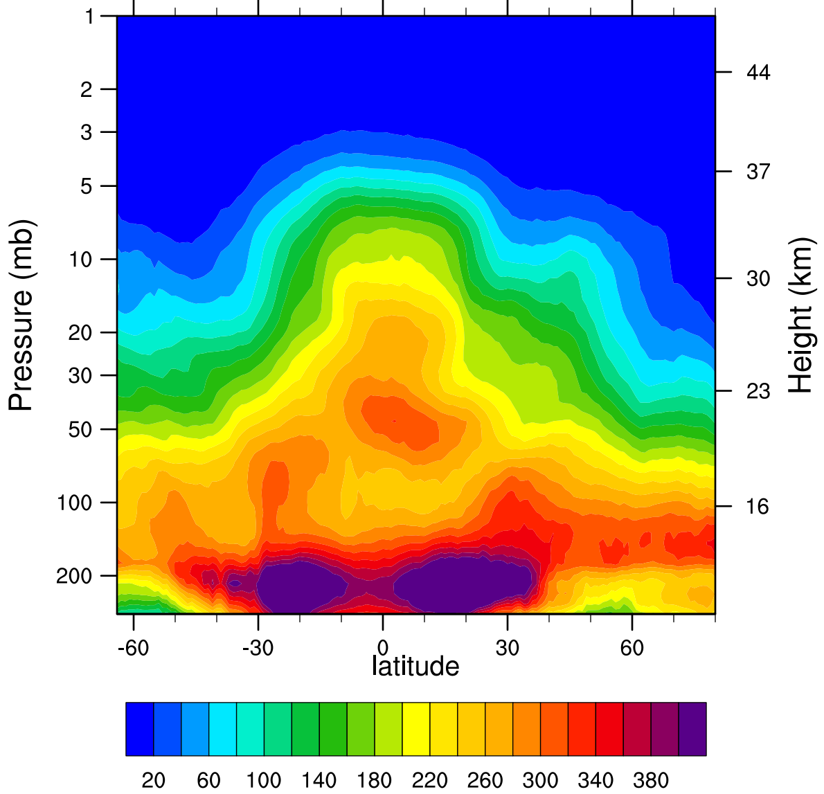
2005d067 N2O_Combined (ppbv)
