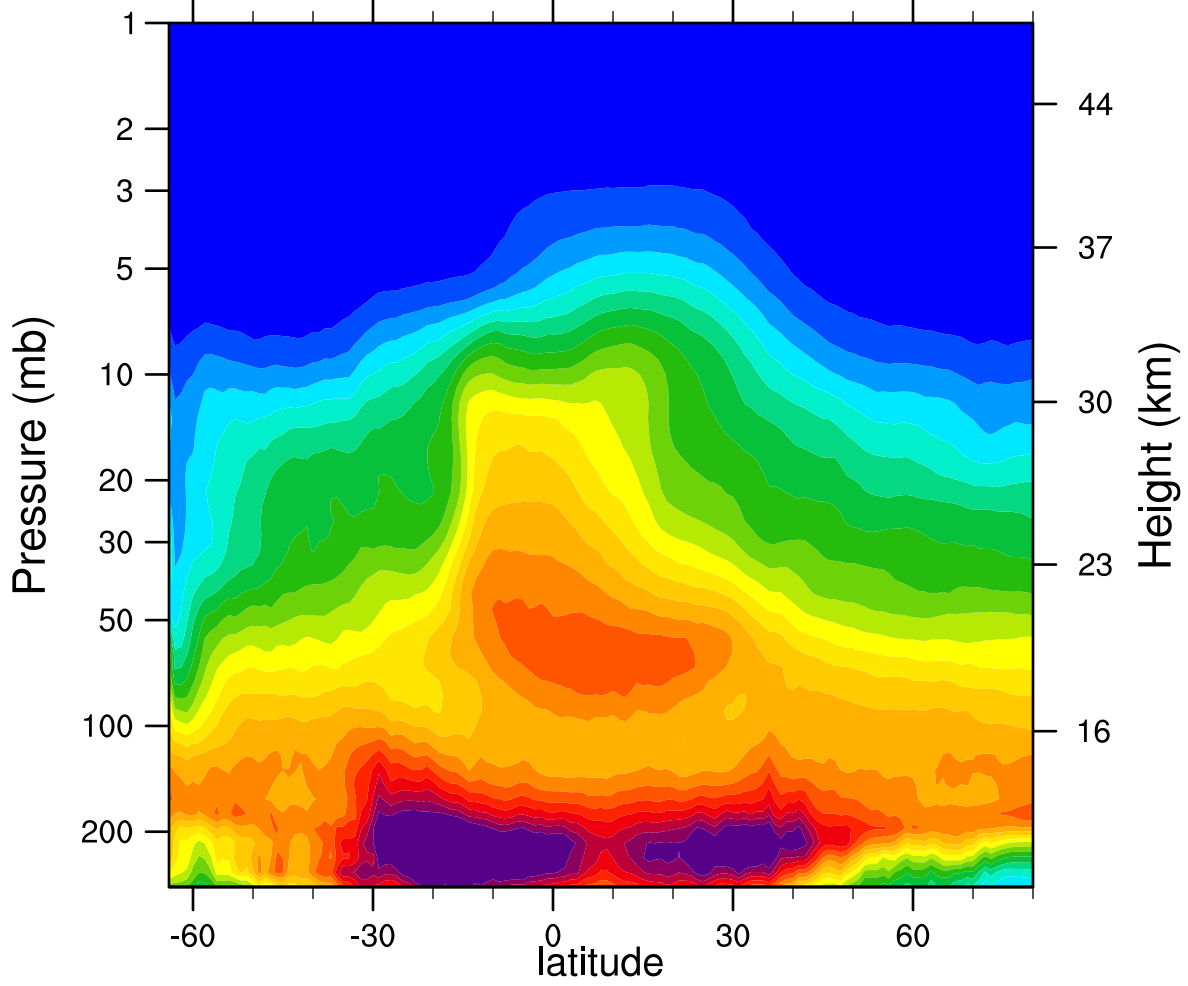
2005d243 N2O_Combined (ppbv)
