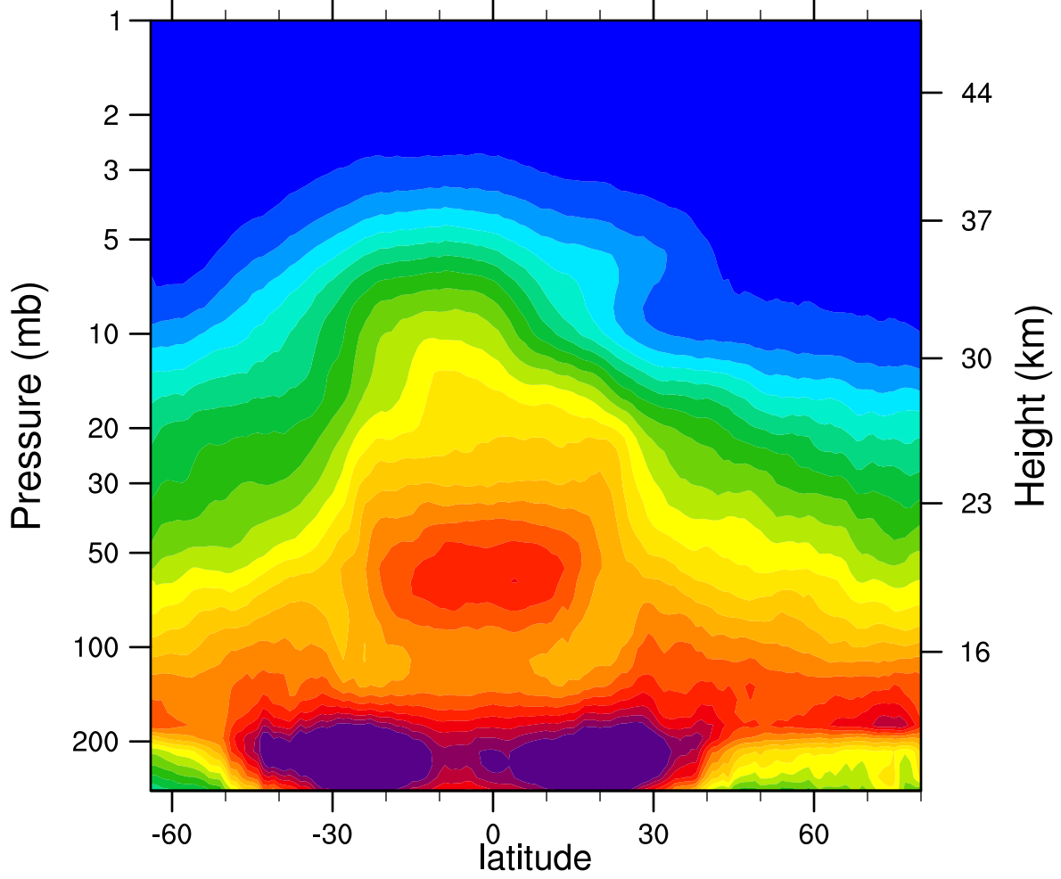
2006d079 N2O_Combined (ppbv)
