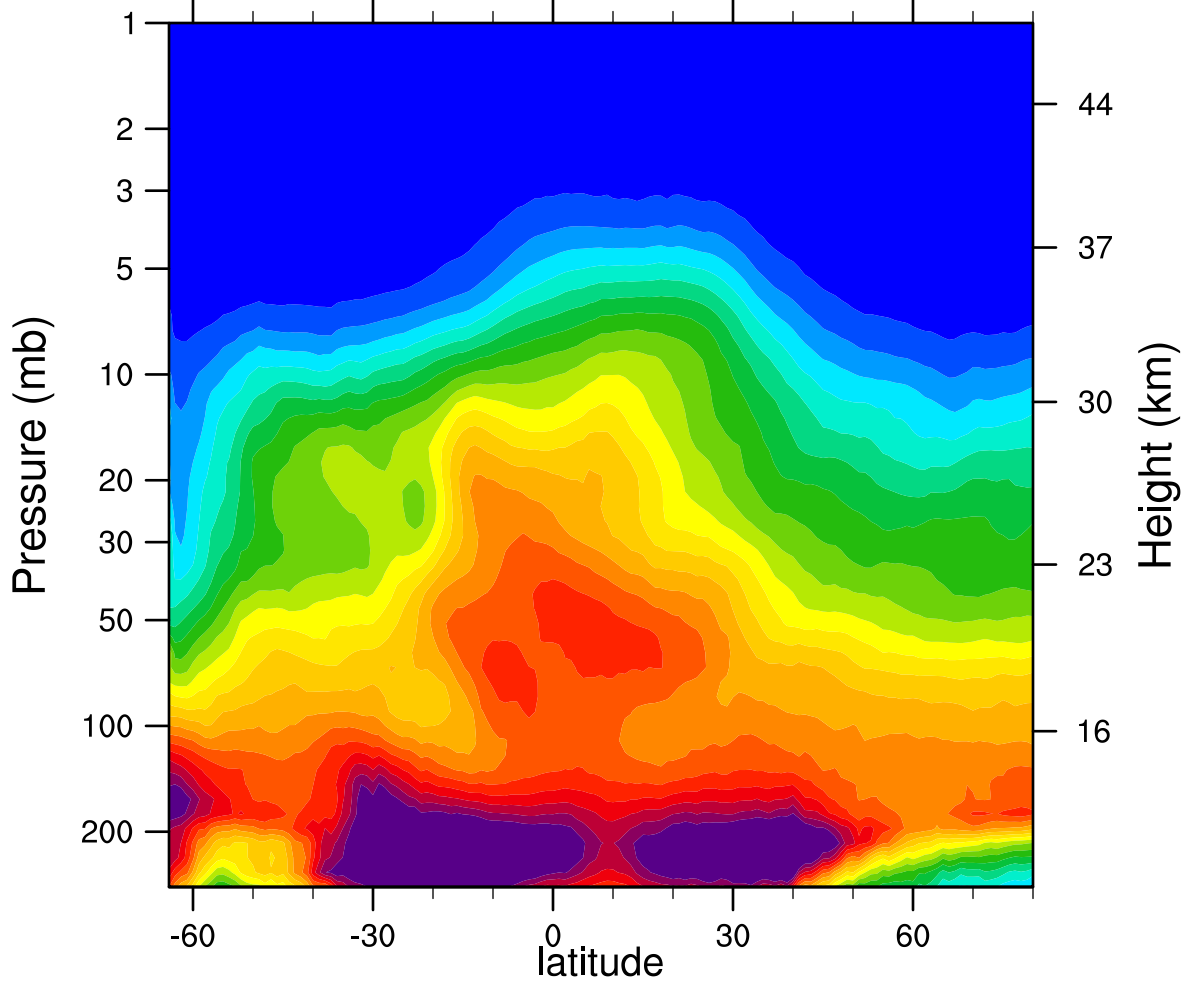
2007d243 N2O_Combined (ppbv)
