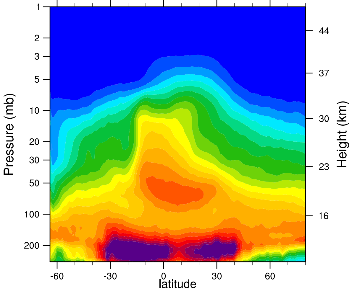
2005d246 N2O_Combined (ppbv)
