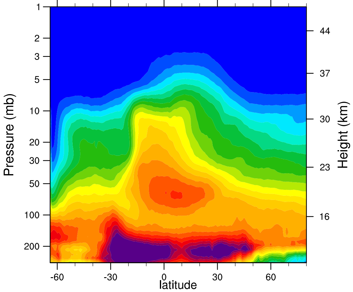
2005d229 N2O_Combined (ppbv)
