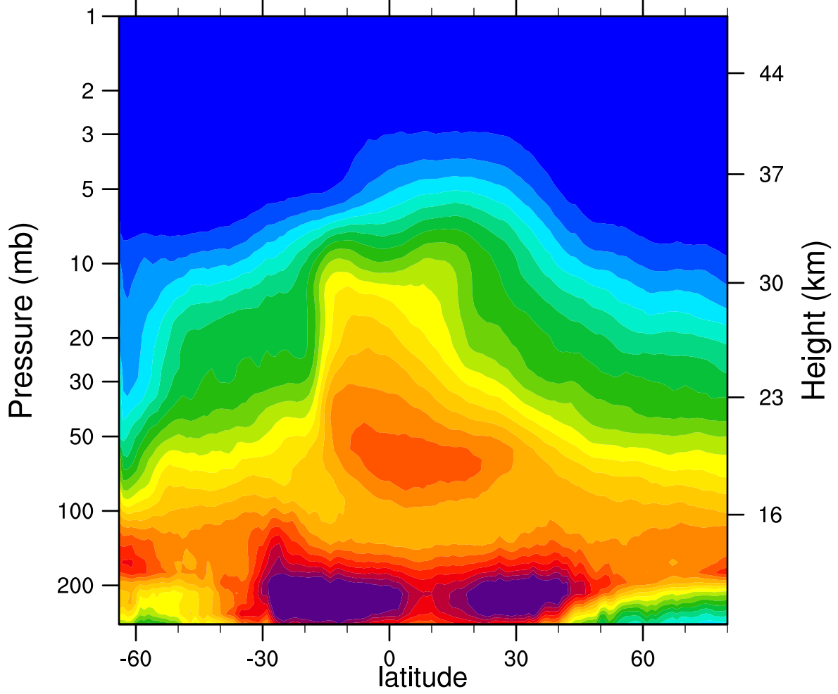
2005d252 N2O_Combined (ppbv)
