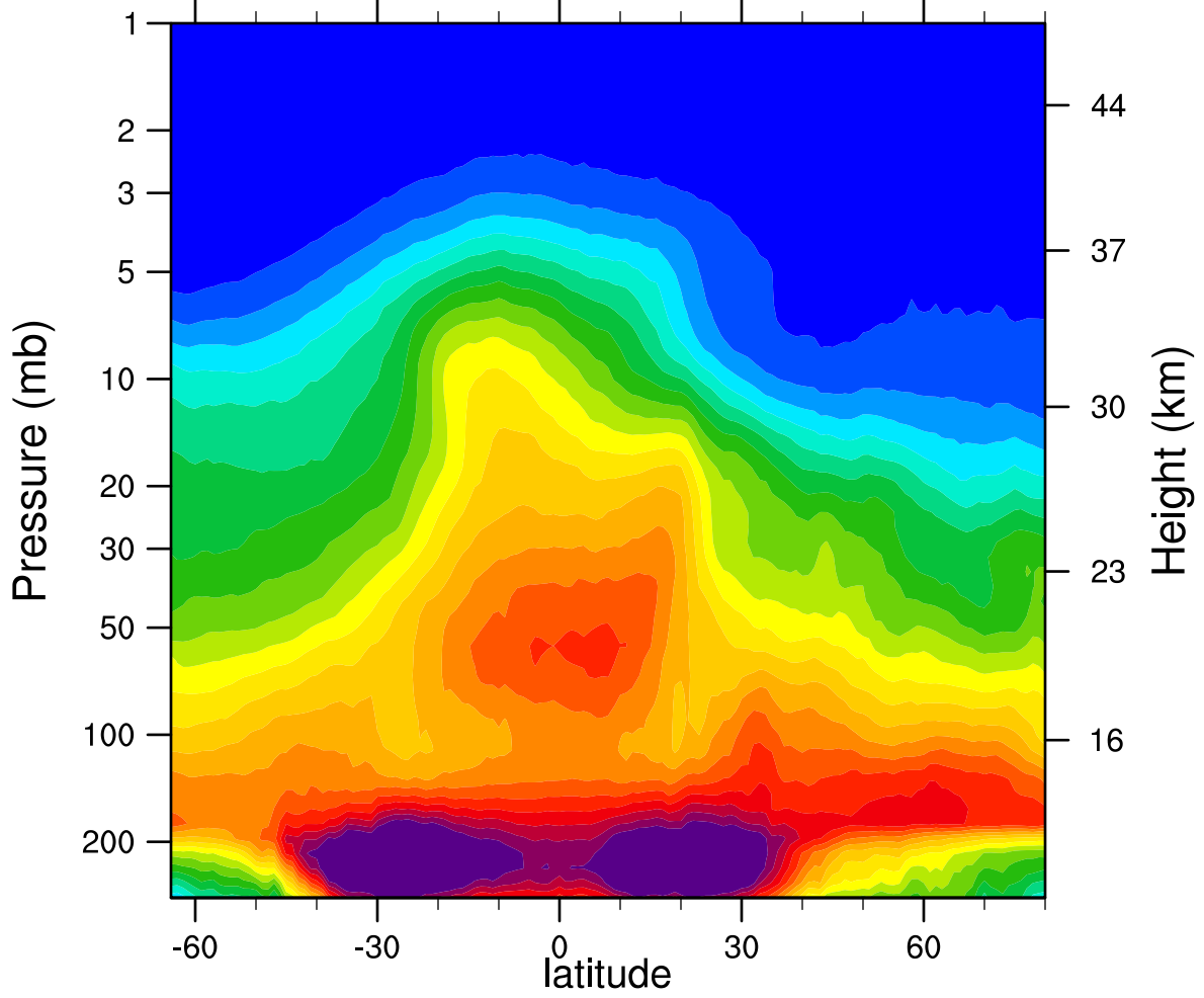
2006d032 N2O_Combined (ppbv)
