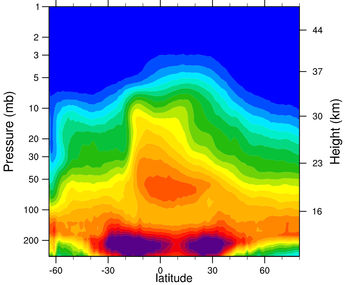
2005d262 N2O_Combined (ppbv)
