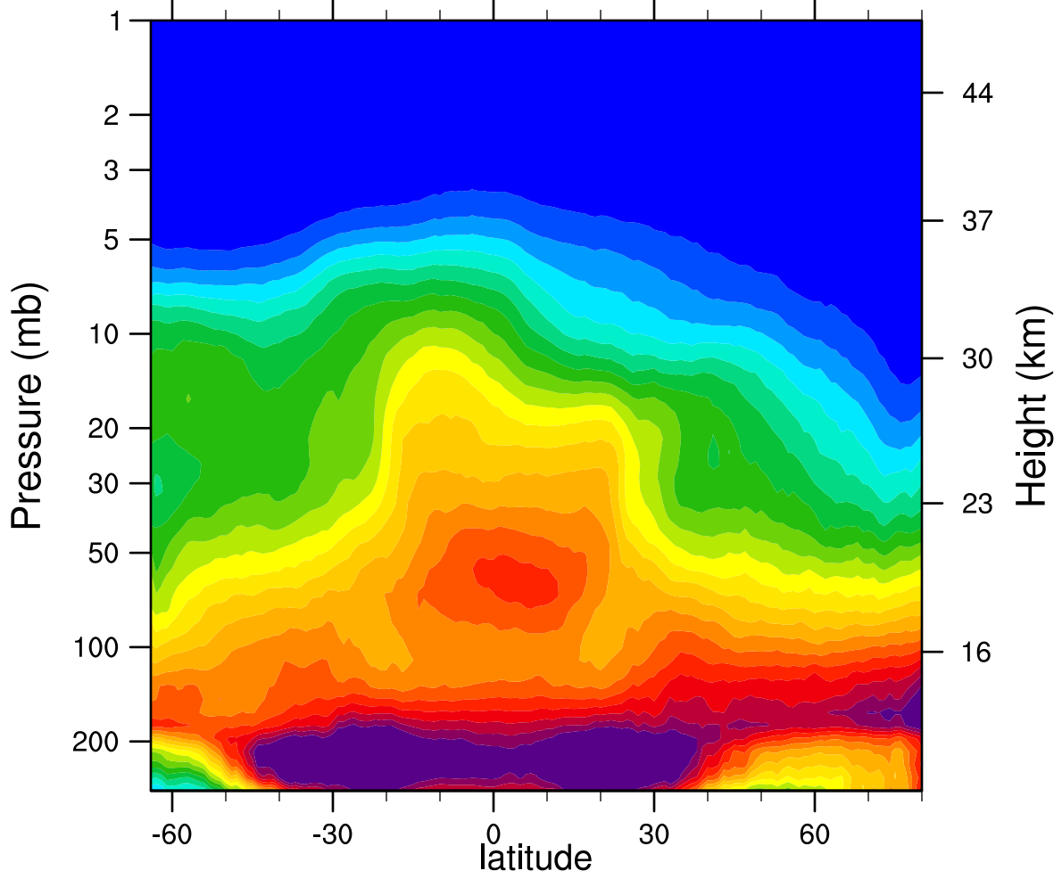
2007d349 N2O_Combined (ppbv)
