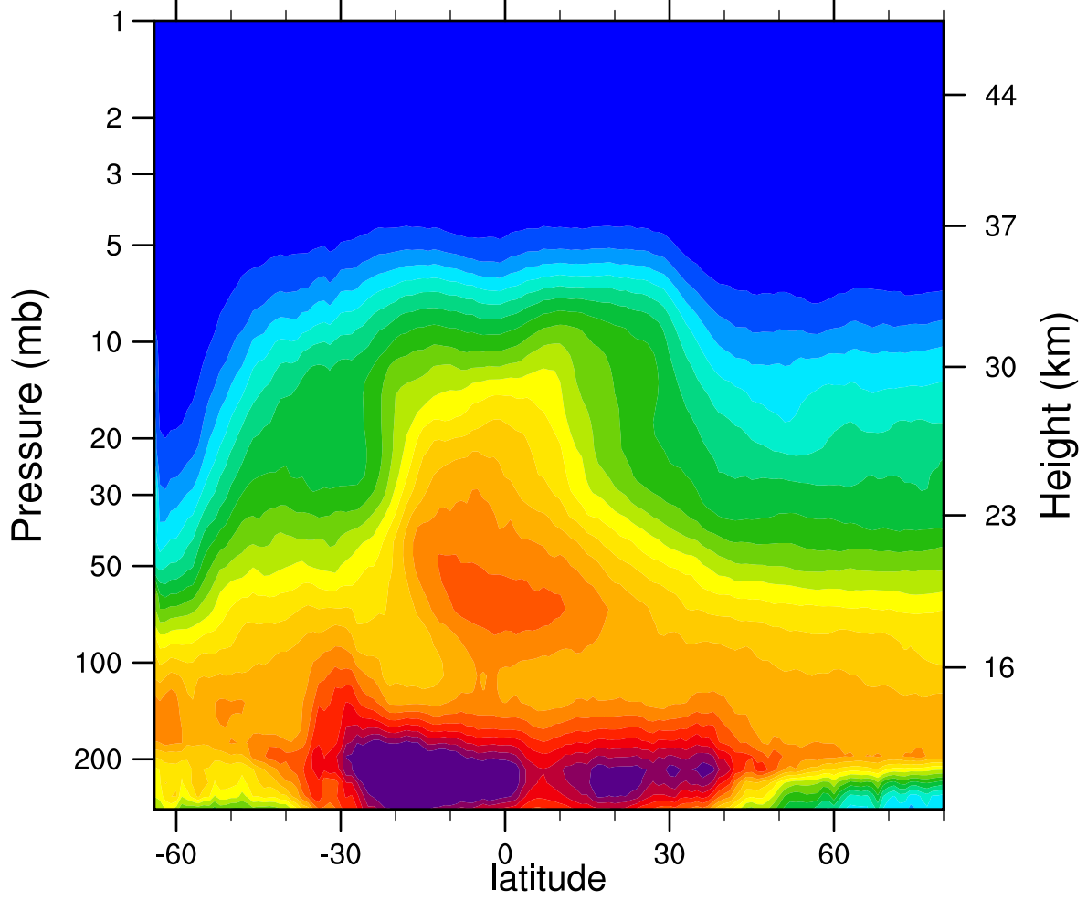
2007d179 N2O_Combined (ppbv)
