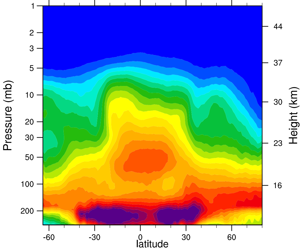
2005d325 N2O_Combined (ppbv)
