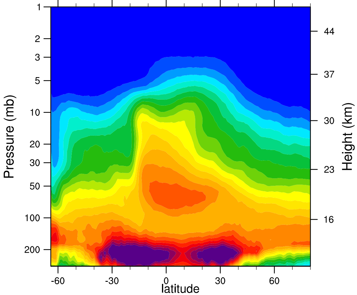
2005d259 N2O_Combined (ppbv)
