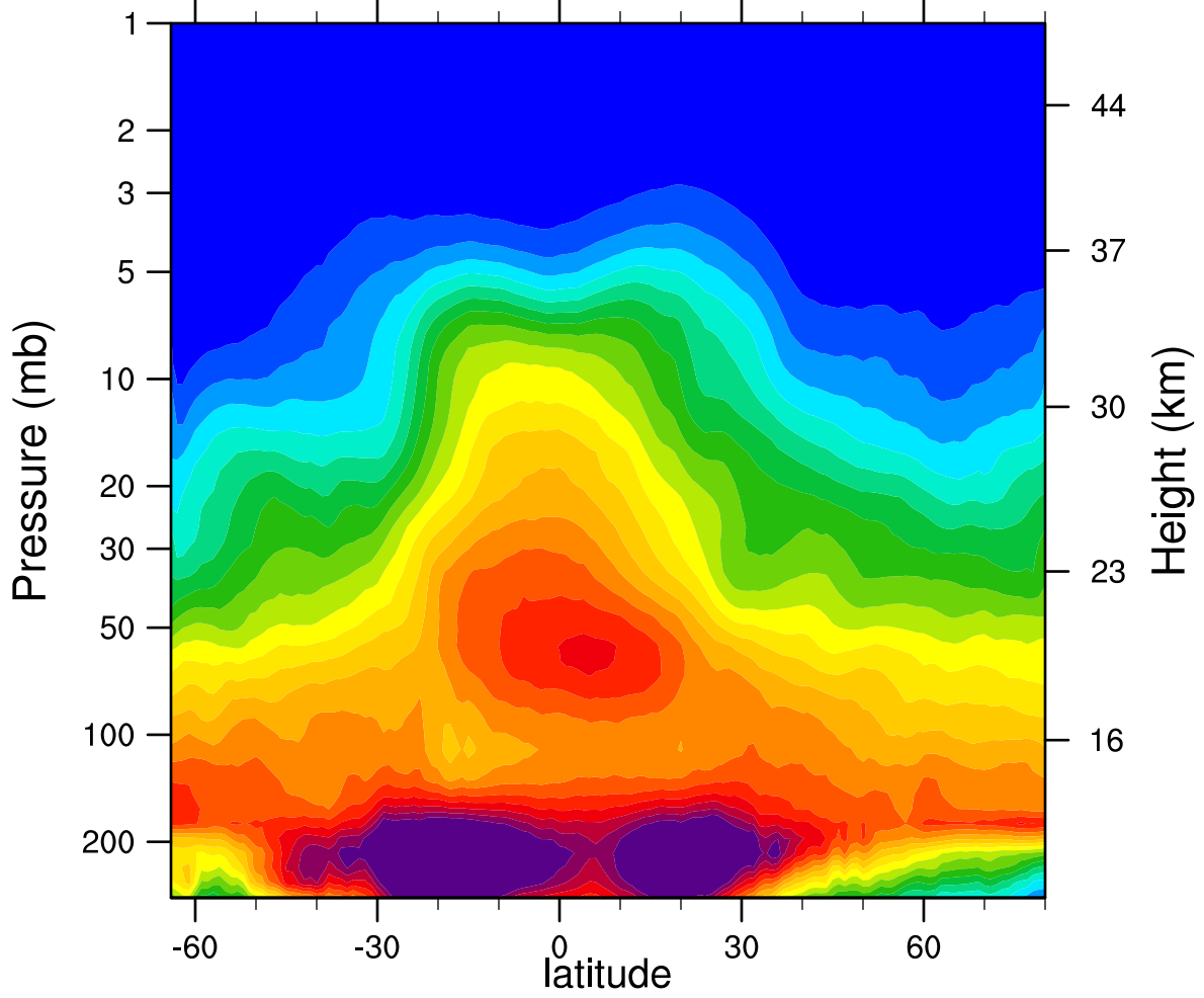
2005d127 N2O_Combined (ppbv)
