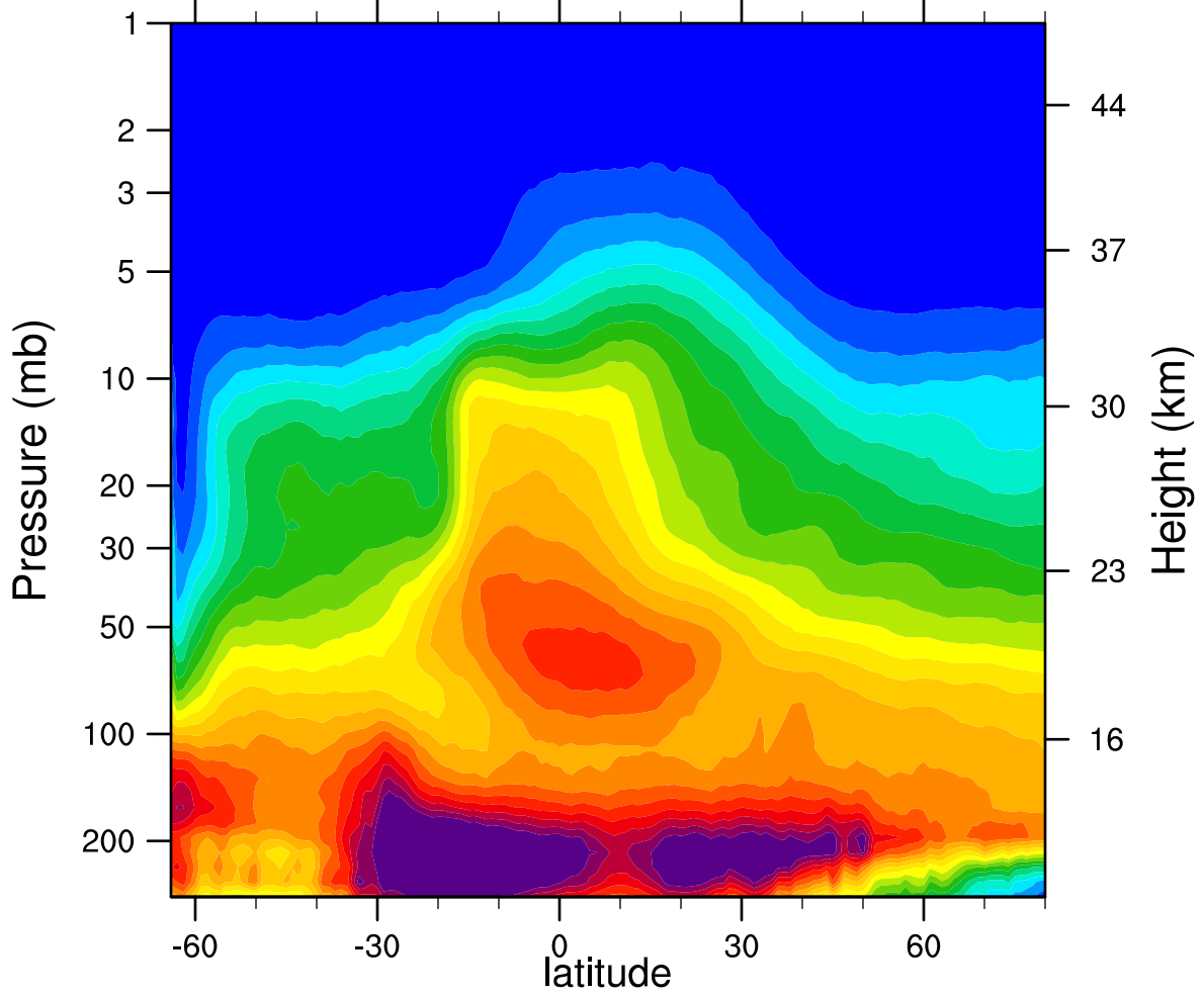
2005d219 N2O_Combined (ppbv)
