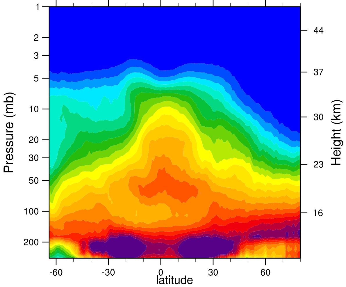
2006d332 N2O_Combined (ppbv)
