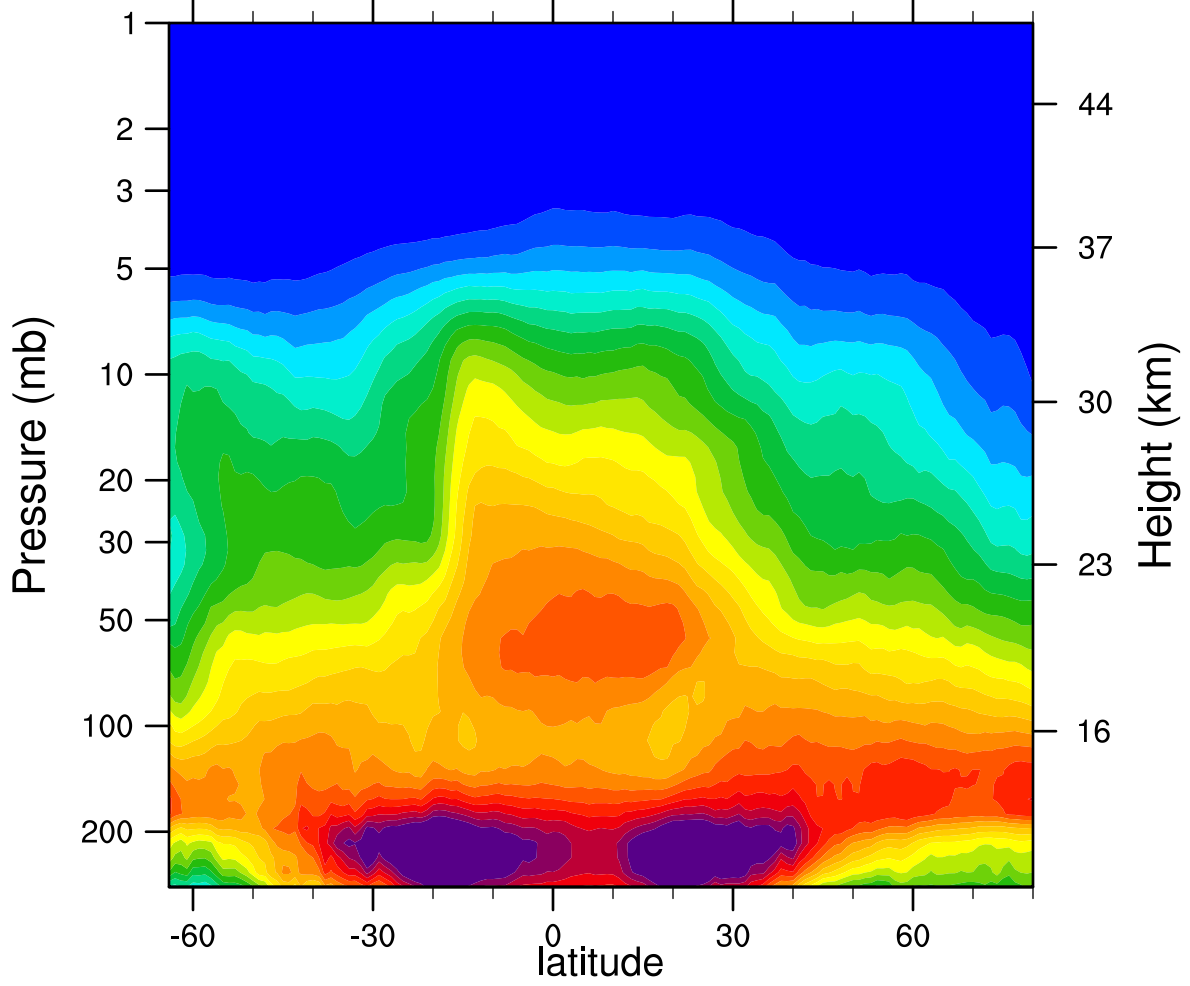
2005d307 N2O_Combined (ppbv)
