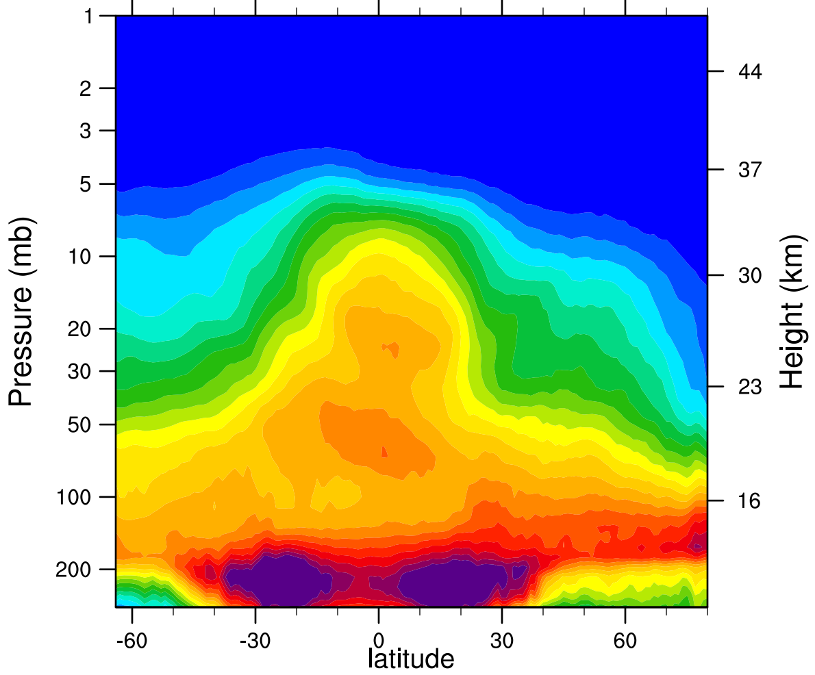
2007d024 N2O_Combined (ppbv)
