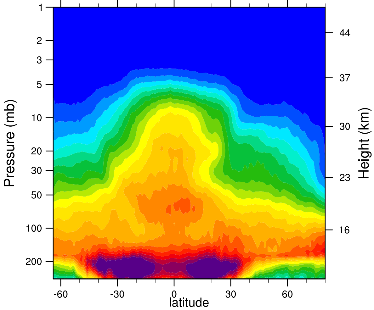
2007d076 N2O_Combined (ppbv)
