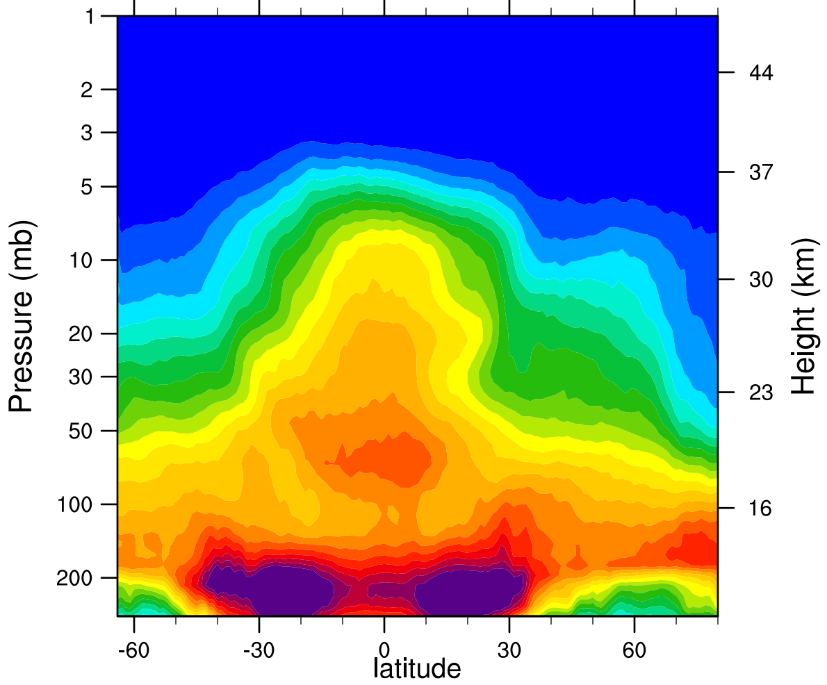
2007d072 N2O_Combined (ppbv)
