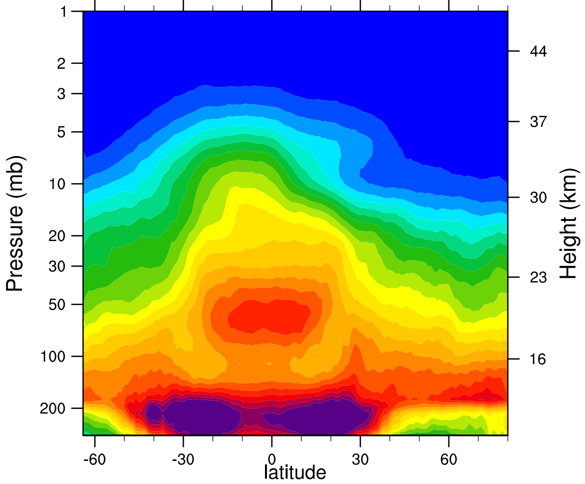
2006d083 N2O_Combined (ppbv)
