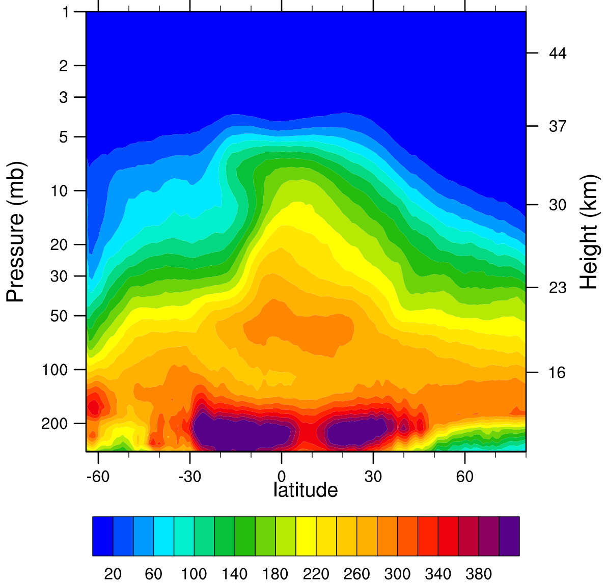
2006d278 N2O_Combined (ppbv)
