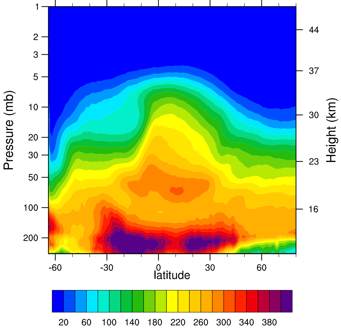
2006d243 N2O_Combined (ppbv)
