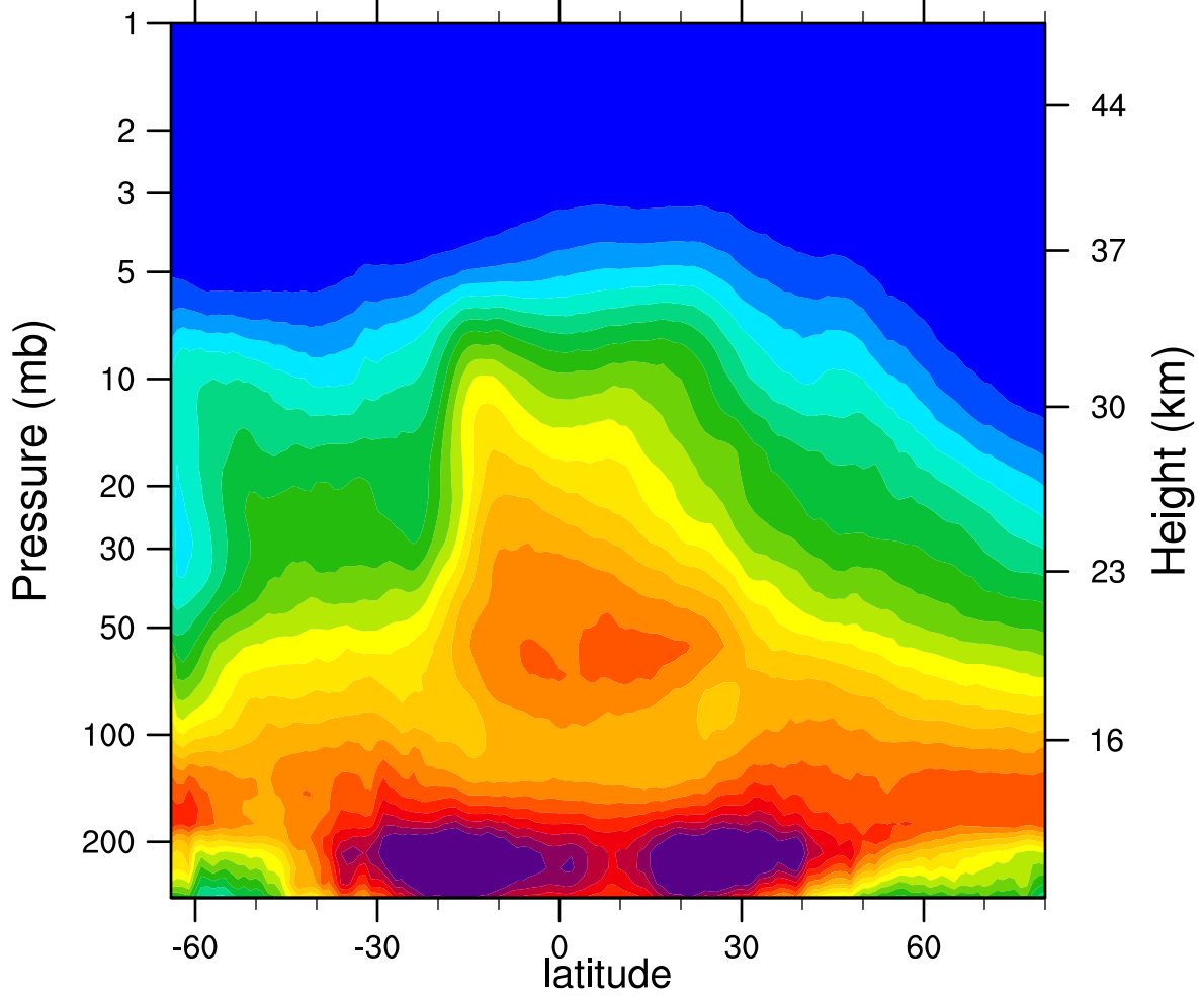
2005d290 N2O_Combined (ppbv)
