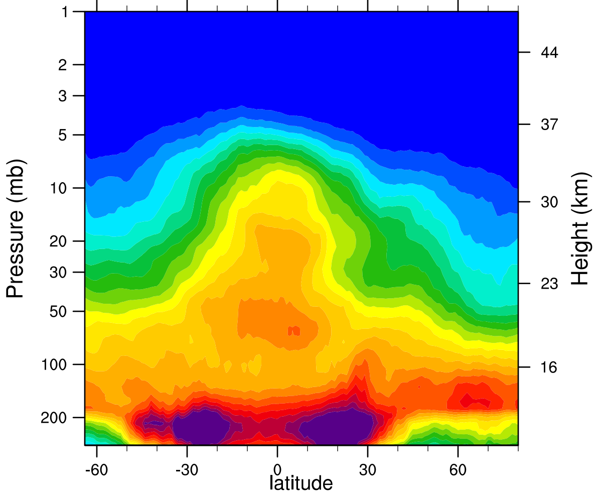
2007d053 N2O_Combined (ppbv)
