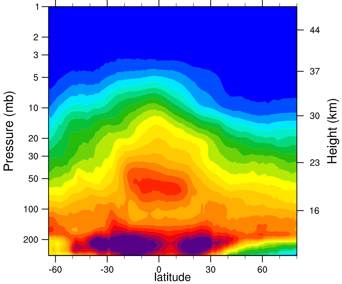
2006d135 N2O_Combined (ppbv)
