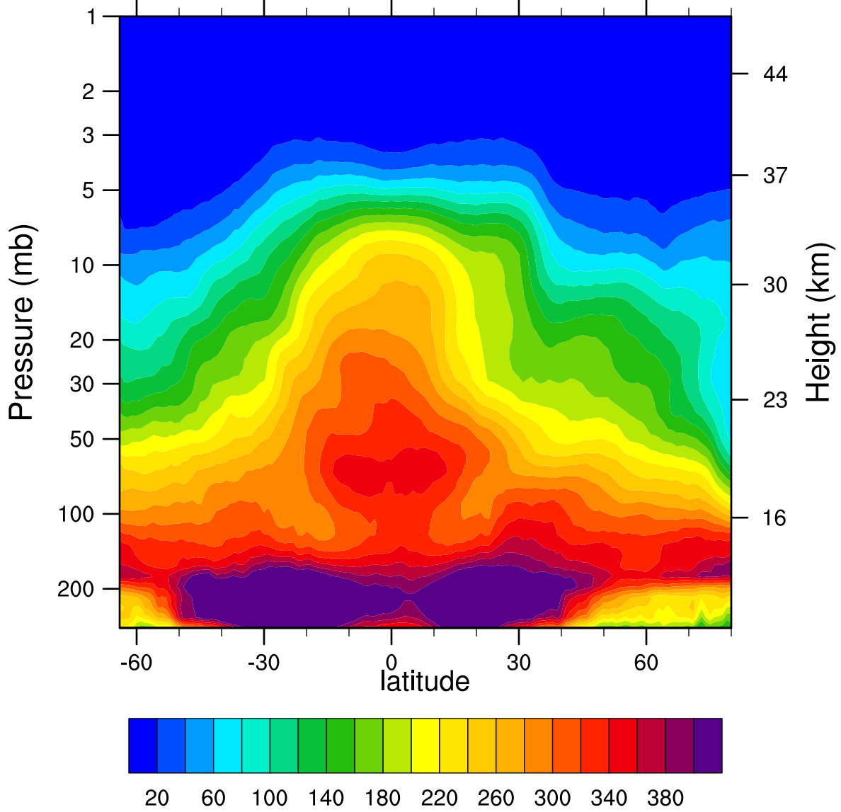
2007d106 N2O_Combined (ppbv)
