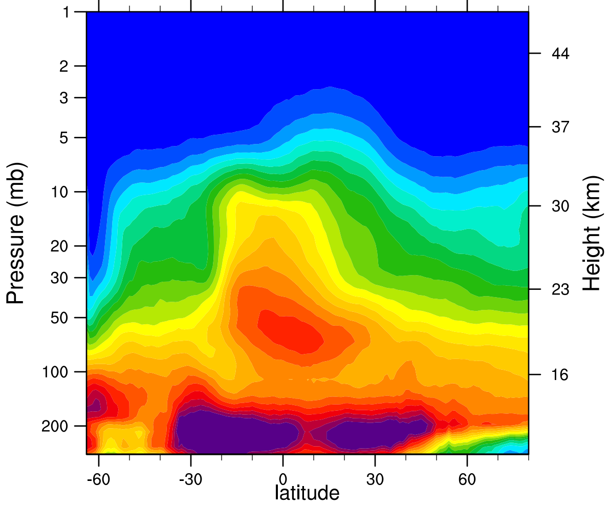
2005d195 N2O_Combined (ppbv)
