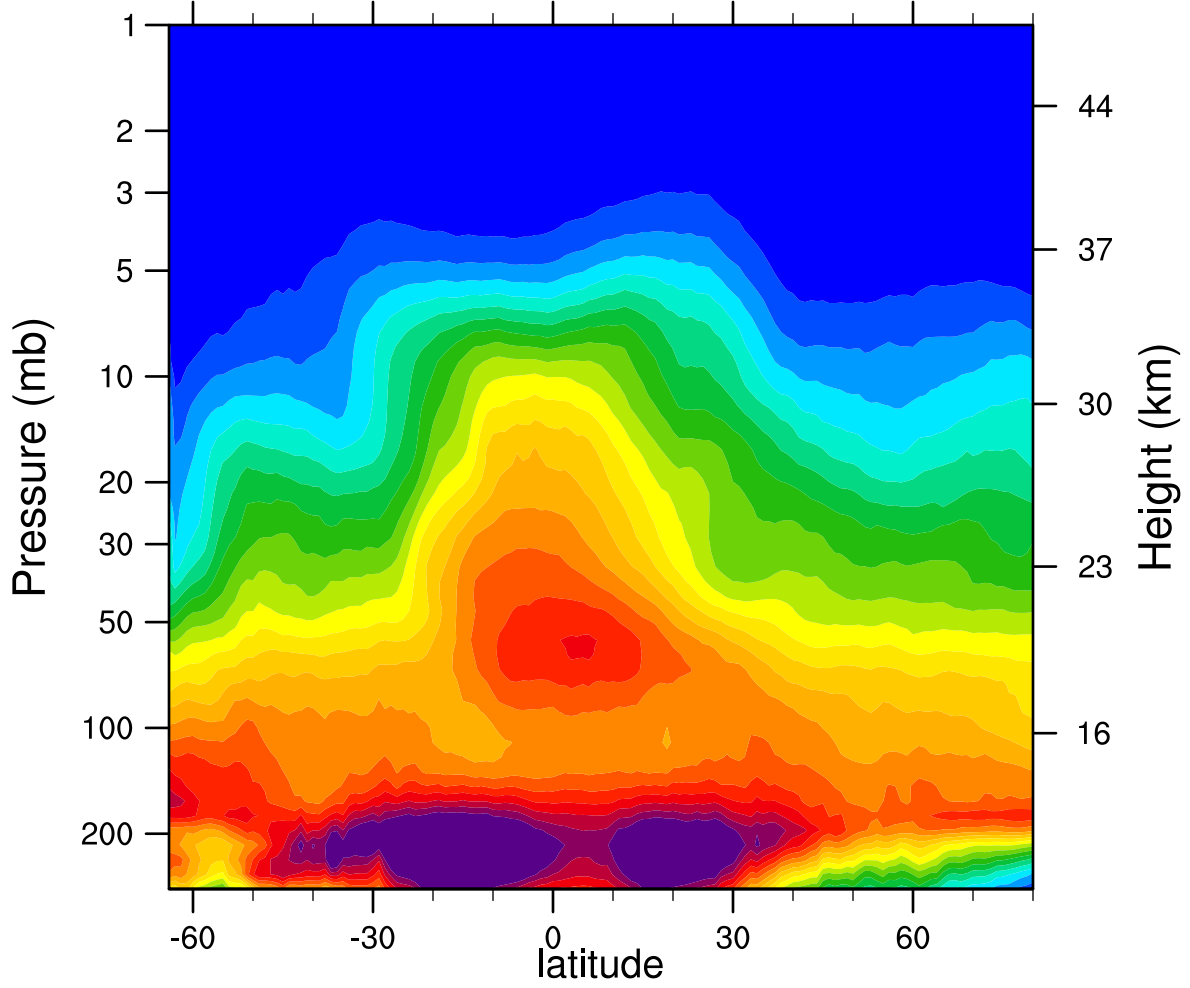
2005d143 N2O_Combined (ppbv)
