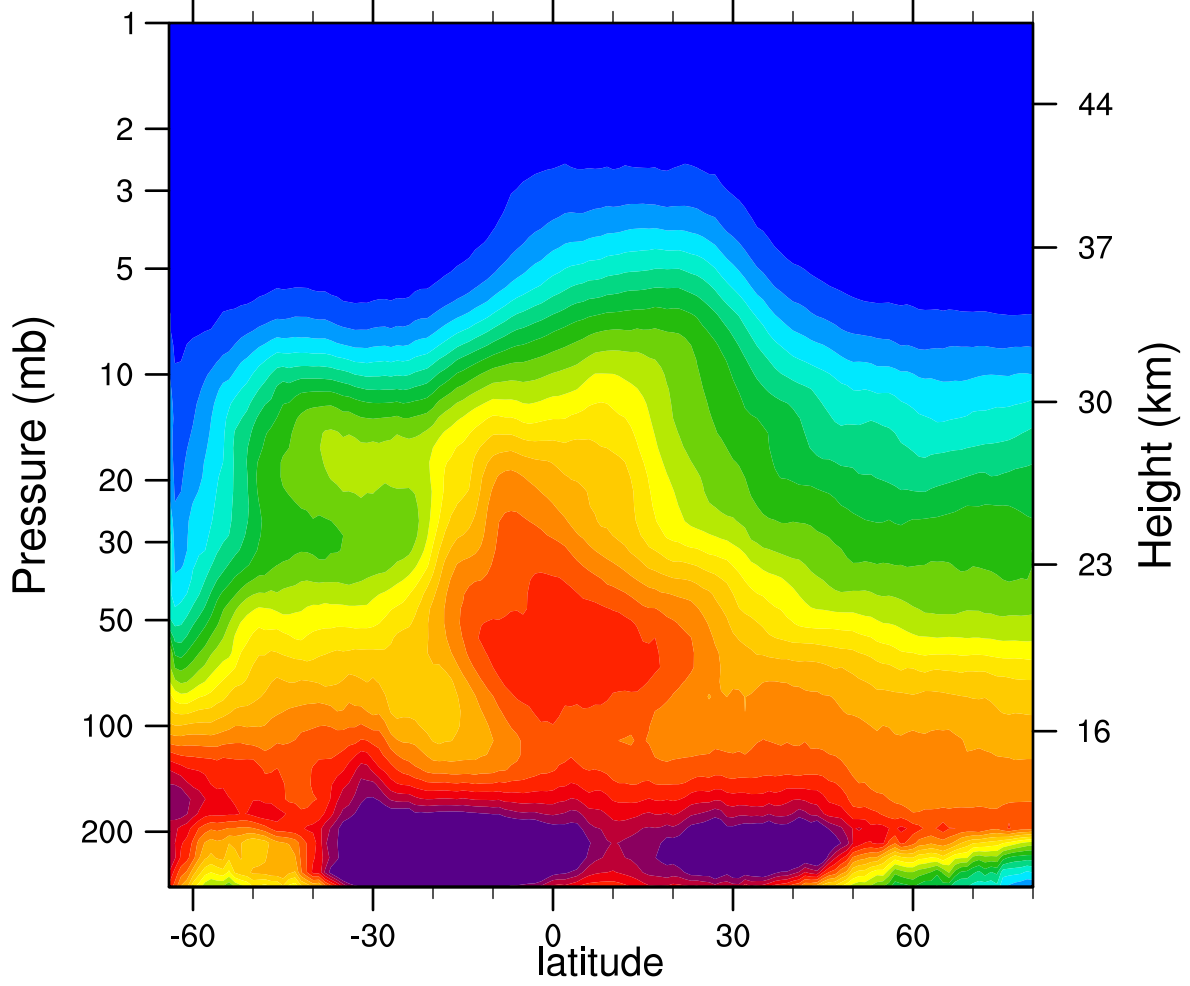
2007d221 N2O_Combined (ppbv)
