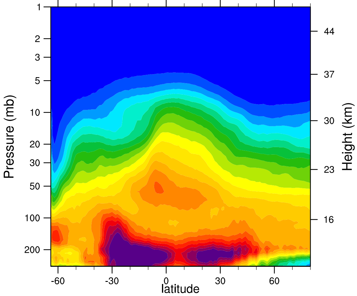
2006d201 N2O_Combined (ppbv)
