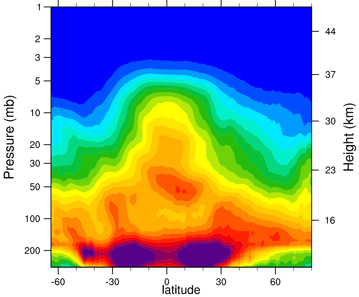
2005d083 N2O_Combined (ppbv)
