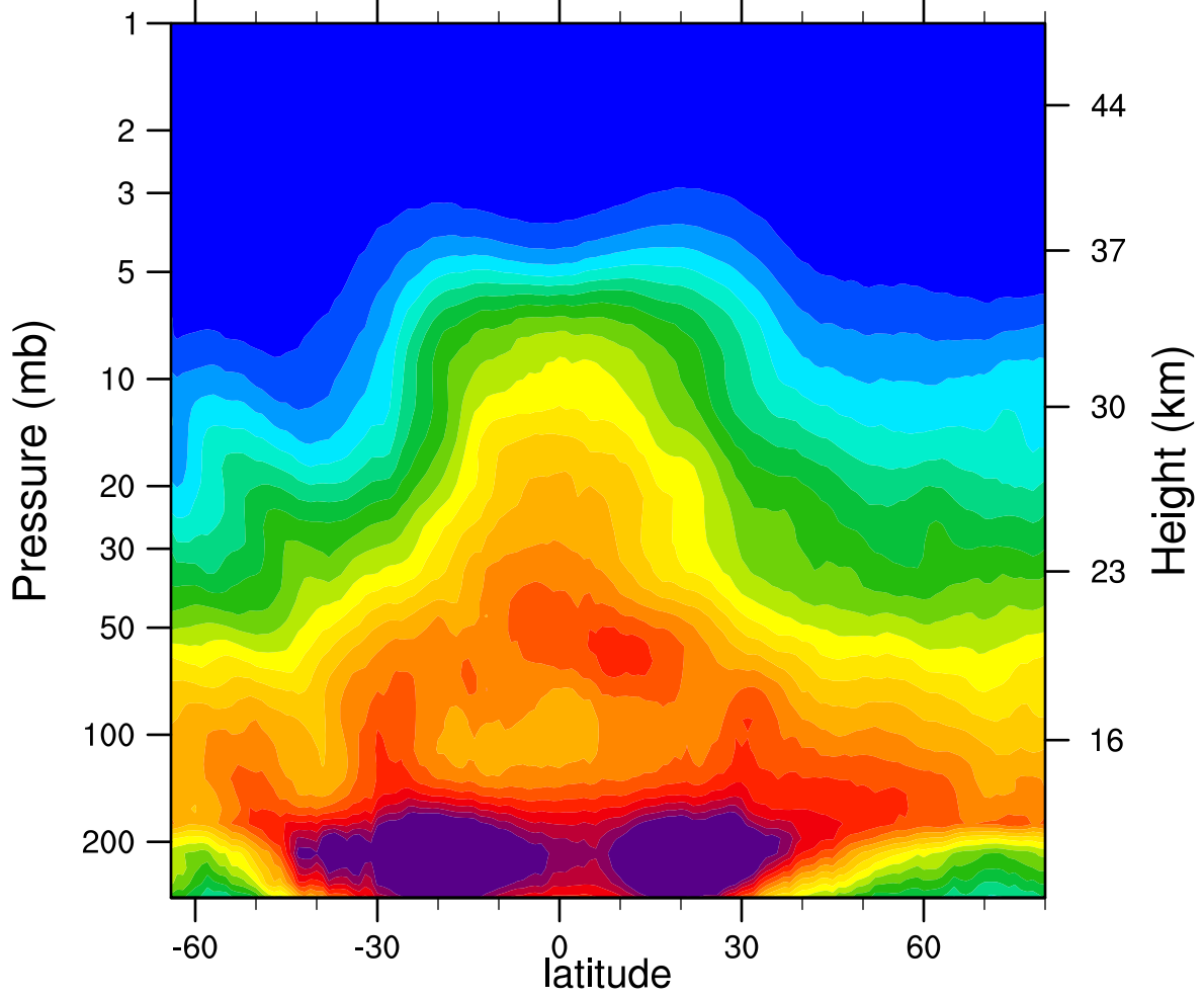
2005d108 N2O_Combined (ppbv)
