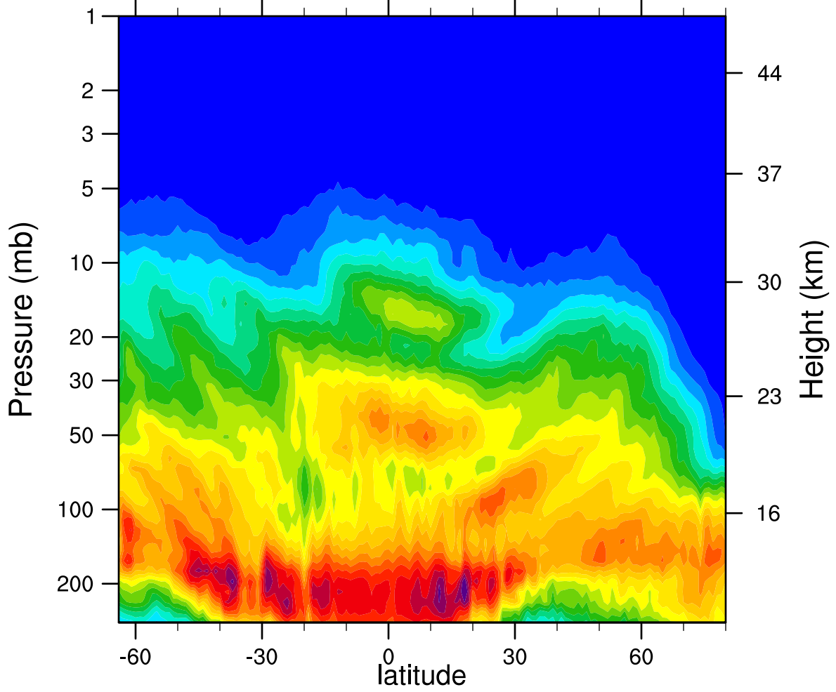
2005d024 N2O_Combined (ppbv)
