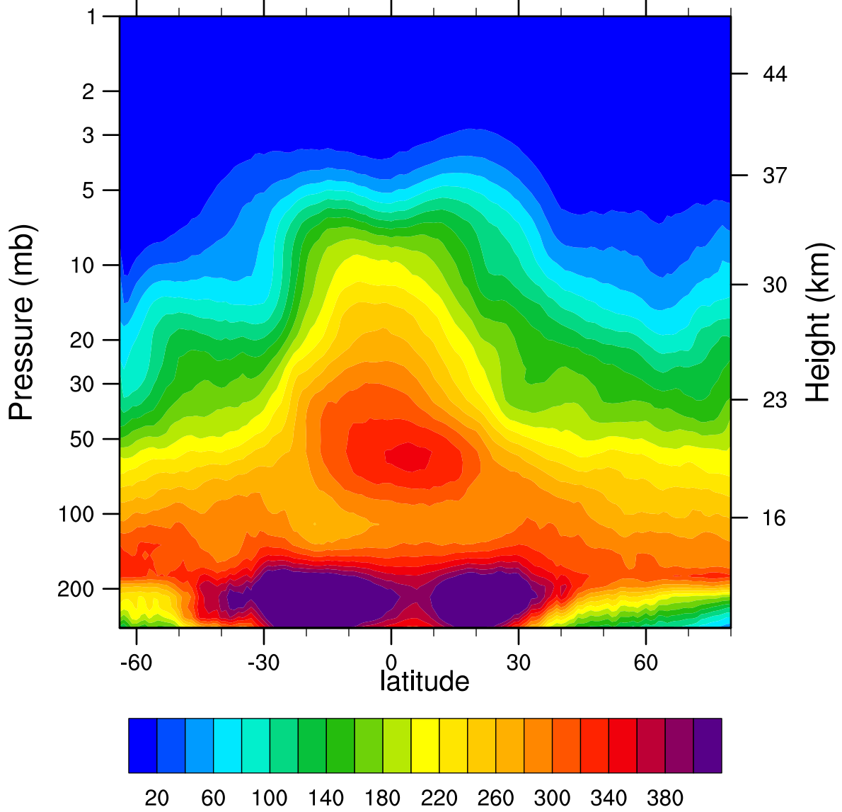
2005d130 N2O_Combined (ppbv)
