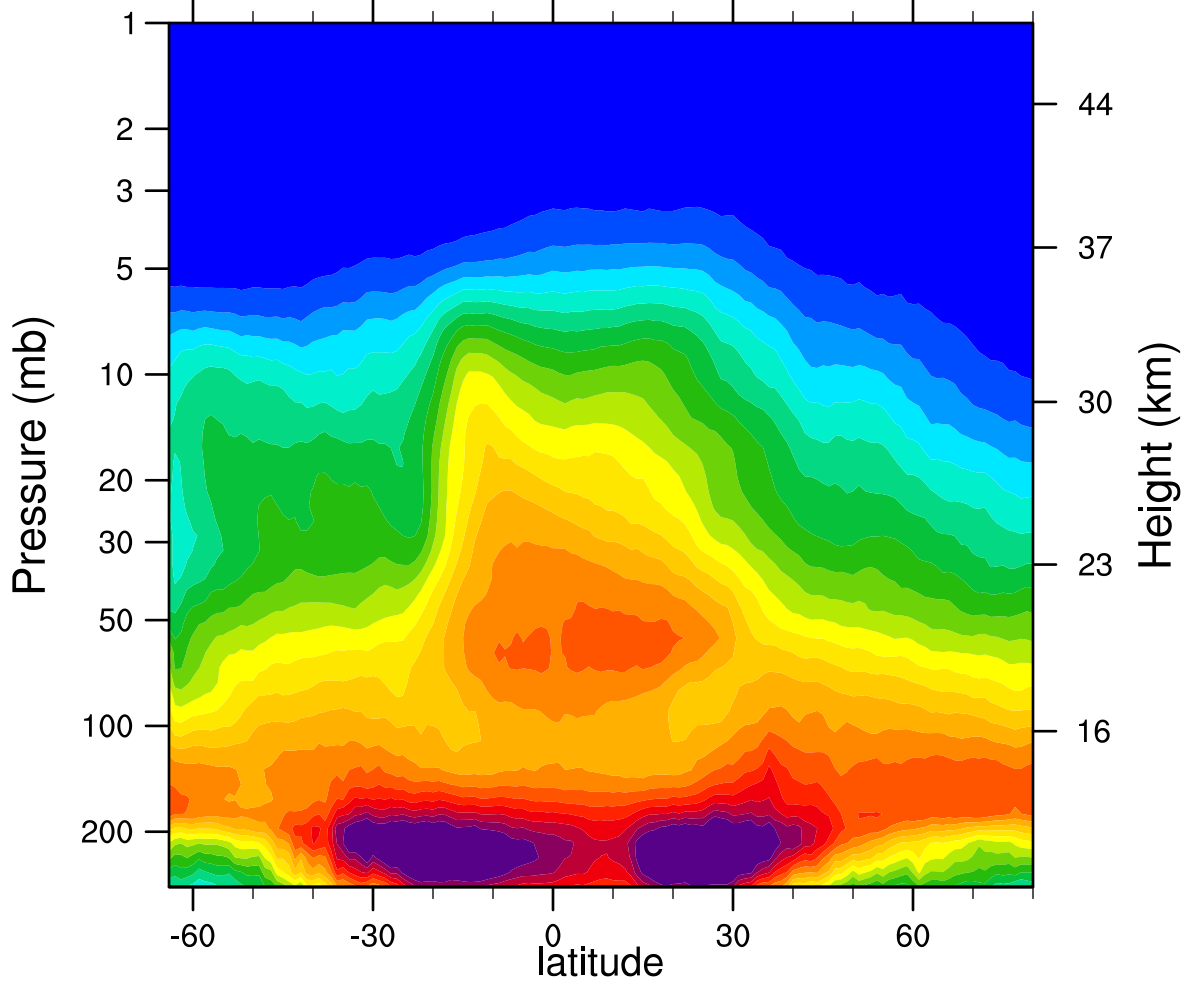
2005d298 N2O_Combined (ppbv)
