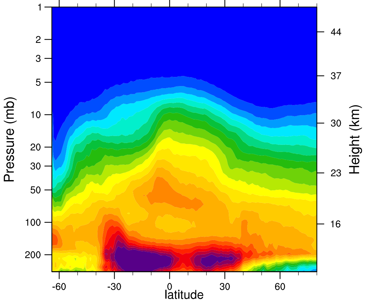
2006d188 N2O_Combined (ppbv)
