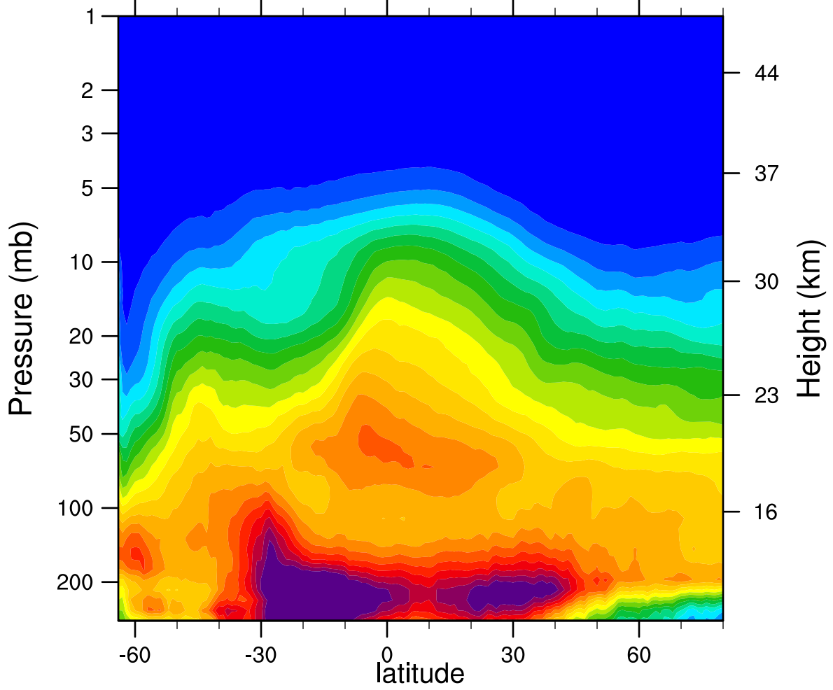
2006d210 N2O_Combined (ppbv)
