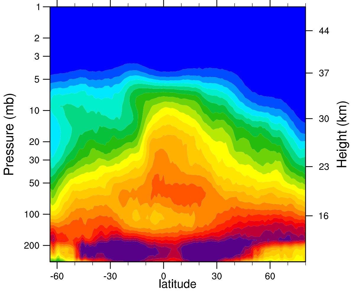
2006d311 N2O_Combined (ppbv)
