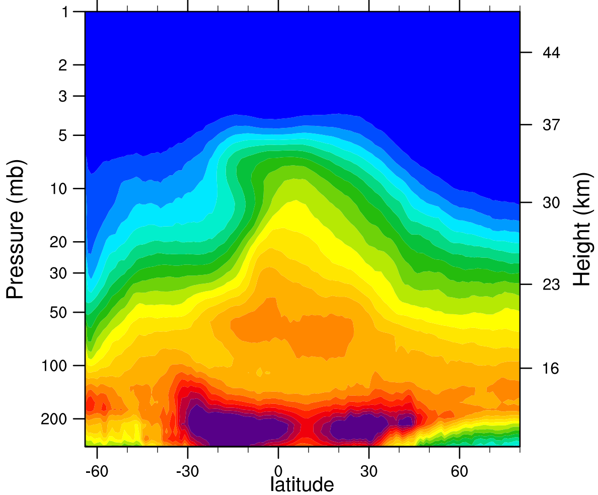
2006d268 N2O_Combined (ppbv)
