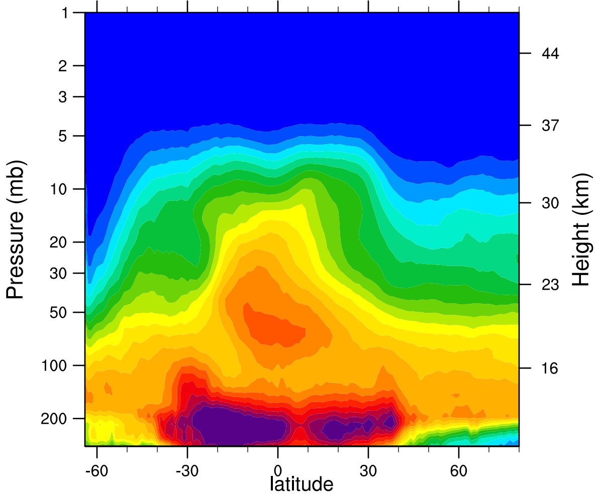
2007d173 N2O_Combined (ppbv)
