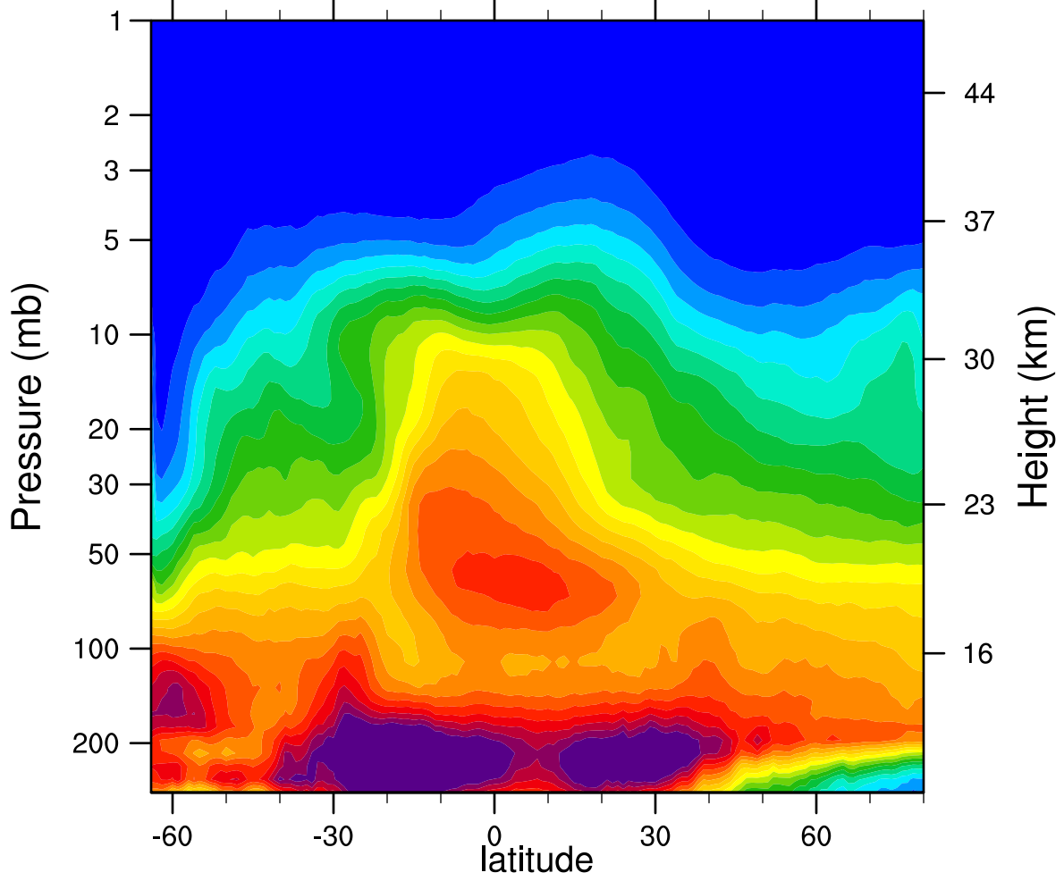
2005d176 N2O_Combined (ppbv)
