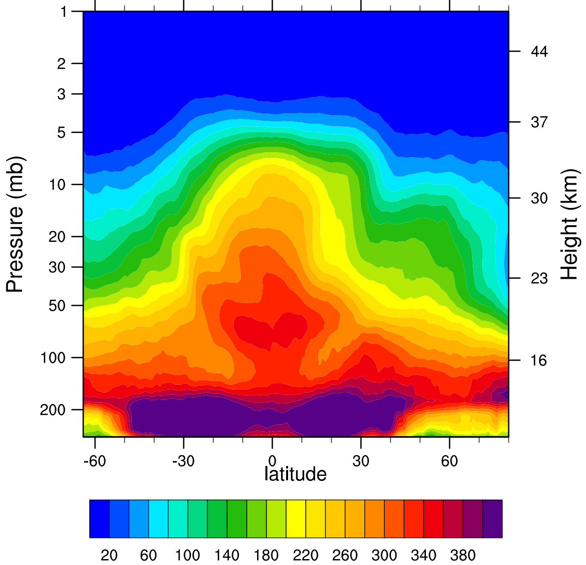
2007d097 N2O_Combined (ppbv)
