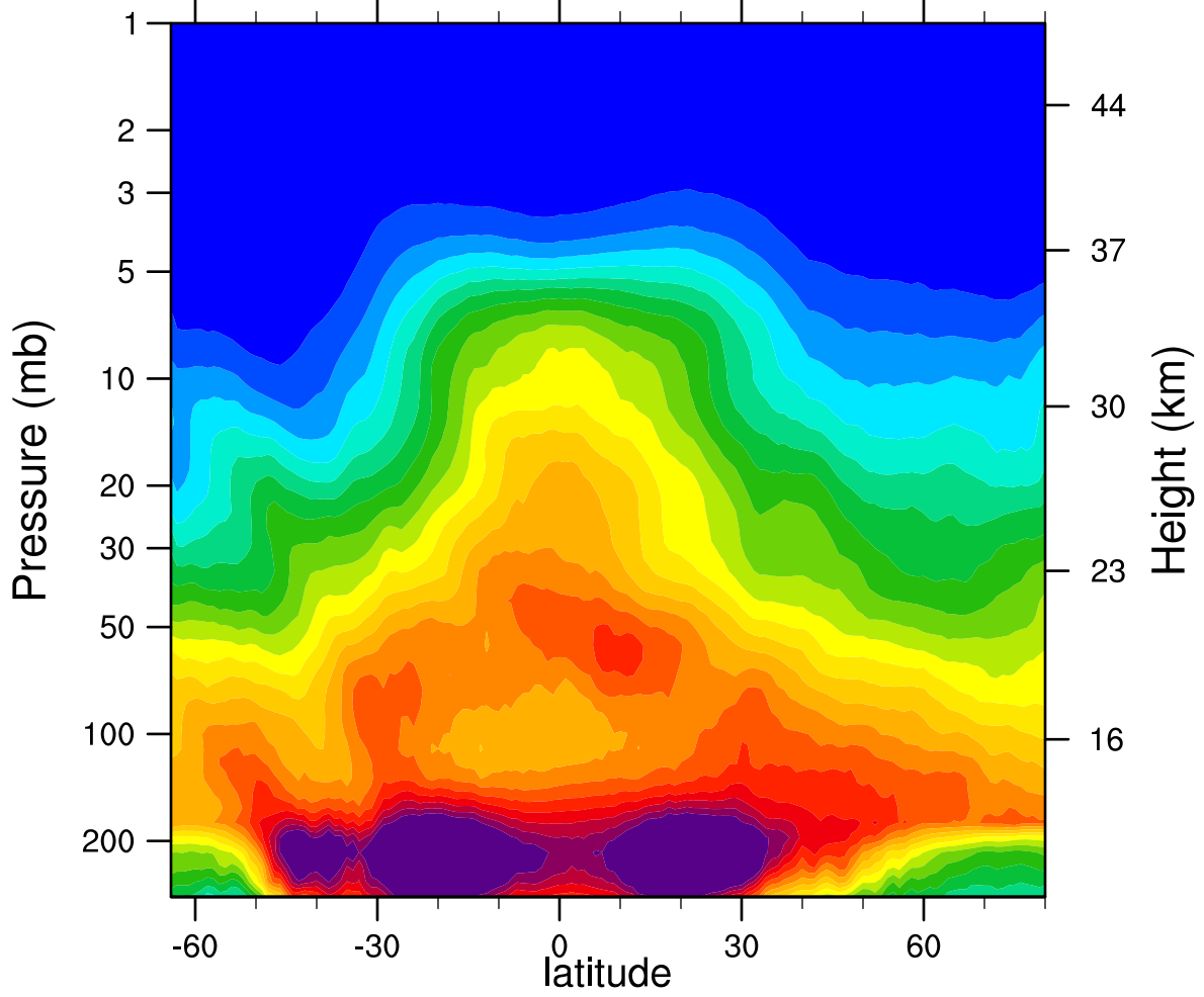
2005d101 N2O_Combined (ppbv)
