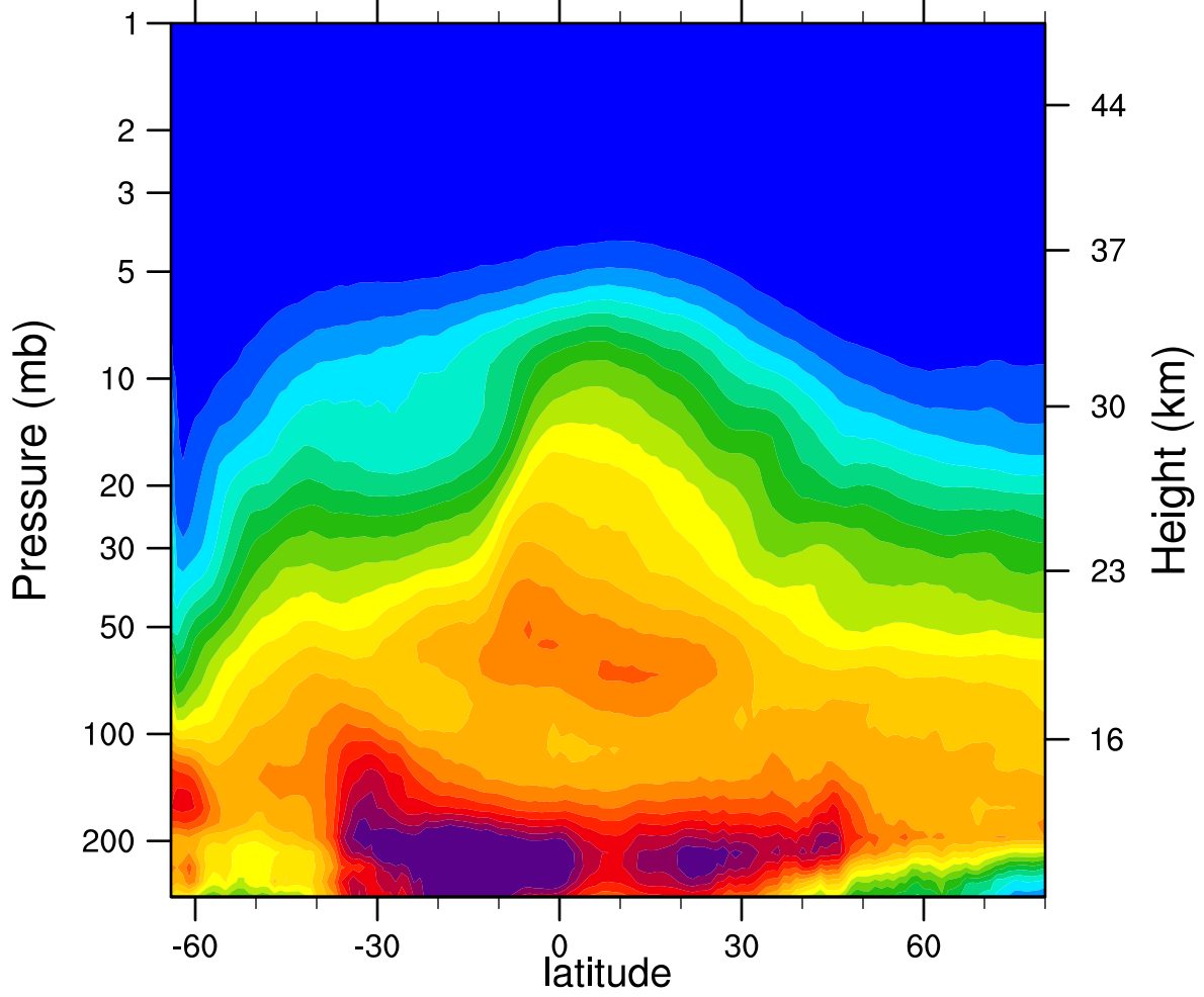
2006d226 N2O_Combined (ppbv)
