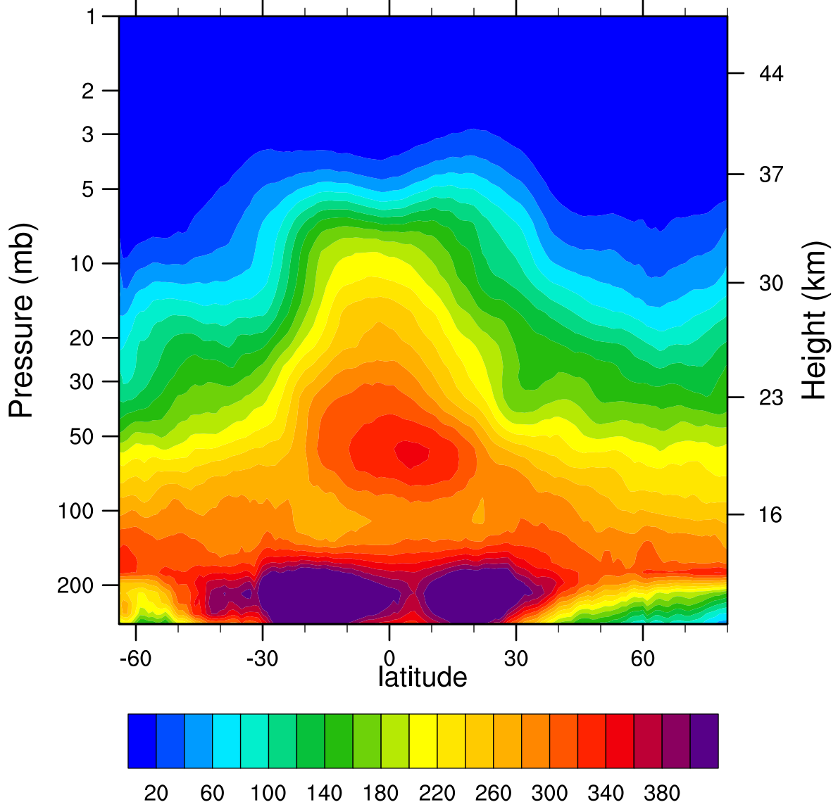
2005d125 N2O_Combined (ppbv)
