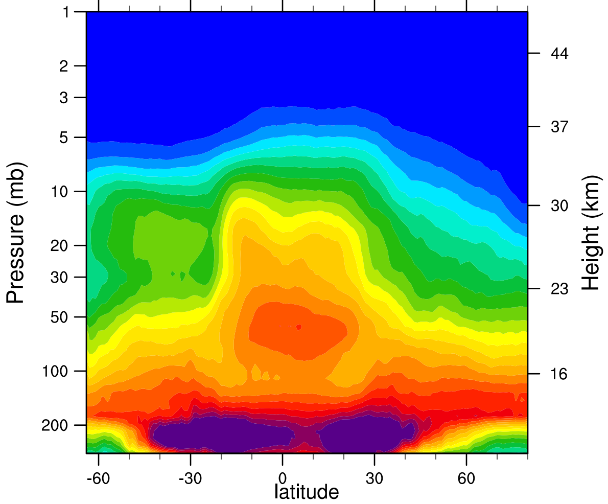
2007d301 N2O_Combined (ppbv)
