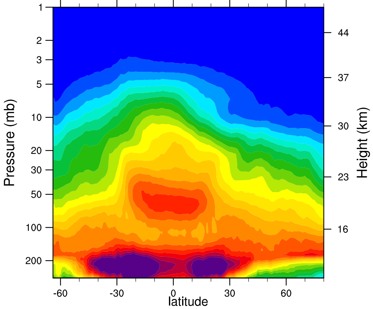
2006d113 N2O_Combined (ppbv)
