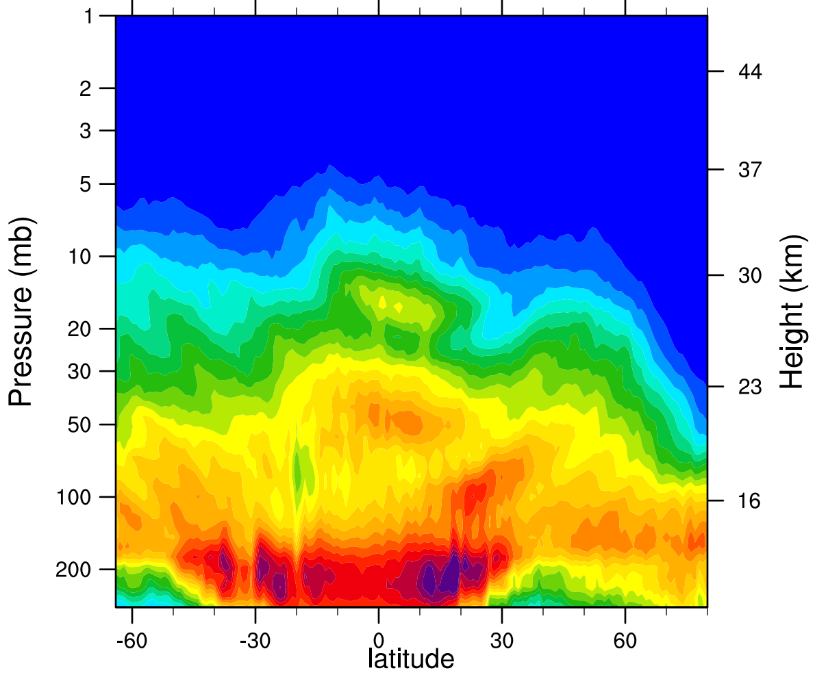
2005d025 N2O_Combined (ppbv)
