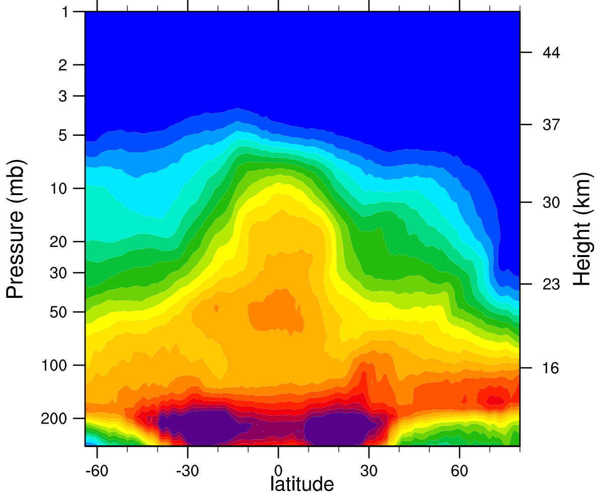
2007d001 N2O_Combined (ppbv)
