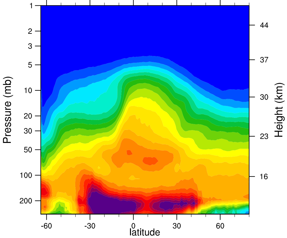
2006d236 N2O_Combined (ppbv)
