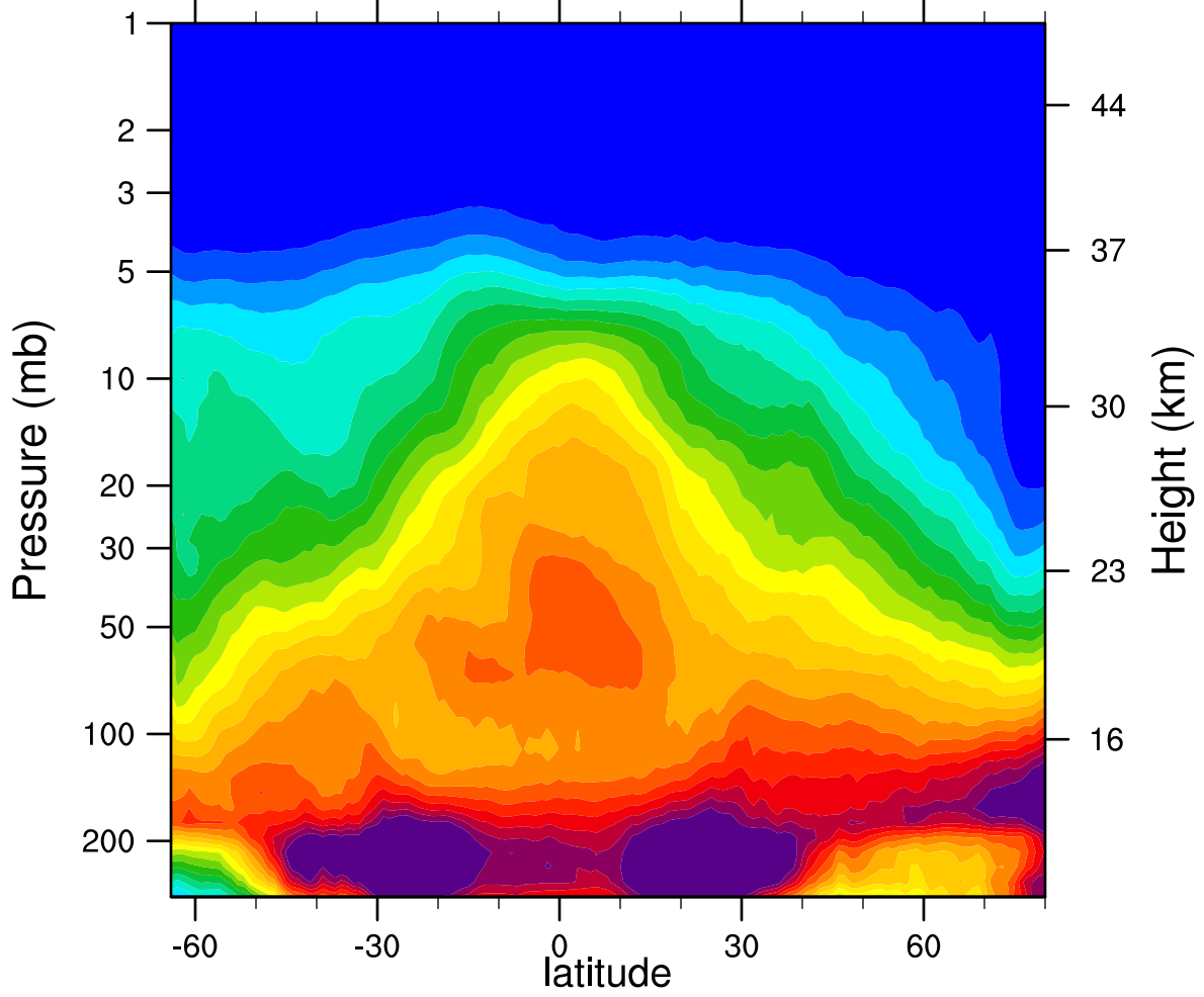
2006d350 N2O_Combined (ppbv)
