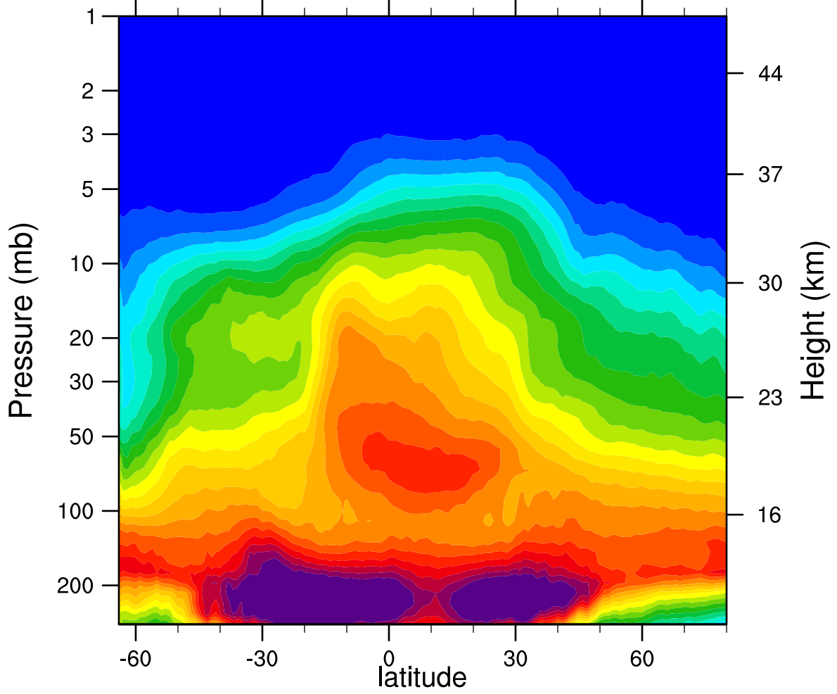
2007d271 N2O_Combined (ppbv)
