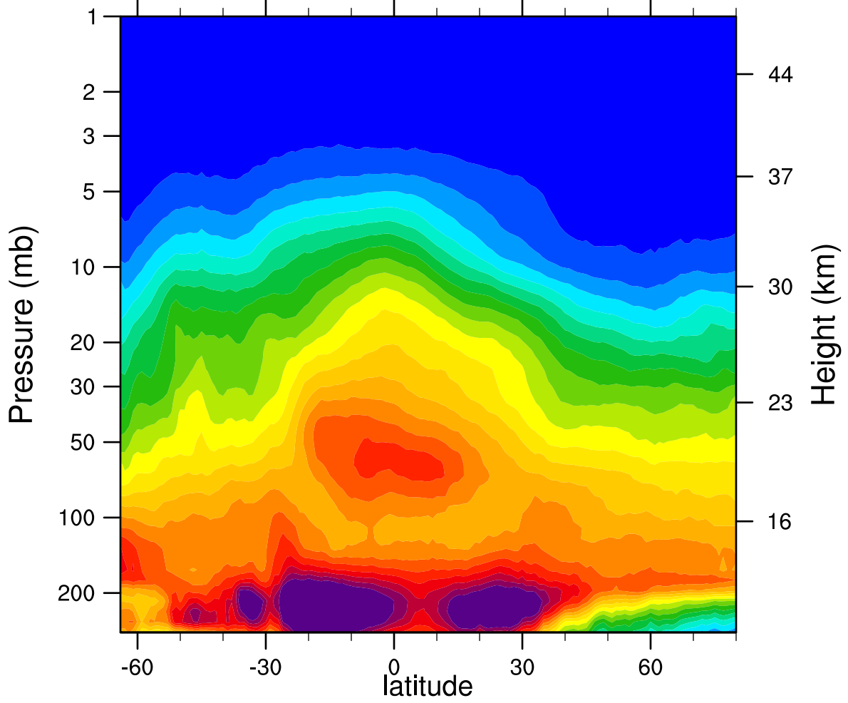
2006d142 N2O_Combined (ppbv)
