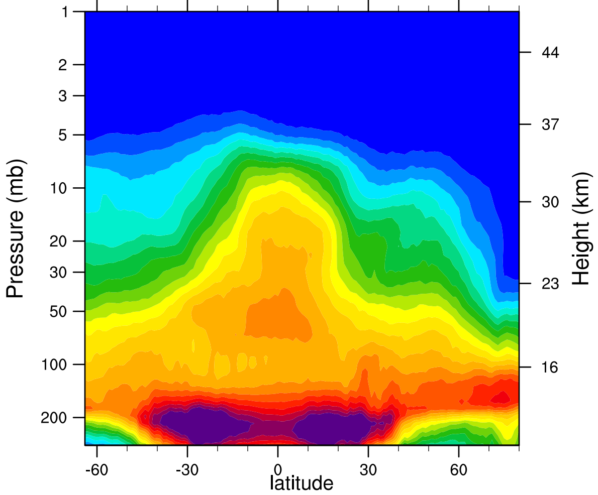
2007d009 N2O_Combined (ppbv)
