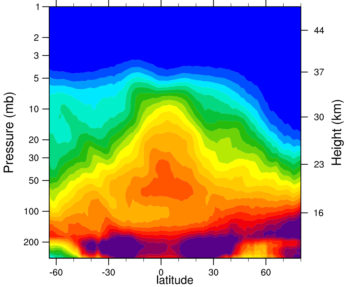
2006d339 N2O_Combined (ppbv)
