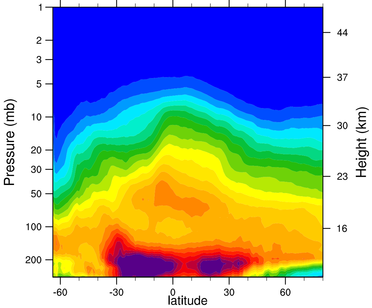
2006d182 N2O_Combined (ppbv)
