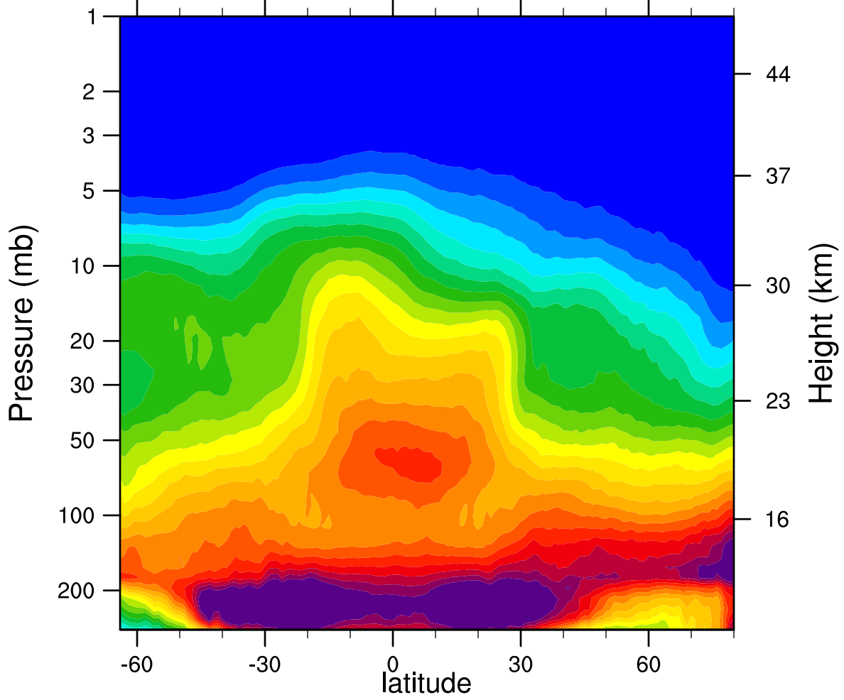
2007d345 N2O_Combined (ppbv)
