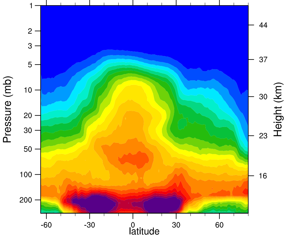
2007d069 N2O_Combined (ppbv)
