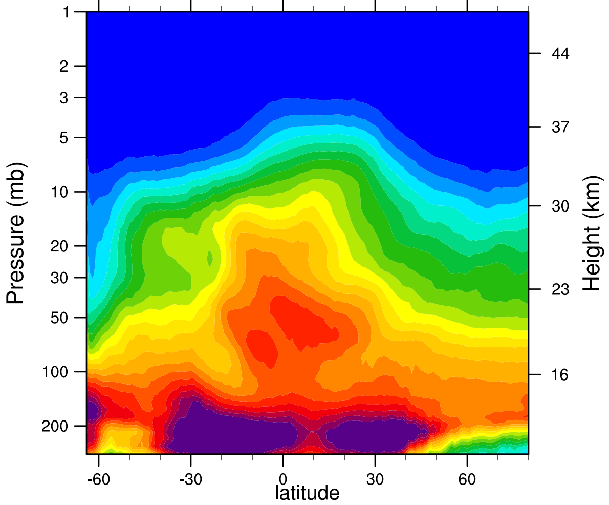
2007d240 N2O_Combined (ppbv)
