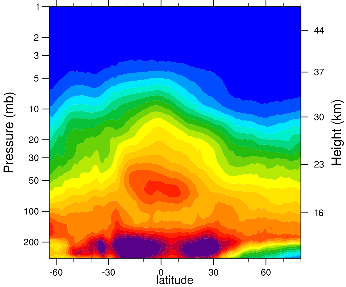
2006d140 N2O_Combined (ppbv)
