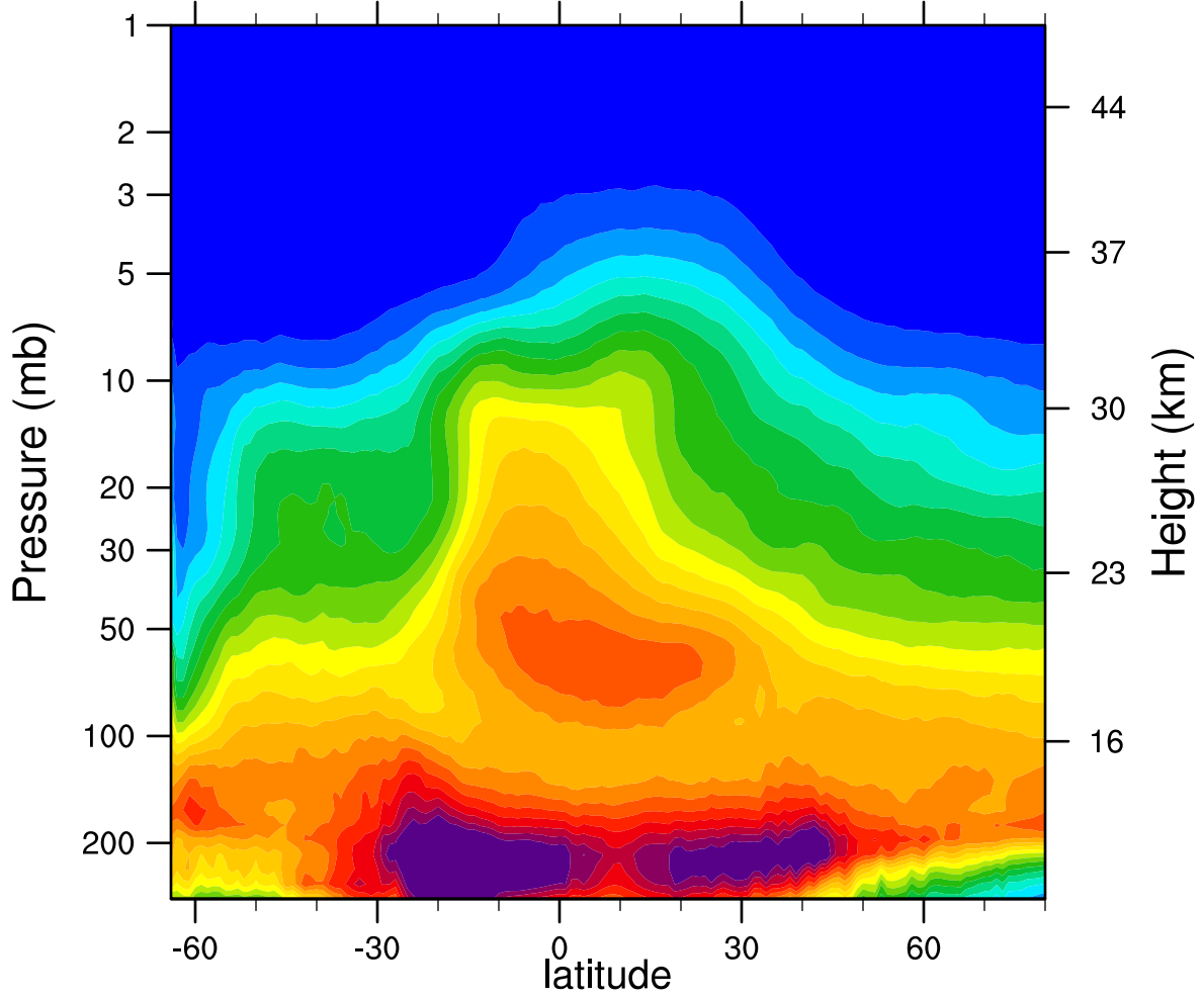
2005d238 N2O_Combined (ppbv)
