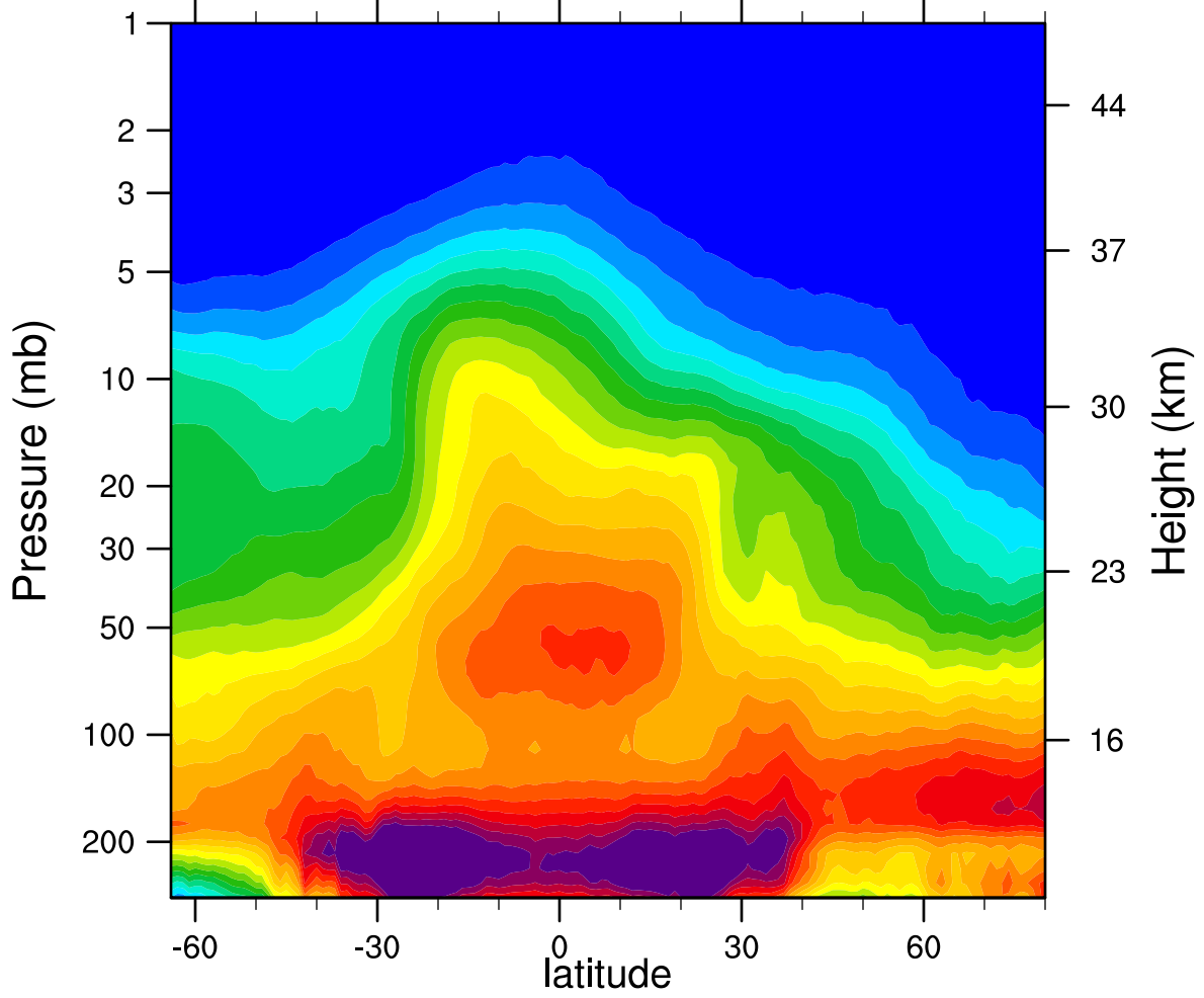
2005d362 N2O_Combined (ppbv)
