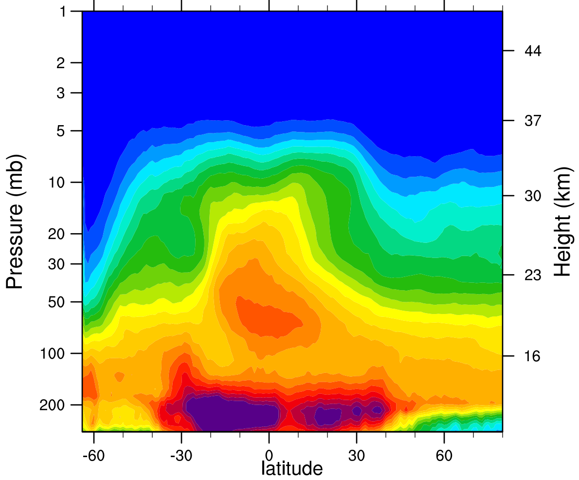
2007d177 N2O_Combined (ppbv)
