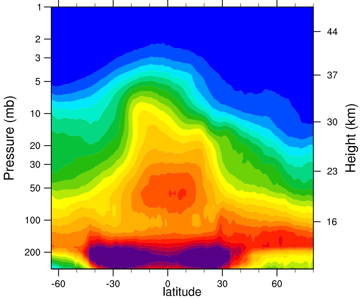
2006d020 N2O_Combined (ppbv)
