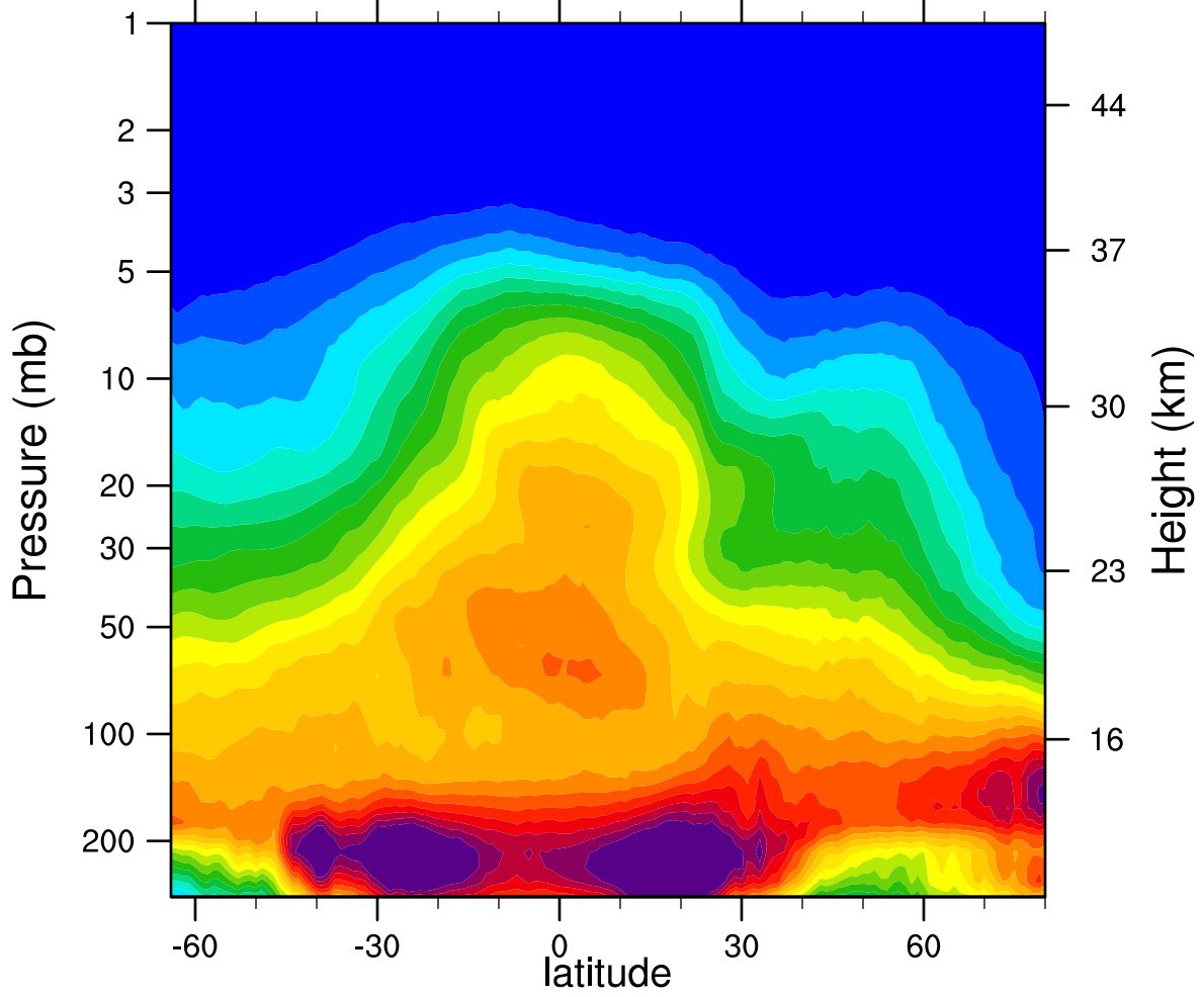
2007d035 N2O_Combined (ppbv)
