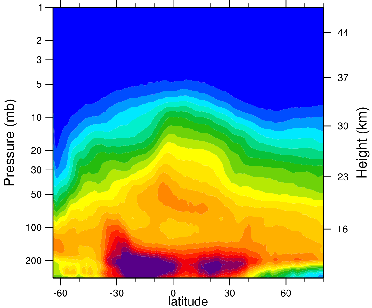
2006d186 N2O_Combined (ppbv)
