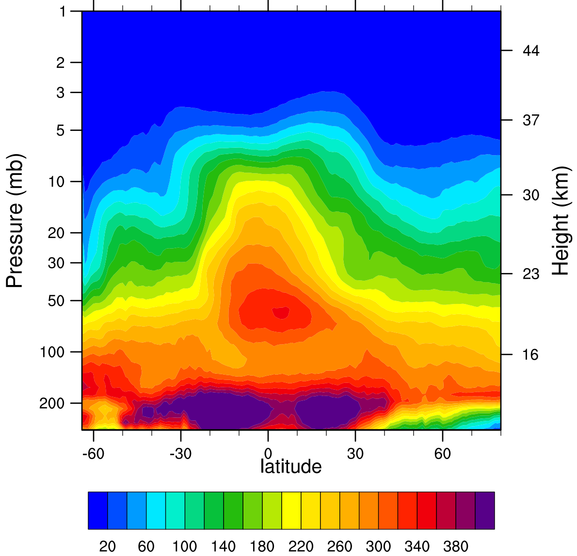
2005d145 N2O_Combined (ppbv)
