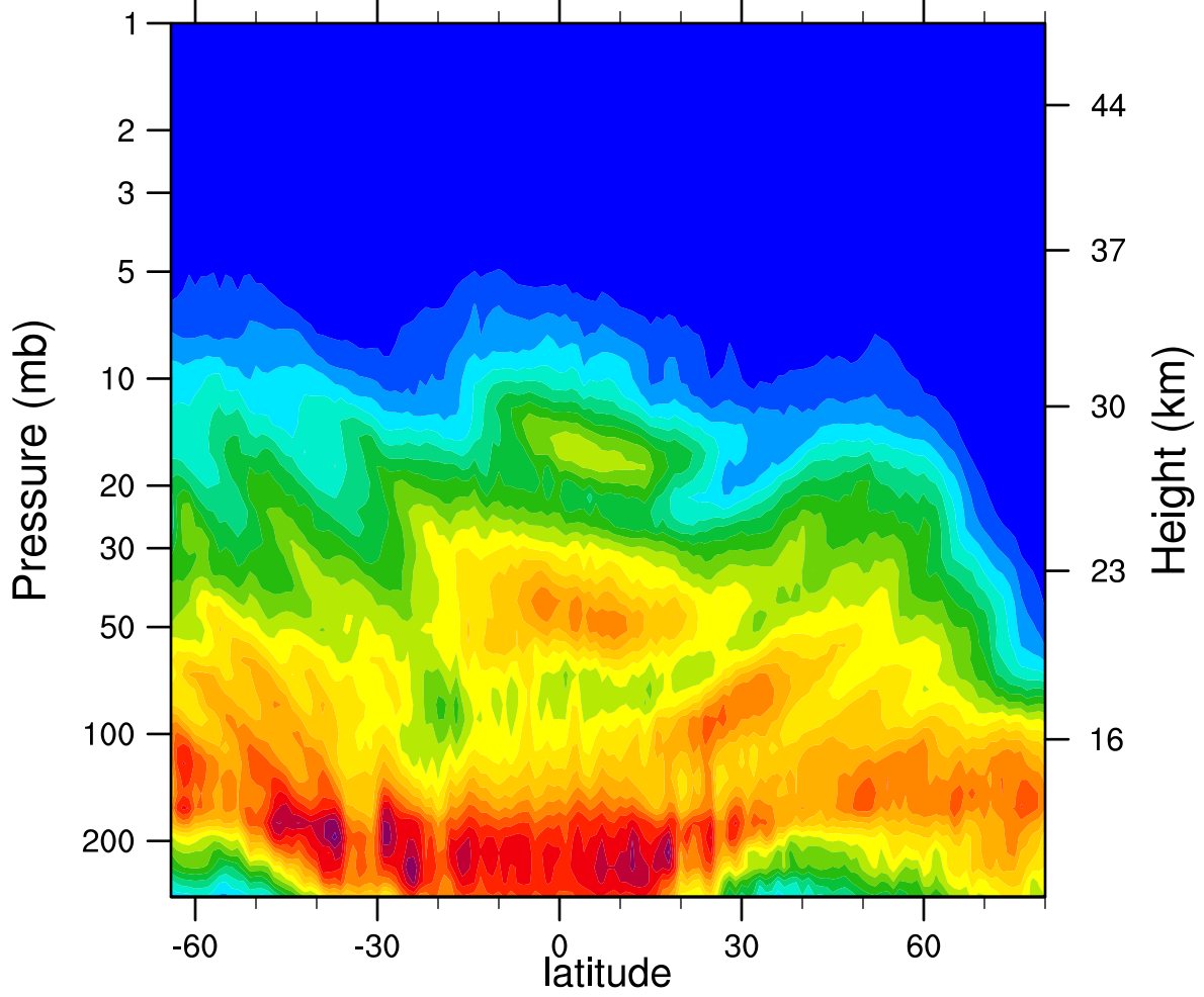
2005d023 N2O_Combined (ppbv)
