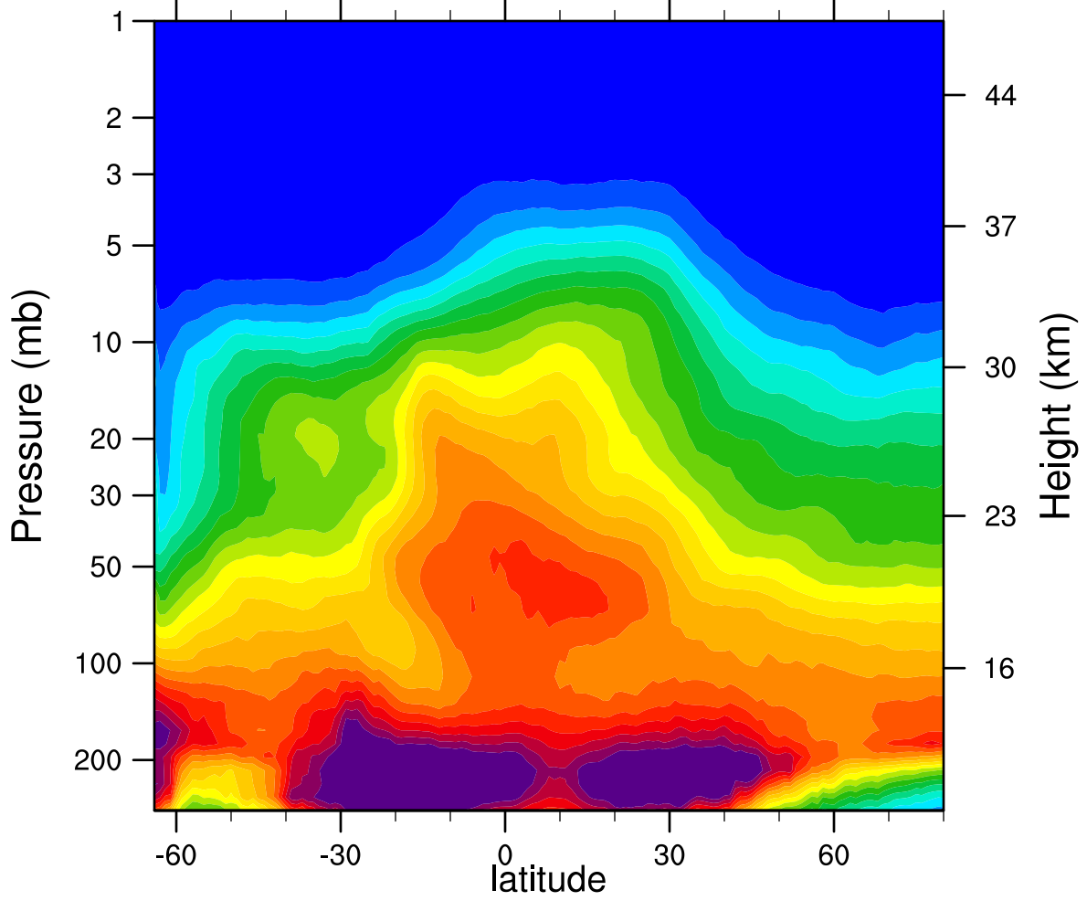
2007d249 N2O_Combined (ppbv)
