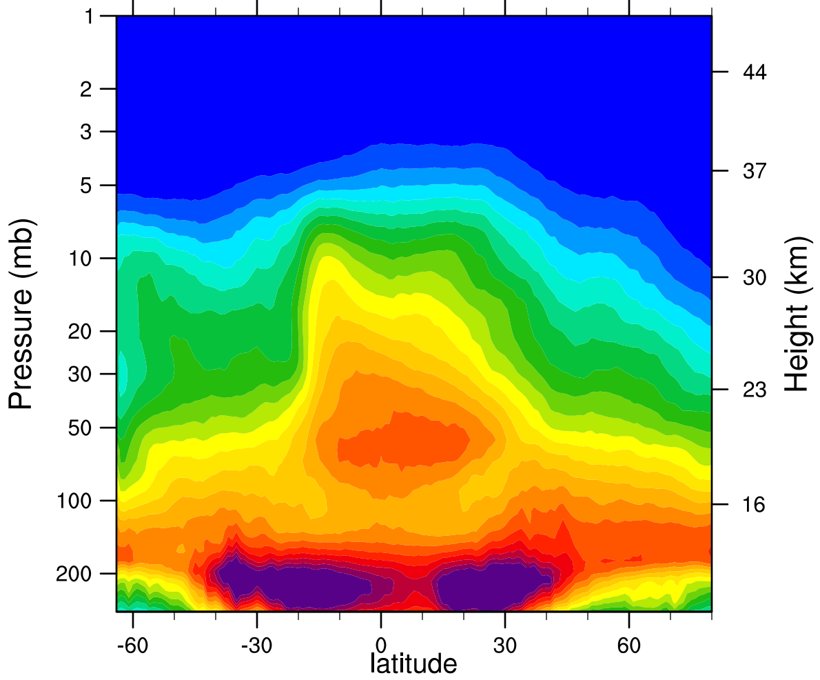
2005d300 N2O_Combined (ppbv)
