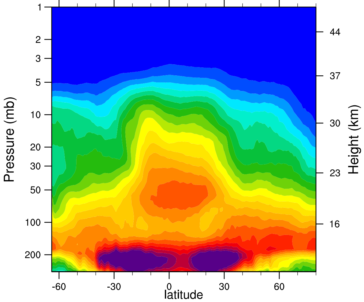
2005d313 N2O_Combined (ppbv)
