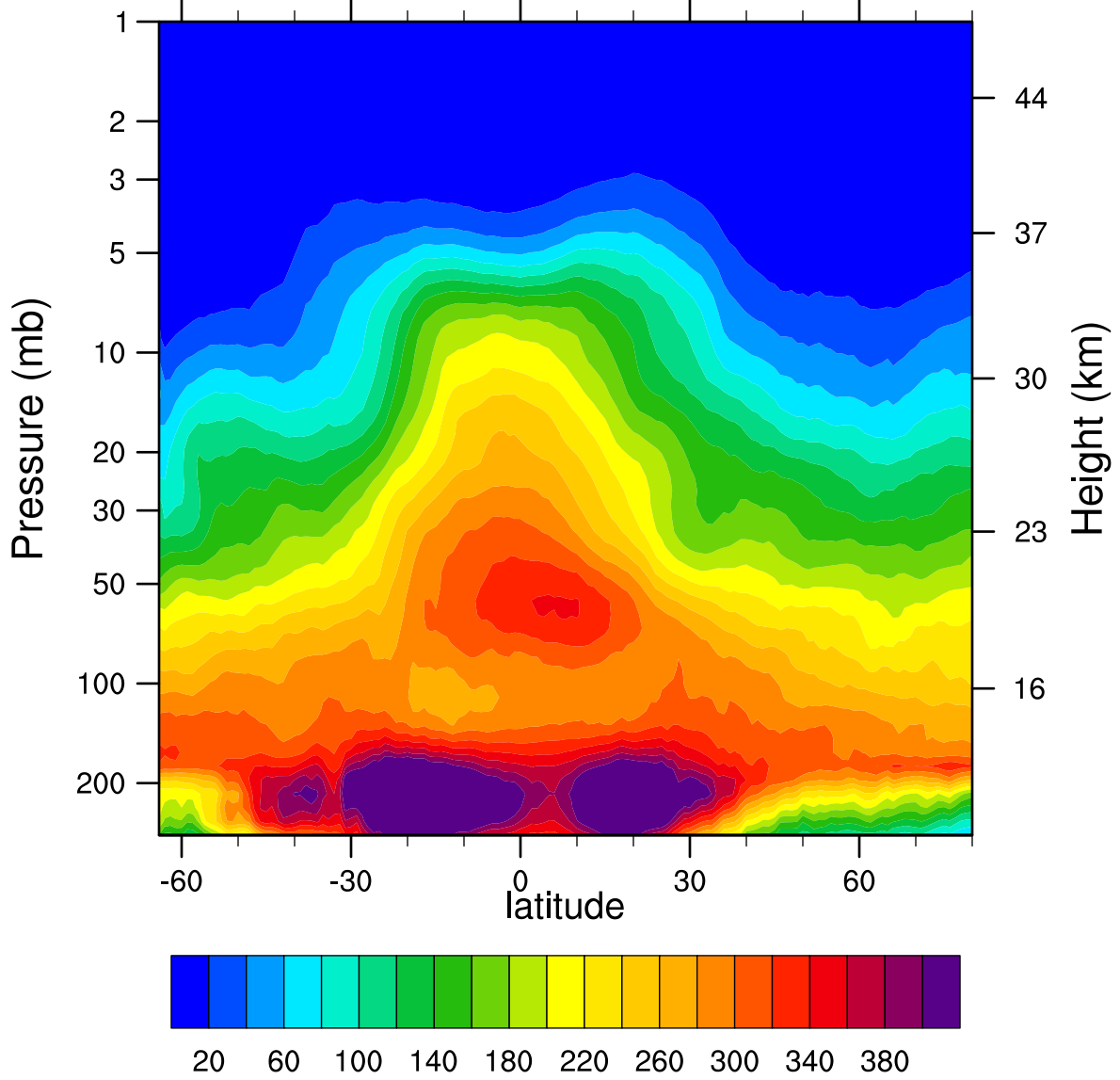
2005d120 N2O_Combined (ppbv)
