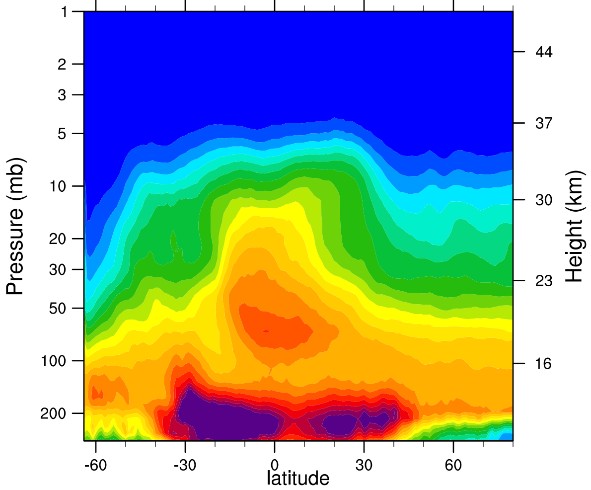
2007d186 N2O_Combined (ppbv)
