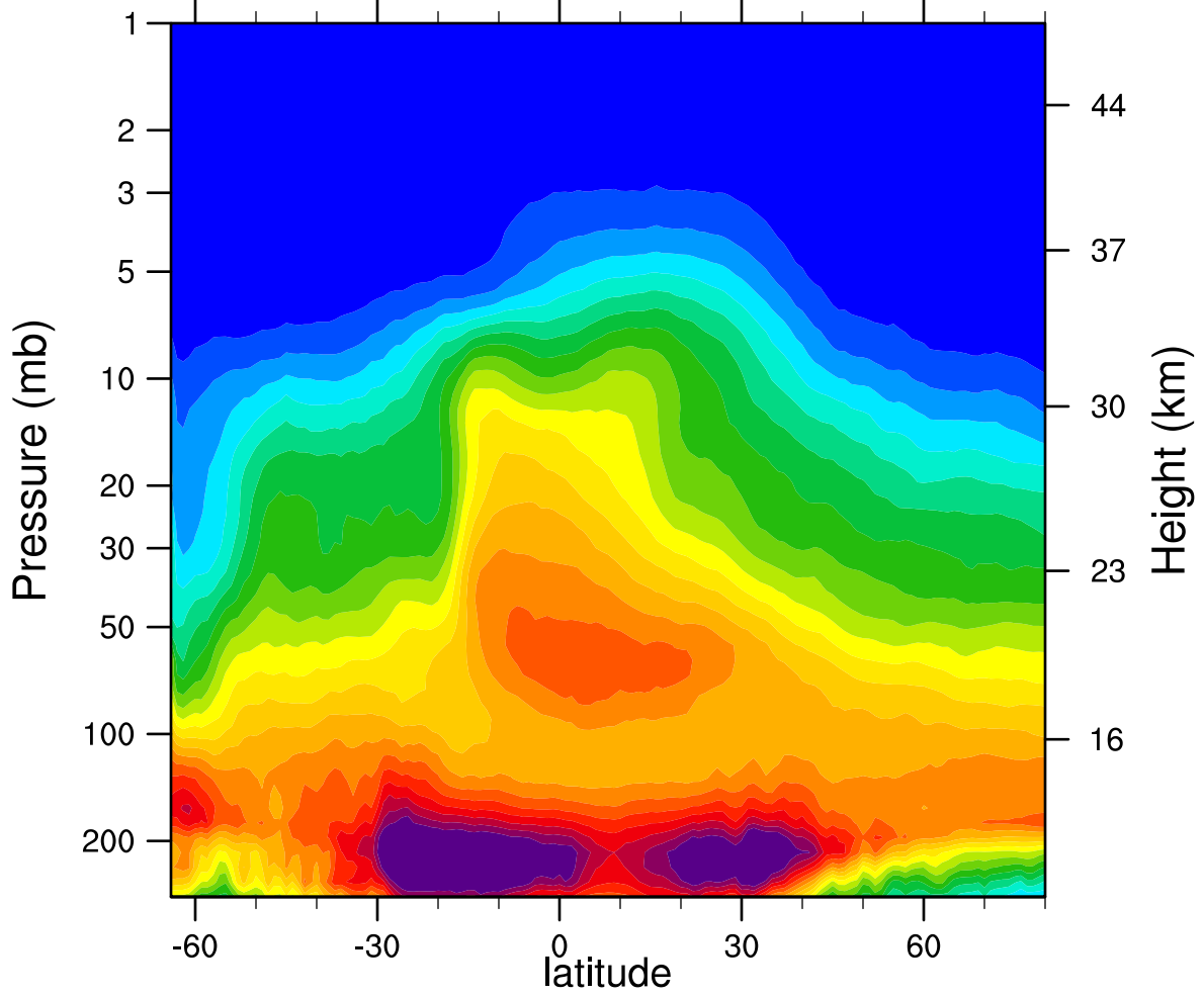
2005d255 N2O_Combined (ppbv)
