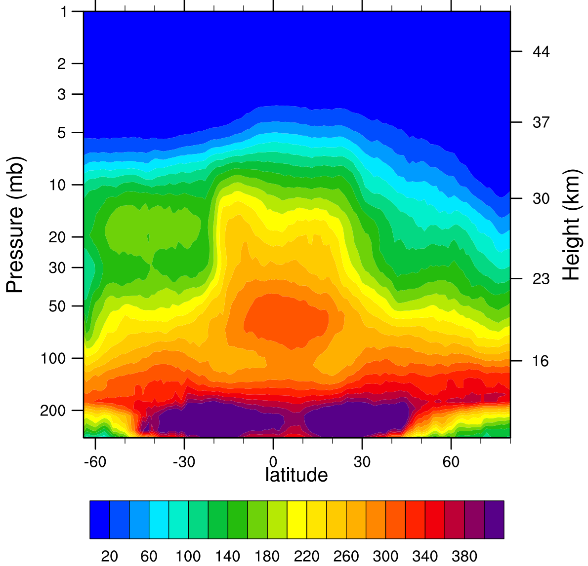
2007d309 N2O_Combined (ppbv)
