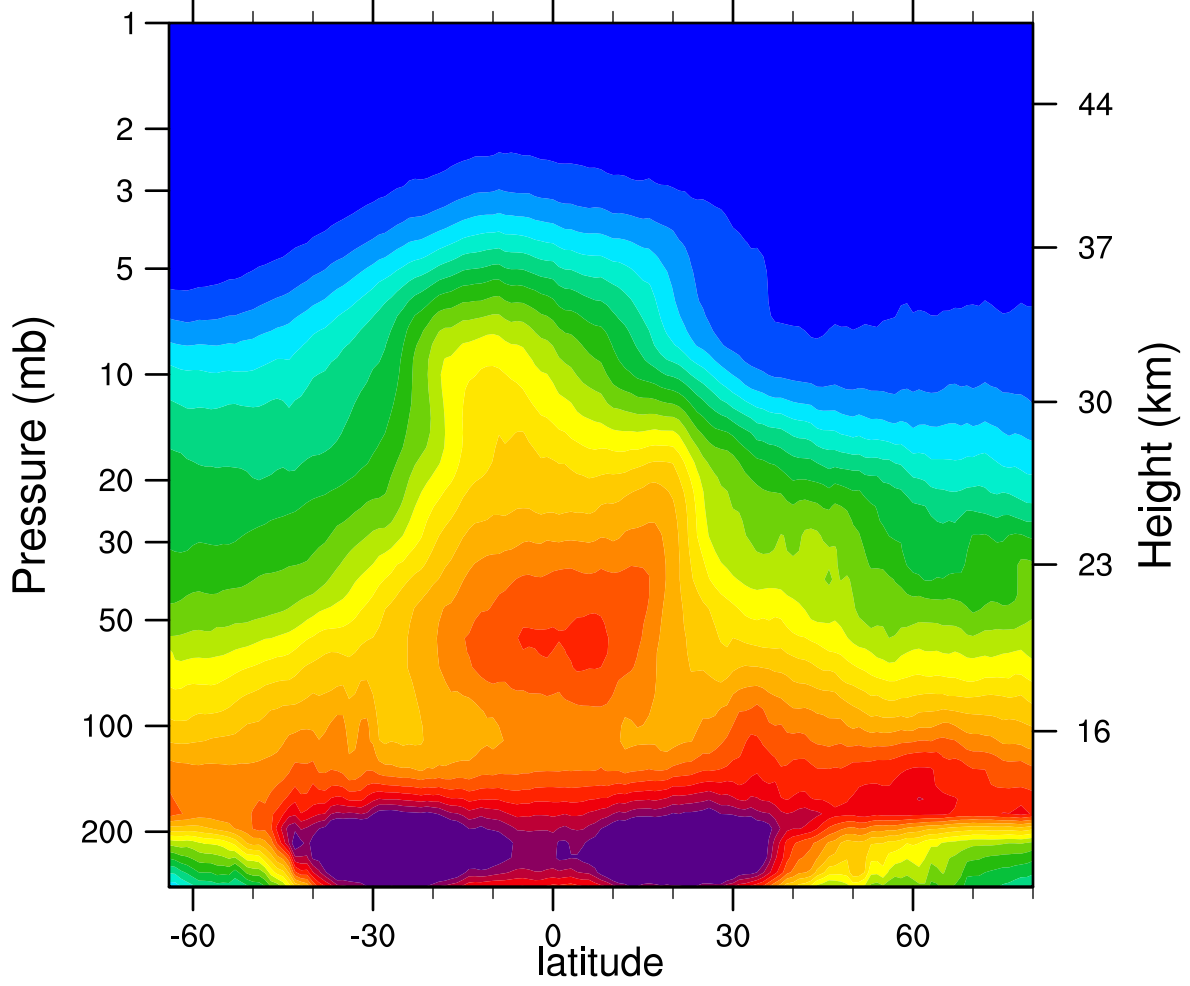
2006d035 N2O_Combined (ppbv)
