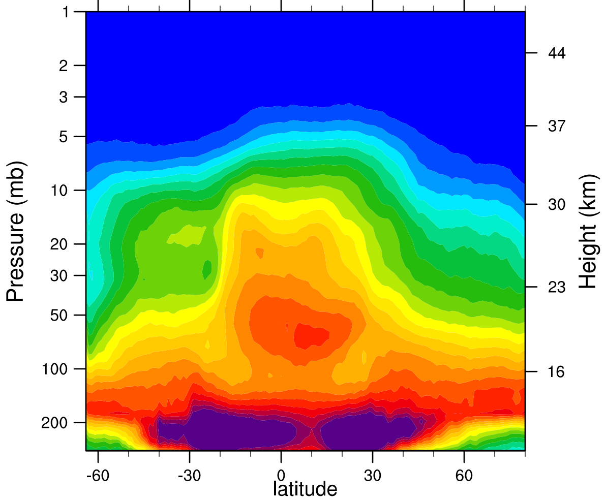
2007d288 N2O_Combined (ppbv)
