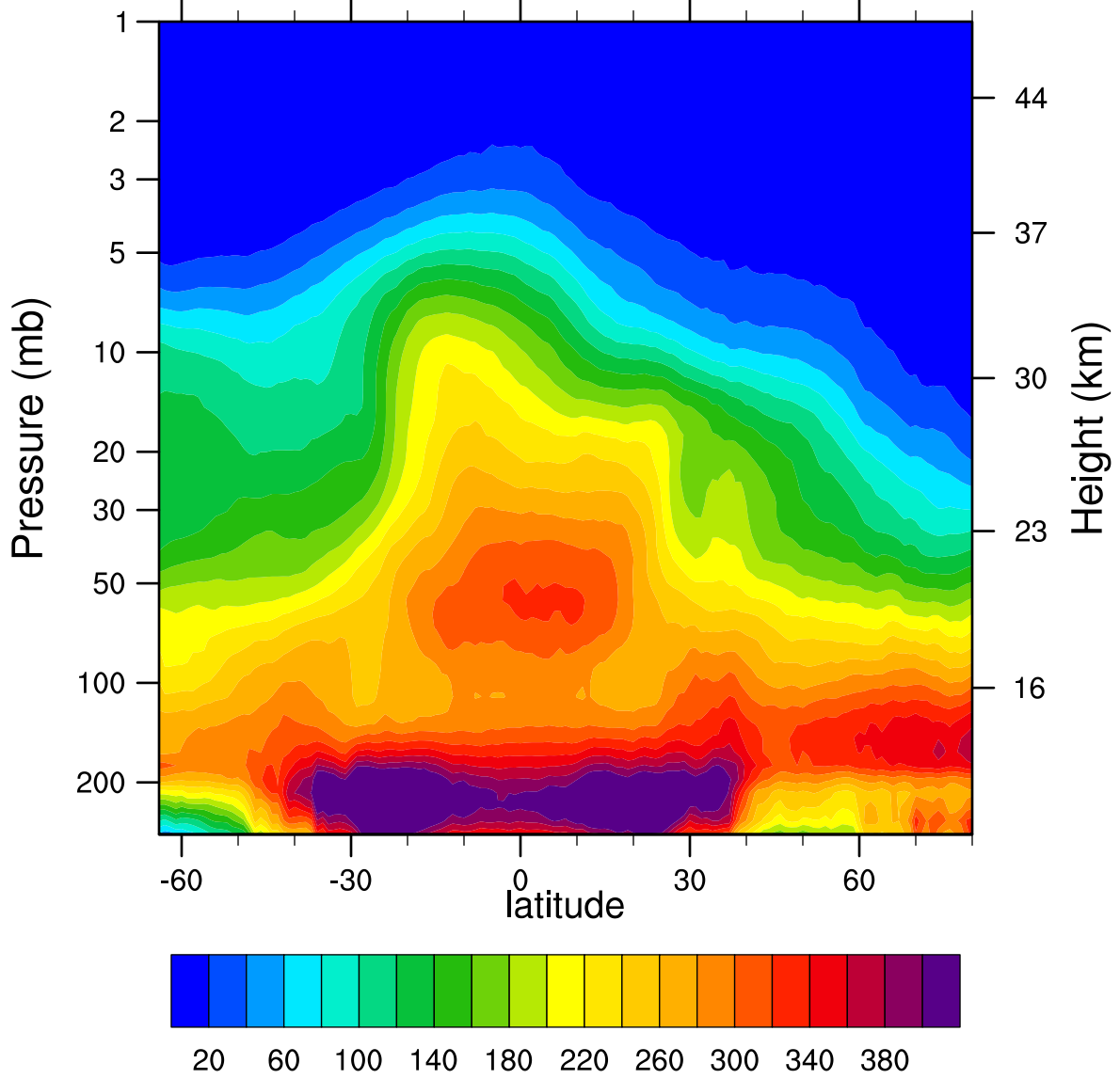
2005d361 N2O_Combined (ppbv)
