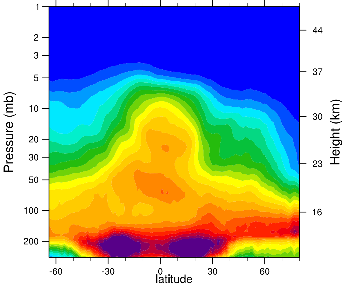
2007d023 N2O_Combined (ppbv)
