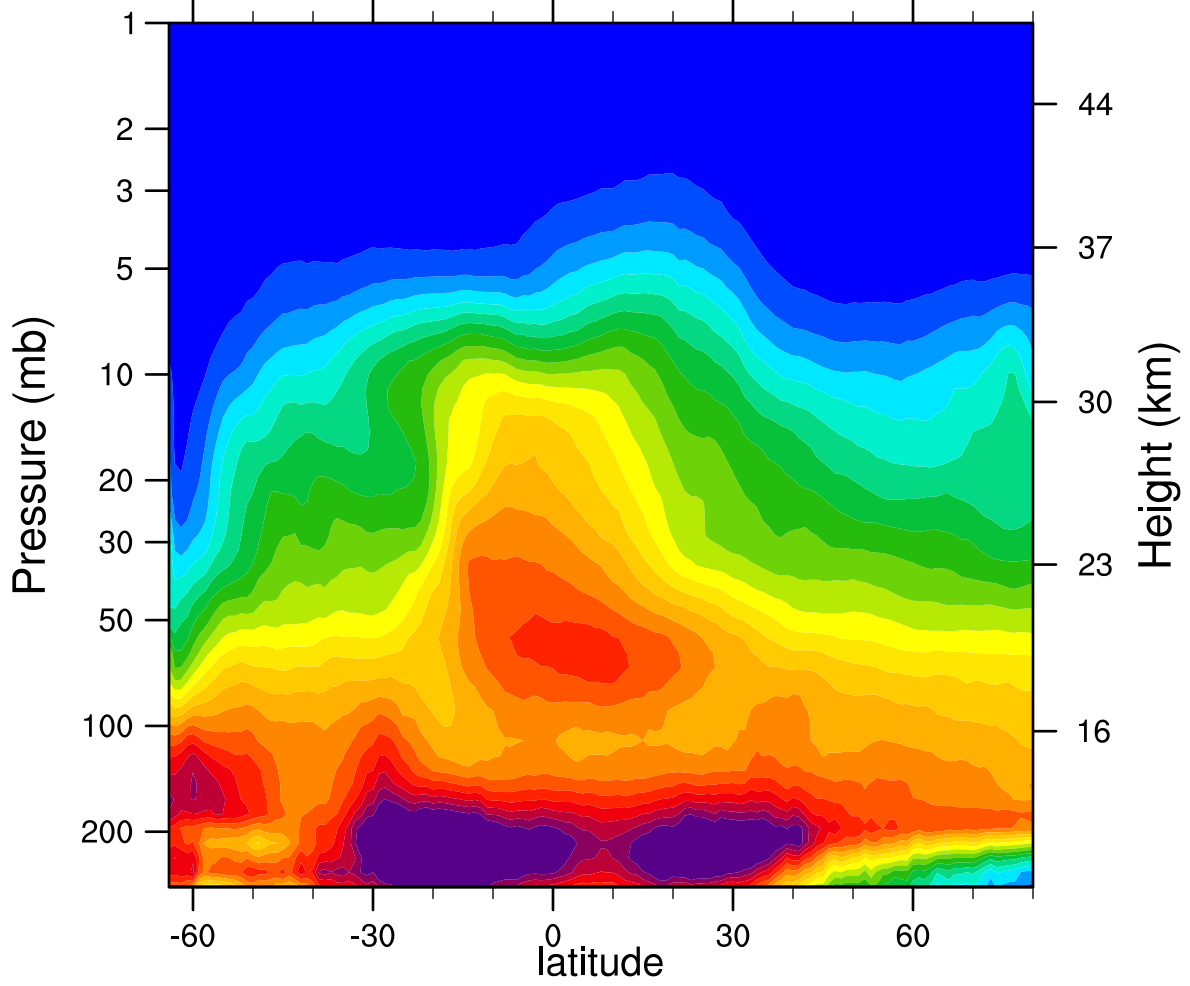
2005d179 N2O_Combined (ppbv)
