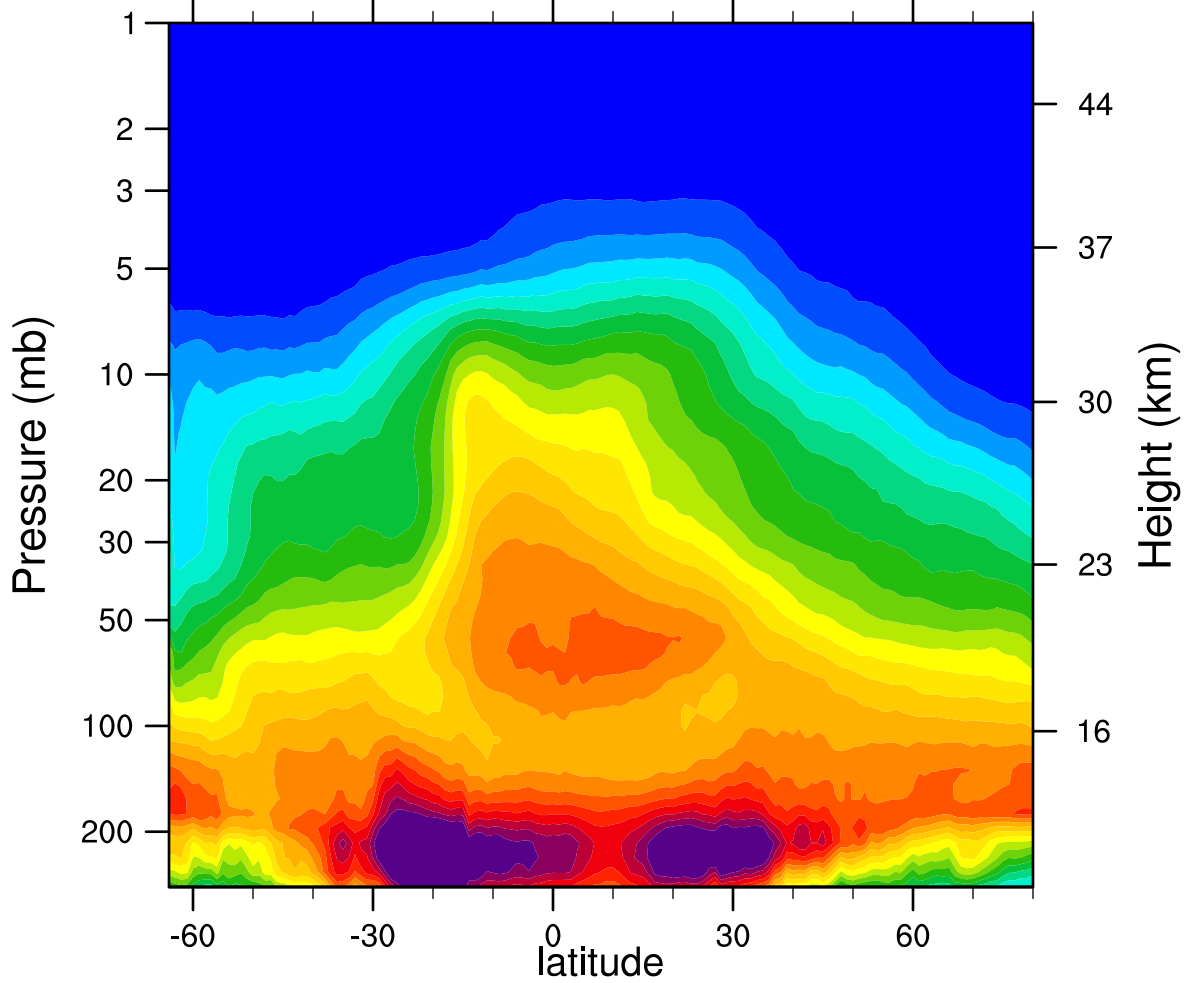
2005d281 N2O_Combined (ppbv)
