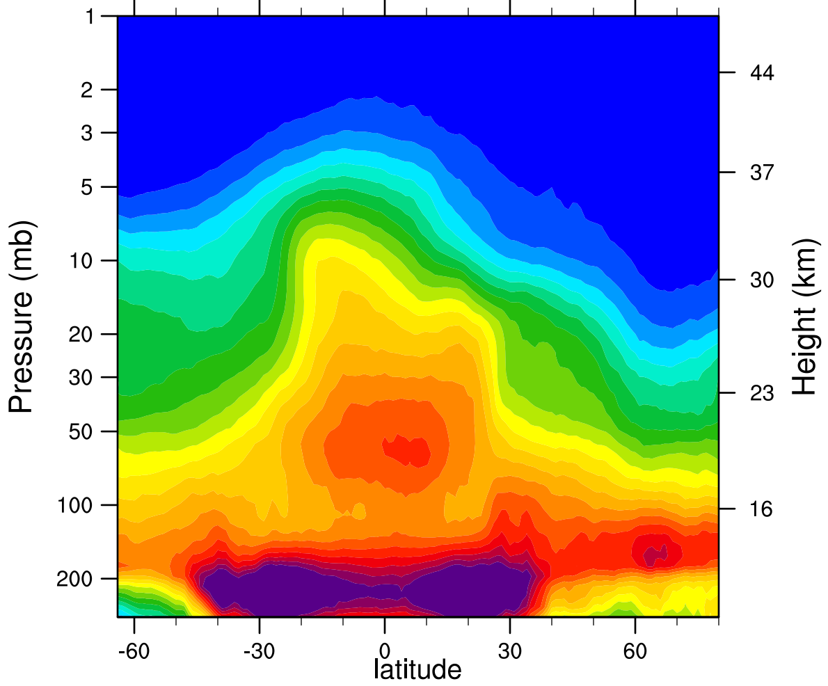
2006d016 N2O_Combined (ppbv)
