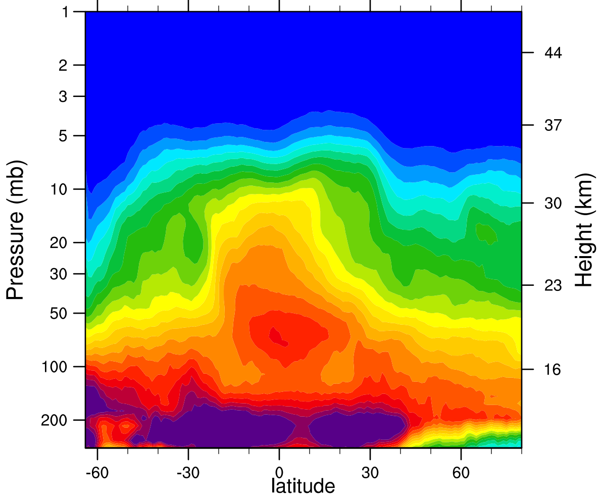
2007d160 N2O_Combined (ppbv)
