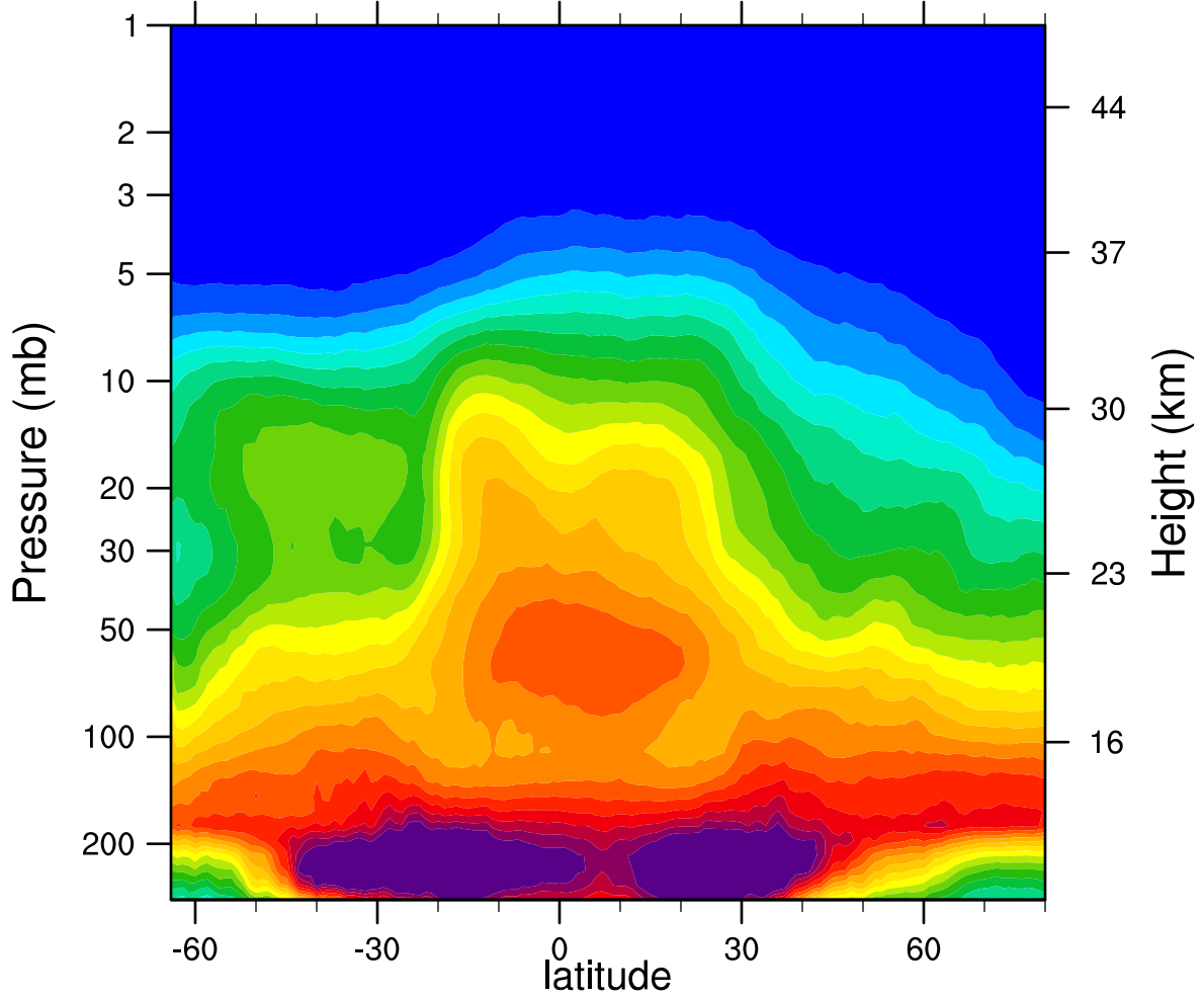
2007d303 N2O_Combined (ppbv)
