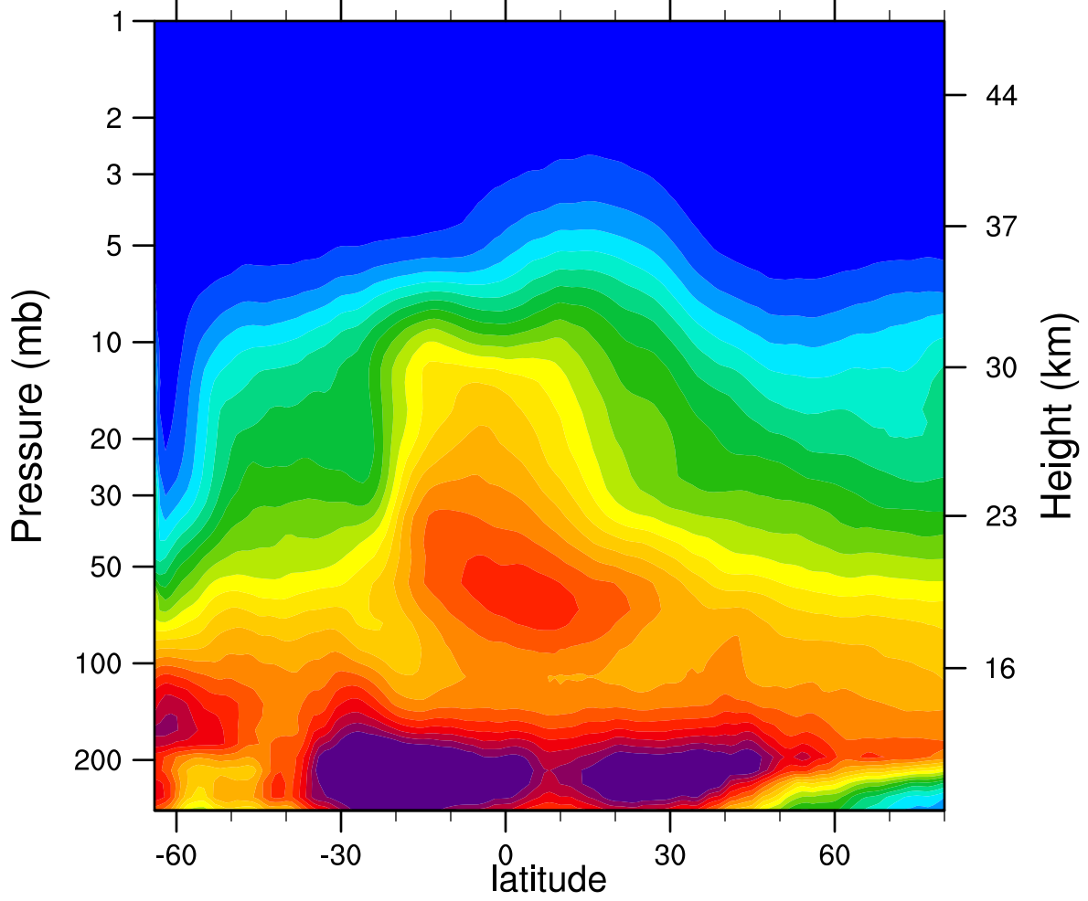
2005d194 N2O_Combined (ppbv)
