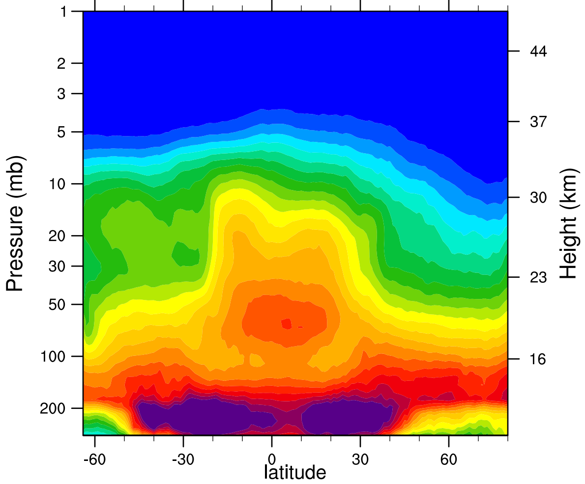
2007d322 N2O_Combined (ppbv)
