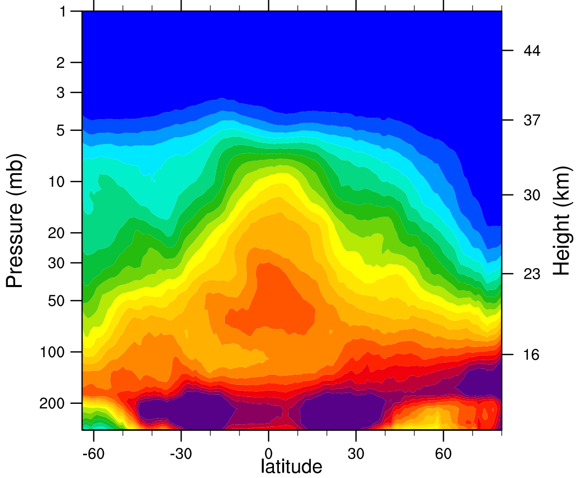
2006d345 N2O_Combined (ppbv)
