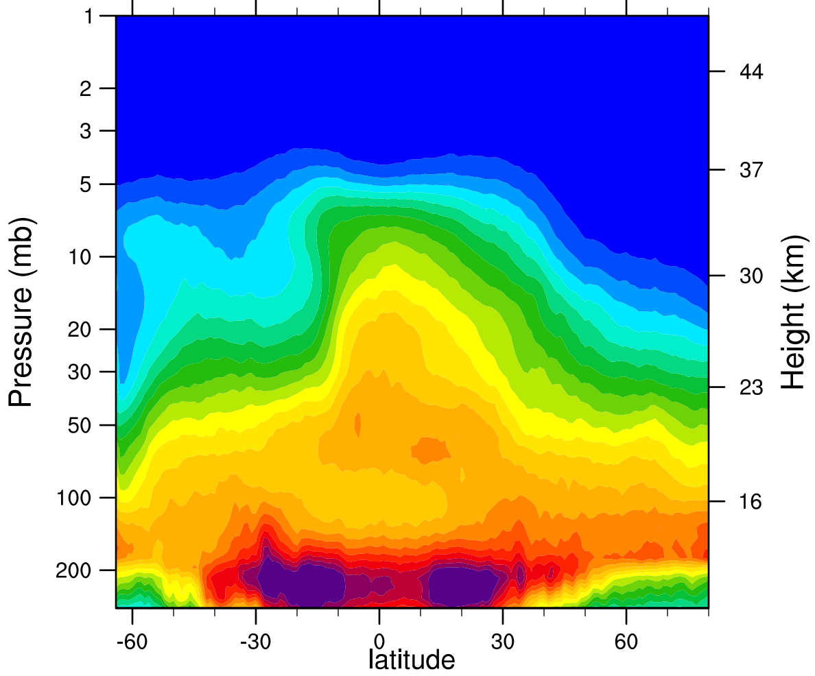
2006d305 N2O_Combined (ppbv)
