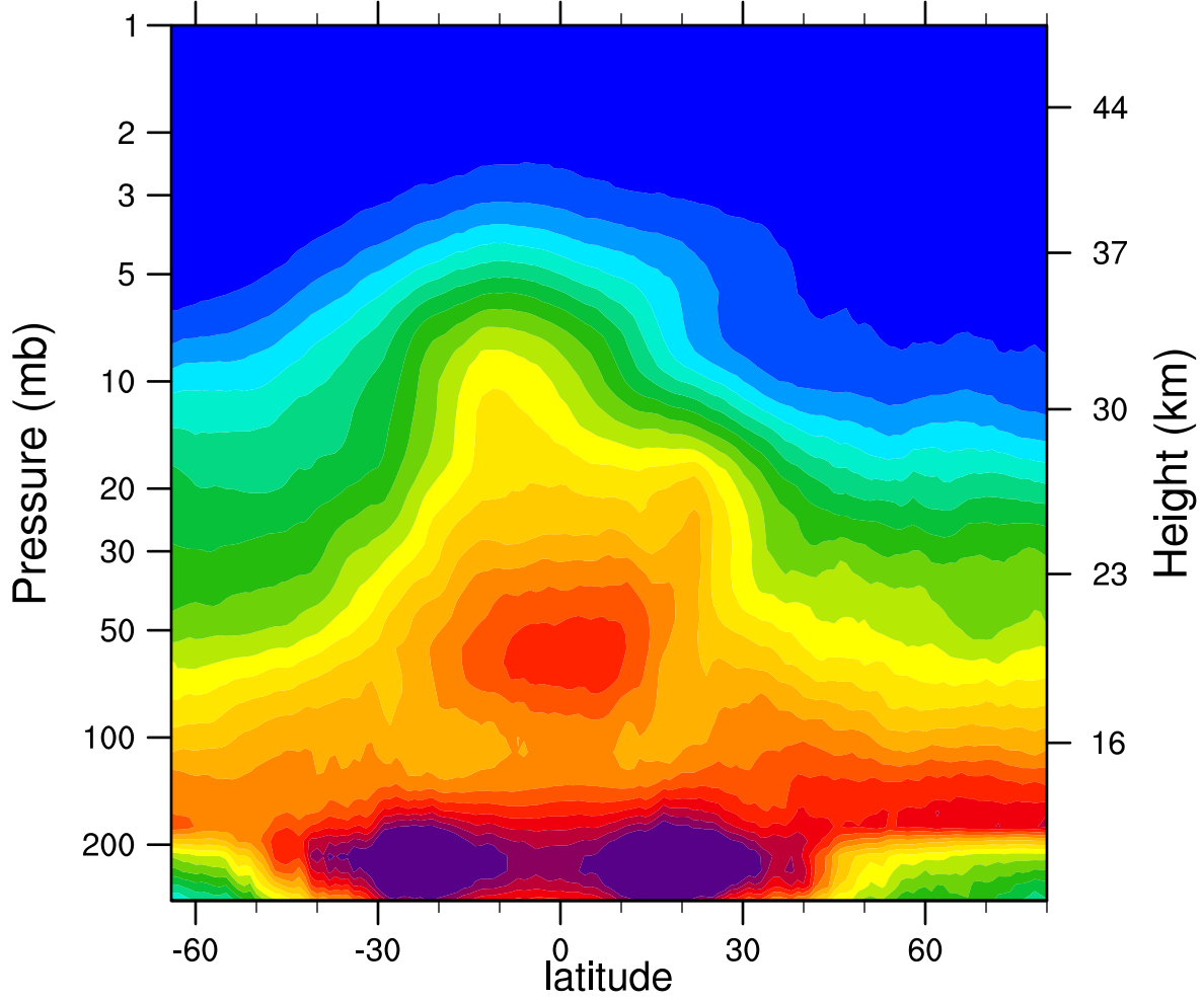
2006d050 N2O_Combined (ppbv)
