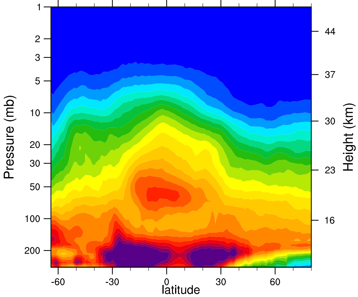
2006d151 N2O_Combined (ppbv)
