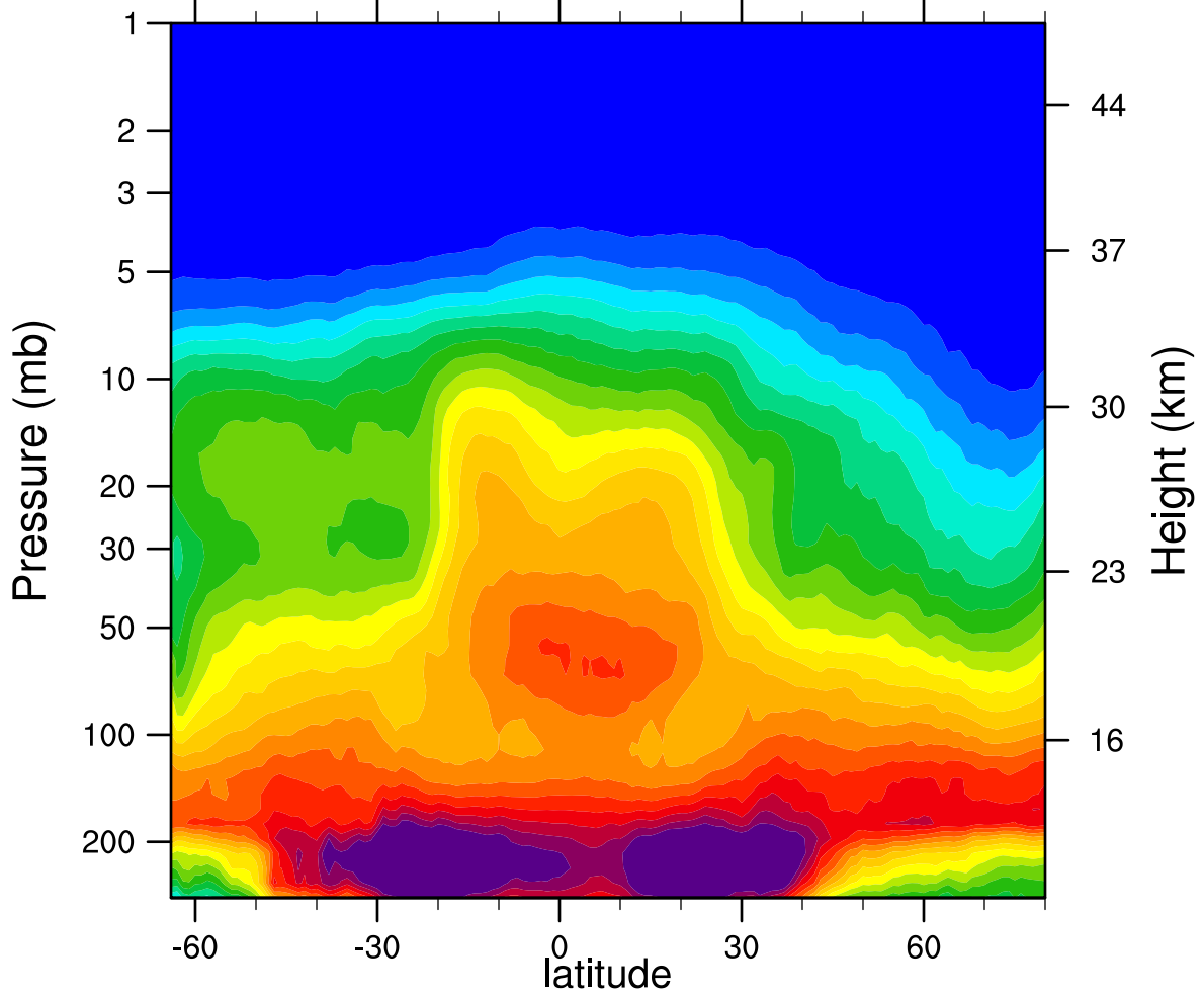
2007d317 N2O_Combined (ppbv)
