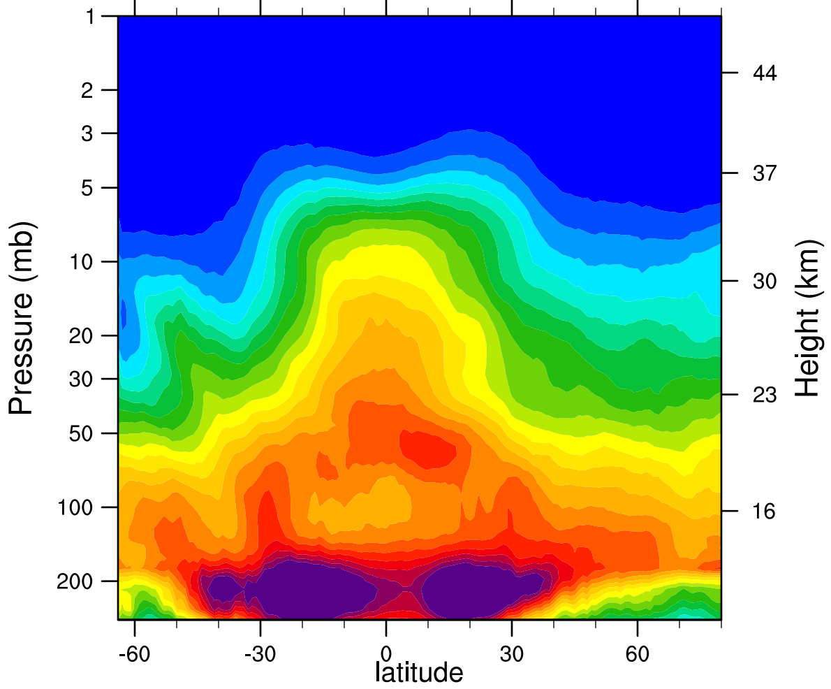
2005d111 N2O_Combined (ppbv)
