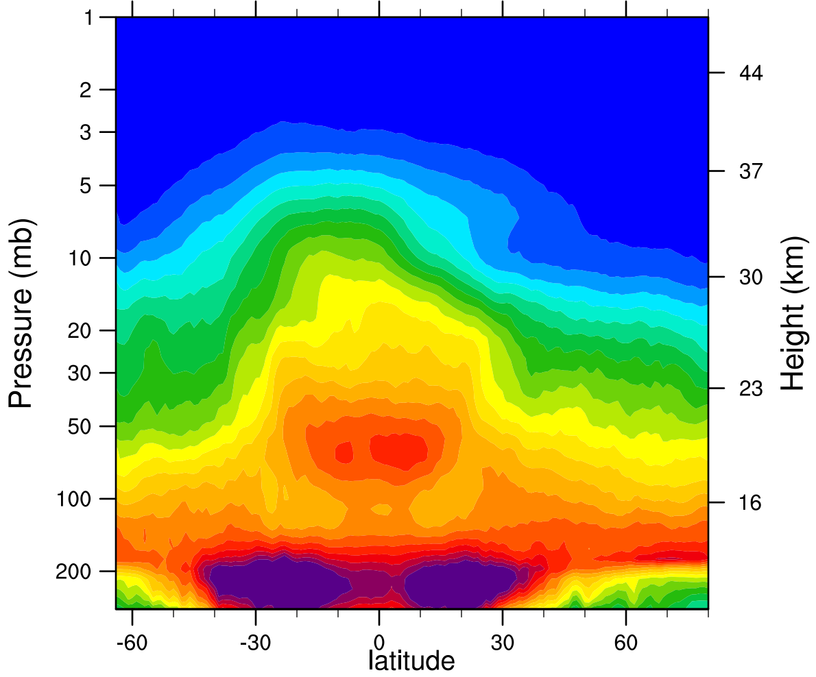
2006d095 N2O_Combined (ppbv)
