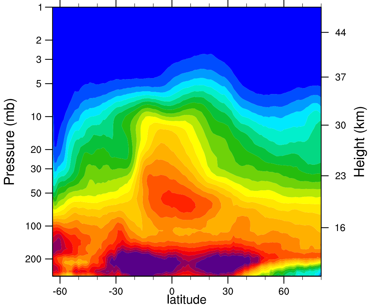
2005d182 N2O_Combined (ppbv)
