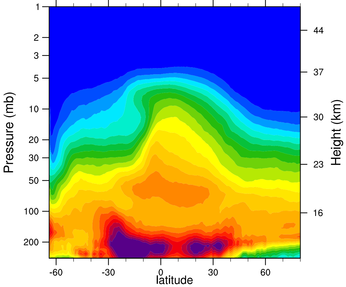
2006d252 N2O_Combined (ppbv)
