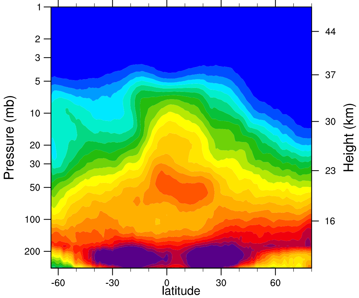
2006d319 N2O_Combined (ppbv)
