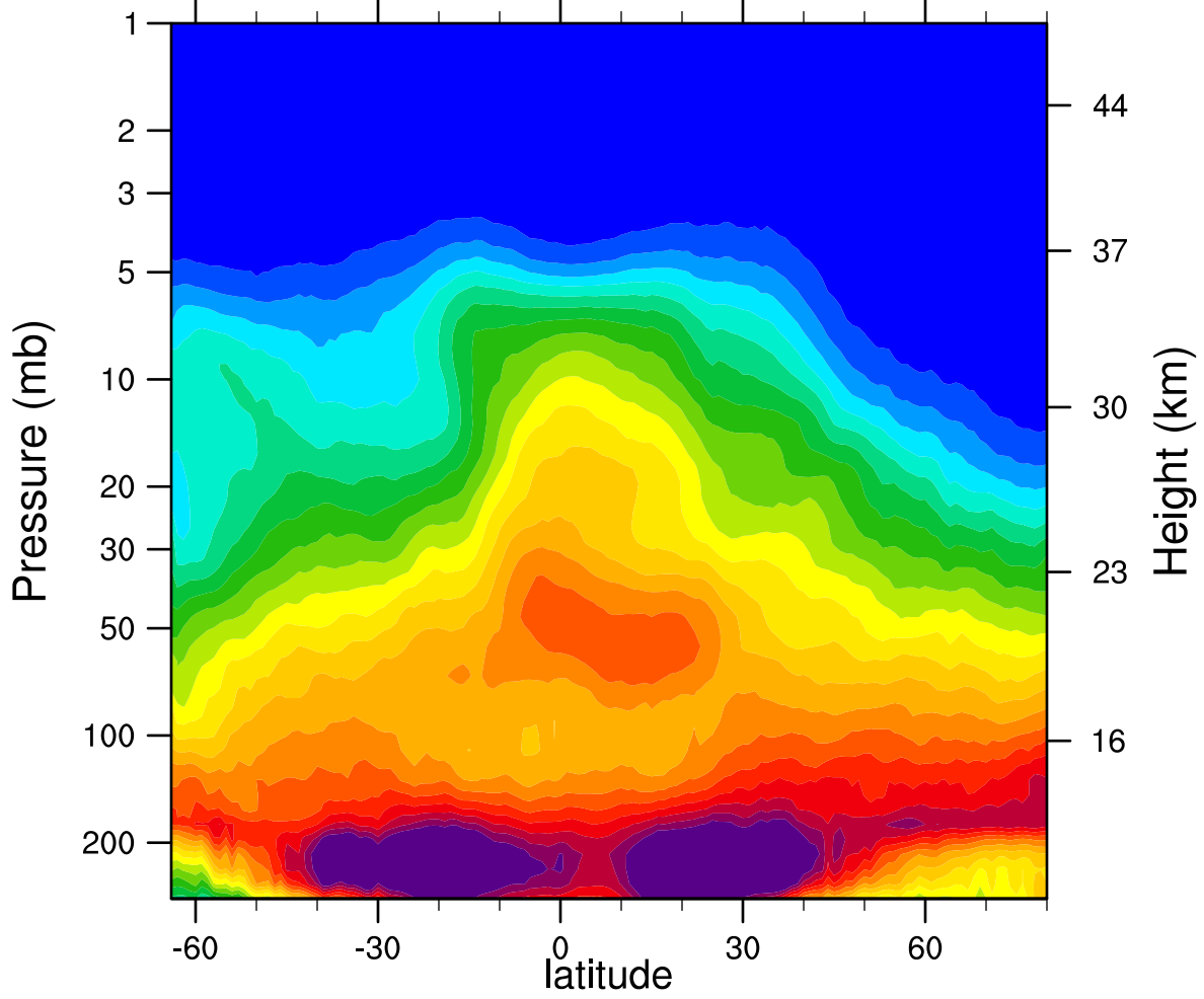
2006d318 N2O_Combined (ppbv)
