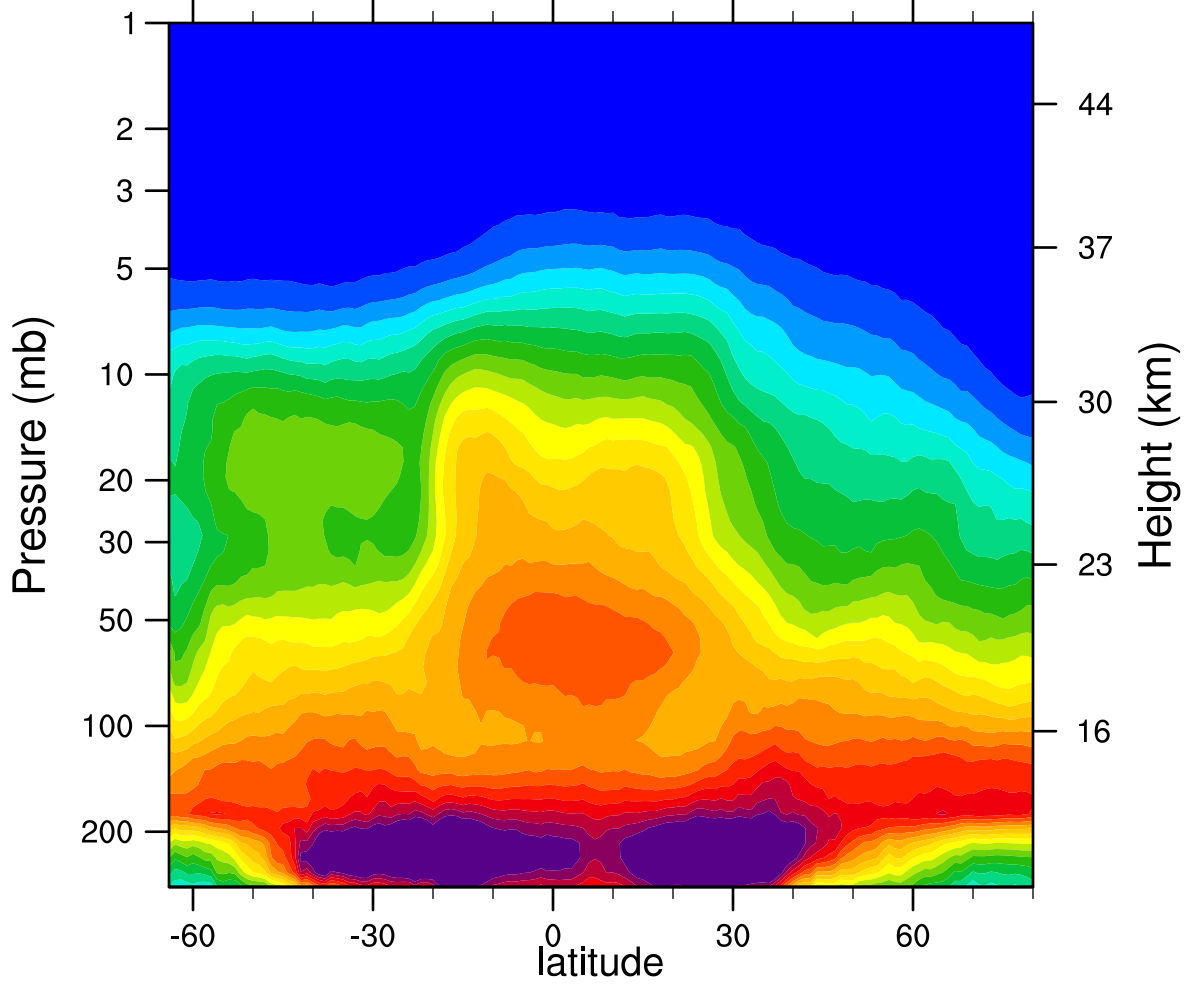
2007d305 N2O_Combined (ppbv)
