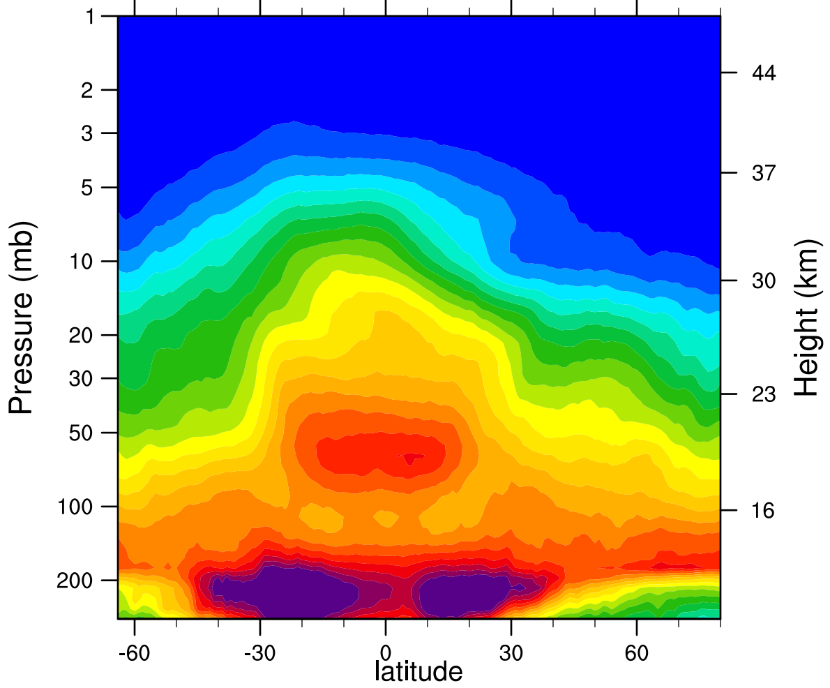
2006d106 N2O_Combined (ppbv)
