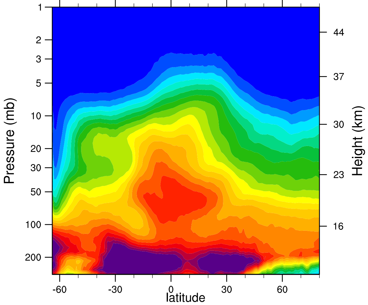
2007d235 N2O_Combined (ppbv)
