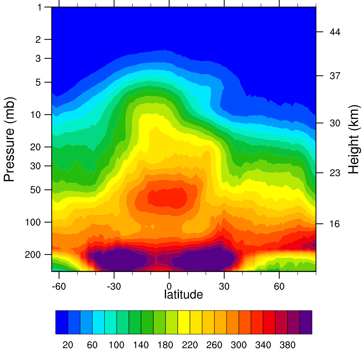
2006d067 N2O_Combined (ppbv)
