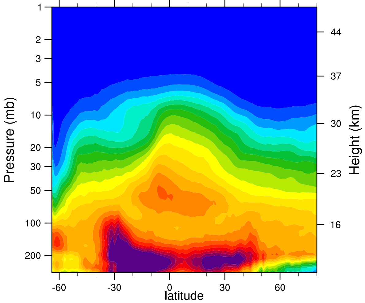
2006d203 N2O_Combined (ppbv)
