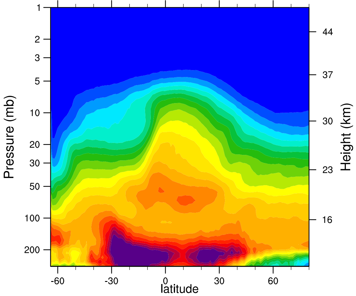
2006d239 N2O_Combined (ppbv)
