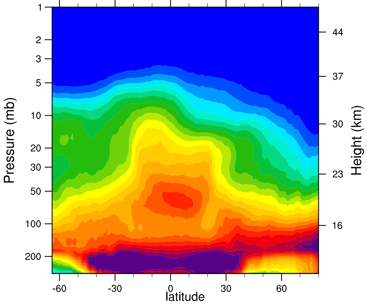
2007d352 N2O_Combined (ppbv)
