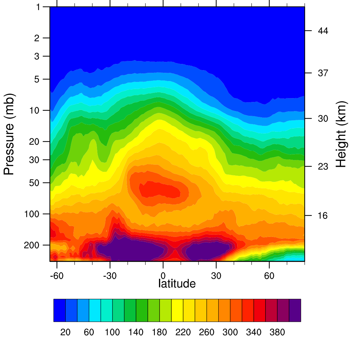
2006d147 N2O_Combined (ppbv)
