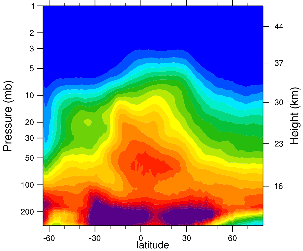
2007d251 N2O_Combined (ppbv)
