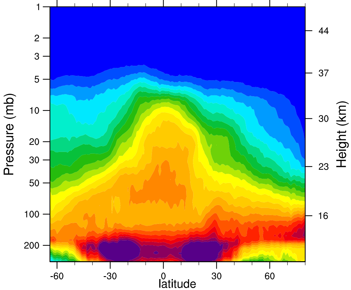
2006d358 N2O_Combined (ppbv)
