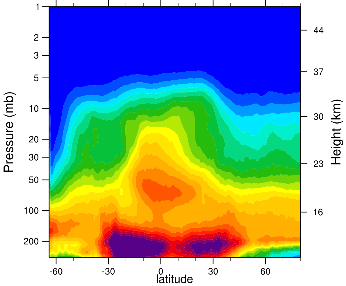
2007d194 N2O_Combined (ppbv)
