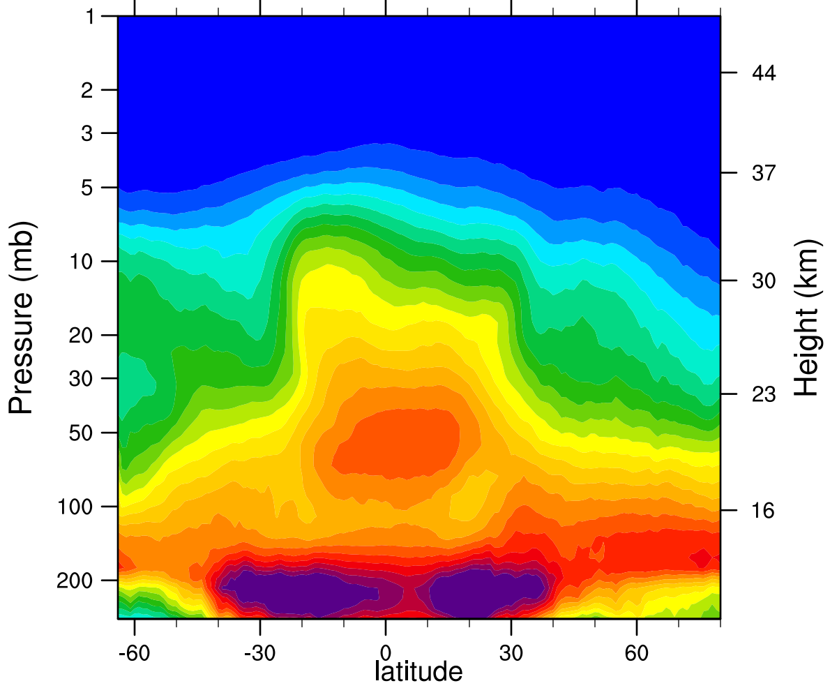
2005d328 N2O_Combined (ppbv)
