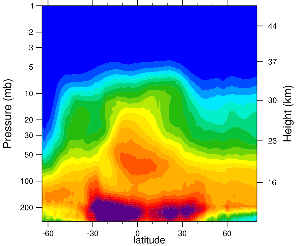
2007d192 N2O_Combined (ppbv)
