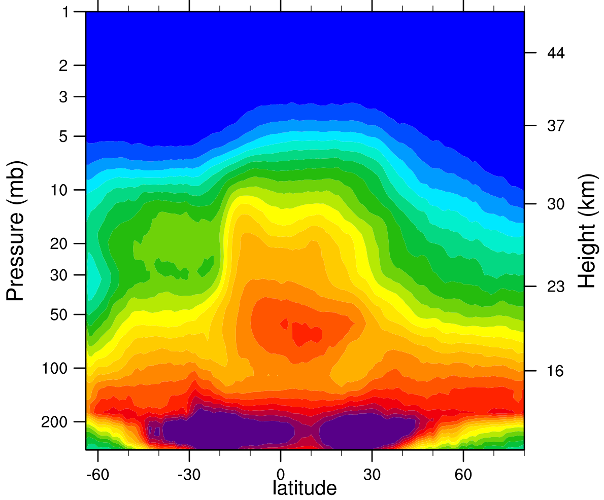
2007d293 N2O_Combined (ppbv)
