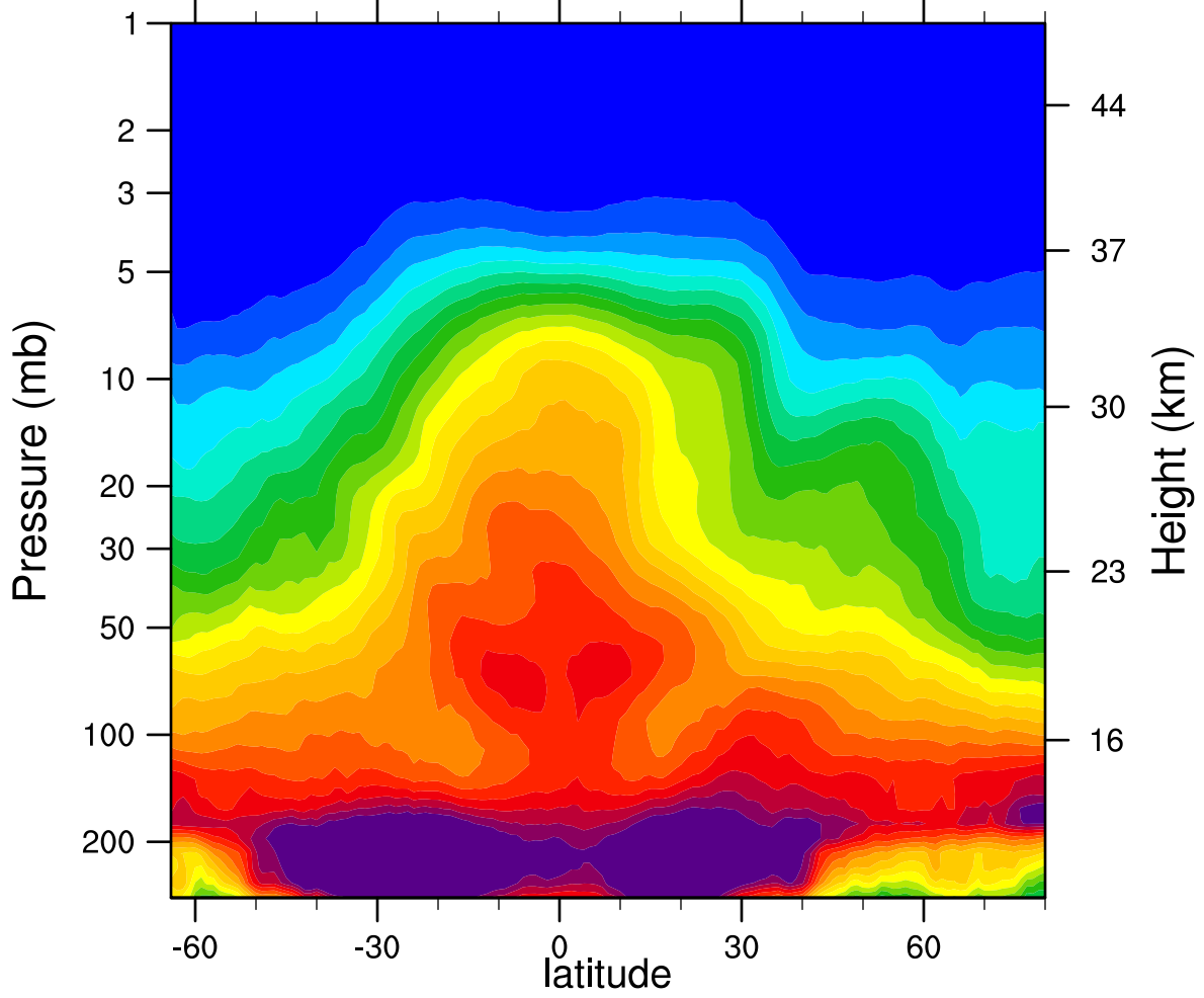
2007d101 N2O_Combined (ppbv)
