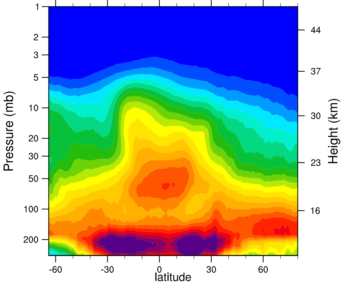
2005d333 N2O_Combined (ppbv)
