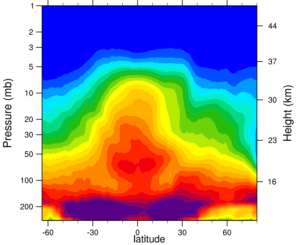
2007d104 N2O_Combined (ppbv)
