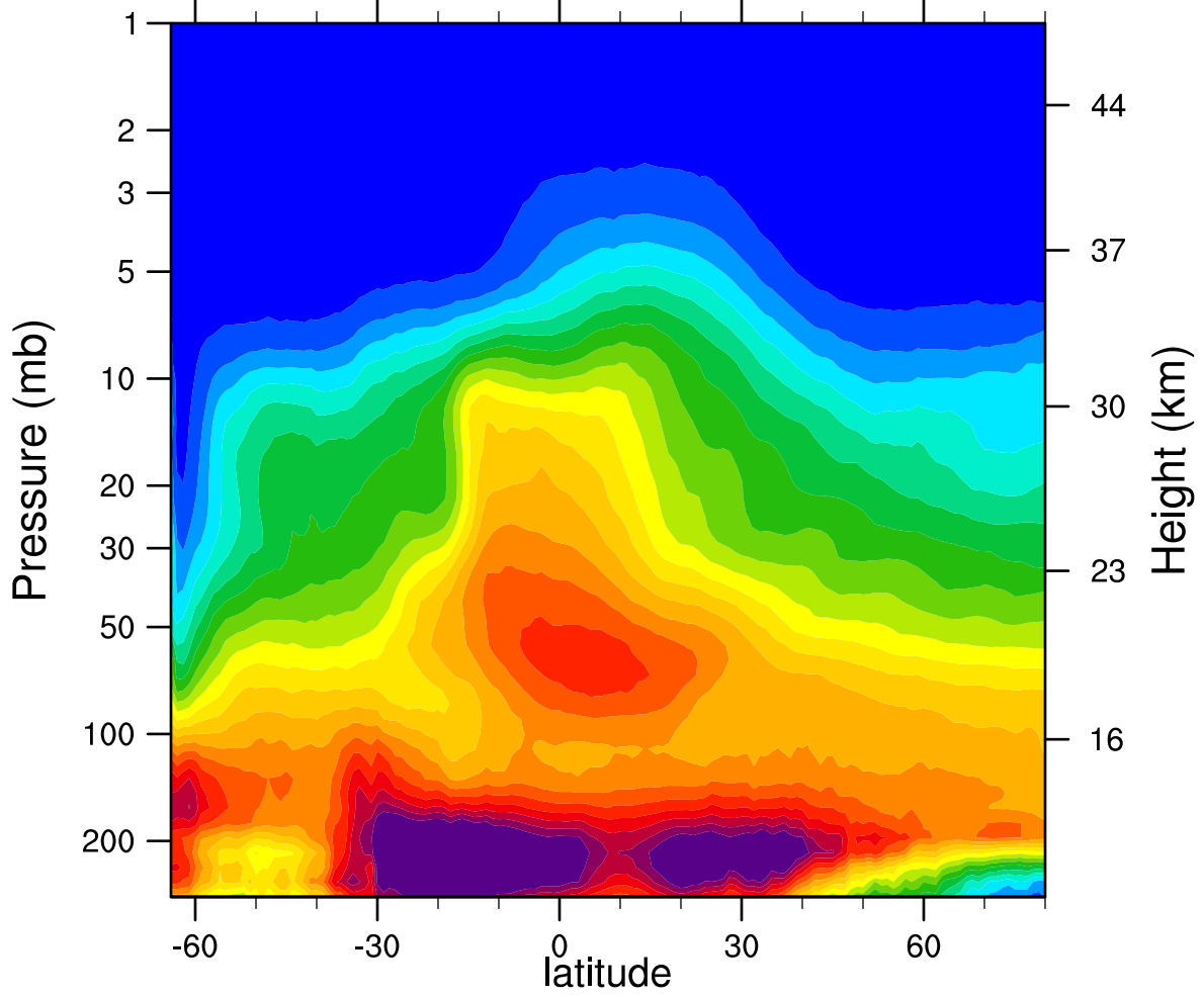
2005d215 N2O_Combined (ppbv)
