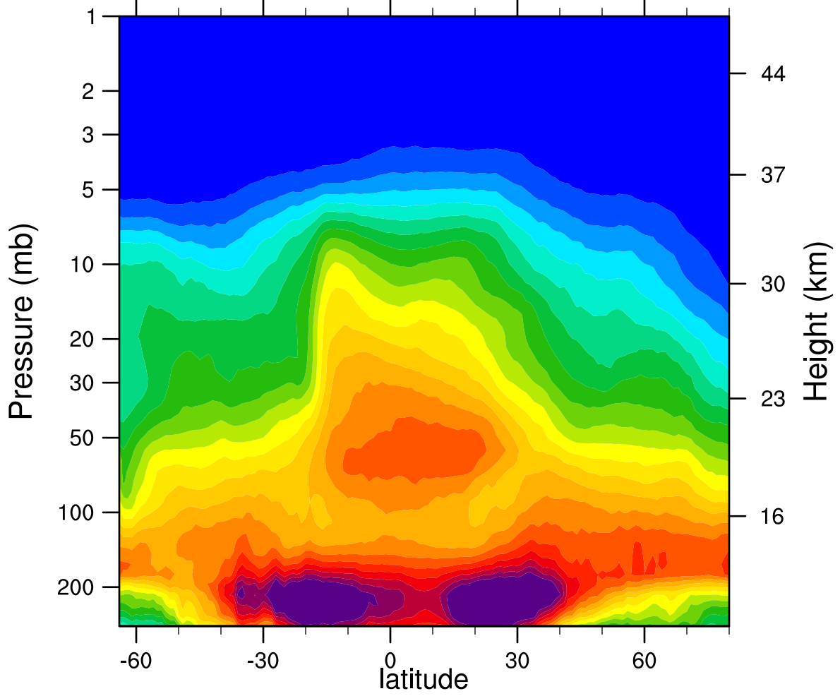
2005d303 N2O_Combined (ppbv)
