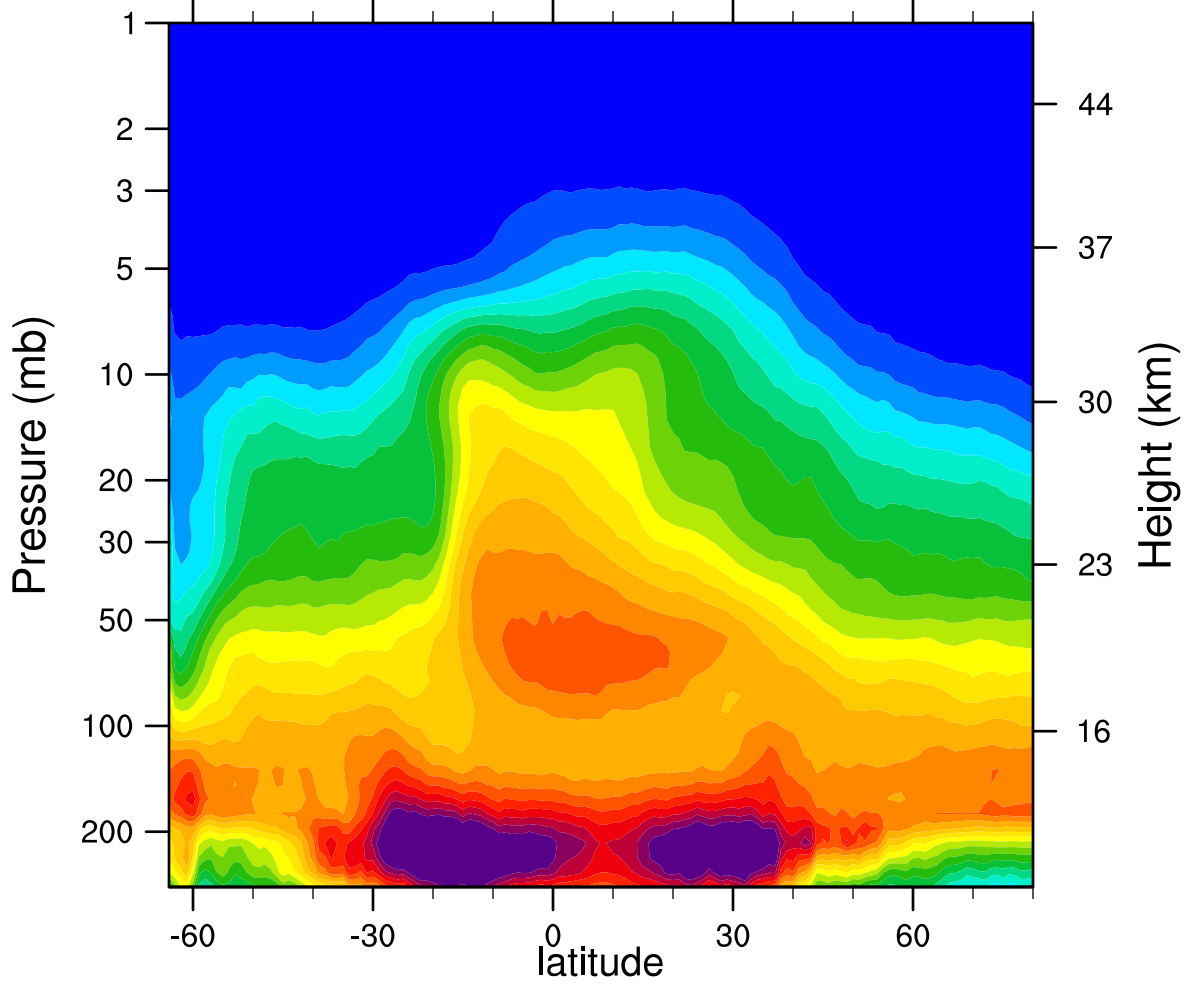
2005d264 N2O_Combined (ppbv)
