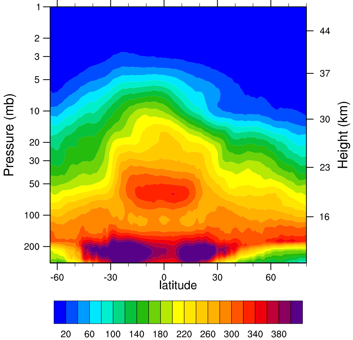
2006d108 N2O_Combined (ppbv)
