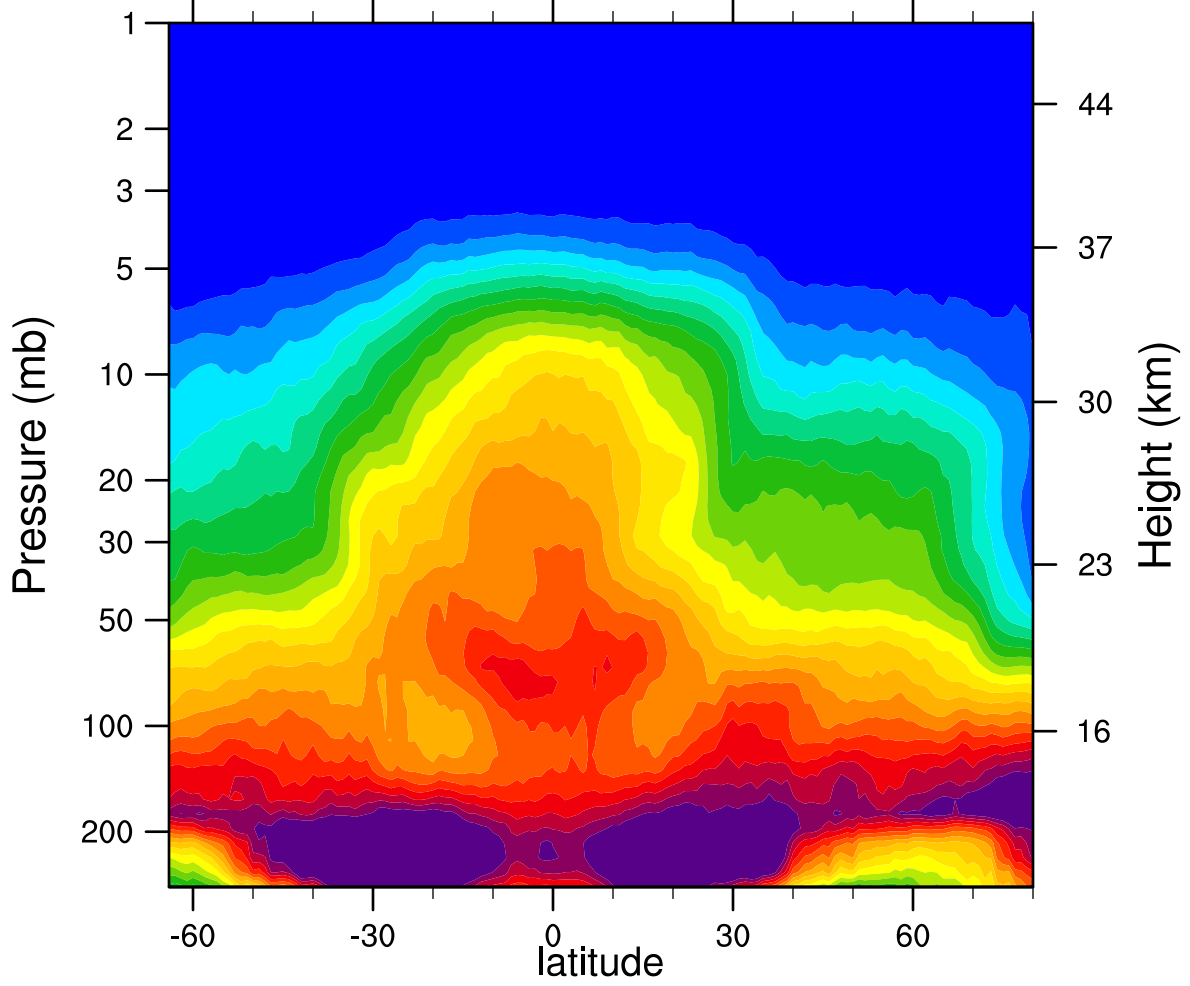
2007d081 N2O_Combined (ppbv)
