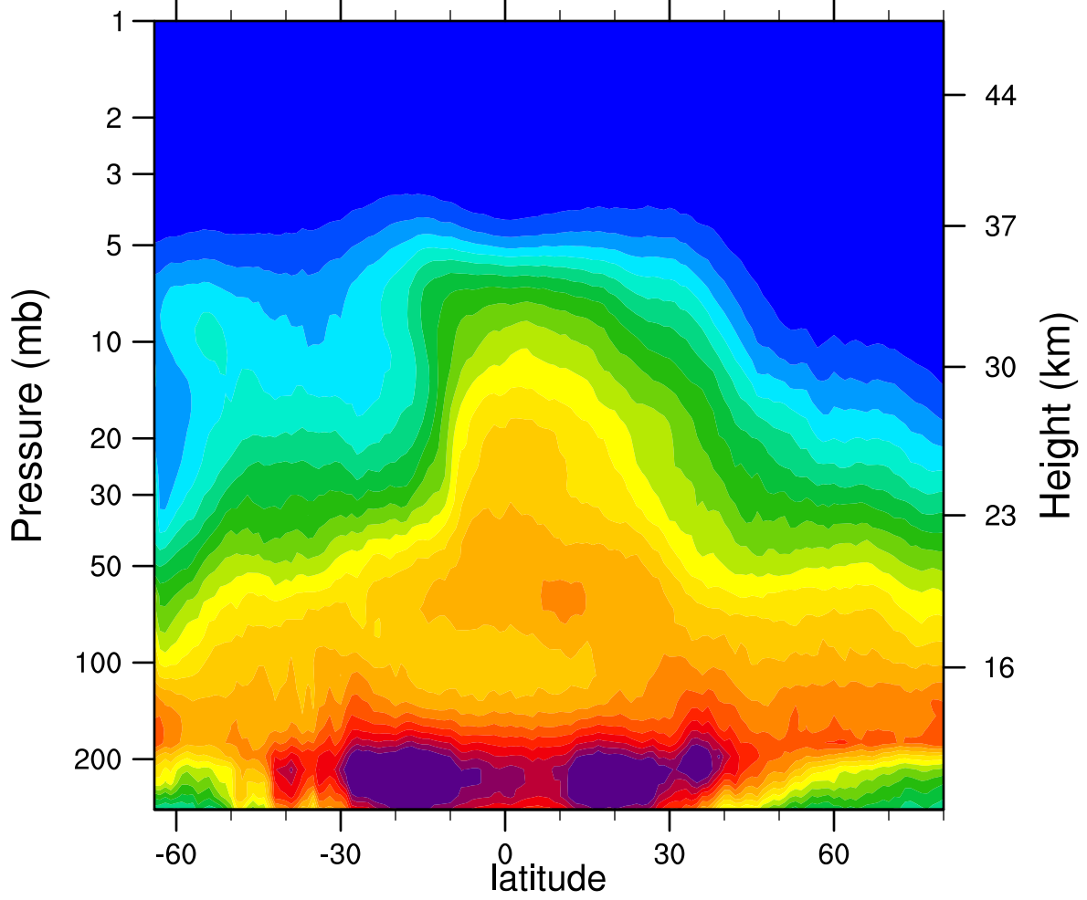
2006d307 N2O_Combined (ppbv)
