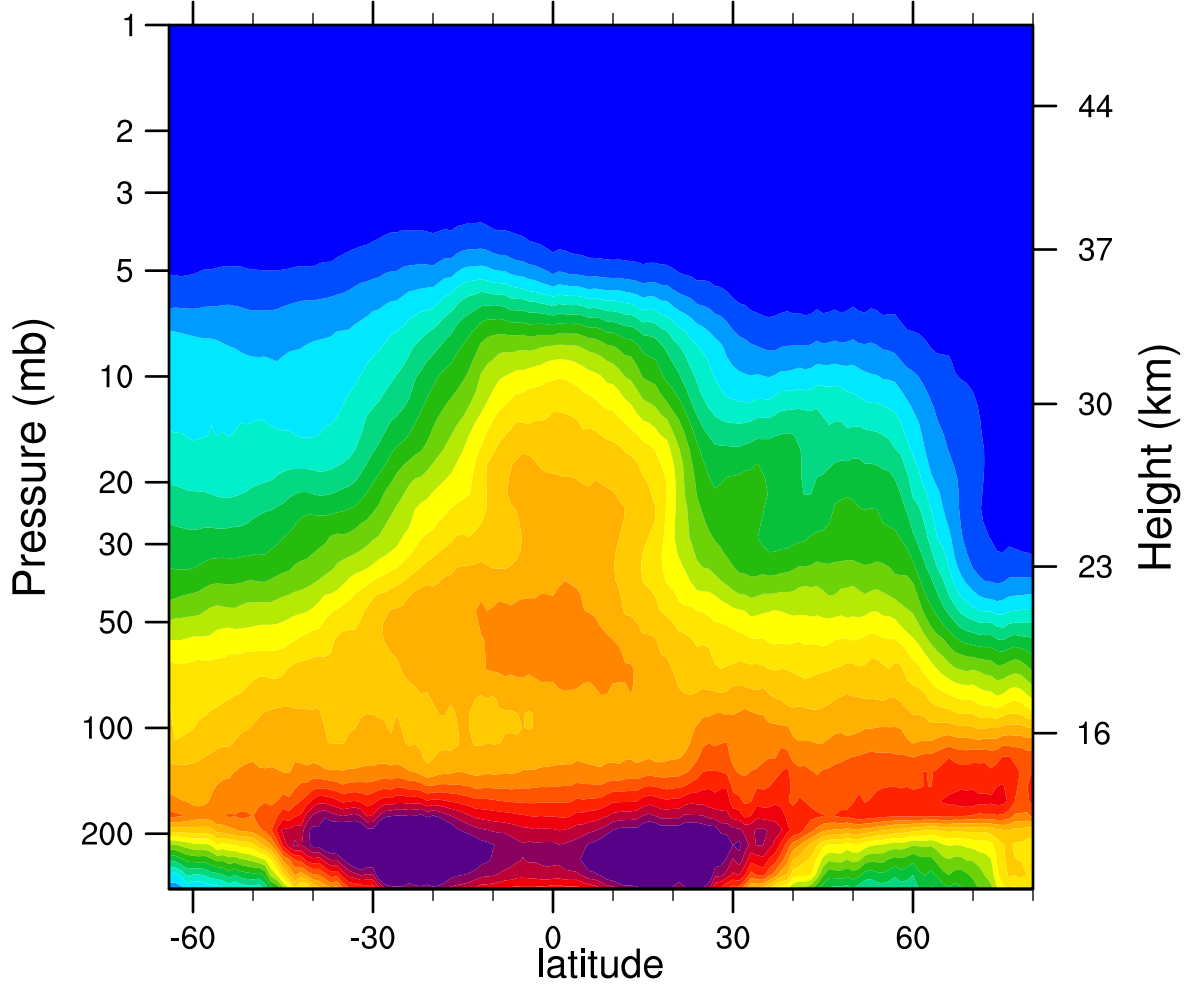
2007d012 N2O_Combined (ppbv)
