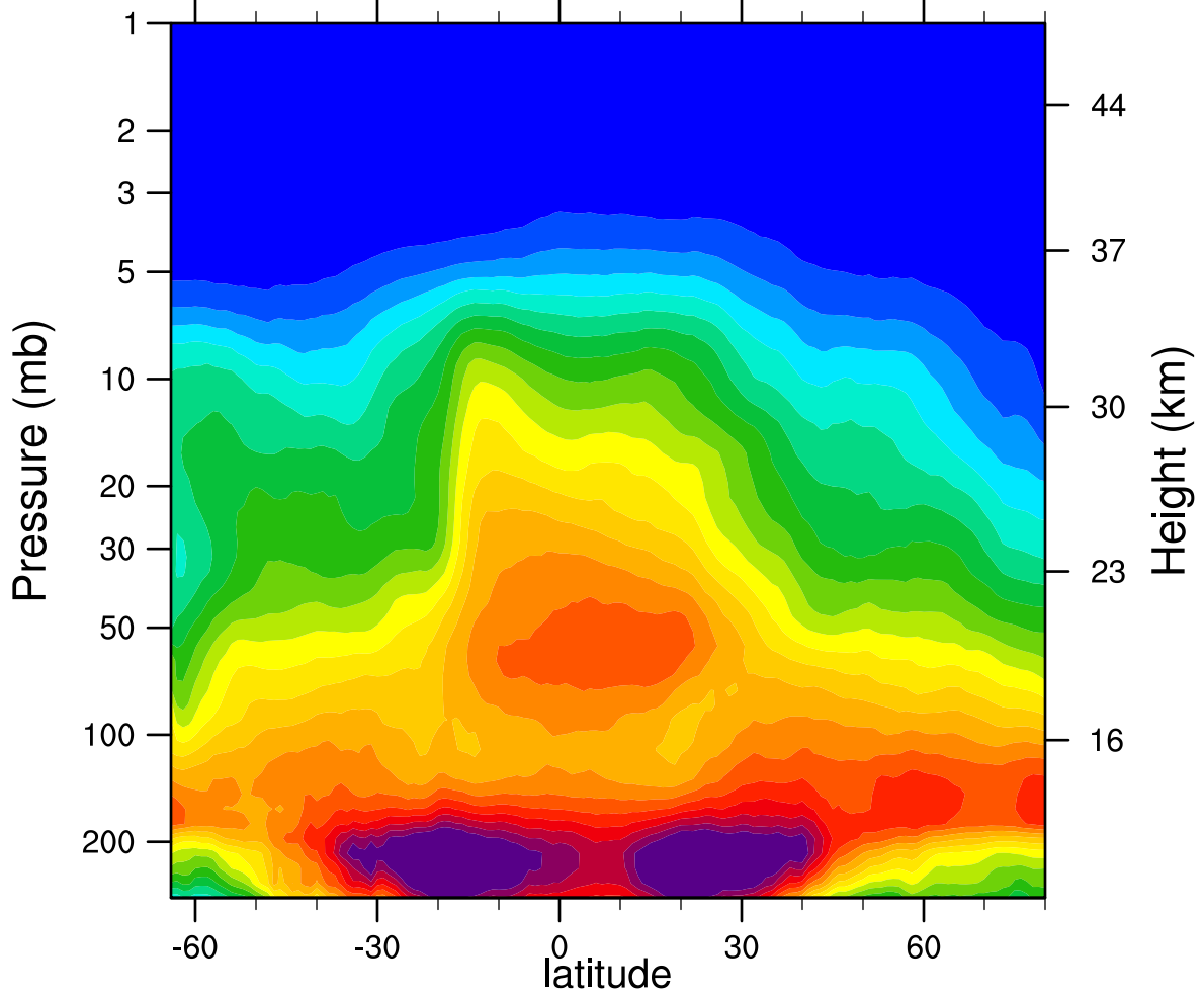
2005d306 N2O_Combined (ppbv)
