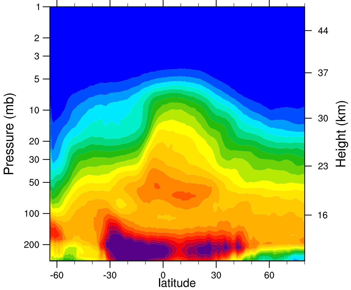
2006d232 N2O_Combined (ppbv)
