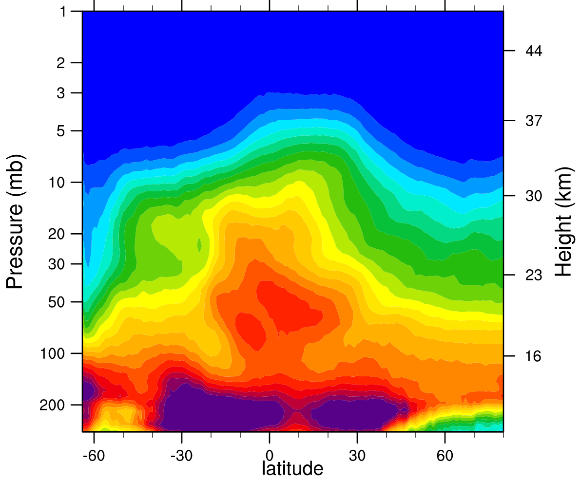
2007d239 N2O_Combined (ppbv)
