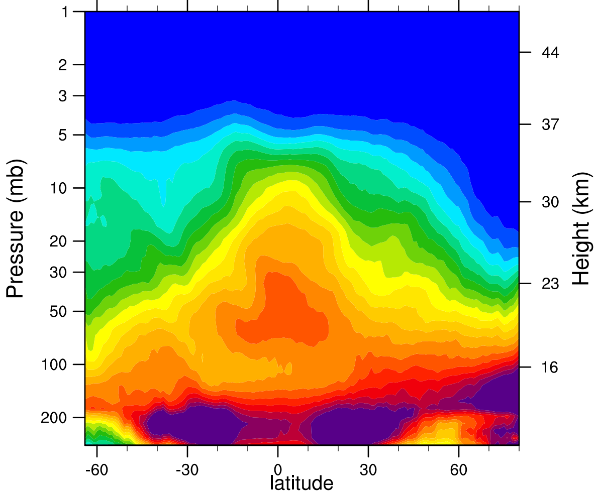
2006d342 N2O_Combined (ppbv)
