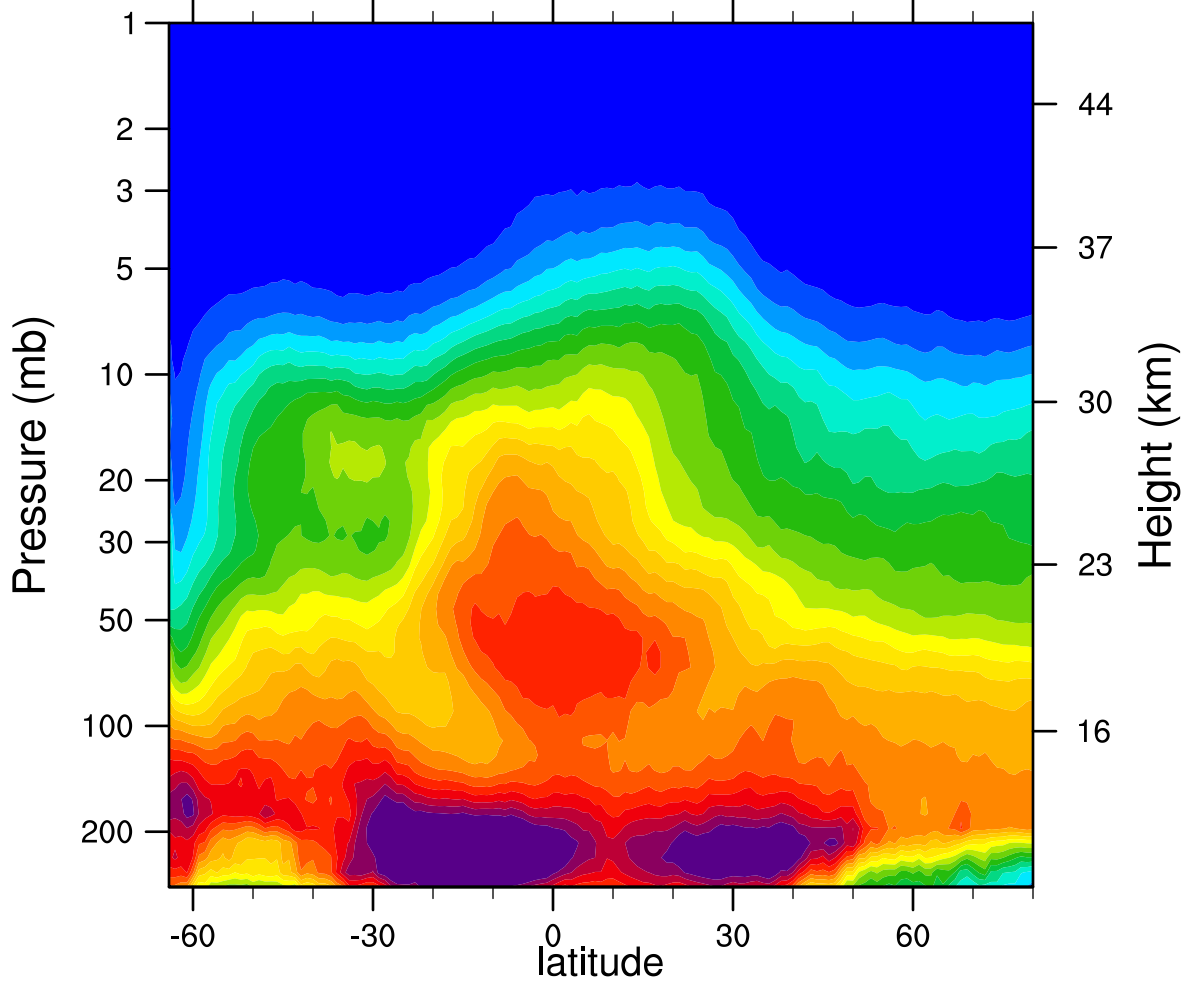
2007d214 N2O_Combined (ppbv)
