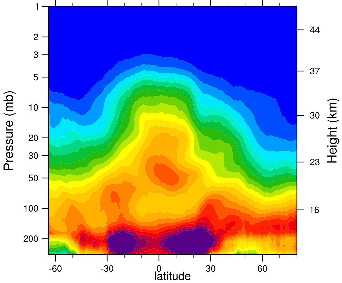
2005d056 N2O_Combined (ppbv)
