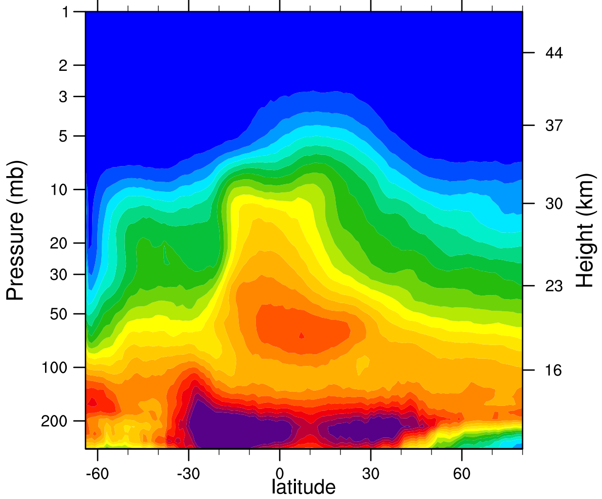
2005d231 N2O_Combined (ppbv)
