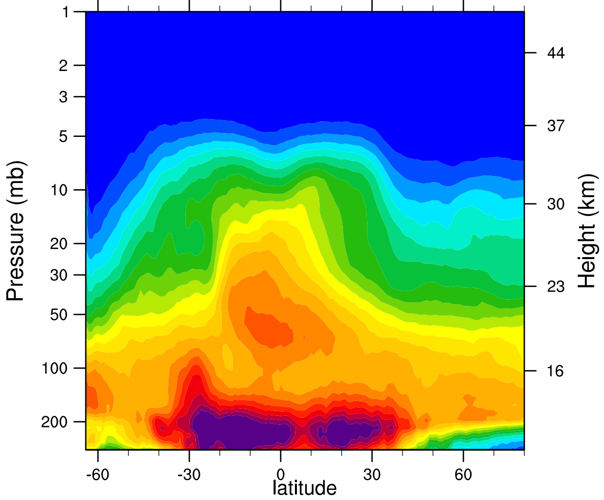
2007d168 N2O_Combined (ppbv)
