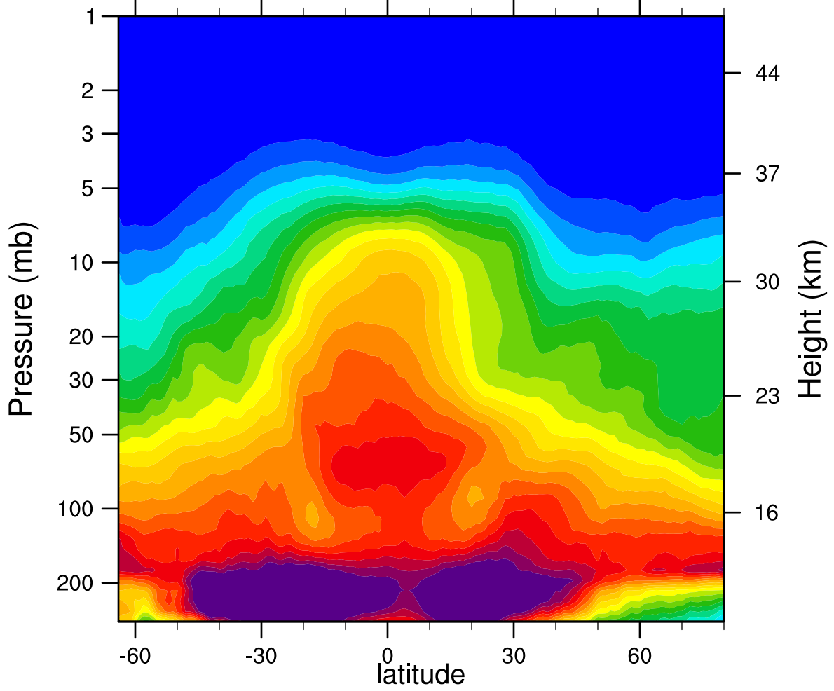
2007d115 N2O_Combined (ppbv)
