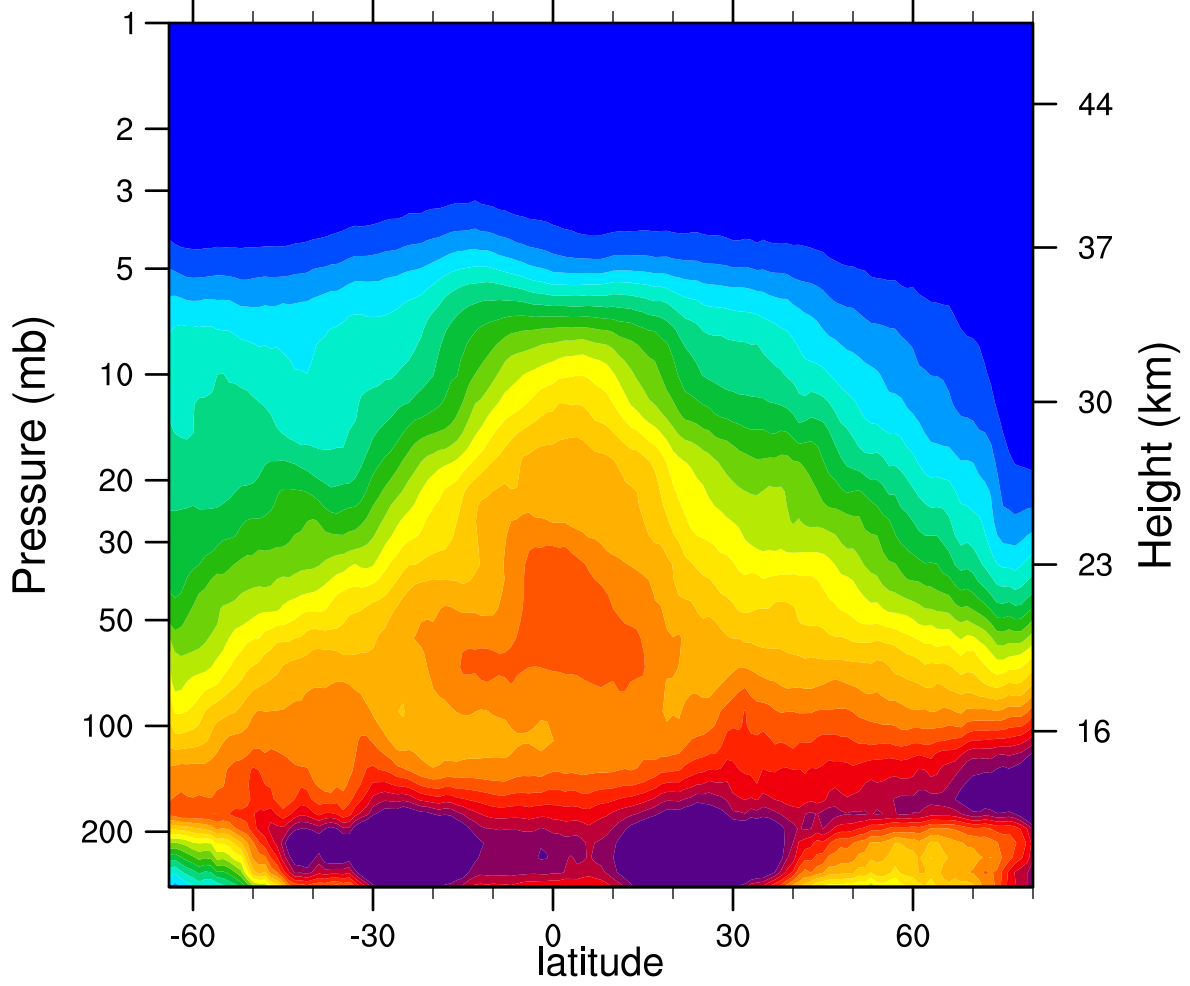
2006d348 N2O_Combined (ppbv)
