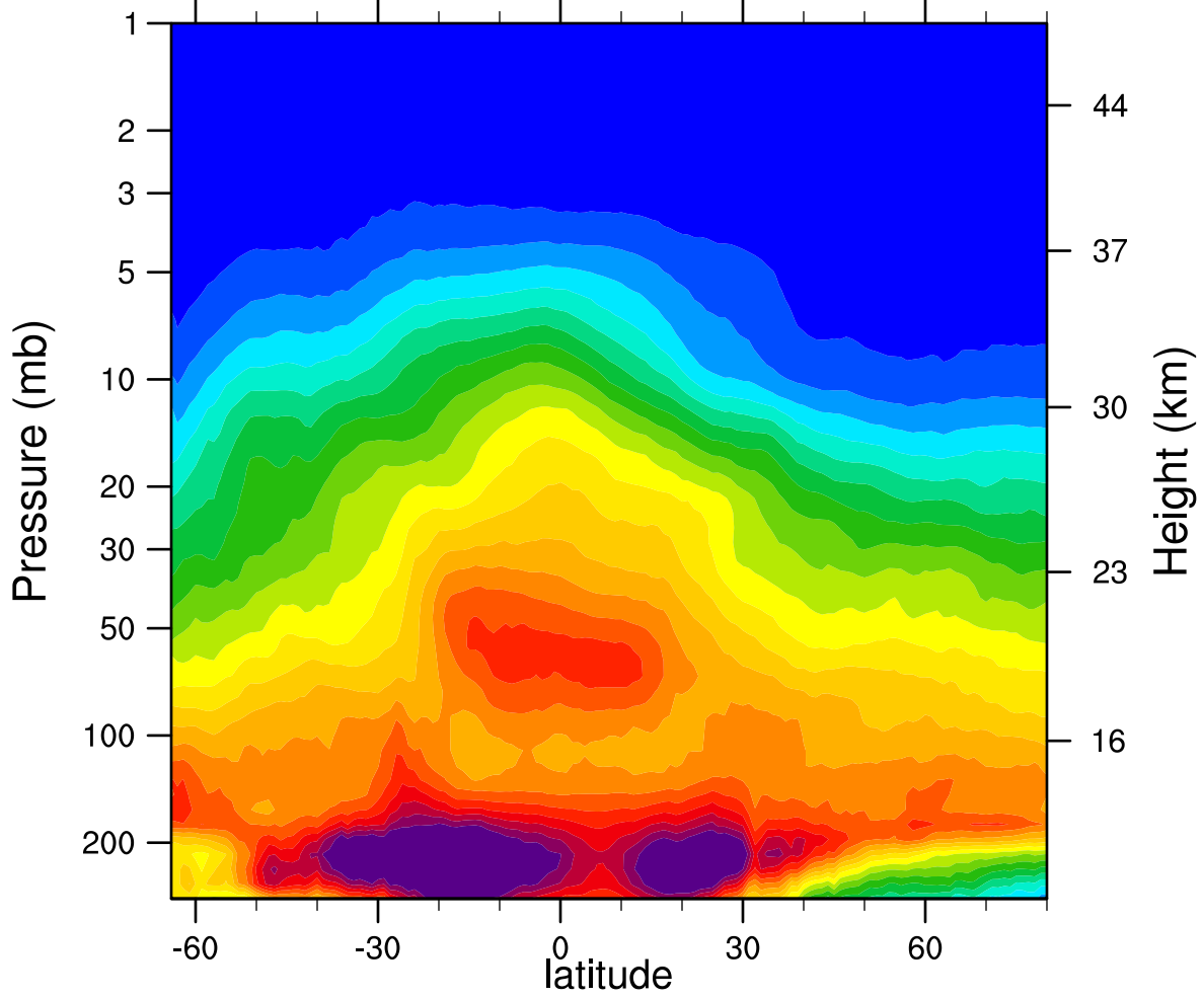
2006d134 N2O_Combined (ppbv)
