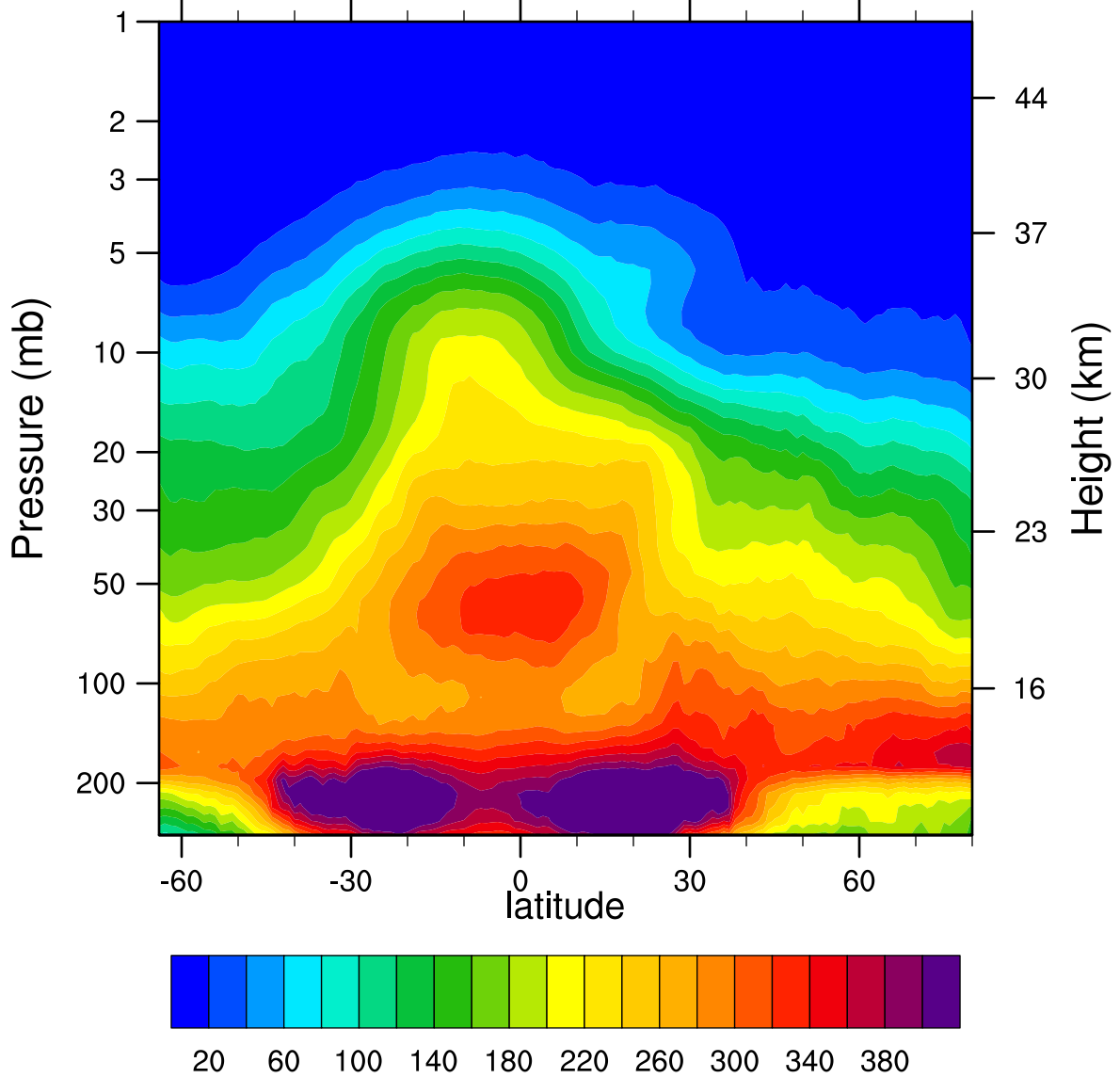
2006d062 N2O_Combined (ppbv)
