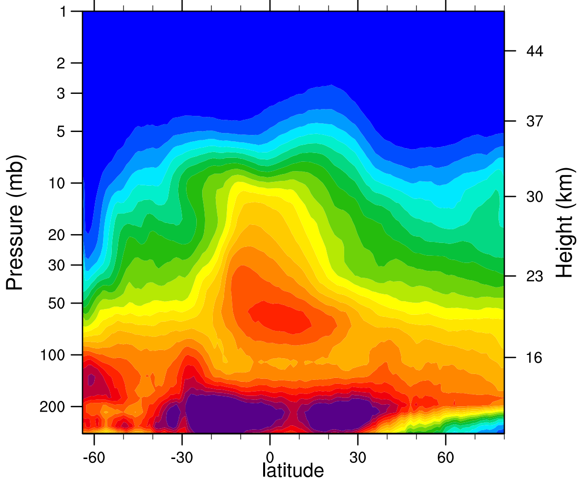
2005d173 N2O_Combined (ppbv)
