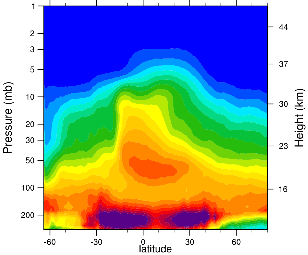
2005d251 N2O_Combined (ppbv)
