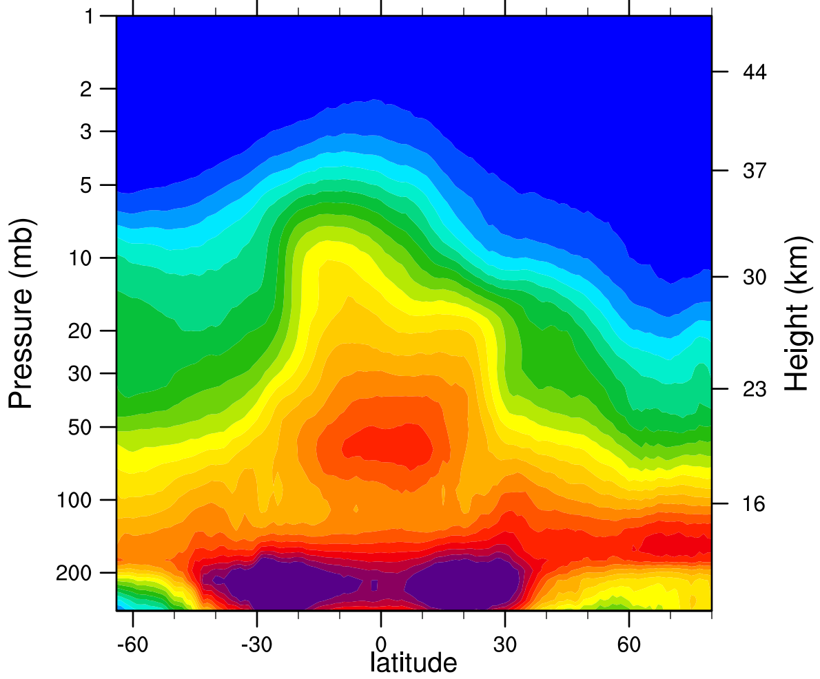
2006d008 N2O_Combined (ppbv)
