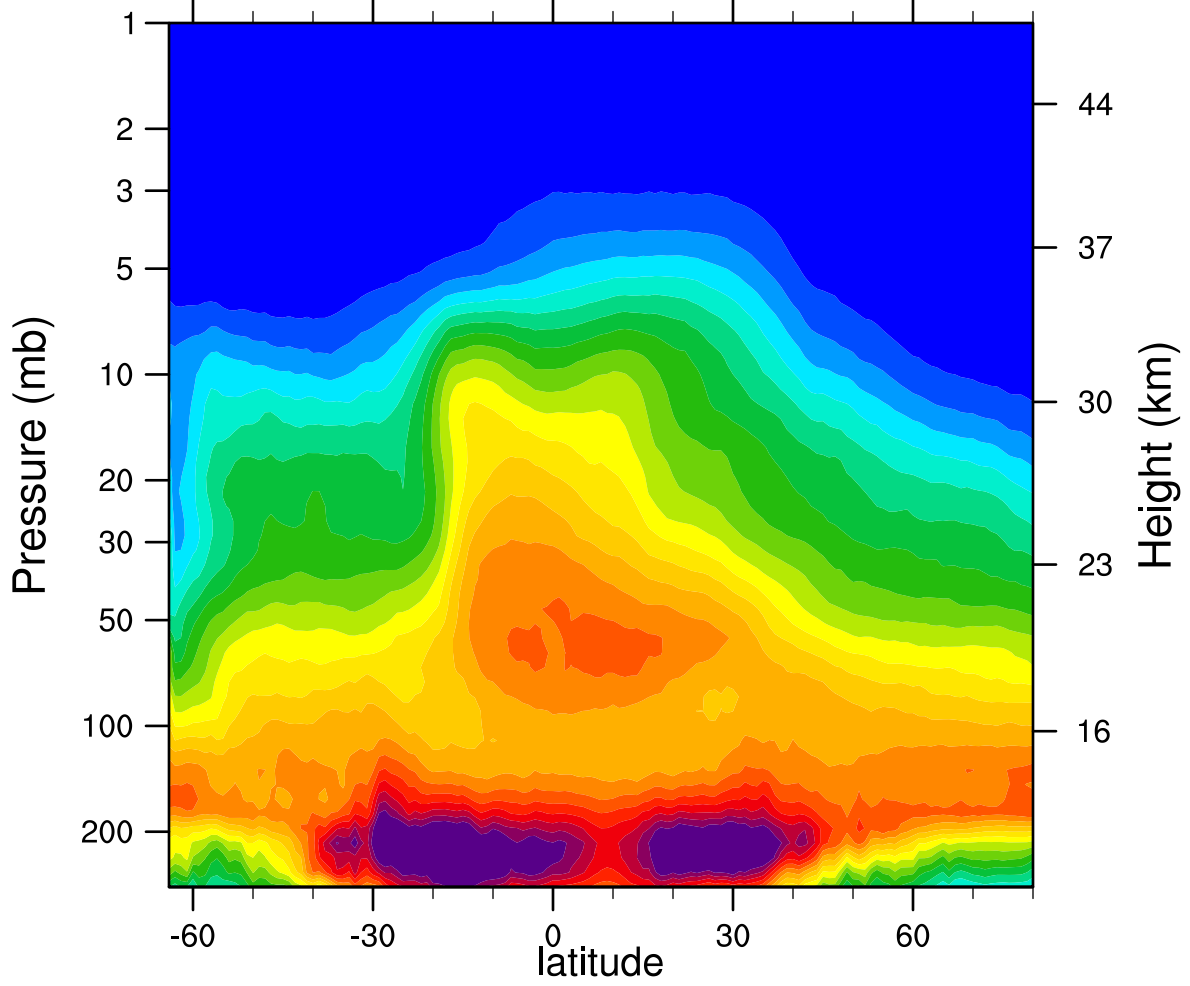
2005d274 N2O_Combined (ppbv)
