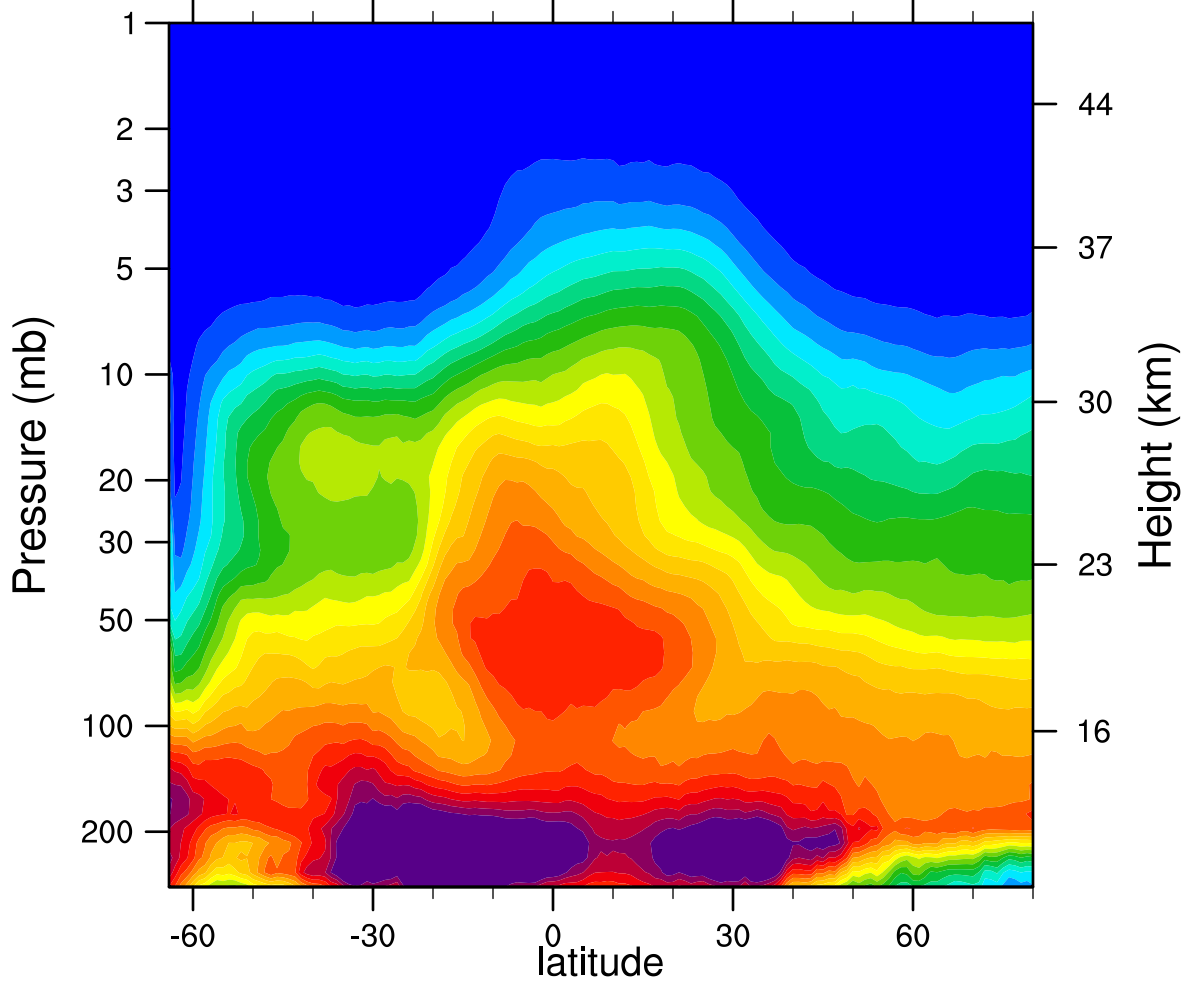
2007d228 N2O_Combined (ppbv)
