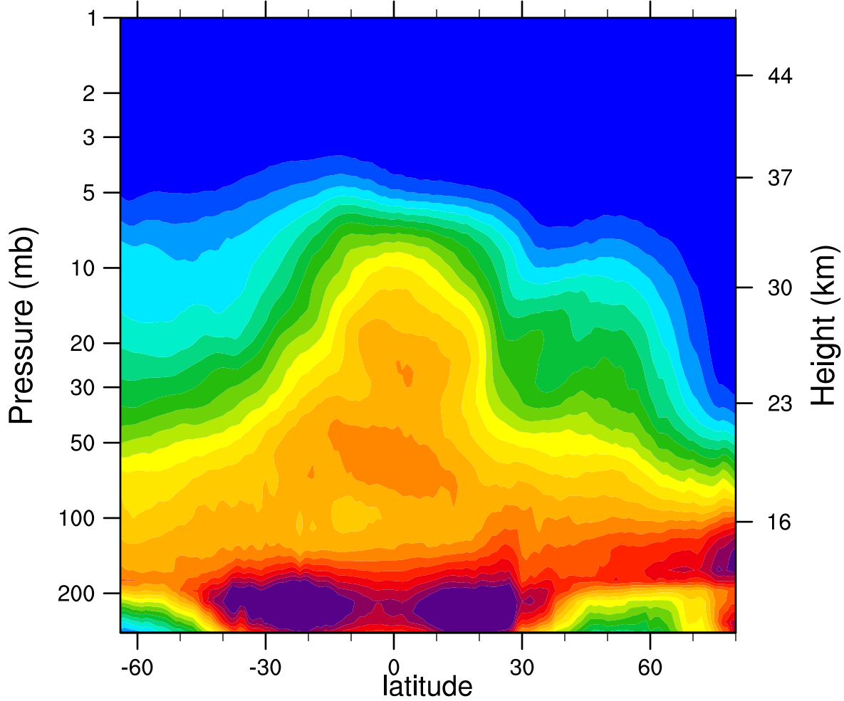
2007d017 N2O_Combined (ppbv)
