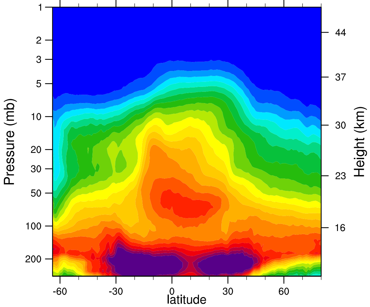
2007d268 N2O_Combined (ppbv)
