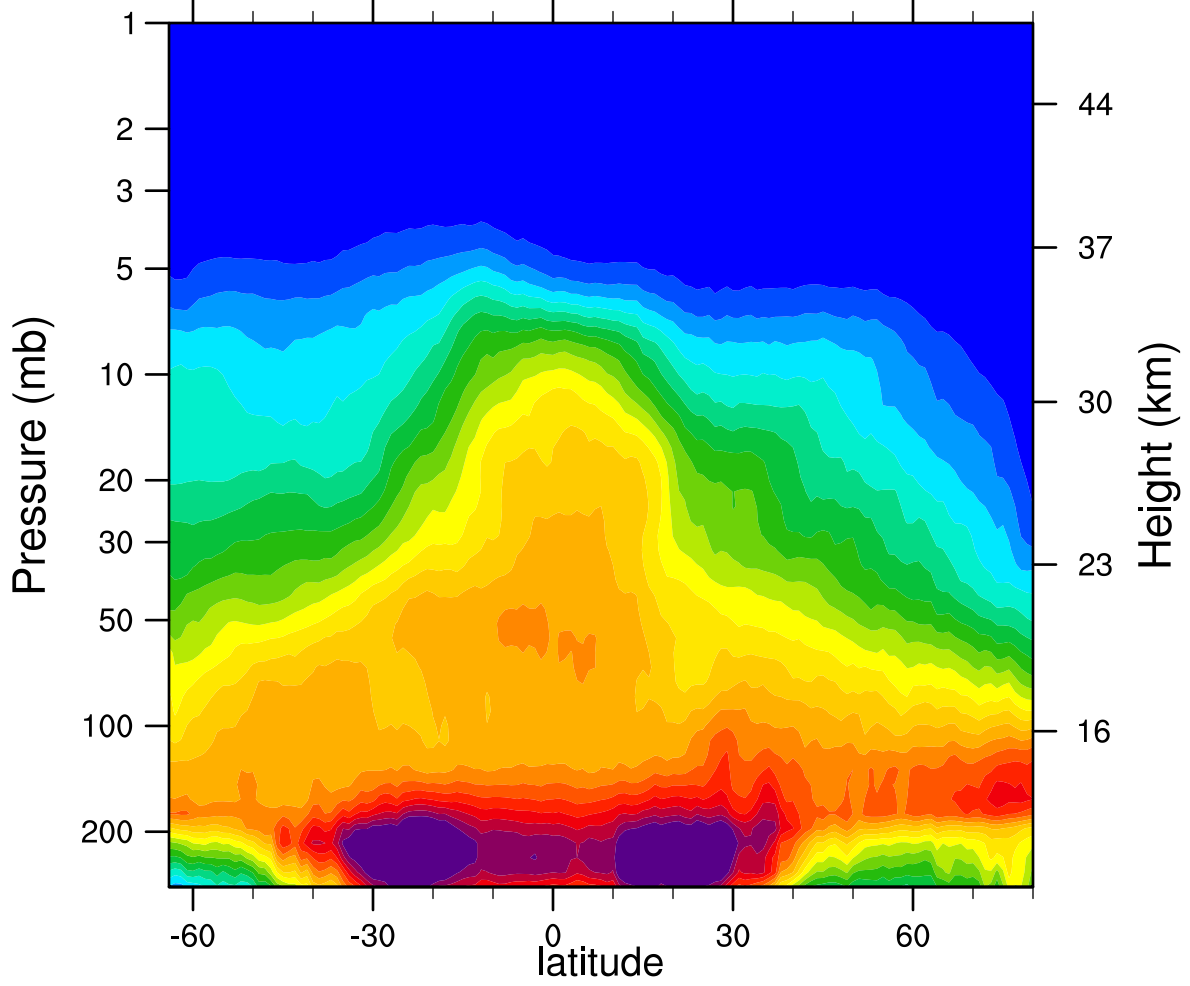
2006d361 N2O_Combined (ppbv)
