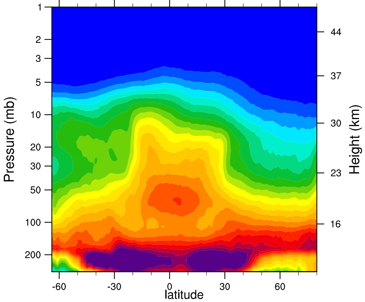
2007d330 N2O_Combined (ppbv)
