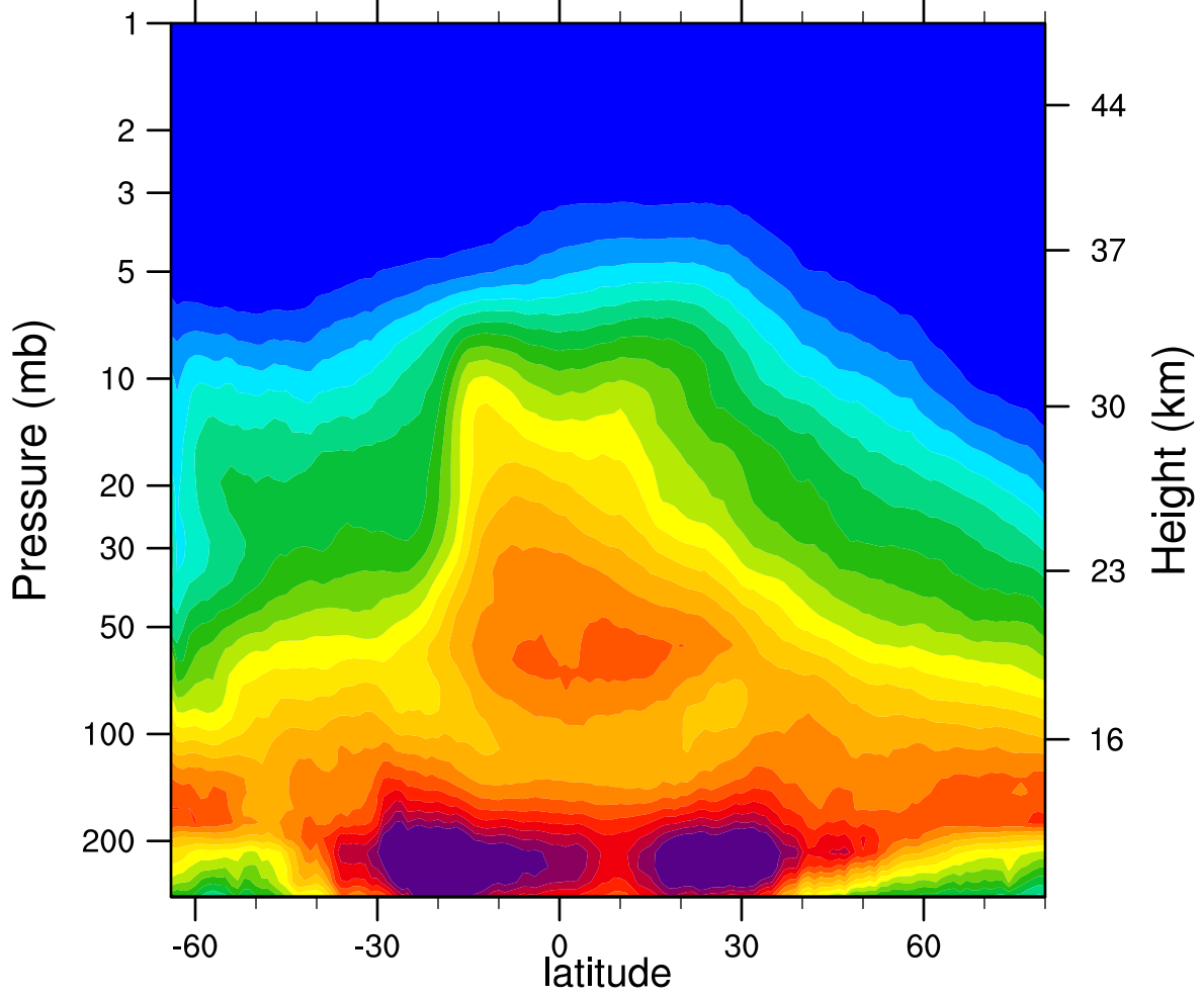
2005d284 N2O_Combined (ppbv)
