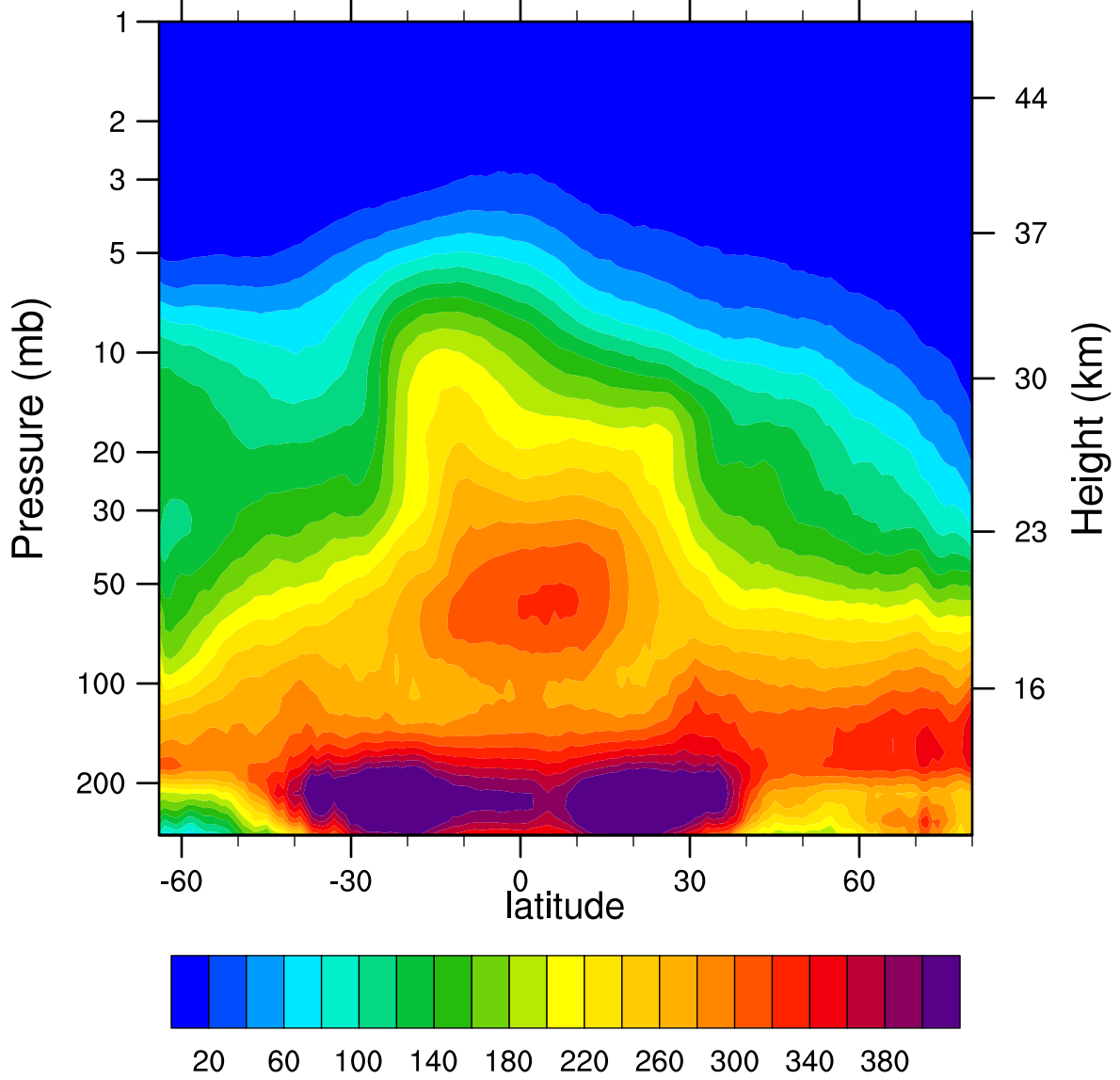
2005d342 N2O_Combined (ppbv)
