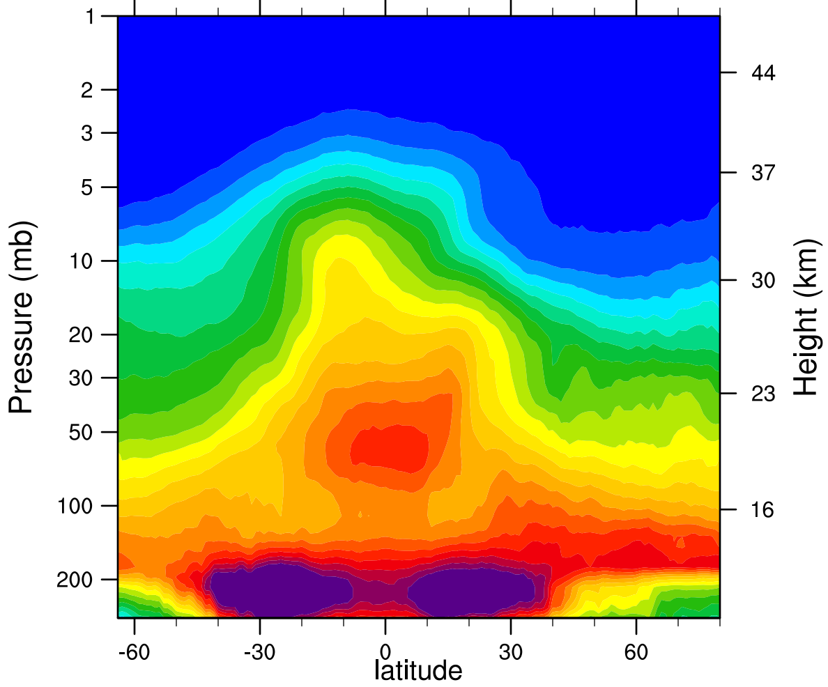
2006d041 N2O_Combined (ppbv)
