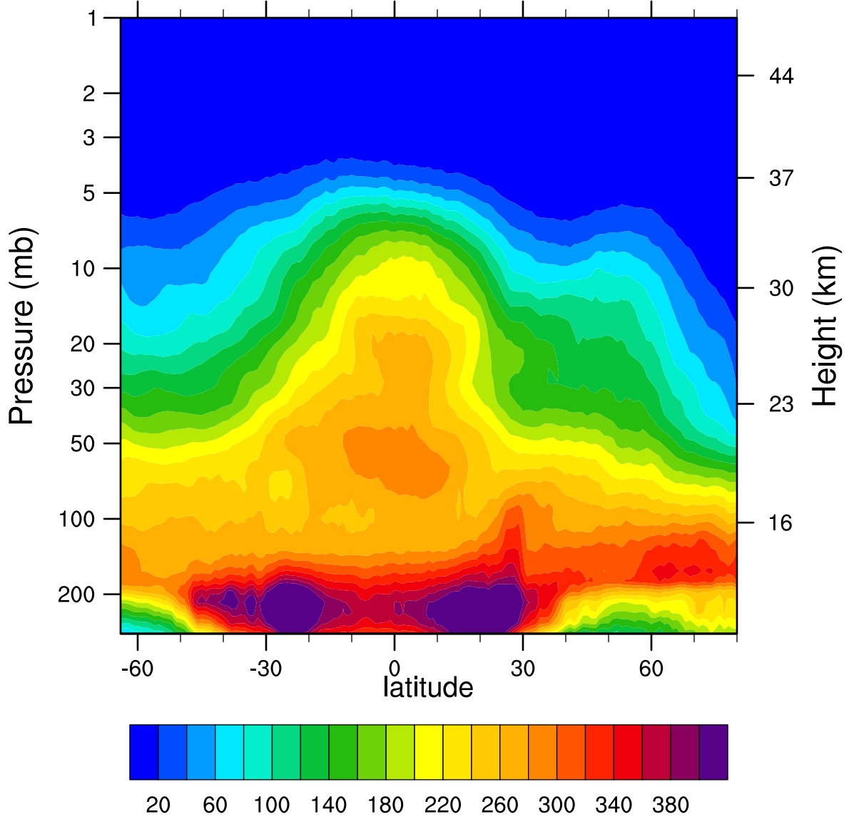
2007d049 N2O_Combined (ppbv)
