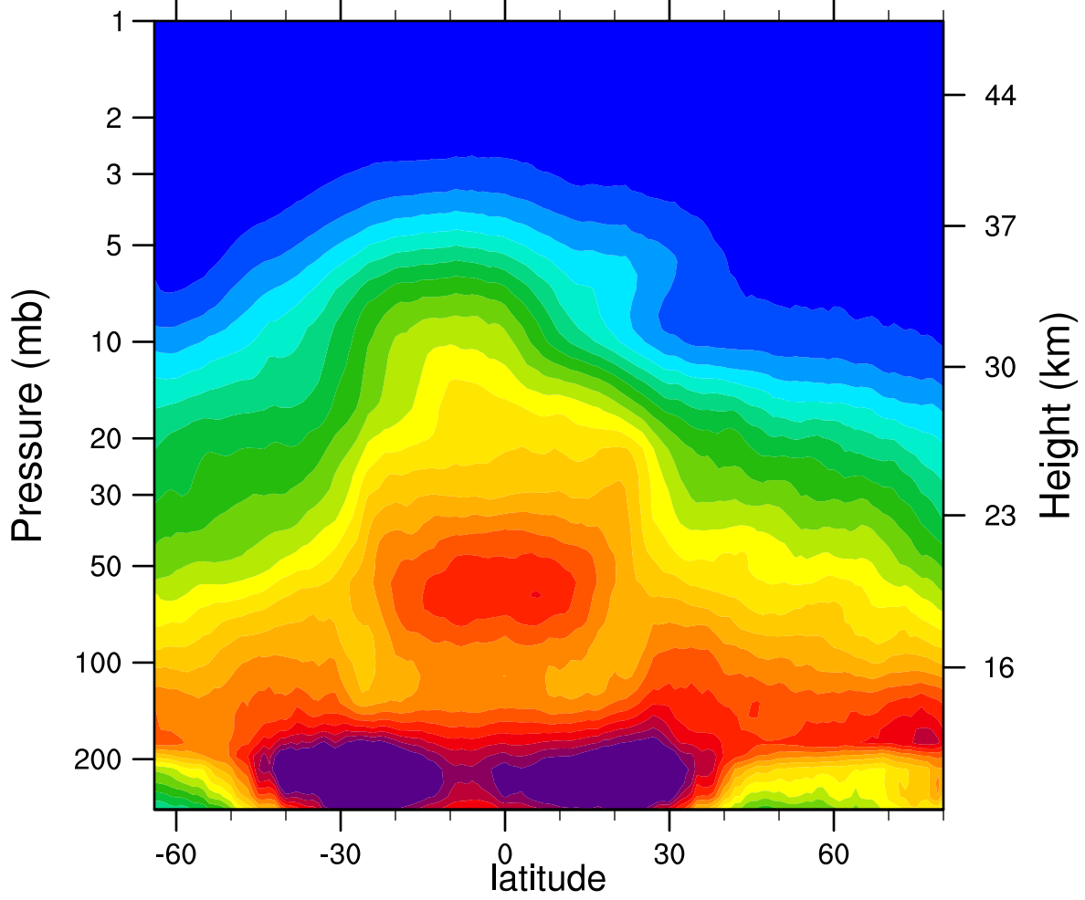
2006d076 N2O_Combined (ppbv)
