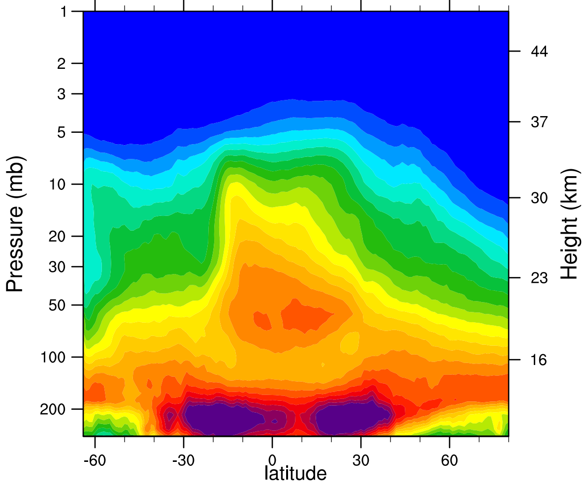
2005d289 N2O_Combined (ppbv)
