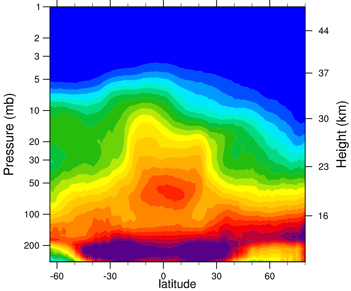
2007d348 N2O_Combined (ppbv)
