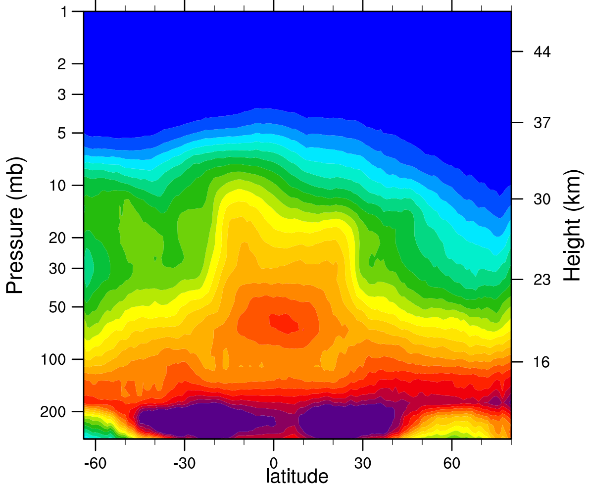
2007d336 N2O_Combined (ppbv)
