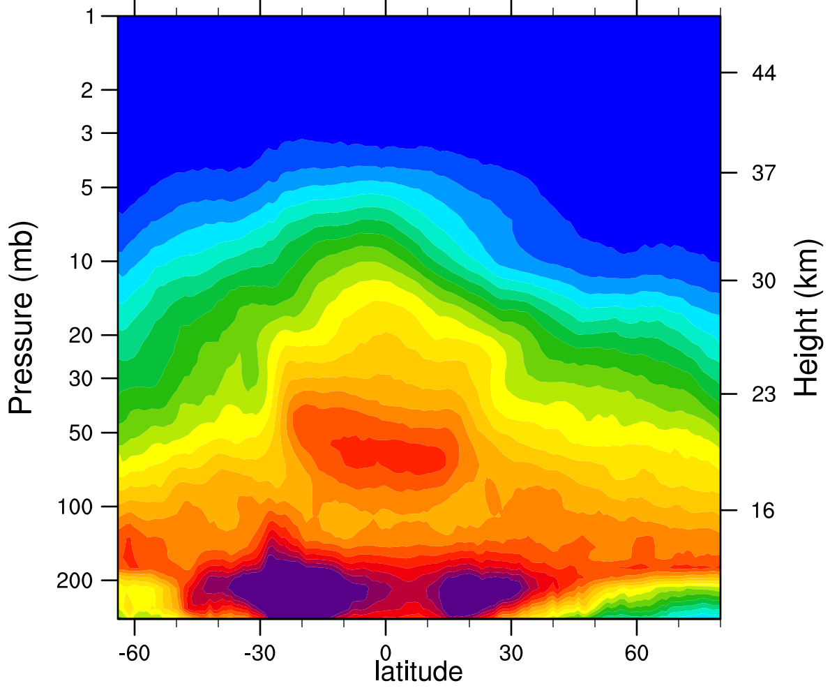
2006d123 N2O_Combined (ppbv)
