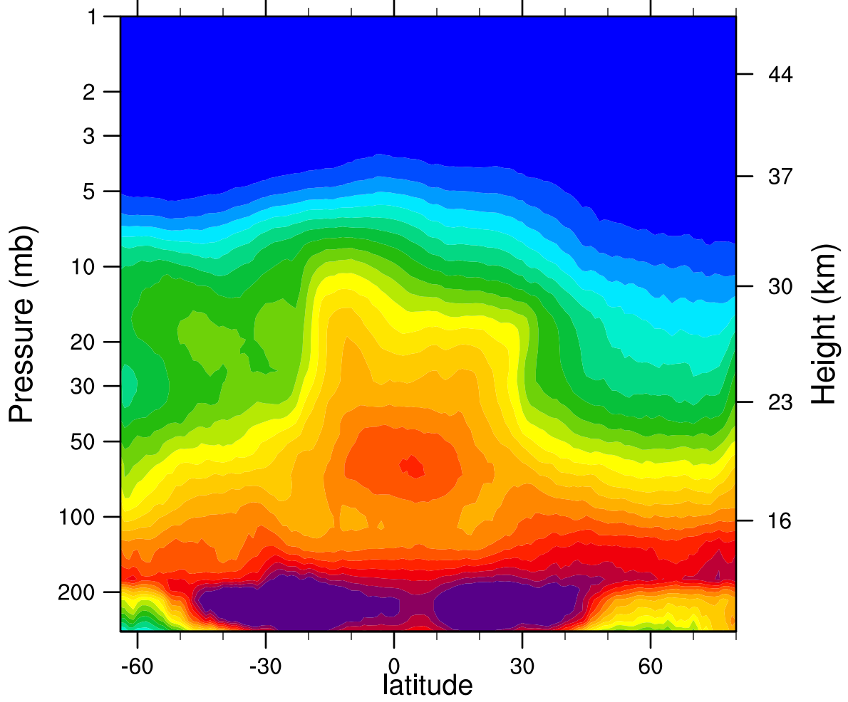
2007d331 N2O_Combined (ppbv)
