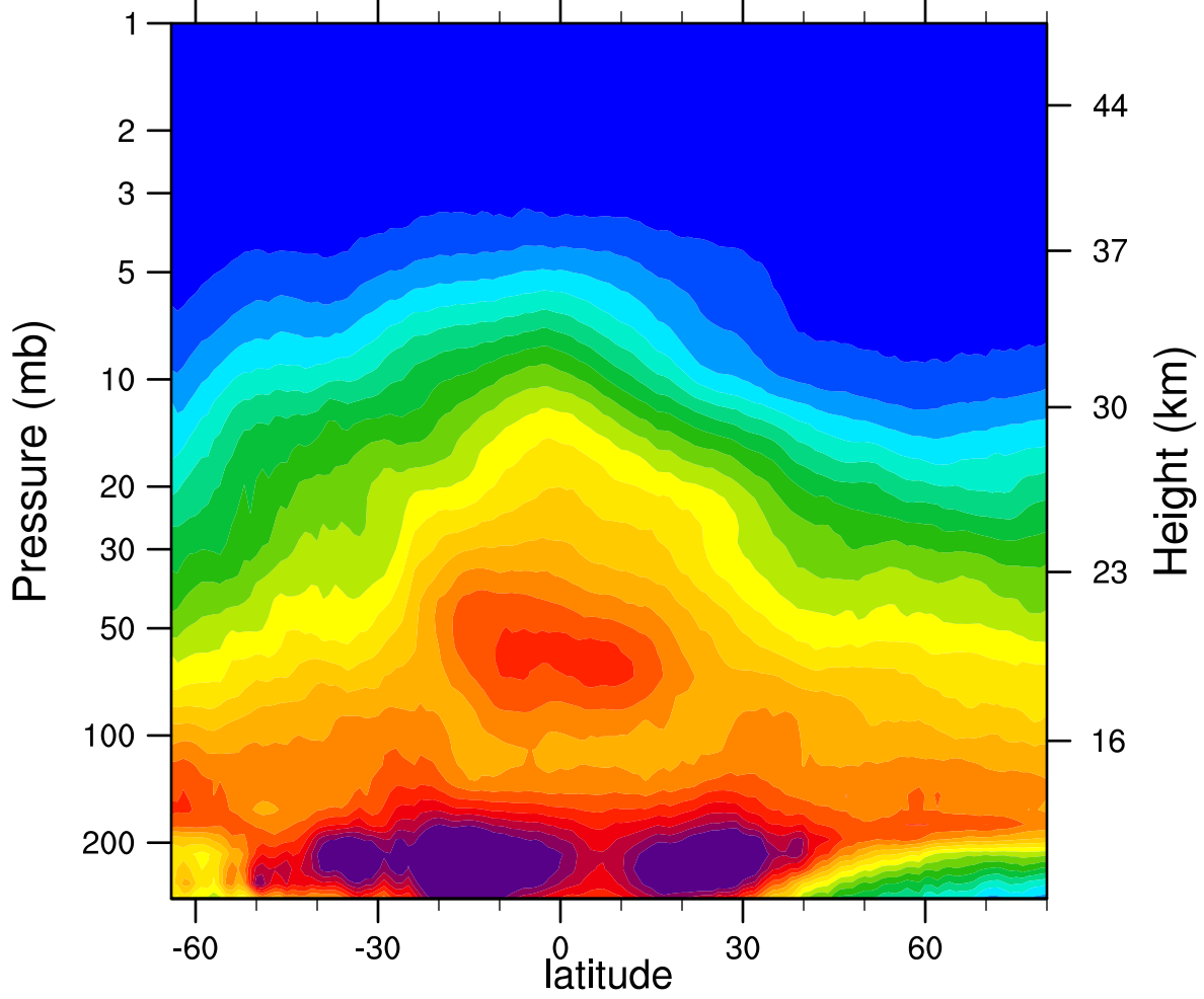
2006d137 N2O_Combined (ppbv)
