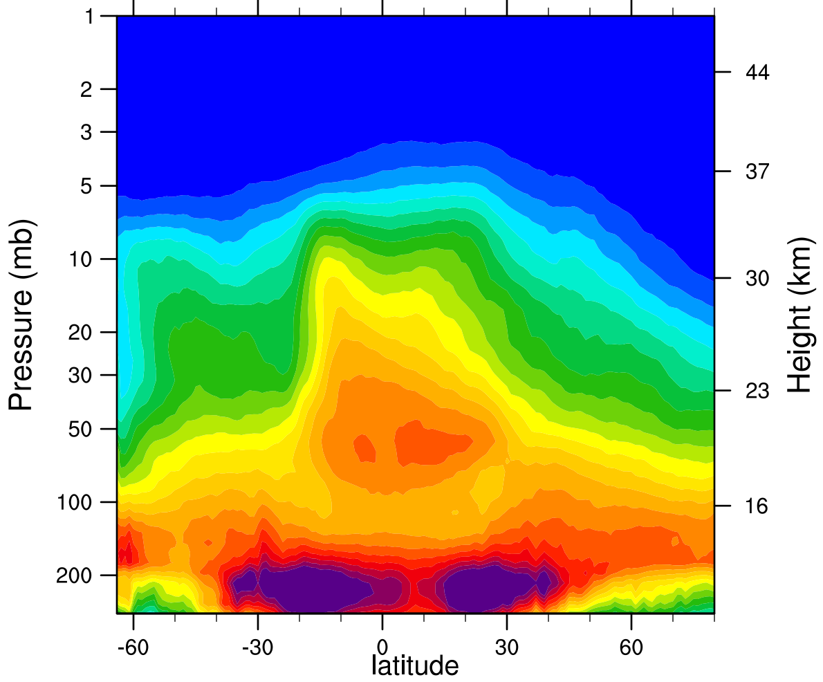
2005d292 N2O_Combined (ppbv)
