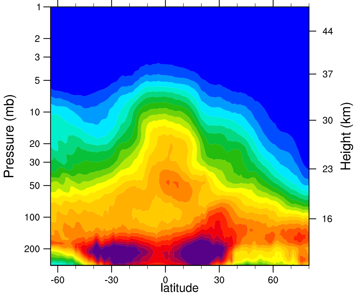
2005d031 N2O_Combined (ppbv)
