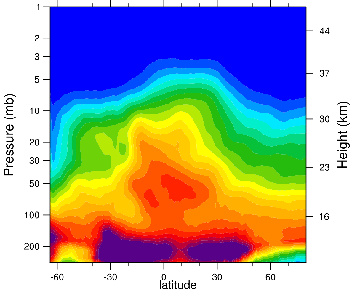
2007d246 N2O_Combined (ppbv)
