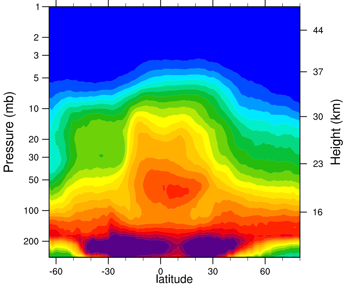
2007d290 N2O_Combined (ppbv)
