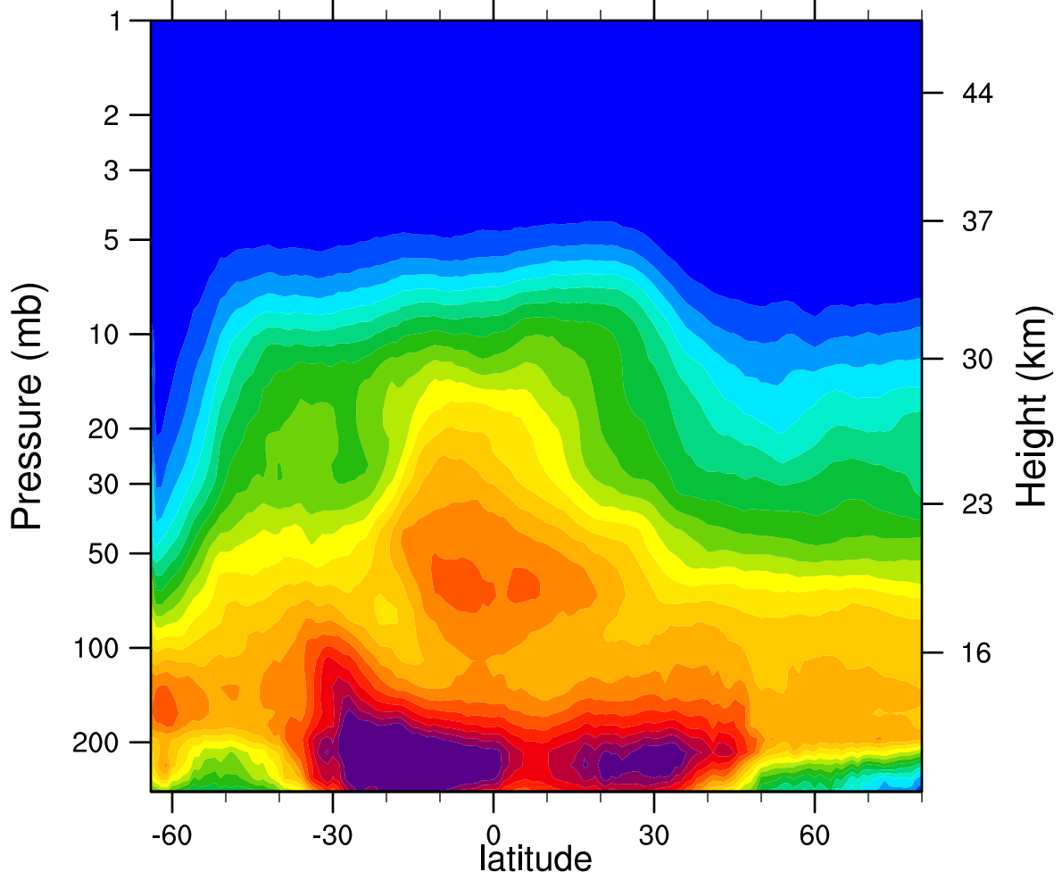
2007d202 N2O_Combined (ppbv)
