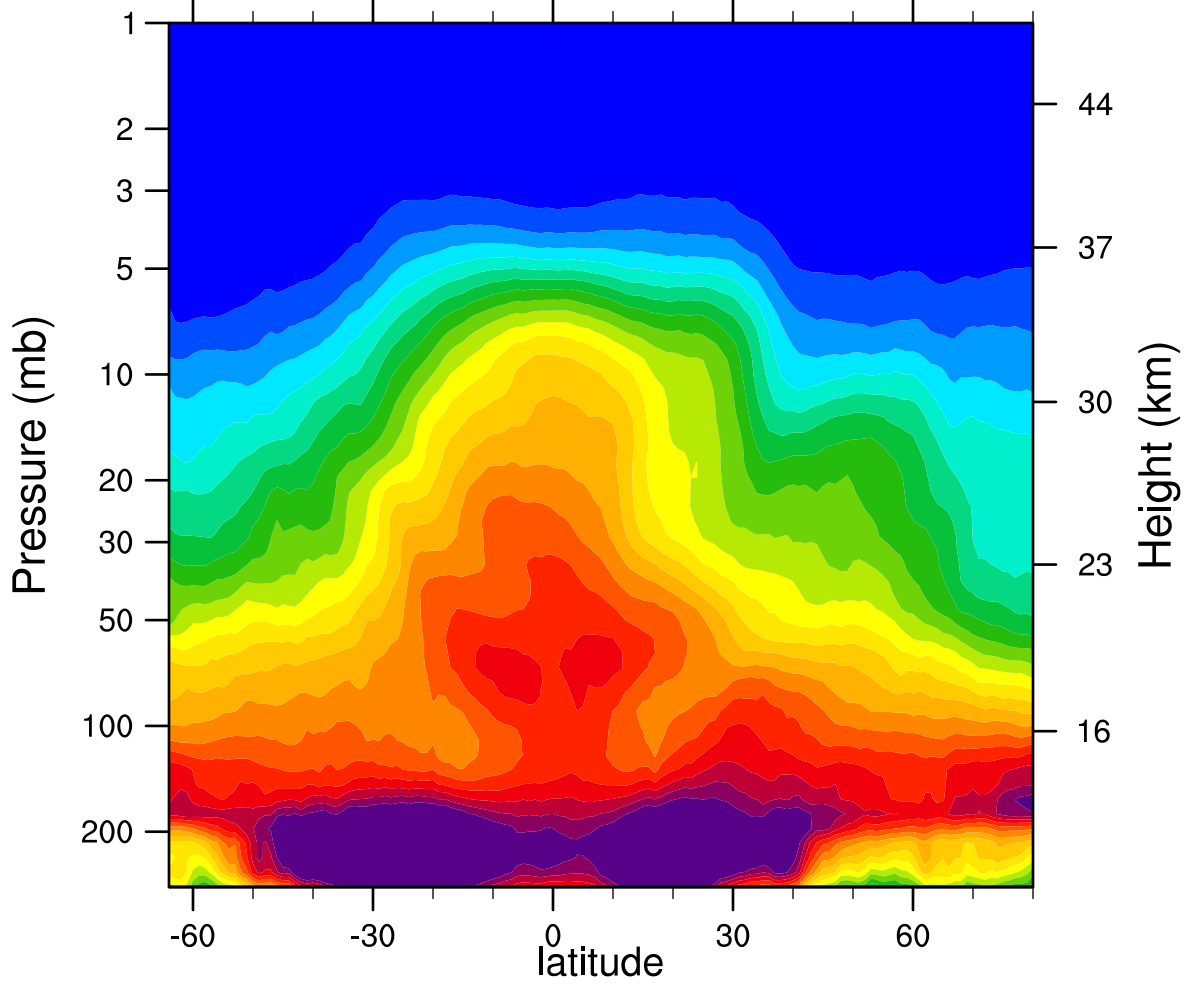
2007d100 N2O_Combined (ppbv)
