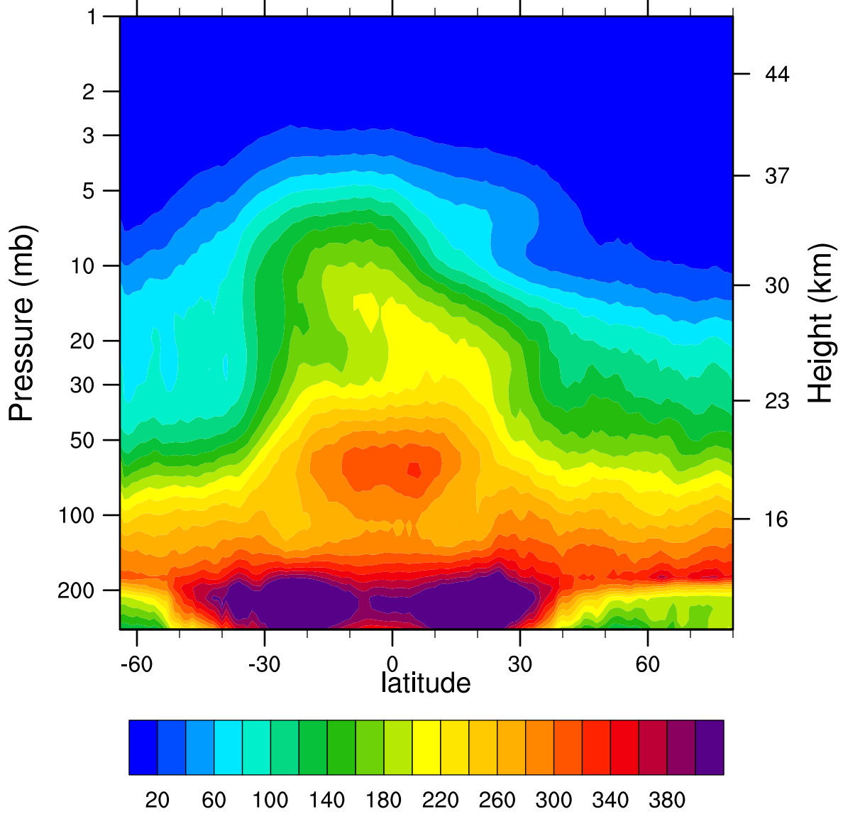
2006d089 N2O_Combined (ppbv)
