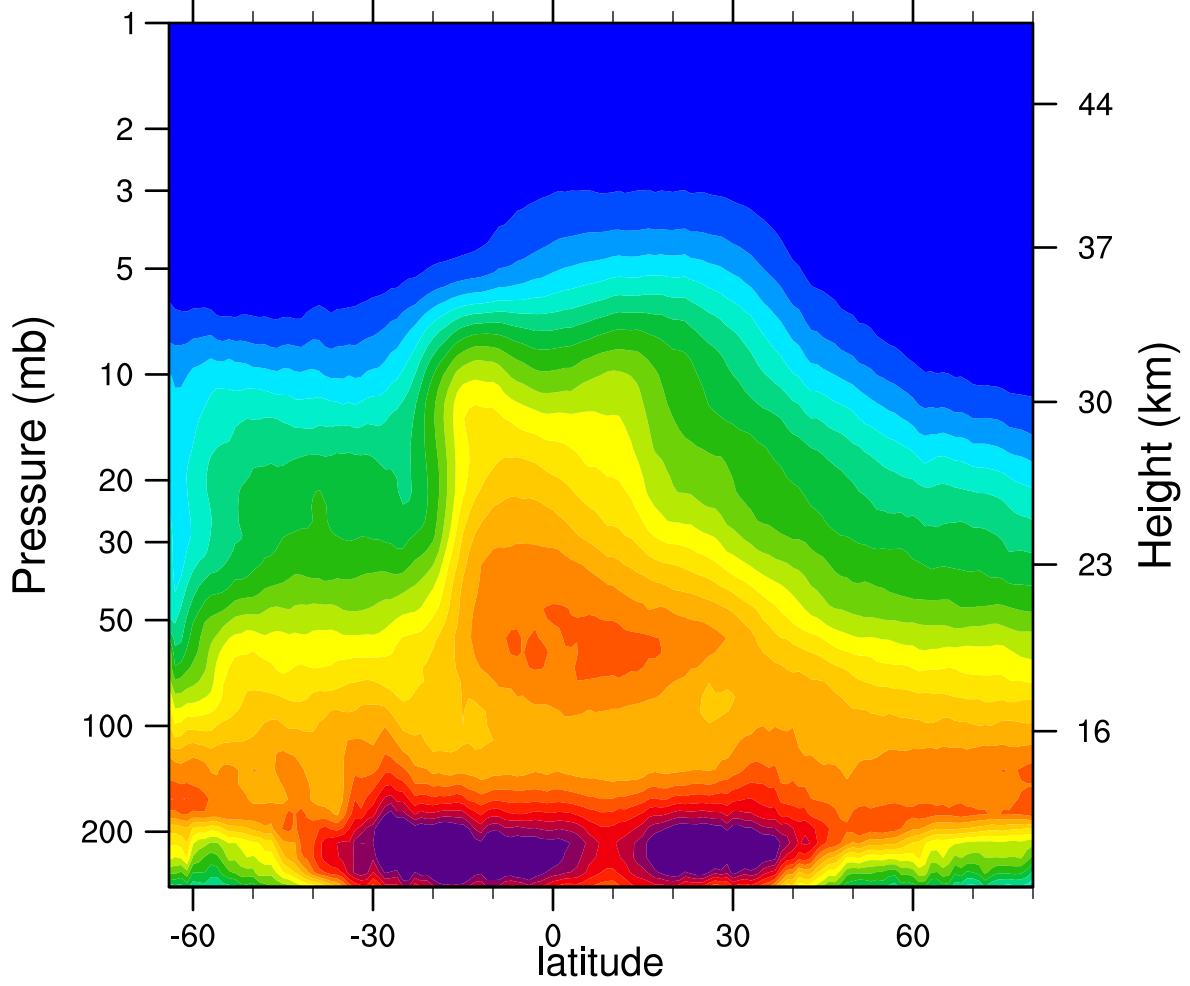
2005d272 N2O_Combined (ppbv)
