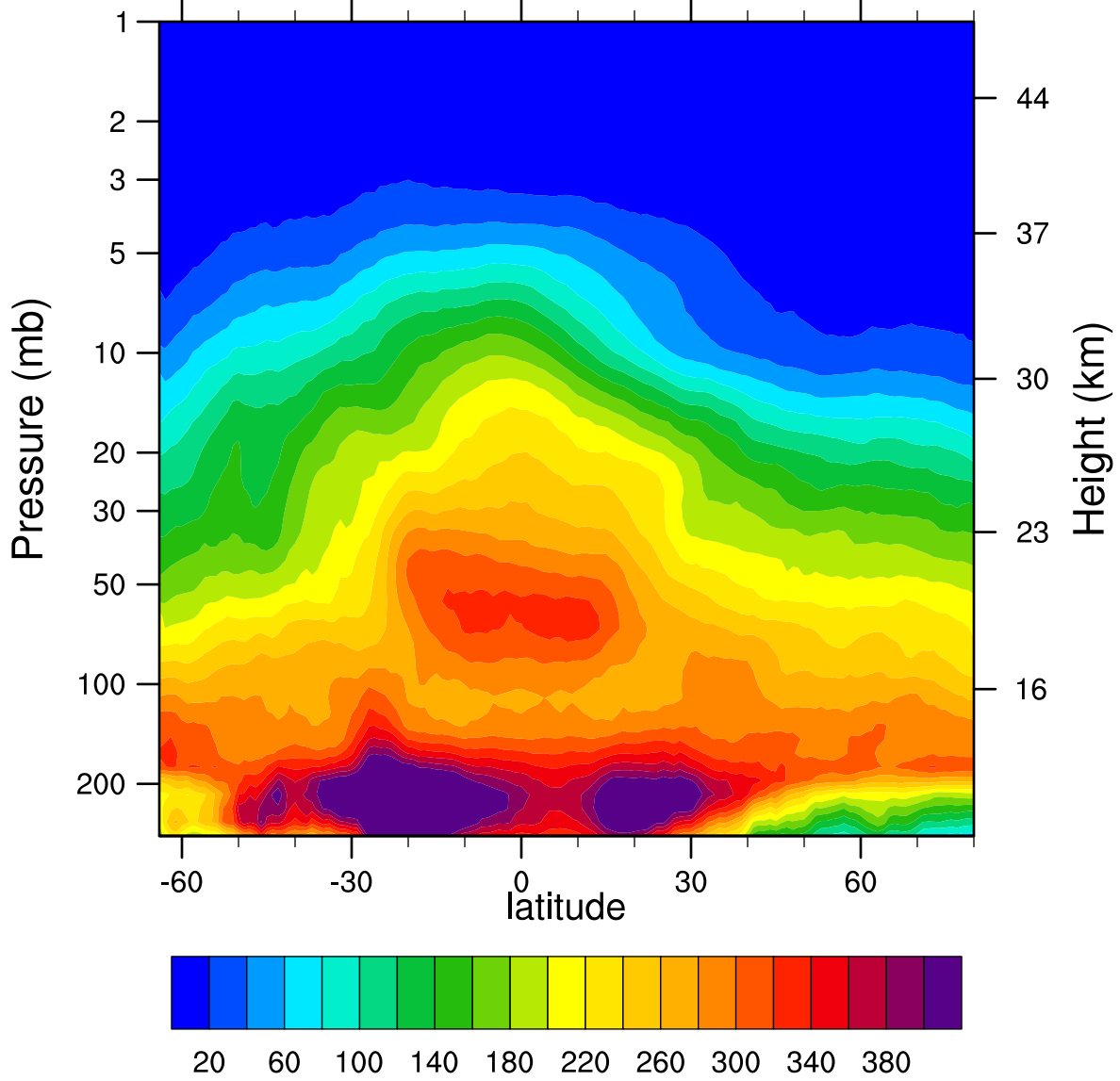
2006d128 N2O_Combined (ppbv)
