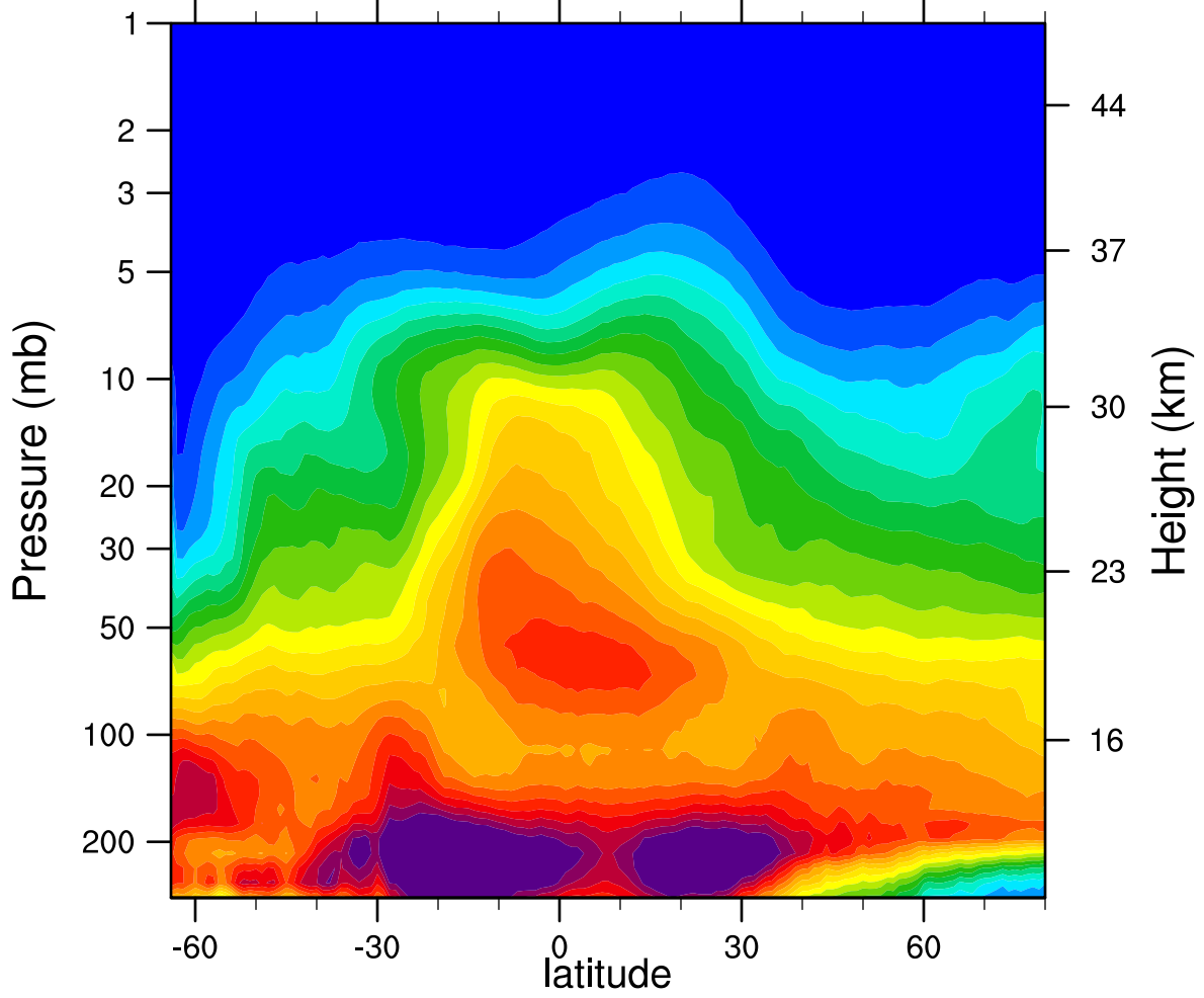
2005d170 N2O_Combined (ppbv)
