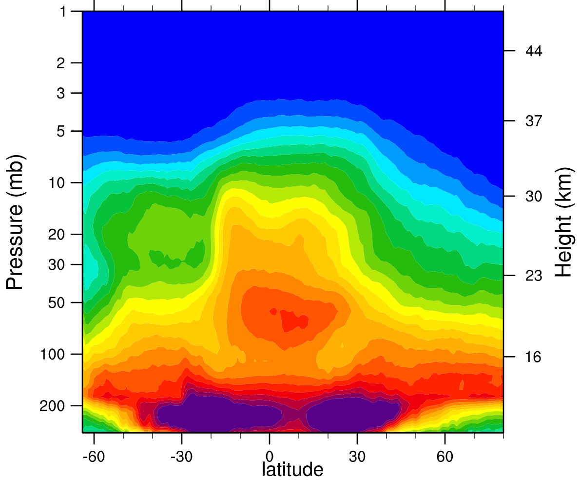
2007d294 N2O_Combined (ppbv)
