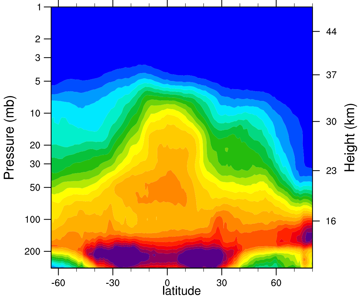
2007d005 N2O_Combined (ppbv)
