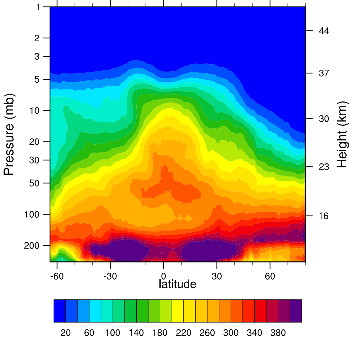
2006d331 N2O_Combined (ppbv)
