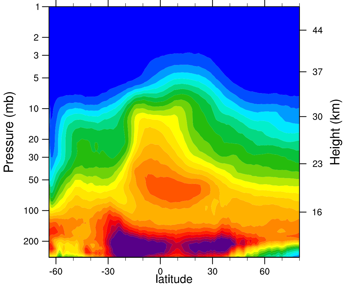
2005d235 N2O_Combined (ppbv)
