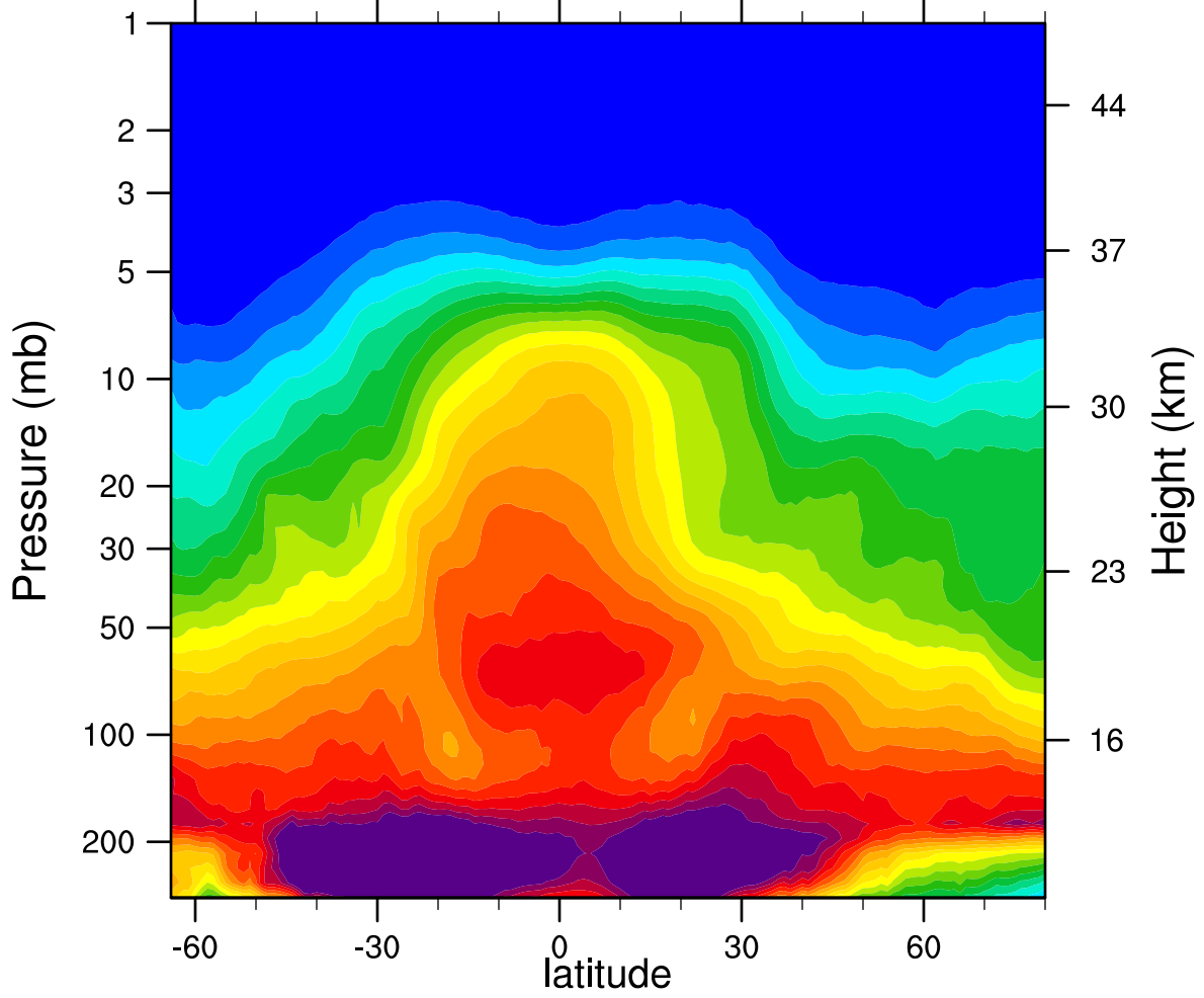
2007d114 N2O_Combined (ppbv)
