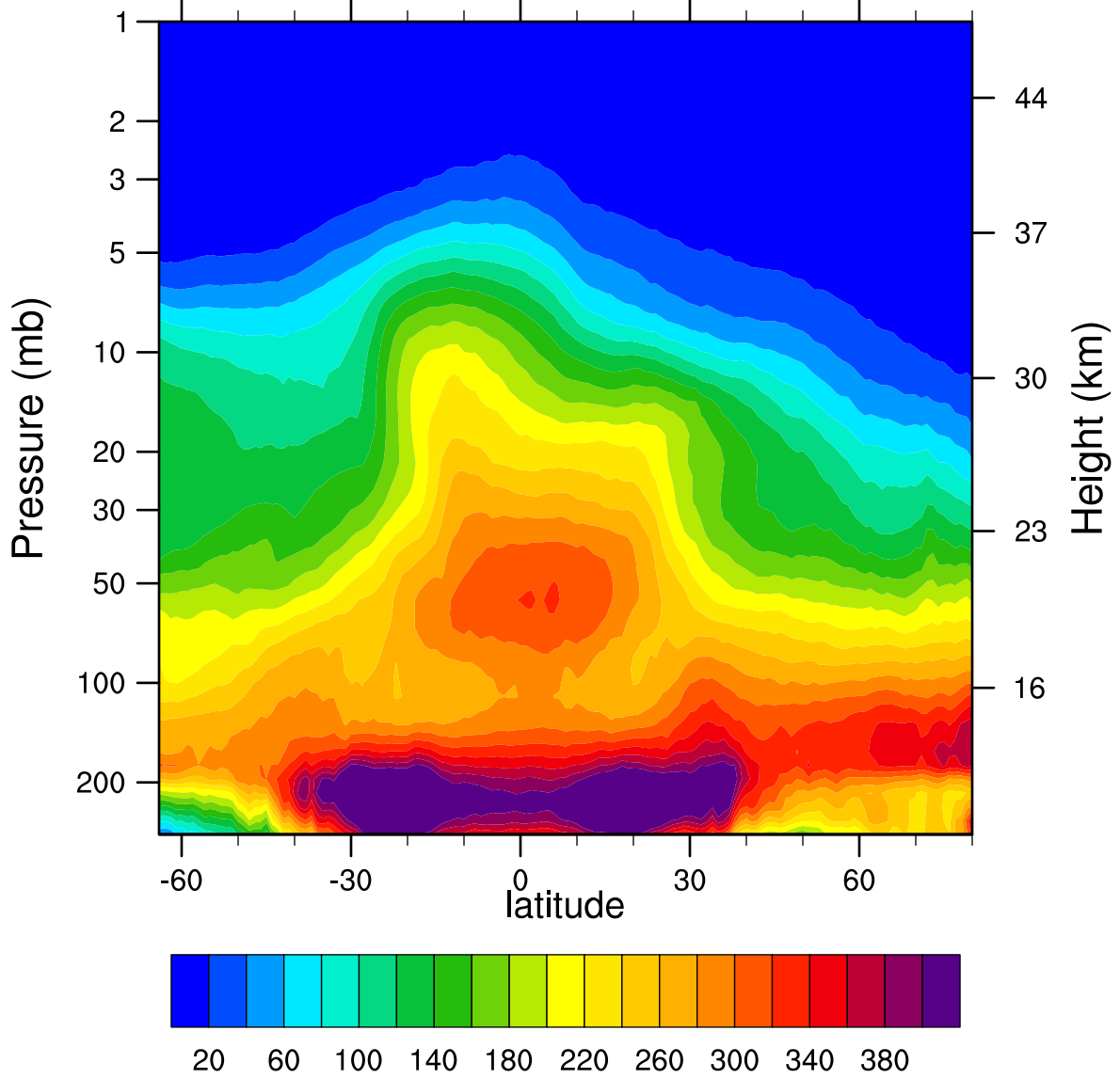
2005d351 N2O_Combined (ppbv)
