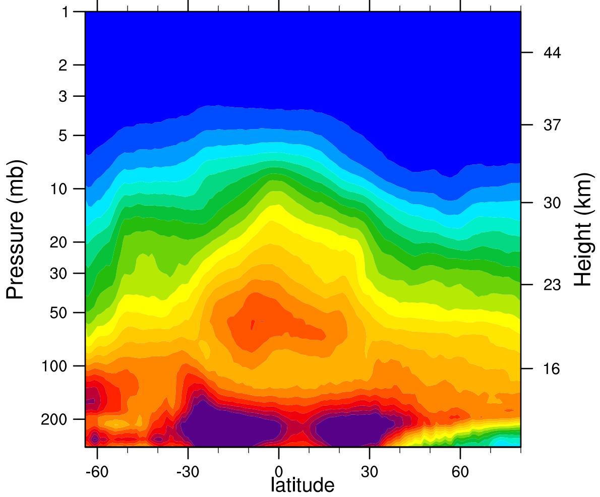
2006d162 N2O_Combined (ppbv)
