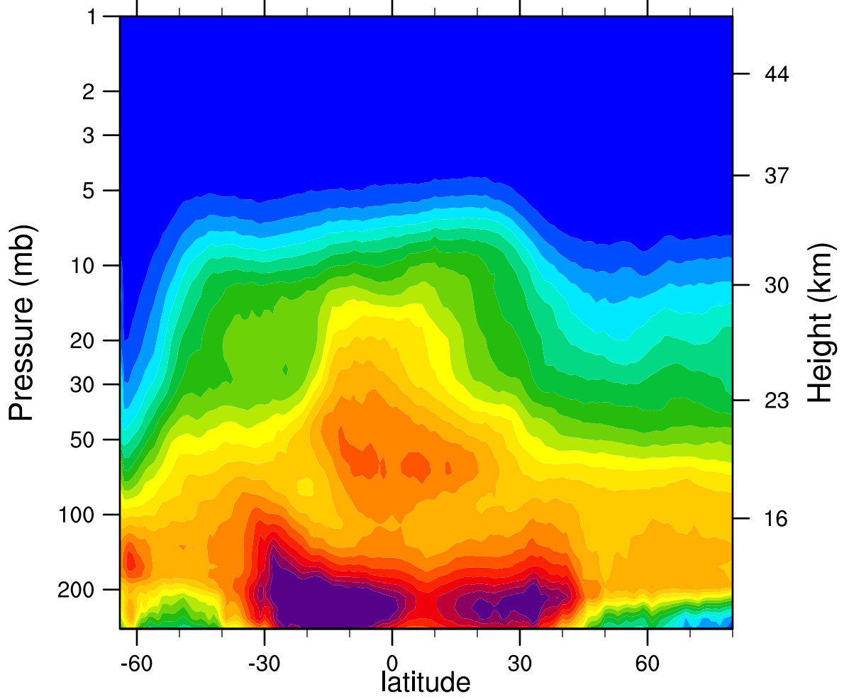
2007d205 N2O_Combined (ppbv)
