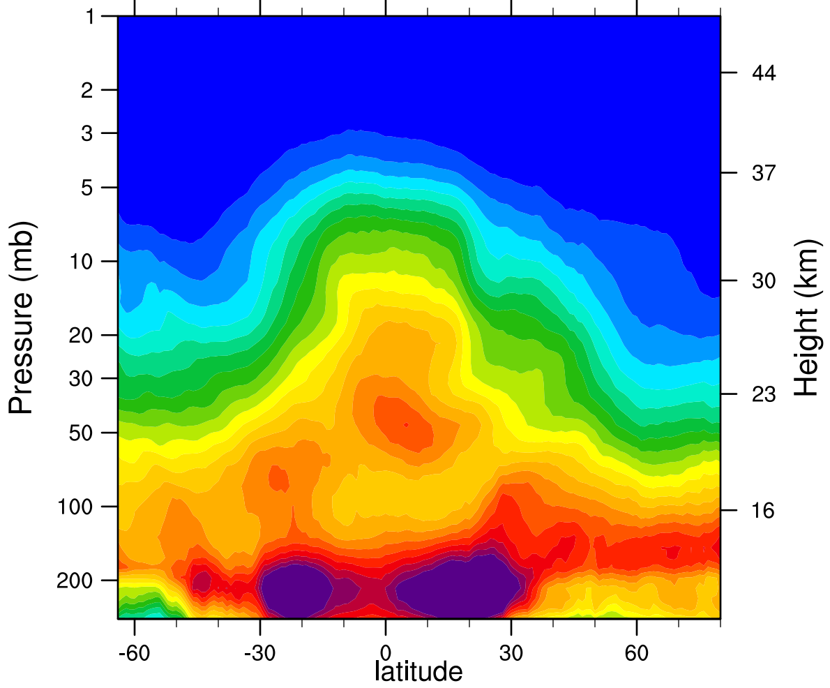
2005d057 N2O_Combined (ppbv)
