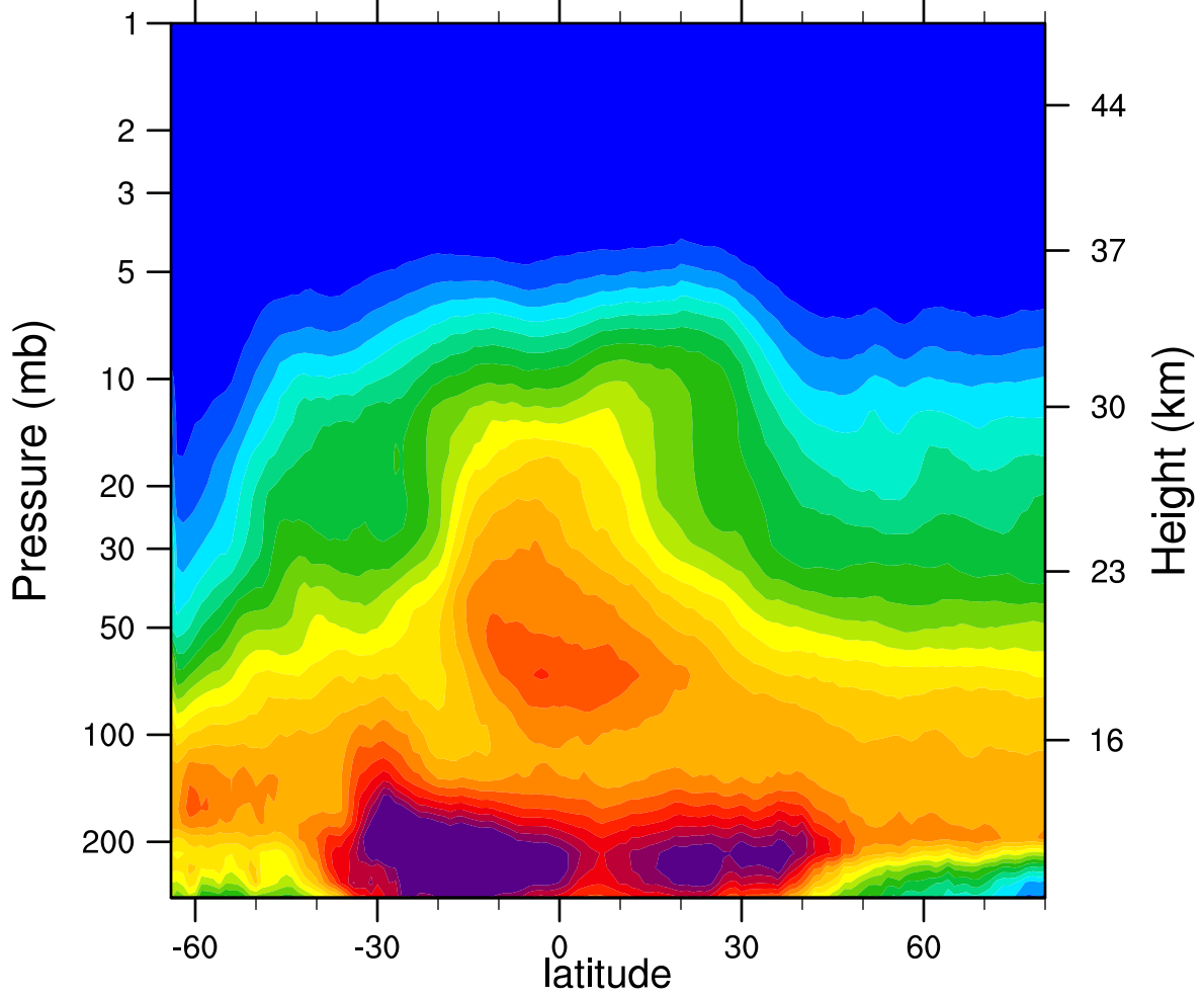
2007d185 N2O_Combined (ppbv)
