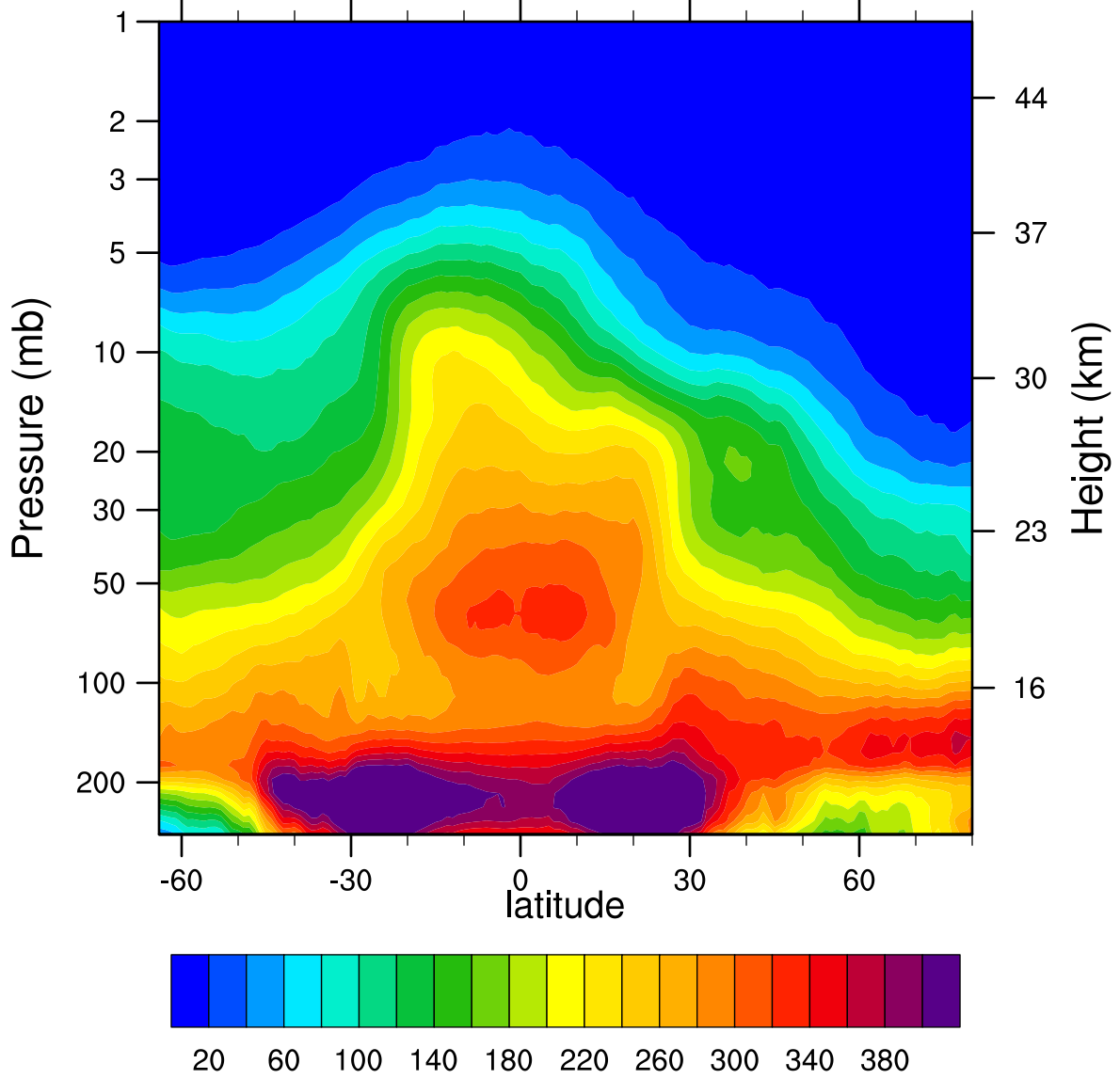
2006d011 N2O_Combined (ppbv)
