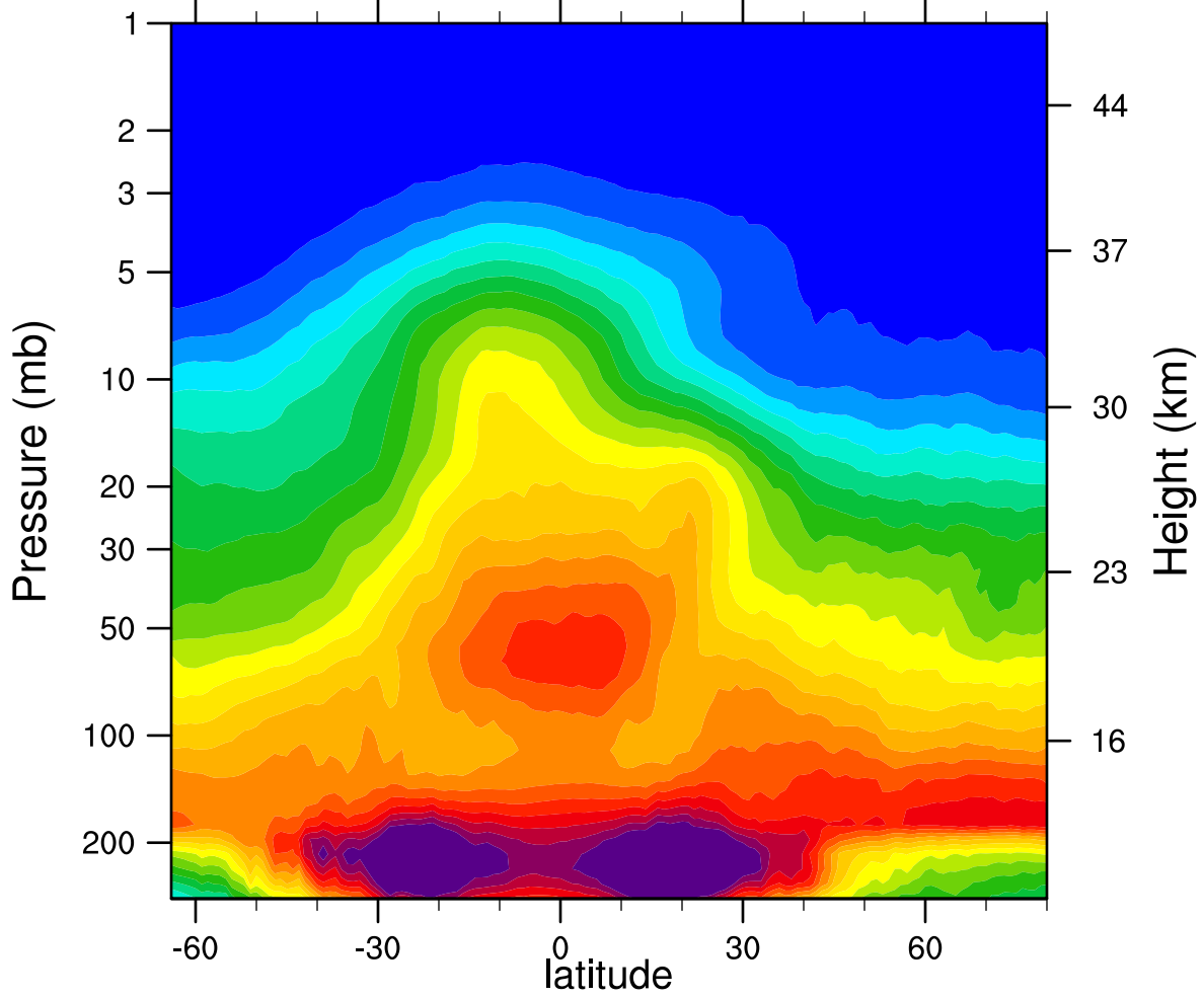
2006d052 N2O_Combined (ppbv)
