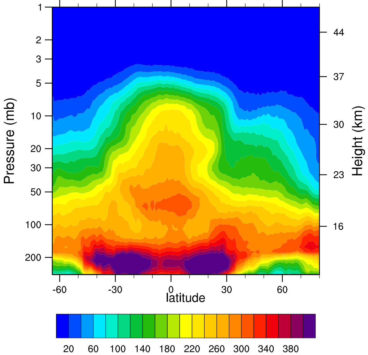
2007d074 N2O_Combined (ppbv)
