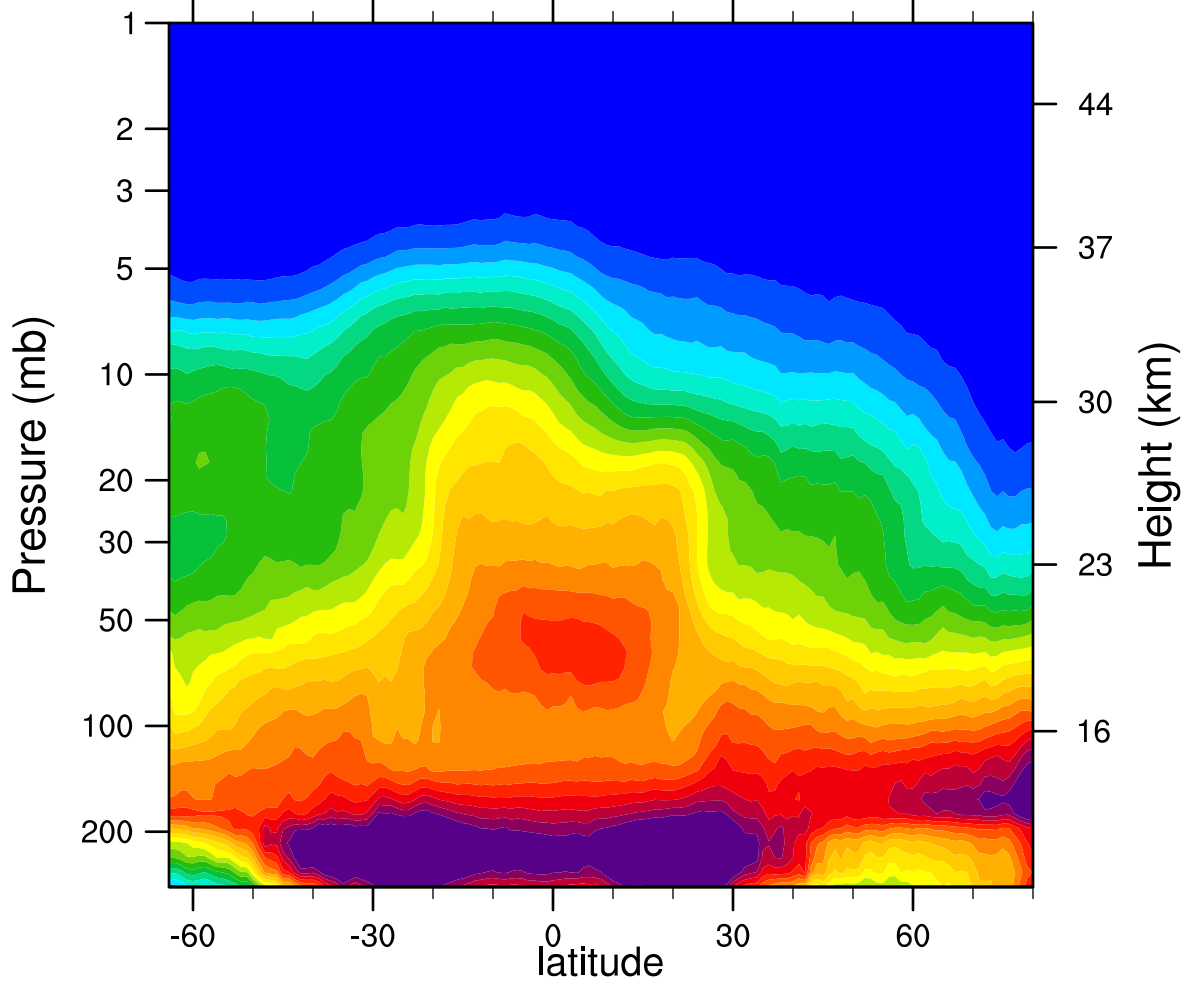
2007d358 N2O_Combined (ppbv)
