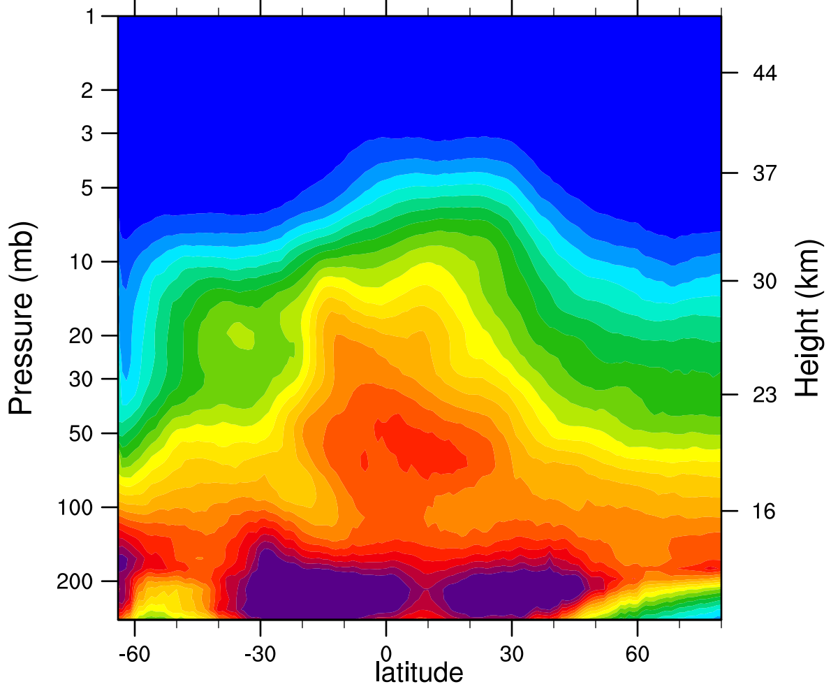
2007d250 N2O_Combined (ppbv)
