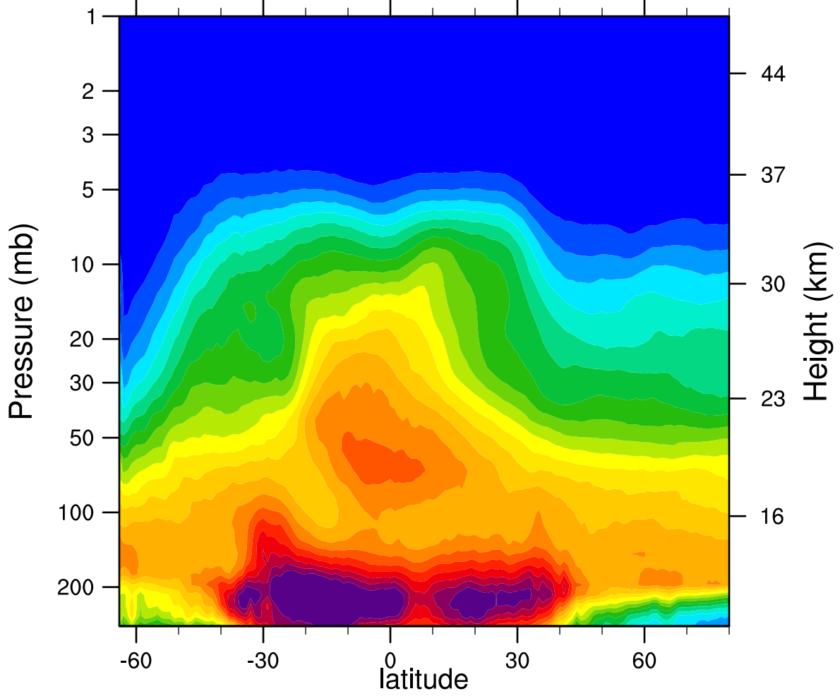
2007d171 N2O_Combined (ppbv)
