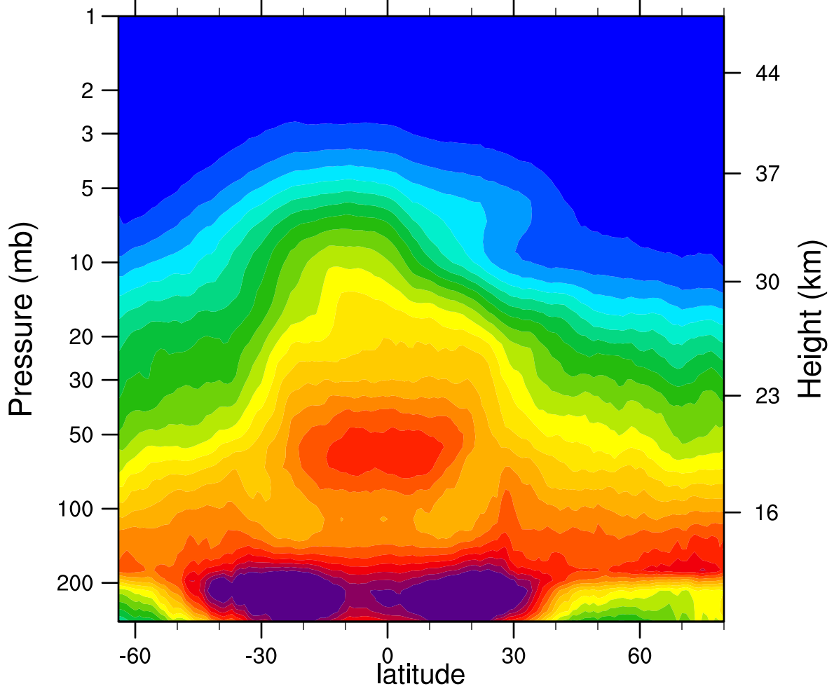
2006d084 N2O_Combined (ppbv)
