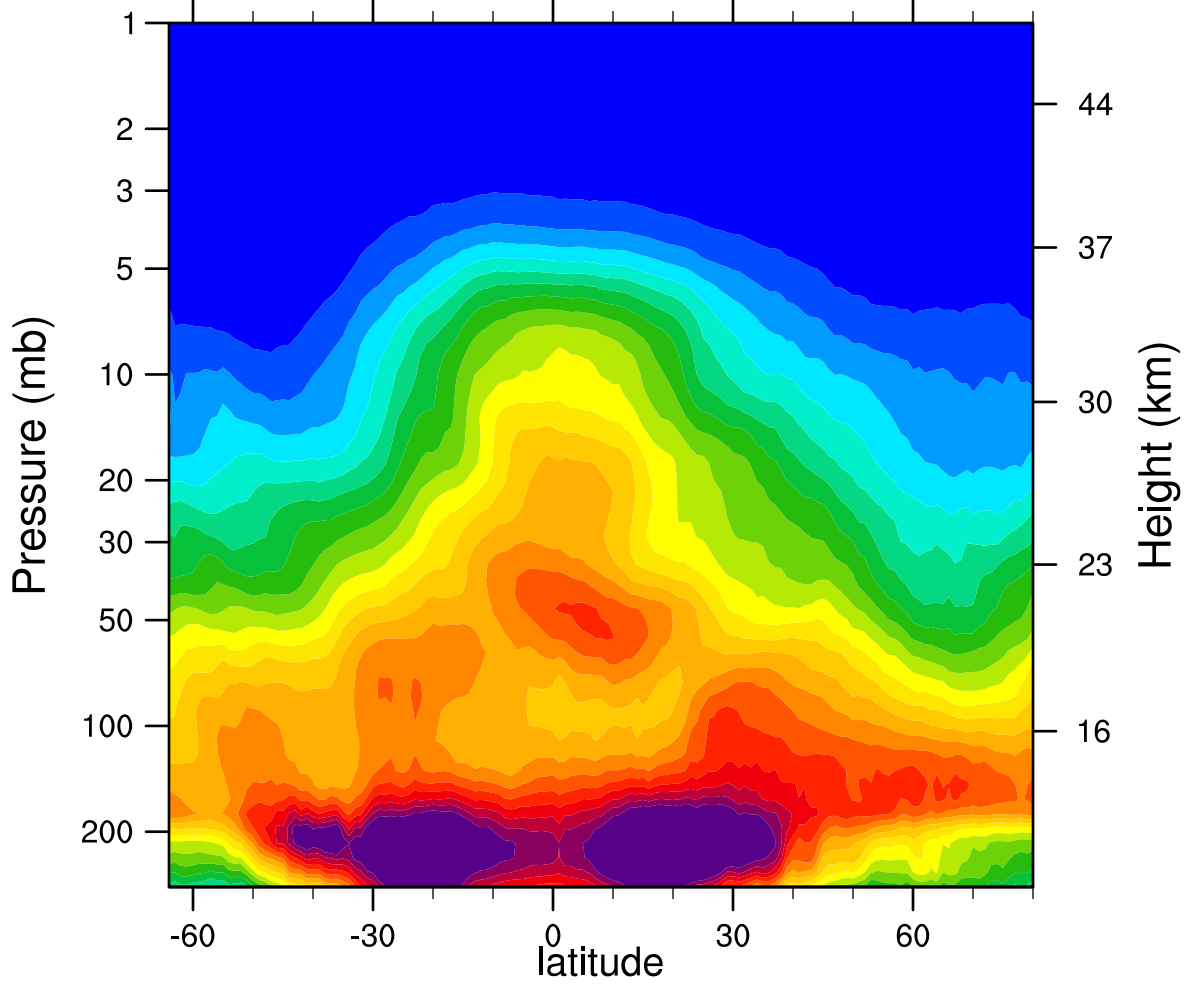
2005d076 N2O_Combined (ppbv)
