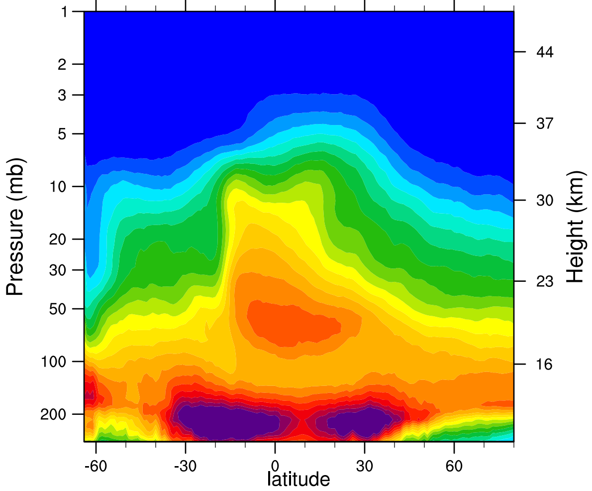
2005d258 N2O_Combined (ppbv)
