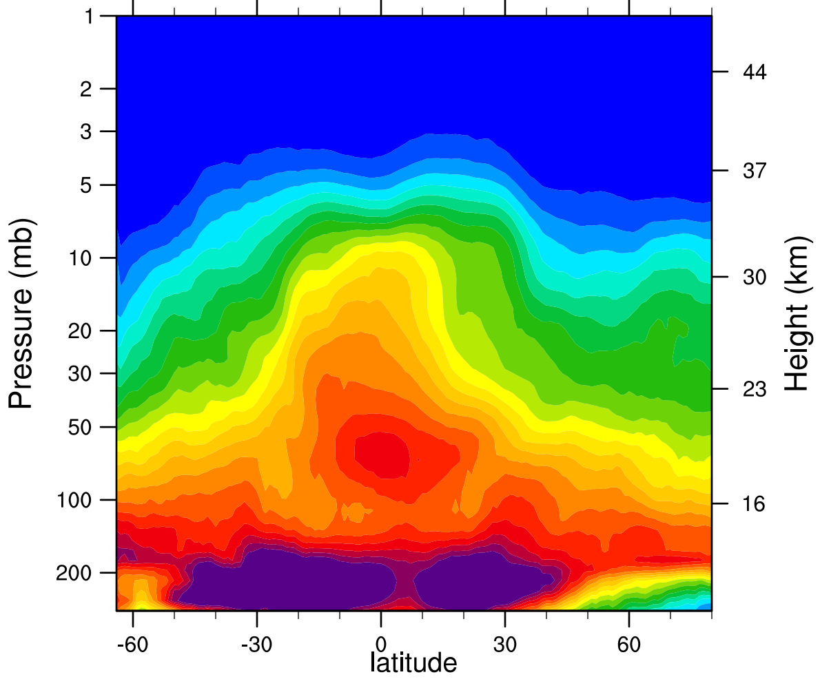
2007d135 N2O_Combined (ppbv)
