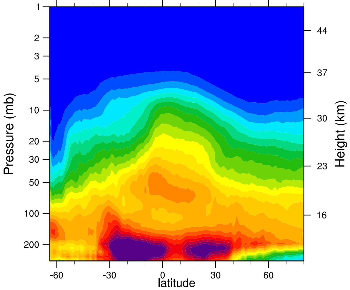
2006d191 N2O_Combined (ppbv)
