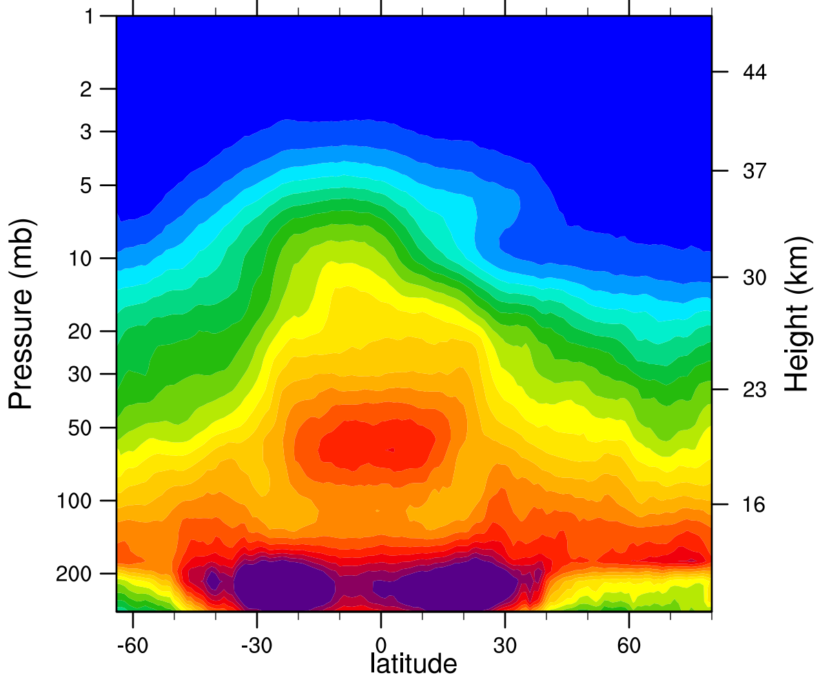
2006d081 N2O_Combined (ppbv)
