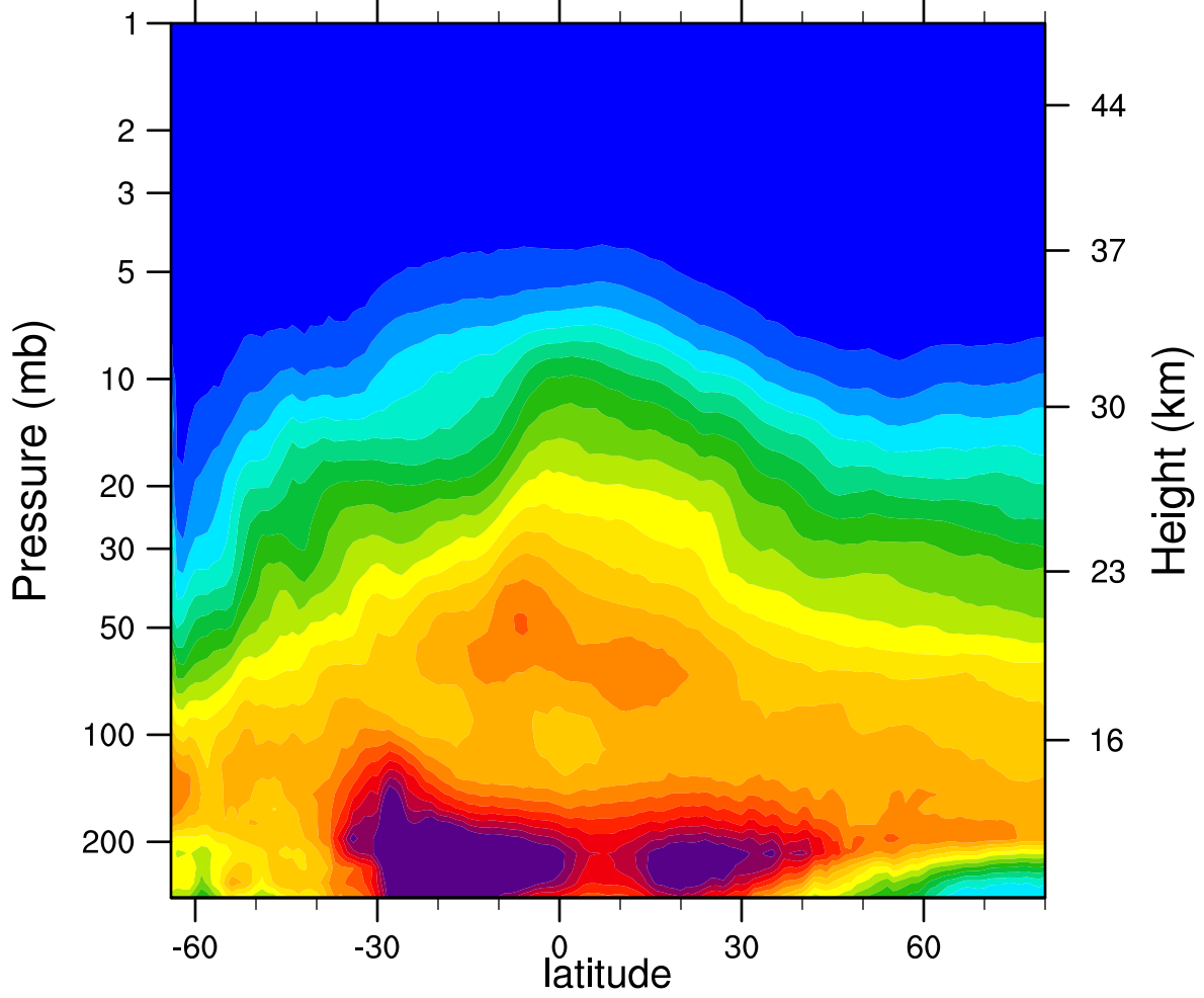
2006d178 N2O_Combined (ppbv)
