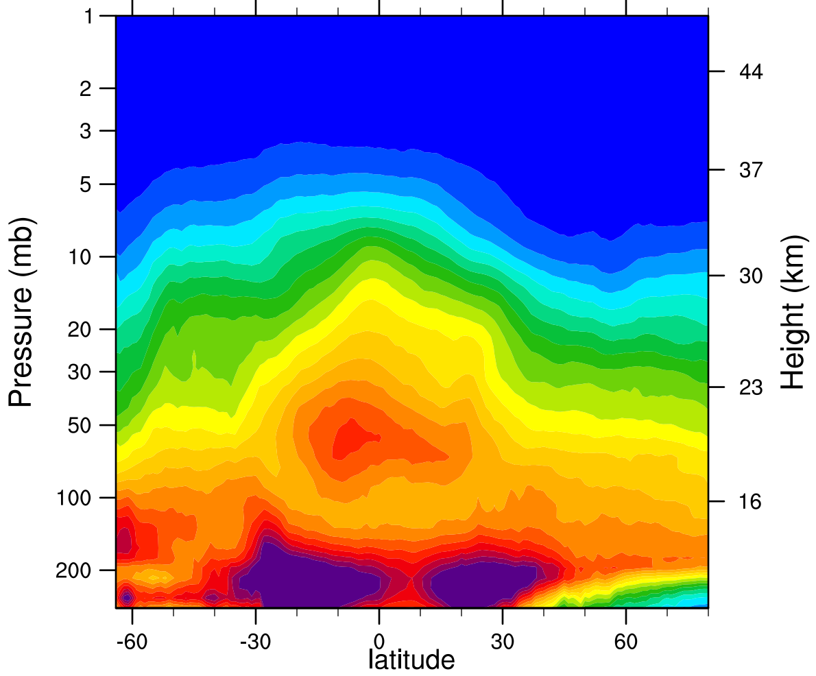
2006d158 N2O_Combined (ppbv)
