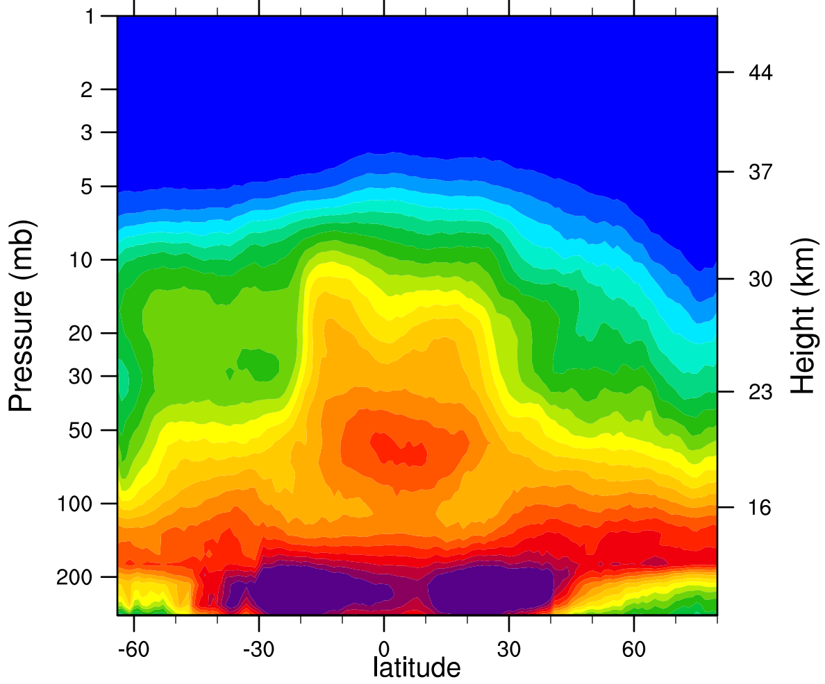
2007d314 N2O_Combined (ppbv)
