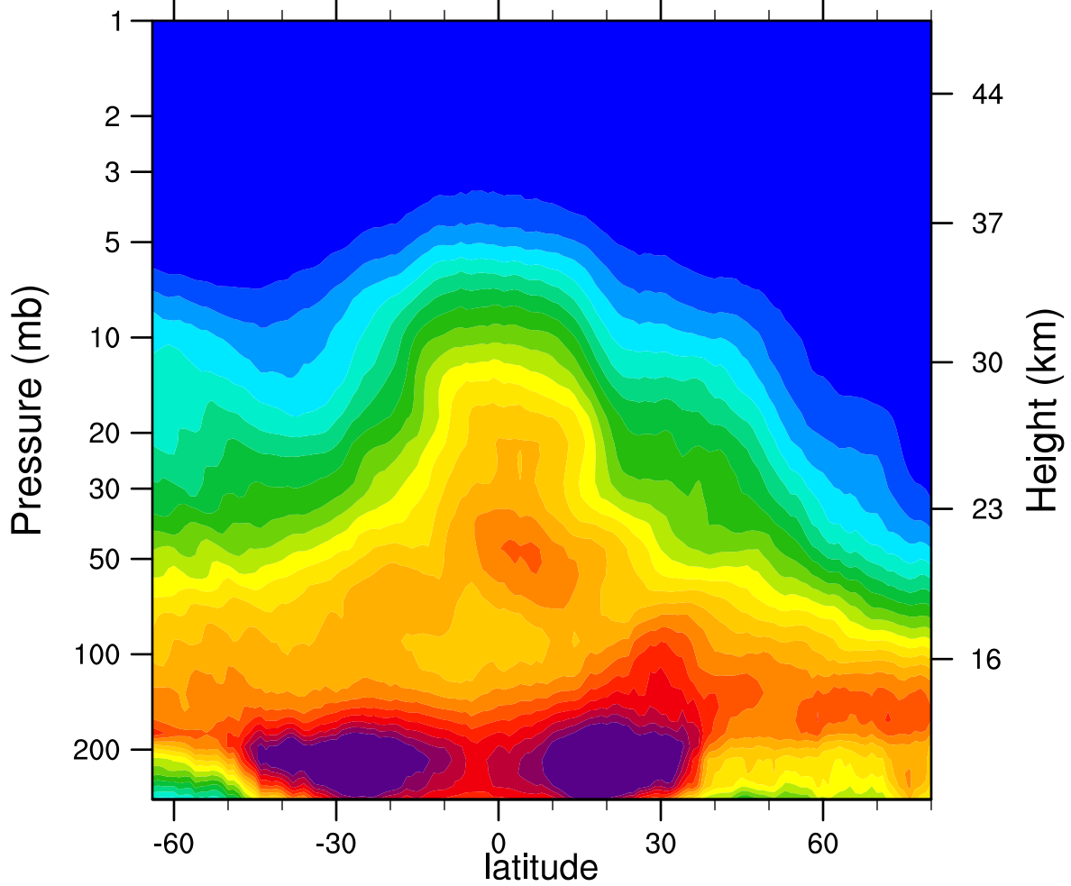
2005d033 N2O_Combined (ppbv)
