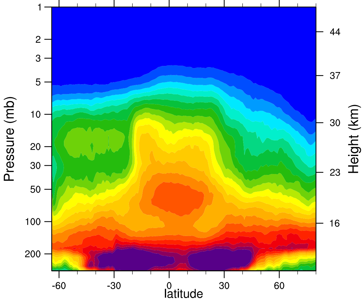
2007d310 N2O_Combined (ppbv)
