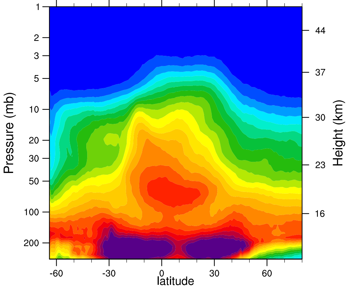
2007d258 N2O_Combined (ppbv)
