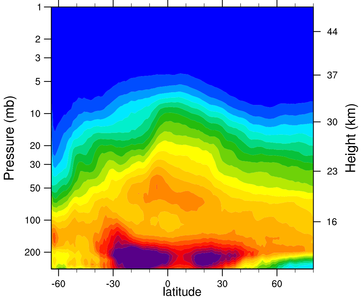
2006d180 N2O_Combined (ppbv)
