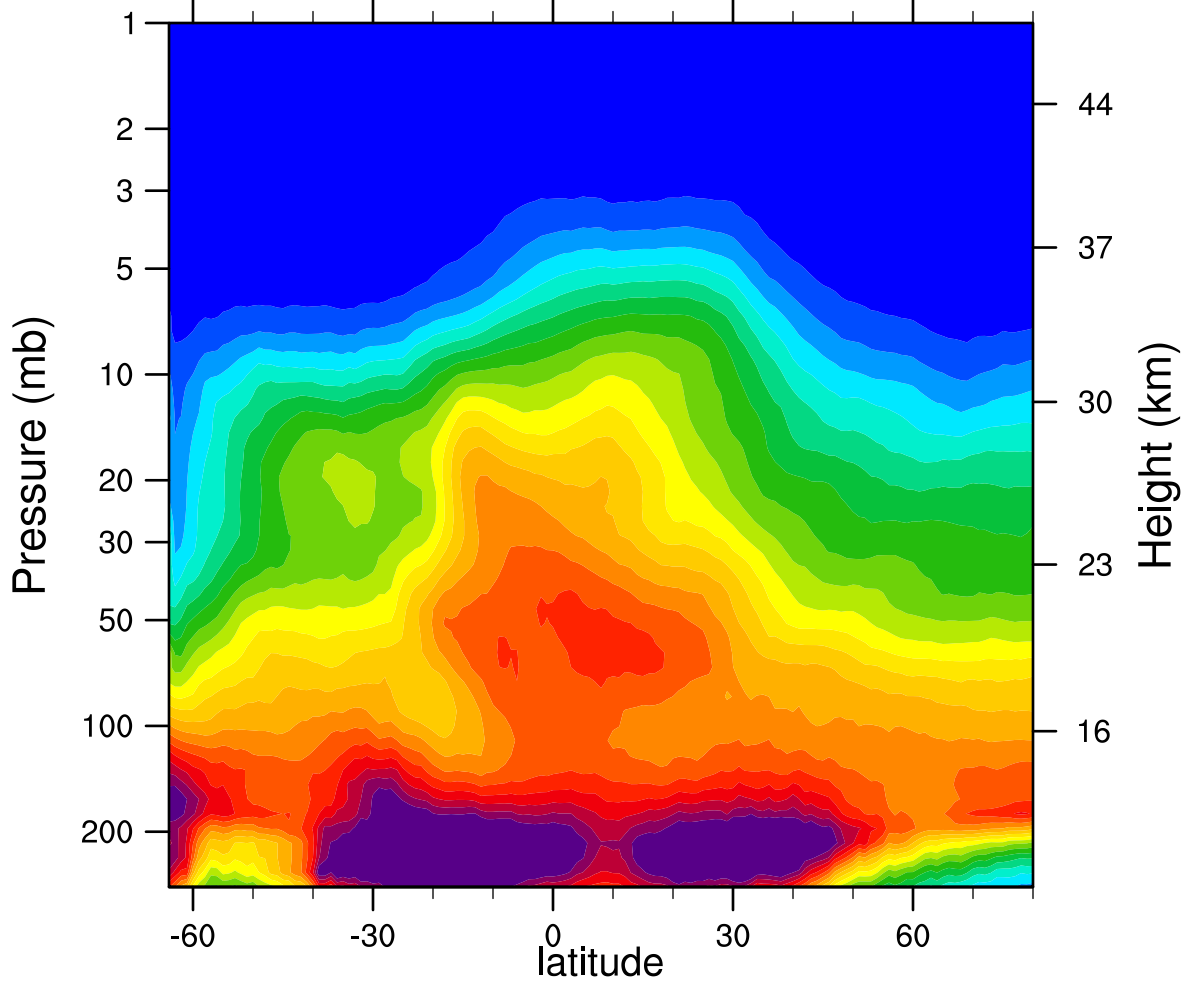
2007d248 N2O_Combined (ppbv)
