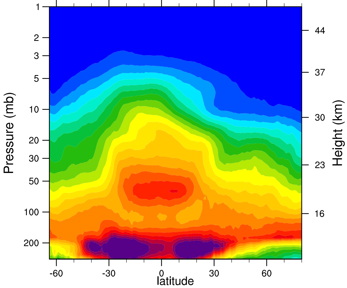
2006d104 N2O_Combined (ppbv)
