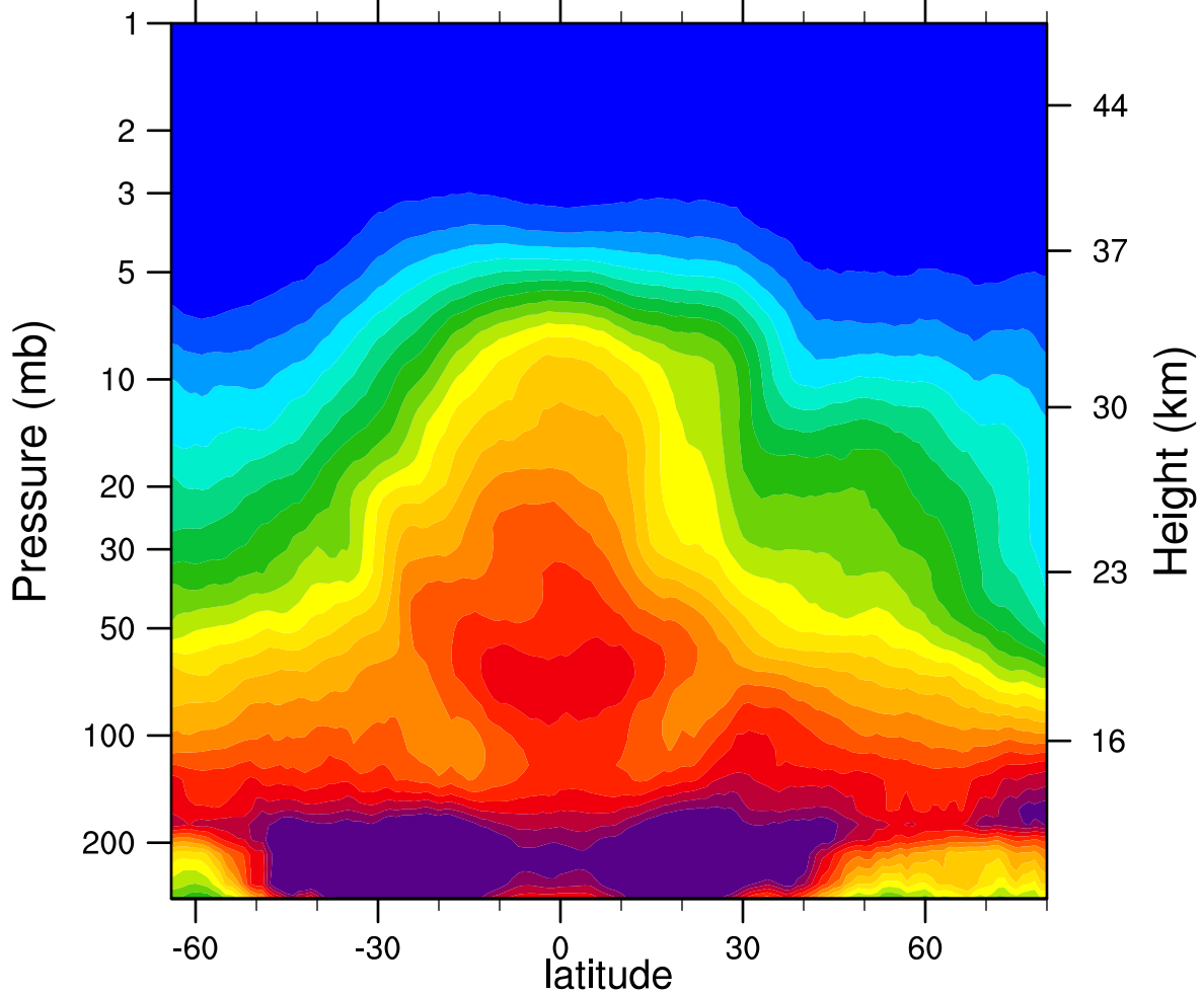
2007d095 N2O_Combined (ppbv)
