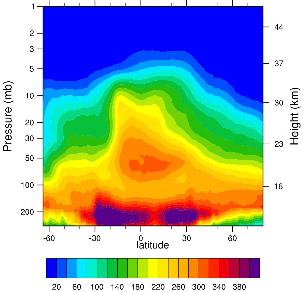
2005d278 N2O_Combined (ppbv)
