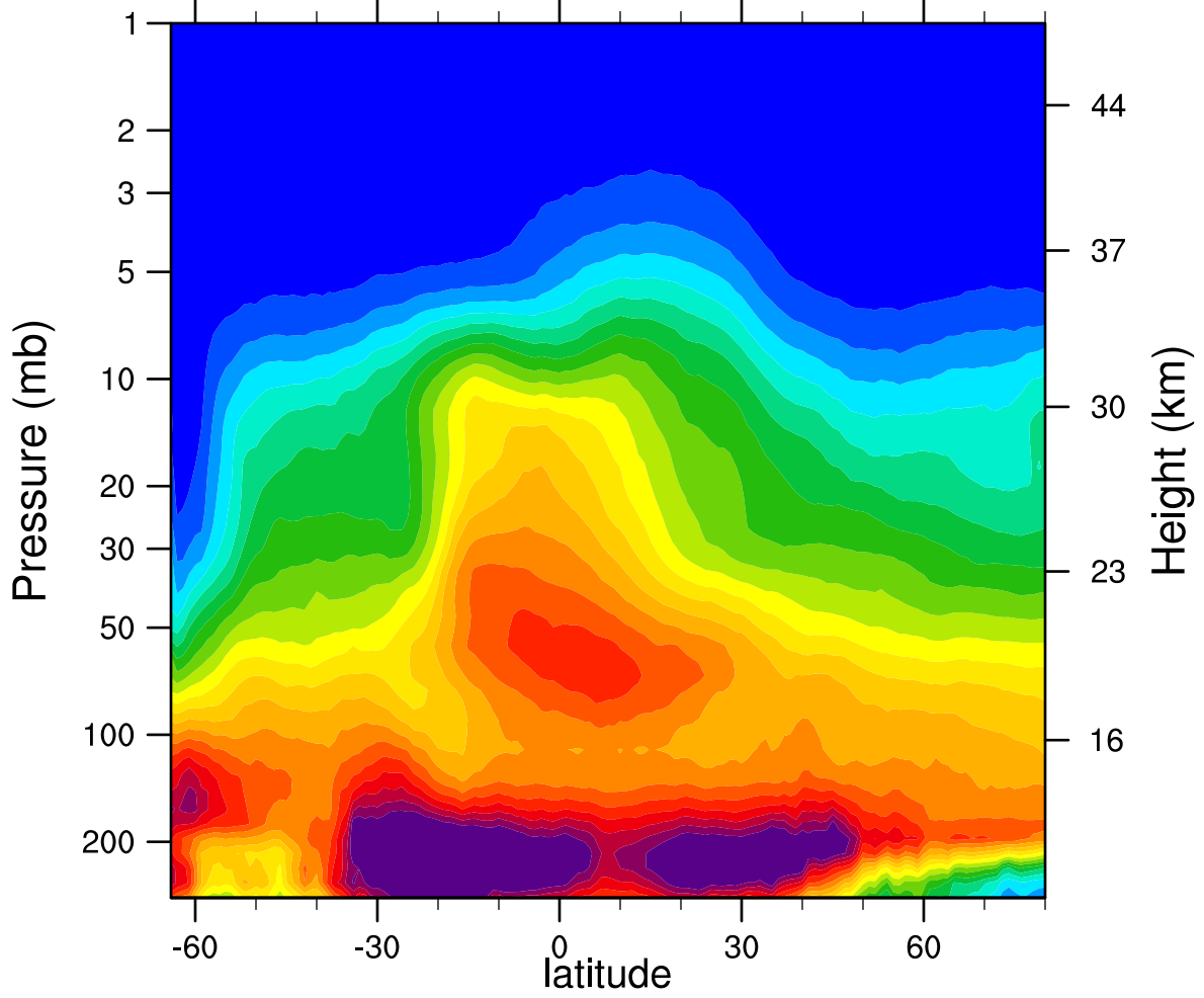
2005d196 N2O_Combined (ppbv)
