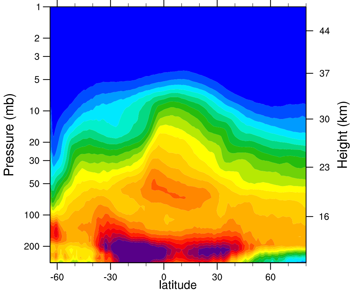
2006d220 N2O_Combined (ppbv)
