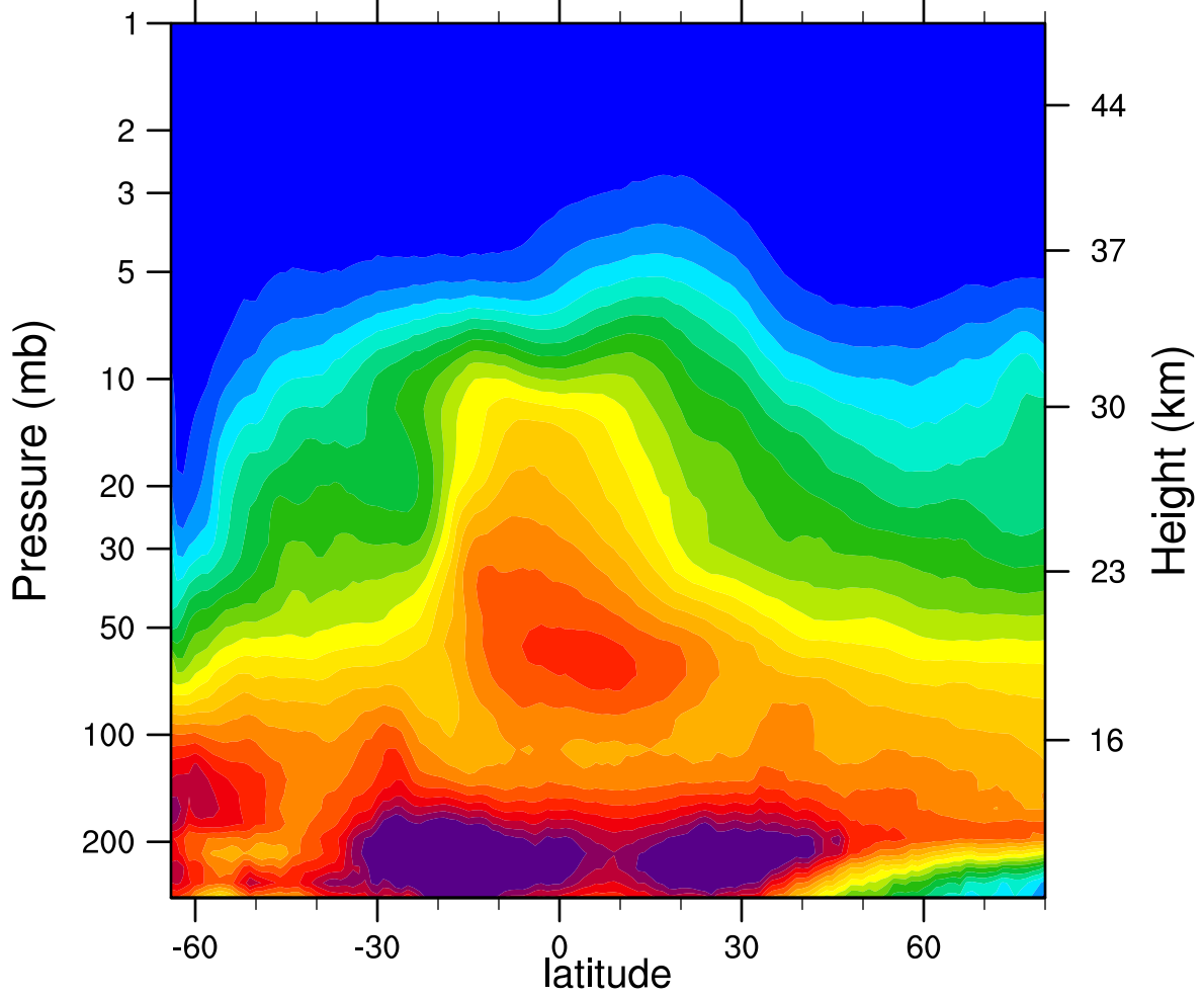
2005d181 N2O_Combined (ppbv)
