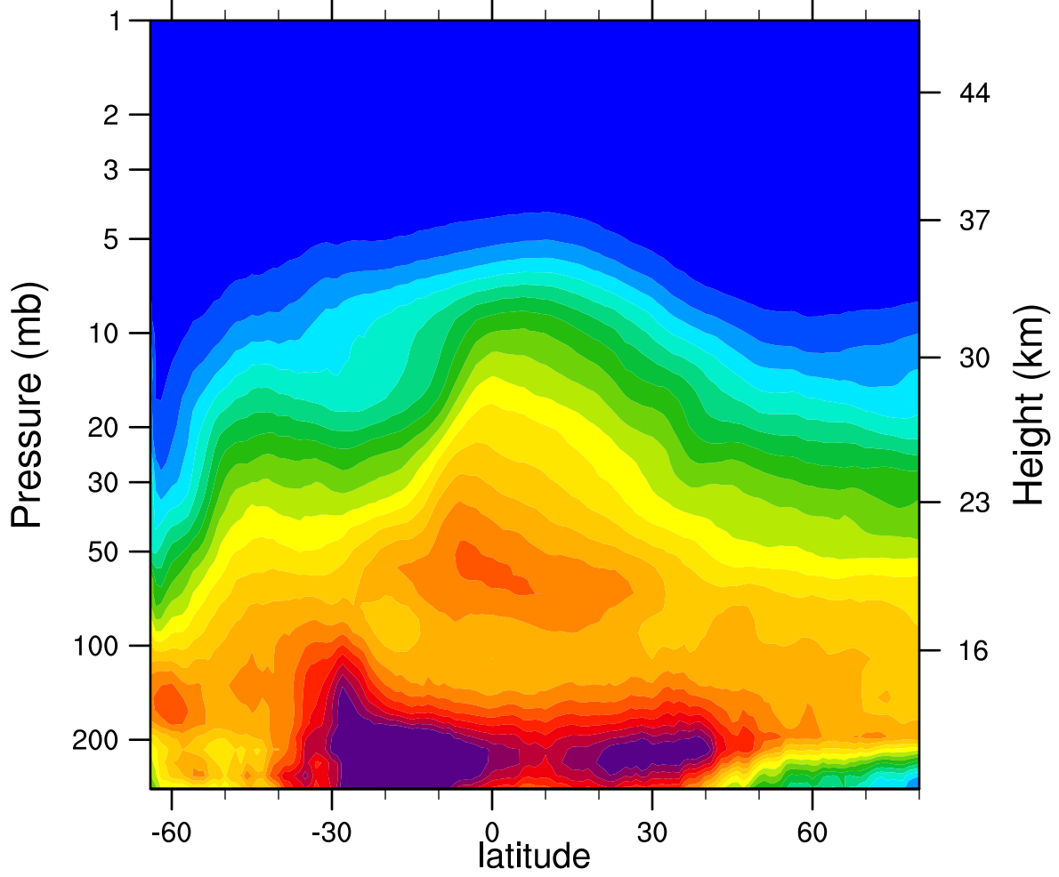
2006d212 N2O_Combined (ppbv)
