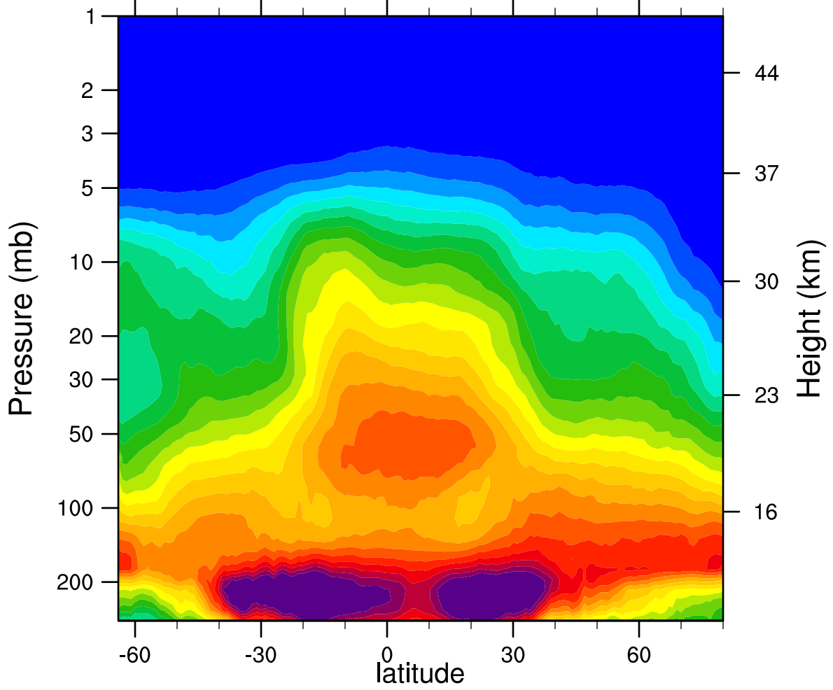
2005d316 N2O_Combined (ppbv)
