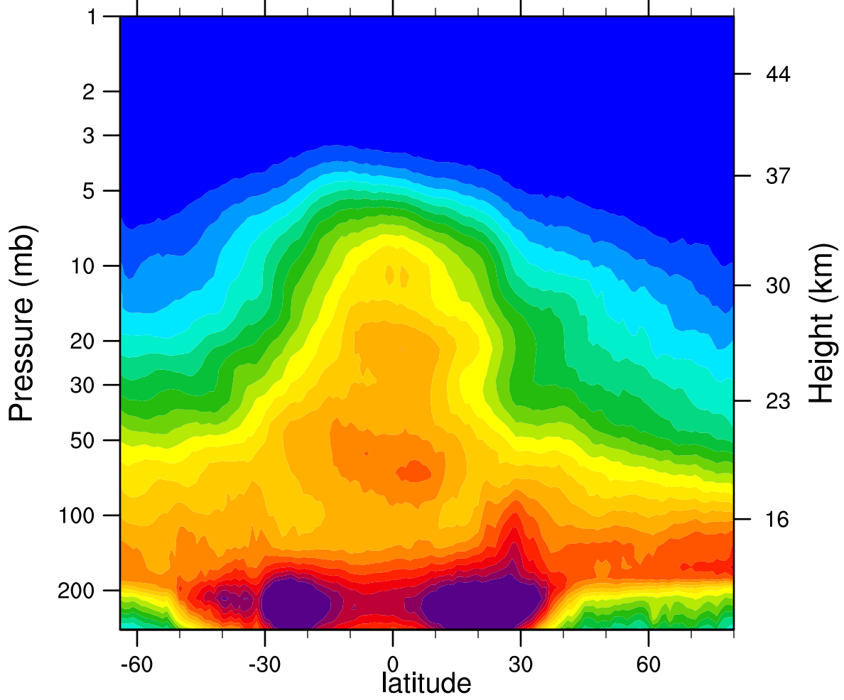
2007d059 N2O_Combined (ppbv)
