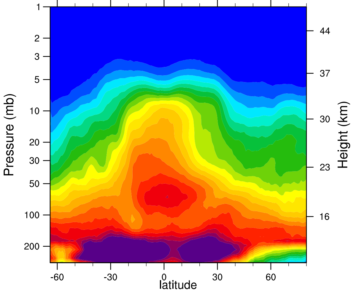
2007d130 N2O_Combined (ppbv)
