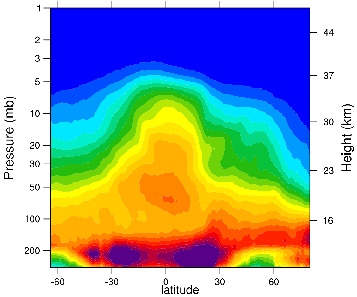
2007d040 N2O_Combined (ppbv)
