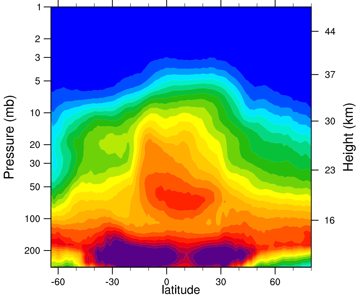
2007d272 N2O_Combined (ppbv)
