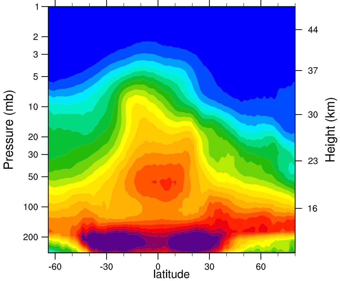
2006d026 N2O_Combined (ppbv)
