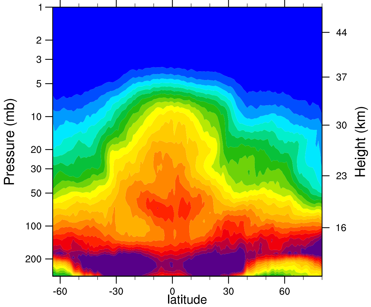
2007d079 N2O_Combined (ppbv)
