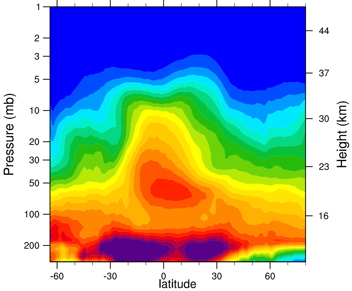
2005d154 N2O_Combined (ppbv)
