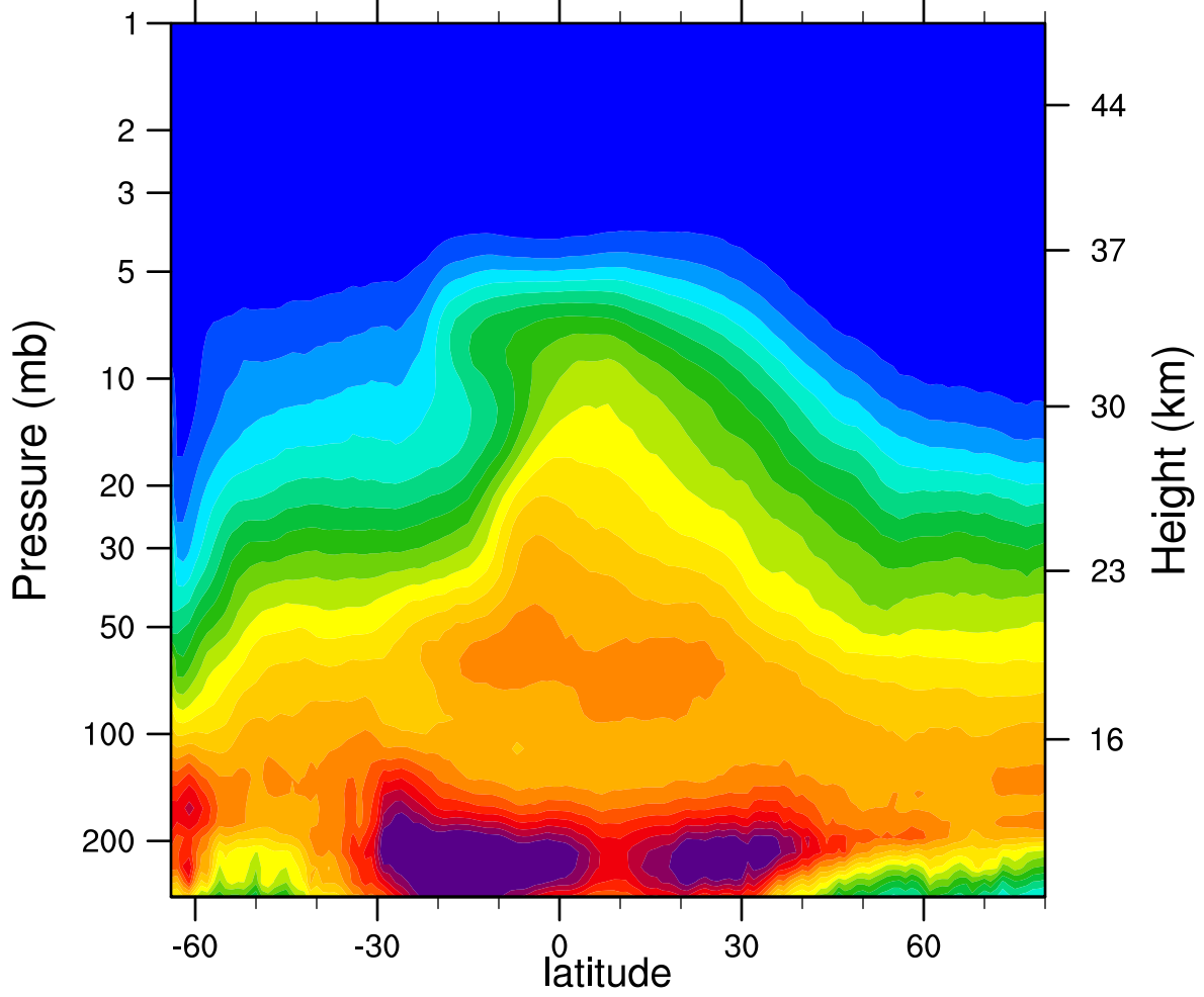
2006d263 N2O_Combined (ppbv)
