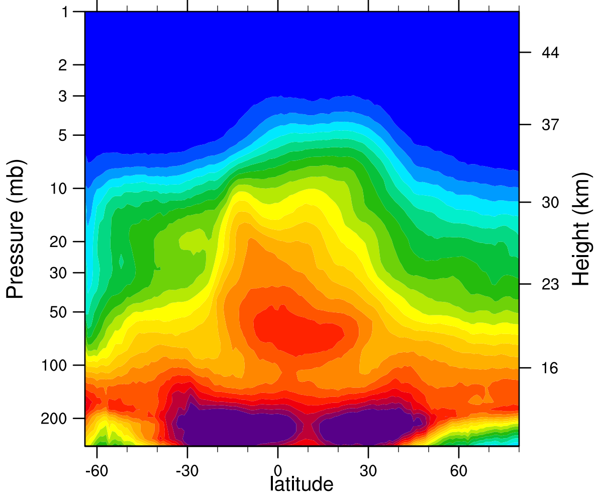
2007d260 N2O_Combined (ppbv)
