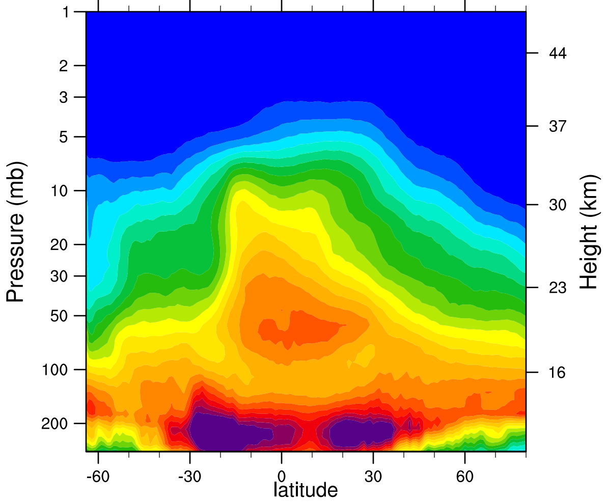
2005d280 N2O_Combined (ppbv)
