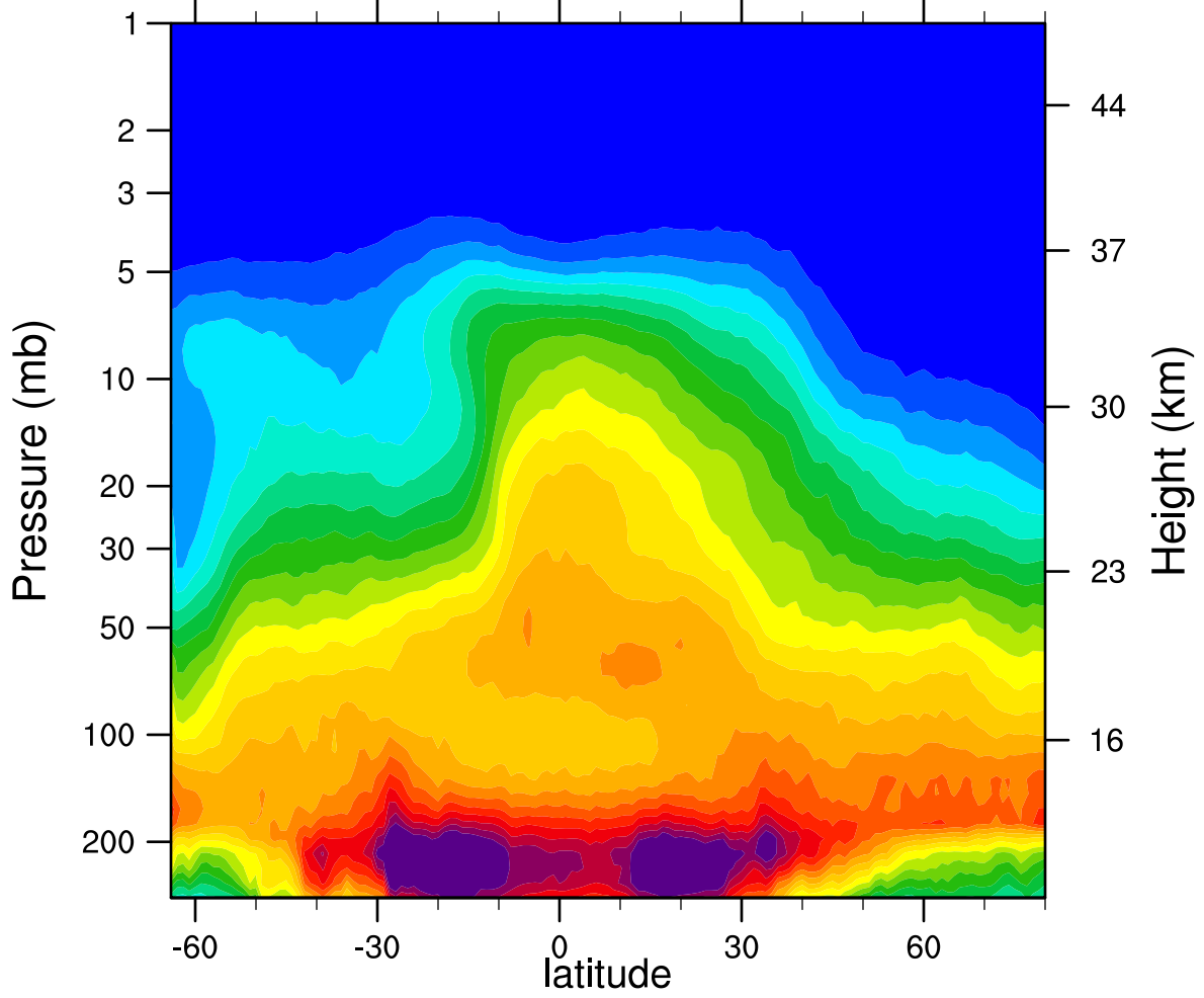
2006d306 N2O_Combined (ppbv)
