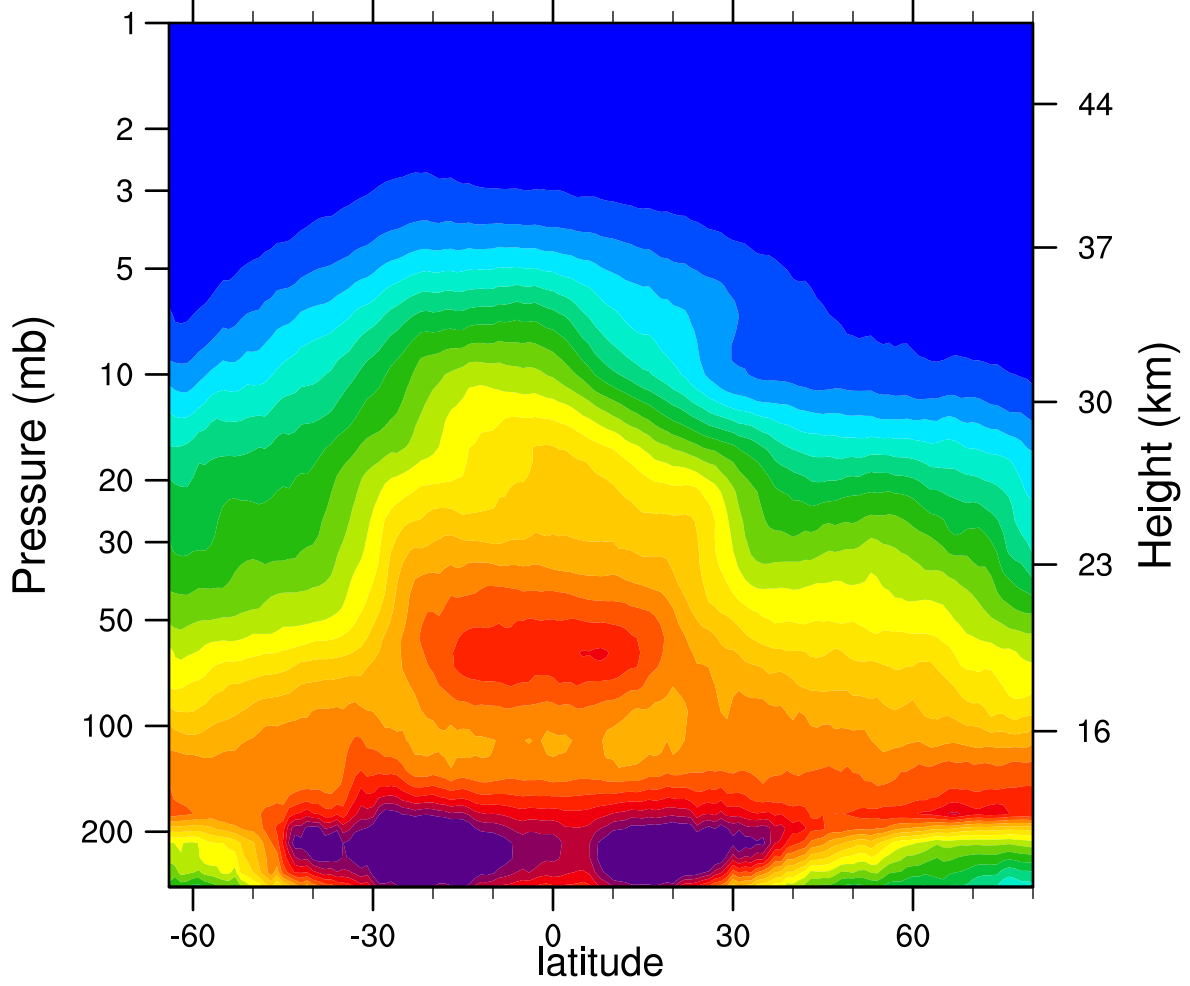
2006d103 N2O_Combined (ppbv)
