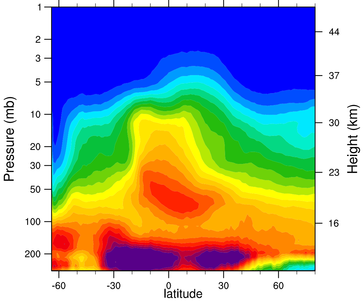
2005d206 N2O_Combined (ppbv)
