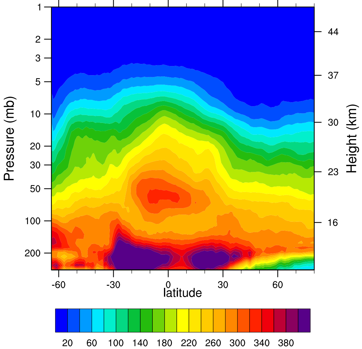
2006d153 N2O_Combined (ppbv)
