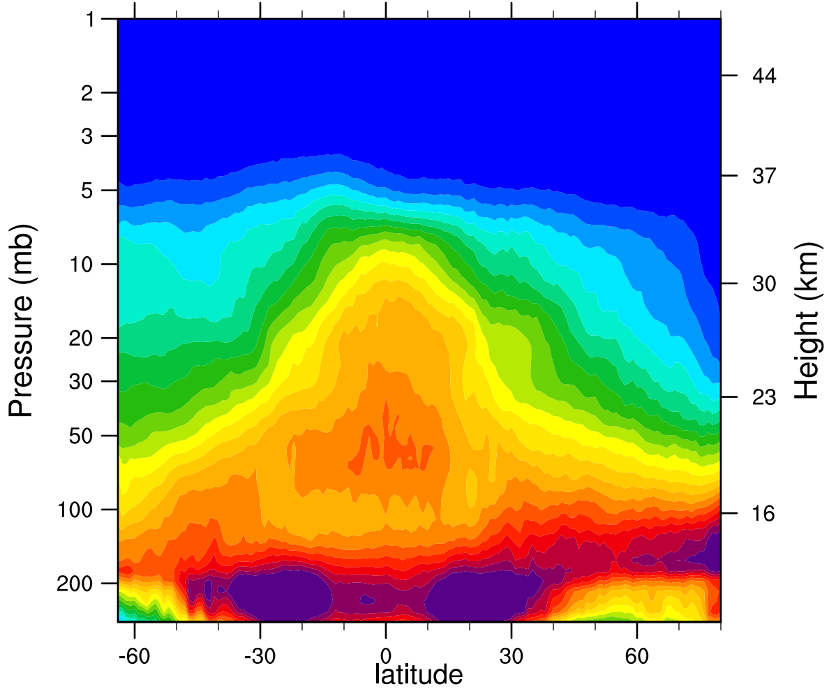
2006d357 N2O_Combined (ppbv)
