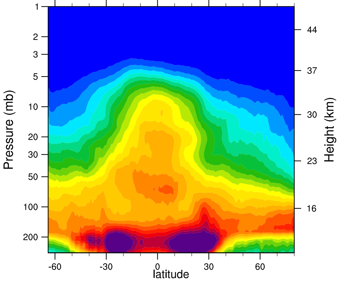
2007d060 N2O_Combined (ppbv)
