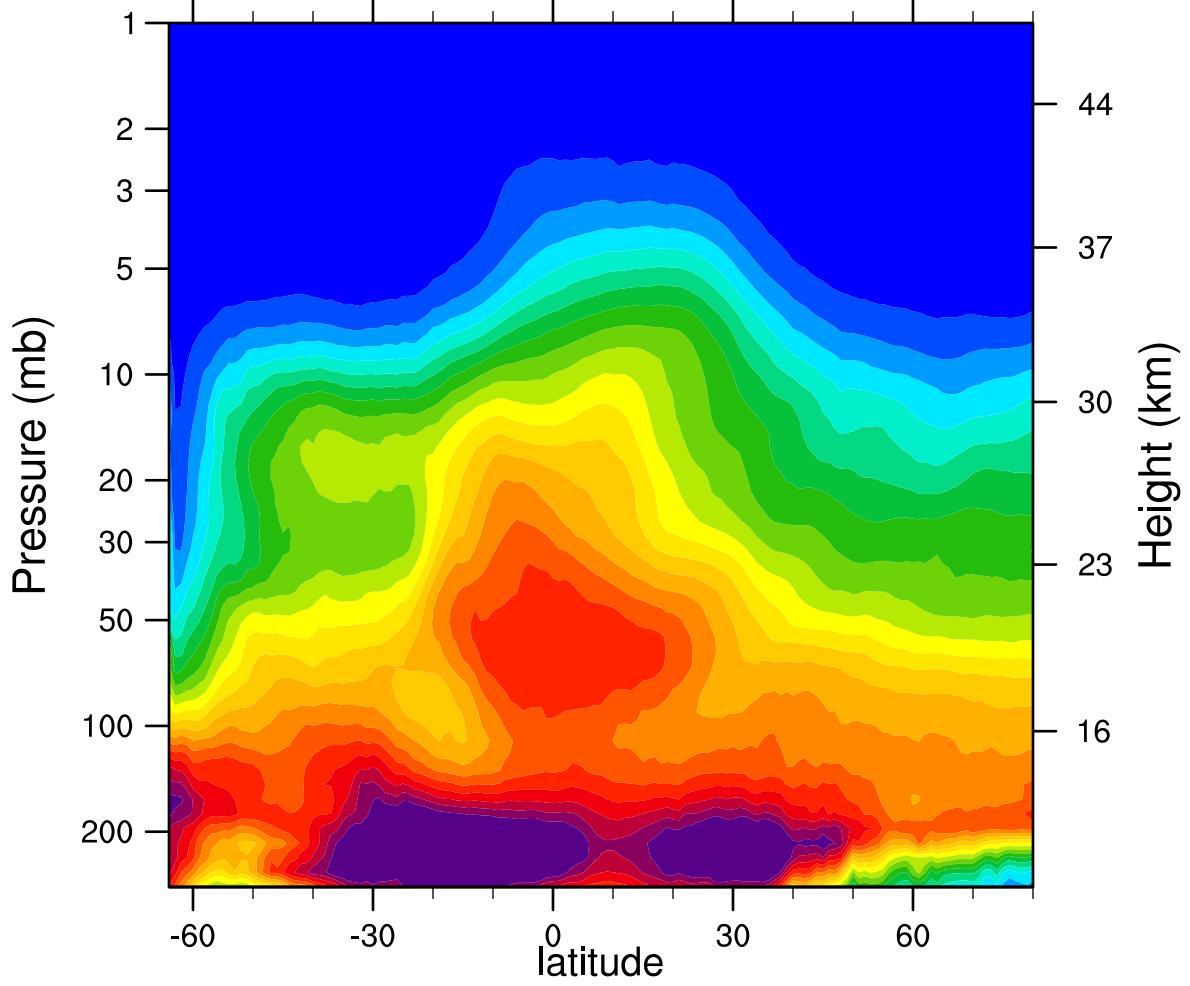
2007d229 N2O_Combined (ppbv)
