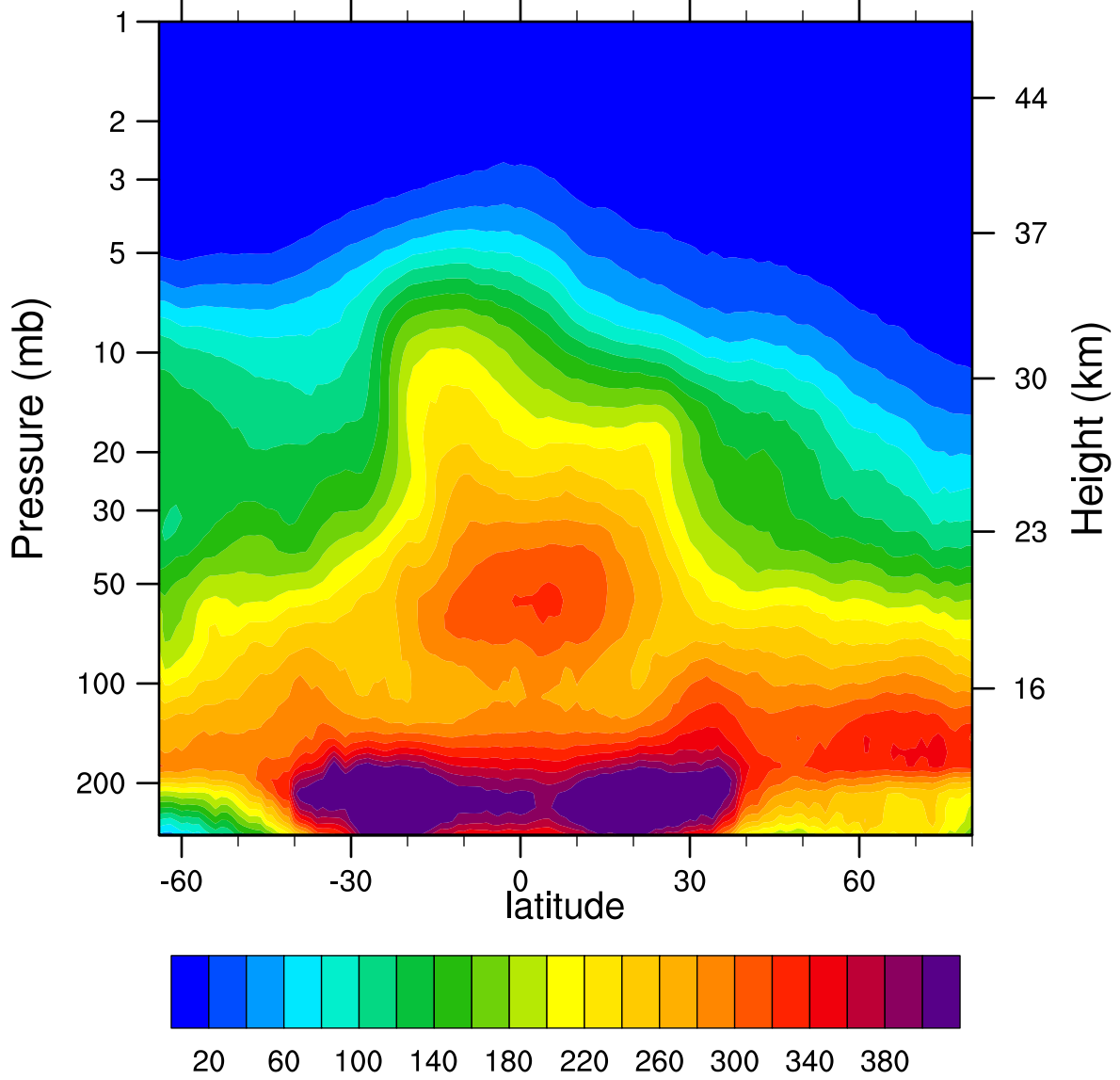
2005d346 N2O_Combined (ppbv)
