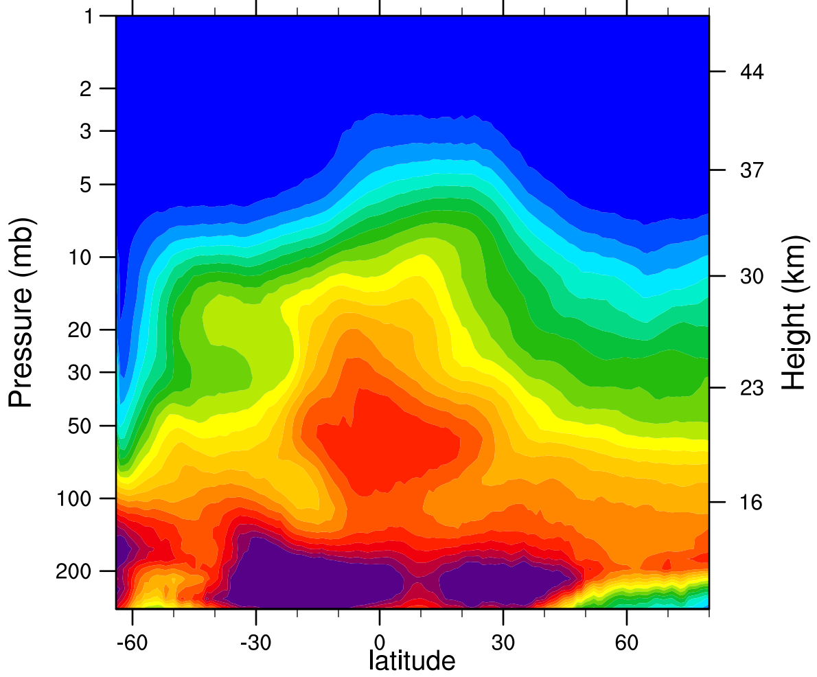
2007d234 N2O_Combined (ppbv)
