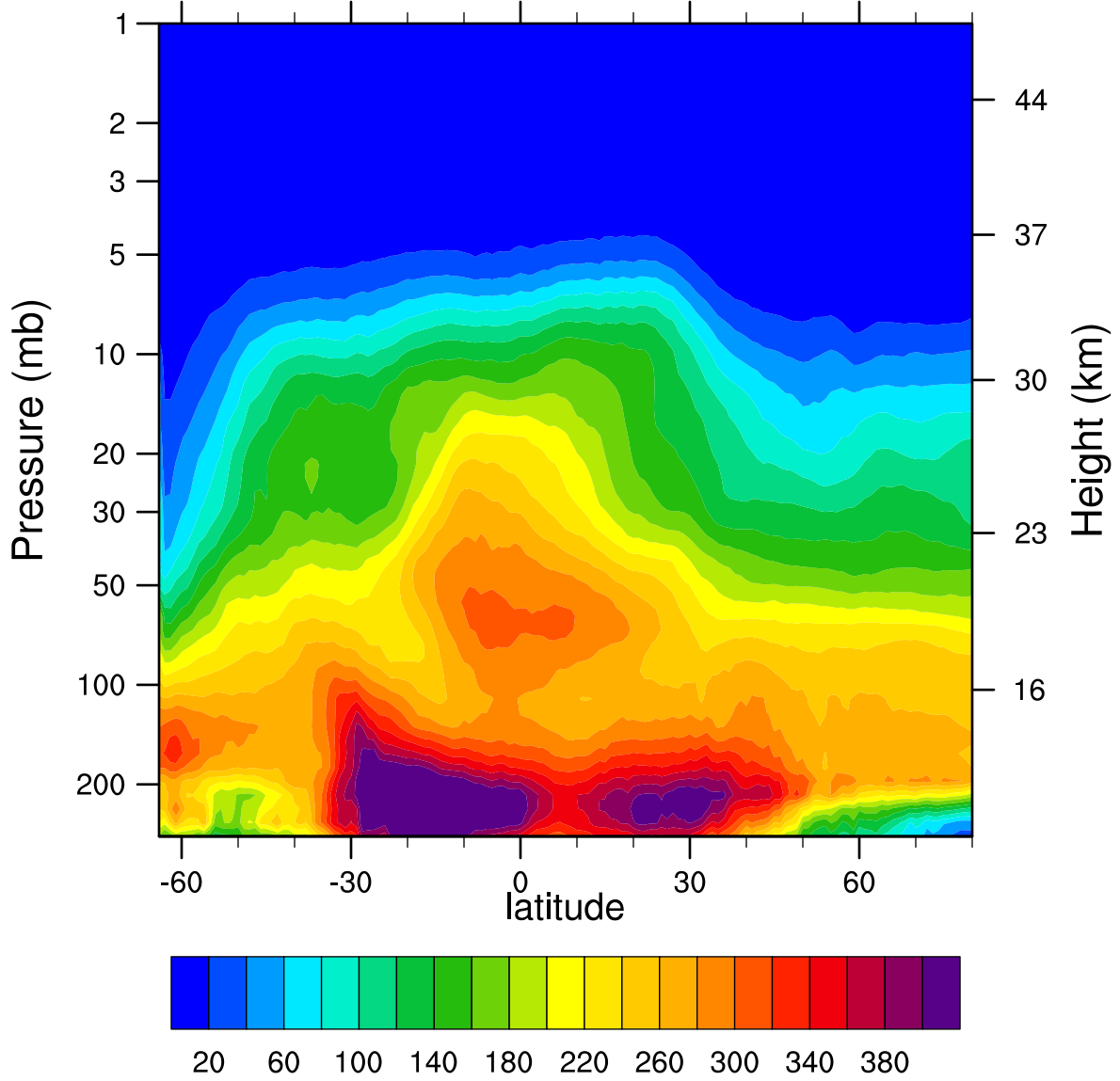
2007d199 N2O_Combined (ppbv)
