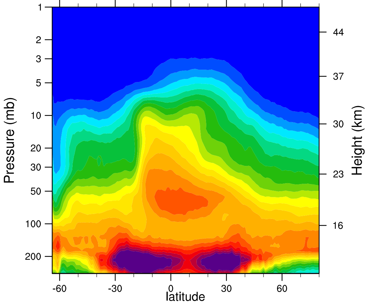
2005d263 N2O_Combined (ppbv)
