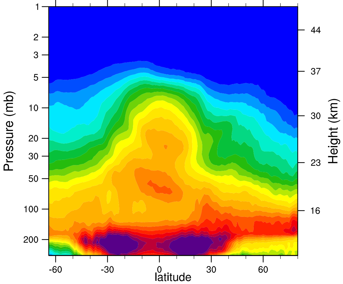
2007d029 N2O_Combined (ppbv)
