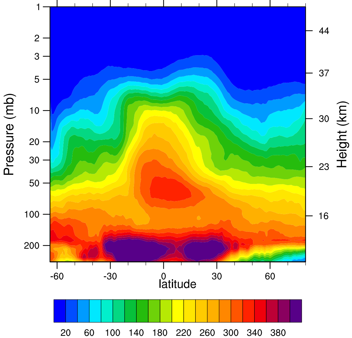
2005d151 N2O_Combined (ppbv)
