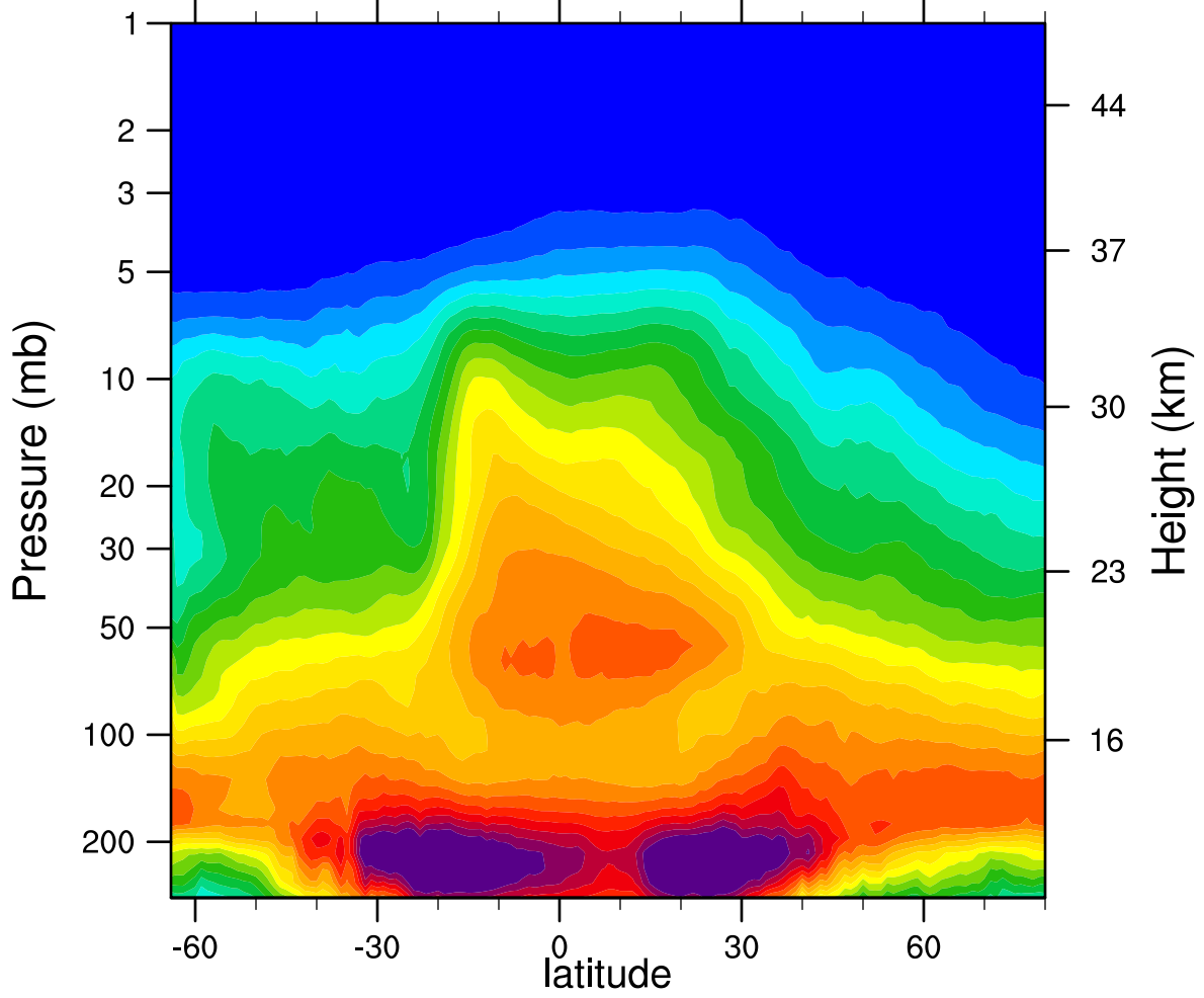
2005d297 N2O_Combined (ppbv)
