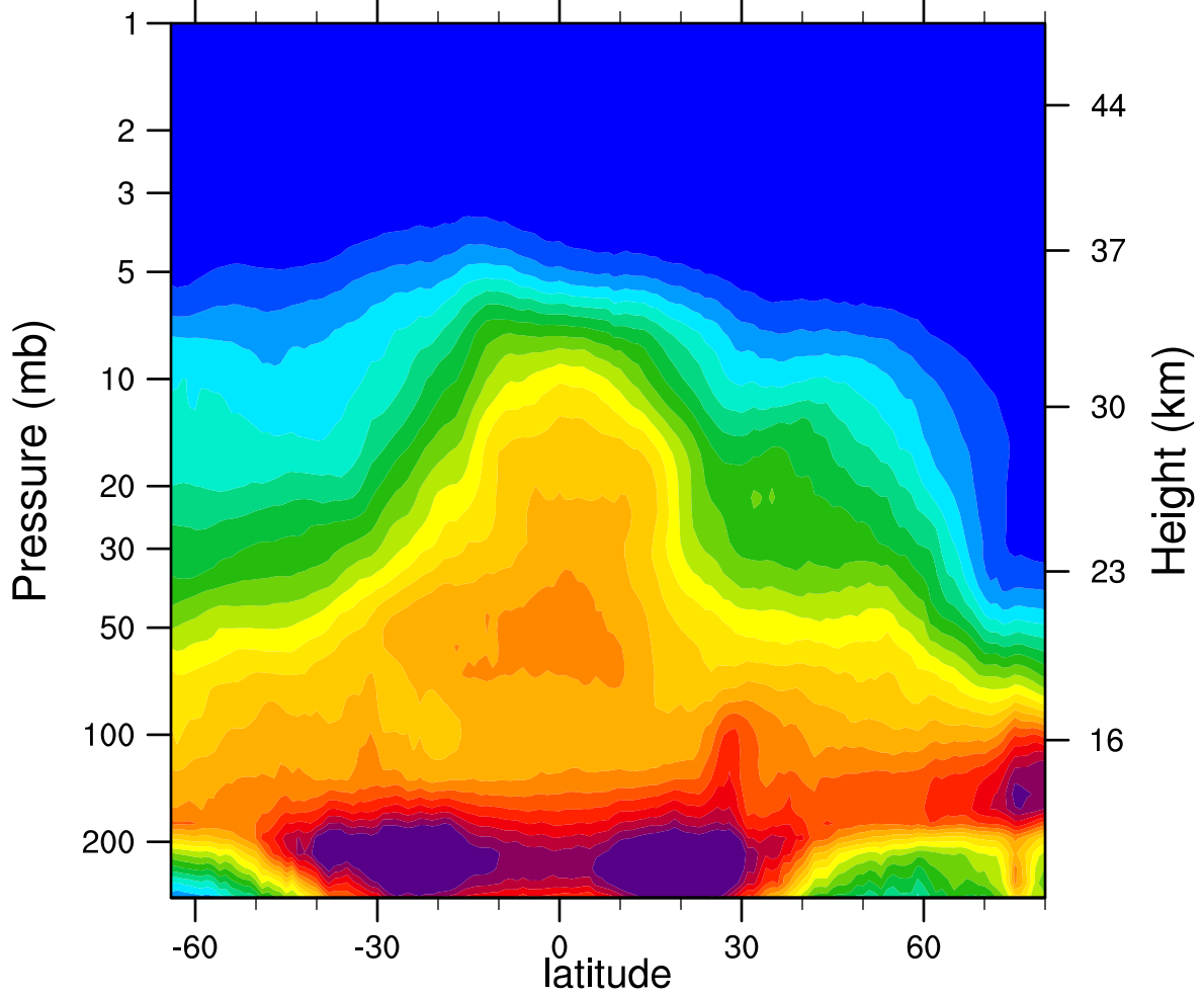
2007d004 N2O_Combined (ppbv)
