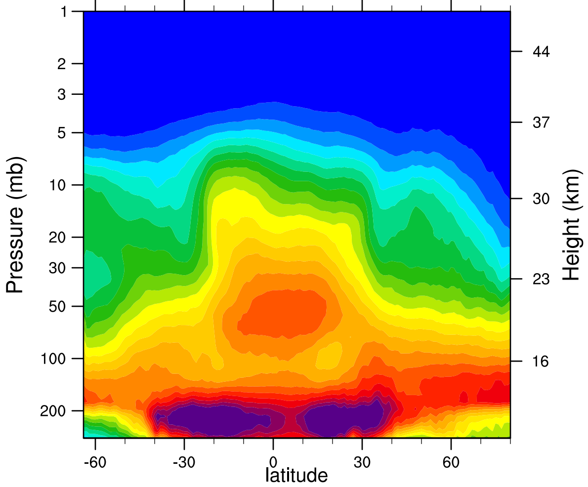
2005d326 N2O_Combined (ppbv)
