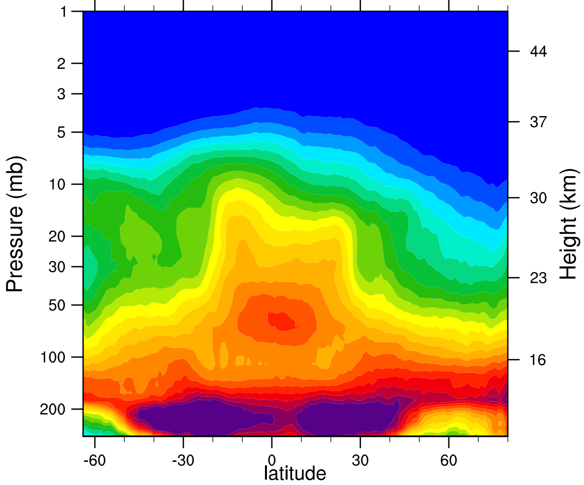
2007d335 N2O_Combined (ppbv)
