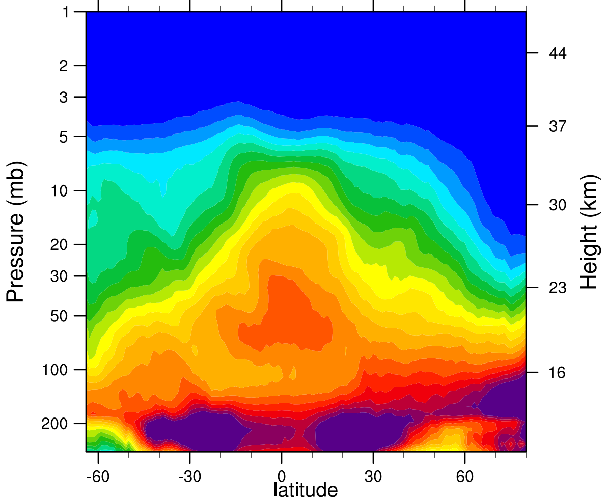
2006d343 N2O_Combined (ppbv)
