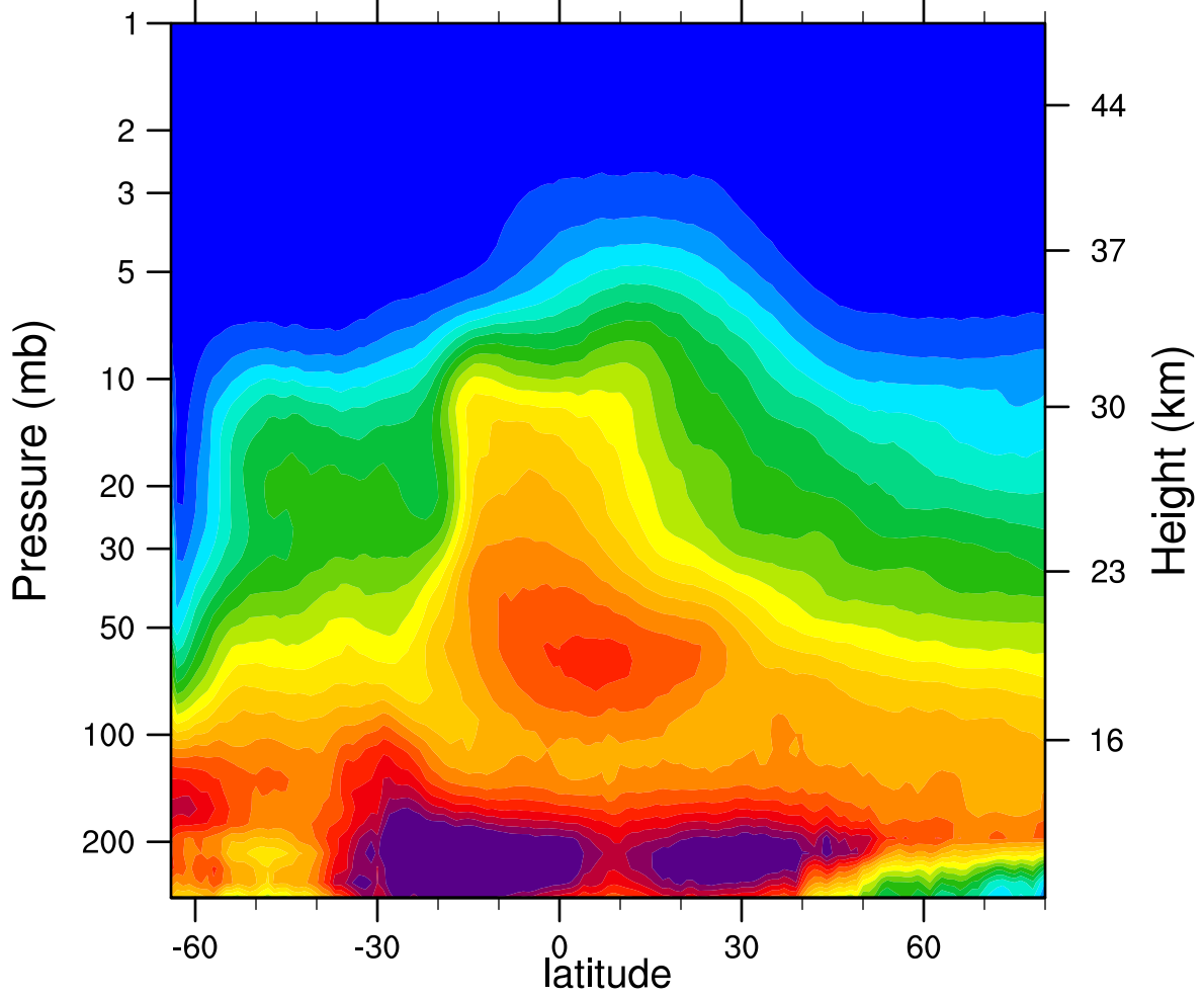
2005d226 N2O_Combined (ppbv)
