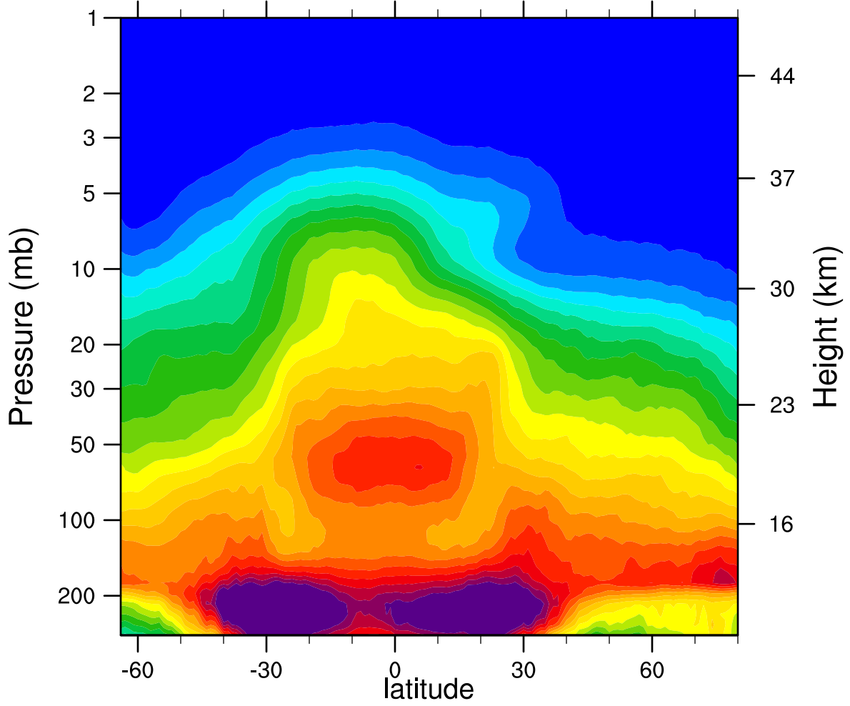
2006d074 N2O_Combined (ppbv)
