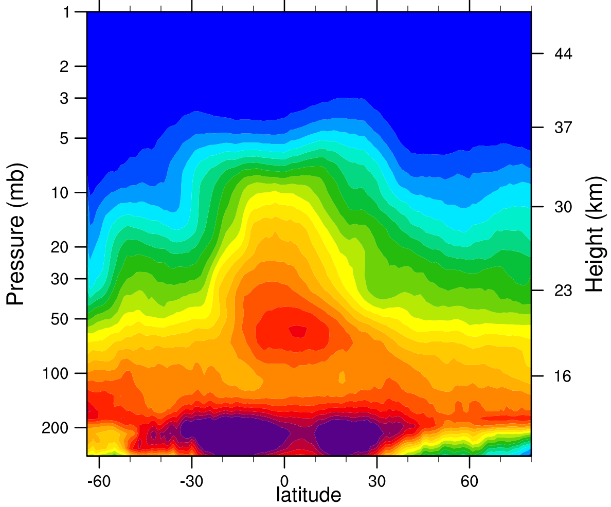
2005d142 N2O_Combined (ppbv)
