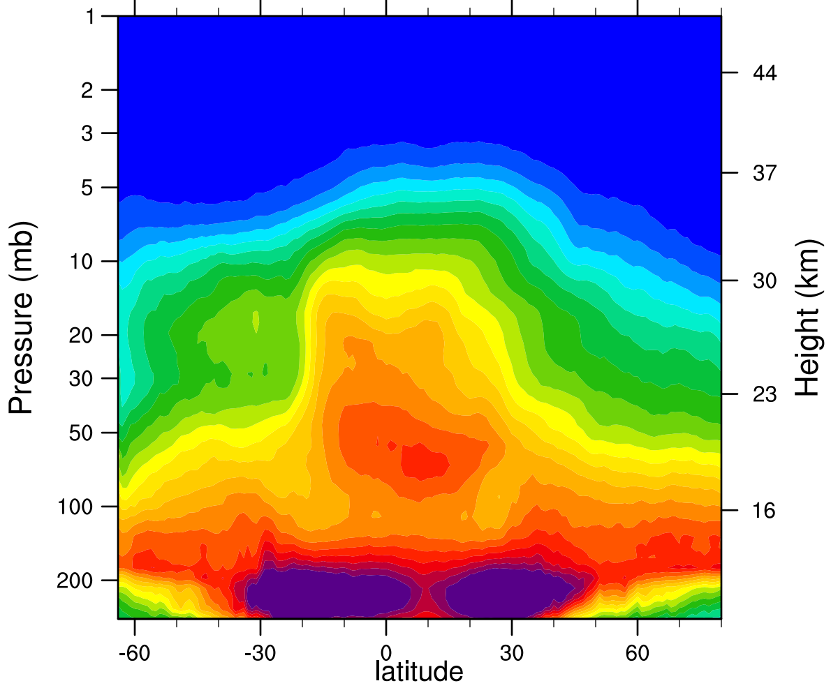
2007d282 N2O_Combined (ppbv)
