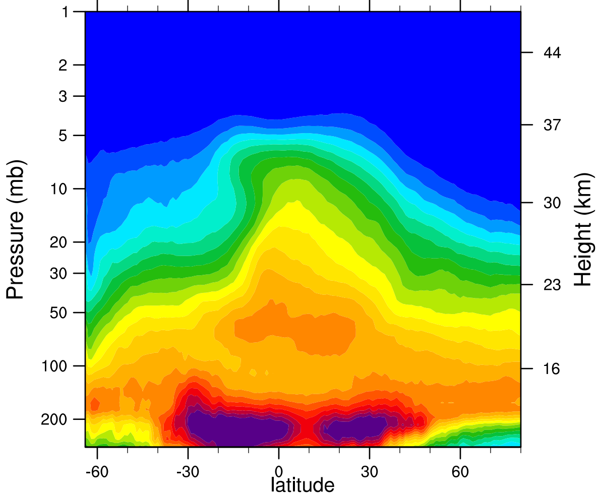
2006d272 N2O_Combined (ppbv)
