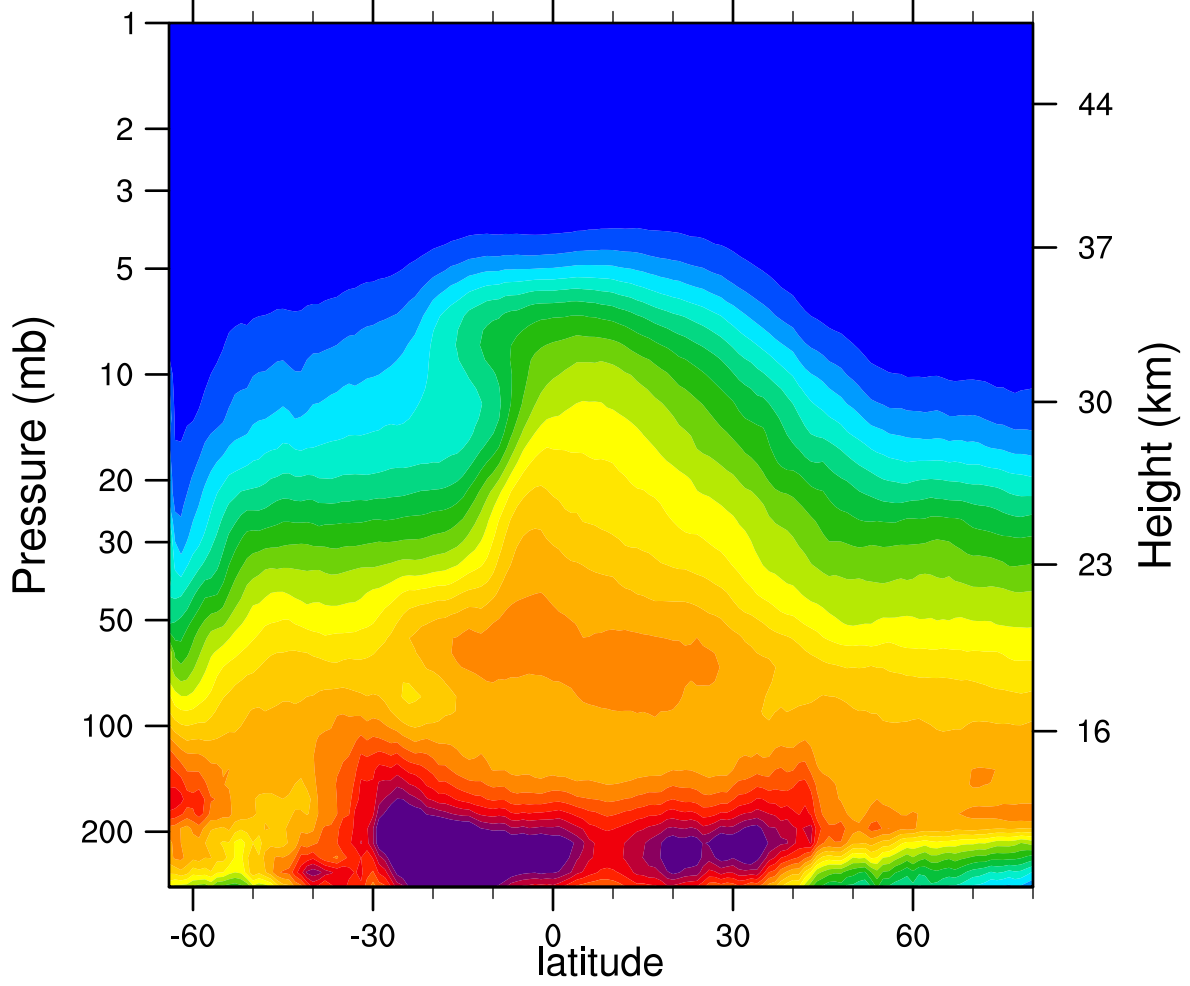
2006d255 N2O_Combined (ppbv)
