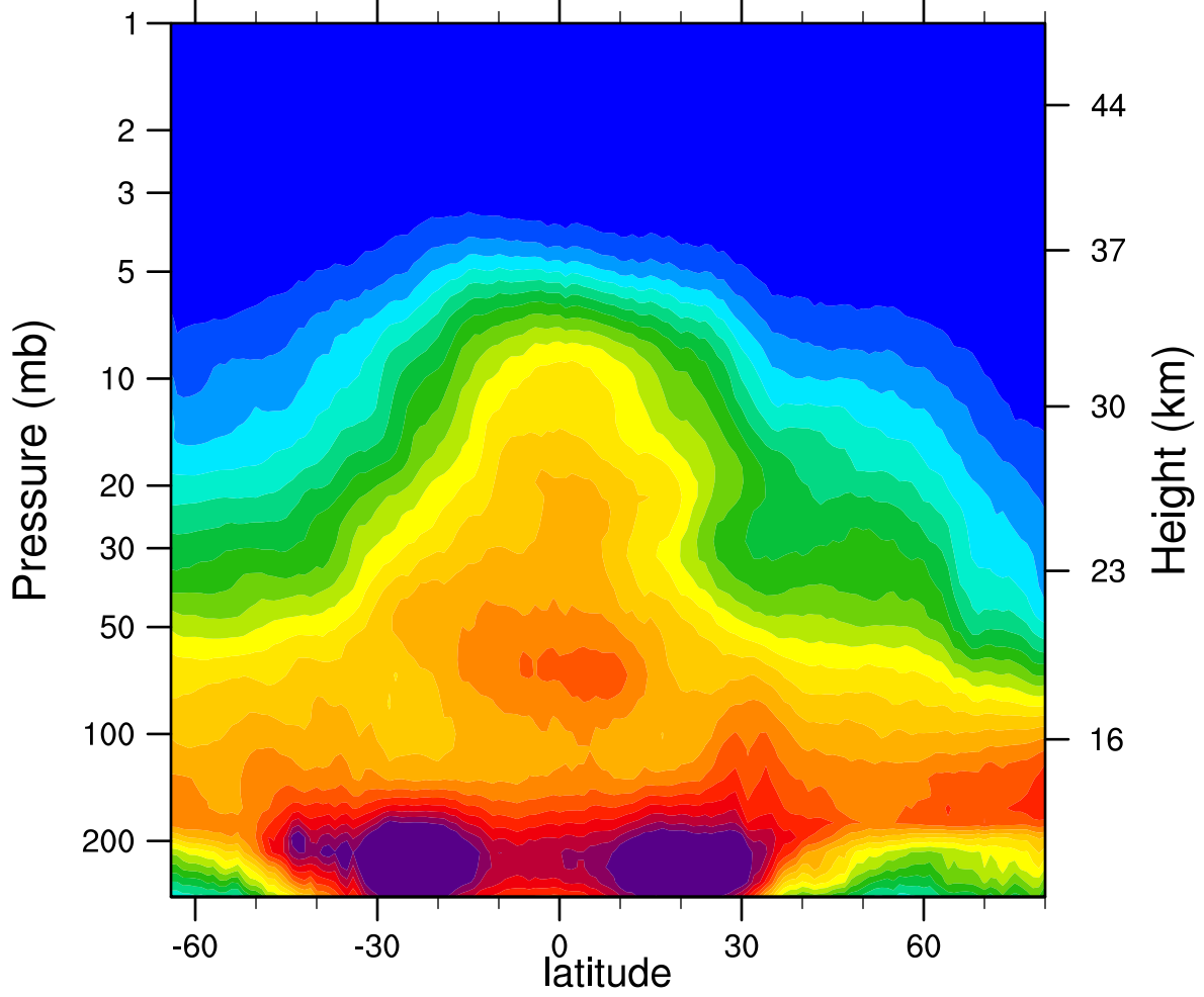
2007d066 N2O_Combined (ppbv)
