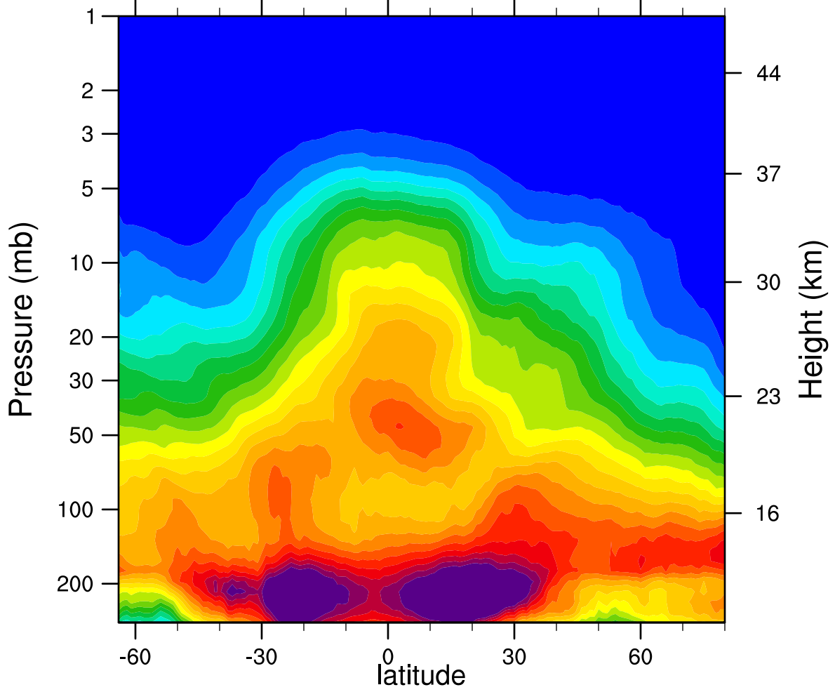
2005d064 N2O_Combined (ppbv)
