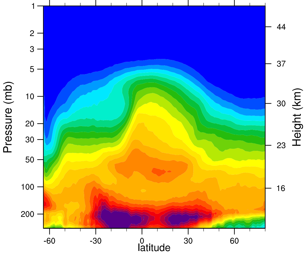
2006d245 N2O_Combined (ppbv)
