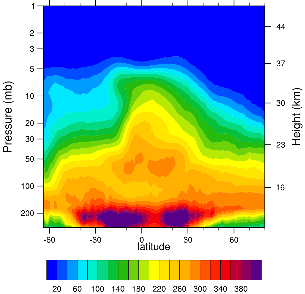
2006d288 N2O_Combined (ppbv)
