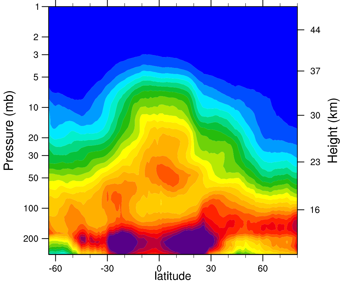
2005d054 N2O_Combined (ppbv)
