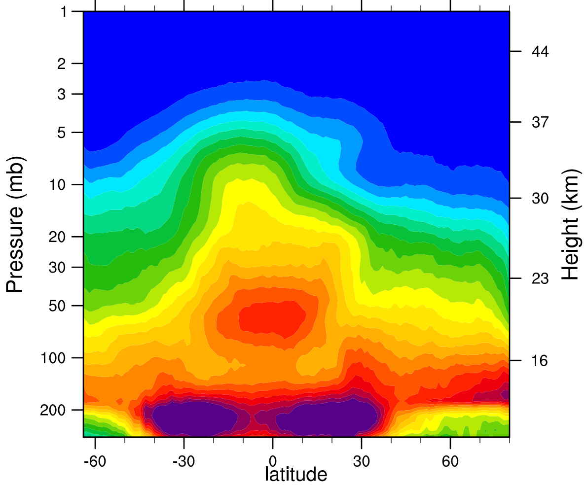
2006d065 N2O_Combined (ppbv)
