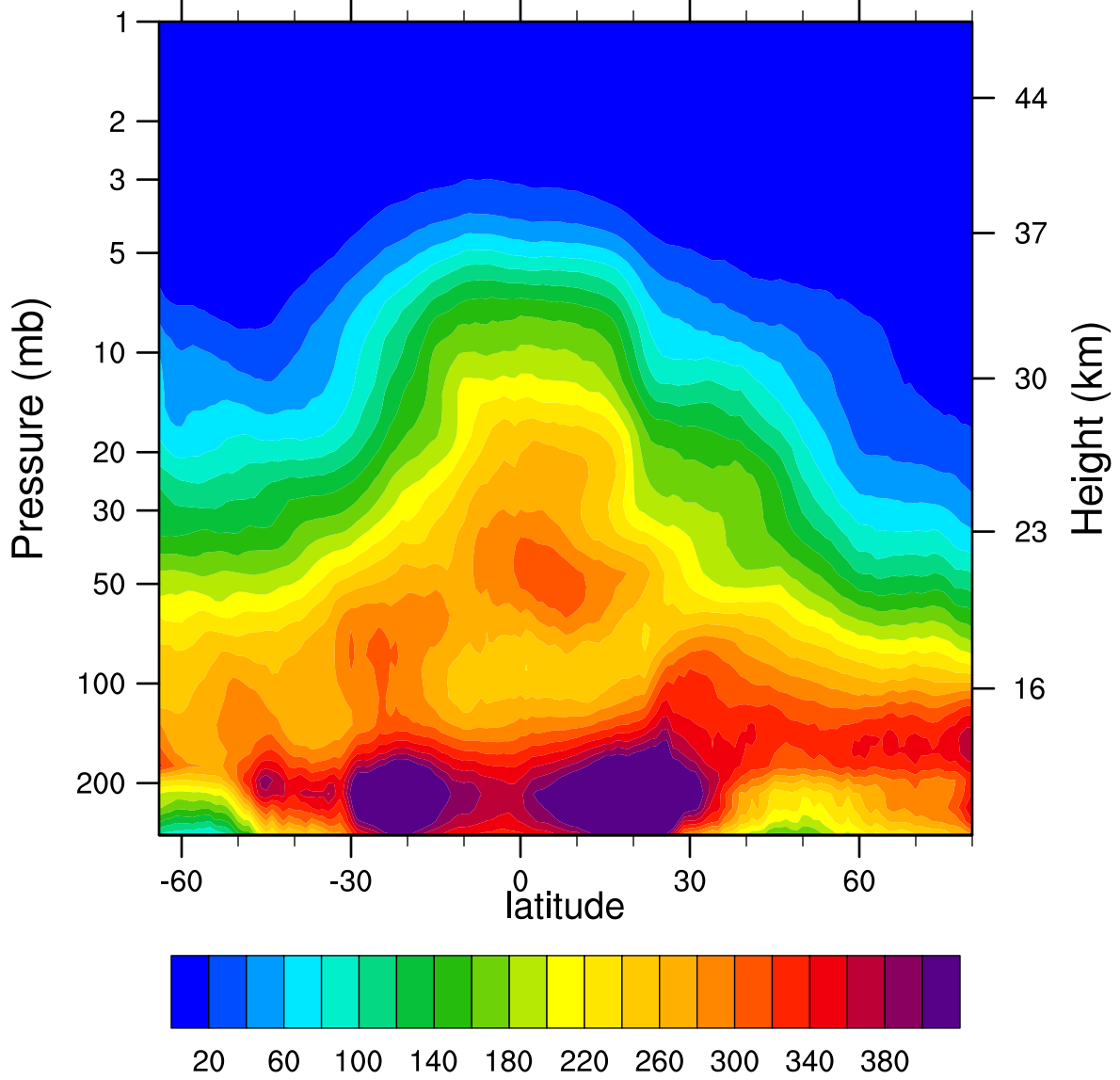
2005d053 N2O_Combined (ppbv)
