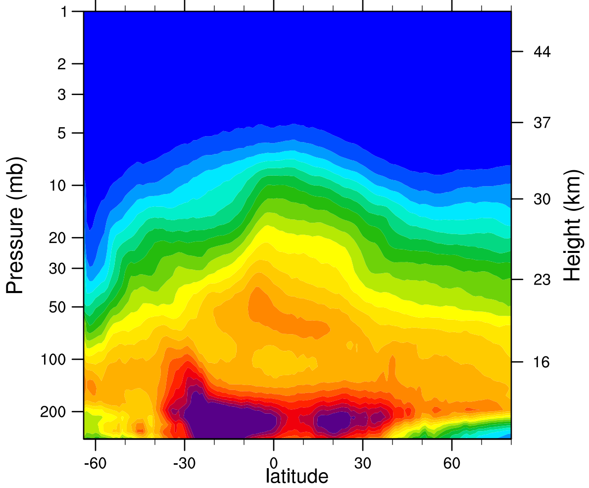
2006d185 N2O_Combined (ppbv)
