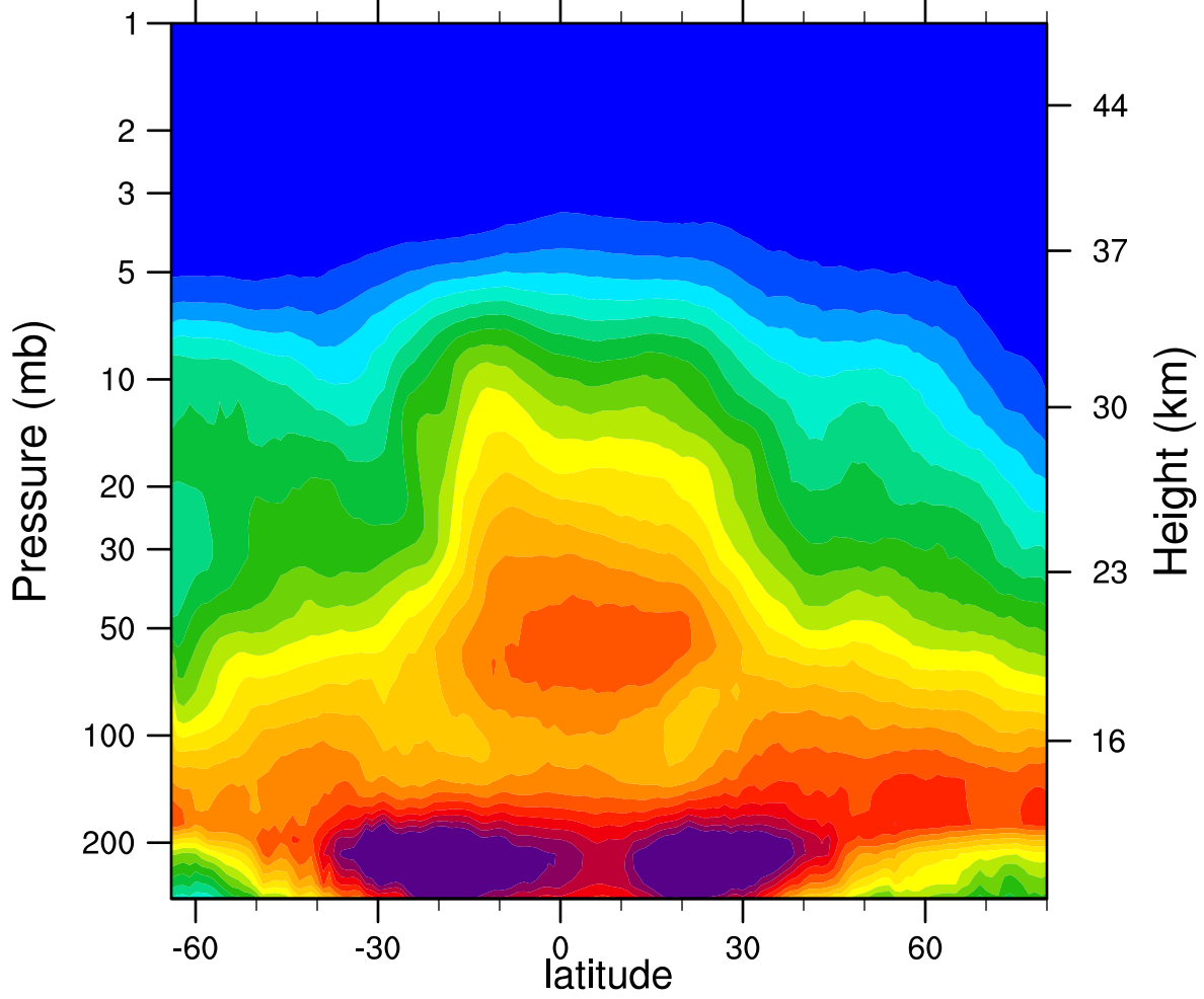
2005d312 N2O_Combined (ppbv)
