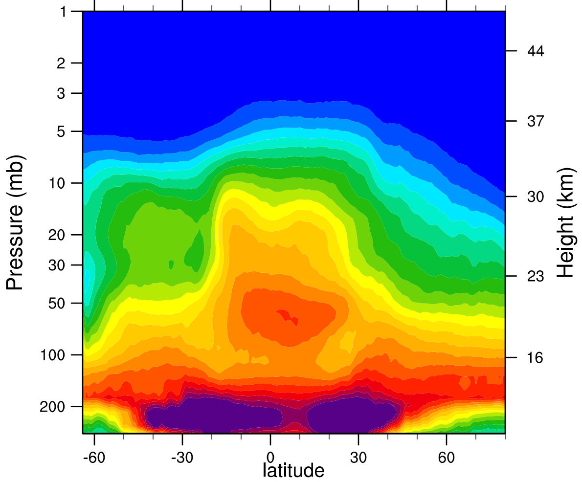
2007d297 N2O_Combined (ppbv)
