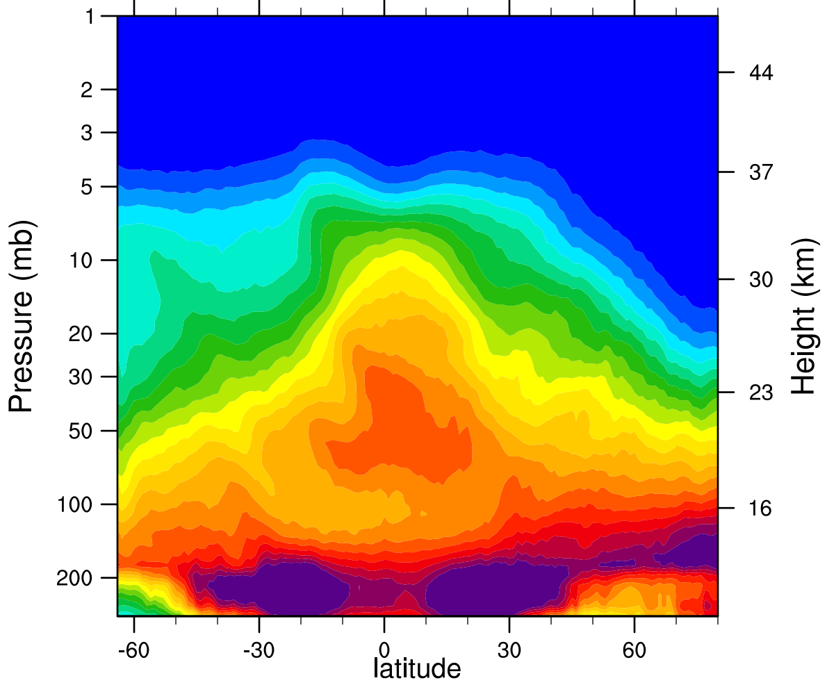
2006d334 N2O_Combined (ppbv)
