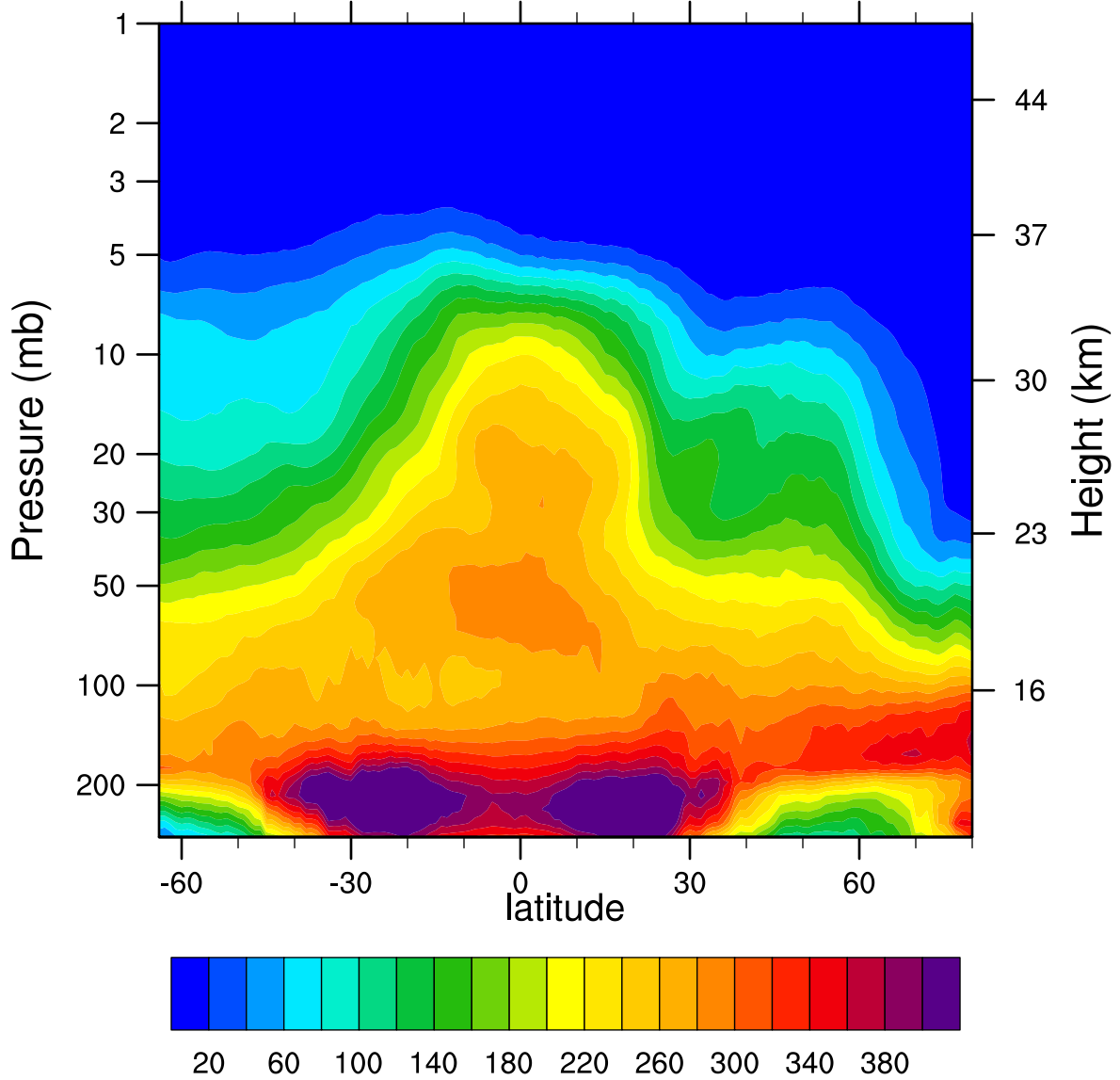
2007d014 N2O_Combined (ppbv)
