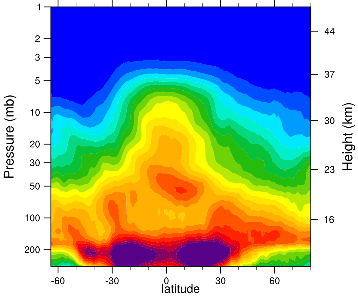
2005d085 N2O_Combined (ppbv)
