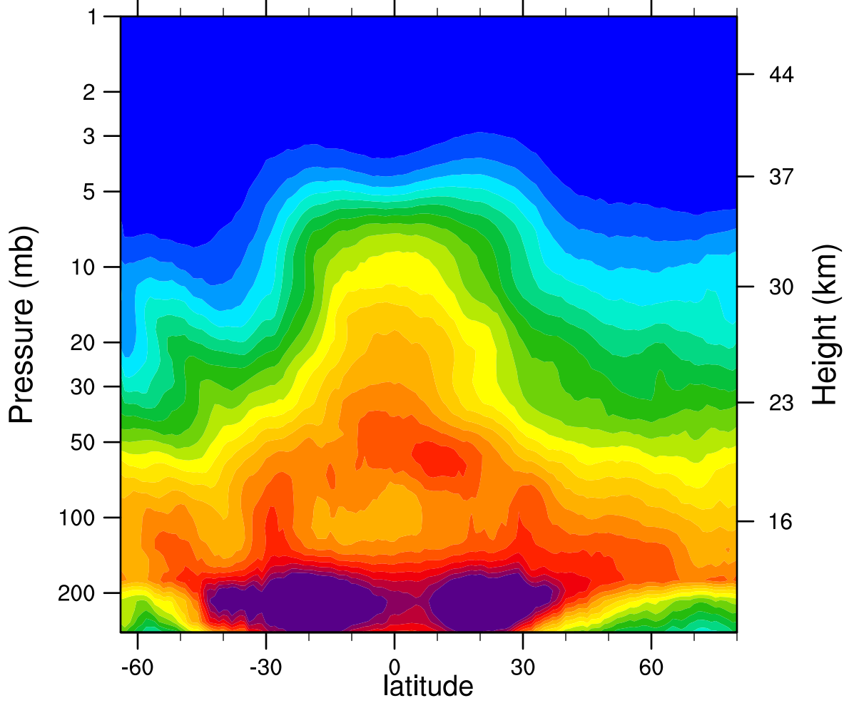
2005d109 N2O_Combined (ppbv)
