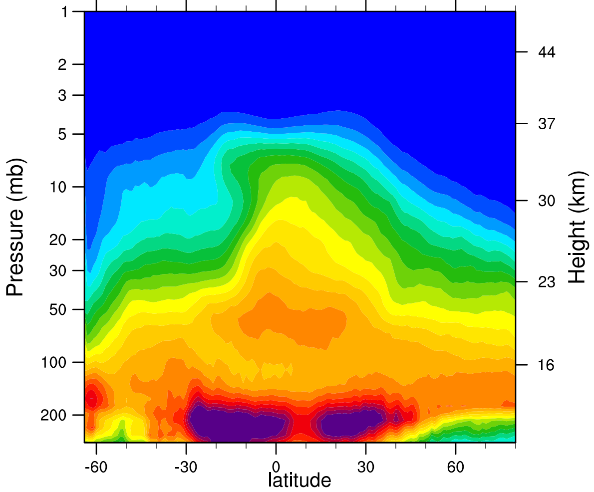
2006d279 N2O_Combined (ppbv)
