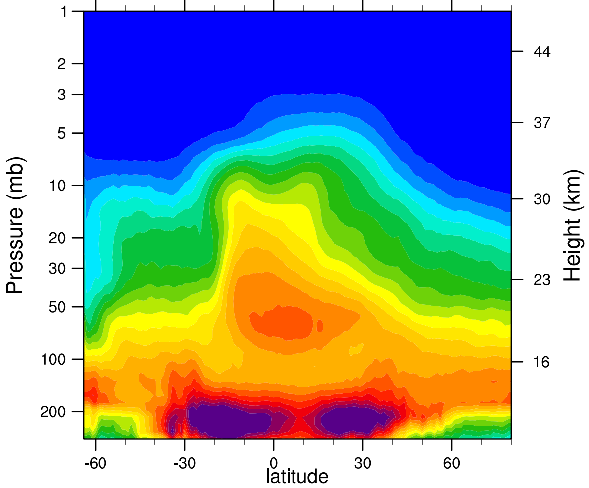
2005d268 N2O_Combined (ppbv)
