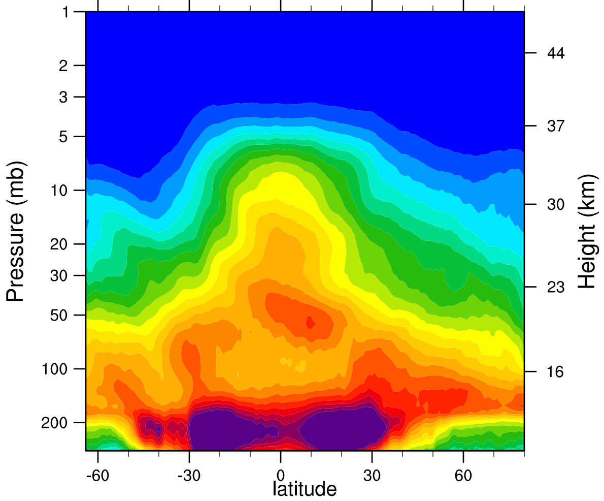
2005d088 N2O_Combined (ppbv)
