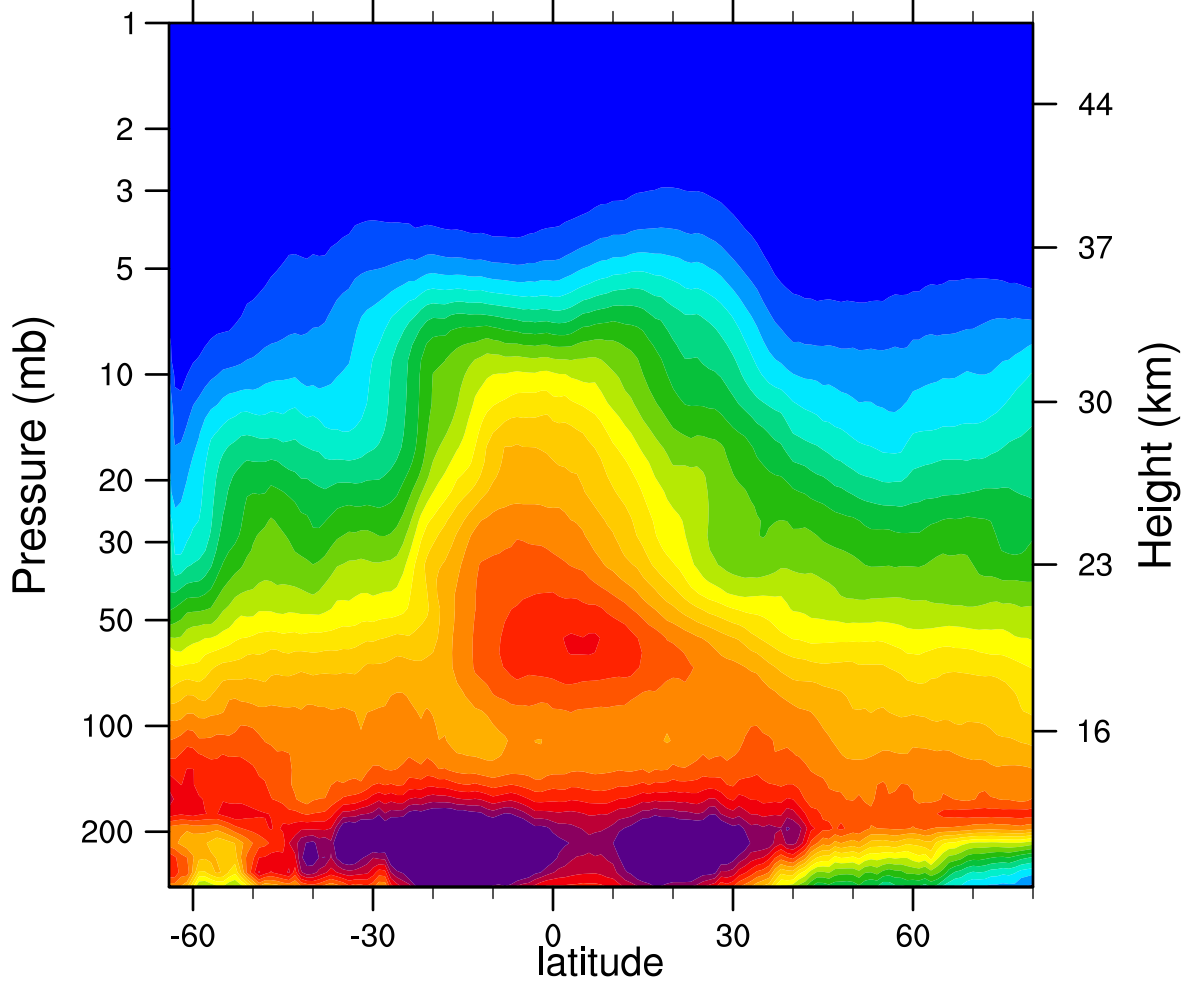
2005d147 N2O_Combined (ppbv)
