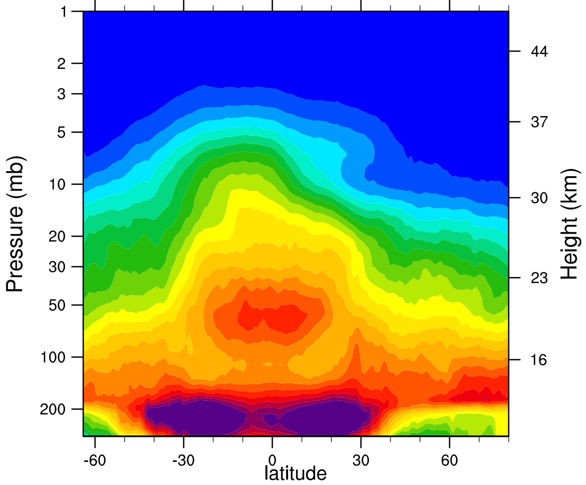
2006d086 N2O_Combined (ppbv)
