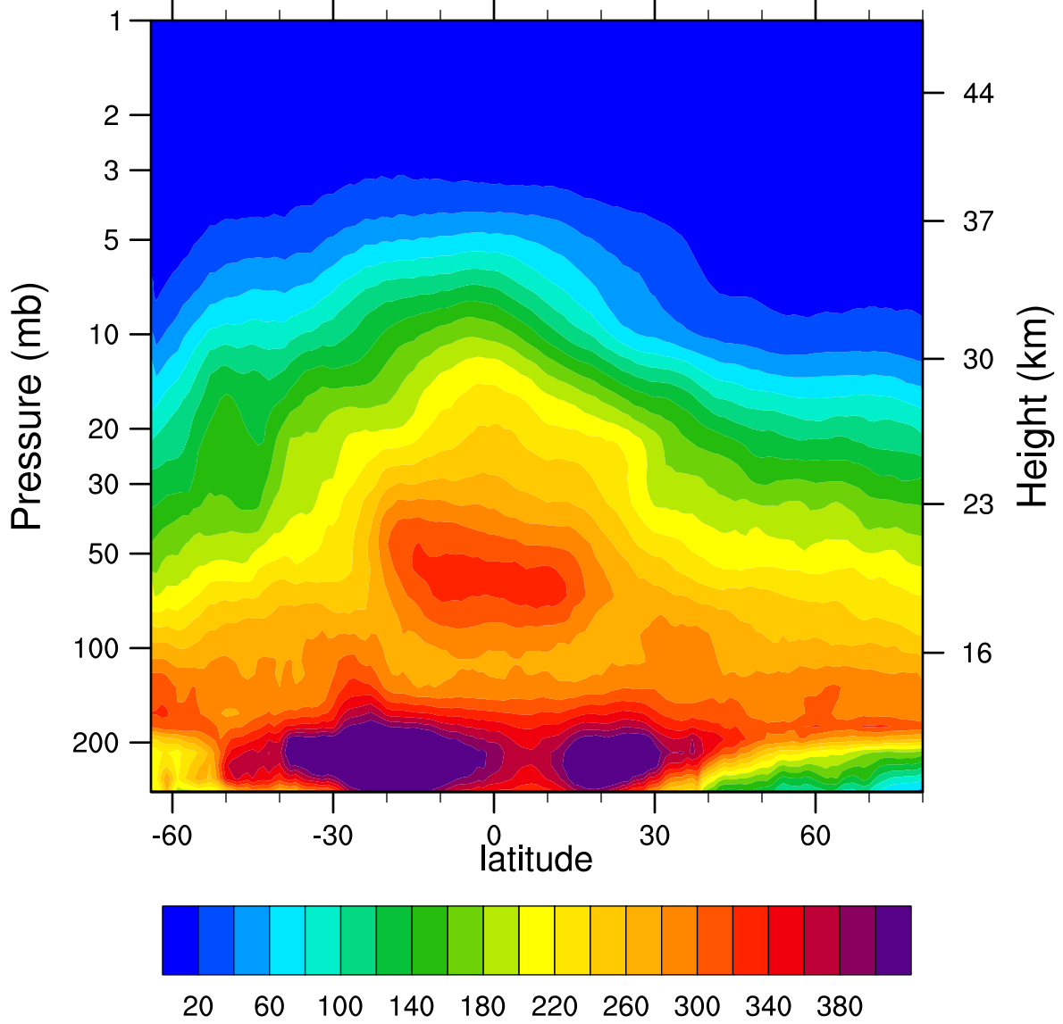
2006d131 N2O_Combined (ppbv)
