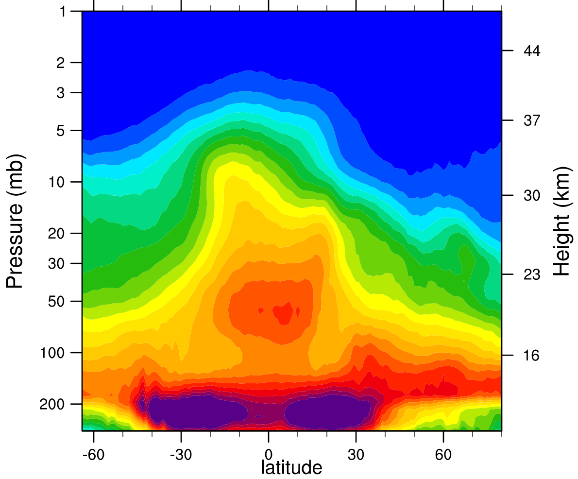
2006d027 N2O_Combined (ppbv)
