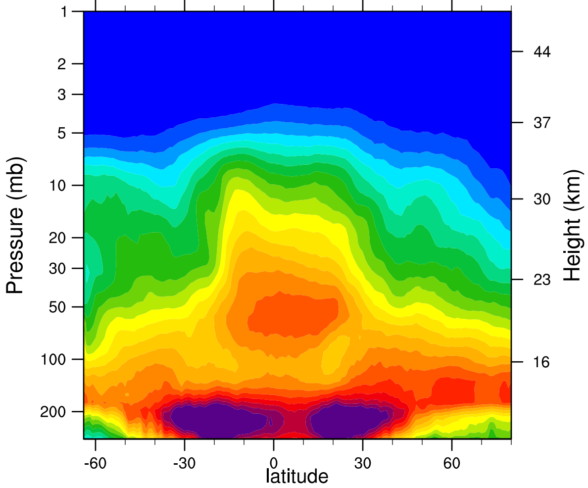
2005d311 N2O_Combined (ppbv)
