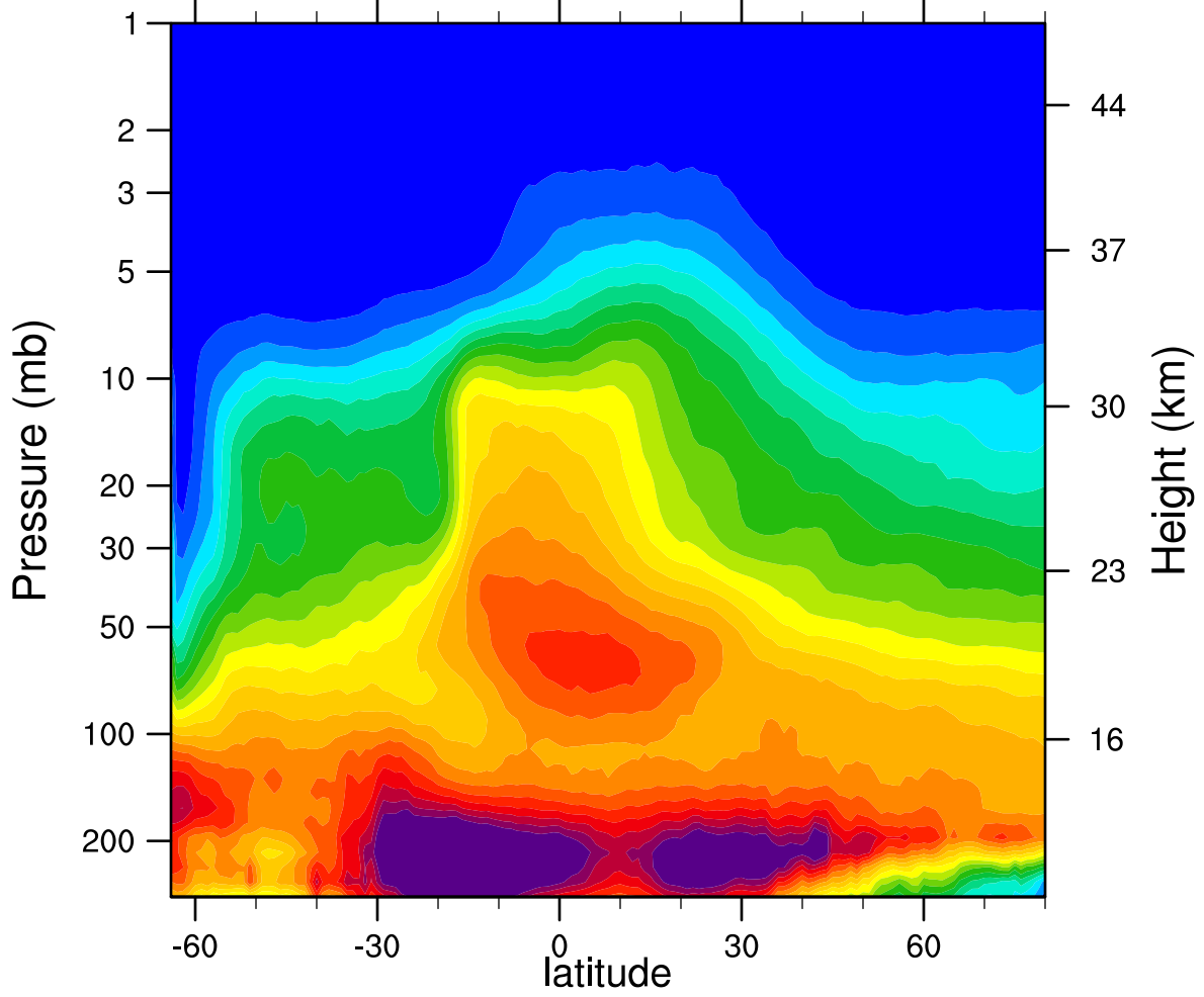
2005d221 N2O_Combined (ppbv)
