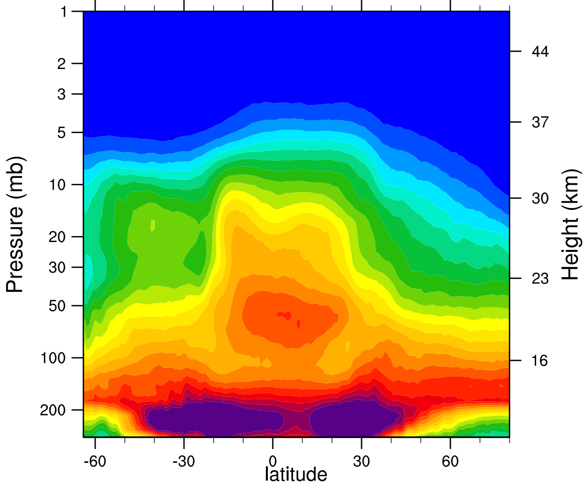
2007d299 N2O_Combined (ppbv)
