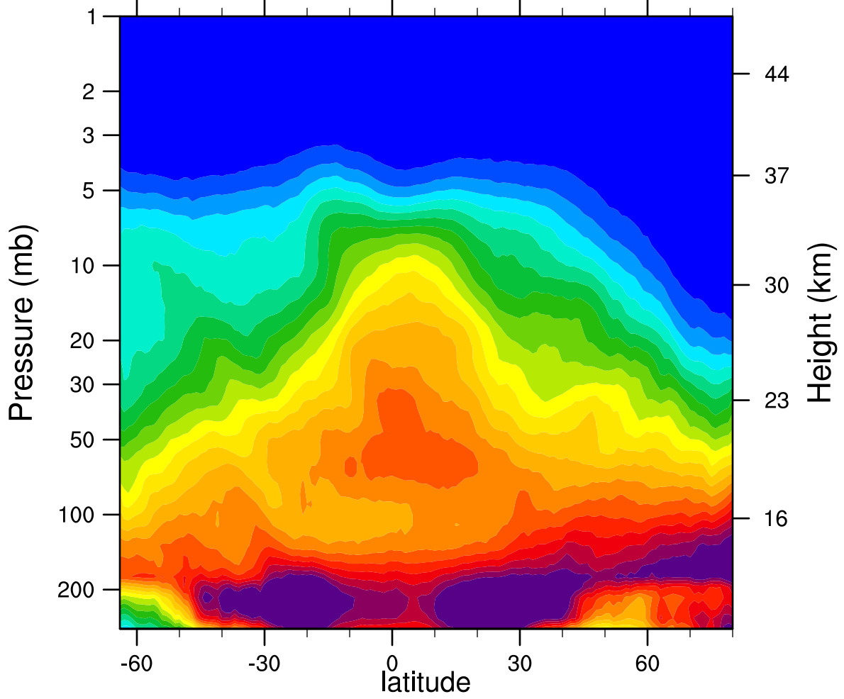
2006d337 N2O_Combined (ppbv)
