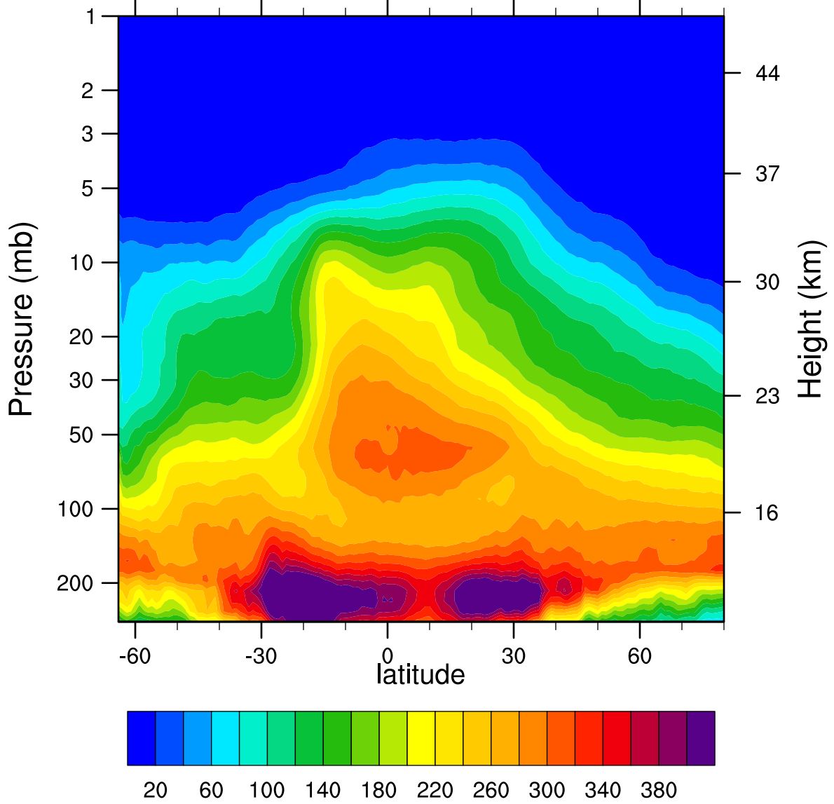
2005d279 N2O_Combined (ppbv)
