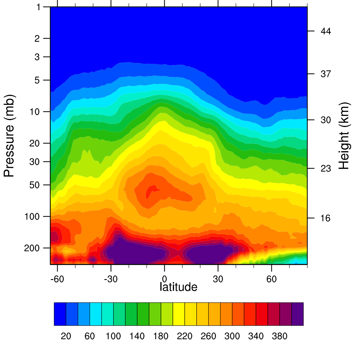
2006d161 N2O_Combined (ppbv)
