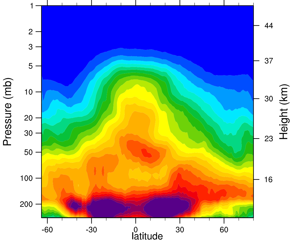
2005d078 N2O_Combined (ppbv)
