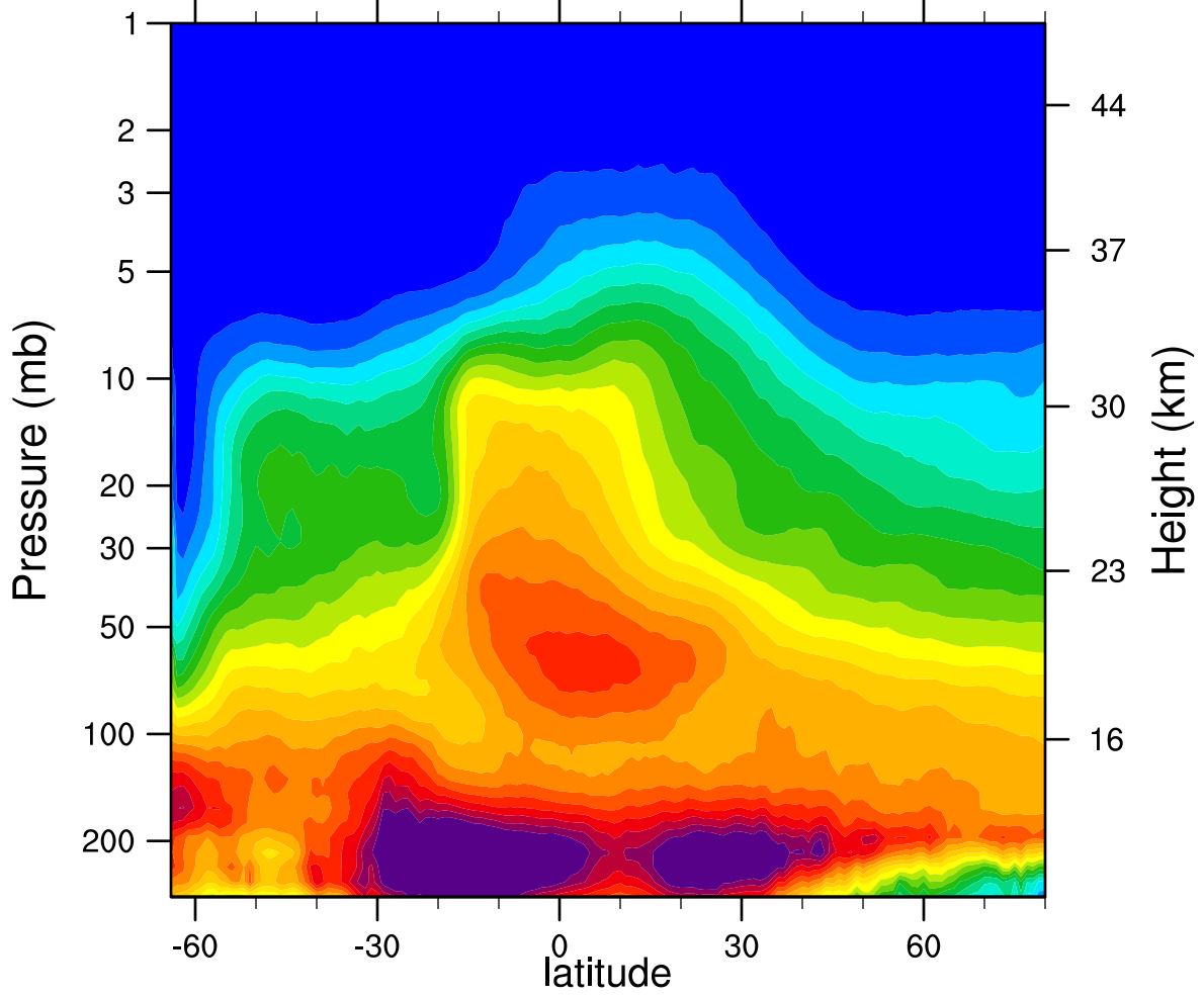
2005d222 N2O_Combined (ppbv)
