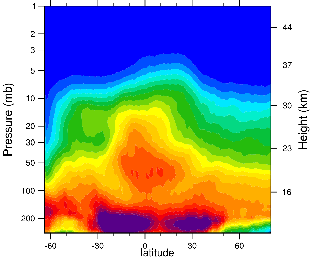
2007d213 N2O_Combined (ppbv)
