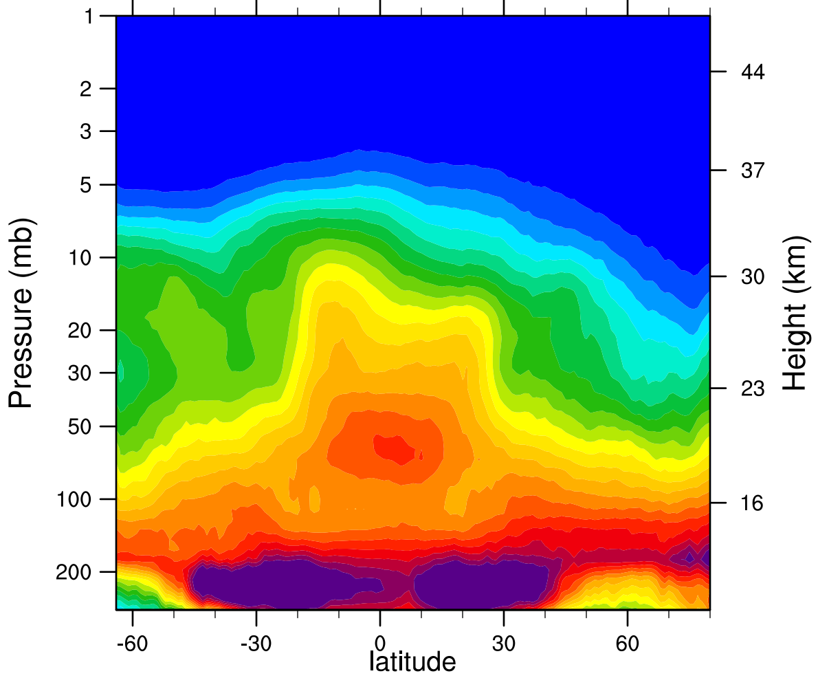
2007d337 N2O_Combined (ppbv)
