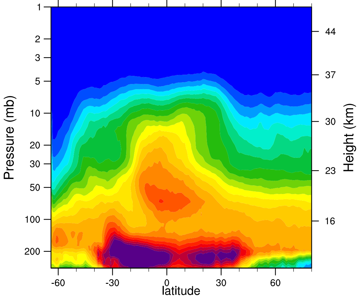
2007d184 N2O_Combined (ppbv)
