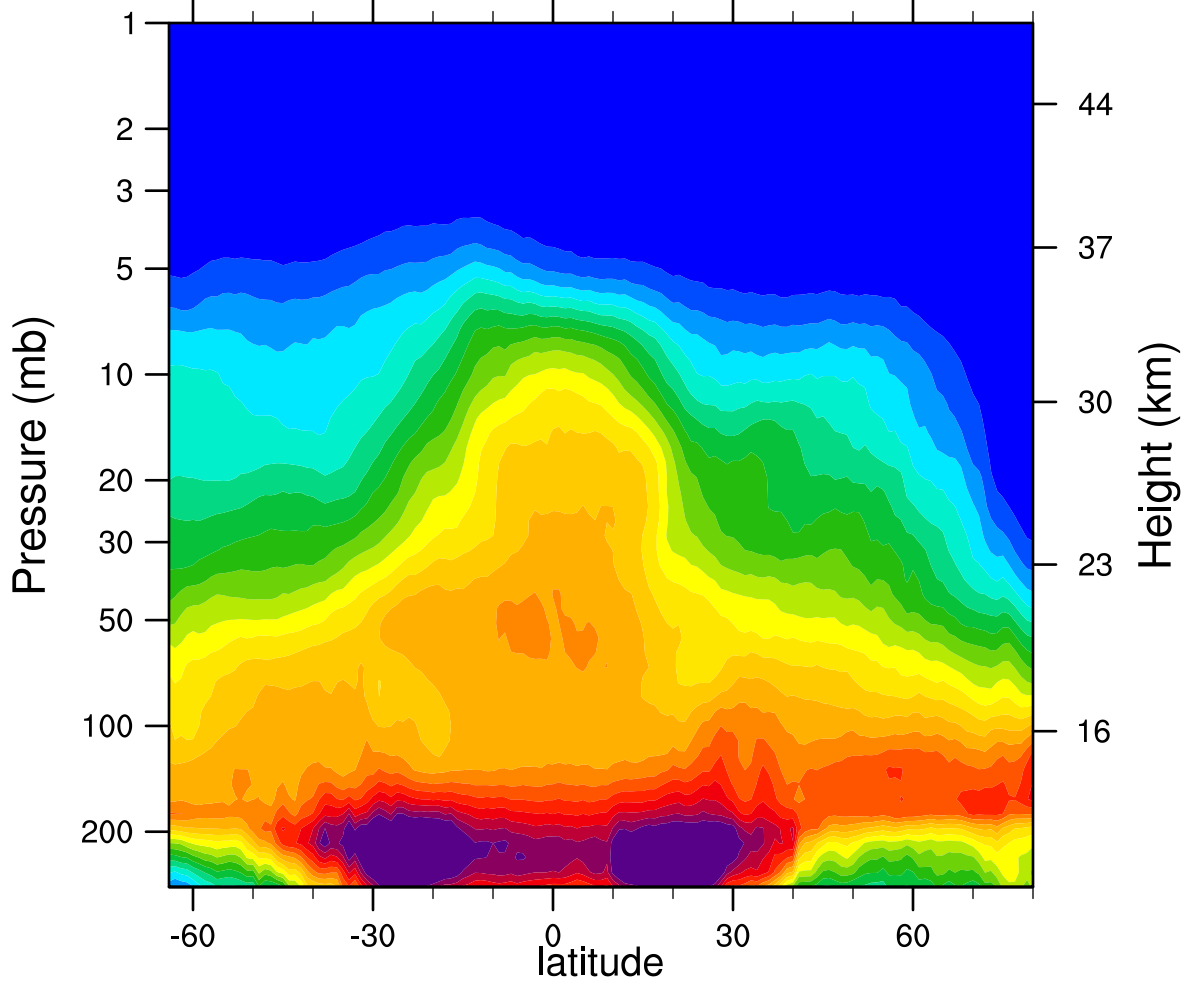
2006d364 N2O_Combined (ppbv)
