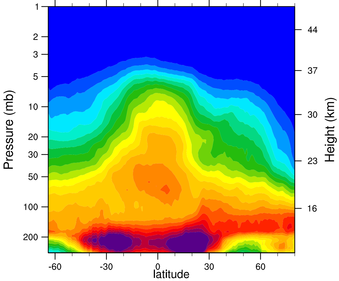
2007d042 N2O_Combined (ppbv)
