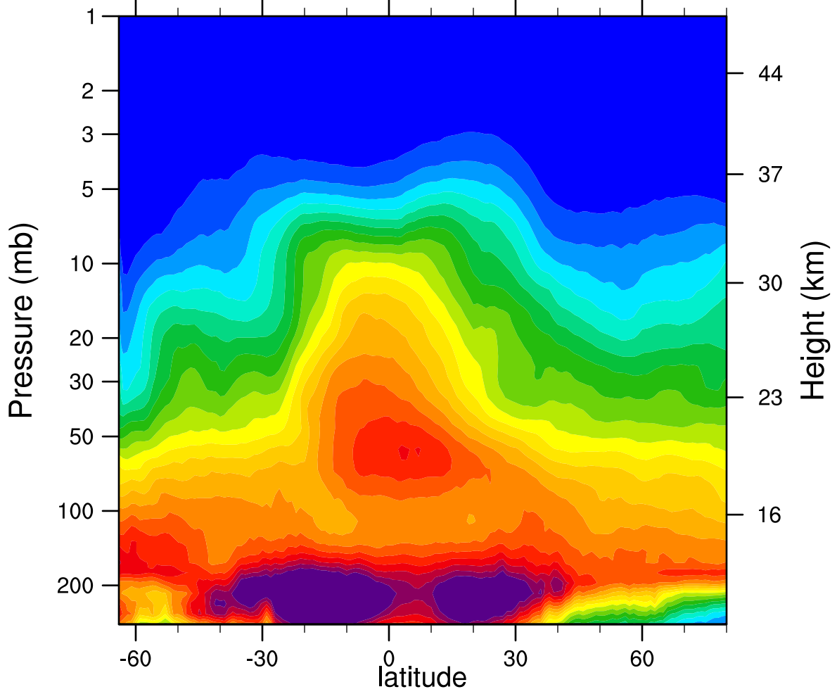
2005d148 N2O_Combined (ppbv)
