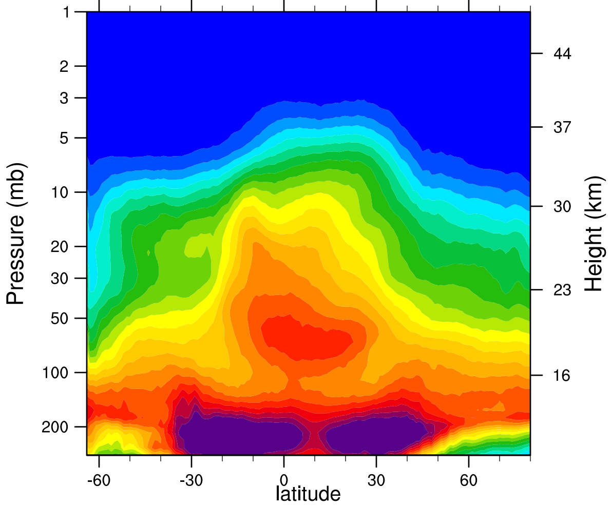
2007d262 N2O_Combined (ppbv)
