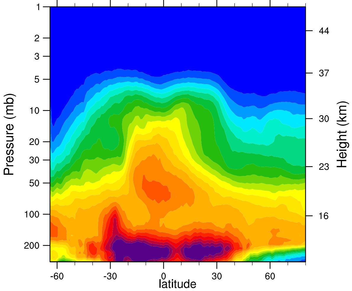
2007d167 N2O_Combined (ppbv)
