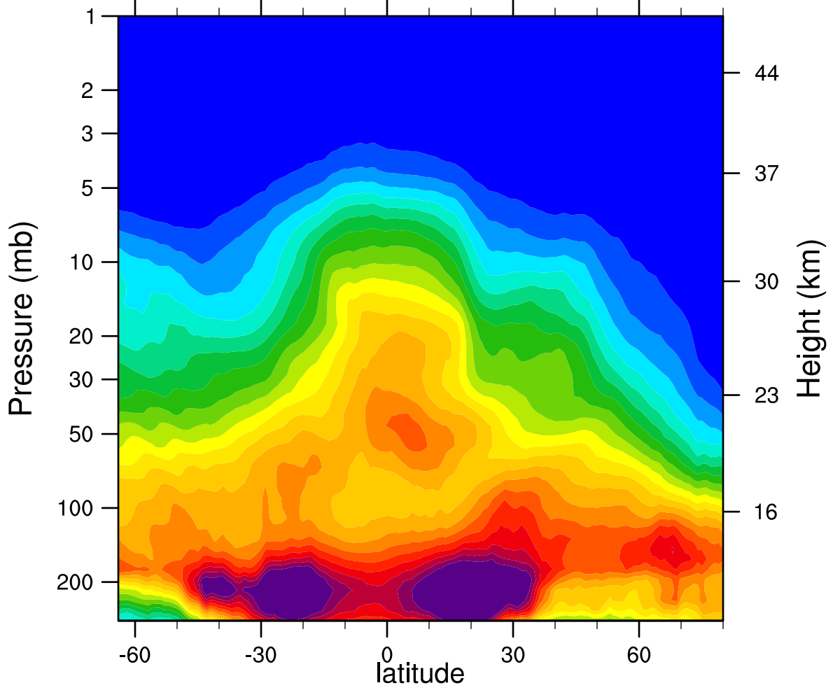
2005d041 N2O_Combined (ppbv)
