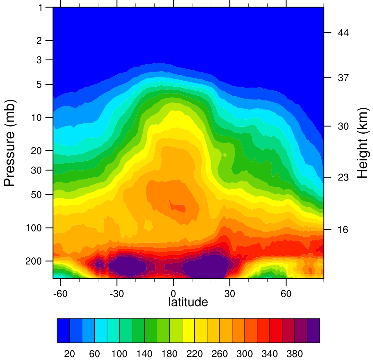
2007d041 N2O_Combined (ppbv)
