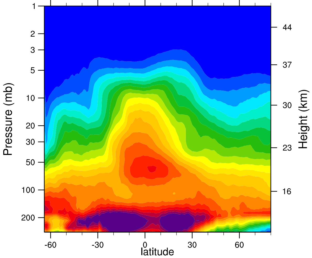
2005d144 N2O_Combined (ppbv)
