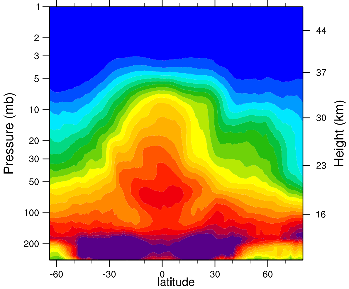
2007d096 N2O_Combined (ppbv)
