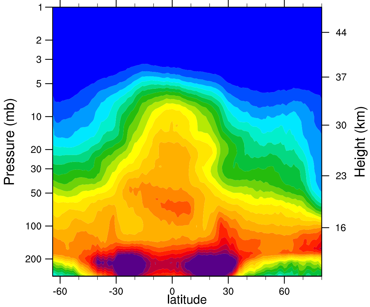
2007d062 N2O_Combined (ppbv)
