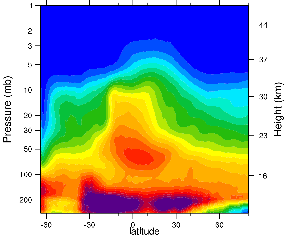
2005d217 N2O_Combined (ppbv)
