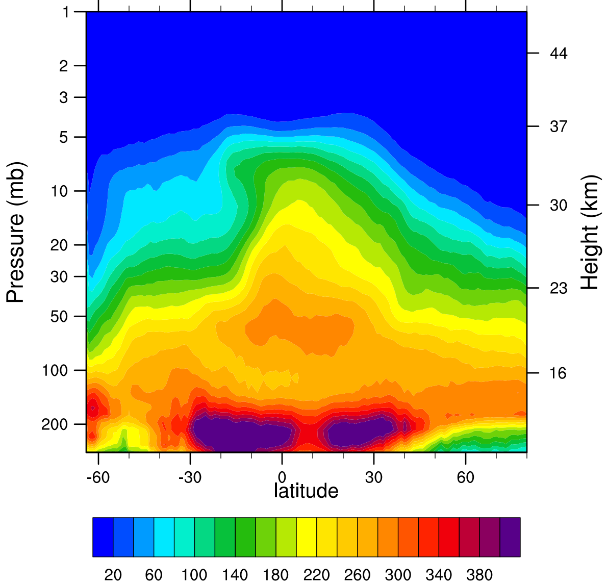
2006d280 N2O_Combined (ppbv)
