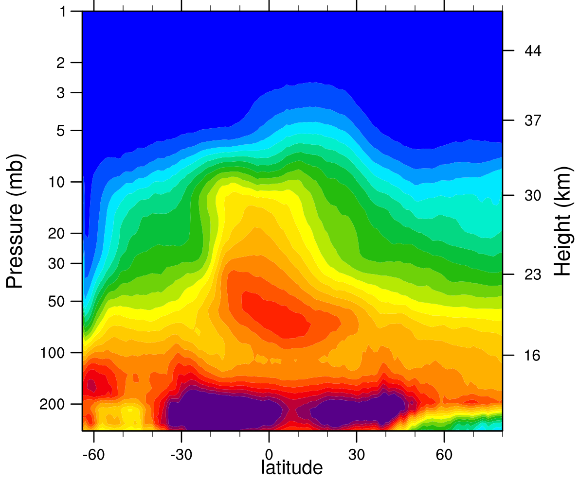
2005d201 N2O_Combined (ppbv)
