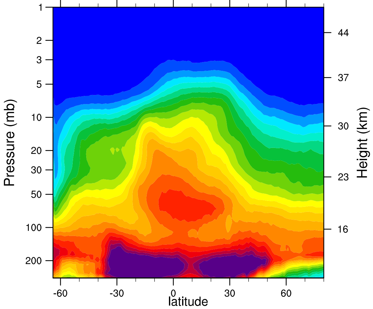
2007d254 N2O_Combined (ppbv)
