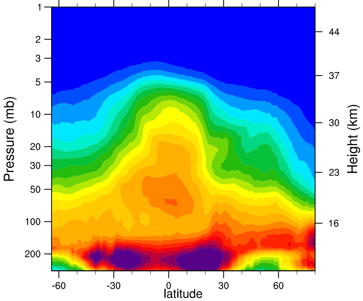
2007d039 N2O_Combined (ppbv)
