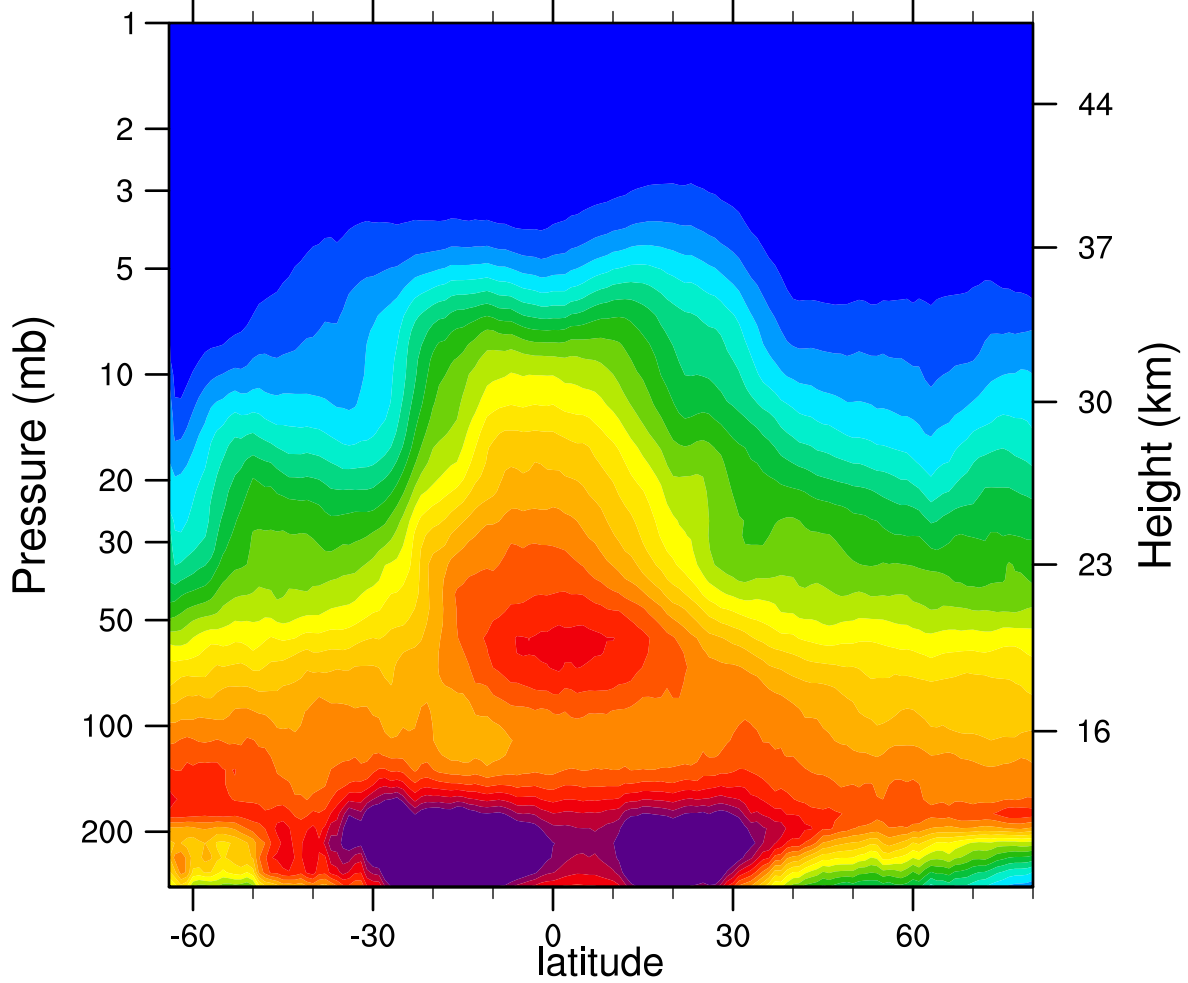
2005d135 N2O_Combined (ppbv)
