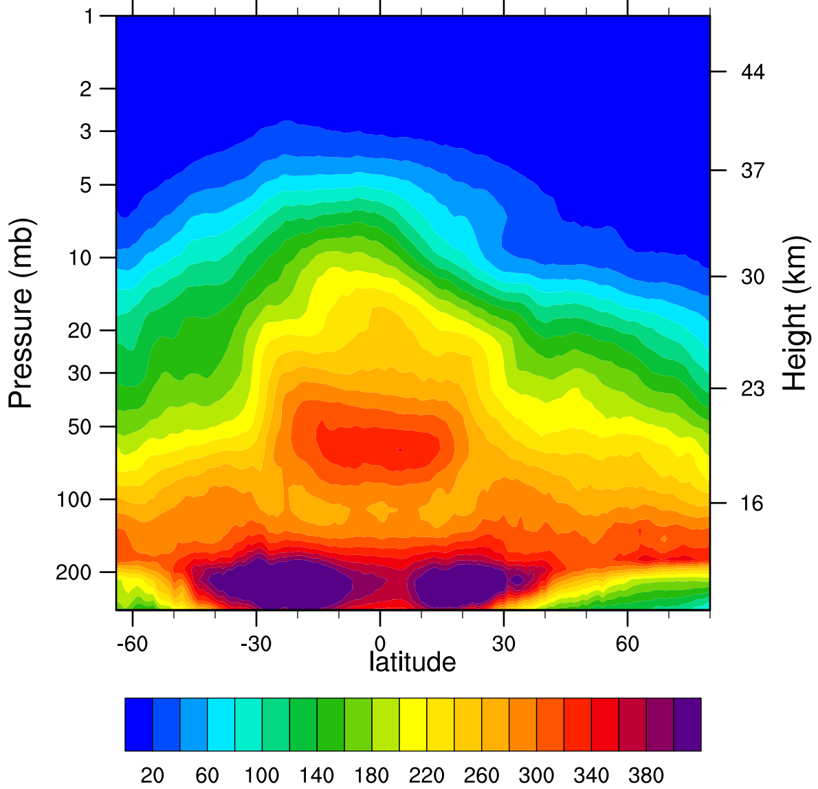
2006d110 N2O_Combined (ppbv)
