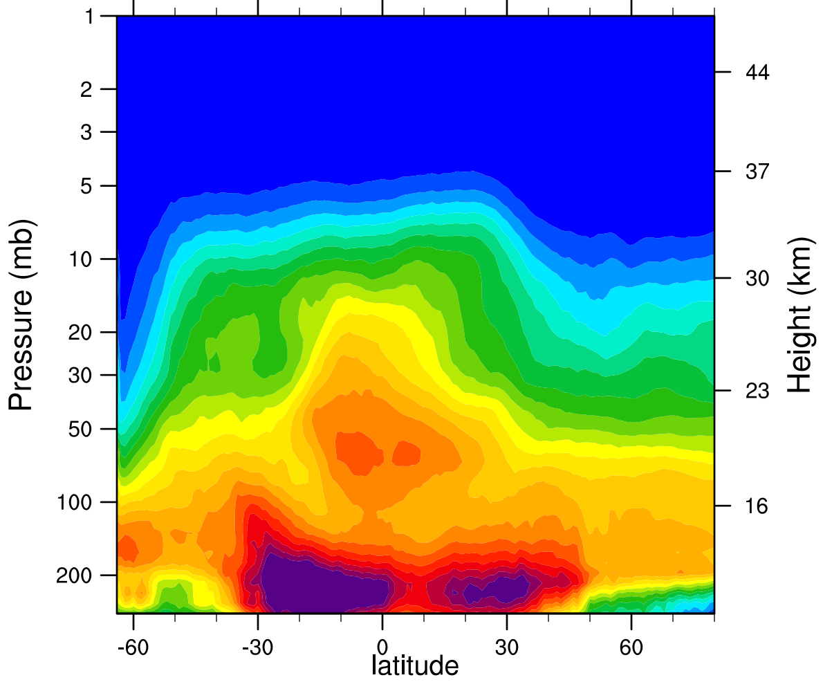
2007d201 N2O_Combined (ppbv)
