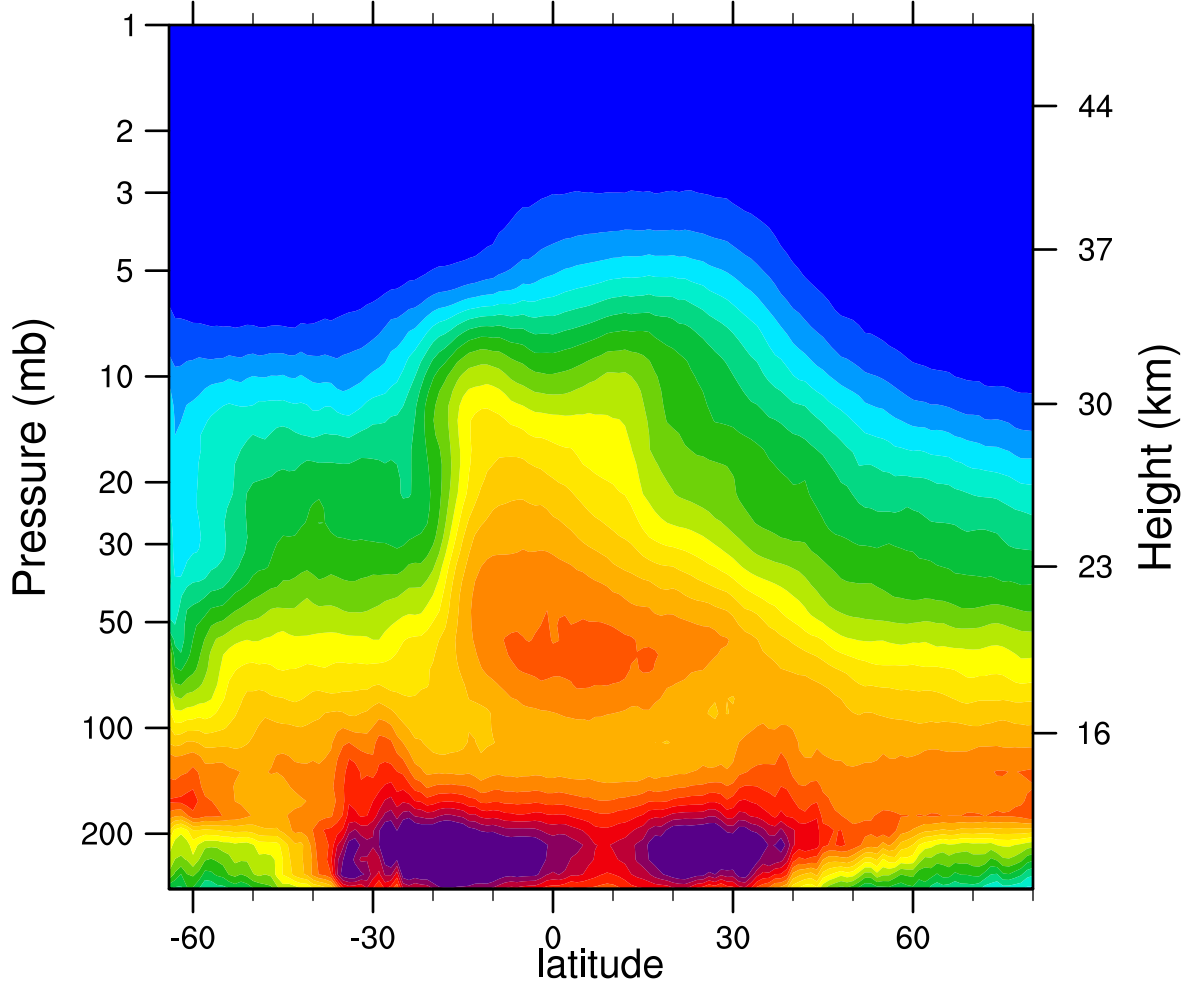
2005d269 N2O_Combined (ppbv)
