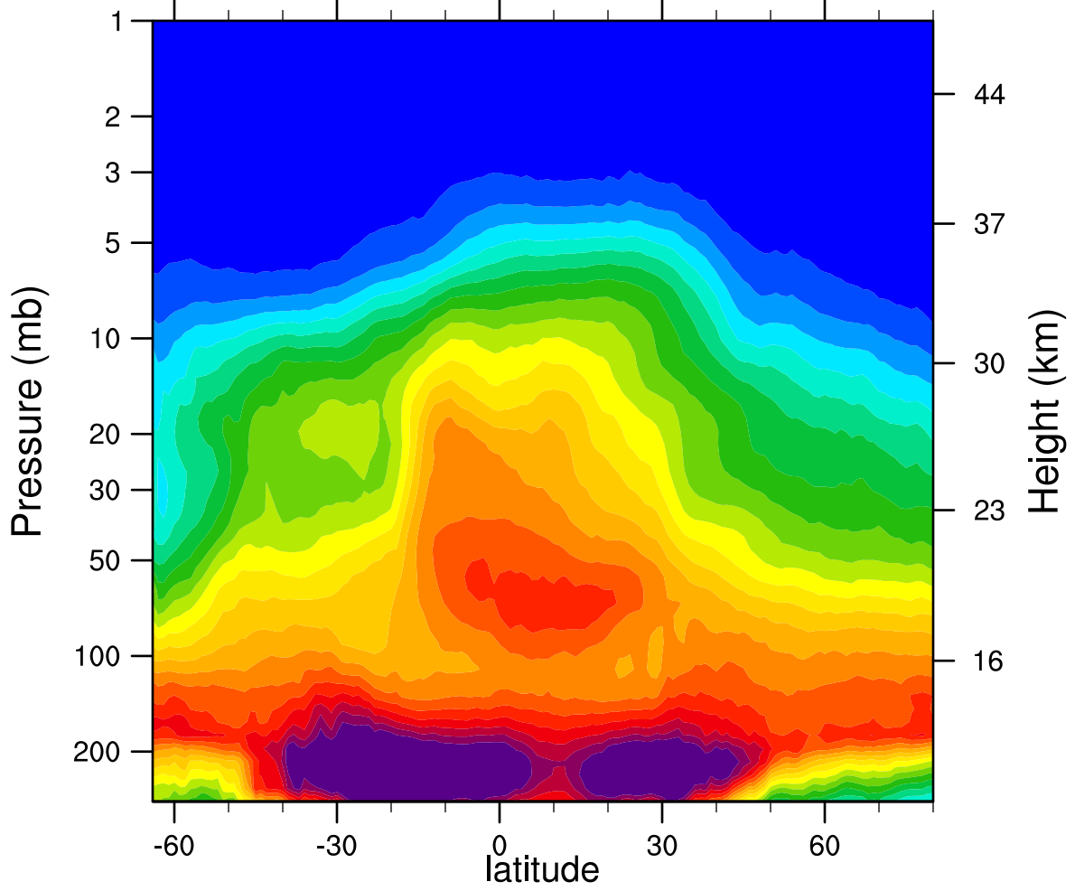
2007d273 N2O_Combined (ppbv)
