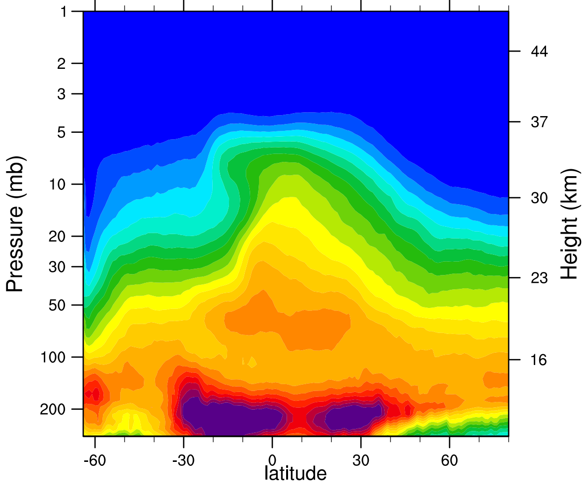
2006d265 N2O_Combined (ppbv)
