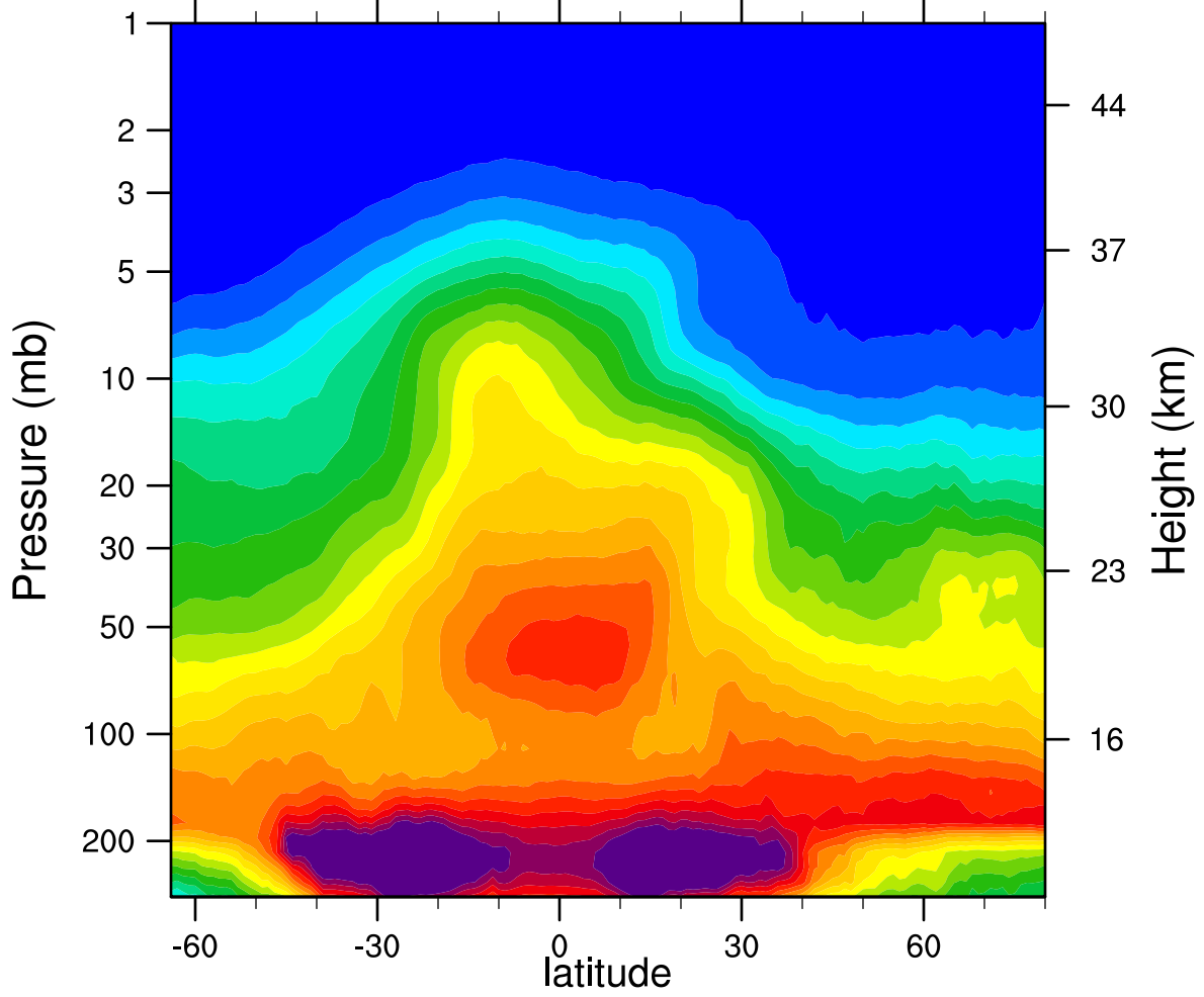
2006d044 N2O_Combined (ppbv)
