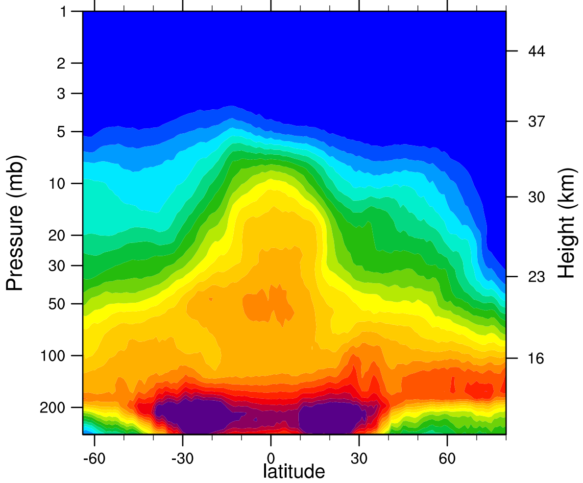
2006d365 N2O_Combined (ppbv)
