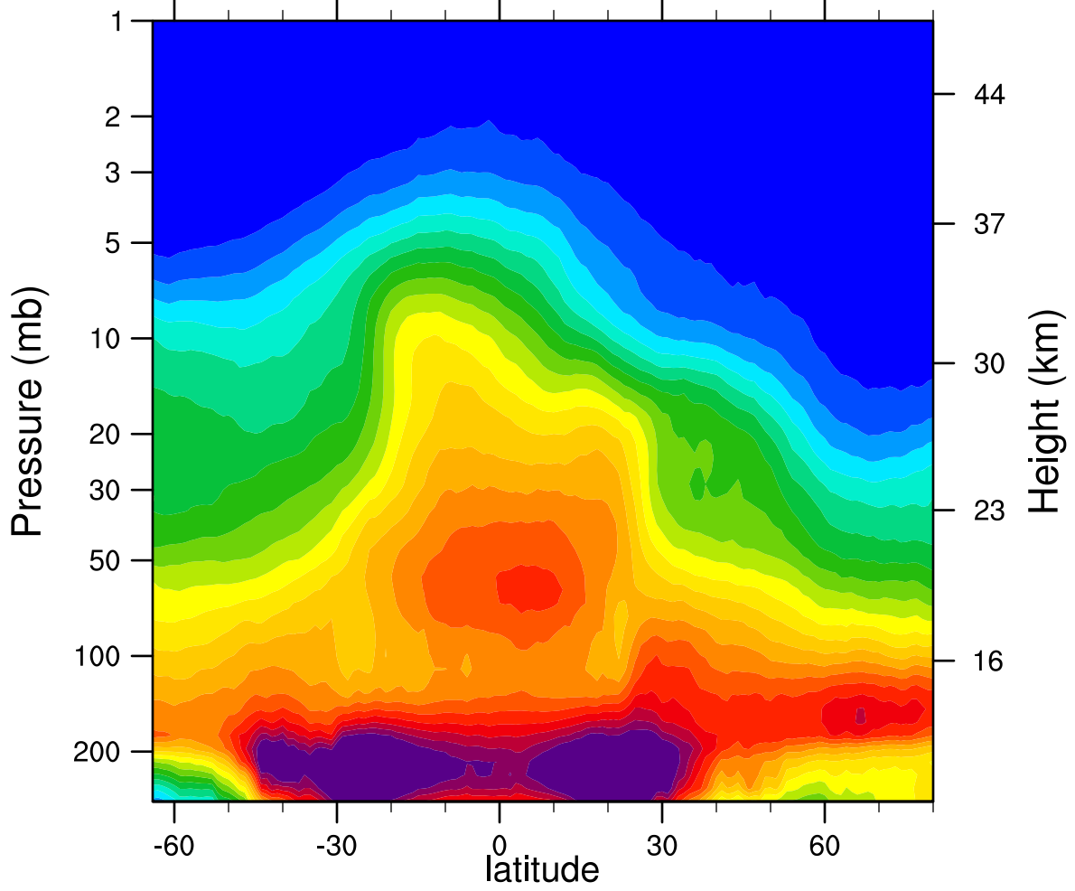
2006d014 N2O_Combined (ppbv)
