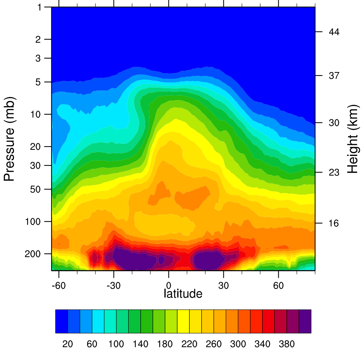
2006d294 N2O_Combined (ppbv)
