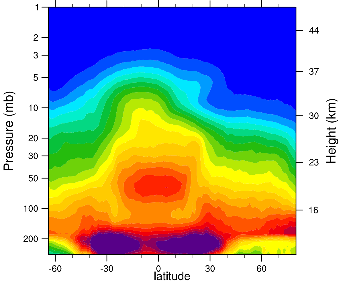
2006d072 N2O_Combined (ppbv)
