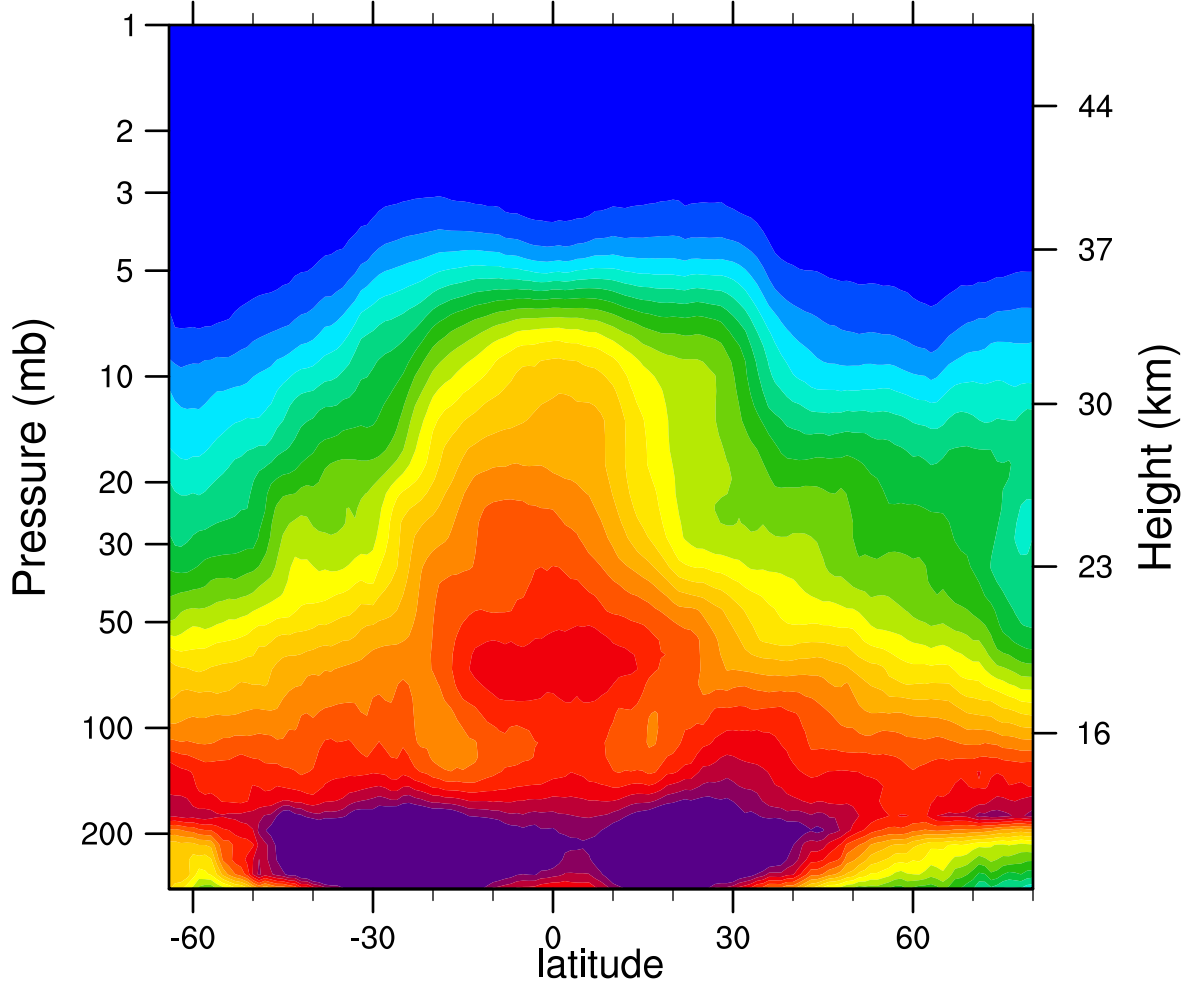
2007d110 N2O_Combined (ppbv)
