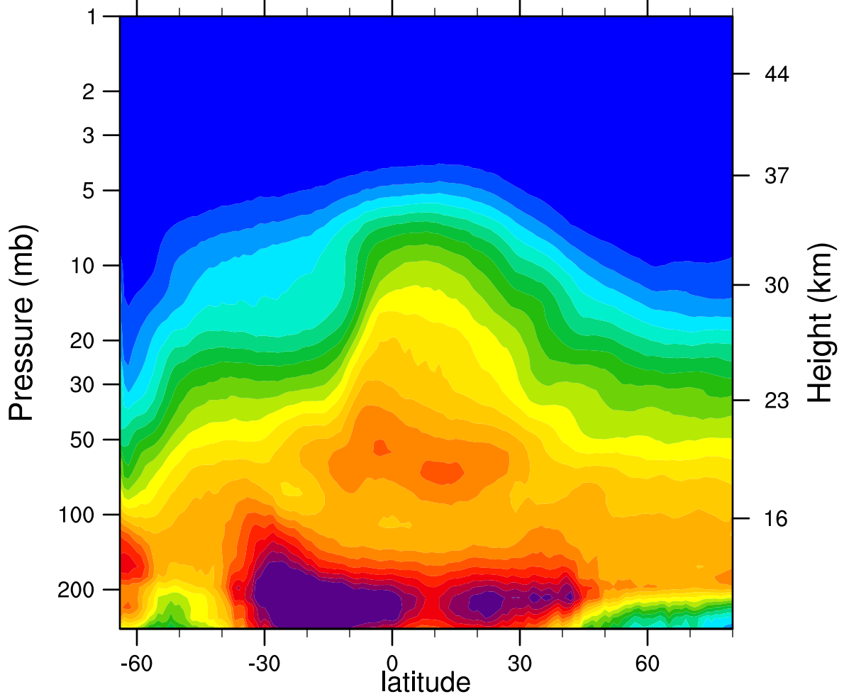
2006d235 N2O_Combined (ppbv)
