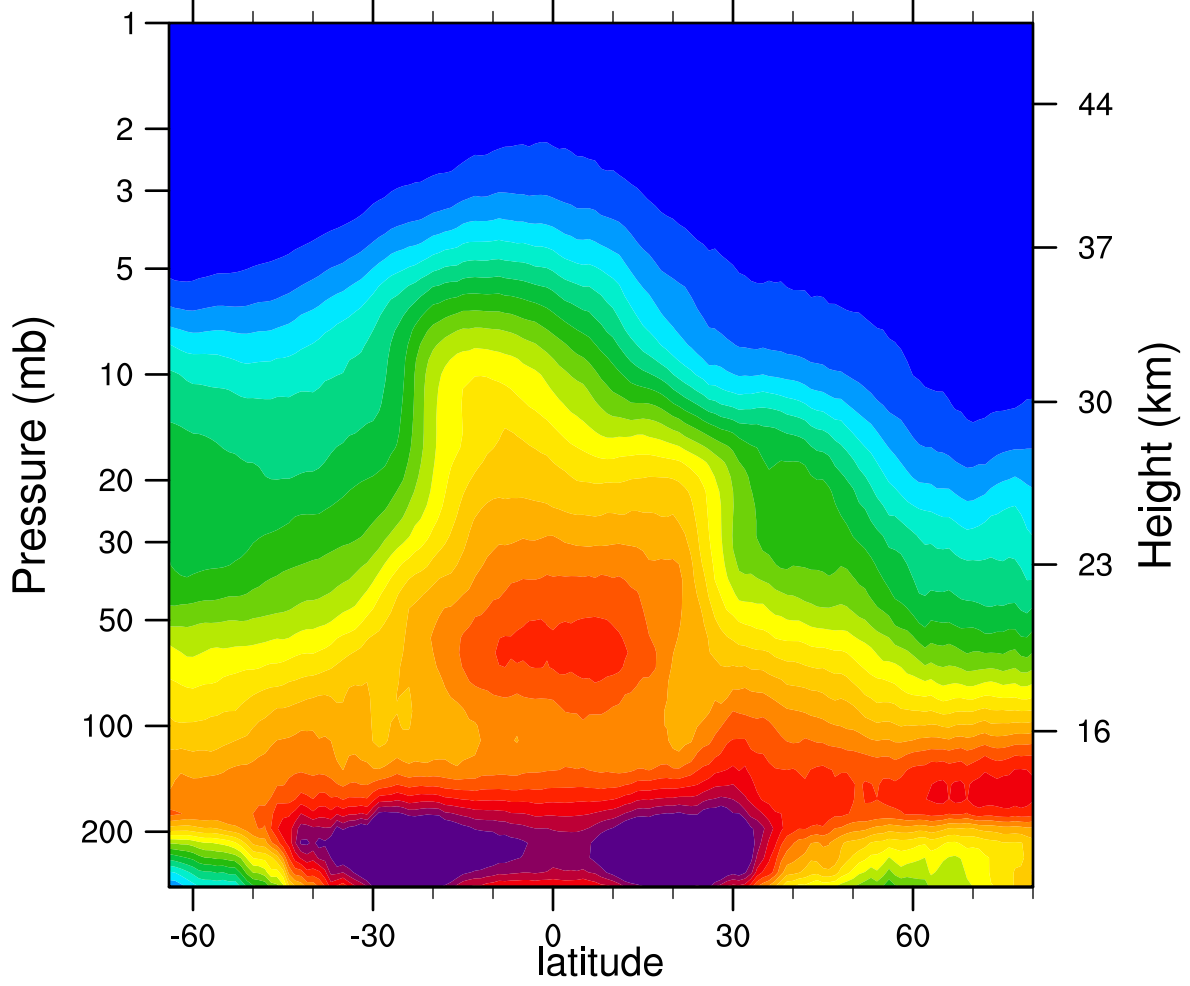
2006d009 N2O_Combined (ppbv)
