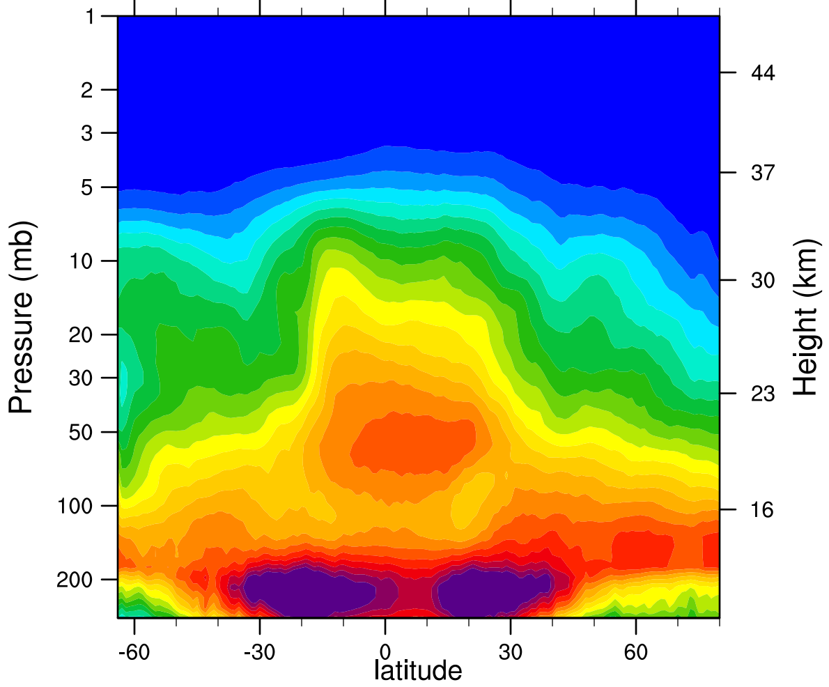
2005d310 N2O_Combined (ppbv)
