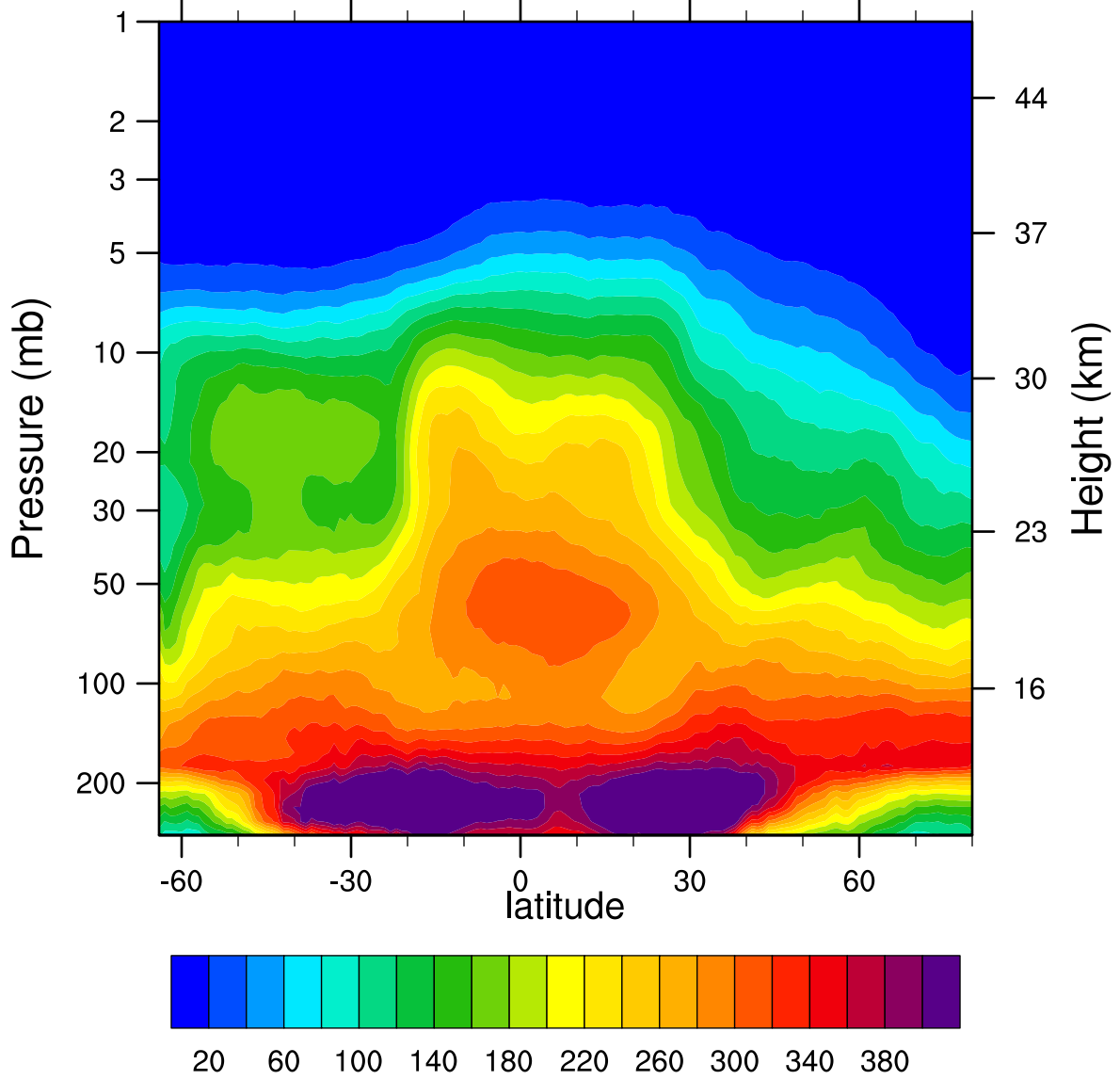
2007d306 N2O_Combined (ppbv)
