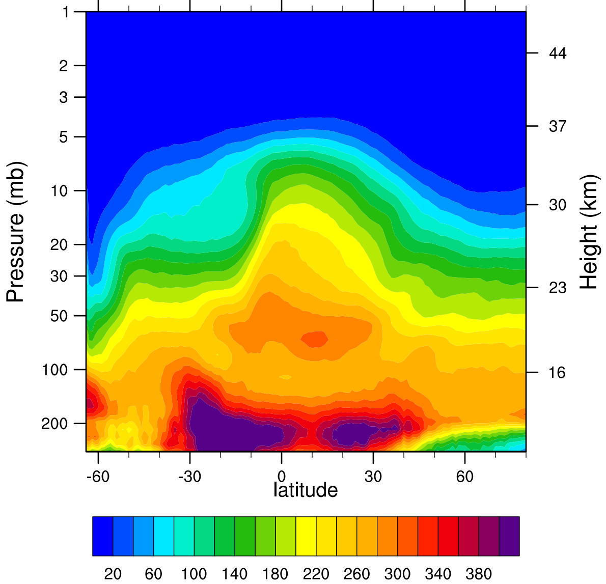
2006d241 N2O_Combined (ppbv)
