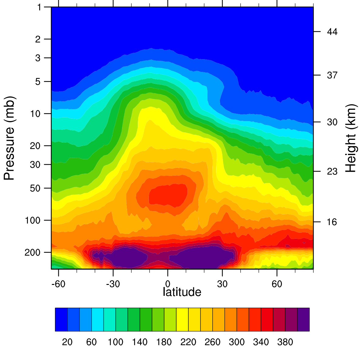
2006d060 N2O_Combined (ppbv)
