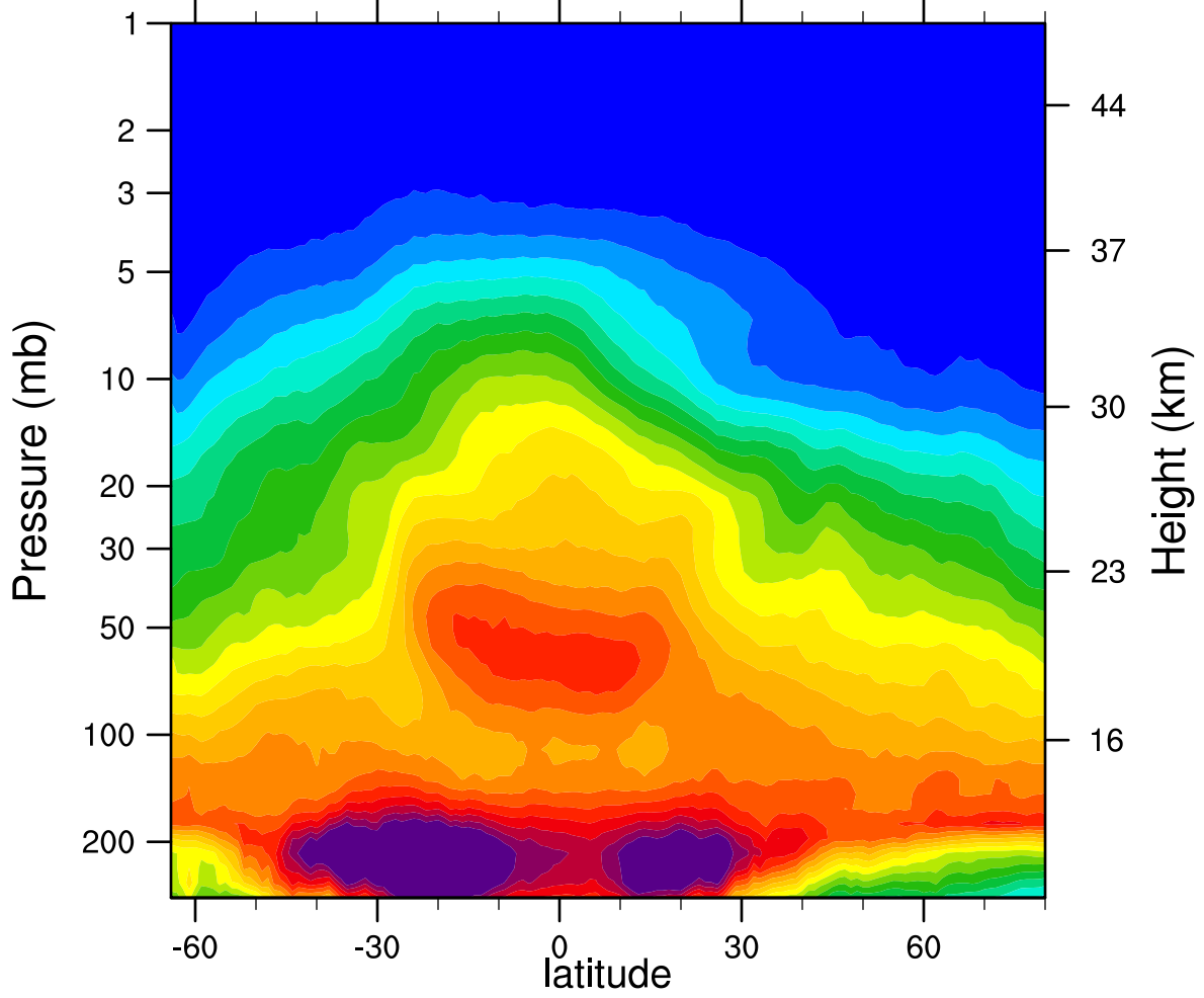
2006d115 N2O_Combined (ppbv)
