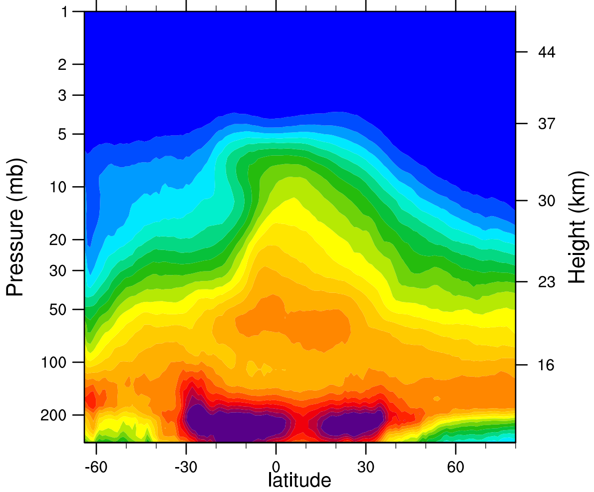
2006d274 N2O_Combined (ppbv)
