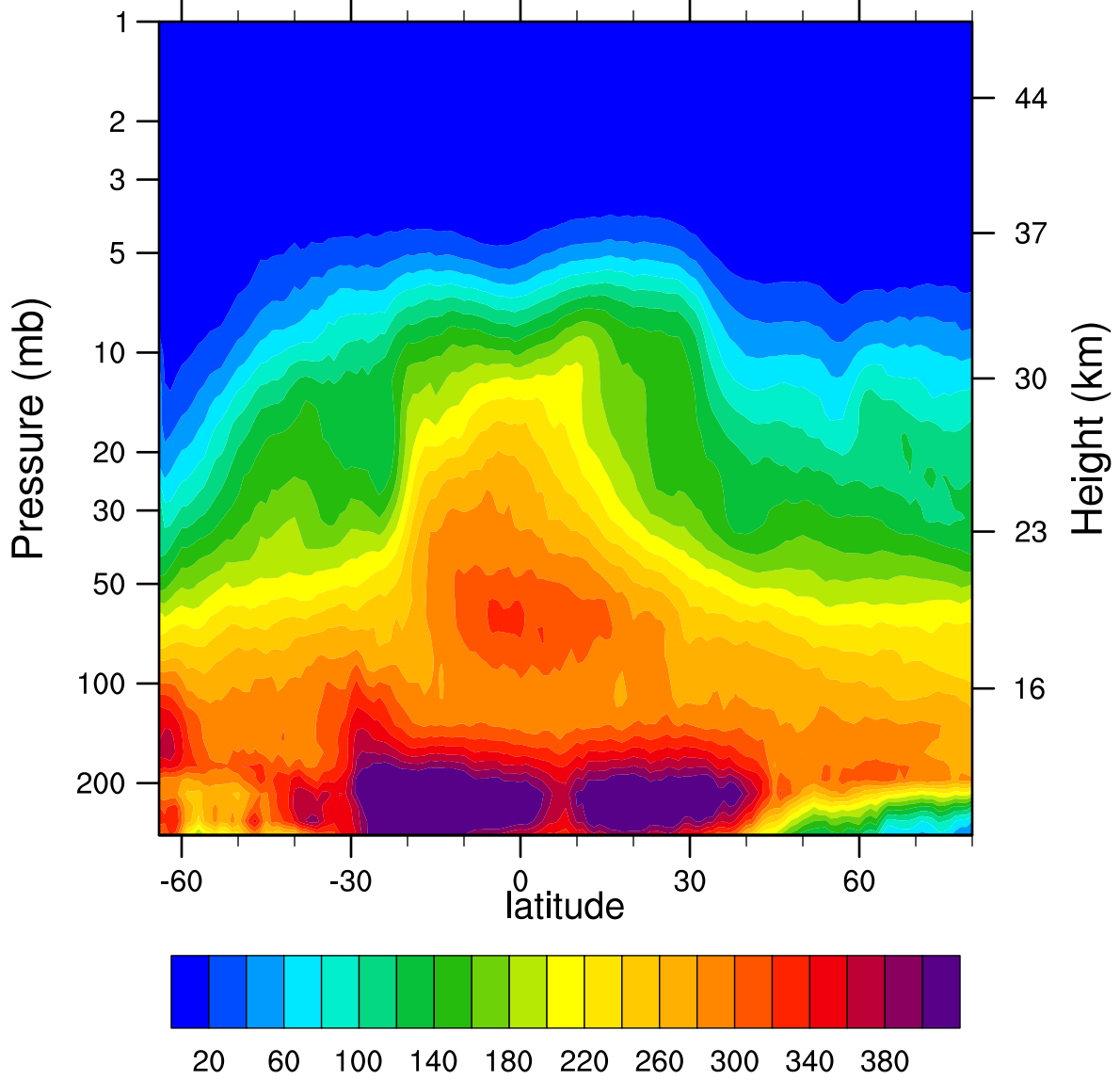
2007d163 N2O_Combined (ppbv)
