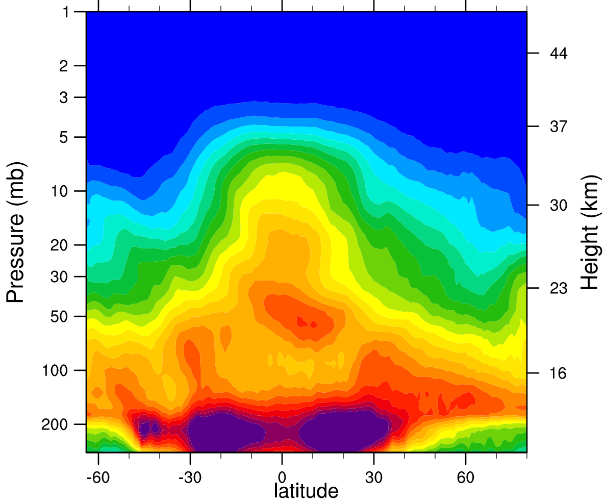
2005d084 N2O_Combined (ppbv)
