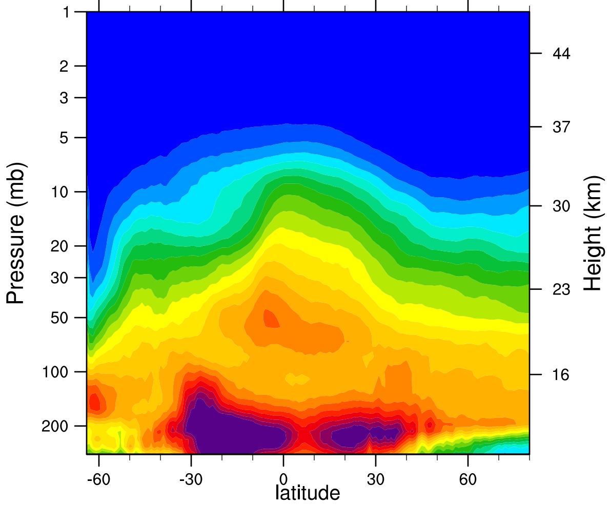
2006d197 N2O_Combined (ppbv)
