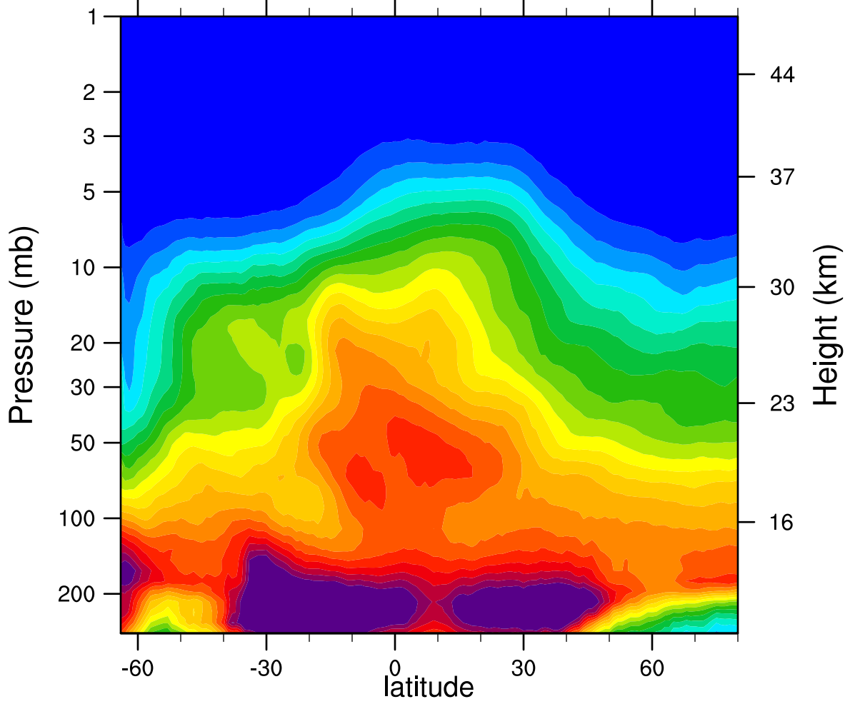
2007d245 N2O_Combined (ppbv)
