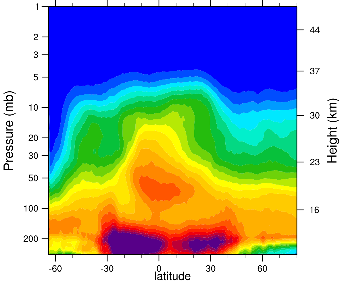
2007d193 N2O_Combined (ppbv)
