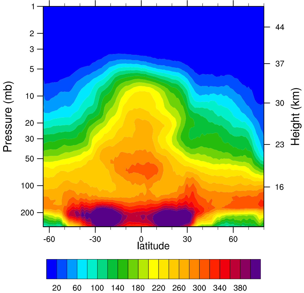
2007d068 N2O_Combined (ppbv)
