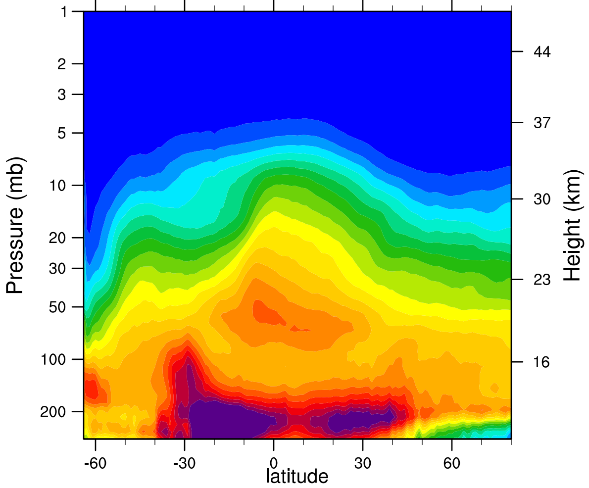
2006d207 N2O_Combined (ppbv)
