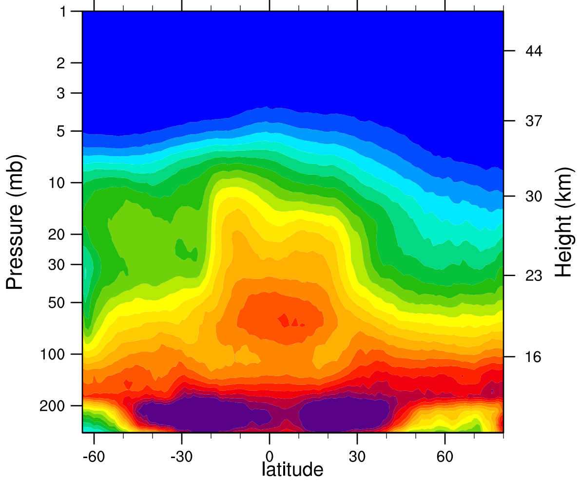
2007d326 N2O_Combined (ppbv)
