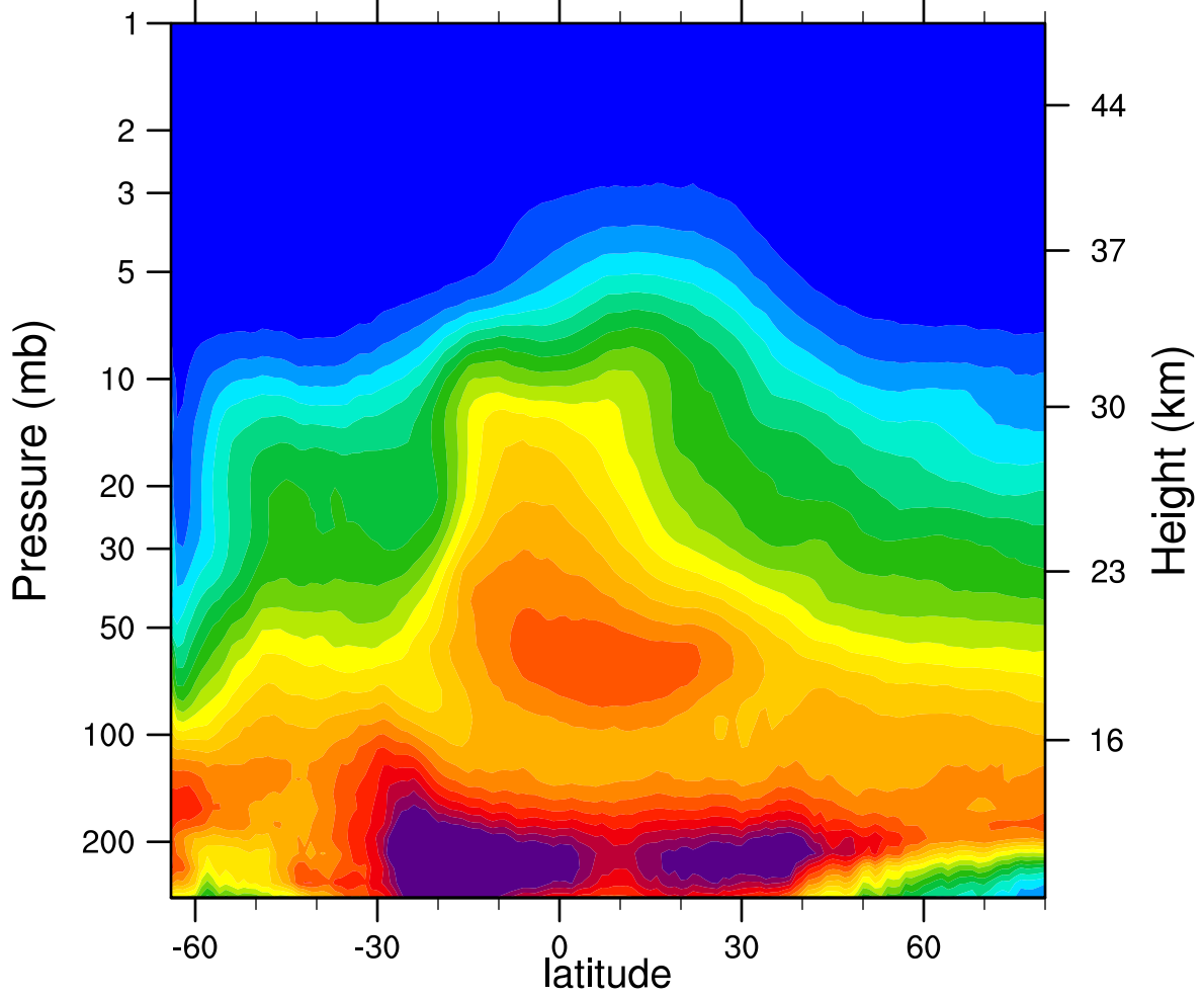
2005d234 N2O_Combined (ppbv)
