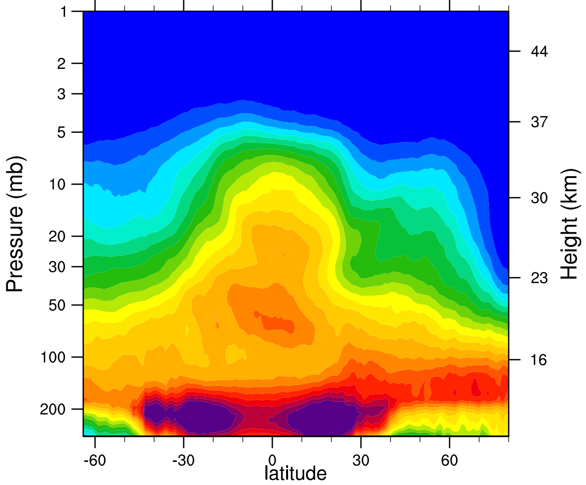
2007d033 N2O_Combined (ppbv)
