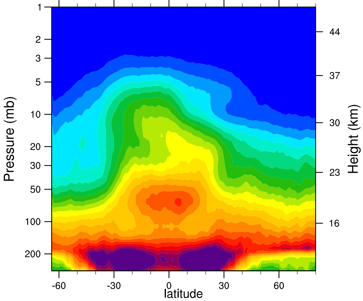
2006d091 N2O_Combined (ppbv)
