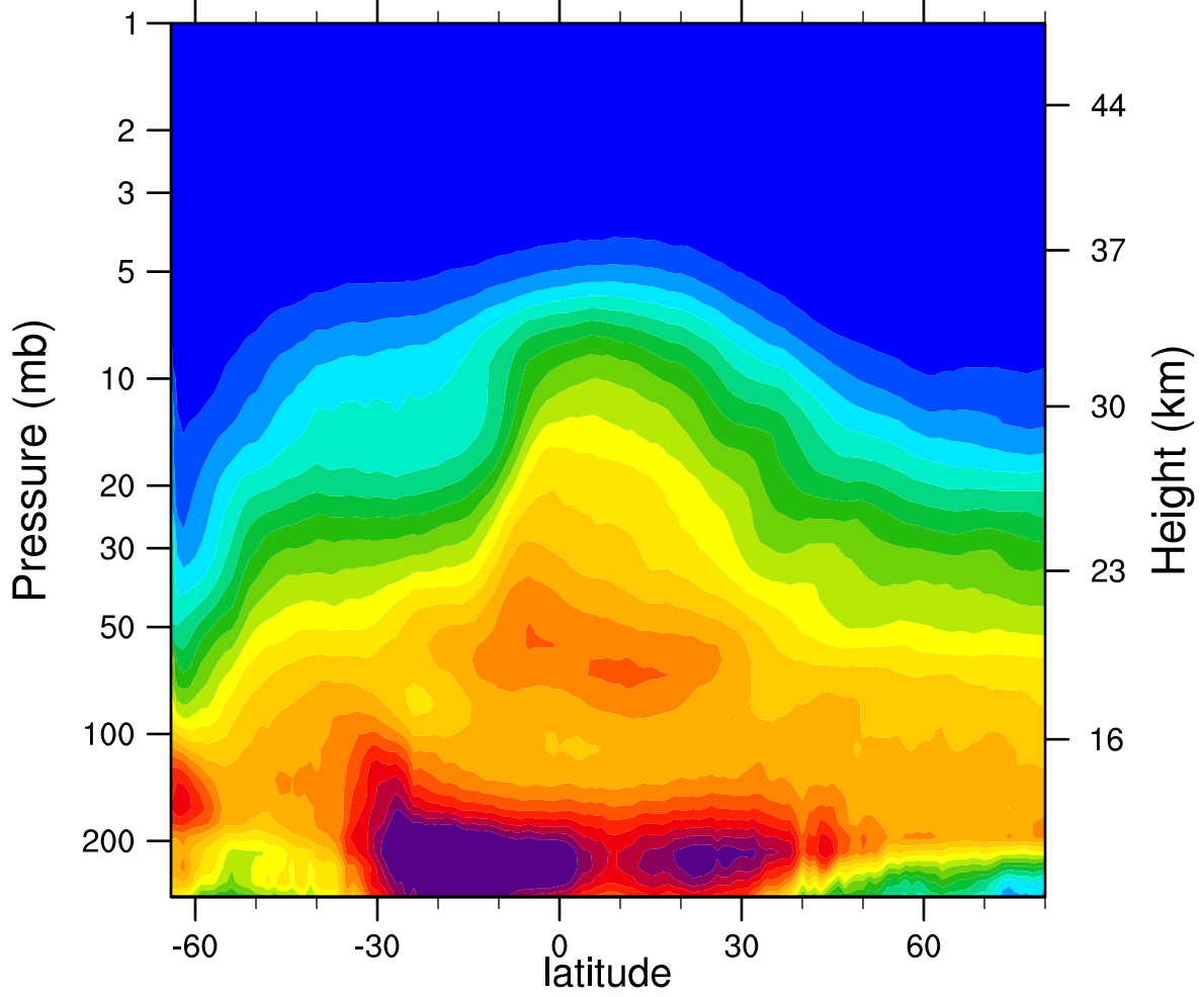
2006d230 N2O_Combined (ppbv)
