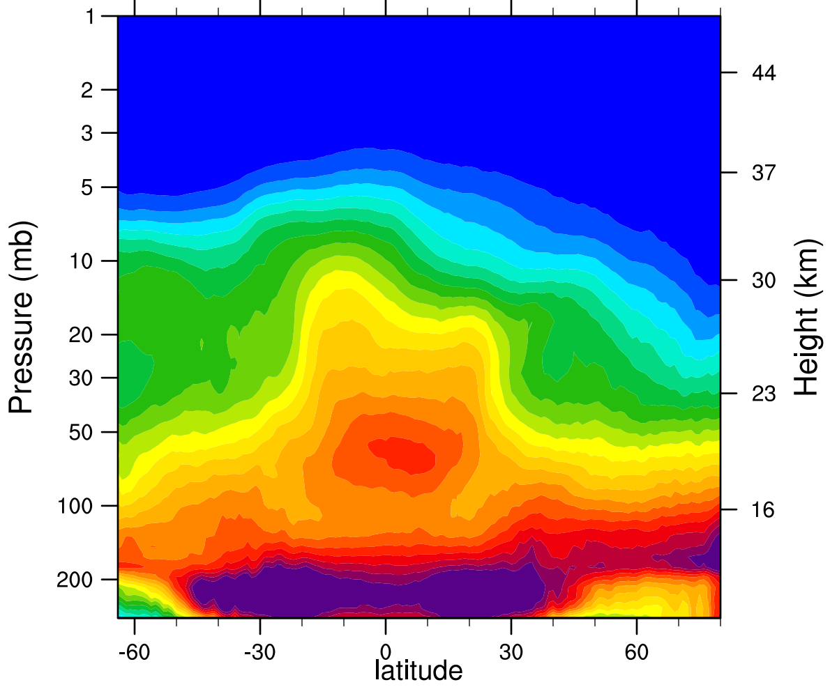
2007d347 N2O_Combined (ppbv)
