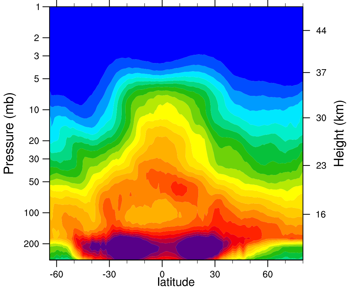
2005d104 N2O_Combined (ppbv)
