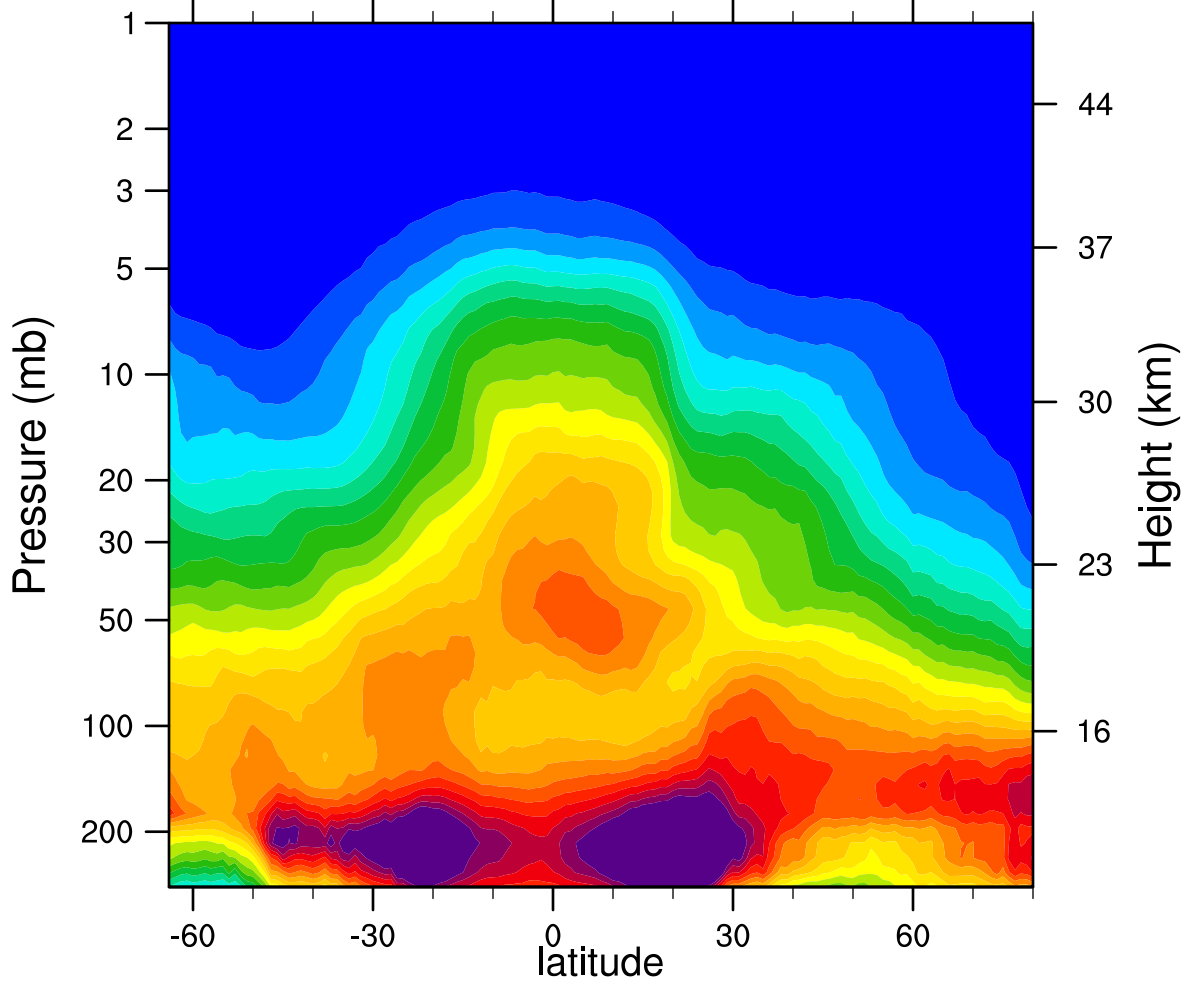
2005d050 N2O_Combined (ppbv)
