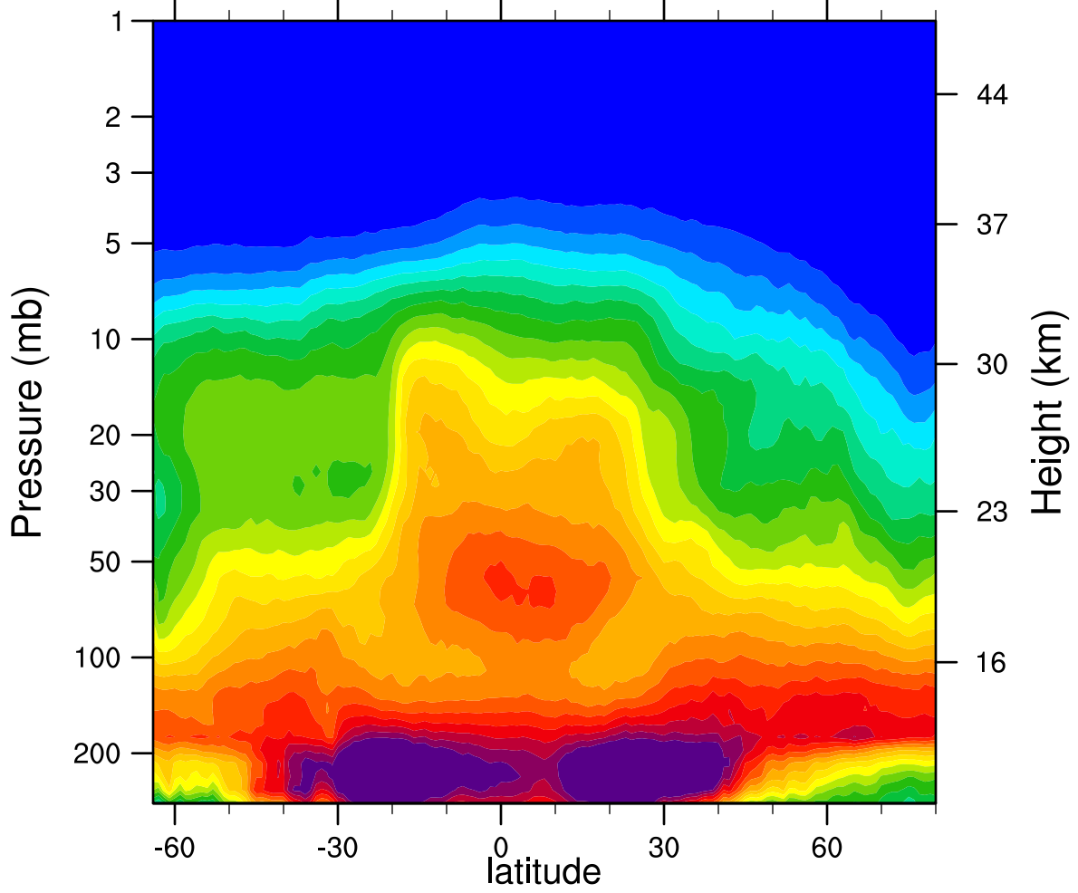
2007d313 N2O_Combined (ppbv)
