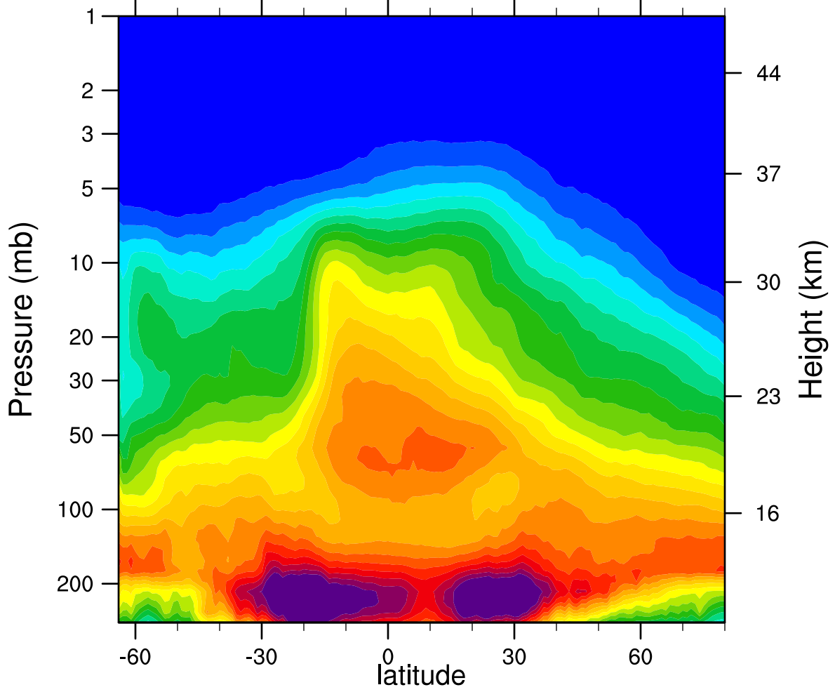
2005d285 N2O_Combined (ppbv)
