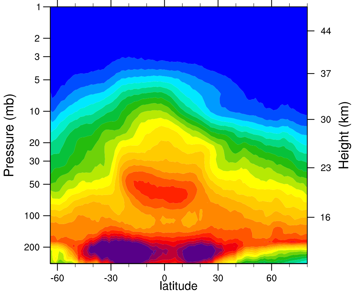
2006d116 N2O_Combined (ppbv)
