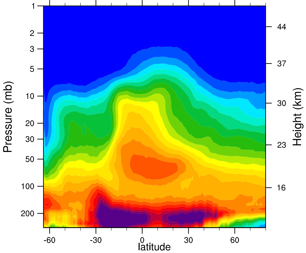
2005d232 N2O_Combined (ppbv)
