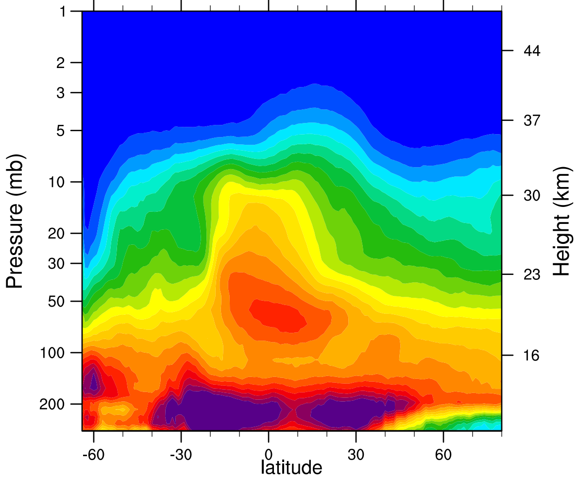
2005d188 N2O_Combined (ppbv)
