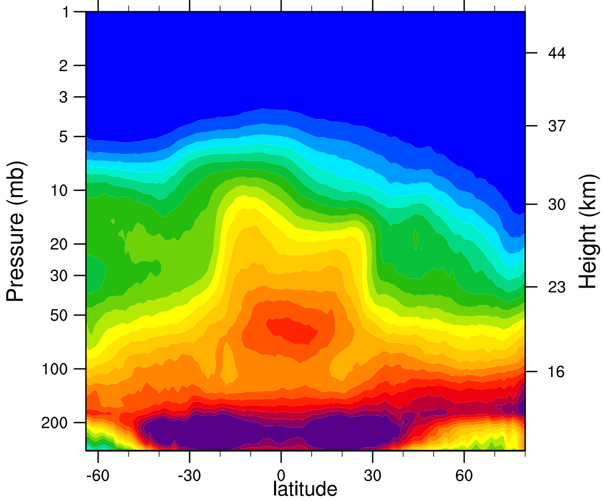
2007d343 N2O_Combined (ppbv)
