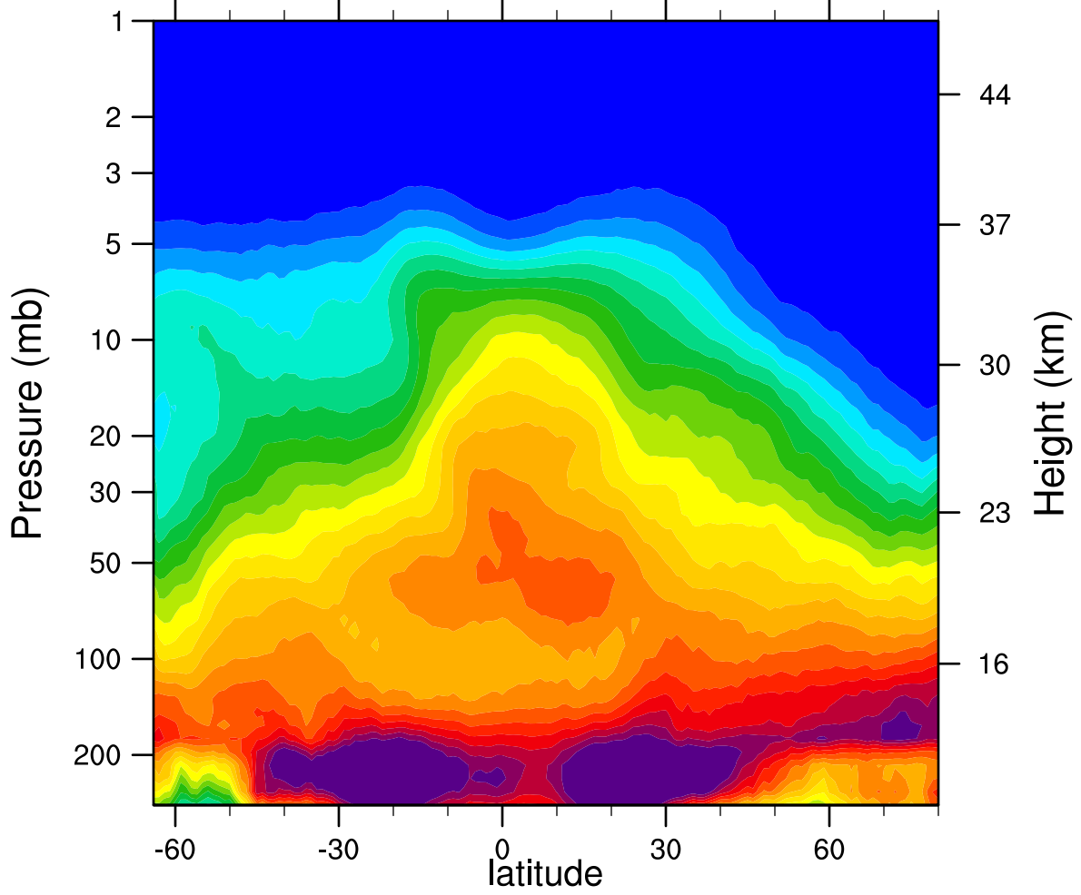
2006d326 N2O_Combined (ppbv)
