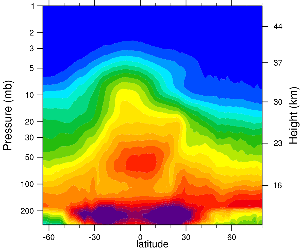
2006d056 N2O_Combined (ppbv)
