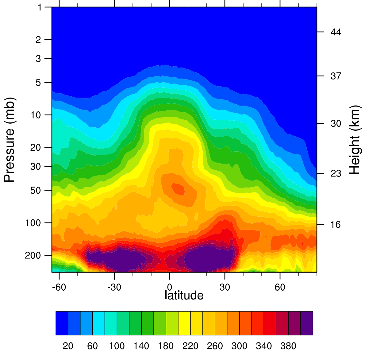
2005d034 N2O_Combined (ppbv)
