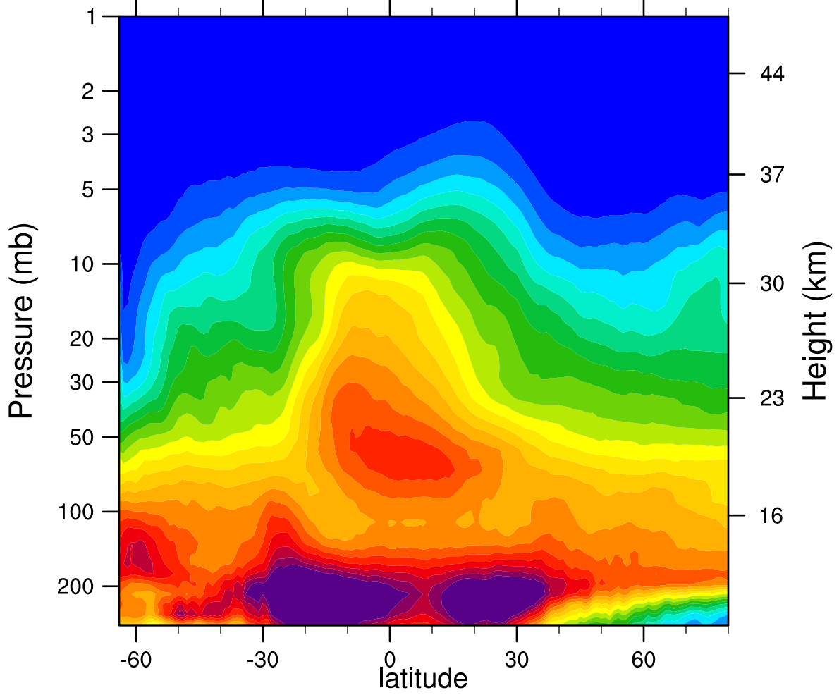
2005d167 N2O_Combined (ppbv)
