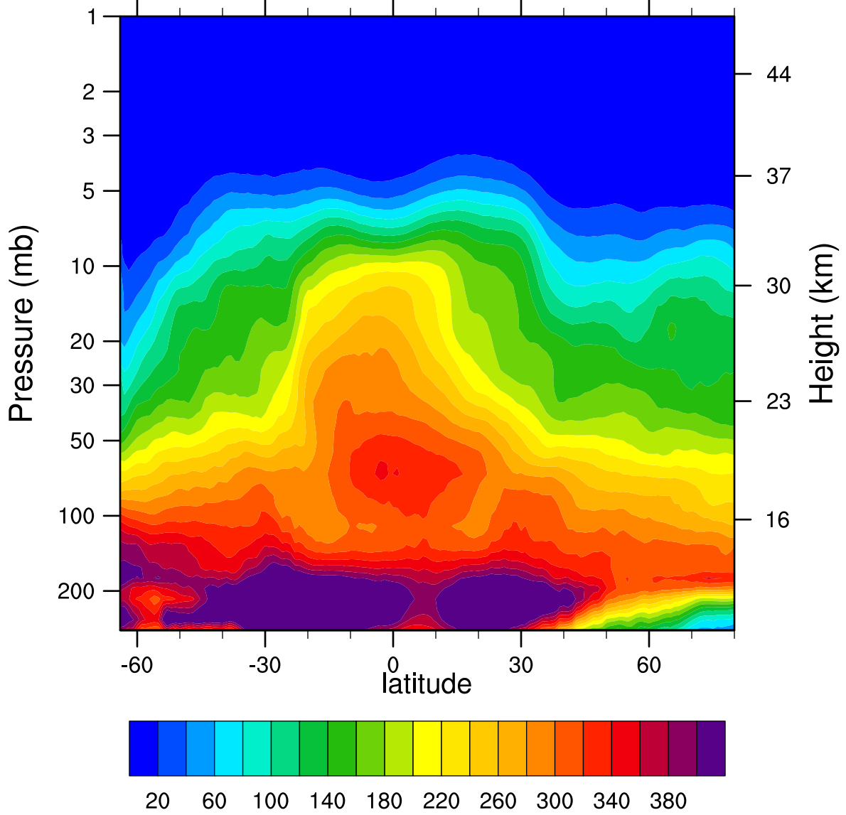
2007d149 N2O_Combined (ppbv)
