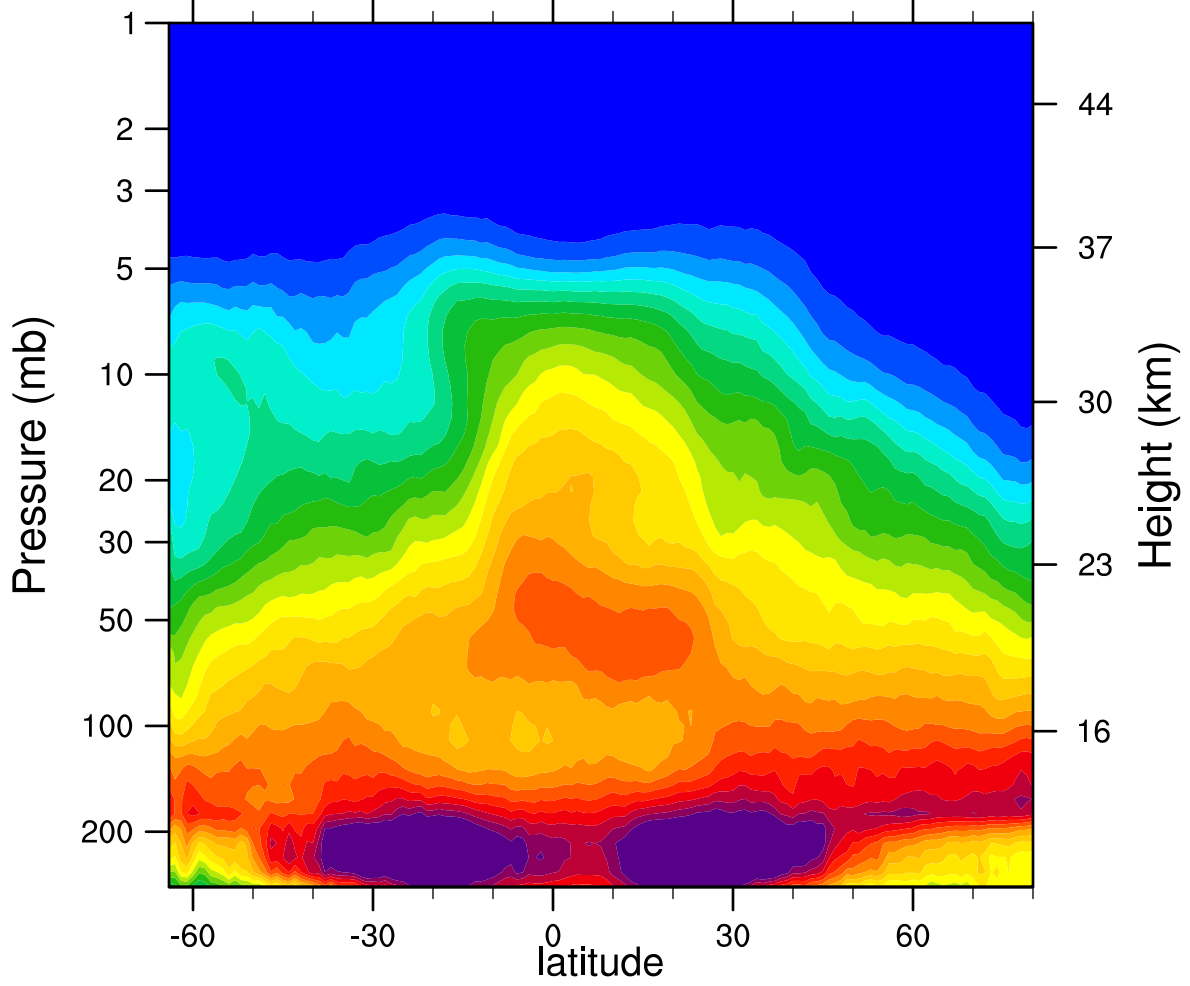
2006d315 N2O_Combined (ppbv)
