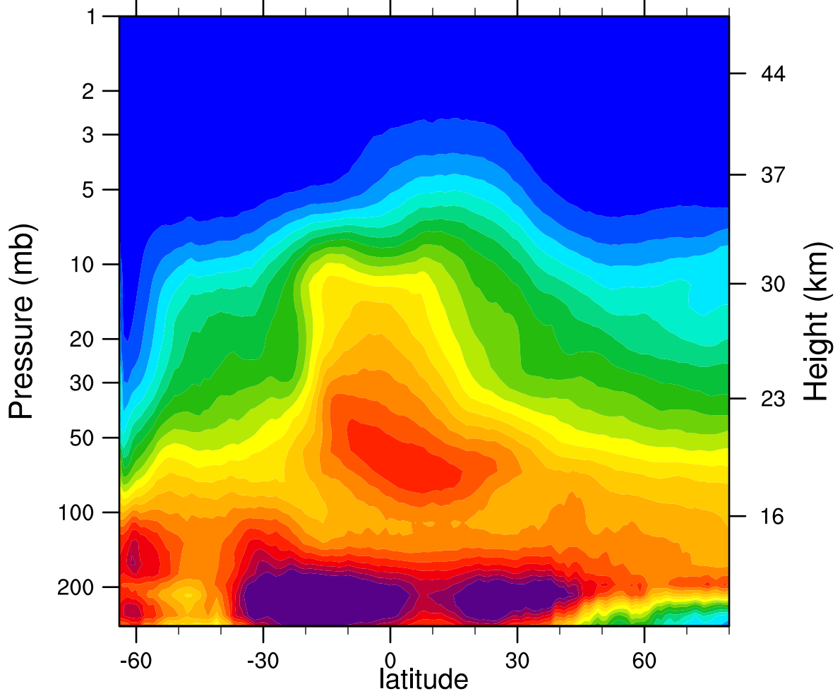
2005d205 N2O_Combined (ppbv)
