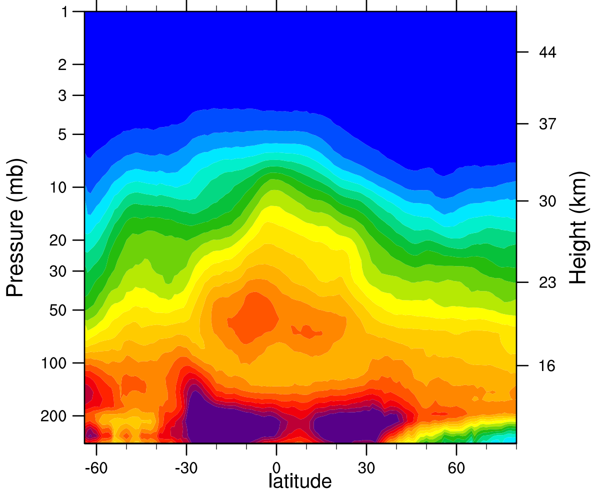
2006d167 N2O_Combined (ppbv)
