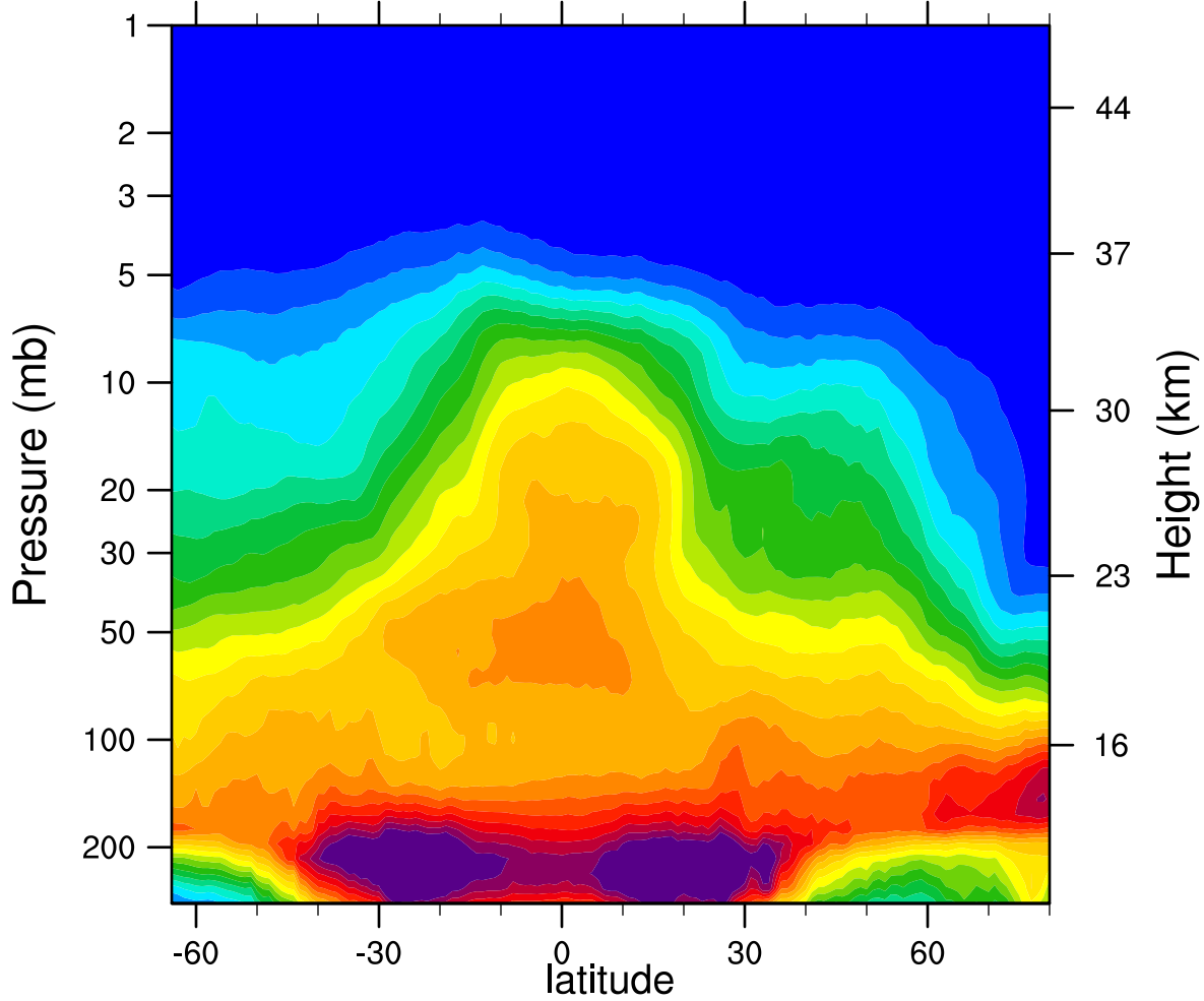
2007d007 N2O_Combined (ppbv)
