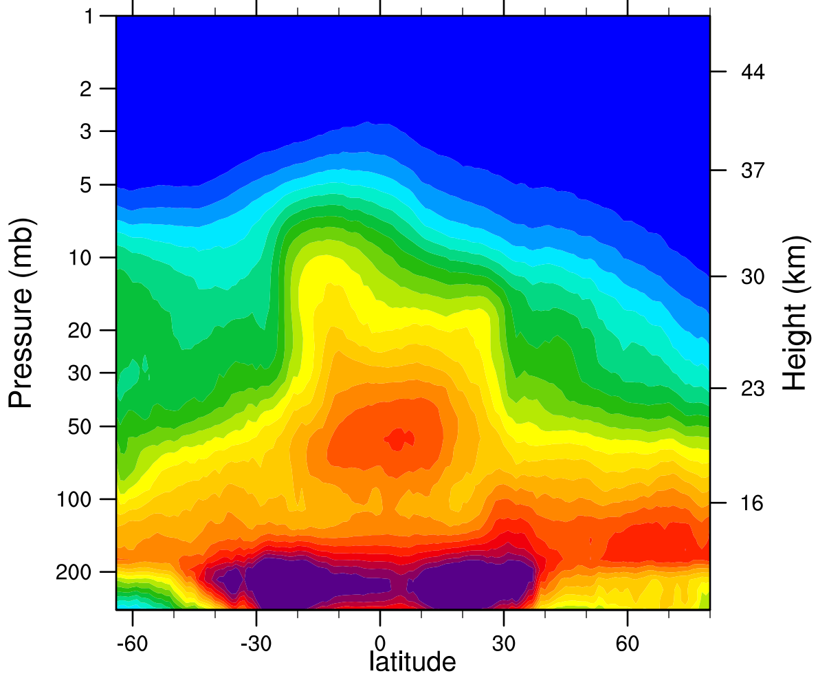
2005d344 N2O_Combined (ppbv)
