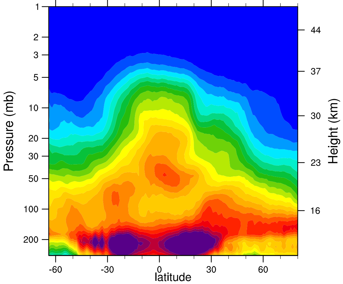
2005d061 N2O_Combined (ppbv)
