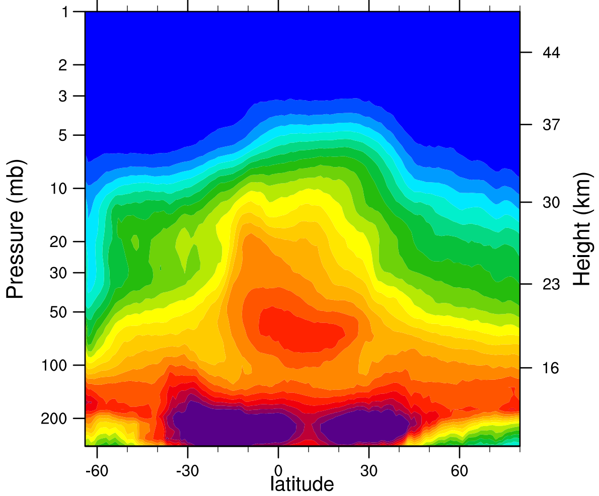
2007d267 N2O_Combined (ppbv)
