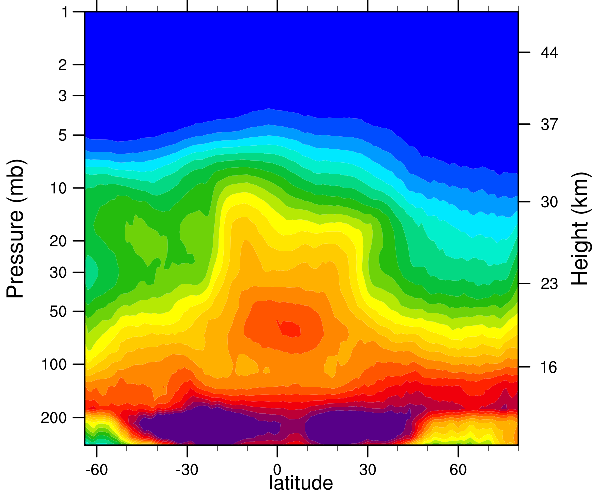
2007d332 N2O_Combined (ppbv)
