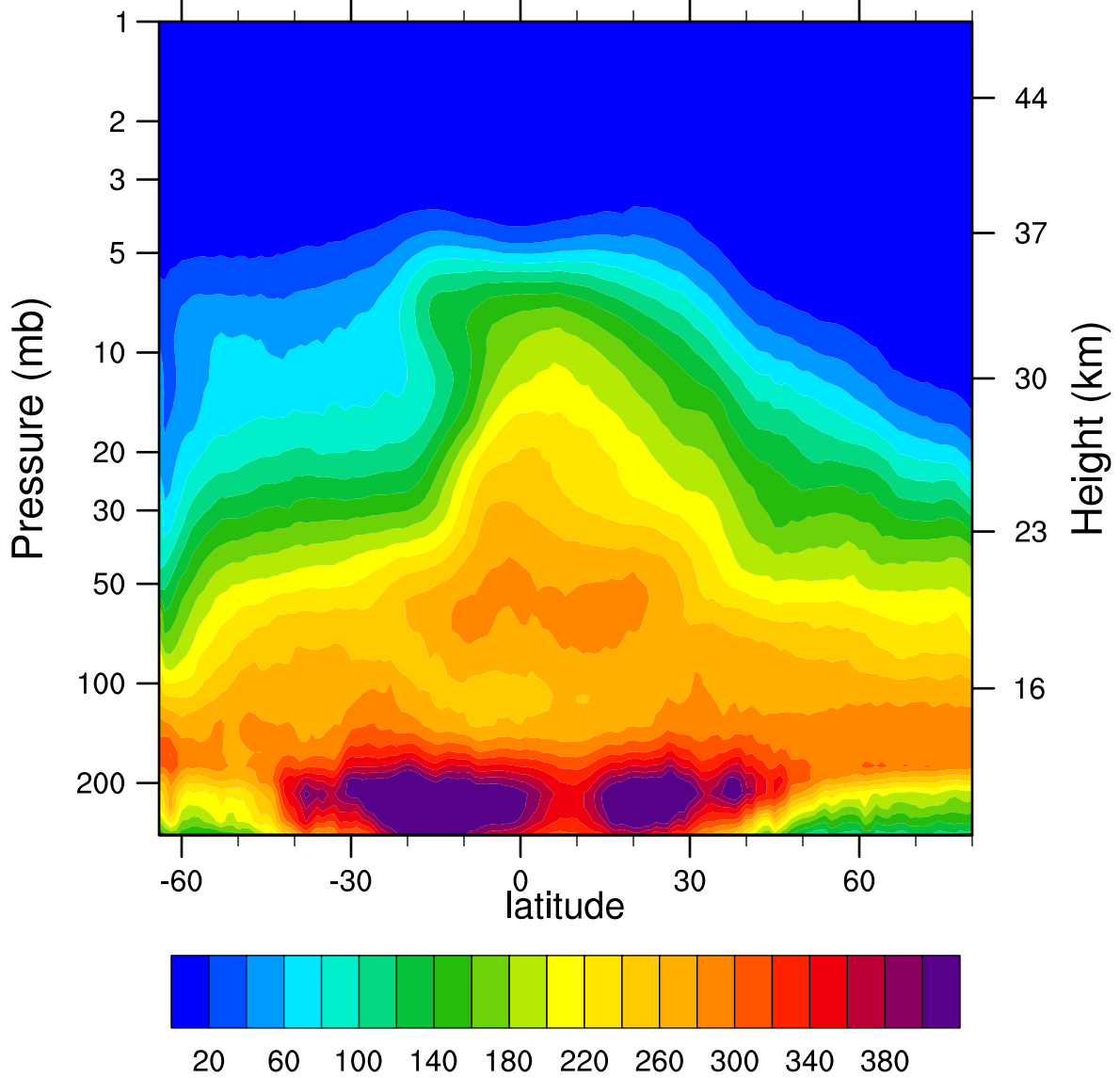
2006d285 N2O_Combined (ppbv)
