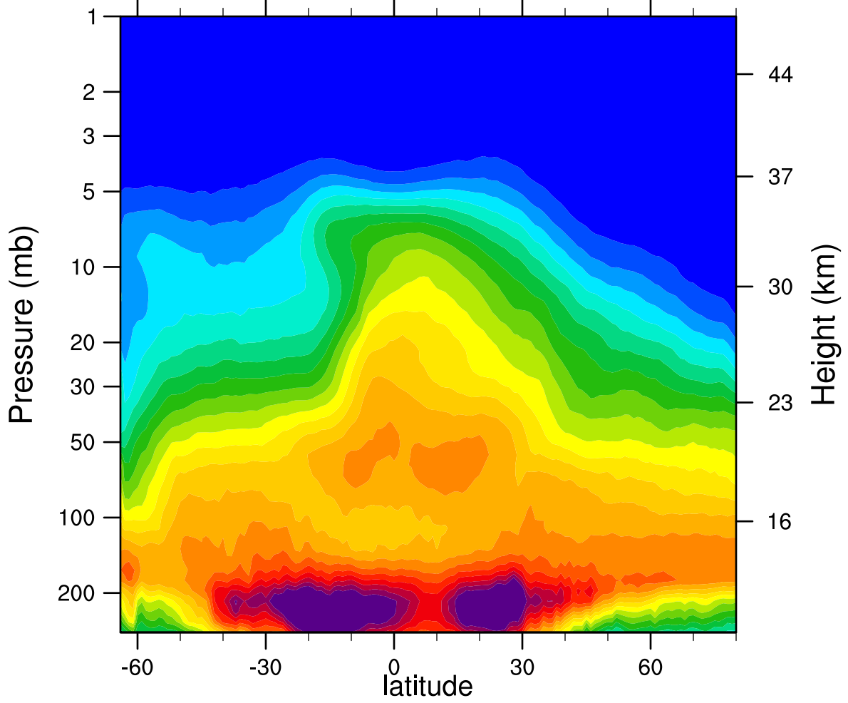
2006d287 N2O_Combined (ppbv)
