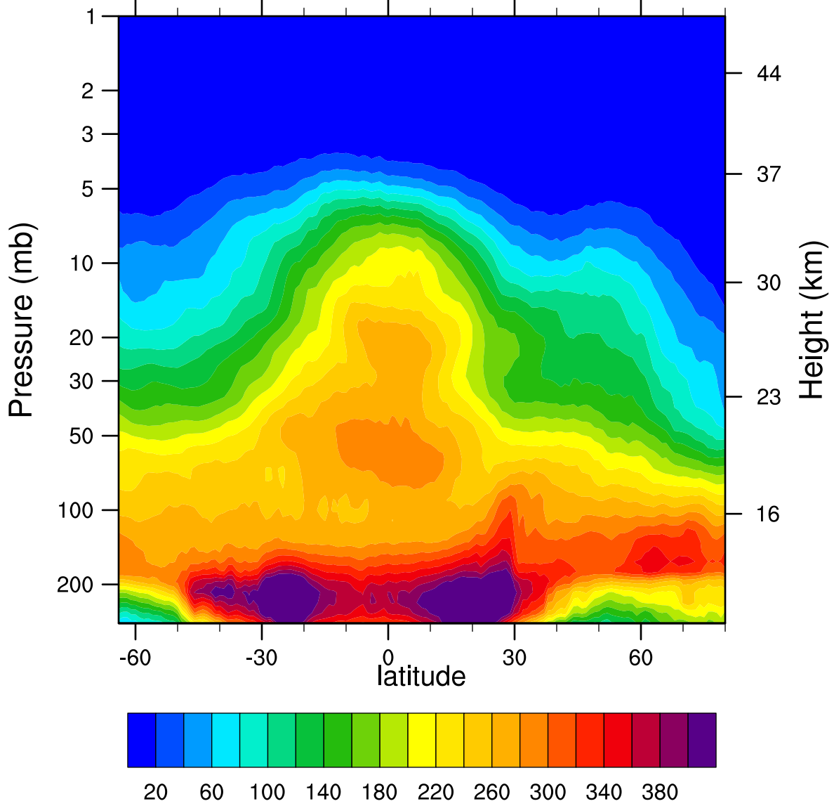
2007d050 N2O_Combined (ppbv)
