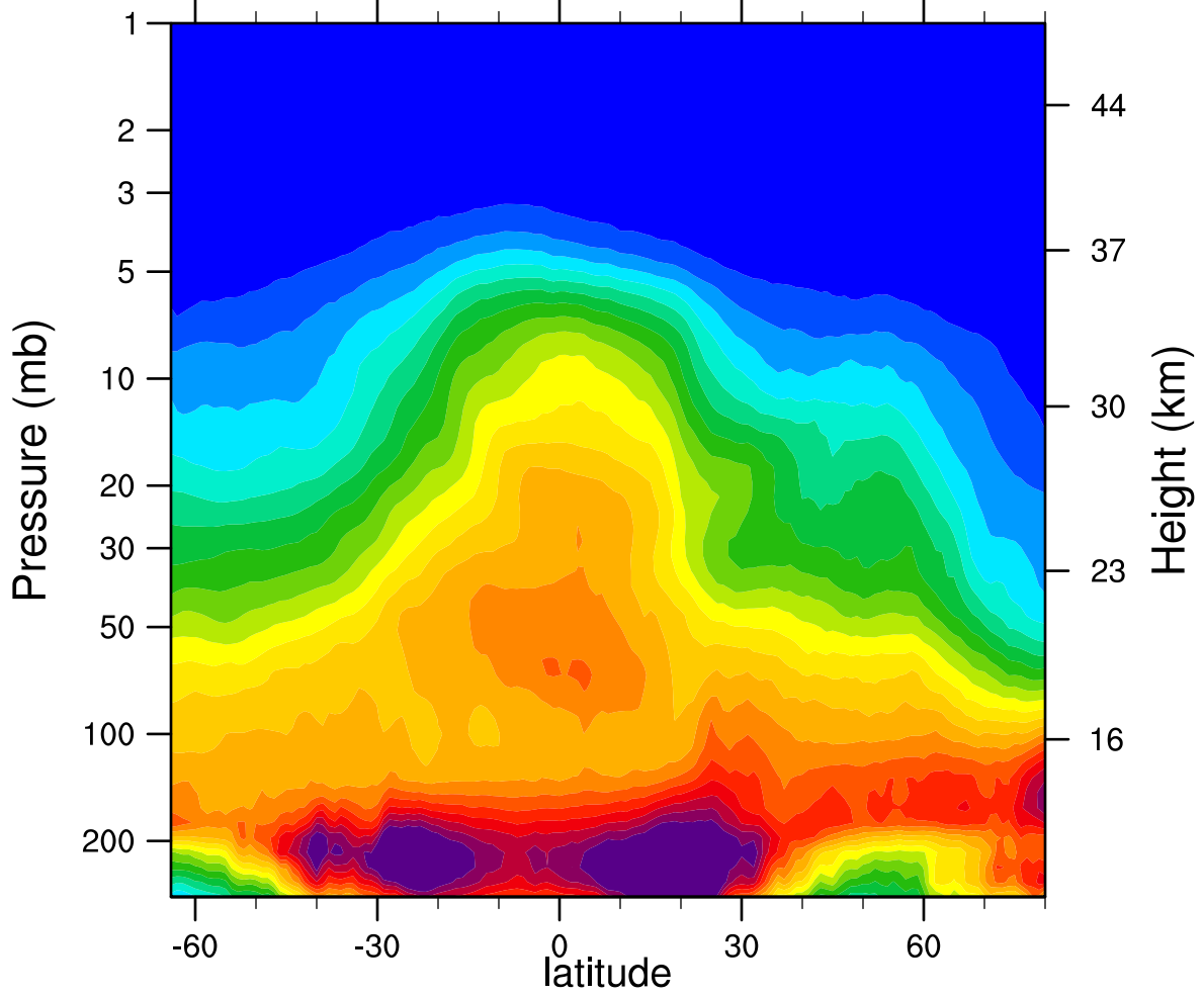
2007d038 N2O_Combined (ppbv)
