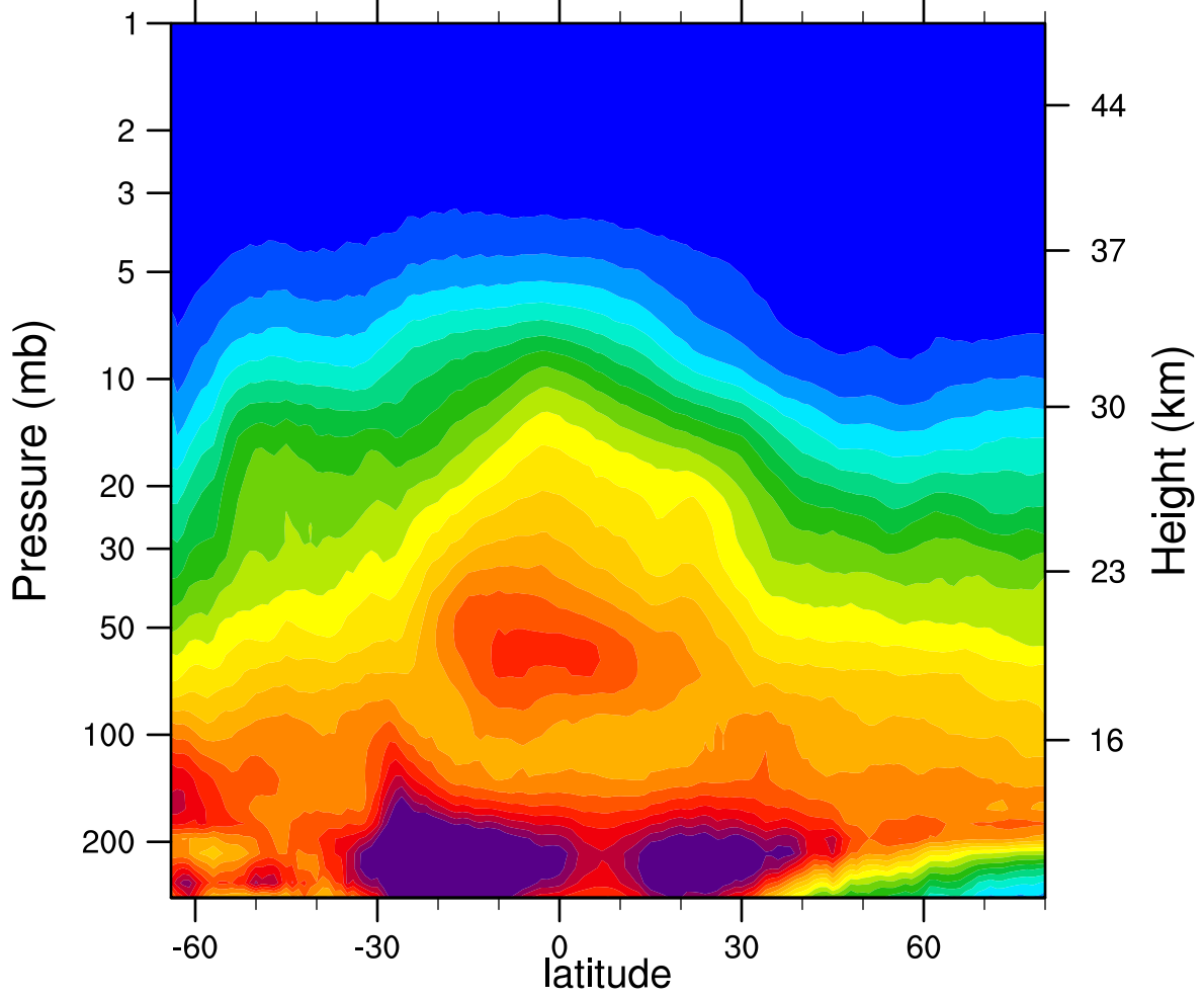
2006d152 N2O_Combined (ppbv)
