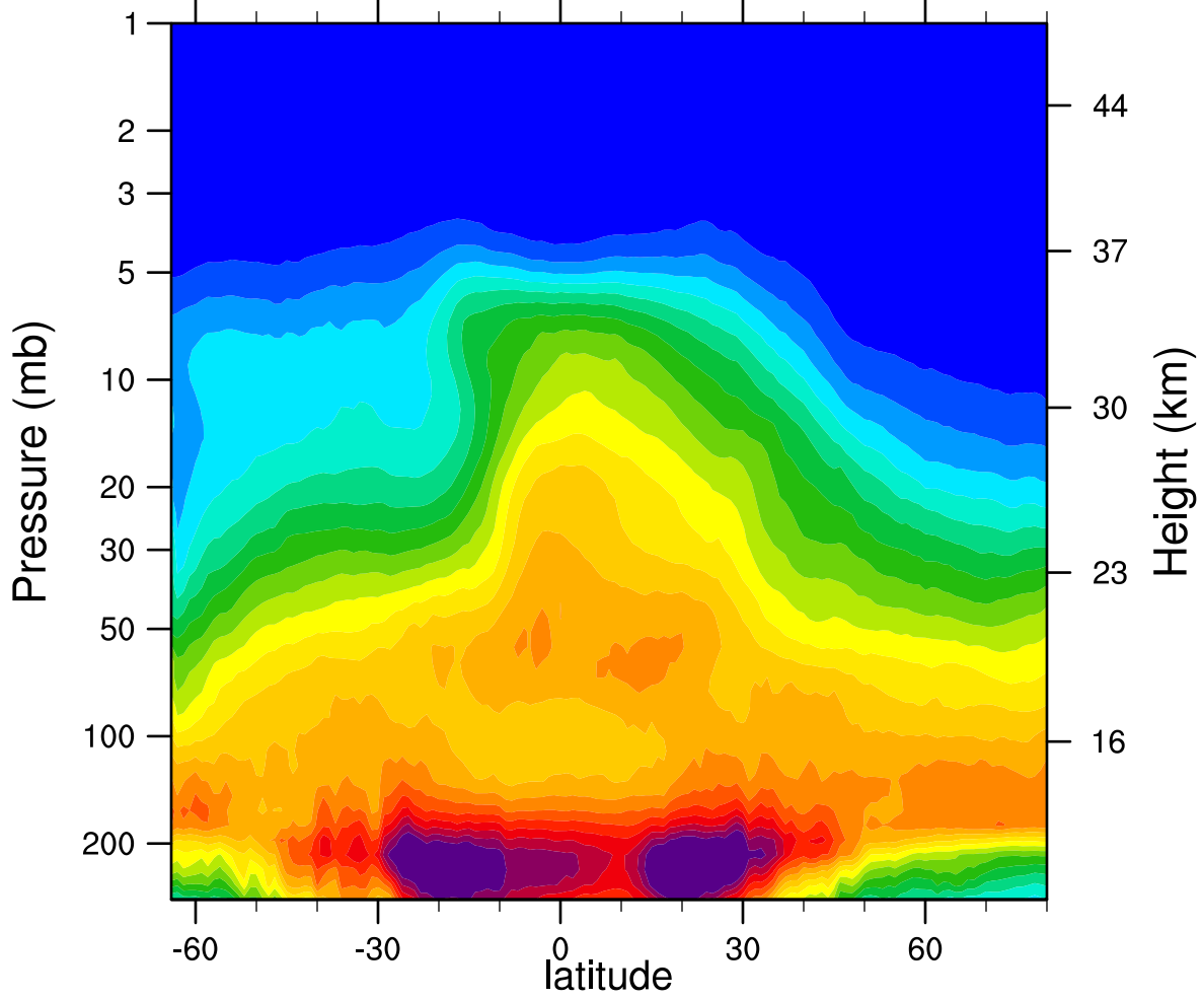
2006d299 N2O_Combined (ppbv)
