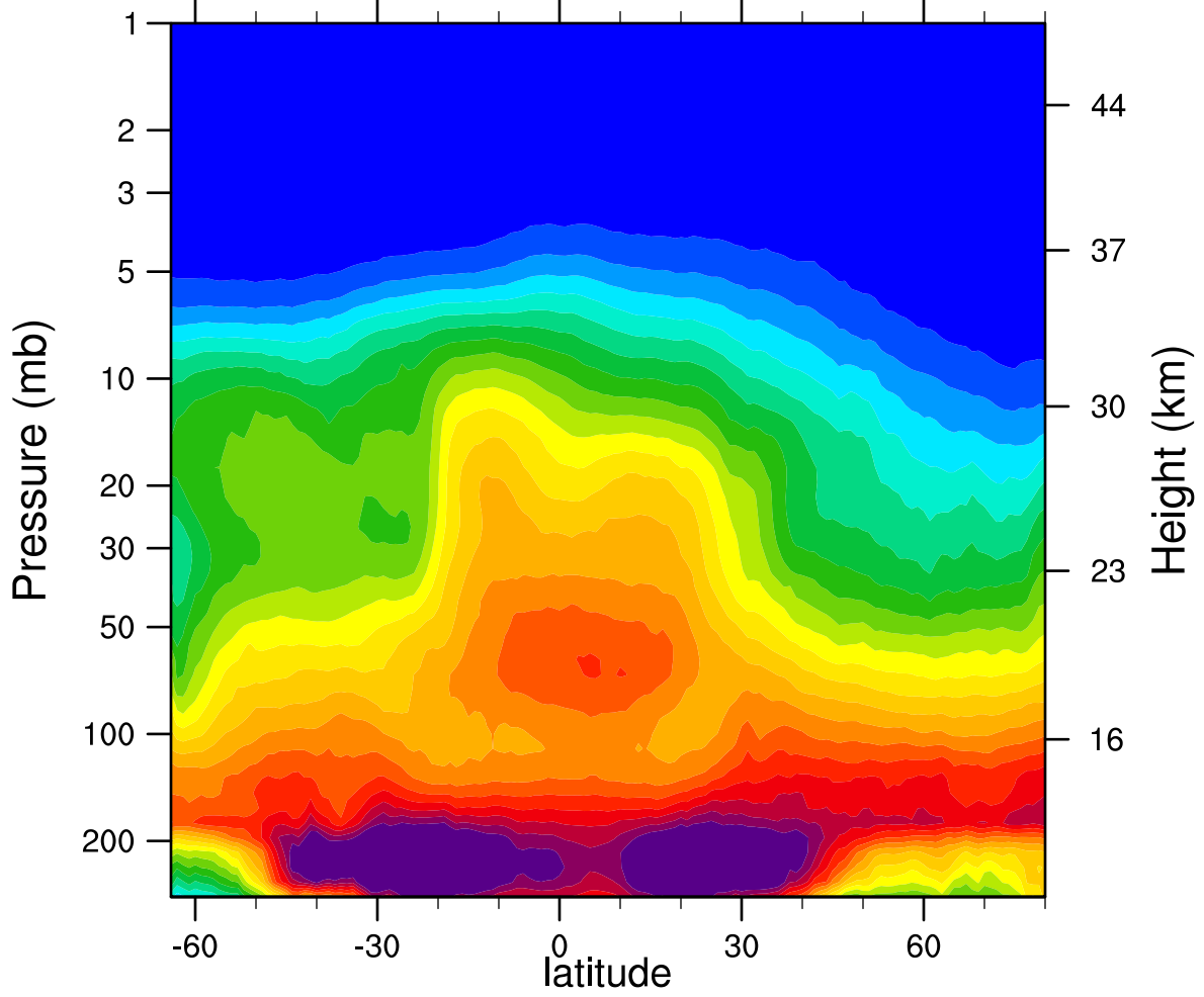
2007d324 N2O_Combined (ppbv)
