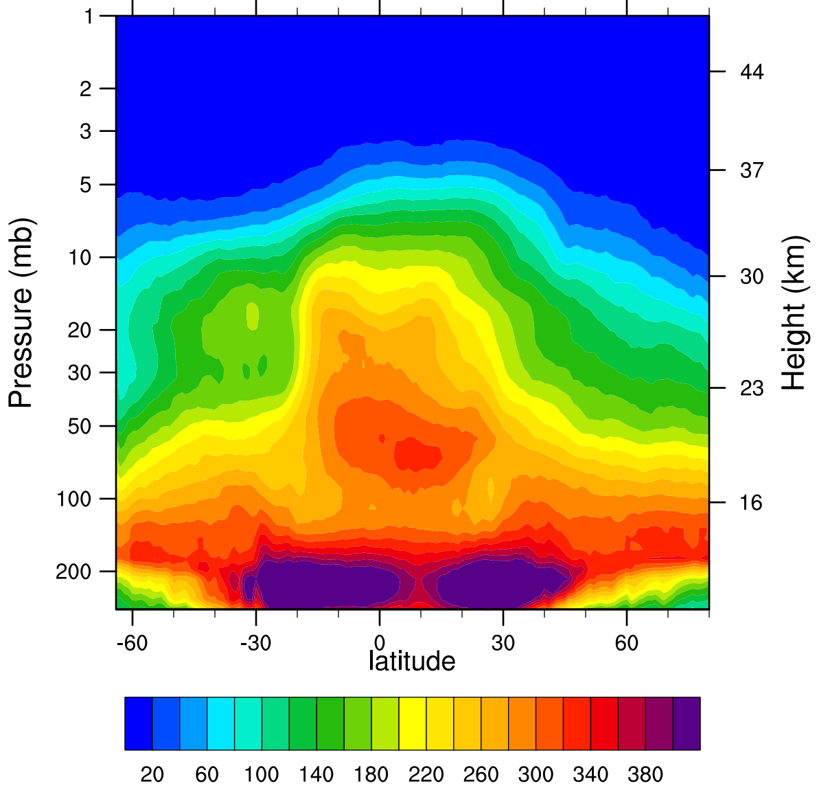
2007d283 N2O_Combined (ppbv)
