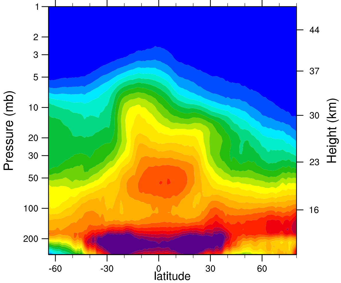
2005d352 N2O_Combined (ppbv)
