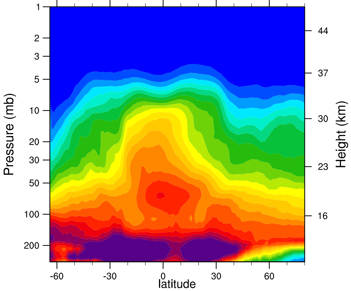
2007d147 N2O_Combined (ppbv)
