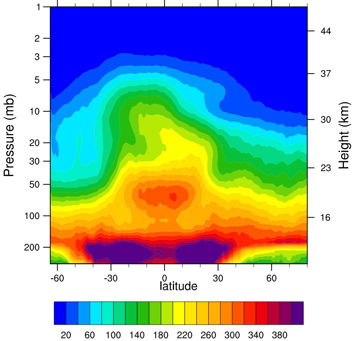
2006d092 N2O_Combined (ppbv)
