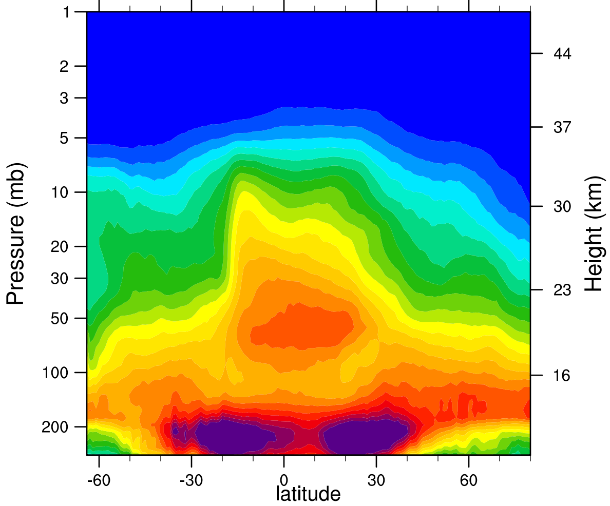
2005d304 N2O_Combined (ppbv)
