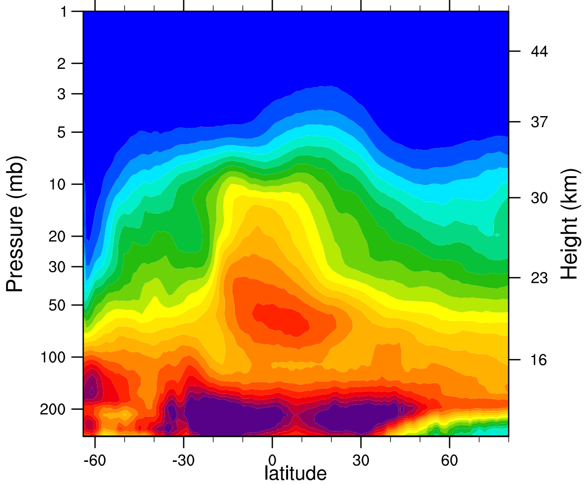
2005d186 N2O_Combined (ppbv)
