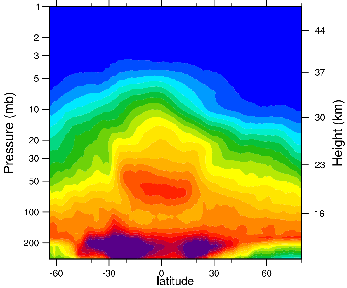
2006d121 N2O_Combined (ppbv)
