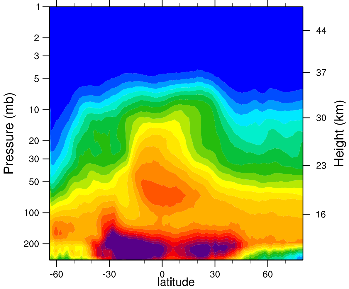
2007d187 N2O_Combined (ppbv)
