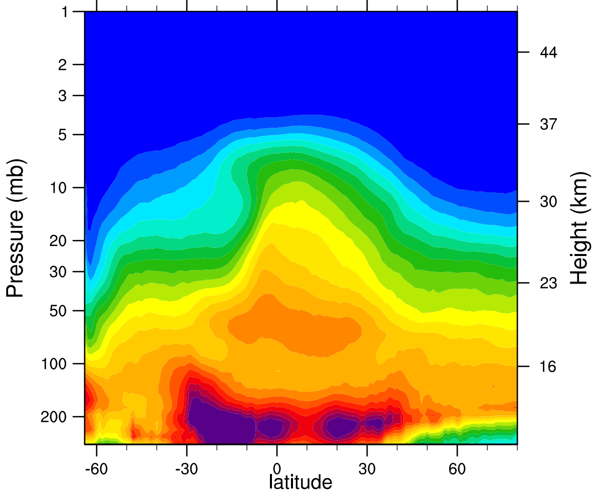
2006d250 N2O_Combined (ppbv)
