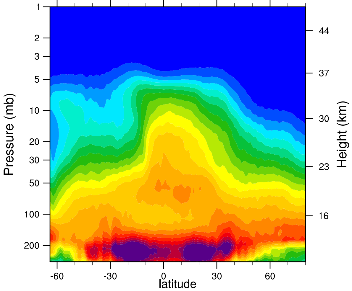
2006d308 N2O_Combined (ppbv)
