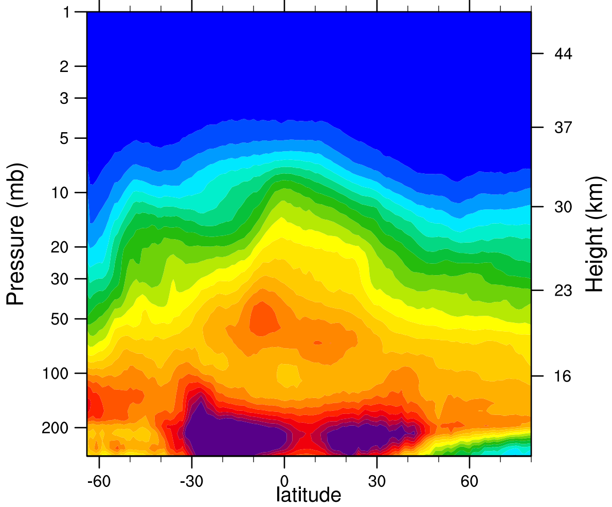
2006d174 N2O_Combined (ppbv)
