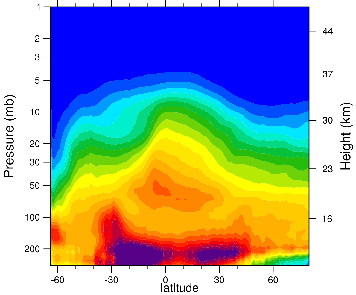
2006d206 N2O_Combined (ppbv)
