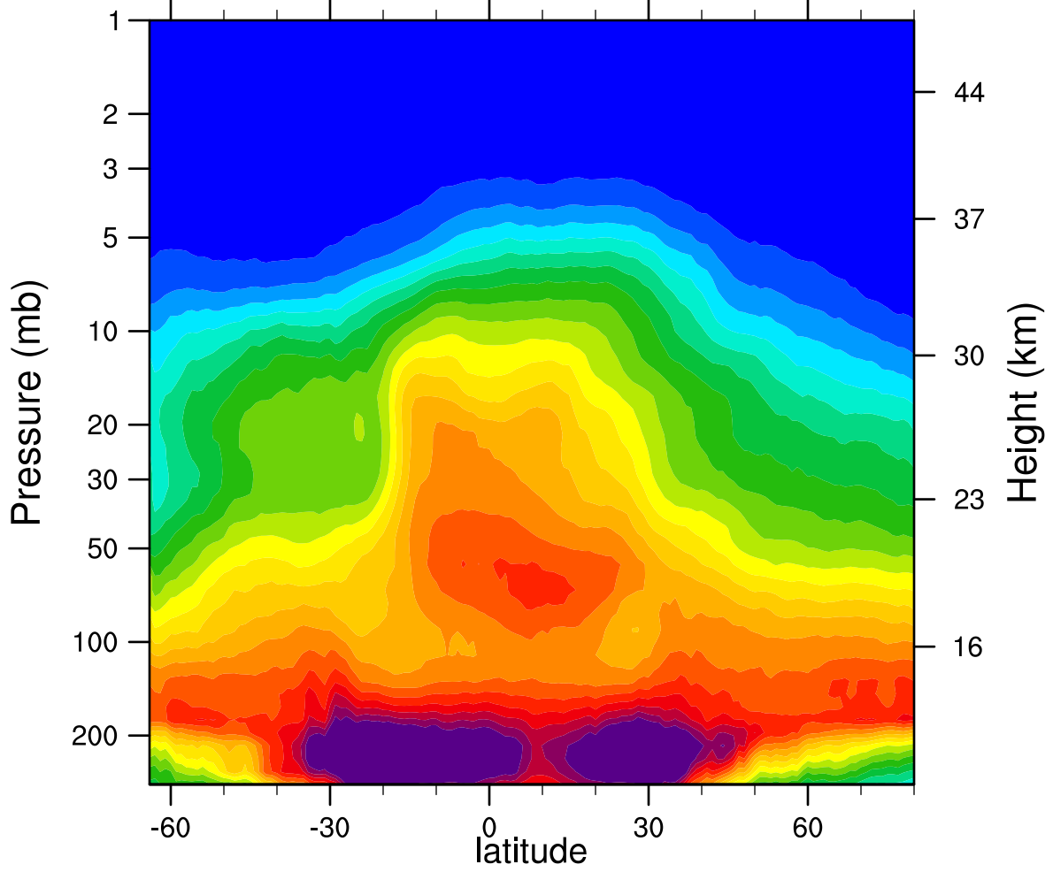
2007d280 N2O_Combined (ppbv)
