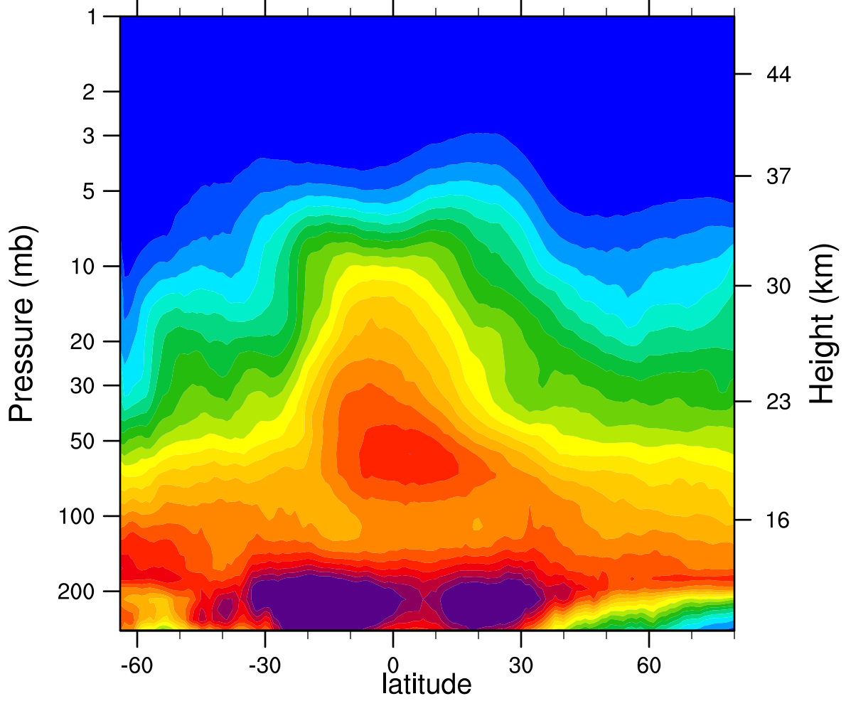
2005d150 N2O_Combined (ppbv)
