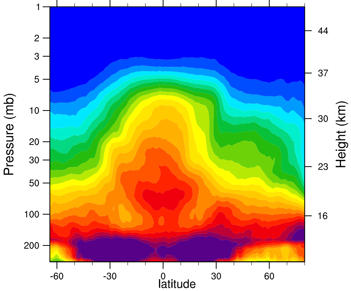
2007d089 N2O_Combined (ppbv)
