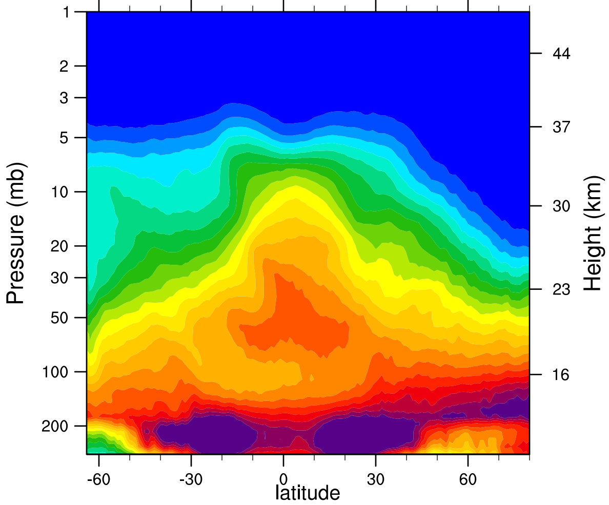
2006d333 N2O_Combined (ppbv)
