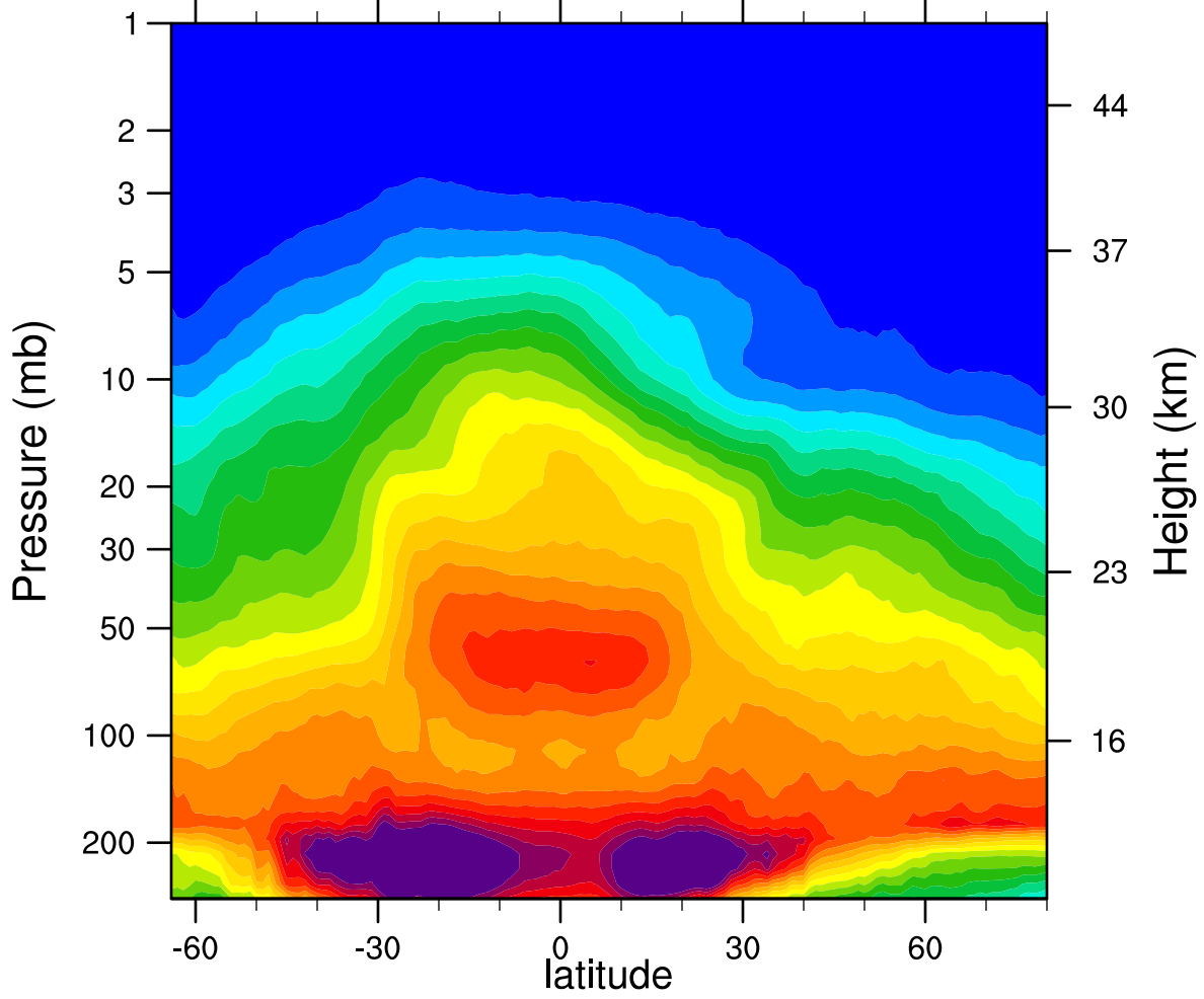
2006d109 N2O_Combined (ppbv)
