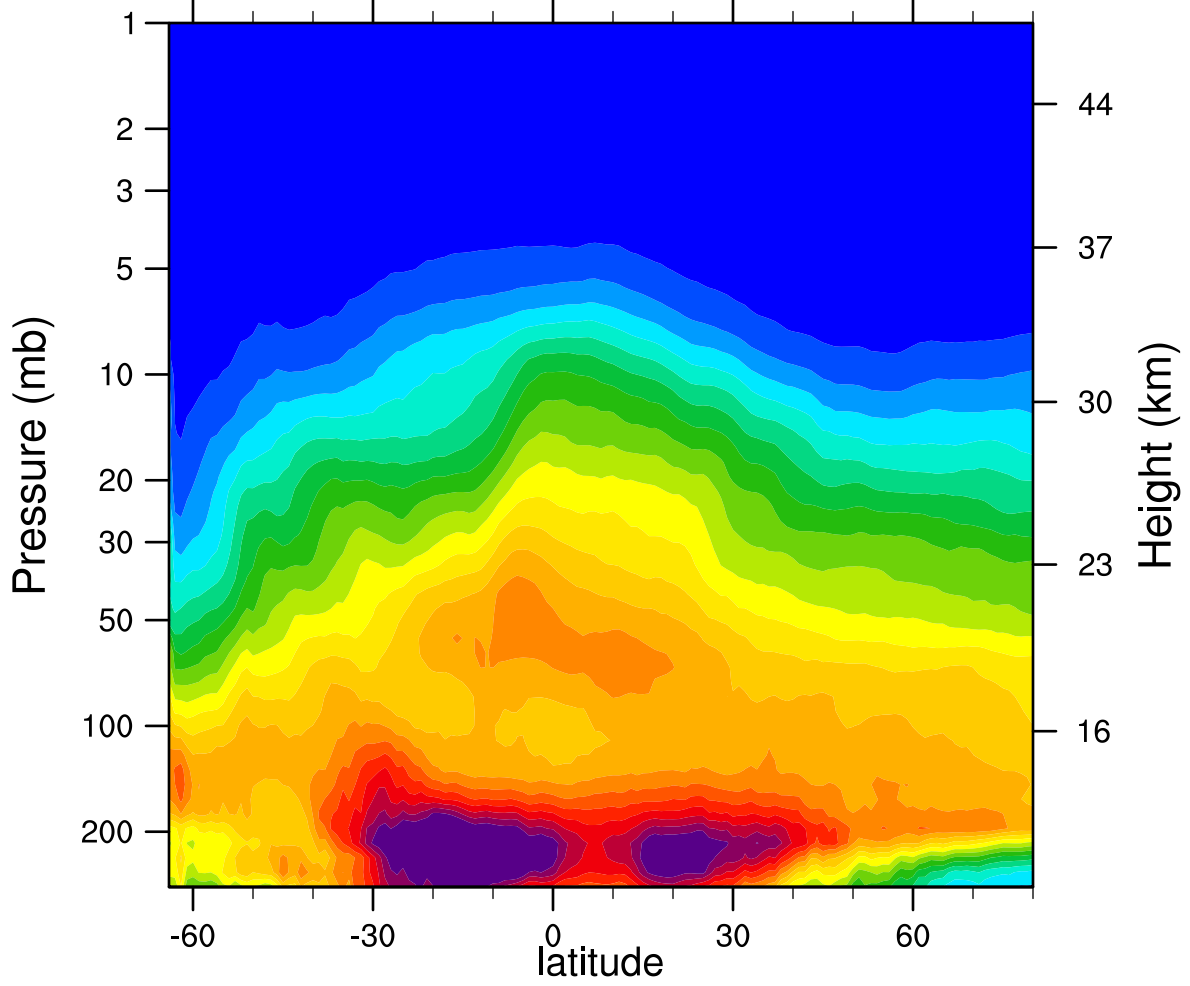
2006d181 N2O_Combined (ppbv)
