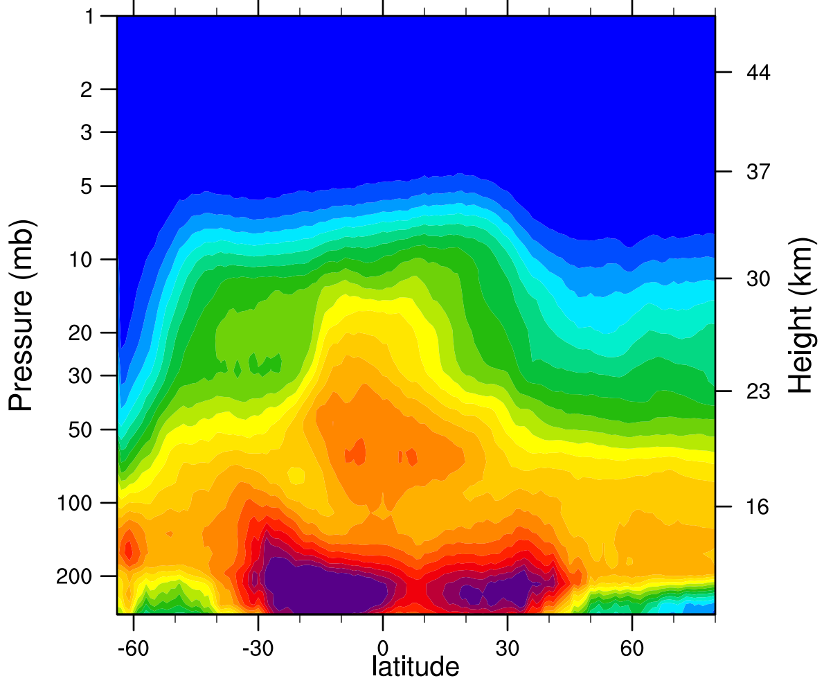
2007d206 N2O_Combined (ppbv)
