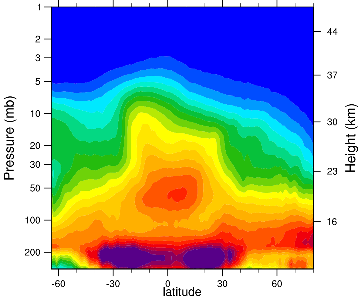
2005d340 N2O_Combined (ppbv)
