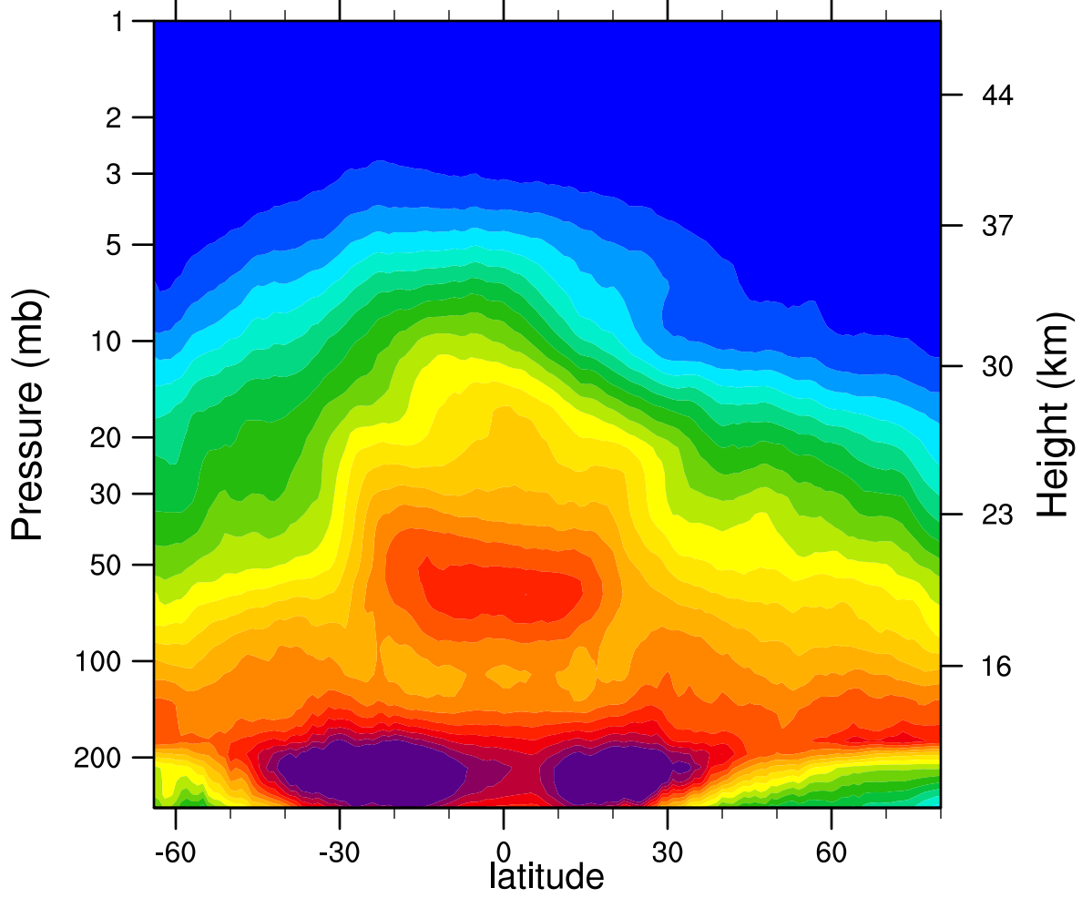
2006d111 N2O_Combined (ppbv)
