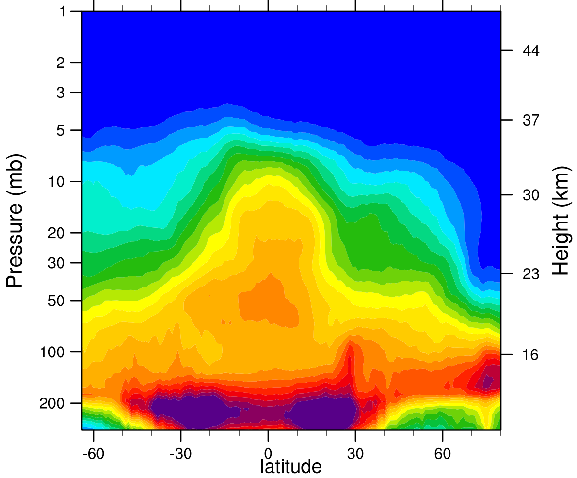
2007d003 N2O_Combined (ppbv)
