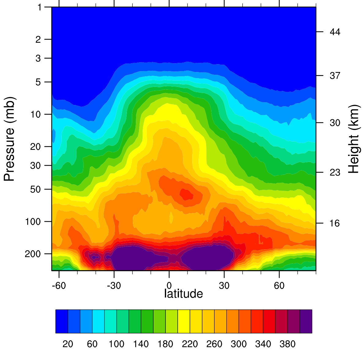
2005d092 N2O_Combined (ppbv)
