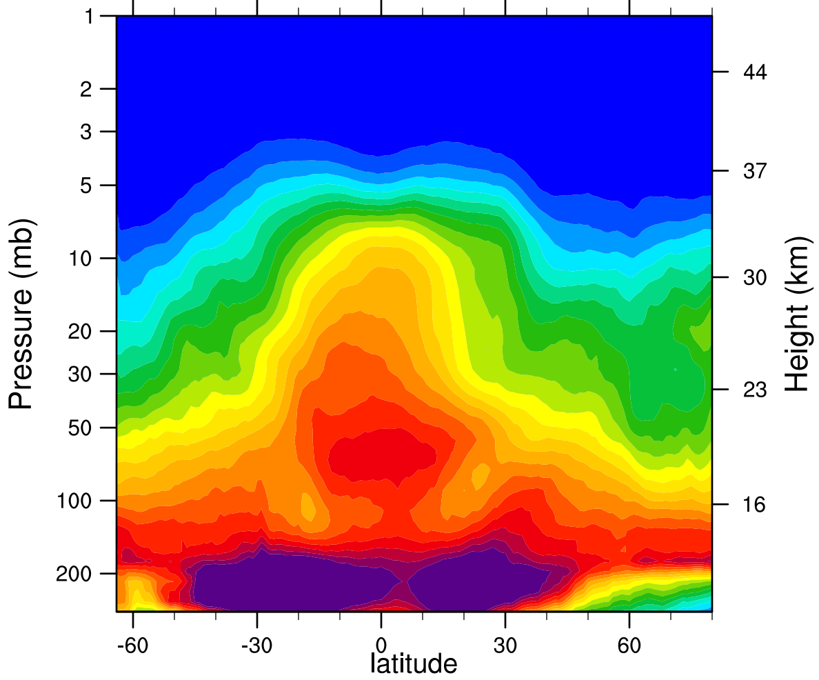
2007d119 N2O_Combined (ppbv)
