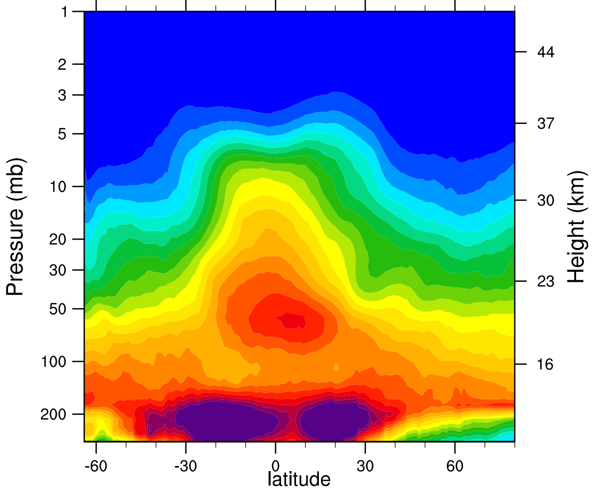
2005d123 N2O_Combined (ppbv)
