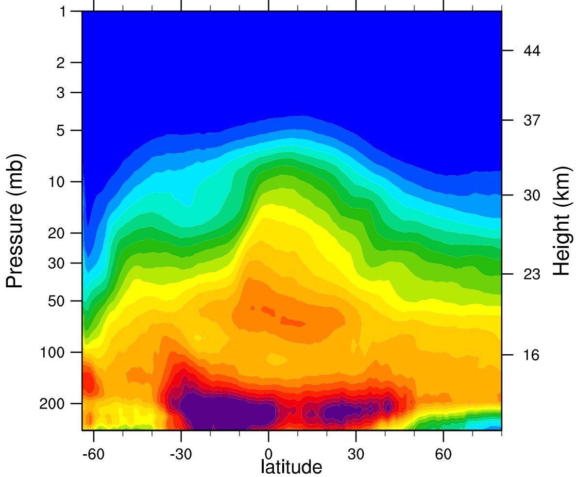
2006d222 N2O_Combined (ppbv)
