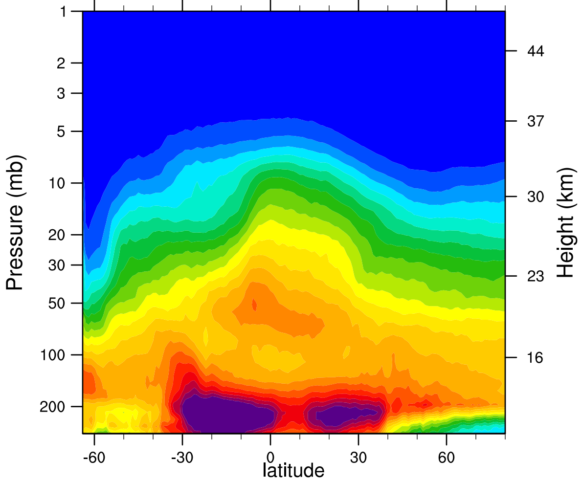
2006d190 N2O_Combined (ppbv)
