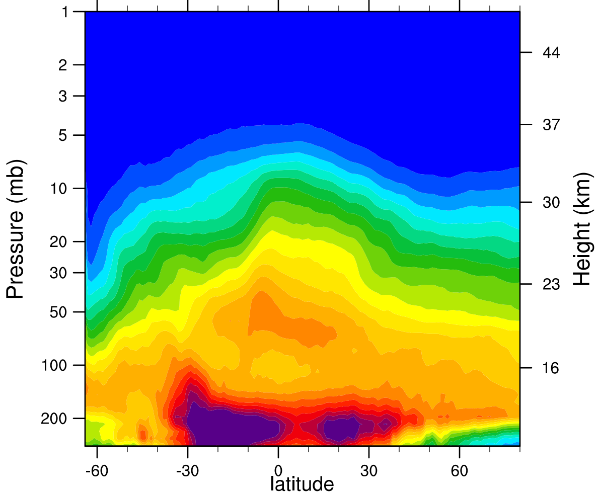
2006d183 N2O_Combined (ppbv)
