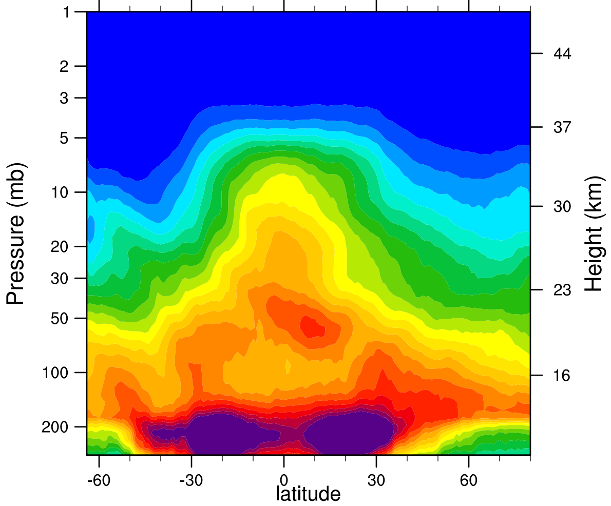
2005d093 N2O_Combined (ppbv)
