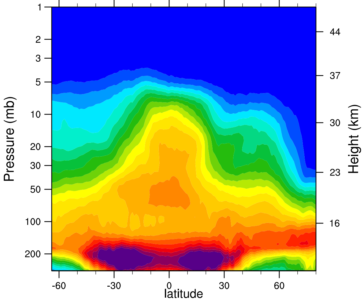
2007d010 N2O_Combined (ppbv)
