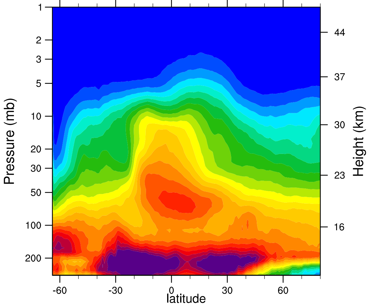
2005d190 N2O_Combined (ppbv)
