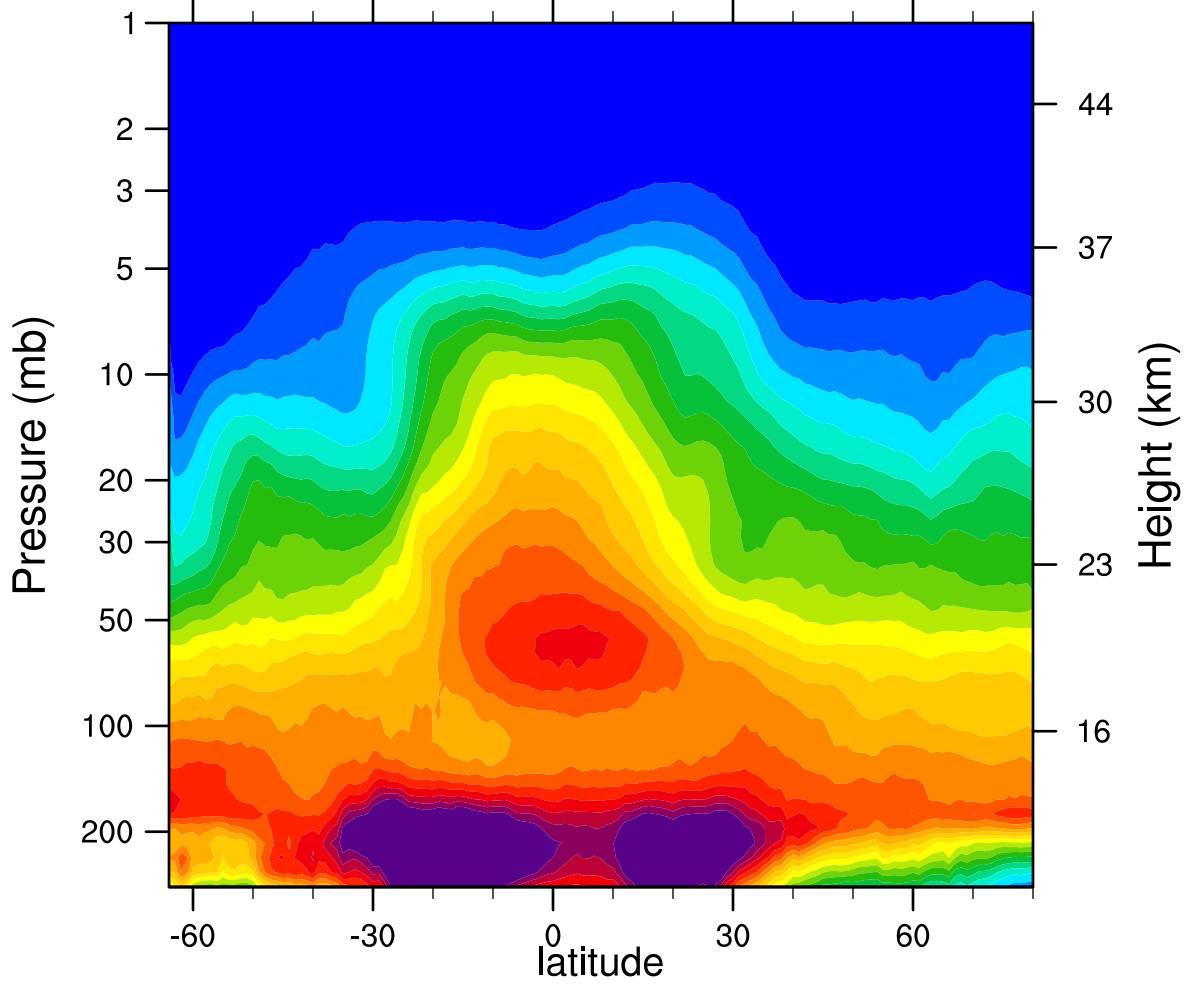
2005d136 N2O_Combined (ppbv)
