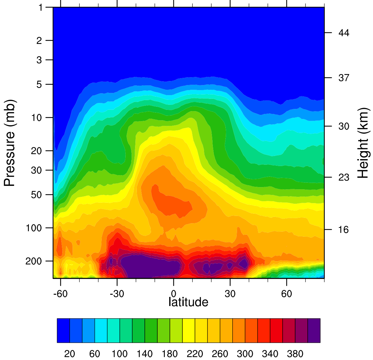
2007d175 N2O_Combined (ppbv)
