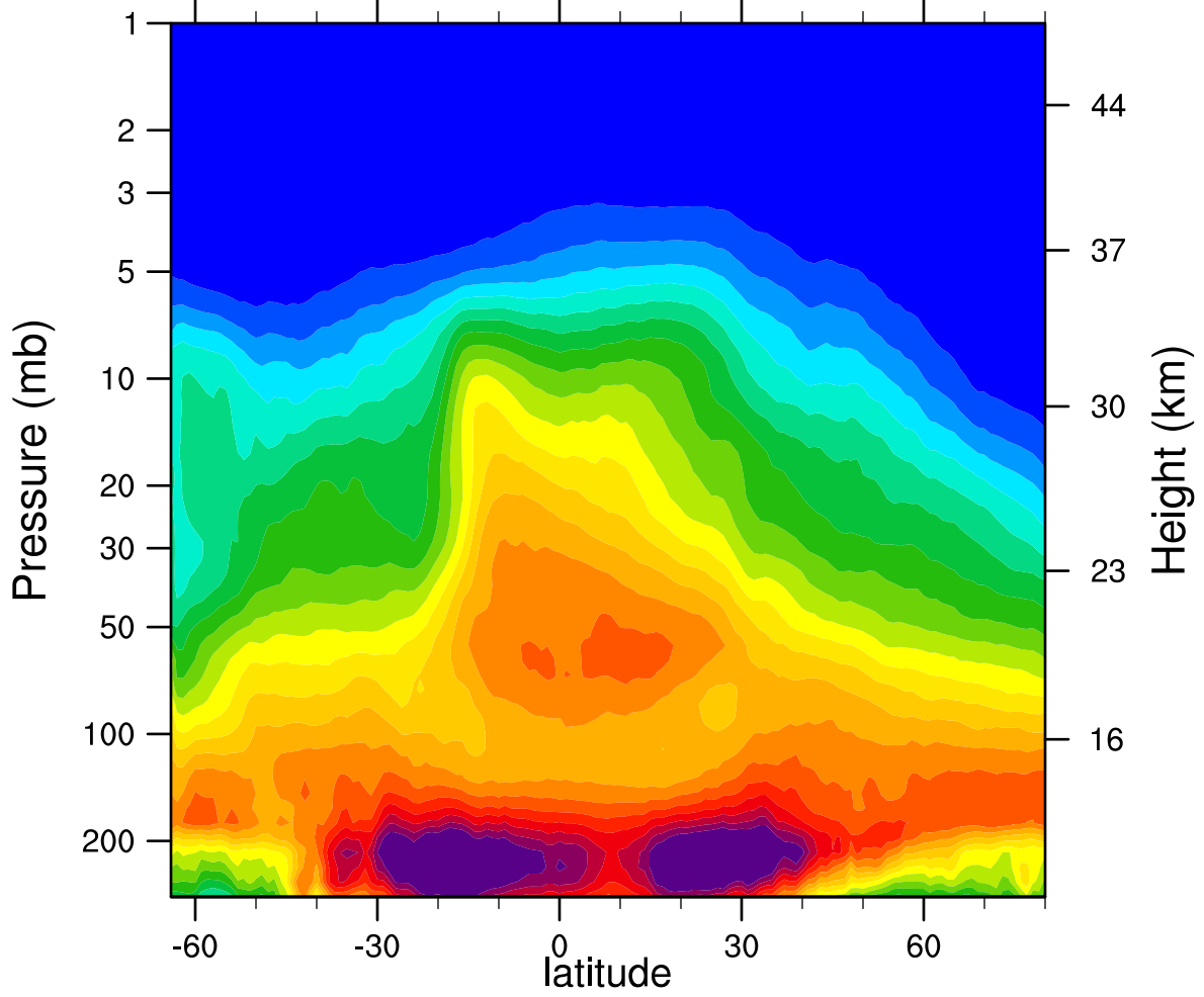
2005d288 N2O_Combined (ppbv)
