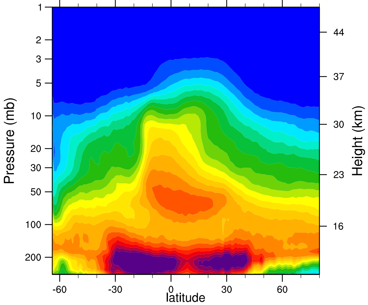
2005d245 N2O_Combined (ppbv)
