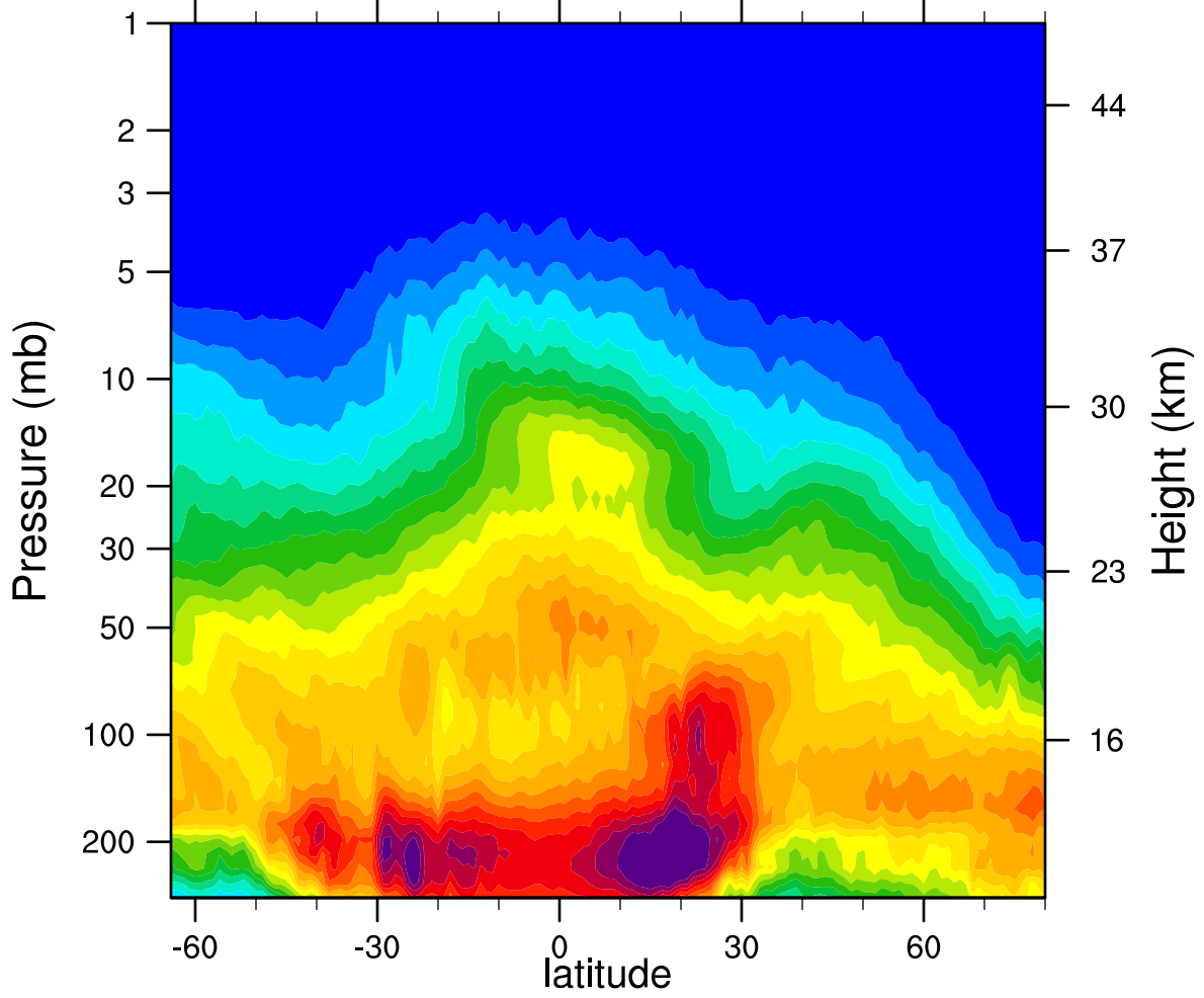
2005d026 N2O_Combined (ppbv)
