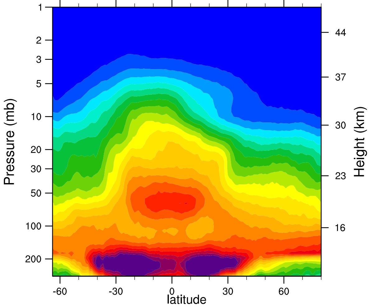
2006d098 N2O_Combined (ppbv)
