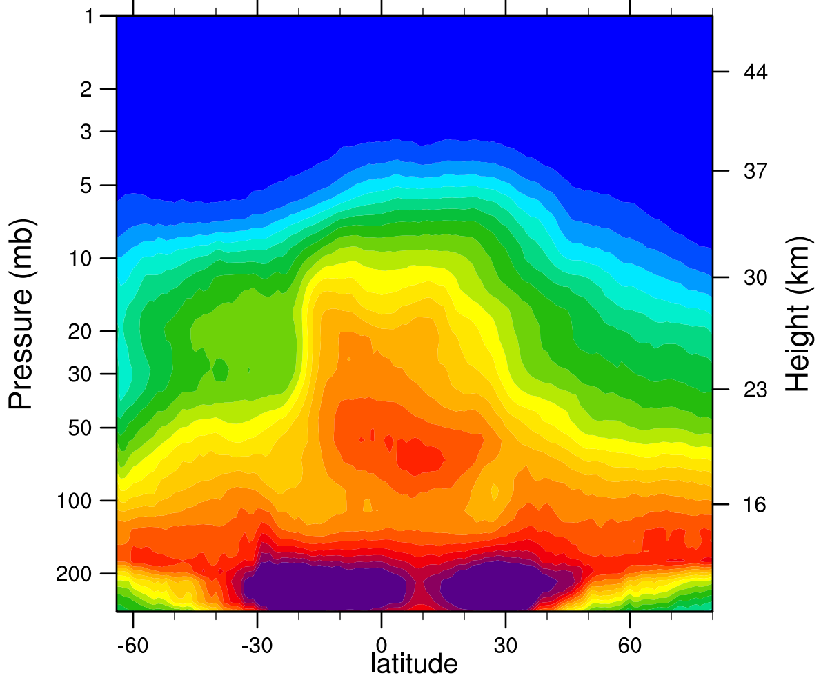
2007d281 N2O_Combined (ppbv)
