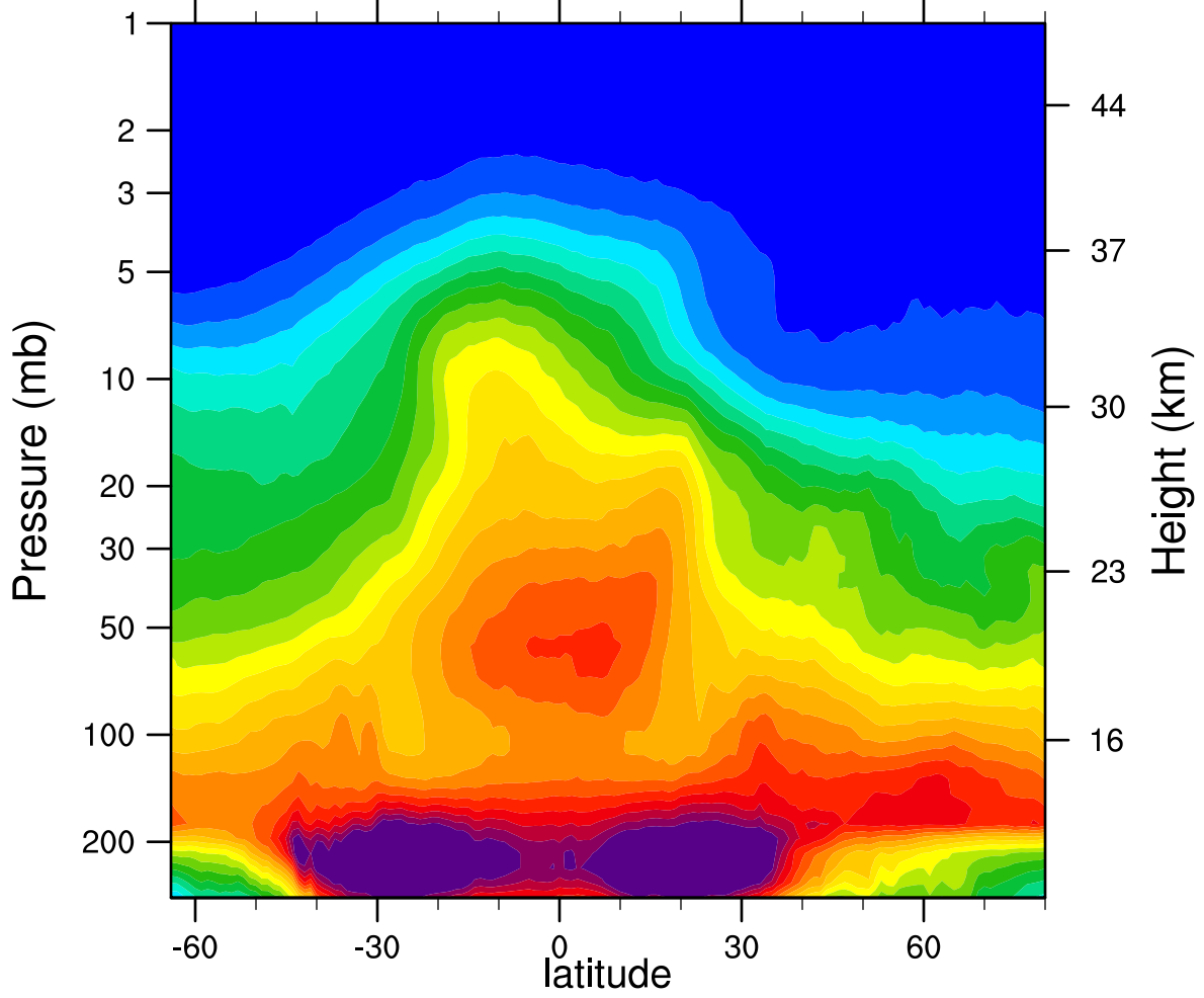
2006d034 N2O_Combined (ppbv)
