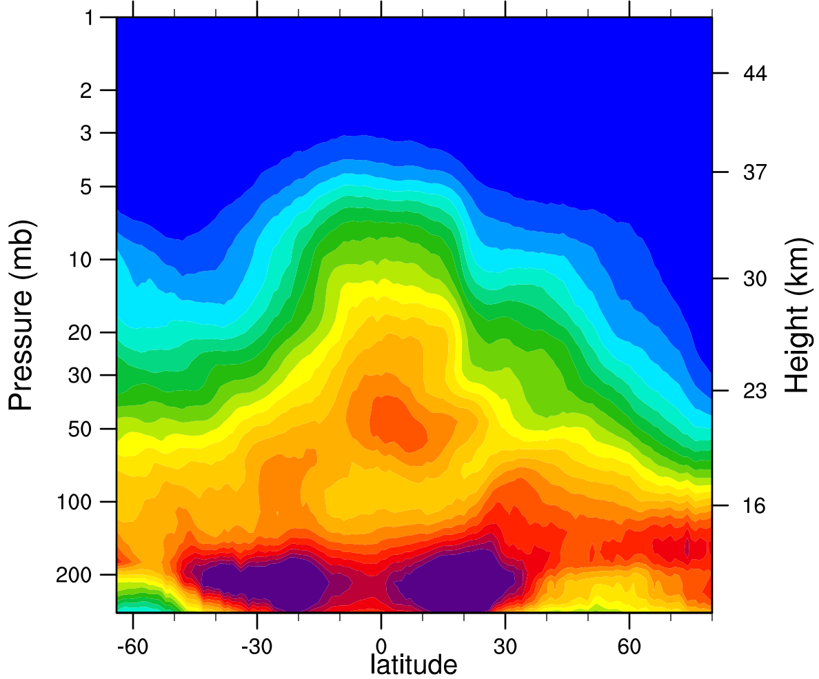
2005d047 N2O_Combined (ppbv)
