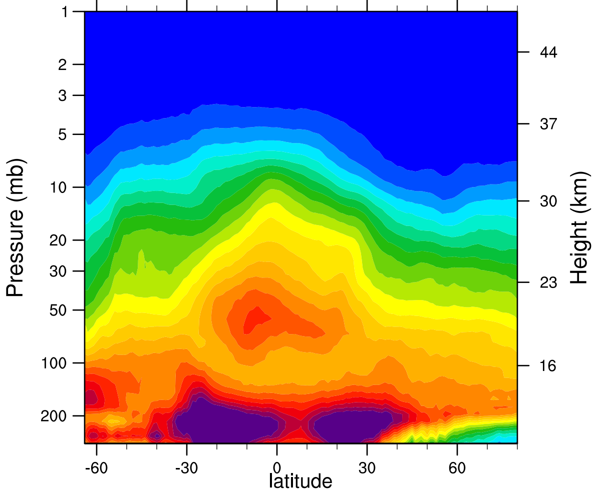
2006d160 N2O_Combined (ppbv)
