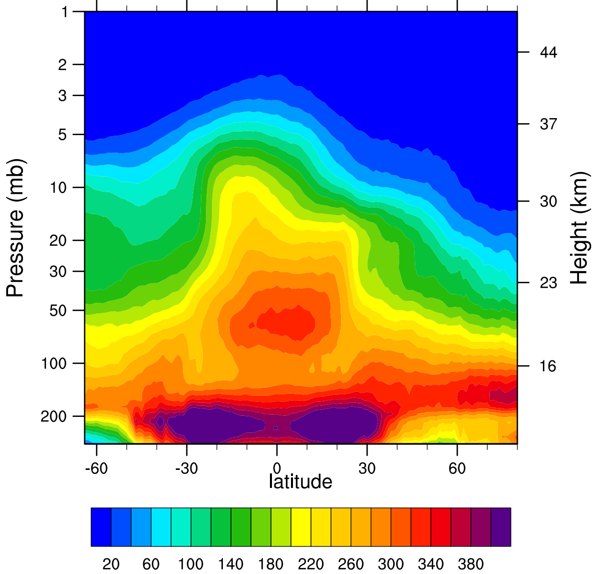
2006d004 N2O_Combined (ppbv)
