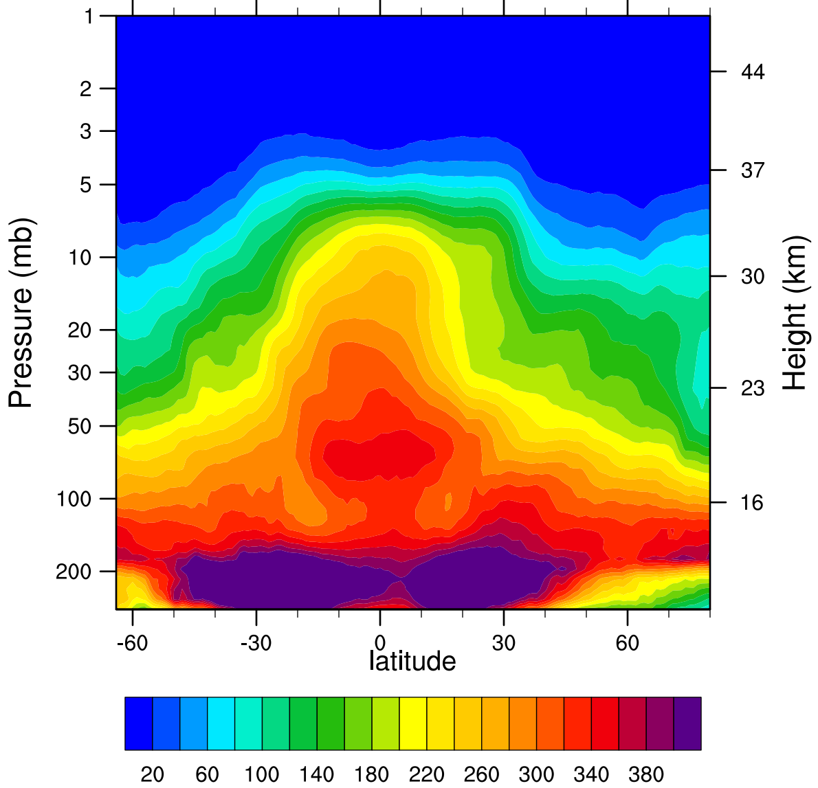
2007d109 N2O_Combined (ppbv)
