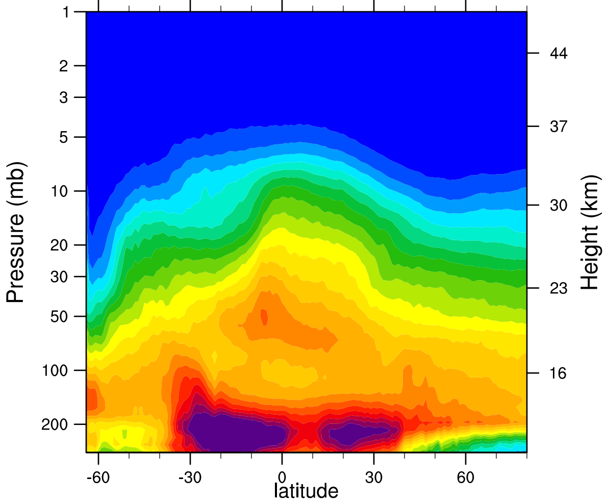
2006d189 N2O_Combined (ppbv)
