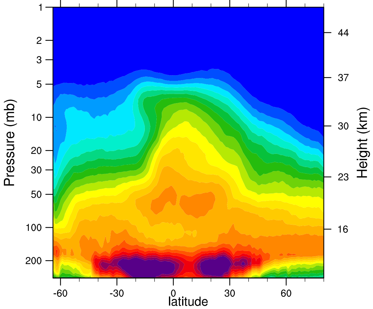
2006d286 N2O_Combined (ppbv)
