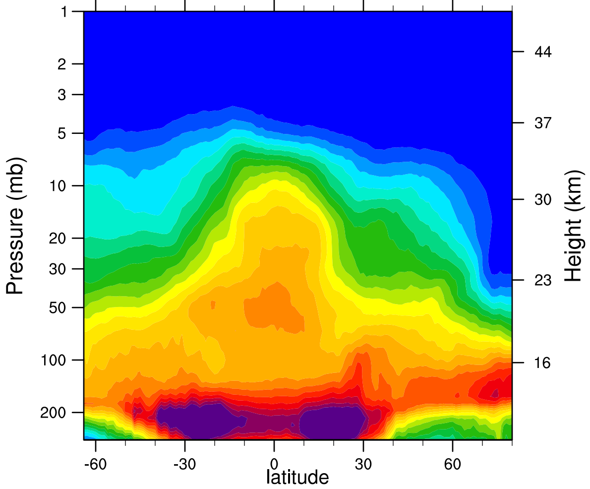
2007d002 N2O_Combined (ppbv)
