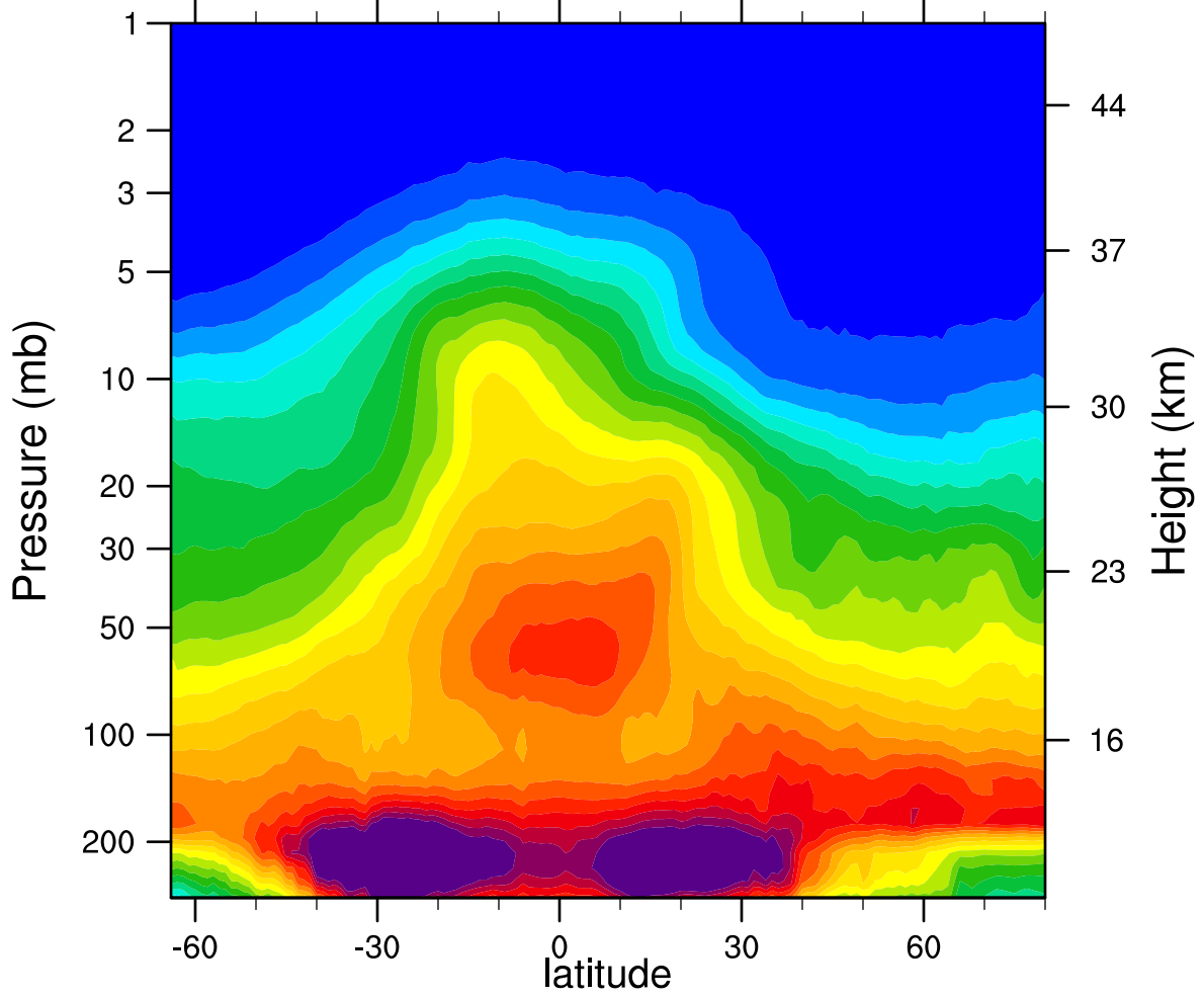
2006d040 N2O_Combined (ppbv)
