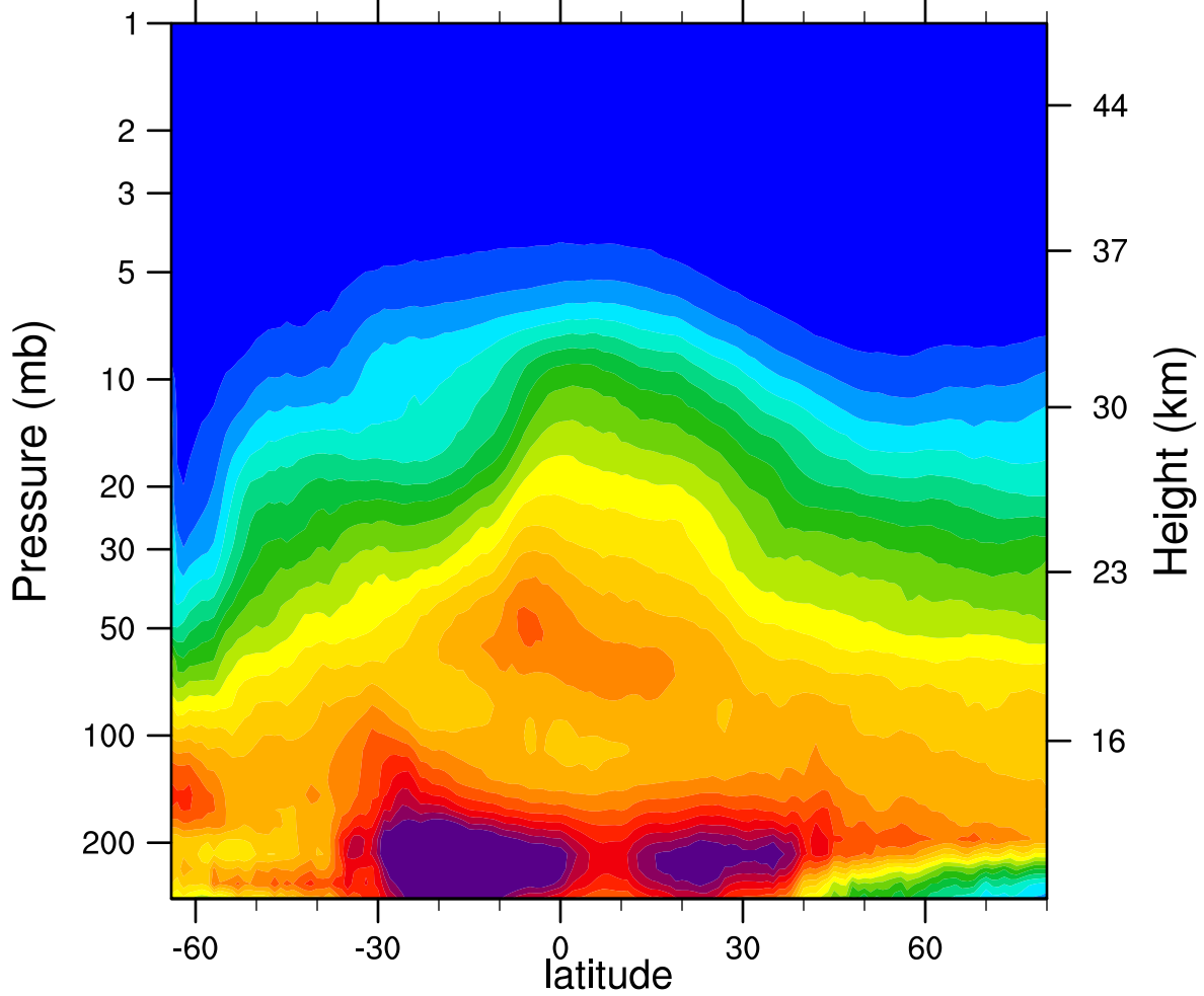
2006d192 N2O_Combined (ppbv)
