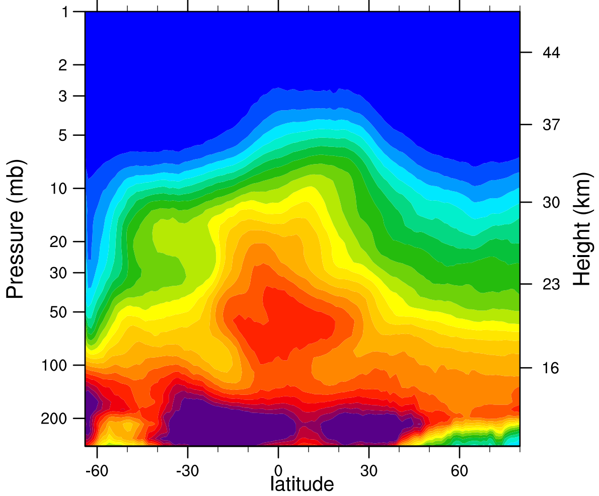
2007d236 N2O_Combined (ppbv)
