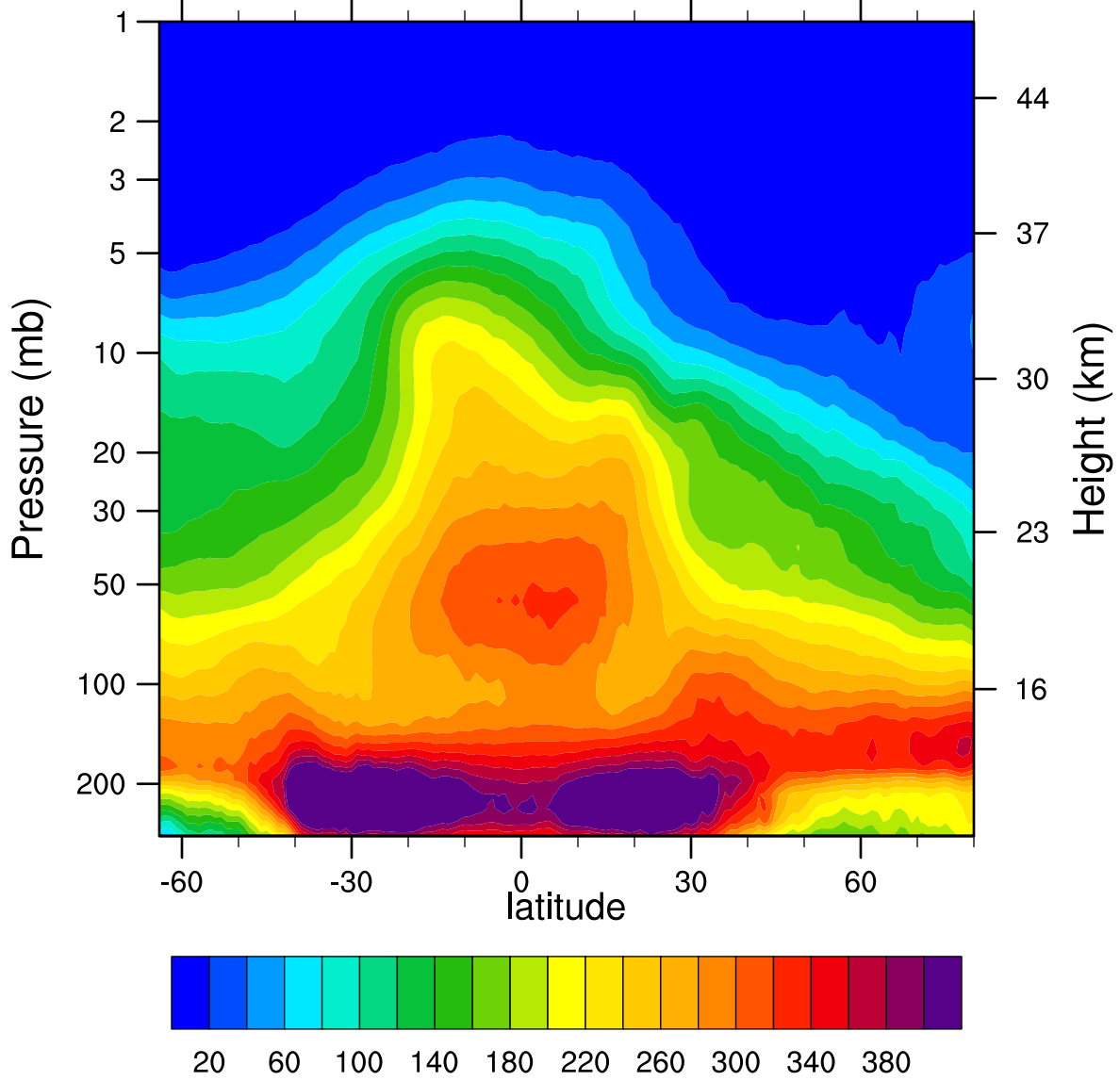
2006d023 N2O_Combined (ppbv)
