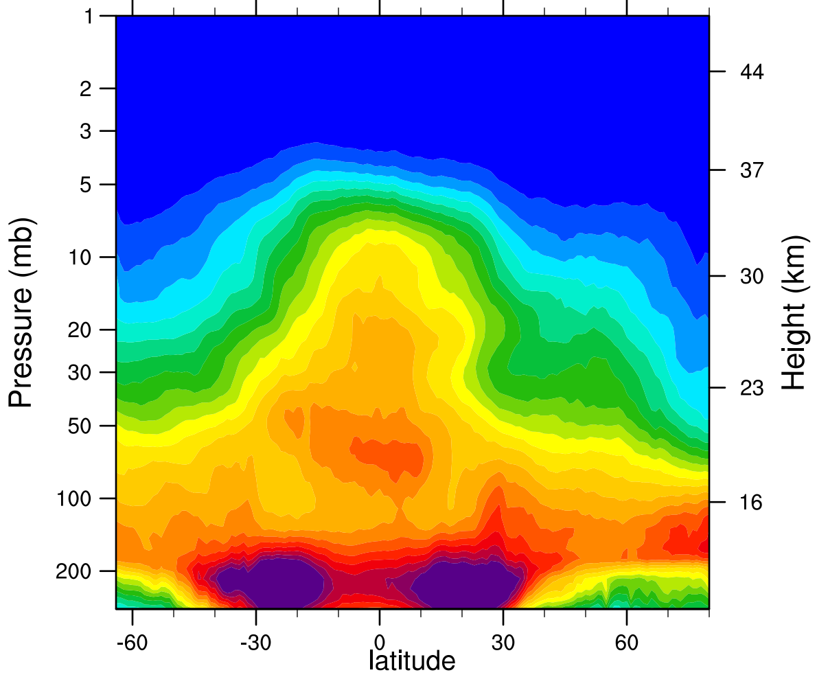
2007d064 N2O_Combined (ppbv)
