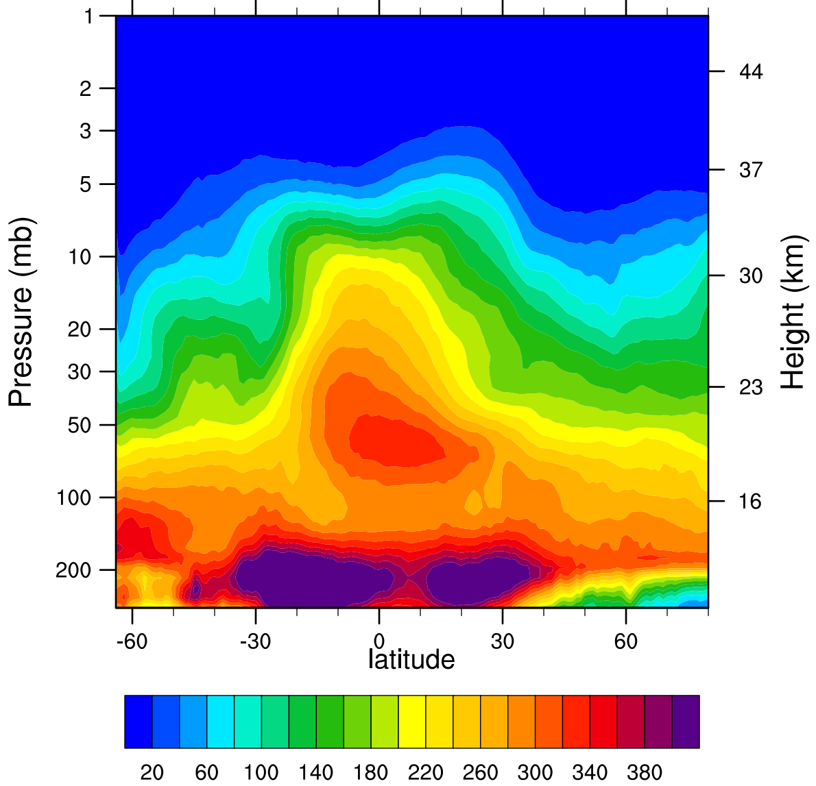
2005d155 N2O_Combined (ppbv)
