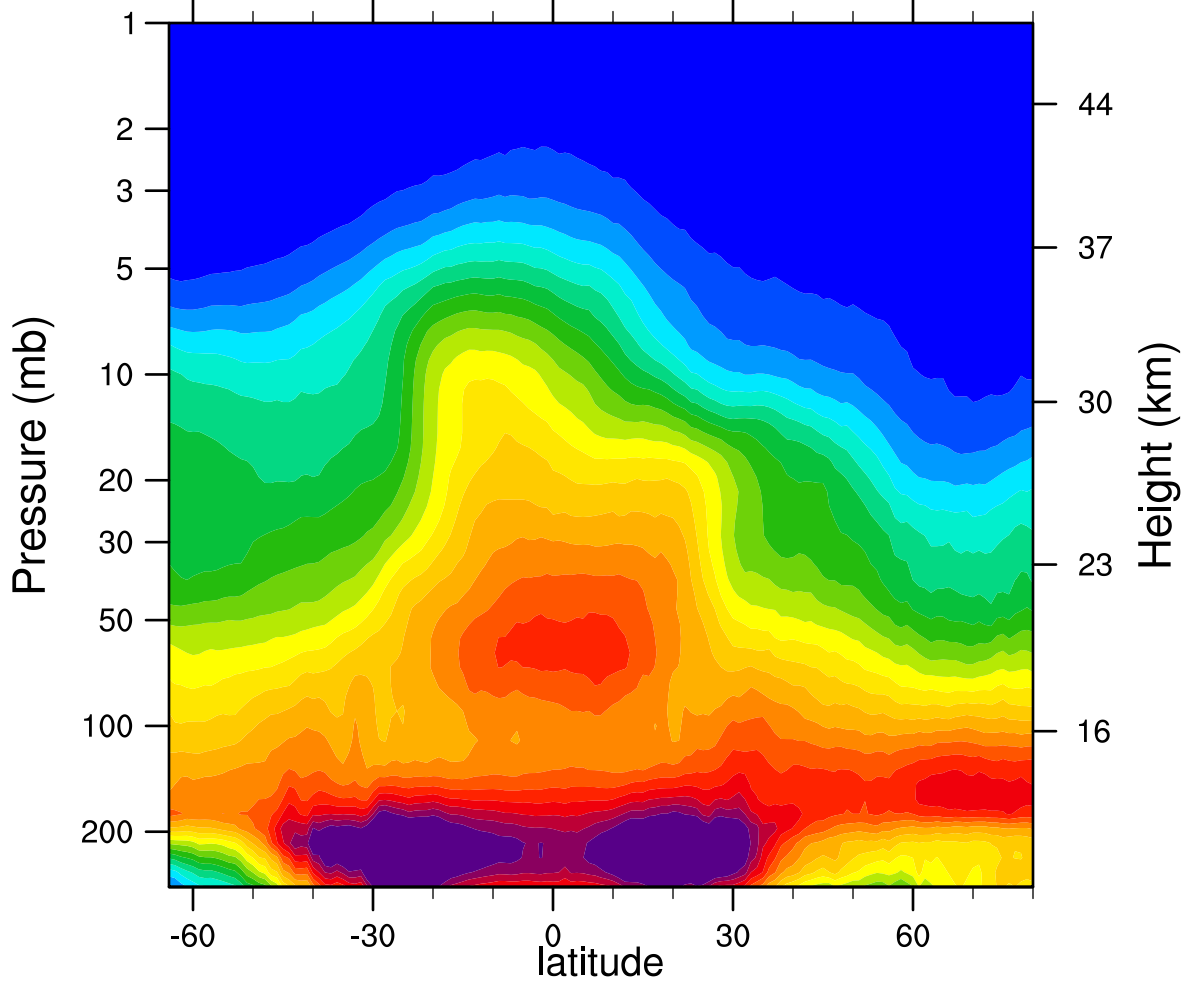
2006d007 N2O_Combined (ppbv)
