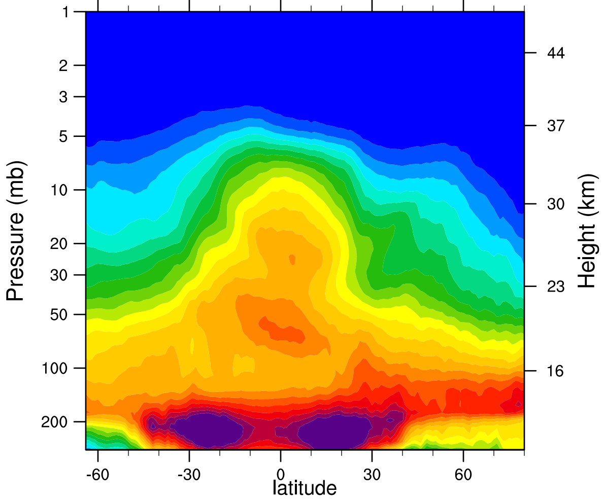
2007d030 N2O_Combined (ppbv)
