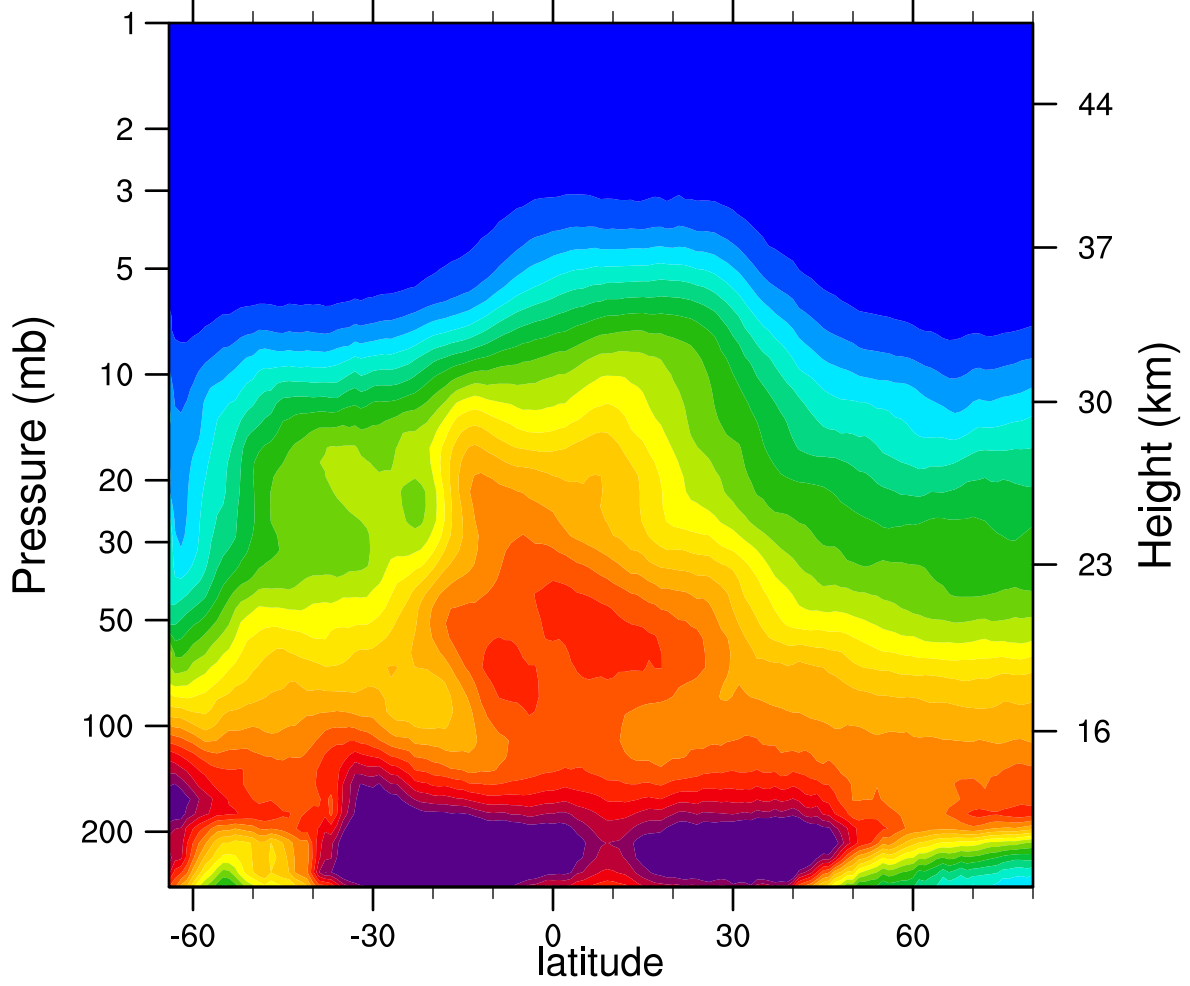
2007d244 N2O_Combined (ppbv)
