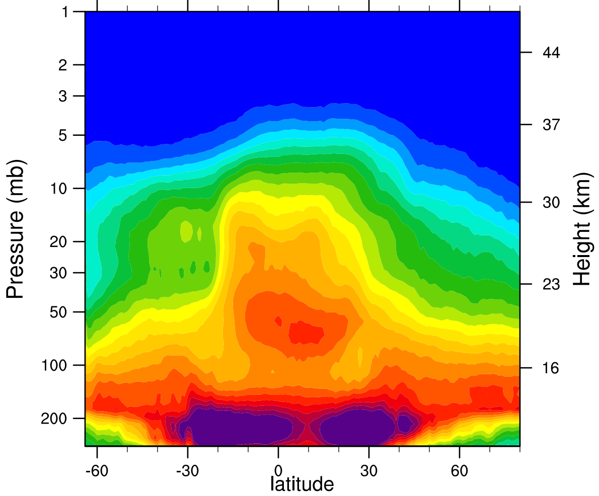
2007d284 N2O_Combined (ppbv)
