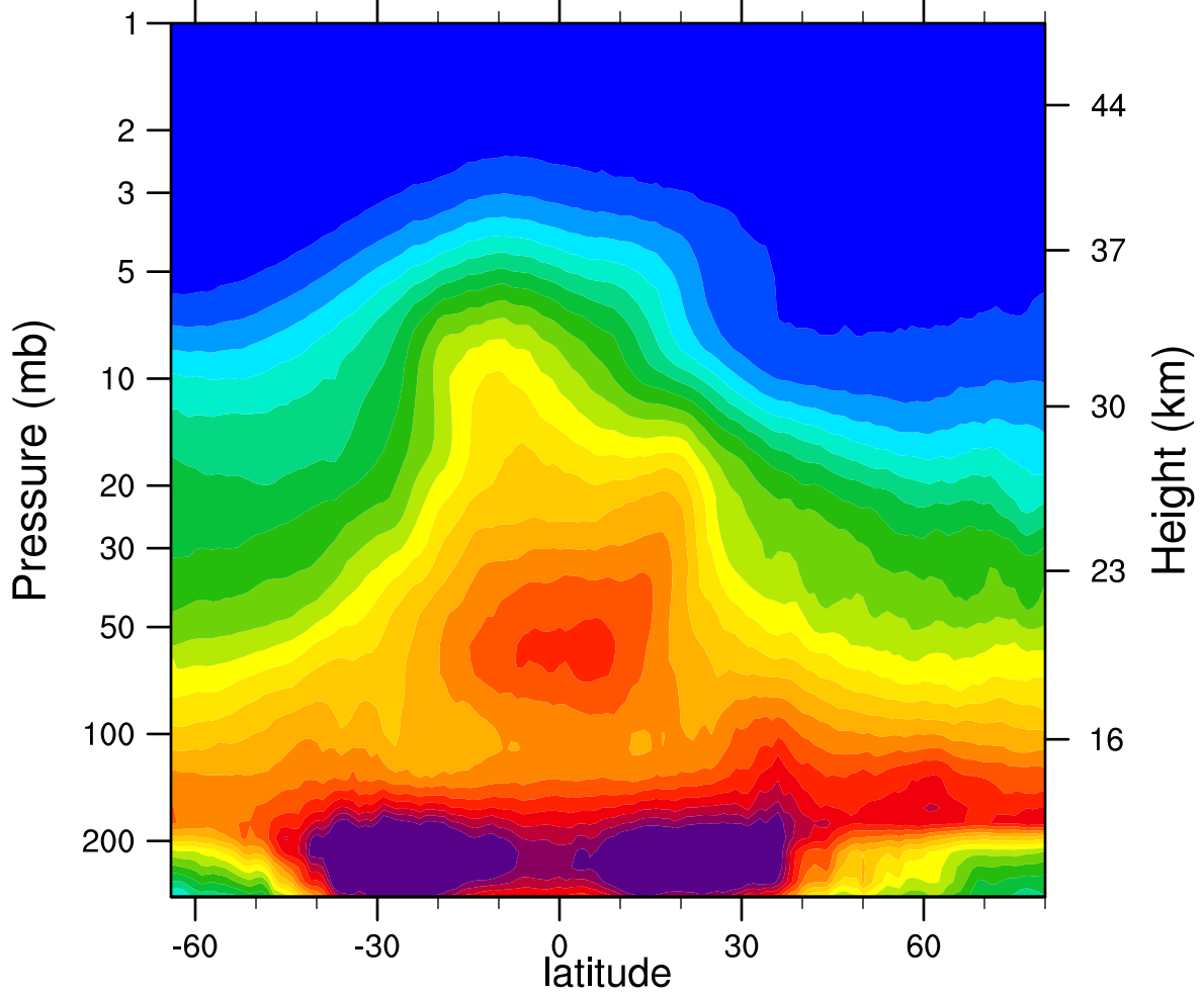
2006d037 N2O_Combined (ppbv)
