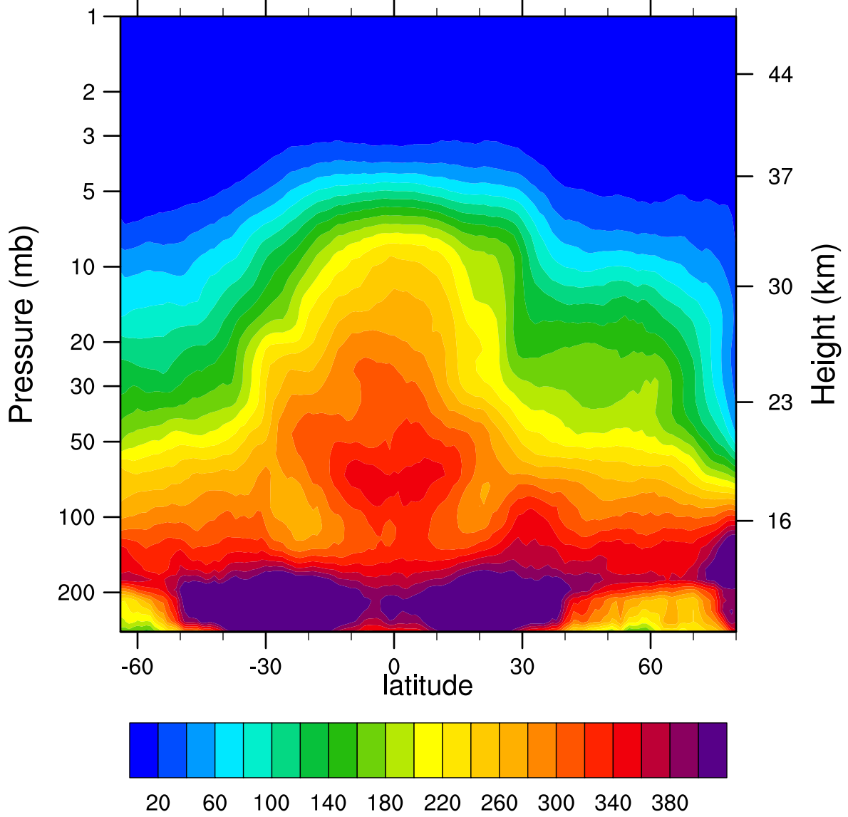
2007d086 N2O_Combined (ppbv)
