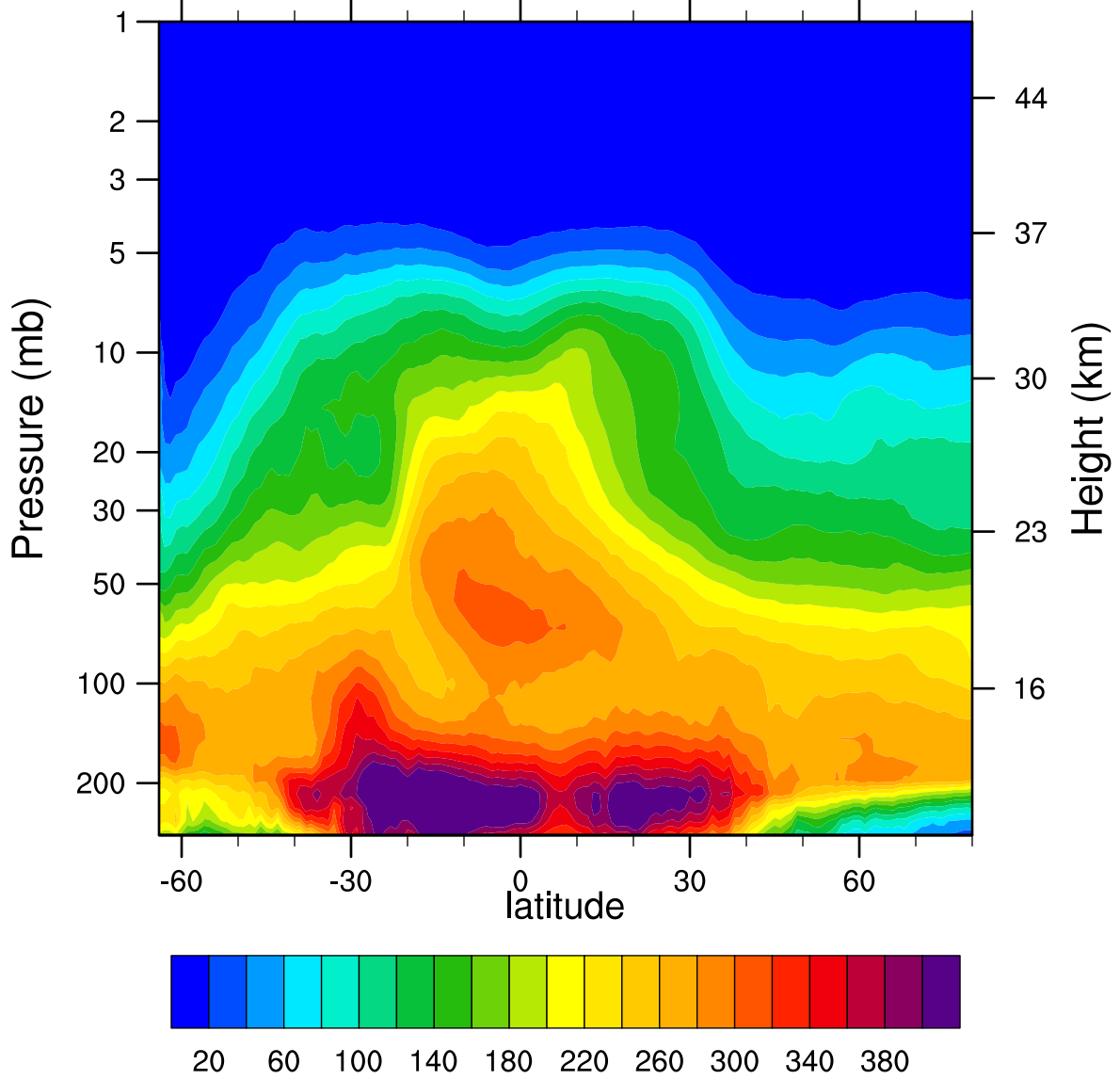
2007d169 N2O_Combined (ppbv)
