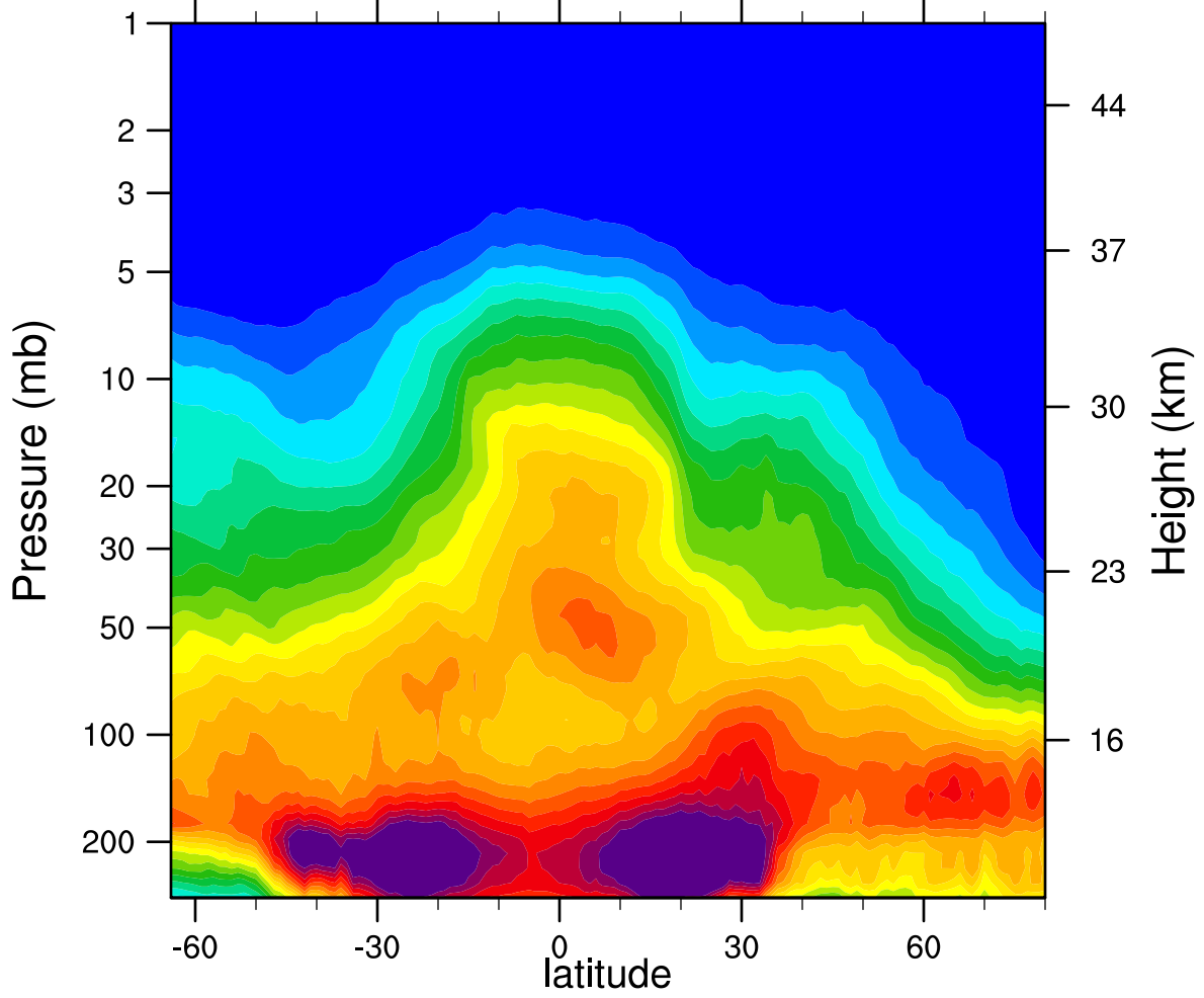
2005d038 N2O_Combined (ppbv)
