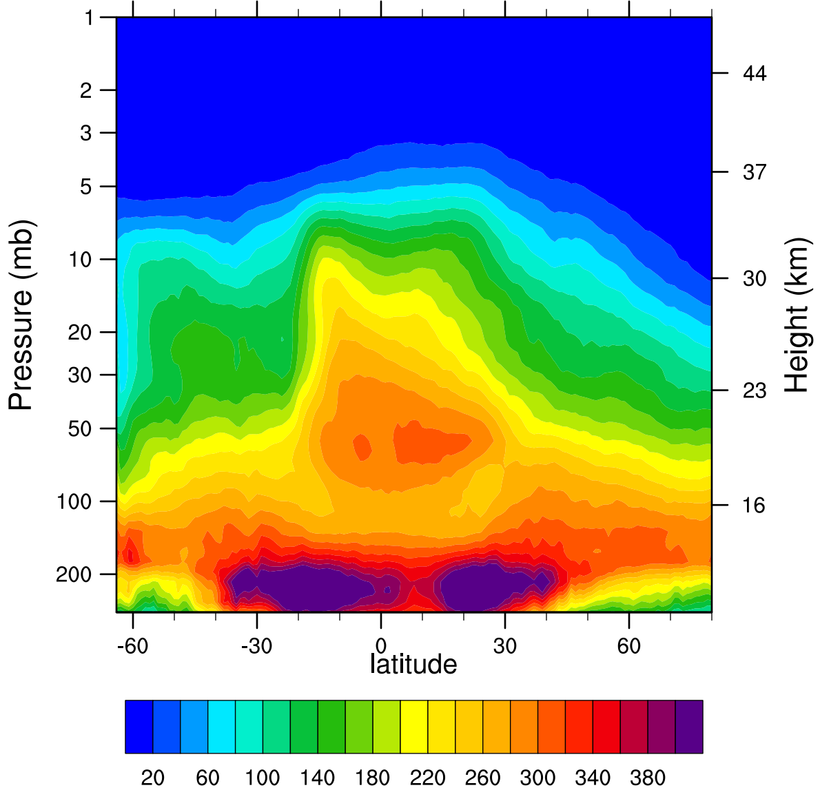
2005d293 N2O_Combined (ppbv)
