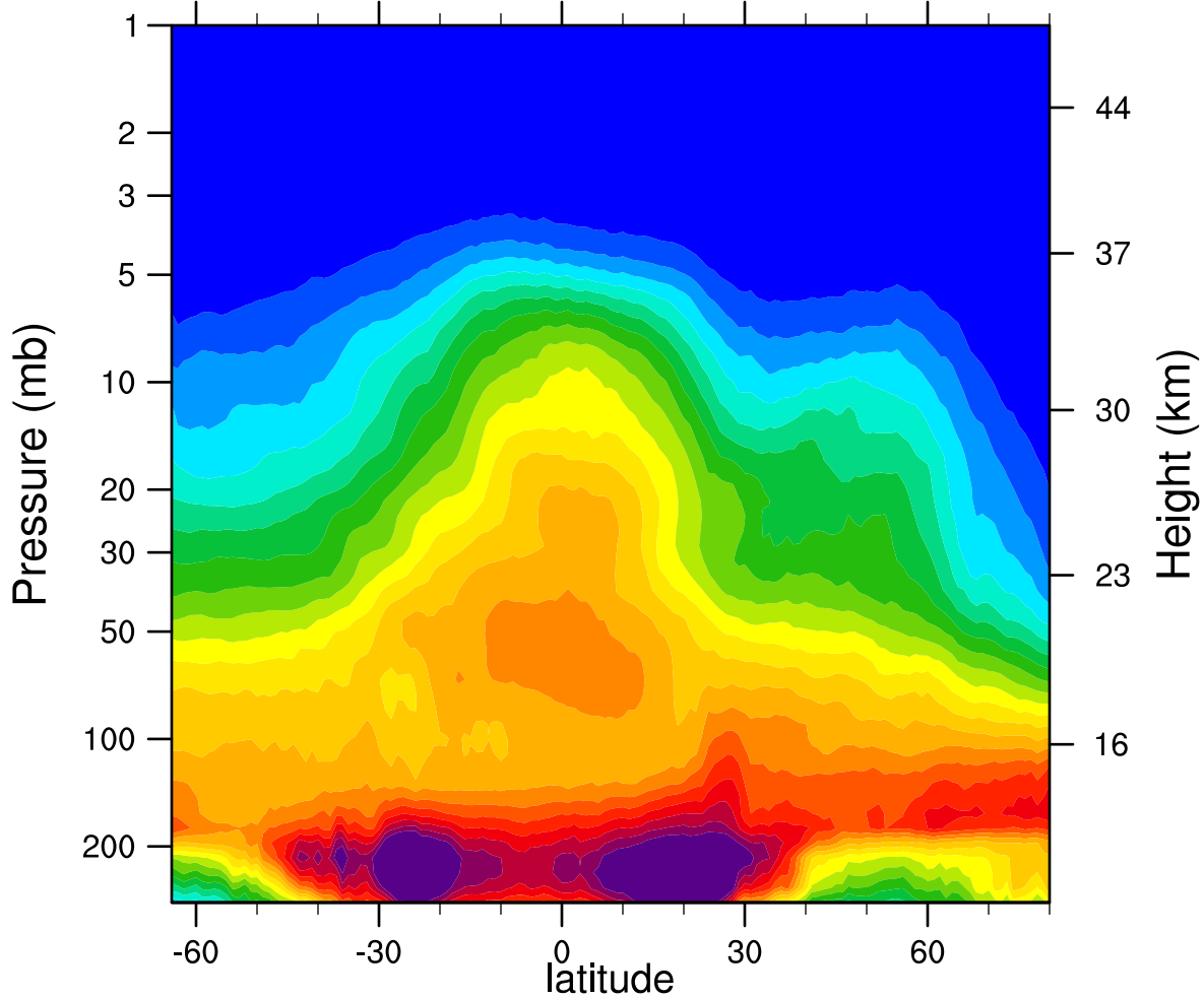
2007d046 N2O_Combined (ppbv)
