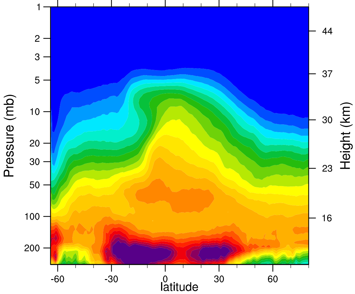
2006d262 N2O_Combined (ppbv)
