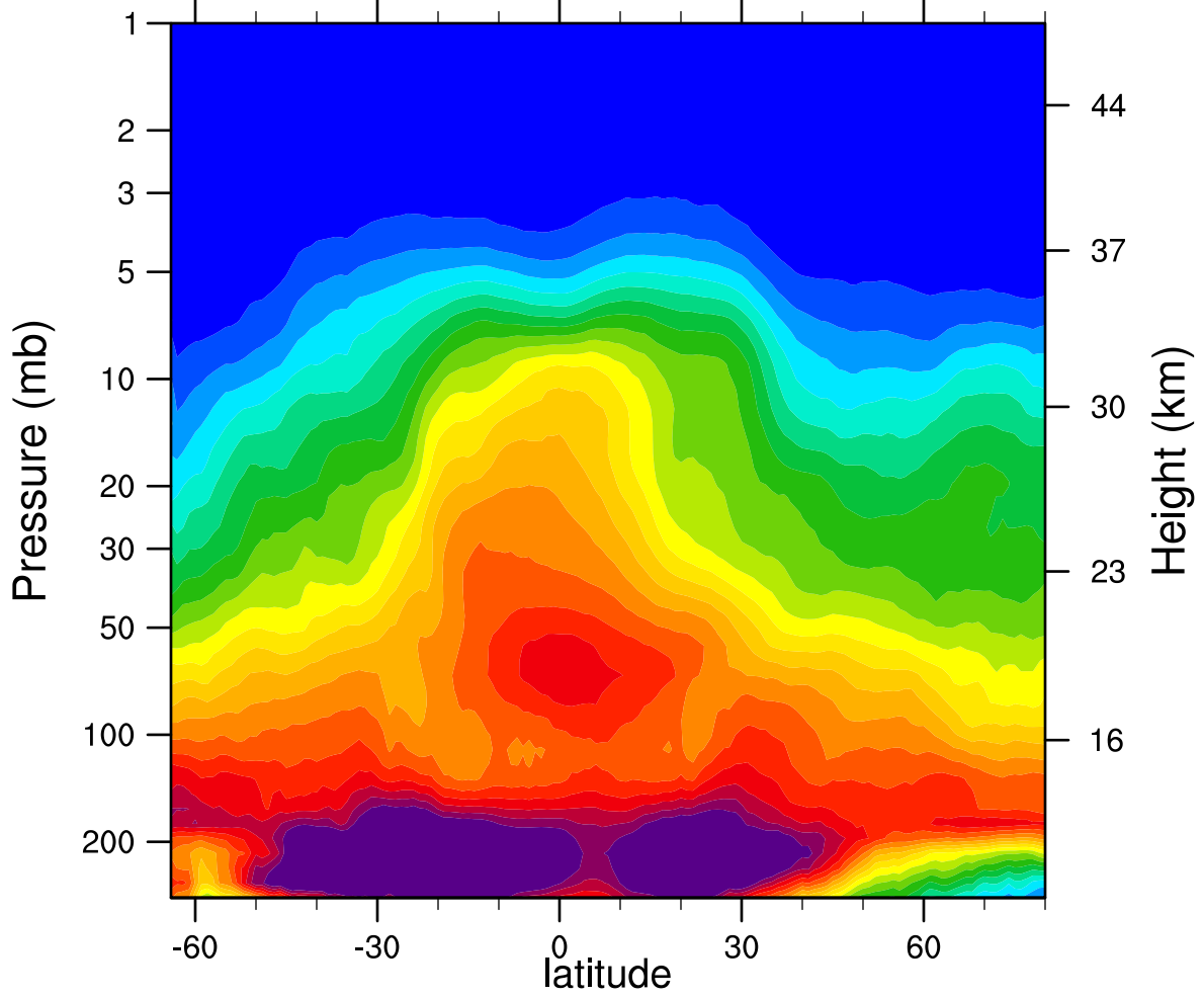
2007d134 N2O_Combined (ppbv)
