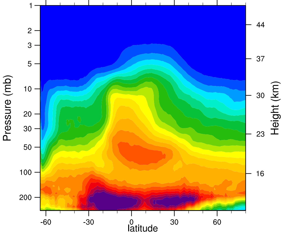
2005d240 N2O_Combined (ppbv)
