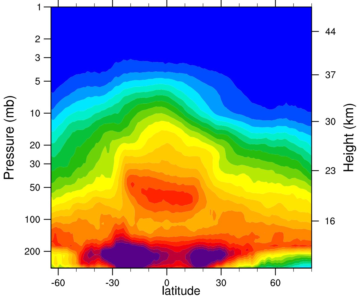
2006d124 N2O_Combined (ppbv)
