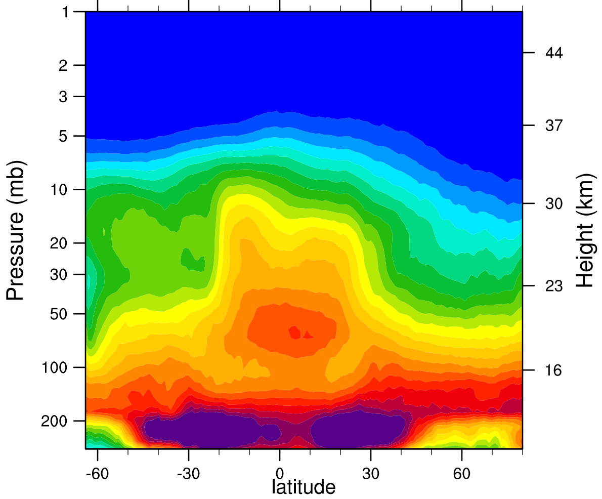
2007d325 N2O_Combined (ppbv)
