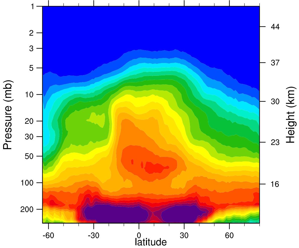
2007d277 N2O_Combined (ppbv)
