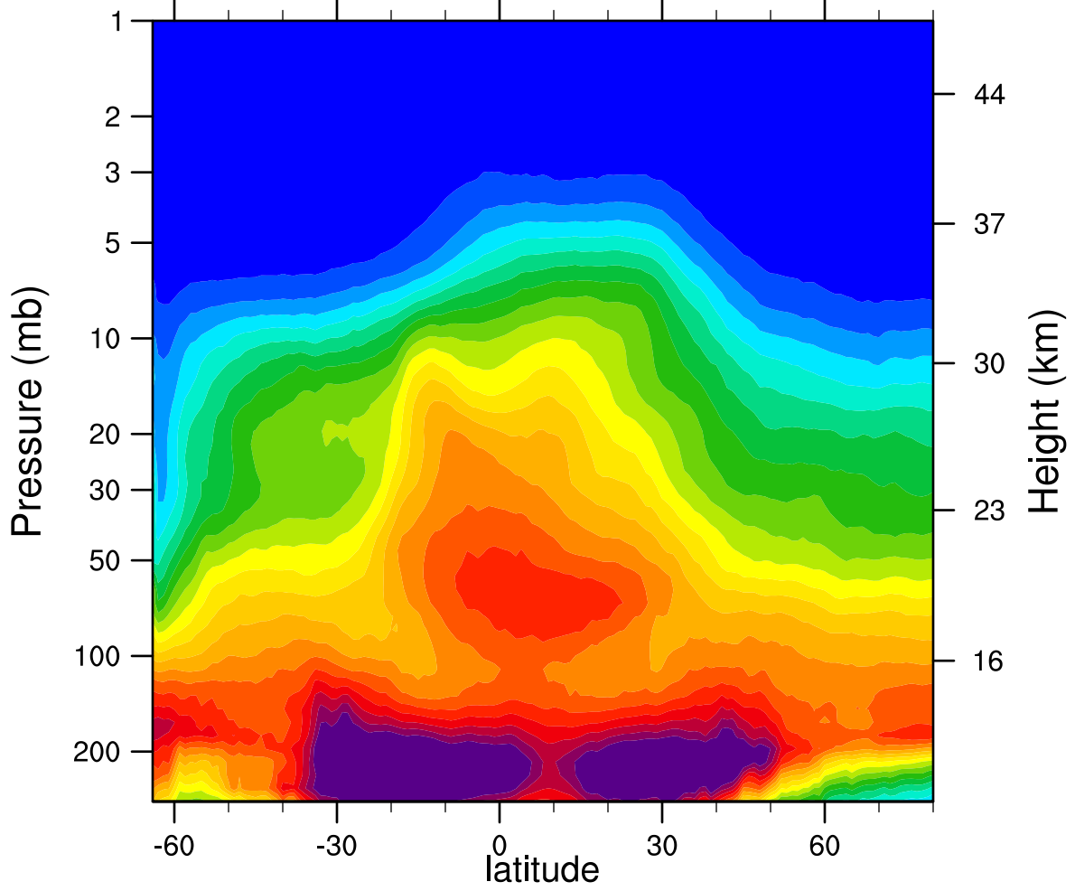
2007d255 N2O_Combined (ppbv)
