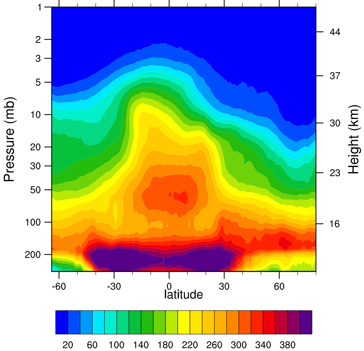
2006d018 N2O_Combined (ppbv)
