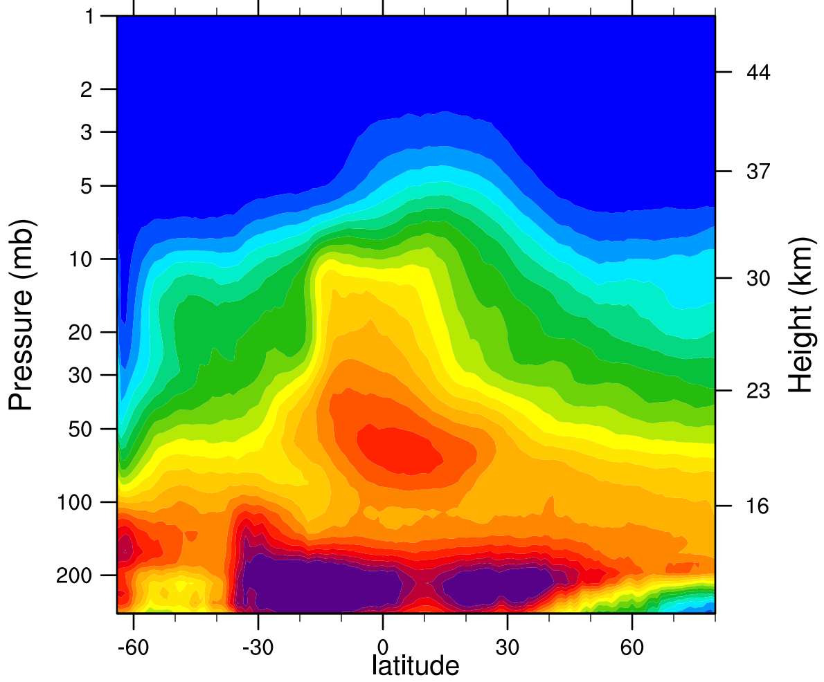
2005d216 N2O_Combined (ppbv)
