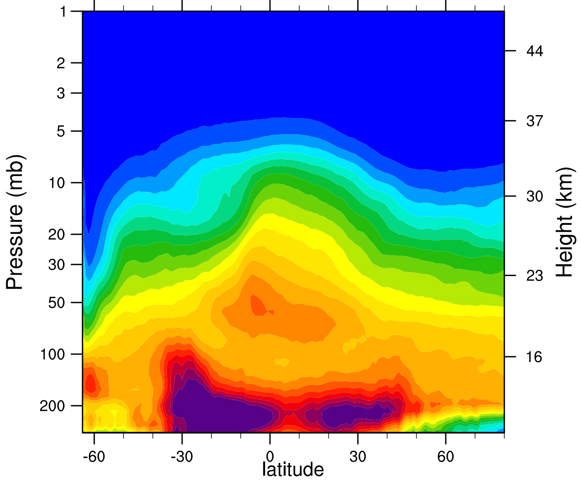
2006d202 N2O_Combined (ppbv)
