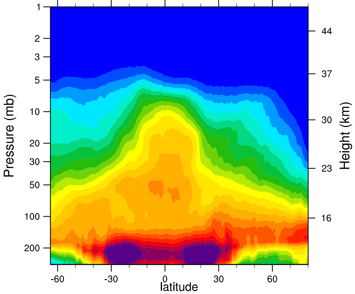
2006d362 N2O_Combined (ppbv)
