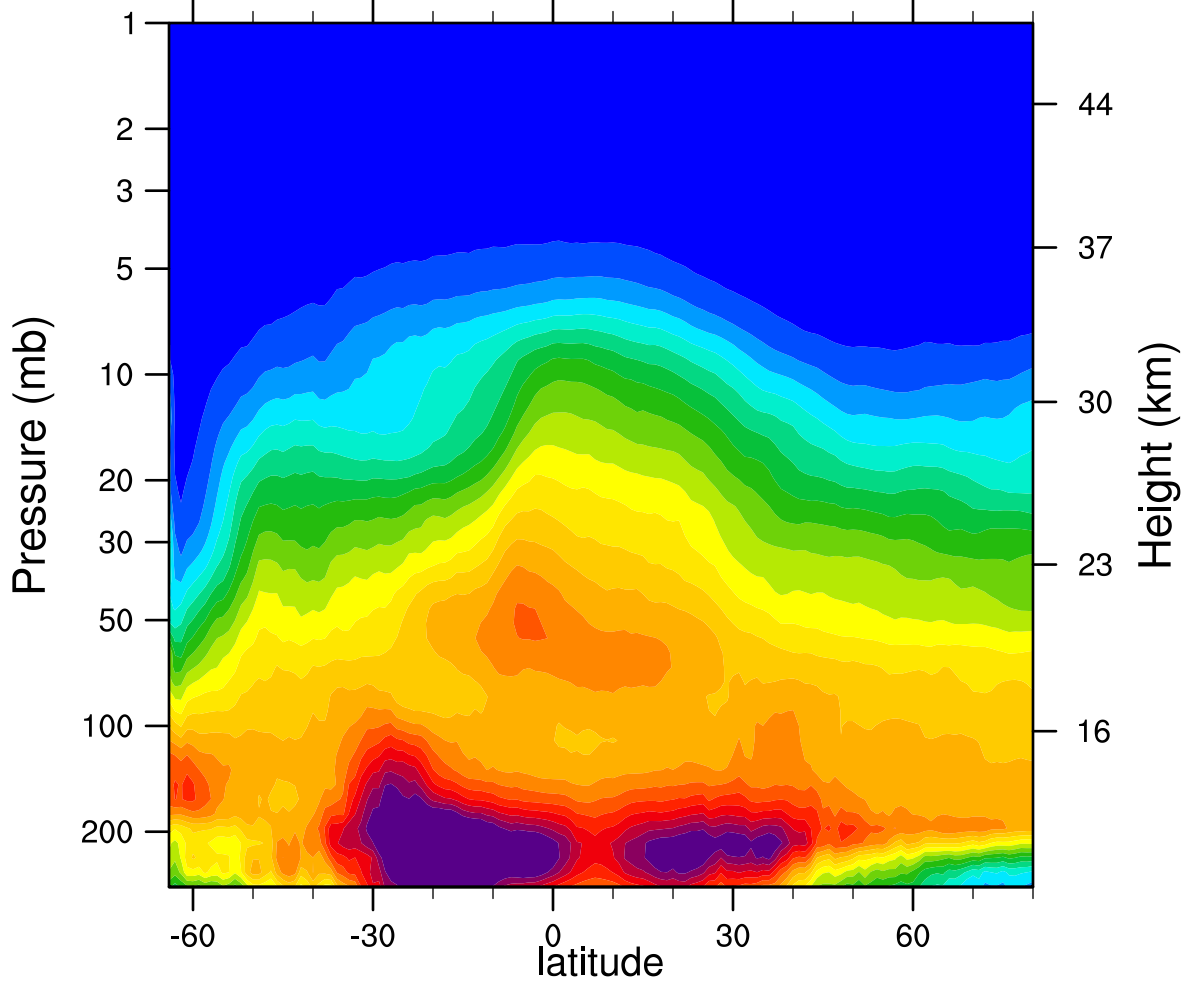
2006d196 N2O_Combined (ppbv)
