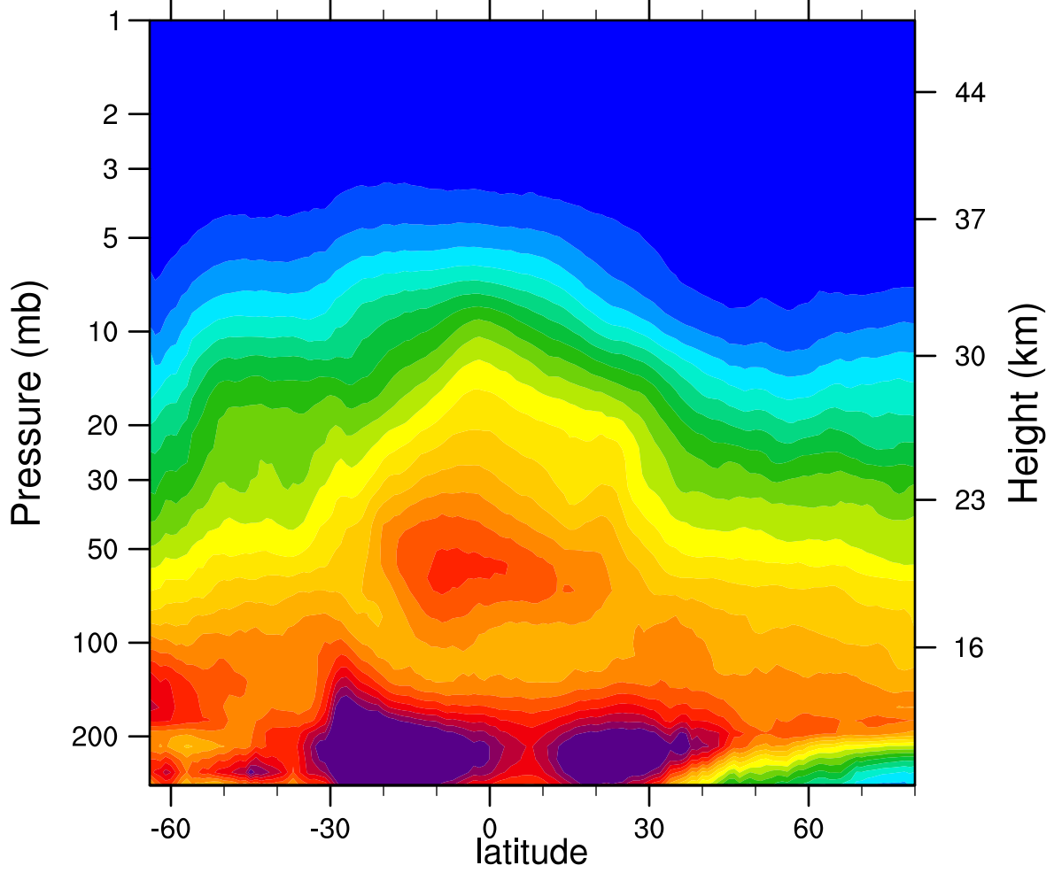
2006d155 N2O_Combined (ppbv)
