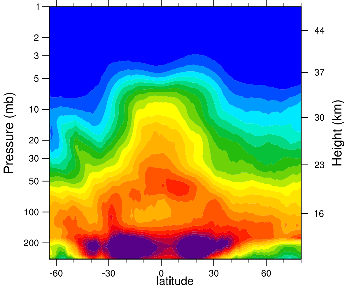
2005d112 N2O_Combined (ppbv)
