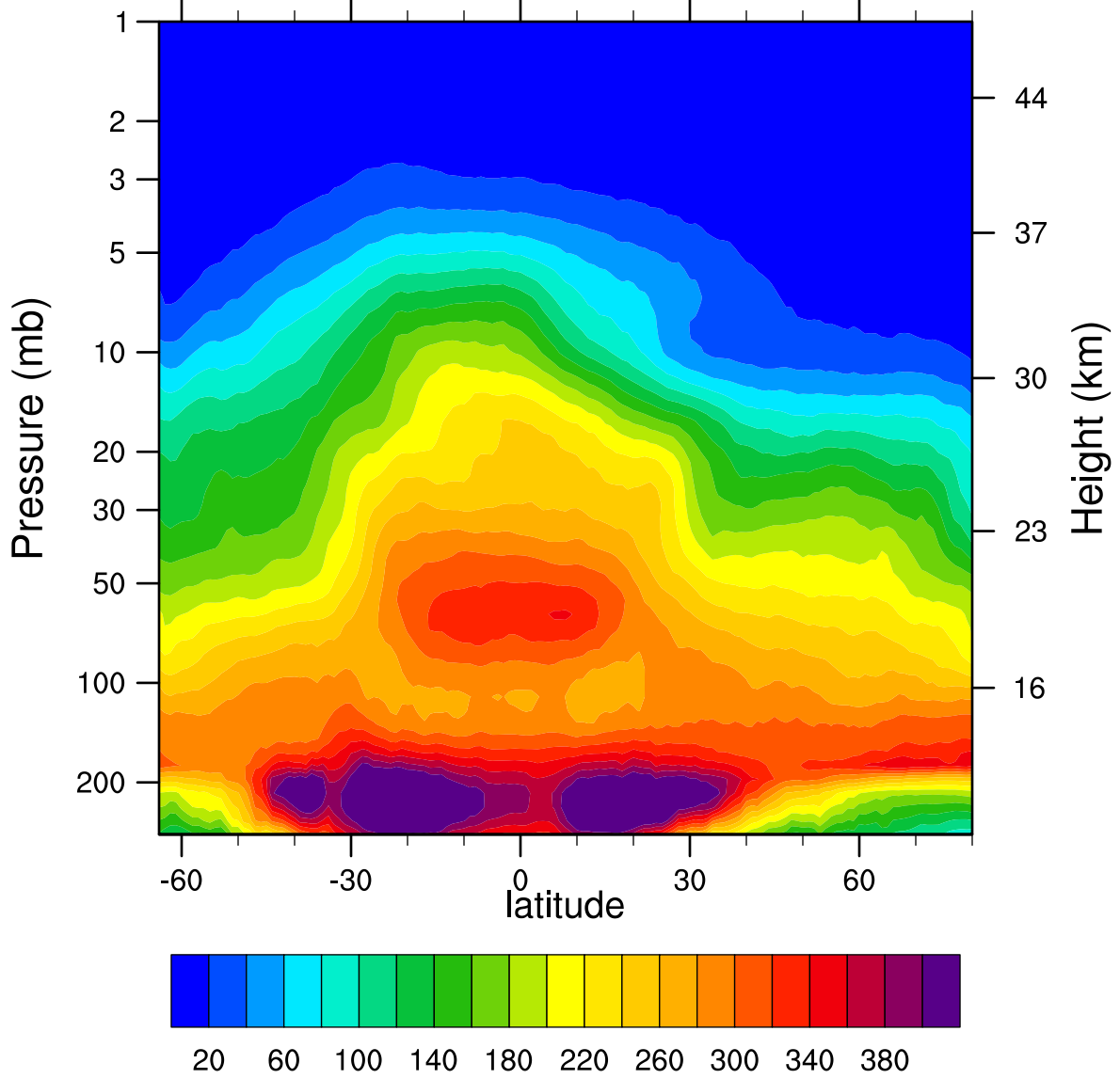
2006d101 N2O_Combined (ppbv)
