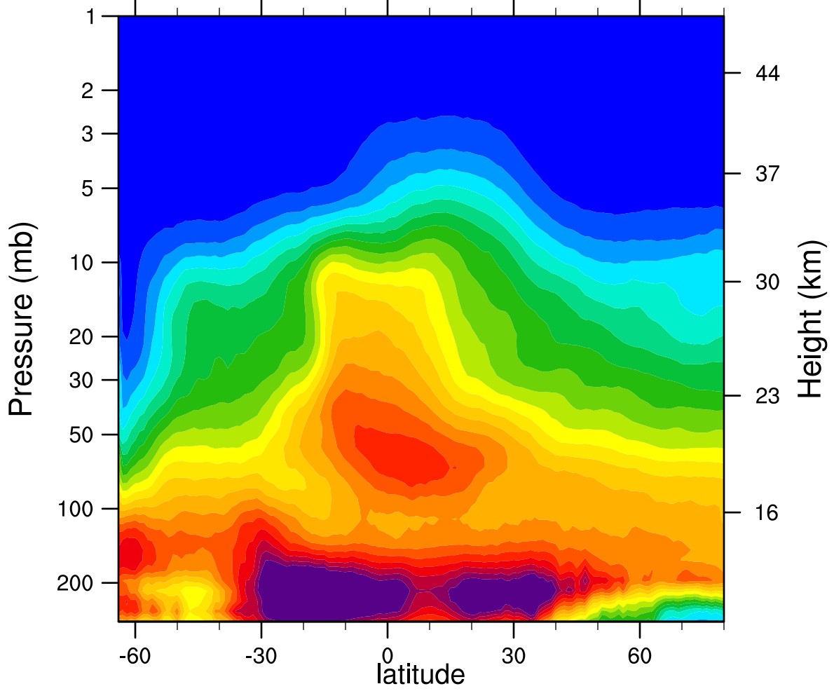
2005d212 N2O_Combined (ppbv)
