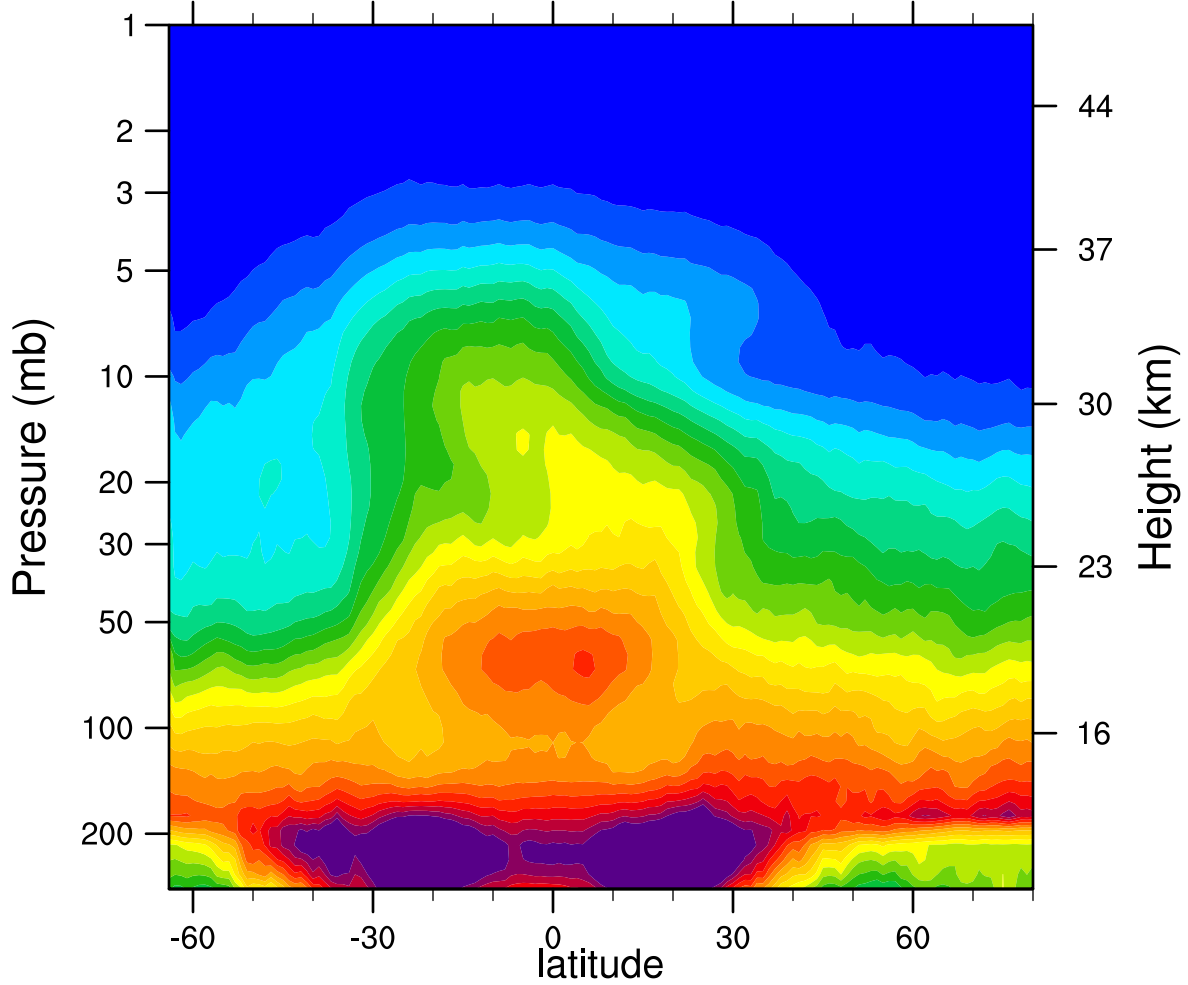
2006d090 N2O_Combined (ppbv)
