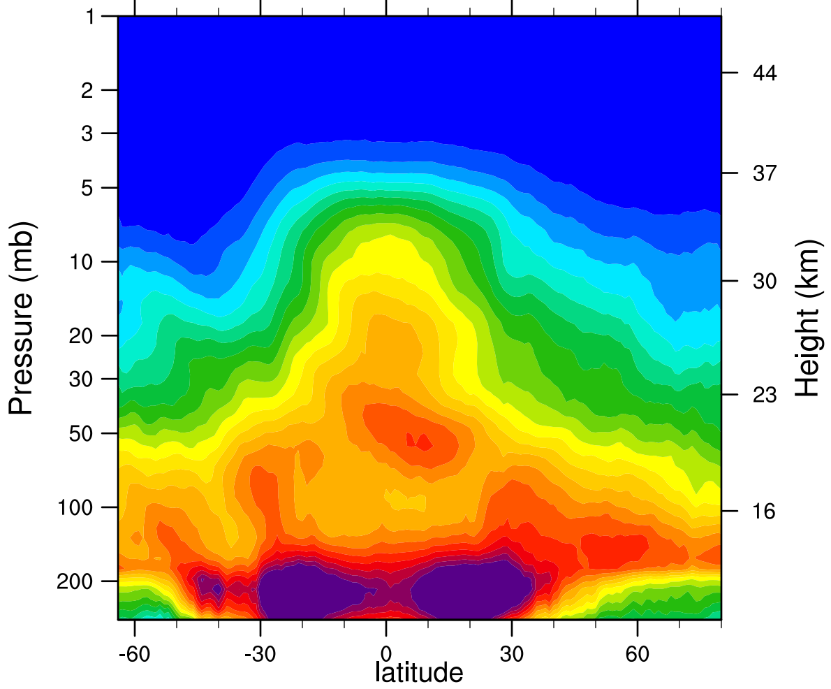
2005d086 N2O_Combined (ppbv)
