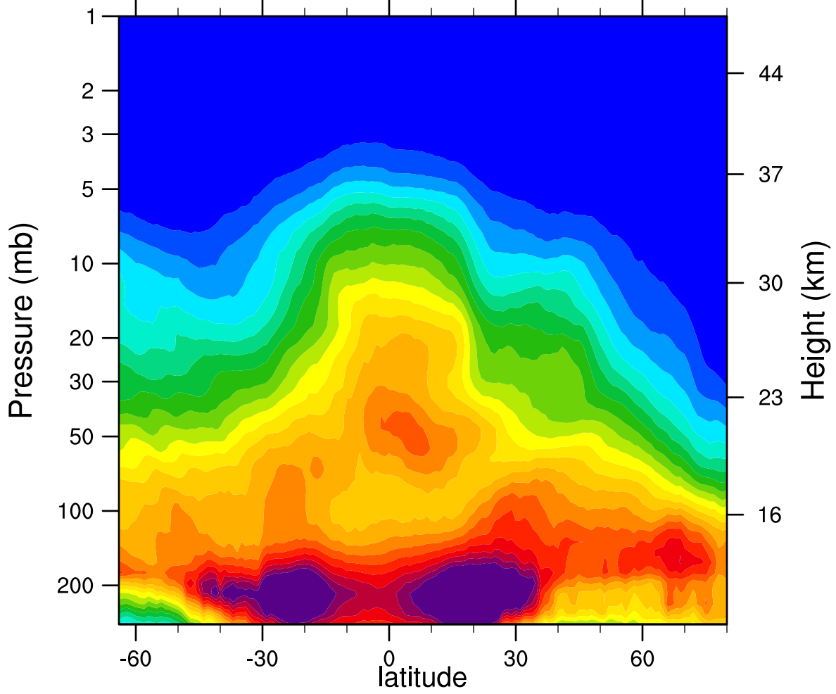
2005d043 N2O_Combined (ppbv)
