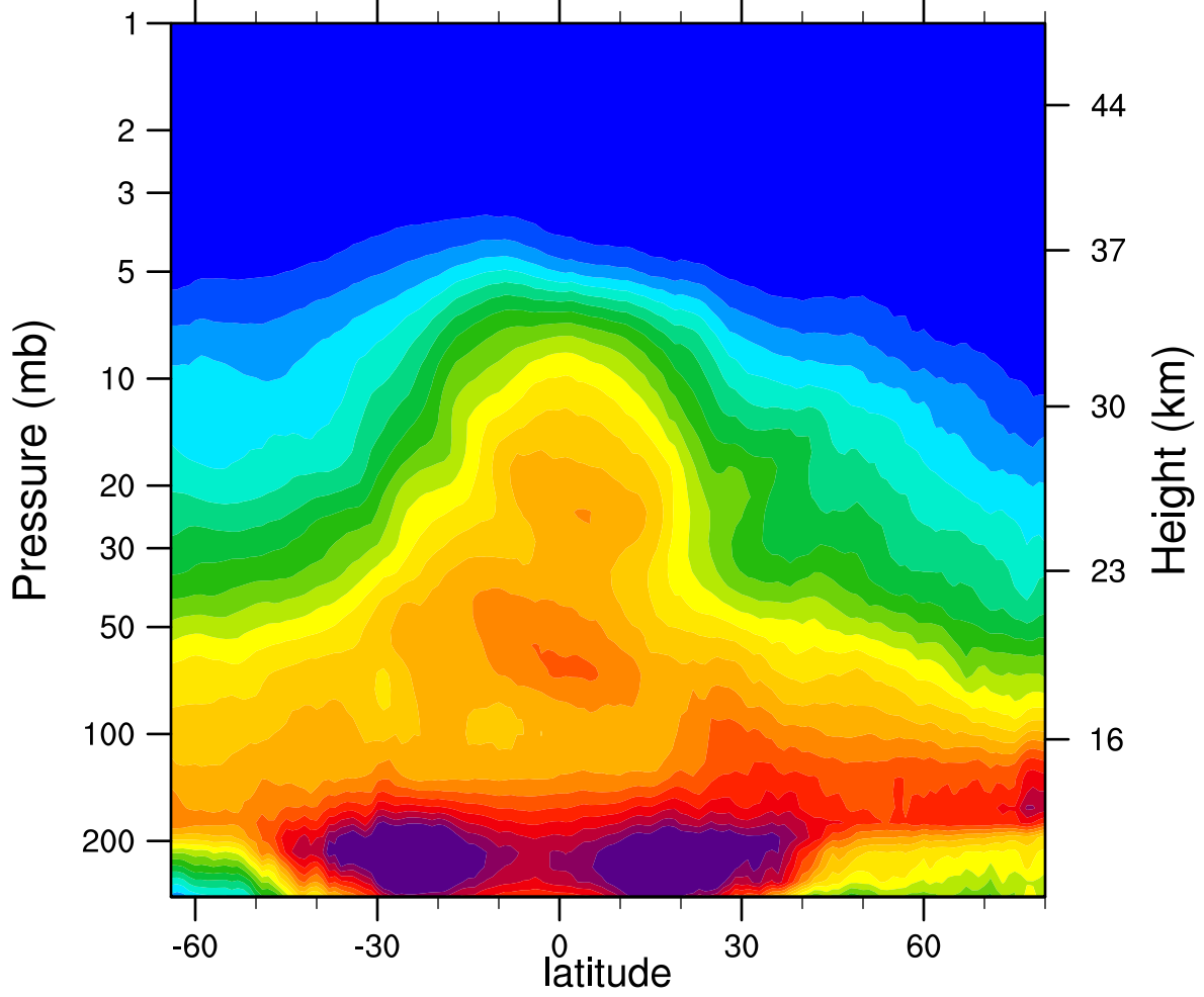
2007d028 N2O_Combined (ppbv)
