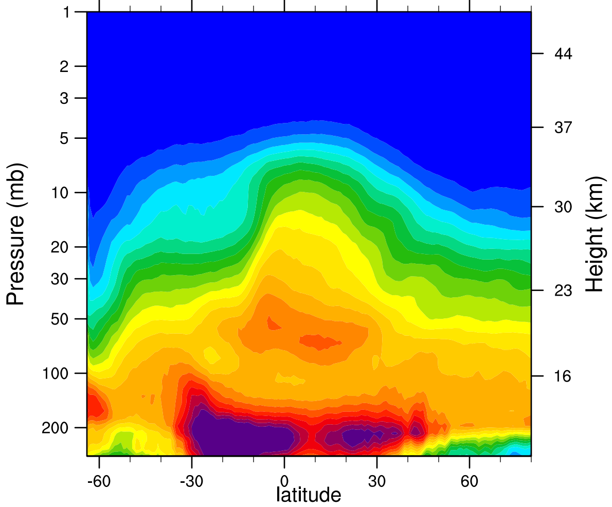
2006d231 N2O_Combined (ppbv)
