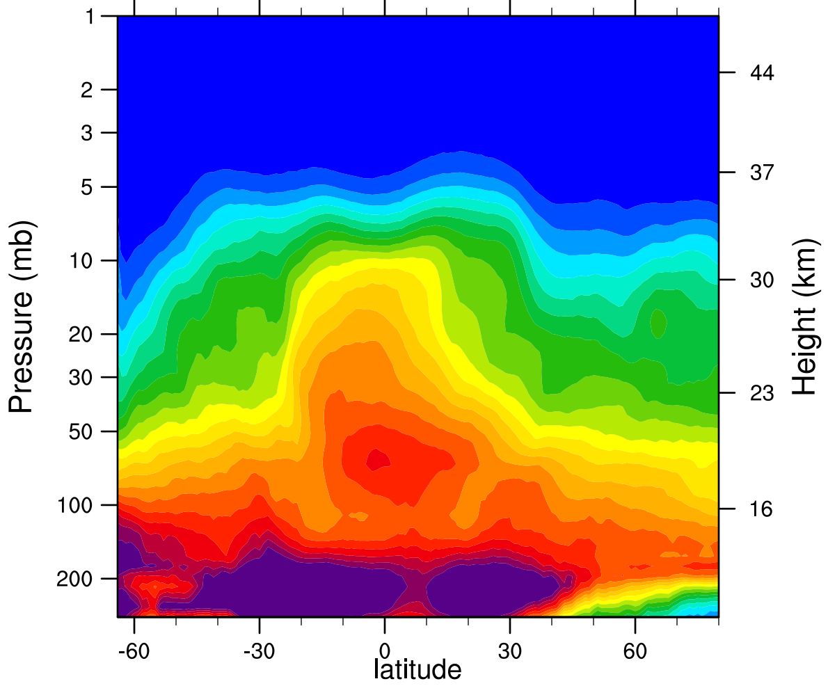
2007d151 N2O_Combined (ppbv)
