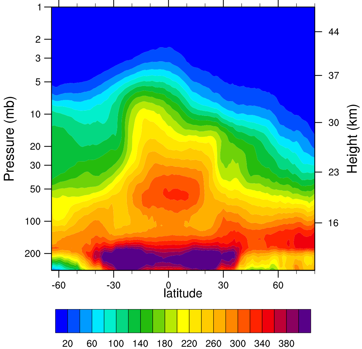
2005d359 N2O_Combined (ppbv)
