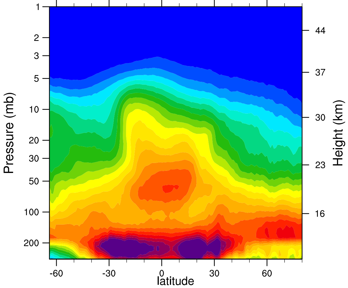
2005d334 N2O_Combined (ppbv)
