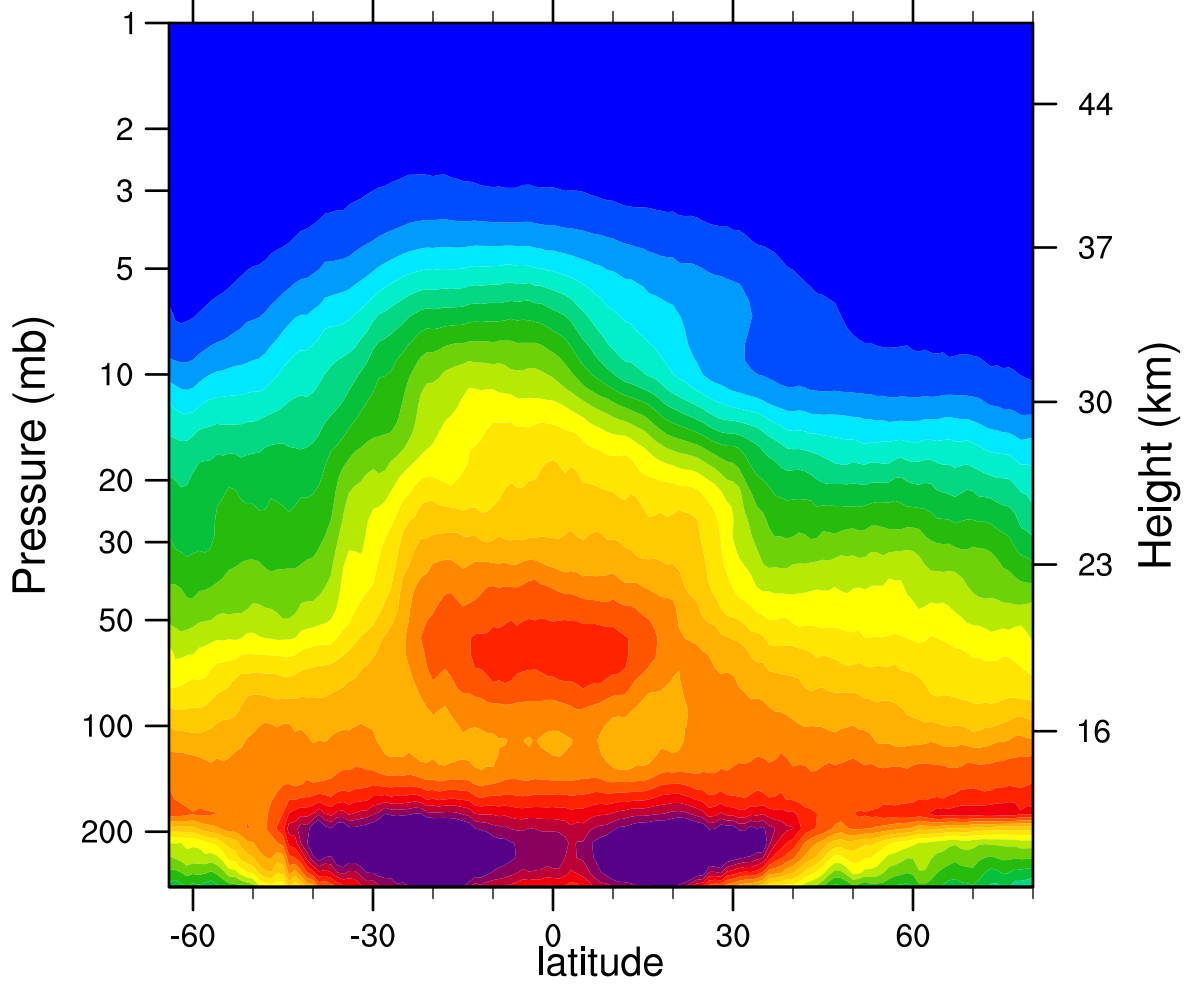
2006d097 N2O_Combined (ppbv)
