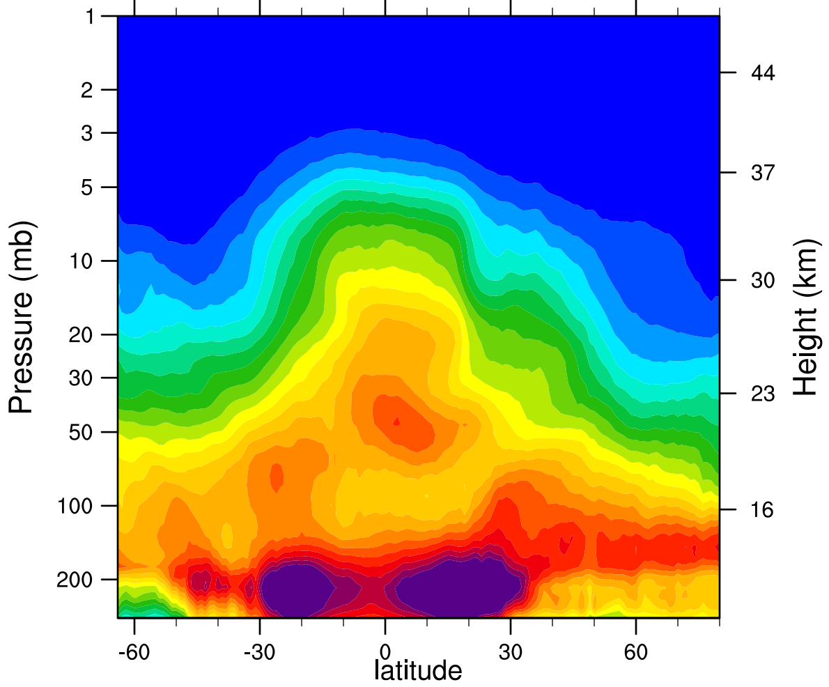
2005d059 N2O_Combined (ppbv)
