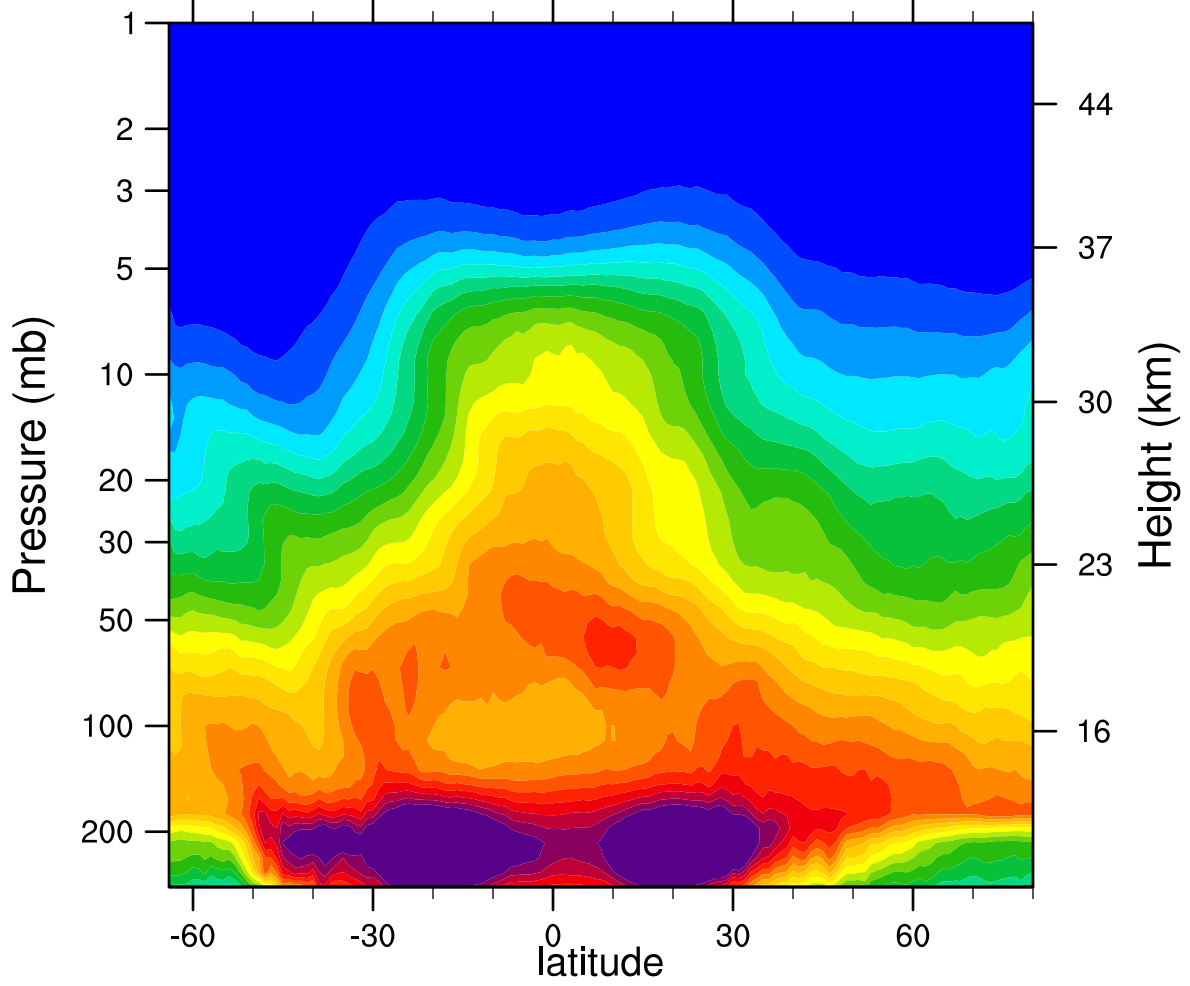
2005d103 N2O_Combined (ppbv)
