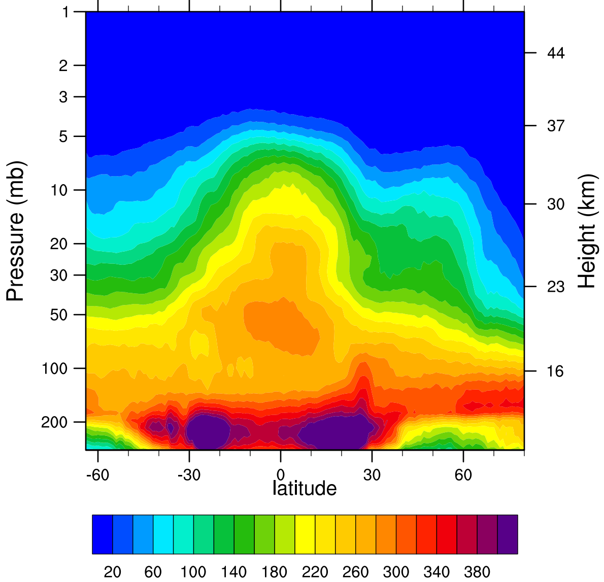
2007d047 N2O_Combined (ppbv)
