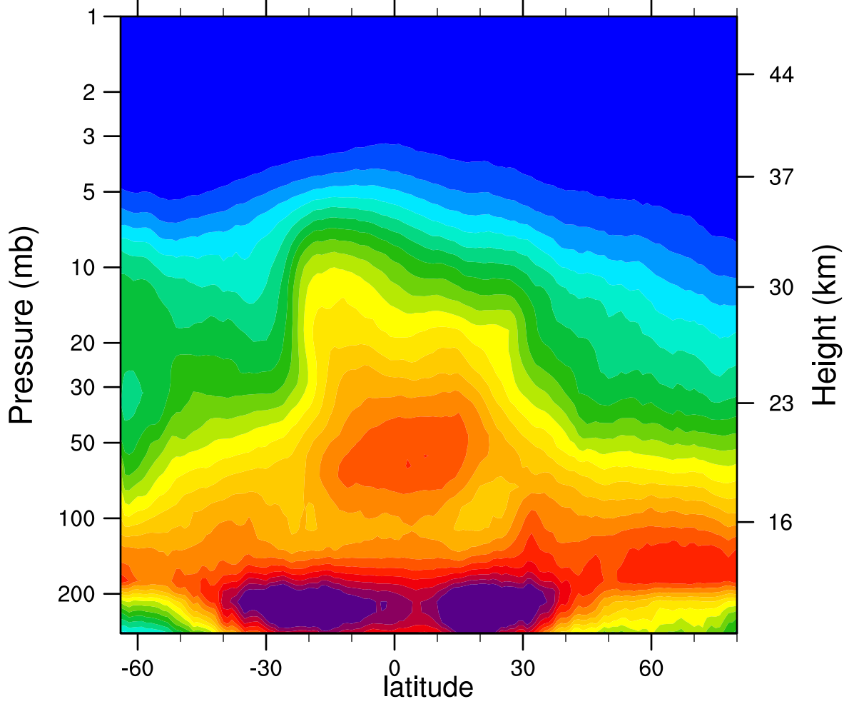
2005d331 N2O_Combined (ppbv)
