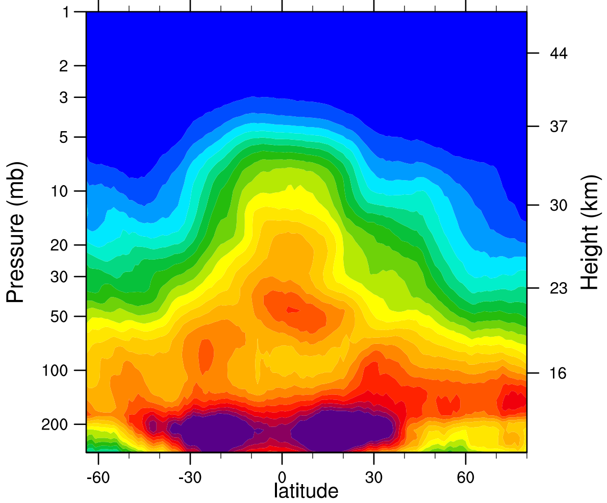
2005d069 N2O_Combined (ppbv)
