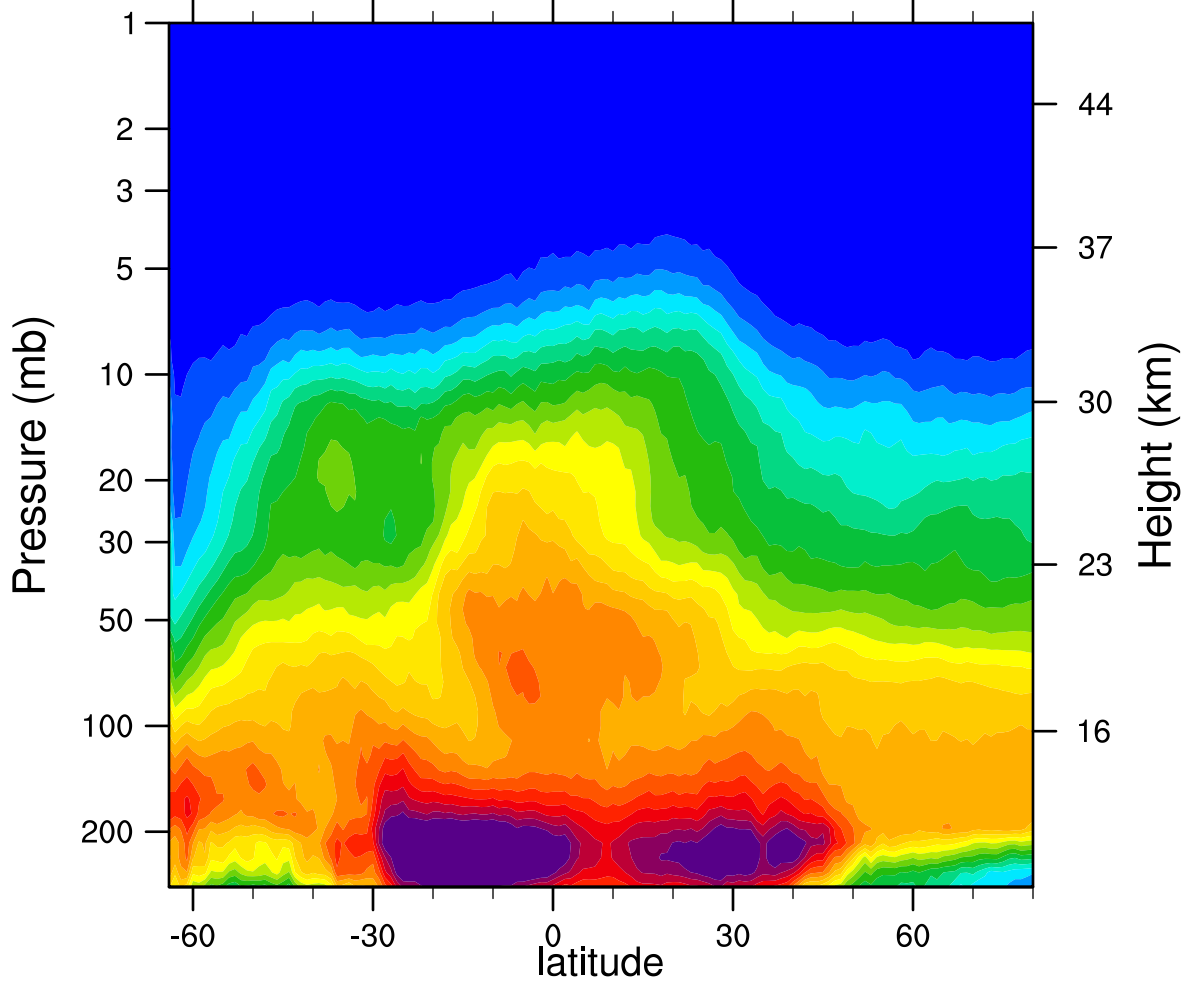
2007d212 N2O_Combined (ppbv)
