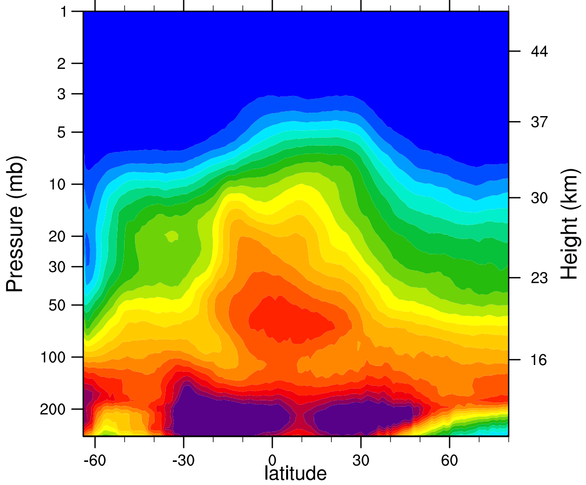
2007d252 N2O_Combined (ppbv)
