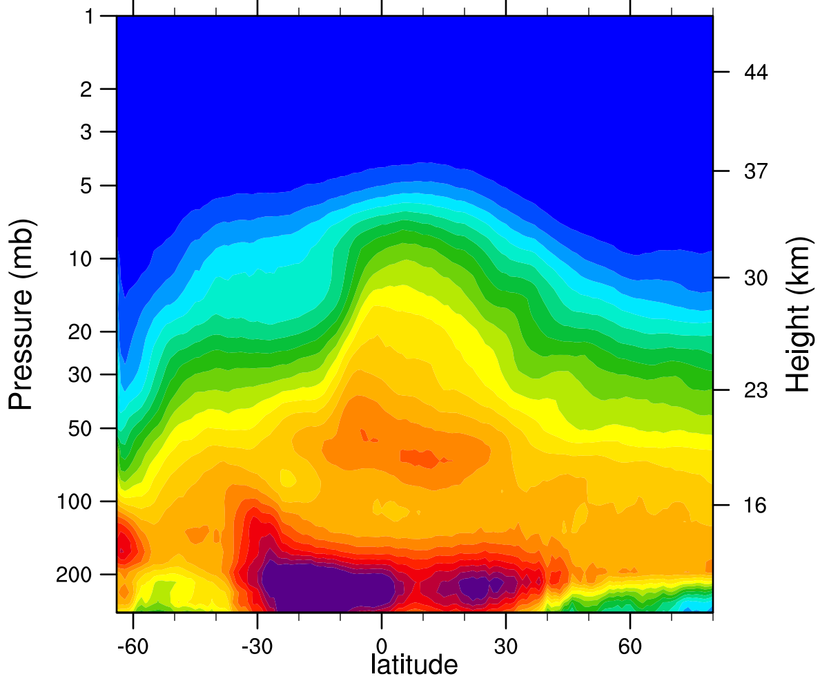
2006d229 N2O_Combined (ppbv)
