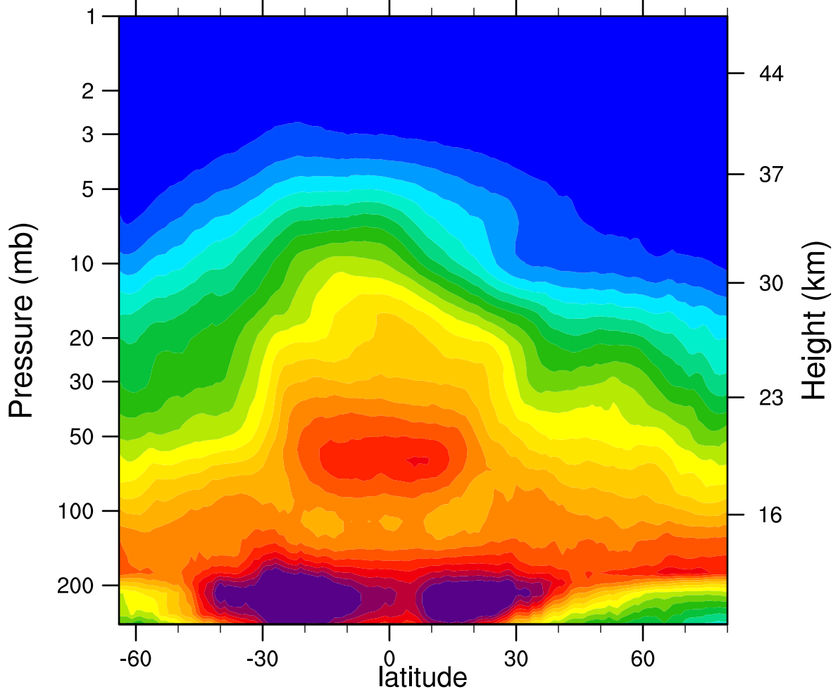
2006d105 N2O_Combined (ppbv)
