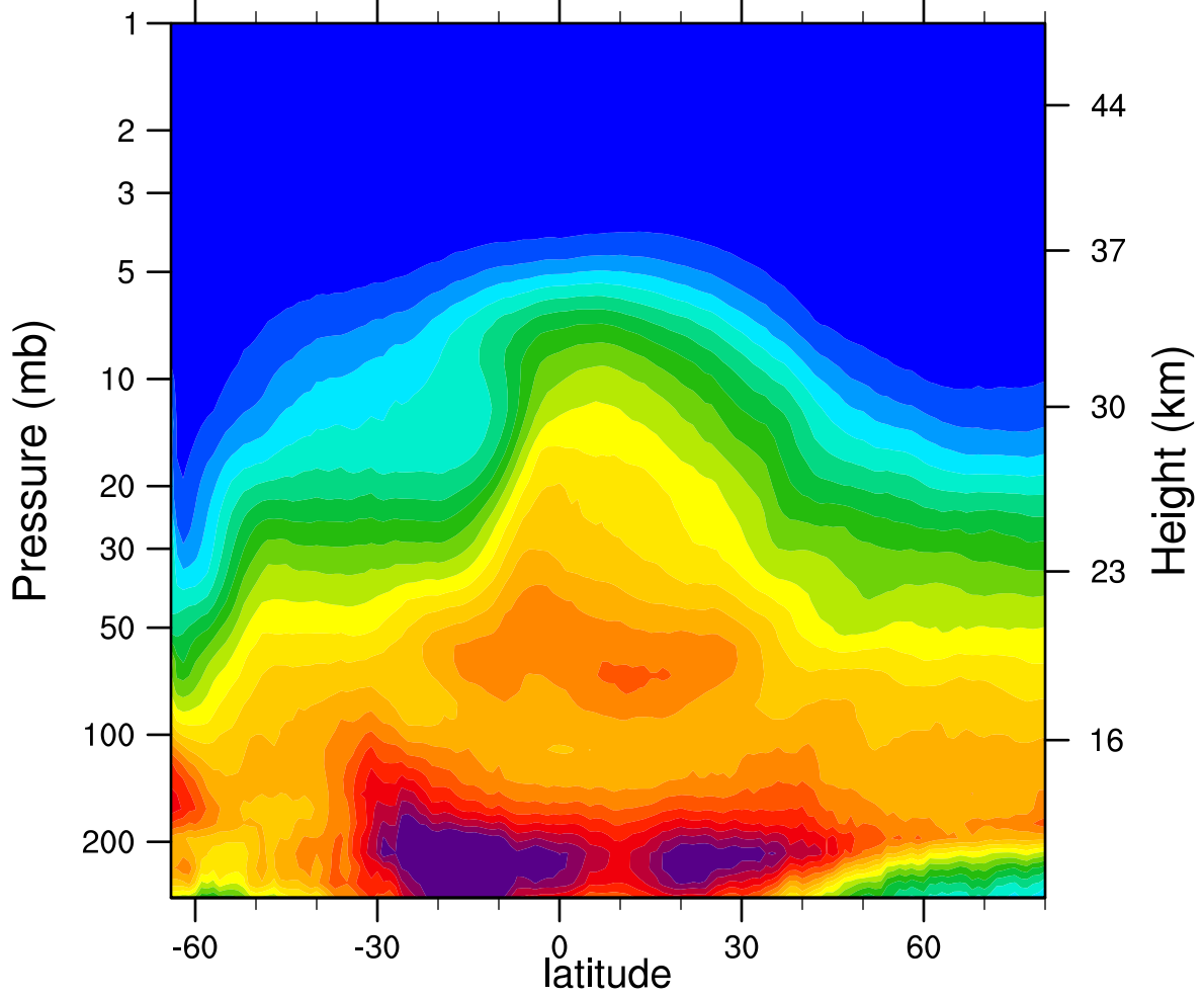
2006d246 N2O_Combined (ppbv)
