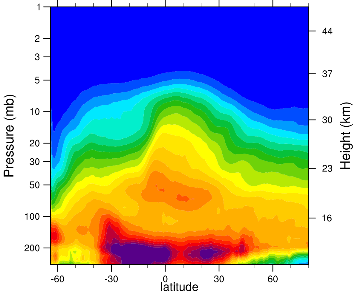
2006d227 N2O_Combined (ppbv)
