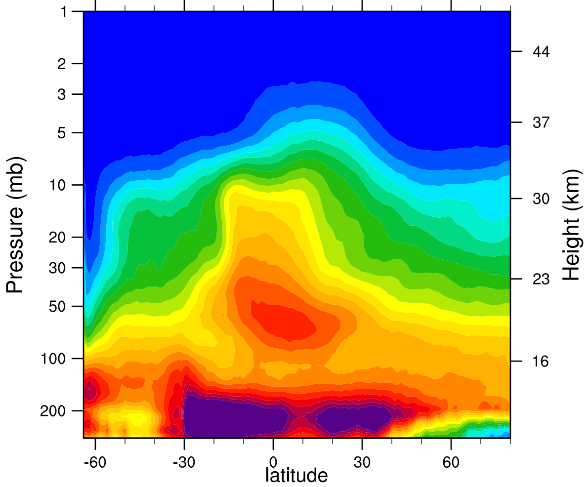
2005d213 N2O_Combined (ppbv)
