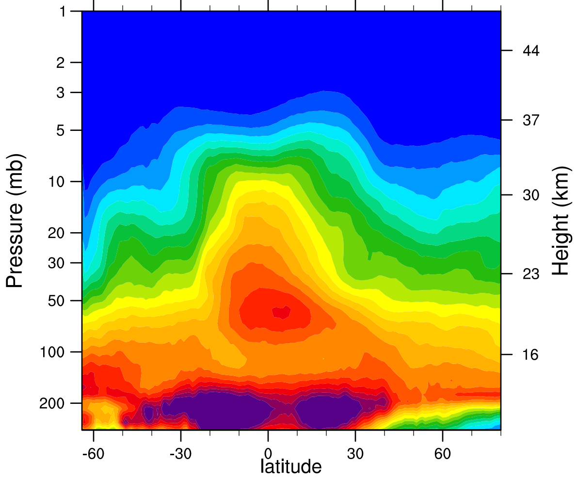
2005d146 N2O_Combined (ppbv)
