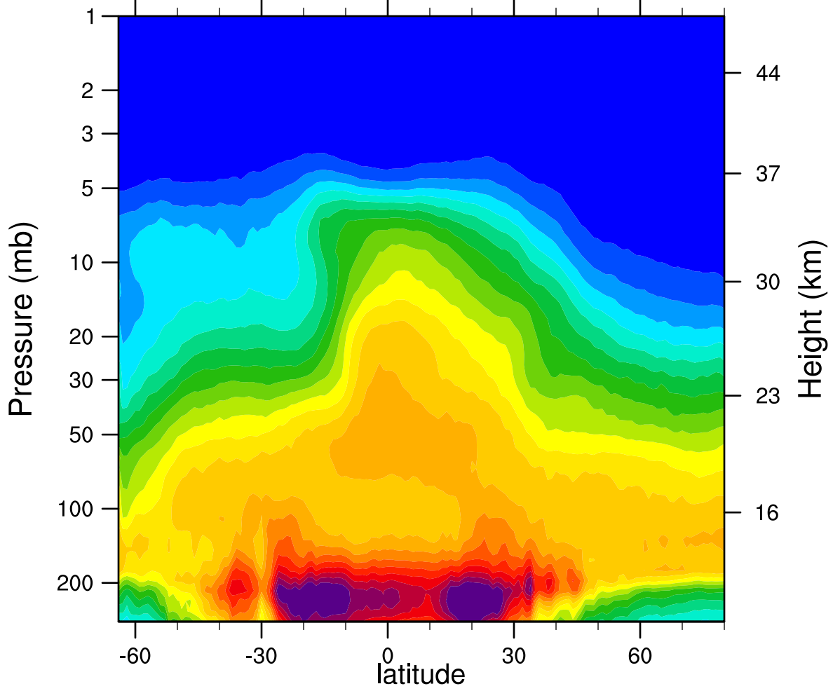
2006d301 N2O_Combined (ppbv)
