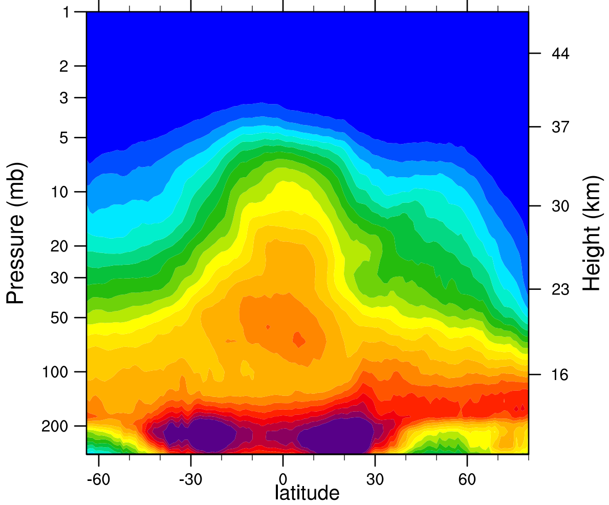
2007d043 N2O_Combined (ppbv)
