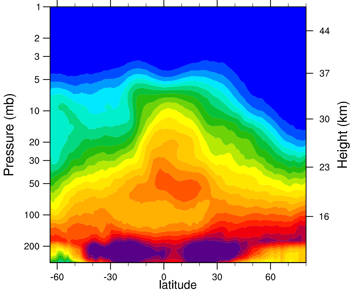
2006d323 N2O_Combined (ppbv)
