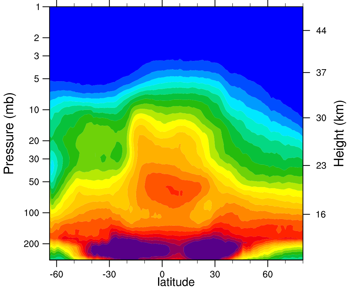
2007d296 N2O_Combined (ppbv)
