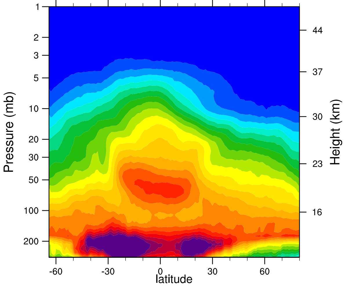
2006d119 N2O_Combined (ppbv)
