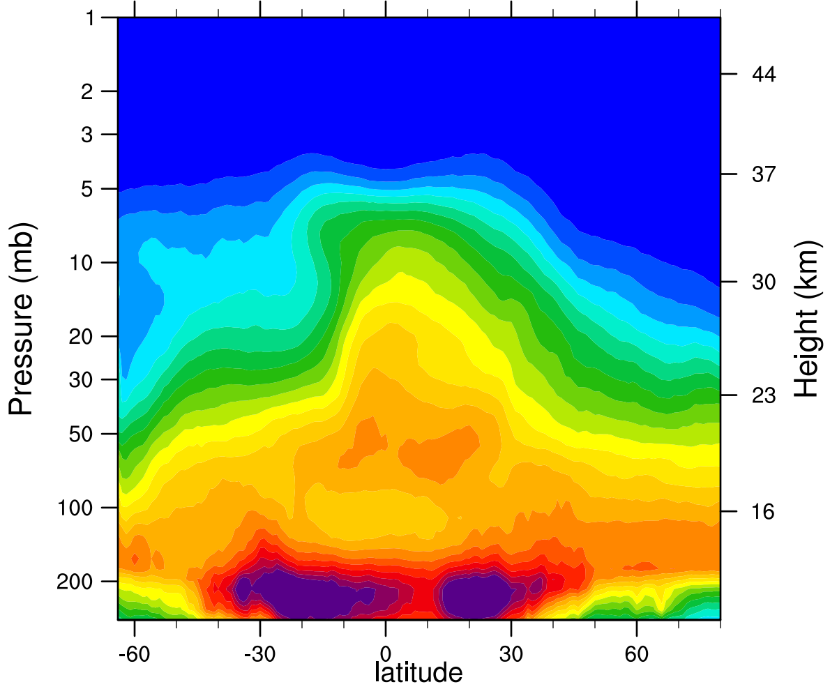
2006d295 N2O_Combined (ppbv)
