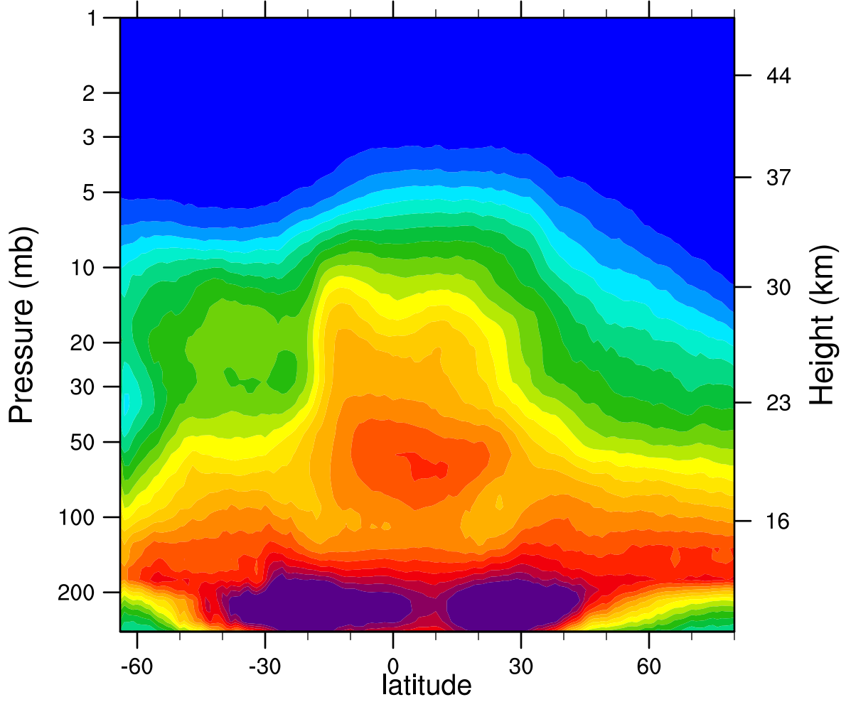
2007d295 N2O_Combined (ppbv)
