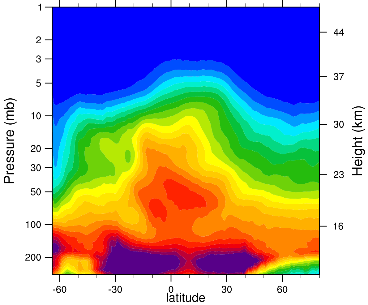
2007d242 N2O_Combined (ppbv)
