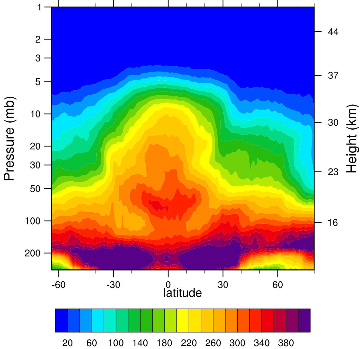
2007d080 N2O_Combined (ppbv)
