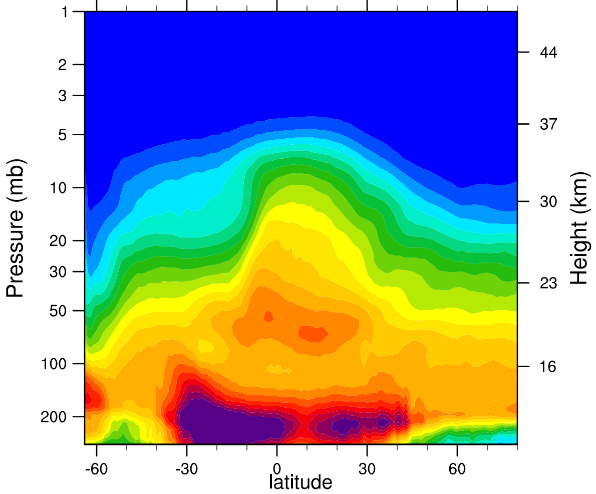
2006d234 N2O_Combined (ppbv)
