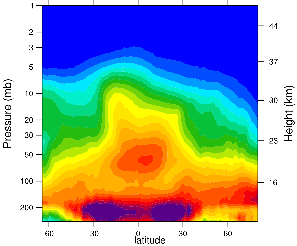
2005d339 N2O_Combined (ppbv)
