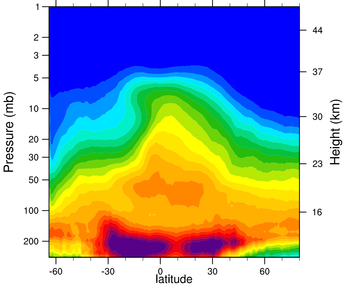
2006d269 N2O_Combined (ppbv)
