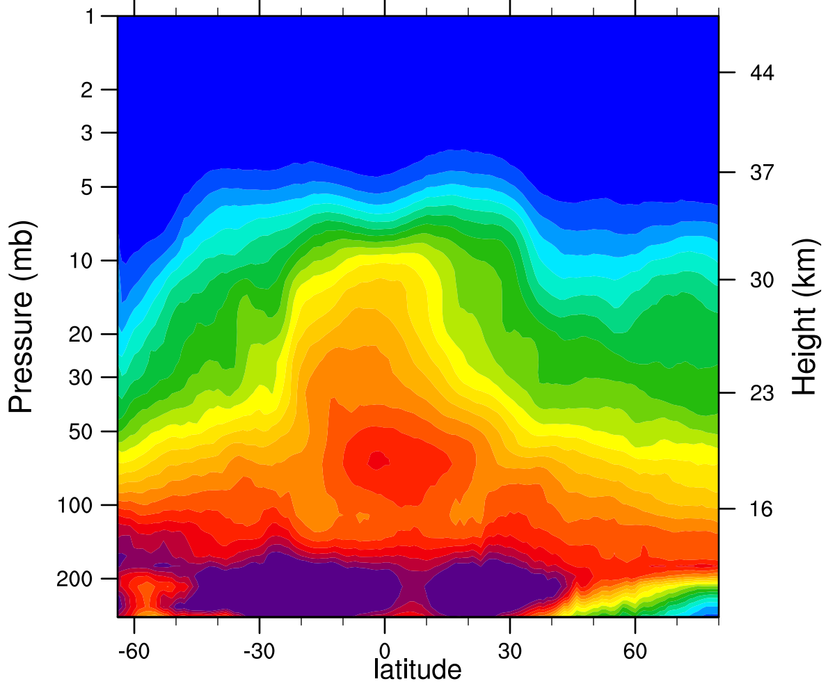
2007d145 N2O_Combined (ppbv)
