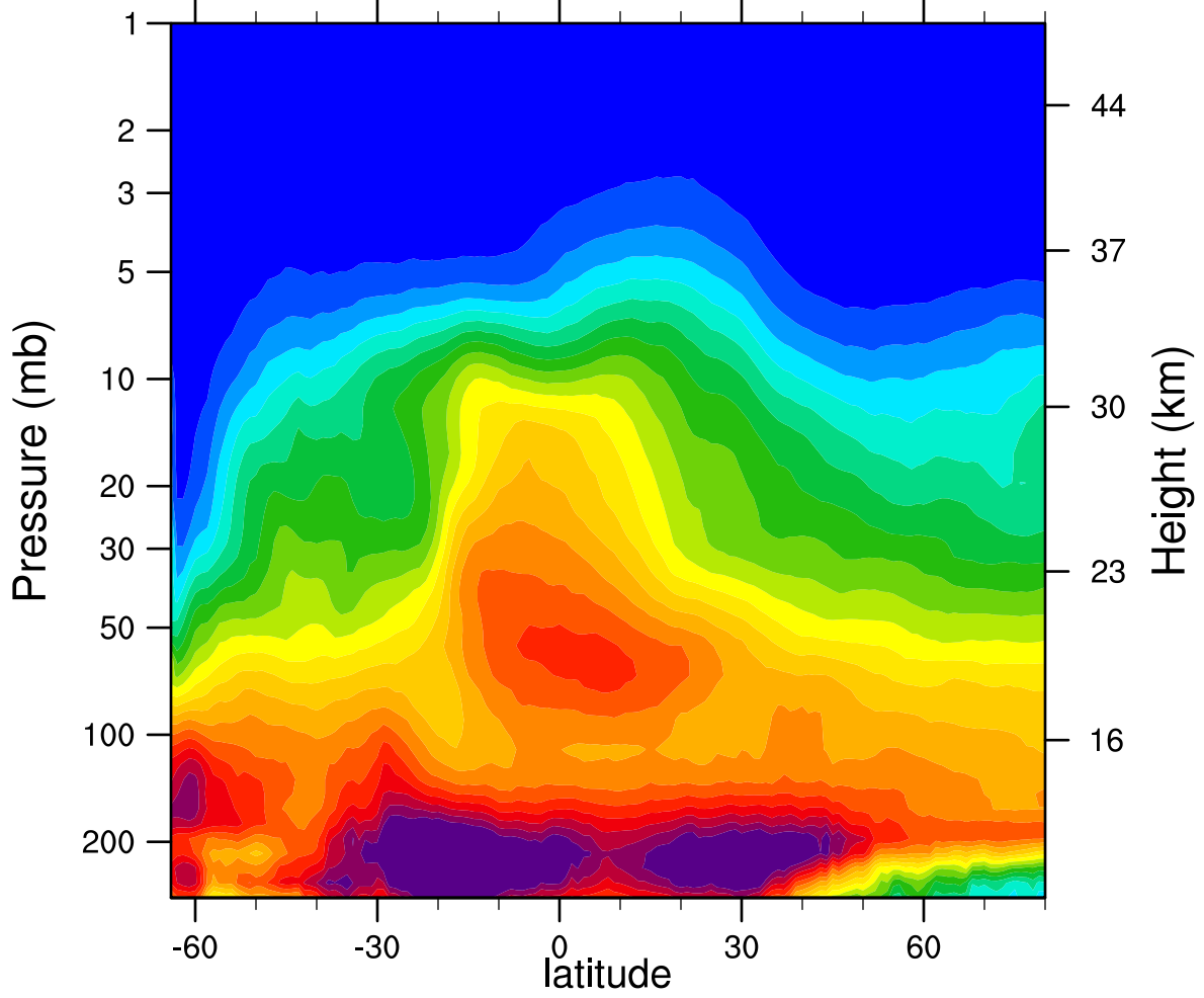
2005d185 N2O_Combined (ppbv)
