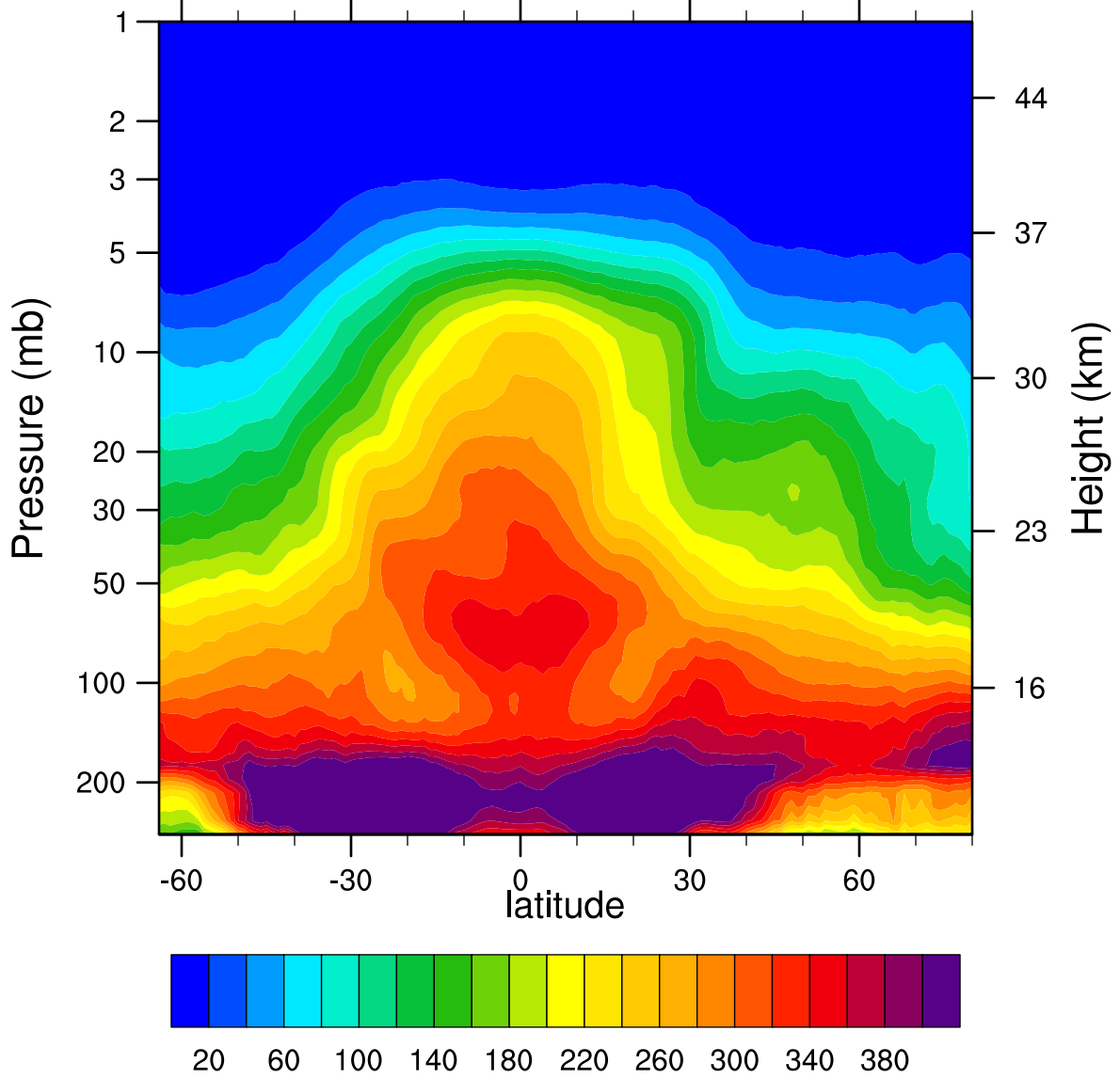
2007d092 N2O_Combined (ppbv)
