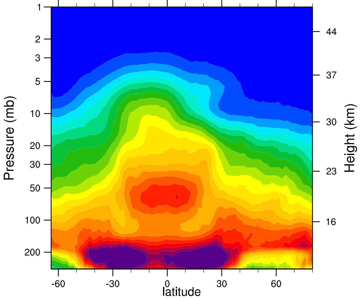
2006d077 N2O_Combined (ppbv)
