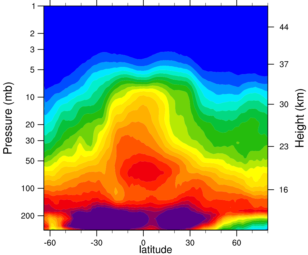
2007d131 N2O_Combined (ppbv)
