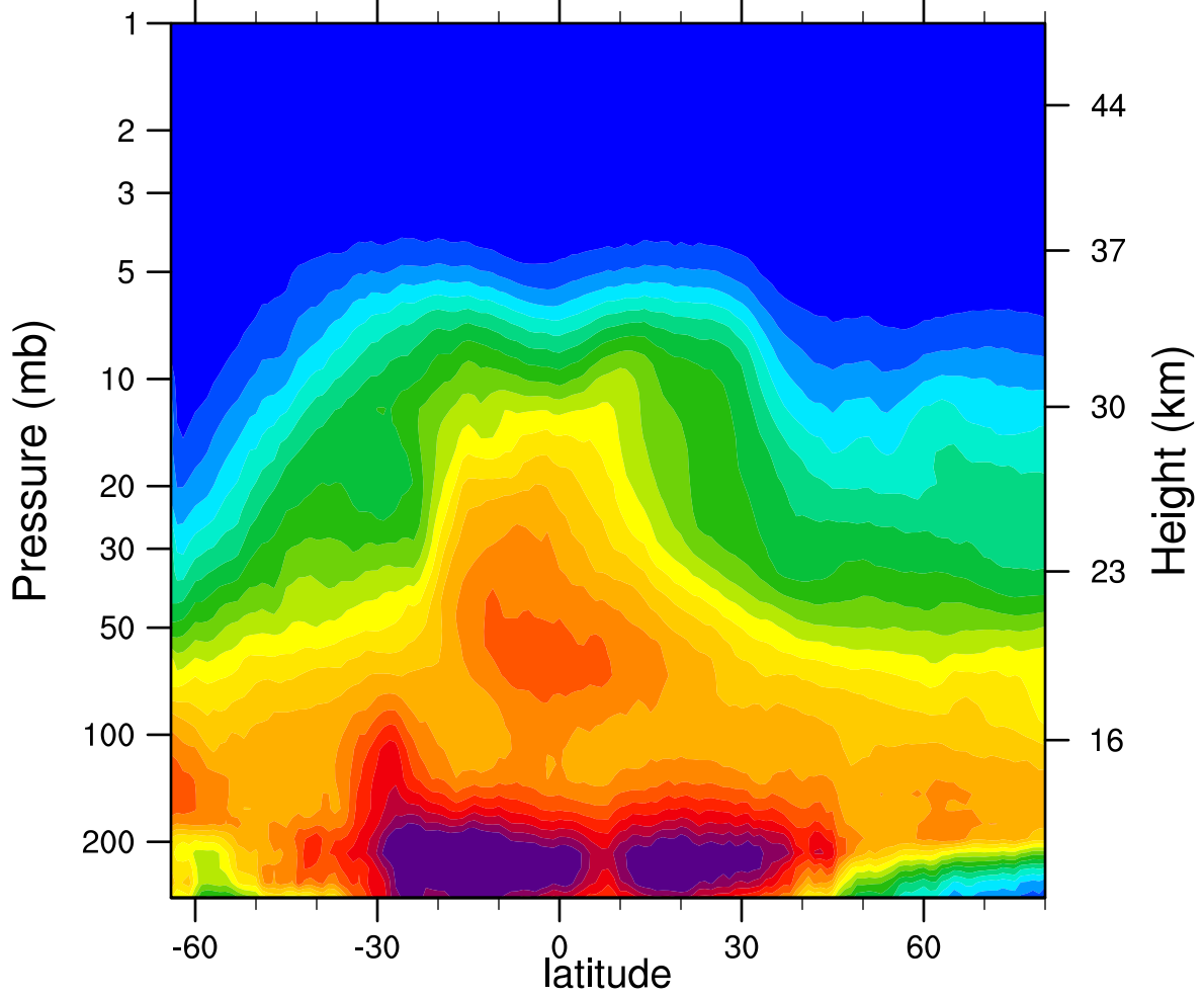
2007d166 N2O_Combined (ppbv)
