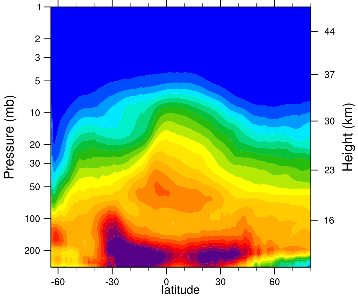
2006d204 N2O_Combined (ppbv)
