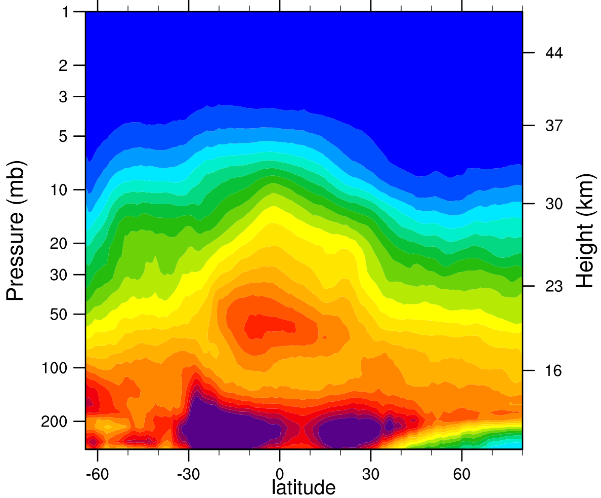
2006d154 N2O_Combined (ppbv)
