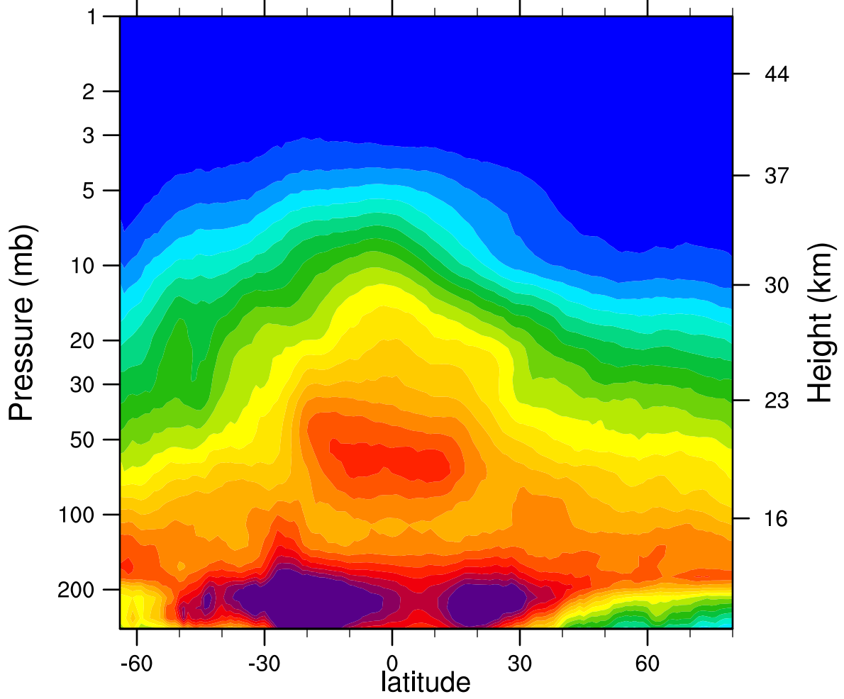
2006d129 N2O_Combined (ppbv)
