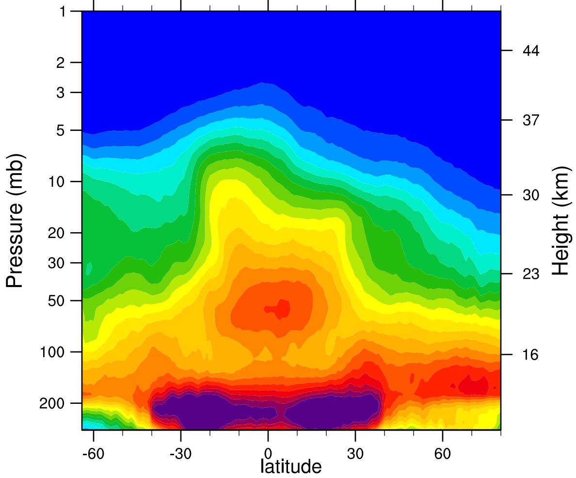
2005d347 N2O_Combined (ppbv)
