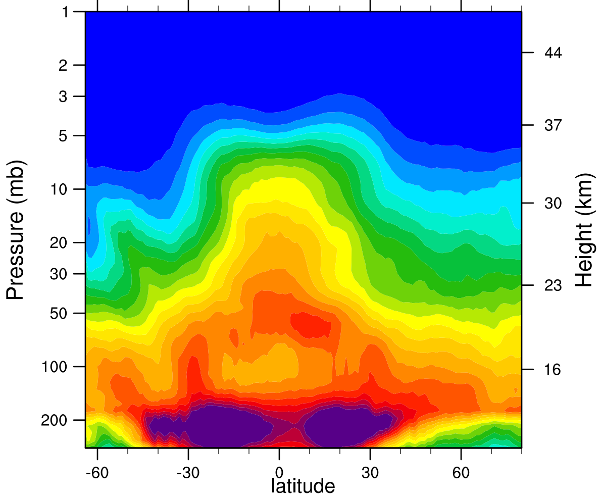
2005d110 N2O_Combined (ppbv)
