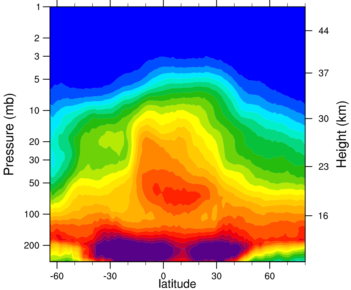
2007d274 N2O_Combined (ppbv)
