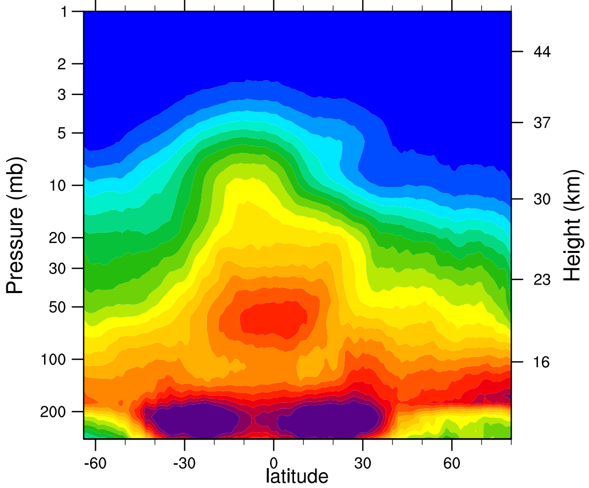
2006d064 N2O_Combined (ppbv)
