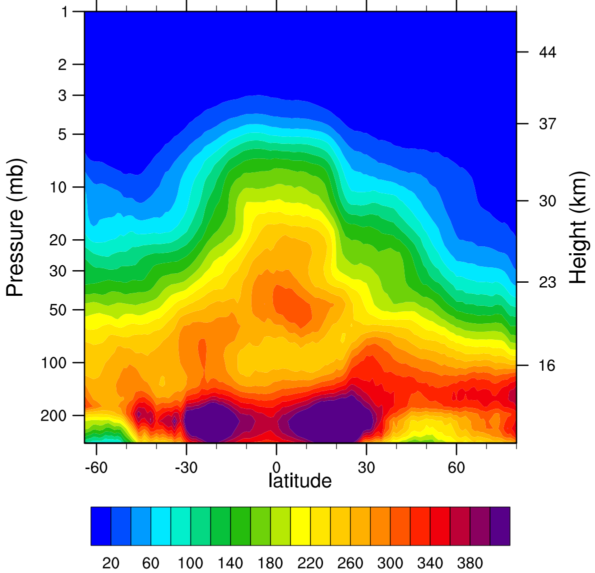
2005d052 N2O_Combined (ppbv)
