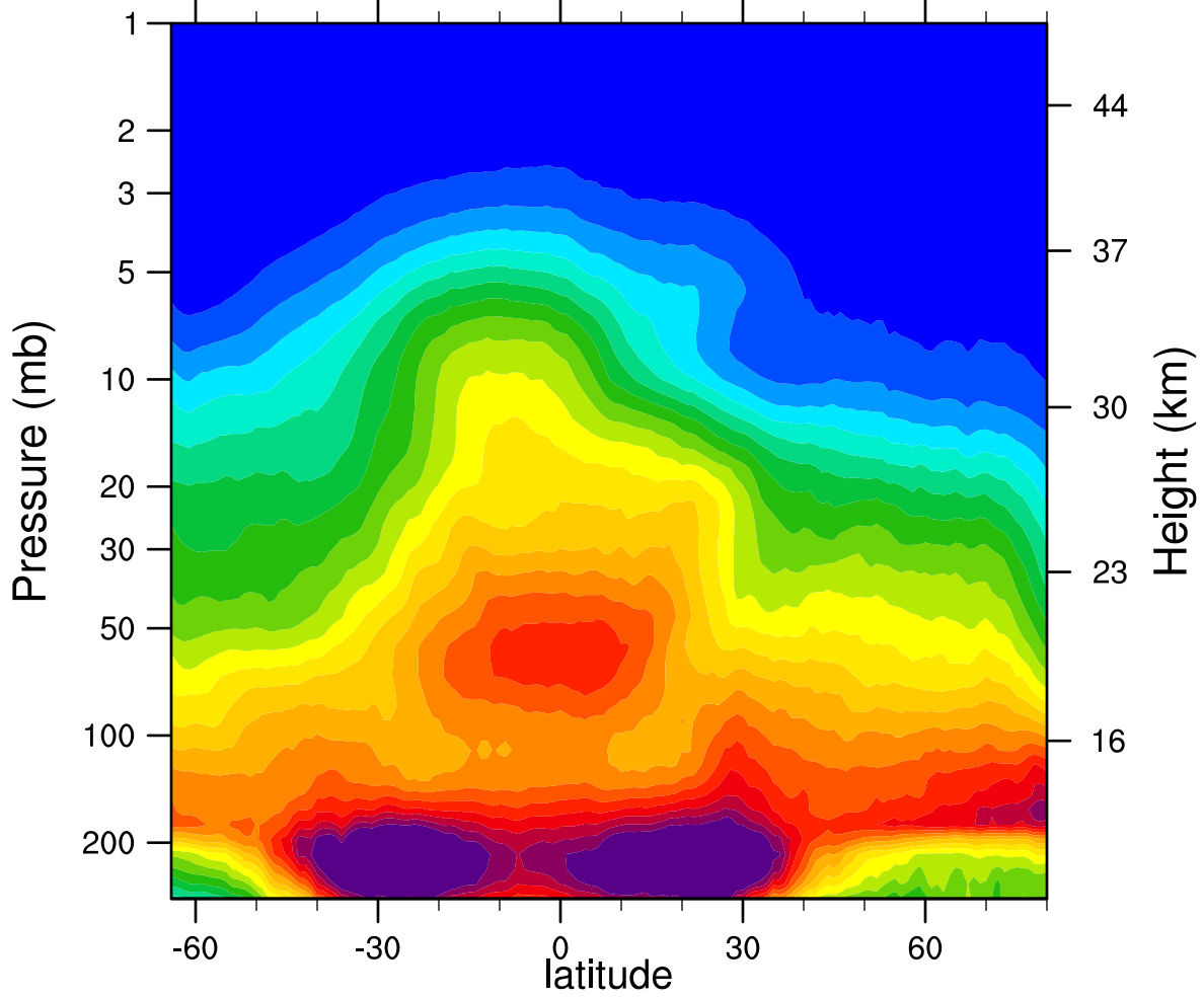
2006d066 N2O_Combined (ppbv)
