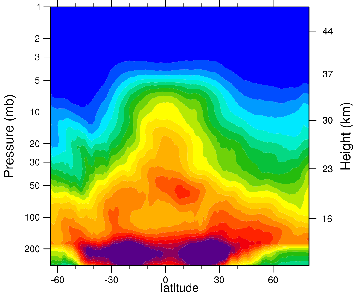
2005d096 N2O_Combined (ppbv)
