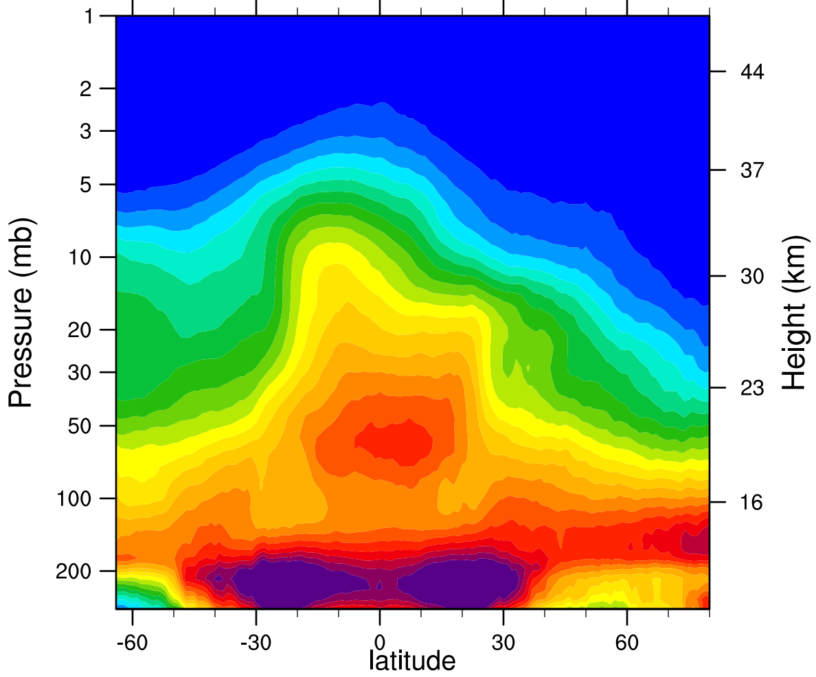
2006d003 N2O_Combined (ppbv)
