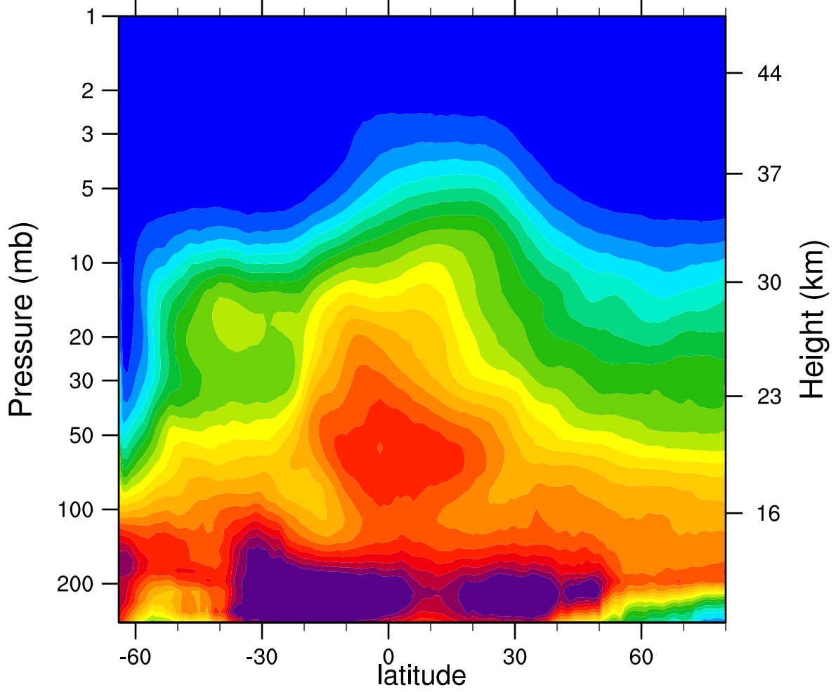
2007d226 N2O_Combined (ppbv)
