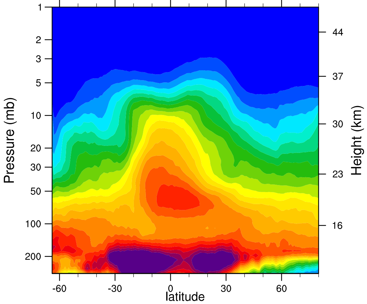
2005d152 N2O_Combined (ppbv)
