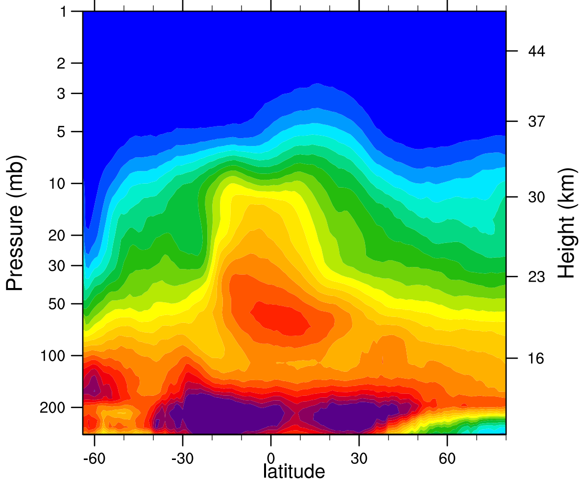
2005d189 N2O_Combined (ppbv)
