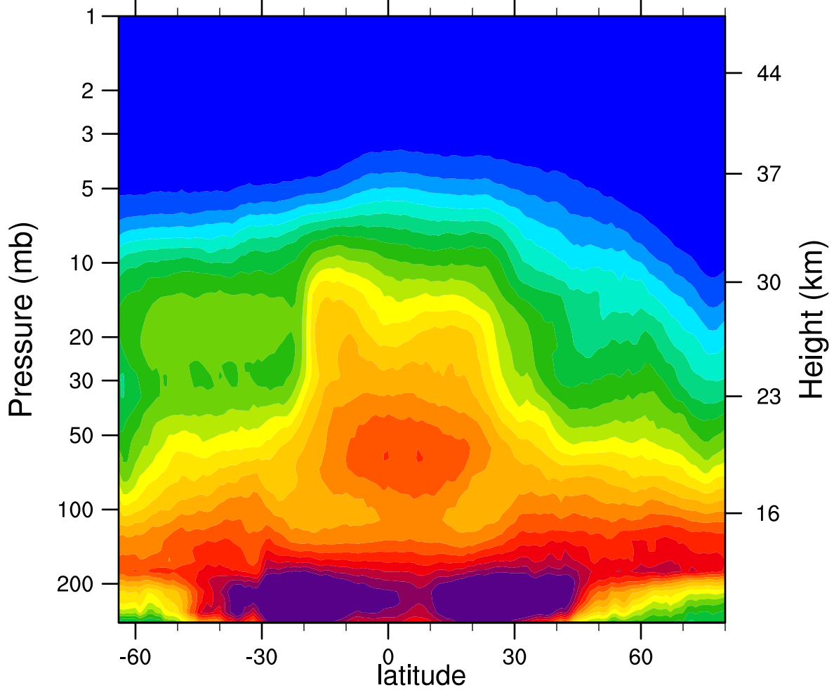
2007d311 N2O_Combined (ppbv)
