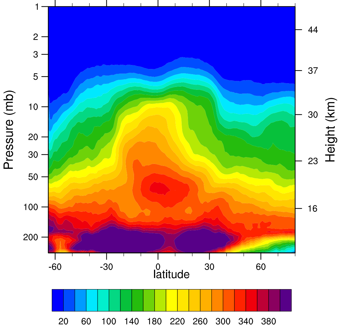
2007d141 N2O_Combined (ppbv)
