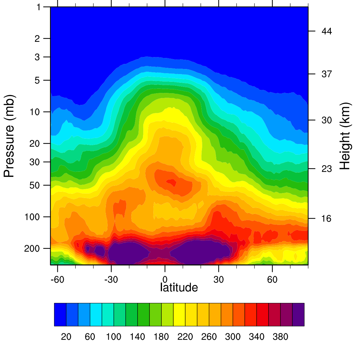
2005d072 N2O_Combined (ppbv)
