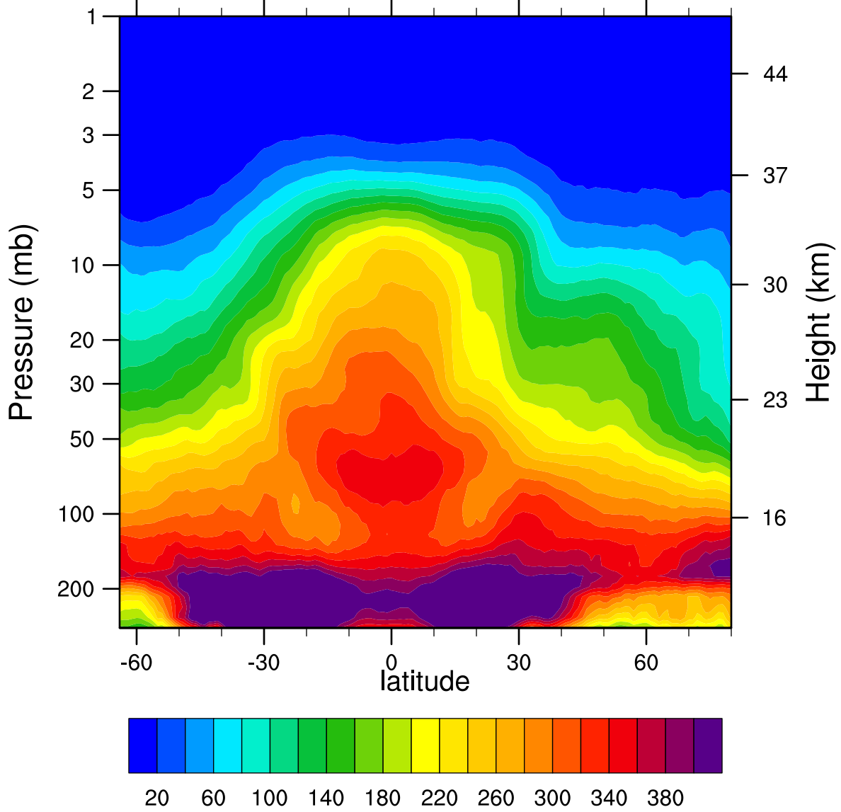
2007d094 N2O_Combined (ppbv)
