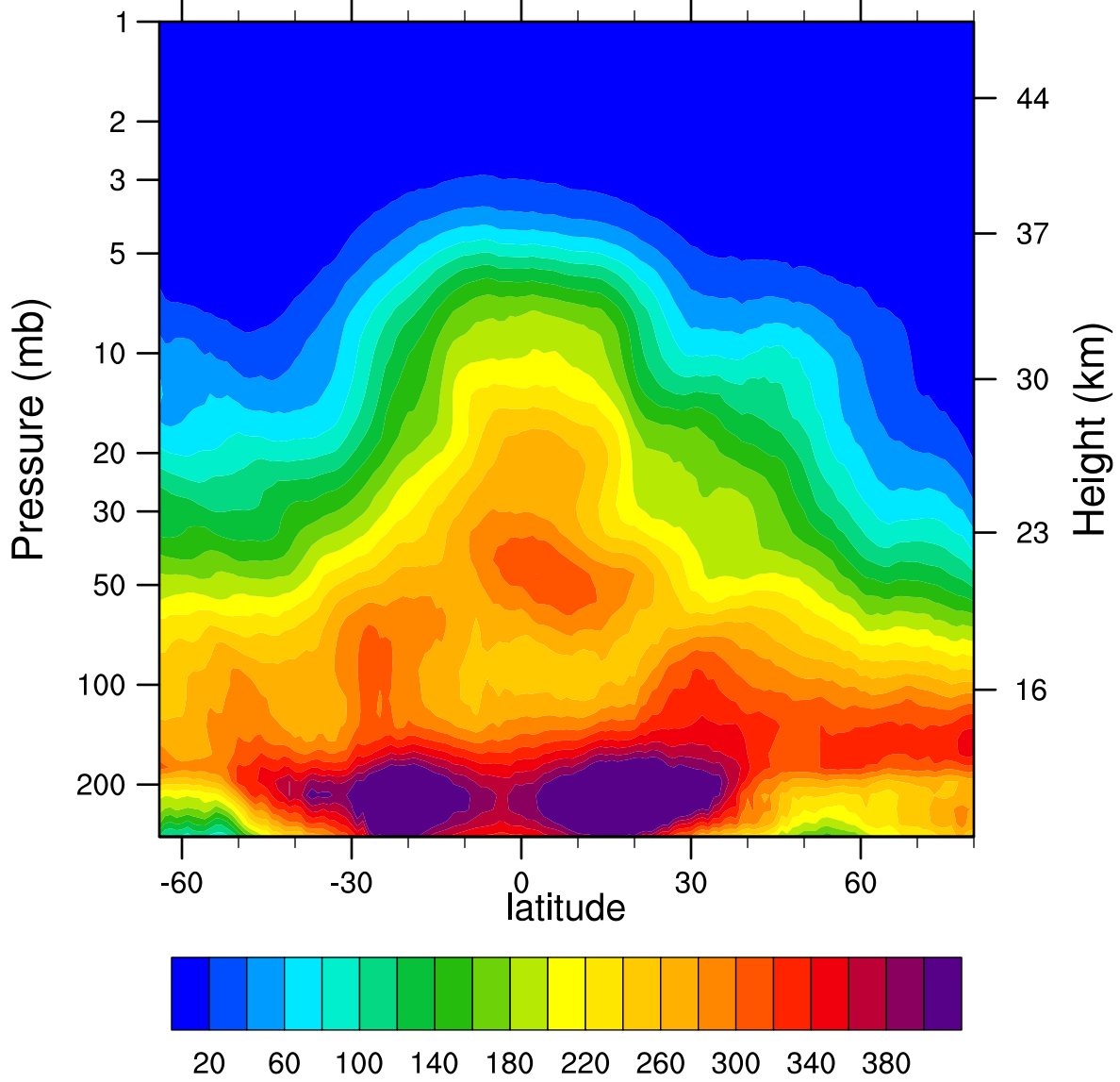
2005d065 N2O_Combined (ppbv)
