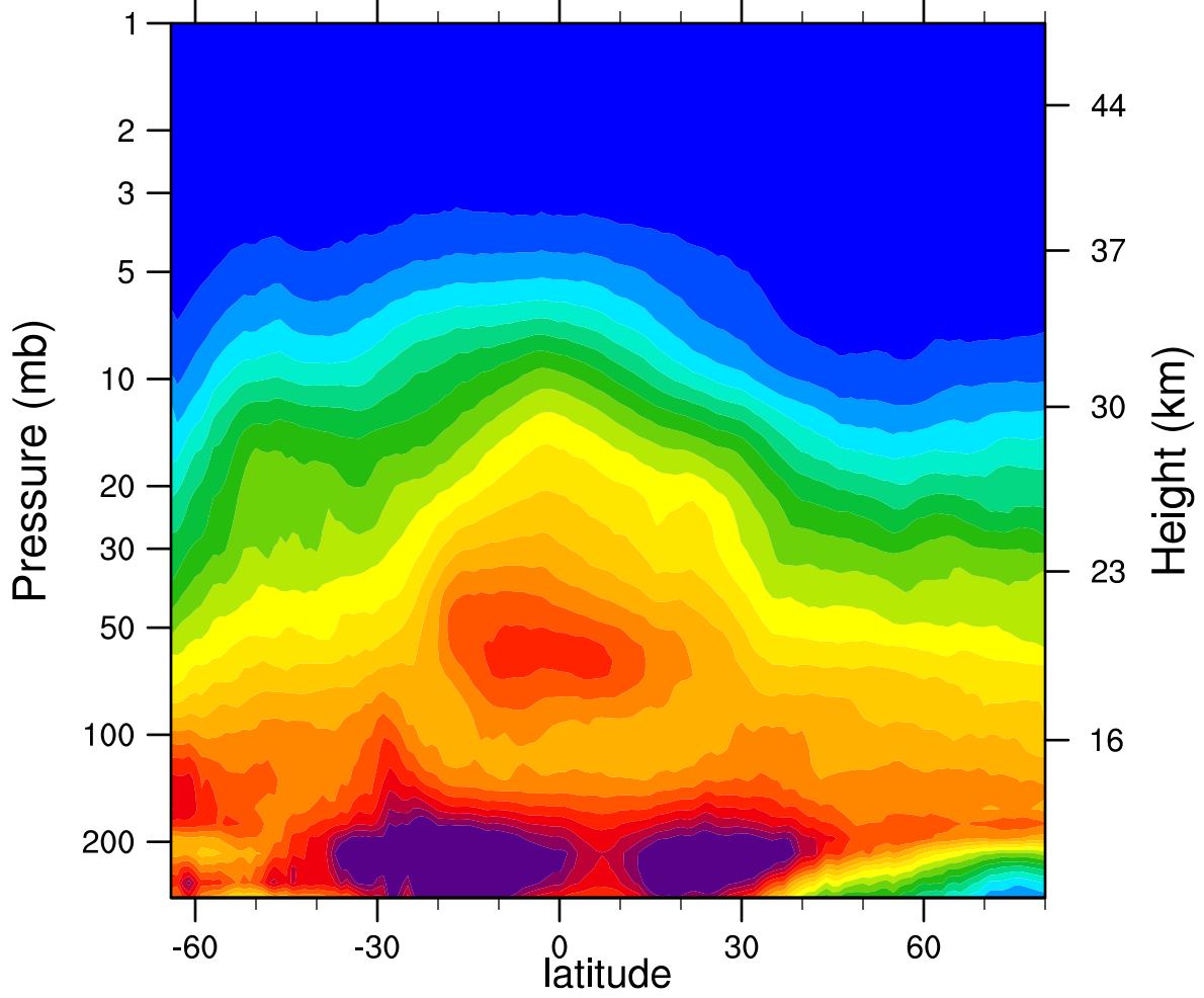
2006d149 N2O_Combined (ppbv)
