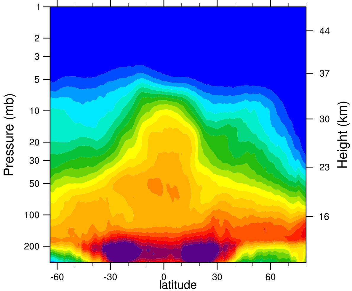
2006d363 N2O_Combined (ppbv)
