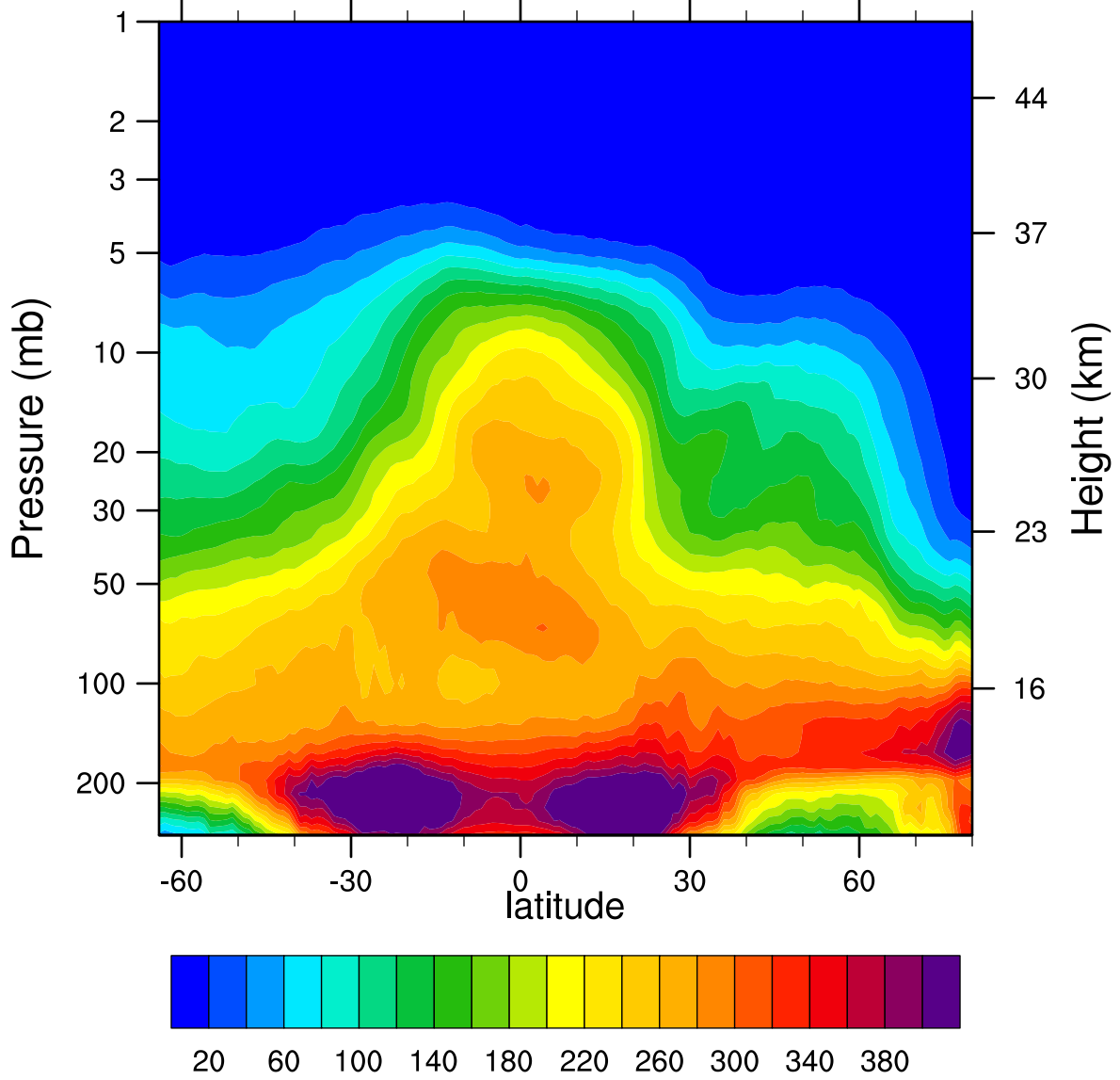
2007d020 N2O_Combined (ppbv)
