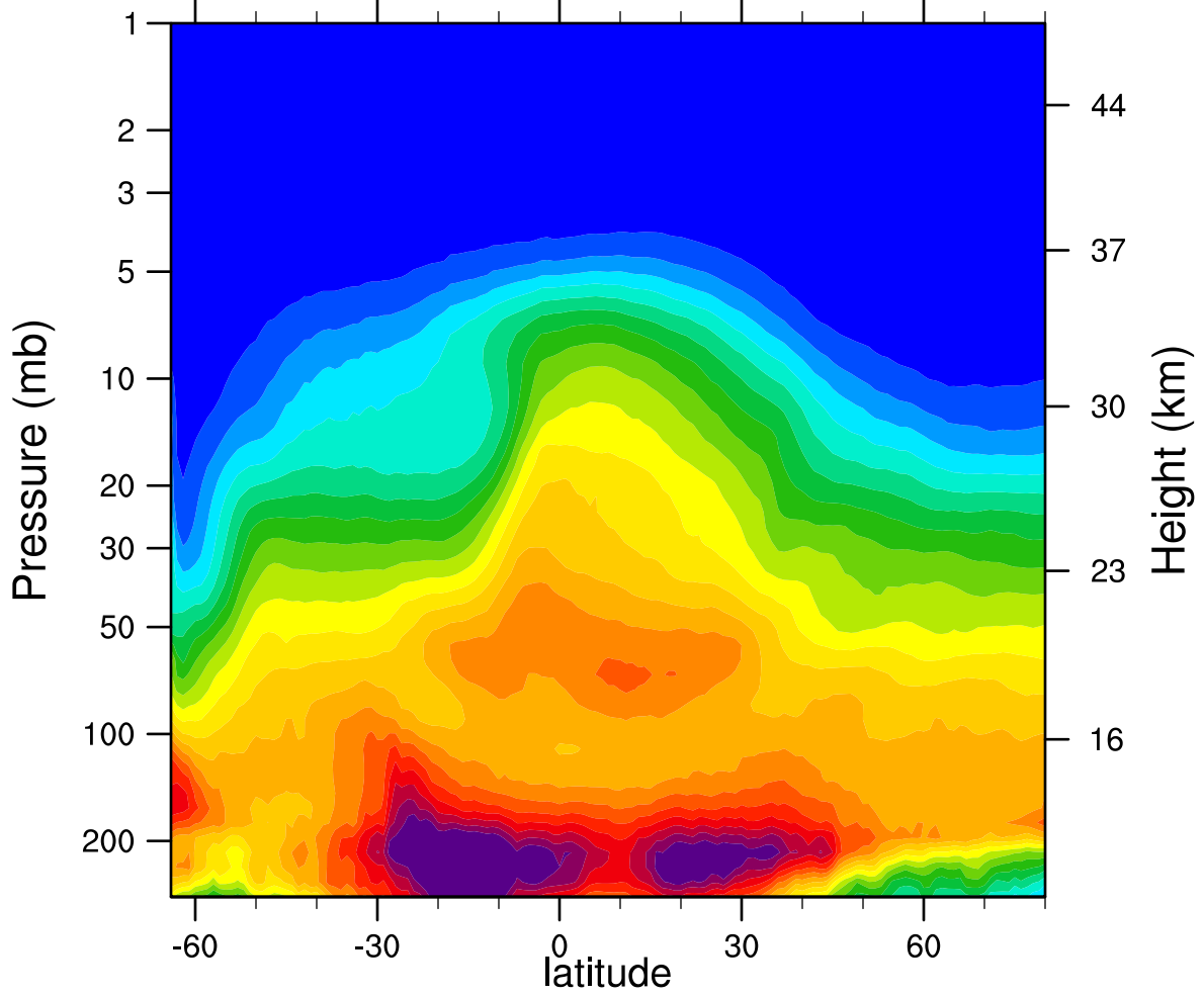
2006d244 N2O_Combined (ppbv)
