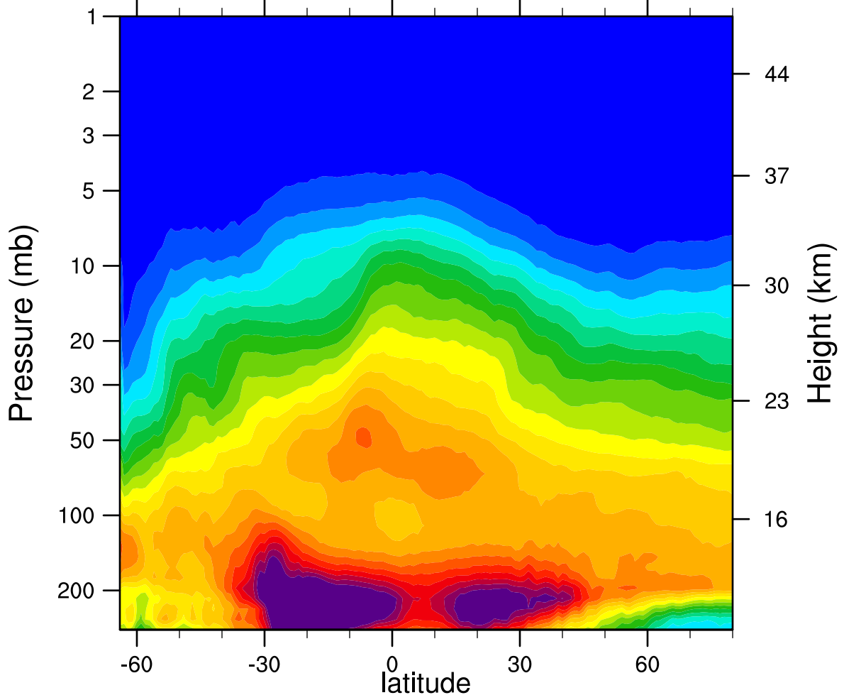
2006d177 N2O_Combined (ppbv)
