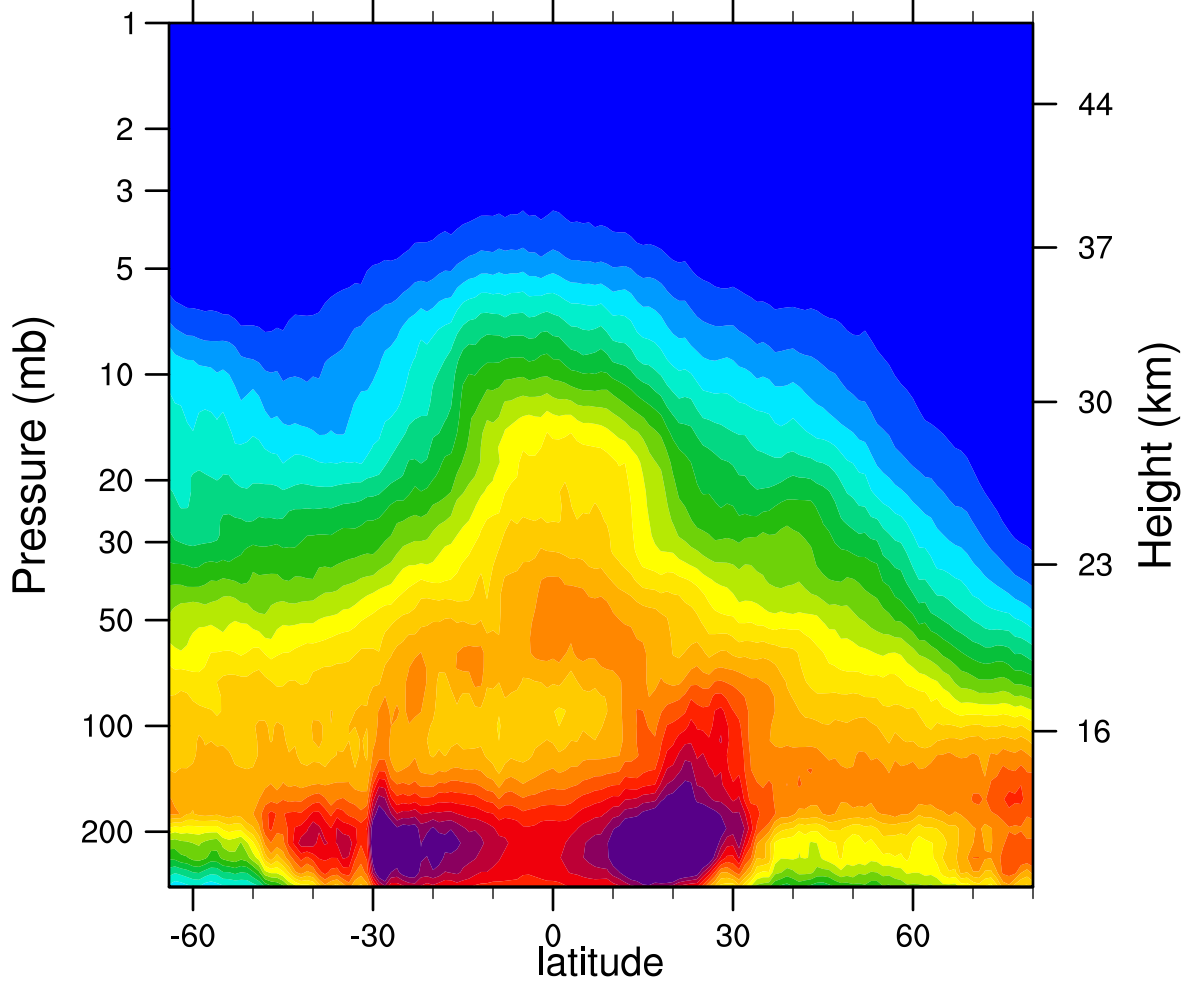
2005d028 N2O_Combined (ppbv)
