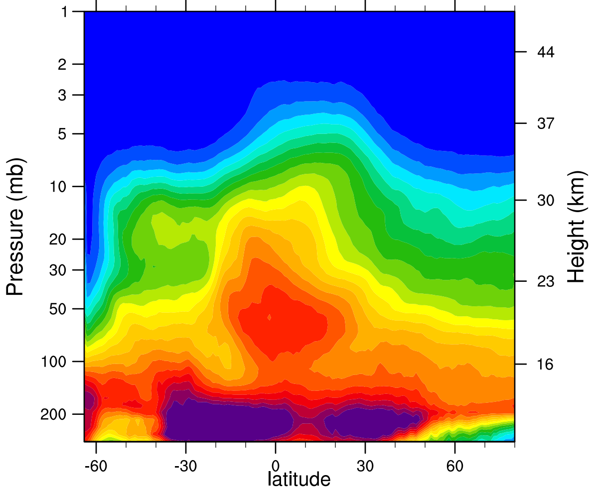
2007d224 N2O_Combined (ppbv)
