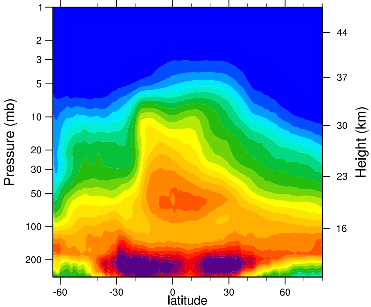
2005d275 N2O_Combined (ppbv)
