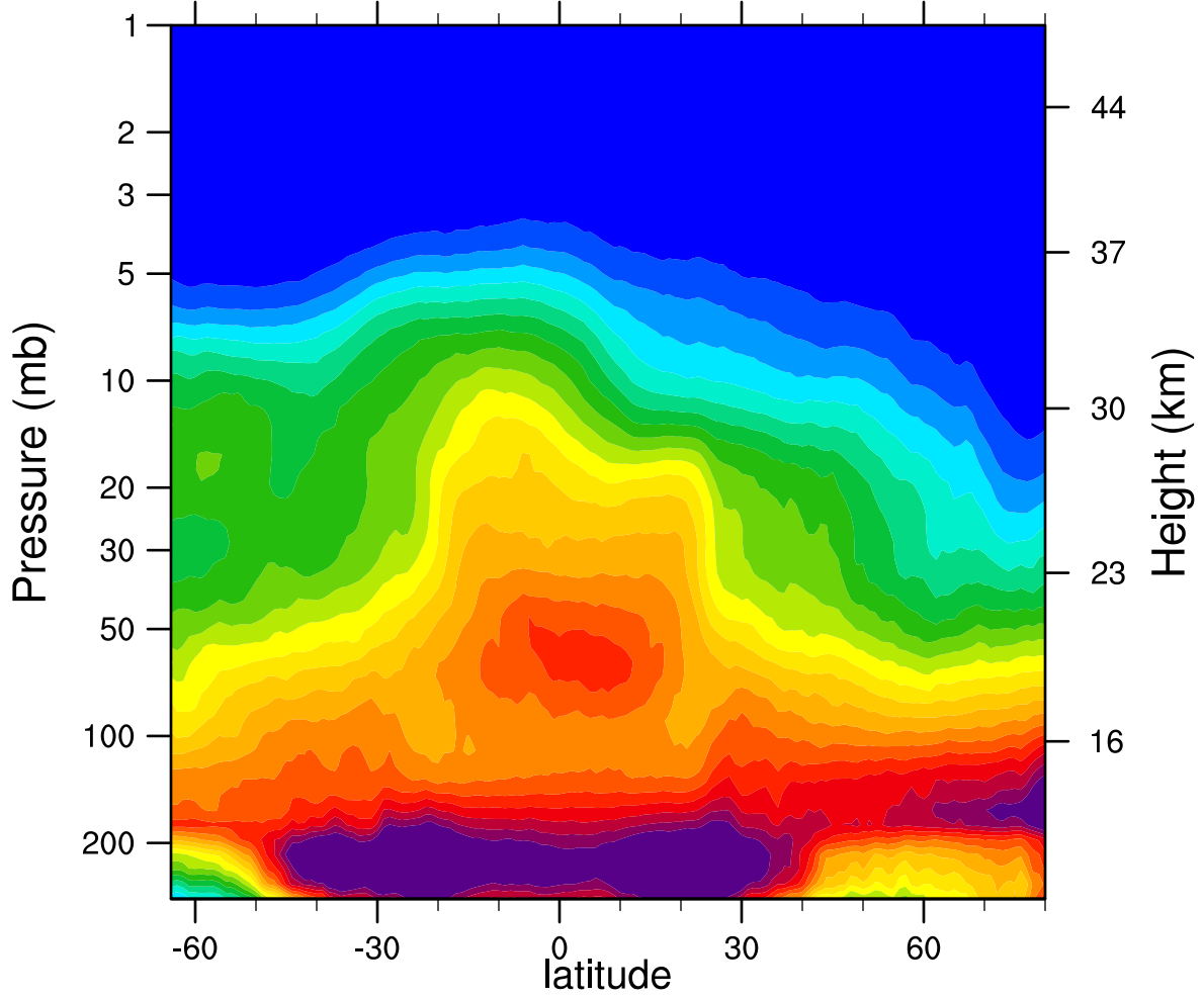
2007d356 N2O_Combined (ppbv)
