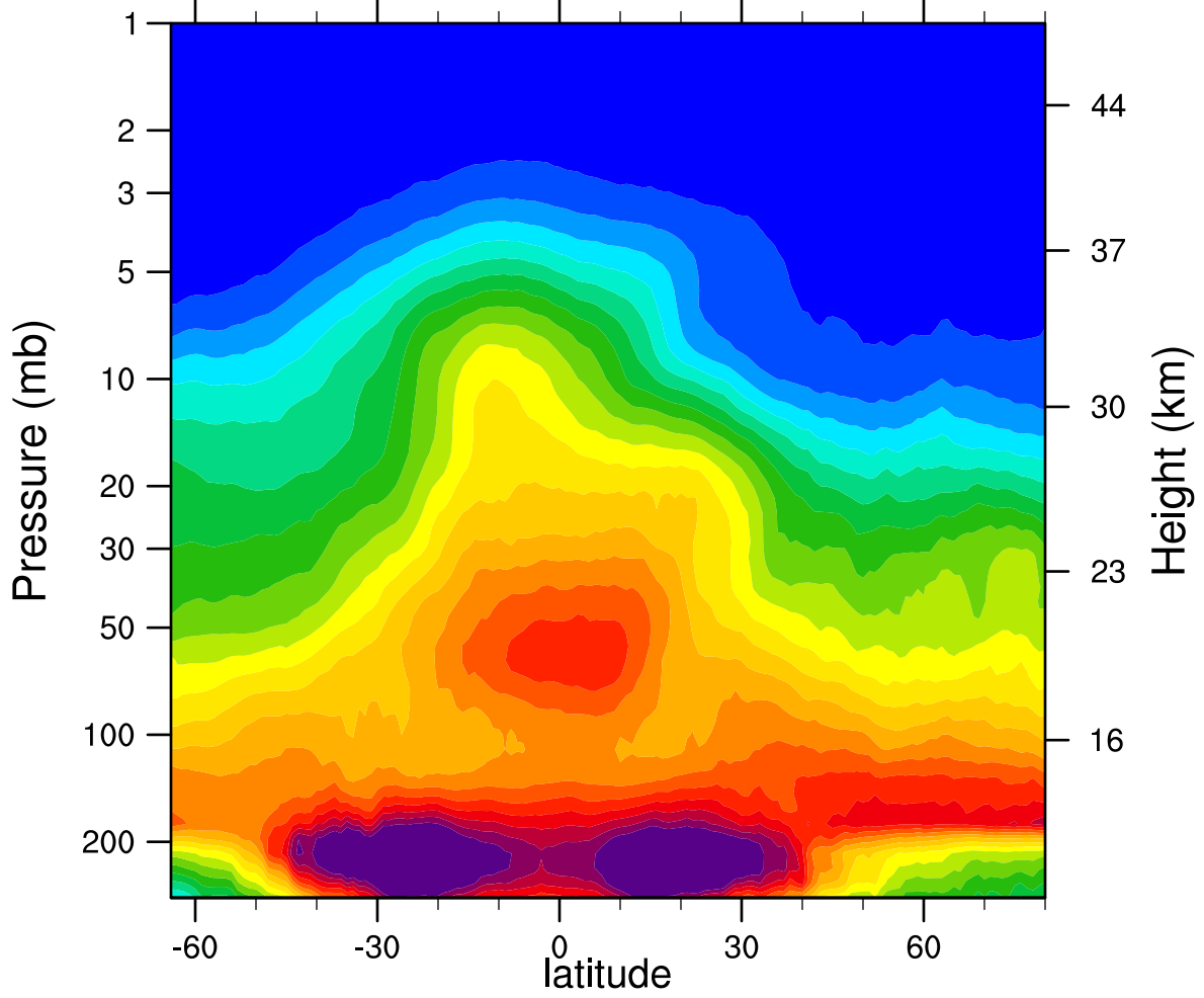
2006d046 N2O_Combined (ppbv)
