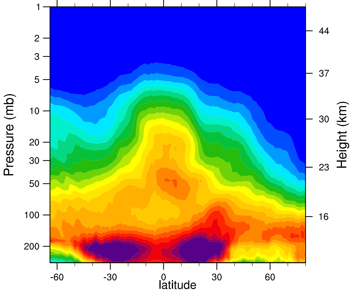
2005d032 N2O_Combined (ppbv)
