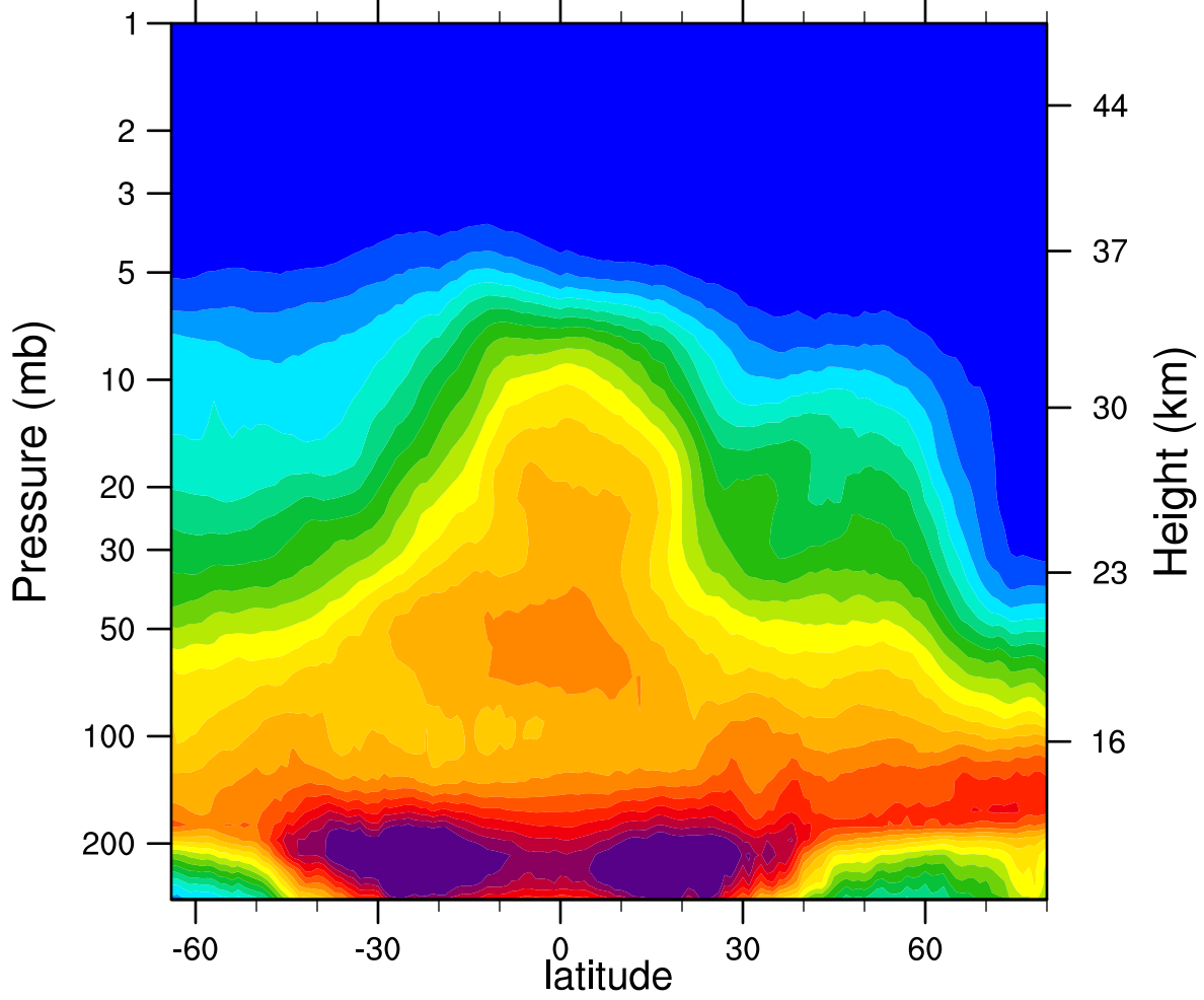
2007d011 N2O_Combined (ppbv)
