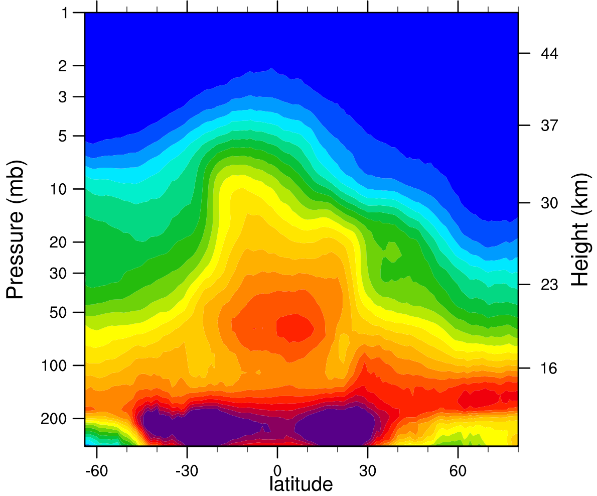
2006d013 N2O_Combined (ppbv)
