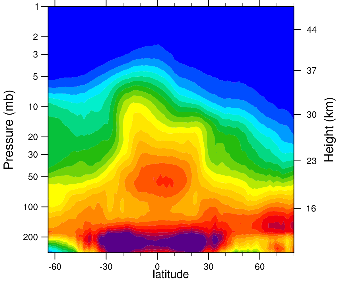
2005d356 N2O_Combined (ppbv)
