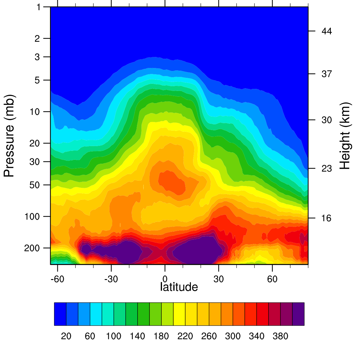
2005d049 N2O_Combined (ppbv)
