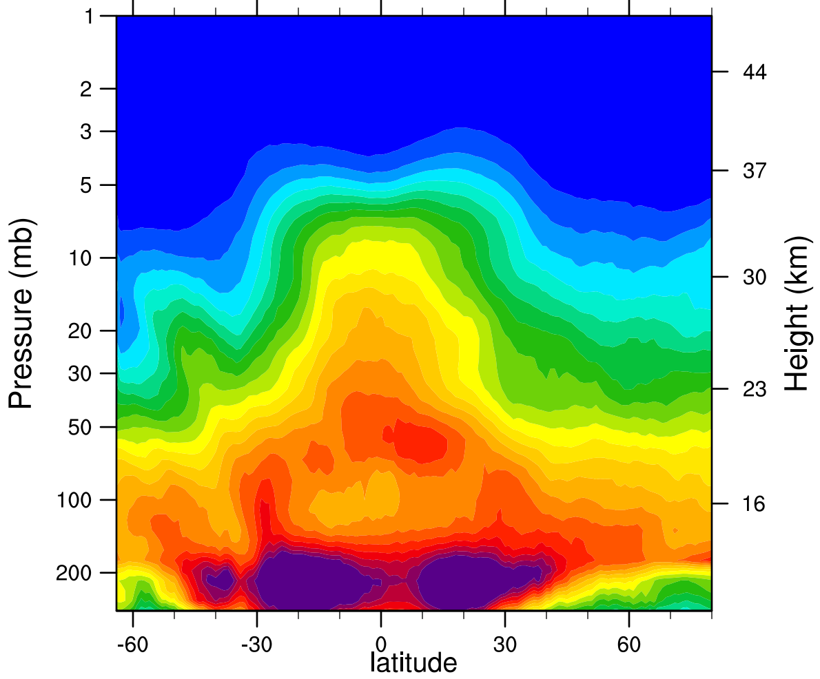
2005d113 N2O_Combined (ppbv)
