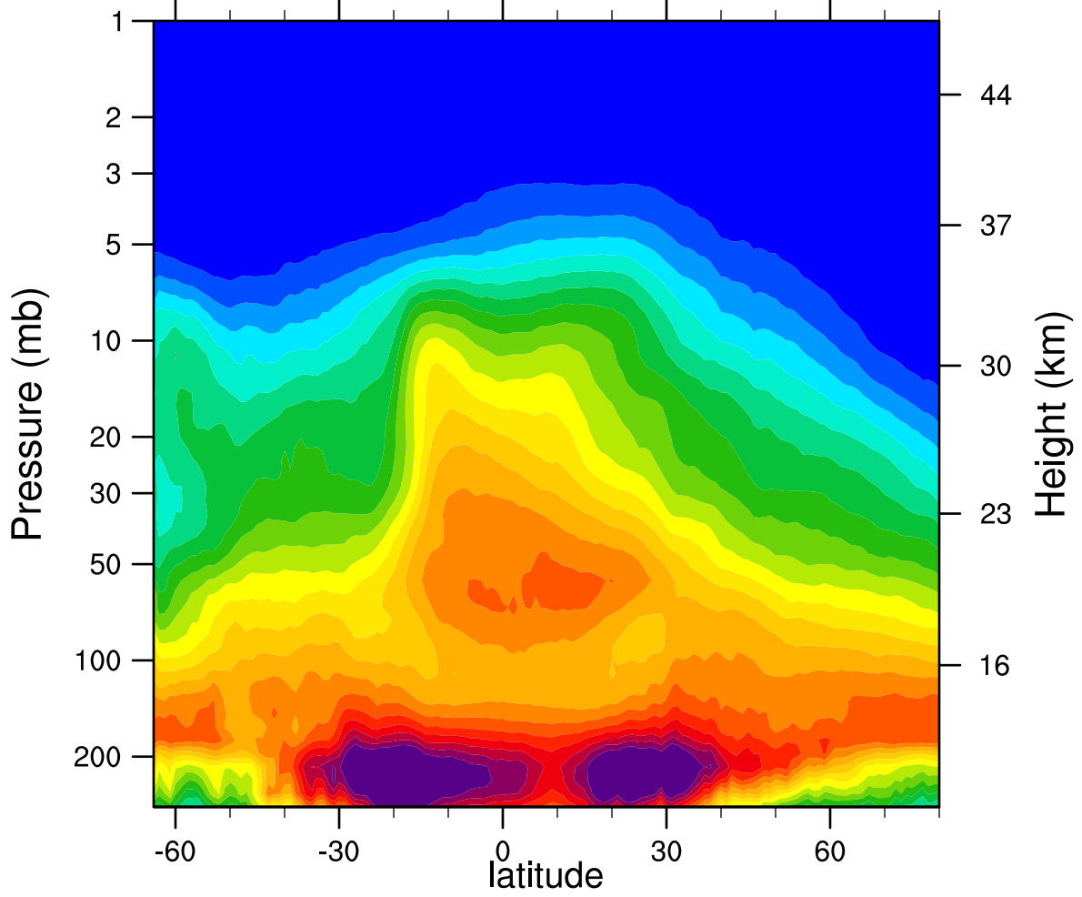
2005d286 N2O_Combined (ppbv)
