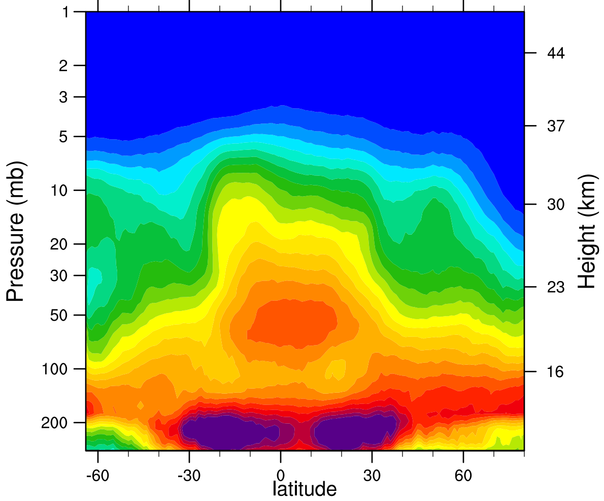
2005d321 N2O_Combined (ppbv)
