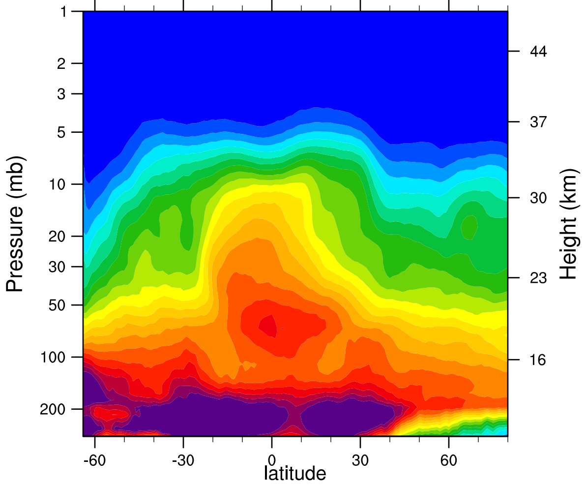
2007d155 N2O_Combined (ppbv)
