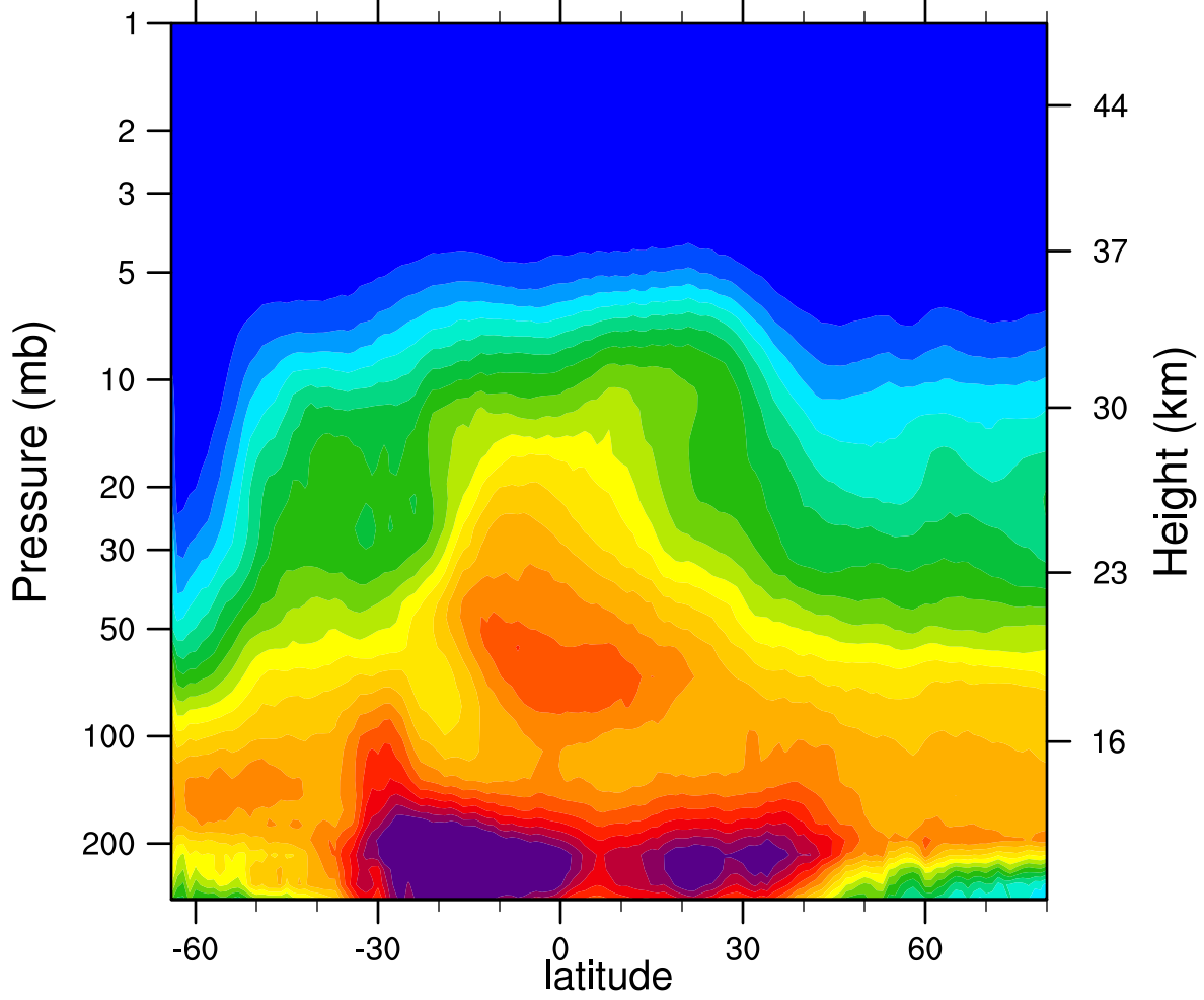
2007d191 N2O_Combined (ppbv)
