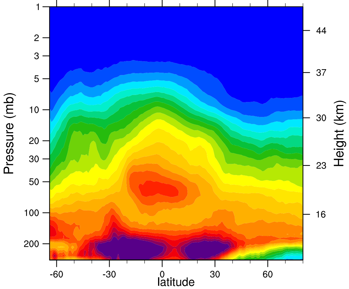
2006d148 N2O_Combined (ppbv)
