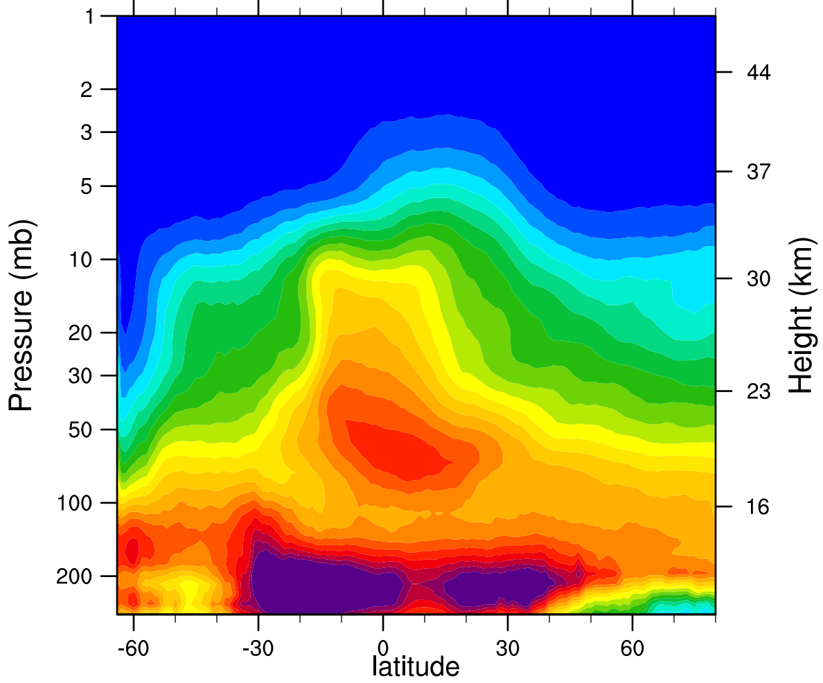
2005d211 N2O_Combined (ppbv)
