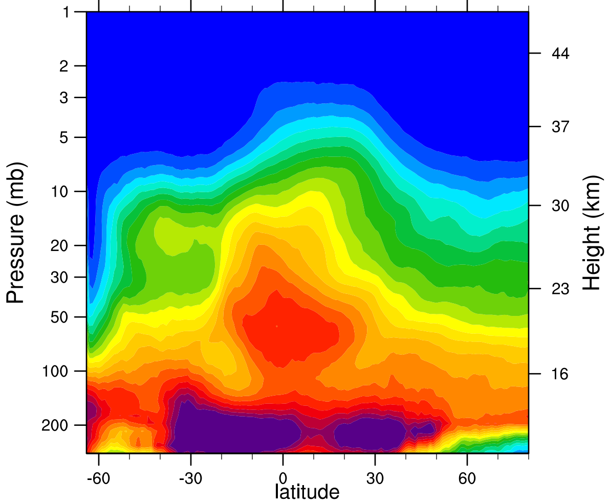
2007d227 N2O_Combined (ppbv)
