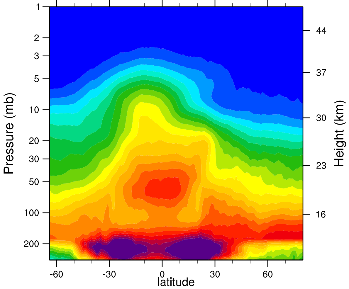
2006d055 N2O_Combined (ppbv)
