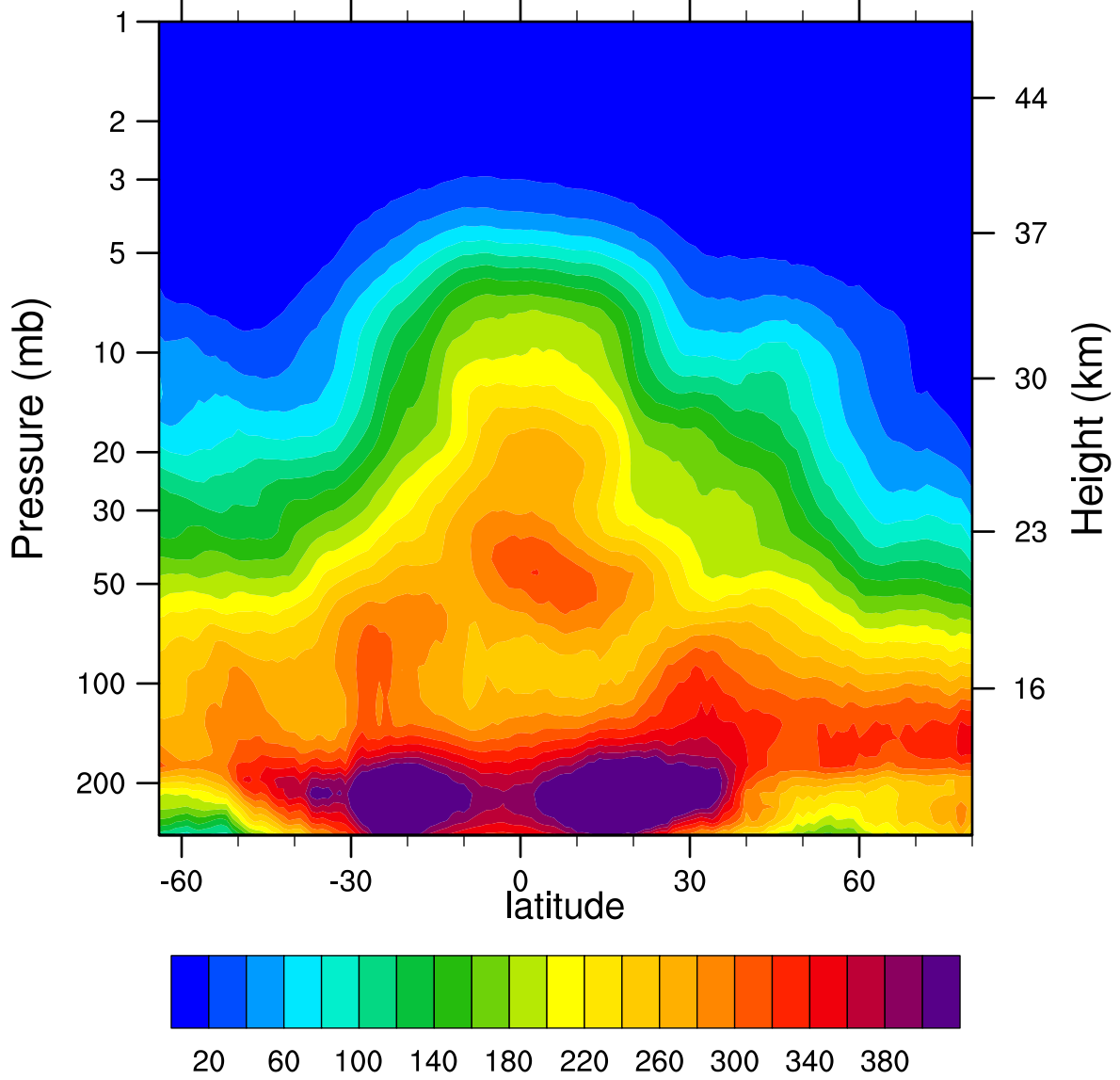
2005d066 N2O_Combined (ppbv)
