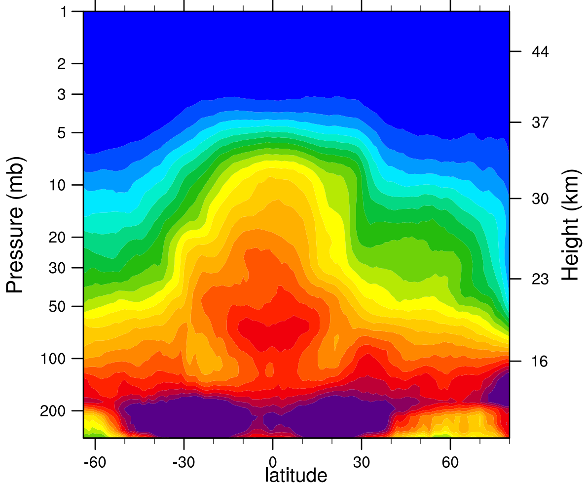
2007d087 N2O_Combined (ppbv)
