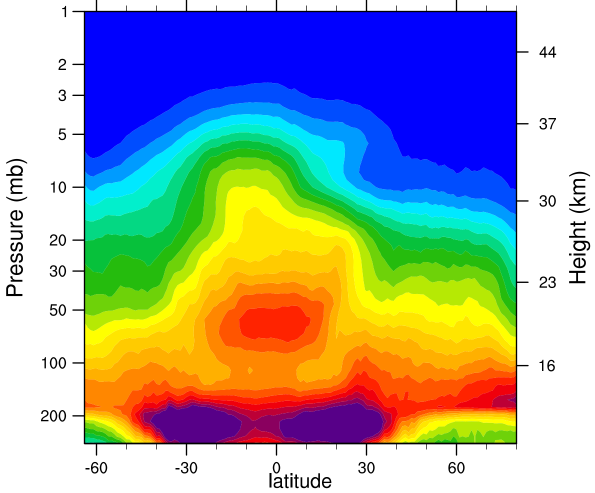
2006d068 N2O_Combined (ppbv)
