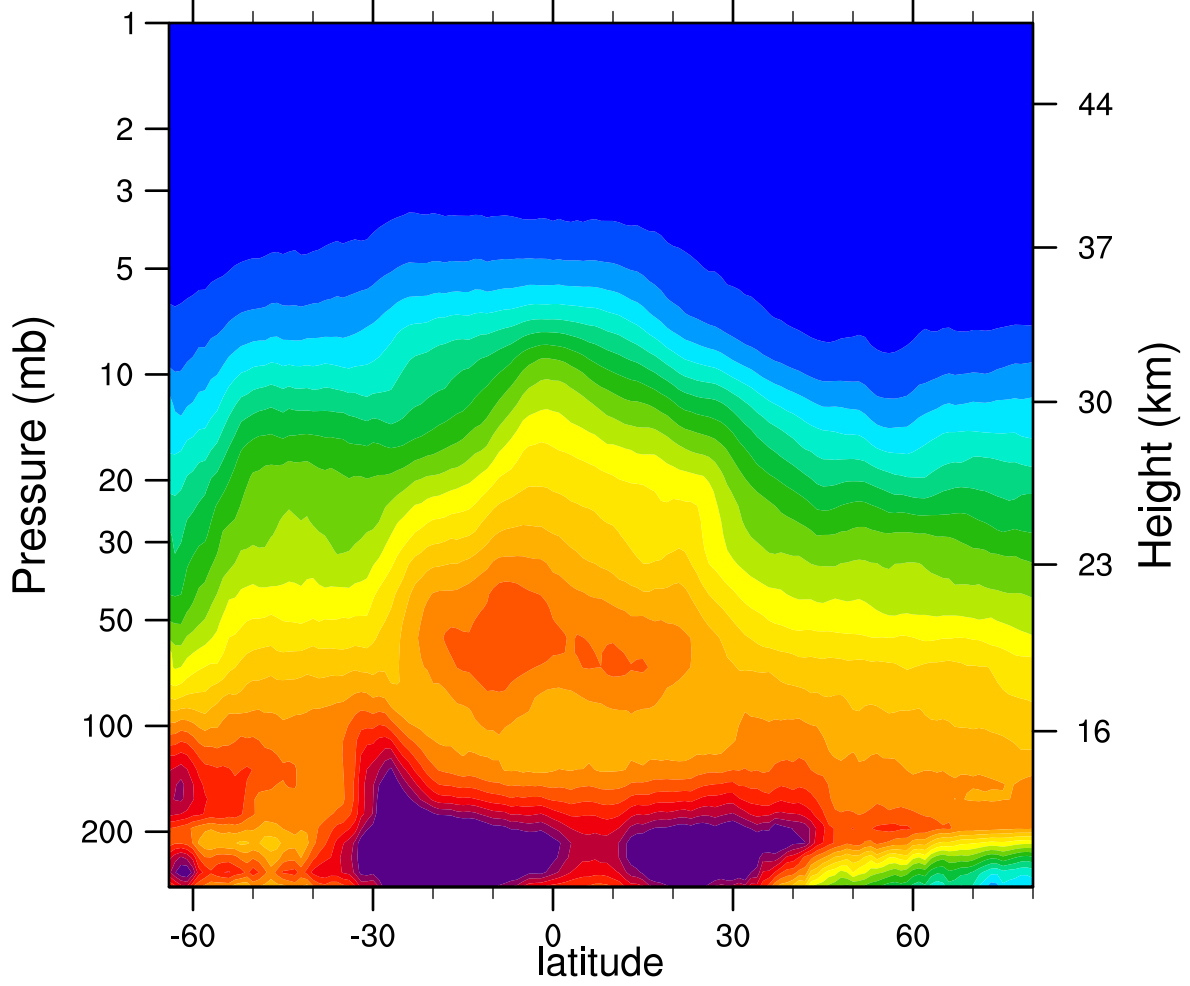
2006d165 N2O_Combined (ppbv)
