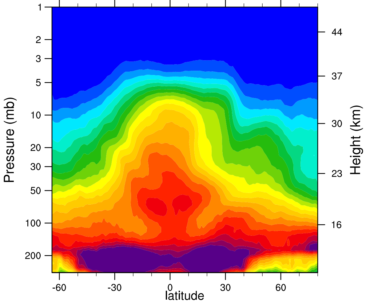
2007d102 N2O_Combined (ppbv)
