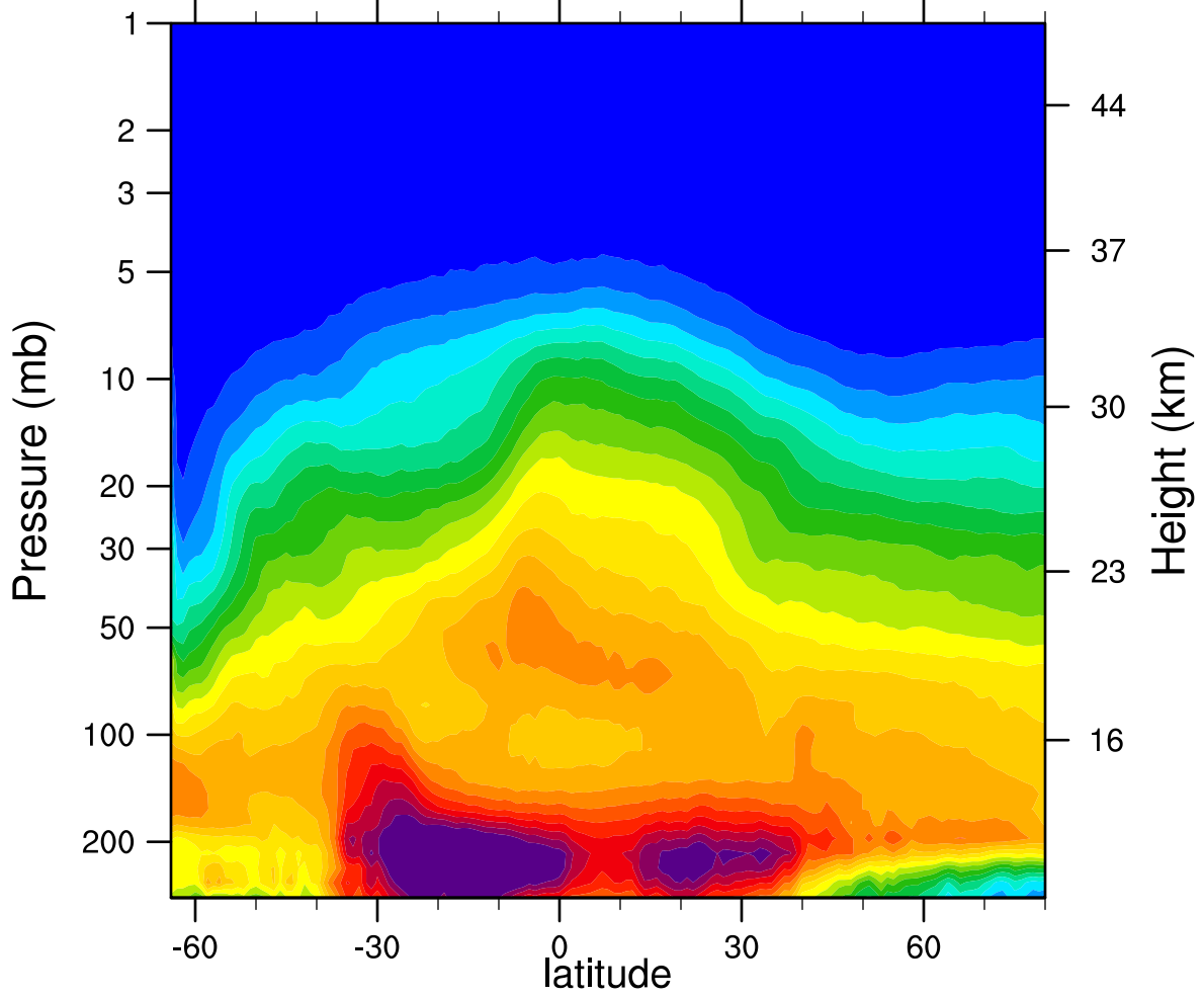
2006d187 N2O_Combined (ppbv)
