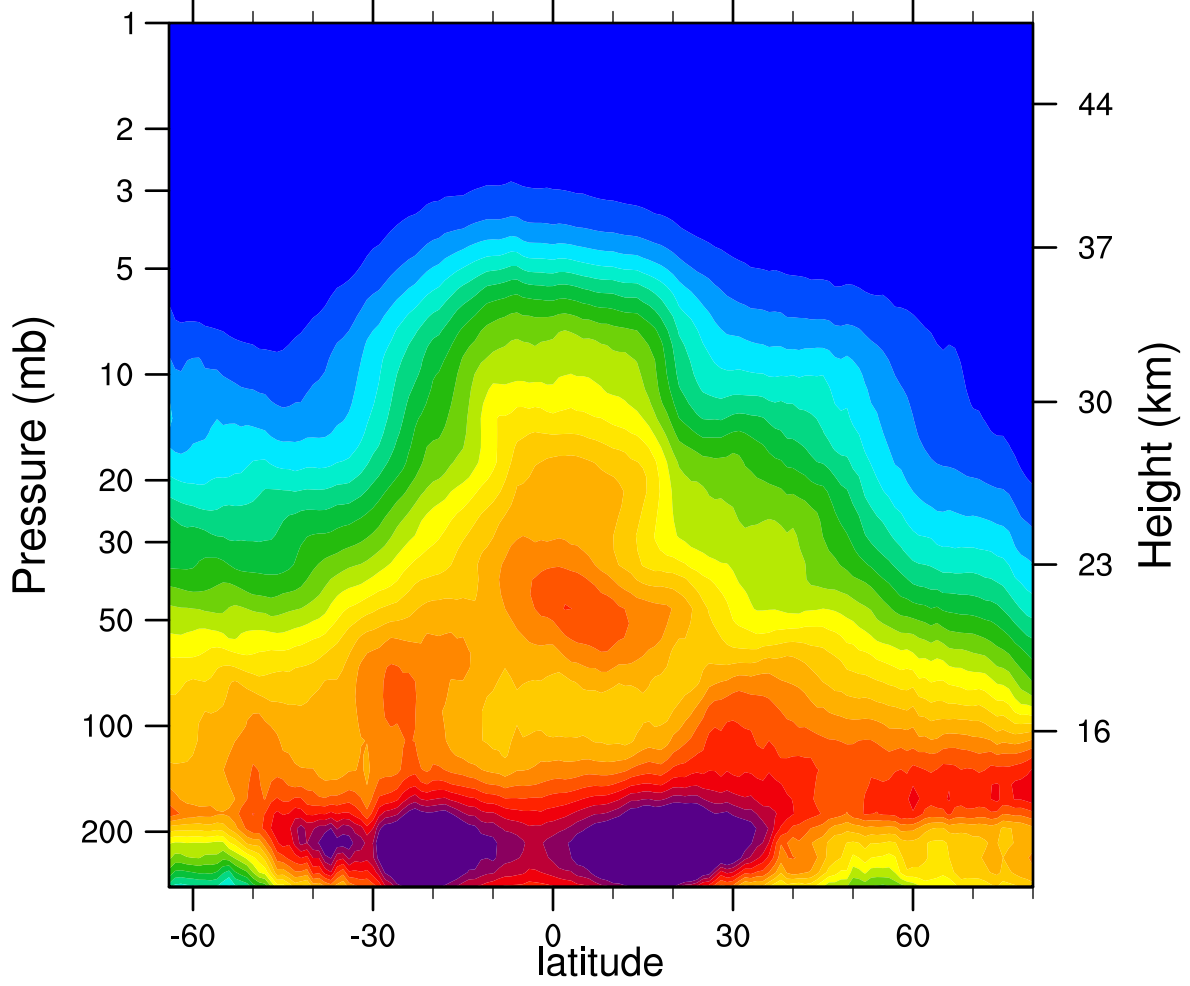
2005d063 N2O_Combined (ppbv)
