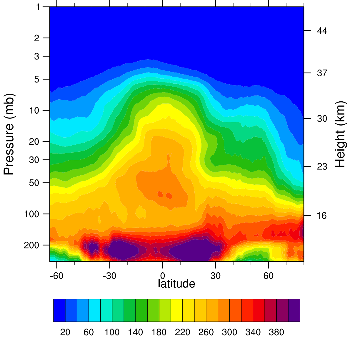
2007d037 N2O_Combined (ppbv)
