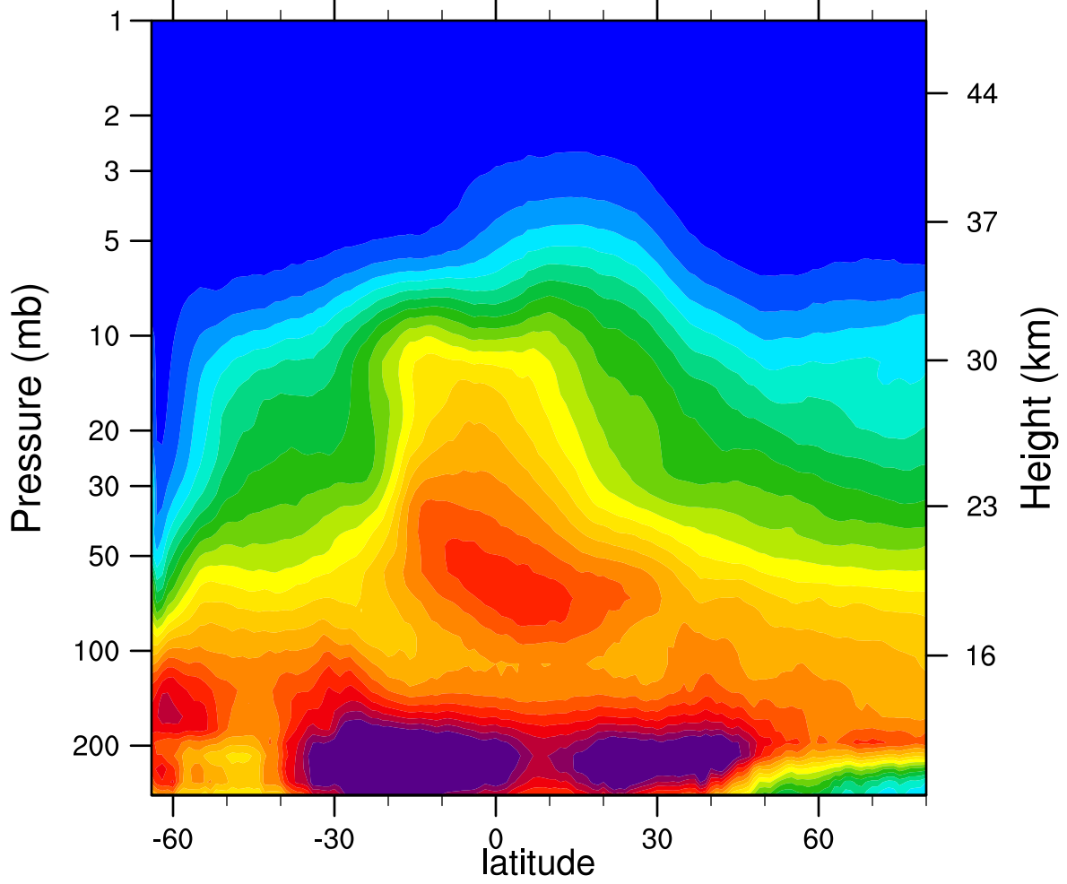
2005d202 N2O_Combined (ppbv)
