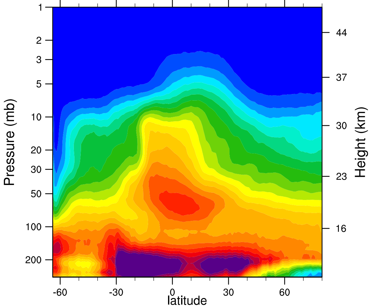
2005d214 N2O_Combined (ppbv)
