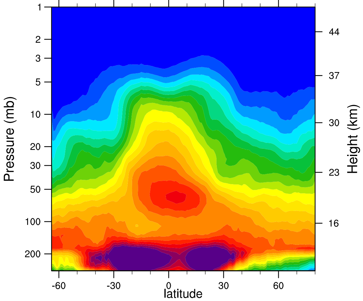
2005d129 N2O_Combined (ppbv)
