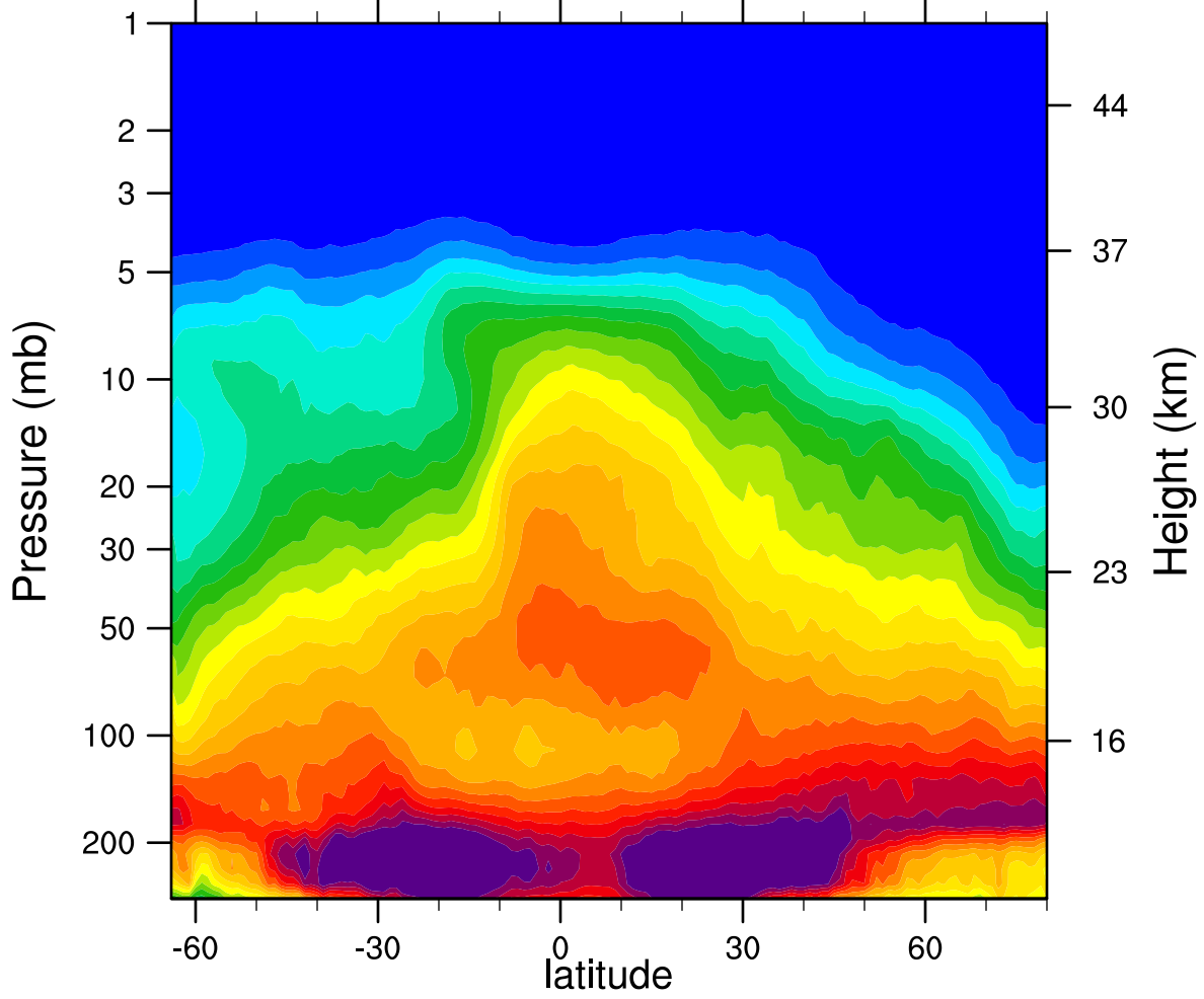
2006d313 N2O_Combined (ppbv)
