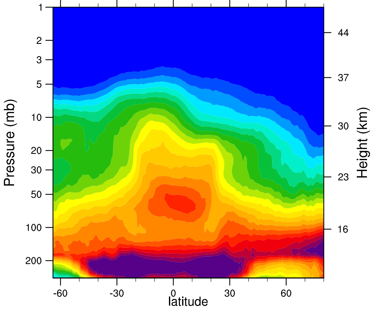
2007d354 N2O_Combined (ppbv)
