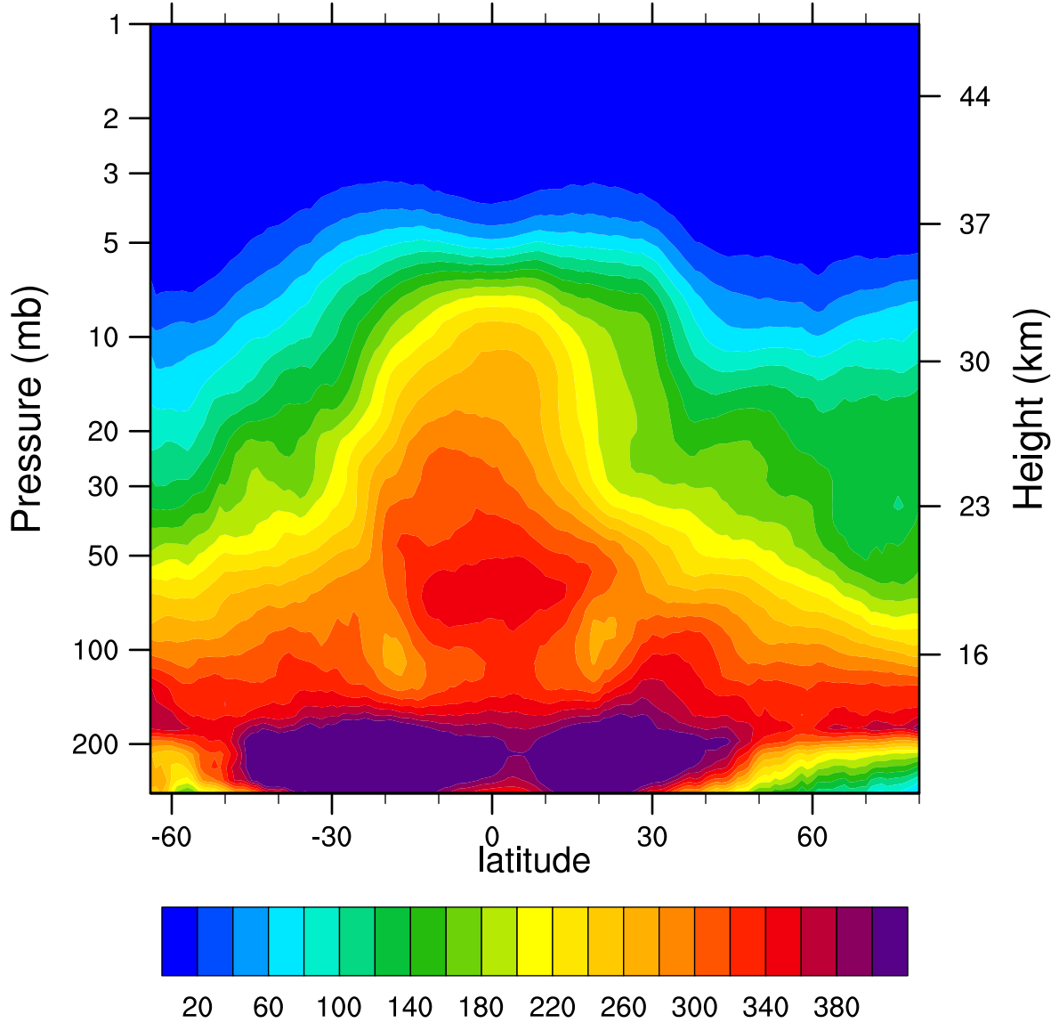
2007d116 N2O_Combined (ppbv)
