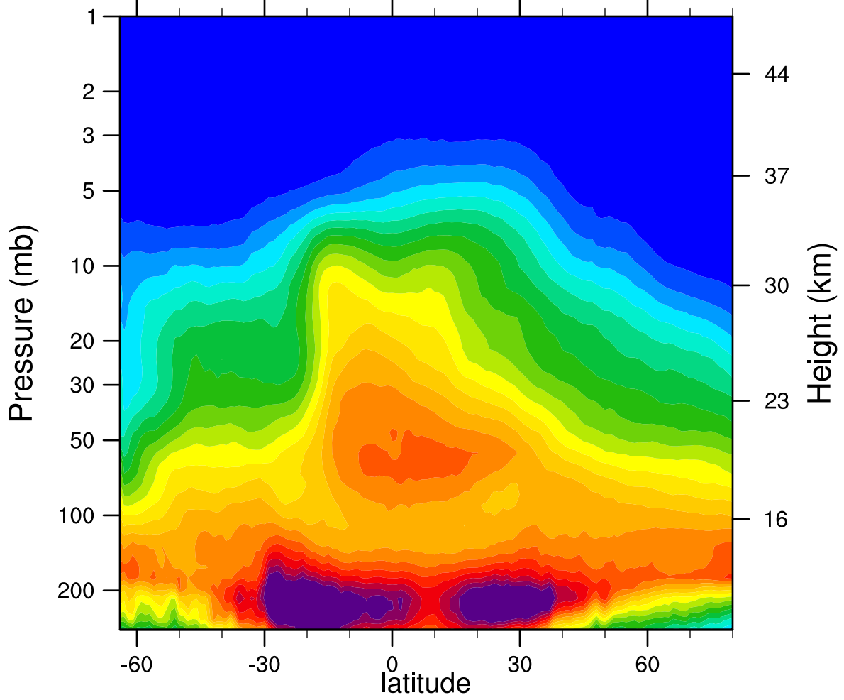
2005d277 N2O_Combined (ppbv)
