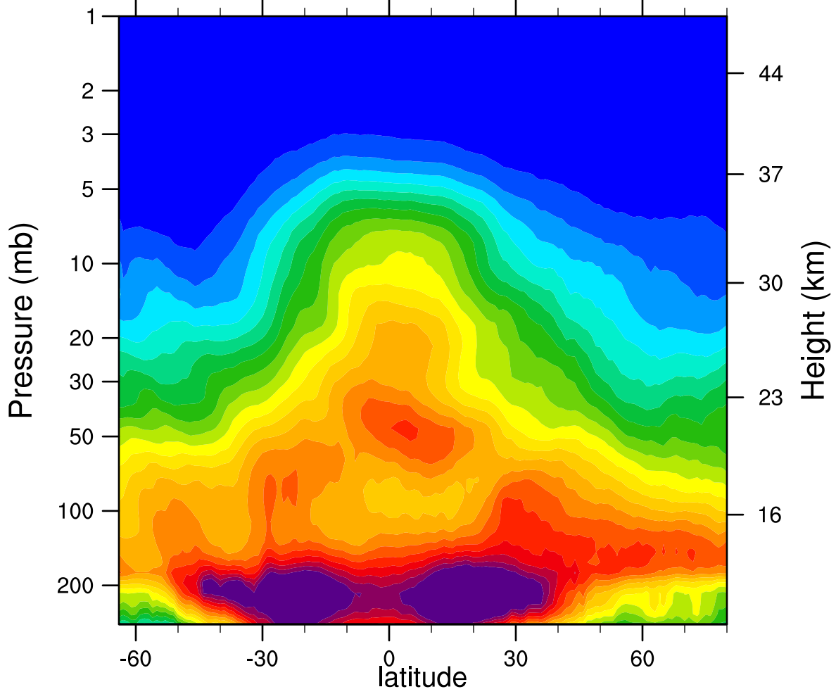
2005d073 N2O_Combined (ppbv)
