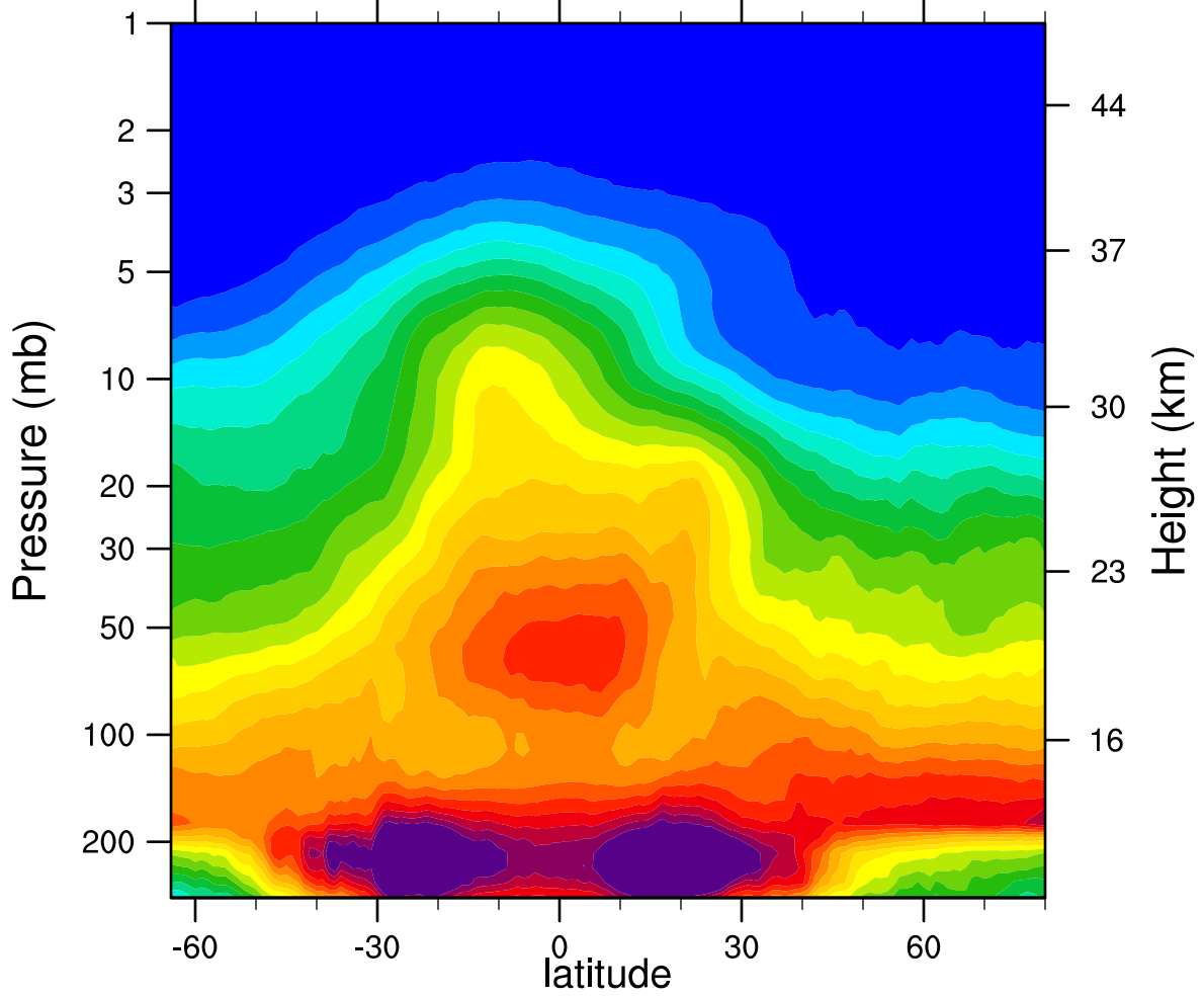
2006d049 N2O_Combined (ppbv)
