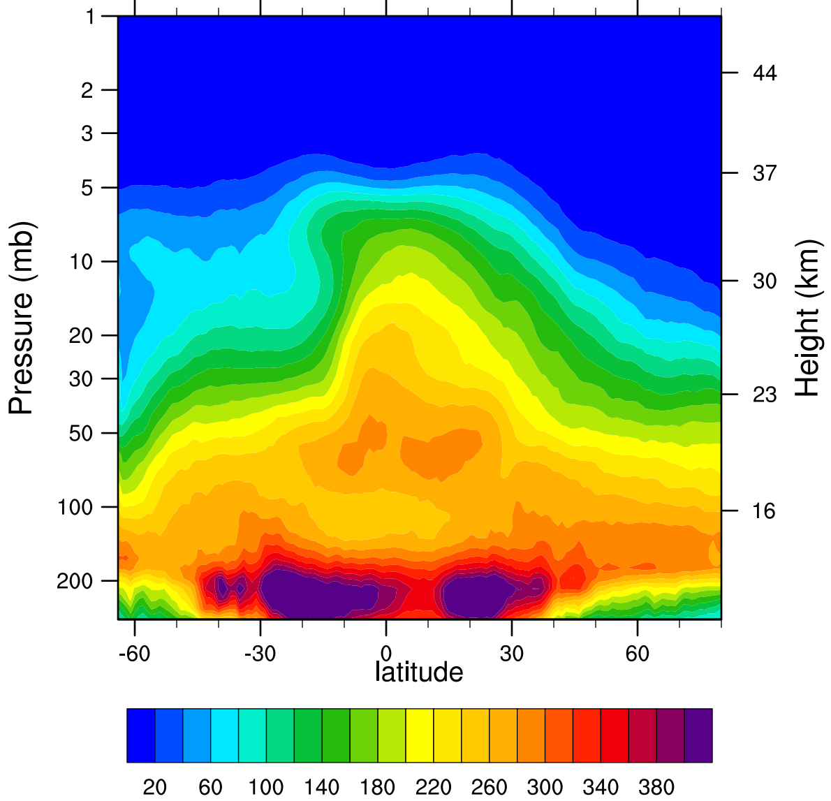
2006d292 N2O_Combined (ppbv)
