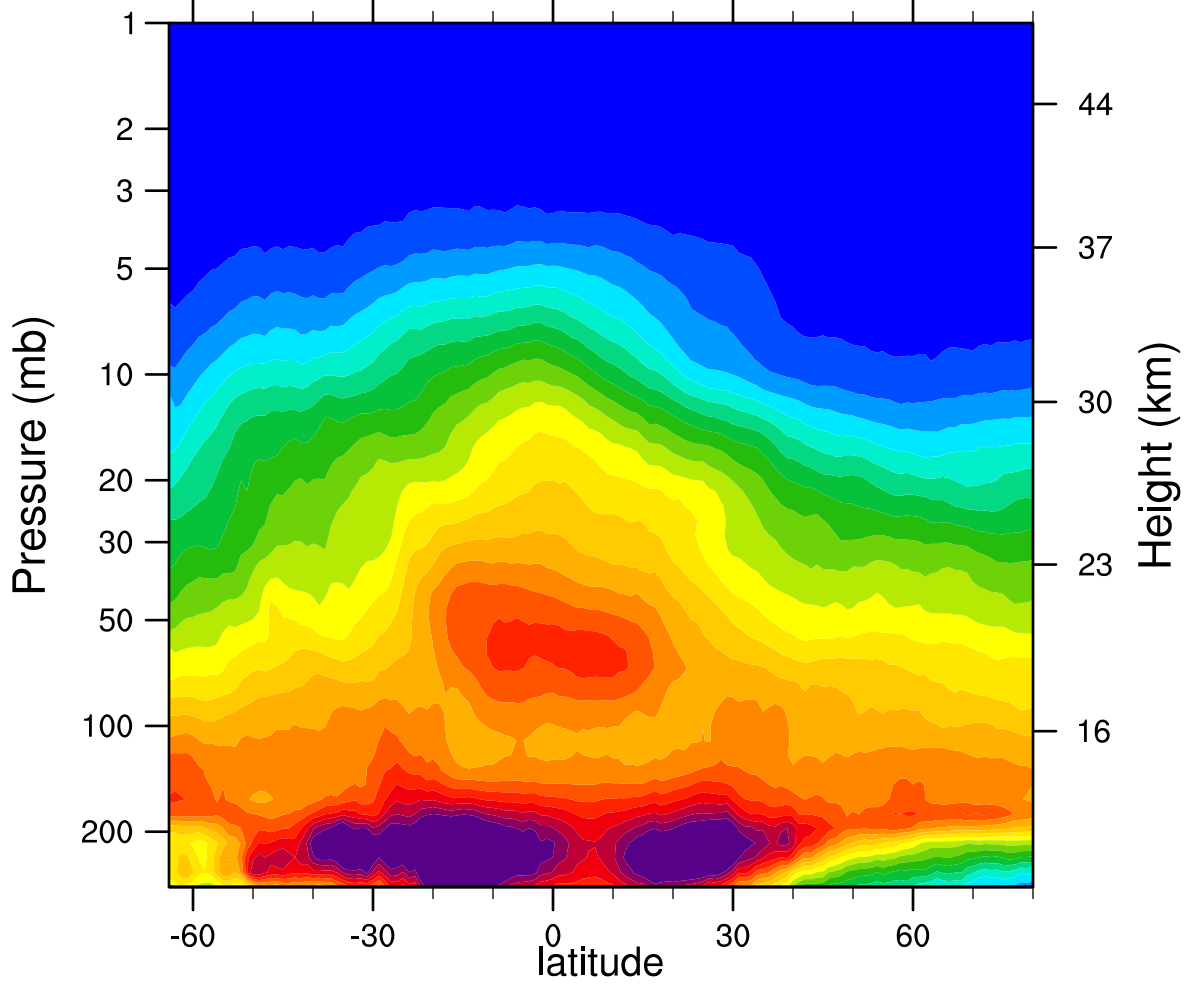
2006d136 N2O_Combined (ppbv)
