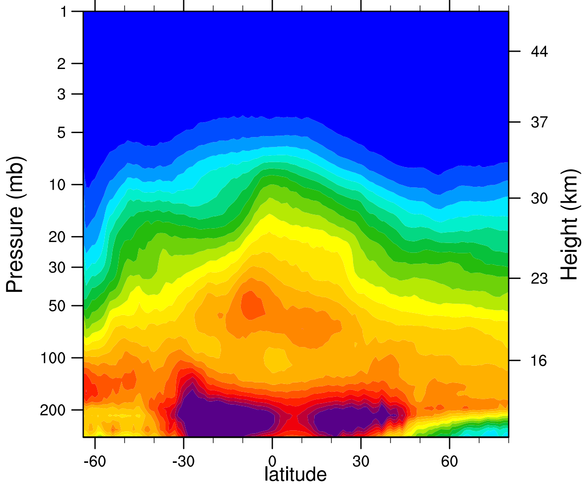
2006d175 N2O_Combined (ppbv)
