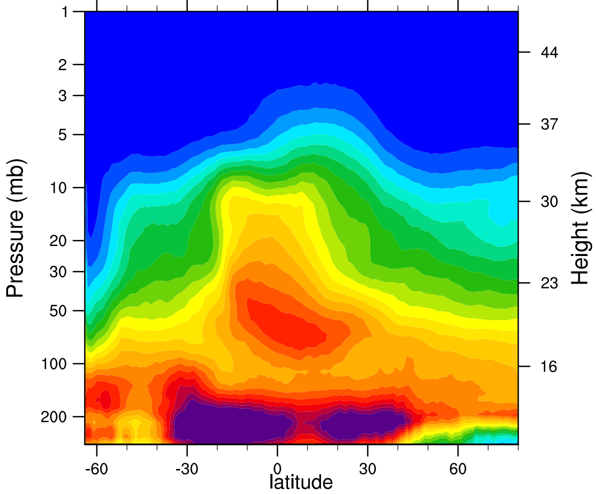
2005d207 N2O_Combined (ppbv)
