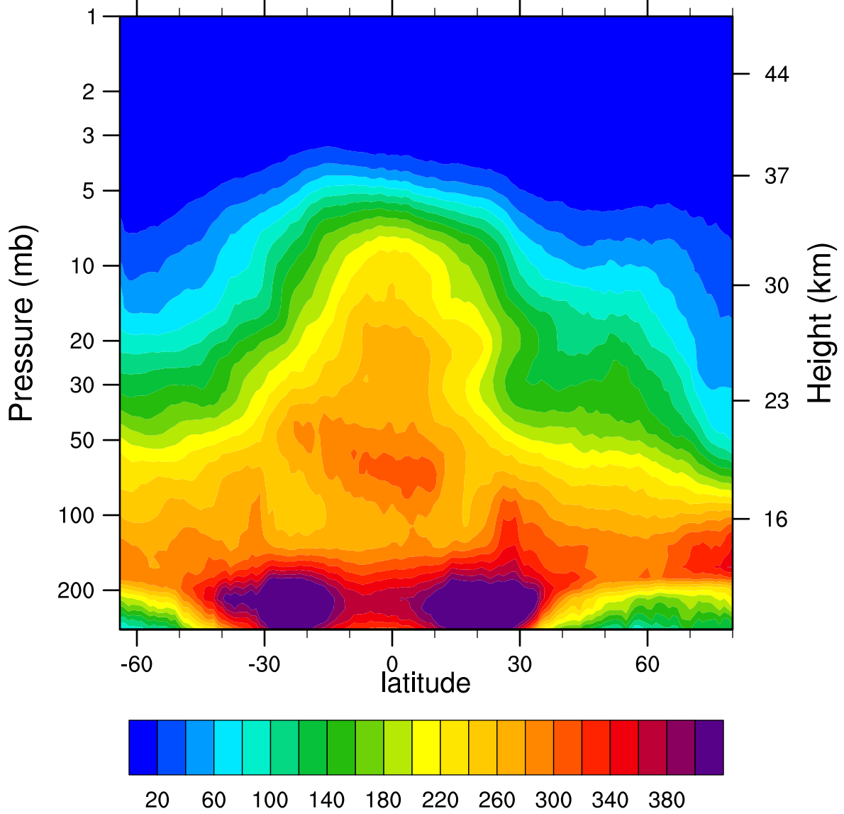
2007d063 N2O_Combined (ppbv)
