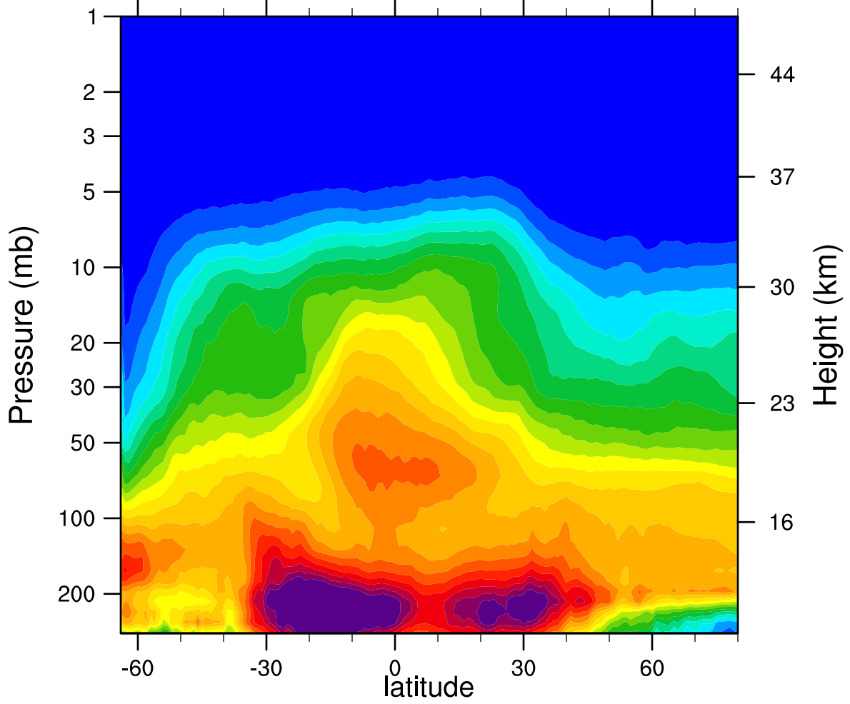
2007d197 N2O_Combined (ppbv)
