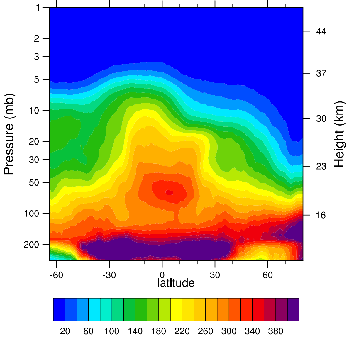
2007d365 N2O_Combined (ppbv)
