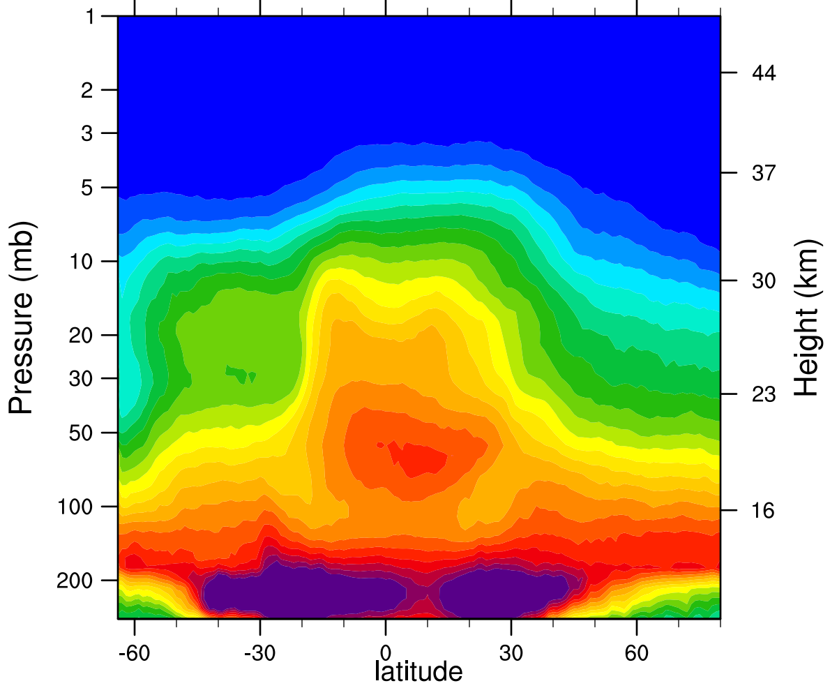
2007d291 N2O_Combined (ppbv)
