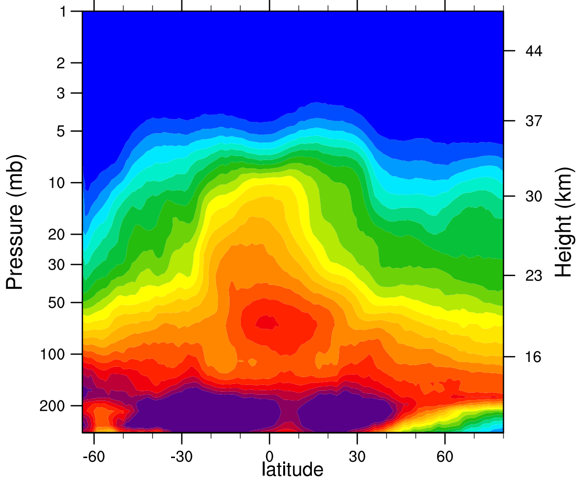
2007d143 N2O_Combined (ppbv)
