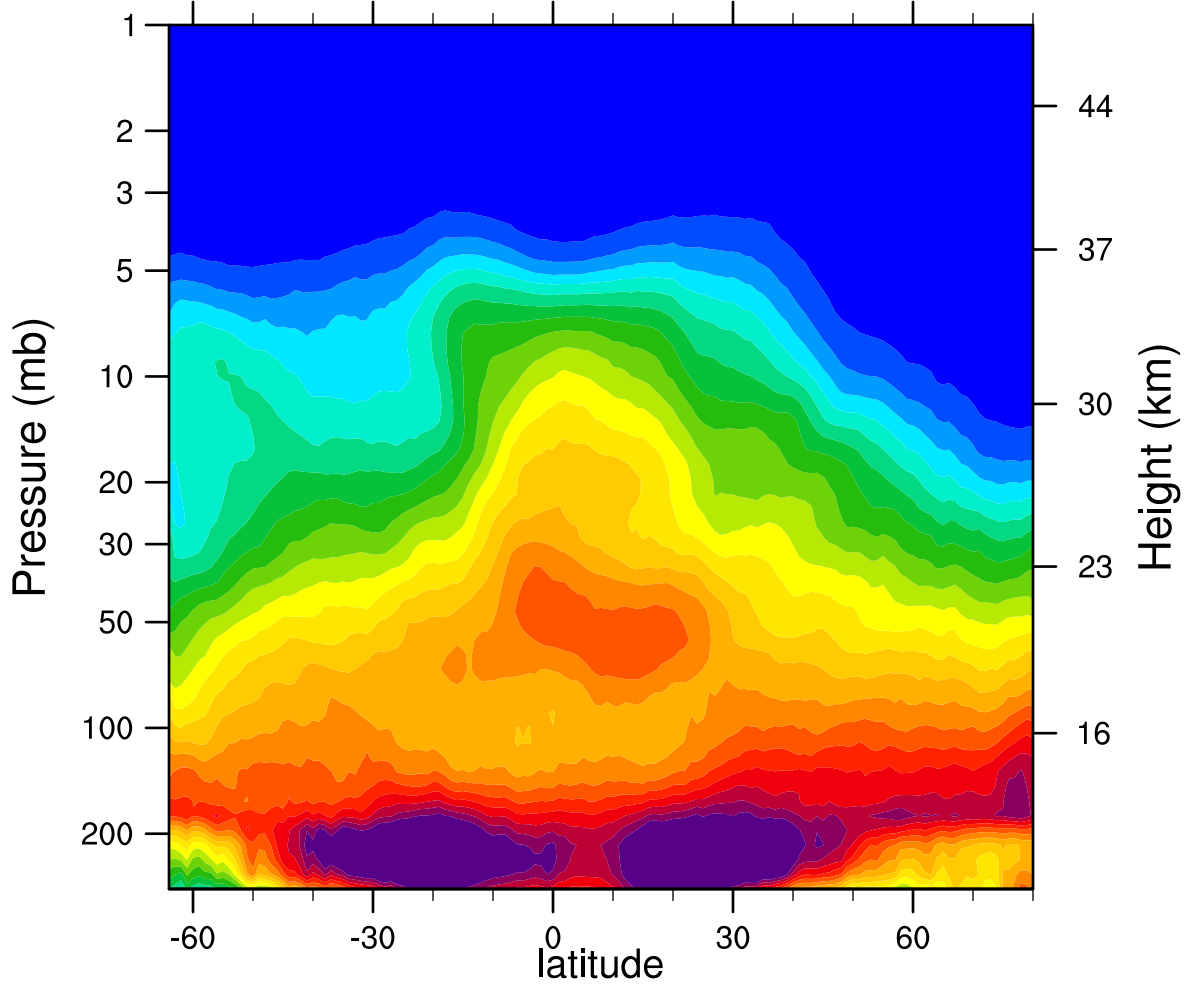
2006d320 N2O_Combined (ppbv)
