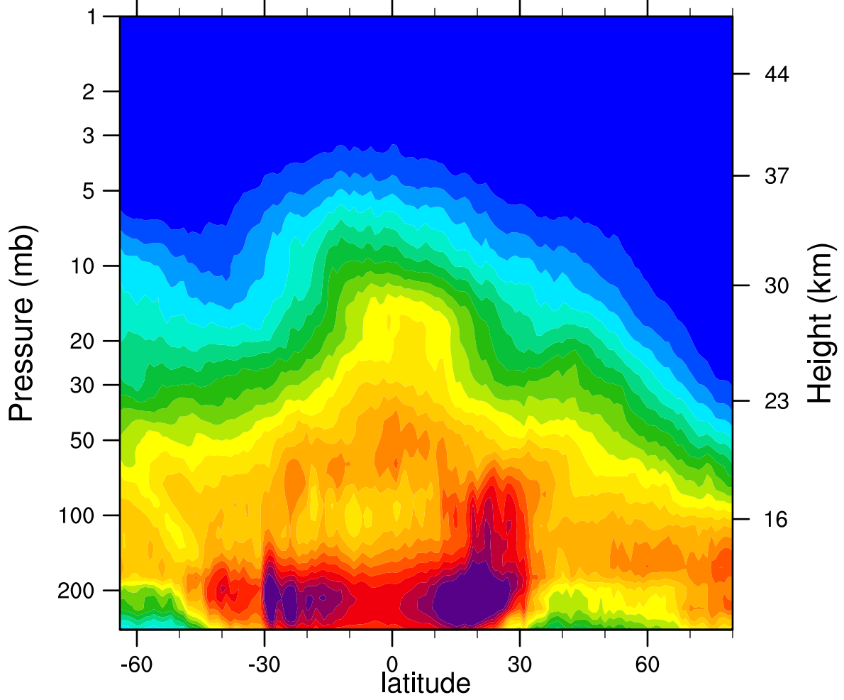
2005d027 N2O_Combined (ppbv)
