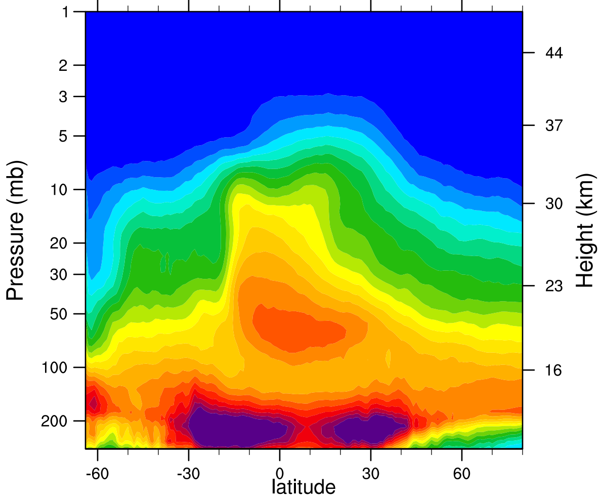
2005d256 N2O_Combined (ppbv)
