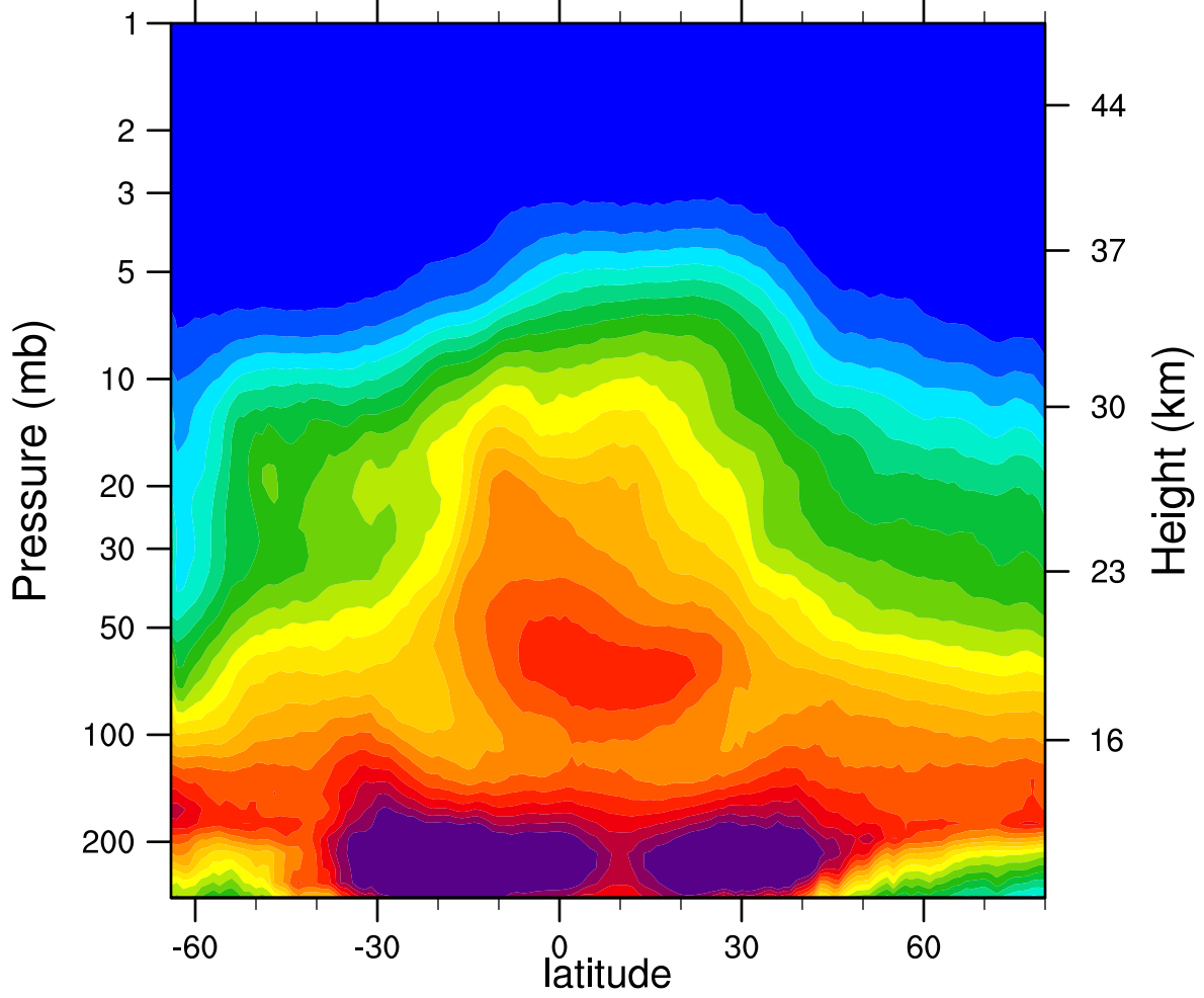
2007d266 N2O_Combined (ppbv)
