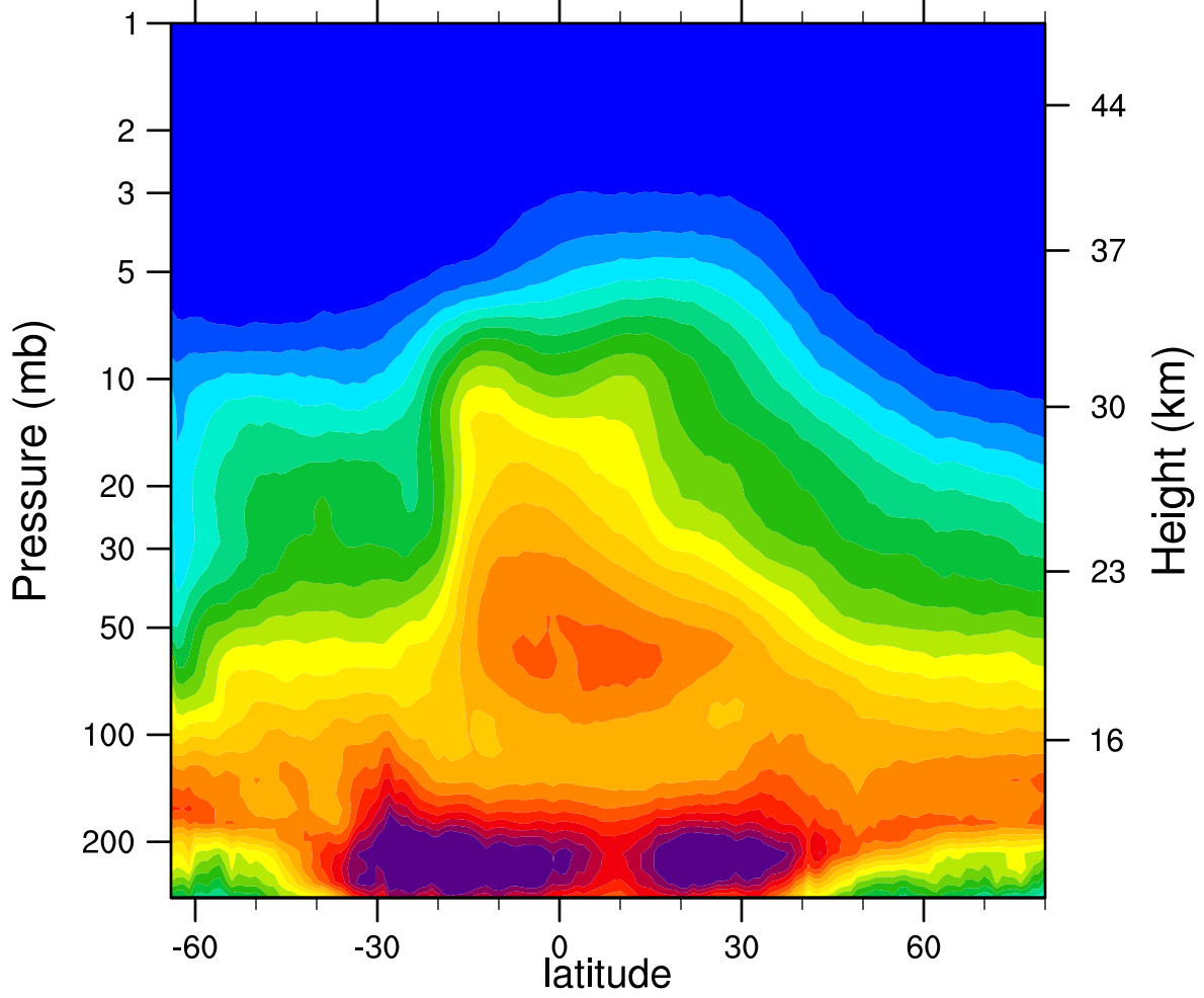
2005d271 N2O_Combined (ppbv)
