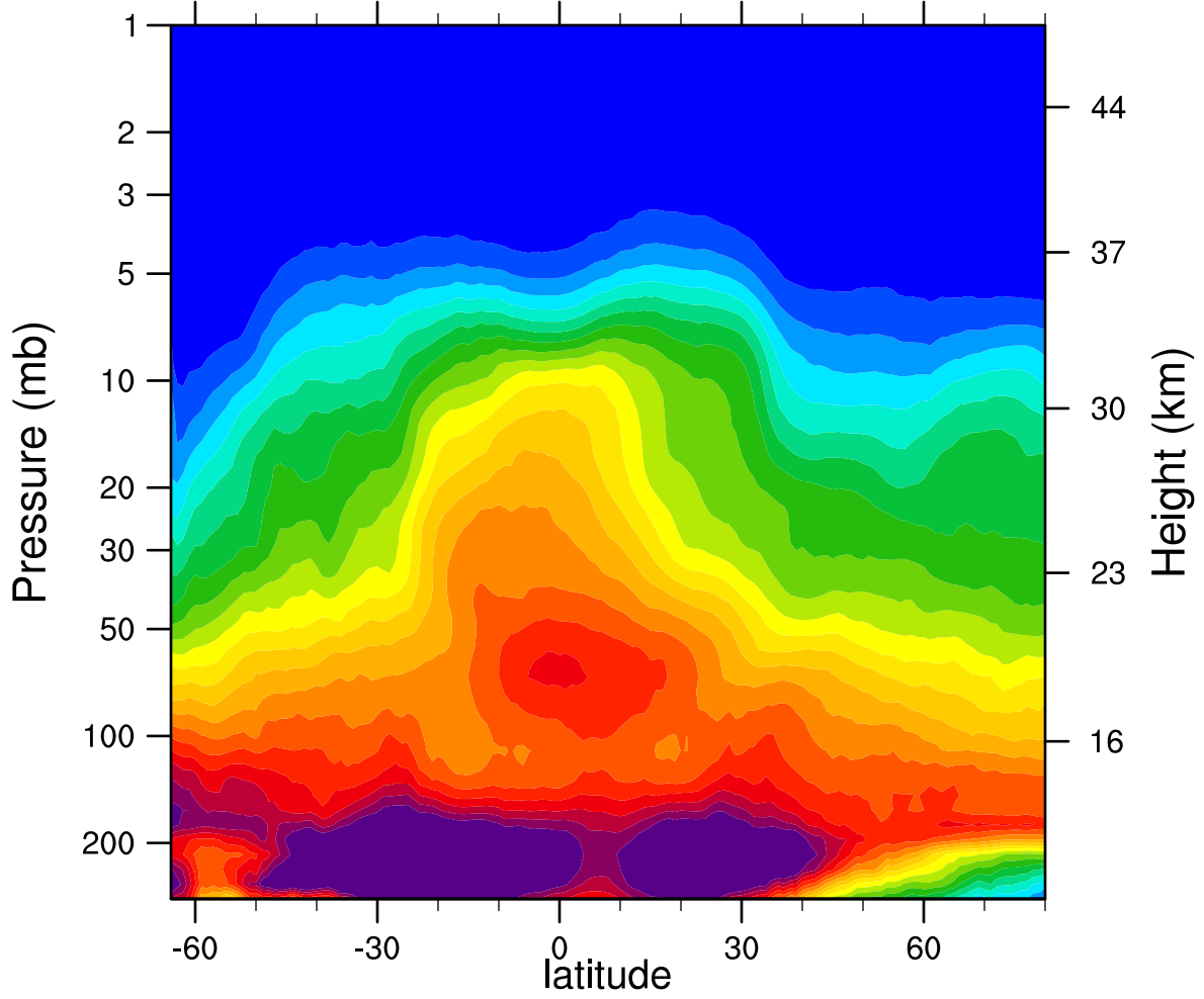
2007d142 N2O_Combined (ppbv)
