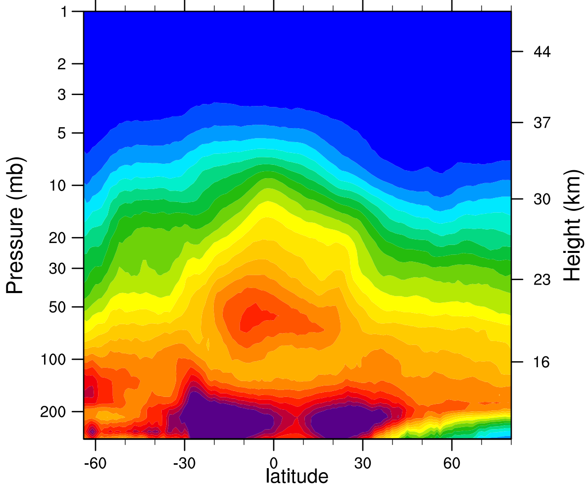
2006d157 N2O_Combined (ppbv)
