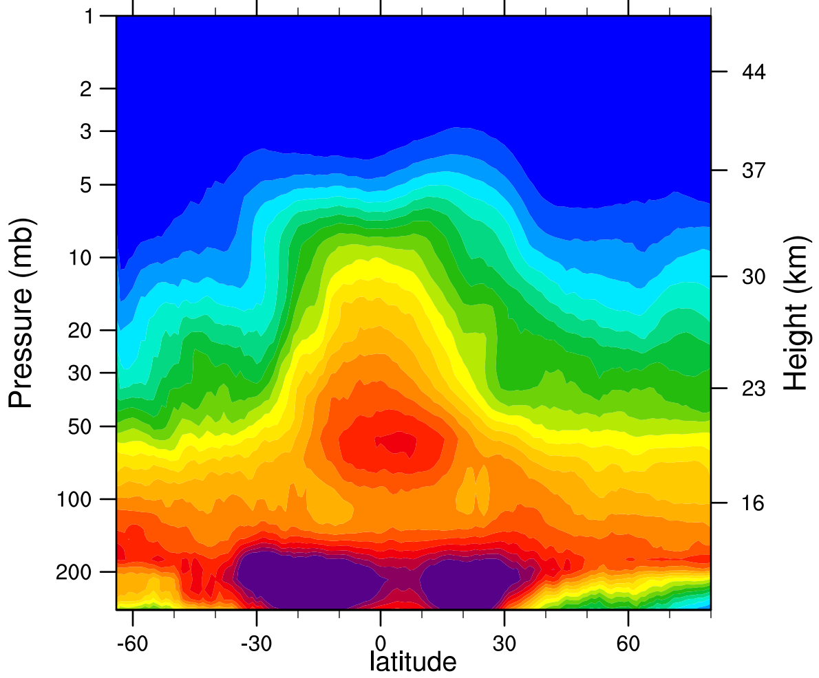
2005d138 N2O_Combined (ppbv)
