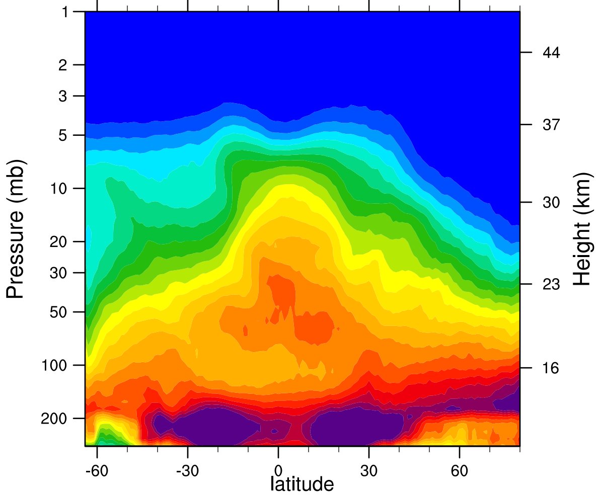
2006d329 N2O_Combined (ppbv)
