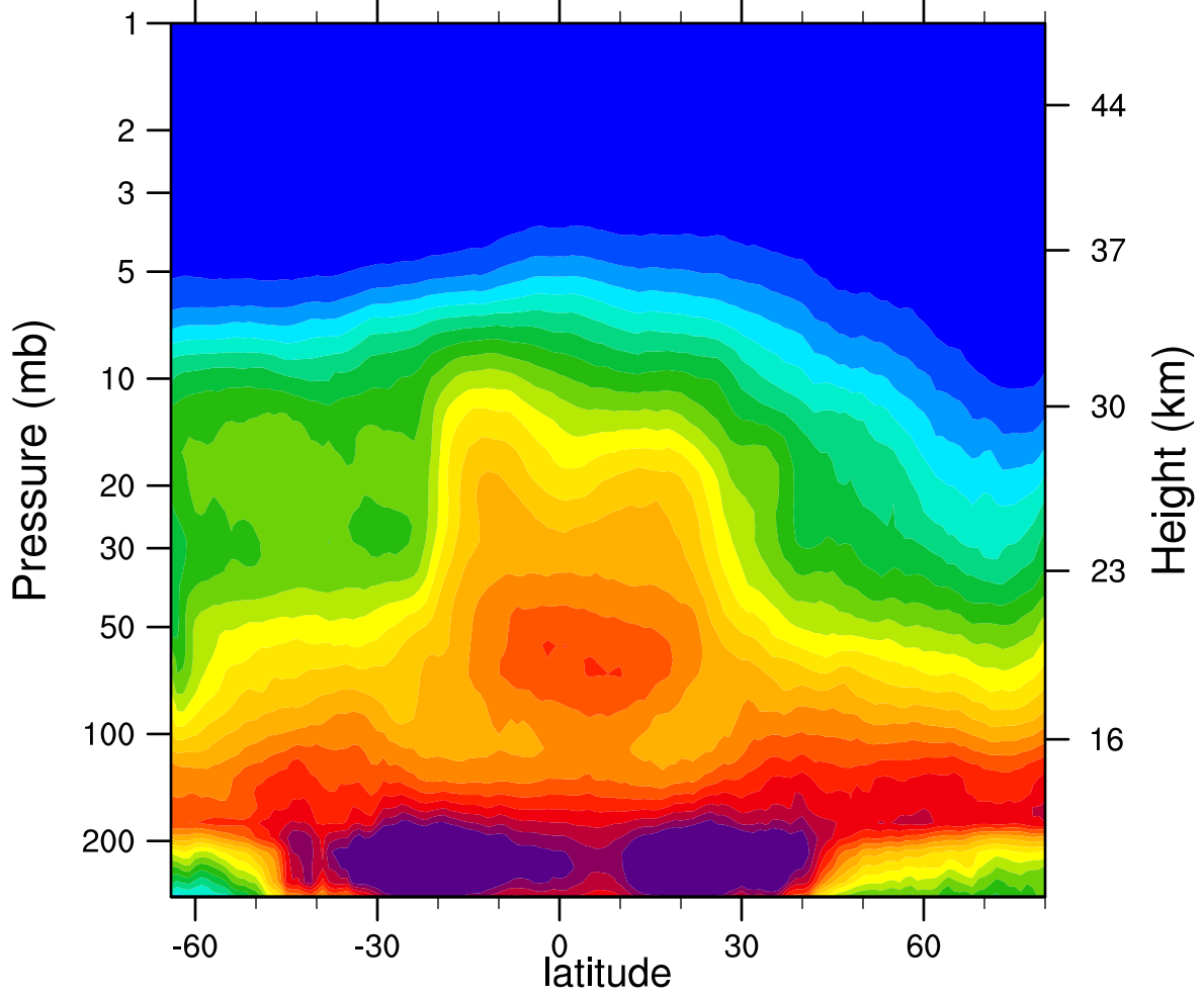
2007d319 N2O_Combined (ppbv)
