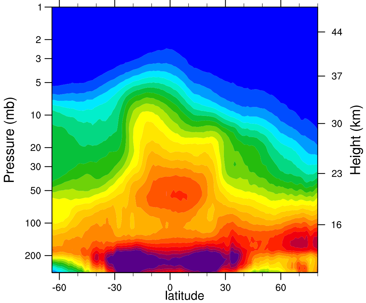
2005d355 N2O_Combined (ppbv)
