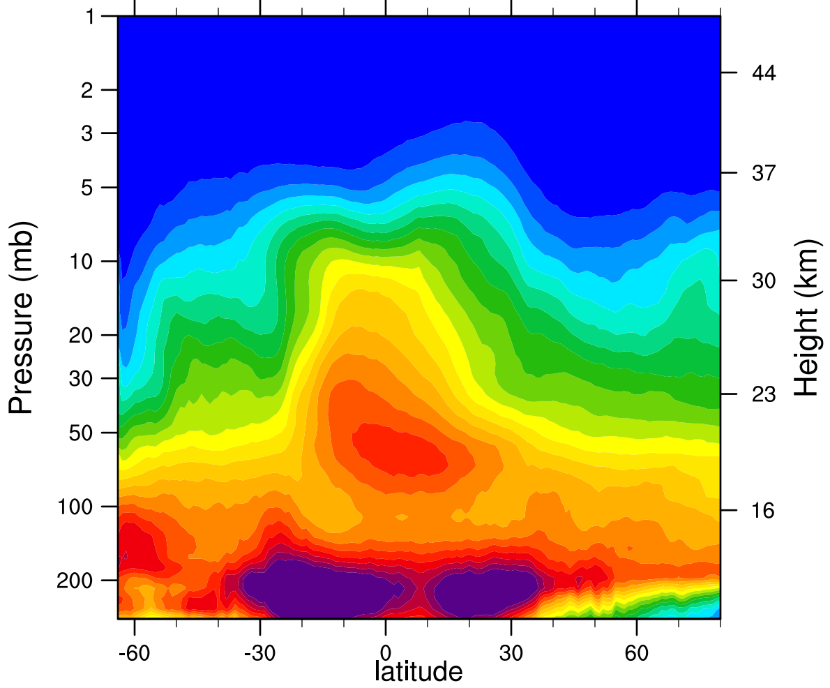
2005d164 N2O_Combined (ppbv)
