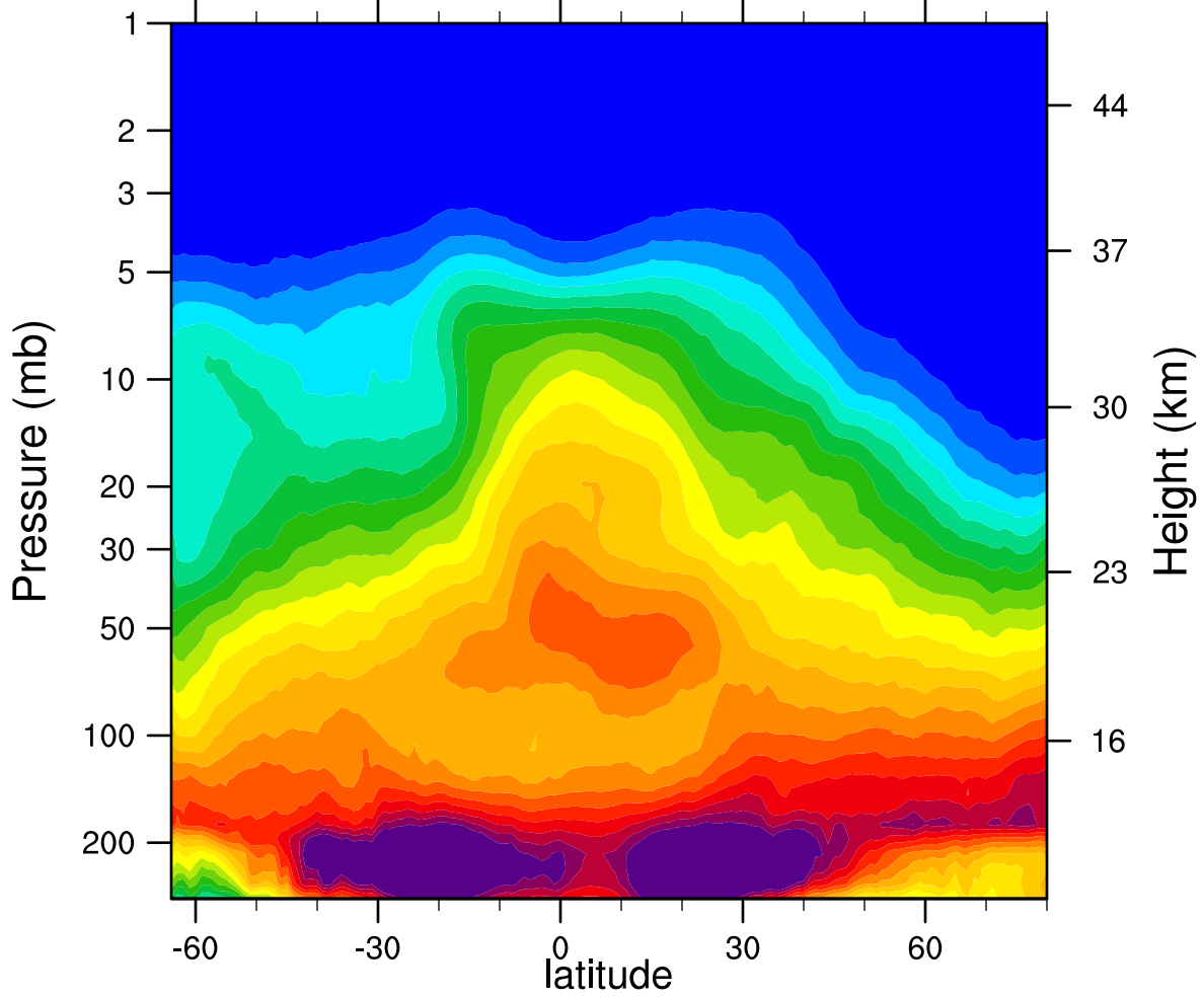
2006d322 N2O_Combined (ppbv)
