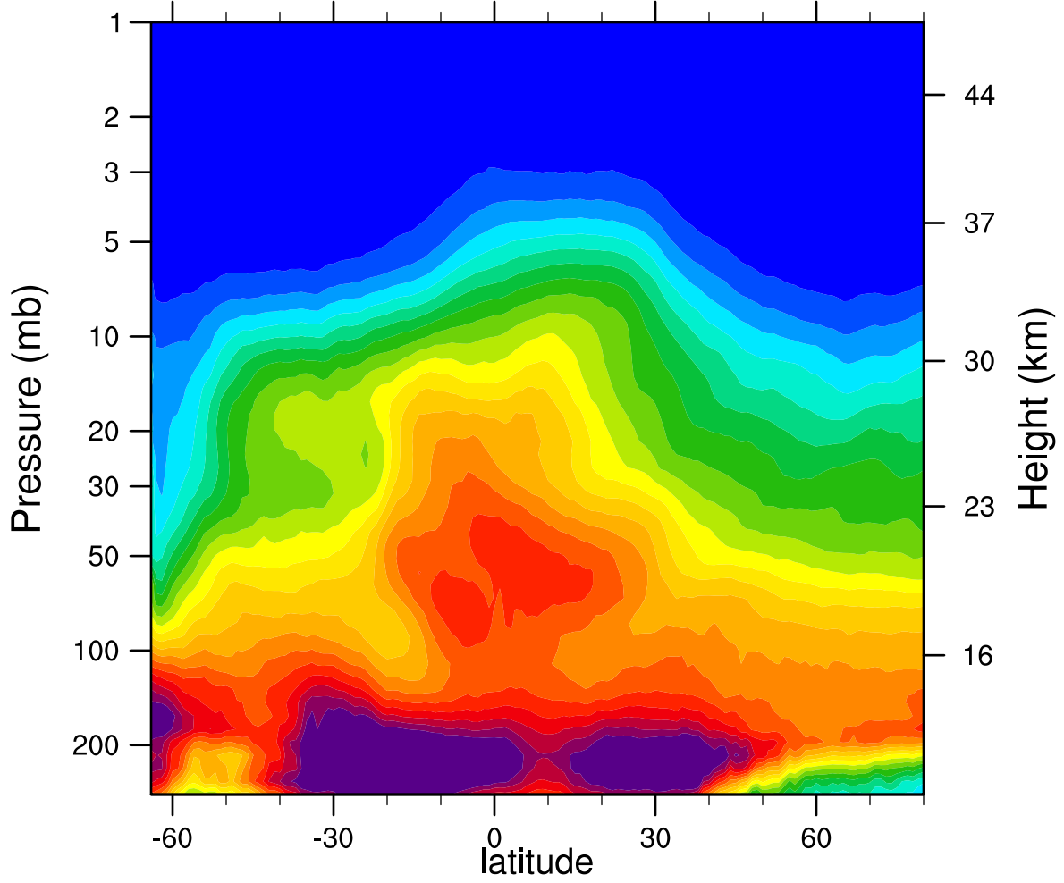
2007d238 N2O_Combined (ppbv)
