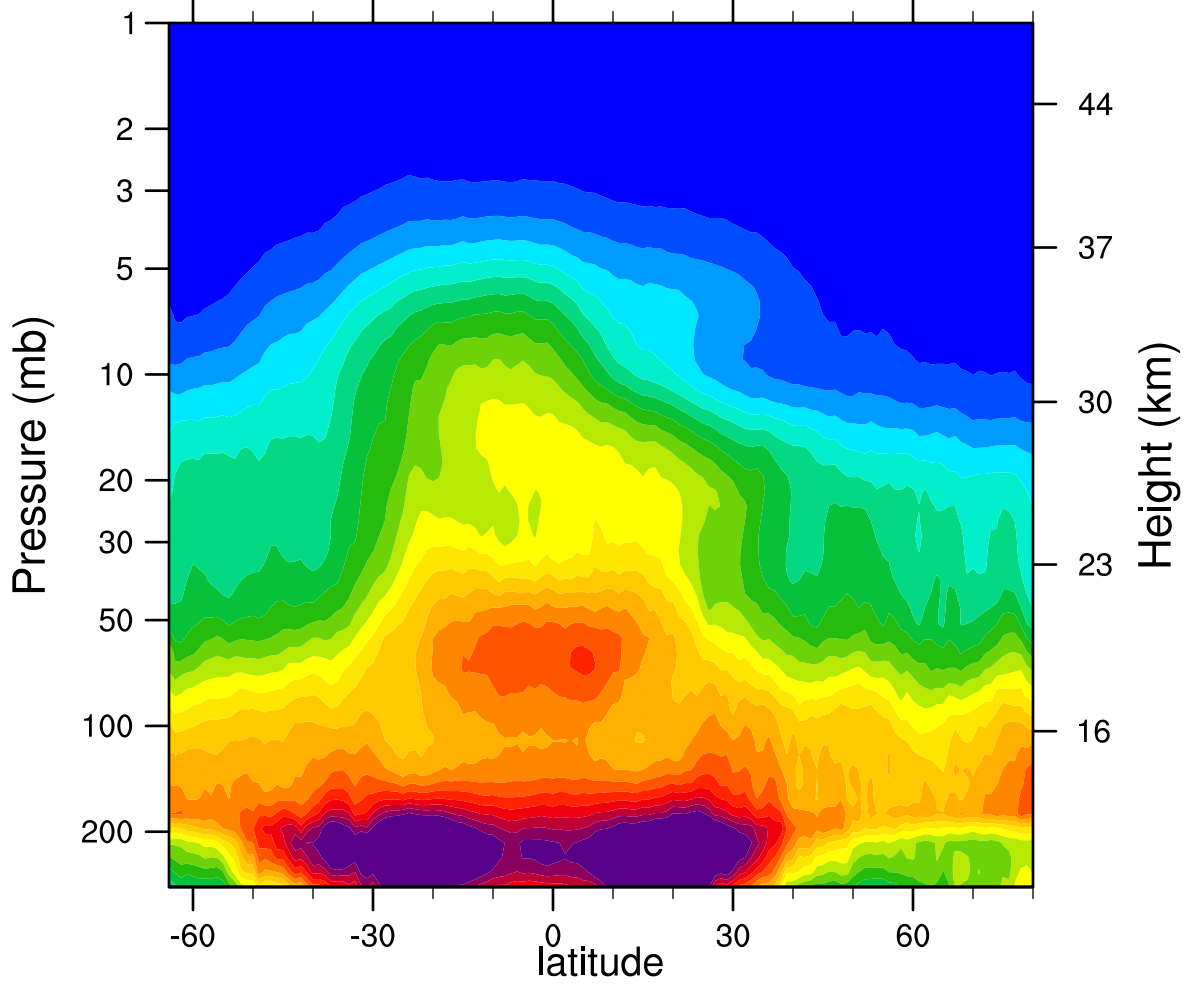
2006d088 N2O_Combined (ppbv)
