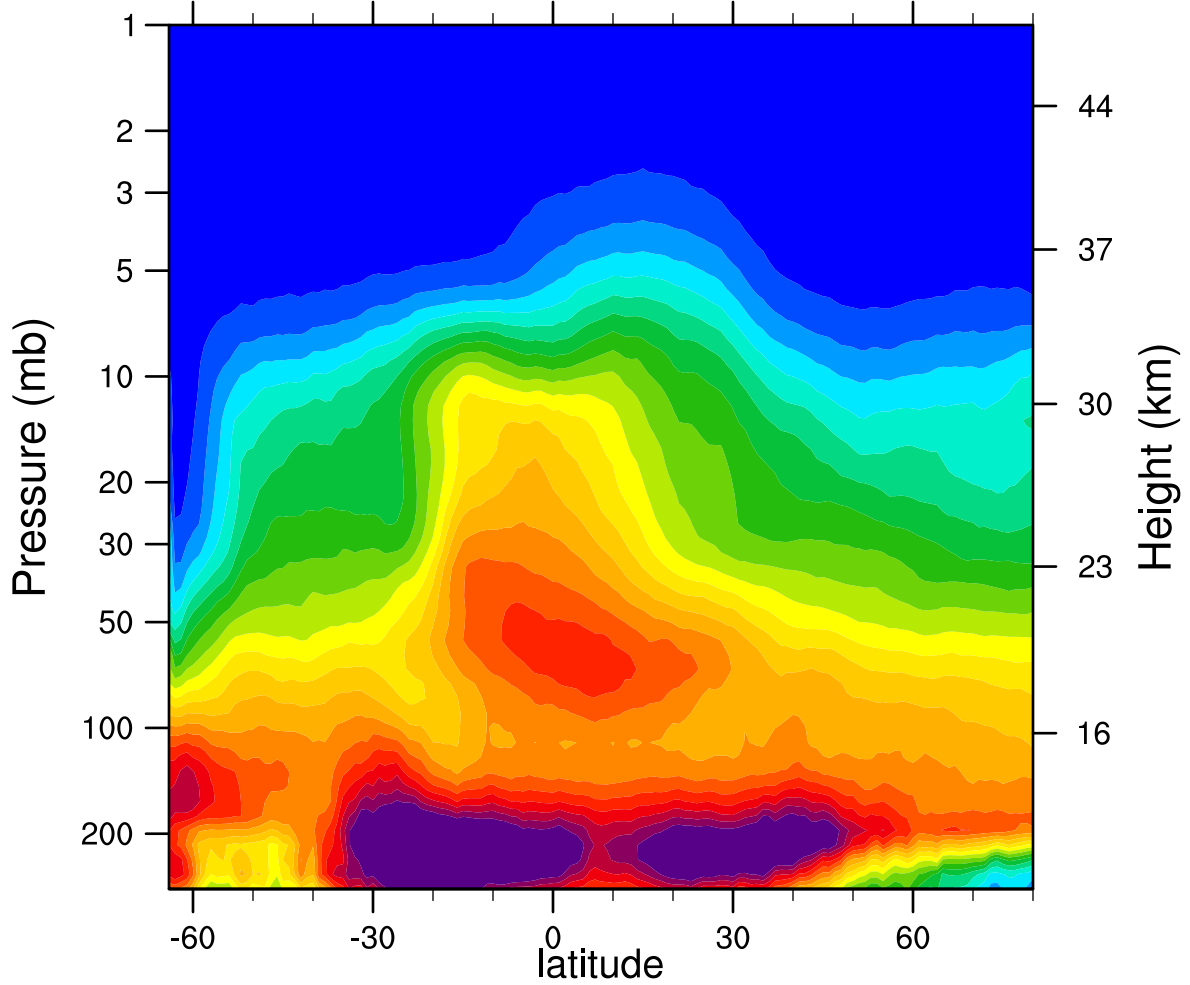
2005d197 N2O_Combined (ppbv)
