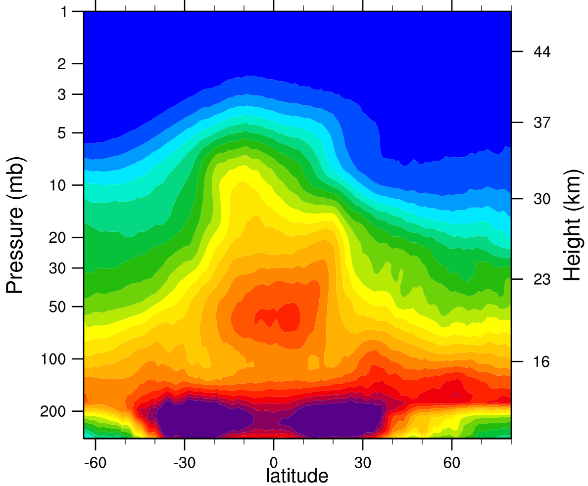
2006d036 N2O_Combined (ppbv)
