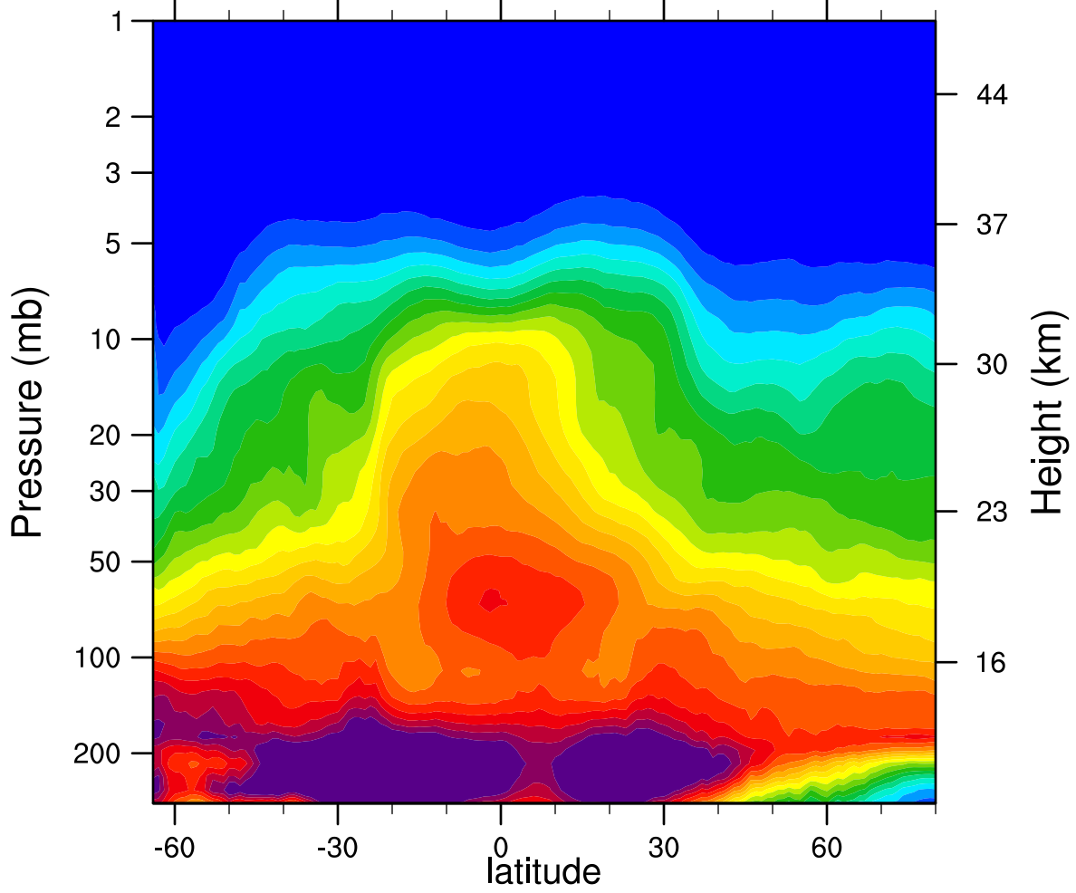
2007d146 N2O_Combined (ppbv)
