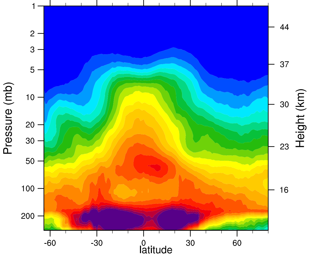
2005d118 N2O_Combined (ppbv)
