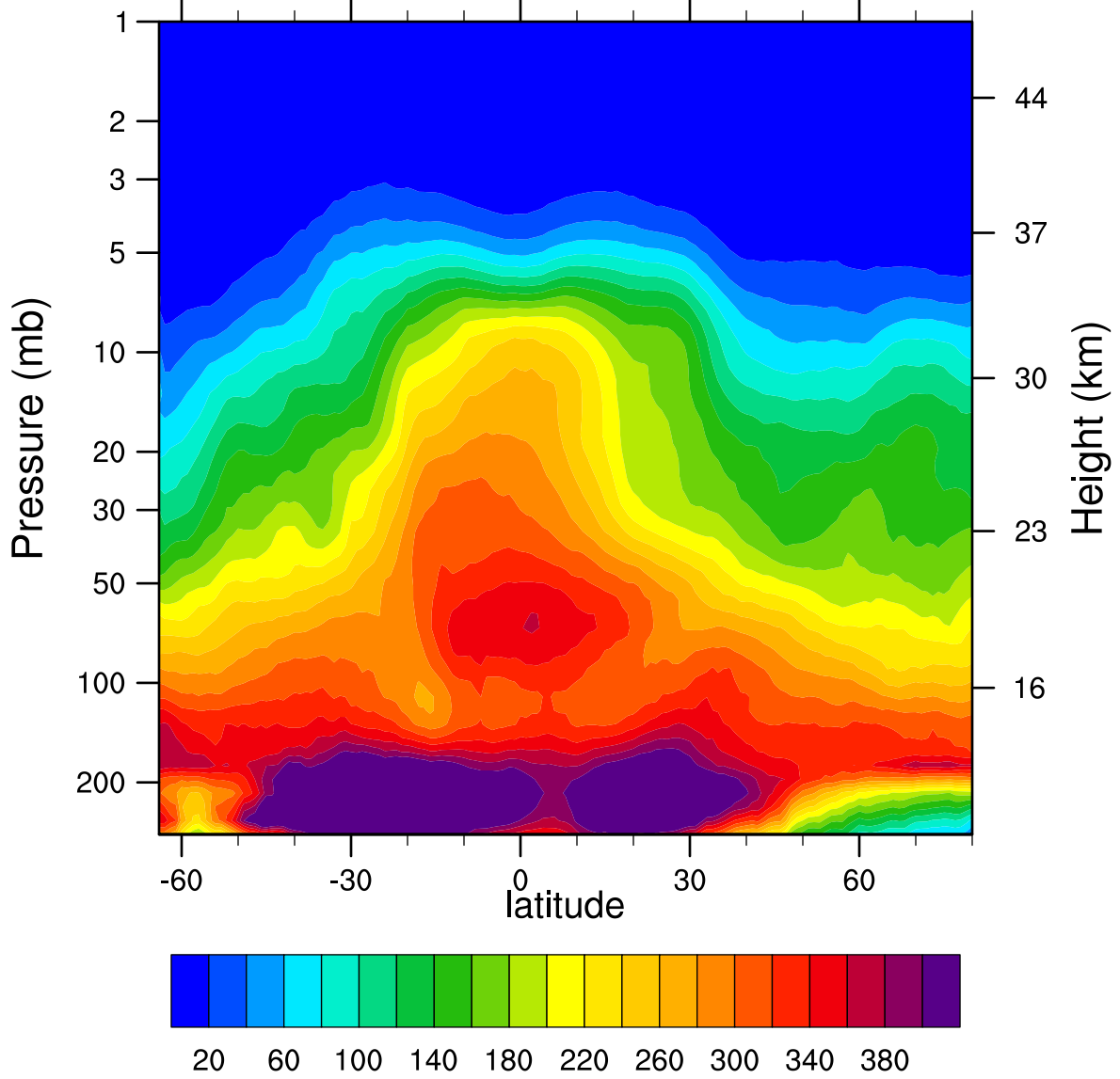
2007d128 N2O_Combined (ppbv)
