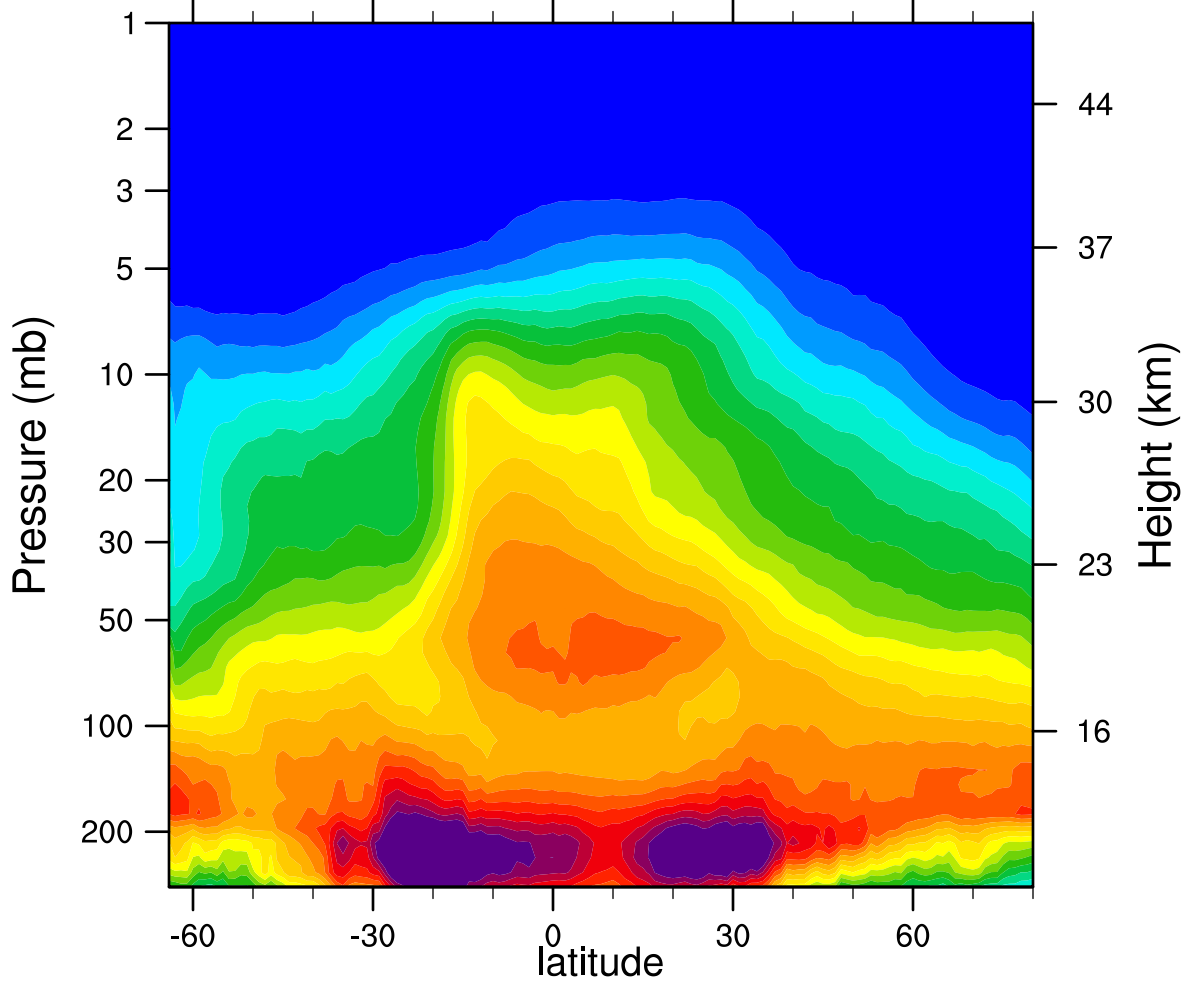
2005d282 N2O_Combined (ppbv)
