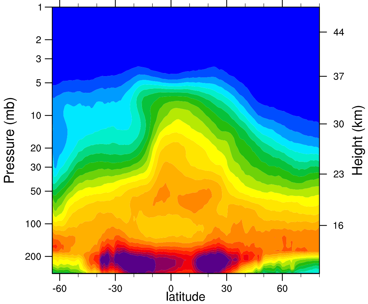
2006d297 N2O_Combined (ppbv)
