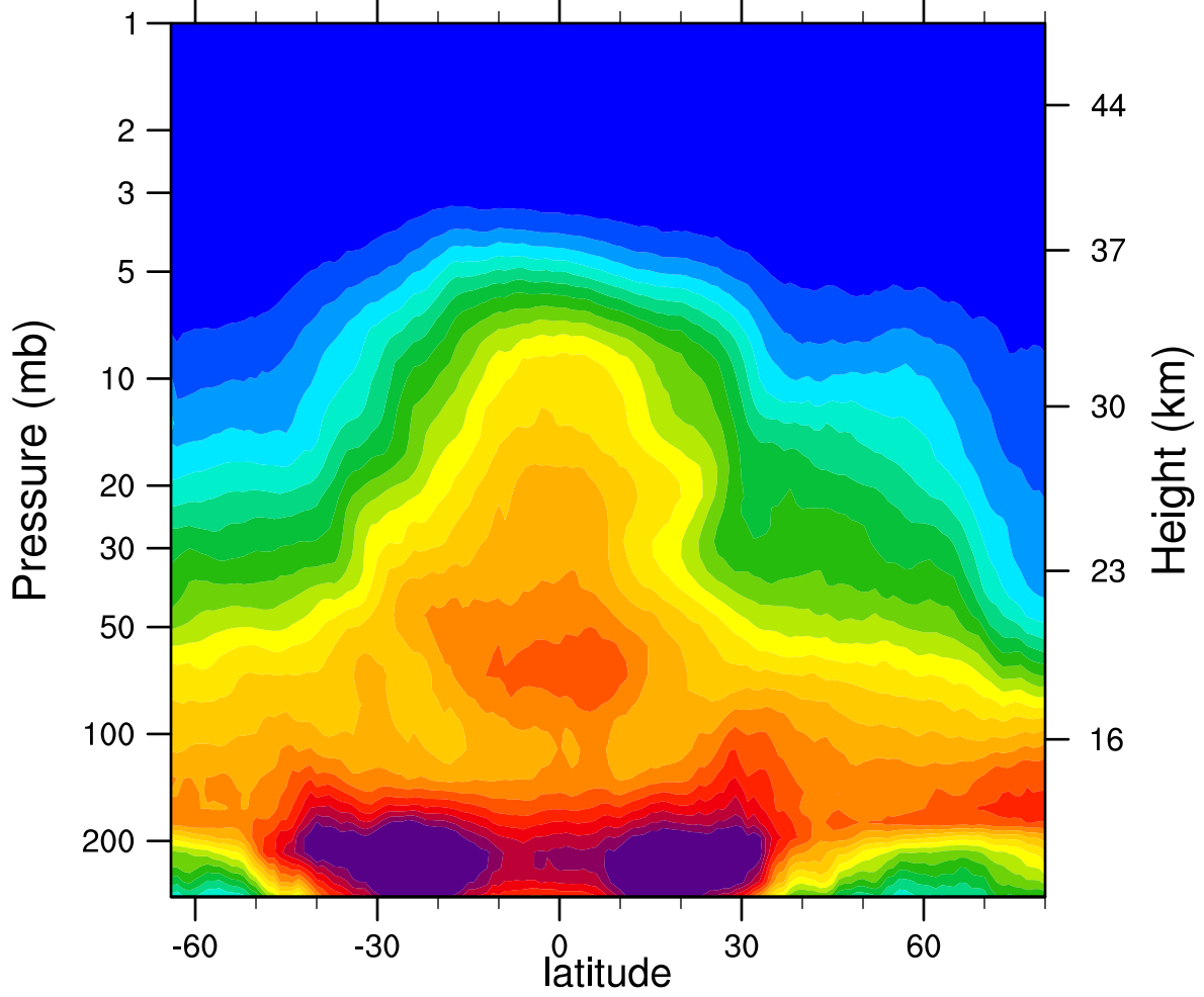
2007d071 N2O_Combined (ppbv)
