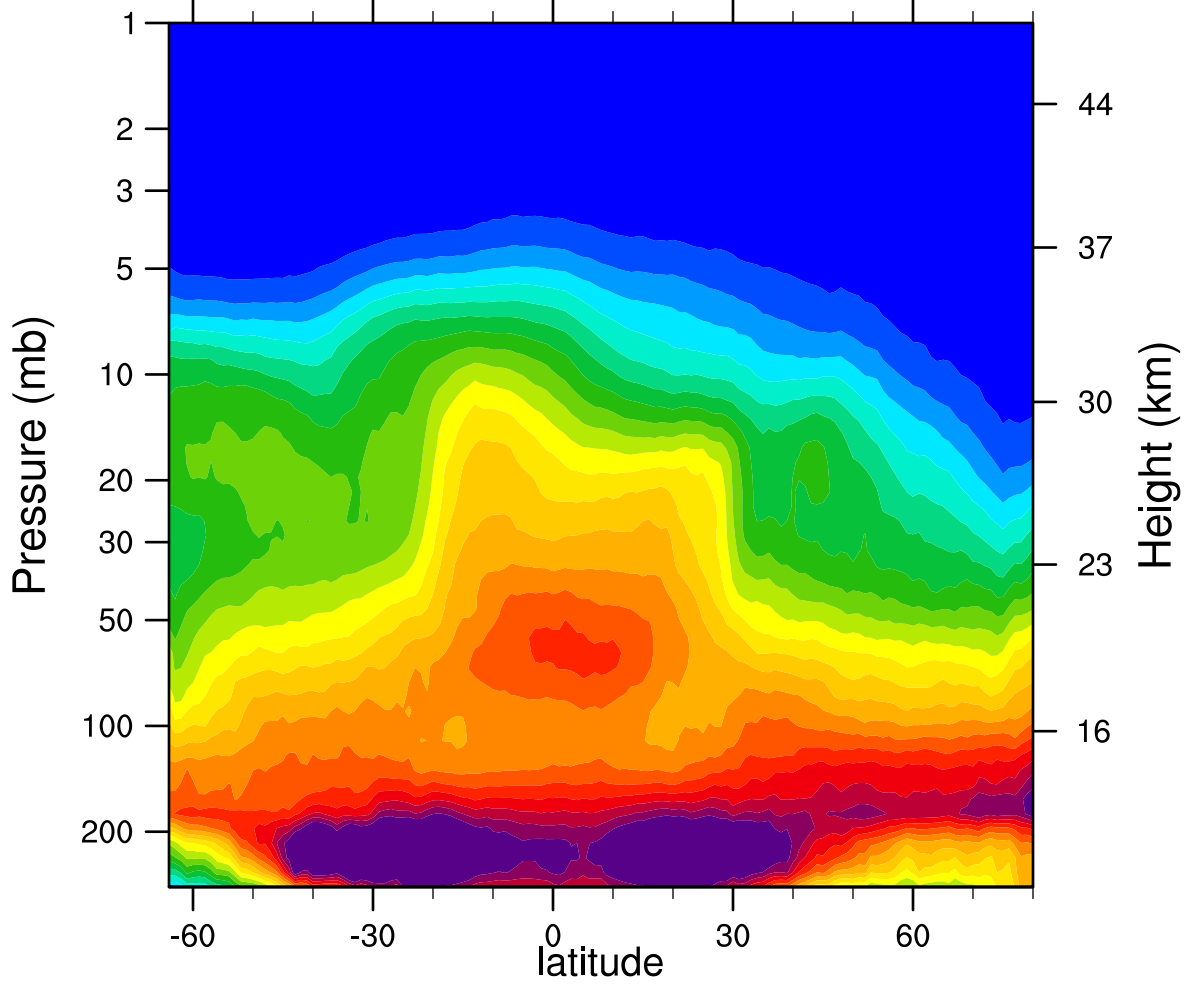
2007d341 N2O_Combined (ppbv)
