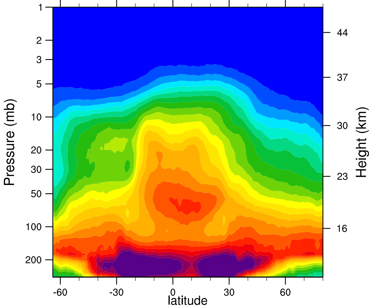
2007d287 N2O_Combined (ppbv)
