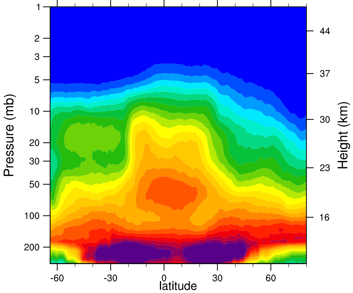
2007d308 N2O_Combined (ppbv)
