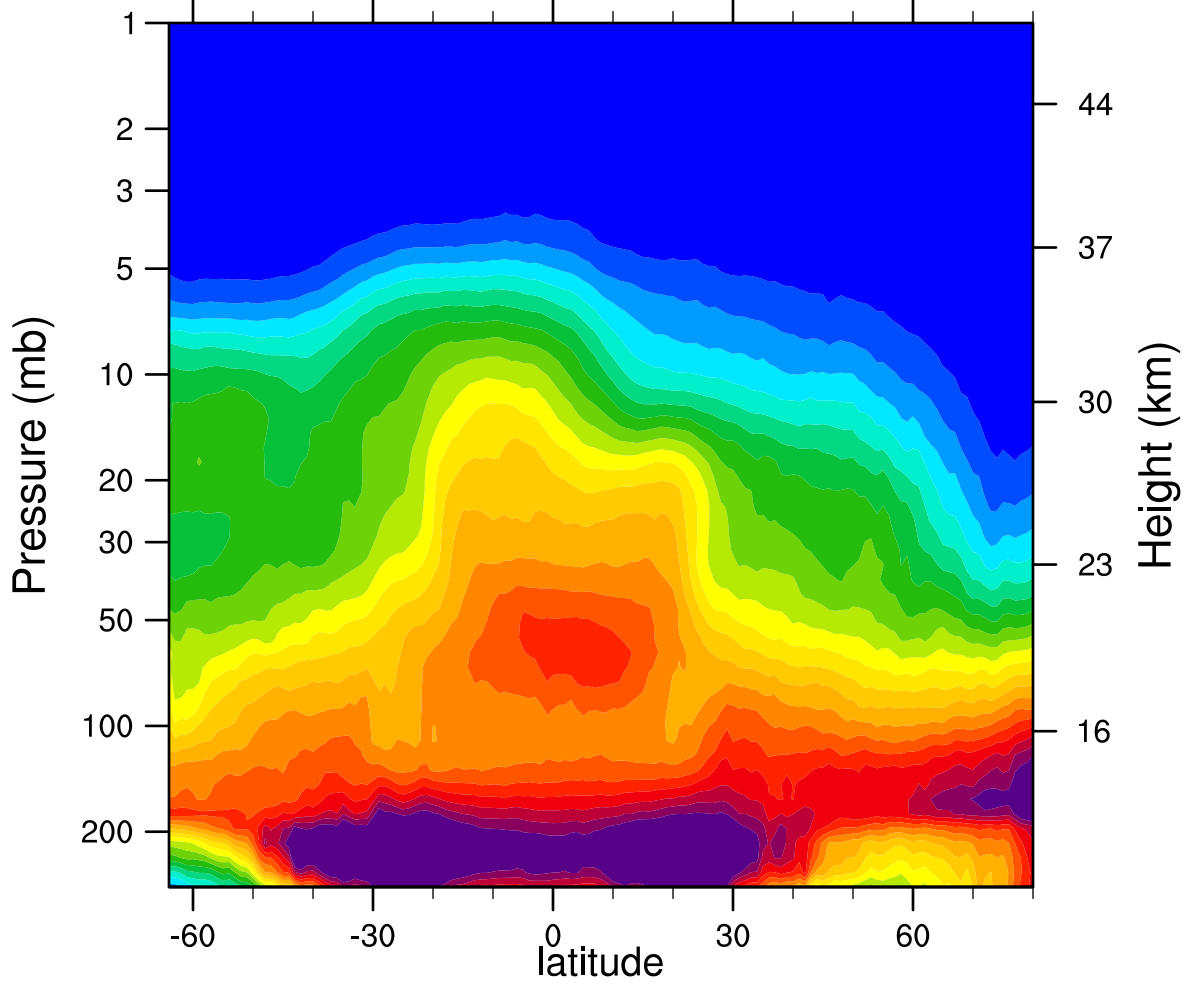
2007d359 N2O_Combined (ppbv)
