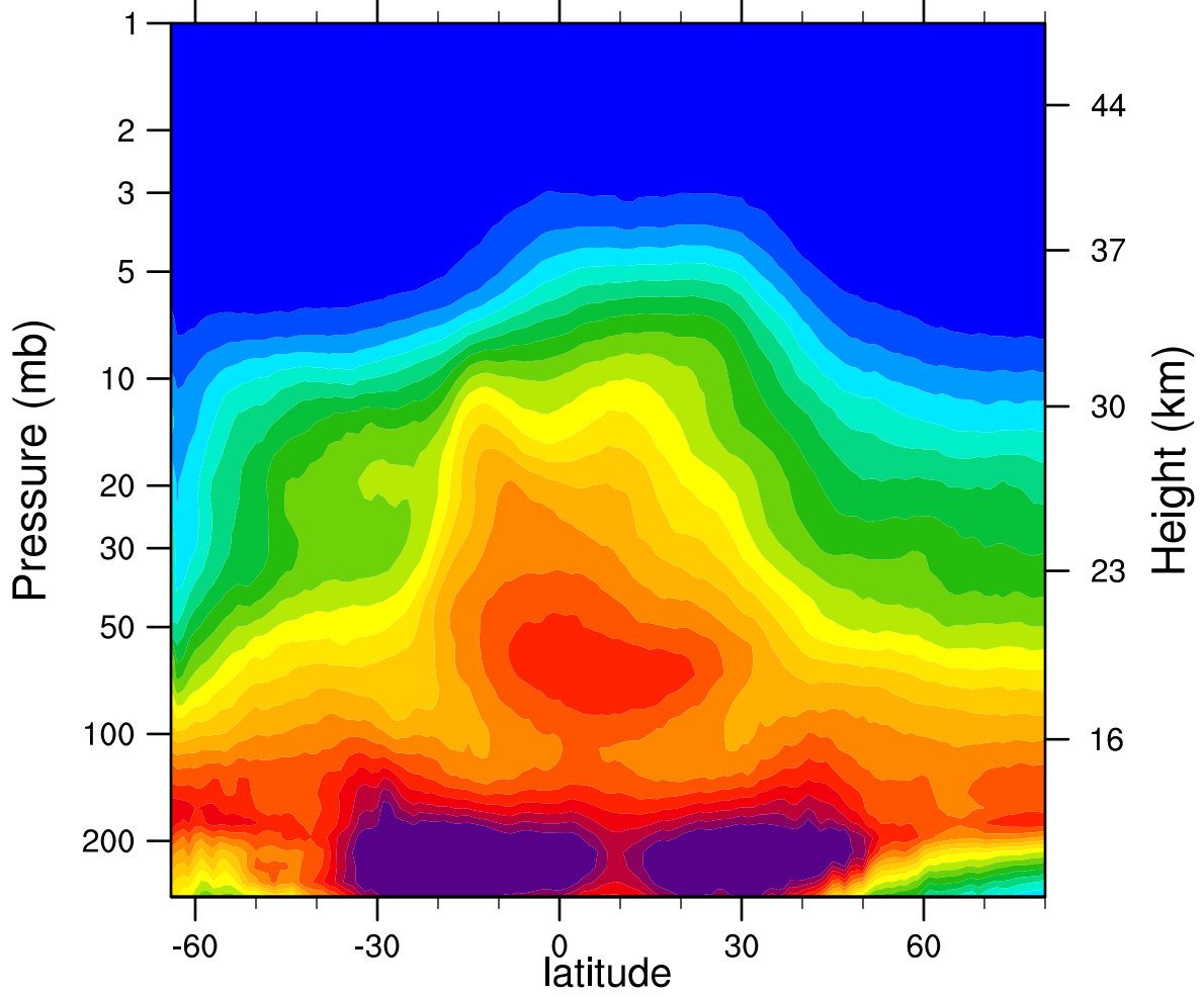
2007d257 N2O_Combined (ppbv)
