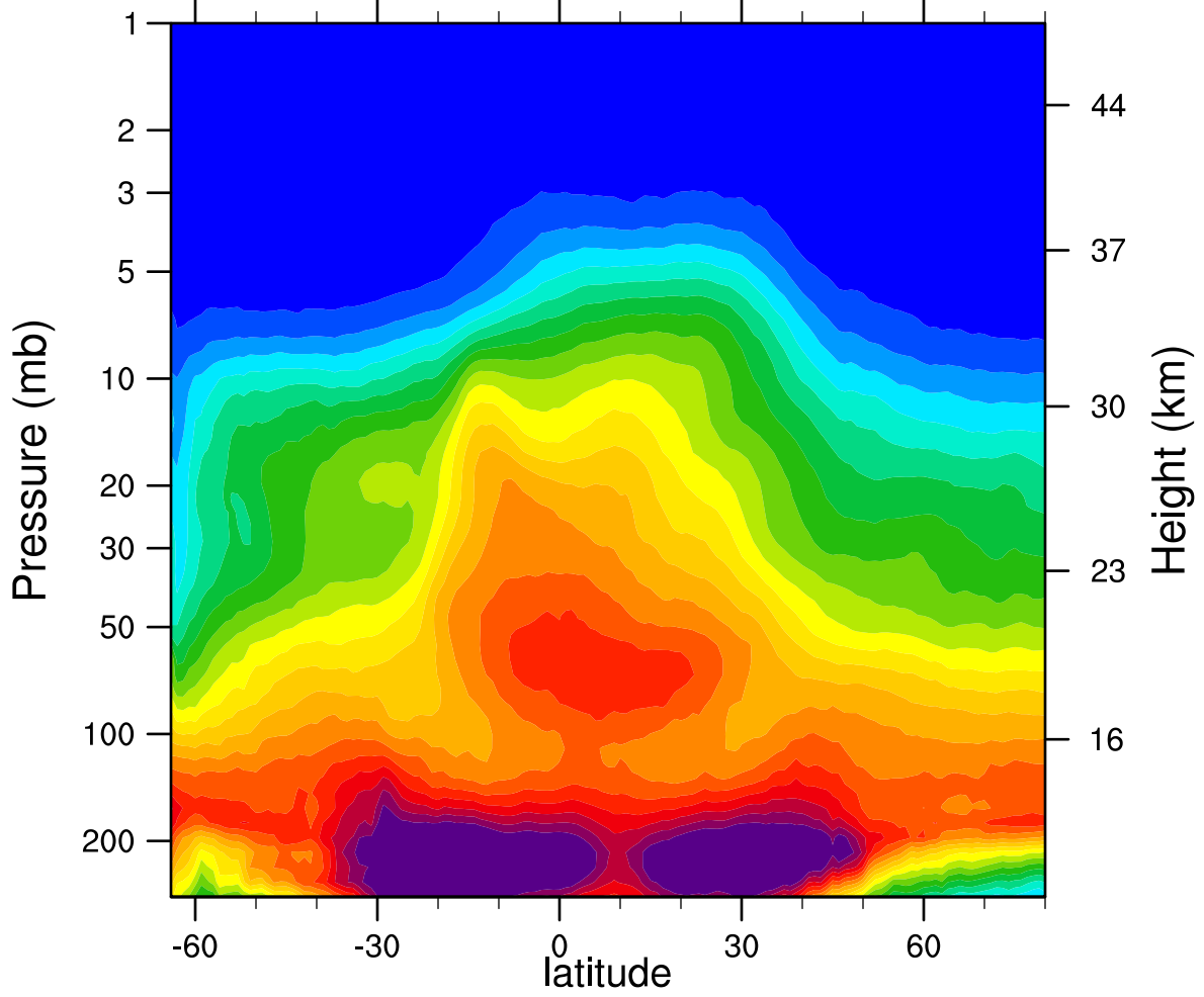
2007d259 N2O_Combined (ppbv)
