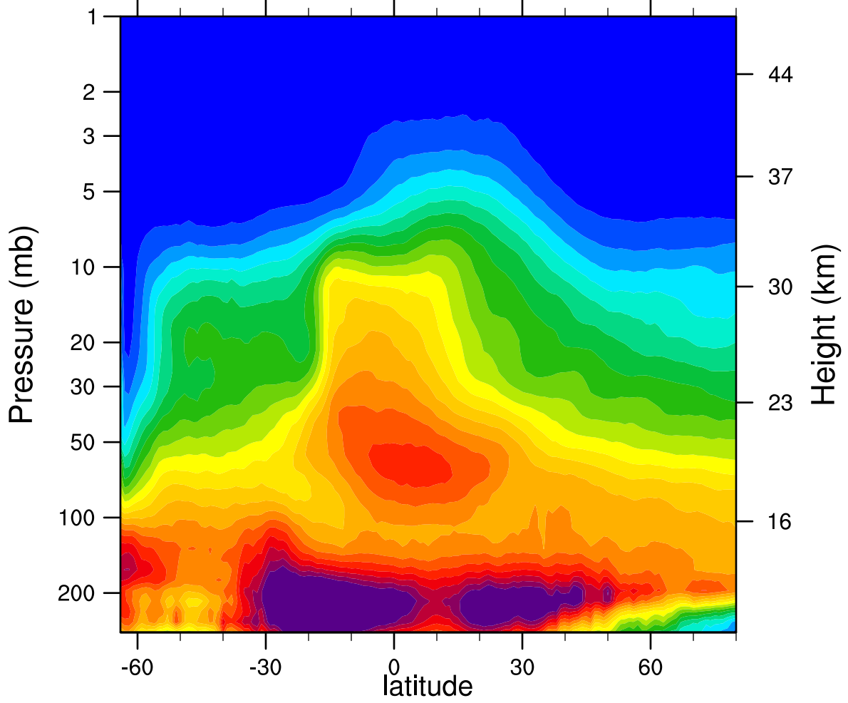
2005d220 N2O_Combined (ppbv)
