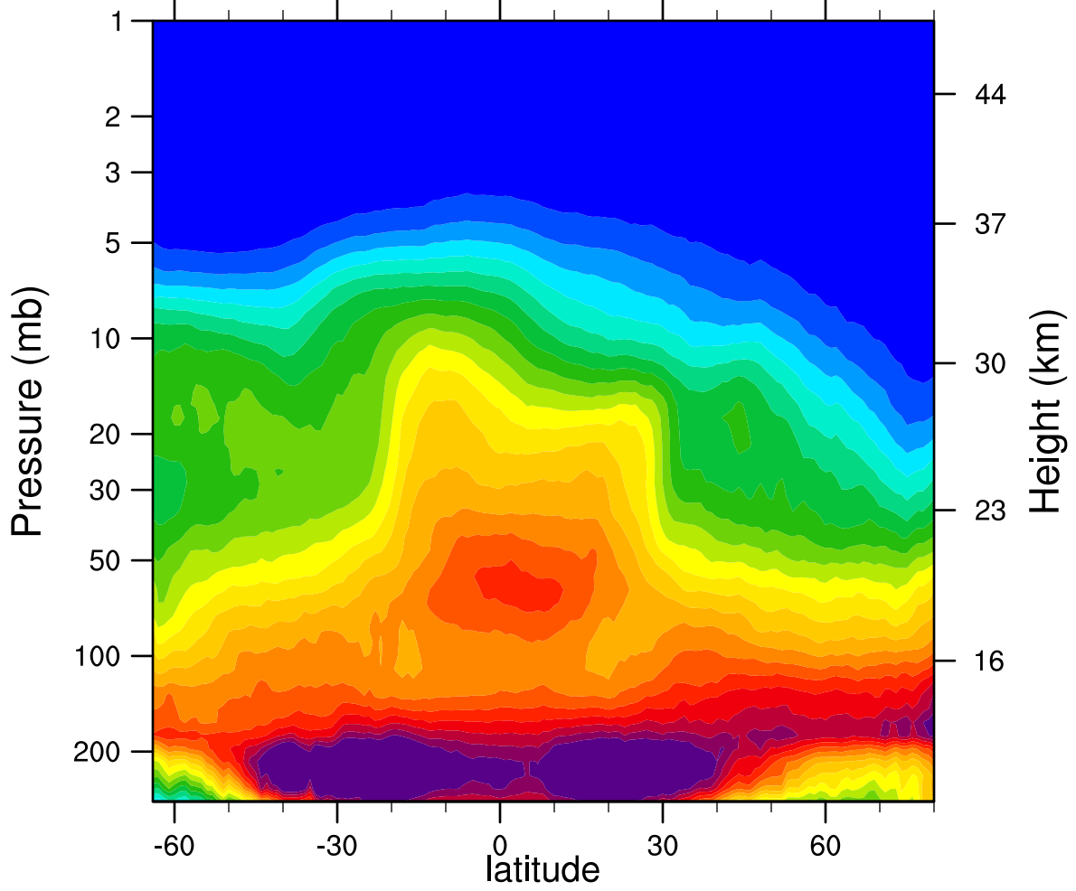
2007d342 N2O_Combined (ppbv)
