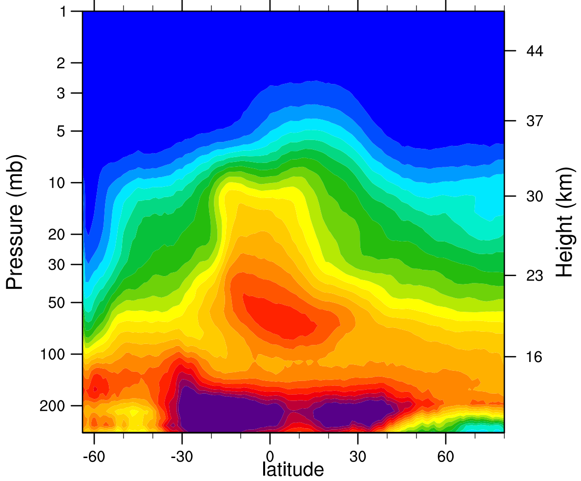
2005d210 N2O_Combined (ppbv)
