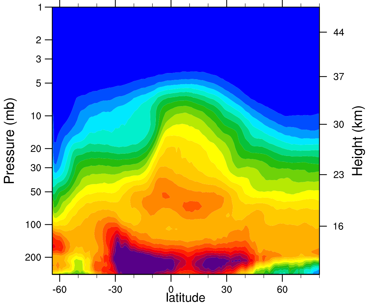
2006d238 N2O_Combined (ppbv)
