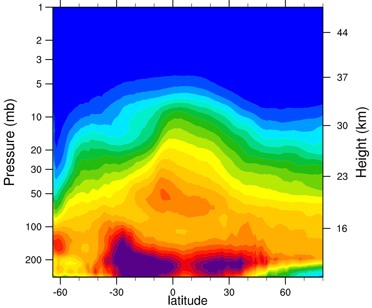
2006d199 N2O_Combined (ppbv)
