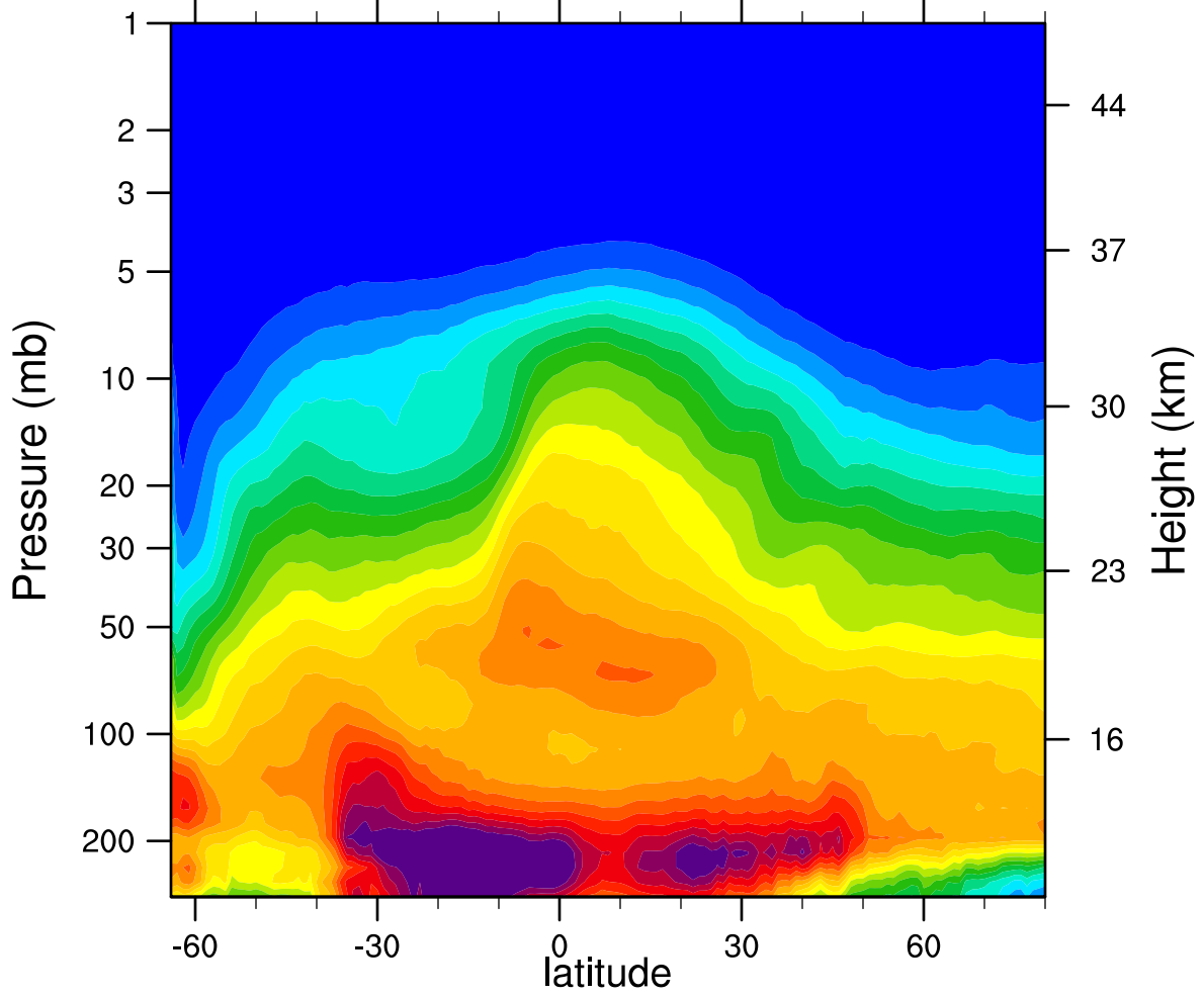
2006d225 N2O_Combined (ppbv)
