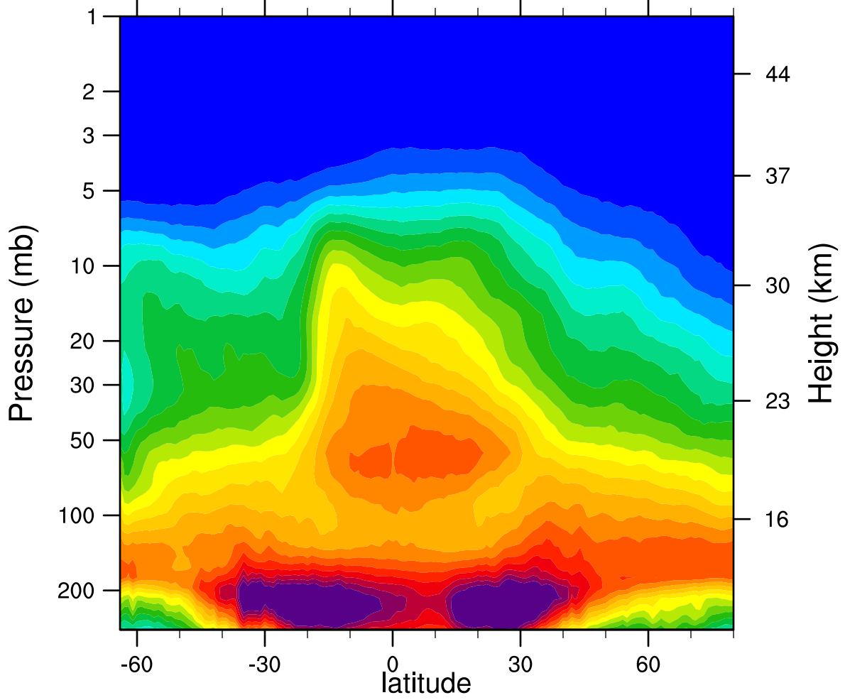
2005d299 N2O_Combined (ppbv)
