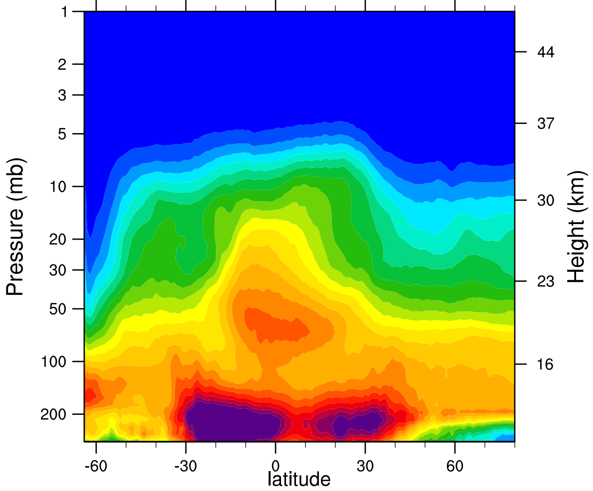
2007d195 N2O_Combined (ppbv)
