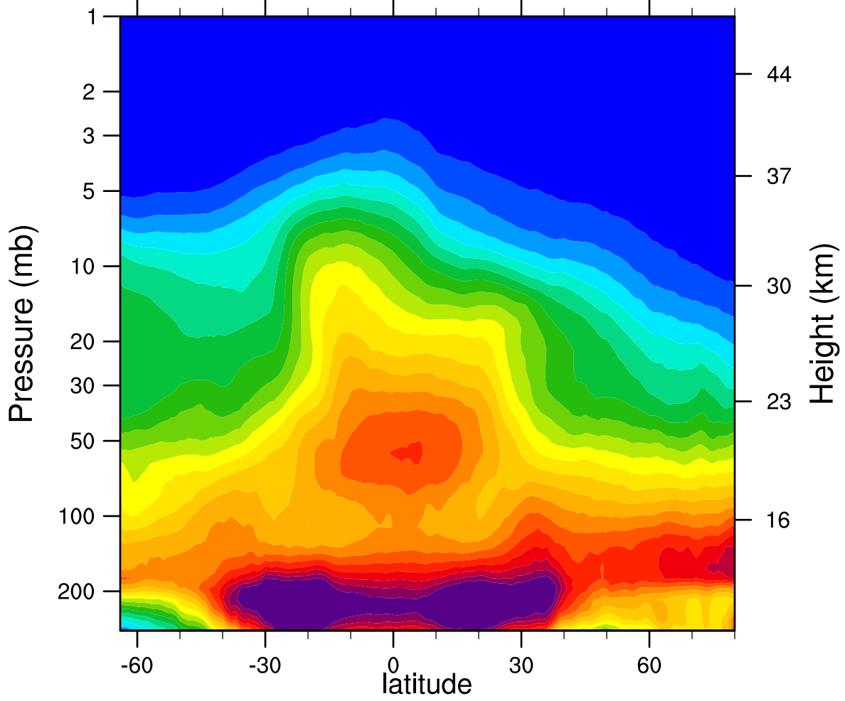
2005d350 N2O_Combined (ppbv)
