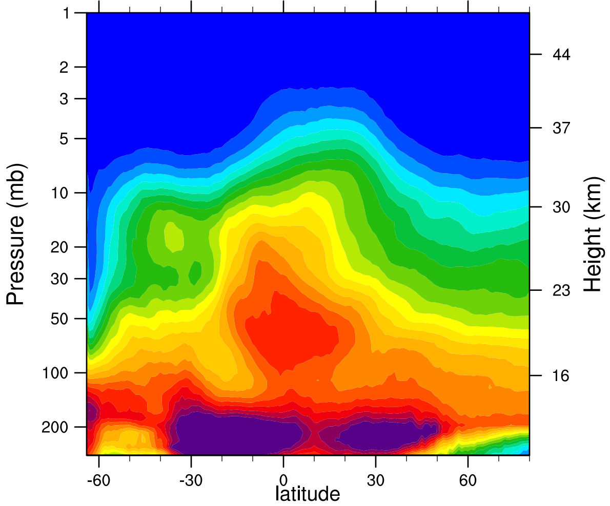
2007d219 N2O_Combined (ppbv)
