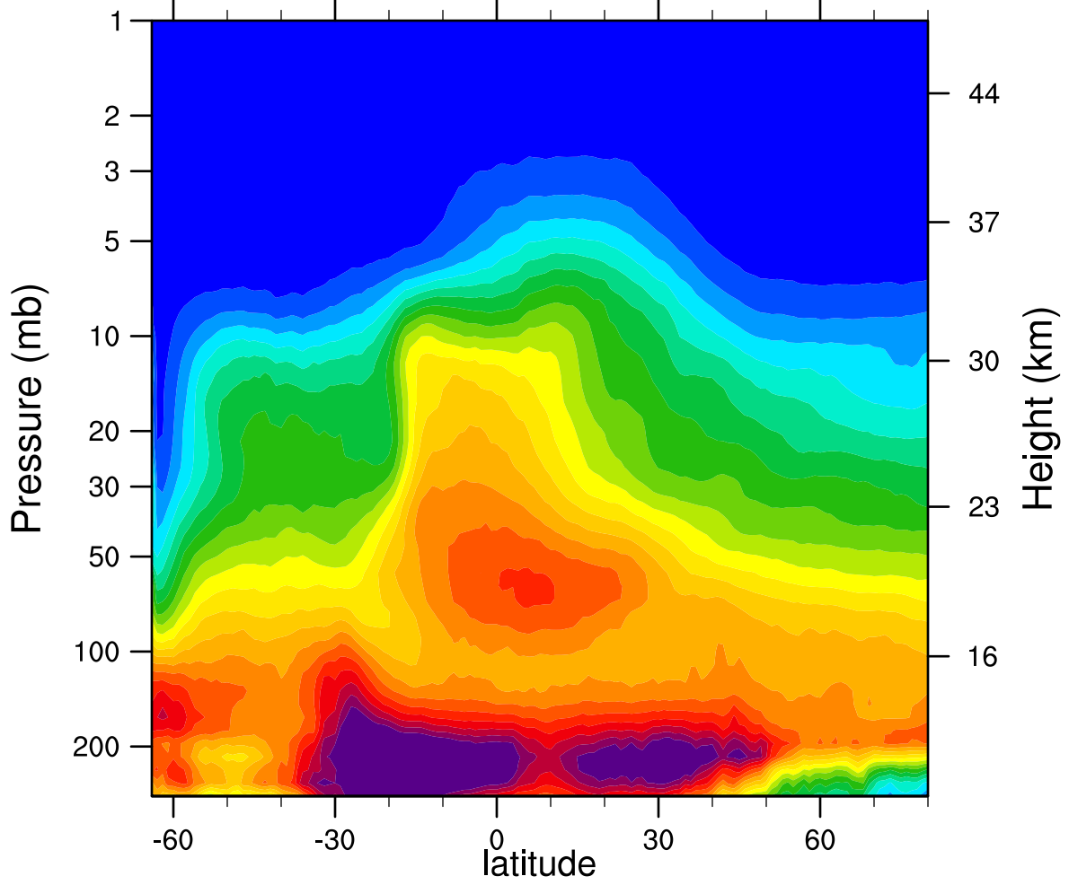
2005d228 N2O_Combined (ppbv)
