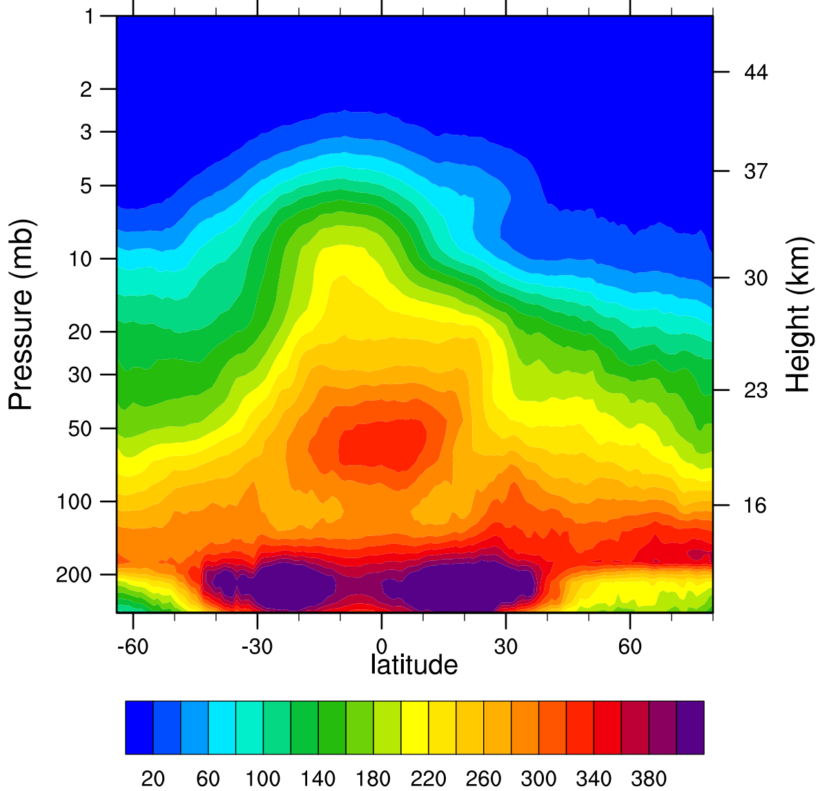
2006d061 N2O_Combined (ppbv)
