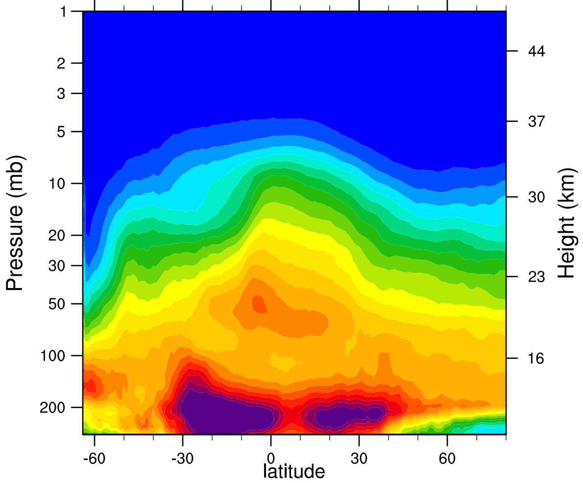
2006d195 N2O_Combined (ppbv)
