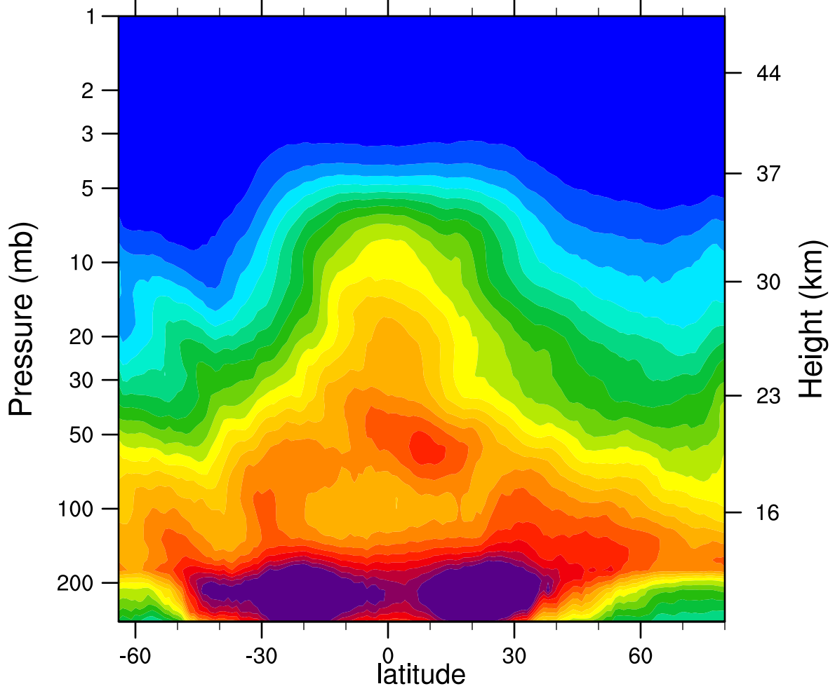
2005d095 N2O_Combined (ppbv)
