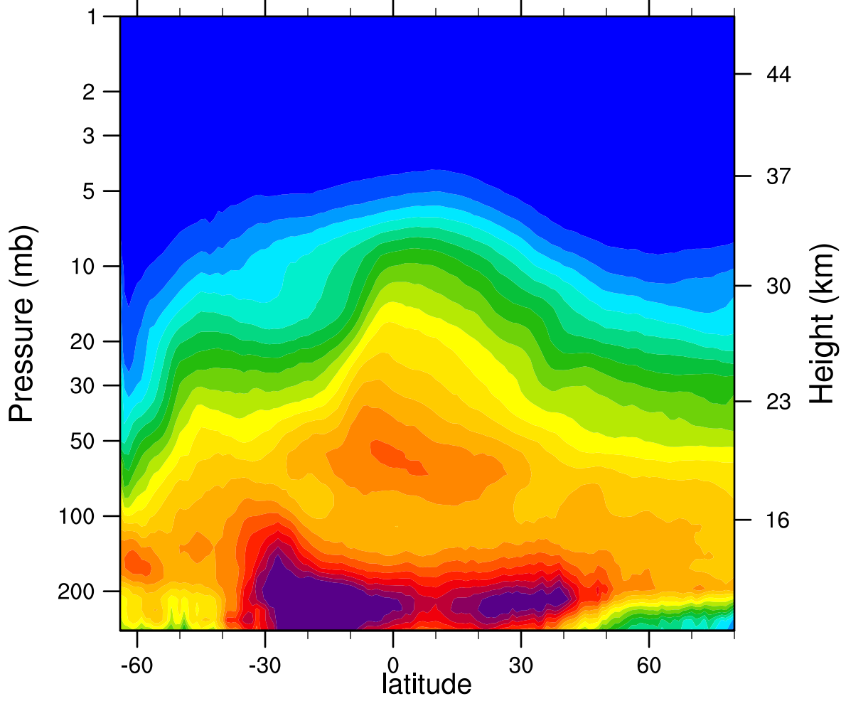
2006d214 N2O_Combined (ppbv)
