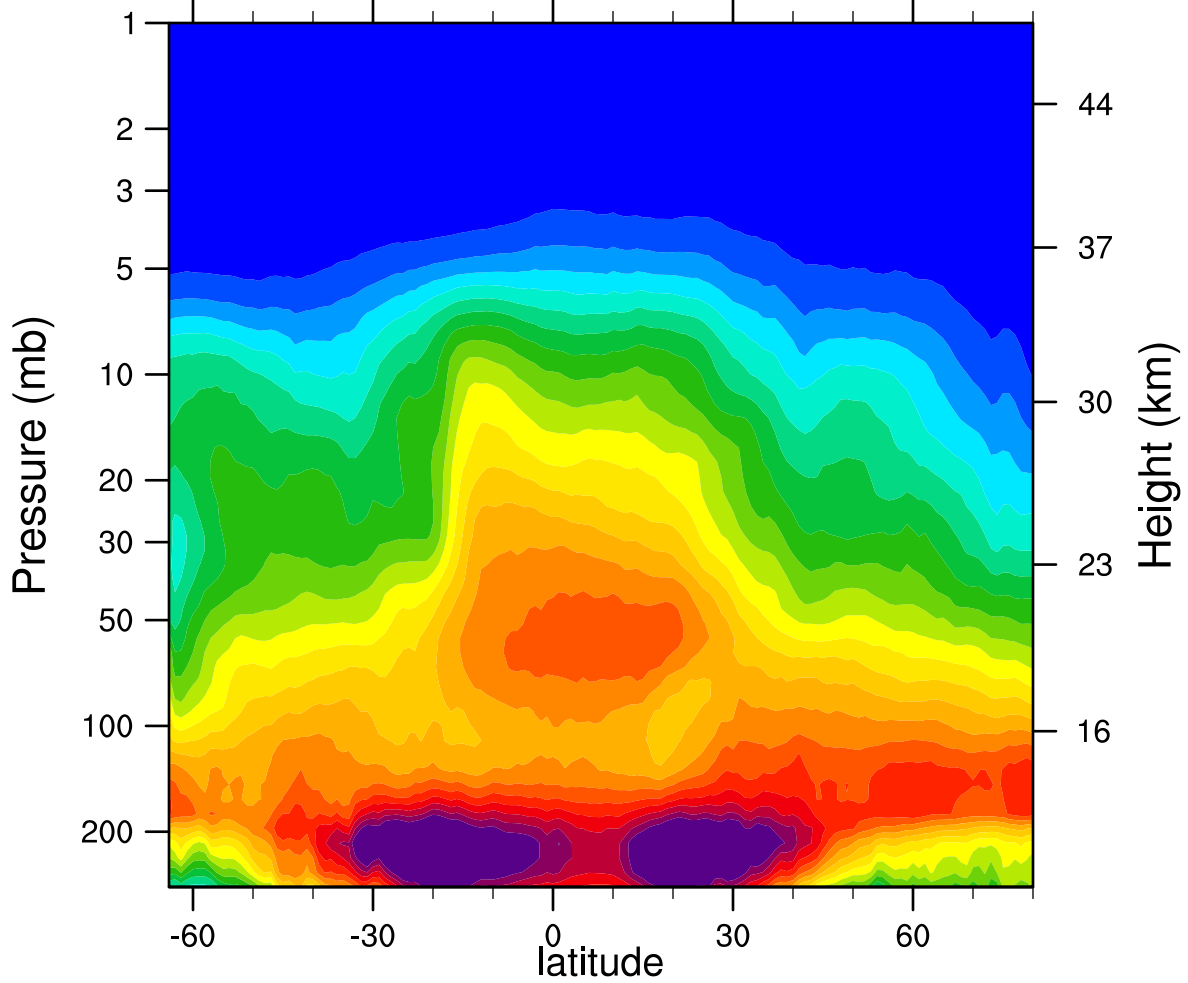
2005d309 N2O_Combined (ppbv)
