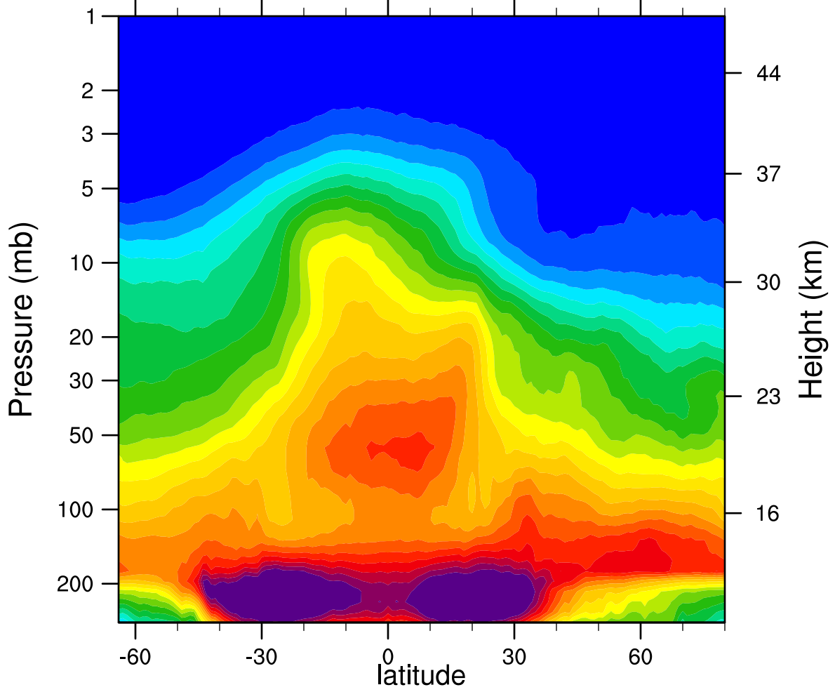
2006d033 N2O_Combined (ppbv)
