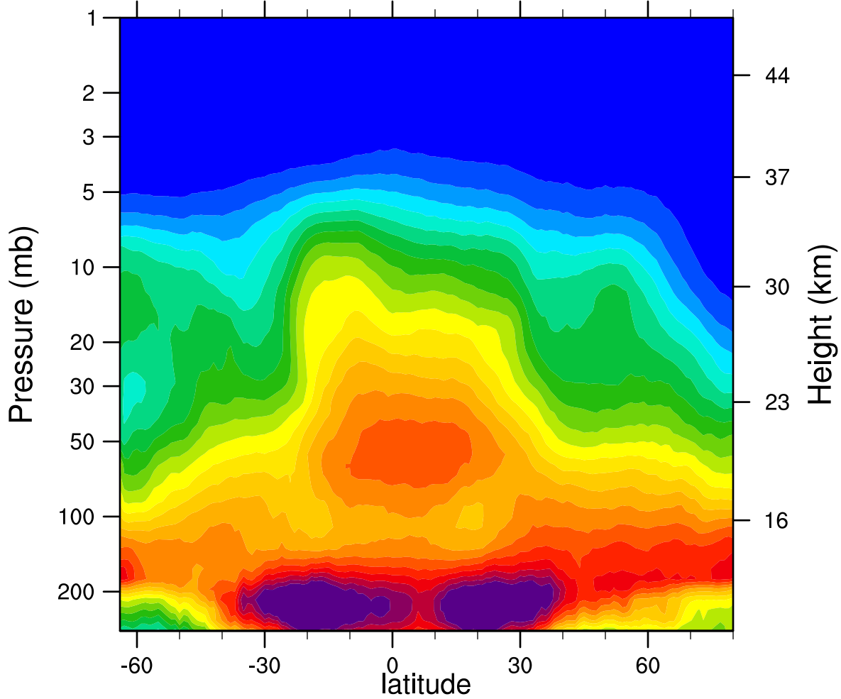
2005d320 N2O_Combined (ppbv)
