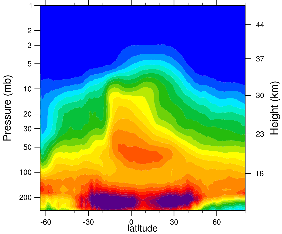
2005d250 N2O_Combined (ppbv)
