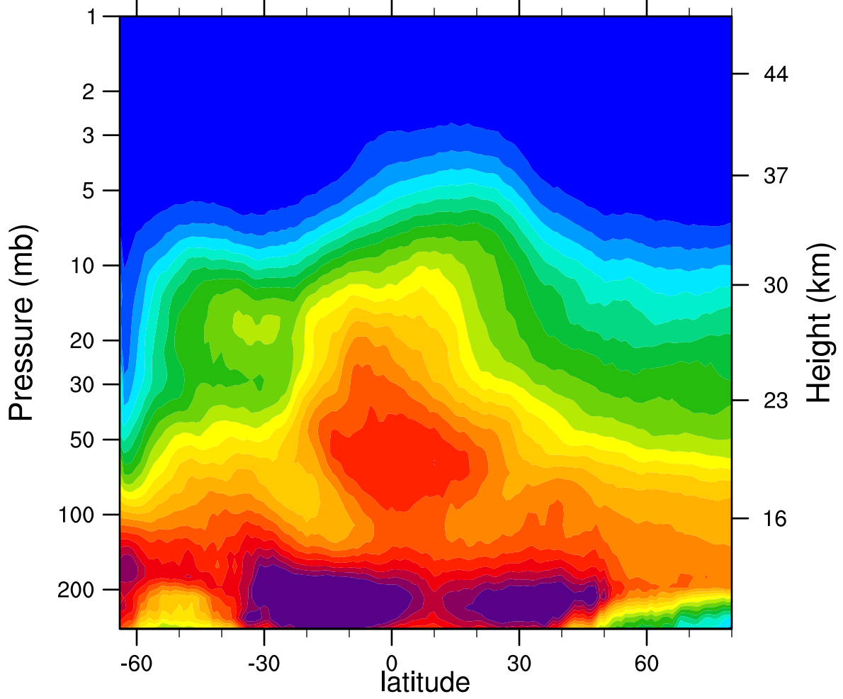
2007d215 N2O_Combined (ppbv)
