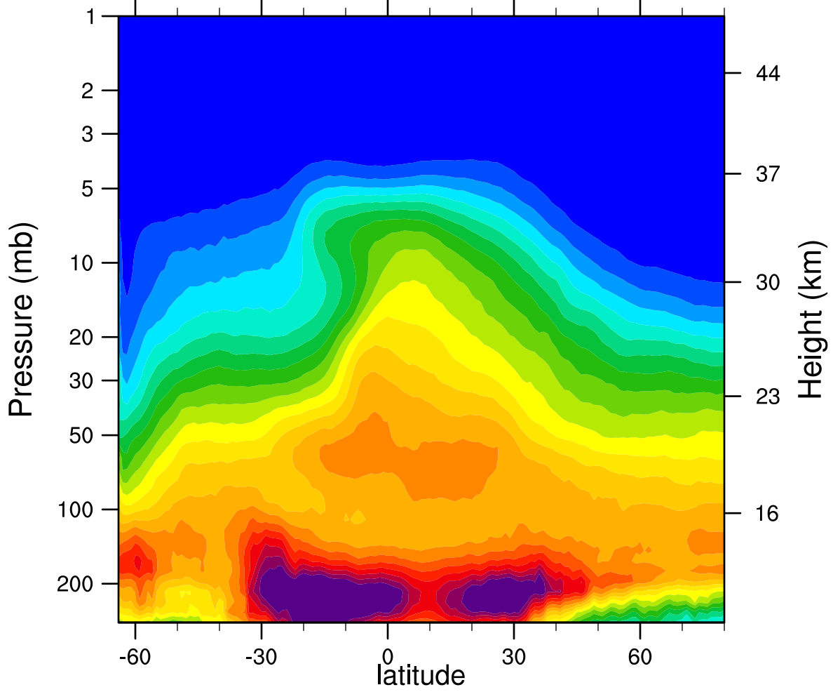
2006d266 N2O_Combined (ppbv)
