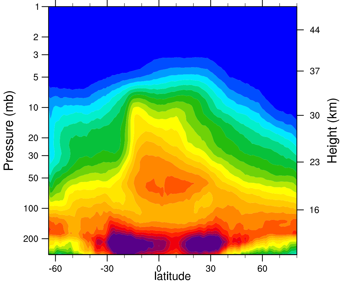
2005d283 N2O_Combined (ppbv)
