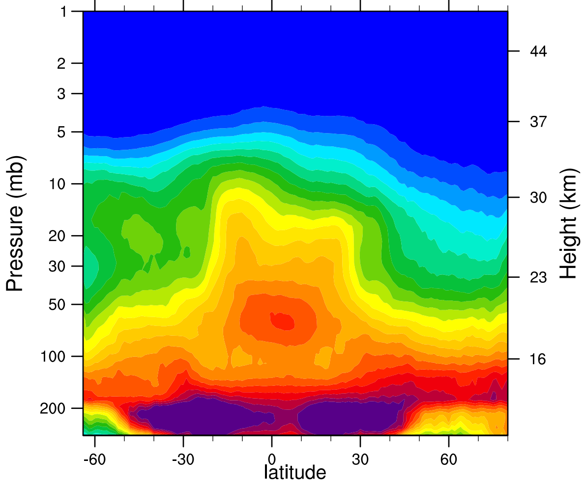
2007d333 N2O_Combined (ppbv)
