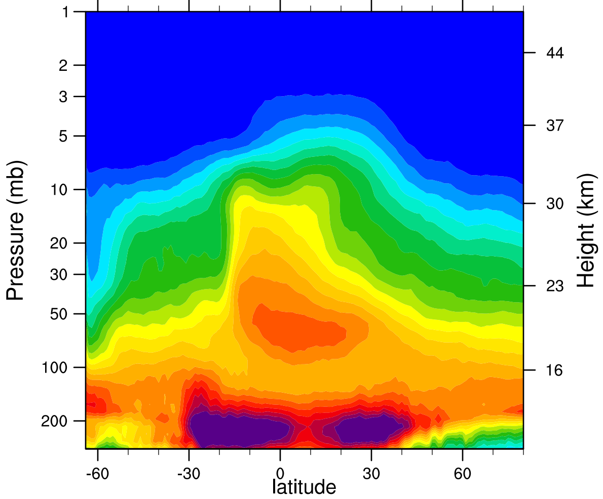
2005d253 N2O_Combined (ppbv)
