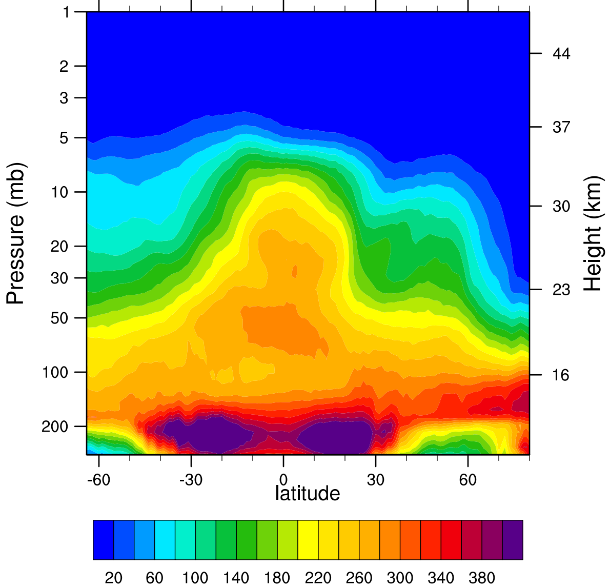
2007d015 N2O_Combined (ppbv)
