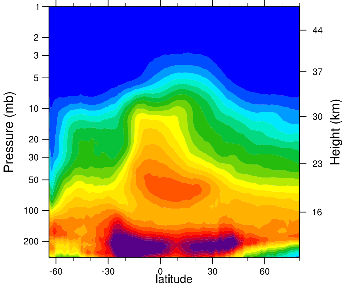
2005d237 N2O_Combined (ppbv)
