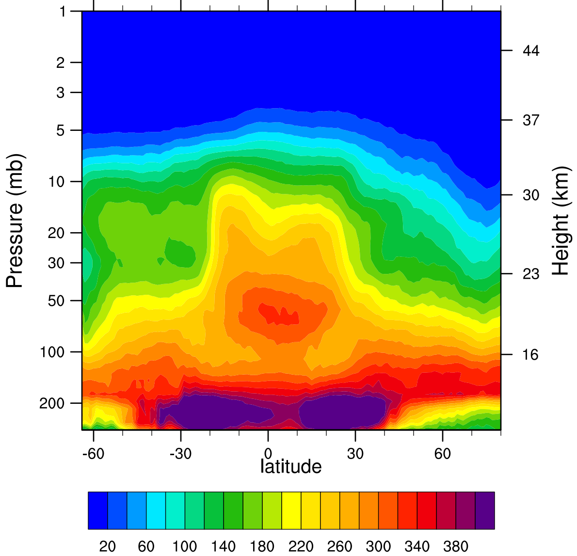
2007d315 N2O_Combined (ppbv)
