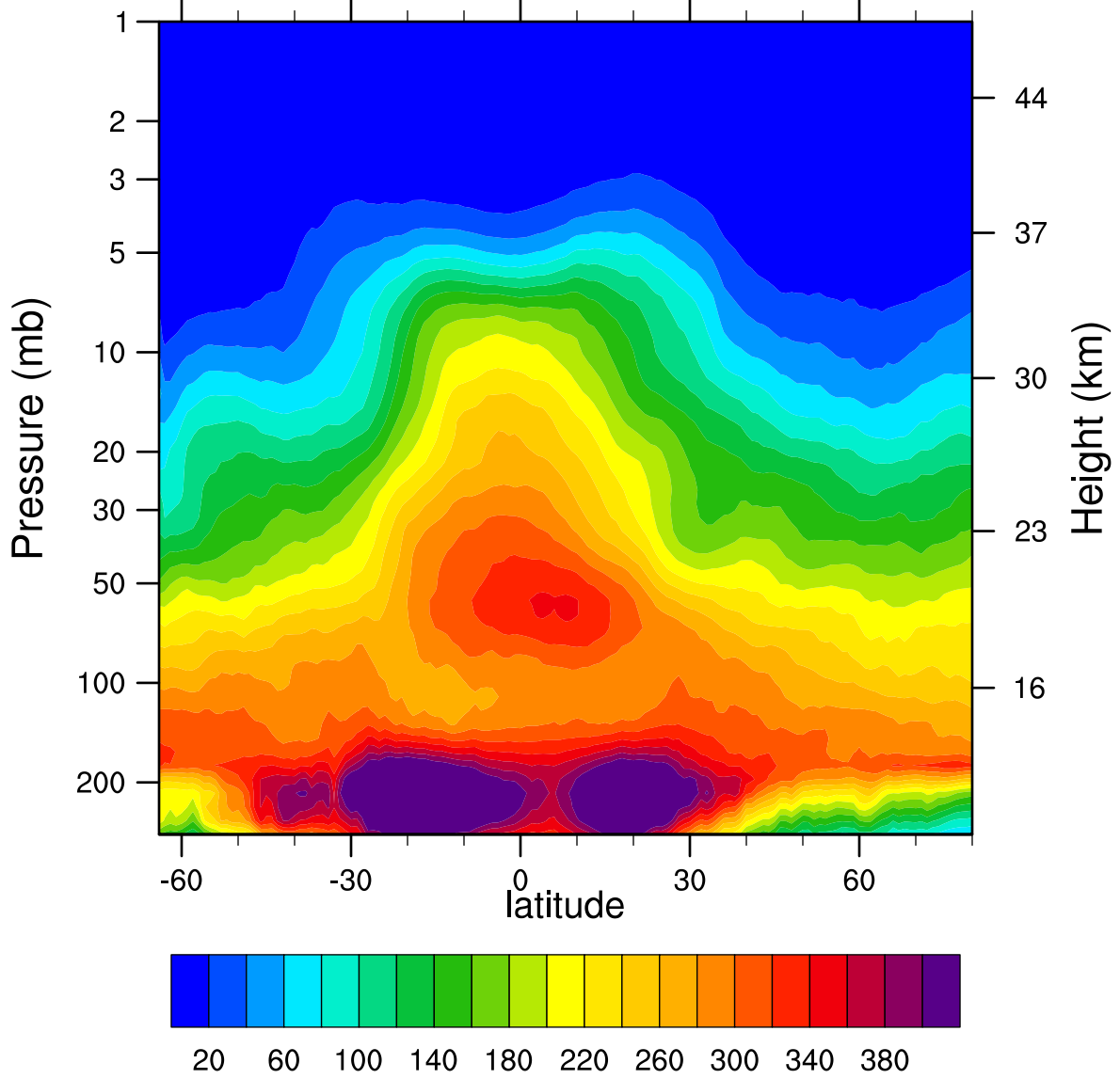
2005d121 N2O_Combined (ppbv)
