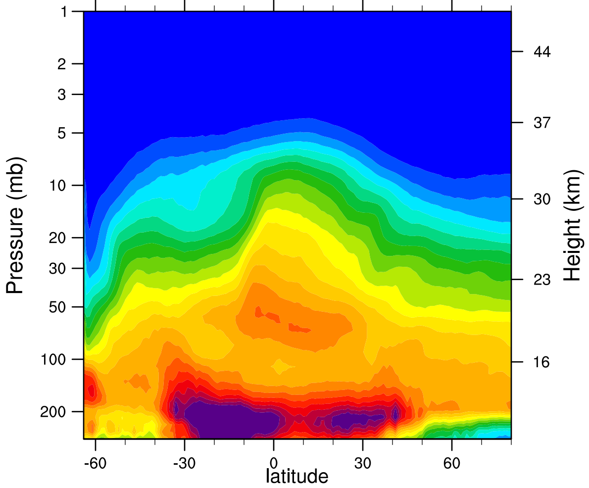
2006d221 N2O_Combined (ppbv)
