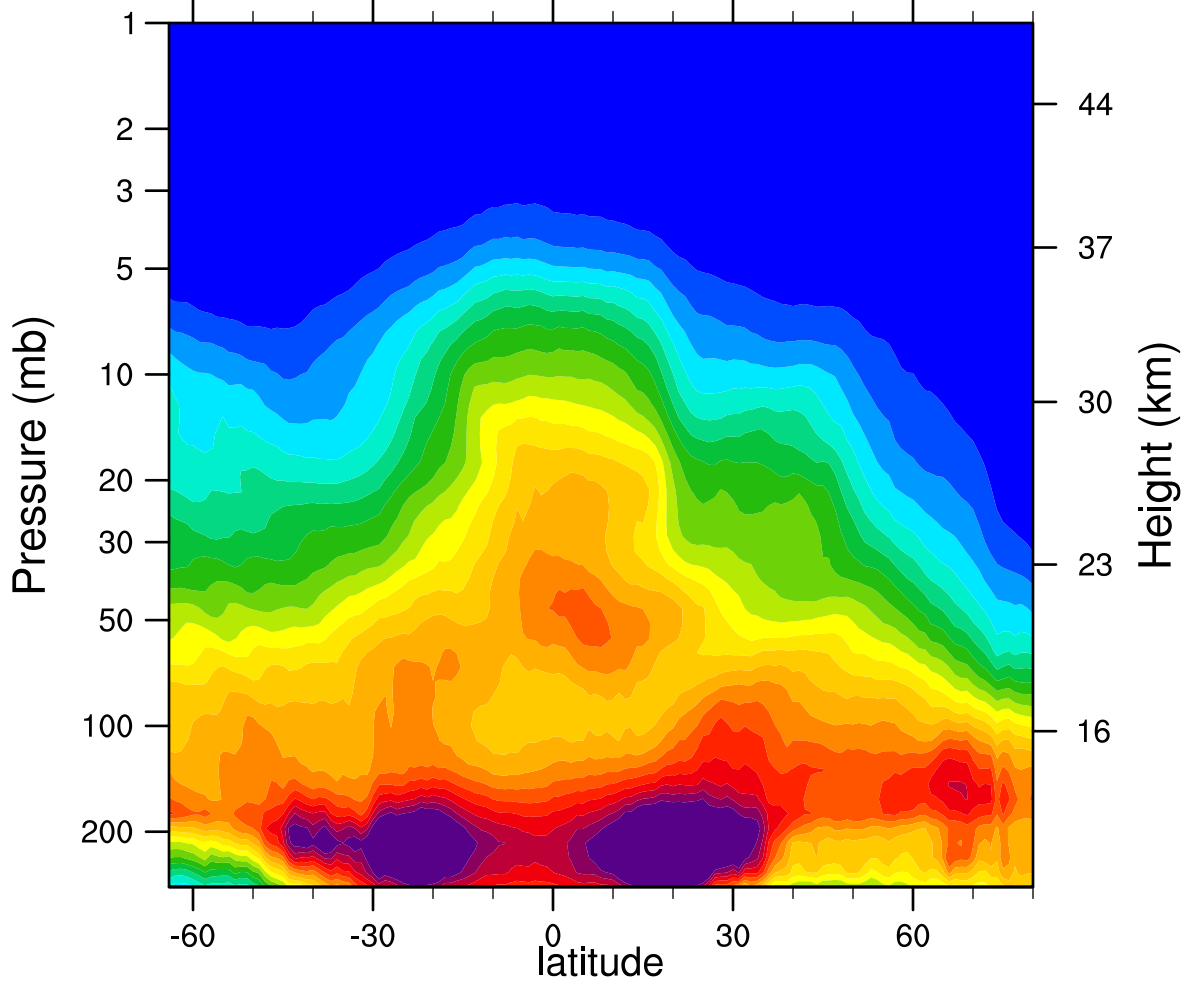
2005d042 N2O_Combined (ppbv)
