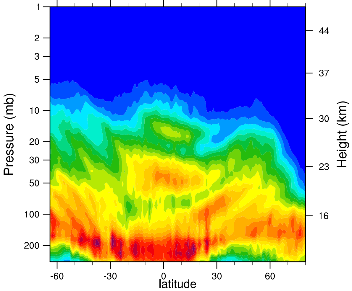
2005d022 N2O_Combined (ppbv)
