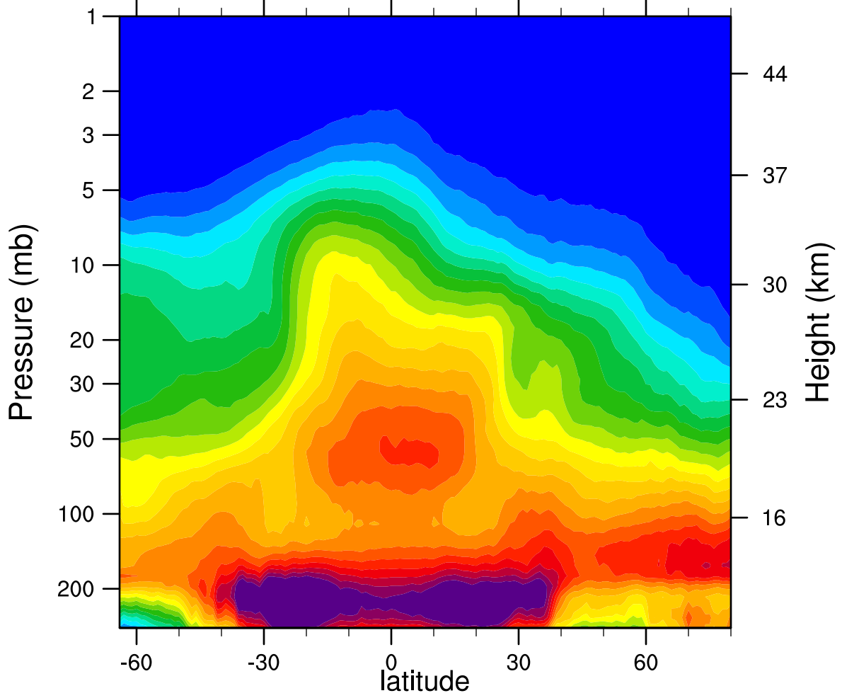
2005d360 N2O_Combined (ppbv)
