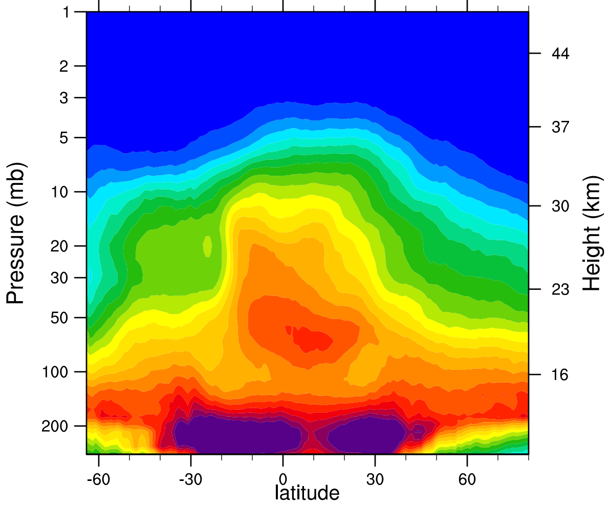
2007d279 N2O_Combined (ppbv)
