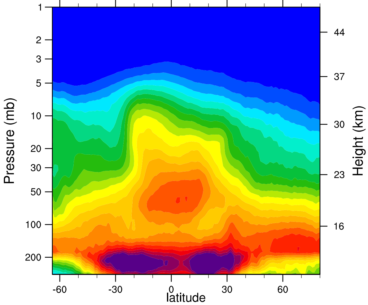
2005d332 N2O_Combined (ppbv)
