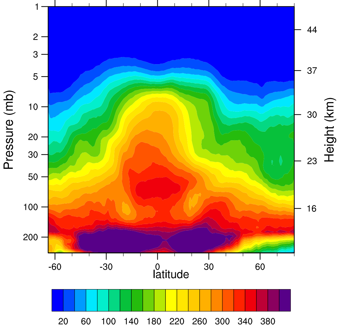
2007d117 N2O_Combined (ppbv)
