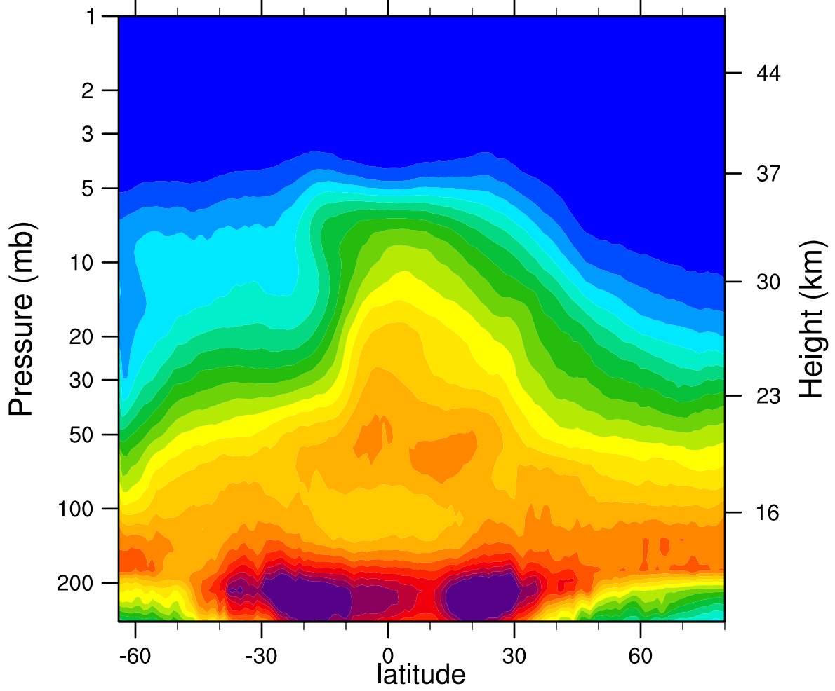
2006d298 N2O_Combined (ppbv)
