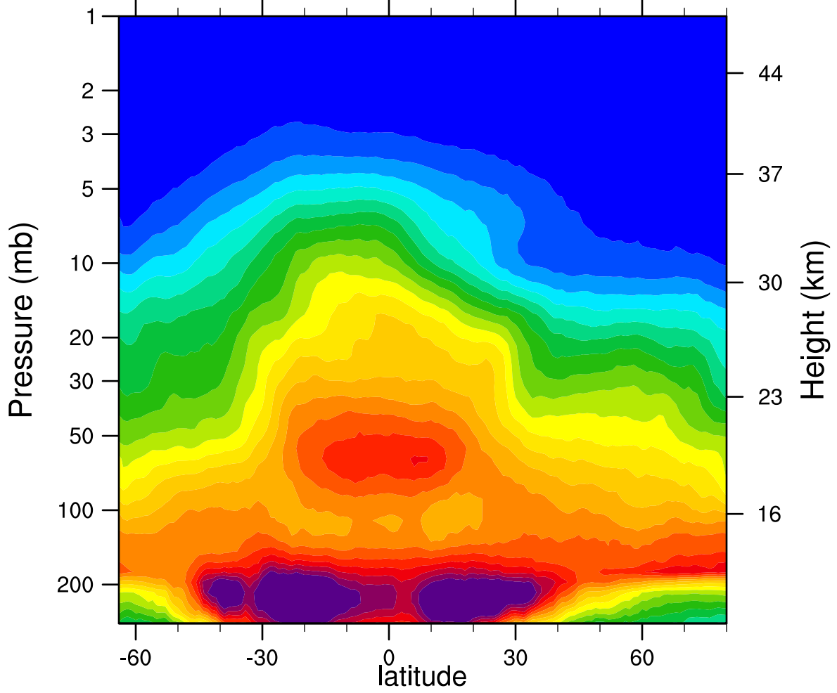
2006d100 N2O_Combined (ppbv)
