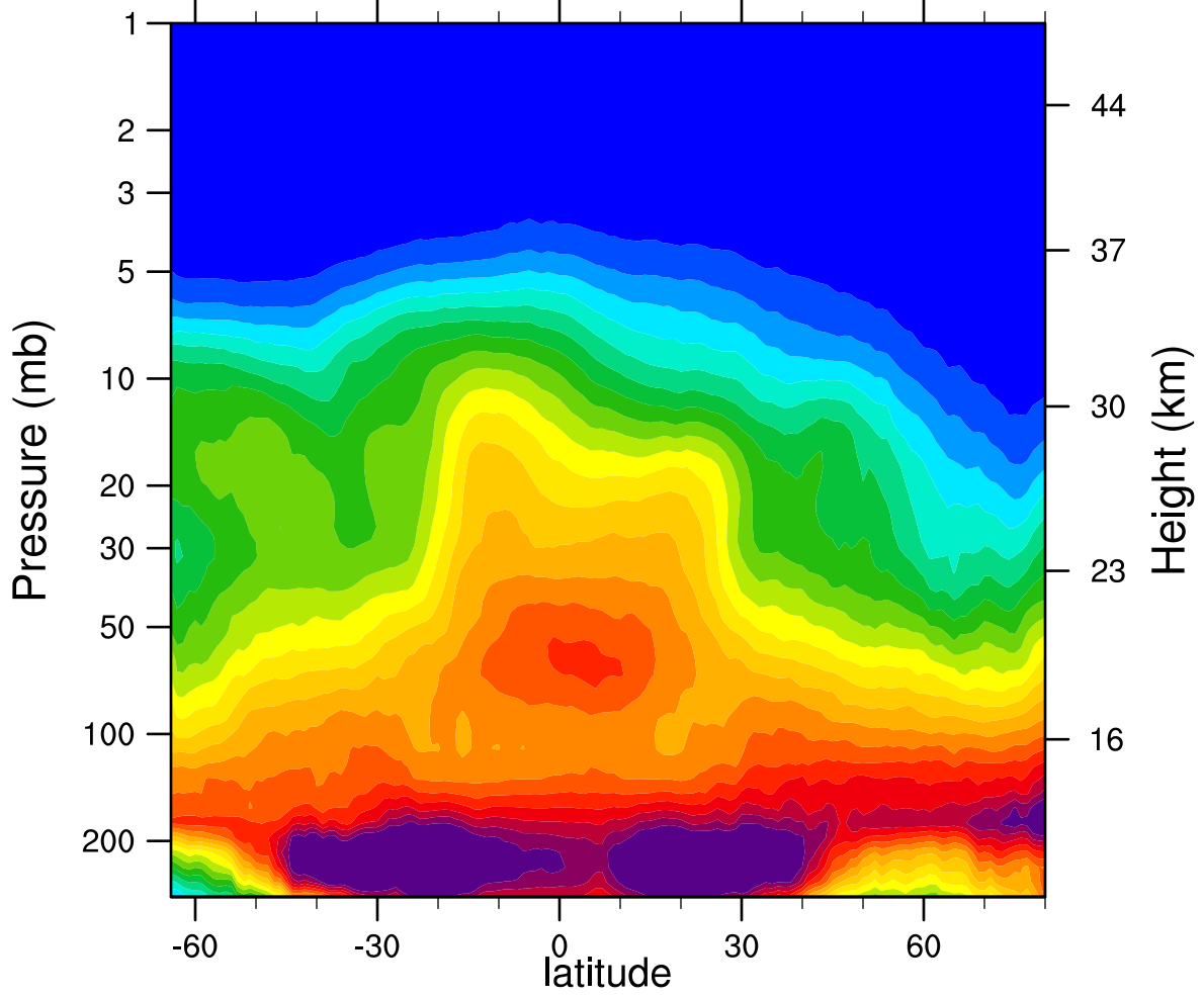
2007d338 N2O_Combined (ppbv)
