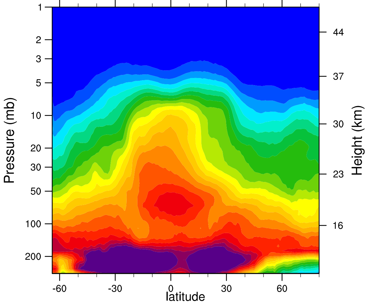
2007d132 N2O_Combined (ppbv)
