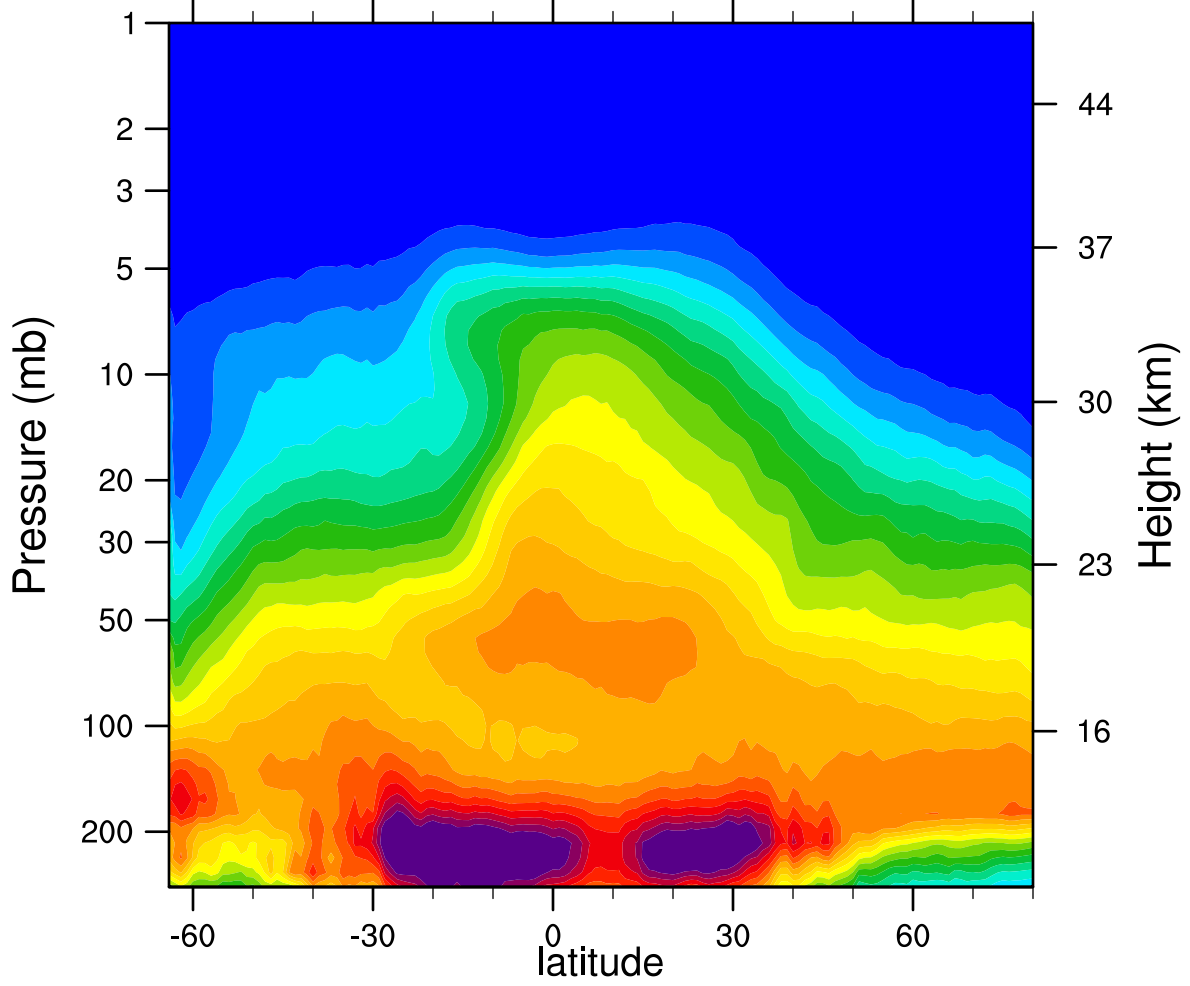
2006d277 N2O_Combined (ppbv)
