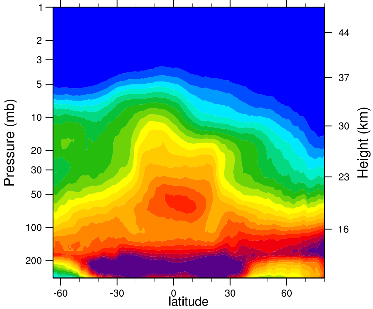
2007d353 N2O_Combined (ppbv)
