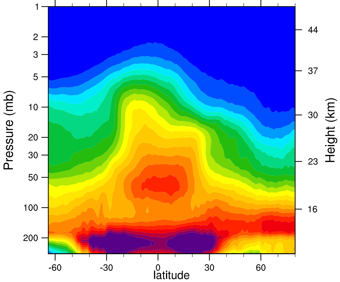
2006d006 N2O_Combined (ppbv)
