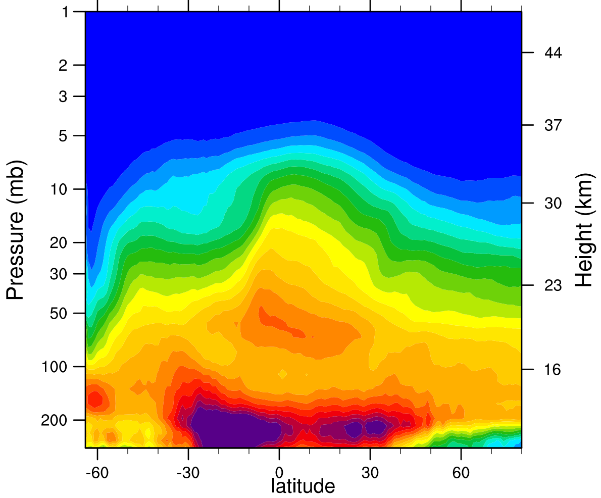
2006d218 N2O_Combined (ppbv)
