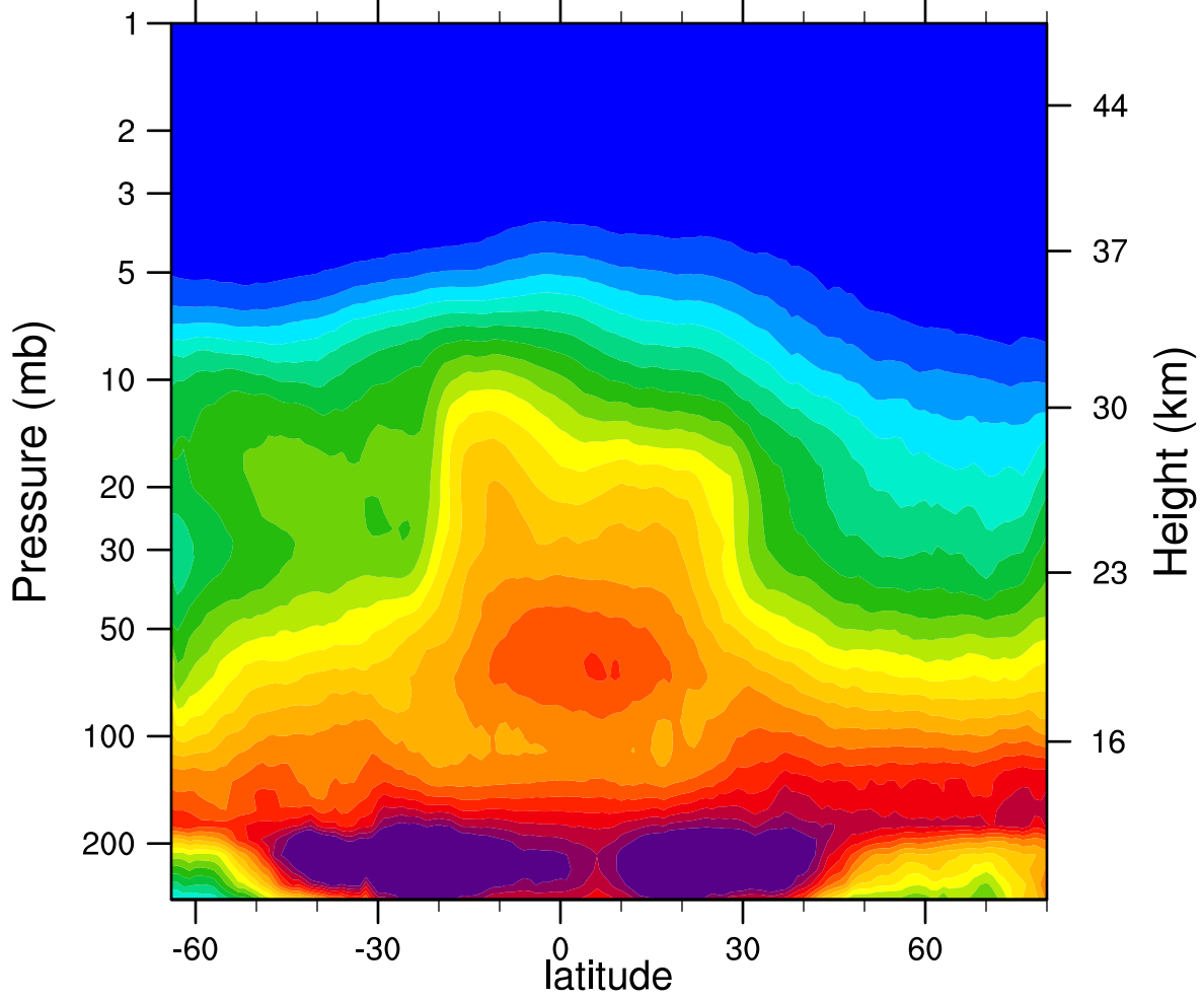
2007d328 N2O_Combined (ppbv)
