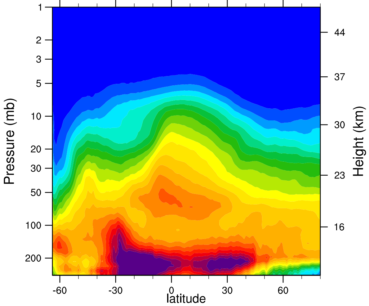
2006d209 N2O_Combined (ppbv)
