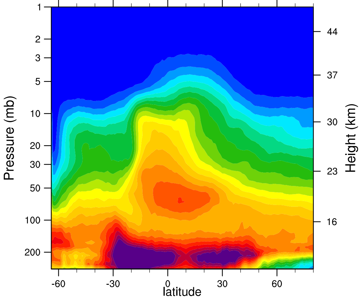
2005d230 N2O_Combined (ppbv)
