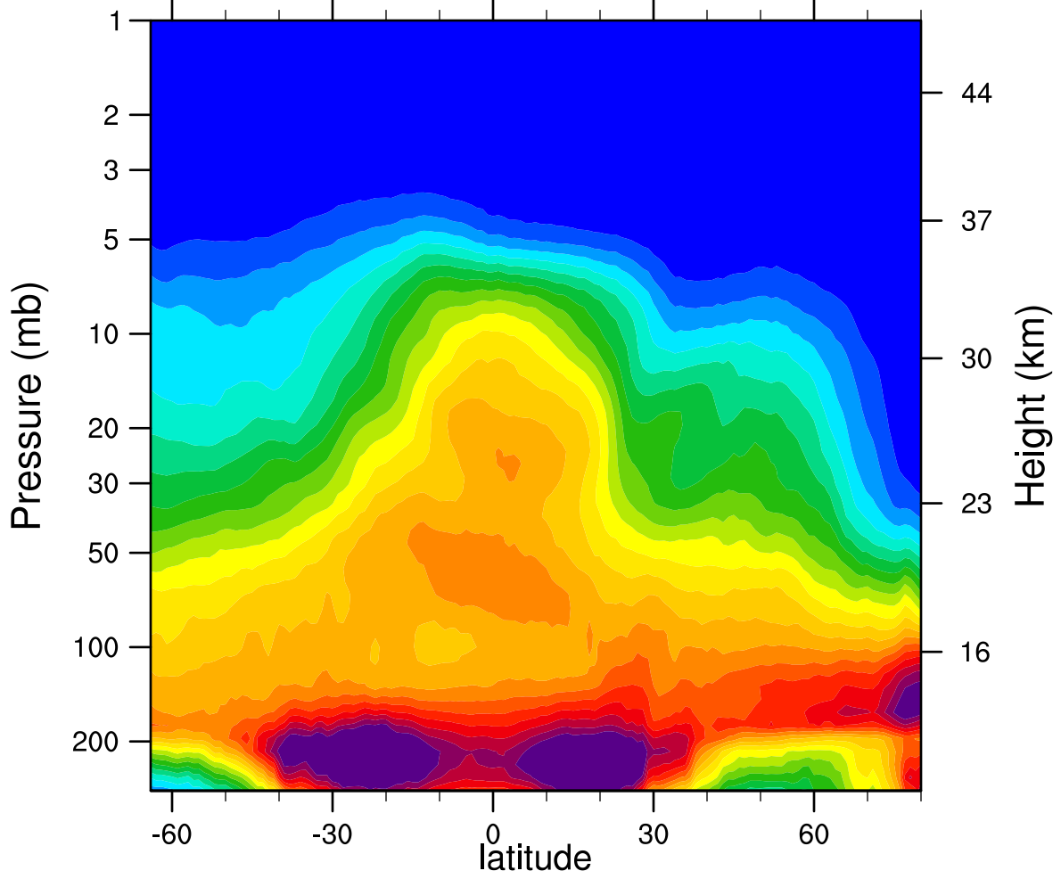
2007d018 N2O_Combined (ppbv)
