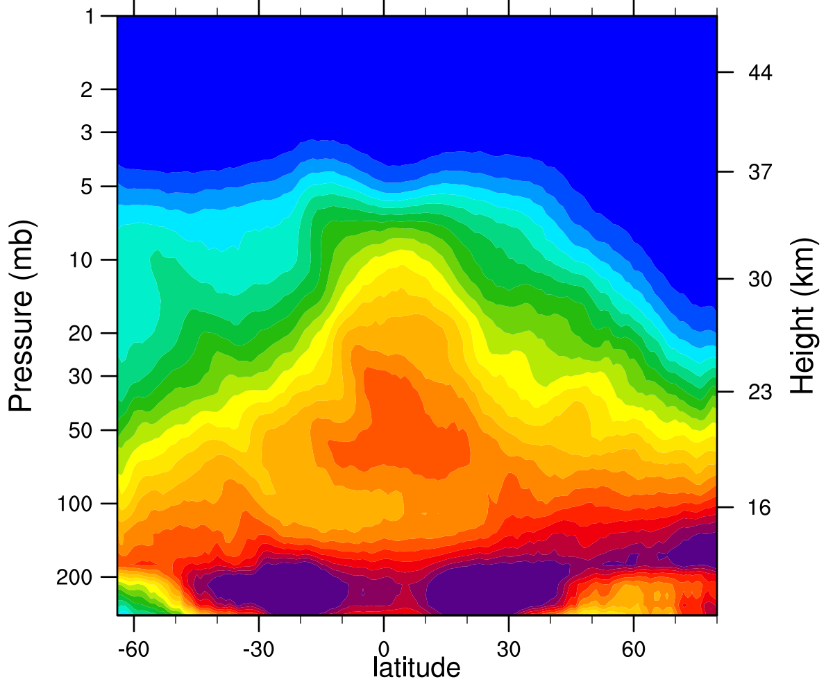
2006d335 N2O_Combined (ppbv)
