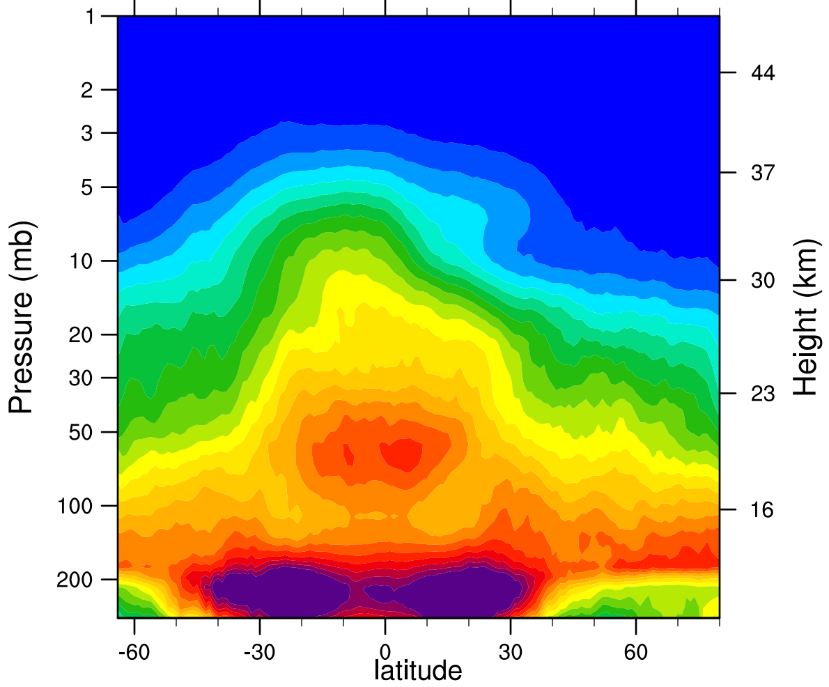
2006d087 N2O_Combined (ppbv)
