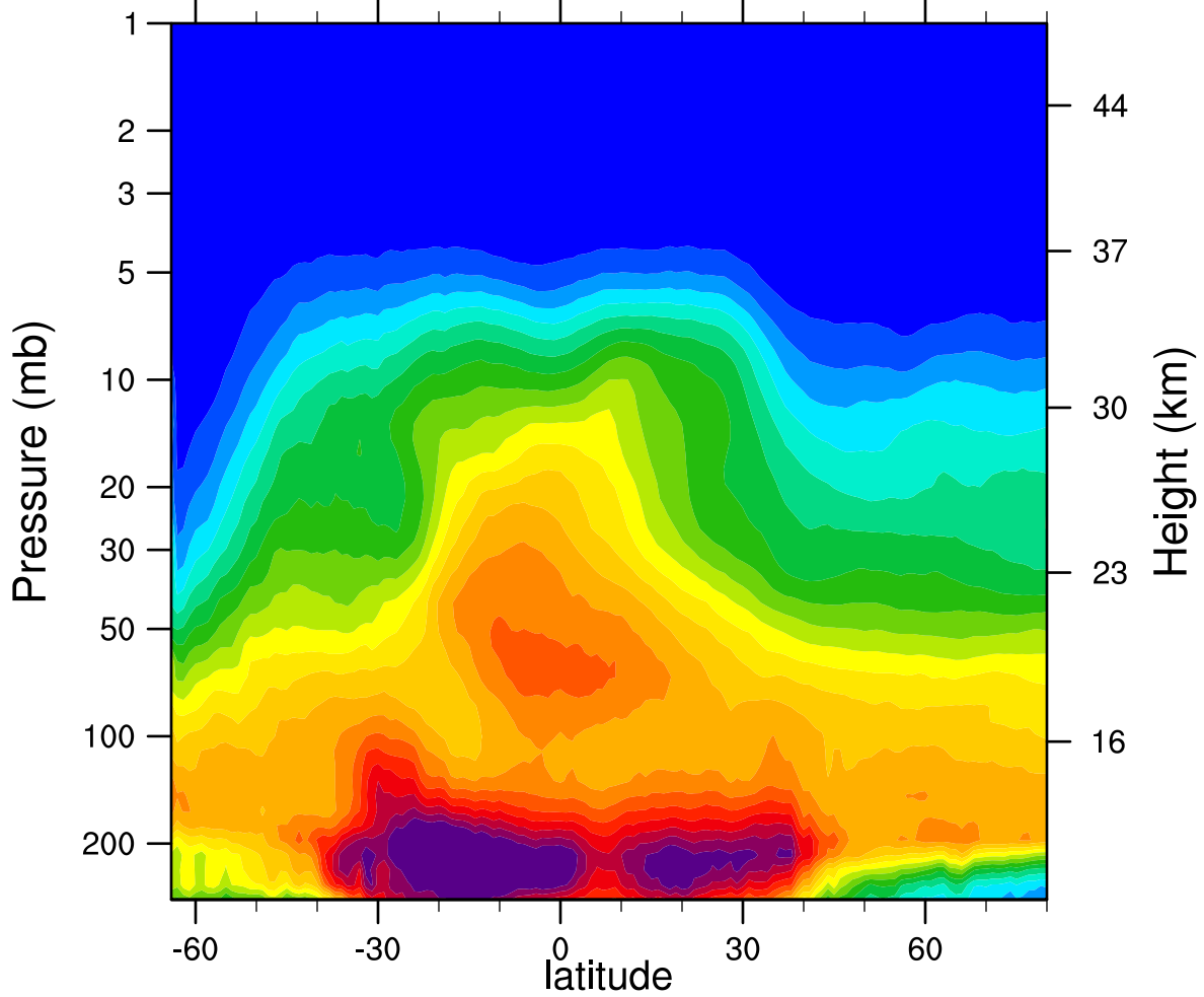
2007d172 N2O_Combined (ppbv)
