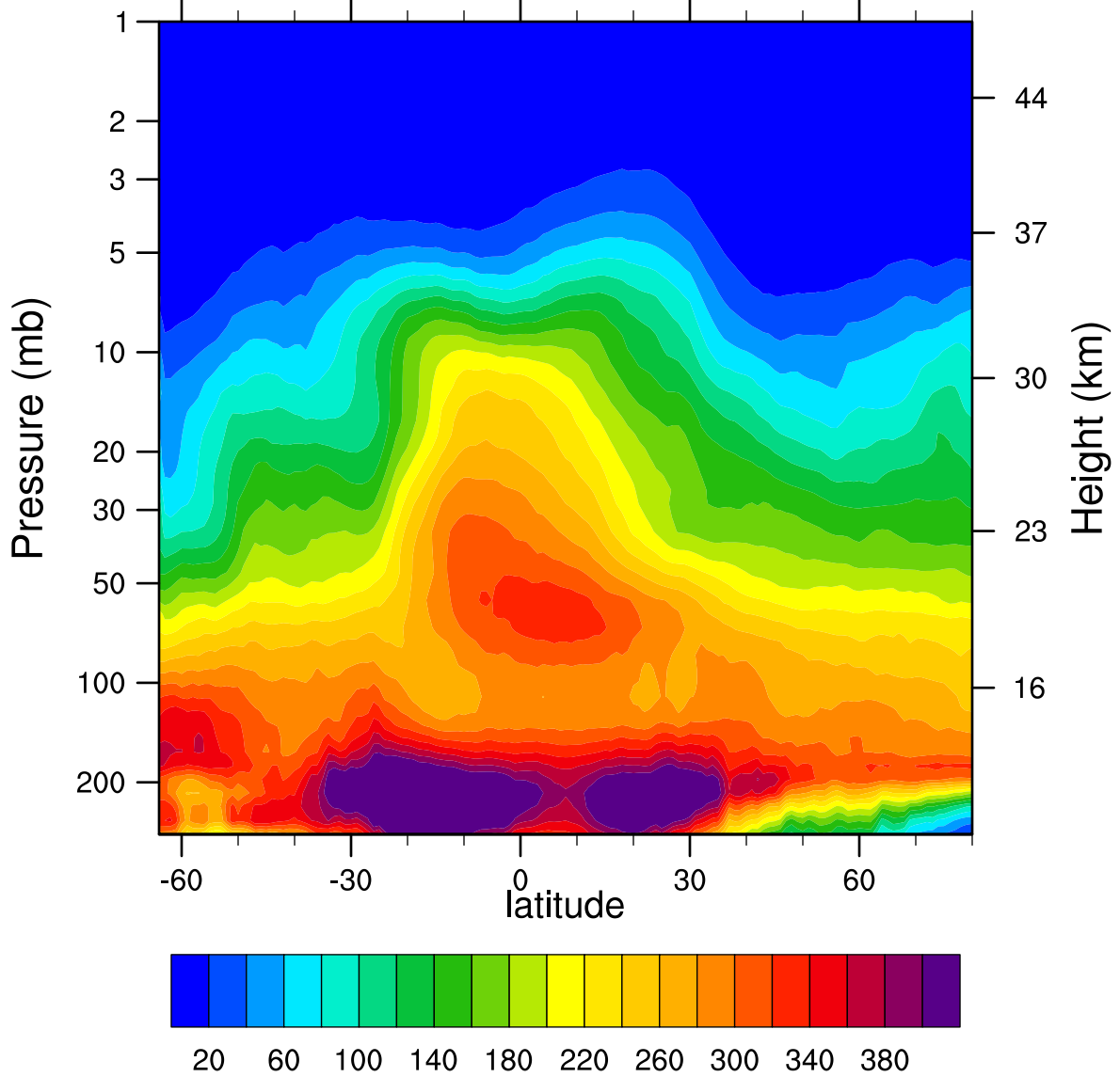
2005d160 N2O_Combined (ppbv)
