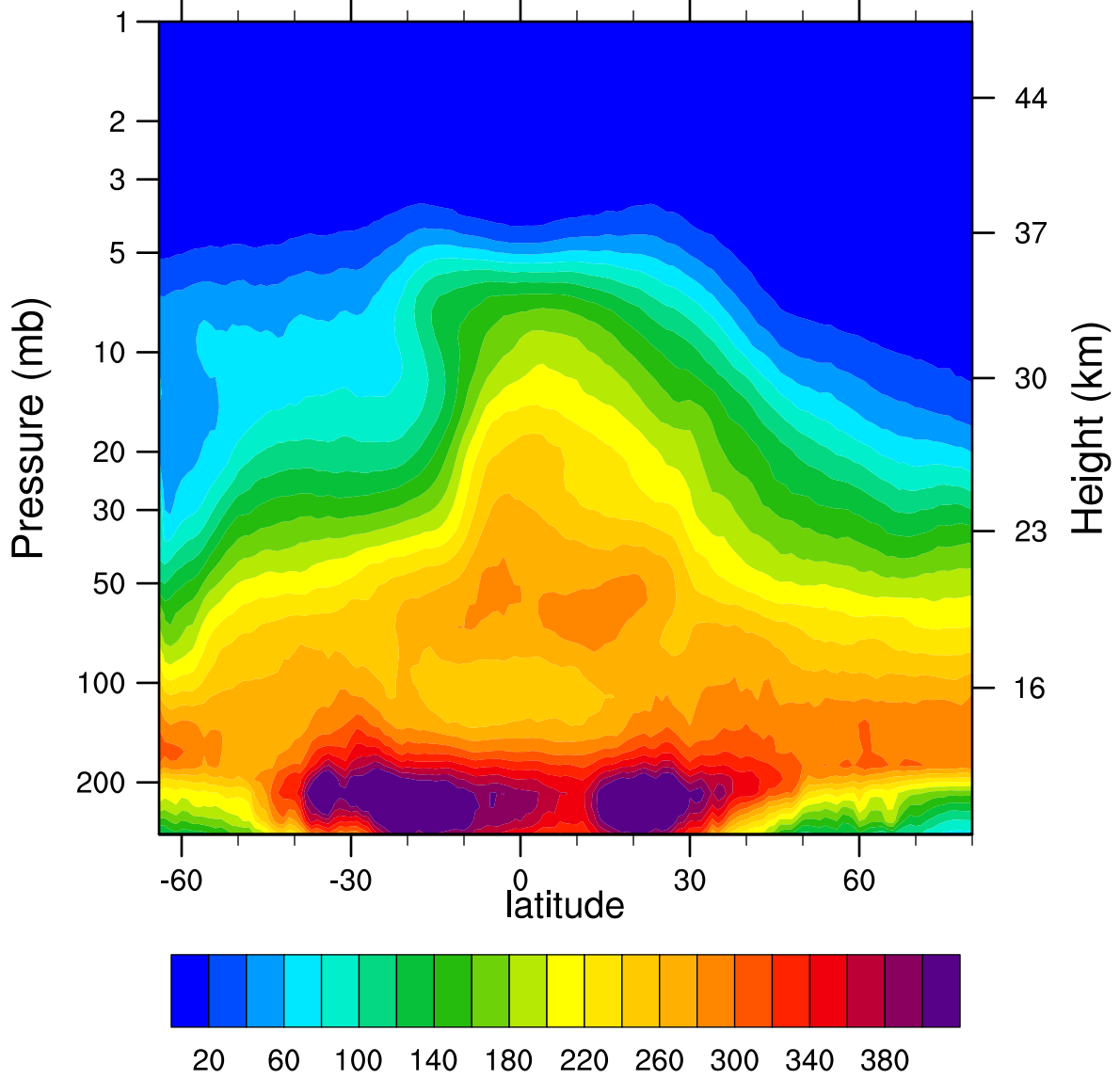
2006d296 N2O_Combined (ppbv)
