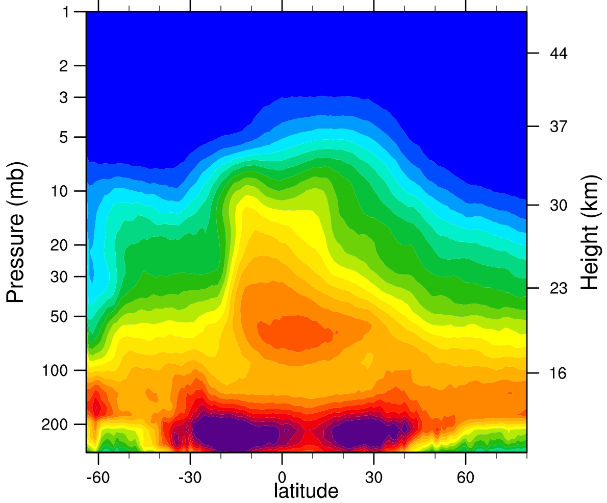
2005d267 N2O_Combined (ppbv)
