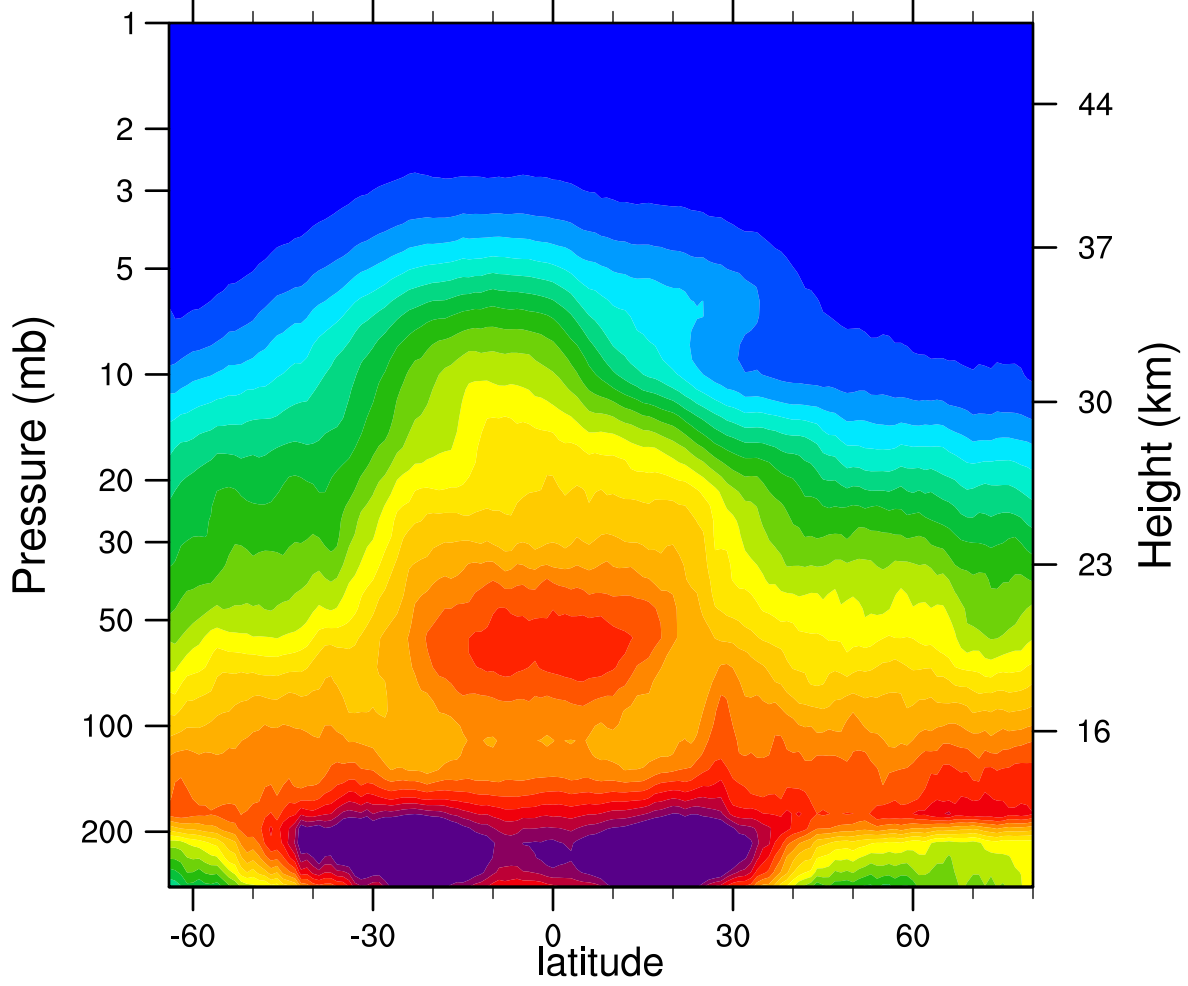
2006d085 N2O_Combined (ppbv)
