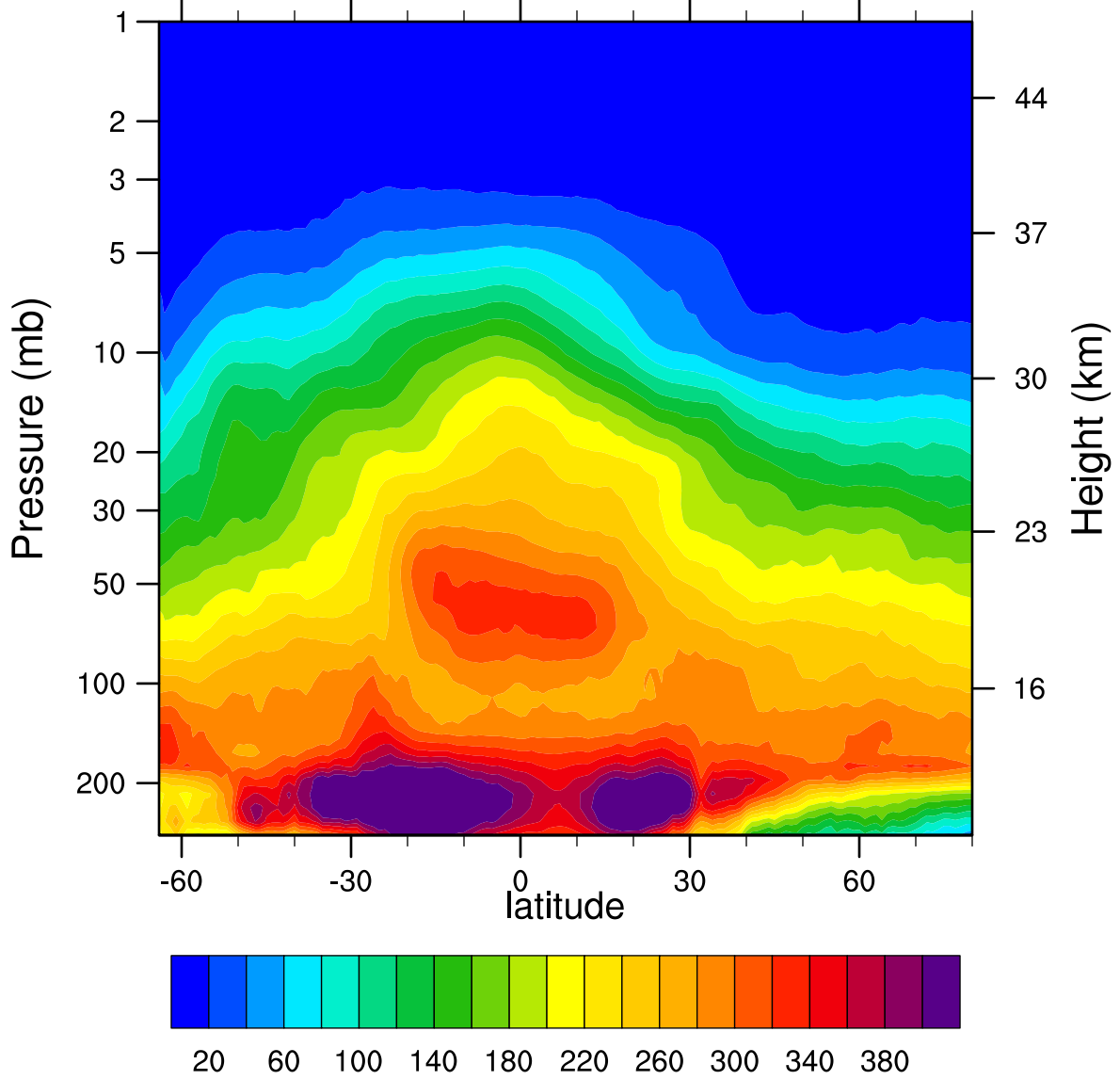
2006d133 N2O_Combined (ppbv)
