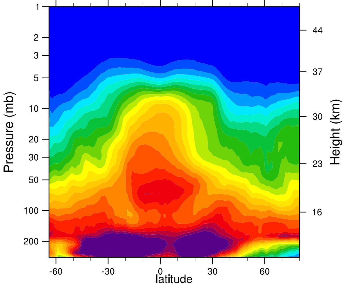
2007d123 N2O_Combined (ppbv)
