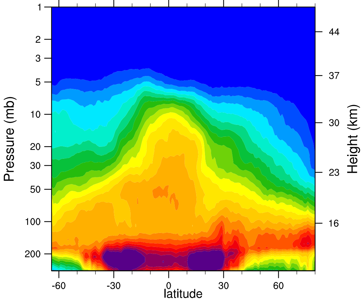
2006d360 N2O_Combined (ppbv)
