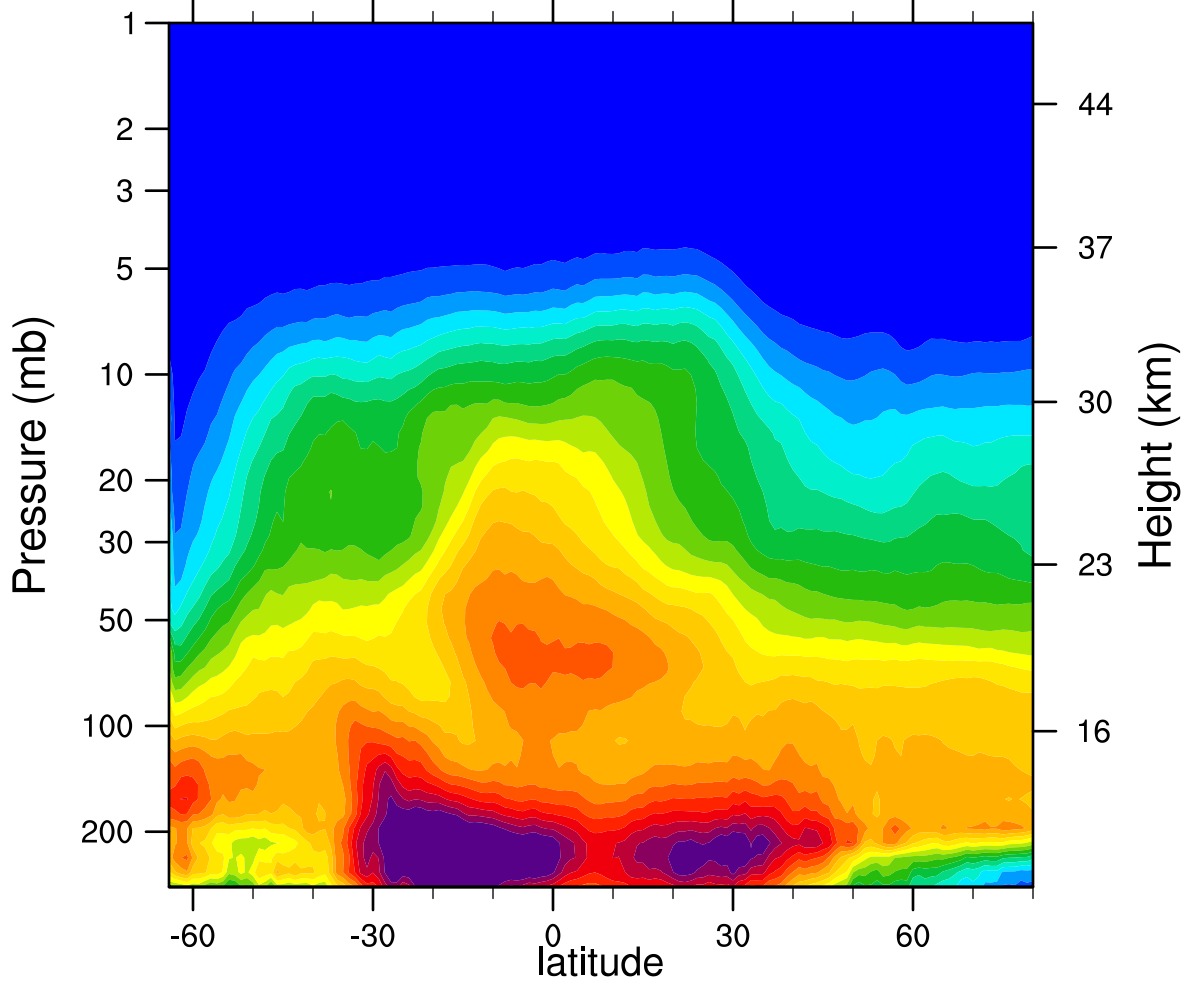
2007d198 N2O_Combined (ppbv)
