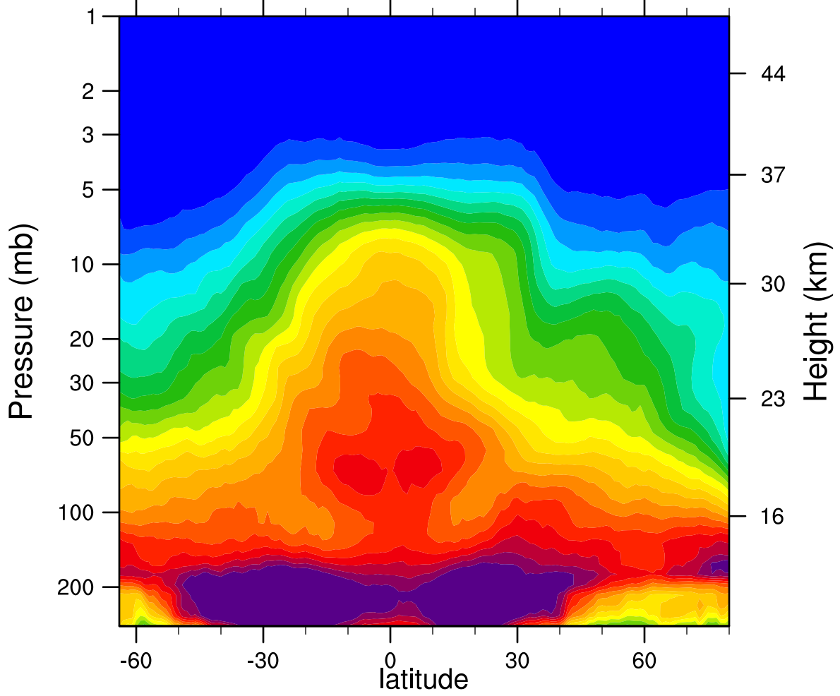
2007d103 N2O_Combined (ppbv)
