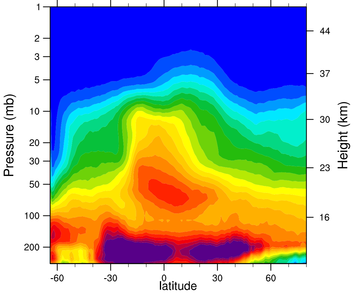
2005d198 N2O_Combined (ppbv)
