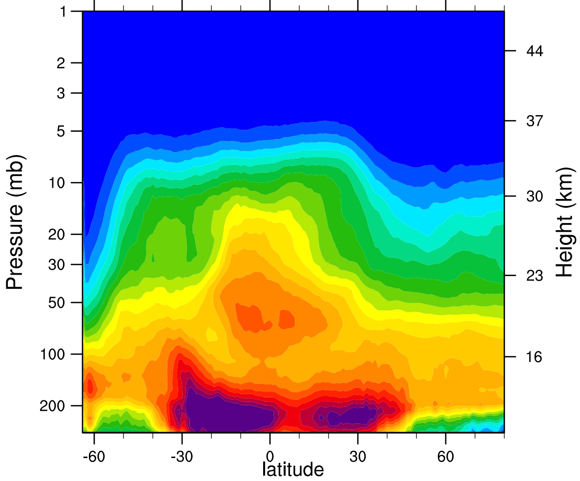
2007d203 N2O_Combined (ppbv)
