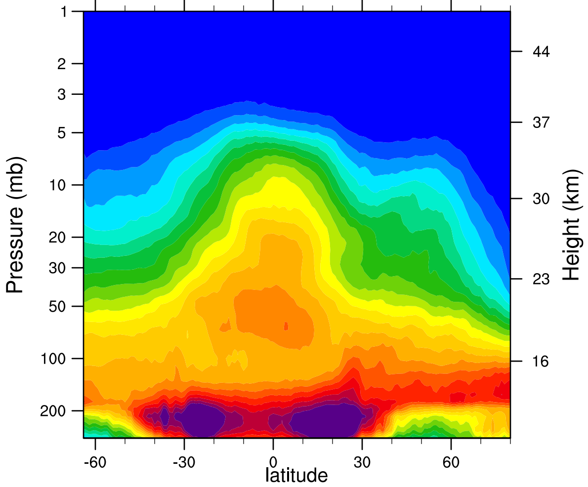
2007d045 N2O_Combined (ppbv)
