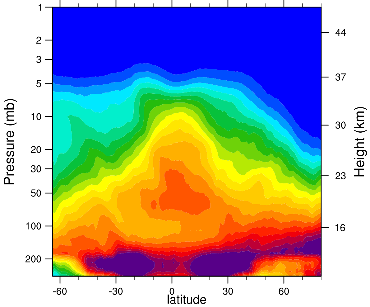
2006d336 N2O_Combined (ppbv)
