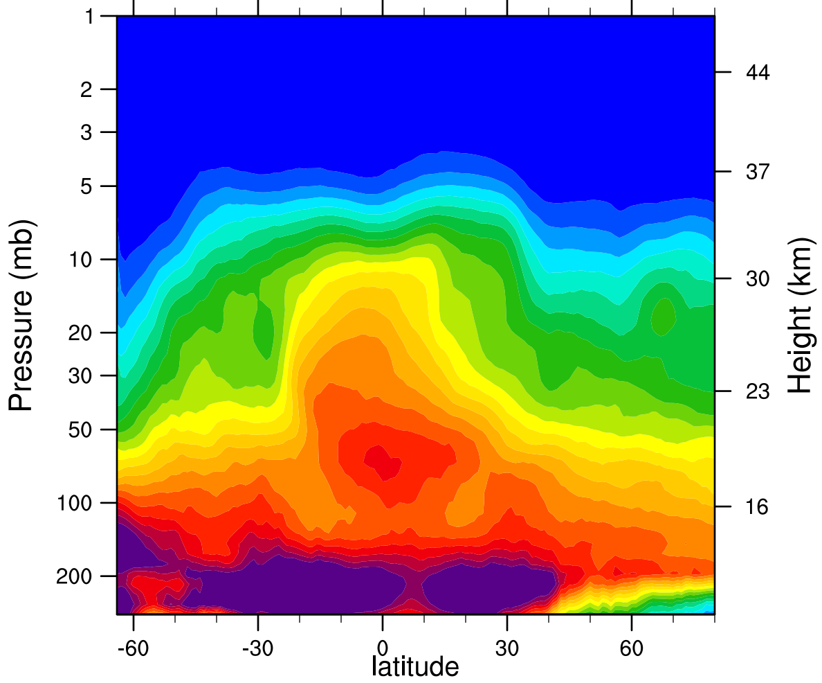
2007d157 N2O_Combined (ppbv)
