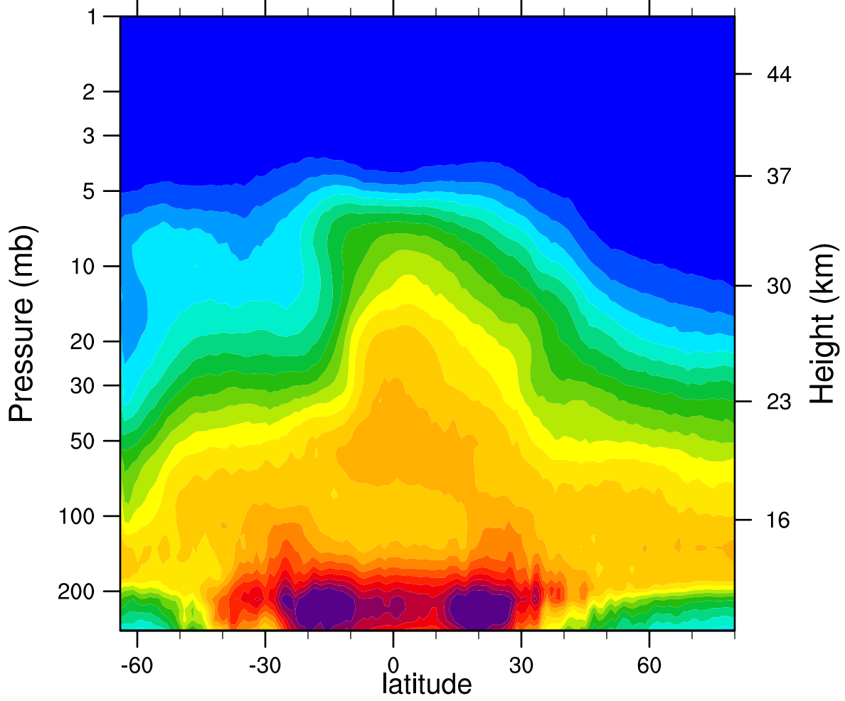
2006d302 N2O_Combined (ppbv)
