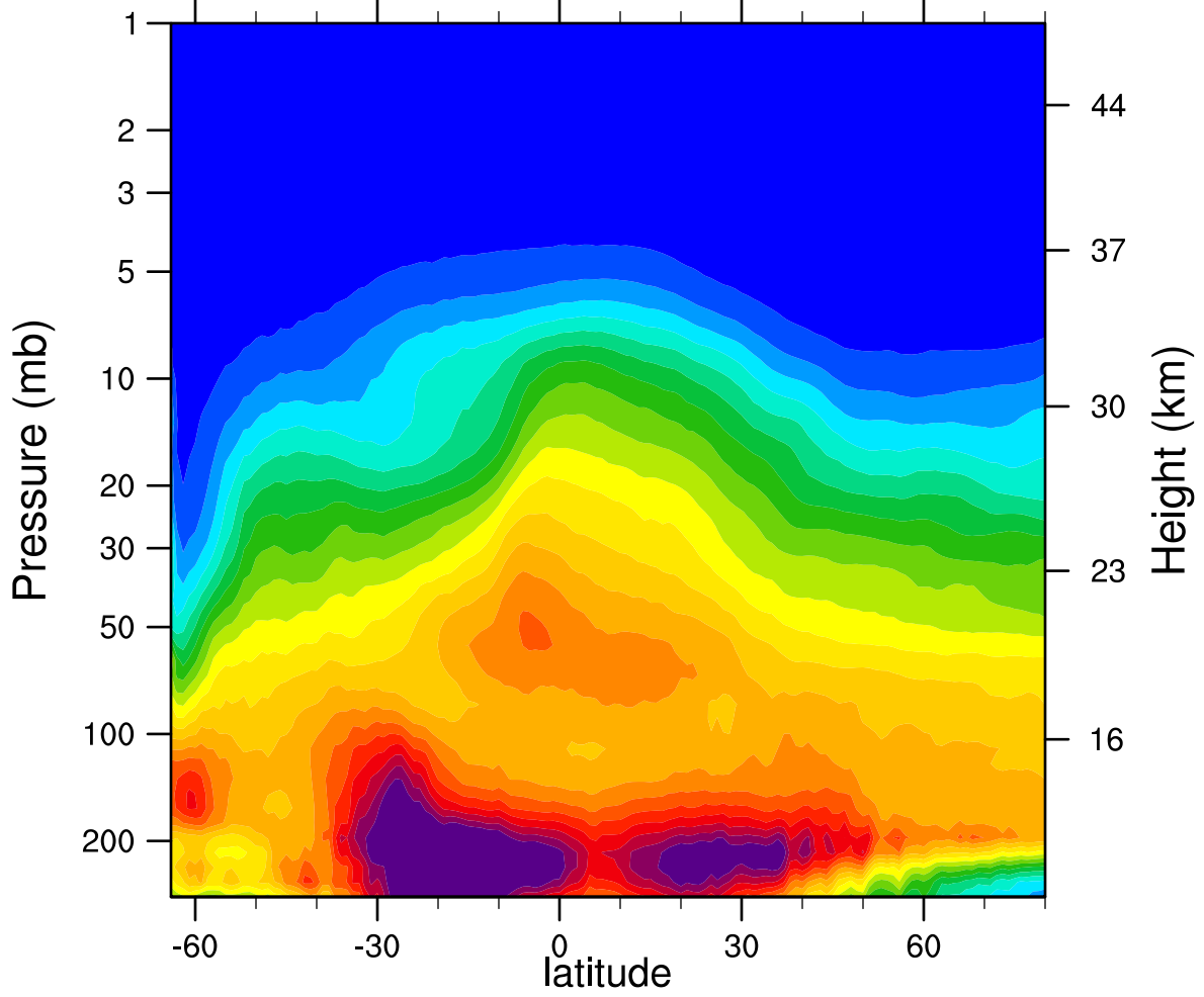
2006d200 N2O_Combined (ppbv)
