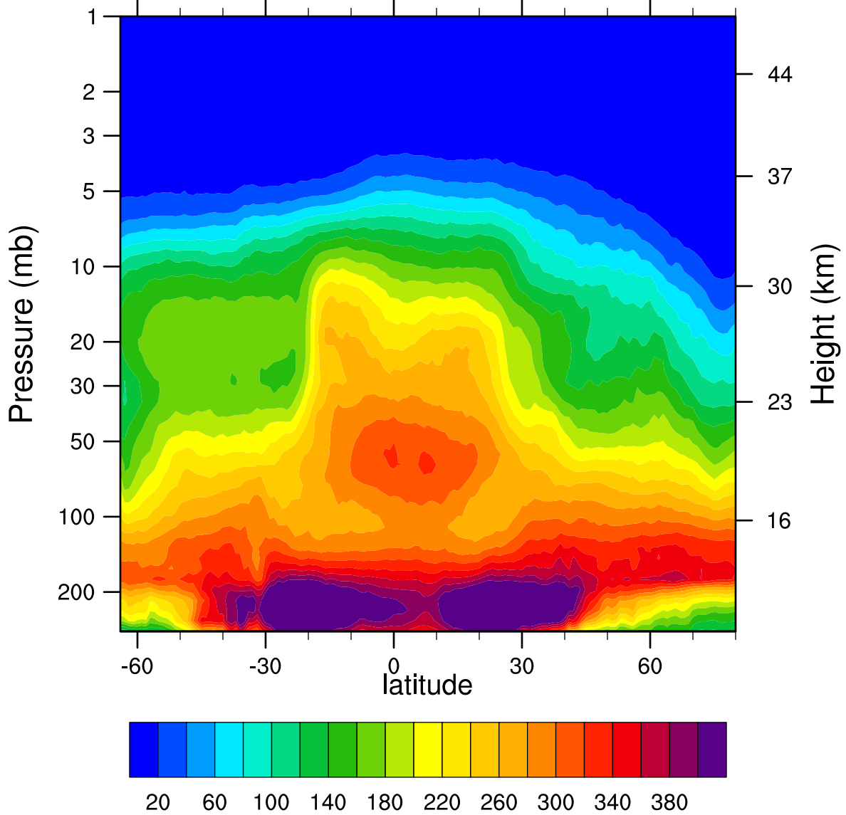
2007d312 N2O_Combined (ppbv)
