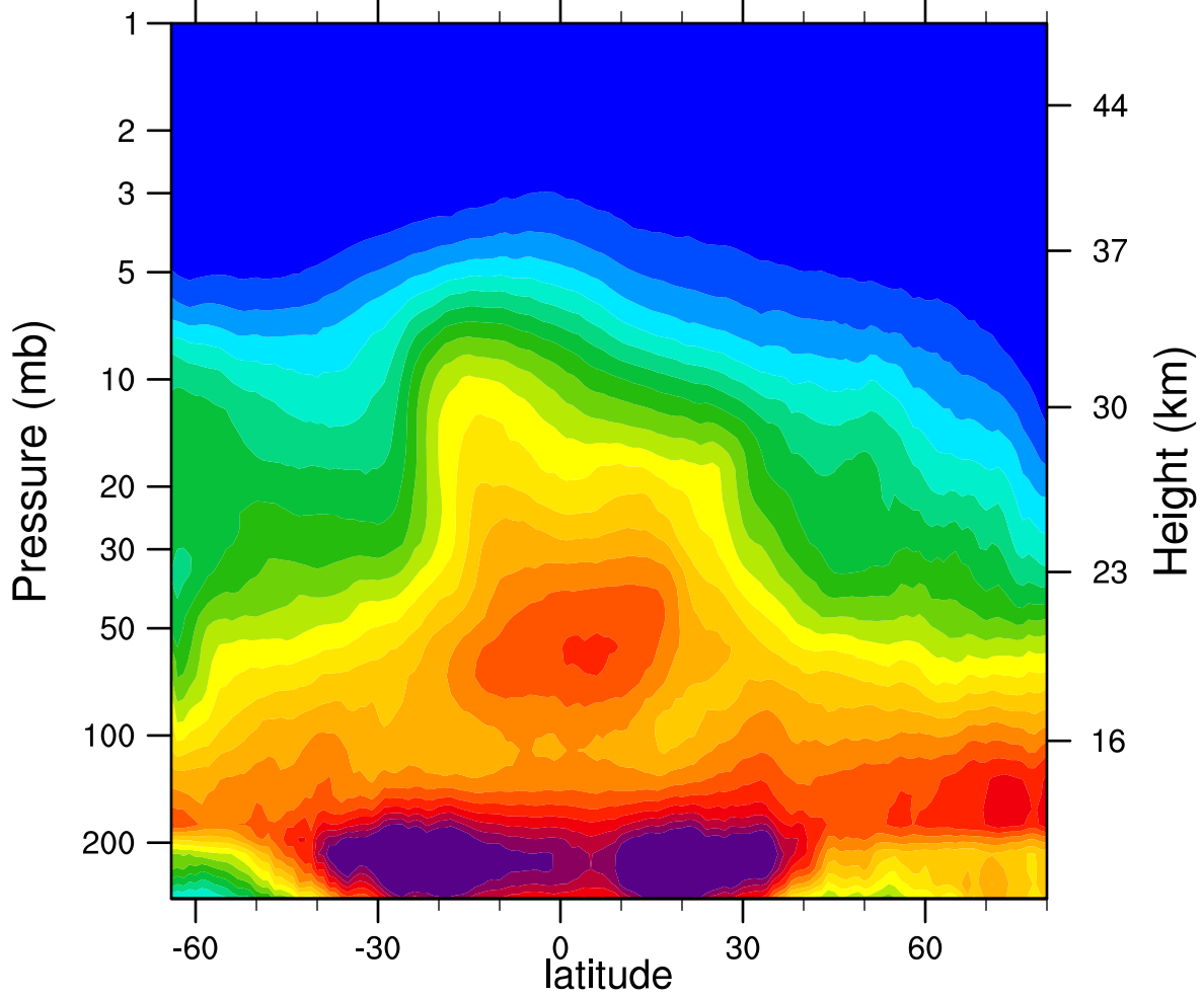
2005d337 N2O_Combined (ppbv)
