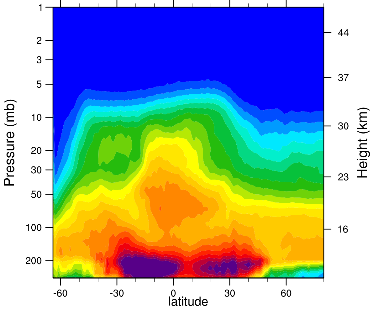
2007d209 N2O_Combined (ppbv)
