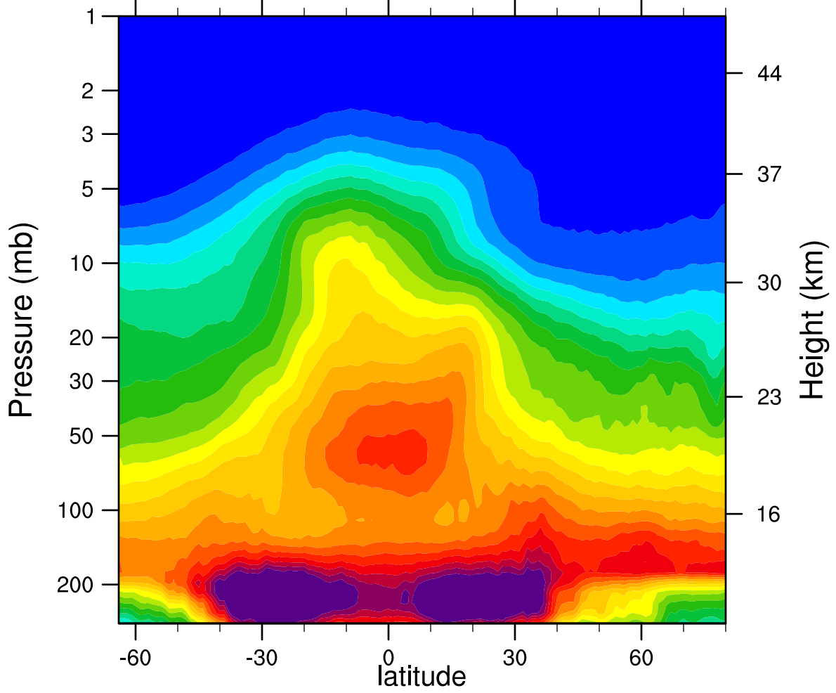
2006d038 N2O_Combined (ppbv)
