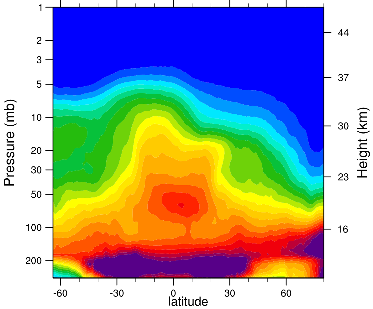
2007d364 N2O_Combined (ppbv)
