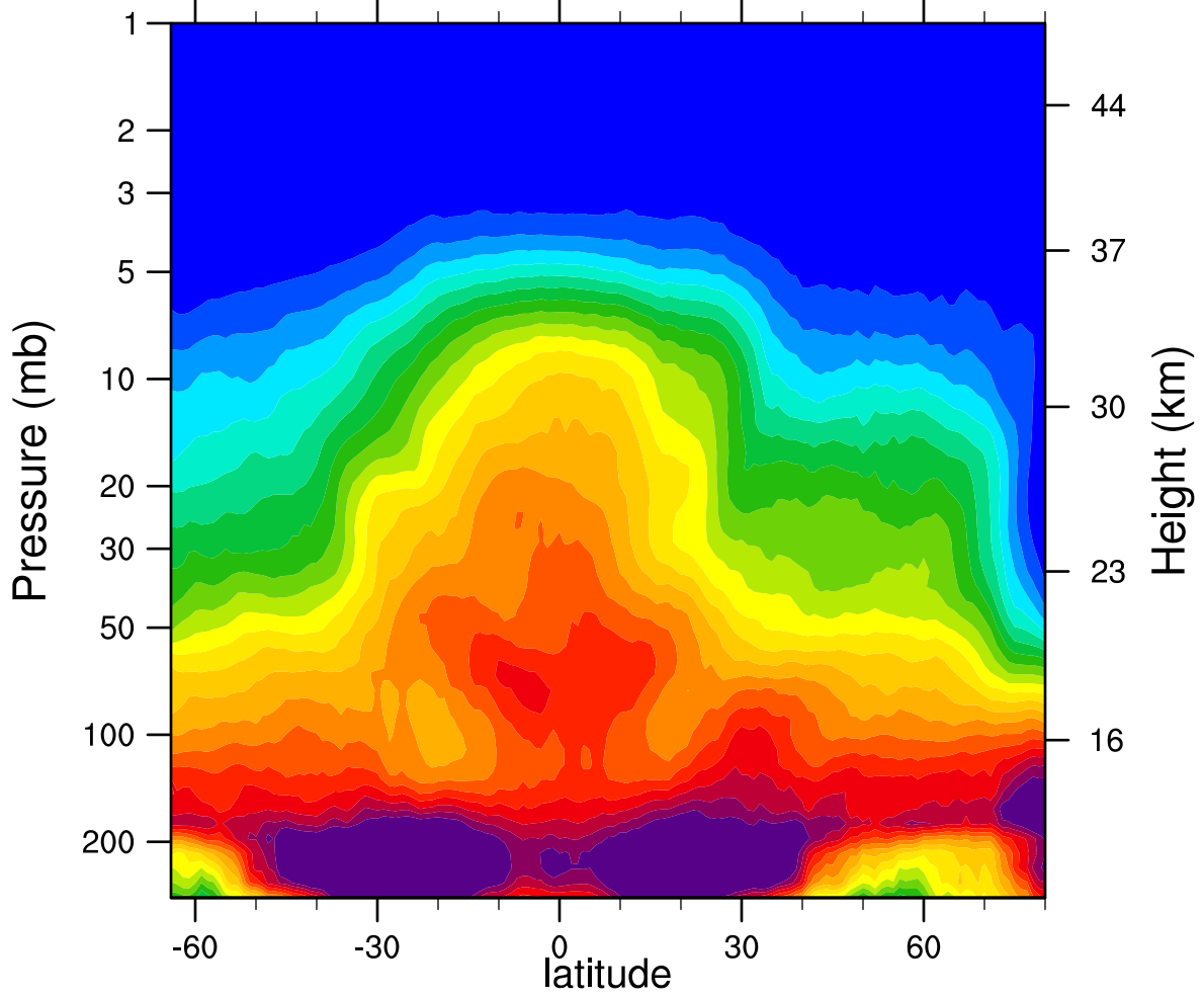
2007d083 N2O_Combined (ppbv)
