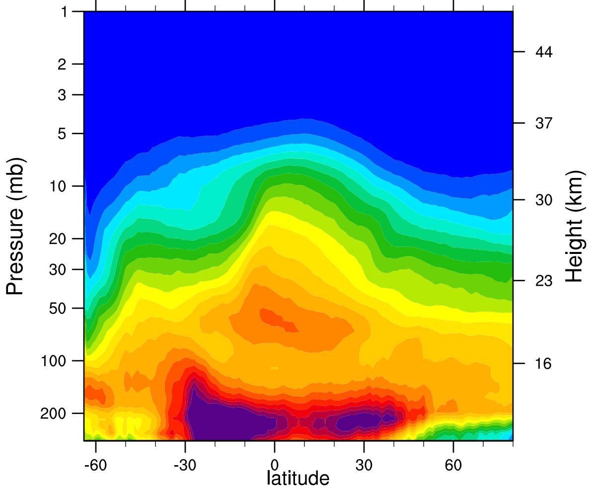
2006d215 N2O_Combined (ppbv)
