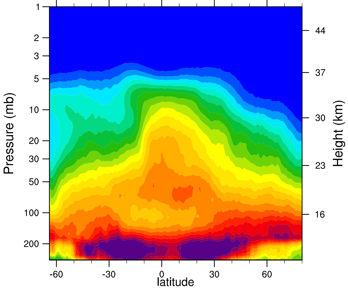
2006d310 N2O_Combined (ppbv)
