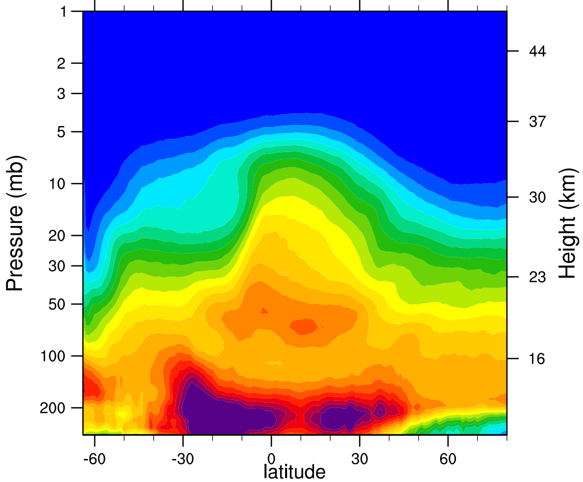
2006d240 N2O_Combined (ppbv)
