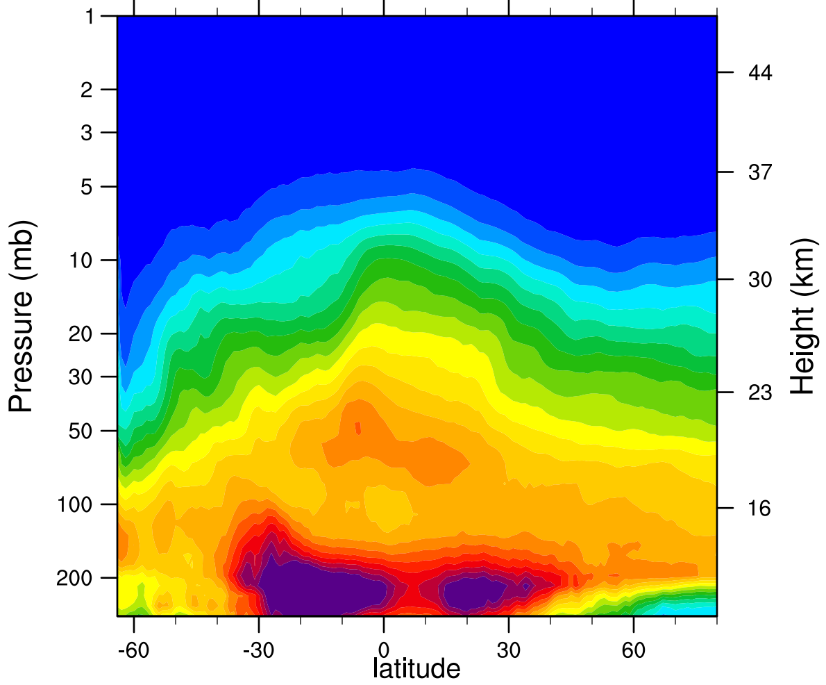
2006d179 N2O_Combined (ppbv)
