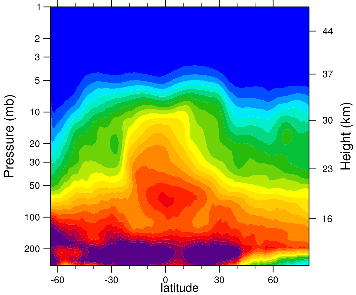
2007d158 N2O_Combined (ppbv)
