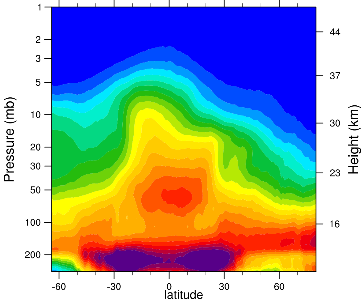
2006d002 N2O_Combined (ppbv)
