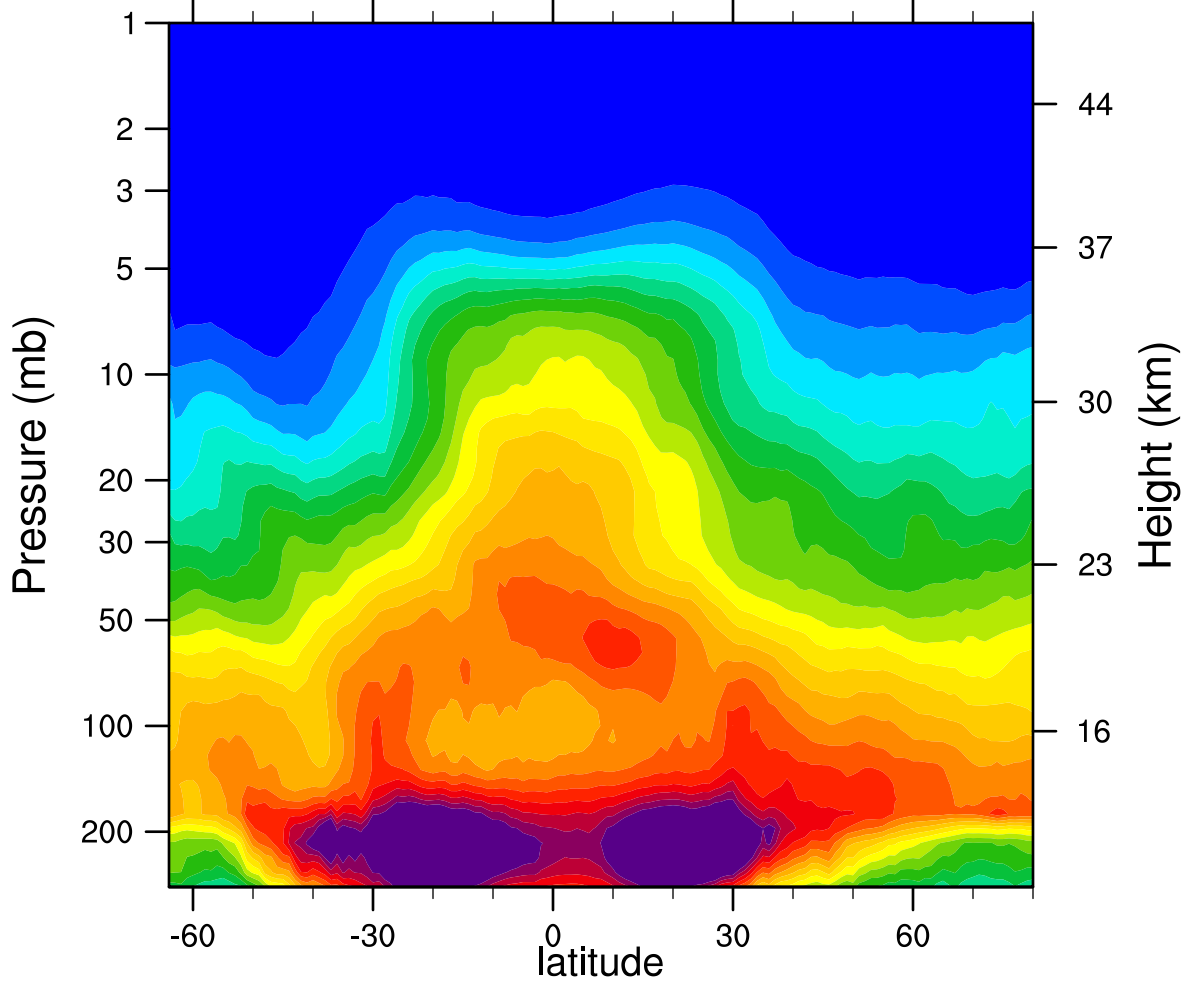
2005d106 N2O_Combined (ppbv)
