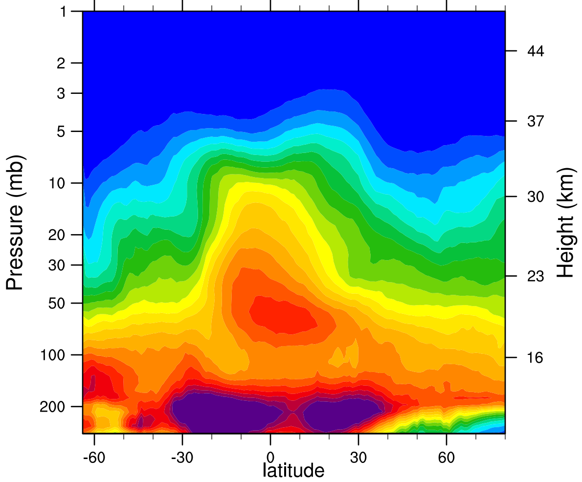
2005d157 N2O_Combined (ppbv)
