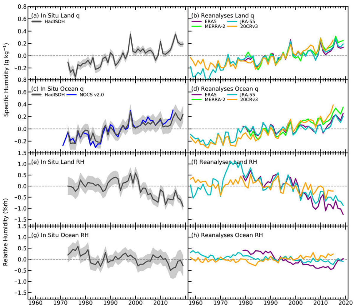
Fig. 2.15. Global average surface humidity annual anomalies (1981–2010 base period). For the in situ datasets, 2-m surface humidity is used over land and \sim 10 -m over the oceans. A 2 std. dev. uncertainty range is shown for HadISDH, capturing the observation, gridbox sampling, and spatial coverage uncertainty. For the reanalysis, 2-m humidity is used over the whole globe. For ERA5 ocean series, only points over open sea are selected, and background forecast values are used as opposed to analysis values because of unreliable use of ship data in producing the analysis. (Sources: HadISDH [Willett et al. 2013, 2014, in review]; NOCSv2.0 [Berry and Kent 2009, 2011]; ERA5 [C3S 2017; Hersbach et al. 2020]; JRA-55 [Ebata et al. 2011]; MERRA-2 [Gelaro et al. 2017]; and 20CRV3 [Slivinski et al. 2019].)
