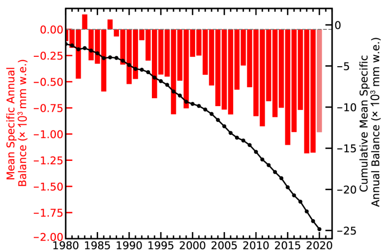
Fig. 2.14. Mass balance of alpine glaciers reporting to the World Glacier Monitoring Service in mm of water equivalent (mm w.e.). The values from 1980 to 2020 are based on average annual value determined for 19 different Alpine regions.
