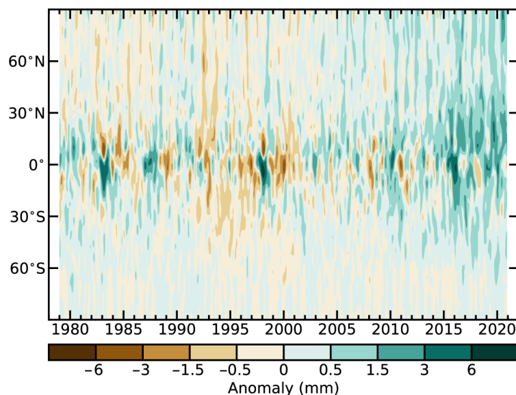
Fig. 2.21. Hövmüller plot of total column water vapor anomalies (mm; base period 1981–2010) derived from the ERA5 reanalysis.
