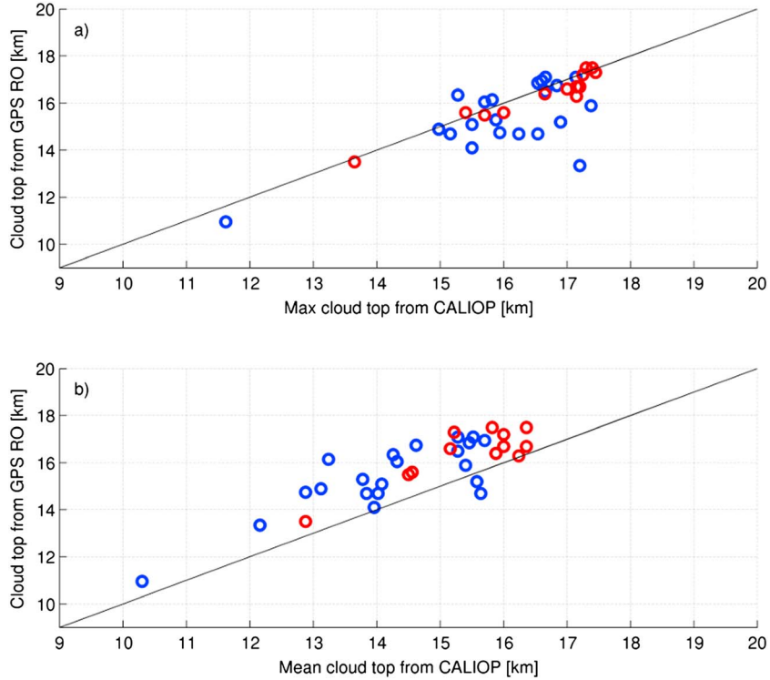
Figure 6. Scatter plot between the cloud top from CALIOP and from GPS ROs, the red circles are the 13 cases closest in time and space (2 h and 100 km). (a) Related to the highest top of the system and (b) with the averaged top of the system. Mean bias, RMSE and correlations are reported in Table 2.
