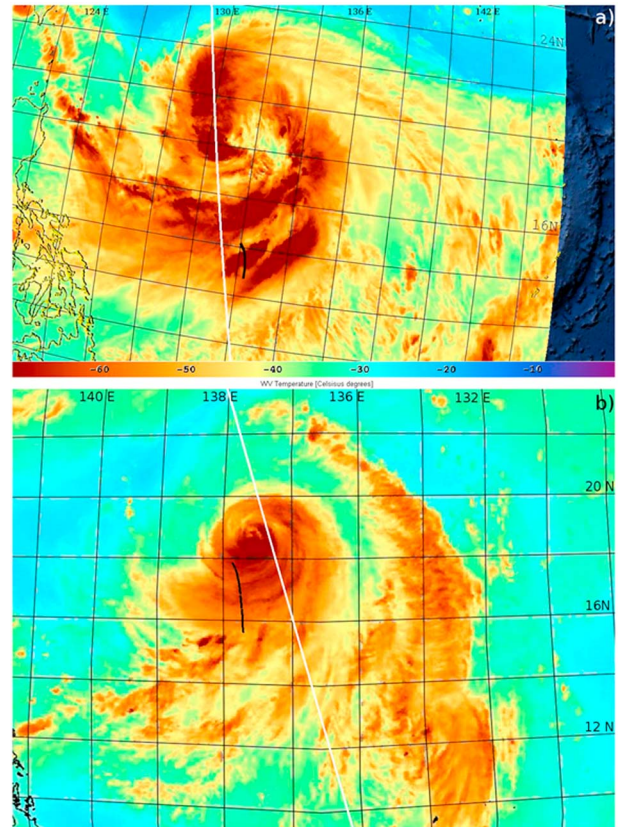
Figure 3. Structure of Krosa (top) on 2 October 2007. Structure of Nakri (bottom) on 31 May 2008. Colors denote GMS brightness temperature (° Celsius) in the water vapor channel (6.5 \mu\text{m} ), with brown denoting low values. The black line denotes the GPS RO tangent points and the white line is the CALIPSO track.
