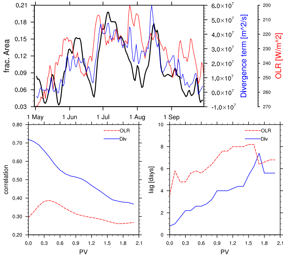
Figure 7. (top) Time series from the year 2006 of daily mean low PV area with PV \leq 0.3 PVU (black) together with integrated divergence over this area (blue) and mean OLR over 15^{\circ}\text{N} – 30^{\circ}\text{N} and 60^{\circ}\text{E} – 120^{\circ}\text{E} (red). (bottom) The 5 year mean (2005–2009) correlation (left) and optimal lag (right) of PV area with divergence (blue) and OLR (red) as a function of PV threshold. The correlations are calculated for each year over the deseasonalized time series from May to September.
