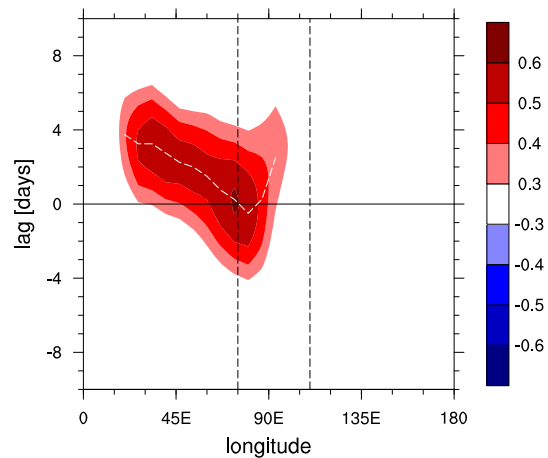
Figure 8. Correlation of low PV area ( PV \leq 0.3 PVU) at each longitude with respect to the divergence term averaged over 70^{\circ}\text{E} – 110^{\circ}\text{E} (indicated by the vertical dashed lines), calculated from data averaged over 2005–2009. The correlations are calculated for each year over the deseasonalized time series from May to September, with periods shorter than 10 days removed from the time series. The dashed white lines give the timing of the maximum correlation at each longitude.
