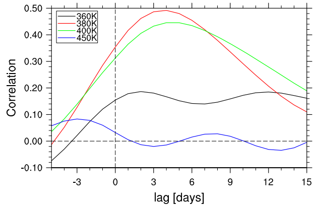
Figure 14. Correlation of the time series of 0.3 PV area at 360 K to the area of high CO concentrations at 360, 380, 400, and 450 K, where the CO thresholds are 100, 80, 65, and 35 ppbv, respectively. Correlations are calculated from deseasonalized May–September time series for each year 2005–2009, and the 5 year mean is shown.
