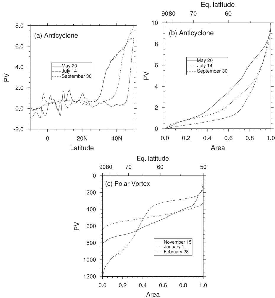
Figure 3. (a) PV at 360 K and at 90^{\circ}\text{E} as a function of latitude for 3 days of the year 2006: 20 May (solid), 14 July (dashed), and 30 September (dotted). (b) Same as Figure 3a but PV in area coordinates (or equivalent latitude, with the lowest PV moved to the pole). The area is calculated in the domain 15^{\circ}\text{N} – 45^{\circ}\text{N} and 0^{\circ}\text{E} – 180^{\circ}\text{E} and is given in relative units (the area of the whole domain is 1.0). (c) Area of PV for the polar vortex at 850 K for 15 November of the year 2005 (solid), 1 January (dashed), and 28 February (dotted) of year 2006. Here, the area is calculated for the Northern Hemisphere poleward of 50^{\circ}\text{N} .
