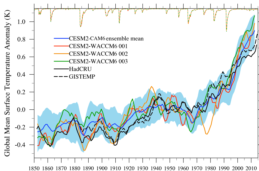
Figure 11. Global mean surface temperature anomalies with respect to the 1920–1980 average with 5 year smoothing. Blue: mean of 10-member CESM2 historical ensemble (blue shading shows the ensemble spread). Three coupled CESM2-WACCM6 historical ensemble members are red (001), orange (002), and green (003) curves. Observed temperatures from Hadley Centre-Climatic Research Unit Version 4 (HadCRUT4) infilled with kriging (Cowtan & Way, 2014) (black solid). Goddard Institute for Space Studies (GISS) Surface Temperature Analysis (Hansen et al., 2010) (black dashed). Top curves are a stratospheric aerosol optical depth index ( 1.15\text{--}2 \times global average) for each coupled CESM2-WACCM6 ensemble member.
