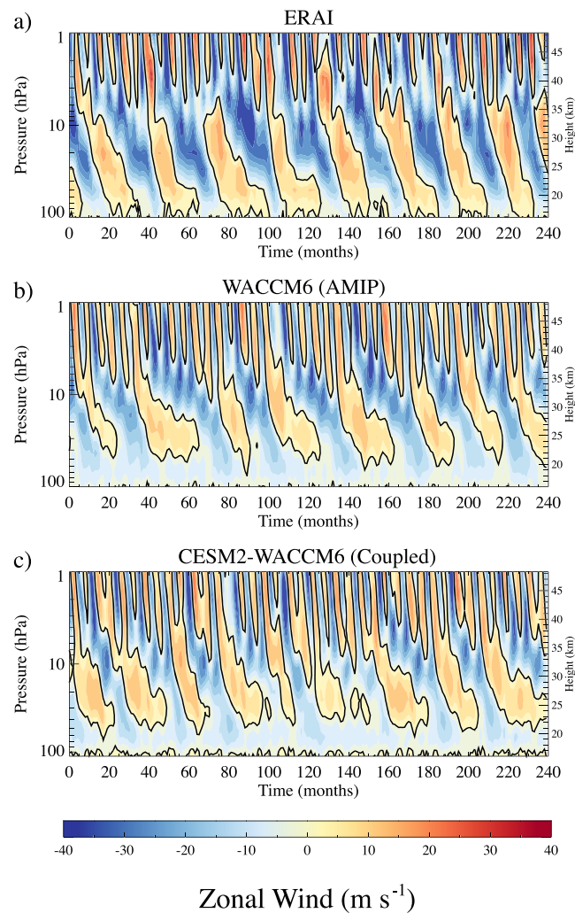
Figure 6. Monthly average zonal wind from 10°S–10°N in (a) European Center Reanalysis (ERA-I), (b) WACCM6 historical simulation with historical SSTs, and (c) fully coupled WACCM6 historical simulation illustrating the quasi-biennial oscillation.
