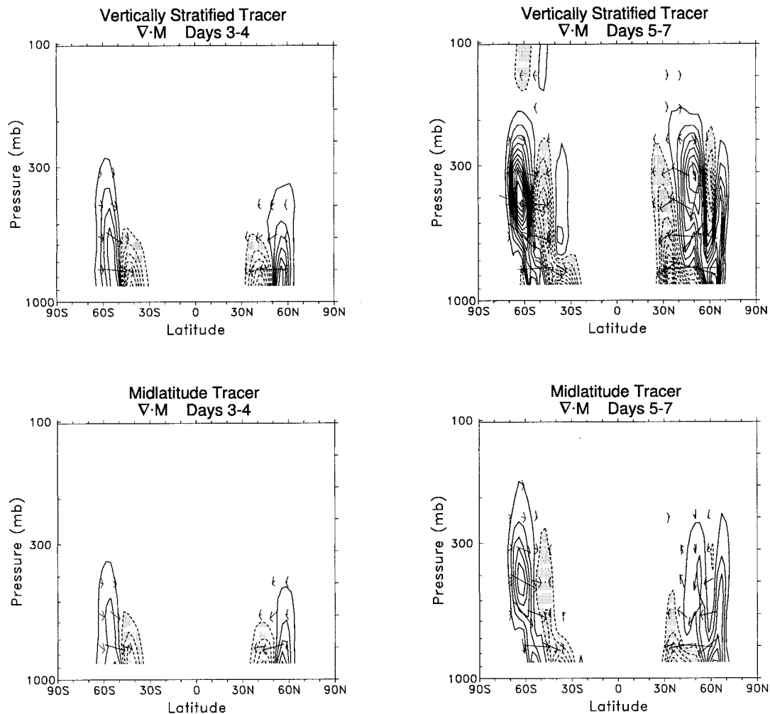
FIG. 11. Meridional cross section of \nabla \cdot \mathbf{M} for the vertically stratified tracer (top) and the midlatitude tracer (bottom) averaged over days 3–4 and 5–7 of the life cycle.
