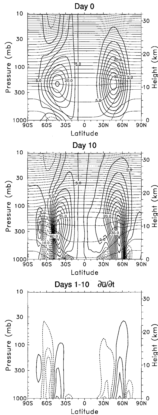
FIG. 1. Zonal mean zonal wind (contour interval of 5 \text{ m s}^{-1} ) and potential temperature field (contours of 260, 280, 300, ... K) on (top) day 0 and (middle) day 10; (bottom) the time tendency of the zonal wind averaged over days 1–10 of the simulation with contours of \pm 0.5, 1.5, 2.5, \dots \text{ m s}^{-1} \text{ day}^{-1} .
